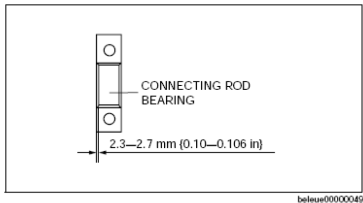
Fig. 92: Installing Connecting Rod Bearing To Connecting Rod And Connecting Rod Caps
