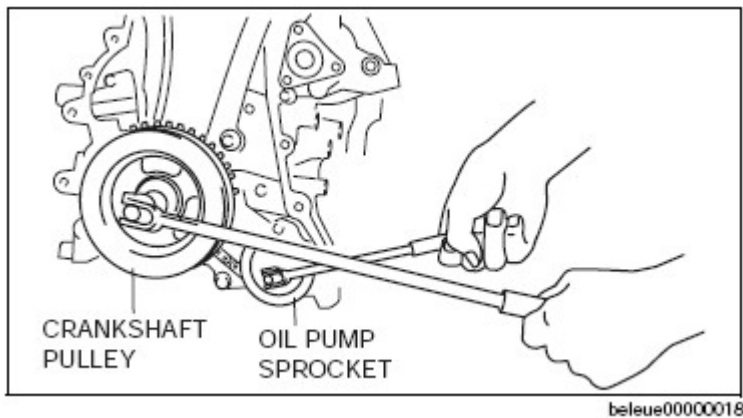
Fig. 8: Removing Crankshaft Pulley And Crankshaft Pulley Lock Bolt
