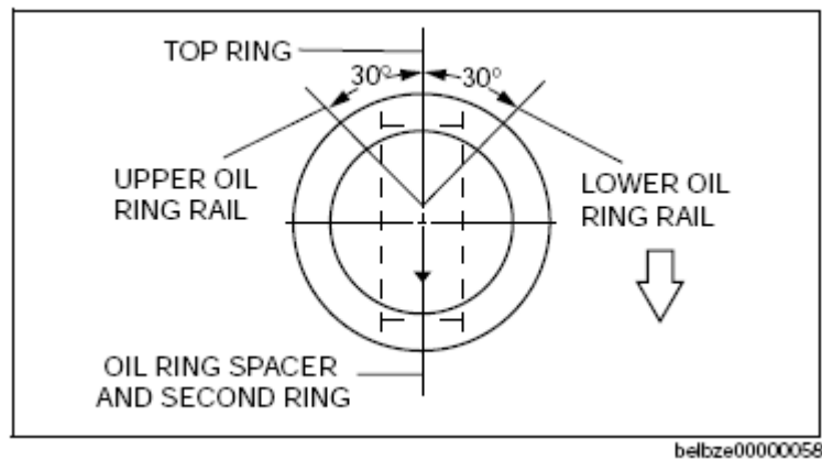
Fig. 91: Identifying Piston Rings End Gap Position
