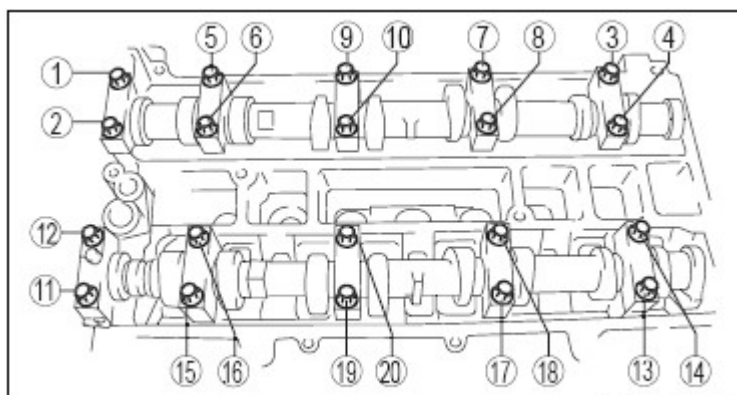
Fig. 78: Identifying Camshaft Cap Bolt Loosening Order
