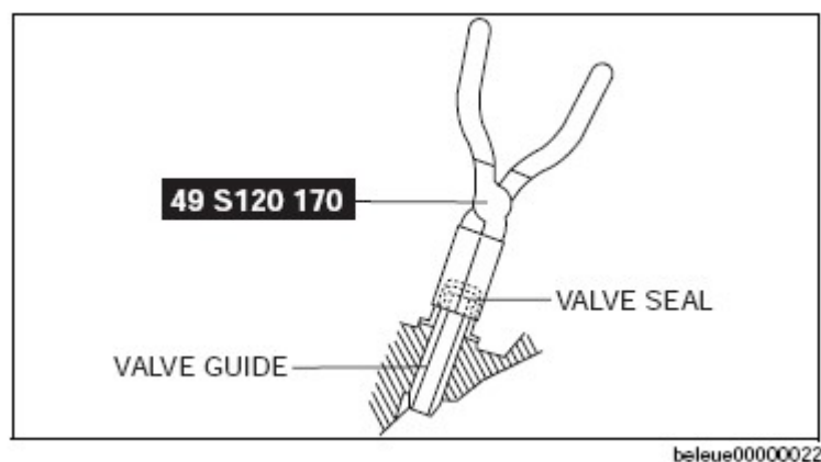
Fig. 15: Removing Valve Seal Using SST
