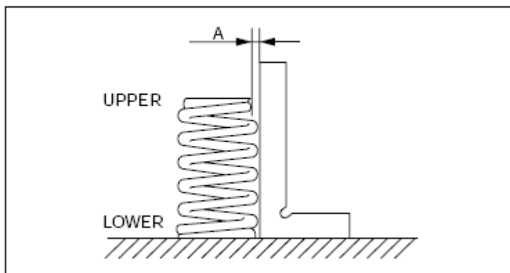
Fig. 37: Measuring Valve Spring Off-Square
