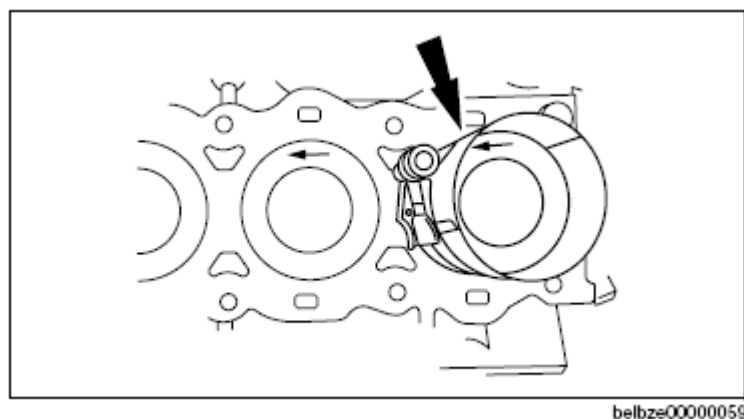
Fig. 93: Inserting Piston And Connecting Rod Into Cylinder With Arrow Mark To Front Of Engine
