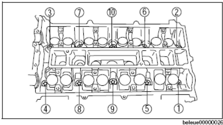
Fig. 12: Identifying Cylinder Head Bolts Loosening Order
