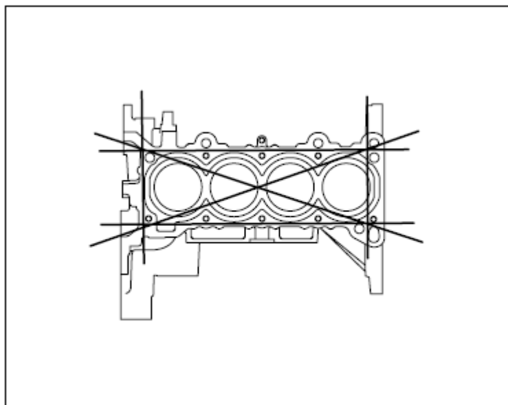
Fig. 49: Measuring Distortion Of Cylinder Block Top Surface In Six Directions
