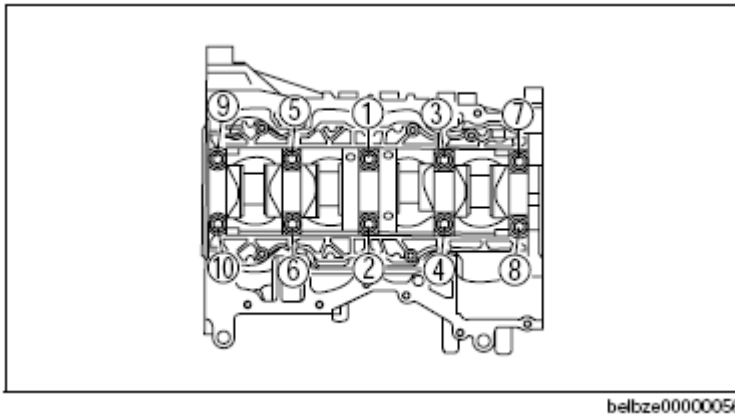
Fig. 89: Identifying Main Bearing Caps Installing Order
