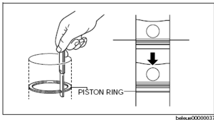
Fig. 54: Measuring Piston Ring End Gap
