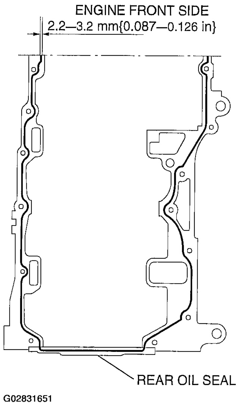
Fig. 95: Applying A Continuous Bead Of Silicone Sealant Courtesy of MAZDA MOTORS CORP.
