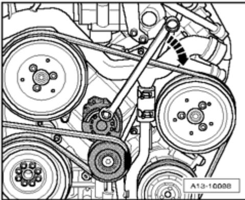
Fig. 65: Slackening Ribbed Belt Courtesy of VOLKSWAGEN UNITED STATES, INC.
