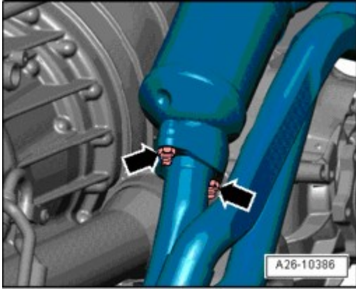
Fig. 92: Removing Nuts
