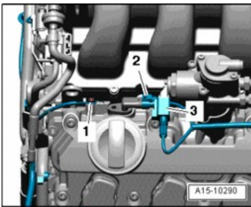
Fig. 346: Cylinder Head Ground Line & Electrical Connectors
