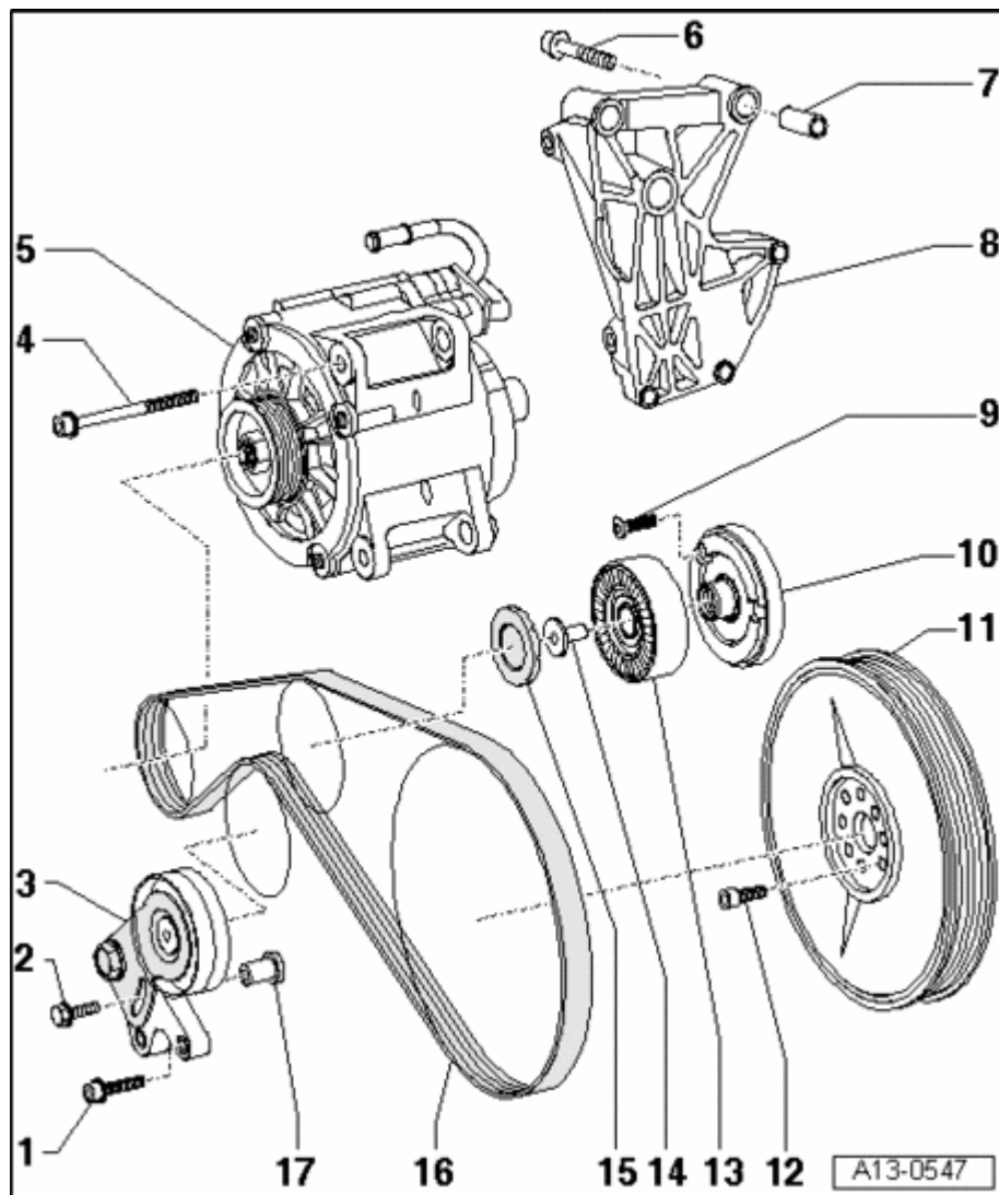
Fig. 133: Ribbed Belt Drive, Component Overview Courtesy of VOLKSWAGEN UNITED STATES, INC.
