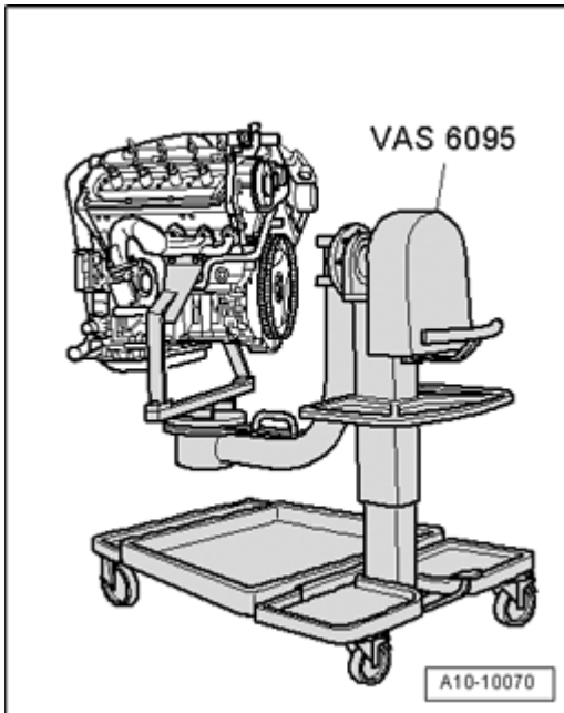
Fig. 117: Securing Engine To Engine And Transmission Holder VAS 6095/1-7 Using Holder VAS 6095 Courtesy of VOLKSWAGEN UNITED STATES, INC.
