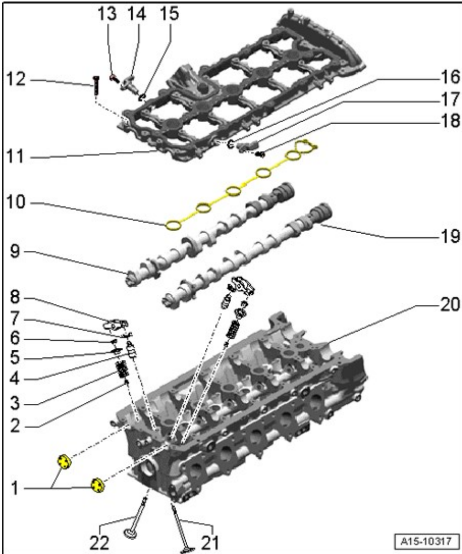
Fig. 336: Valvetrain, Component Overview
