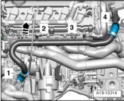
Fig. 478: Removing Bolts, Oil Dipstick Guide Tube Upward & Loosening Hose Clamps And Removing Left Coolant Pipe From Coolant Hoses
