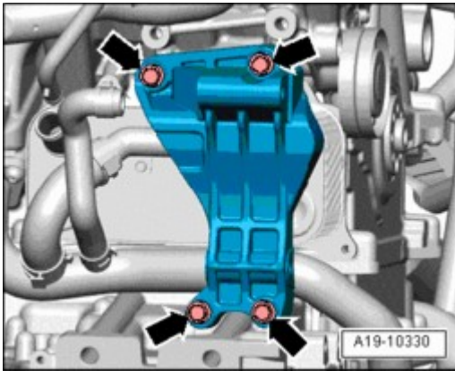
Fig. 472: Removing Bolts And Air Generator Bracket
