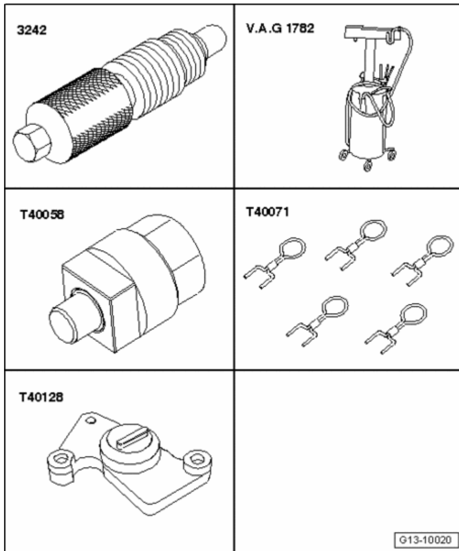
Fig. 221: Identifying Special Tools - Power Take-Off, Oil Pump And Balancing Shaft Drive Chain, Removing And Installing
