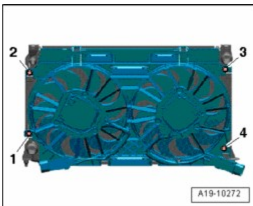
Fig. 504: Removing Screws And Fan Shroud
