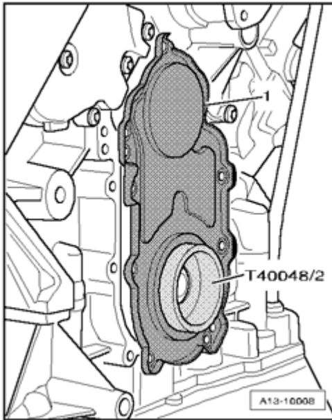
Fig. 650: Identifying Coolant Hose & Coolant Pump Housing Bolts Courtesy of VOLKSWAGEN UNITED STATES, INC.
