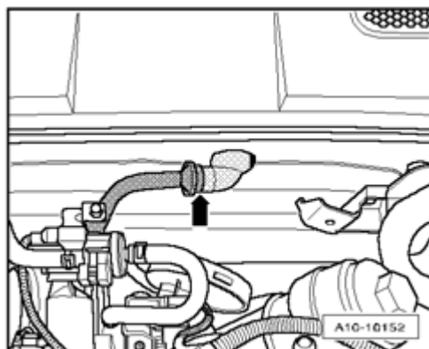
Fig. 452: Removing Drive Shaft For Oil Pump Courtesy of VOLKSWAGEN UNITED STATES, INC.
