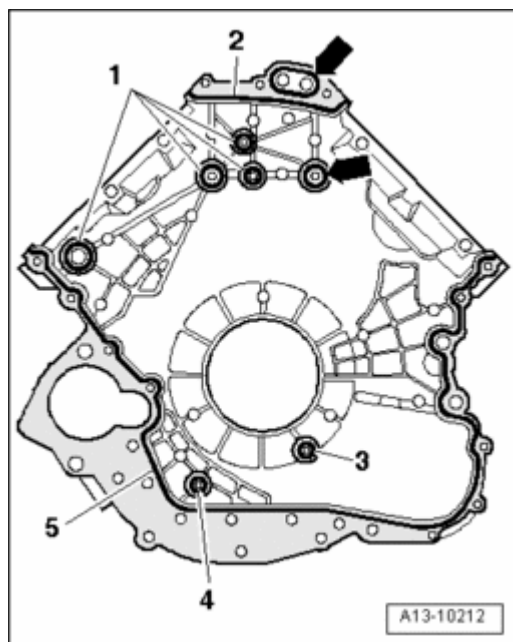
Fig. 701: Removing Quick-Release Fasteners, Screws And Noise Insulation Courtesy of VOLKSWAGEN UNITED STATES, INC.
