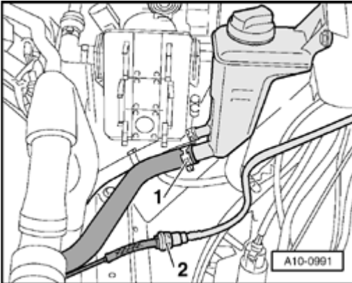
Fig. 38: Disconnecting Hose From Power Steering Fluid Reservoir & Vacuum Hose To Vacuum Reservoir
