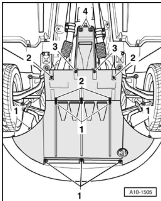
Fig. 235: Identifying Scissor Lift Platform VAS 6131 Courtesy of VOLKSWAGEN UNITED STATES, INC.
