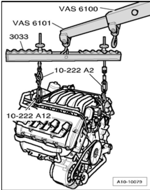
Fig. 105: Engaging Engine Sling 3033 On Additional Hook 10-222 A/2 And On Workshop Crane VAS 6100 With Lift Arm Extension For Workshop Crane VAS 6101
