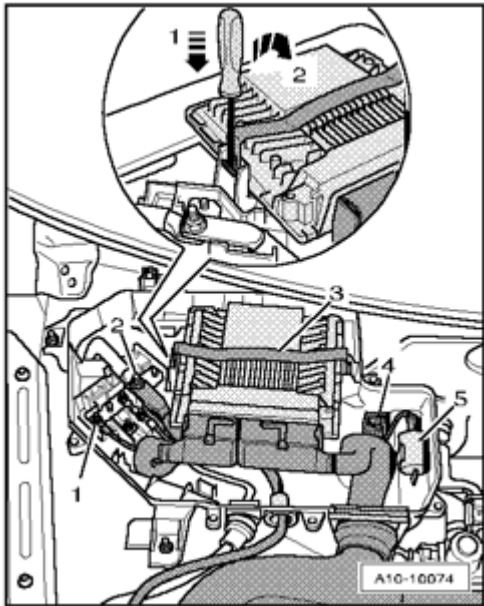
Fig. 567: Identifying 2-Pin Electrical Harness Connector & Terminals Courtesy of VOLKSWAGEN UNITED STATES, INC.
