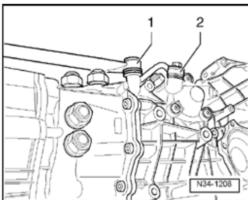
Fig. 116: Identifying Push Rod And Connecting Rod For Selector Rod Courtesy of VOLKSWAGEN UNITED STATES, INC.
