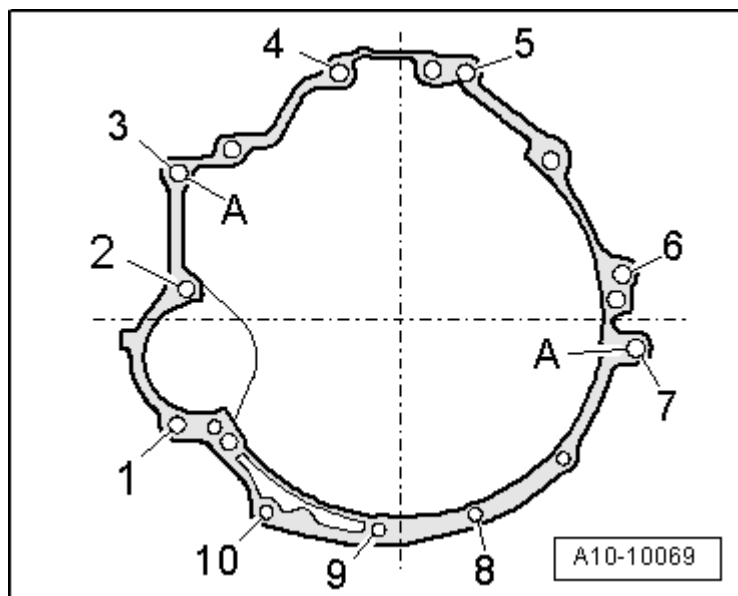
Fig. 512: Removing Front Engine Cover
