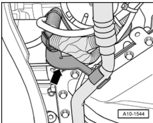
Fig. 178: Removing Refrigerant Line On Bracket Courtesy of VOLKSWAGEN UNITED STATES, INC.
