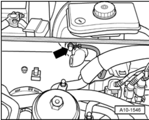
Fig. 55: Removing Ground (GND) Connection Courtesy of VOLKSWAGEN UNITED STATES, INC.
