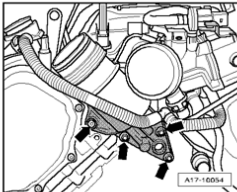
Fig. 689: Disconnecting Vacuum Hose & Air Guide Hose From Throttle Valve Control Module Courtesy of VOLKSWAGEN UNITED STATES, INC.
