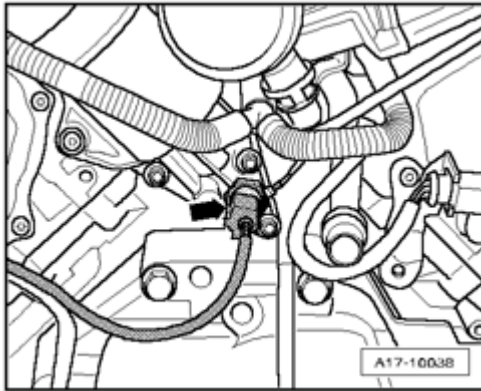
Fig. 688: Identifying Electrical Harness Connectors, Secondary Air Injection (AIR) Pump Hose, Air Guide Hose & Mass Air Flow (MAF) Sensor Courtesy of VOLKSWAGEN UNITED STATES, INC.
