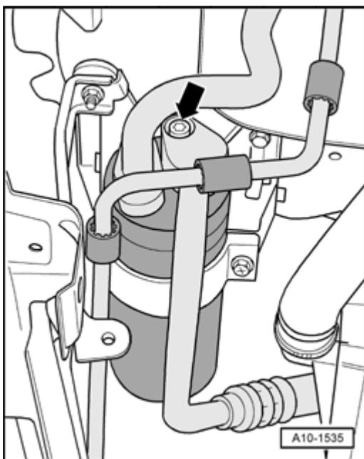
Fig. 179: Removing Bolt And Disconnecting Refrigerant Line To A/C Compressor Courtesy of VOLKSWAGEN UNITED STATES, INC.
