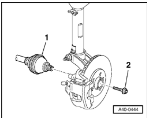
Fig. 63: Identifying Collar Bolt For Right Drive Axle Courtesy of VOLKSWAGEN UNITED STATES, INC.
