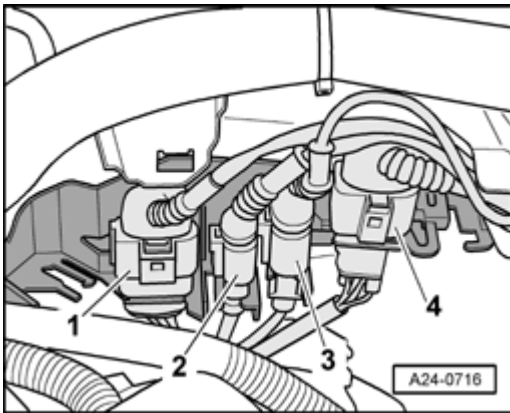
Fig. 56: Removing Bracket For Electrical Harness Connectors At Left From Bulkhead Courtesy of VOLKSWAGEN UNITED STATES, INC.
