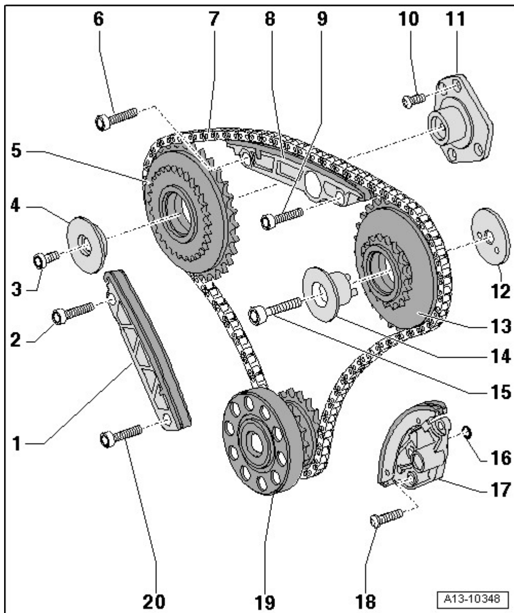
Fig. 15: Timing Mechanism Drive Chain Overview
