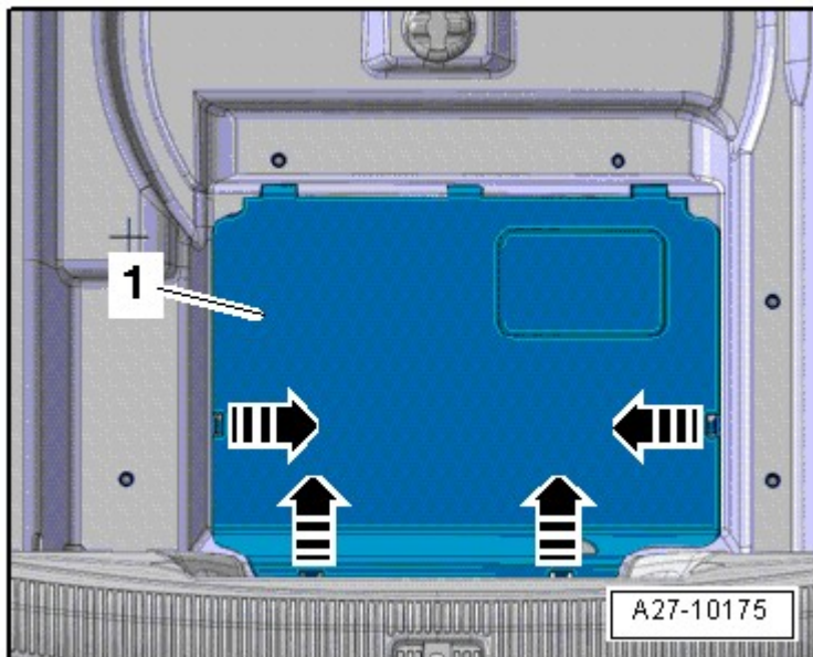
Fig. 9: Pressing Release Tabs And Open Flap Courtesy of AUDI OF AMERICA, LLC
