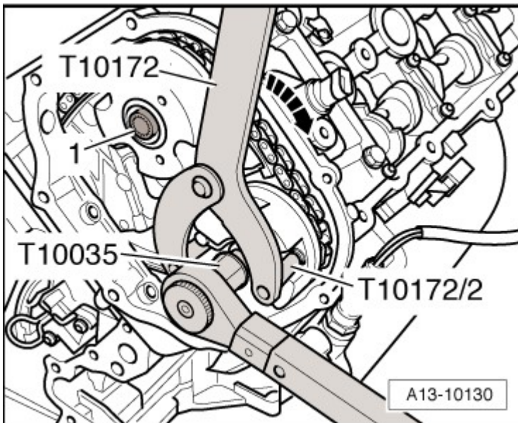
Fig. 83: Removing/ Installing Right Camshaft Adjuster
