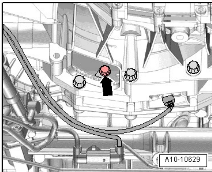
Fig. 80: Identifying Clutch Module First Bolt Installation Location
