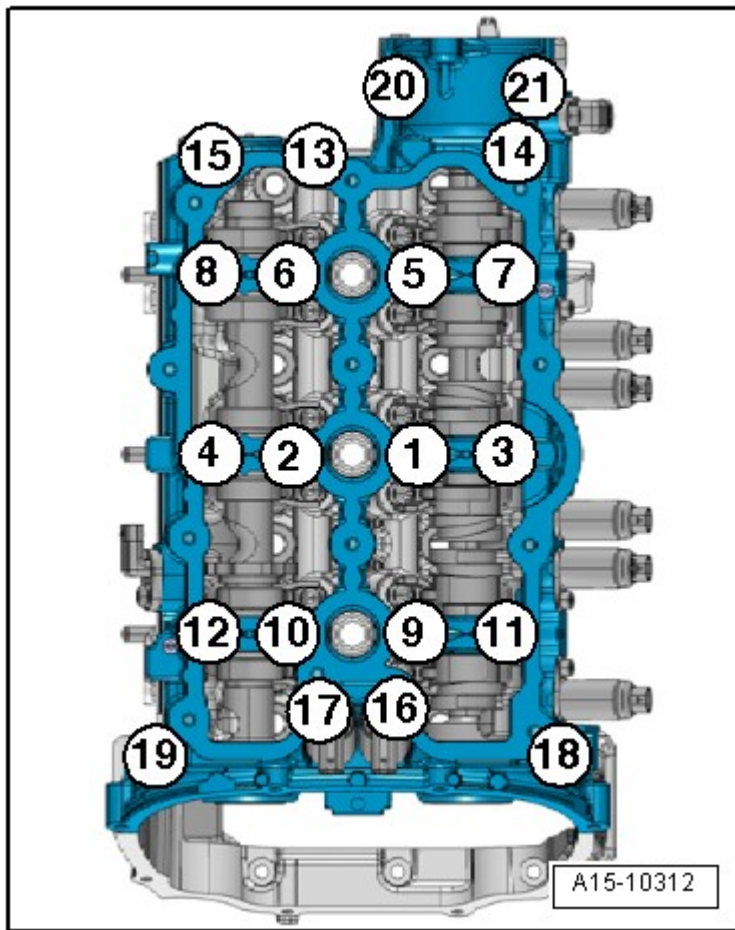
Fig. 18: Identifying Sequence Of Guide Frame Bolts
