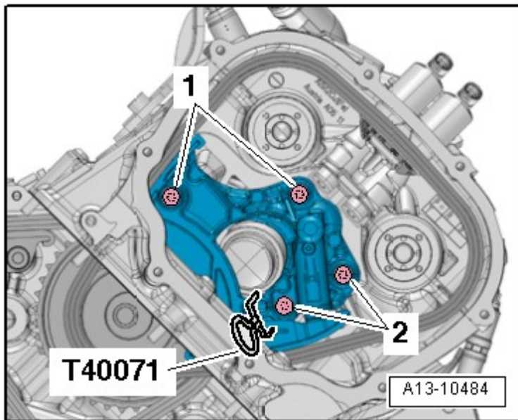
Fig. 57: Identifying Chain Tensioner Components Courtesy of AUDI OF AMERICA, LLC
