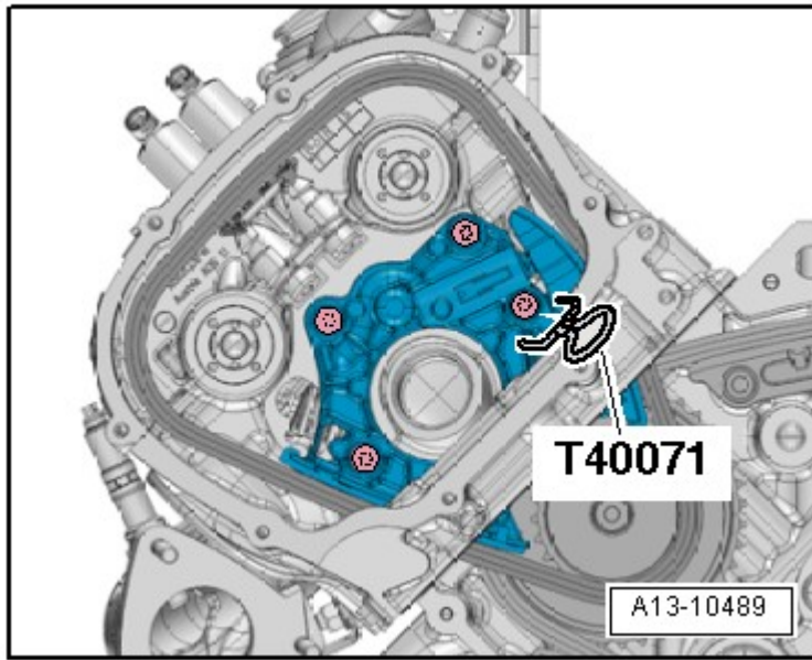
Fig. 56: Identifying Special Tool - T40071 Courtesy of AUDI OF AMERICA, LLC
