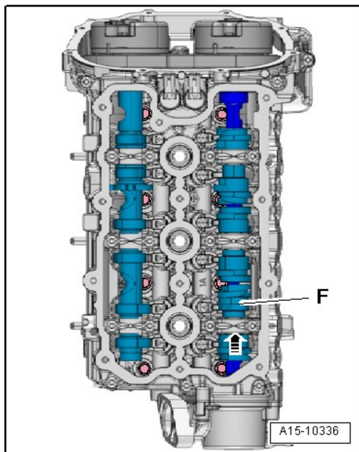
Fig. 111: Sliding Unloaded Camshaft Sliders (Right Cylinder Head)
