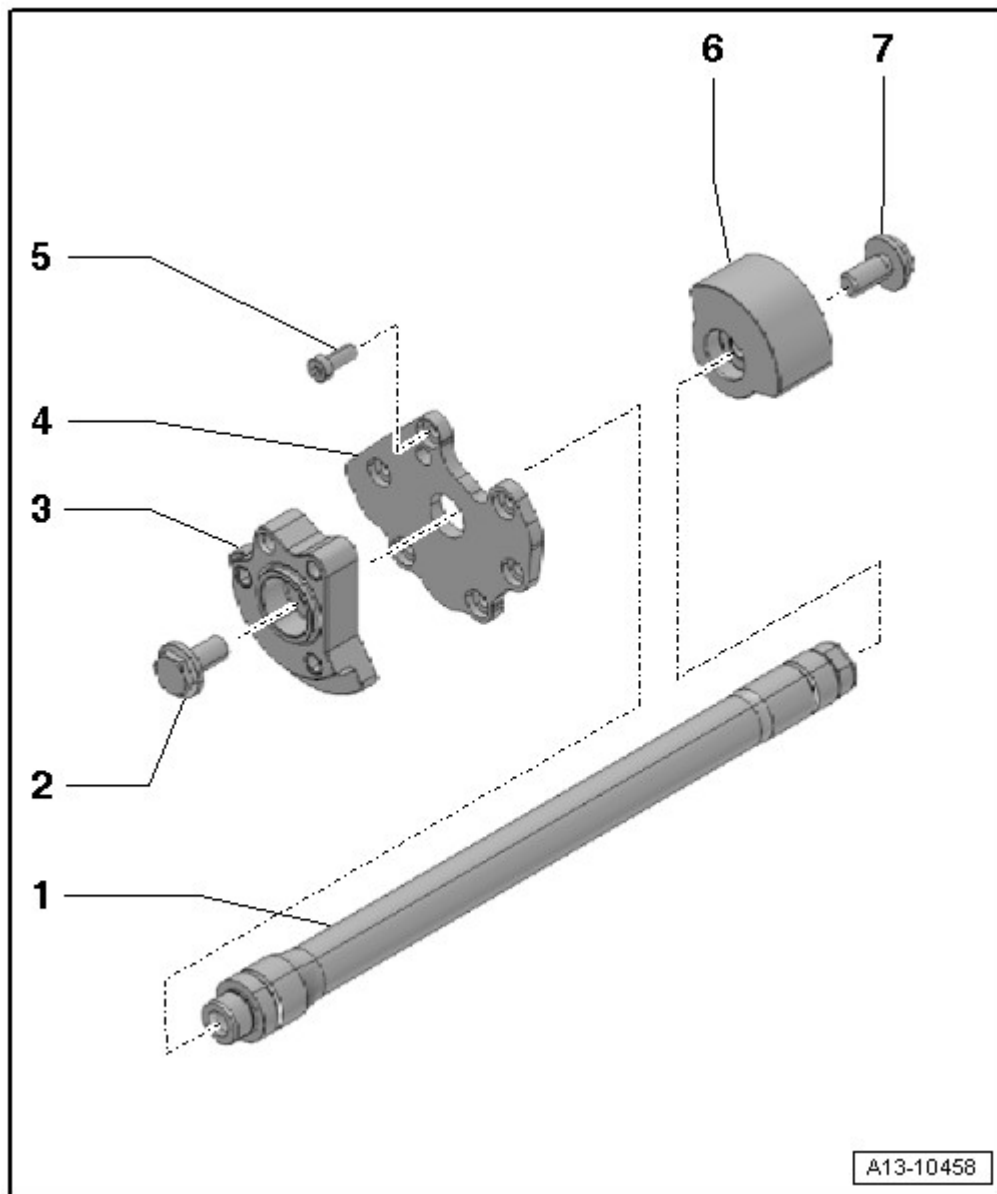
Fig. 1: Balance Shaft Overview Courtesy of AUDI OF AMERICA, LLC
