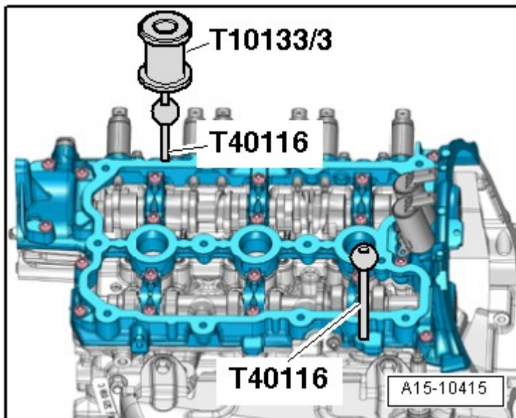
Fig. 55: Removing Special Tool T40116 With T10133/3
