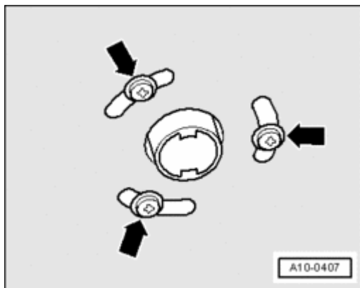
Fig. 336: Identifying Exhaust Pipe Fasteners
