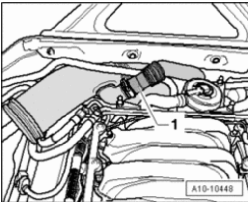
Fig. 297: Removing Hose
