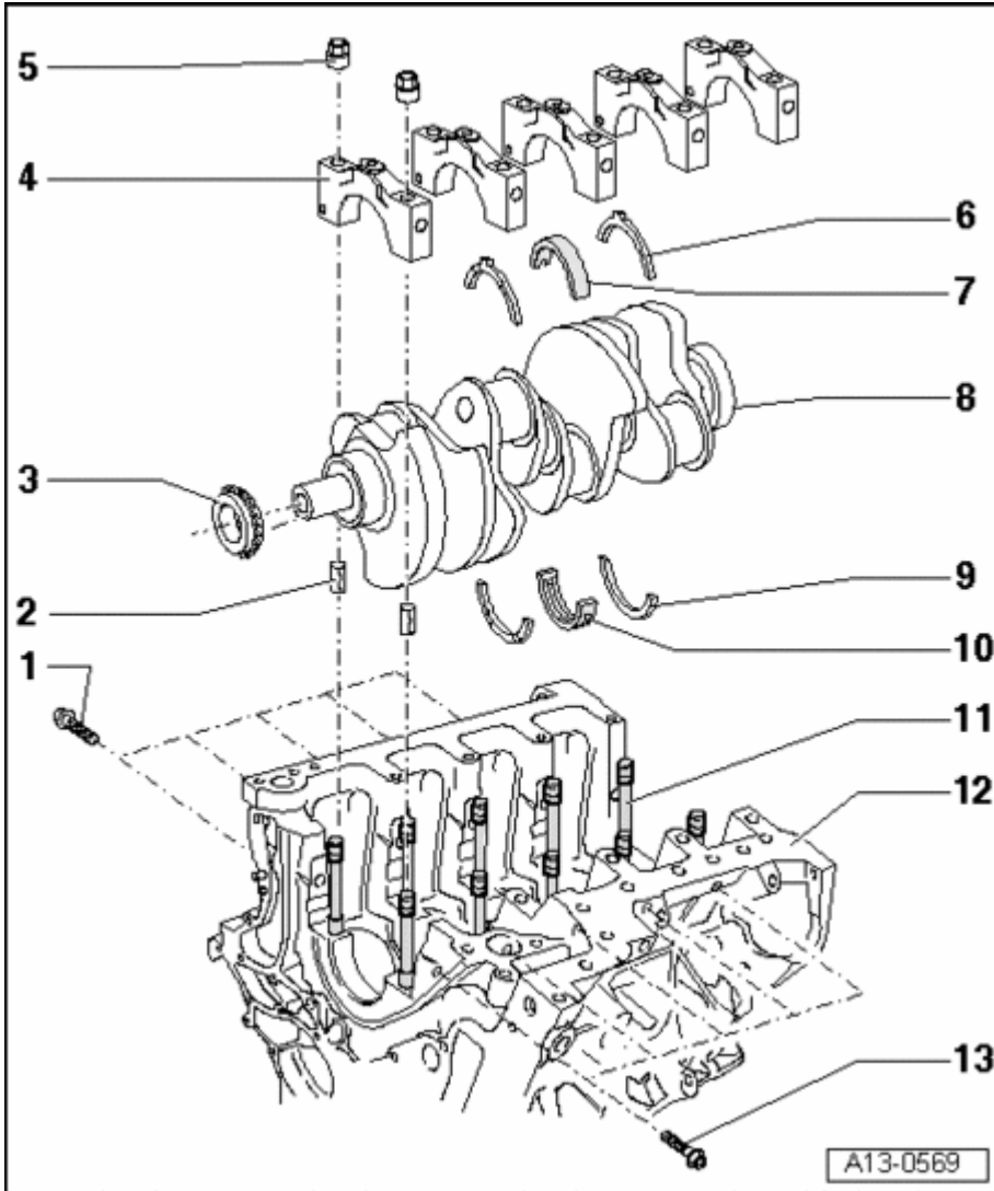
Fig. 235: Crankshaft, Assembly Overview
