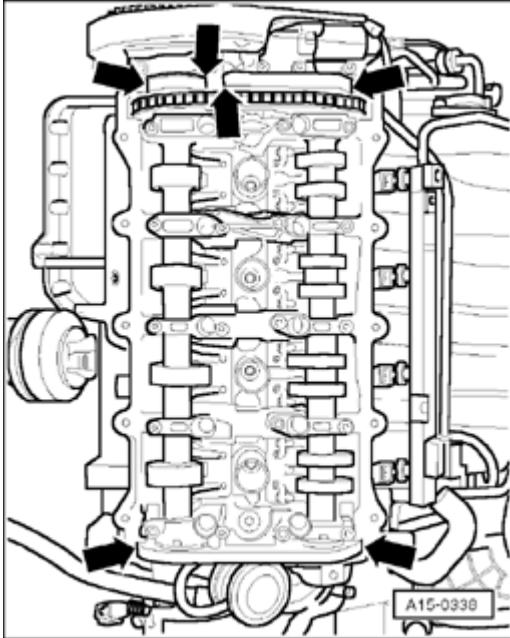
Fig. 261: Applying Thin Layer Of Sealant To Edges Of Sealing Surfaces Between Bearing Cap And Cylinder Head
