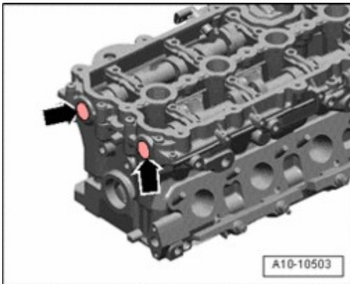
Fig. 365: Driving Sealing Plugs In Flush Courtesy of VOLKSWAGEN UNITED STATES, INC.
