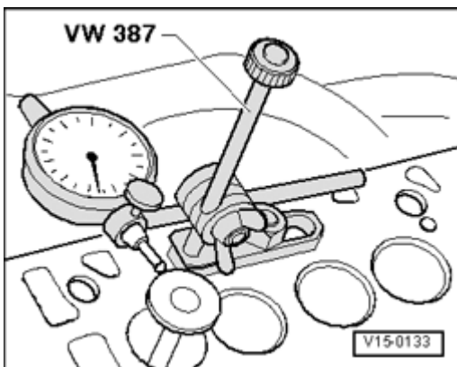
Fig. 456: Identifying Special Tool - VW 387 Installed
