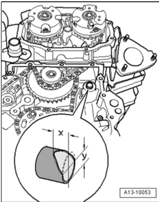
Fig. 268: Chamfering Alignment Bushing With A File
