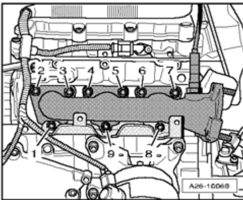
Fig. 608: Removing Nuts, Bracket For Heat Shield & Exhaust Manifold
