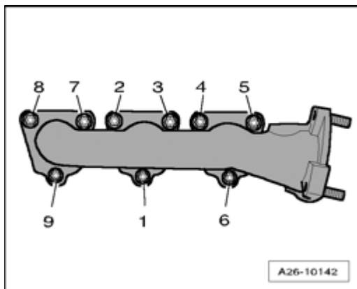
Fig. 609: Exhaust Manifold Tightening Sequence
