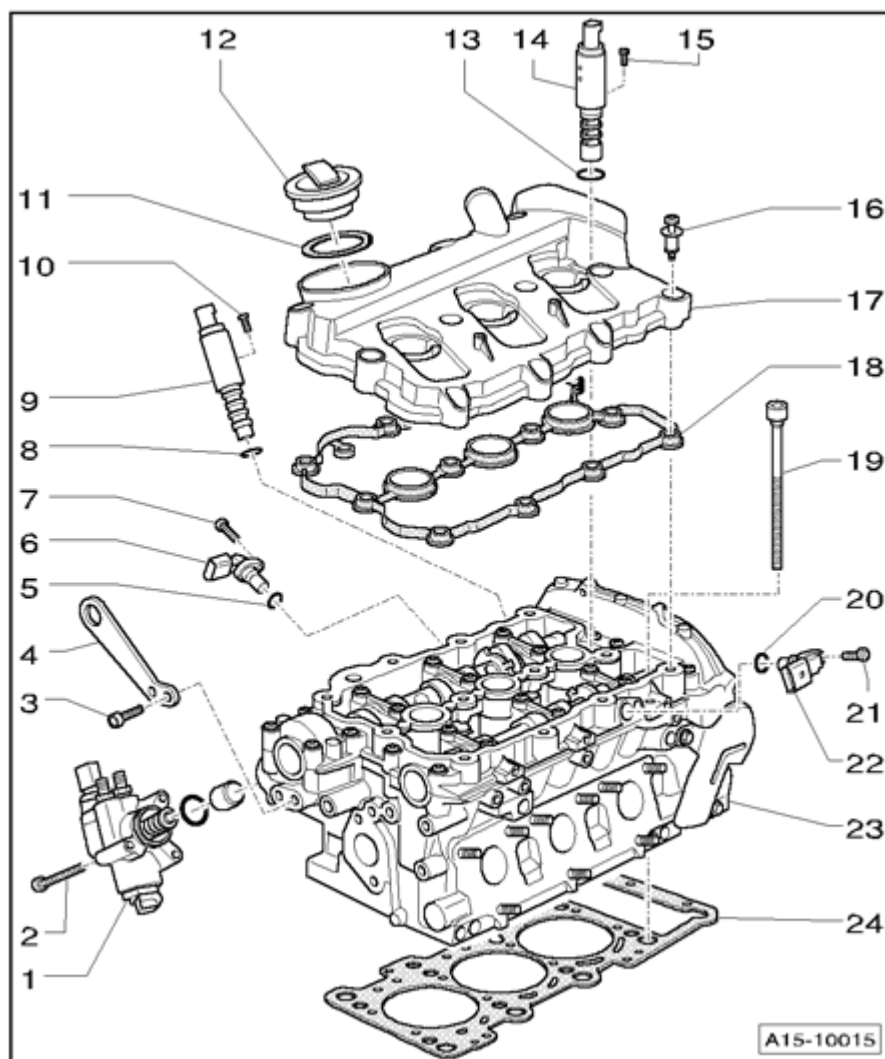
Fig. 361: Cylinder Head, Component Overview
