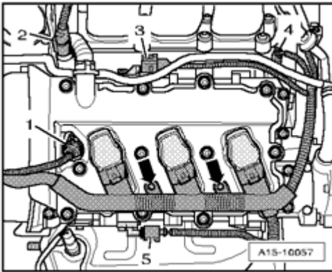
Fig. 432: Disconnecting Electrical Harness Connectors
