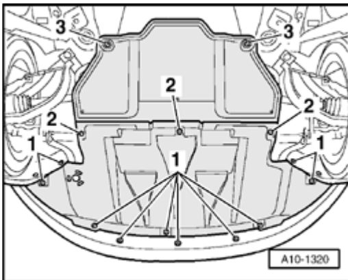
Fig. 521: Identifying Quick-Release Fasteners And Noise Insulation
