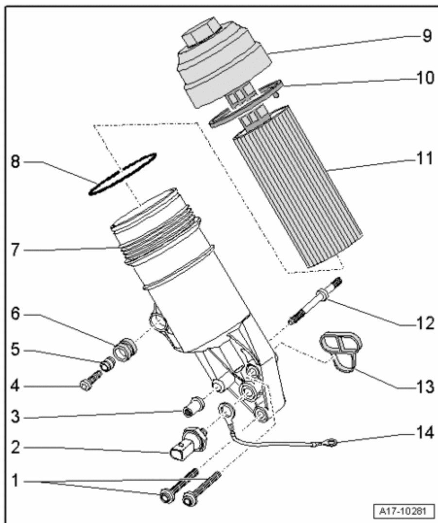
Fig. 492: Oil Filter Housing, Component Overview (Vehicles From 05.2008) Courtesy of VOLKSWAGEN UNITED STATES, INC.
