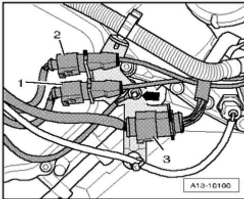
Fig. 498: Disconnecting Electrical Harness Connectors Courtesy of VOLKSWAGEN UNITED STATES, INC.
