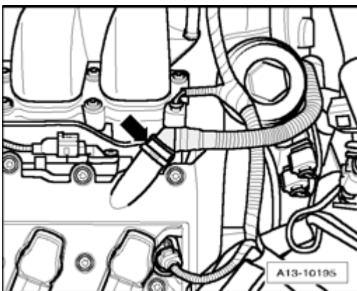
Fig. 499: Removing Crankcase Ventilation Hose At Left Cylinder Head Cover Courtesy of VOLKSWAGEN UNITED STATES, INC.
