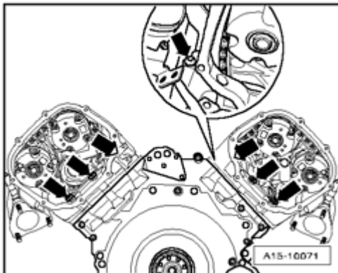
Fig. 420: Removing/Installing Bolts At Rear Of Cylinder Head
