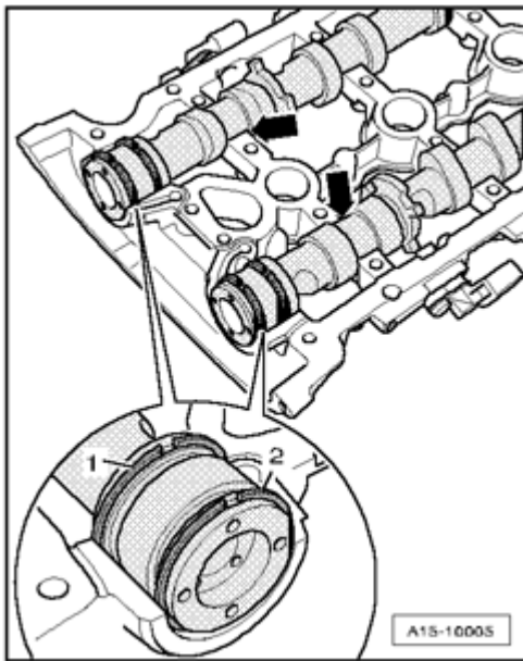
Fig. 443: Setting Camshafts Into Guide Frame
