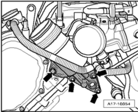
Fig. 502: Removing Oil Filter Housing Bolts
