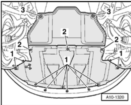
Fig. 473: Identifying Quick-Release Fasteners And Noise Insulation Courtesy of VOLKSWAGEN UNITED STATES, INC.
