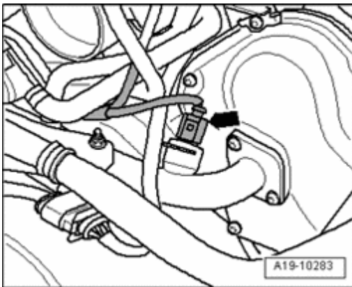
Fig. 306: Relieving Tension On Chain Rail With Screwdriver And Lock Rail With 3 mm Allen Key
