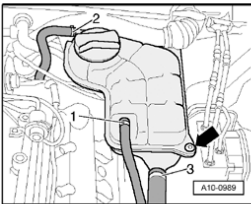
Fig. 350: Removing Coolant Hoses Courtesy of VOLKSWAGEN UNITED STATES, INC.
