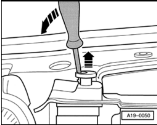
Fig. 469: Loosening Both Radiator Retaining Bolts, Pulling Up And Removing Courtesy of VOLKSWAGEN UNITED STATES, INC.
