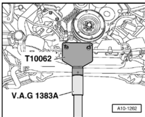
Fig. 86: Tightening T10062 Support On Threaded Holes For Torque Support Courtesy of VOLKSWAGEN UNITED STATES, INC.
