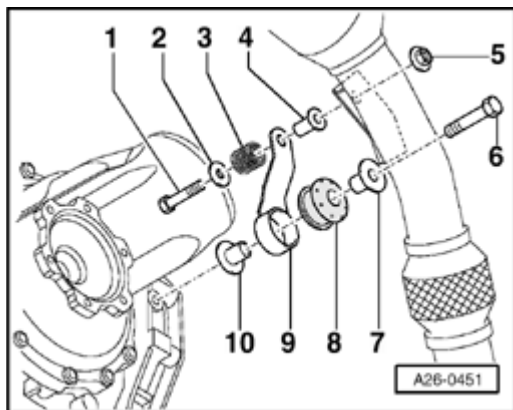
Fig. 483: Individual Left Mounting Components For Vehicles With Automatic Transmission 01J Courtesy of VOLKSWAGEN UNITED STATES, INC.
