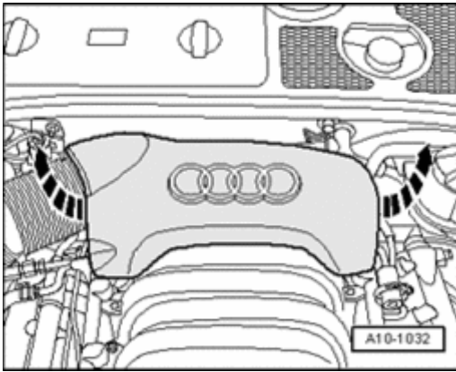
Fig. 224: Removing Rear Engine Cover Courtesy of VOLKSWAGEN UNITED STATES, INC.
