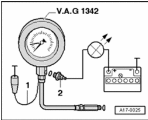
○ Disconnect electrical harness connector at oil pressure switch (arrow).
