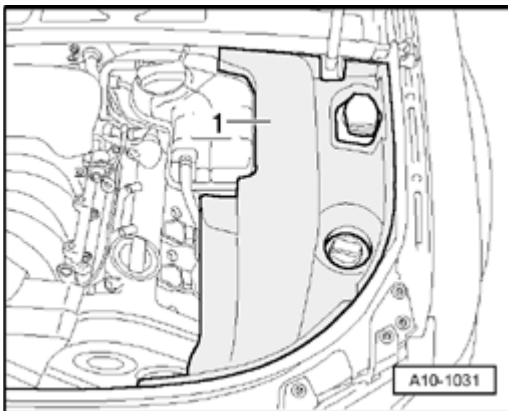
Fig. 225: Removing Cover In Engine Compartment (Left Side) Courtesy of VOLKSWAGEN UNITED STATES, INC.
