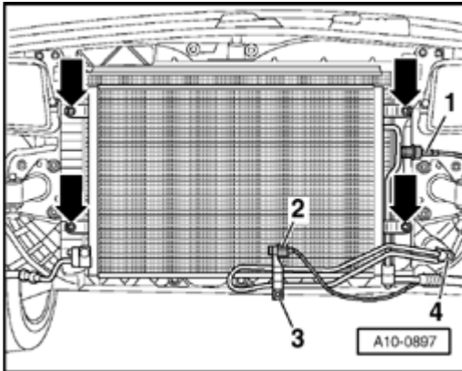
Fig. 468: Identifying Outside Air Temperature Sensor G17, Bolts & High Pressure Sensor G65 Electrical Harness Connector
