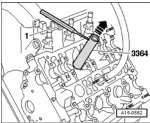
Fig. 326: Positioning Lower Part Of 3364 Valve Stem Removal Tool At Valve Stem Oil Seal Courtesy of VOLKSWAGEN UNITED STATES, INC.
