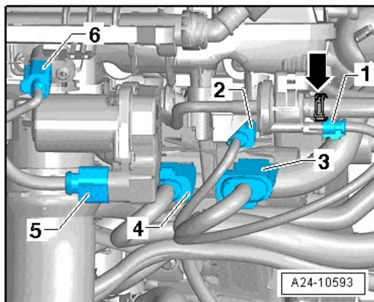
Fig. 175: Identifying Connectors
