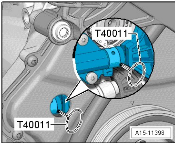
Fig. 75: Securing Chain Tensioner
