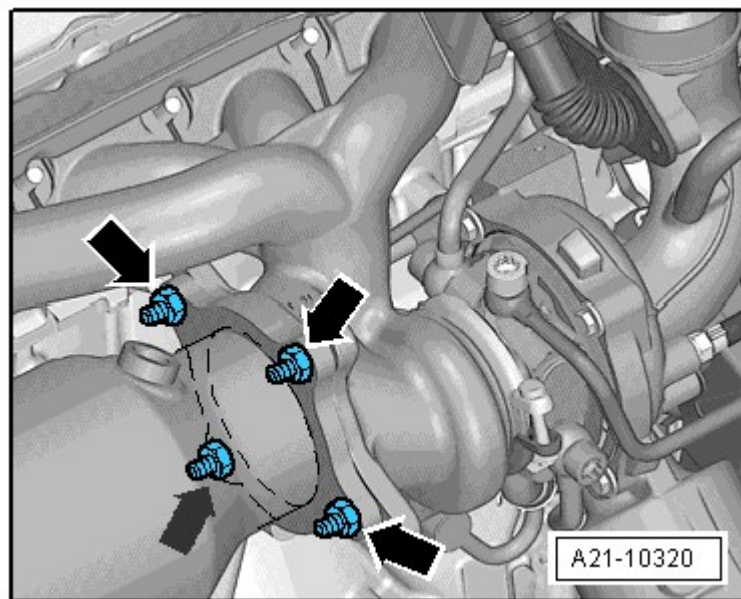
Fig. 186: Identifying Nuts
