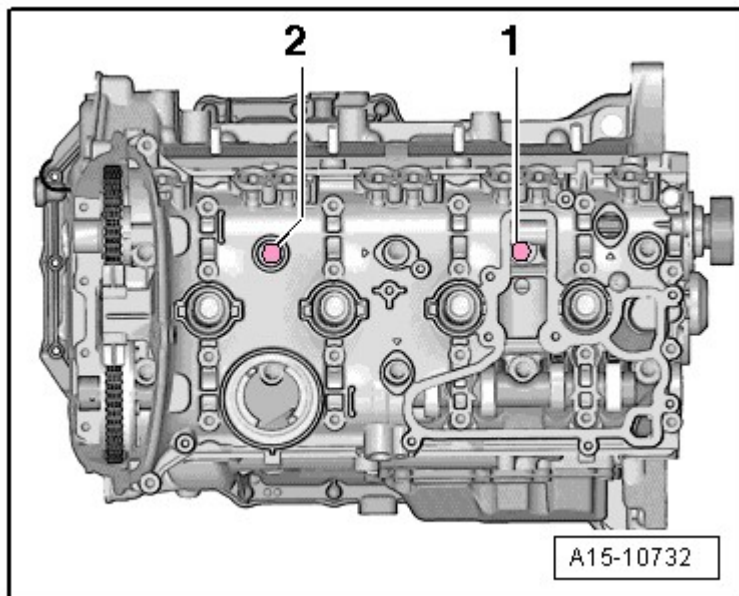
Fig. 170: Identifying Bolts
