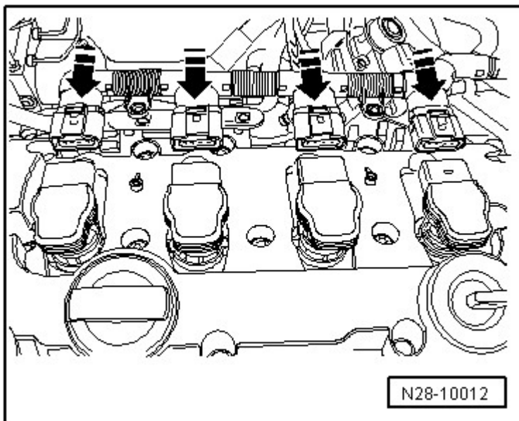
Fig. 38: Connecting Connectors To Ignition Coils
