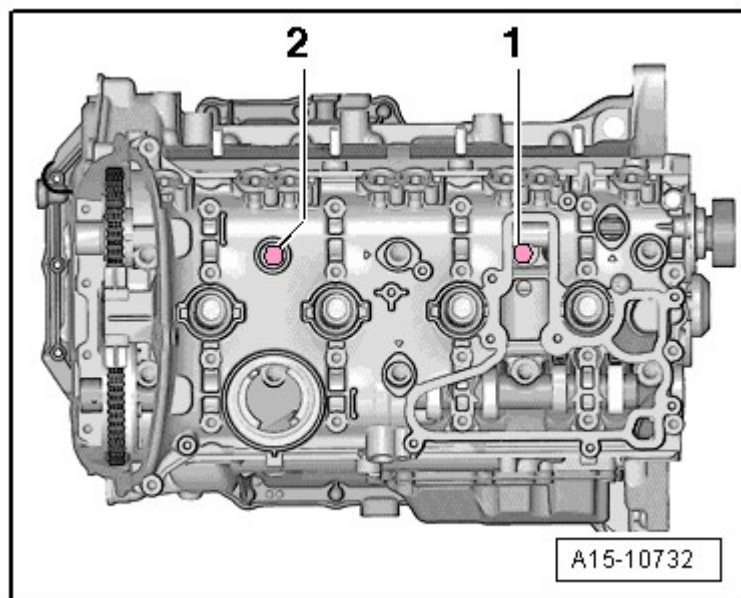
Fig. 170: Identifying Bolts
