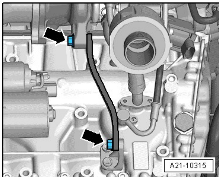
Fig. 184: Identifying Bolts
