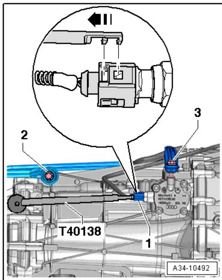
Fig. 40: Disconnecting Connector
