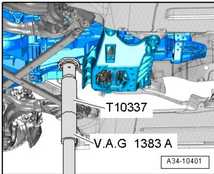
Fig. 37: Supporting Transmission With V.A.G 1383
