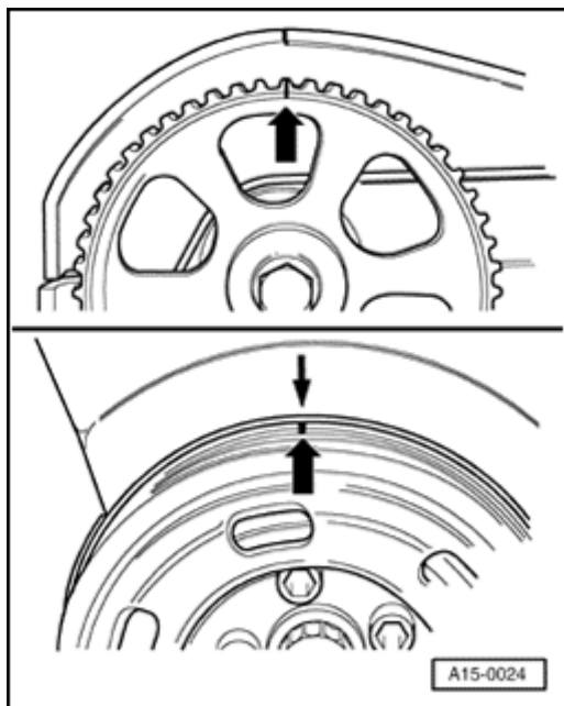
Fig. 105: Identifying Marking On Camshaft Gear Aligned With Marking On Cylinder Head Cover Courtesy of VOLKSWAGEN UNITED STATES, INC.
