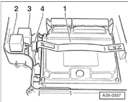
Fig. 385: Location Of Secondary Air Injection (AIR) Pump Relay J299 Courtesy of VOLKSWAGEN UNITED STATES, INC.
