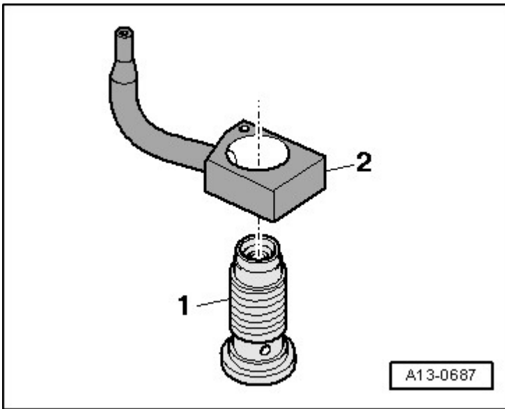
Fig. 21: Oil Spray Jet and Pressure Relief Valve
