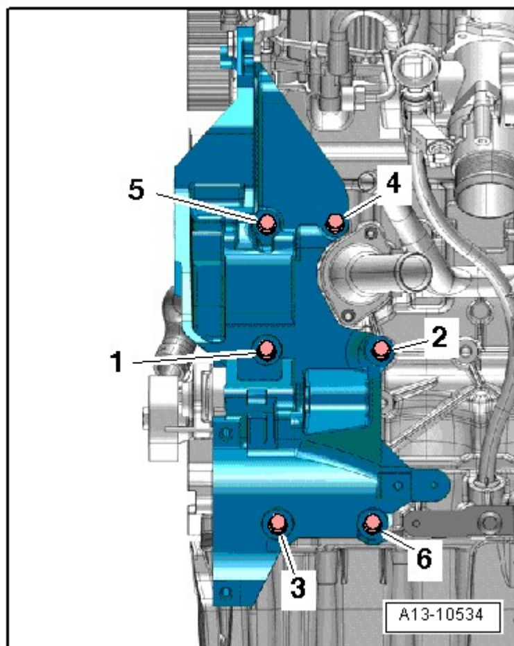
Fig. 54: Tightening Sequence
