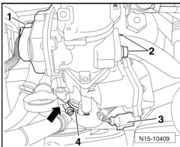
Fig. 74: Identifying Connectors
