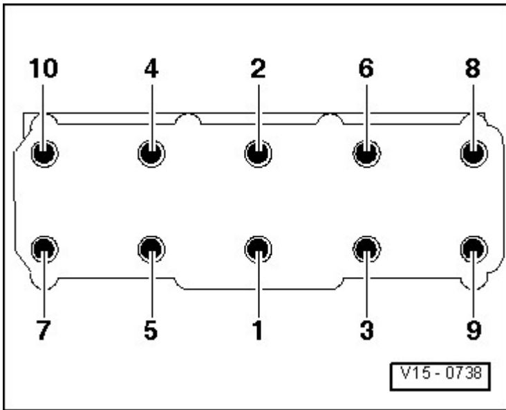
Fig. 8: Cylinder Head Bolt Tightening Sequence Courtesy of AUDI OF AMERICA, LLC
