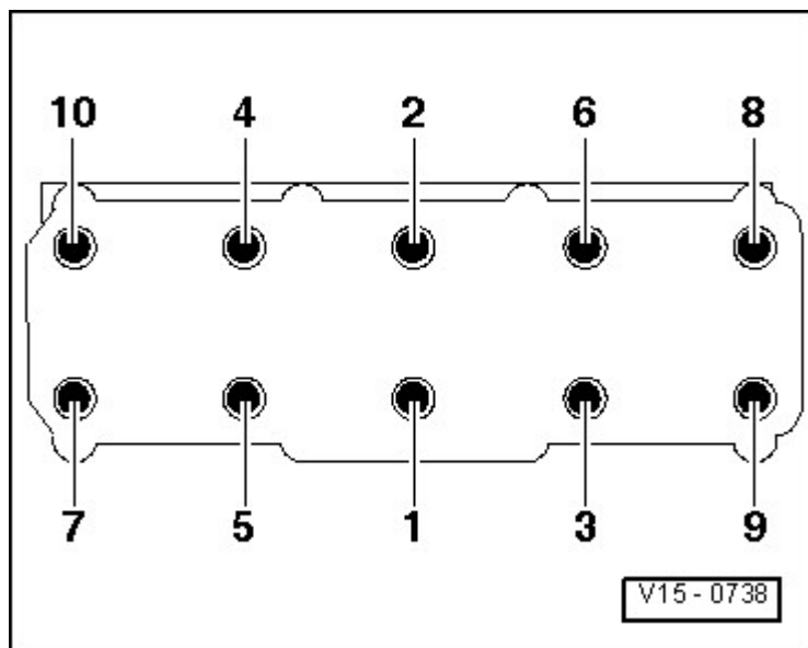
Fig. 95: Cylinder Head Bolt Tightening Sequence
