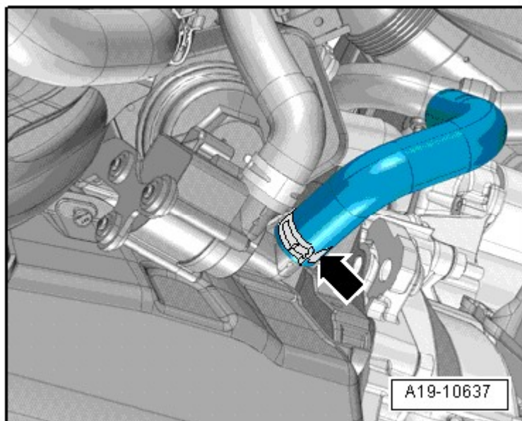
Fig. 39: Identifying Hose Clamp
