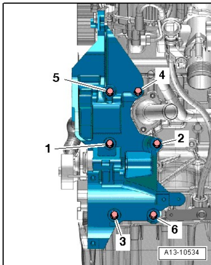
Fig. 22: Tightening Sequence
