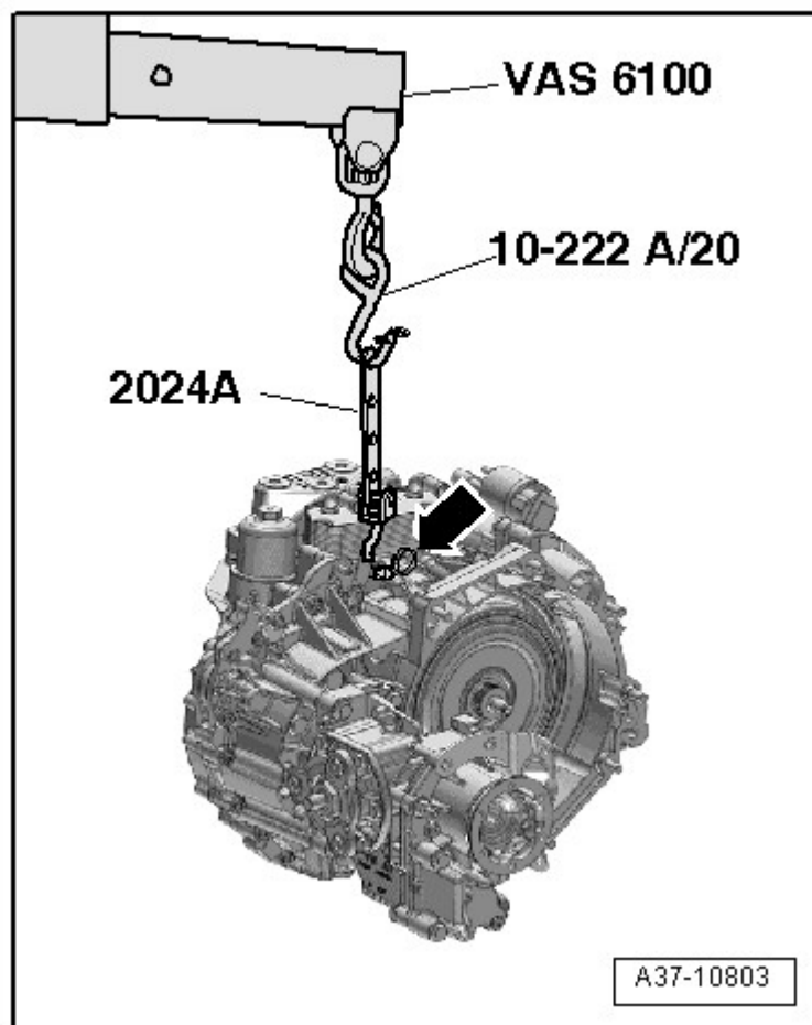
Fig. 106: Installing 2024 A To Transmission Courtesy of AUDI OF AMERICA, LLC
