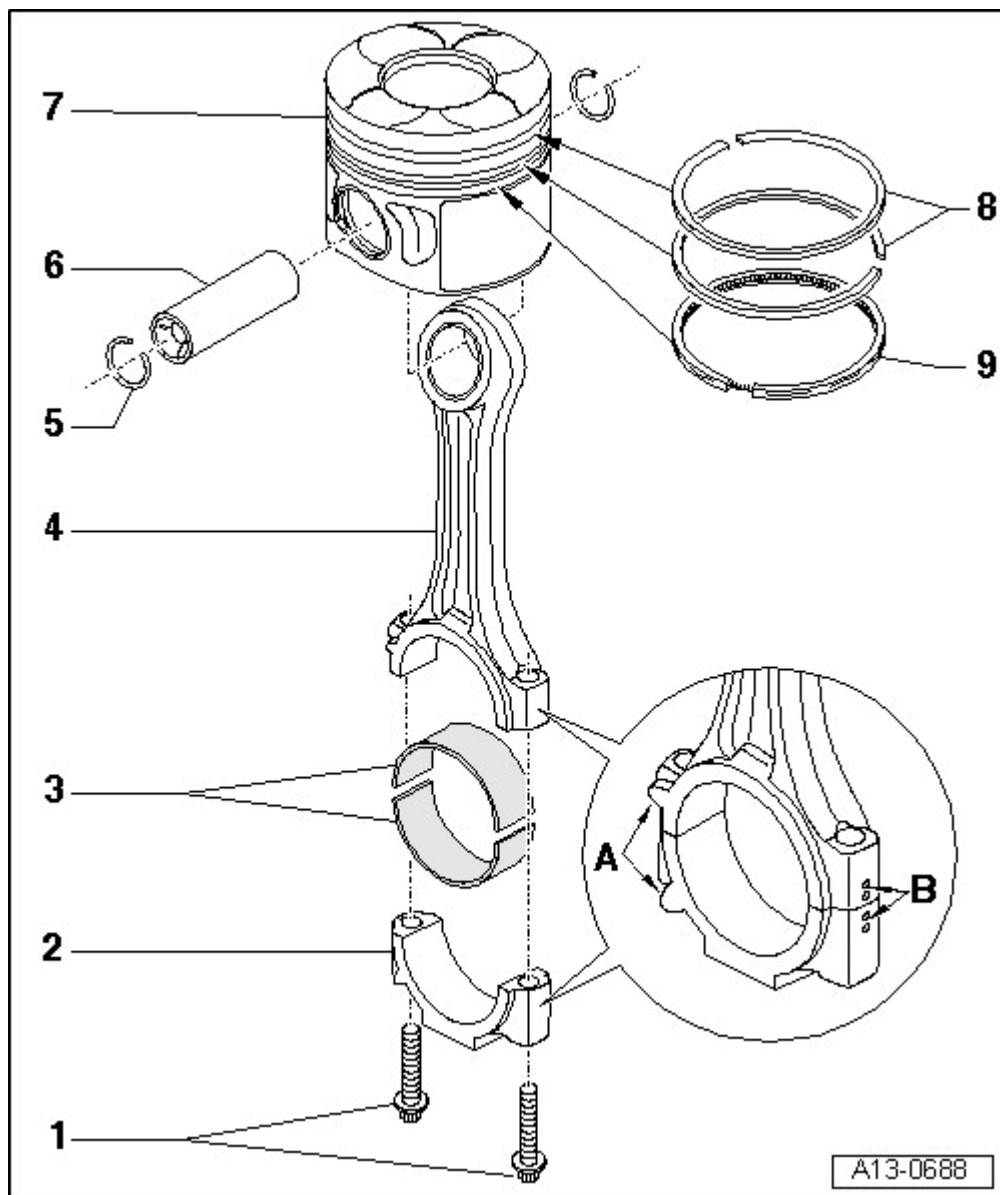
Fig. 12: Pistons And Connecting Rod Assembly Overview
