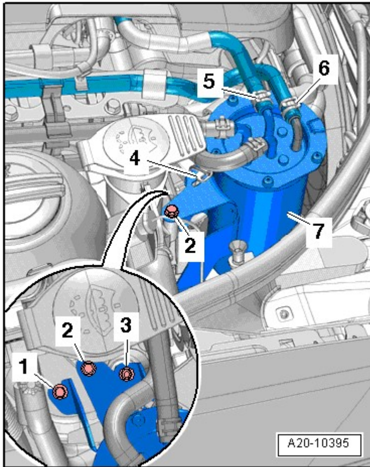
Fig. 25: Identifying Fuel Filter, Bracket And Bolts
