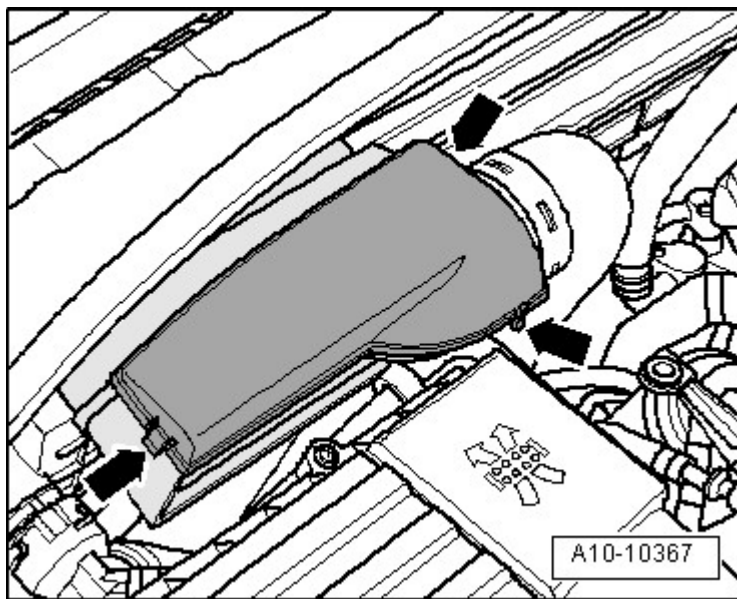
Fig. 27: Identifying Air Duct Cover Slide Clips
