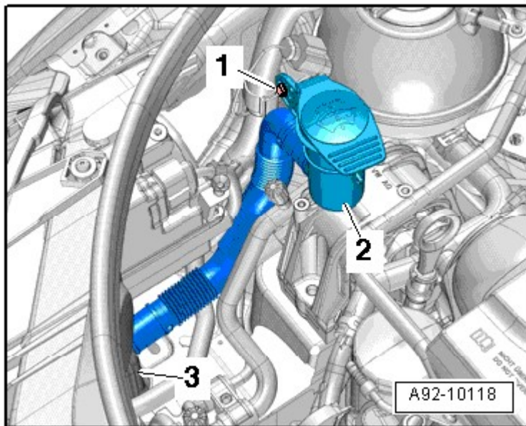
Fig. 21: Identifying Windshield Wiper Fluid Reservoir Filler Tube -2- And Bolt Courtesy of AUDI OF AMERICA, LLC
