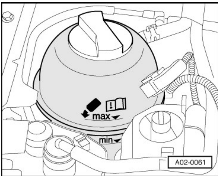
Fig. 25: Coolant Level Markings Courtesy of AUDI OF AMERICA, LLC
