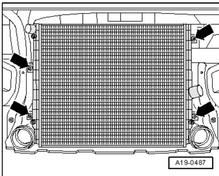
Fig. 40: Identifying Radiator Bolts
