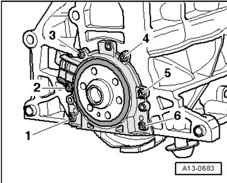
Fig. 10: Tightening Sequence
