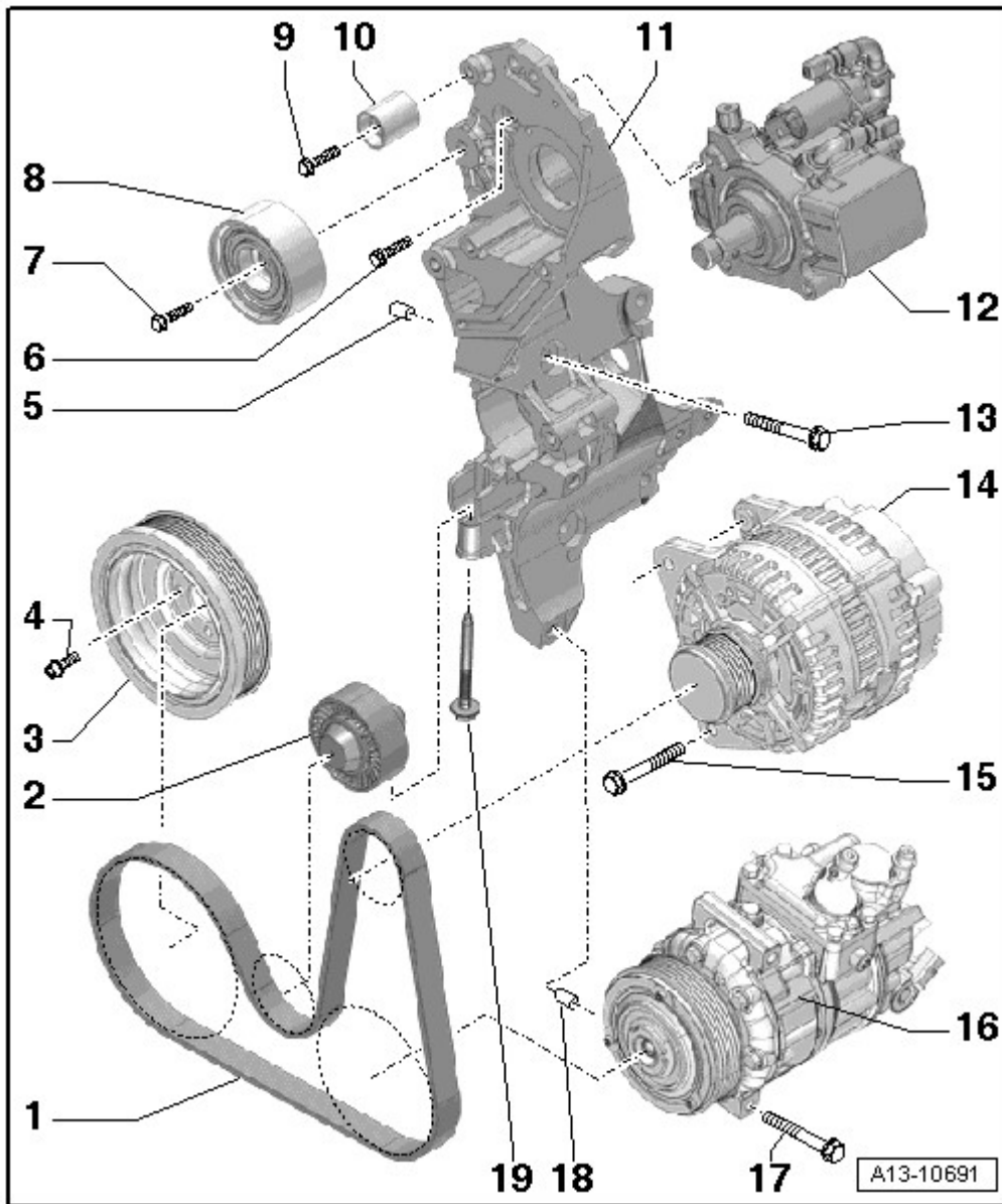
Fig. 3: Identifying Ribbed Belt With Tensioning Roller, Overview Courtesy of AUDI OF AMERICA, LLC
