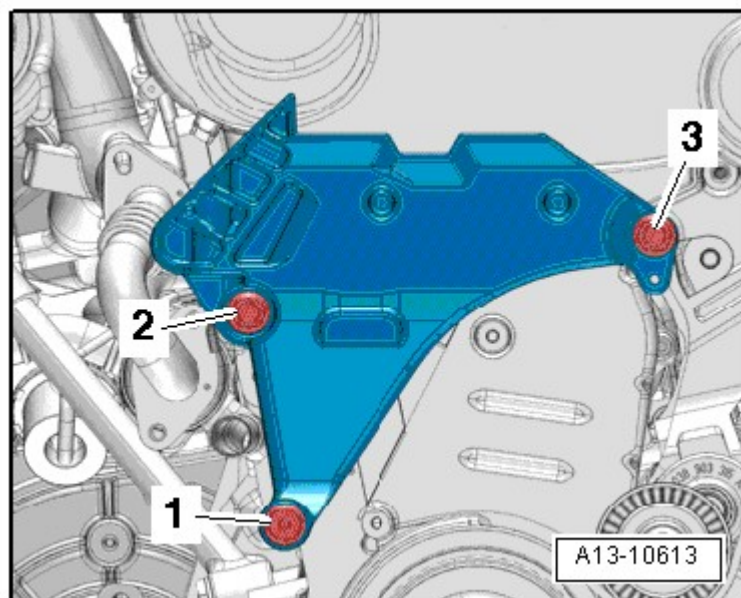
Fig. 18: Identifying Engine Support Bolts
