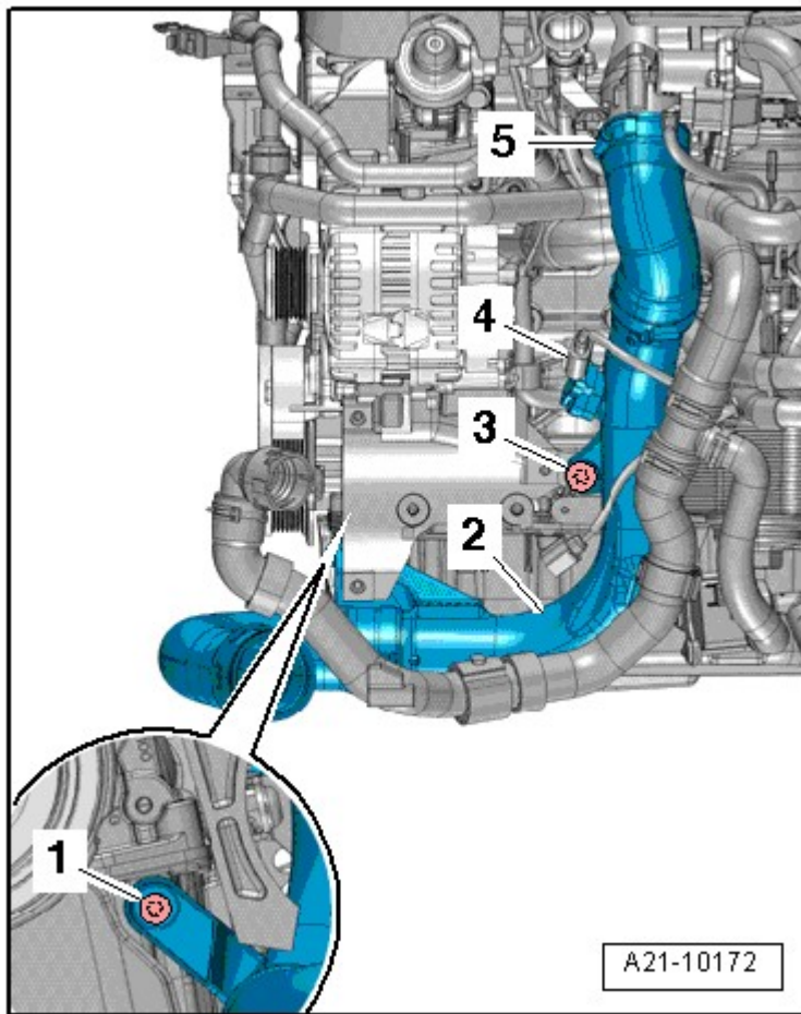
Fig. 65: Identifying Bolts -1- And -3- For Removal
