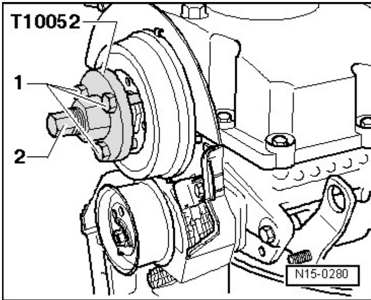
Fig. 89: Identifying Puller T10052 Courtesy of AUDI OF AMERICA, LLC
