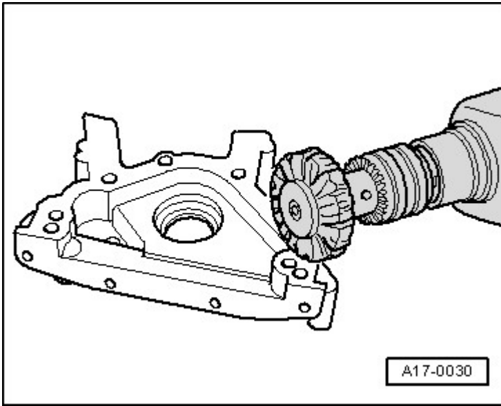
Fig. 61: Identifying Rotating Plastic Brush Courtesy of AUDI OF AMERICA, LLC
