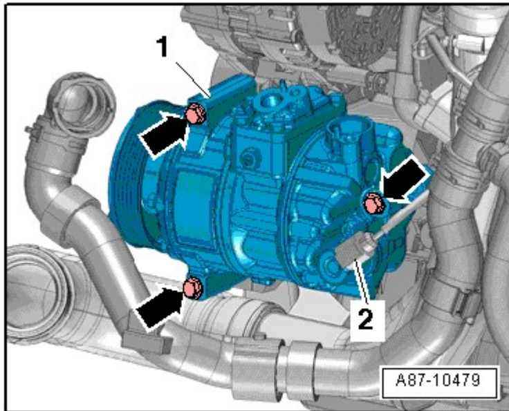
Fig. 86: Identifying A/C Compressor Bolts
