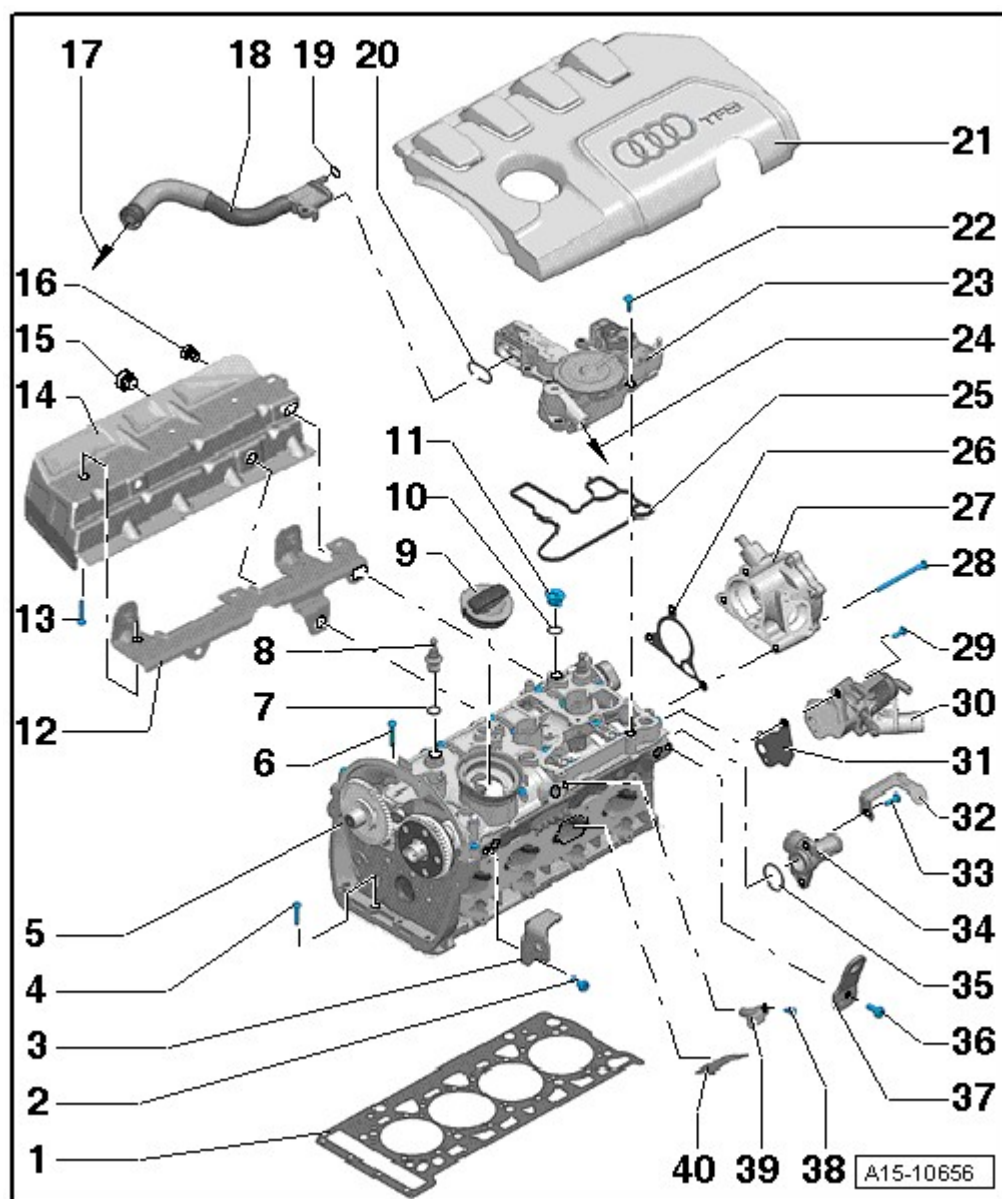
Fig. 10: Identifying Cylinder Head Assembly Overview
