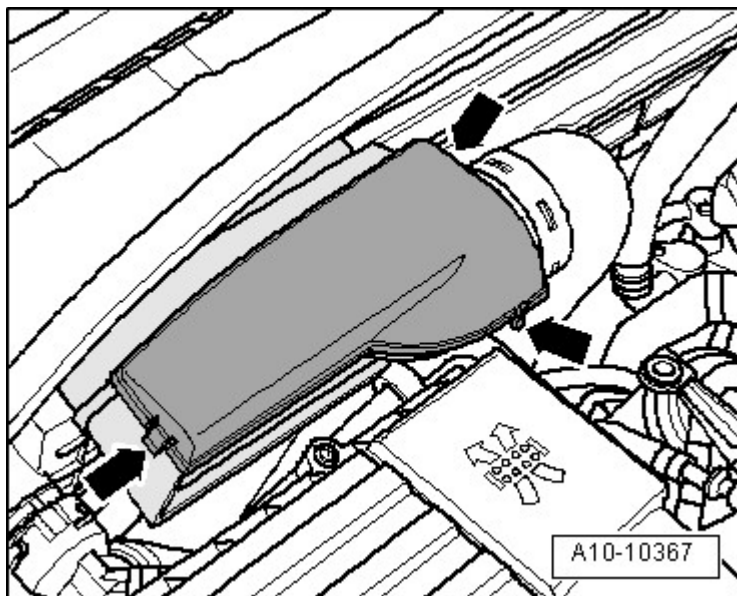
Fig. 136: Identifying Air Duct Cover Slide Clips
