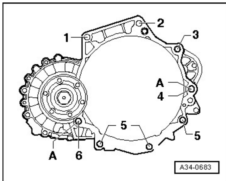
Fig. 100: Manual Transmission To Engine Bolts
