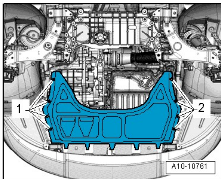
Fig. 53: Identifying Center Noise Insulation
