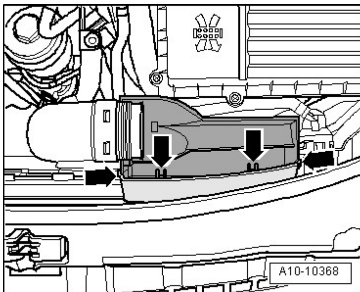
Fig. 137: Identifying Lower Air Guide Clips
