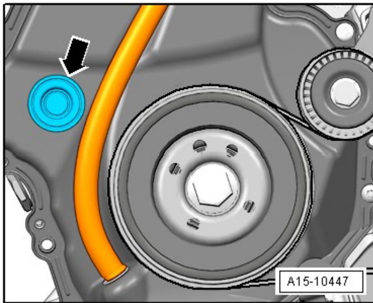
Fig. 124: Locating Plug
