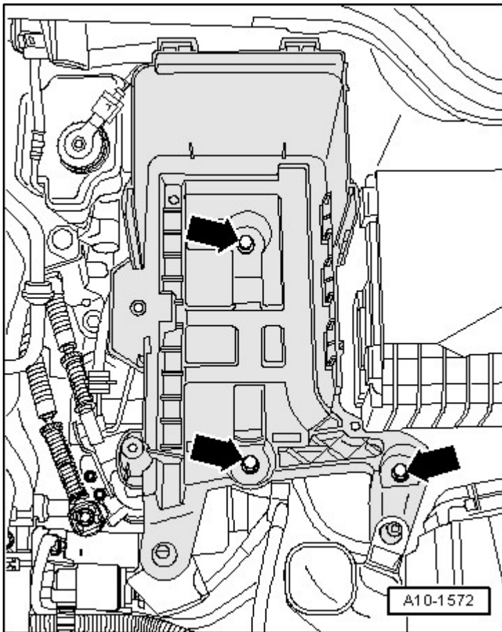
Fig. 8: Battery Carrier Nuts
