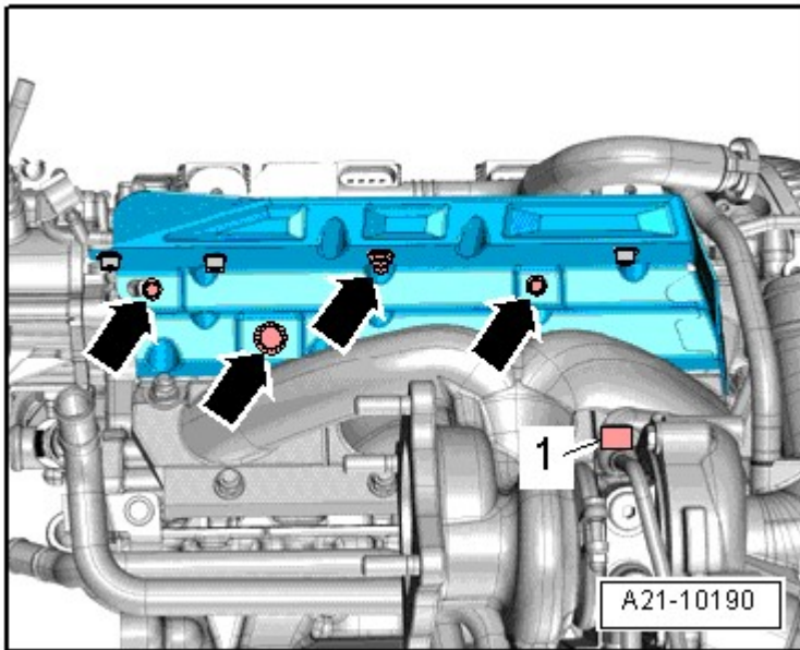
Fig. 104: Identifying Turbocharger And Heatshield
