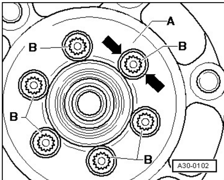
Fig. 52: Identifying Dual-Mass Flywheel & Bolts
