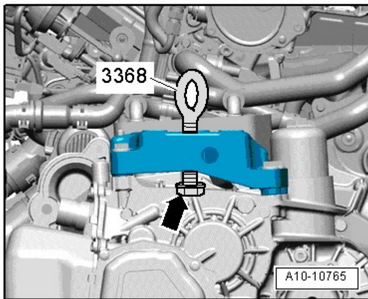
Fig. 97: Lifting Eyebolt 3368
