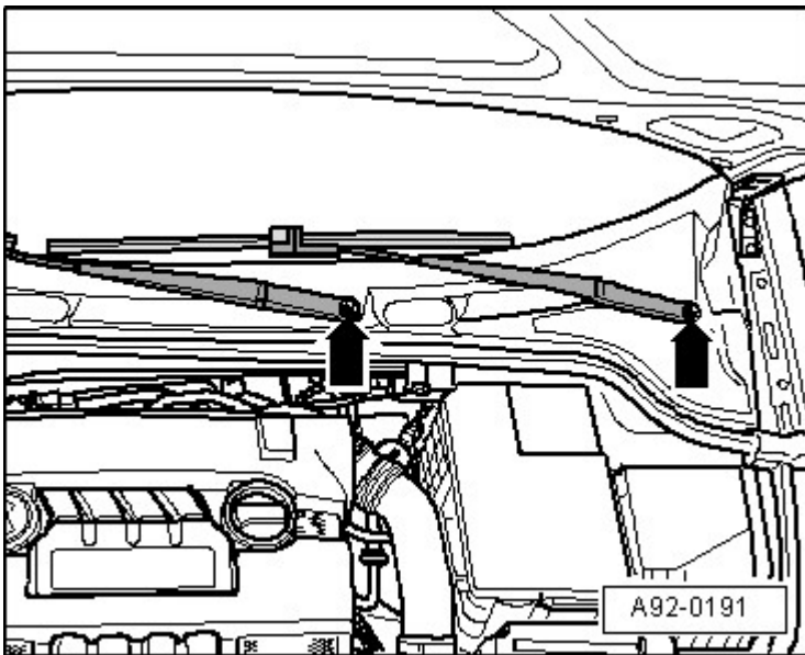
Fig. 51: Identifying Wiper Arm Nuts Courtesy of AUDI OF AMERICA, LLC
