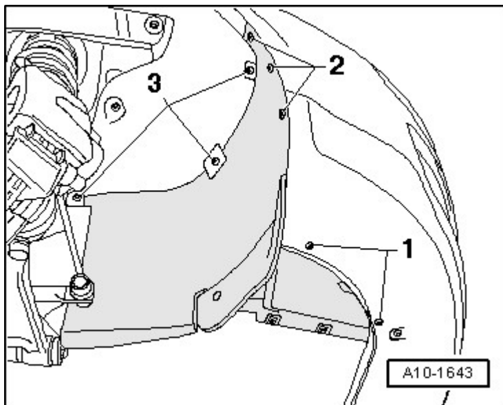
Fig. 24: Identifying Fasteners
