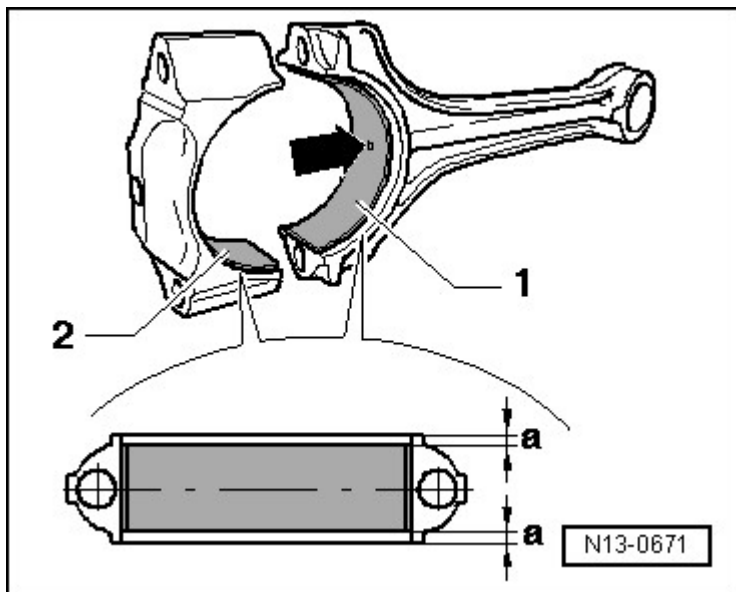
Fig. 18: Bearing Shells - Installed Positions
