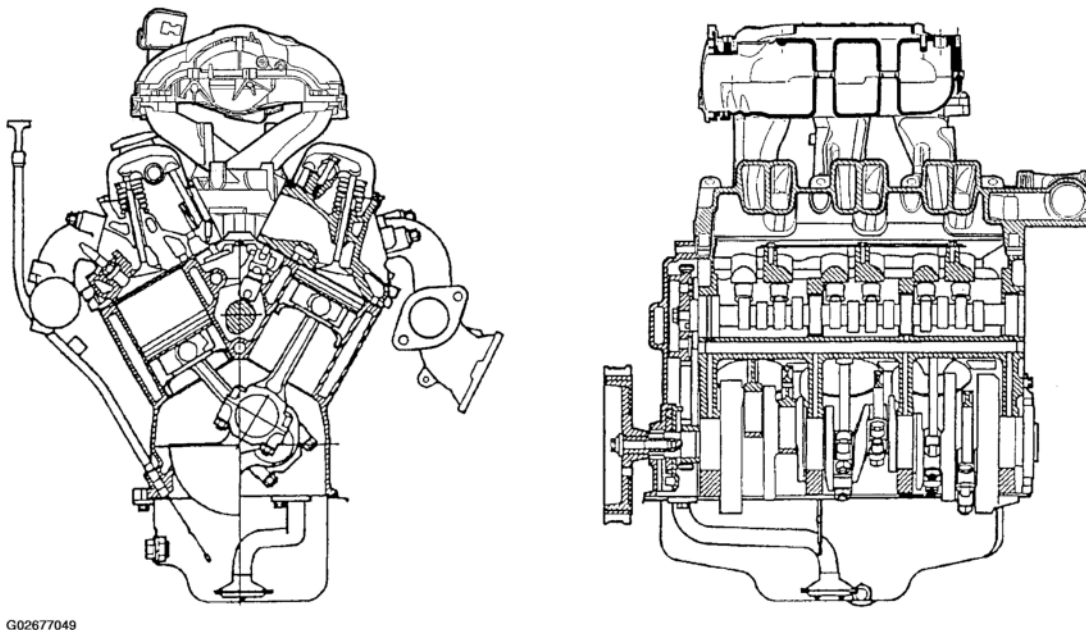
Fig. 1: Identifying 3.3/3.8L V-6 Engines Courtesy of DAIMLERCHRYSLER CORP.
