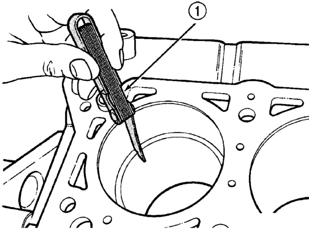
1 - FEELER GAUGE
