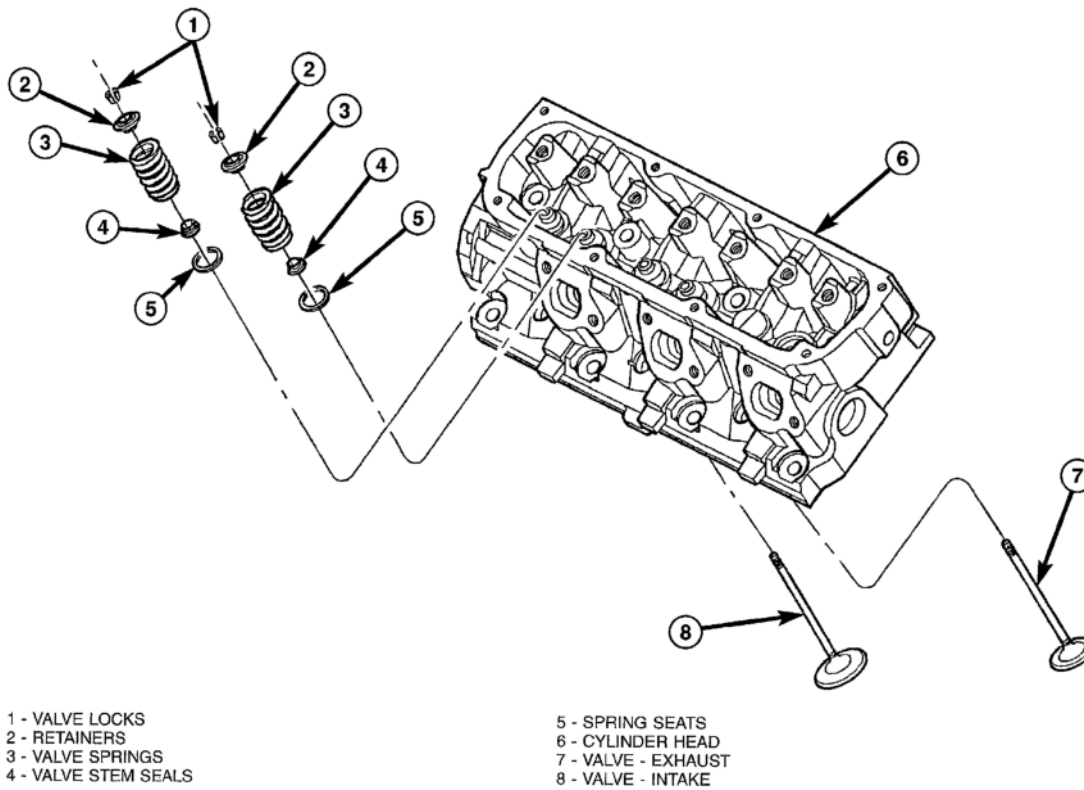
Fig. 47: Identifying Cylinder Head And Components Courtesy of DAIMLERCHRYSLER CORP.
