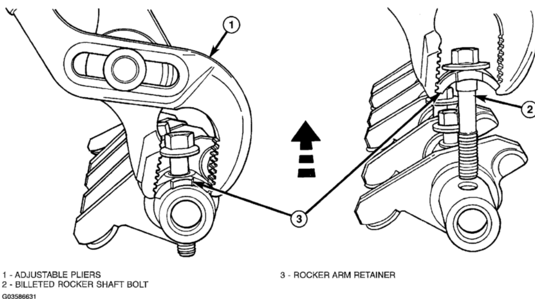
Fig. 71: Removing Rocker Arm Retainer Courtesy of DAIMLERCHRYSLER CORP.
