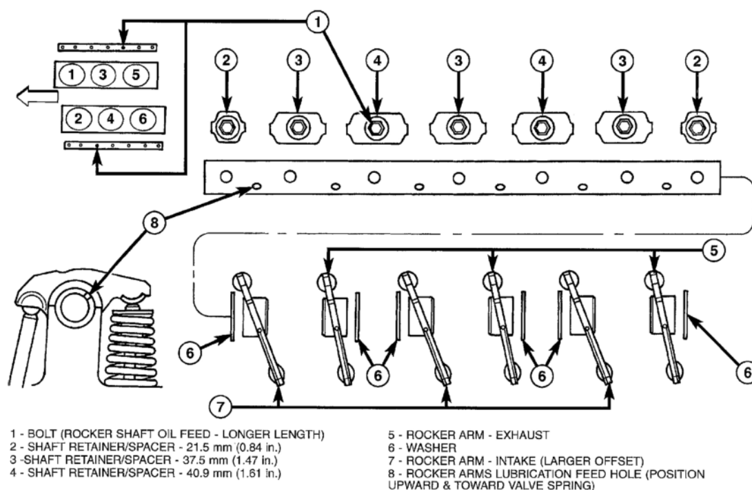
Fig. 72: Positioning Rocker Arm And Shaft Assemblies On Pedestal Mounts Courtesy of DAIMLERCHRYSLER CORP.
