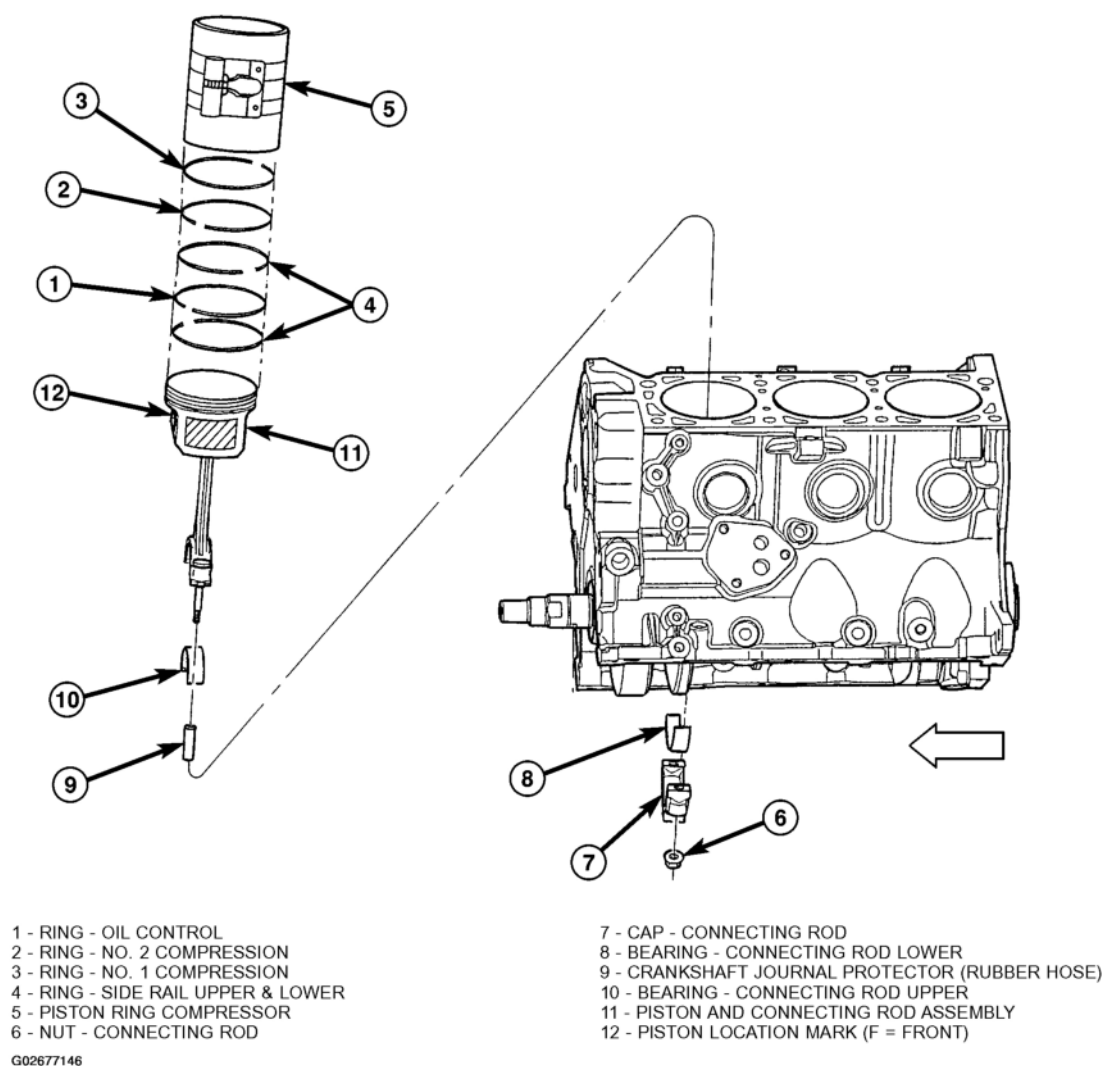
Fig. 89: Installing Piston And Connecting Rod Courtesy of DAIMLERCHRYSLER CORP.
