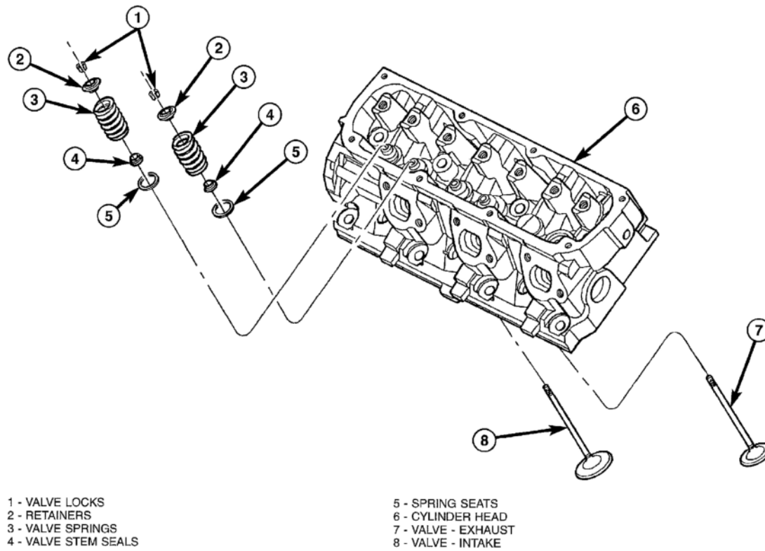
Fig. 64: Identifying Valve Components Courtesy of DAIMLERCHRYSLER CORP.
