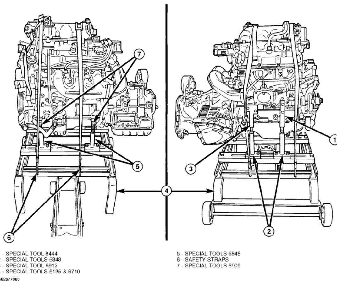
Fig. 17: Positioning Engine Cradle Support Post Mounts Courtesy of DAIMLERCHRYSLER CORP.
