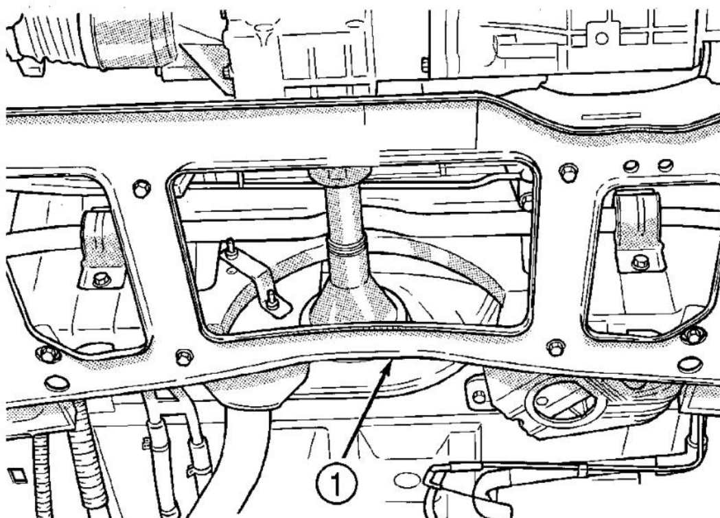
1 - CRADLE PLATE
