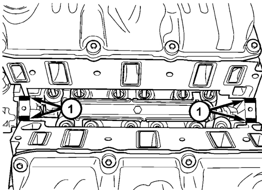
1 - SEALER LOCATIONS
