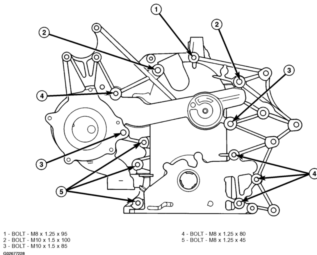
Fig. 171: Identifying Timing Chain Cover Bolt Locations Courtesy of DAIMLERCHRYSLER CORP.
