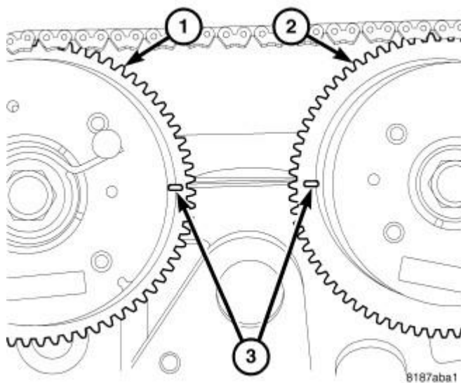
Fig. 148: Camshaft Timing Courtesy of CHRYSLER LLC
