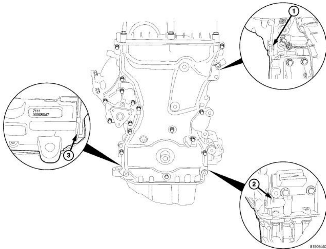
Fig. 351: TIMING CHAIN COVER PRY POINTS Courtesy of CHRYSLER LLC
