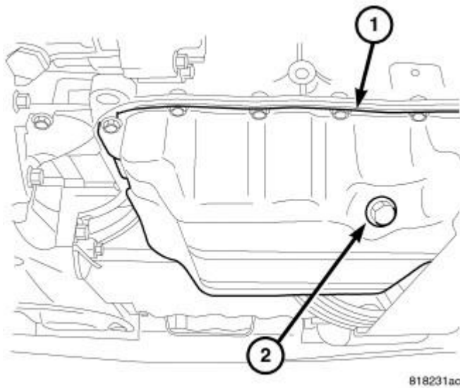
Fig. 180: OIL DRAIN PLUG
