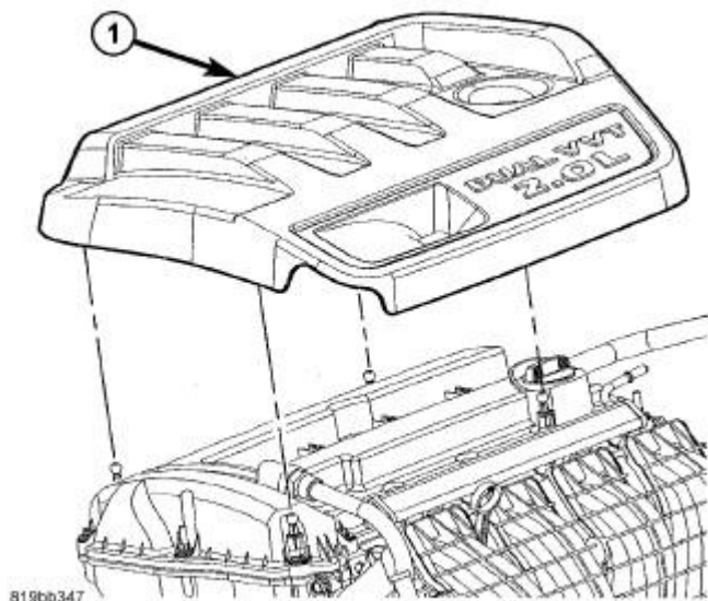
Fig. 26: ENGINE COVER-2.0L
