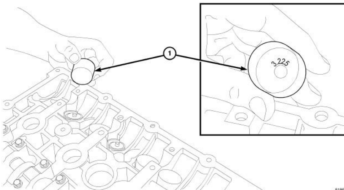
Fig. 123: TAPPET IDENTIFICATION
