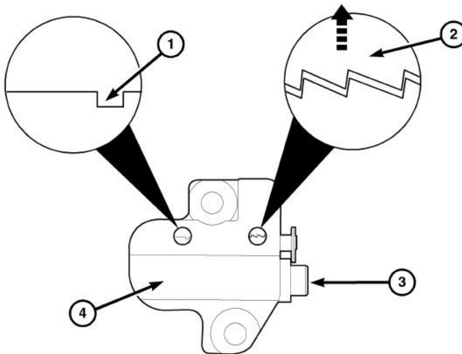
Fig. 131: TENSIONER RESET Courtesy of CHRYSLER LLC
