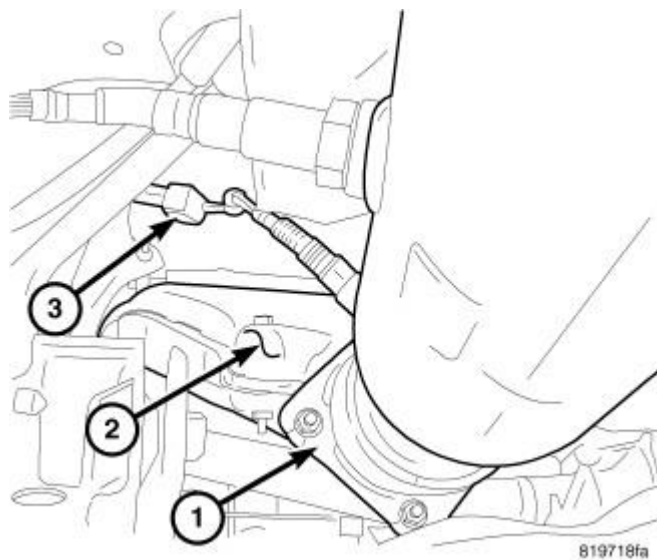
Fig. 19: CAT AT EXHAUST MANIFOLD Courtesy of CHRYSLER LLC
