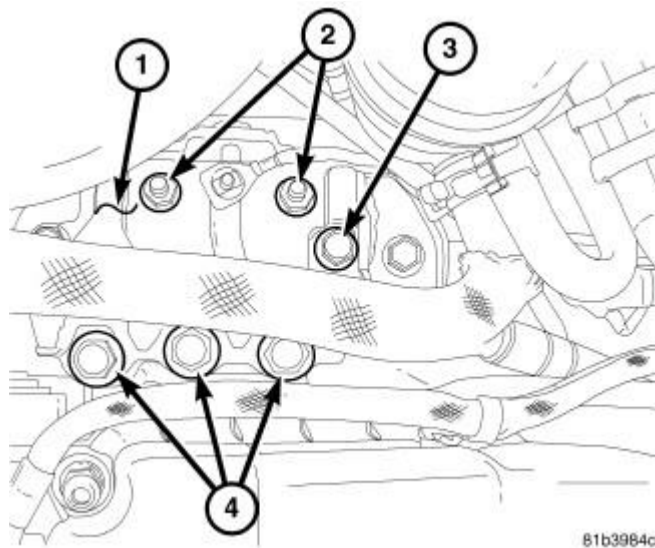
Fig. 360: Right Engine Mount Bracket & Retaining Bolts Courtesy of CHRYSLER LLC
