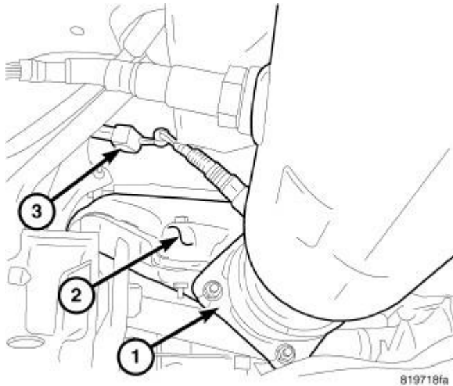
Fig. 32: CAT AT EXHAUST MANIFOLD Courtesy of CHRYSLER LLC
