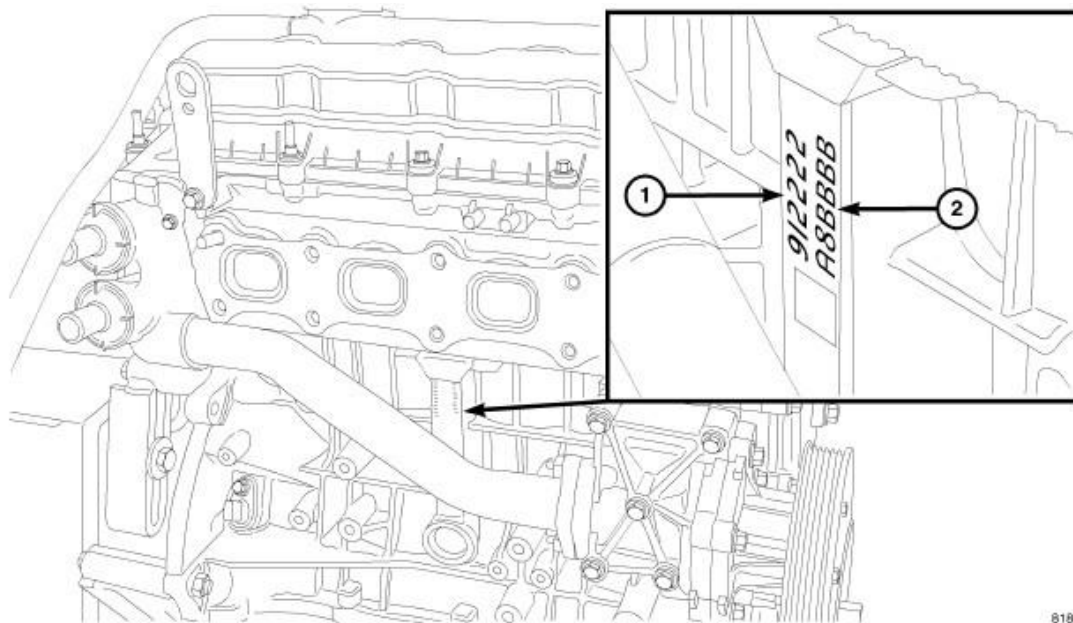
Fig. 177: MAIN BEARING SELECTION CHART Courtesy of CHRYSLER LLC
