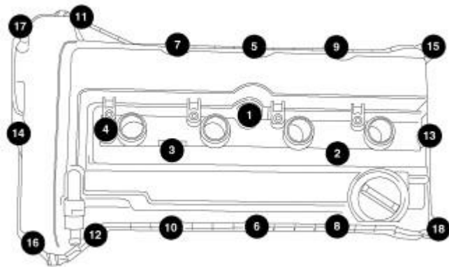
Fig. 342: Removing/Installing Cylinder Head Cover Bolts In Sequence Courtesy of CHRYSLER LLC
