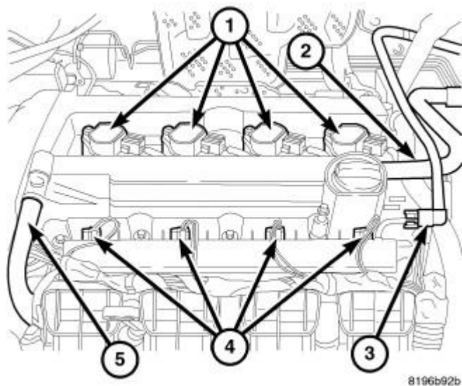
Fig. 159: Coil Connector
