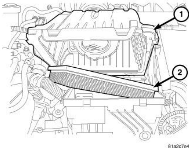
Fig. 58: AIR FILTER ELEMENT Courtesy of CHRYSLER LLC
