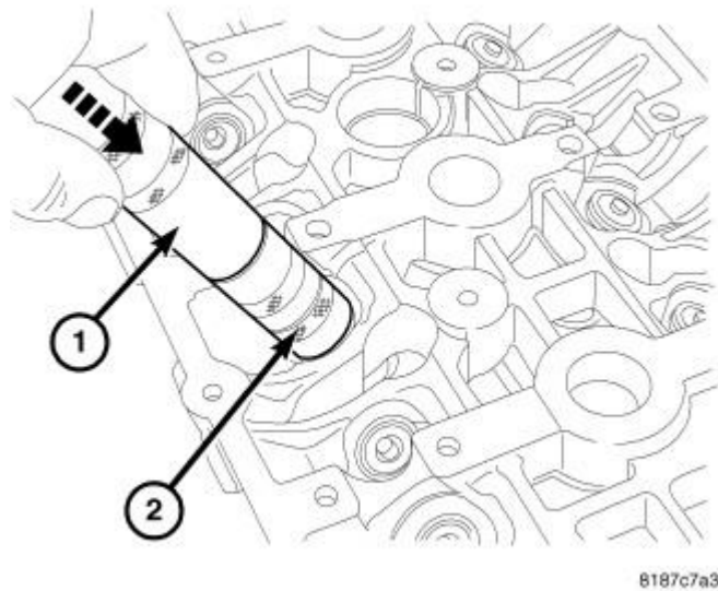
Fig. 166: VALVE INSTALLATION
