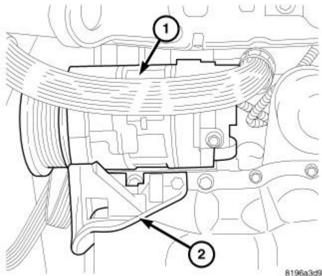
Fig. 275: A/C COMPRESSOR Courtesy of CHRYSLER LLC
