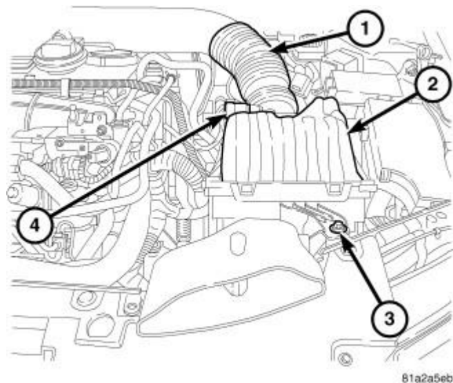
Fig. 319: Air Cleaner Housing & Retaining Bolt
