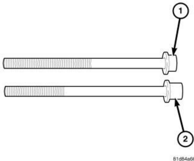
Fig. 94: CYLINDER HEAD BOLT IDENTIFICATION Courtesy of CHRYSLER LLC
