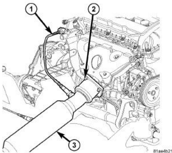
Fig. 107: CATALYTIC CONVERTER - 2.0L/2.4L
