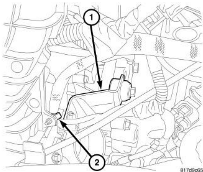
Fig. 16: THROTTLE BODY SUPPORT
