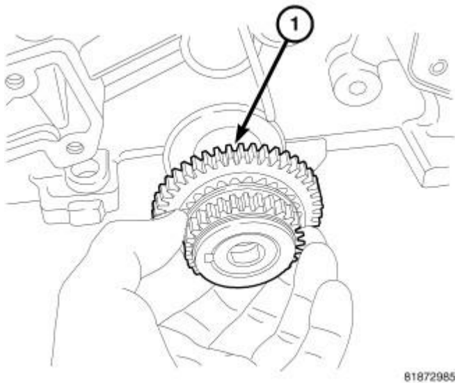
Fig. 327: CRANKSHAFT SPROCKET Courtesy of CHRYSLER LLC
