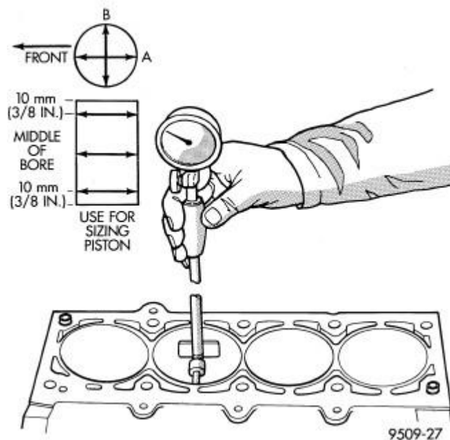
Fig. 214: Checking Cylinder Bore Size
