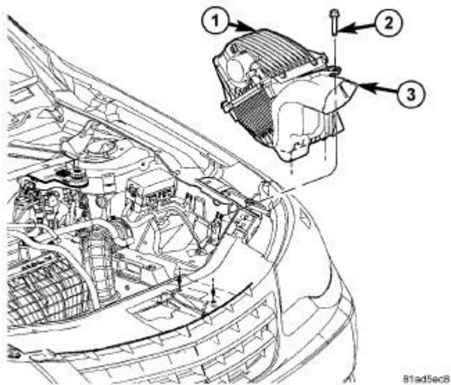
Fig. 44: Air Cleaner Housing Assembly Courtesy of CHRYSLER LLC
