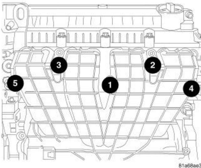
Fig. 84: Removing/Installing Intake Bolts In Sequence Courtesy of CHRYSLER LLC
