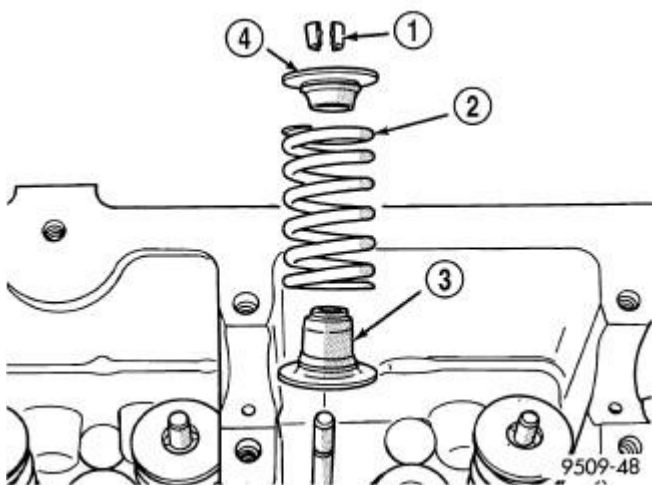
Fig. 167: Valve Stem Seal/Valve Spring Seat
