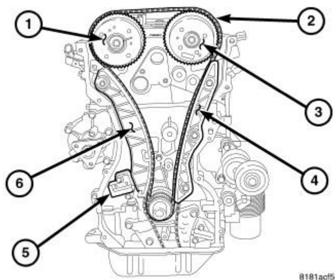
Fig. 337: TIMING DRIVE Courtesy of CHRYSLER LLC
