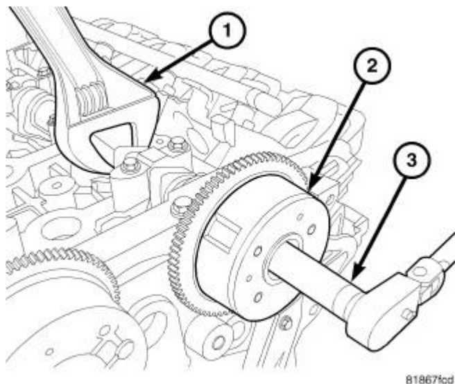
Fig. 116: Cam Phaser Installation Courtesy of CHRYSLER LLC
