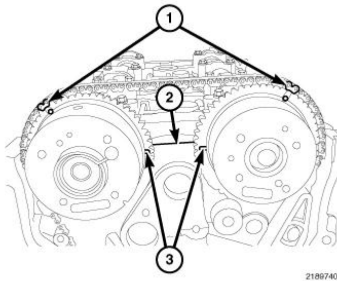
Fig. 142: Timing Chain Timing Marks
