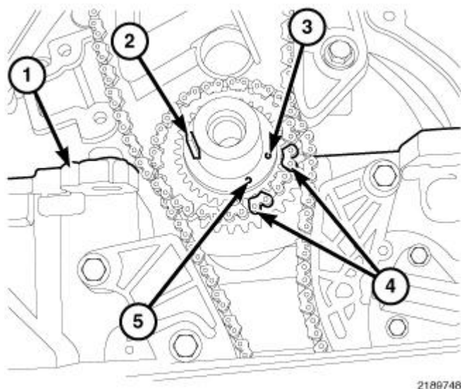
Fig. 324: Crankshaft Timing Marks
