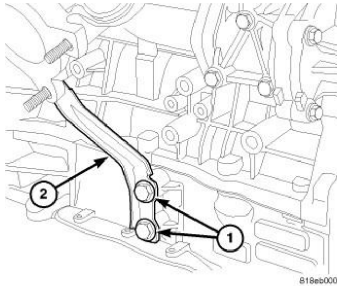
Fig. 304: EXHAUST MANIFOLD SUPPORT BRACKET Courtesy of CHRYSLER LLC
