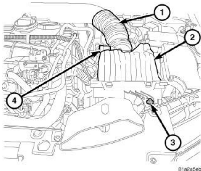
Fig. 61: Air Cleaner Housing & Retaining Bolt Courtesy of CHRYSLER LLC
