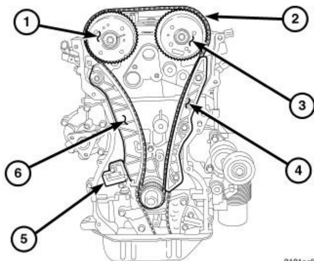
Fig. 105: TIMING DRIVE
