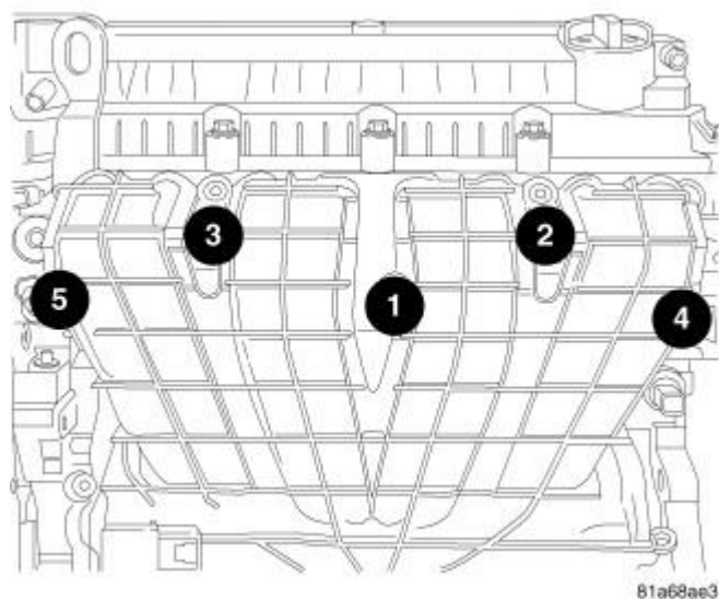
Fig. 17: INTAKE TORQUE SEQUENCE
