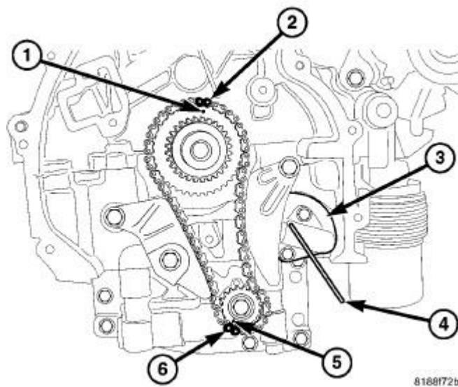
Fig. 332: BSM TENSIONER Courtesy of CHRYSLER LLC
