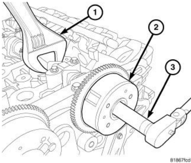
Fig. 115: CAM PHASER INSTALLATION
