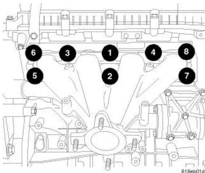
Fig. 306: EXHAUST MANIFOLD BOLT TORQUE SEQUENCE Courtesy of CHRYSLER LLC
