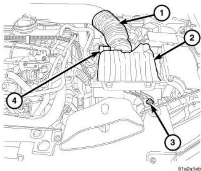
Fig. 312: Air Cleaner Housing & Retaining Bolt
