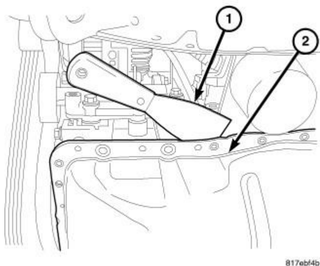
Fig. 276: OIL PAN REMOVAL Courtesy of CHRYSLER LLC
