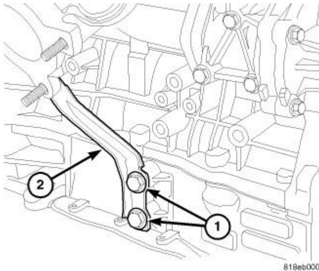
Fig. 308: EXHAUST MANIFOLD SUPPORT BRACKET Courtesy of CHRYSLER LLC
