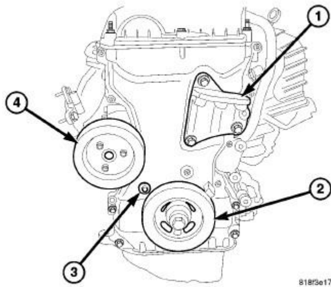
Fig. 350: ENGINE FRONT Courtesy of CHRYSLER LLC
