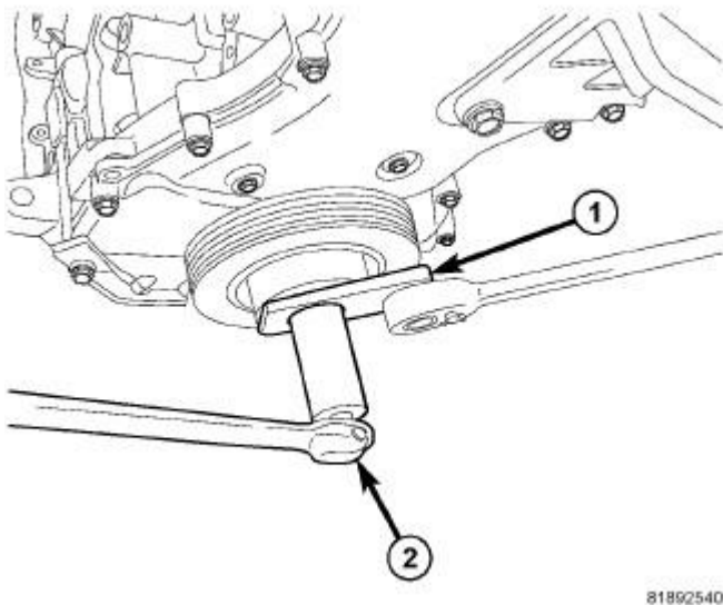
Fig. 201: DAMPER REMOVAL/INSTALLATION Courtesy of CHRYSLER LLC
