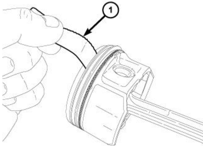
Fig. 209: Checking Piston Ring To Groove Side Clearance Courtesy of CHRYSLER LLC
