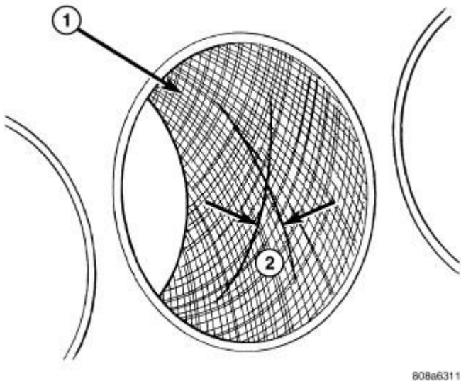
Fig. 171: Cylinder Bore Cross-Hatch Pattern Courtesy of CHRYSLER LLC
