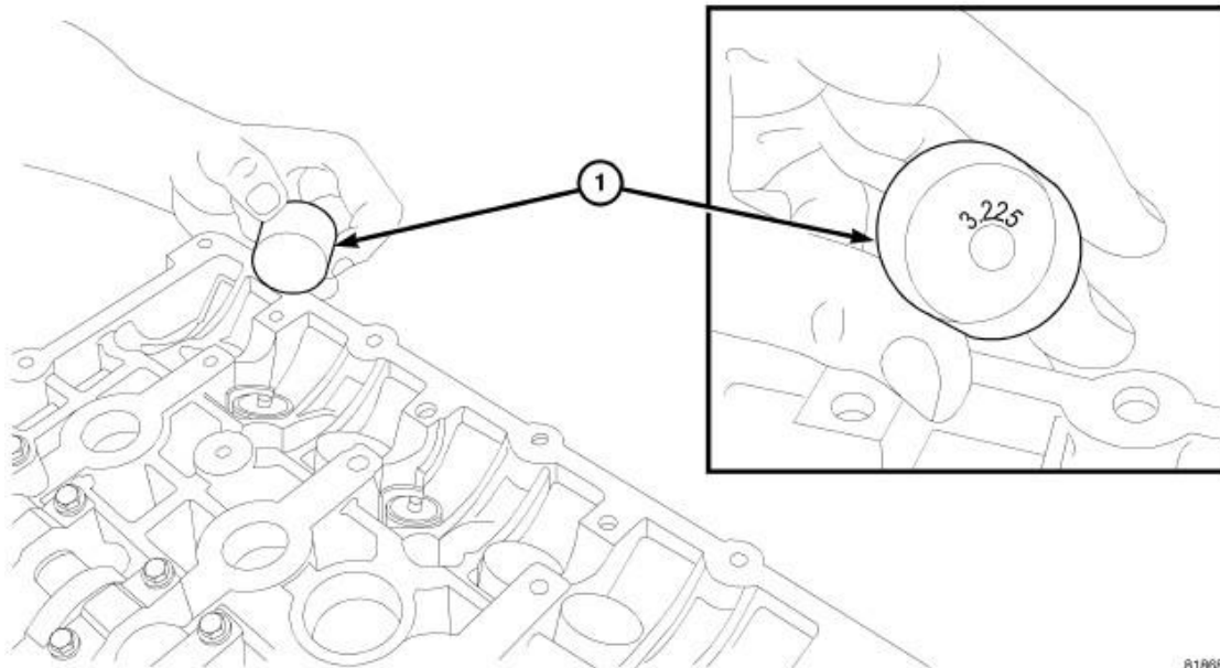
Fig. 122: TAPPET IDENTIFICATION
