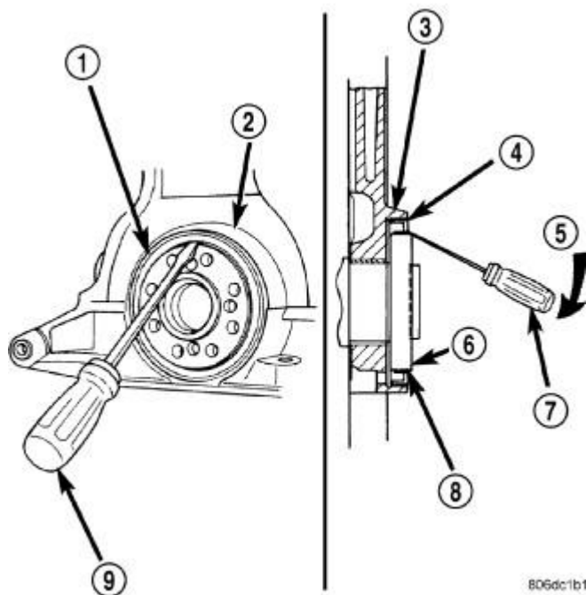
Fig. 227: Rear Crankshaft Oil Seal - Removal
