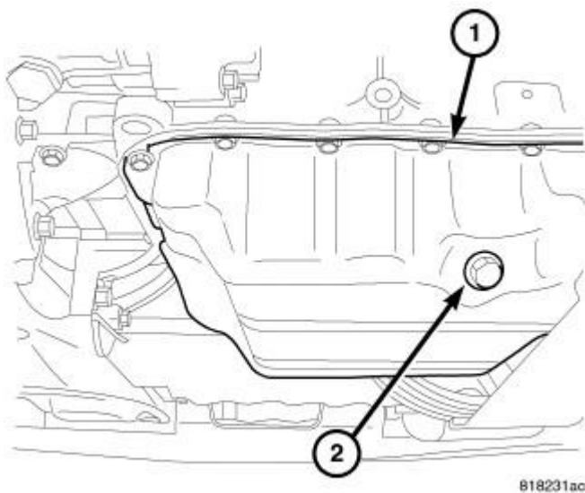
Fig. 270: OIL DRAIN PLUG Courtesy of CHRYSLER LLC
