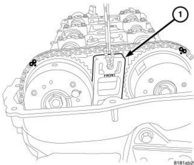
Fig. 132: WEDGE TOOL Courtesy of CHRYSLER LLC
