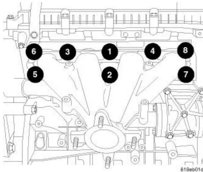
Fig. 305: EXHAUST MANIFOLD BOLT TORQUE SEQUENCE Courtesy of CHRYSLER LLC
