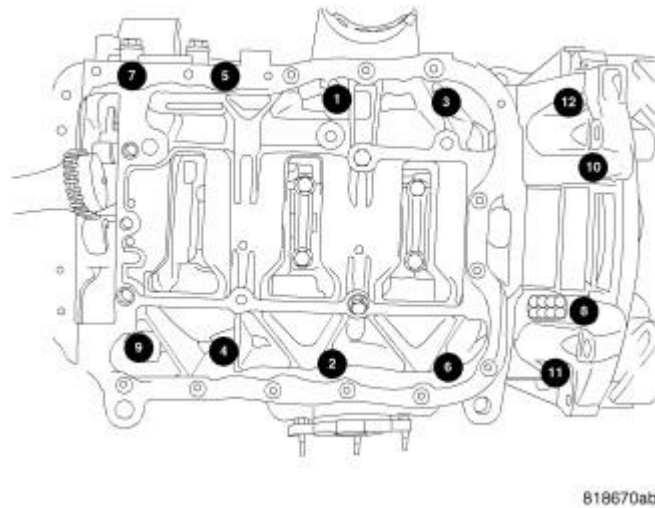
Fig. 207: LADDER FRAME TORQUE Courtesy of CHRYSLER LLC
