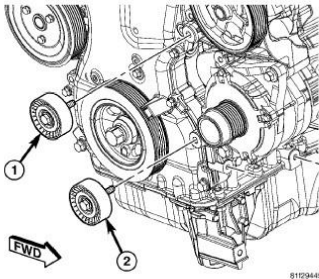
Fig. 75: Removing/Installing Accessory Drive Belt Lower Idler Pulley Courtesy of CHRYSLER LLC
