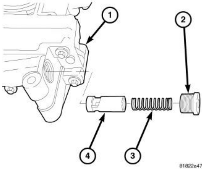
Fig. 301: OIL PRESSURE RELIEF VALVE
