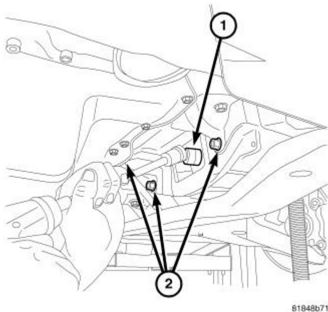
Fig. 21: MODULAR CLUTCH TO FLEX PLATE BOLTS Courtesy of CHRYSLER LLC
