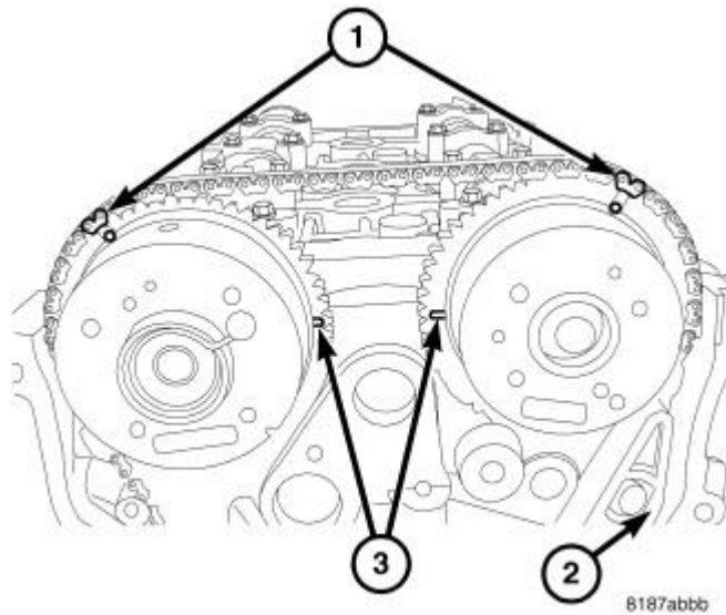
Fig. 129: TIMING CHAIN TIMING MARKS Courtesy of CHRYSLER LLC
