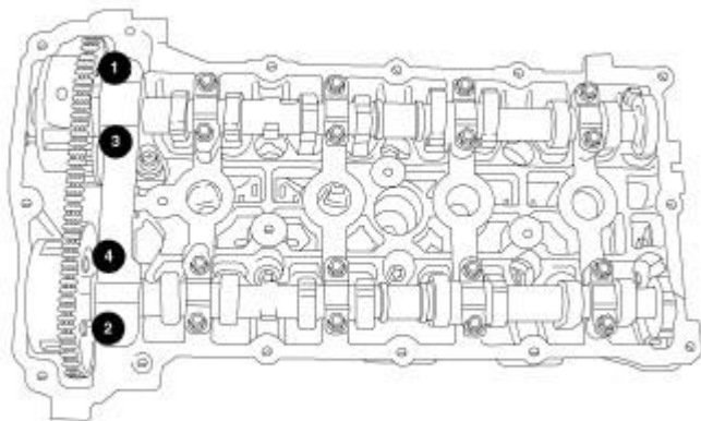
Fig. 134: FRONT CAM CAP REMOVAL SEQUENCE
