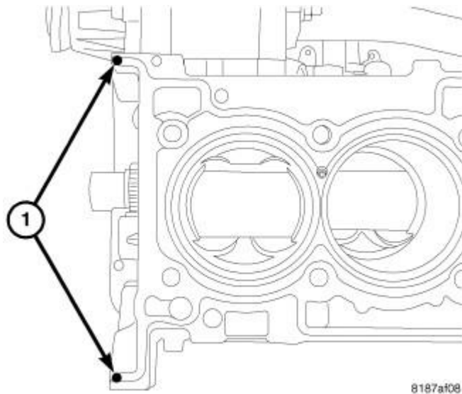
Fig. 93: CYLINDER HEAD GASKET RTV Courtesy of CHRYSLER LLC
