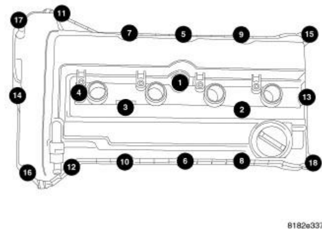
Fig. 154: Removing/Installing Cylinder Head Cover Bolts In Sequence Courtesy of CHRYSLER LLC
