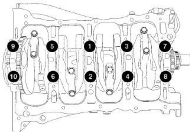
Fig. 187: MAIN BEARING CAP TORQUE SEQUENCE
