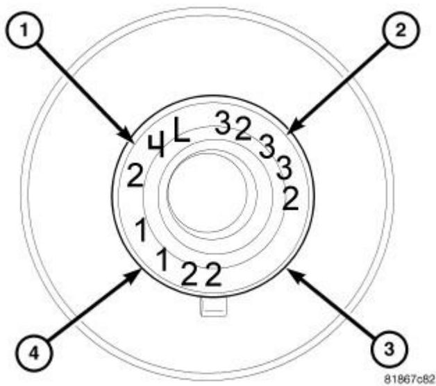
Fig. 173: BEARING SELECTION
