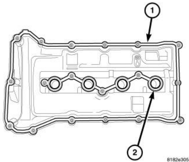
Fig. 149: GASKET LOCATION
