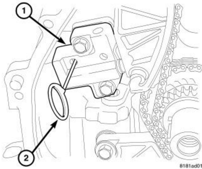
Fig. 373: TIMING CHAIN TENSIONER
