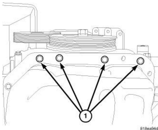
Fig. 72: TIMING CHAIN COVER LOWER BOLTS Courtesy of CHRYSLER LLC
