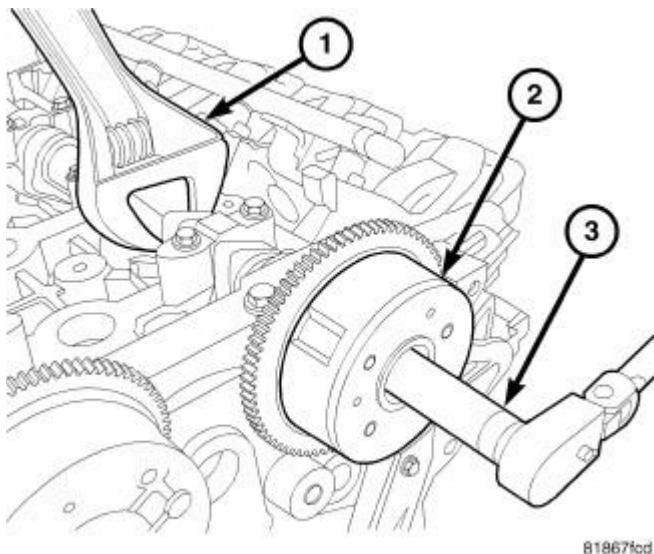
Fig. 333: CAM PHASER INSTALLATION Courtesy of CHRYSLER LLC
