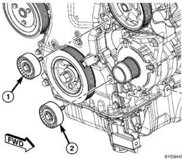
Fig. 363: Removing/Installing Accessory Drive Belt Lower Idler Pulley Courtesy of CHRYSLER LLC
