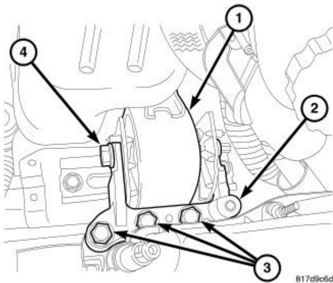
Fig. 237: RIGHT ENGINE MOUNT Courtesy of CHRYSLER LLC
