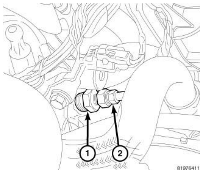
Fig. 245: OIL PRESSURE ADAPTER 9879
