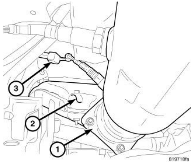
Fig. 309: CAT AT EXHAUST MANIFOLD Courtesy of CHRYSLER LLC
