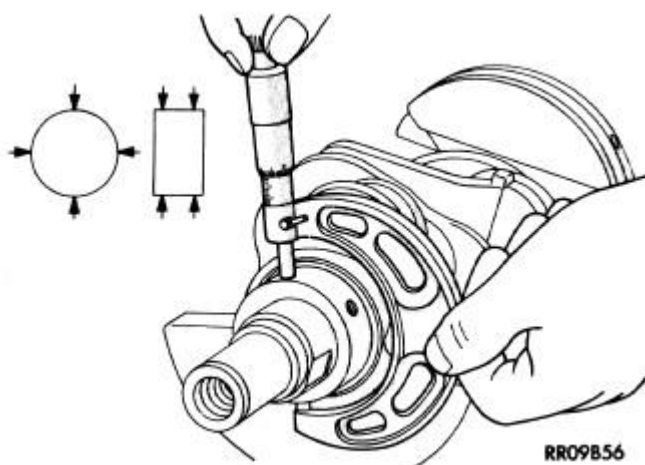
Fig. 188: Crankshaft Journal Measurements - Typical Courtesy of CHRYSLER LLC
