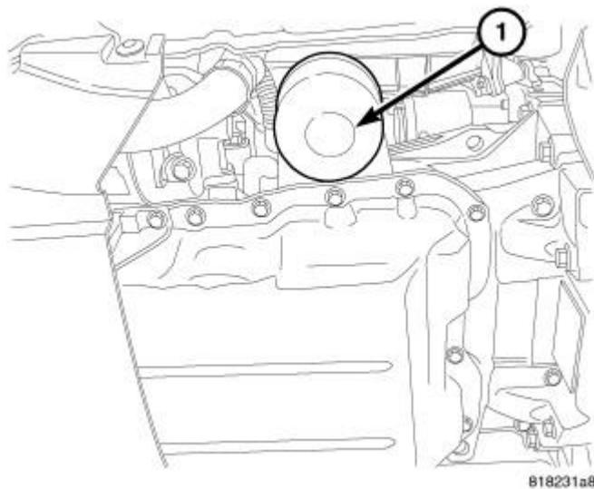
Fig. 216: Oil Filter
