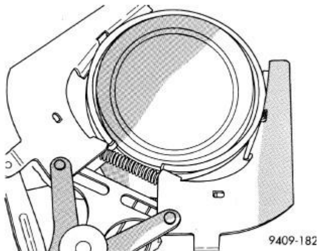
Fig. 210: Piston Rings-Removing and Installing Courtesy of CHRYSLER LLC
