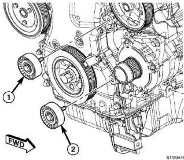
Fig. 70: Removing/Installing Accessory Drive Belt Lower Idler Pulley Courtesy of CHRYSLER LLC
