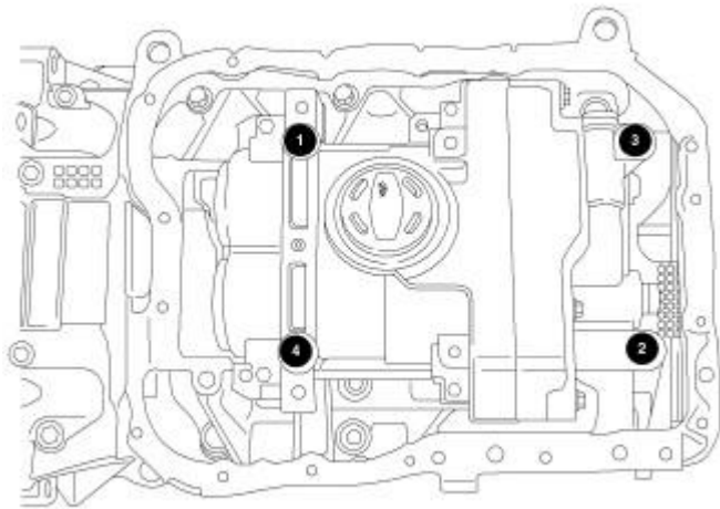
Fig. 291: BSM TORQUE SEQUENCE Courtesy of CHRYSLER LLC
