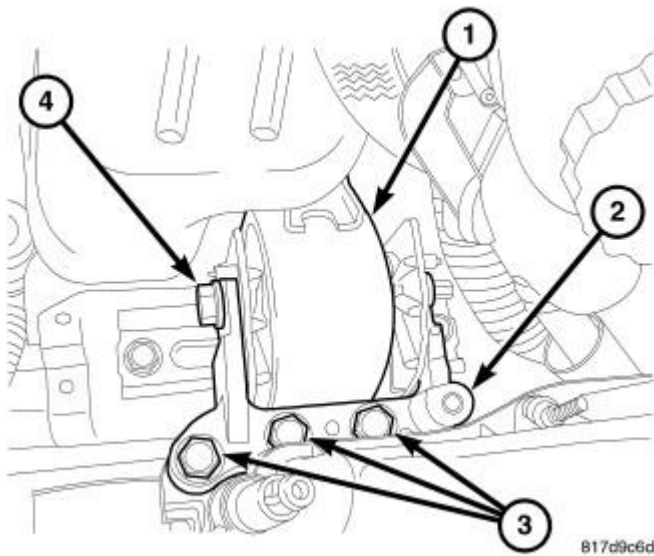
Fig. 236: RIGHT ENGINE MOUNT Courtesy of CHRYSLER LLC
