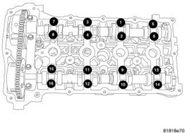
Fig. 103: CAM CAP TORQUE SEQUENCE
