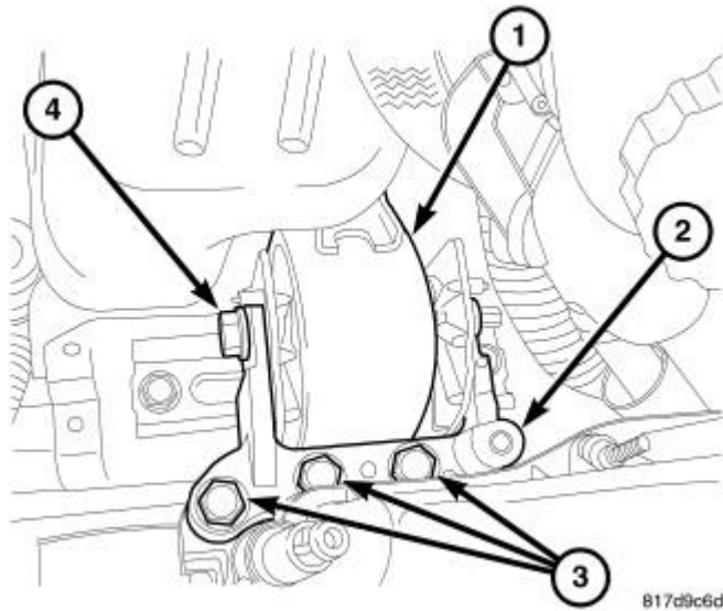
Fig. 28: RIGHT ENGINE MOUNT
