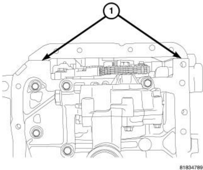
Fig. 277: SEALER LOCATION Courtesy of CHRYSLER LLC
