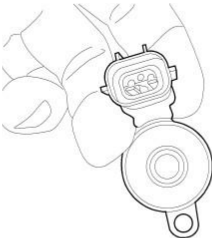
Fig. 257: SOLENOID MOUNTING TAB 1/1 Courtesy of CHRYSLER LLC
