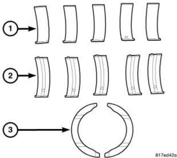
Fig. 192: BEARING IDENTIFICATION
