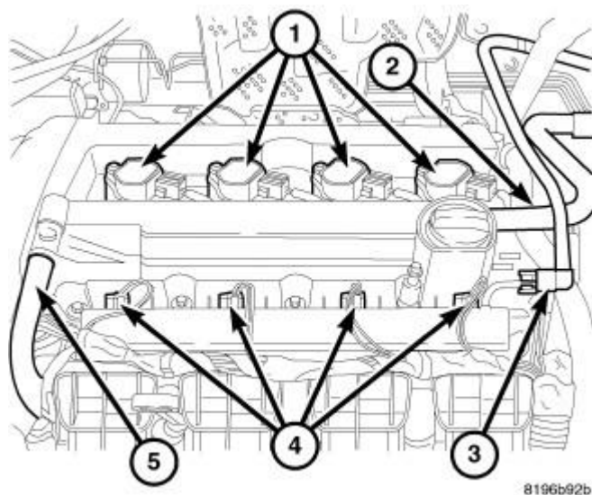
Fig. 110: COIL CONNECTOR Courtesy of CHRYSLER LLC
