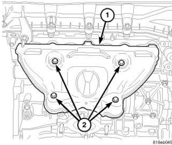
Fig. 307: EXHAUST MANIFOLD HEAT SHIELD Courtesy of CHRYSLER LLC
