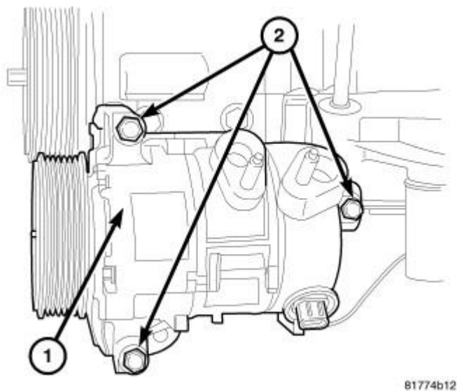
Fig. 298: Removing/Installing A/C Compressor Courtesy of CHRYSLER LLC
