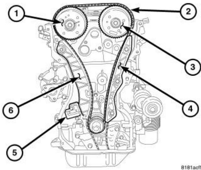
Fig. 321: TIMING DRIVE Courtesy of CHRYSLER LLC
