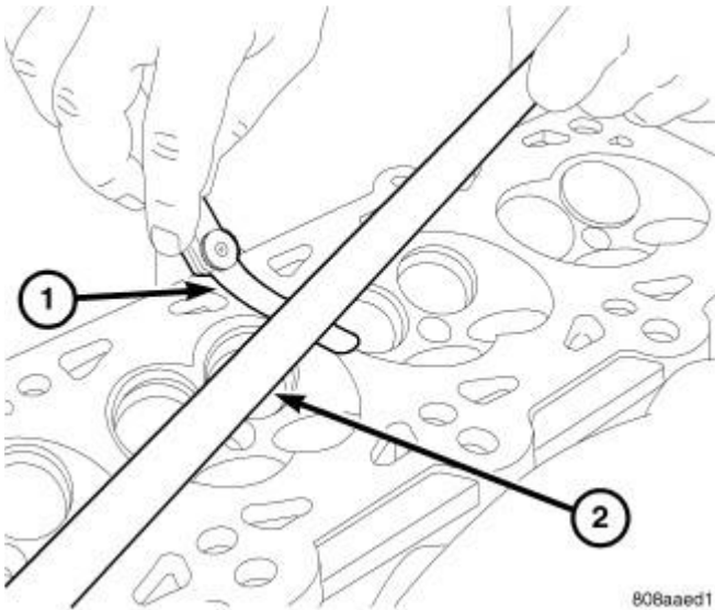
Fig. 89: Checking Cylinder Head Flatness
