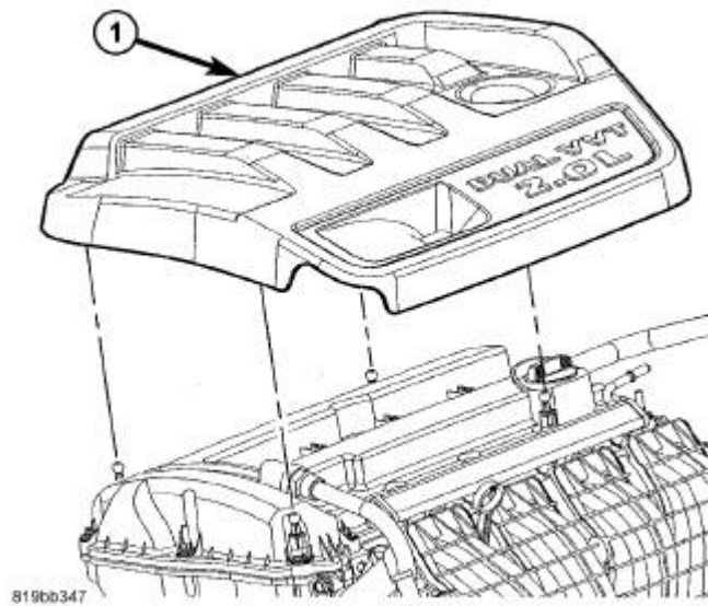
Fig. 45: ENGINE COVER-2.0L Courtesy of CHRYSLER LLC
