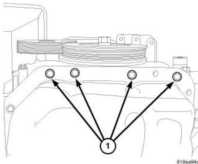
Fig. 347: TIMING CHAIN COVER LOWER BOLTS Courtesy of CHRYSLER LLC
