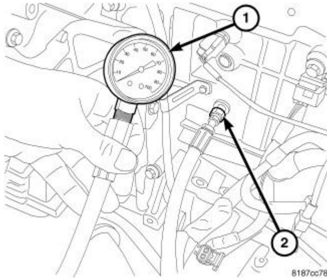
Fig. 249: OIL PRESSURE GAUGE Courtesy of CHRYSLER LLC
