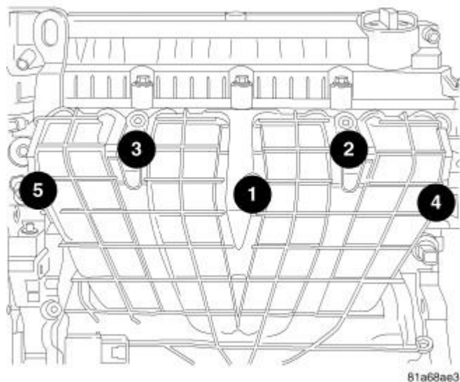
Fig. 316: Removing/Installing Intake Bolts - Torque Sequence Courtesy of CHRYSLER LLC
