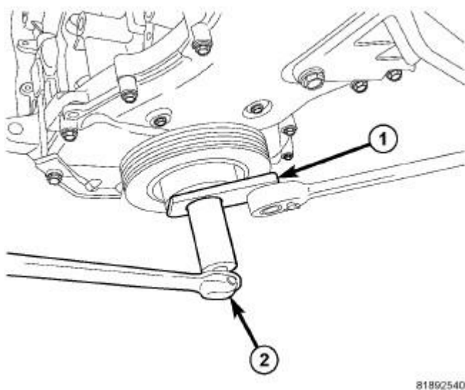
Fig. 220: Damper Removal Courtesy of CHRYSLER LLC
