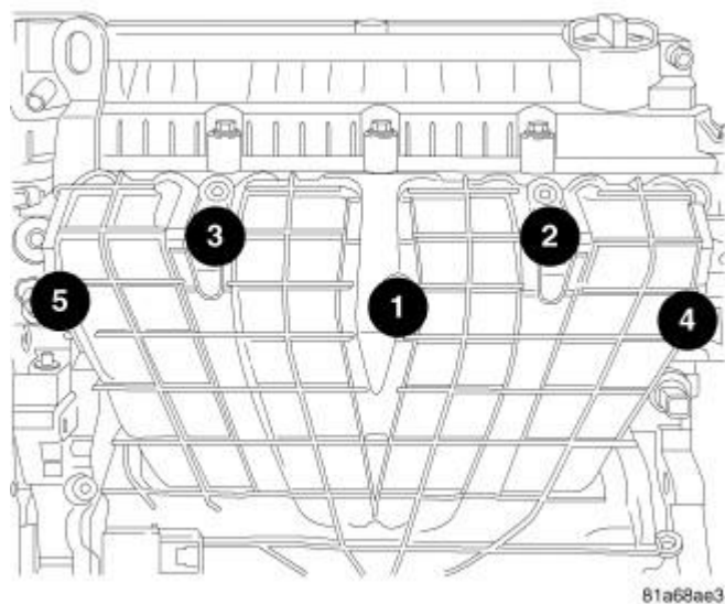
Fig. 109: INTAKE TORQUE SEQUENCE Courtesy of CHRYSLER LLC
