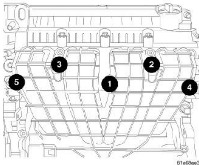
Fig. 37: INTAKE TORQUE SEQUENCE Courtesy of CHRYSLER LLC
