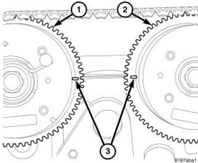
Fig. 323: Camshaft Timing Courtesy of CHRYSLER LLC
