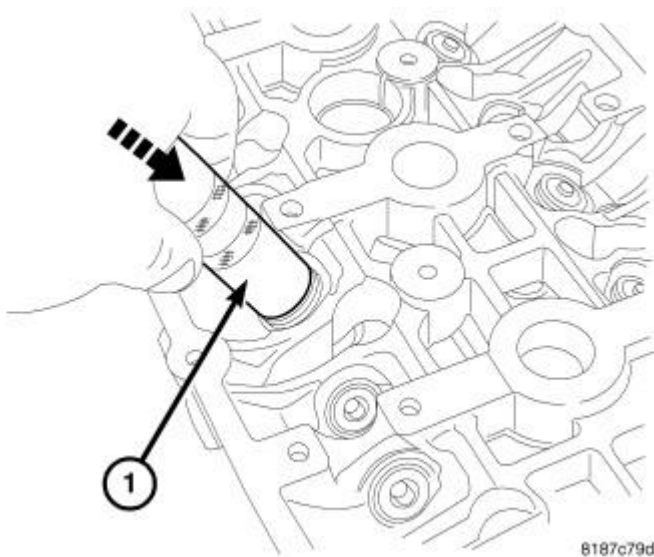
Fig. 164: VALVE REMOVAL Courtesy of CHRYSLER LLC
