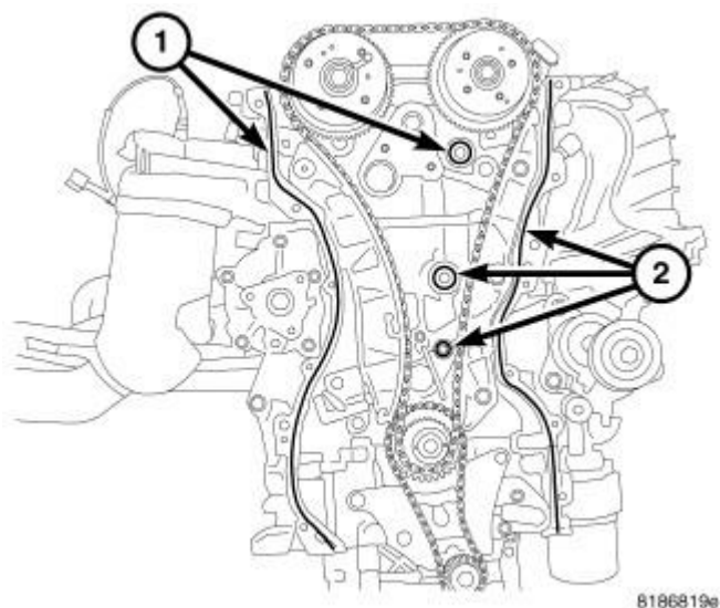
Fig. 356: TIMING CHAIN COVER SEALING Courtesy of CHRYSLER LLC
