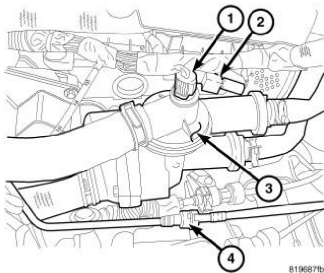
Fig. 111: COOLANT ADAPTER Courtesy of CHRYSLER LLC
