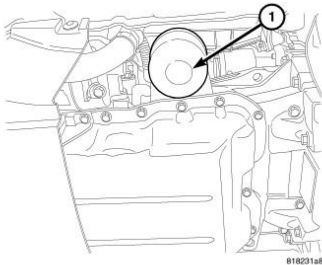
Fig. 271: OIL FILTER Courtesy of CHRYSLER LLC
