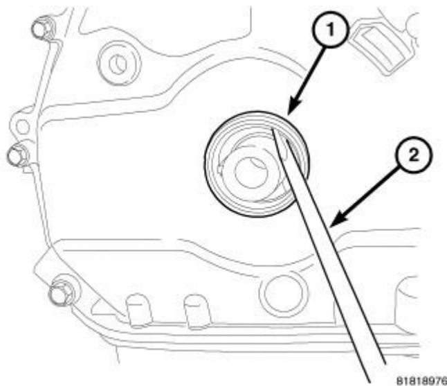
Fig. 221: FRONT CRANKSHAFT SEAL REMOVAL Courtesy of CHRYSLER LLC
