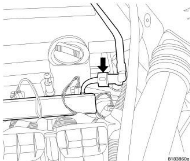
Fig. 79: FUEL LINE AT RAIL Courtesy of CHRYSLER LLC
