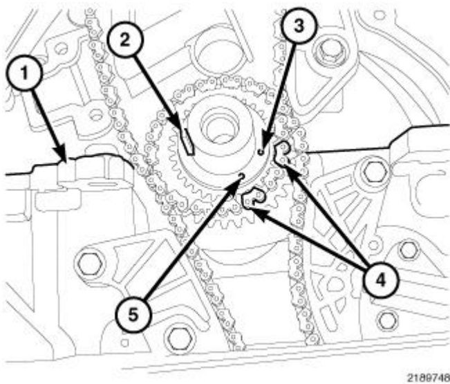
Fig. 334: Crankshaft Timing Marks Courtesy of CHRYSLER LLC
