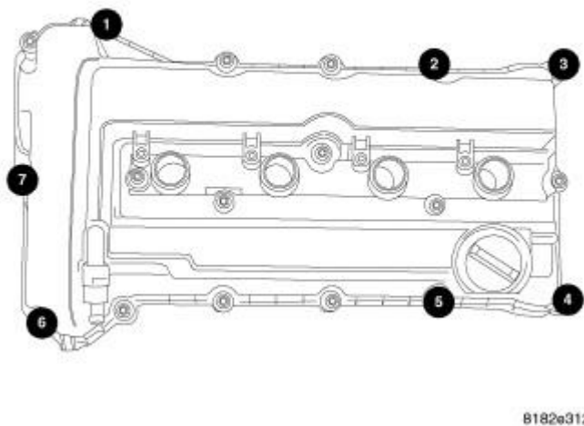
Fig. 156: STUD LOCATION Courtesy of CHRYSLER LLC
