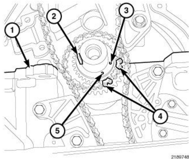
Fig. 336: Crankshaft Timing Marks Courtesy of CHRYSLER LLC
