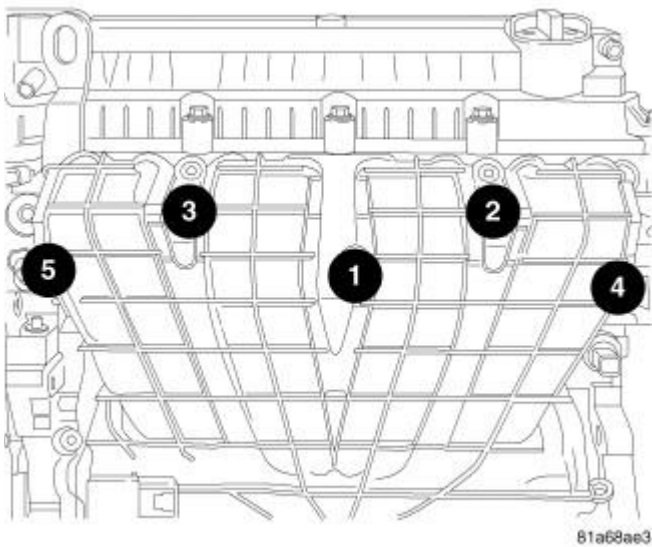
Fig. 317: Removing/Installing Intake Bolts - Torque Sequence Courtesy of CHRYSLER LLC
