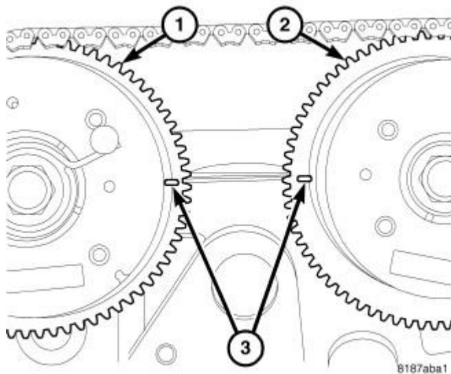
Fig. 102: Camshaft Timing Courtesy of CHRYSLER LLC
