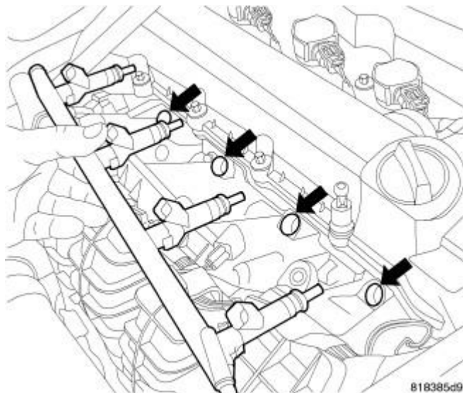
Fig. 81: RAIL REMOVAL/INSTALL Courtesy of CHRYSLER LLC
