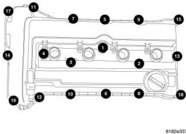
Fig. 365: Cylinder Head Cover Bolt Torque Sequence Courtesy of CHRYSLER LLC
