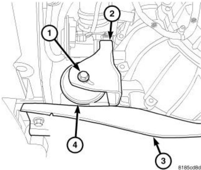
Fig. 230: FRONT MOUNT THROUGH BOLT Courtesy of CHRYSLER LLC
