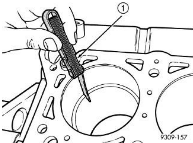
Fig. 208: Check Gap on Piston Rings Courtesy of CHRYSLER LLC
