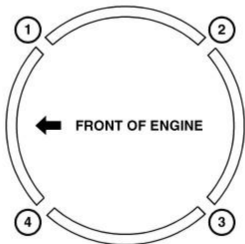
Fig. 218: Piston Ring End Gap Position Courtesy of CHRYSLER LLC
