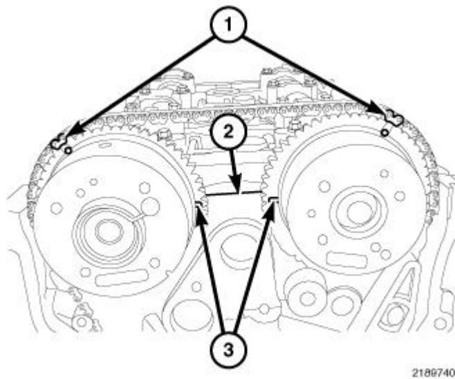
Fig. 335: Timing Chain Timing Marks Courtesy of CHRYSLER LLC
