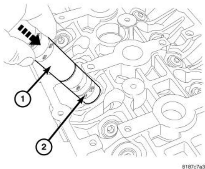
Fig. 168: VALVE INSTALLATION Courtesy of CHRYSLER LLC
