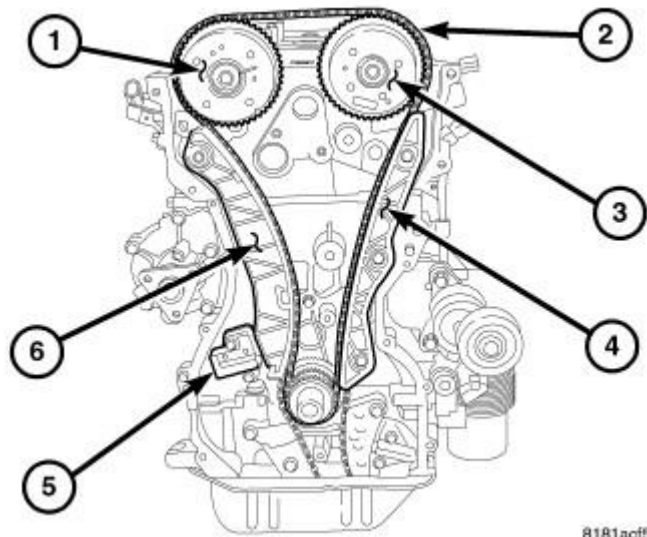
Fig. 326: Timing Drive
