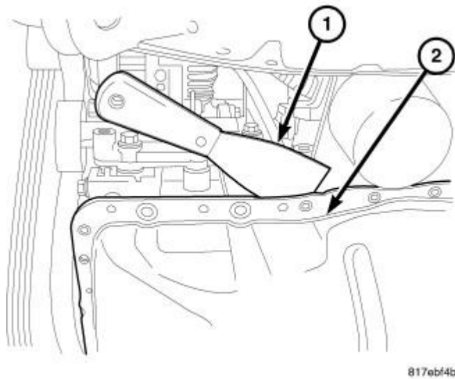
Fig. 183: OIL PAN REMOVAL Courtesy of CHRYSLER LLC
