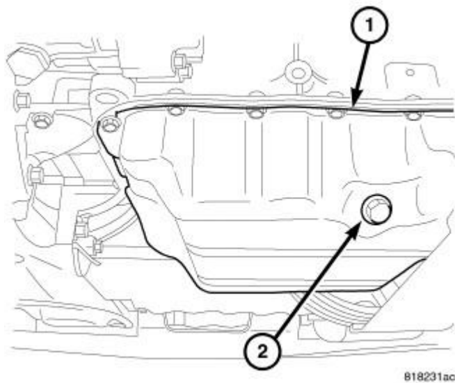
Fig. 274: OIL DRAIN PLUG Courtesy of CHRYSLER LLC
