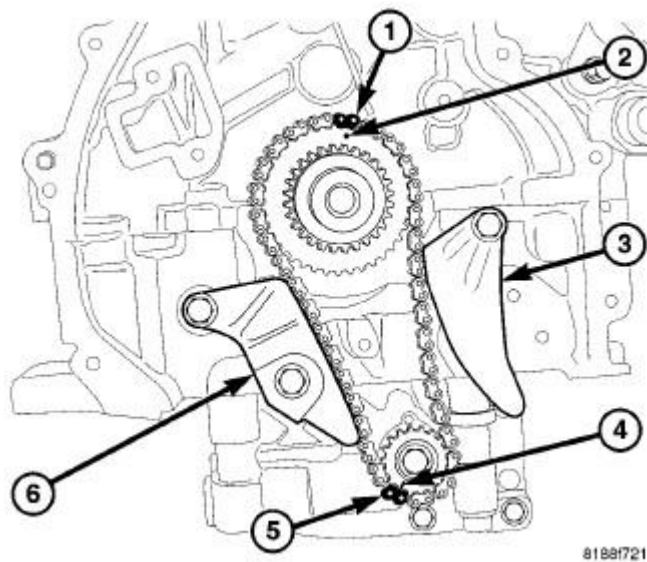
Fig. 290: BSM TIMING Courtesy of CHRYSLER LLC
