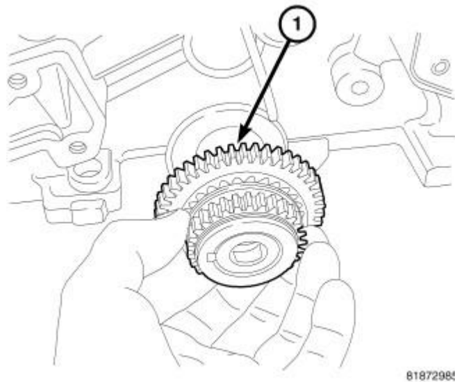
Fig. 184: CRANKSHAFT SPROCKET Courtesy of CHRYSLER LLC
