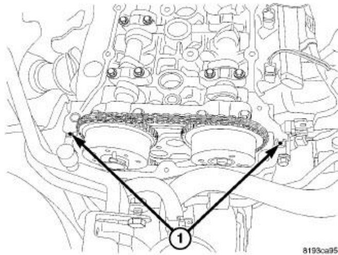
Fig. 157: Applying RTV To Cylinder Head/Front Cover T-Joint Courtesy of CHRYSLER LLC
