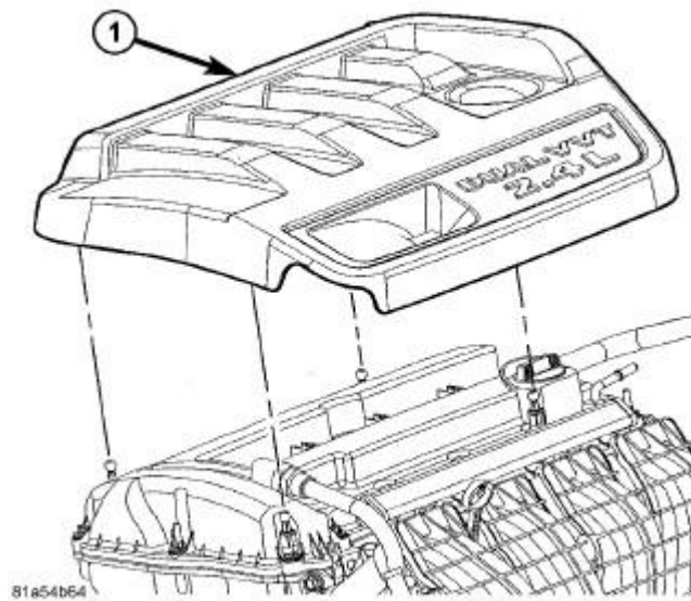
Fig. 370: Engine Cover Courtesy of CHRYSLER LLC
