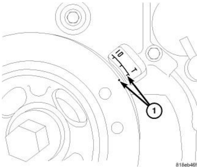
Fig. 161: TDC Courtesy of CHRYSLER LLC
