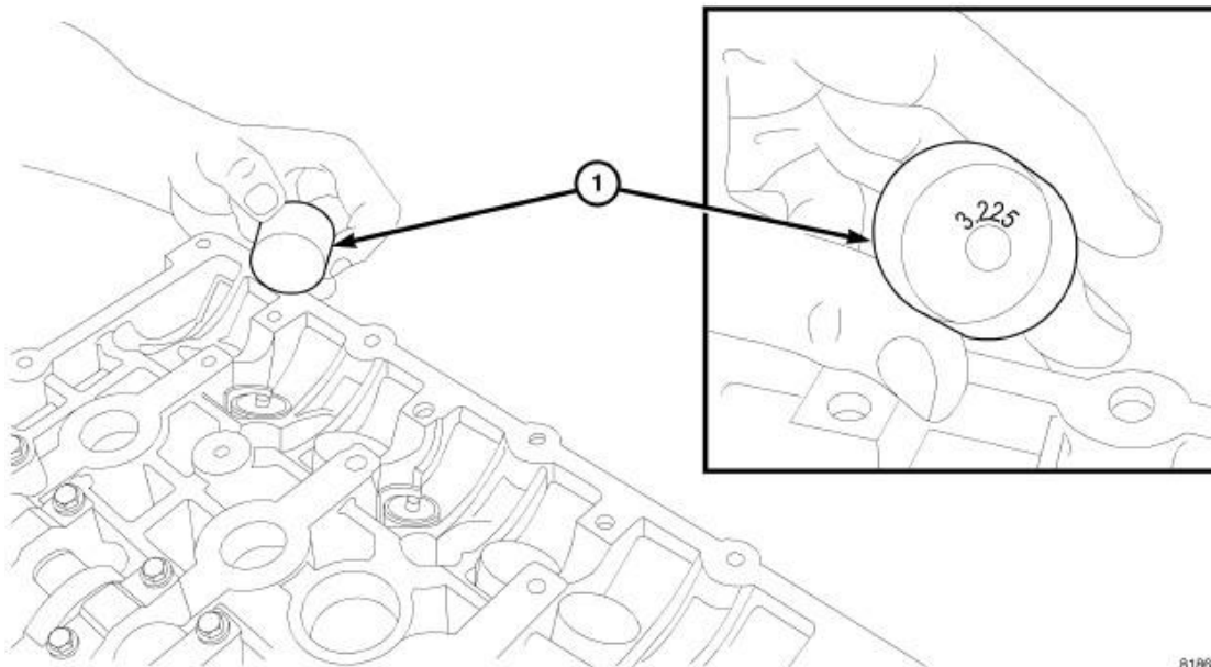
Fig. 119: TAPPET IDENTIFICATION Courtesy of CHRYSLER LLC
