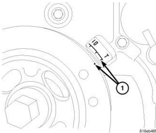
Fig. 343: TDC Courtesy of CHRYSLER LLC
