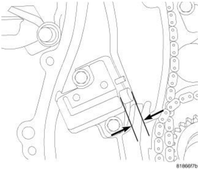
Fig. 328: Measuring Distance From Tensioner Body & Edge Of Chain Guide Courtesy of CHRYSLER LLC
