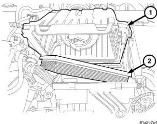
Fig. 59: AIR FILTER ELEMENT Courtesy of CHRYSLER LLC
