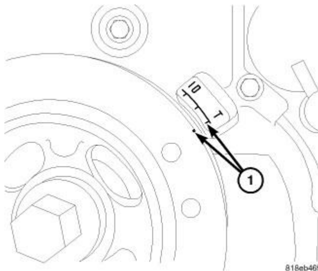
Fig. 128: TDC Courtesy of CHRYSLER LLC
