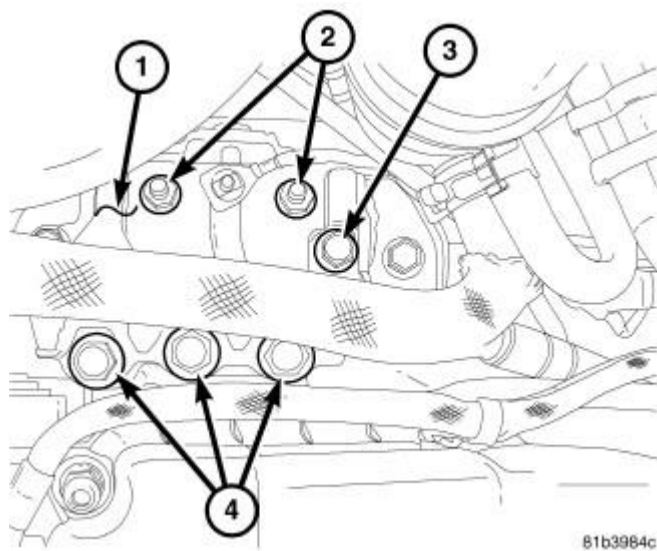
Fig. 65: Right Engine Mount Bracket & Retaining Bolts Courtesy of CHRYSLER LLC
