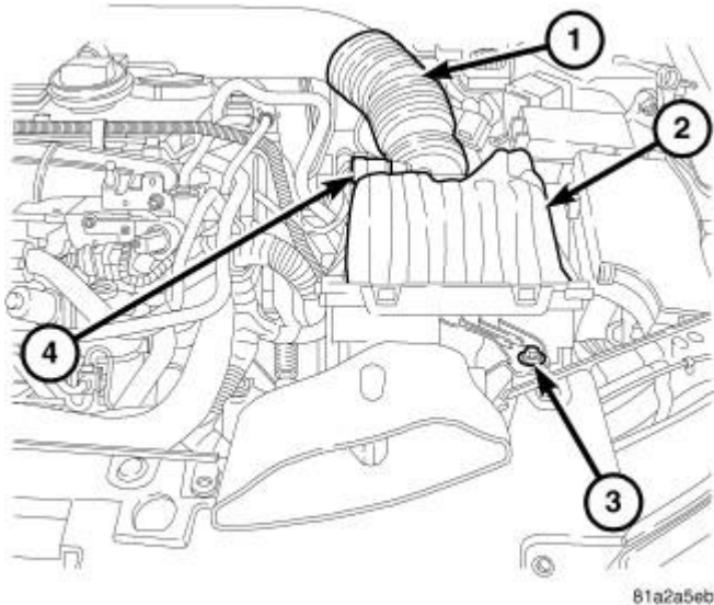
Fig. 113: Air Cleaner Housing & Retaining Bolt Courtesy of CHRYSLER LLC
