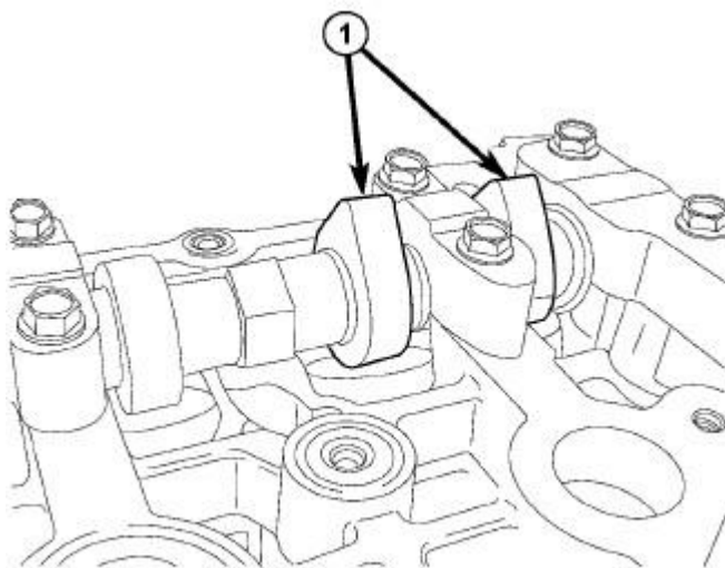
Fig. 118: LOBES VERTICAL Courtesy of CHRYSLER LLC
