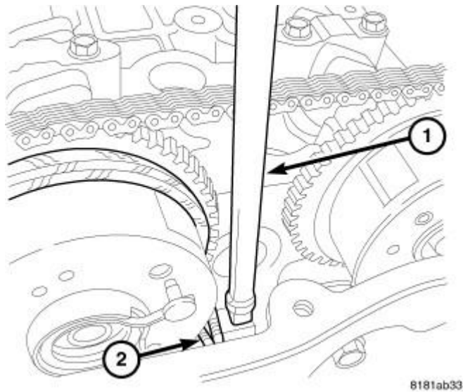
Fig. 133: SEATING WEDGE TOOL
