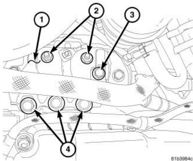
Fig. 24: Right Engine Mount Bracket & Retaining Bolts Courtesy of CHRYSLER LLC
