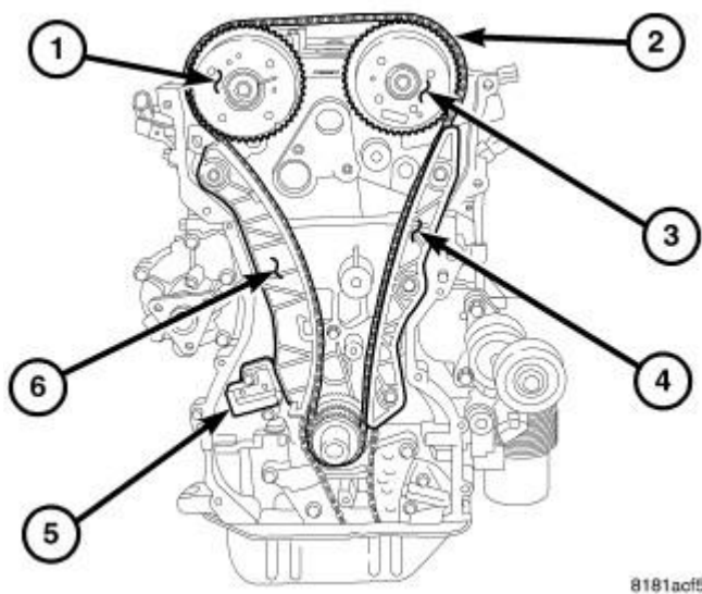
Fig. 371: TIMING DRIVE Courtesy of CHRYSLER LLC
