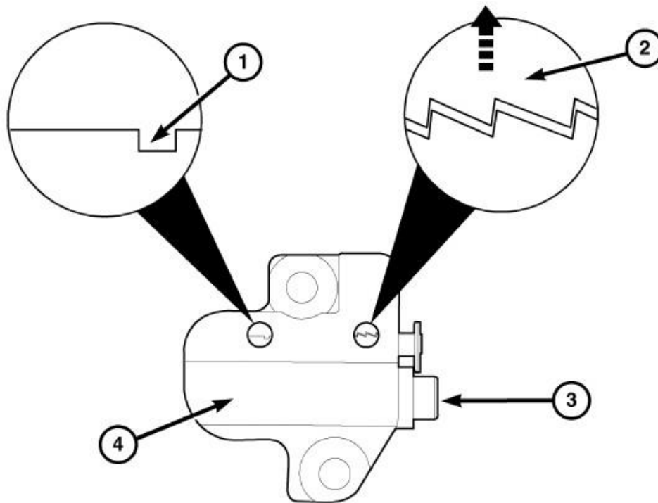
Fig. 372: TENSIONER RESET Courtesy of CHRYSLER LLC
