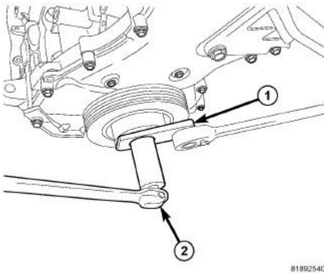
Fig. 200: DAMPER REMOVAL Courtesy of CHRYSLER LLC
