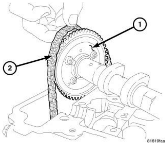
Fig. 137: CHAIN REMOVAL Courtesy of CHRYSLER LLC
