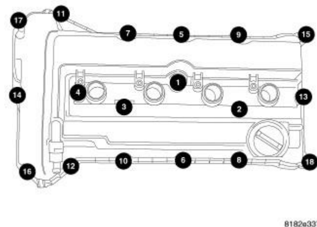
Fig. 158: Remove/Install Cylinder Head Cover Bolts In Sequence
