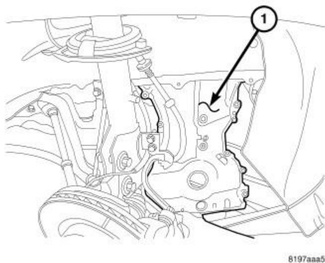
Fig. 357: TIMING CHAIN COVER REMOVAL Courtesy of CHRYSLER LLC
