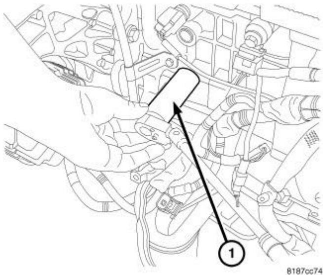
Fig. 297: OIL SENDER Courtesy of CHRYSLER LLC
