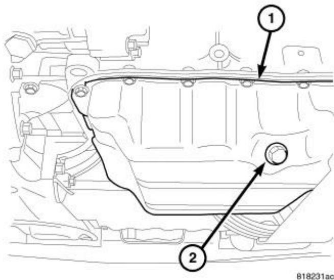
Fig. 18: OIL DRAIN PLUG Courtesy of CHRYSLER LLC
