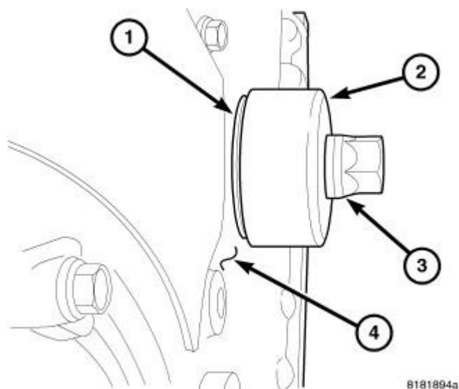
Fig. 223: INSTALLING FRONT SEAL Courtesy of CHRYSLER LLC
