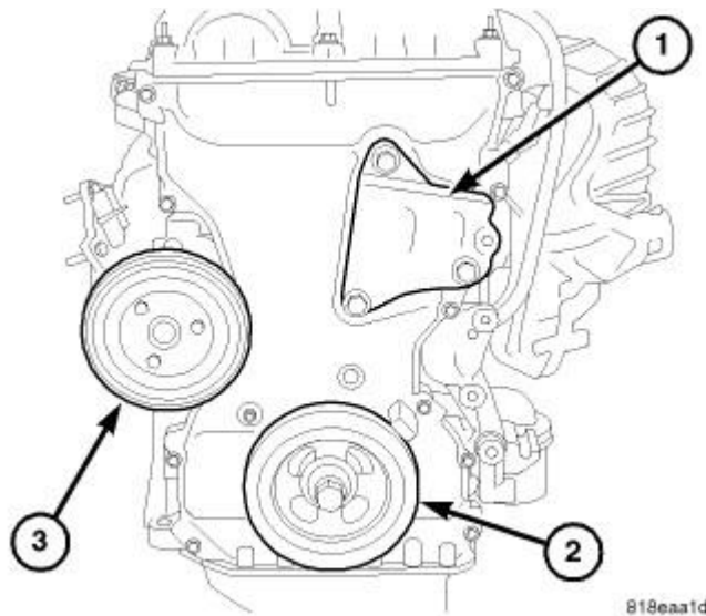
Fig. 358: RIGHT ENGINE MOUNT BRACKET Courtesy of CHRYSLER LLC
