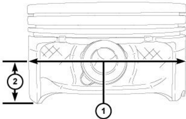
Fig. 213: Piston Pin Measurements
