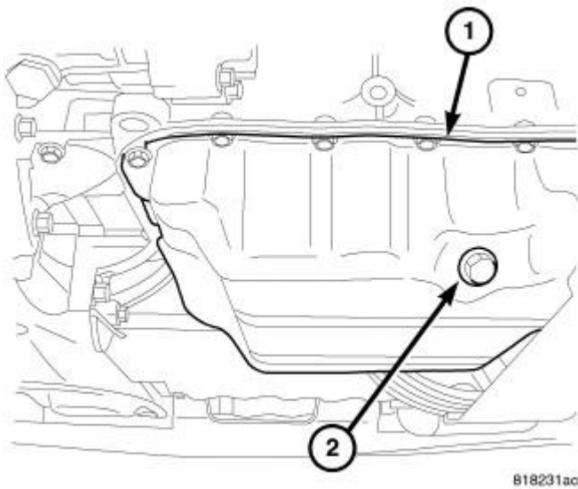
Fig. 215: Oil Drain Plug
