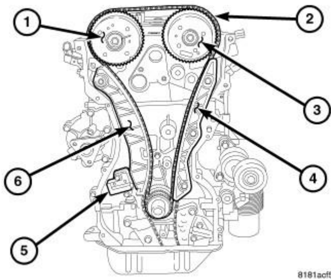
Fig. 78: TIMING DRIVE Courtesy of CHRYSLER LLC
