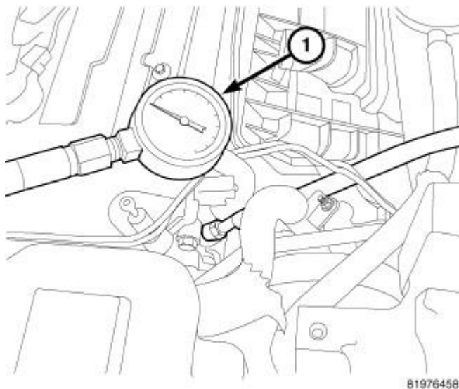
Fig. 244: OIL PSI GAUGE
