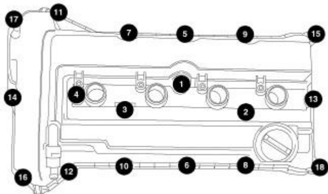
Fig. 121: Cylinder Head Cover Bolt Torque Sequence
