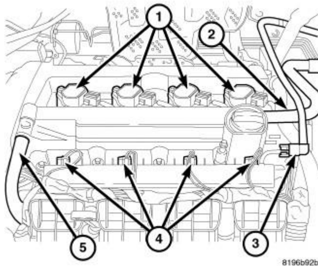
Fig. 153: COIL CONNECTOR Courtesy of CHRYSLER LLC
