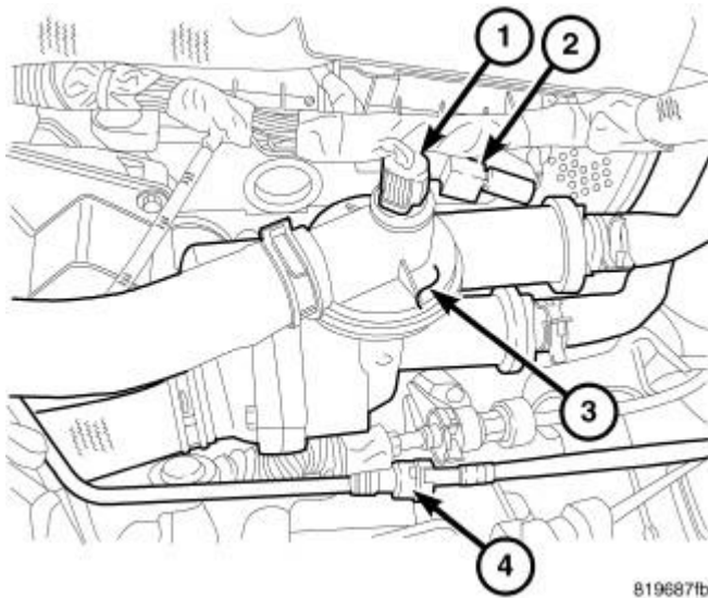
Fig. 85: COOLANT ADAPTER Courtesy of CHRYSLER LLC
