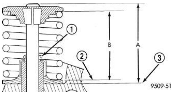
Fig. 169: Checking Spring Installed Height and Valve Tip Height Dimensions Courtesy of CHRYSLER LLC
