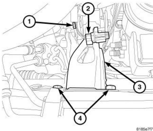
Fig. 235: REAR MOUNT-ATX Courtesy of CHRYSLER LLC
