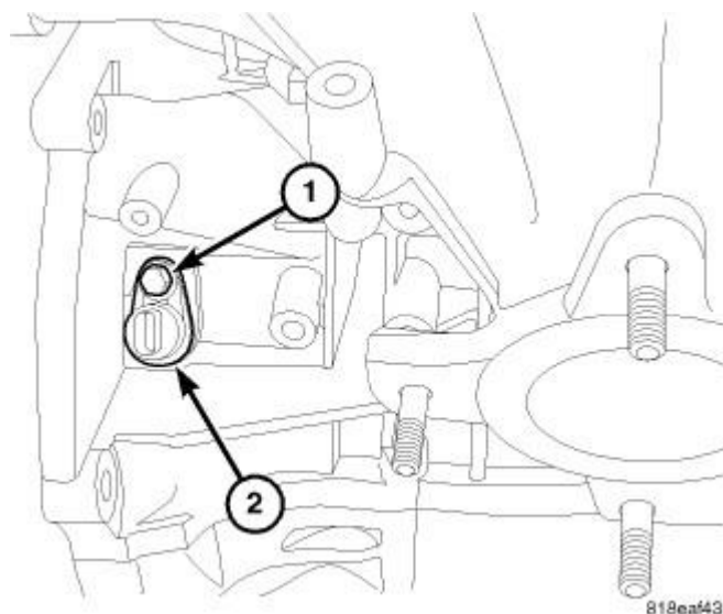
Fig. 195: CRANKSHAFT POSITION SENSOR Courtesy of CHRYSLER LLC
