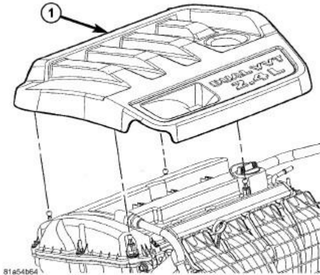
Fig. 62: Engine Cover Courtesy of CHRYSLER LLC
