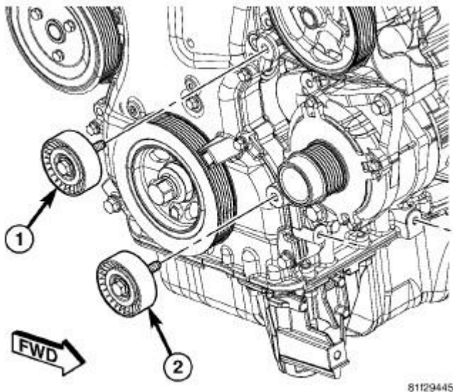
Fig. 359: Removing/Installing Accessory Drive Belt Lower Idler Pulley Courtesy of CHRYSLER LLC
