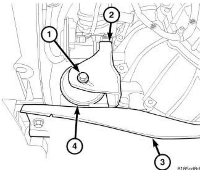
Fig. 231: FRONT MOUNT THROUGH BOLT Courtesy of CHRYSLER LLC
