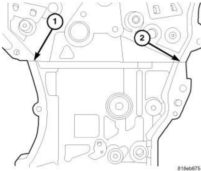
Fig. 353: FRONT COVER UPPER T-JOINT Courtesy of CHRYSLER LLC
