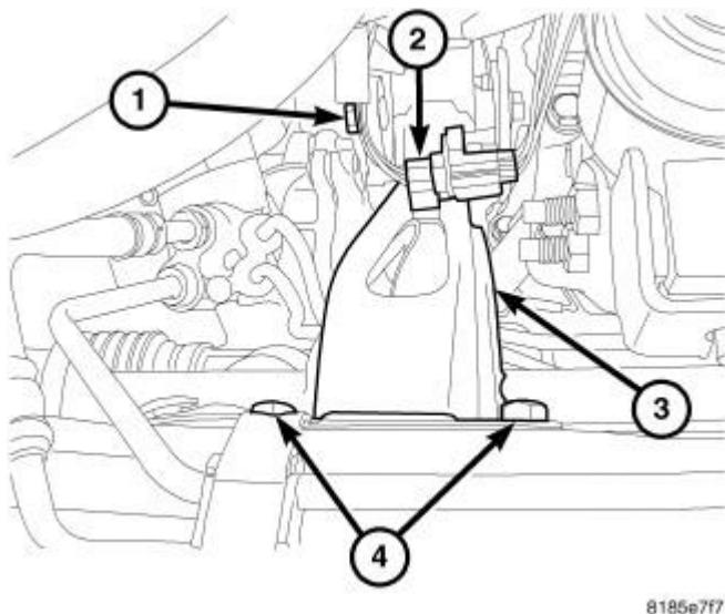
Fig. 234: REAR MOUNT-ATX Courtesy of CHRYSLER LLC
