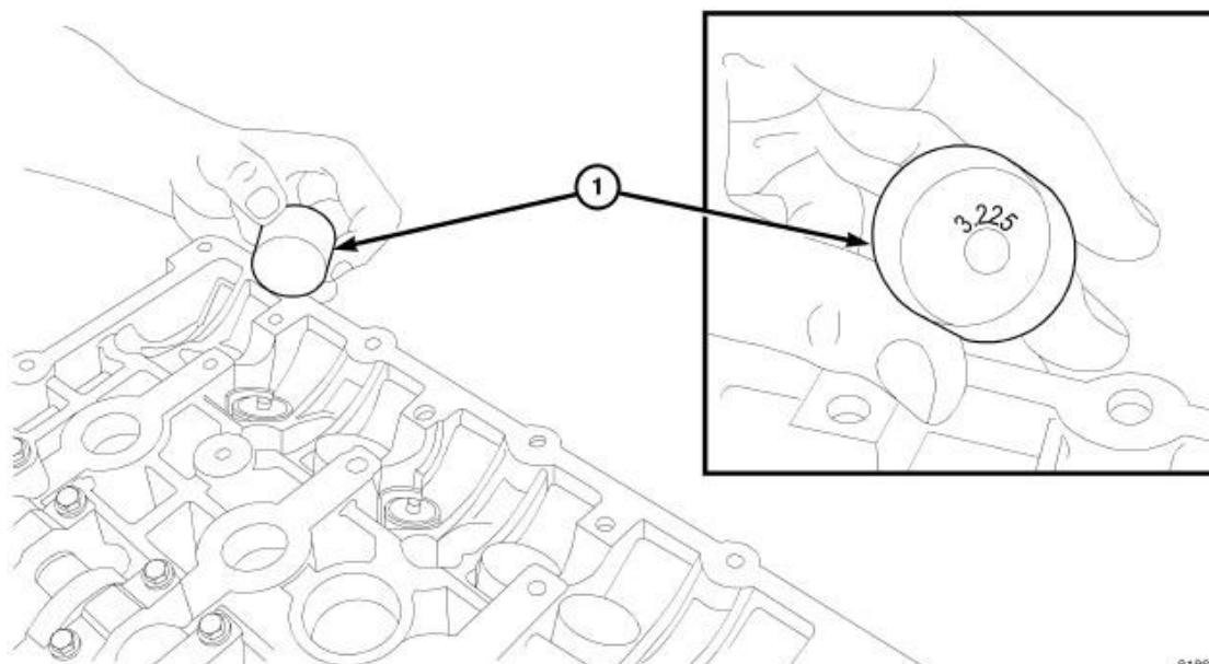
Fig. 120: TAPPET IDENTIFICATION
