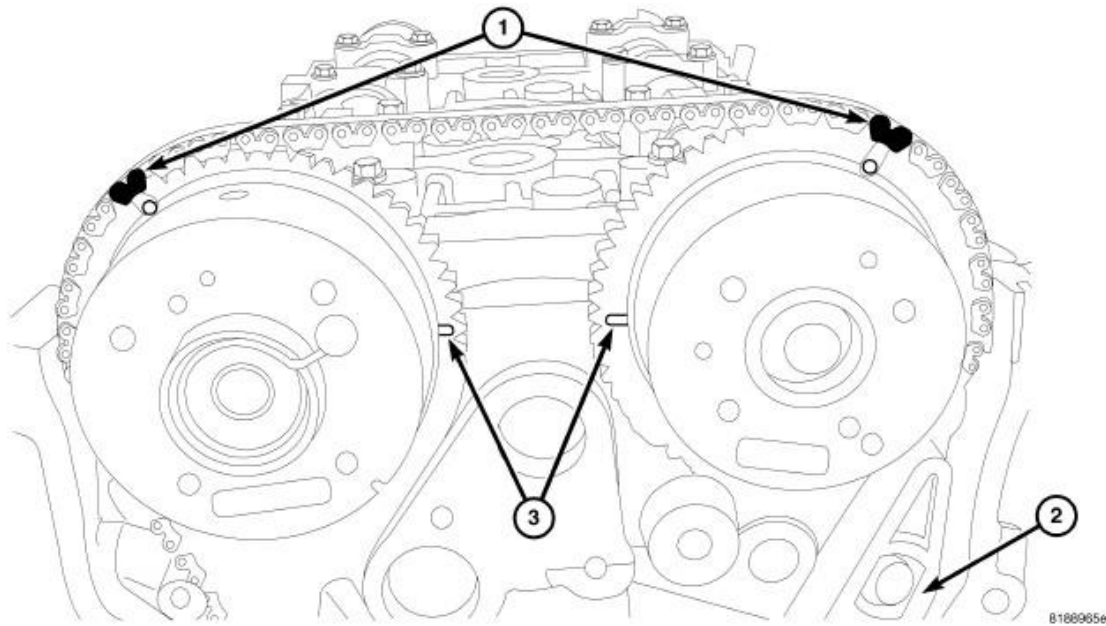
Fig. 145: TIMING CHAIN TIMING MARKS Courtesy of CHRYSLER LLC
