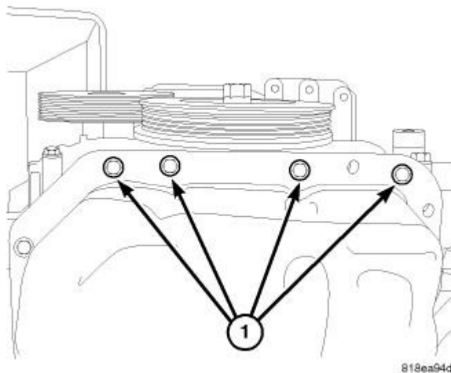
Fig. 361: TIMING CHAIN COVER LOWER BOLTS Courtesy of CHRYSLER LLC
