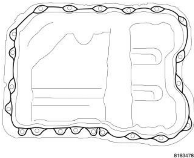
Fig. 278: SEALING OIL PAN Courtesy of CHRYSLER LLC
