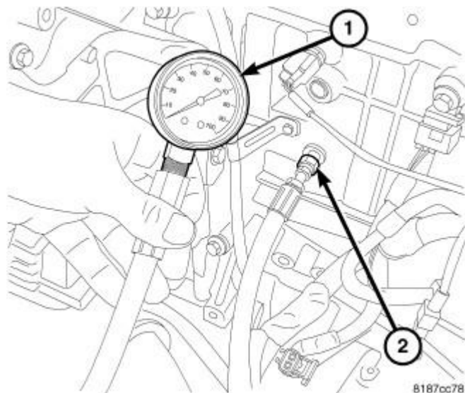
Fig. 248: OIL PRESSURE GAUGE
