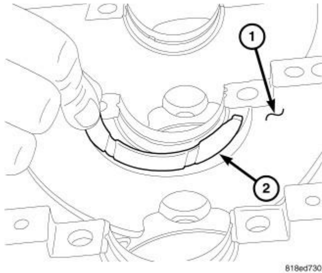
Fig. 191: INSTALLING THRUST BEARING
