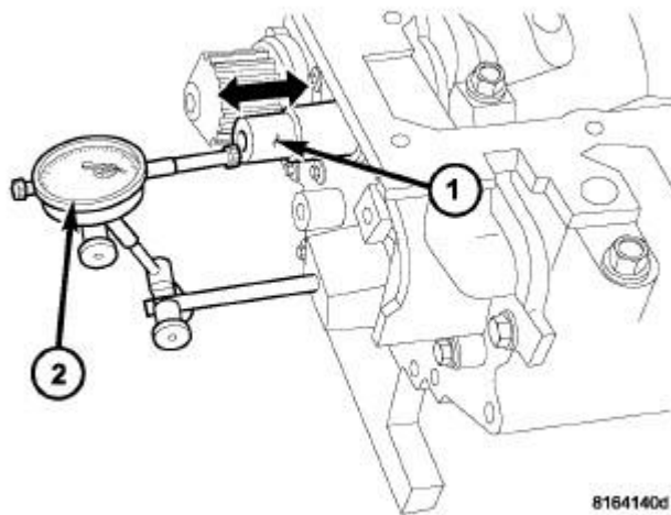
Fig. 178: Checking Crankshaft End Play- Dial Indicator Courtesy of CHRYSLER LLC
