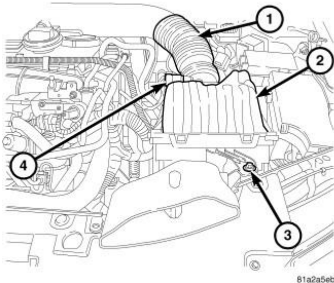
Fig. 63: Air Cleaner Housing & Retaining Bolt Courtesy of CHRYSLER LLC
