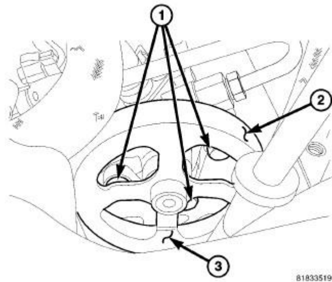
Fig. 341: POWER STEERING PUMP - GAS Courtesy of CHRYSLER LLC
