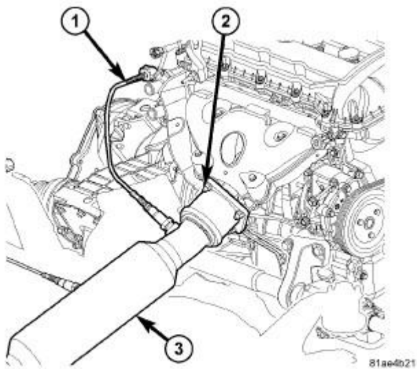
Fig. 73: CATALYTIC CONVERTER - 2.0L/2.4L Courtesy of CHRYSLER LLC
