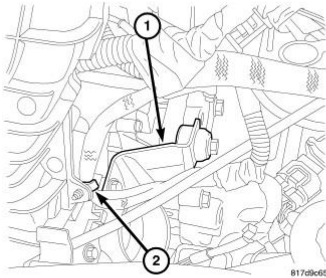
Fig. 83: Throttle Body Support Bracket Courtesy of CHRYSLER LLC
