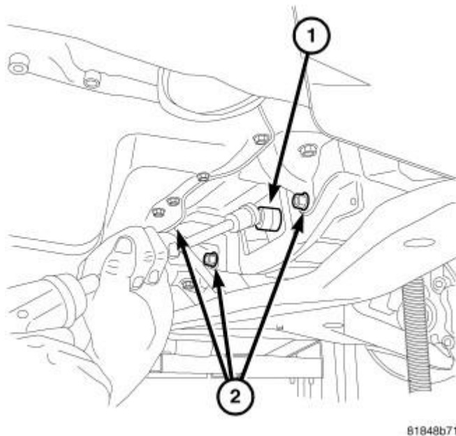
Fig. 33: MODULAR CLUTCH TO FLEX PLATE BOLTS Courtesy of CHRYSLER LLC
