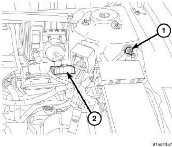
Fig. 43: BATTERY CABLE Courtesy of CHRYSLER LLC
