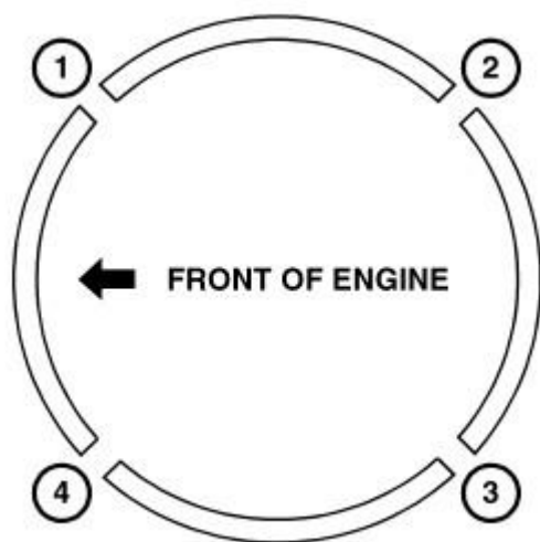
Fig. 212: PISTON RING END GAP POSITION Courtesy of CHRYSLER LLC
