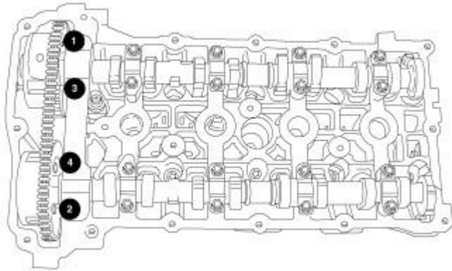
Fig. 87: FRONT CAM CAP REMOVAL SEQUENCE
