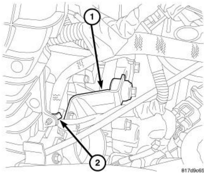
Fig. 38: THROTTLE BODY SUPPORT
