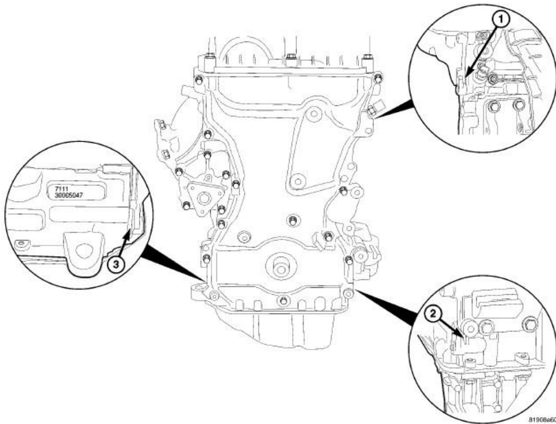
Fig. 77: TIMING CHAIN COVER PRY POINTS Courtesy of CHRYSLER LLC
