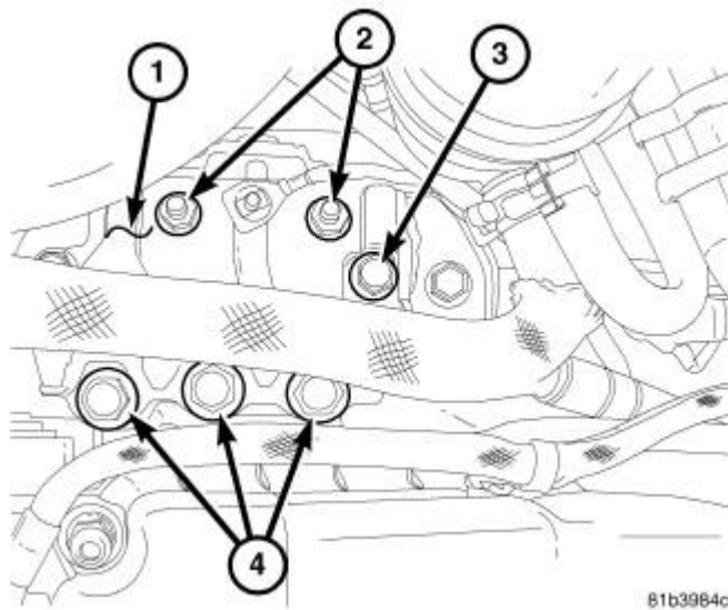
Fig. 367: Right Engine Mount Bracket & Retaining Bolts Courtesy of CHRYSLER LLC
