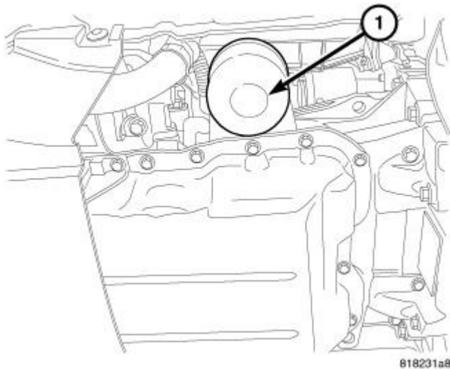
Fig. 35: OIL FILTER Courtesy of CHRYSLER LLC
