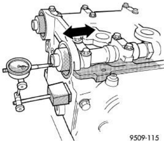
Fig. 126: Camshaft End Play Courtesy of CHRYSLER LLC
