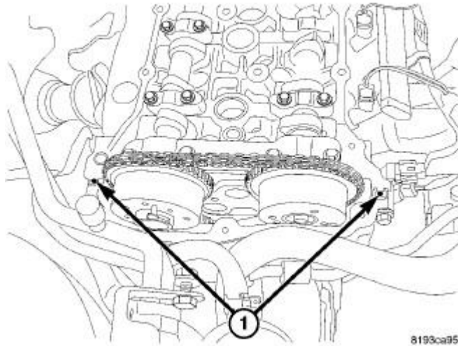
Fig. 149: Cylinder Head/Front Cover T-Joints Courtesy of CHRYSLER GROUP, LLC
