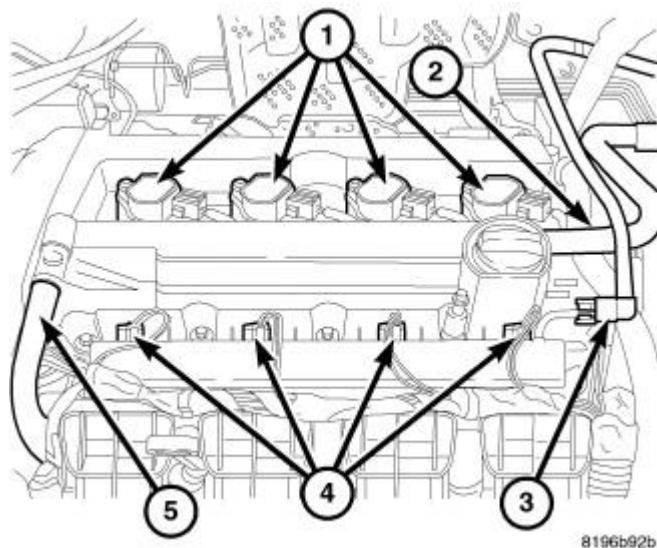
Fig. 17: Ignition Coils, Air Hose, Fuel Line, Injectors & PCV Hose Courtesy of CHRYSLER GROUP, LLC
