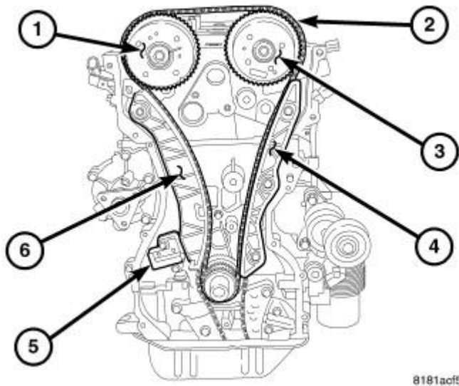
Fig. 342: Timing Drive System Courtesy of CHRYSLER GROUP, LLC
