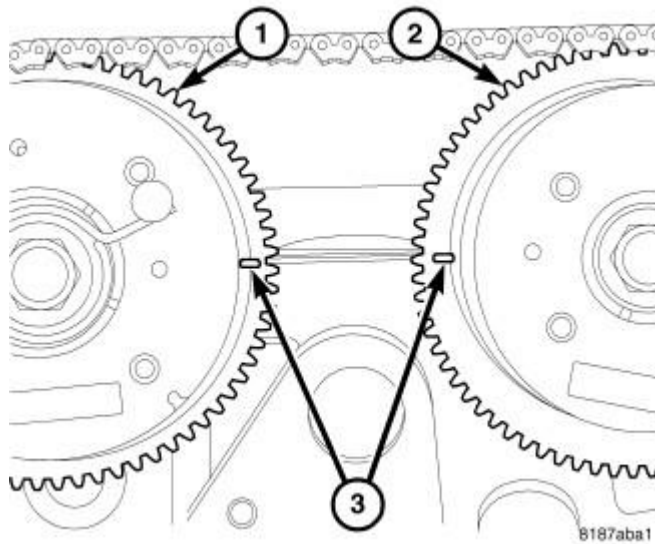
Fig. 94: Camshaft Timing Marks
