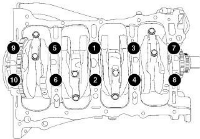
Fig. 184: Main Bearing Cap Removal/Installation Sequence Courtesy of CHRYSLER GROUP, LLC
