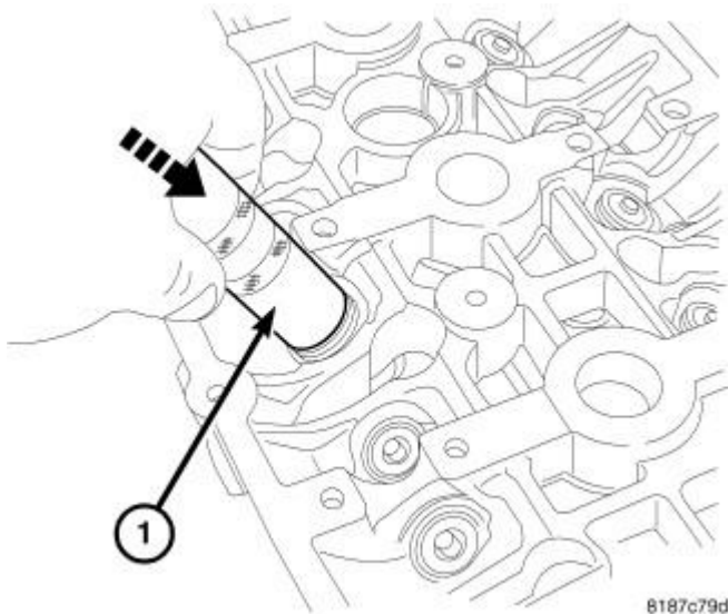
Fig. 153: Valve Removal
