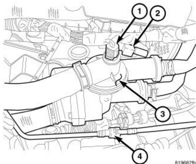
Fig. 16: Coolant Temperature Sensor Connector, Capacitor Connector & Coolant Adapter Courtesy of CHRYSLER GROUP, LLC
