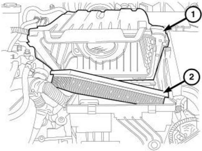
Fig. 50: Air Cleaner Housing Cover & Air Filter Element
