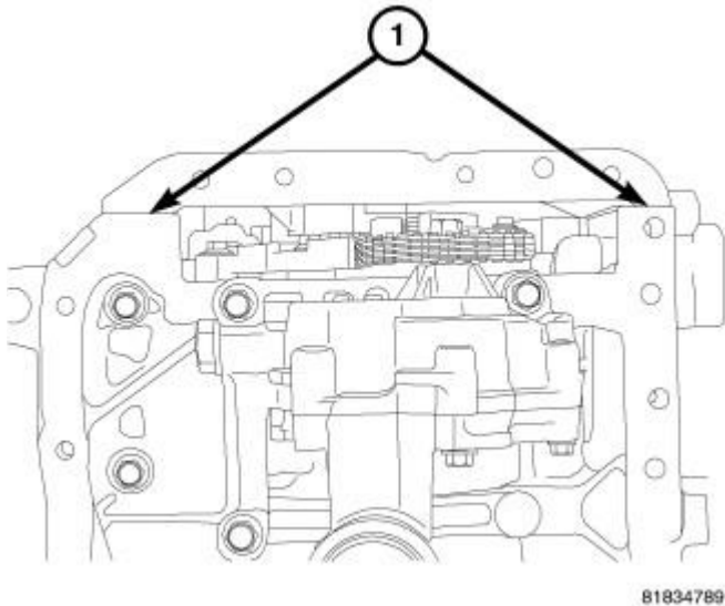
Fig. 287: Sealer Location
