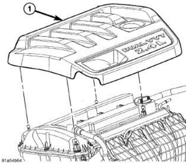
Fig. 10: Engine Cover - 2.4L Courtesy of CHRYSLER GROUP, LLC
