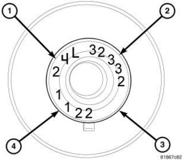
Fig. 166: Bearing Selection
