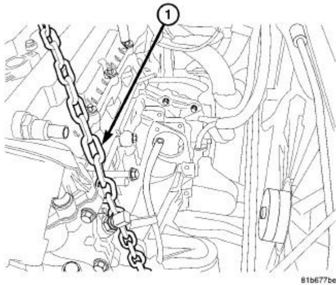
Fig. 214: Lift Chain
