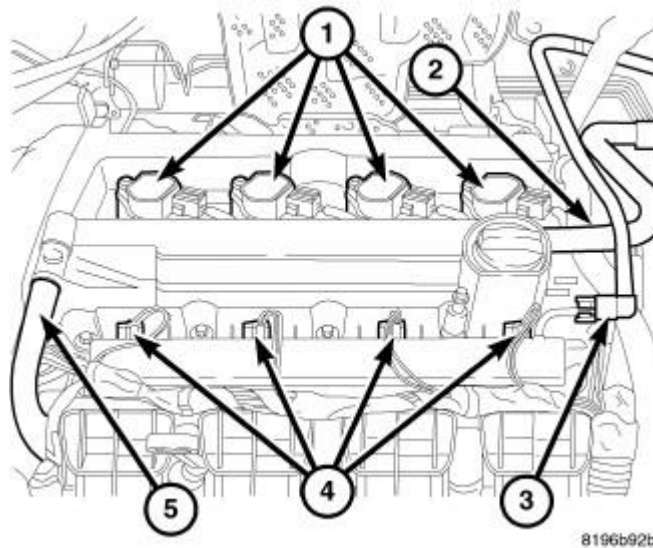
Fig. 11: Ignition Coils, Air Hose, Fuel Line, Injectors & PCV Hose Courtesy of CHRYSLER GROUP, LLC
