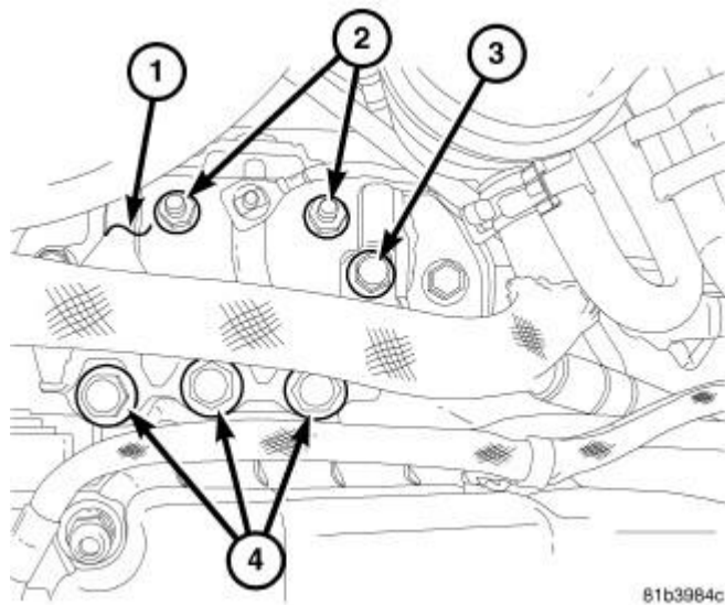
Fig. 384: Power Steering Hose Hold Down, Right Engine Mount Bracket & Fasteners Courtesy of CHRYSLER GROUP, LLC
