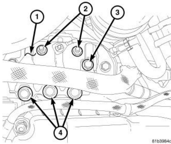
Fig. 365: Power Steering Hose Hold Down, Right Engine Mount Bracket & Fasteners Courtesy of CHRYSLER GROUP, LLC
