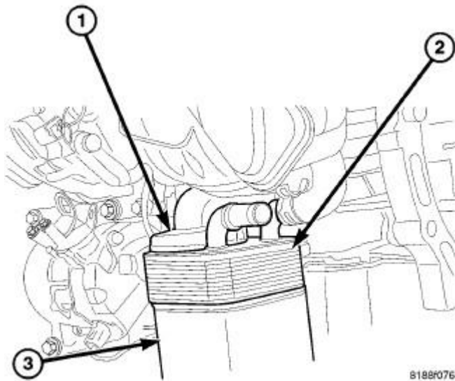
Fig. 272: Oil Cooler Housing, Oil Cooler & Oil Filter Courtesy of CHRYSLER GROUP, LLC
