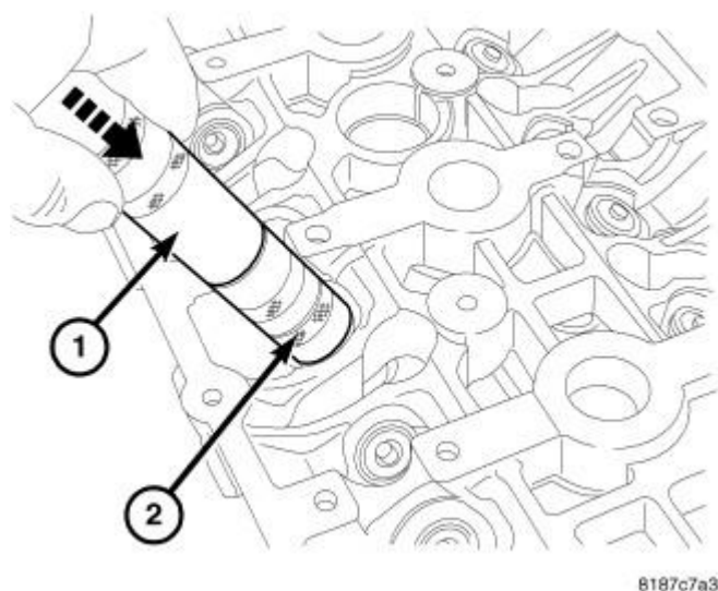
Fig. 156: Valve Installation
