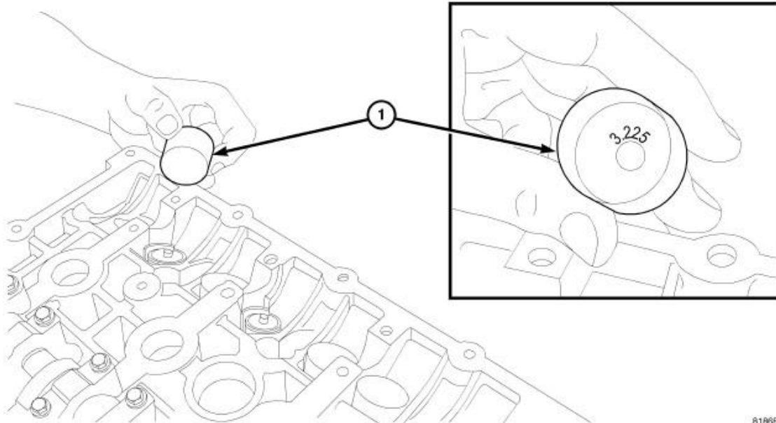
Fig. 114: Tappet Identification
