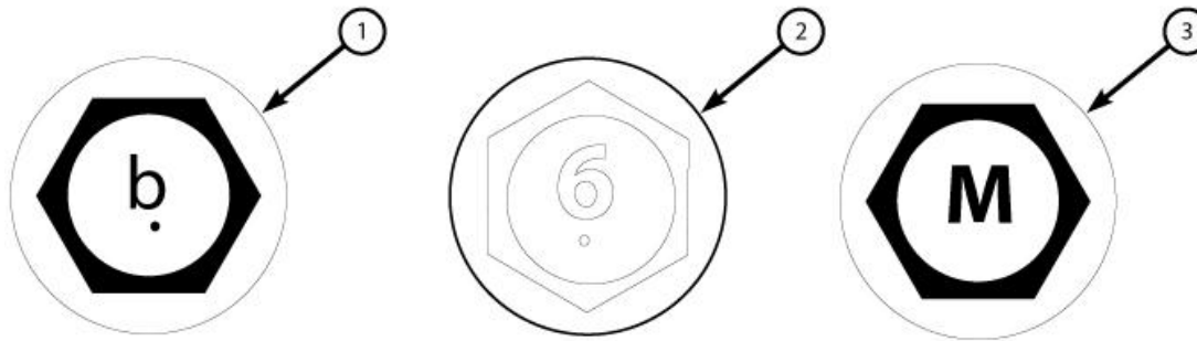
Fig. 183: Main Bolt Identification Courtesy of CHRYSLER GROUP, LLC
