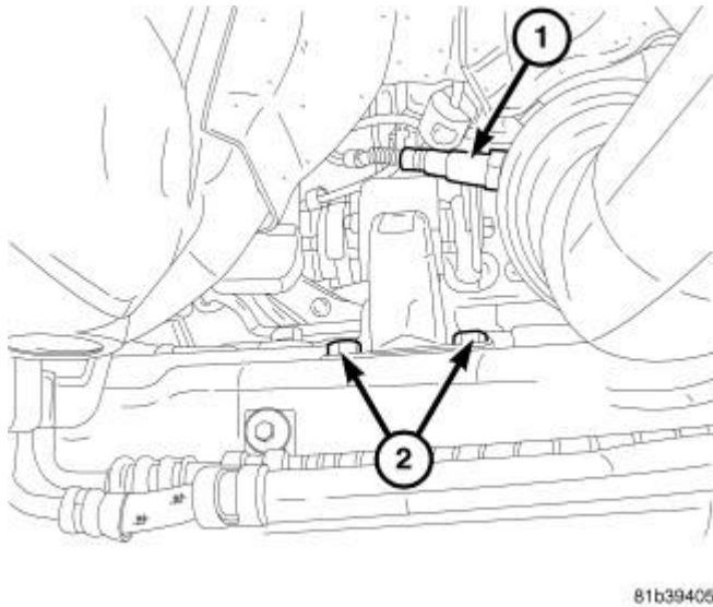
Fig. 240: Oxygen Sensor & Rear Mount Retaining Bolts Courtesy of CHRYSLER GROUP, LLC
