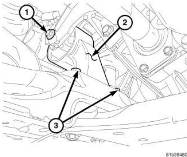
Fig. 241: Rear Engine Mount & Bolts Courtesy of CHRYSLER GROUP, LLC
