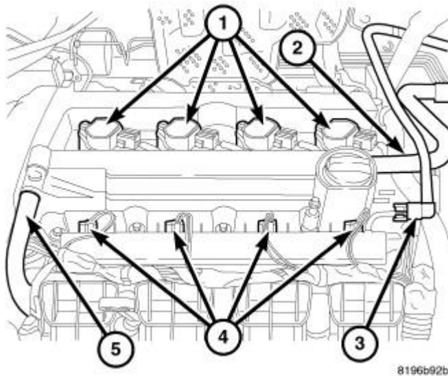
Fig. 333: Ignition Coils, Air Hose, Fuel Line, Injectors & PCV Hose Courtesy of CHRYSLER GROUP, LLC
