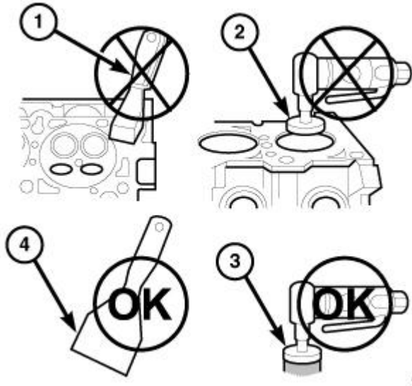
Fig. 4: Proper Tool Usage For Surface Preparation Courtesy of CHRYSLER GROUP, LLC
