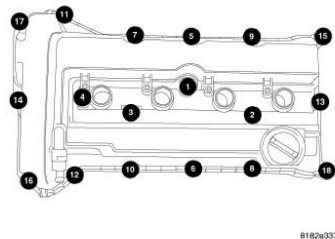
Fig. 150: Remove/Install Cylinder Head Cover Bolts In Sequence
