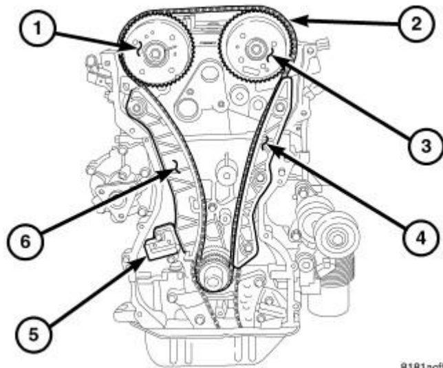
Fig. 342: Timing Drive System
