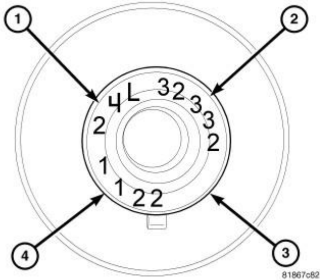
Fig. 166: Bearing Selection Courtesy of CHRYSLER LLC
