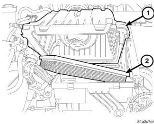
Fig. 51: Air Cleaner Housing Cover & Air Filter Element Courtesy of CHRYSLER LLC
