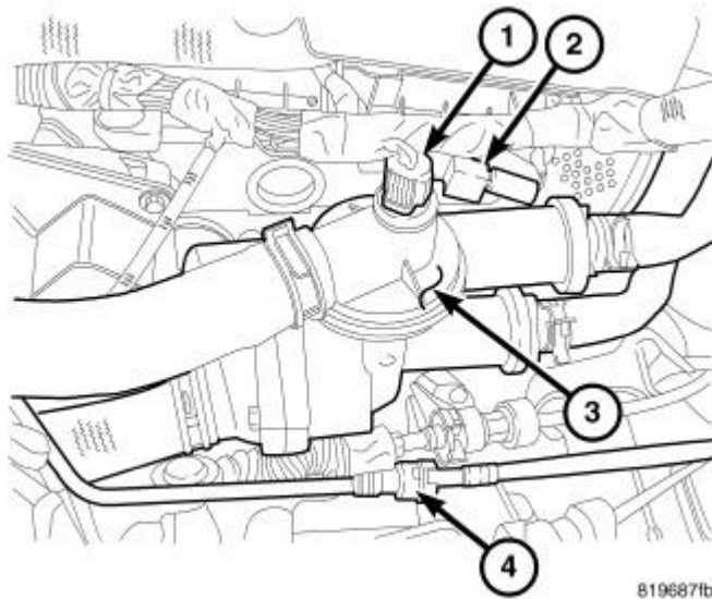
Fig. 16: Coolant Temperature Sensor Connector, Capacitor Connector & Coolant Adapter Courtesy of CHRYSLER LLC
