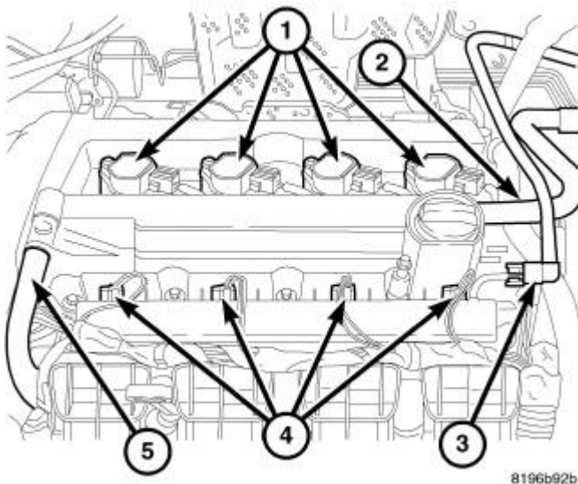
Fig. 41: Coil Connectors, Air Hose, Fuel Line, Injectors & PCV Hose Courtesy of CHRYSLER LLC
