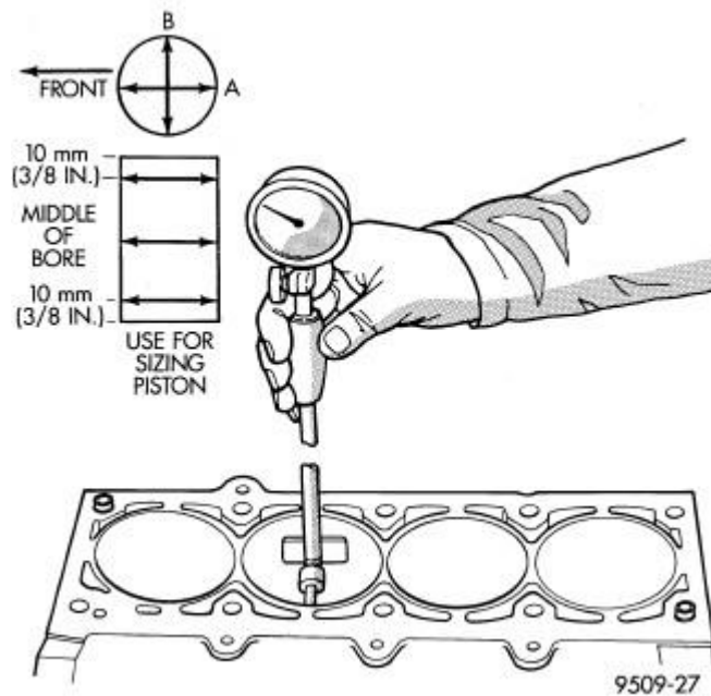
Fig. 204: Checking Cylinder Bore Size
