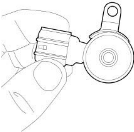
Fig. 270: Solenoid Mounting Tab 1/2 Courtesy of CHRYSLER LLC
