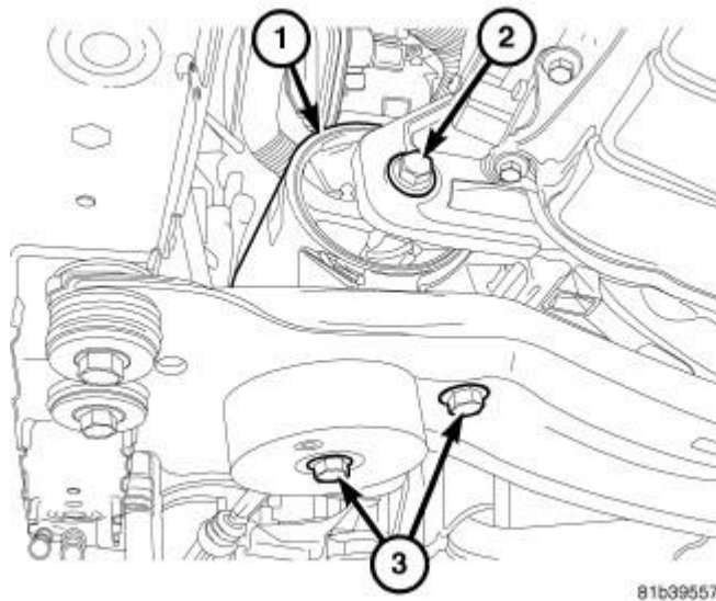
Fig. 226: Front Mount & Bolts Courtesy of CHRYSLER LLC
