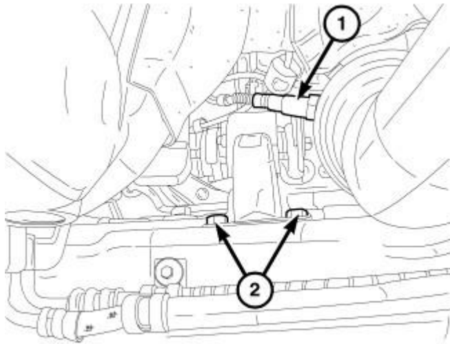
Fig. 240: Oxygen Sensor & Rear Mount Retaining Bolts Courtesy of CHRYSLER LLC
