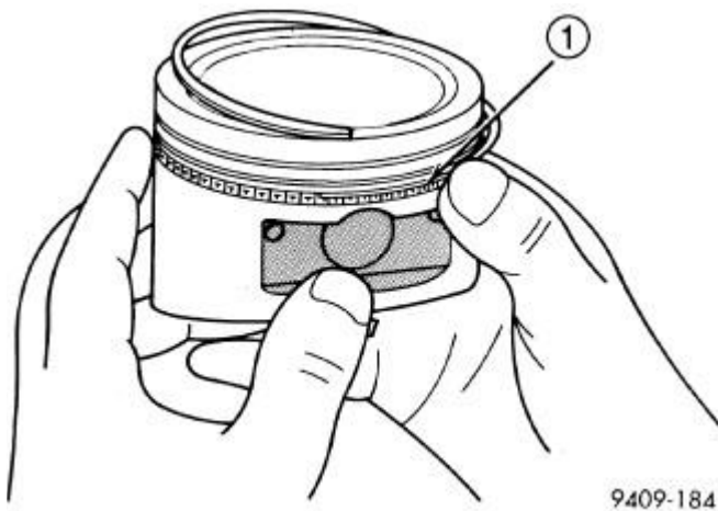
Fig. 201: Installing Side Rail Courtesy of CHRYSLER LLC
