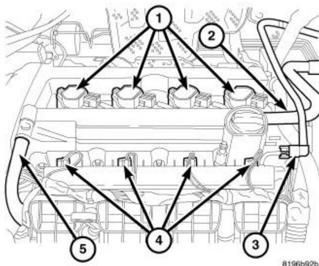
Fig. 17: Coil Connectors, Air Hose, Fuel Line, Injectors & PCV Hose Courtesy of CHRYSLER LLC
