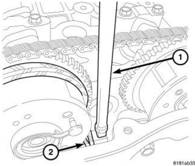
Fig. 125: Seating Wedge Tool 9701
