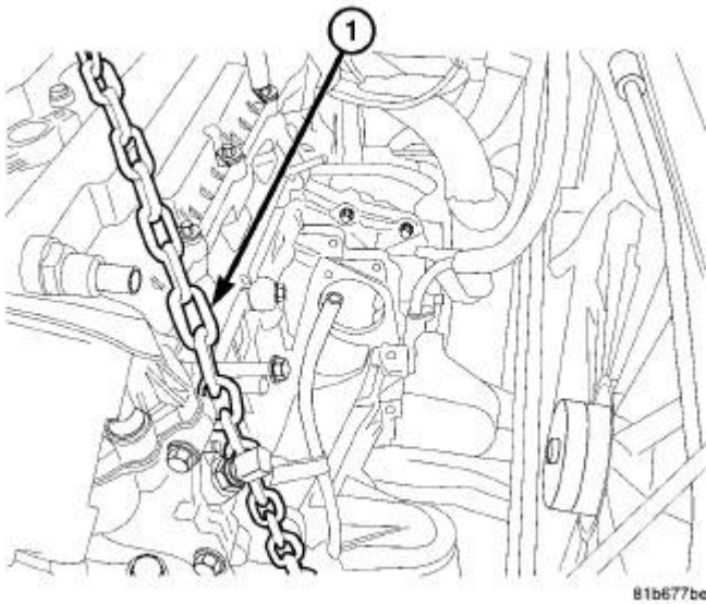
Fig. 206: Lift Chain
