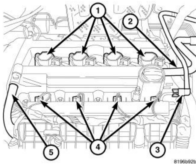
Fig. 328: Coil Connectors, Air Hose, Fuel Line, Injectors & PCV Hose Courtesy of CHRYSLER LLC
