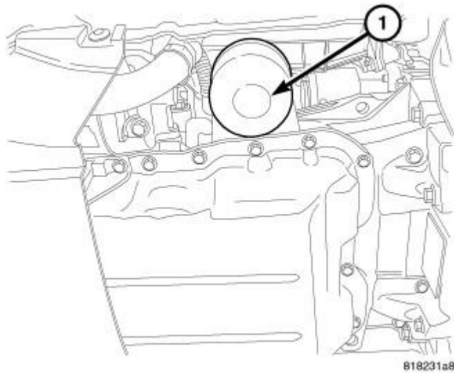
Fig. 171: Oil Filter Courtesy of CHRYSLER LLC
