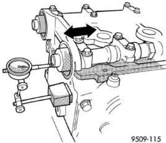
Fig. 118: Measuring Camshaft End Play Courtesy of CHRYSLER LLC
