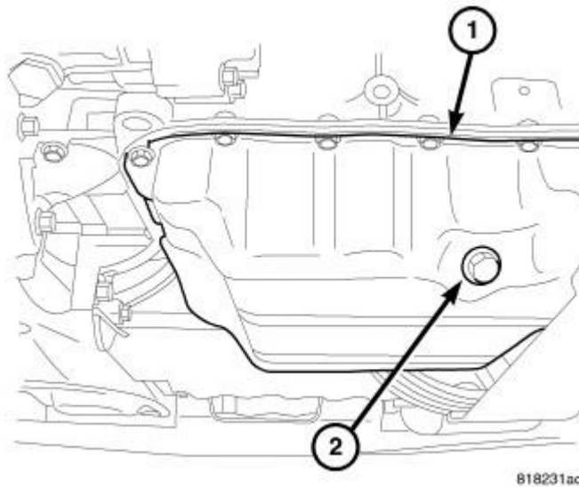
Fig. 289: Oil Drain Plug & Oil Pan Courtesy of CHRYSLER LLC
