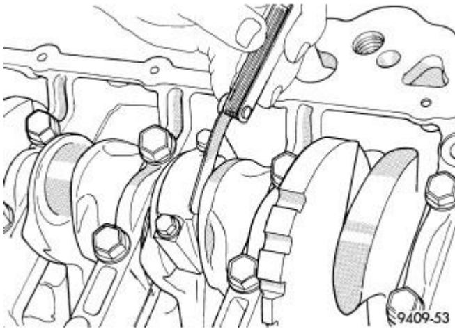
Fig. 165: Connecting Rod Side Clearance Courtesy of CHRYSLER LLC
