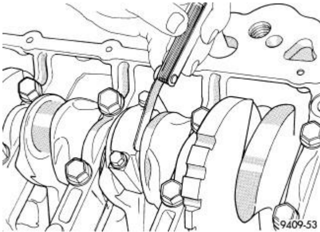
Fig. 213: Connecting Rod Side Clearance Courtesy of CHRYSLER LLC
