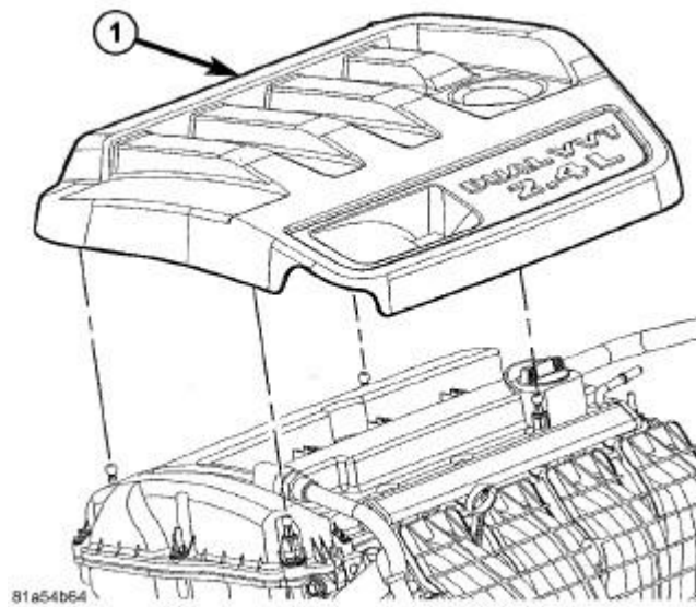
Fig. 336: Engine Cover - 2.4L Courtesy of CHRYSLER LLC
