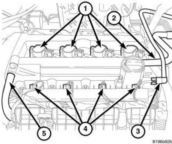
Fig. 145: Coil Connectors, Air Hose, Fuel Line, Injectors & PCV Hose Courtesy of CHRYSLER LLC
