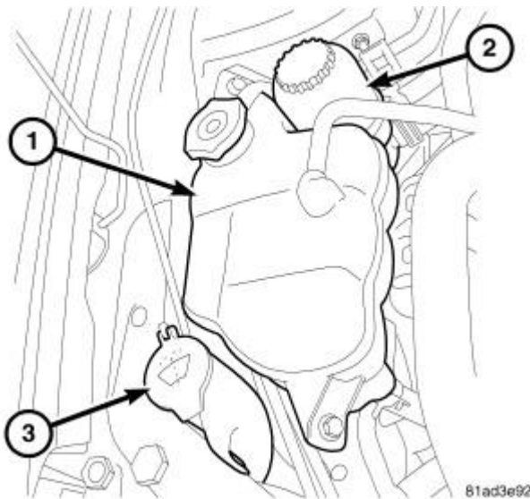
Fig. 14: Coolant Reservoir, Power Steering Reservoir & Windshield Washer Bottle Courtesy of CHRYSLER LLC
