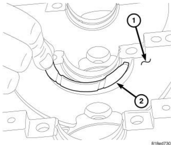
Fig. 181: Removing/Installing Thrust Bearings
