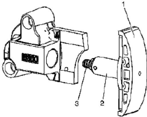
Fig. 498: Identifying Primary Timing Chain Tensioner Courtesy of SUZUKI OF AMERICA CORP.
