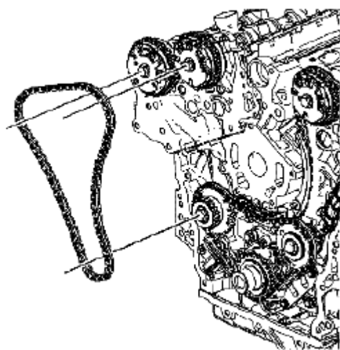
Fig. 905: Identifying Right Secondary Camshaft Drive Chain Courtesy of SUZUKI OF AMERICA CORP.
