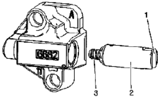
Fig. 525: Identifying Right Secondary Timing Chain Tensioner Courtesy of SUZUKI OF AMERICA CORP.
