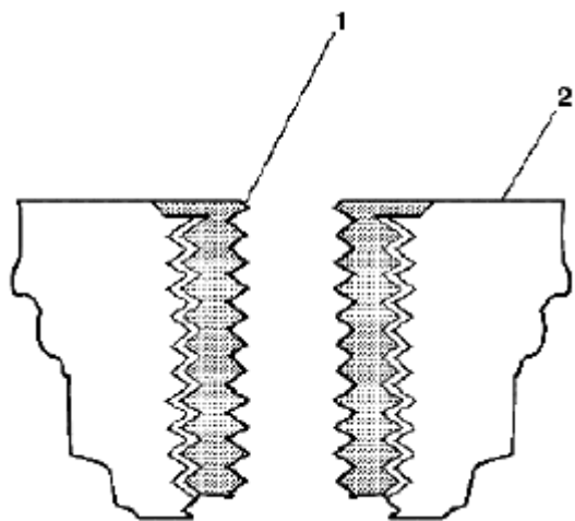
Fig. 607: Identifying Insert & Surface Of Base Material Courtesy of SUZUKI OF AMERICA CORP.
