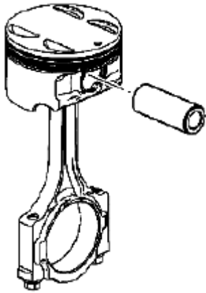
Fig. 419: Identifying Piston Pin
