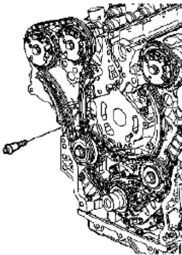
Fig. 314: Identifying Right Secondary Camshaft Drive Chain Shoe Bolt Courtesy of SUZUKI OF AMERICA CORP.
