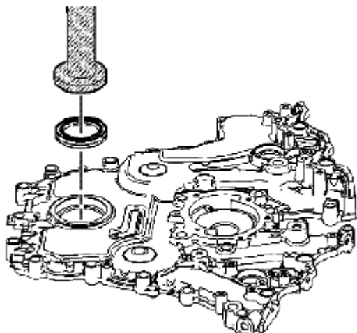
Fig. 532: Installing Crankshaft Front Oil Seal Courtesy of SUZUKI OF AMERICA CORP.
