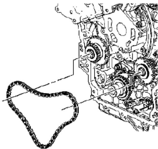
Fig. 859: Identifying Primary Camshaft Drive Chain Courtesy of SUZUKI OF AMERICA CORP.
