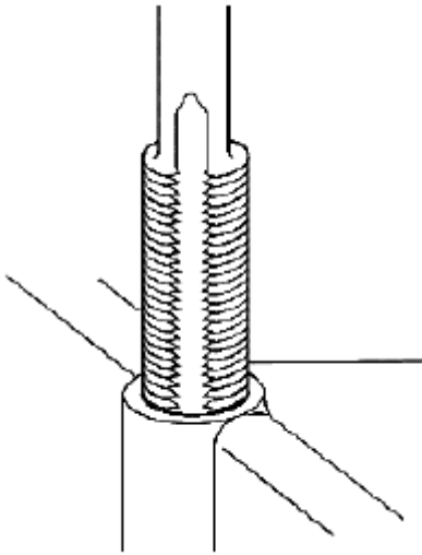
Fig. 597: Applying Threads Of Drilled Hole Courtesy of SUZUKI OF AMERICA CORP.
