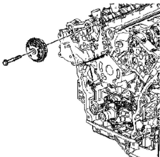
Fig. 356: Identifying Right Intake Camshaft Position Actuator & Bolt Courtesy of SUZUKI OF AMERICA CORP.
