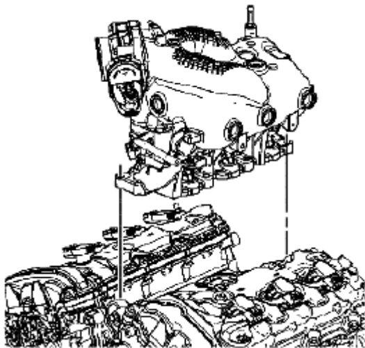
Fig. 278: Identifying Intake Manifold Assembly Courtesy of SUZUKI OF AMERICA CORP.
