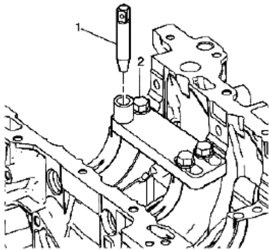
Fig. 674: Positioning Alignment Pin Through Bushing Courtesy of SUZUKI OF AMERICA CORP.
