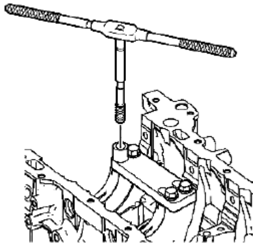
Fig. 685: Applying Threads Of Drilled Hole By Hand Courtesy of SUZUKI OF AMERICA CORP.
