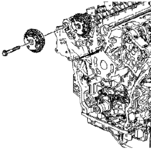
Fig. 781: Identifying Right Exhaust Camshaft Position Actuator & Bolt Courtesy of SUZUKI OF AMERICA CORP.
