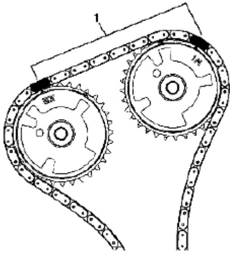
Fig. 900: Identifying Timing Camshaft Drive Chain Link Mark (2 Of 5) Courtesy of SUZUKI OF AMERICA CORP.
