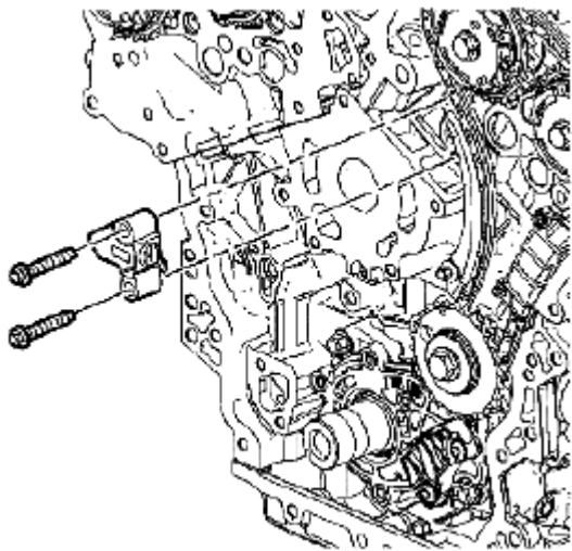
Fig. 132: Identifying Left Bank Secondary Camshaft Drive Chain Tensioner Courtesy of SUZUKI OF AMERICA CORP.
