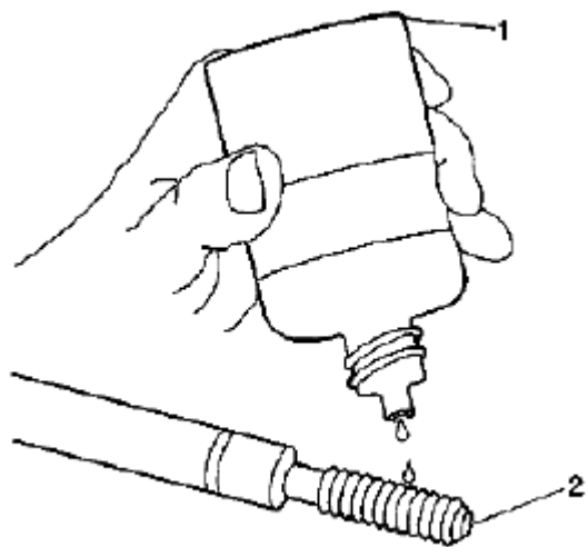
Fig. 682: Lubricating Threads Of Driver Installation Tool Courtesy of SUZUKI OF AMERICA CORP.
