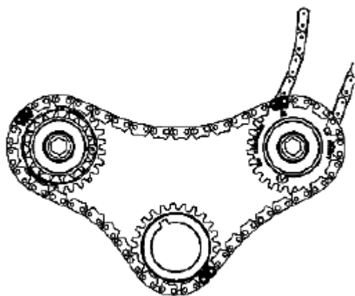
Fig. 854: Identifying Primary Camshaft Drive Chain Mark Courtesy of SUZUKI OF AMERICA CORP.
