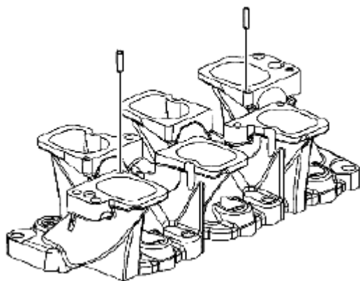
Fig. 569: Identifying Upper-To-Lower Intake Manifold Alignment Pins Courtesy of SUZUKI OF AMERICA CORP.
