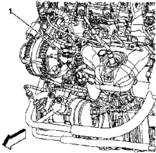
Fig. 46: Connecting Generator Electrical Connector Courtesy of SUZUKI OF AMERICA CORP.
