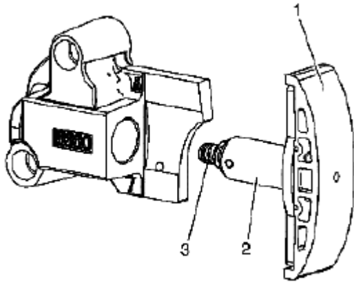
Fig. 523: Identifying Primary Timing Chain Tensioner Courtesy of SUZUKI OF AMERICA CORP.
