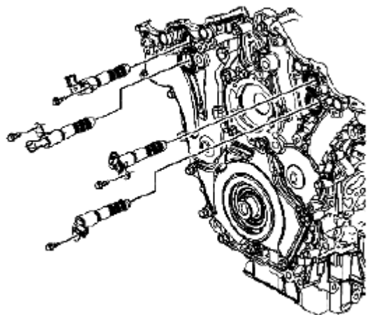
Fig. 301: Identifying Camshaft Position Actuator Valve & Bolts Courtesy of SUZUKI OF AMERICA CORP.
