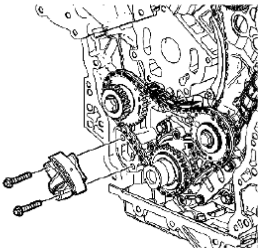
Fig. 324: Identifying Primary Camshaft Drive Chain Tensioner & Bolts Courtesy of SUZUKI OF AMERICA CORP.
