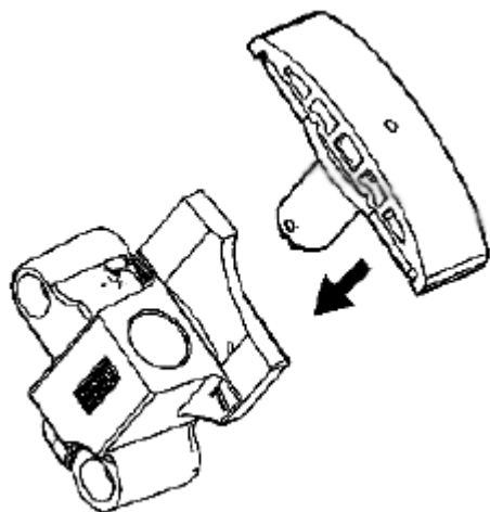
Fig. 873: Installing Plunger Into Primary Camshaft Drive Chain Tensioner Body Courtesy of SUZUKI OF AMERICA CORP.
