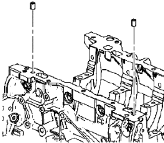
Fig. 391: Identifying Cylinder Block-To-Oil Pan Alignment Dowels Courtesy of SUZUKI OF AMERICA CORP.
