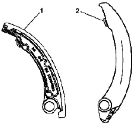
Fig. 137: Identifying Left Secondary Camshaft Drive Chain Shoe (2 Of 3) Courtesy of SUZUKI OF AMERICA CORP.
