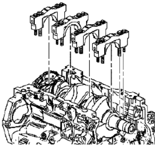
Fig. 705: Identifying Crankshaft Main Bearing Caps Courtesy of SUZUKI OF AMERICA CORP.
