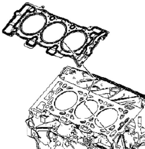
Fig. 221: Identifying Cylinder Head Gasket Courtesy of SUZUKI OF AMERICA CORP.
