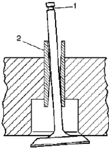
Fig. 451: Identifying Valve Stem-To-Guide Clearance Courtesy of SUZUKI OF AMERICA CORP.
