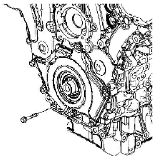
Fig. 945: Identifying Engine Front Cover Bolts (2 Of 2) Courtesy of SUZUKI OF AMERICA CORP.
