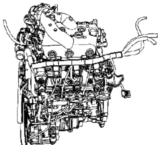
Fig. 78: Identifying Engine Harness Retaining Clips Courtesy of SUZUKI OF AMERICA CORP.
