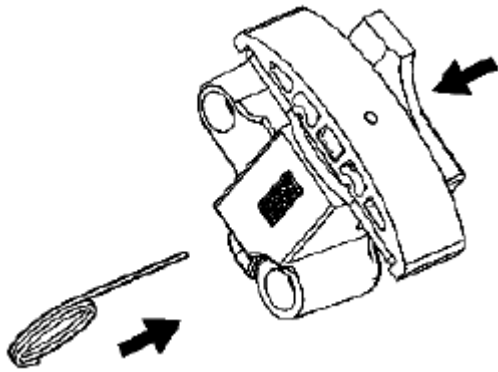
Fig. 874: Inserting EN 46112 Into Hole Of Primary Camshaft Drive Chain Tensioner Body Courtesy of SUZUKI OF AMERICA CORP.
