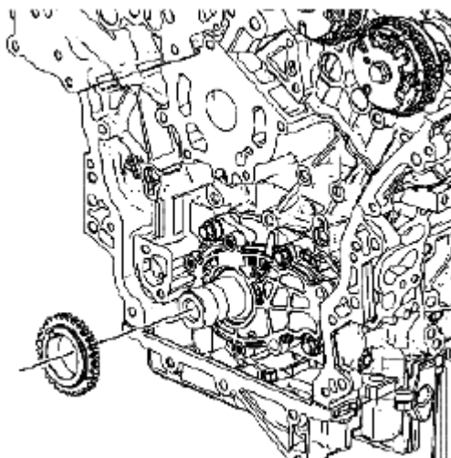
Fig. 799: Identifying Crankshaft Sprocket Courtesy of SUZUKI OF AMERICA CORP.
