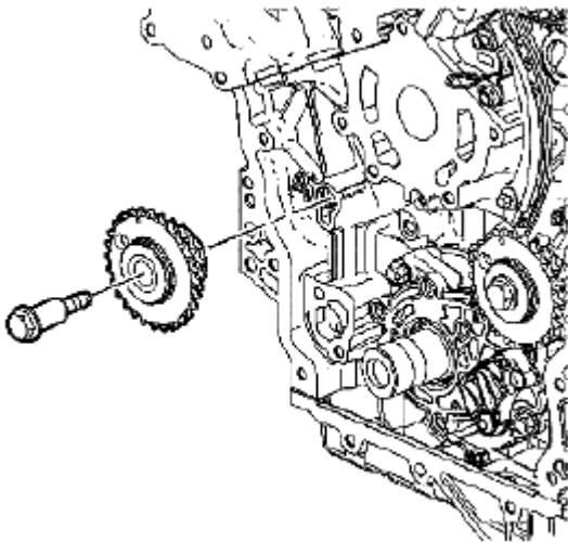
Fig. 154: Identifying Left Bank Camshaft Intermediate Drive Chain Idler Courtesy of SUZUKI OF AMERICA CORP.
