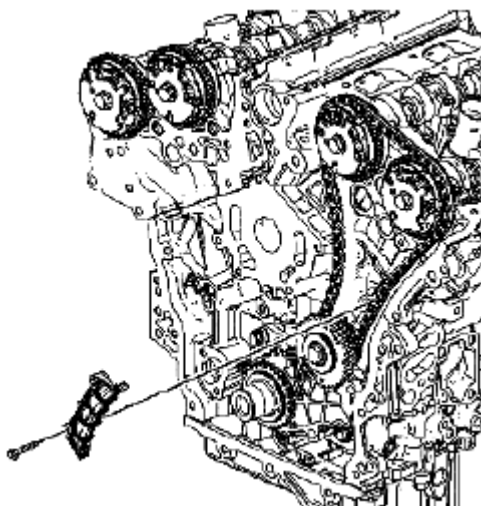
Fig. 343: Identifying Left Secondary Camshaft Drive Chain Guide Bolts Courtesy of SUZUKI OF AMERICA CORP.
