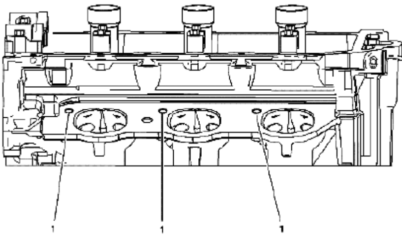
Fig. 1019: Identifying Right Cylinder Head Intake Face Courtesy of SUZUKI OF AMERICA CORP.
