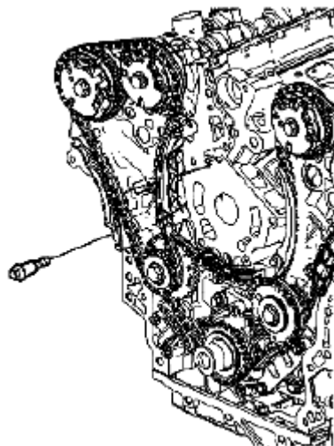
Fig. 920: Identifying Secondary Camshaft Drive Chain Shoe Bolt Courtesy of SUZUKI OF AMERICA CORP.
