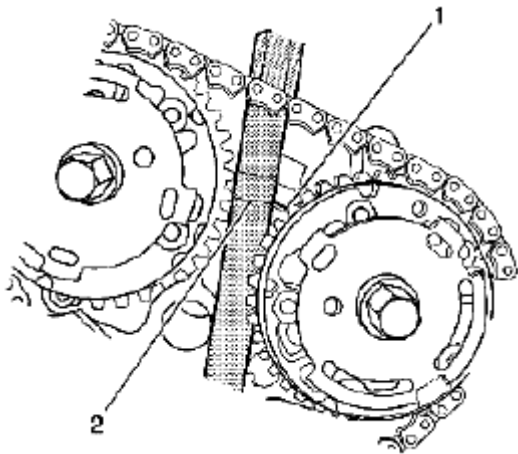
Fig. 162: Inserting EN-48313 Between Camshaft Actuators Courtesy of SUZUKI OF AMERICA CORP.
