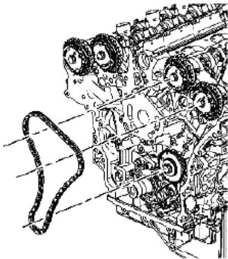
Fig. 128: Identifying Left Bank Secondary Camshaft Drive Chain Courtesy of SUZUKI OF AMERICA CORP.
