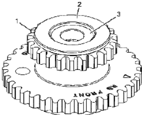
Fig. 510: Identifying Front Of Right Intermediate Sprocket Courtesy of SUZUKI OF AMERICA CORP.
