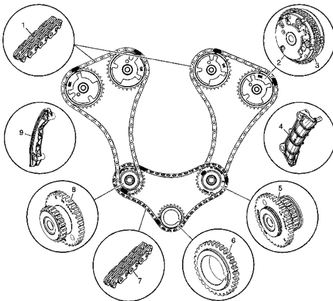
Fig. 2: Camshaft Timing Drive Design Identification - Second Design 2007 - Present Courtesy of SUZUKI OF AMERICA CORP.
