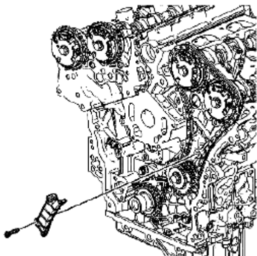
Fig. 822: Identifying Left Secondary Camshaft Drive Chain Guide & Bolt Courtesy of SUZUKI OF AMERICA CORP.
