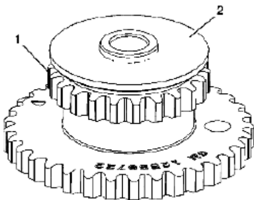
Fig. 509: Identifying Back Of Left Intermediate Sprocket Courtesy of SUZUKI OF AMERICA CORP.
