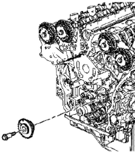
Fig. 155: Identifying Right Bank Camshaft Intermediate Drive Chain Idler Courtesy of SUZUKI OF AMERICA CORP.
