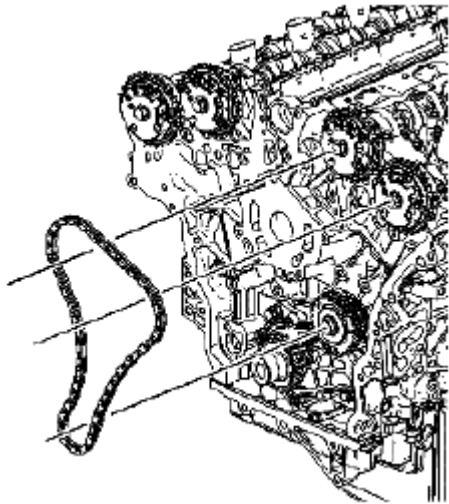
Fig. 807: Identifying Left Secondary Camshaft Drive Chain Courtesy of SUZUKI OF AMERICA CORP.
