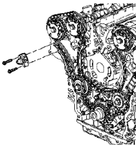
Fig. 310: Identifying Right Secondary Camshaft Drive Chain Tensioner & Bolts Courtesy of SUZUKI OF AMERICA CORP.
