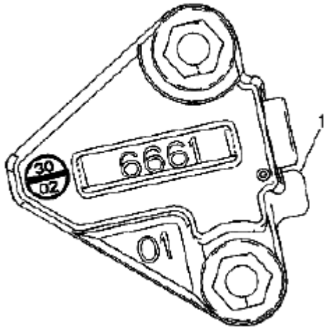
Fig. 837: Identifying Left Secondary Camshaft Drive Chain Tensioner Gasket Tab Courtesy of SUZUKI OF AMERICA CORP.
