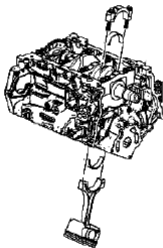
Fig. 733: Identifying Connecting Rod & Connecting Rod Cap Courtesy of SUZUKI OF AMERICA CORP.
