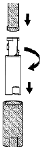
Fig. 931: Resetting Right Secondary Camshaft Drive Chain Tensioner Plunger Using J 45027 Courtesy of SUZUKI OF AMERICA CORP.
