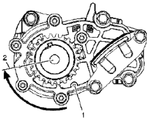
Fig. 881: Aligning Timing Mark On Crankshaft Sprocket Timing Mark And Oil Pump Cover Courtesy of SUZUKI OF AMERICA CORP.
