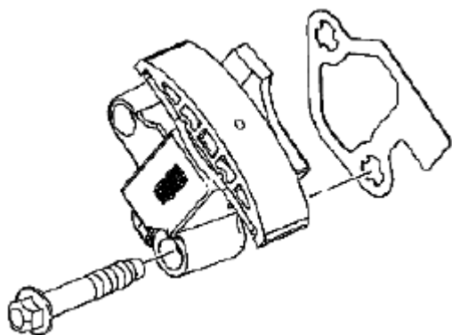
Fig. 888: Identifying Primary Camshaft Drive Chain Tensioner, Gasket & Bolt Courtesy of SUZUKI OF AMERICA CORP.
