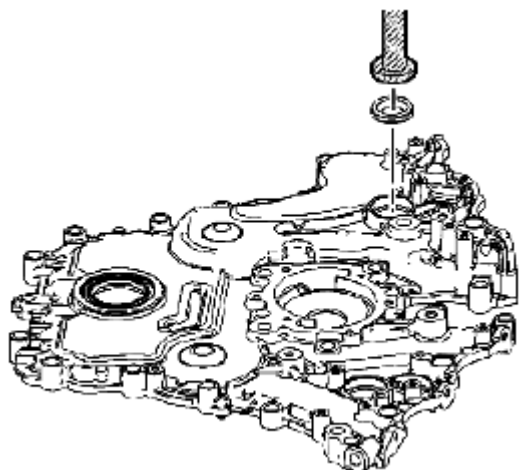
Fig. 534: Installing Camshaft Position Actuator Valve Oil Seals Courtesy of SUZUKI OF AMERICA CORP.
