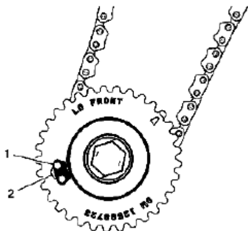
Fig. 816: Identifying Timing Camshaft Drive Chain Link Courtesy of SUZUKI OF AMERICA CORP.
