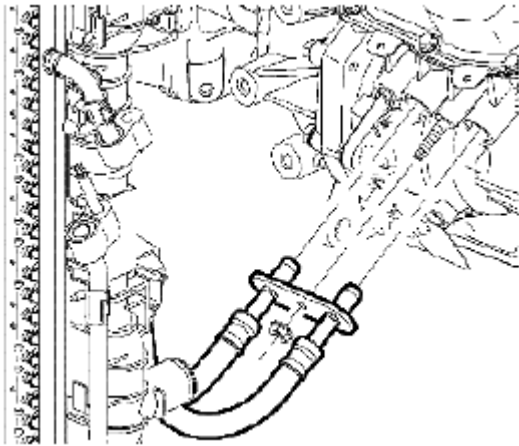
Fig. 258: Connecting Transaxle Oil Cooler Lines To Transaxle Courtesy of SUZUKI OF AMERICA CORP.
