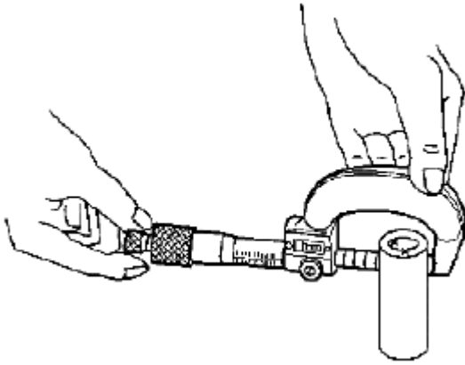
Fig. 422: Measuring Piston Pin Courtesy of SUZUKI OF AMERICA CORP.
