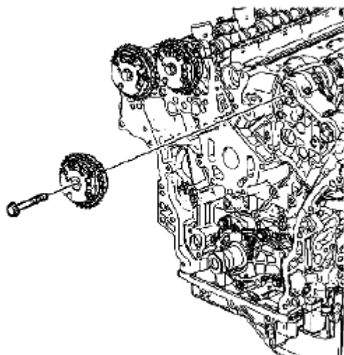
Fig. 785: Identifying Left Intake Camshaft Position Actuator & Bolt Courtesy of SUZUKI OF AMERICA CORP.
