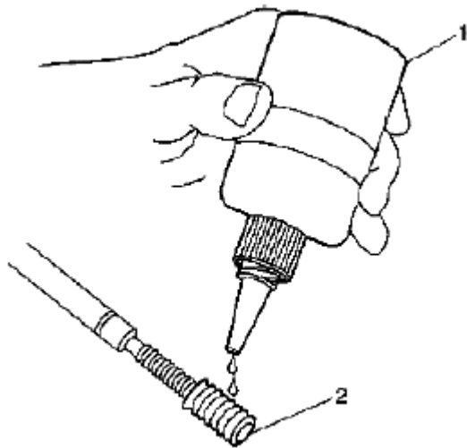
Fig. 684: Applying Threadlock Sealant To Insert OD Threads Courtesy of SUZUKI OF AMERICA CORP.
