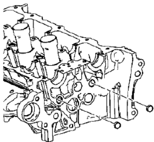
Fig. 445: Identifying Cylinder Head Oil Gallery Expansion Plugs Courtesy of SUZUKI OF AMERICA CORP.
