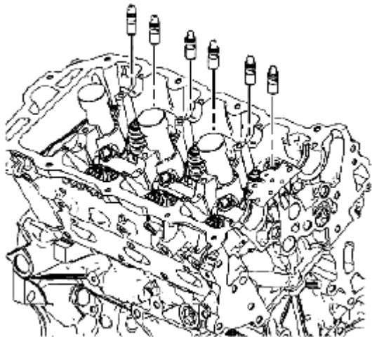
Fig. 192: Identifying Valve Lifters - Left Side Courtesy of SUZUKI OF AMERICA CORP.
