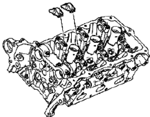
Fig. 189: Identifying Rocker Arms
