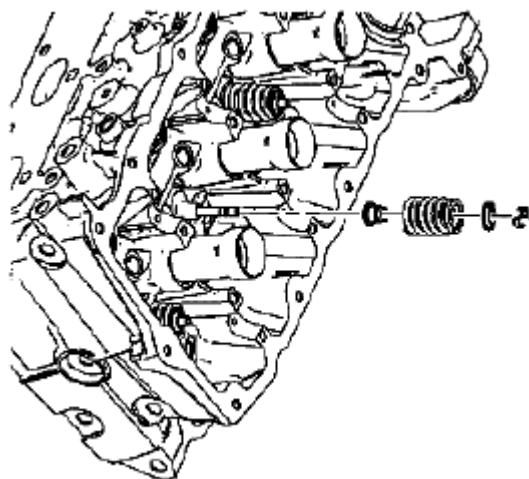
Fig. 442: Identifying Valve Spring Retainer & Valve Spring Courtesy of SUZUKI OF AMERICA CORP.
