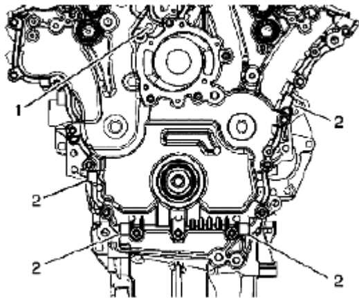
Fig. 295: Identifying Jackscrew Hole Courtesy of SUZUKI OF AMERICA CORP.
