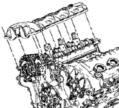
Fig. 111: Identifying Right Camshaft Cover
