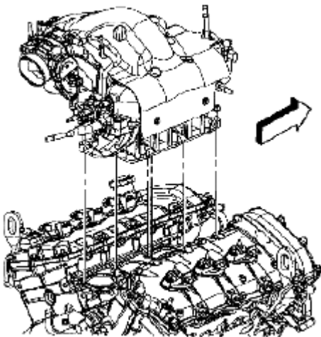
Fig. 80: Installing Upper Intake Manifold And Gasket Courtesy of SUZUKI OF AMERICA CORP.
