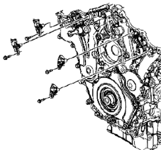
Fig. 948: Identifying Camshaft Position Sensors Courtesy of SUZUKI OF AMERICA CORP.
