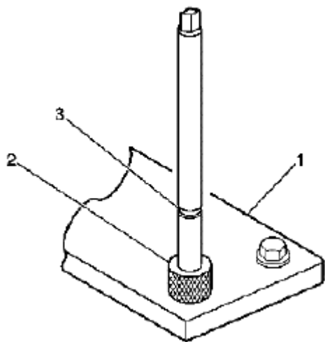
Fig. 671: Identifying Mark & Drill Bushing Courtesy of SUZUKI OF AMERICA CORP.
