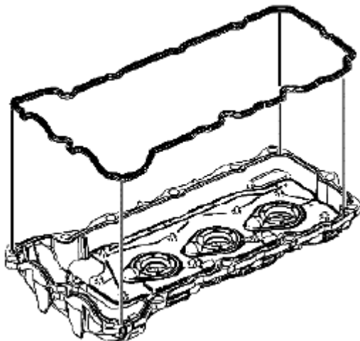
Fig. 538: Identifying Left Camshaft Cover Gasket Courtesy of SUZUKI OF AMERICA CORP.
