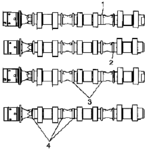
Fig. 766: Identifying Camshaft Identification Ring Courtesy of SUZUKI OF AMERICA CORP.
