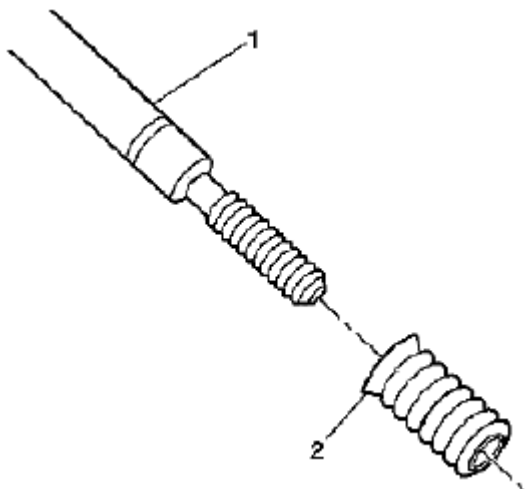
Fig. 618: Applying Insert Onto Driver Installation Tool Courtesy of SUZUKI OF AMERICA CORP.
