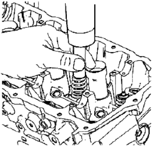
Fig. 439: Tapping On Valve Spring Retainer Courtesy of SUZUKI OF AMERICA CORP.
