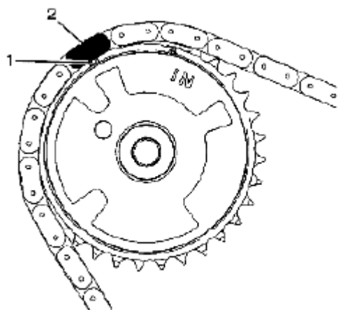
Fig. 811: Identifying Timing Camshaft Drive Chain Link Mark (3 Of 4) Courtesy of SUZUKI OF AMERICA CORP.
