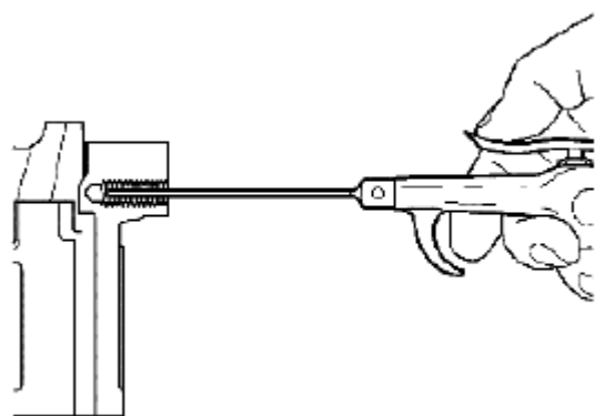
Fig. 630: Applying Compressed Air Into Tapped Hole Courtesy of SUZUKI OF AMERICA CORP.
