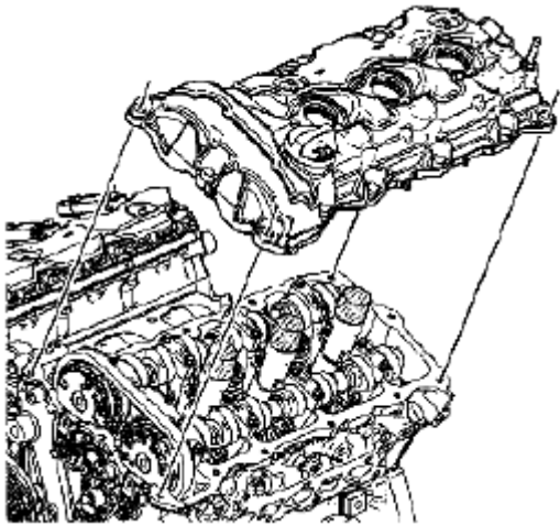
Fig. 963: Identifying Left Camshaft Cover Courtesy of SUZUKI OF AMERICA CORP.
