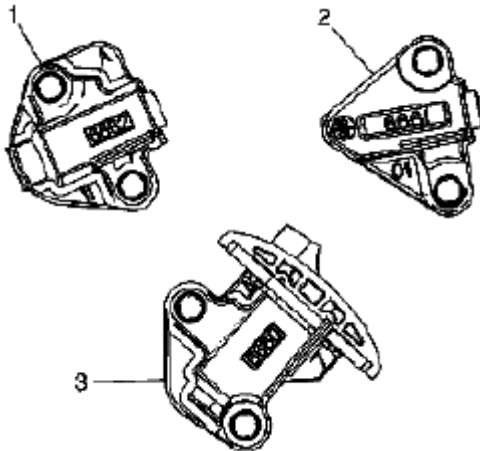
Fig. 840: Identifying Secondary Camshaft Drive Chain Tensioner Courtesy of SUZUKI OF AMERICA CORP.
