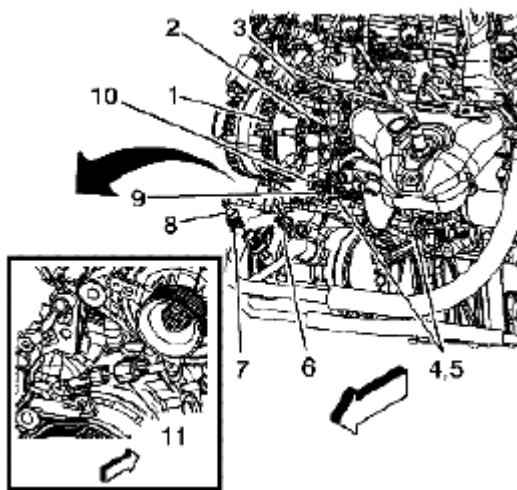
Fig. 237: Disconnecting Engine Wiring Harness Electrical Connector Courtesy of SUZUKI OF AMERICA CORP.
