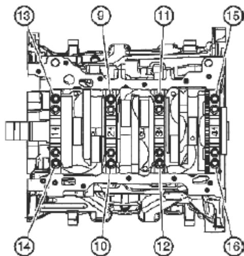
Fig. 722: Tightening Outboard Bolts In Sequence Courtesy of SUZUKI OF AMERICA CORP.
