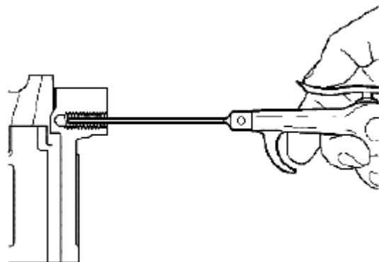
Fig. 679: Applying Compressed Air Into Tapped Hole Courtesy of SUZUKI OF AMERICA CORP.
