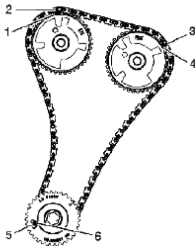
Fig. 848: Identifying Left Secondary Camshaft Drive Chain Timing Mark Courtesy of SUZUKI OF AMERICA CORP.
