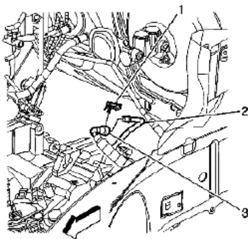
Fig. 259: Connecting Engine Fuel Hose/Pipe To Chassis Fuel Hose/Pipe Courtesy of SUZUKI OF AMERICA CORP.
