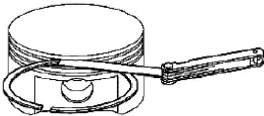
Fig. 425: Measuring Piston Ring Side Clearance Courtesy of SUZUKI OF AMERICA CORP.
