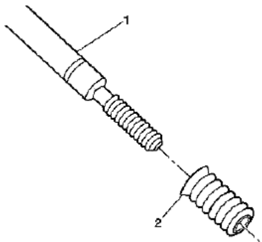
Fig. 634: Applying Insert Onto Driver Installation Tool Courtesy of SUZUKI OF AMERICA CORP.
