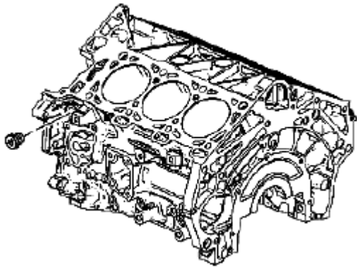
Fig. 396: Identifying M20 Left Side Oil Gallery Threaded Plug Courtesy of SUZUKI OF AMERICA CORP.
