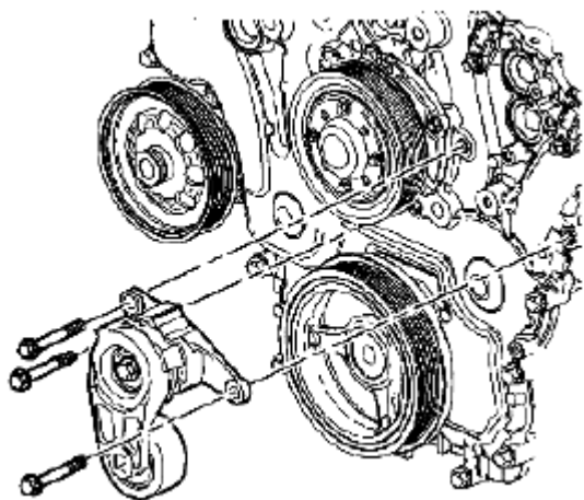
Fig. 261: Identifying Drive Belt Tensioner Assembly & Bolts Courtesy of SUZUKI OF AMERICA CORP.
