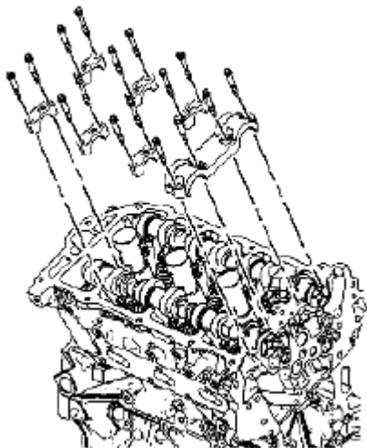
Fig. 368: Identifying Camshaft Bearing Cap & Bolts Courtesy of SUZUKI OF AMERICA CORP.
