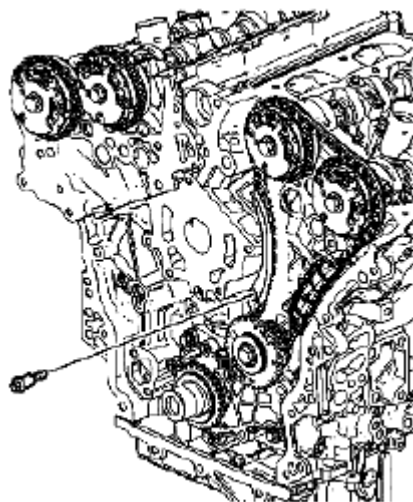
Fig. 830: Identifying Secondary Camshaft Drive Chain Shoe Bolt Courtesy of SUZUKI OF AMERICA CORP.
