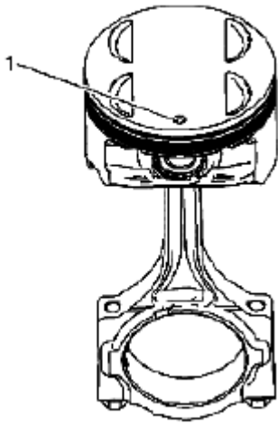
Fig. 724: Identifying Piston Dot
