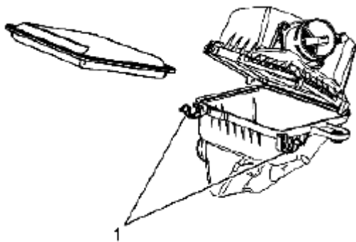
Fig. 27: Identifying Air Cleaner Element Courtesy of SUZUKI OF AMERICA CORP.
