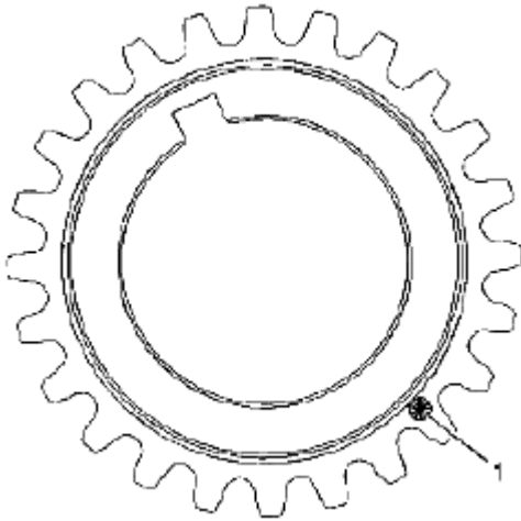
Fig. 148: Identifying Crankshaft Sprocket Timing Mark Courtesy of SUZUKI OF AMERICA CORP.
