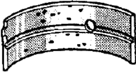
Fig. 405: Identifying Damage Crankshaft Bearing Courtesy of SUZUKI OF AMERICA CORP.
