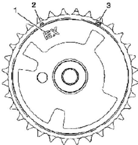
Fig. 780: Identifying Timing Mark Courtesy of SUZUKI OF AMERICA CORP.
