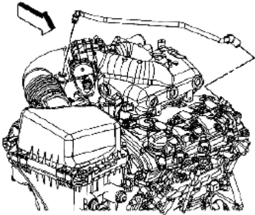
Fig. 23: Locating Positive Crankcase Ventilation (PCV) Tube Courtesy of SUZUKI OF AMERICA CORP.
