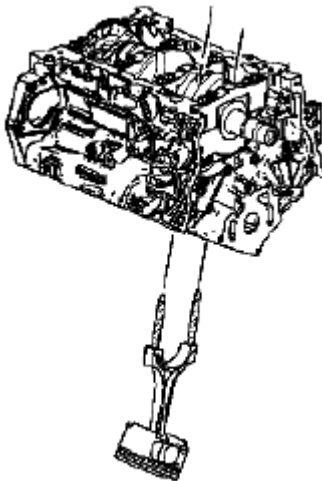
Fig. 379: Identifying Connecting Rod & Piston Assembly Courtesy of SUZUKI OF AMERICA CORP.
