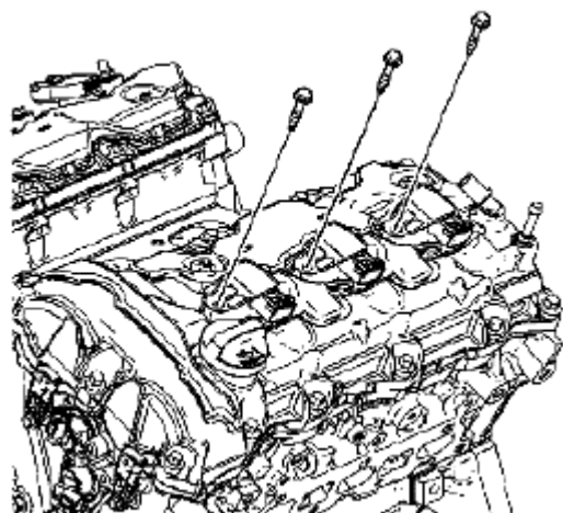
Fig. 969: Identifying Ignition Coil Bolts Courtesy of SUZUKI OF AMERICA CORP.
