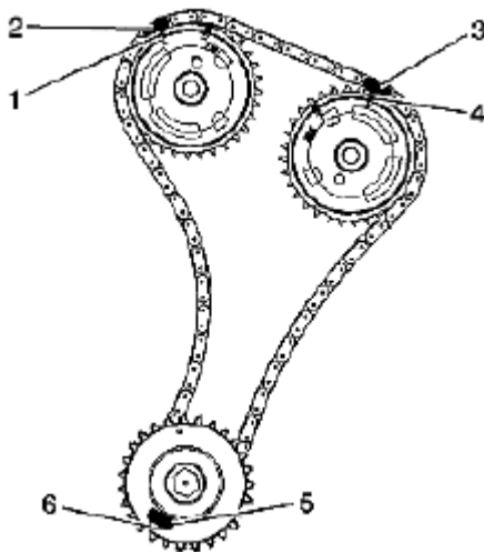
Fig. 167: Identifying Camshaft Timing Chain Mark
