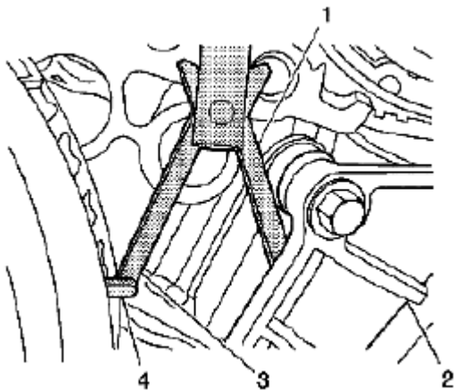
Fig. 163: Inserting Leg Of Tool Behind Timing Chain Guide Courtesy of SUZUKI OF AMERICA CORP.
