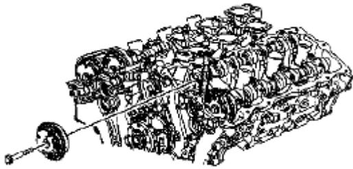
Fig. 166: Identifying Camshaft Position Actuator Bolt Courtesy of SUZUKI OF AMERICA CORP.
