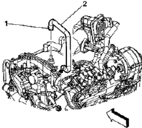
Fig. 260: Connecting Brake Booster Vacuum Hose To Intake Manifold Courtesy of SUZUKI OF AMERICA CORP.
