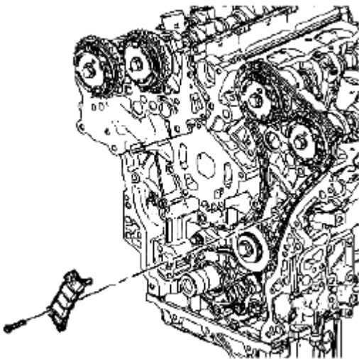
Fig. 143: Identifying Left Bank Secondary Camshaft Drive Chain Guide (2 Of 2) Courtesy of SUZUKI OF AMERICA CORP.
