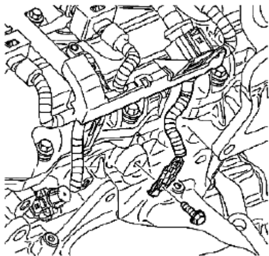
Fig. 213: Identifying Wiring Harness Ground Courtesy of SUZUKI OF AMERICA CORP.
