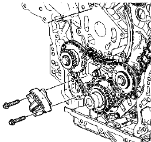
Fig. 889: Identifying Primary Camshaft Drive Chain Tensioner & Bolts Courtesy of SUZUKI OF AMERICA CORP.
