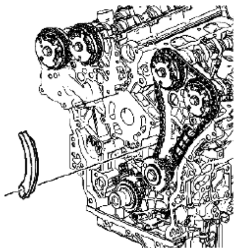
Fig. 341: Identifying Left Secondary Camshaft Drive Chain Shoe Courtesy of SUZUKI OF AMERICA CORP.
