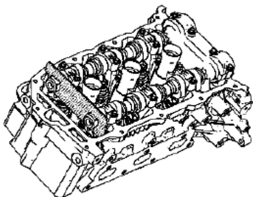
Fig. 308: Identifying EN 46105-1 On Right Camshafts Courtesy of SUZUKI OF AMERICA CORP.
