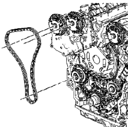
Fig. 320: Identifying Right Secondary Camshaft Drive Chain Courtesy of SUZUKI OF AMERICA CORP.
