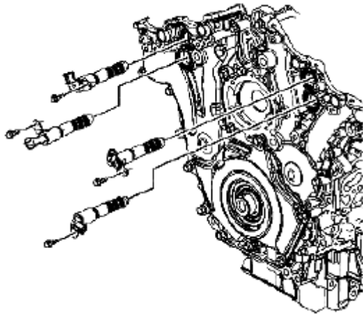
Fig. 957: Identifying Camshaft Position Actuator Valves Courtesy of SUZUKI OF AMERICA CORP.
