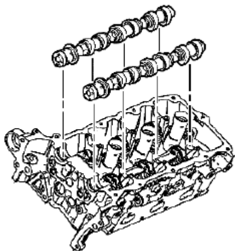
Fig. 361: Identifying Camshafts Courtesy of SUZUKI OF AMERICA CORP.
