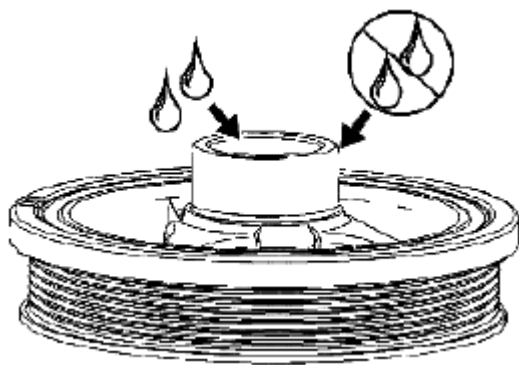
Fig. 93: Applying Lubricant To Inside Of Crankshaft Balancer Hub Bore Courtesy of SUZUKI OF AMERICA CORP.
