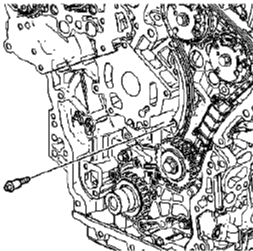
Fig. 827: Identifying Secondary Camshaft Drive Chain Shoe Bolt Courtesy of SUZUKI OF AMERICA CORP.
