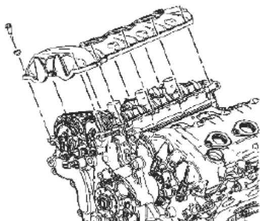
Fig. 107: Identifying Right Camshaft Cover & Bolts Courtesy of SUZUKI OF AMERICA CORP.
