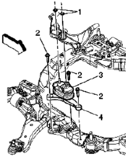
Fig. 57: Removing Lower Bracket Bolts Courtesy of SUZUKI OF AMERICA CORP.
