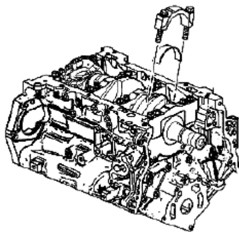
Fig. 732: Identifying Connecting Rod Cap
