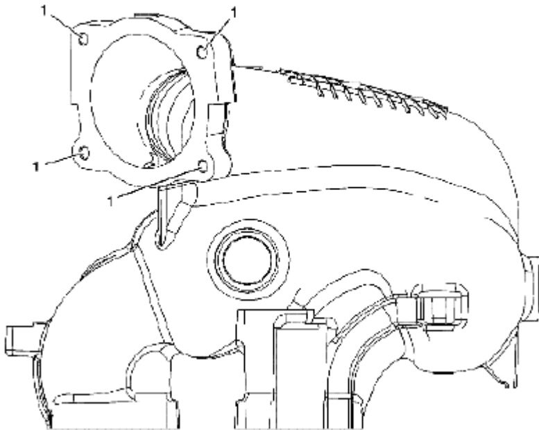
Fig. 1031: Identifying Upper Intake Manifold - Front Courtesy of SUZUKI OF AMERICA CORP.
