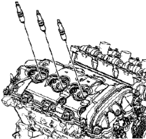
Fig. 978: Identifying Spark Plugs Courtesy of SUZUKI OF AMERICA CORP.
