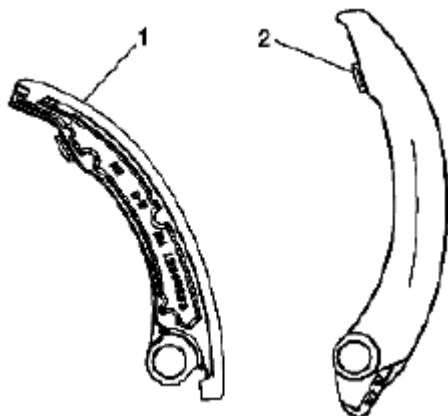
Fig. 915: Identifying Right Secondary Camshaft Drive Chain Shoe (1 Of 2) Courtesy of SUZUKI OF AMERICA CORP.
