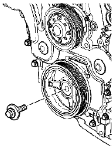
Fig. 95: Identifying Crankshaft Balancer Bolt Courtesy of SUZUKI OF AMERICA CORP.
