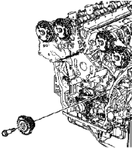
Fig. 346: Identifying Left Camshaft Intermediate Drive Chain Idler And Bolt Courtesy of SUZUKI OF AMERICA CORP.
