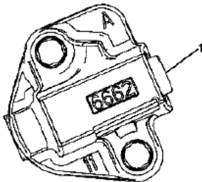
Fig. 936: Identifying Right Secondary Camshaft Drive Chain Tensioner Gasket Tab Courtesy of SUZUKI OF AMERICA CORP.
