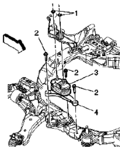
Fig. 59: Removing Mount & Lower Bracket Courtesy of SUZUKI OF AMERICA CORP.
