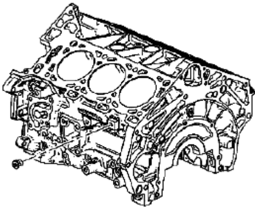
Fig. 395: Identifying M14 Left Side Coolant Drain Threaded Plug Courtesy of SUZUKI OF AMERICA CORP.
