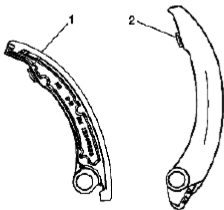
Fig. 825: Identifying Left Secondary Camshaft Drive Chain Shoe (1 Of 2) Courtesy of SUZUKI OF AMERICA CORP.
