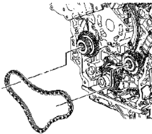
Fig. 146: Identifying Primary Camshaft Timing Chain Courtesy of SUZUKI OF AMERICA CORP.
