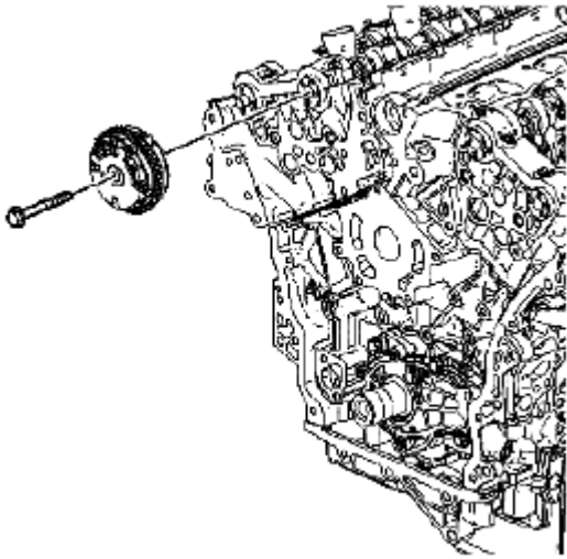
Fig. 357: Identifying Right Intake Camshaft Position Actuator & Bolt Courtesy of SUZUKI OF AMERICA CORP.
