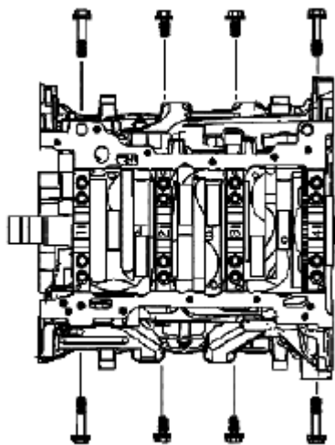
Fig. 720: Identifying Short/Inner Side Main Cap Bolts Courtesy of SUZUKI OF AMERICA CORP.
