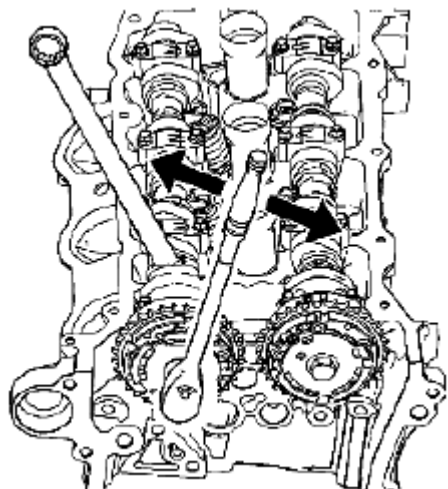
Fig. 176: Loosening Camshaft Position Actuator Bolt Courtesy of SUZUKI OF AMERICA CORP.
