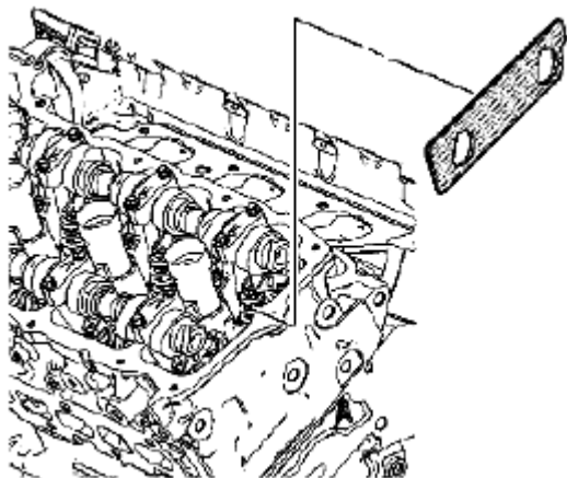
Fig. 959: Identifying Special Tool (EN 46105-2) Courtesy of SUZUKI OF AMERICA CORP.
