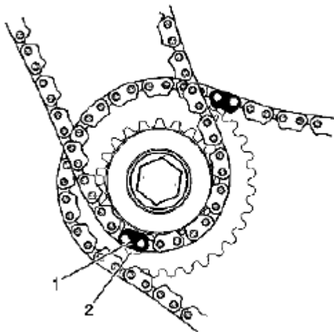
Fig. 906: Identifying Timing Camshaft Drive Chain Link Mark (1 Of 5) Courtesy of SUZUKI OF AMERICA CORP.
