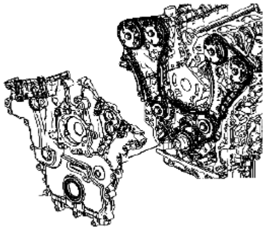
Fig. 306: Identifying Engine Front Cover Courtesy of SUZUKI OF AMERICA CORP.
