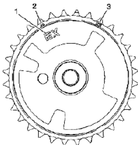
Fig. 791: Identifying Timing Mark
