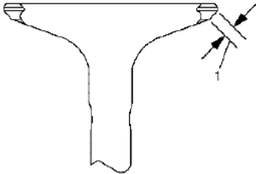
Fig. 455: Identifying Seat Width On Valve Face Courtesy of SUZUKI OF AMERICA CORP.
