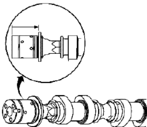
Fig. 472: Identifying Camshaft Thrust Width Courtesy of SUZUKI OF AMERICA CORP.
