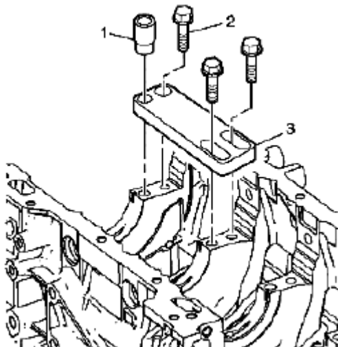
Fig. 673: Positioning Fixture Plate With Bushing Courtesy of SUZUKI OF AMERICA CORP.
