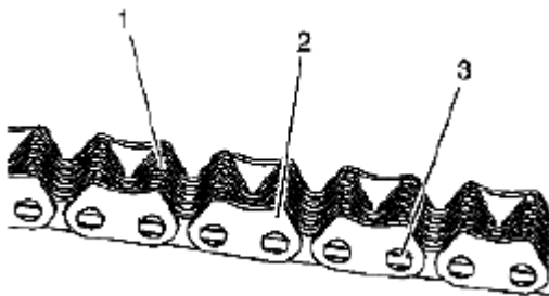
Fig. 513: Identifying Secondary Timing Chain Courtesy of SUZUKI OF AMERICA CORP.
