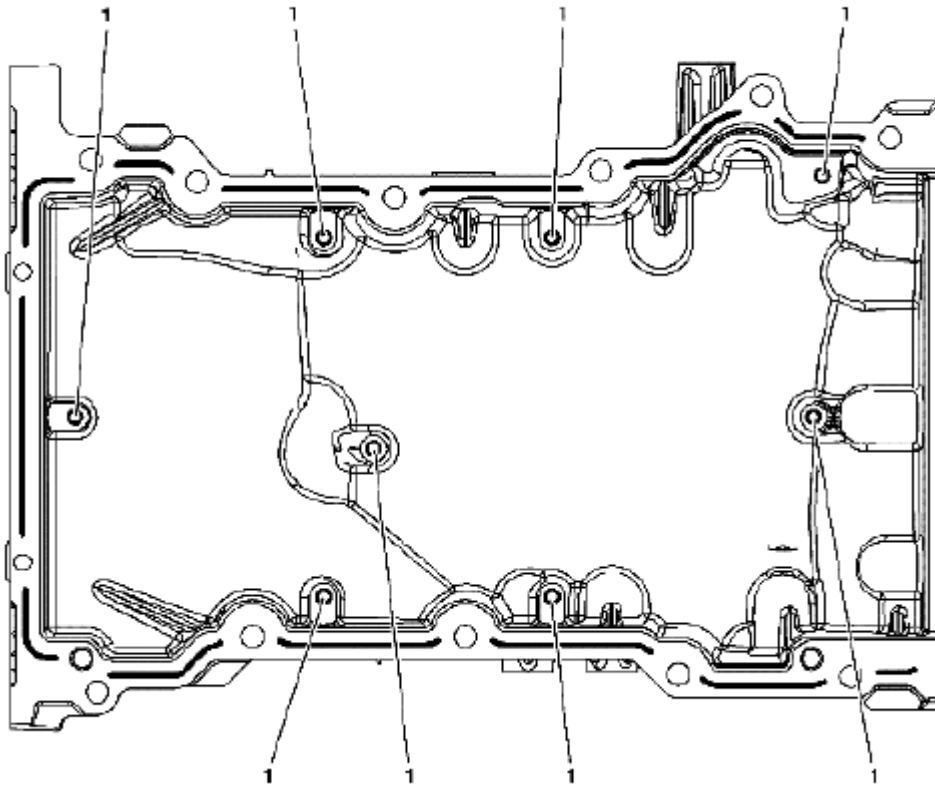
Fig. 1037: Identifying Oil Pan Top Courtesy of SUZUKI OF AMERICA CORP.
