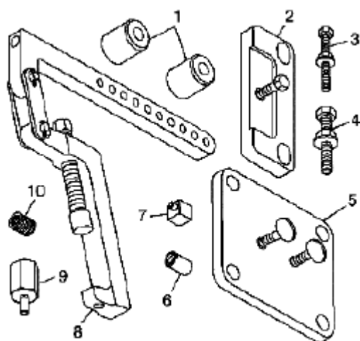
Fig. 731: Identifying J 43690-100 Rod Bearing Clearance Tool - Adapter Kit Courtesy of SUZUKI OF AMERICA CORP.
