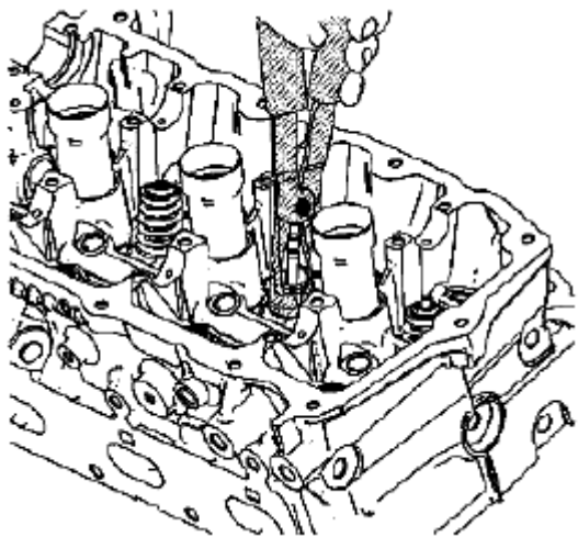
Fig. 462: Identifying Valve Stem Oil Seals Courtesy of SUZUKI OF AMERICA CORP.
