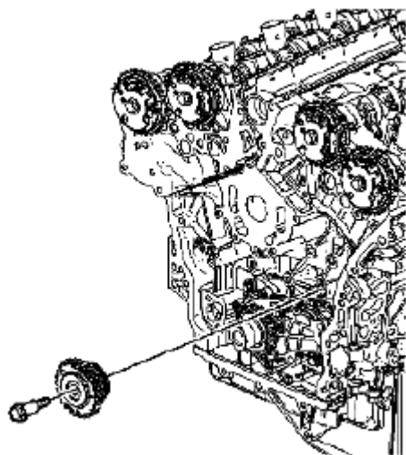
Fig. 802: Identifying Camshaft Intermediate Drive Chain Idler & Bolt Courtesy of SUZUKI OF AMERICA CORP.
