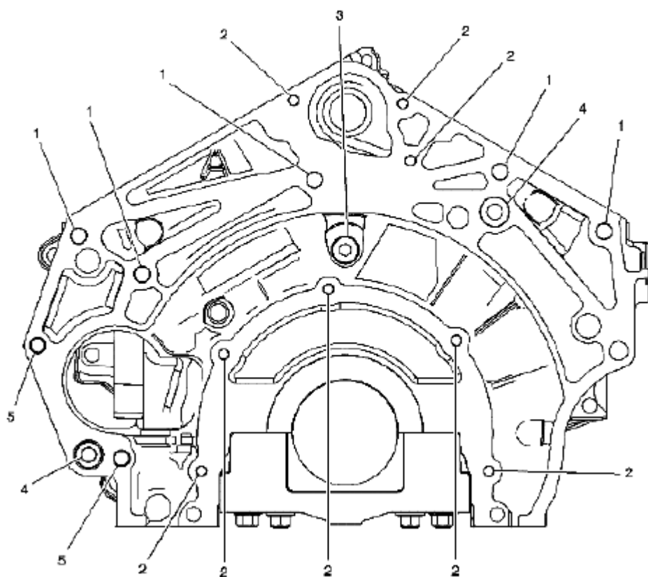
Fig. 1025: Identifying Engine Block Rear Courtesy of SUZUKI OF AMERICA CORP.
