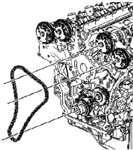
Fig. 815: Identifying Left Secondary Camshaft Drive Chain Courtesy of SUZUKI OF AMERICA CORP.
