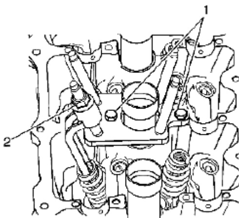
Fig. 196: Identifying Valve Spring Compressor Nut Courtesy of SUZUKI OF AMERICA CORP.
