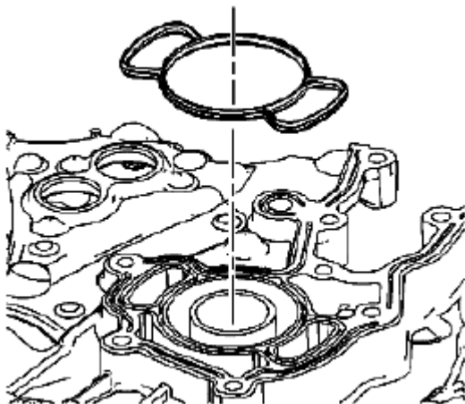
Fig. 950: Identifying Cylinder Block Seal
