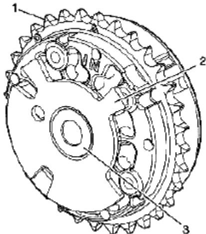
Fig. 480: Identifying Intake Camshaft Position Actuators Courtesy of SUZUKI OF AMERICA CORP.
