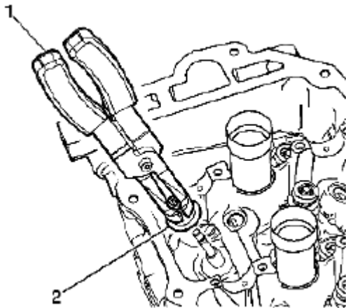
Fig. 200: Identifying Valve Stem Seal (2 Of 2) Courtesy of SUZUKI OF AMERICA CORP.
