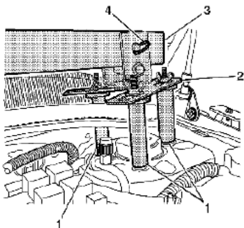
Fig. 1038: Identifying Special Tool (J-28467-13) Courtesy of SUZUKI OF AMERICA CORP.
