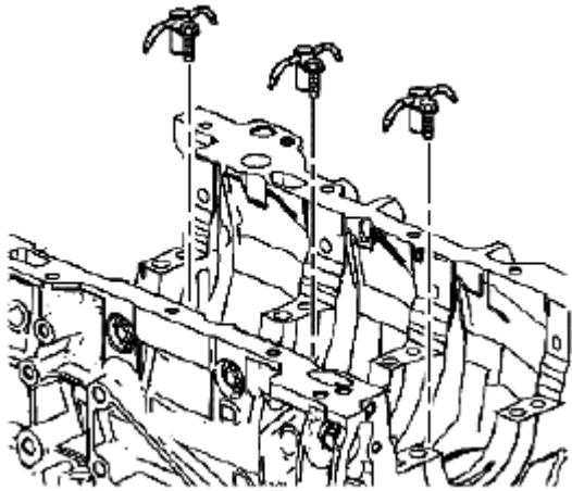
Fig. 389: Identifying Oil Jets
