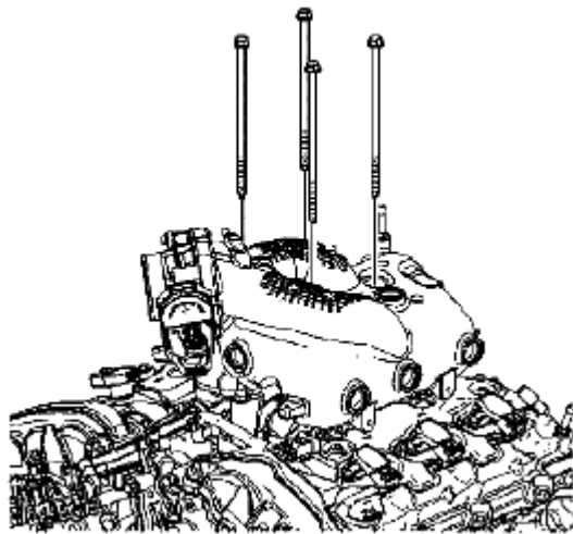
Fig. 276: Identifying Long Intake Manifold Bolts Courtesy of SUZUKI OF AMERICA CORP.
