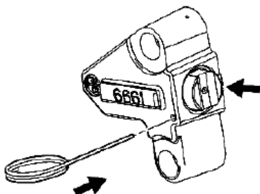
Fig. 843: Inserting EN 46112 Into Access Hole Of Left Secondary Camshaft Drive Chain Tensioner Body
