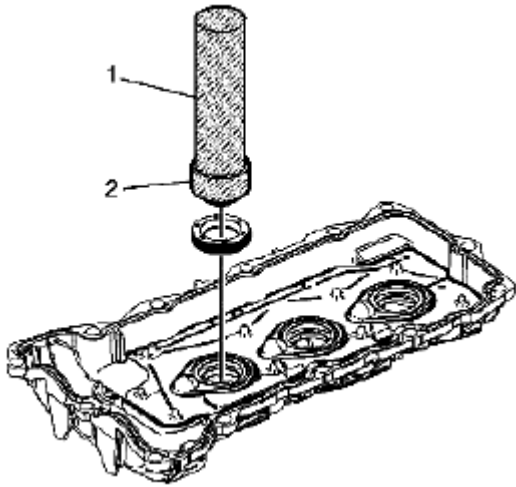
Fig. 551: Installing Left Spark Plug Shield Tube Seals Courtesy of SUZUKI OF AMERICA CORP.
