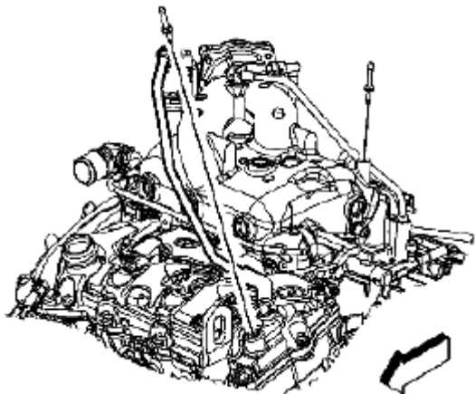
Fig. 86: Installing Fresh Air PCV Line To Air Cleaner Inlet Duct Courtesy of SUZUKI OF AMERICA CORP.
