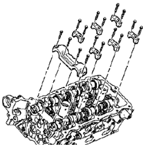
Fig. 360: Identifying Camshaft Bearing Cap & Bolts Courtesy of SUZUKI OF AMERICA CORP.
