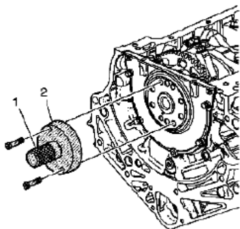
Fig. 740: Identifying Special Tool (EN-47839) Courtesy of SUZUKI OF AMERICA CORP.
