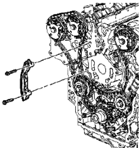
Fig. 912: Identifying Secondary Camshaft Drive Chain Guide Bolts Courtesy of SUZUKI OF AMERICA CORP.
