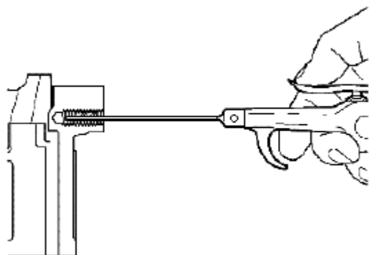
Fig. 614: Applying Compressed Air Into Tapped Hole Courtesy of SUZUKI OF AMERICA CORP.
