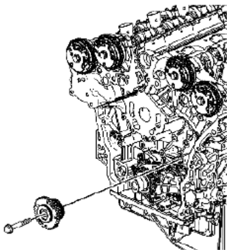
Fig. 347: Identifying Left Camshaft Intermediate Drive Chain Idler & Bolt Courtesy of SUZUKI OF AMERICA CORP.
