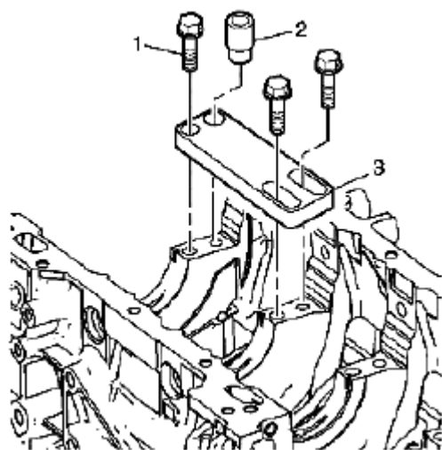
Fig. 672: Identifying Fixture Plate & Bolts Courtesy of SUZUKI OF AMERICA CORP.
