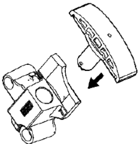
Fig. 886: Installing Plunger Into Primary Camshaft Drive Chain Tensioner Body Courtesy of SUZUKI OF AMERICA CORP.
