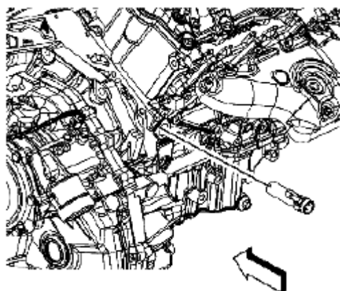
Fig. 246: Identifying Engine Coolant Heater Courtesy of SUZUKI OF AMERICA CORP.
