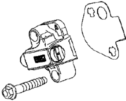
Fig. 311: Identifying Right Secondary Camshaft Drive Chain Tensioner Gasket Courtesy of SUZUKI OF AMERICA CORP.
