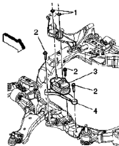
Fig. 50: Removing Mount & Lower Bracket Courtesy of SUZUKI OF AMERICA CORP.
