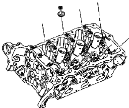
Fig. 203: Identifying Valve Spring Keepers Courtesy of SUZUKI OF AMERICA CORP.
