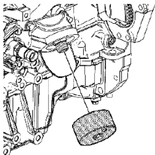
Fig. 1010: Identifying Special Tool (EN-47971) Courtesy of SUZUKI OF AMERICA CORP.
