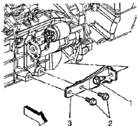
Fig. 240: Removing Engine-To-Transaxle Brace Bolts Courtesy of SUZUKI OF AMERICA CORP.
