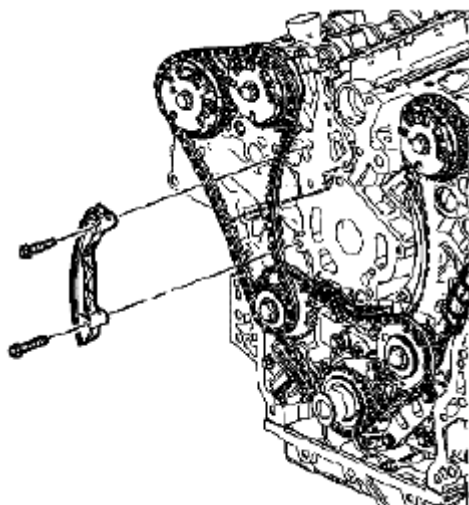
Fig. 319: Identifying Right Secondary Camshaft Drive Chain Guide & Bolts Courtesy of SUZUKI OF AMERICA CORP.
