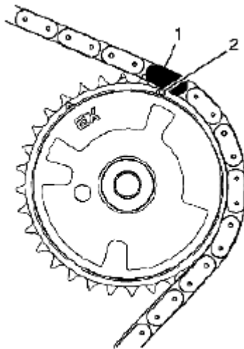
Fig. 810: Identifying Timing Camshaft Drive Chain Link Mark (2 Of 4) Courtesy of SUZUKI OF AMERICA CORP.
