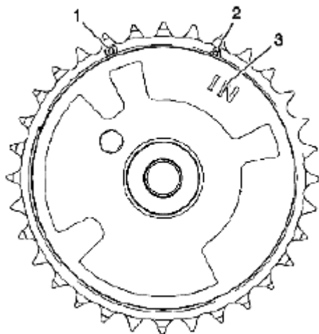
Fig. 784: Identifying Timing Mark Courtesy of SUZUKI OF AMERICA CORP.
