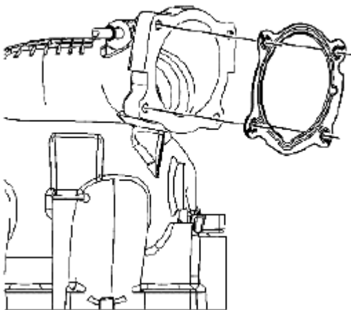
Fig. 582: Identifying Throttle Body Gasket Courtesy of SUZUKI OF AMERICA CORP.
