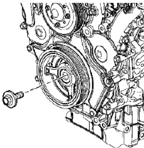
Fig. 1000: Identifying Crankshaft Balancer Bolt Courtesy of SUZUKI OF AMERICA CORP.
