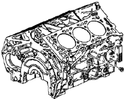
Fig. 695: Identifying M14 Right Side Coolant Drain Threaded Plug Courtesy of SUZUKI OF AMERICA CORP.
