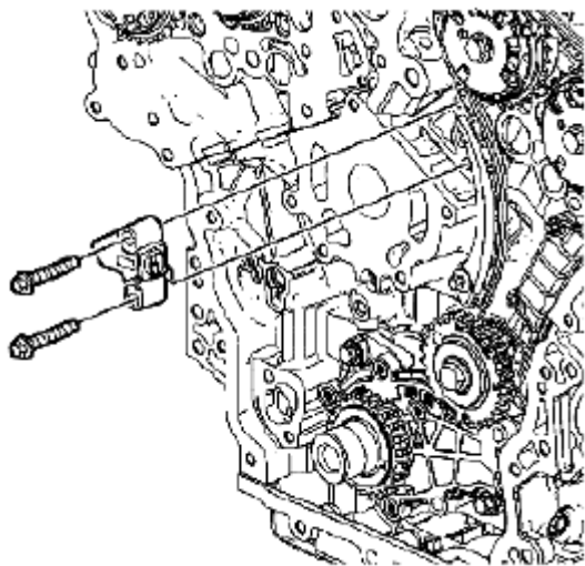
Fig. 334: Identifying Left Secondary Camshaft Drive Chain Tensioner & Bolts Courtesy of SUZUKI OF AMERICA CORP.
