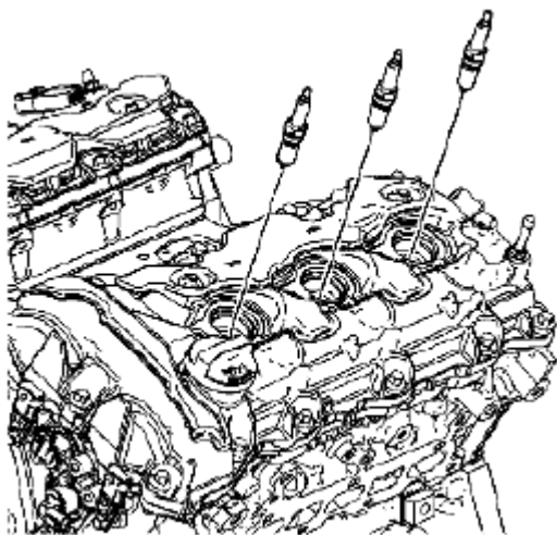
Fig. 966: Identifying Spark Plugs (1 Of 2) Courtesy of SUZUKI OF AMERICA CORP.
