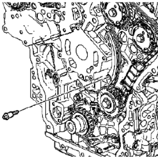
Fig. 135: Identifying Left Secondary Camshaft Drive Chain Shoe Bolt Courtesy of SUZUKI OF AMERICA CORP.
