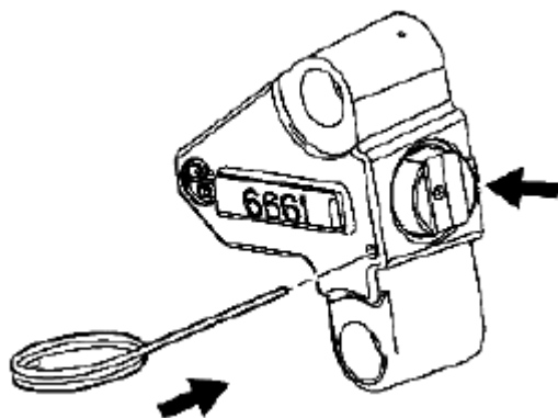
Fig. 834: Inserting EN 46112 Into Access Hole In Left Secondary Camshaft Drive Chain Tensioner Body
