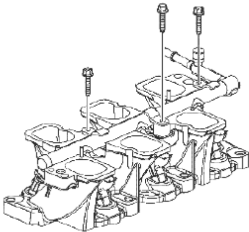
Fig. 567: Identifying Fuel Injector Rail Bolts Courtesy of SUZUKI OF AMERICA CORP.
