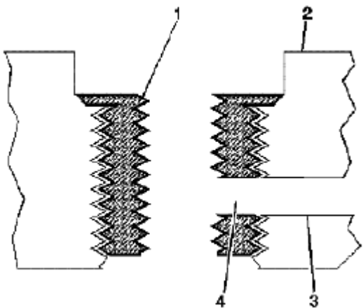
Fig. 624: Identifying Engine Coolant Passage Courtesy of SUZUKI OF AMERICA CORP.
