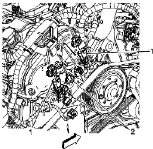
Fig. 249: Connecting Cylinder Head Engine Wiring Harness Electrical Connector Courtesy of SUZUKI OF AMERICA CORP.
