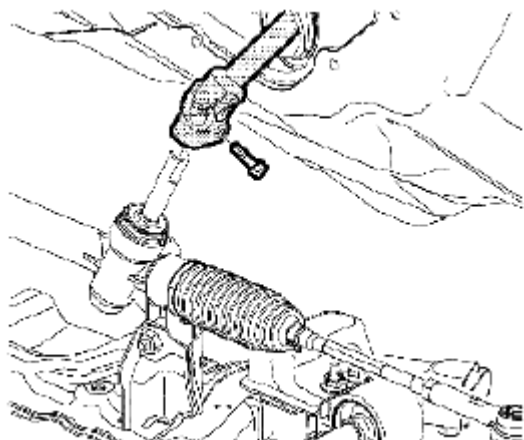
Fig. 228: Identifying Steering Intermediate Shaft Pinch Bolt Courtesy of SUZUKI OF AMERICA CORP.
