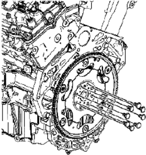
Fig. 265: Identifying Engine Flywheel Bolts Courtesy of SUZUKI OF AMERICA CORP.
