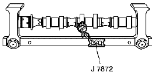
Fig. 474: Measuring Camshaft Lobes Courtesy of SUZUKI OF AMERICA CORP.
