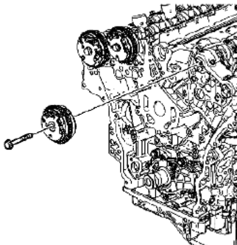
Fig. 171: Identifying Left Intake Camshaft Position Actuator Courtesy of SUZUKI OF AMERICA CORP.
