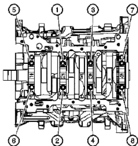
Fig. 708: Tightening Inboard Bolts In Sequence Courtesy of SUZUKI OF AMERICA CORP.
