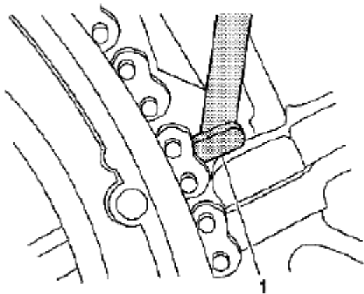
Fig. 164: Identifying Slack In Chain Between Actuators Courtesy of SUZUKI OF AMERICA CORP.
