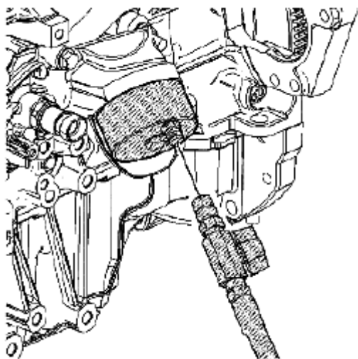
Fig. 1006: Installing Special Tool (J 45299) Flexible Hose To Fitting Courtesy of SUZUKI OF AMERICA CORP.
