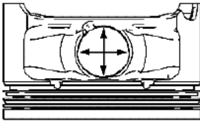
Fig. 423: Measuring Piston Pin Bore Courtesy of SUZUKI OF AMERICA CORP.
