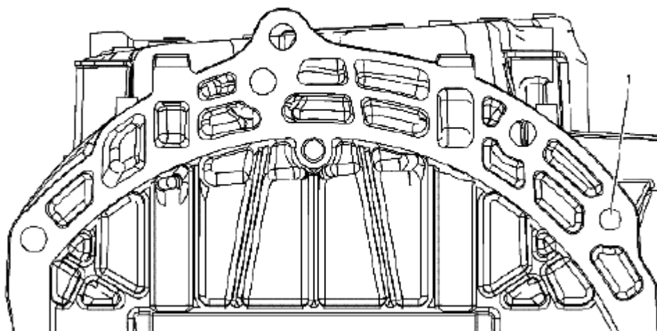
Fig. 1036: Identifying Oil Pan Rear
