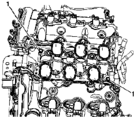
Fig. 88: Identifying Lower Intake Manifold Bolts Courtesy of SUZUKI OF AMERICA CORP.
