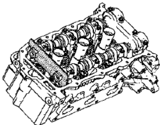
Fig. 298: Identifying EN 46105-1 On Right Camshafts Courtesy of SUZUKI OF AMERICA CORP.
