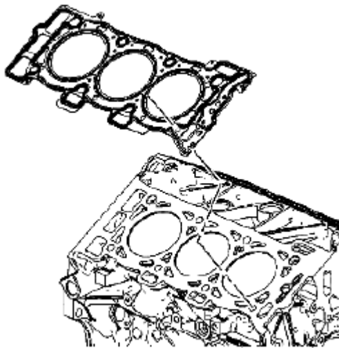
Fig. 220: Identifying Cylinder Head Gasket Courtesy of SUZUKI OF AMERICA CORP.
