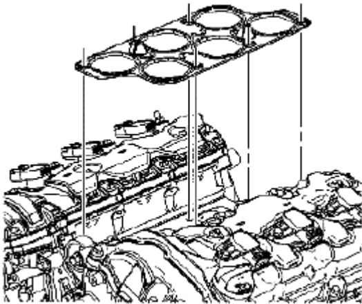
Fig. 279: Identifying Lower Intake Manifold Gasket Courtesy of SUZUKI OF AMERICA CORP.
