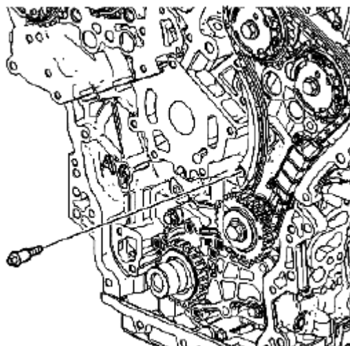
Fig. 139: Identifying Secondary Camshaft Drive Chain Shoe Bolt Courtesy of SUZUKI OF AMERICA CORP.
