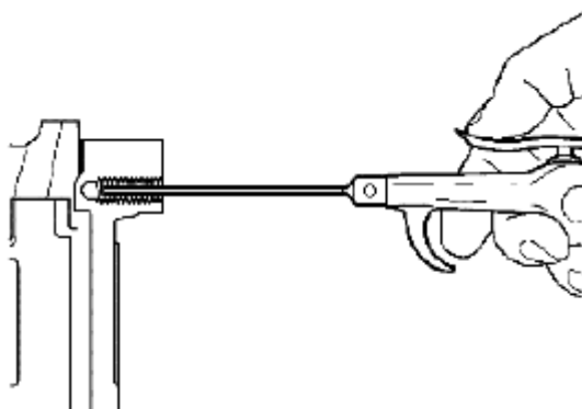
Fig. 594: Applying Compressed Air Into Tapped Hole Courtesy of SUZUKI OF AMERICA CORP.
