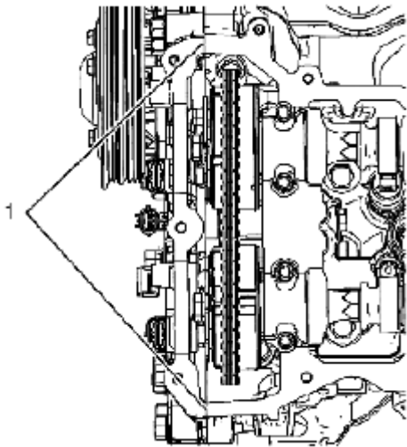
Fig. 962: Placing Bead Of RTV Sealant On Engine Front Cover Split Lines Courtesy of SUZUKI OF AMERICA CORP.
