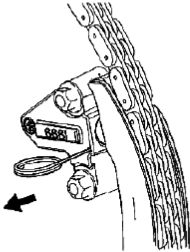
Fig. 838: Pulling EN 46112 From Left Secondary Camshaft Drive Chain Tensioner Courtesy of SUZUKI OF AMERICA CORP.
