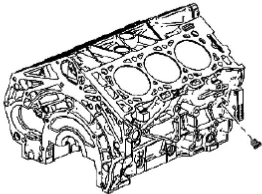
Fig. 392: Identifying M14 Right Side Oil Gallery Threaded Plug Courtesy of SUZUKI OF AMERICA CORP.
