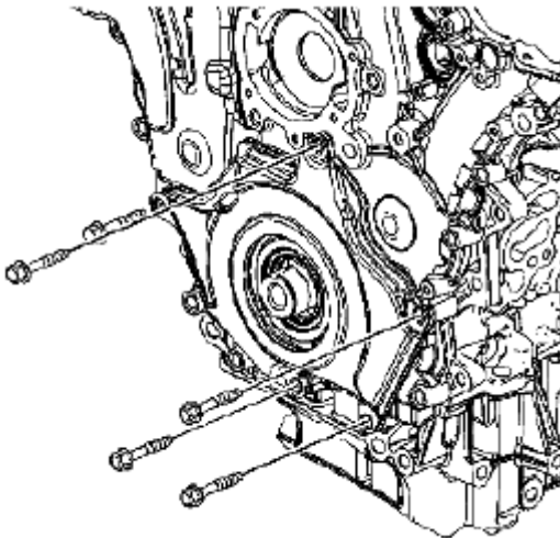
Fig. 954: Identifying Engine Front Cover Bolts Courtesy of SUZUKI OF AMERICA CORP.
