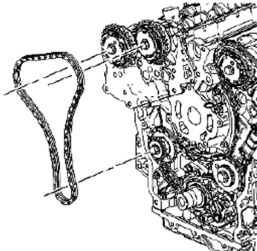
Fig. 130: Identifying Right Bank Secondary Camshaft Drive Chain Courtesy of SUZUKI OF AMERICA CORP.
