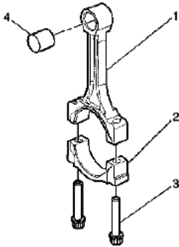
Fig. 427: Identifying Piston Pin Bushing Courtesy of SUZUKI OF AMERICA CORP.
