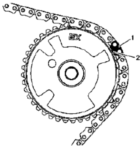
Fig. 818: Identifying Timing Camshaft Drive Chain Link Mark (2 Of 4) Courtesy of SUZUKI OF AMERICA CORP.
