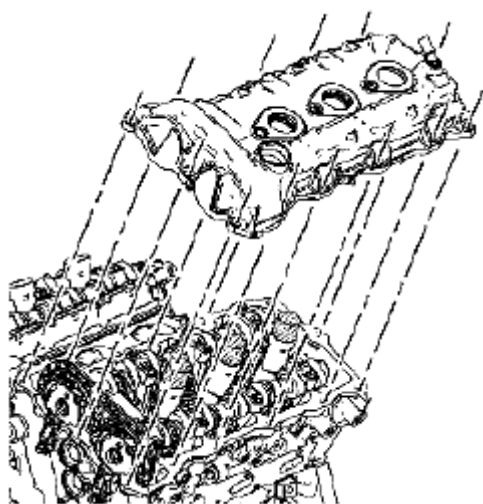
Fig. 103: Identifying Left Camshaft Cover Courtesy of SUZUKI OF AMERICA CORP.
