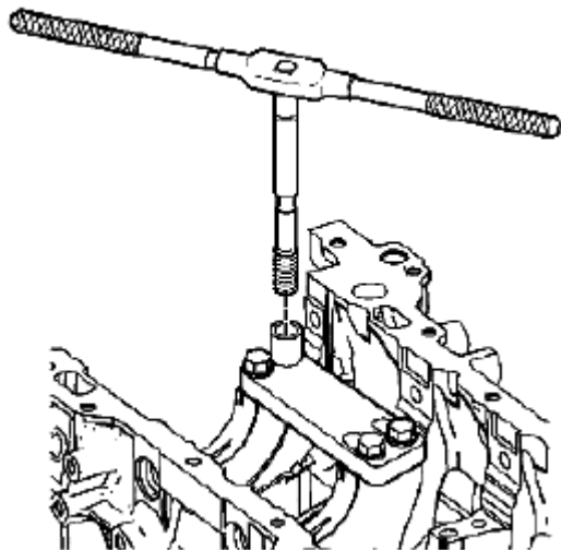
Fig. 670: Applying Threads Of Drilled Hole By Hand Courtesy of SUZUKI OF AMERICA CORP.
