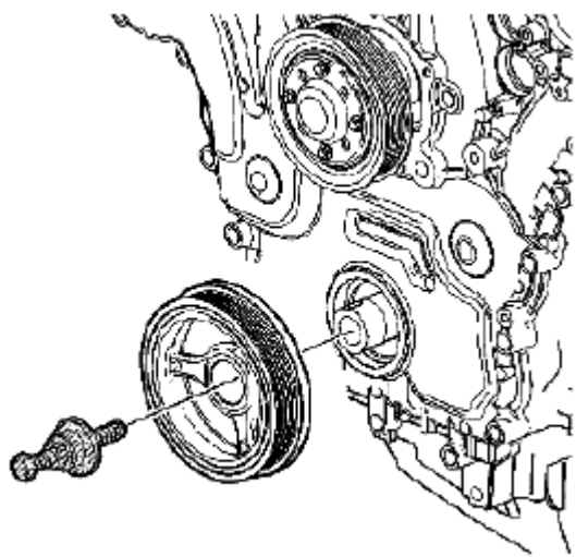
Fig. 94: Placing Crankshaft Balancer On Crankshaft Courtesy of SUZUKI OF AMERICA CORP.
