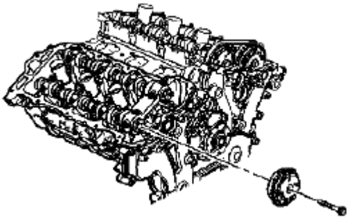
Fig. 174: Identifying Intake Camshaft Position Actuator & Bolt Courtesy of SUZUKI OF AMERICA CORP.
