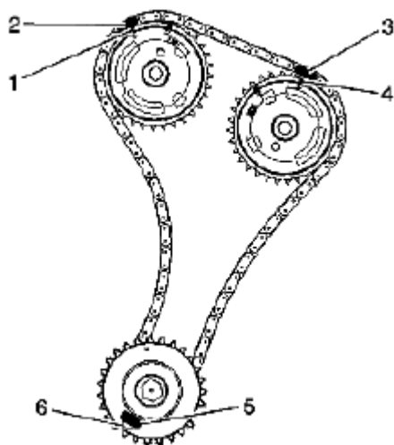
Fig. 179: Identifying Timing Chain Mark
