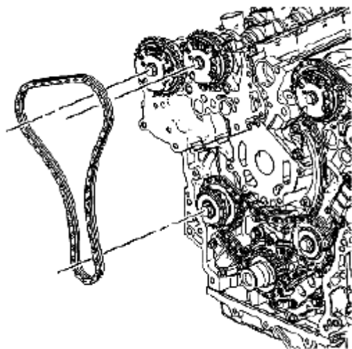
Fig. 898: Identifying Right Secondary Camshaft Drive Chain Courtesy of SUZUKI OF AMERICA CORP.
