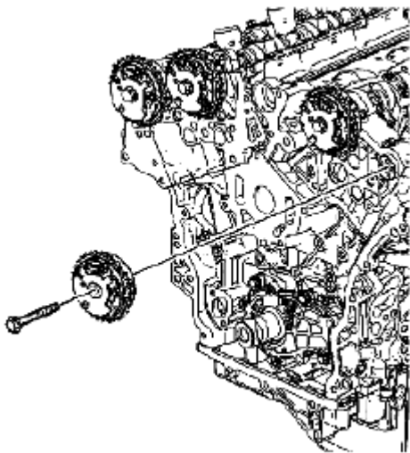
Fig. 792: Identifying Left Exhaust Camshaft Position Actuator & Bolt Courtesy of SUZUKI OF AMERICA CORP.
