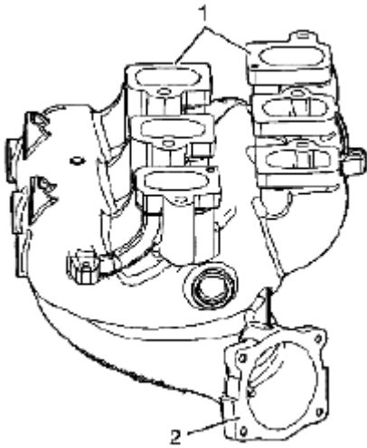
Fig. 572: Identifying Upper Intake Manifold Parts (3 Of 3) Courtesy of SUZUKI OF AMERICA CORP.
