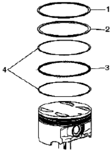
Fig. 434: Identifying Piston Ring
