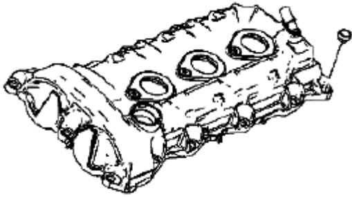
Fig. 101: Identifying Camshaft Cover Bolt Courtesy of SUZUKI OF AMERICA CORP.
