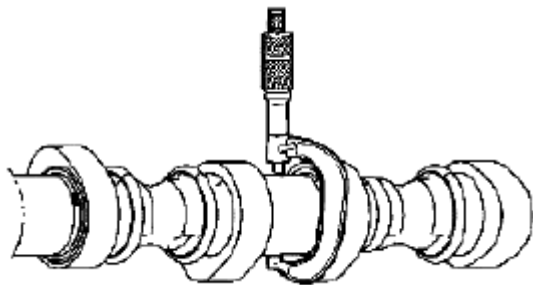
Fig. 470: Measuring Camshaft Journals For Diameter Courtesy of SUZUKI OF AMERICA CORP.
