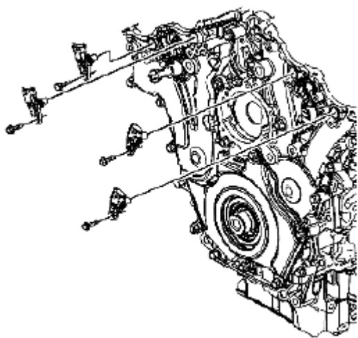
Fig. 300: Identifying Camshaft Position Sensor & Bolts Courtesy of SUZUKI OF AMERICA CORP.
