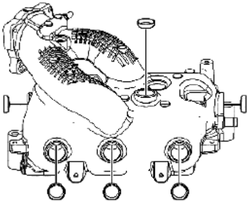
Fig. 581: Identifying Expansion Plugs Courtesy of SUZUKI OF AMERICA CORP.
