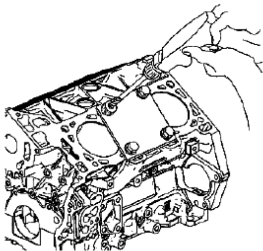
Fig. 644: Drilling Out Threads Of Damaged Hole Courtesy of SUZUKI OF AMERICA CORP.
