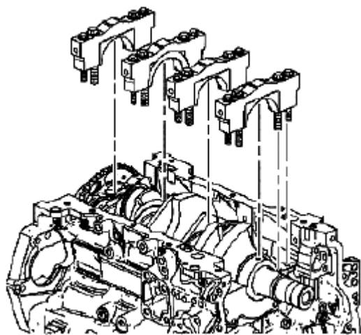
Fig. 384: Identifying Crankshaft Bearing Caps Courtesy of SUZUKI OF AMERICA CORP.
