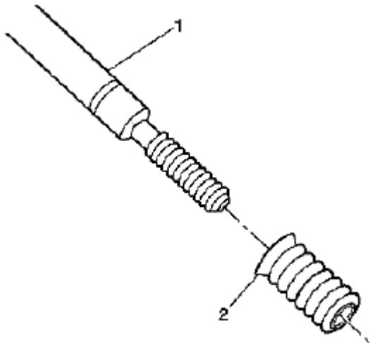
Fig. 653: Applying Insert Onto Driver Installation Tool Courtesy of SUZUKI OF AMERICA CORP.
