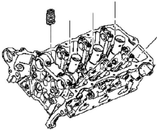
Fig. 210: Identifying Valve Spring Courtesy of SUZUKI OF AMERICA CORP.
