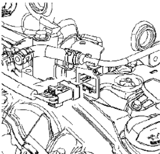
Fig. 270: Identifying Fuel Injector Harness Connector Courtesy of SUZUKI OF AMERICA CORP.
