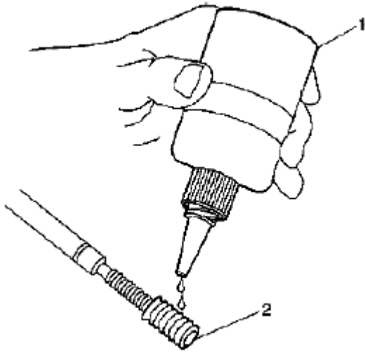
Fig. 635: Applying Threadlock Sealant To Insert OD Threads Courtesy of SUZUKI OF AMERICA CORP.
