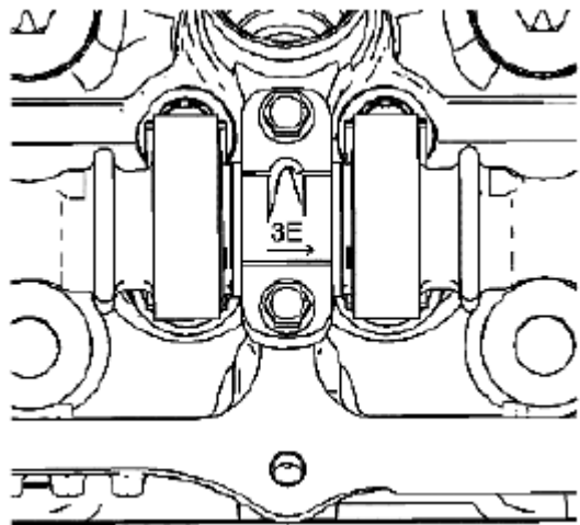
Fig. 367: Identifying Markings On Bearing Caps Courtesy of SUZUKI OF AMERICA CORP.
