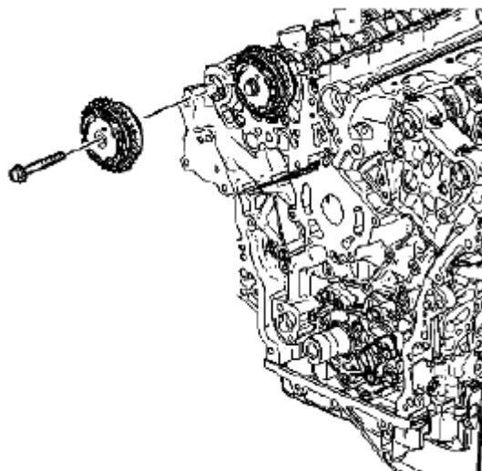
Fig. 169: Identifying Camshaft Position Actuator Courtesy of SUZUKI OF AMERICA CORP.
