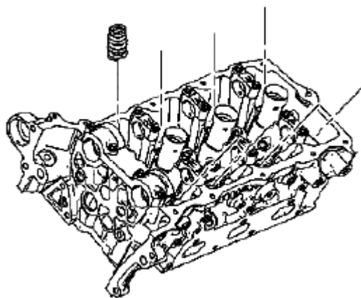
Fig. 201: Identifying Valve Spring Courtesy of SUZUKI OF AMERICA CORP.
