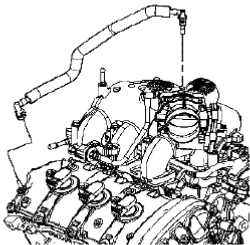
Fig. 988: Identifying Dirty Air Positive Crankcase Ventilation (PCV) Hose Courtesy of SUZUKI OF AMERICA CORP.
