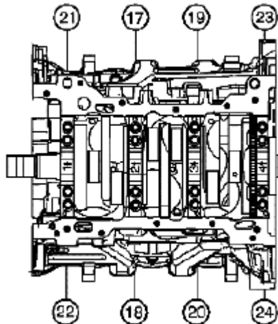
Fig. 710: Tightening Short/Inner Bolts In Sequence Courtesy of SUZUKI OF AMERICA CORP.
