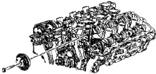
Fig. 168: Identifying Exhaust Camshaft Position Actuator Bolt Courtesy of SUZUKI OF AMERICA CORP.
