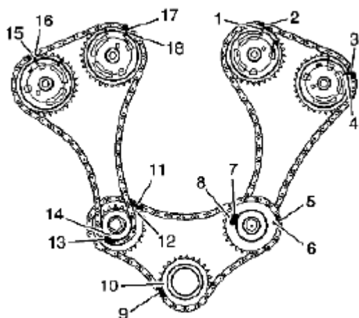
Fig. 185: Identifying Camshaft Timing Chain Mark Courtesy of SUZUKI OF AMERICA CORP.
