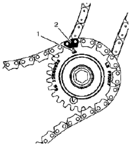
Fig. 855: Identifying Left Camshaft Intermediate Drive Chain Idler Timing Mark Courtesy of SUZUKI OF AMERICA CORP.
