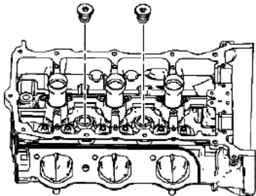
Fig. 460: Identifying Cylinder Head Coolant Threaded Plugs Courtesy of SUZUKI OF AMERICA CORP.
