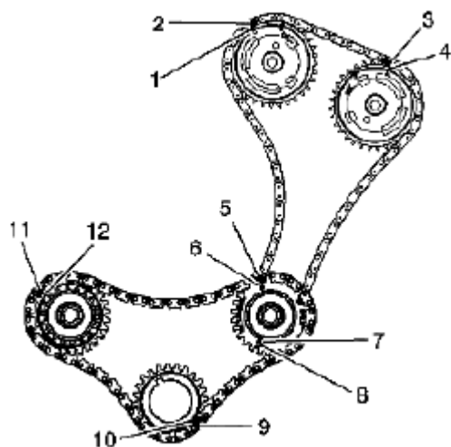
Fig. 879: Identifying Left Secondary Camshaft Drive Chain Timing Mark Courtesy of SUZUKI OF AMERICA CORP.
