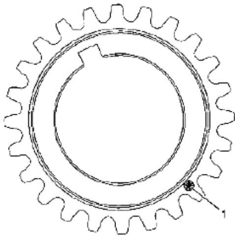
Fig. 795: Identifying Crankshaft Sprocket Timing Mark Courtesy of SUZUKI OF AMERICA CORP.
