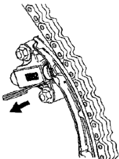
Fig. 937: Pulling EN 46112 From Right Camshaft Drive Chain Tensioner Courtesy of SUZUKI OF AMERICA CORP.
