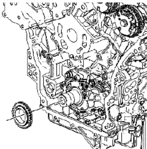
Fig. 349: Identifying Crankshaft Sprocket Courtesy of SUZUKI OF AMERICA CORP.
