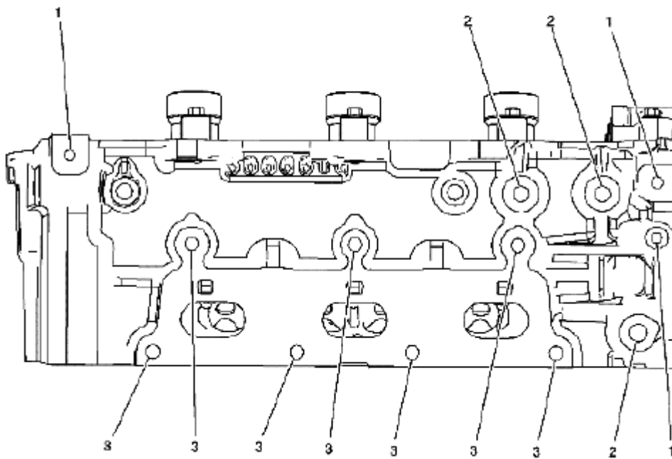
Fig. 1020: Identifying Right Cylinder Head Exhaust Face
