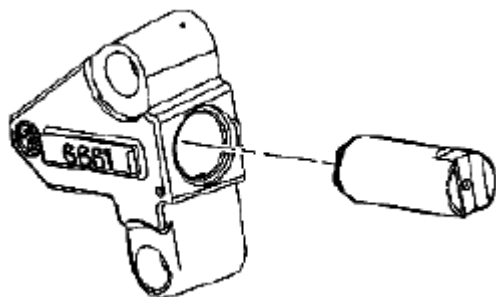
Fig. 842: Identifying Plunger & Left Secondary Camshaft Drive Chain Tensioner Body Courtesy of SUZUKI OF AMERICA CORP.
