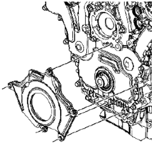
Fig. 293: Identifying Engine Front Cover Deadener Courtesy of SUZUKI OF AMERICA CORP.
