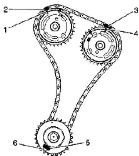
Fig. 178: Identifying Timing Chain Mark Courtesy of SUZUKI OF AMERICA CORP.
