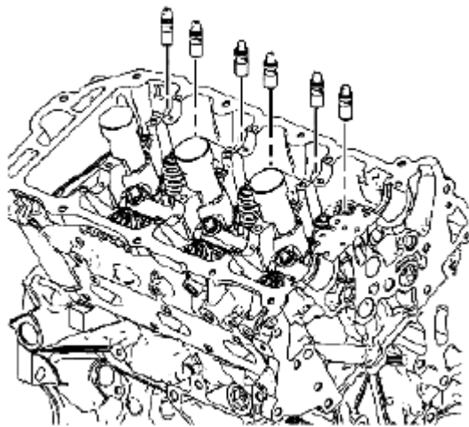
Fig. 745: Identifying SHLA In Cylinder Head Courtesy of SUZUKI OF AMERICA CORP.
