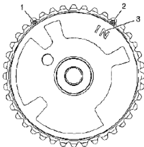
Fig. 778: Identifying Timing Mark Courtesy of SUZUKI OF AMERICA CORP.
