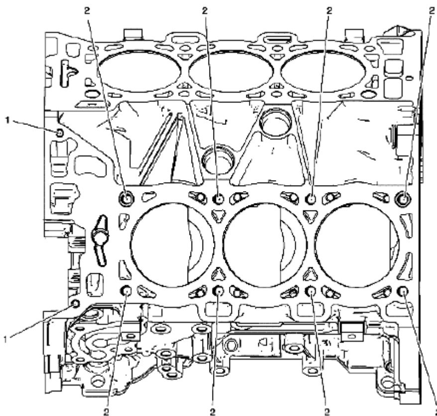
Fig. 1027: Identifying Engine Block Left Deck Face Courtesy of SUZUKI OF AMERICA CORP.
