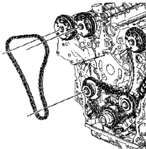
Fig. 321: Identifying Right Secondary Camshaft Drive Chain Courtesy of SUZUKI OF AMERICA CORP.
