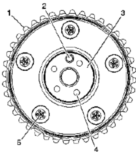
Fig. 502: Identifying Back Of Exhaust Camshaft Position Actuators
