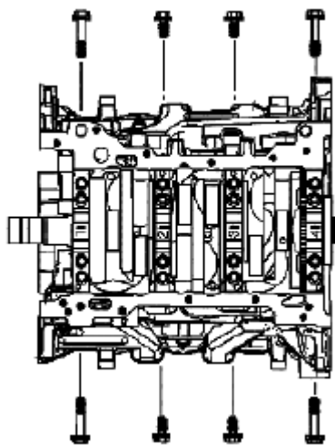
Fig. 383: Identifying Crankshaft Bearing Cap Side Bolts Courtesy of SUZUKI OF AMERICA CORP.
