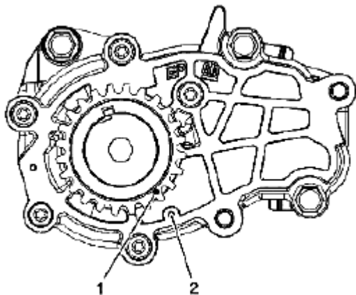
Fig. 806: Aligning Timing Mark On Crankshaft Sprocket Timing Mark & Oil Pump Cover Courtesy of SUZUKI OF AMERICA CORP.
