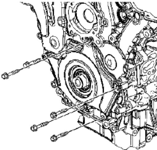
Fig. 944: Identifying Engine Front Cover Bolts (1 Of 2) Courtesy of SUZUKI OF AMERICA CORP.
