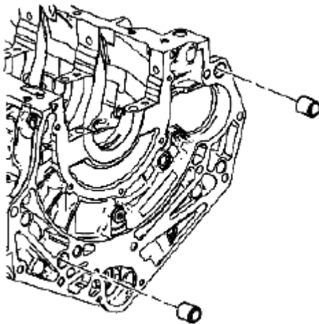
Fig. 690: Identifying Cylinder Block-To-Transmission Alignment Dowels Courtesy of SUZUKI OF AMERICA CORP.
