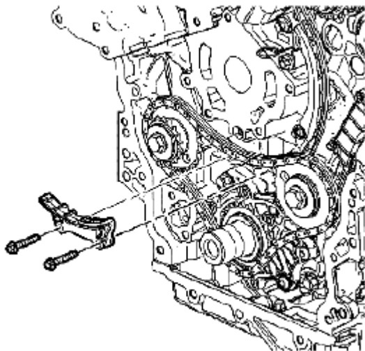
Fig. 159: Identifying Primary Upper Camshaft Drive Chain Guide Courtesy of SUZUKI OF AMERICA CORP.
