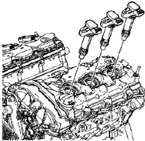
Fig. 281: Identifying Ignition Coils Courtesy of SUZUKI OF AMERICA CORP.
