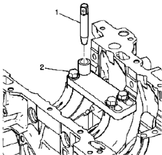
Fig. 659: Positioning Alignment Pin Through Bushing Courtesy of SUZUKI OF AMERICA CORP.
