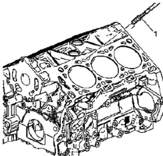
Fig. 655: Applying Insert & Installation Driver Into Tapped Hole By Hand Courtesy of SUZUKI OF AMERICA CORP.
