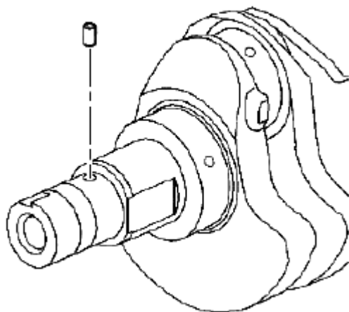
Fig. 386: Identifying Crankshaft Sprocket Drive Pin Courtesy of SUZUKI OF AMERICA CORP.
