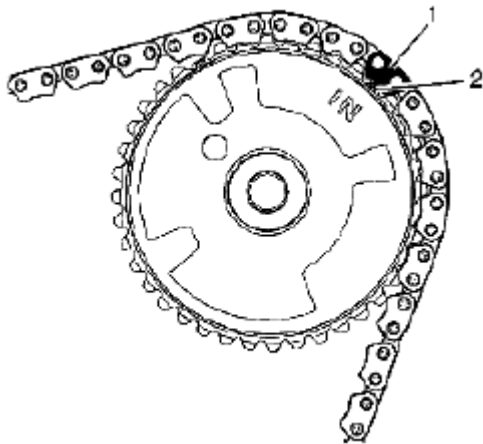
Fig. 909: Identifying Timing Camshaft Drive Chain Link Mark (4 Of 5) Courtesy of SUZUKI OF AMERICA CORP.
