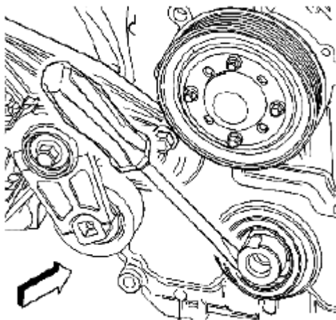
Fig. 97: Removing Crankshaft Oil Seal Using Flat-Bladed Tool Courtesy of SUZUKI OF AMERICA CORP.
