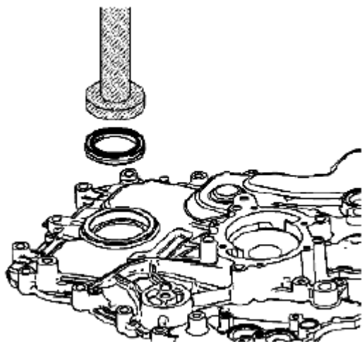
Fig. 98: Installing Crankshaft Front Oil Seal Courtesy of SUZUKI OF AMERICA CORP.
