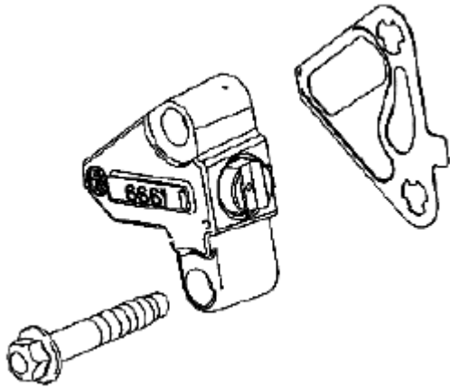
Fig. 844: Identifying Left Secondary Camshaft Drive Chain Tensioner, Gasket & Bolt Courtesy of SUZUKI OF AMERICA CORP.
