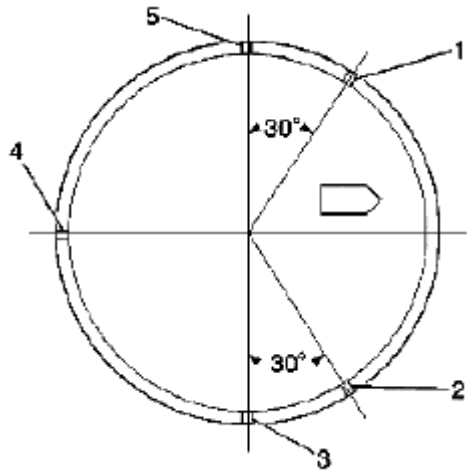
Fig. 436: Identifying Piston Rings Gap Direction Courtesy of SUZUKI OF AMERICA CORP.
