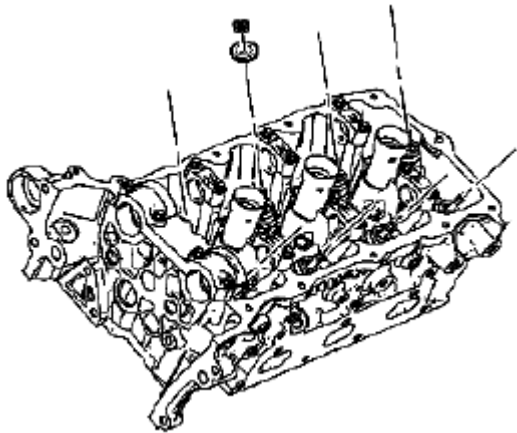
Fig. 197: Identifying Valve Spring Retainer Courtesy of SUZUKI OF AMERICA CORP.
