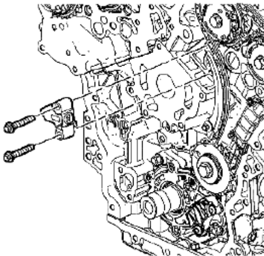
Fig. 131: Identifying Left Bank Secondary Camshaft Drive Chain Tensioner Courtesy of SUZUKI OF AMERICA CORP.
