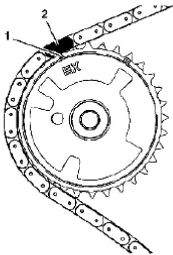
Fig. 901: Identifying Timing Camshaft Drive Chain Link Mark (3 Of 5) Courtesy of SUZUKI OF AMERICA CORP.
