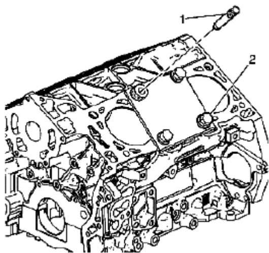
Fig. 643: Positioning Alignment Pin Through Bushing & Into Cylinder Head Bolt Hole Courtesy of SUZUKI OF AMERICA CORP.
