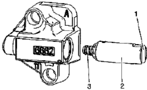
Fig. 500: Identifying Right Secondary Timing Chain Tensioner Courtesy of SUZUKI OF AMERICA CORP.
