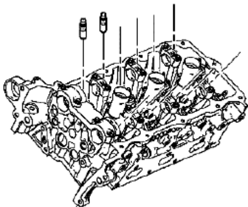
Fig. 193: Identifying Valve Lifters - Right Side Courtesy of SUZUKI OF AMERICA CORP.
