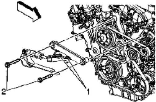
Fig. 66: Installing Engine Mount Strut Bracket To Cylinder Head Bolts Courtesy of SUZUKI OF AMERICA CORP.
