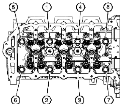
Fig. 743: Tightening M11 Cylinder Head Bolts Courtesy of SUZUKI OF AMERICA CORP.
