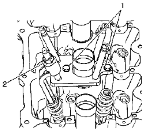
Fig. 202: Identifying Valve Spring Compressor Nut Courtesy of SUZUKI OF AMERICA CORP.
