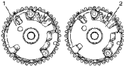
Fig. 787: Identifying Right Intake Camshaft Position Actuator & Left Intake Camshaft Position Actuator Courtesy of SUZUKI OF AMERICA CORP.
