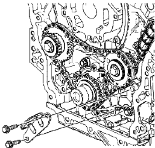
Fig. 329: Identifying Primary Camshaft Drive Chain Lower Guide & Bolts Courtesy of SUZUKI OF AMERICA CORP.
