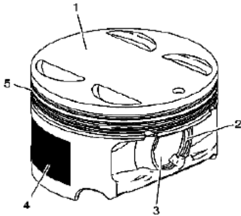
Fig. 420: Identifying Piston Inspection Points Courtesy of SUZUKI OF AMERICA CORP.
