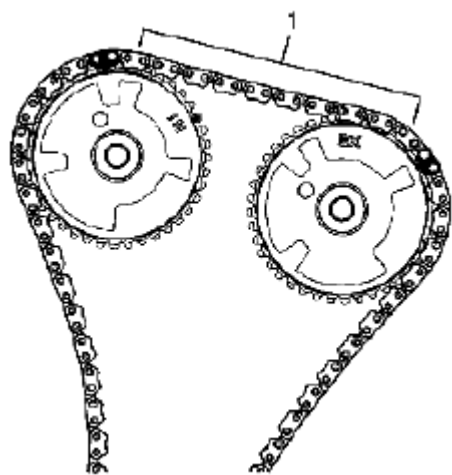
Fig. 817: Identifying Timing Camshaft Drive Chain Link Mark (1 Of 4) Courtesy of SUZUKI OF AMERICA CORP.
