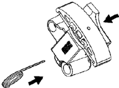
Fig. 887: Inserting EN 46112 Into Access Hole Of Primary Camshaft Drive Chain Tensioner Body Courtesy of SUZUKI OF AMERICA CORP.
