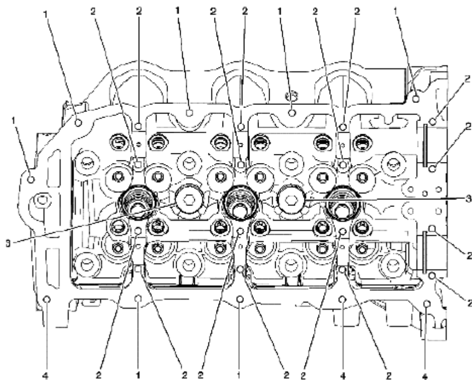
Fig. 1017: Identifying Right Cylinder Head Camshaft Cover Face Courtesy of SUZUKI OF AMERICA CORP.
