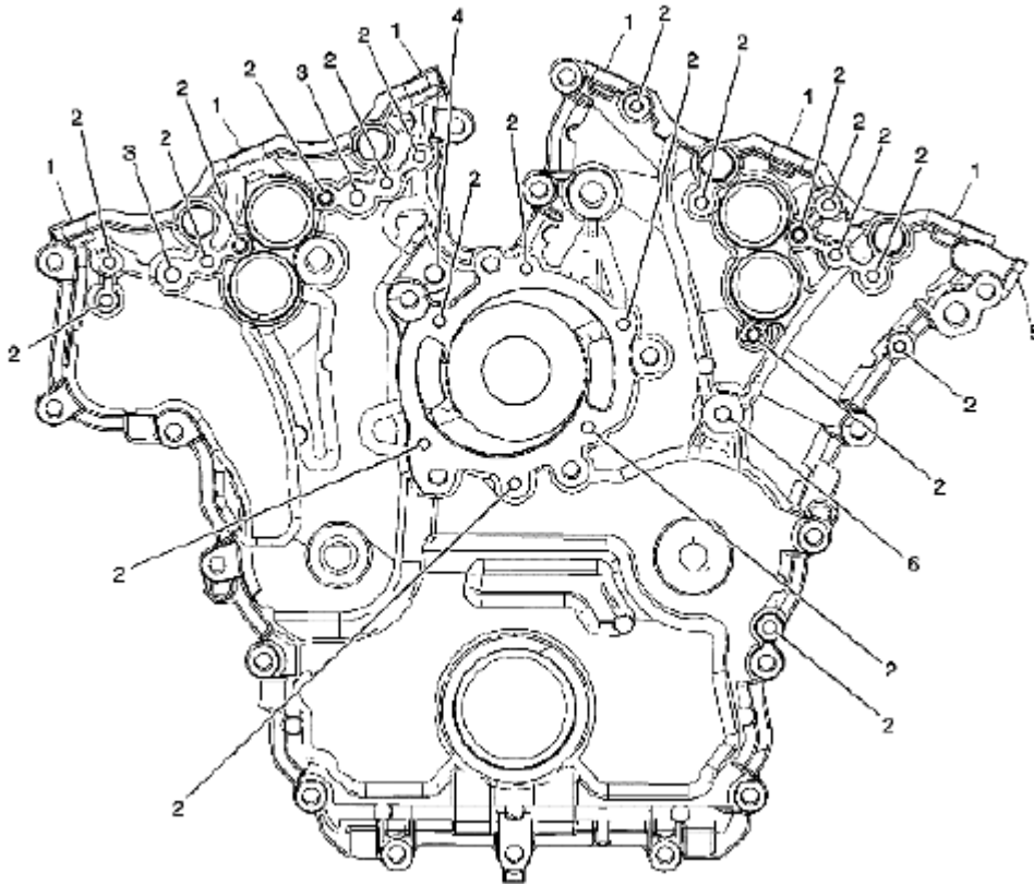
Fig. 1029: Identifying Engine Front Cover Courtesy of SUZUKI OF AMERICA CORP.
