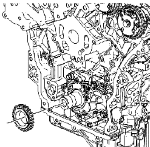
Fig. 348: Identifying Crankshaft Sprocket Courtesy of SUZUKI OF AMERICA CORP.
