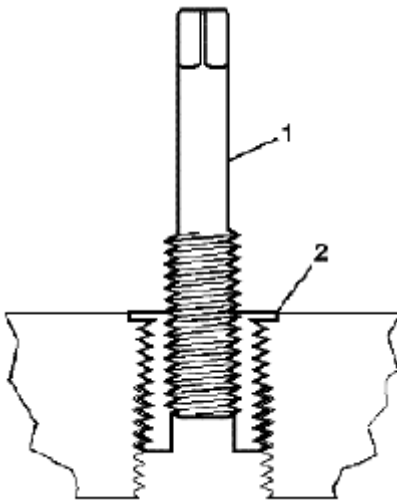
Fig. 605: Applying Insert Into Tapped Hole (2 Of 3) Courtesy of SUZUKI OF AMERICA CORP.
