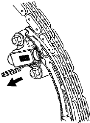
Fig. 928: Pulling EN 46112 From Right Camshaft Drive Chain Tensioner Courtesy of SUZUKI OF AMERICA CORP.
