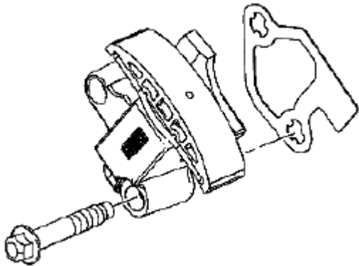
Fig. 323: Identifying Primary Camshaft Drive Chain Tensioner Gasket Courtesy of SUZUKI OF AMERICA CORP.
