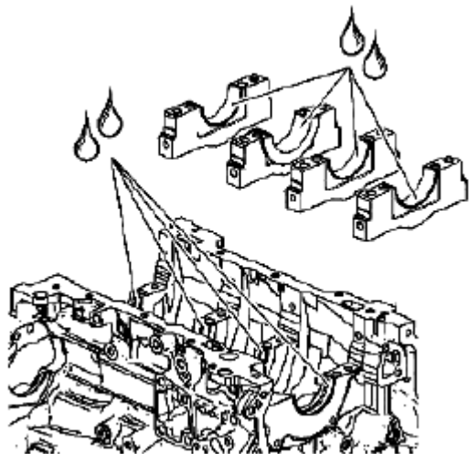
Fig. 715: Applying Liberal Amount Of Crankshaft Prelube To Upper & Lower Bearing Surfaces Courtesy of SUZUKI OF AMERICA CORP.
