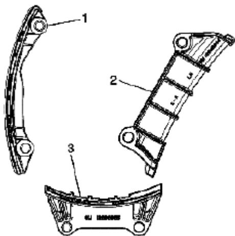
Fig. 821: Identifying Left Secondary Camshaft Drive Chain Guide Courtesy of SUZUKI OF AMERICA CORP.
