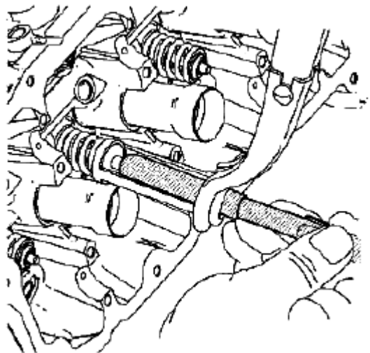
Fig. 467: Compressing Valve Springs Courtesy of SUZUKI OF AMERICA CORP.
