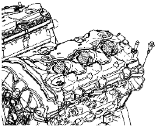
Fig. 964: Identifying Left Camshaft Cover Bolts Courtesy of SUZUKI OF AMERICA CORP.
