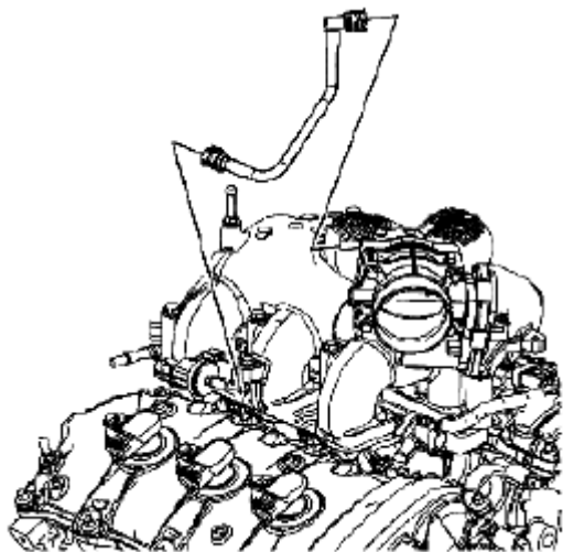
Fig. 987: Identifying Intake Manifold-To-Solenoid EVAP Hose Courtesy of SUZUKI OF AMERICA CORP.
