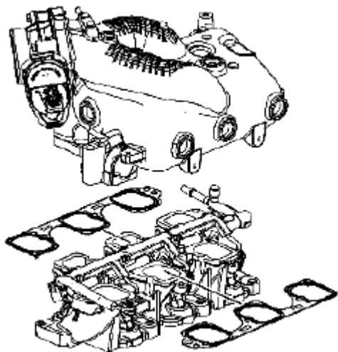
Fig. 561: Identifying Upper-To-Lower Intake Manifold Gaskets Courtesy of SUZUKI OF AMERICA CORP.
