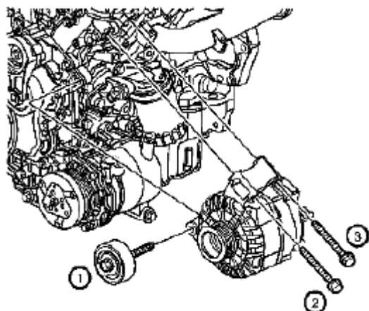
Fig. 44: Identifying Generator & Idler Pulley Bolt Courtesy of SUZUKI OF AMERICA CORP.
