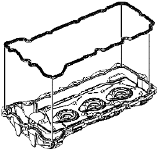
Fig. 552: Identifying Left Camshaft Cover Gasket Courtesy of SUZUKI OF AMERICA CORP.
