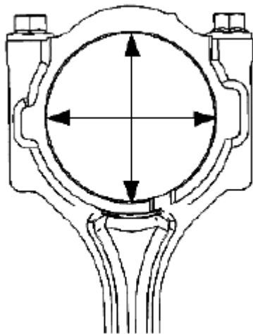
Fig. 430: Measuring Connecting Rod Crankshaft Bearing Bore
