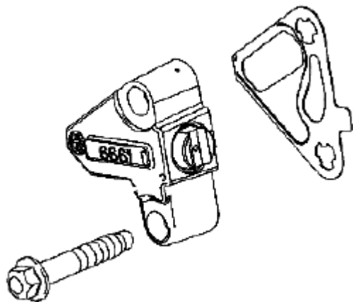
Fig. 835: Identifying Left Secondary Camshaft Drive Chain Tensioner, Gasket & Bolt Courtesy of SUZUKI OF AMERICA CORP.
