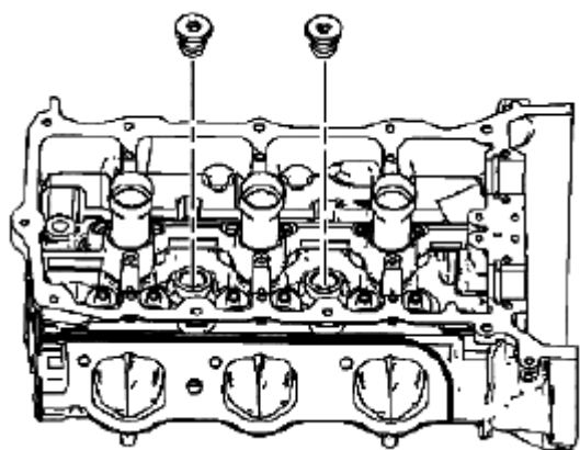
Fig. 446: Identifying Cylinder Head Coolant Threaded Plugs Courtesy of SUZUKI OF AMERICA CORP.
