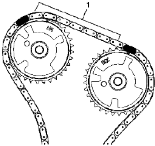
Fig. 809: Identifying Timing Camshaft Drive Chain Link Mark (1 Of 4) Courtesy of SUZUKI OF AMERICA CORP.
