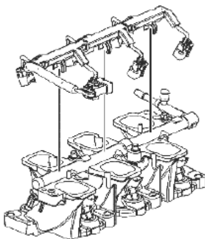
Fig. 566: Identifying Fuel Injector Wiring Harness Connectors Courtesy of SUZUKI OF AMERICA CORP.
