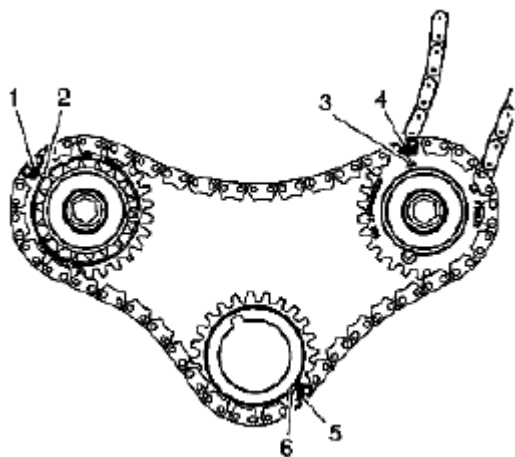
Fig. 858: Identifying Timing Camshaft Drive Chain Links Mark Courtesy of SUZUKI OF AMERICA CORP.
