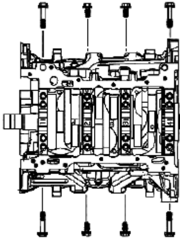
Fig. 706: Identifying Short/Inner Side Main Cap Bolts Courtesy of SUZUKI OF AMERICA CORP.
