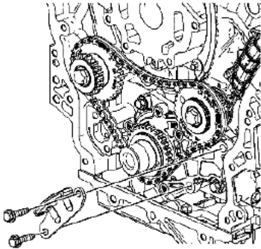
Fig. 866: Identifying Primary Camshaft Drive Chain Lower Guide & Bolts Courtesy of SUZUKI OF AMERICA CORP.
