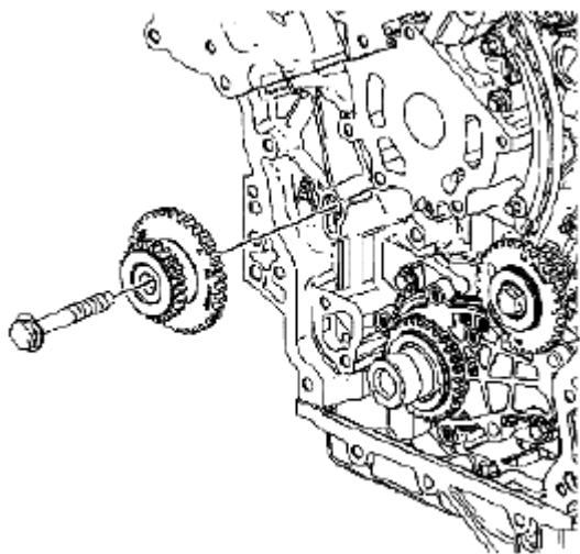
Fig. 333: Identifying Right Camshaft Intermediate Drive Chain Idler & Bolt Courtesy of SUZUKI OF AMERICA CORP.
