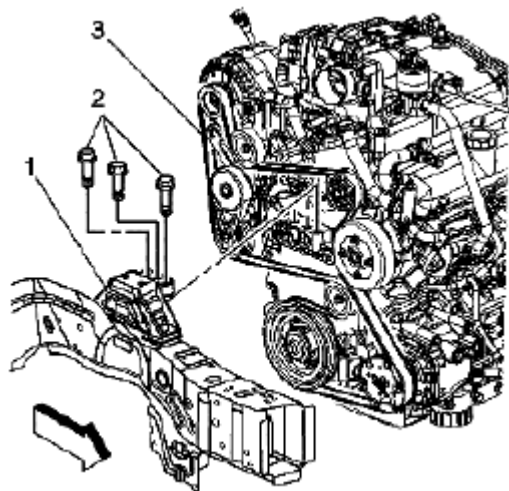
Fig. 233: Removing Right Engine Mount To Engine Courtesy of SUZUKI OF AMERICA CORP.
