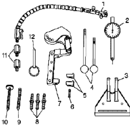
Fig. 730: Identifying J 43690 Rod Bearing Clearance Checking Tool Courtesy of SUZUKI OF AMERICA CORP.
