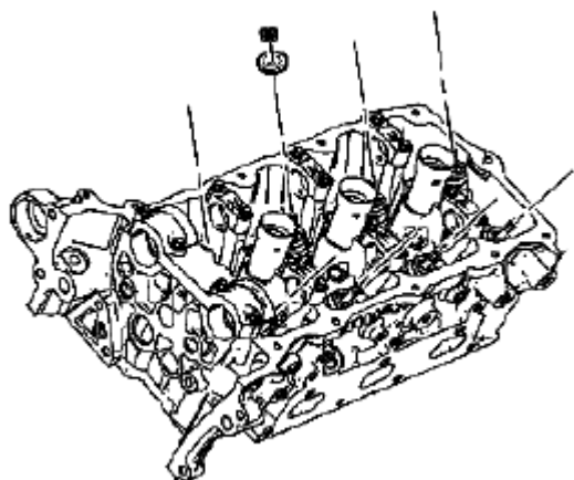
Fig. 212: Identifying Valve Spring Keepers Courtesy of SUZUKI OF AMERICA CORP.
