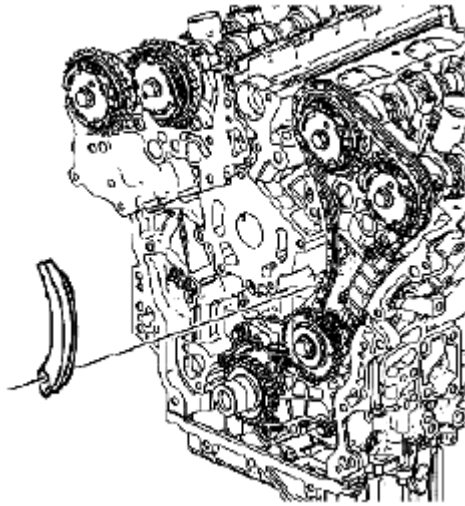
Fig. 136: Identifying Left Secondary Camshaft Drive Chain Shoe (1 Of 3) Courtesy of SUZUKI OF AMERICA CORP.
