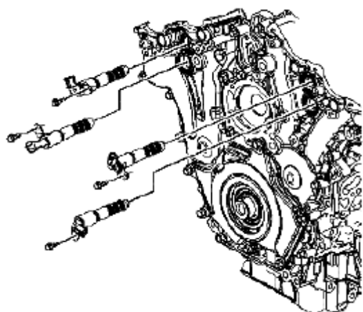
Fig. 947: Identifying Camshaft Position Actuator Valves Courtesy of SUZUKI OF AMERICA CORP.
