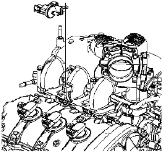
Fig. 985: Identifying Evaporative Emissions (EVAP) Solenoid Courtesy of SUZUKI OF AMERICA CORP.
