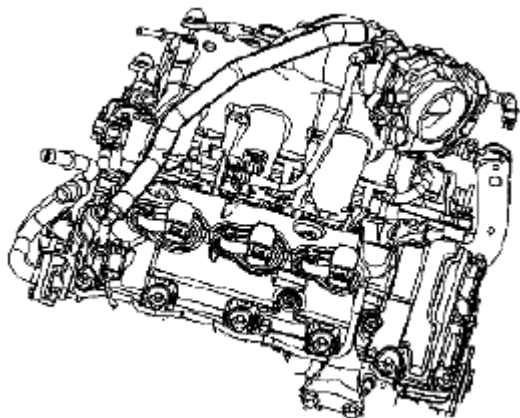
Fig. 72: Identifying Positive Crankcase Ventilation (PVC) Fresh Air Pipe (2 Of 2) Courtesy of SUZUKI OF AMERICA CORP.
