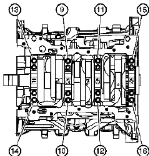
Fig. 709: Tightening Outboard Bolts In Sequence Courtesy of SUZUKI OF AMERICA CORP.
