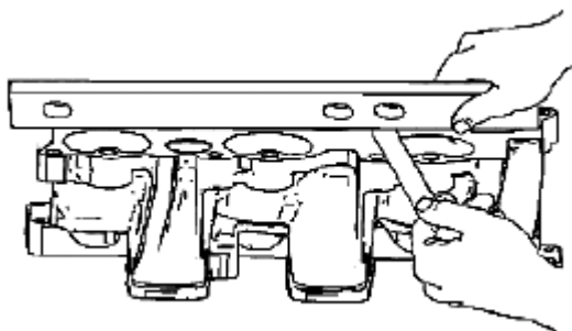
Fig. 576: Checking Lower Intake Manifold Sealing Surfaces For Warpage Courtesy of SUZUKI OF AMERICA CORP.
