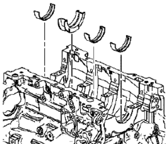
Fig. 700: Identifying Upper Crankshaft Bearings Courtesy of SUZUKI OF AMERICA CORP.
