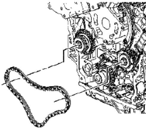
Fig. 853: Identifying Primary Camshaft Drive Chain Courtesy of SUZUKI OF AMERICA CORP.
