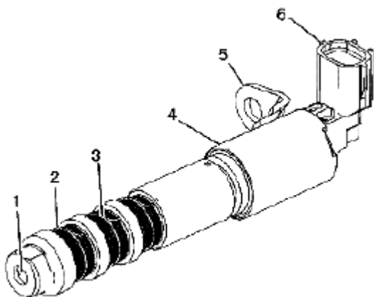
Fig. 482: Identifying Camshaft Position Actuator Oil Control Valves Courtesy of SUZUKI OF AMERICA CORP.
