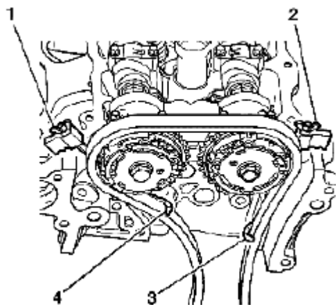
Fig. 177: Identifying Timing Chain Courtesy of SUZUKI OF AMERICA CORP.
