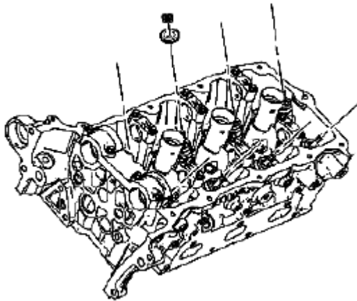
Fig. 206: Identifying Valve Keepers Courtesy of SUZUKI OF AMERICA CORP.
