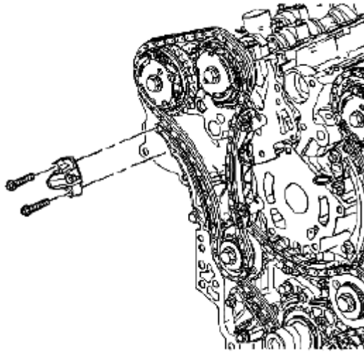
Fig. 133: Identifying Right Bank Secondary Camshaft Drive Chain Tensioner Courtesy of SUZUKI OF AMERICA CORP.
