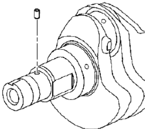
Fig. 702: Identifying Crankshaft Sprocket Drive Pin Courtesy of SUZUKI OF AMERICA CORP.
