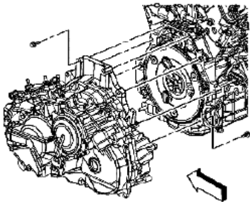
Fig. 242: Separating Automatic Transaxle From Engine Courtesy of SUZUKI OF AMERICA CORP.
