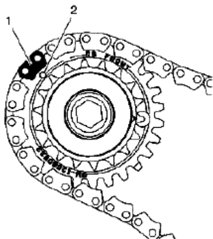
Fig. 856: Identifying Right Camshaft Intermediate Drive Chain Idler Timing Mark Courtesy of SUZUKI OF AMERICA CORP.
