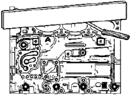
Fig. 403: Checking Deck Flatness
