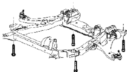
Fig. 234: Identifying Frame-To-Body Bolts Courtesy of SUZUKI OF AMERICA CORP.
