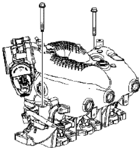
Fig. 559: Identifying Upper-To-Lower Intake Manifold Bolts Courtesy of SUZUKI OF AMERICA CORP.
