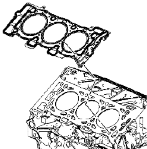
Fig. 373: Identifying Right Cylinder Head Gasket Courtesy of SUZUKI OF AMERICA CORP.
