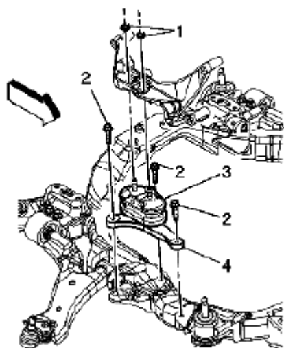
Fig. 52: Installing Engine Mount To Lower Bracket Courtesy of SUZUKI OF AMERICA CORP.
