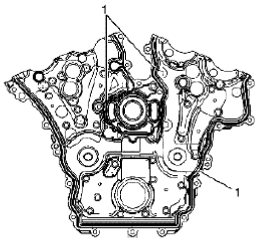
Fig. 529: Identifying RTV Sealant On Engine Front Cover Courtesy of SUZUKI OF AMERICA CORP.
