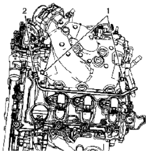
Fig. 77: Identifying Bleed Pipe Bolts Courtesy of SUZUKI OF AMERICA CORP.
