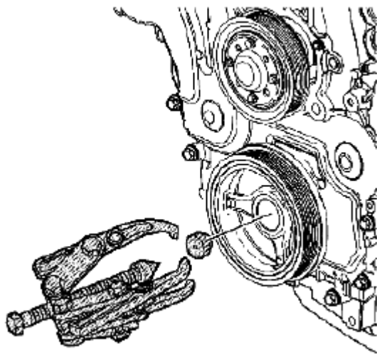
Fig. 91: Identifying Special Tool (J 41816) Courtesy of SUZUKI OF AMERICA CORP.
