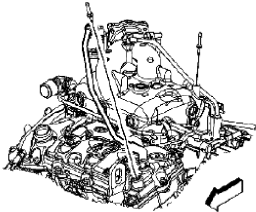
Fig. 73: Identifying Fresh Air Positive Crankcase Ventilation (PCV) Line Courtesy of SUZUKI OF AMERICA CORP.
