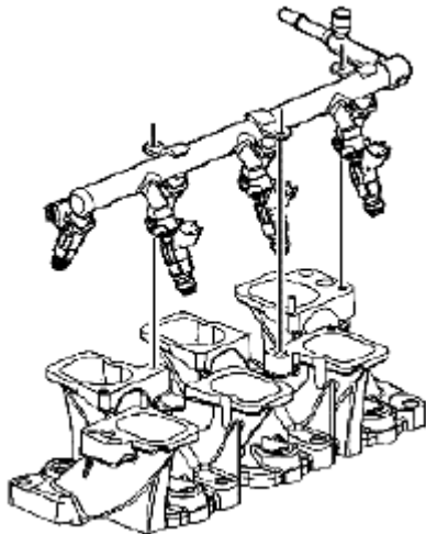
Fig. 568: Identifying Fuel Injector Rail Courtesy of SUZUKI OF AMERICA CORP.
