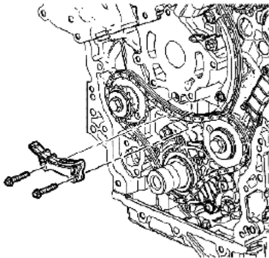
Fig. 158: Identifying Primary Upper Camshaft Drive Chain Guide Courtesy of SUZUKI OF AMERICA CORP.
