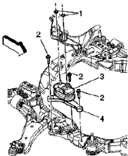
Fig. 60: Installing Engine Mount & Lower Bracket Courtesy of SUZUKI OF AMERICA CORP.
