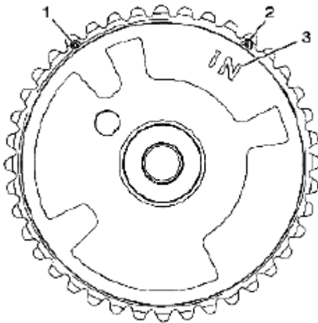
Fig. 789: Identifying Timing Mark Courtesy of SUZUKI OF AMERICA CORP.
