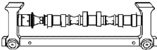
Fig. 469: Securing Camshaft In Suitable Fixture Courtesy of SUZUKI OF AMERICA CORP.
