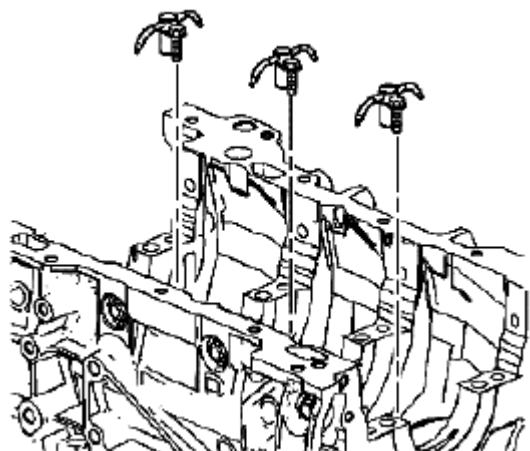
Fig. 699: Identifying Oil Jets
