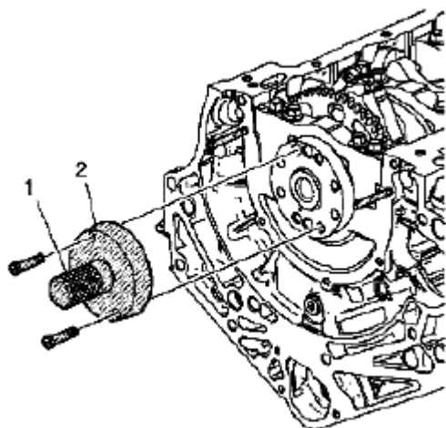
Fig. 735: Identifying Special Tool (EN-47839) Courtesy of SUZUKI OF AMERICA CORP.
