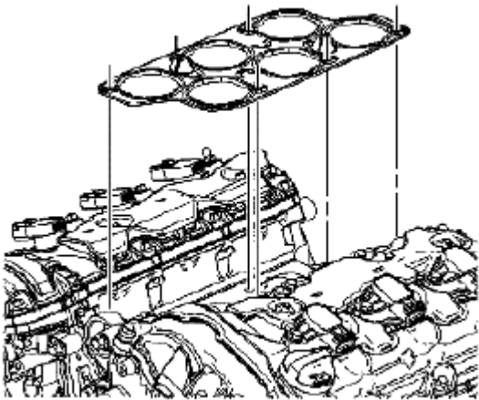
Fig. 981: Identifying Lower Intake Manifold Gasket Courtesy of SUZUKI OF AMERICA CORP.
