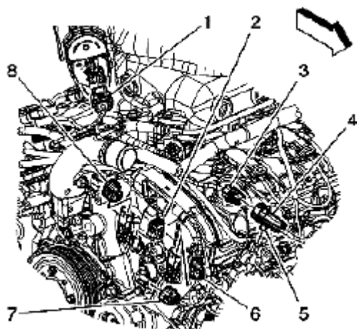
Fig. 34: Engine Wiring Harness Electrical Connectors Courtesy of SUZUKI OF AMERICA CORP.
