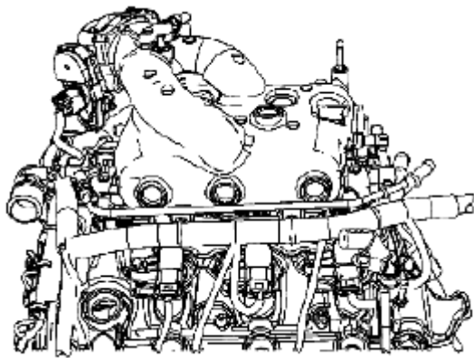
Fig. 85: Connecting ETC Electrical Connector Courtesy of SUZUKI OF AMERICA CORP.
