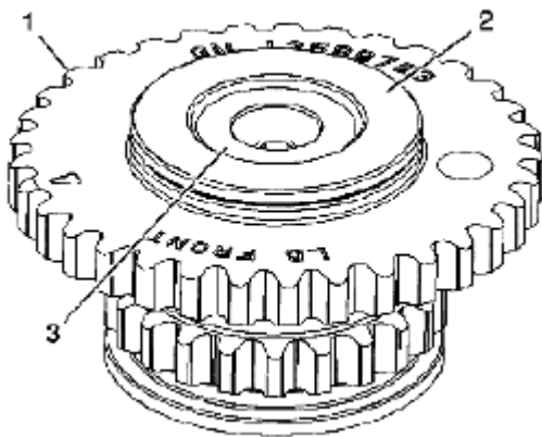
Fig. 508: Identifying Front Of Left Intermediate Sprocket Courtesy of SUZUKI OF AMERICA CORP.
