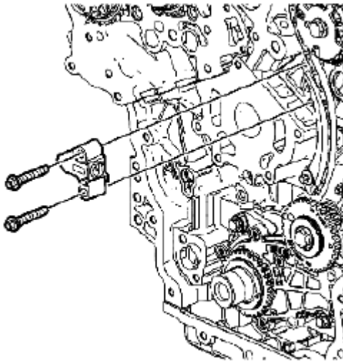
Fig. 336: Identifying Left Secondary Camshaft Drive Chain Tensioner And Bolts Courtesy of SUZUKI OF AMERICA CORP.
