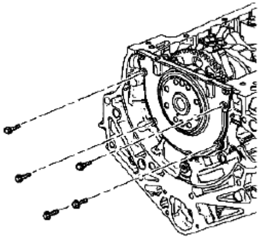
Fig. 226: Identifying Crankshaft Rear Oil Seal & Housing (2 Of 2) Courtesy of SUZUKI OF AMERICA CORP.
