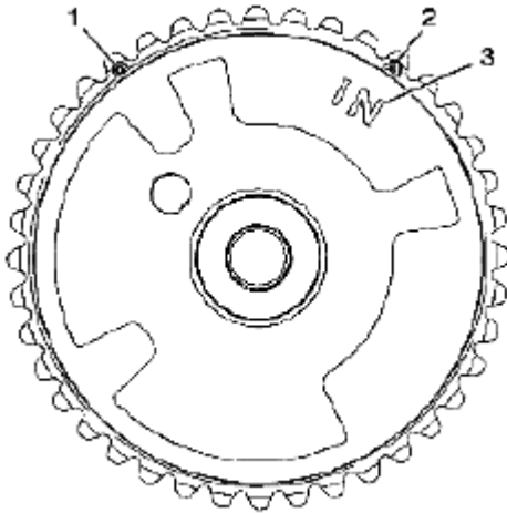
Fig. 786: Identifying Timing Mark Courtesy of SUZUKI OF AMERICA CORP.
