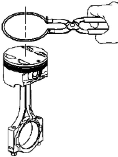
Fig. 417: Removing Piston Rings Using Piston Ring Expander Courtesy of SUZUKI OF AMERICA CORP.
