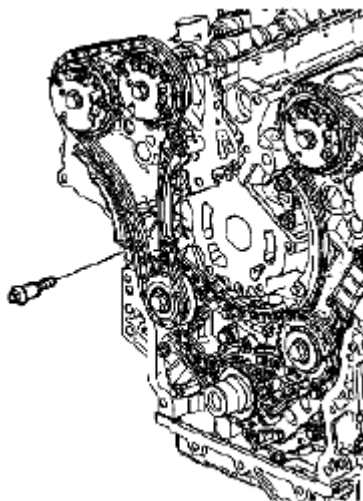
Fig. 917: Identifying Secondary Camshaft Drive Chain Shoe Bolt Courtesy of SUZUKI OF AMERICA CORP.
