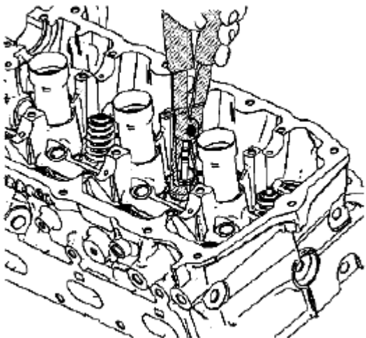
Fig. 444: Identifying Valve Stem Oil Seal Courtesy of SUZUKI OF AMERICA CORP.
