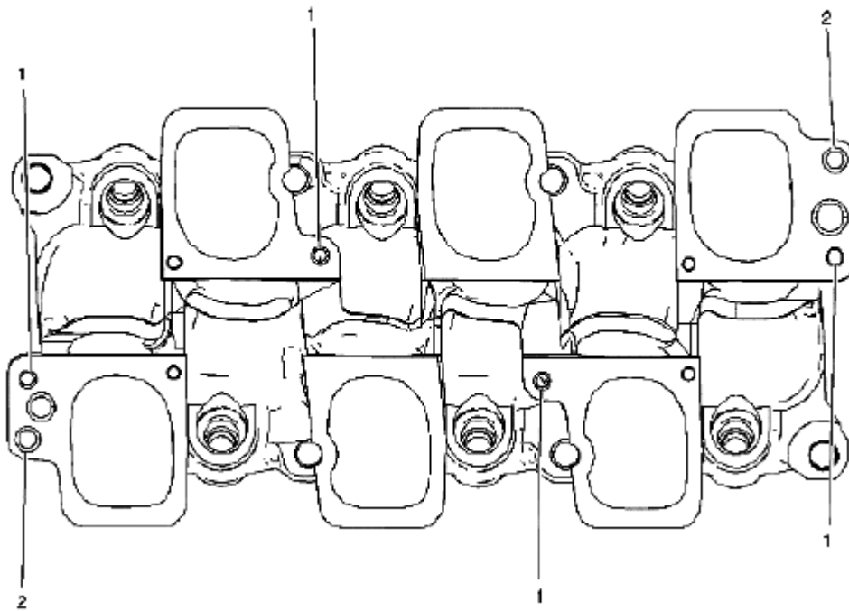
Fig. 1032: Identifying Lower Intake Manifold - Top Courtesy of SUZUKI OF AMERICA CORP.
