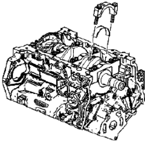
Fig. 728: Identifying Connecting Rod Cap Courtesy of SUZUKI OF AMERICA CORP.
