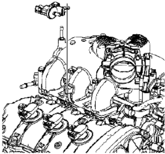
Fig. 275: Identifying EVAP Solenoid Courtesy of SUZUKI OF AMERICA CORP.
