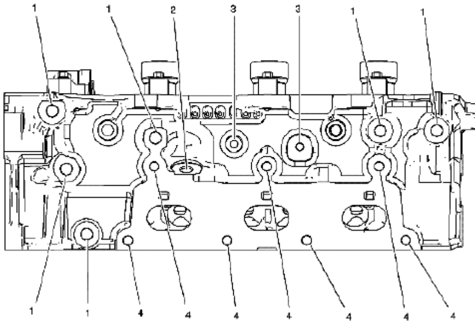
Fig. 1015: Identifying Left Cylinder Head Exhaust Face Courtesy of SUZUKI OF AMERICA CORP.
