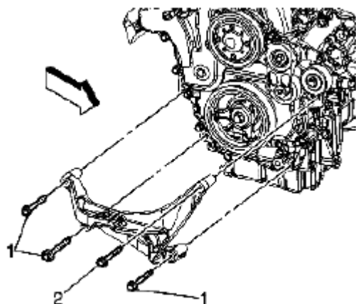
Fig. 55: Installing Right Upper Engine Mount Bracket Bolt Courtesy of SUZUKI OF AMERICA CORP.
