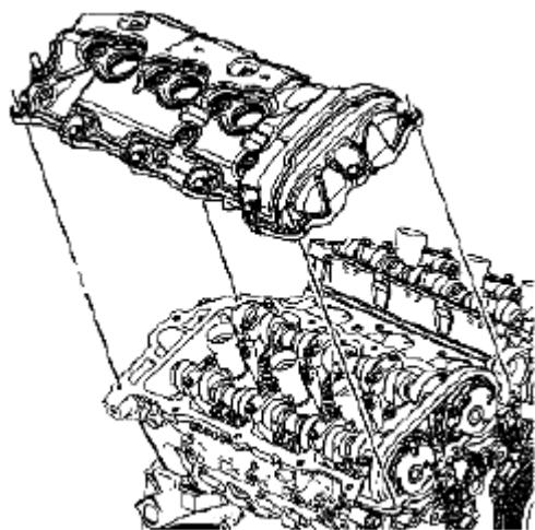
Fig. 289: Identifying Right Camshaft Cover Courtesy of SUZUKI OF AMERICA CORP.
