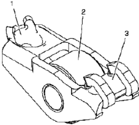
Fig. 762: Identifying Camshaft Followers (1 Of 2) Courtesy of SUZUKI OF AMERICA CORP.
