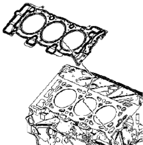
Fig. 741: Identifying Right Cylinder Head Gasket Courtesy of SUZUKI OF AMERICA CORP.
