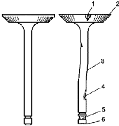
Fig. 453: Identifying Damage Valve Courtesy of SUZUKI OF AMERICA CORP.
