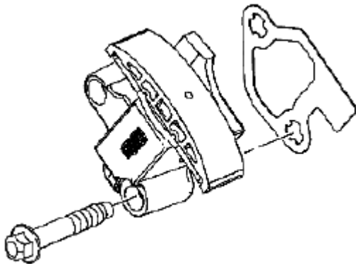
Fig. 875: Identifying Primary Camshaft Drive Chain Tensioner, Gasket & Bolt Courtesy of SUZUKI OF AMERICA CORP.
