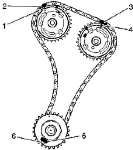
Fig. 161: Identifying Camshaft Timing Chain Mark Courtesy of SUZUKI OF AMERICA CORP.
