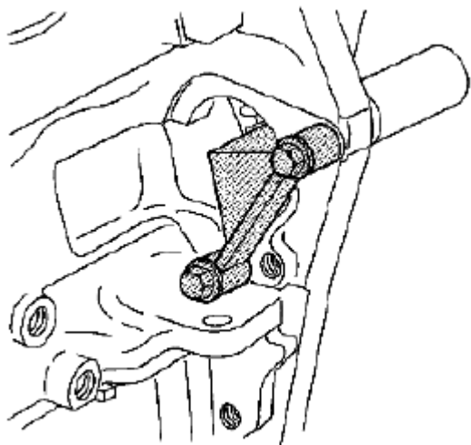
Fig. 92: Installing EN 46106 Through Starter Mounting Hole Courtesy of SUZUKI OF AMERICA CORP.
