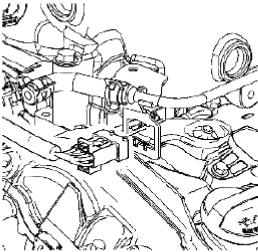
Fig. 990: Identifying Fuel Injector Harness Connector Courtesy of SUZUKI OF AMERICA CORP.
