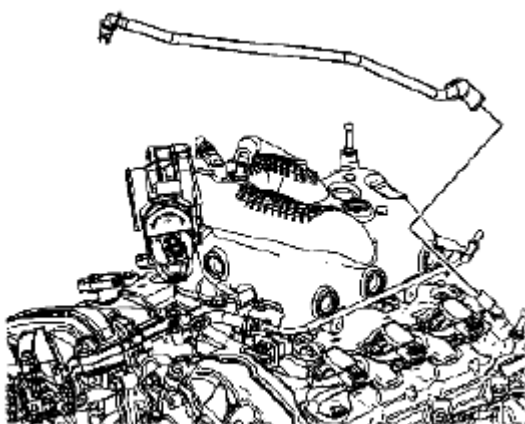
Fig. 992: Identifying Fresh Air PCV Hose Courtesy of SUZUKI OF AMERICA CORP.
