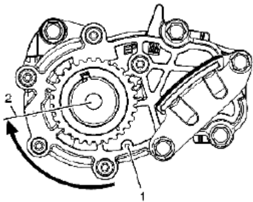
Fig. 894: Identifying Crankshaft Sprocket Mark Courtesy of SUZUKI OF AMERICA CORP.
