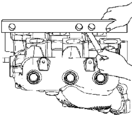
Fig. 573: Checking Upper Intake Manifold Sealing Surface For Warpage Courtesy of SUZUKI OF AMERICA CORP.
