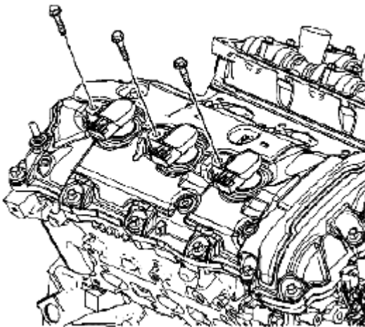
Fig. 980: Identifying Ignition Coil Bolts Courtesy of SUZUKI OF AMERICA CORP.
