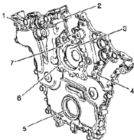
Fig. 530: Identifying Engine Front Cover Courtesy of SUZUKI OF AMERICA CORP.
