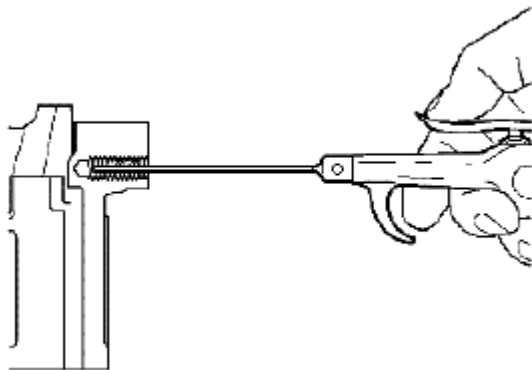
Fig. 627: Applying Compressed Air Into Tapped Hole Courtesy of SUZUKI OF AMERICA CORP.
