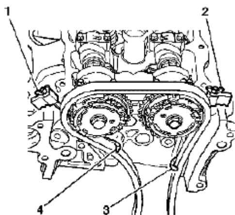
Fig. 183: Identifying Timing Chain Courtesy of SUZUKI OF AMERICA CORP.
