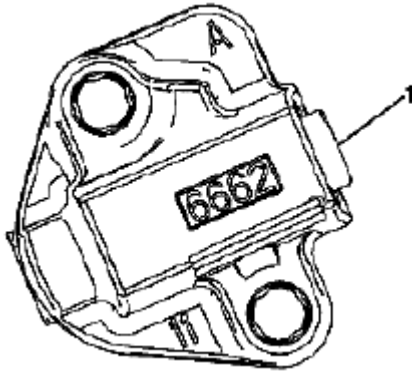
Fig. 927: Identifying Right Secondary Camshaft Drive Chain Tensioner Gasket Tab Courtesy of SUZUKI OF AMERICA CORP.
