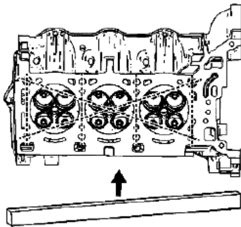
Fig. 450: Checking Deck Flatness Courtesy of SUZUKI OF AMERICA CORP.
