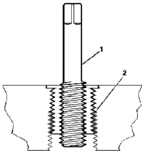
Fig. 606: Applying Insert Into Tapped Hole (3 Of 3) Courtesy of SUZUKI OF AMERICA CORP.
