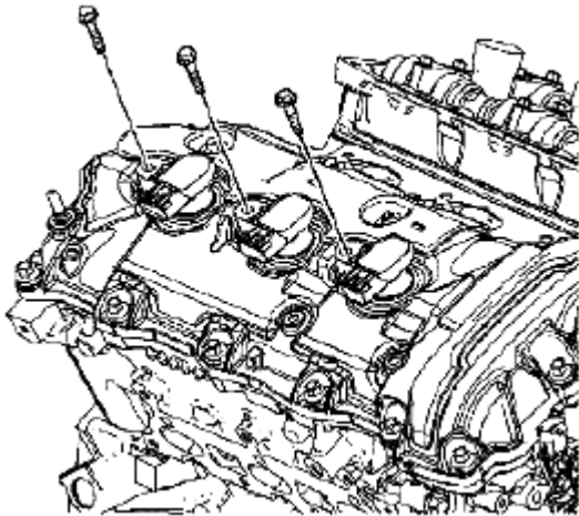
Fig. 285: Identifying Ignition Coil Bolts Courtesy of SUZUKI OF AMERICA CORP.
