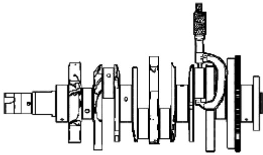
Fig. 412: Checking Crankpins For Undersize Courtesy of SUZUKI OF AMERICA CORP.
