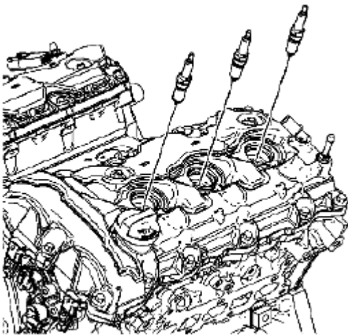
Fig. 282: Identifying Spark Plugs Courtesy of SUZUKI OF AMERICA CORP.
