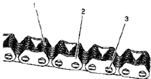
Fig. 514: Identifying Primary Timing Chain Courtesy of SUZUKI OF AMERICA CORP.
