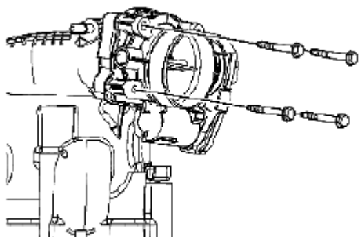
Fig. 562: Identifying Throttle Body Bolts Courtesy of SUZUKI OF AMERICA CORP.
