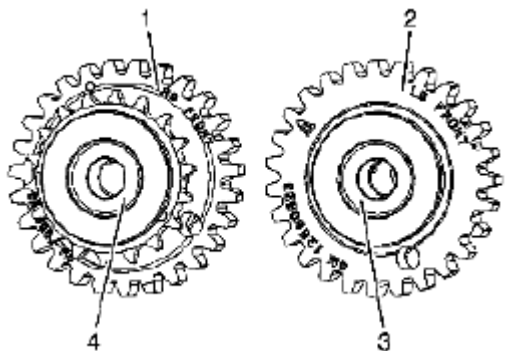
Fig. 849: Identifying Right Camshaft Intermediate Drive Chain Idler Courtesy of SUZUKI OF AMERICA CORP.
