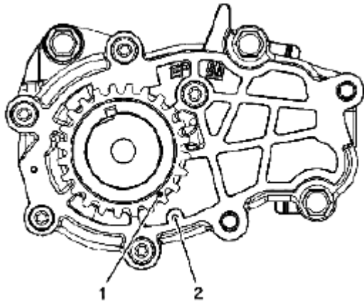
Fig. 150: Identifying Crankshaft Sprocket Timing Mark Courtesy of SUZUKI OF AMERICA CORP.
