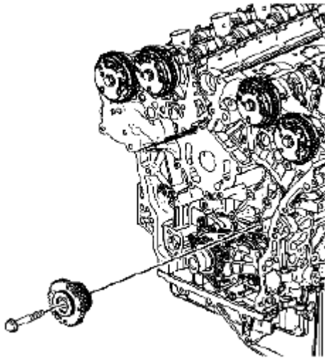
Fig. 804: Identifying Camshaft Intermediate Drive Chain Idler & Bolt Courtesy of SUZUKI OF AMERICA CORP.
