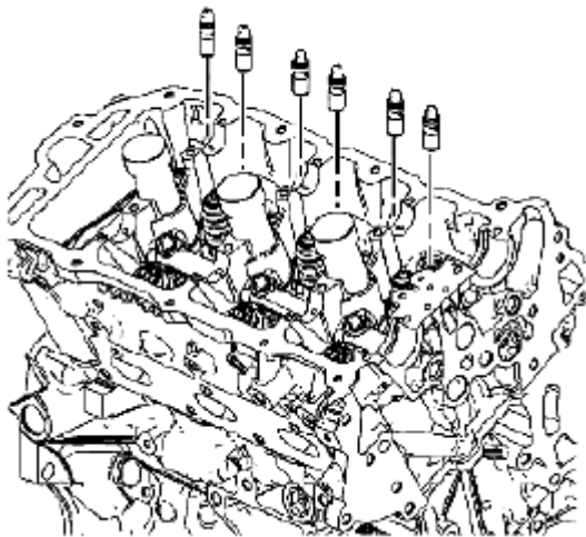
Fig. 191: Identifying Valve Lifters - Left Side
