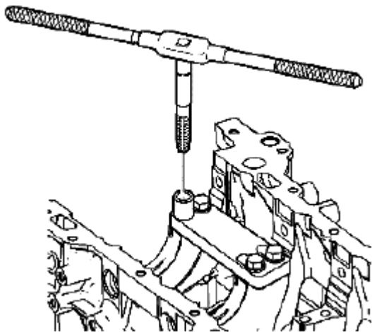
Fig. 677: Applying Threads Of Drilled Hole By Hand Courtesy of SUZUKI OF AMERICA CORP.
