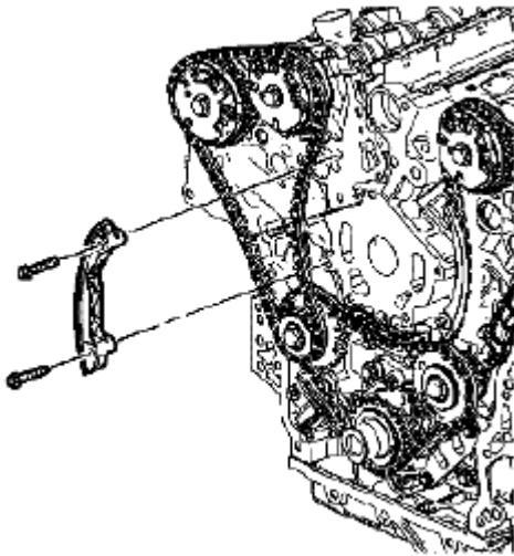
Fig. 914: Identifying Secondary Camshaft Drive Chain Guide & Bolts Courtesy of SUZUKI OF AMERICA CORP.
