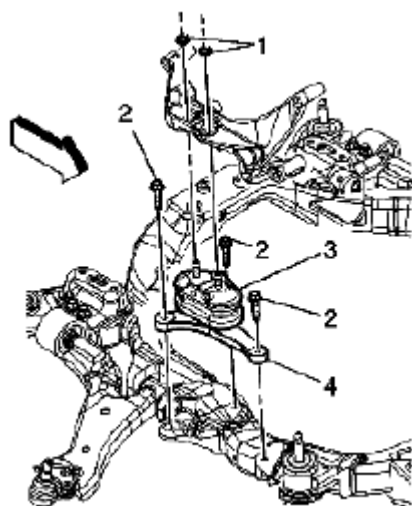
Fig. 54: Installing Lower Bracket Bolts Courtesy of SUZUKI OF AMERICA CORP.
