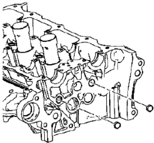
Fig. 461: Identifying Cylinder Head Oil Gallery Expansion Plugs Courtesy of SUZUKI OF AMERICA CORP.
