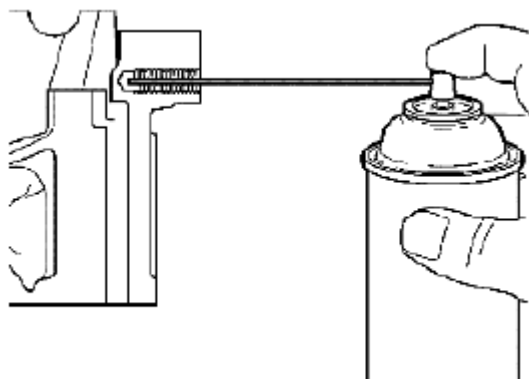
Fig. 680: Applying Spray Cleaner Into Tapped Hole Courtesy of SUZUKI OF AMERICA CORP.
