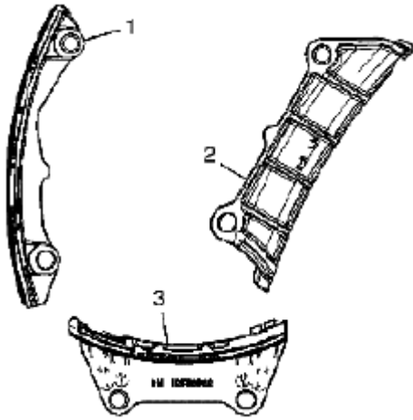
Fig. 913: Identifying Right Secondary Camshaft Drive Chain Guide Courtesy of SUZUKI OF AMERICA CORP.
