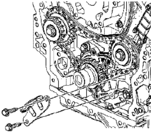
Fig. 865: Identifying Primary Camshaft Drive Chain Lower Guide & Bolts Courtesy of SUZUKI OF AMERICA CORP.
