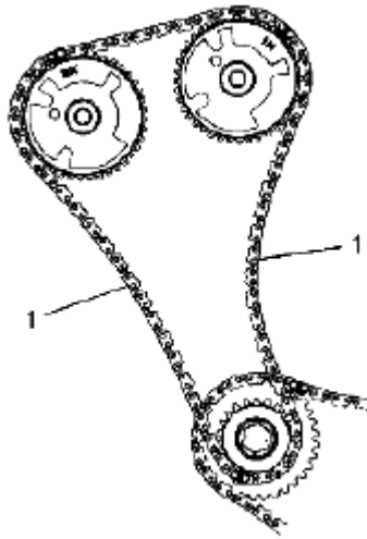
Fig. 910: Identifying Timing Camshaft Drive Chain Link Mark (5 Of 5)
