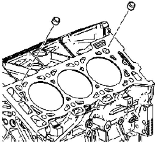
Fig. 688: Identifying Cylinder Block-To-Cylinder Head Alignment Dowels Courtesy of SUZUKI OF AMERICA CORP.
