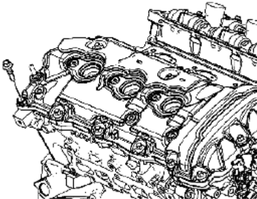
Fig. 288: Identifying Right Camshaft Cover Bolts Courtesy of SUZUKI OF AMERICA CORP.
