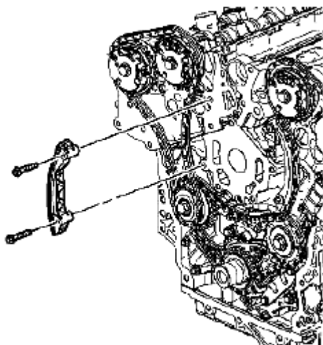
Fig. 318: Identifying Right Secondary Camshaft Drive Chain Guide & Bolts Courtesy of SUZUKI OF AMERICA CORP.
