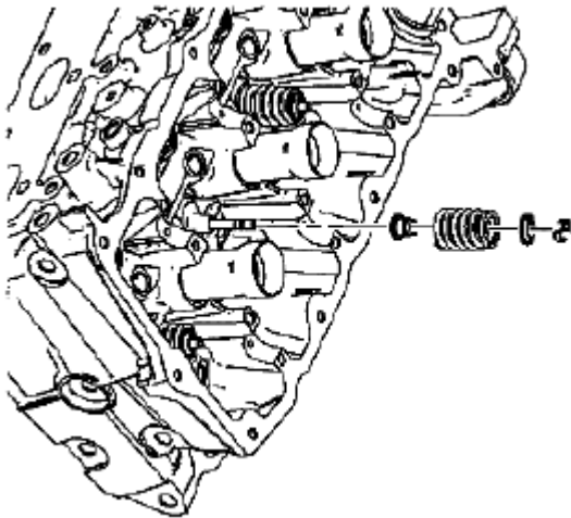
Fig. 464: Identifying Valve Spring & Valve Spring Retainer
