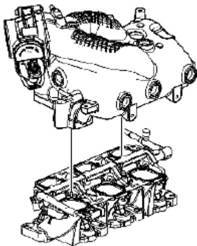
Fig. 586: Identifying Upper Intake Manifold Courtesy of SUZUKI OF AMERICA CORP.
