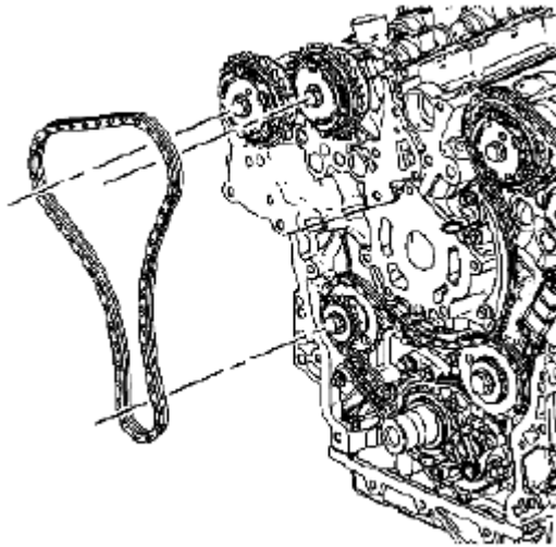
Fig. 129: Identifying Right Bank Secondary Camshaft Drive Chain Courtesy of SUZUKI OF AMERICA CORP.
