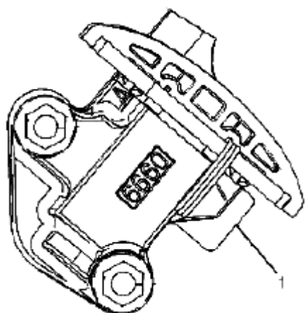
Fig. 890: Identifying Primary Camshaft Drive Chain Tensioner Gasket Tab Courtesy of SUZUKI OF AMERICA CORP.
