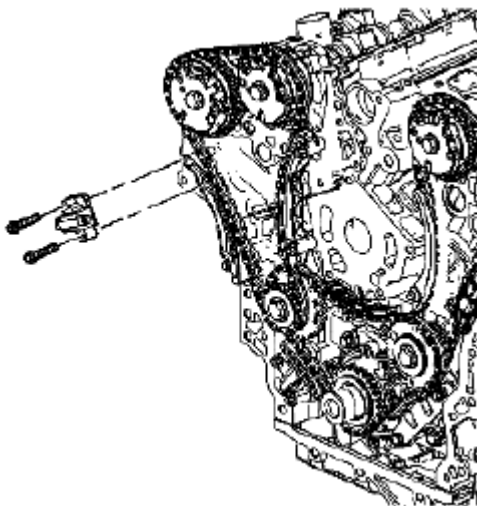
Fig. 312: Identifying Right Secondary Camshaft Drive Chain Tensioner & Bolts Courtesy of SUZUKI OF AMERICA CORP.
