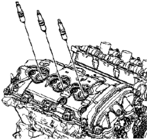
Fig. 287: Identifying Spark Plugs Courtesy of SUZUKI OF AMERICA CORP.
