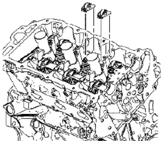
Fig. 188: Identifying Rocker Arms
