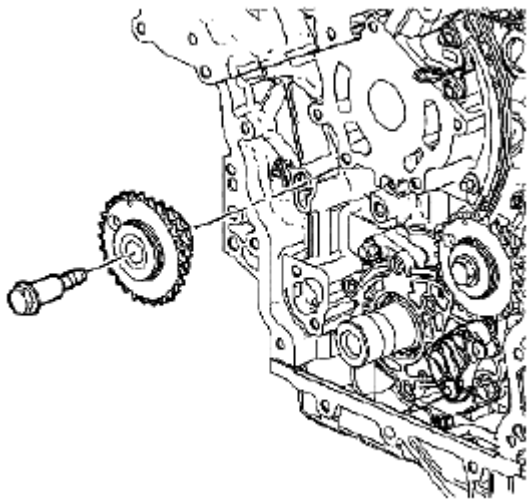
Fig. 153: Identifying Left Bank Camshaft Intermediate Drive Chain Idler Courtesy of SUZUKI OF AMERICA CORP.
