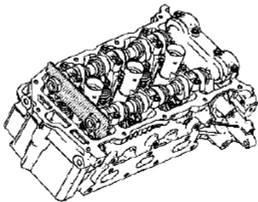
Fig. 883: Identifying EN 46105-1 Onto Rear Of Right Camshafts Courtesy of SUZUKI OF AMERICA CORP.
