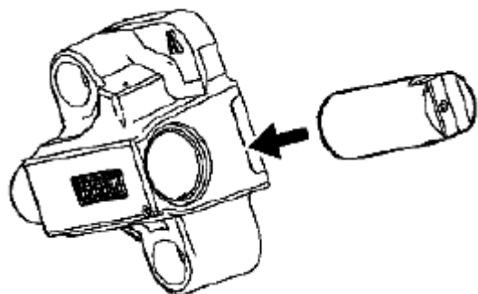
Fig. 932: Installing Plunger Into Right Secondary Camshaft Drive Chain Tensioner Body Courtesy of SUZUKI OF AMERICA CORP.
