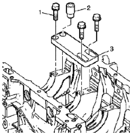
Fig. 658: Positioning Fixture Plate With Bushing Over Crankshaft Main Cap Bolt Hole Courtesy of SUZUKI OF AMERICA CORP.
