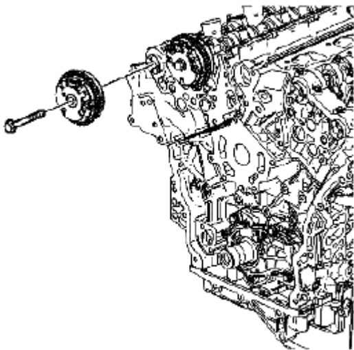
Fig. 783: Identifying Right Exhaust Camshaft Position Actuator & Bolt
