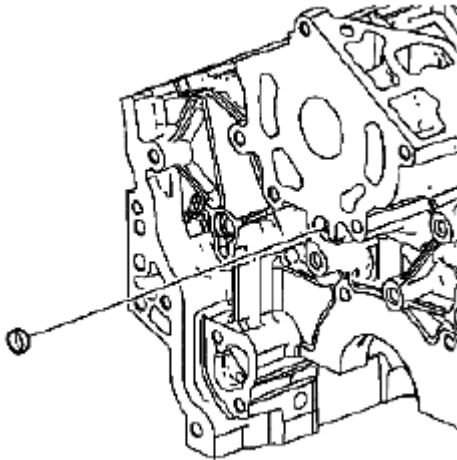
Fig. 689: Identifying Front Oil Gallery Expansion Plug Courtesy of SUZUKI OF AMERICA CORP.
