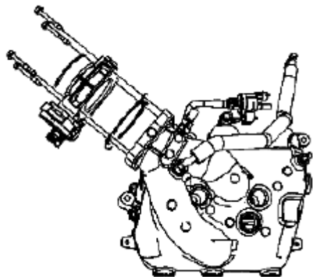
Fig. 35: Identifying Throttle Body & Gasket Courtesy of SUZUKI OF AMERICA CORP.
