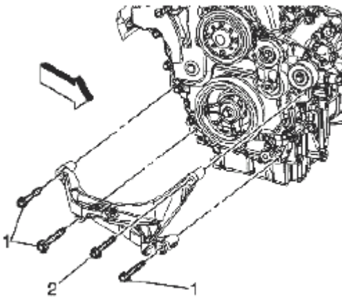
Fig. 56: Removing Upper Engine Mount Bracket Bolts Courtesy of SUZUKI OF AMERICA CORP.
