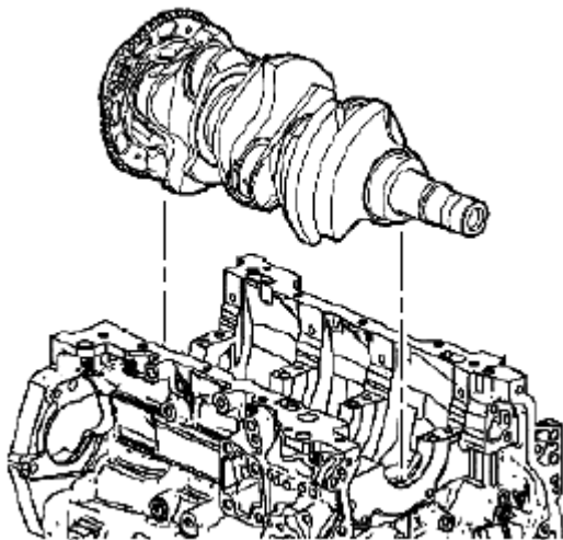
Fig. 714: Identifying Crankshaft Courtesy of SUZUKI OF AMERICA CORP.
