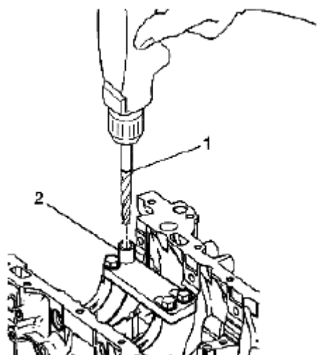
Fig. 660: Drilling Crankshaft Main Bolt Hole Courtesy of SUZUKI OF AMERICA CORP.
