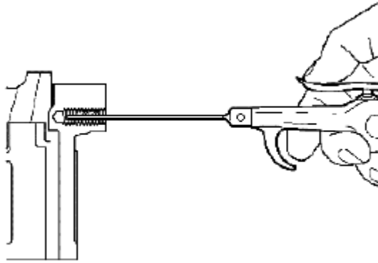
Fig. 612: Applying Compressed Air Into Tapped Hole Courtesy of SUZUKI OF AMERICA CORP.
