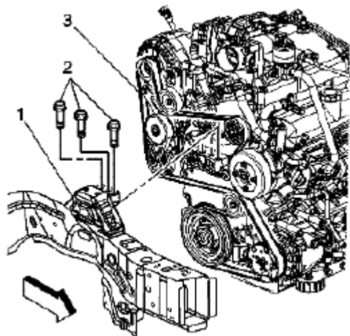
Fig. 252: Securing Right Engine Mount To Engine Courtesy of SUZUKI OF AMERICA CORP.
