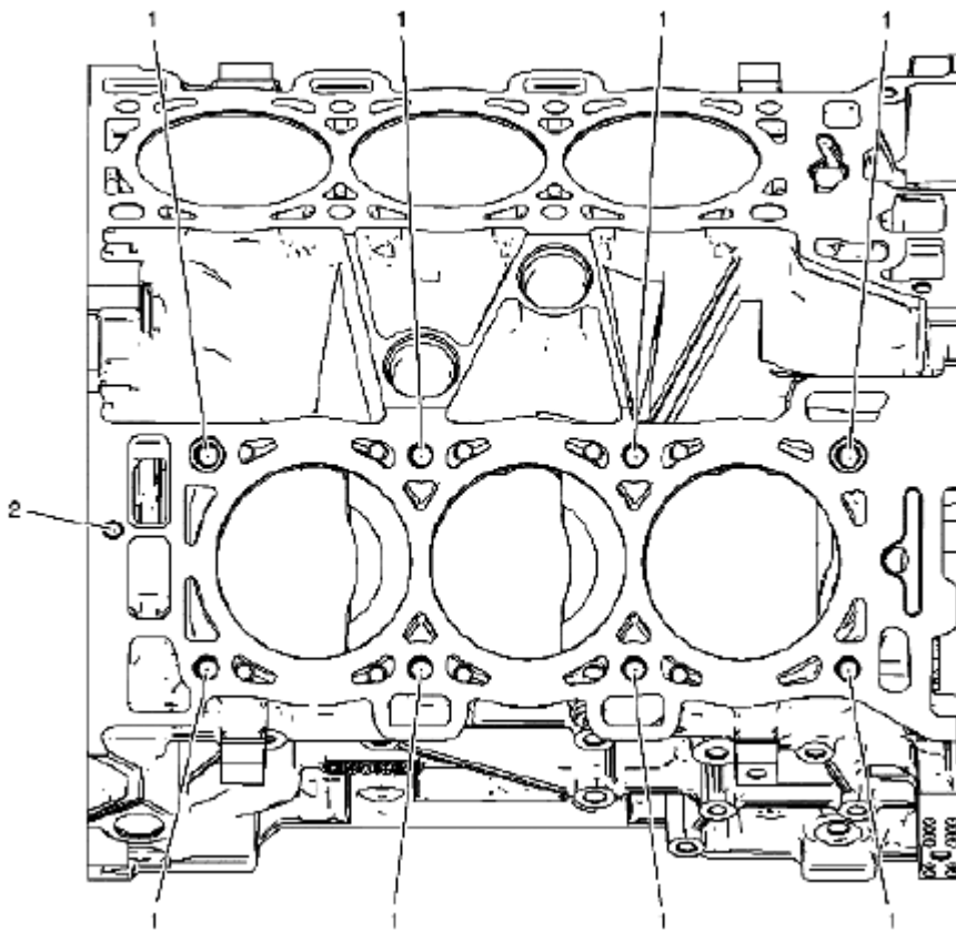
Fig. 1028: Identifying Engine Block Right Deck Face Courtesy of SUZUKI OF AMERICA CORP.
