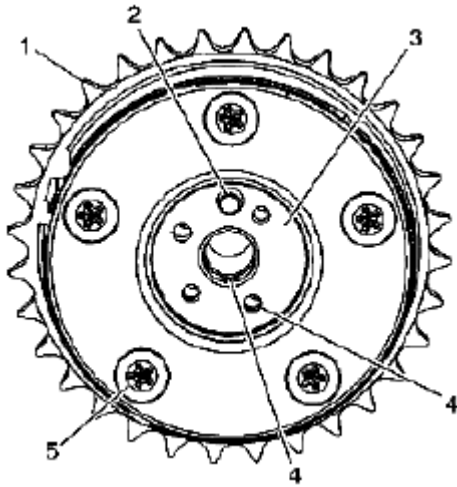
Fig. 479: Identifying Exhaust Camshaft Position Actuators (2 Of 2) Courtesy of SUZUKI OF AMERICA CORP.
