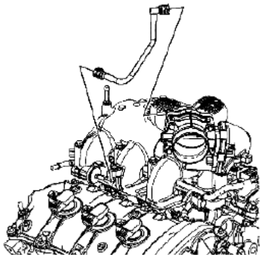
Fig. 273: Identifying Intake Manifold-To-Solenoid Evaporative Emissions (EVAP) Hose Courtesy of SUZUKI OF AMERICA CORP.
