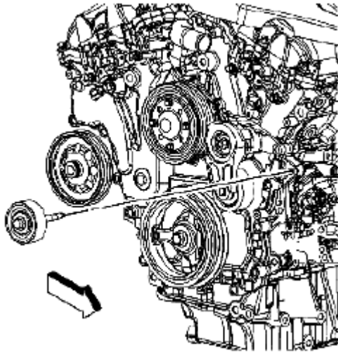
Fig. 42: Removing Drive Belt Idler Pulley Courtesy of SUZUKI OF AMERICA CORP.
