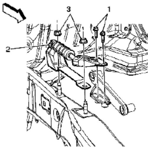
Fig. 64: Installing Engine Mount Strut To Bracket Bolts Courtesy of SUZUKI OF AMERICA CORP.
