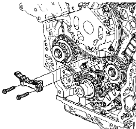
Fig. 868: Identifying Upper Primary Camshaft Drive Chain Guide & Bolts Courtesy of SUZUKI OF AMERICA CORP.
