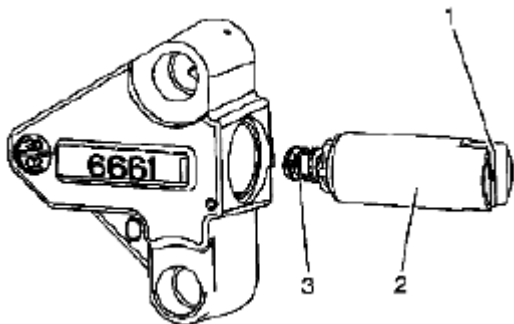
Fig. 499: Identifying Left Secondary Timing Chain Tensioner Courtesy of SUZUKI OF AMERICA CORP.
