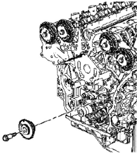
Fig. 152: Identifying Right Bank Secondary Camshaft Drive Chain Tensioner Courtesy of SUZUKI OF AMERICA CORP.
