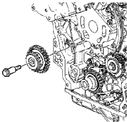
Fig. 850: Identifying Camshaft Intermediate Drive Chain Idler & Bolt Courtesy of SUZUKI OF AMERICA CORP.
