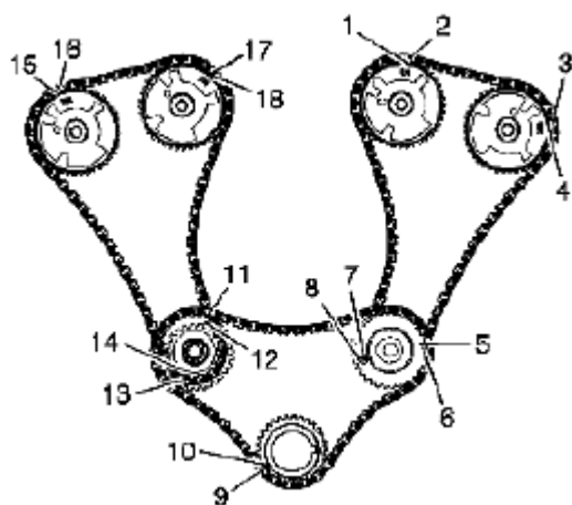
Fig. 938: Identifying Camshaft Drive Chain Timing Mark Courtesy of SUZUKI OF AMERICA CORP.
