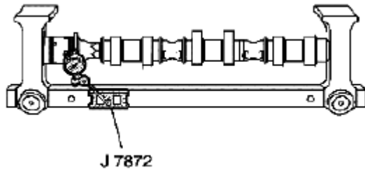
Fig. 473: Measuring Camshaft Thrust Wall Surface For Runout Courtesy of SUZUKI OF AMERICA CORP.
