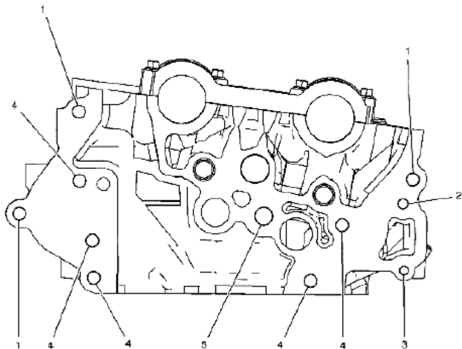
Fig. 1018: Identifying Right Cylinder Head Front Face Courtesy of SUZUKI OF AMERICA CORP.
