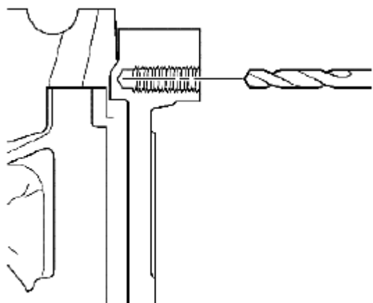
Fig. 589: Applying Drilling, Counterboring & Tapping Of Hole Courtesy of SUZUKI OF AMERICA CORP.
