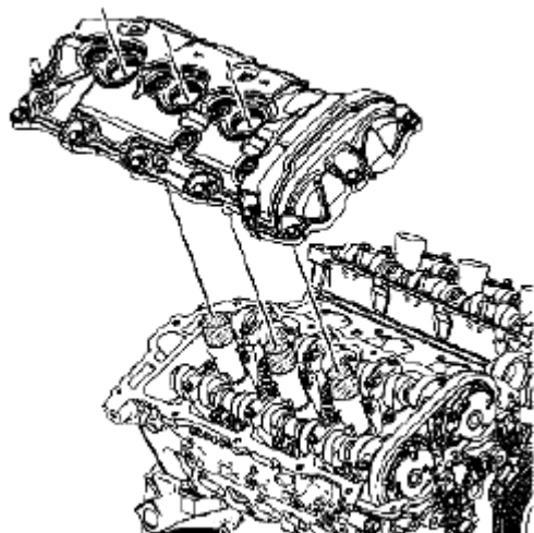
Fig. 974: Identifying Right Camshaft Cover Courtesy of SUZUKI OF AMERICA CORP.
