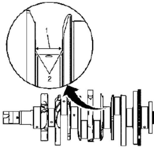
Fig. 410: Identifying Crankshaft Thrust Wall Width Courtesy of SUZUKI OF AMERICA CORP.
