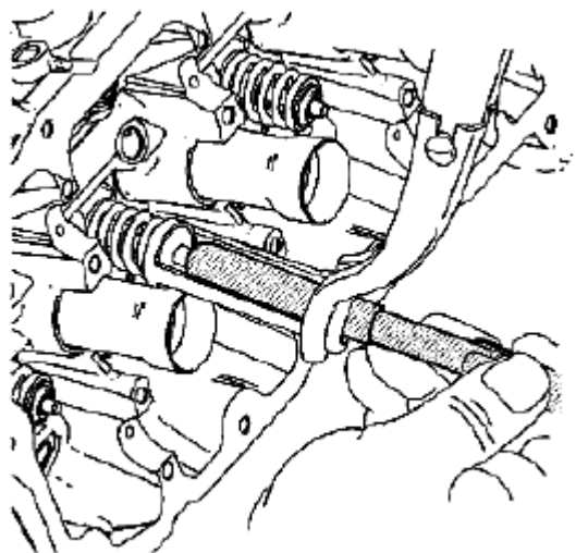
Fig. 441: Compressing Valve Spring Courtesy of SUZUKI OF AMERICA CORP.
