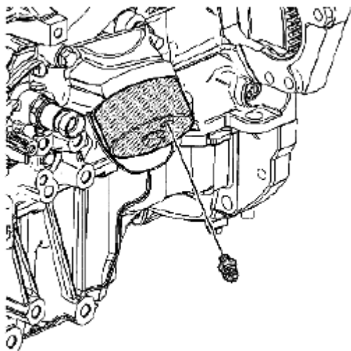
Fig. 1005: Installing 1/8 NPT Fitting From Special Tool (J 45299) Into Port On EN-47971 Courtesy of SUZUKI OF AMERICA CORP.
