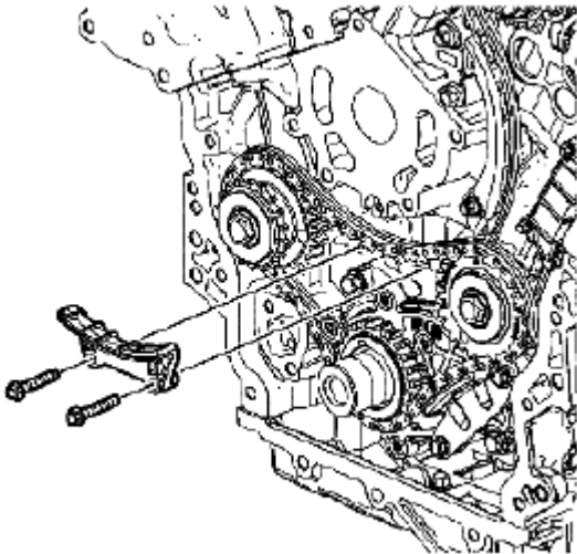
Fig. 326: Identifying Primary Camshaft Drive Chain Upper Guide & Bolts Courtesy of SUZUKI OF AMERICA CORP.
