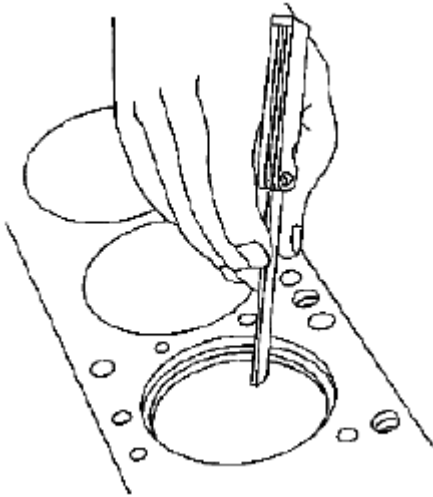
Fig. 424: Measuring Piston Ring End Gap Courtesy of SUZUKI OF AMERICA CORP.
