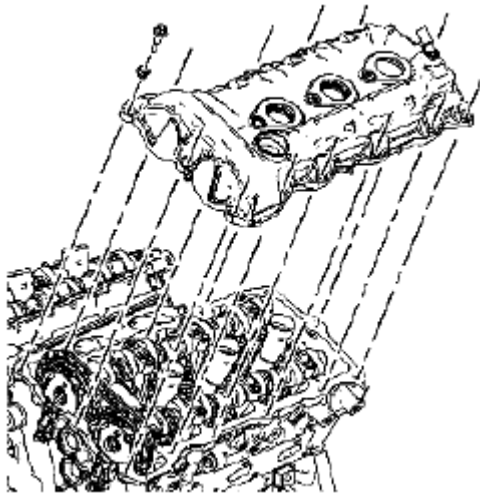
Fig. 99: Identifying Left Camshaft Cover & Bolts Courtesy of SUZUKI OF AMERICA CORP.
