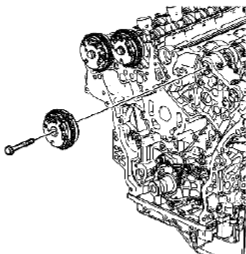
Fig. 790: Identifying Camshaft Position Actuator & Bolt Courtesy of SUZUKI OF AMERICA CORP.
