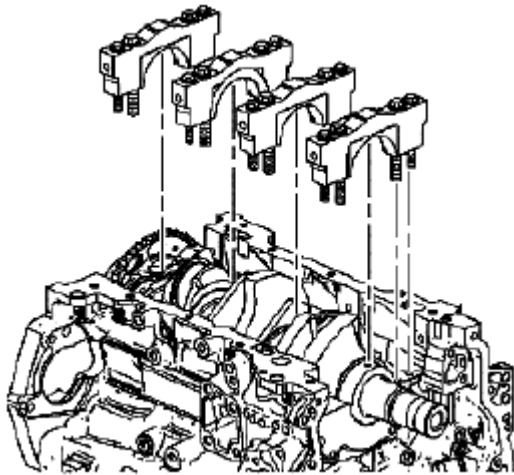
Fig. 718: Identifying Crankshaft Main Bearing Caps Courtesy of SUZUKI OF AMERICA CORP.
