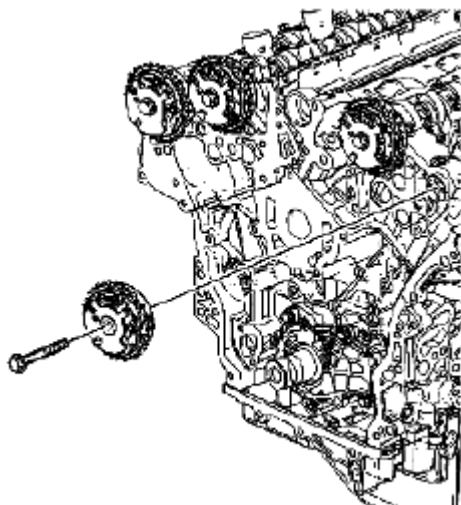
Fig. 350: Identifying Left Exhaust Camshaft Position Actuator & Bolt Courtesy of SUZUKI OF AMERICA CORP.
