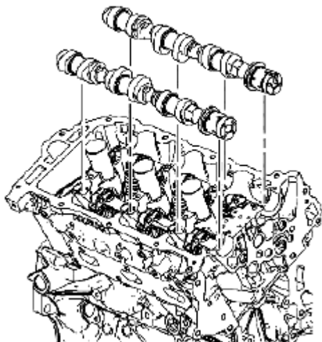
Fig. 752: Identifying Right Intake & Right Exhaust Camshafts Courtesy of SUZUKI OF AMERICA CORP.
