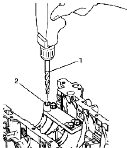
Fig. 675: Drilling Out Threads Of Damaged Hole Courtesy of SUZUKI OF AMERICA CORP.
