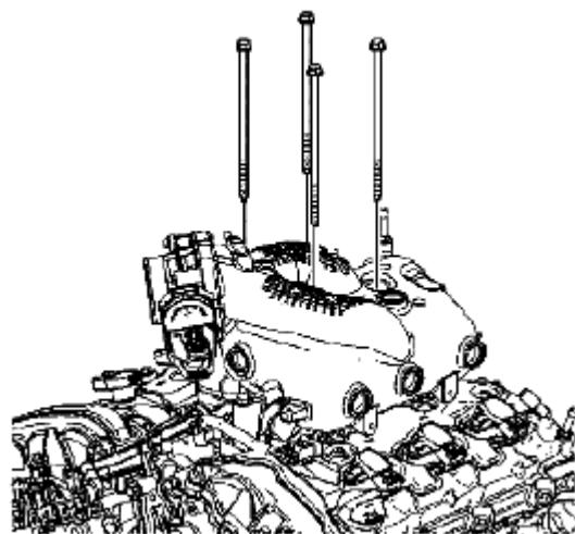
Fig. 984: Identifying Long Intake Manifold Bolts Courtesy of SUZUKI OF AMERICA CORP.
