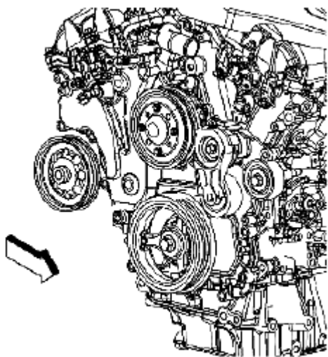
Fig. 39: Locating Drive Belt Tensioner Courtesy of SUZUKI OF AMERICA CORP.
