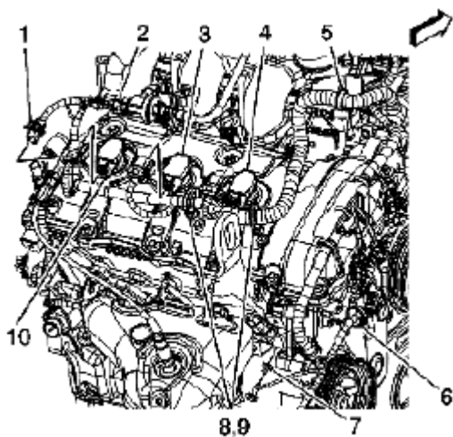
Fig. 250: Connecting Engine Wiring Harness Electrical Connector Courtesy of SUZUKI OF AMERICA CORP.
