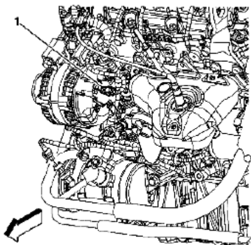
Fig. 40: Disconnecting Generator Electrical Connector Courtesy of SUZUKI OF AMERICA CORP.
