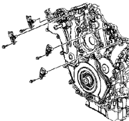
Fig. 290: Identifying Camshaft Position Sensor & Bolts Courtesy of SUZUKI OF AMERICA CORP.
