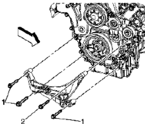
Fig. 62: Installing Right Upper Engine Mount Bracket Bolt Courtesy of SUZUKI OF AMERICA CORP.
