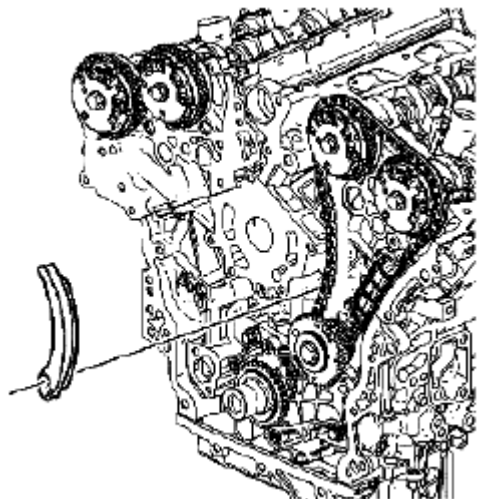
Fig. 829: Identifying Left Secondary Camshaft Drive Chain Shoe (2 Of 2) Courtesy of SUZUKI OF AMERICA CORP.
