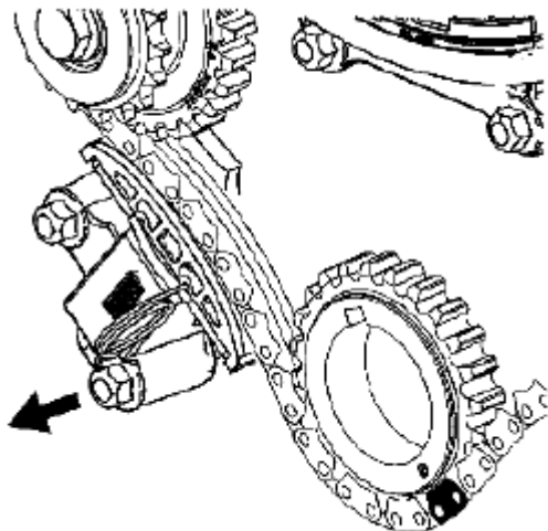
Fig. 878: Pulling EN 46112 From Primary Camshaft Drive Chain Tensioner Courtesy of SUZUKI OF AMERICA CORP.
