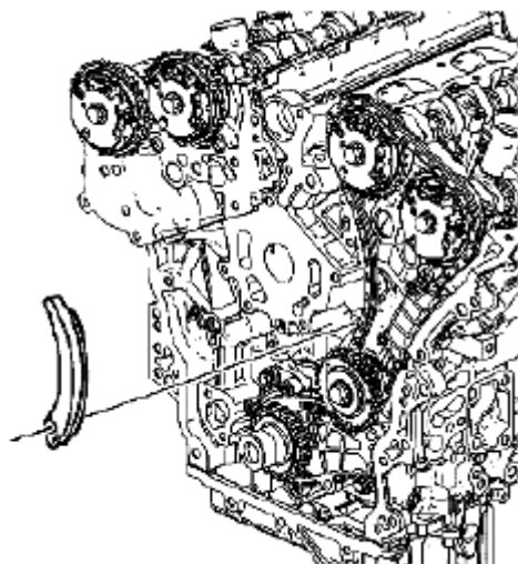
Fig. 339: Identifying Left Secondary Camshaft Drive Chain Shoe Courtesy of SUZUKI OF AMERICA CORP.
