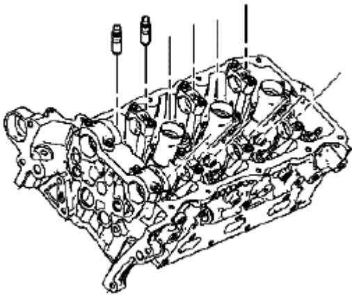
Fig. 194: Identifying Valve Lifters - Right Side Courtesy of SUZUKI OF AMERICA CORP.
