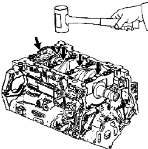
Fig. 707: Tapping Crankshaft Main Bearing Caps Courtesy of SUZUKI OF AMERICA CORP.
