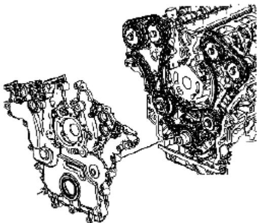
Fig. 124: Identifying Engine Front Cover Courtesy of SUZUKI OF AMERICA CORP.
