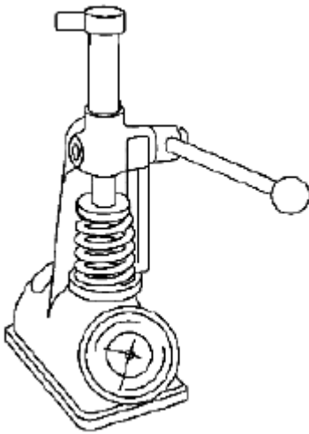
Fig. 452: Measuring Valve Spring Tension Courtesy of SUZUKI OF AMERICA CORP.
