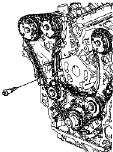
Fig. 316: Identifying Right Secondary Camshaft Drive Chain Shoe Bolt Courtesy of SUZUKI OF AMERICA CORP.
