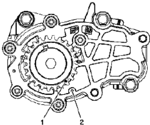
Fig. 797: Aligning Timing Mark On Crankshaft Sprocket Timing Mark & Oil Pump Cover Courtesy of SUZUKI OF AMERICA CORP.
