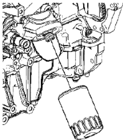
Fig. 1011: Identifying Oil Filter
