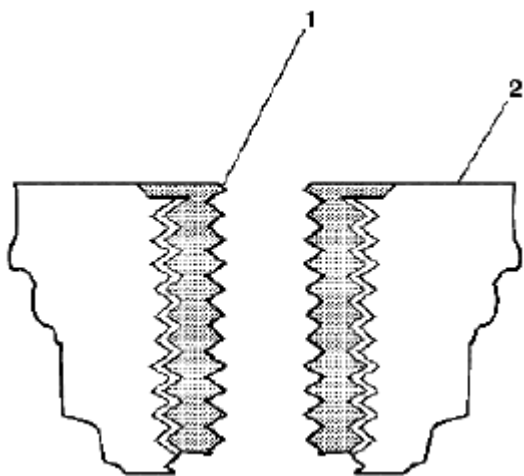
Fig. 592: Identifying Hole Flange & Surface Courtesy of SUZUKI OF AMERICA CORP.
