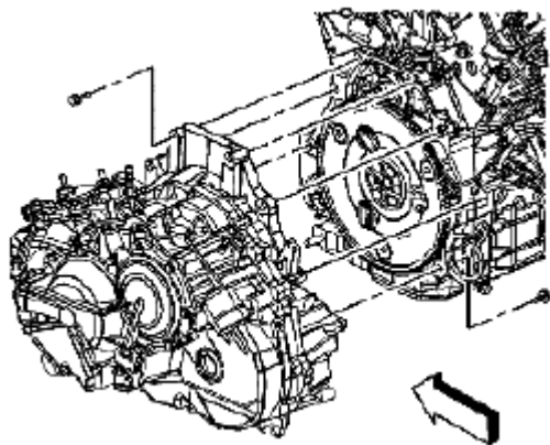
Fig. 243: Aligning Engine To Frame & Automatic Transaxle Courtesy of SUZUKI OF AMERICA CORP.
