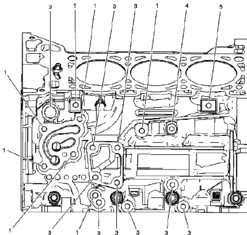
Fig. 1023: Identifying Engine Block Left Side Courtesy of SUZUKI OF AMERICA CORP.
