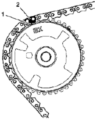
Fig. 908: Identifying Timing Camshaft Drive Chain Link Mark (3 Of 5) Courtesy of SUZUKI OF AMERICA CORP.
