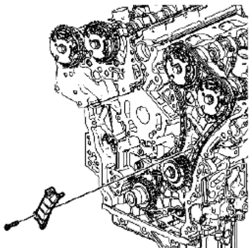
Fig. 342: Identifying Left Secondary Camshaft Drive Chain Guide Bolts Courtesy of SUZUKI OF AMERICA CORP.
