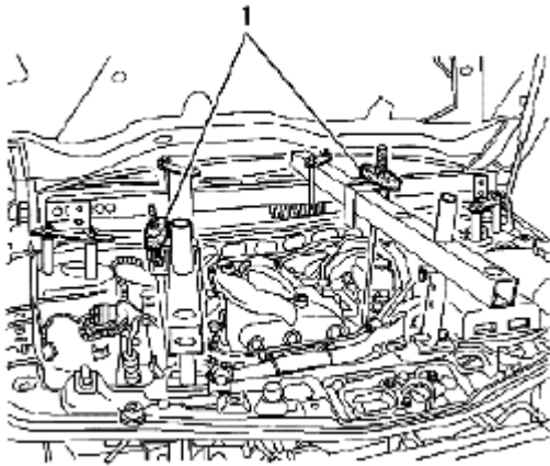
Fig. 1048: Identifying Special Tool (J-28467-34) Courtesy of SUZUKI OF AMERICA CORP.
