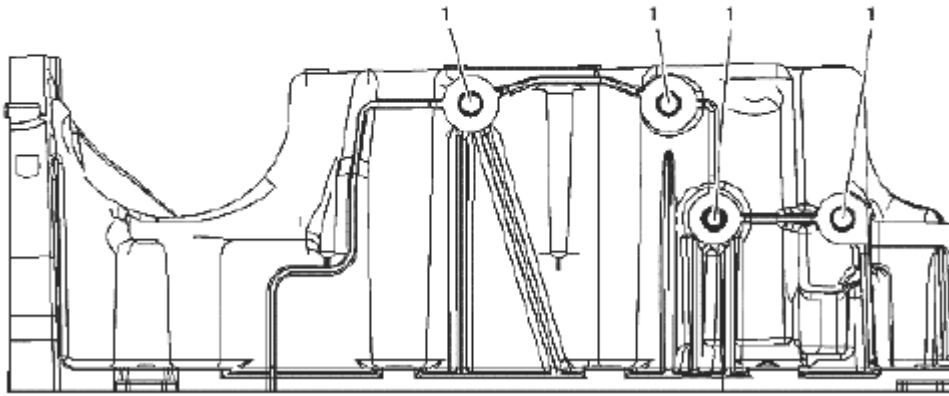
Fig. 1034: Identifying Oil Pan Left Side Courtesy of SUZUKI OF AMERICA CORP.
