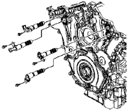
Fig. 291: Identifying Camshaft Position Actuator Valve & Bolts Courtesy of SUZUKI OF AMERICA CORP.
