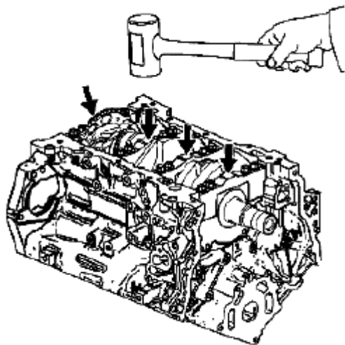
Fig. 719: Tapping Crankshaft Main Bearing Caps Courtesy of SUZUKI OF AMERICA CORP.
