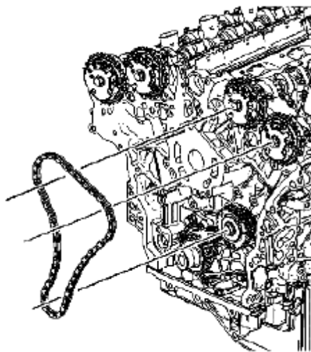
Fig. 344: Identifying Left Secondary Camshaft Drive Chain Courtesy of SUZUKI OF AMERICA CORP.
