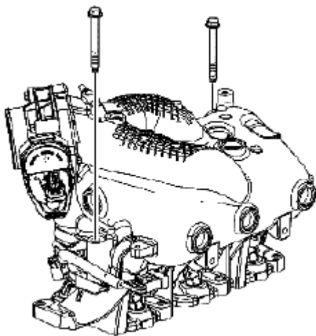
Fig. 587: Identifying Upper-To-Lower Intake Manifold Bolts Courtesy of SUZUKI OF AMERICA CORP.
