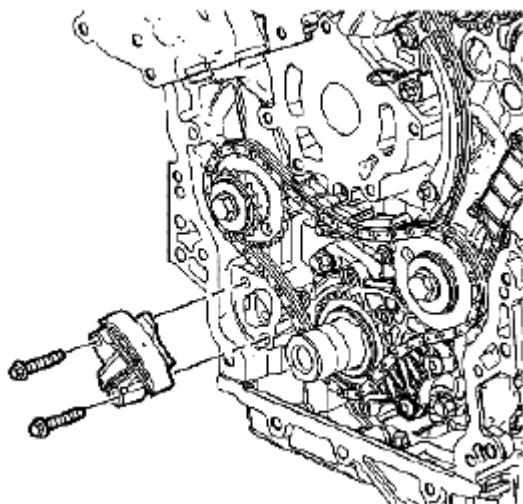
Fig. 157: Identifying Primary Camshaft Drive Chain Tensioner Courtesy of SUZUKI OF AMERICA CORP.
