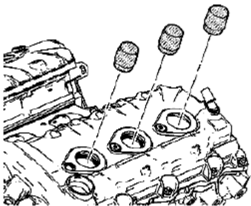
Fig. 106: Installing EN 46101 On Spark Plug Tubes Courtesy of SUZUKI OF AMERICA CORP.
