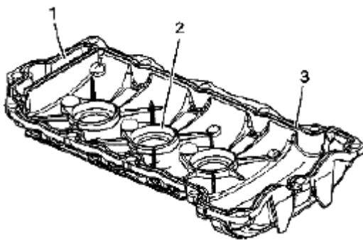
Fig. 546: Identifying Right Camshaft Cover Courtesy of SUZUKI OF AMERICA CORP.
