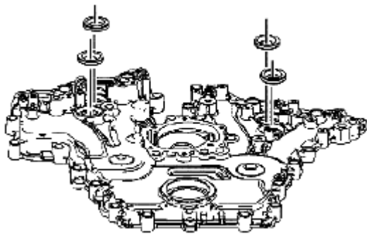
Fig. 527: Identifying Camshaft Position Actuator Valve Oil Seals Courtesy of SUZUKI OF AMERICA CORP.
