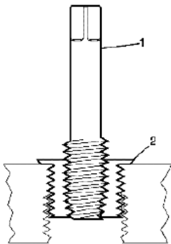
Fig. 637: Applying Insert Into Tapped Hole Courtesy of SUZUKI OF AMERICA CORP.
