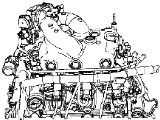
Fig. 74: Disconnecting Electronic Throttle Control (ETC) Electrical Connector Courtesy of SUZUKI OF AMERICA CORP.
