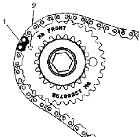
Fig. 862: Identifying Right Camshaft Intermediate Drive Chain Idler Timing Mark Courtesy of SUZUKI OF AMERICA CORP.
