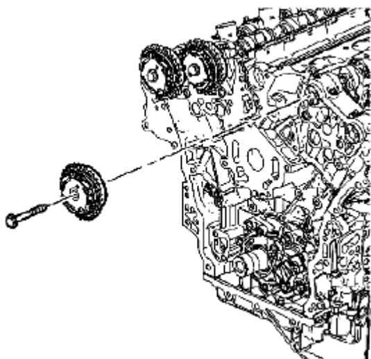
Fig. 170: Identifying Camshaft Position Actuator Courtesy of SUZUKI OF AMERICA CORP.
