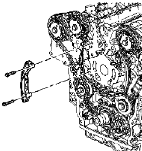
Fig. 144: Identifying Right Bank Secondary Camshaft Drive Chain Guide Courtesy of SUZUKI OF AMERICA CORP.
