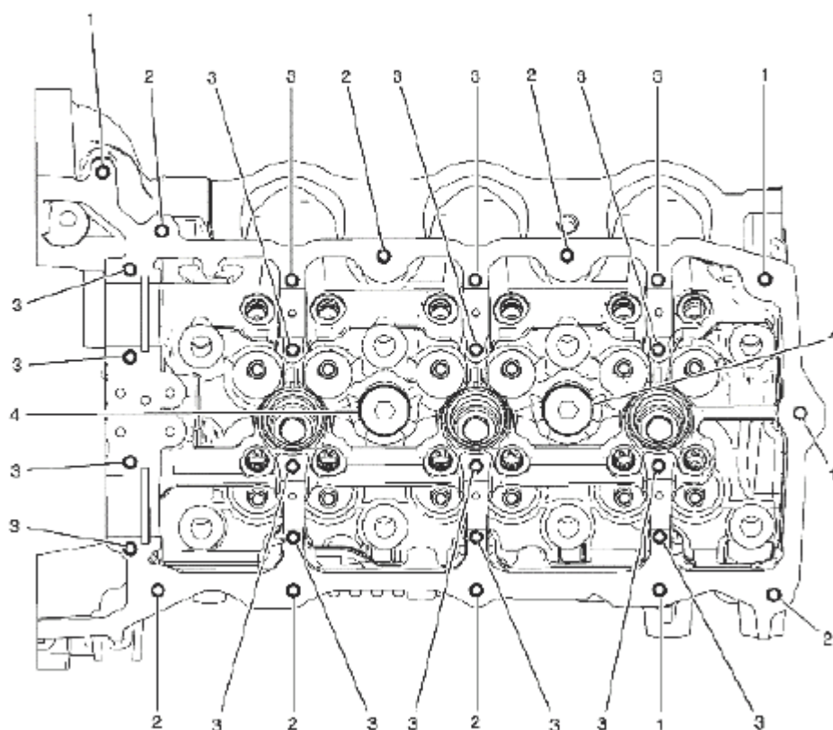
Fig. 1012: Identifying Left Cylinder Head Camshaft Cover Face Courtesy of SUZUKI OF AMERICA CORP.
