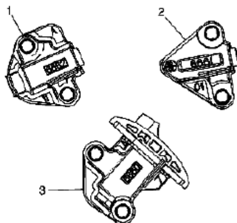
Fig. 921: Identifying Right Secondary Camshaft Drive Chain Tensioner Courtesy of SUZUKI OF AMERICA CORP.
