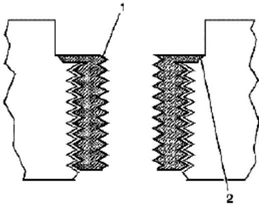
Fig. 623: Identifying Insert & Proper Installation Courtesy of SUZUKI OF AMERICA CORP.
