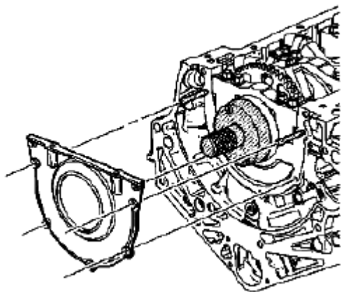
Fig. 737: Identifying Crankshaft Rear Oil Seal Housing Courtesy of SUZUKI OF AMERICA CORP.
