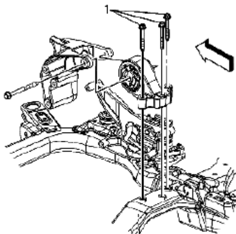
Fig. 48: Installing Engine Mount Bracket To Engine Mount Bolt Courtesy of SUZUKI OF AMERICA CORP.
