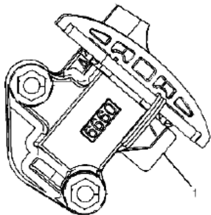
Fig. 877: Identifying Primary Camshaft Drive Chain Tensioner Gasket Tab Courtesy of SUZUKI OF AMERICA CORP.
