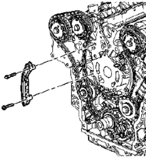
Fig. 145: Identifying Right Bank Secondary Camshaft Drive Chain Guide Courtesy of SUZUKI OF AMERICA CORP.
