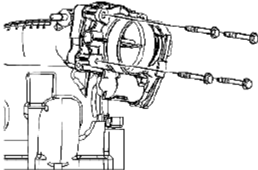
Fig. 584: Identifying Throttle Body Bolts
