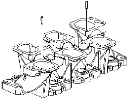
Fig. 577: Identifying Upper-To-Lower Intake Manifold Alignment Pins Courtesy of SUZUKI OF AMERICA CORP.
