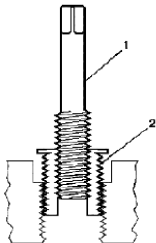
Fig. 620: Applying Insert Into Tapped Hole (1 Of 2) Courtesy of SUZUKI OF AMERICA CORP.
