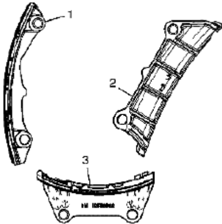
Fig. 869: Identifying Upper Primary Camshaft Drive Chain Guide Courtesy of SUZUKI OF AMERICA CORP.
