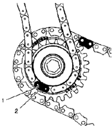
Fig. 899: Identifying Timing Camshaft Drive Chain Link Mark (1 Of 5) Courtesy of SUZUKI OF AMERICA CORP.
