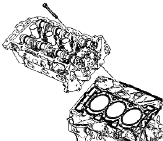
Fig. 222: Identifying Cylinder Head Courtesy of SUZUKI OF AMERICA CORP.
