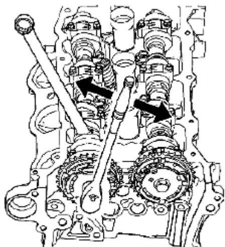
Fig. 182: Loosening Camshaft Position Actuator Bolt Courtesy of SUZUKI OF AMERICA CORP.
