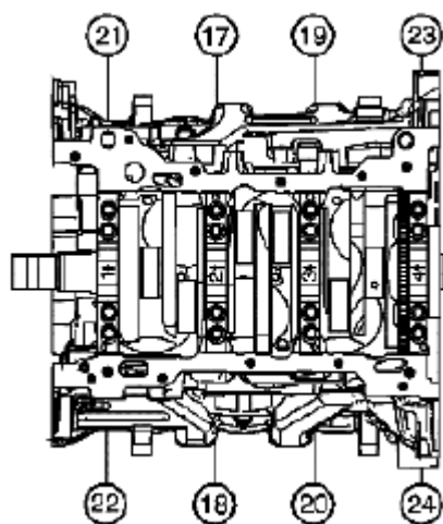
Fig. 723: Tightening Short/Inner Bolts In Sequence Courtesy of SUZUKI OF AMERICA CORP.
