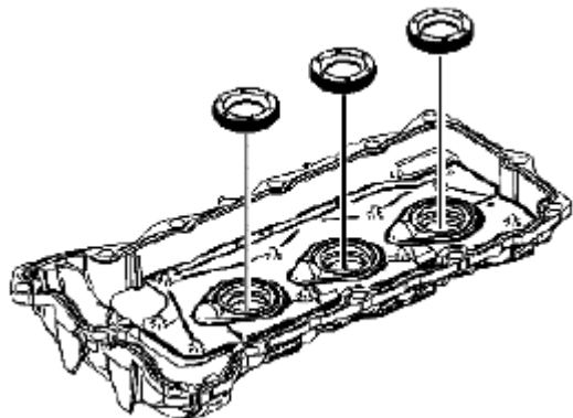
Fig. 539: Identifying Left Spark Plug Shield Tube Seals Courtesy of SUZUKI OF AMERICA CORP.
