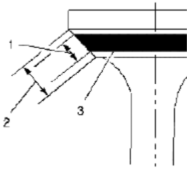
Fig. 457: Identifying Valve Face
