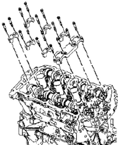
Fig. 755: Identifying Camshaft Bearing Thrust Caps & Bolts Courtesy of SUZUKI OF AMERICA CORP.
