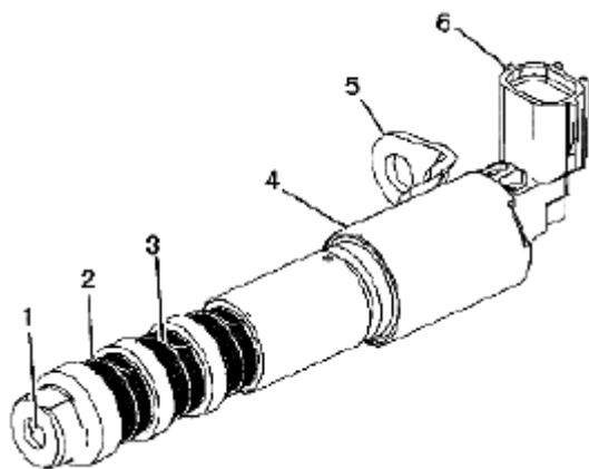
Fig. 507: Identifying Camshaft Position Actuator Oil Control Valves Courtesy of SUZUKI OF AMERICA CORP.
