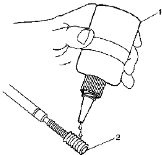
Fig. 619: Applying Threadlock Sealant To Insert OD Threads Courtesy of SUZUKI OF AMERICA CORP.
