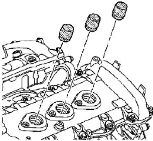
Fig. 114: Installing EN 46101 Onto Spark Plug Tubes Courtesy of SUZUKI OF AMERICA CORP.
