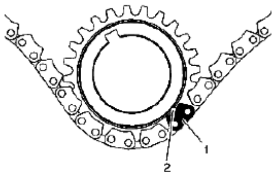
Fig. 857: Identifying Crankshaft Sprocket Timing Mark Courtesy of SUZUKI OF AMERICA CORP.
