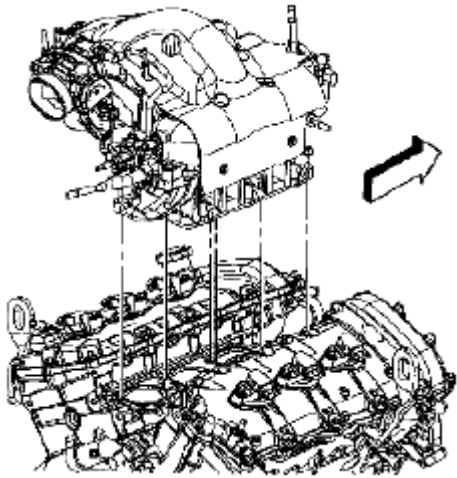
Fig. 79: Removing Upper Intake Manifold & Gasket Courtesy of SUZUKI OF AMERICA CORP.
