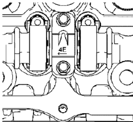
Fig. 359: Identifying Markings On Bearing Caps Courtesy of SUZUKI OF AMERICA CORP.
