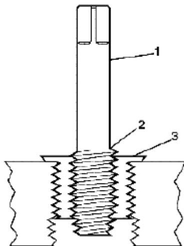
Fig. 638: Applying Insert Into Tapped Hole Courtesy of SUZUKI OF AMERICA CORP.
