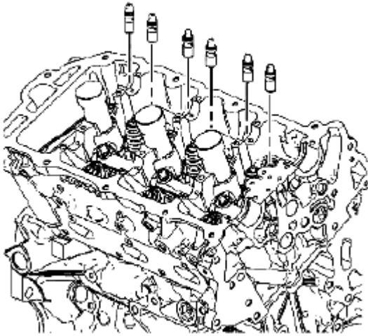
Fig. 371: Identifying Valve Lifters
