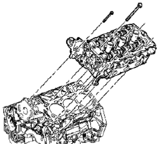
Fig. 758: Identifying Left Cylinder Head Courtesy of SUZUKI OF AMERICA CORP.
