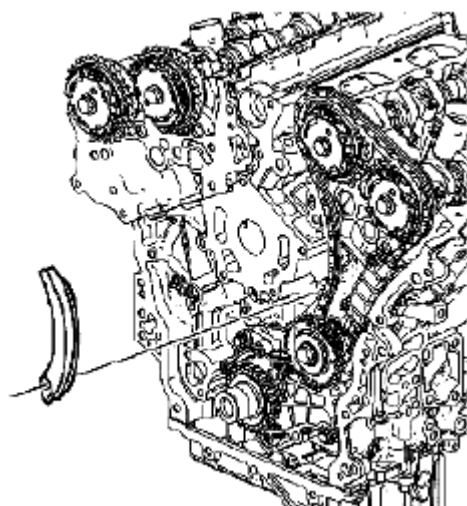
Fig. 138: Identifying Left Secondary Camshaft Drive Chain Shoe (3 Of 3) Courtesy of SUZUKI OF AMERICA CORP.
