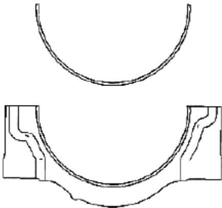
Fig. 381: Identifying Lower Connecting Rod Bearing Courtesy of SUZUKI OF AMERICA CORP.
