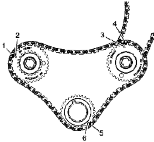
Fig. 864: Identifying Timing Camshaft Drive Chain Links Mark Courtesy of SUZUKI OF AMERICA CORP.
