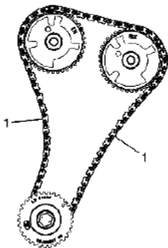
Fig. 820: Identifying Timing Camshaft Drive Chain Link Mark (4 Of 4) Courtesy of SUZUKI OF AMERICA CORP.
