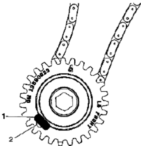
Fig. 808: Identifying Timing Camshaft Drive Chain Link Courtesy of SUZUKI OF AMERICA CORP.
