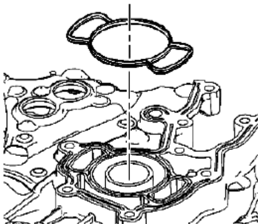
Fig. 528: Identifying Water Pump Seal Courtesy of SUZUKI OF AMERICA CORP.
