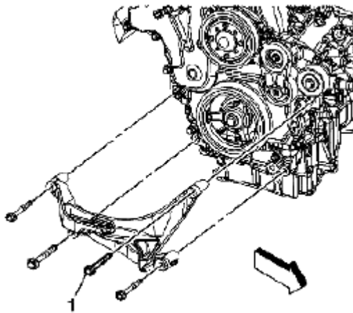
Fig. 58: Removing Upper Bracket Bolt From Bracket Courtesy of SUZUKI OF AMERICA CORP.
