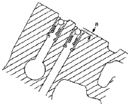
Fig. 448: Identifying Cylinder Head Deck Surface Courtesy of SUZUKI OF AMERICA CORP.
