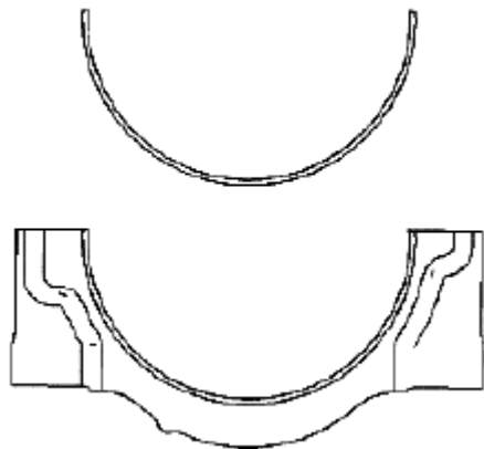
Fig. 438: Identifying Lower Connecting Rod Bearings Courtesy of SUZUKI OF AMERICA CORP.
