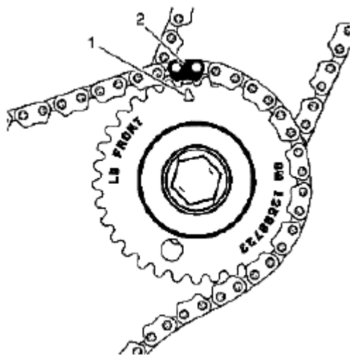
Fig. 861: Identifying Left Camshaft Intermediate Drive Chain Idler Timing Mark Courtesy of SUZUKI OF AMERICA CORP.
