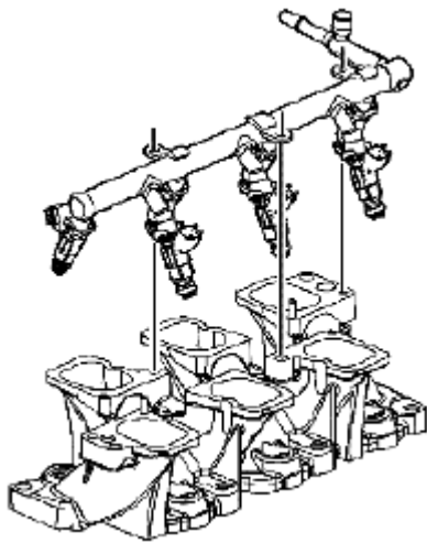
Fig. 578: Identifying Fuel Injector Rail Courtesy of SUZUKI OF AMERICA CORP.
