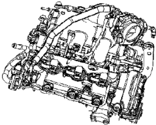
Fig. 84: Connecting PCV Line To Top Of Intake Manifold Courtesy of SUZUKI OF AMERICA CORP.
