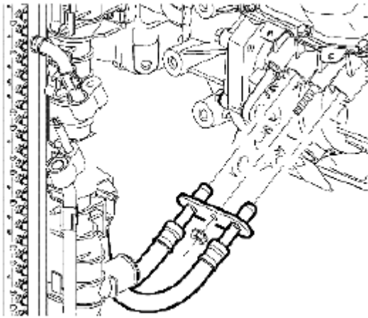
Fig. 227: Disconnecting Transaxle Oil Cooler Lines From Transaxle Courtesy of SUZUKI OF AMERICA CORP.
