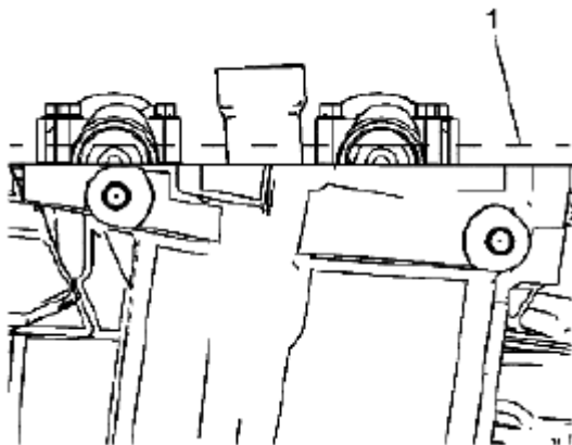
Fig. 753: Identifying Camshafts Parallel Line Courtesy of SUZUKI OF AMERICA CORP.
