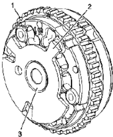
Fig. 503: Identifying Front Of Left Intake Camshaft Position Actuators Courtesy of SUZUKI OF AMERICA CORP.
