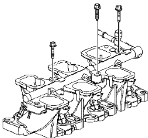
Fig. 579: Identifying Fuel Injector Rail Bolts Courtesy of SUZUKI OF AMERICA CORP.
