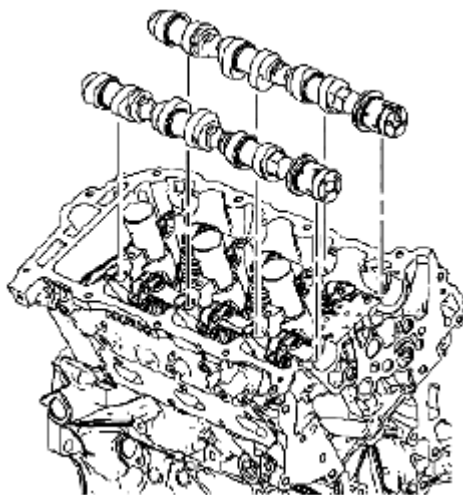
Fig. 369: Identifying Camshafts Courtesy of SUZUKI OF AMERICA CORP.
