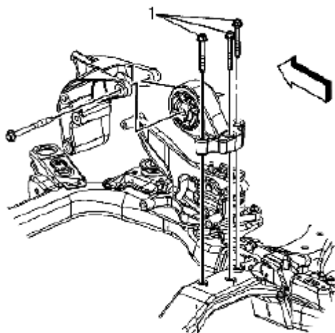
Fig. 47: Removing Engine Mount Bracket To Engine Mount Bolt Courtesy of SUZUKI OF AMERICA CORP.
