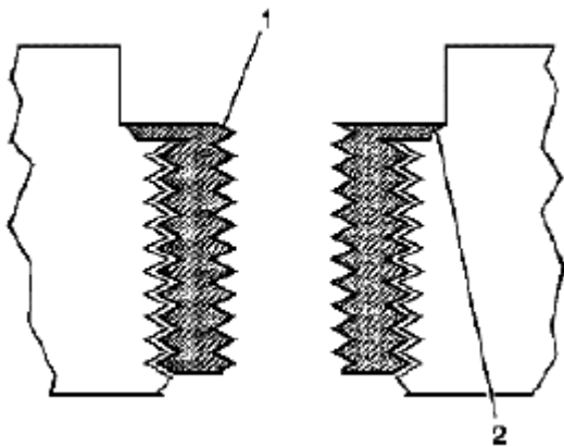
Fig. 609: Identifying Insert & Counterbore Courtesy of SUZUKI OF AMERICA CORP.
