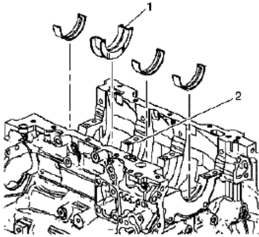
Fig. 387: Identifying Crankshaft Upper Bearing Halves Courtesy of SUZUKI OF AMERICA CORP.
