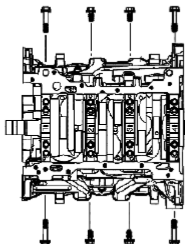
Fig. 711: Identifying Crankshaft Bearing Cap Side Bolts Courtesy of SUZUKI OF AMERICA CORP.
