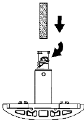
Fig. 872: Resetting Primary Camshaft Drive Chain Tensioner Plunger Using J 45027 Courtesy of SUZUKI OF AMERICA CORP.
