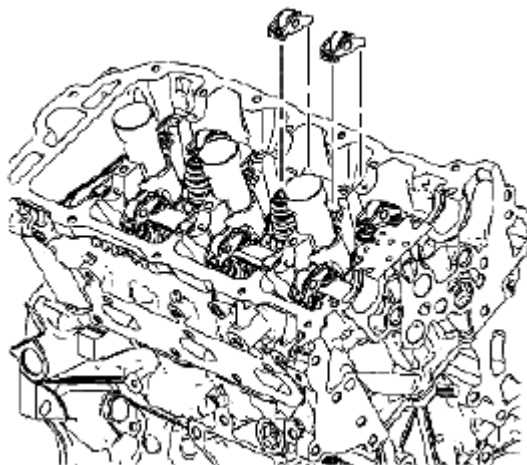
Fig. 747: Identifying Camshaft Followers Courtesy of SUZUKI OF AMERICA CORP.
