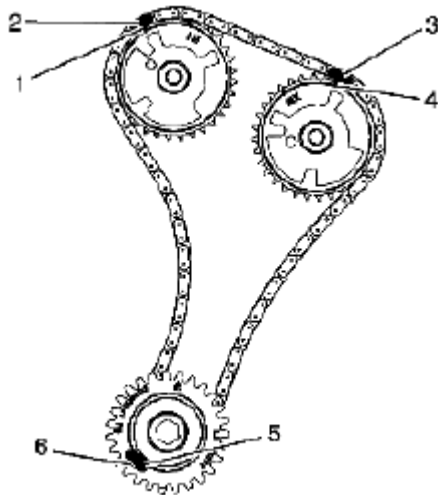
Fig. 839: Identifying Left Secondary Camshaft Drive Chain Timing Mark Courtesy of SUZUKI OF AMERICA CORP.
