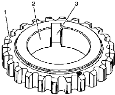
Fig. 487: Identifying Crankshaft Sprocket Courtesy of SUZUKI OF AMERICA CORP.
