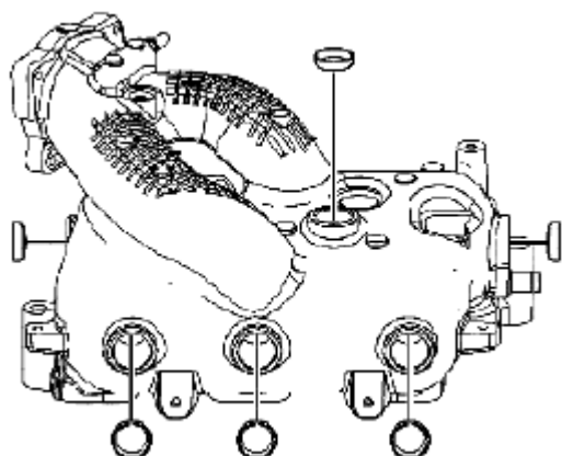
Fig. 565: Identifying Upper Intake Manifold Expansion Plugs Courtesy of SUZUKI OF AMERICA CORP.
