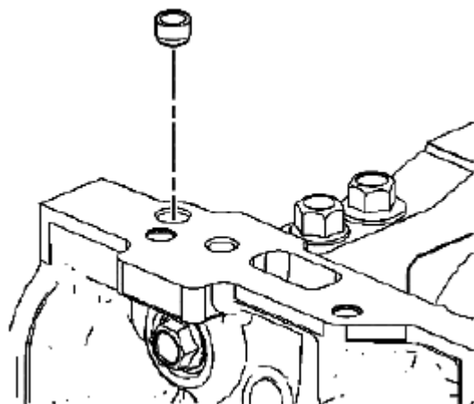
Fig. 698: Identifying Right Front Oil Pan Rail Oil Gallery Expansion Plug Courtesy of SUZUKI OF AMERICA CORP.
