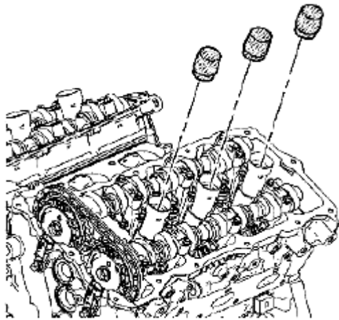
Fig. 100: Inserting EN 46101 Onto Spark Plug Tubes Courtesy of SUZUKI OF AMERICA CORP.
