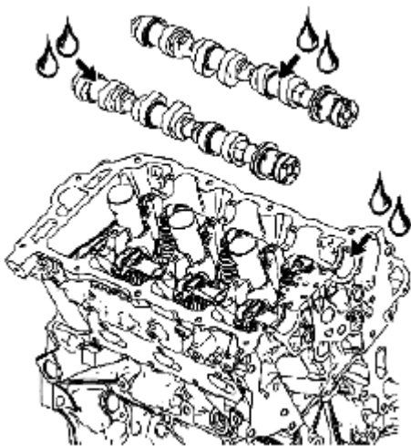
Fig. 751: Applying Liberal Amount Of Lubricant To Camshaft Journals & Right Cylinder Head Camshaft Carriers Courtesy of SUZUKI OF AMERICA CORP.
