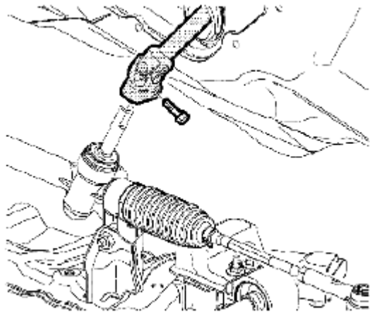
Fig. 257: Identifying Pinch Bolt Courtesy of SUZUKI OF AMERICA CORP.
