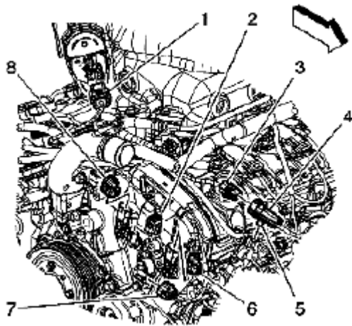
Fig. 36: Identifying Engine Wiring Harness Electrical Connectors Courtesy of SUZUKI OF AMERICA CORP.
