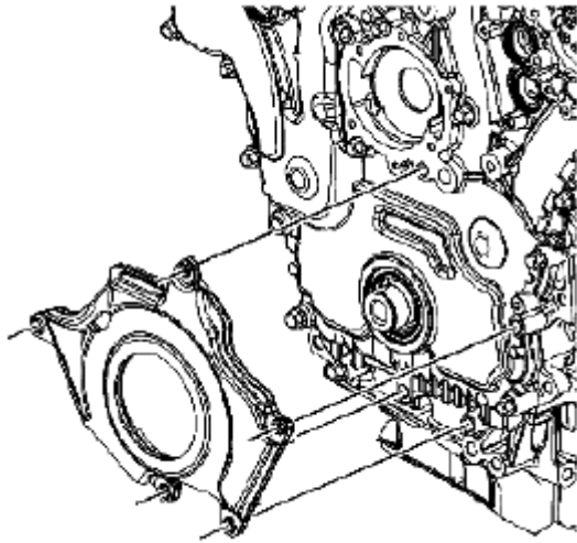
Fig. 303: Identifying Engine Front Cover Deadener Courtesy of SUZUKI OF AMERICA CORP.
