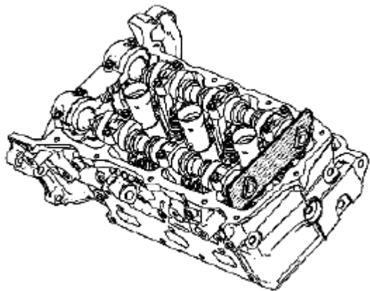
Fig. 895: Identifying EN 46105-2 Onto Rear Of Left Camshafts Courtesy of SUZUKI OF AMERICA CORP.
