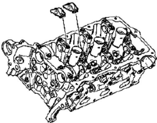
Fig. 763: Identifying Camshaft Followers (2 Of 2) Courtesy of SUZUKI OF AMERICA CORP.
