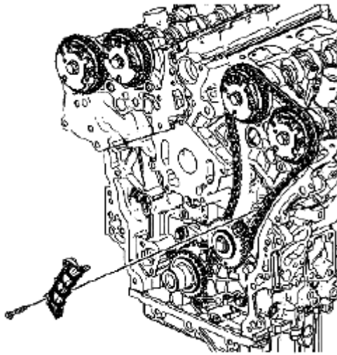
Fig. 824: Identifying Left Secondary Camshaft Drive Chain Guide & Bolt Courtesy of SUZUKI OF AMERICA CORP.
