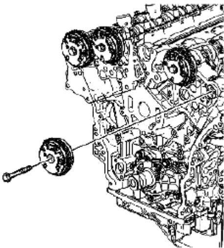
Fig. 351: Identifying Left Exhaust Camshaft Position Actuator & Bolt Courtesy of SUZUKI OF AMERICA CORP.
