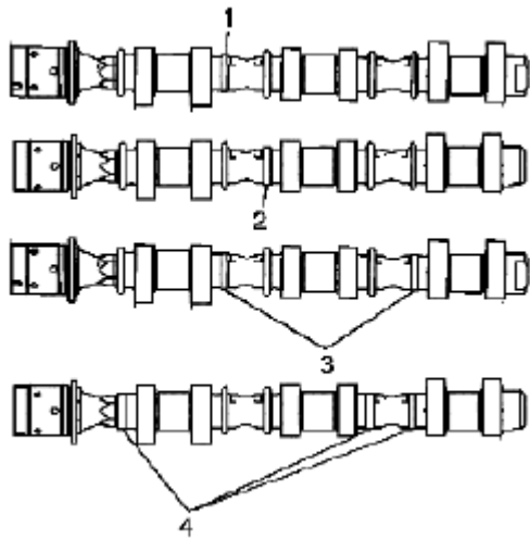
Fig. 750: Identifying Camshaft Identification Ring Courtesy of SUZUKI OF AMERICA CORP.
