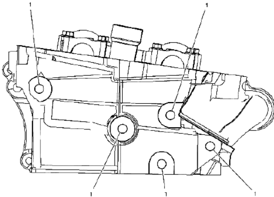
Fig. 1016: Identifying Left Cylinder Head Rear Face Courtesy of SUZUKI OF AMERICA CORP.
