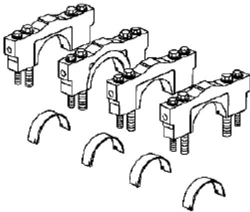
Fig. 388: Identifying Crankshaft Lower Bearing Halves & Crankshaft Bearing Caps Courtesy of SUZUKI OF AMERICA CORP.
