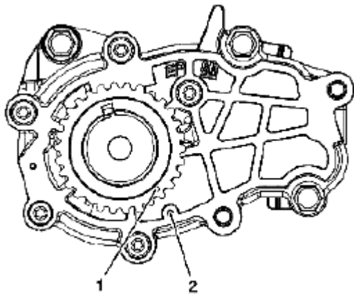
Fig. 814: Aligning Timing Mark On Crankshaft Sprocket Timing Mark & Oil Pump Cover Courtesy of SUZUKI OF AMERICA CORP.
