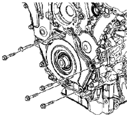
Fig. 302: Identifying Engine Front Cover Bolts Courtesy of SUZUKI OF AMERICA CORP.
