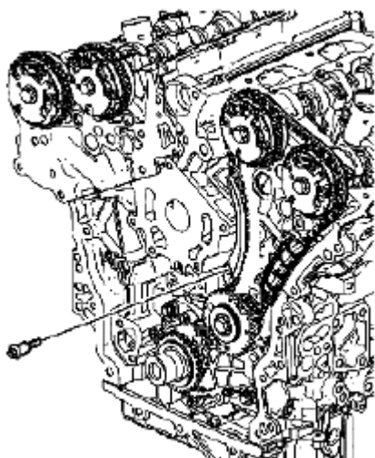
Fig. 340: Identifying Left Secondary Camshaft Drive Chain Shoe Bolt Courtesy of SUZUKI OF AMERICA CORP.
