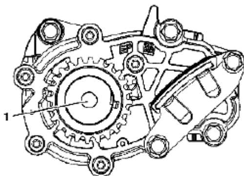
Fig. 897: Identifying Stage 2 Timing Drive Assembly Position Courtesy of SUZUKI OF AMERICA CORP.
