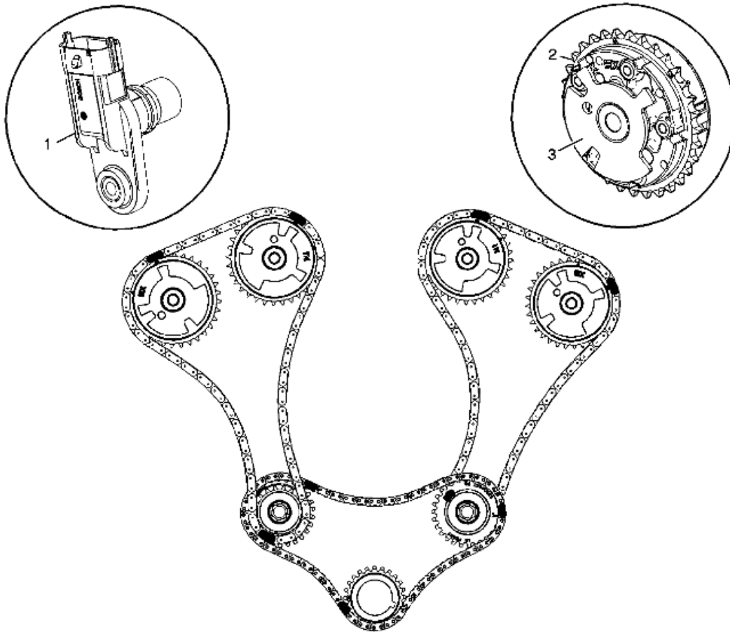
Fig. 1: Camshaft Timing Drive Design Identification - First Design 2007 Courtesy of SUZUKI OF AMERICA CORP.
