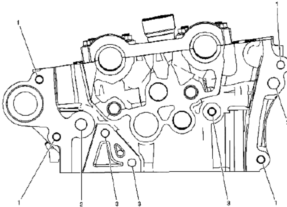
Fig. 1013: Identifying Left Cylinder Head Front Face Courtesy of SUZUKI OF AMERICA CORP.
