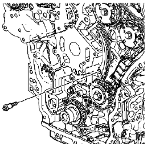
Fig. 338: Identifying Left Secondary Camshaft Drive Chain Shoe Bolt Courtesy of SUZUKI OF AMERICA CORP.
