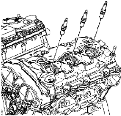
Fig. 967: Identifying Spark Plugs (2 Of 2) Courtesy of SUZUKI OF AMERICA CORP.
