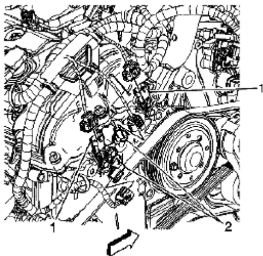
Fig. 236: Disconnecting Cylinder Head Engine Electrical Wiring Harness
