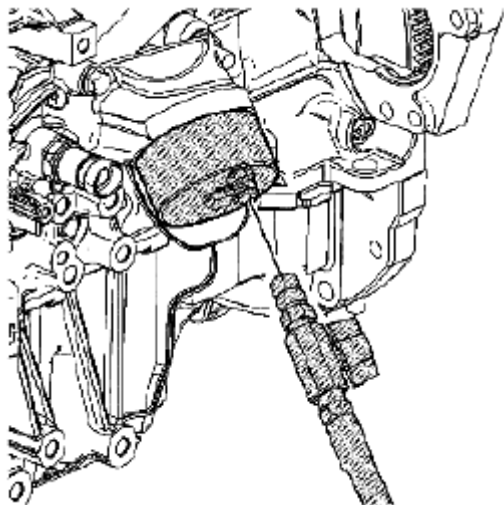
Fig. 1008: Identifying Special Tool (J 45299) Courtesy of SUZUKI OF AMERICA CORP.
