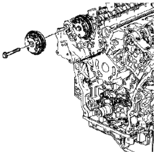
Fig. 355: Identifying Right Exhaust Camshaft Position Actuator And Bolt Courtesy of SUZUKI OF AMERICA CORP.
