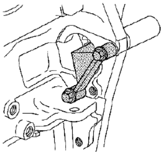
Fig. 89: Installing EN 46106 Through Starter Mounting Hole Courtesy of SUZUKI OF AMERICA CORP.
