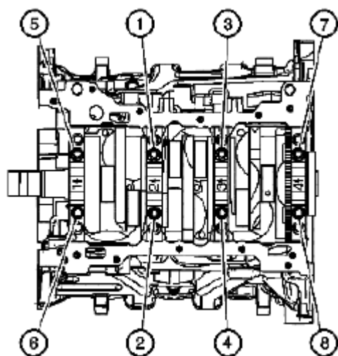
Fig. 721: Tightening Inboard Bolts In Sequence Courtesy of SUZUKI OF AMERICA CORP.
