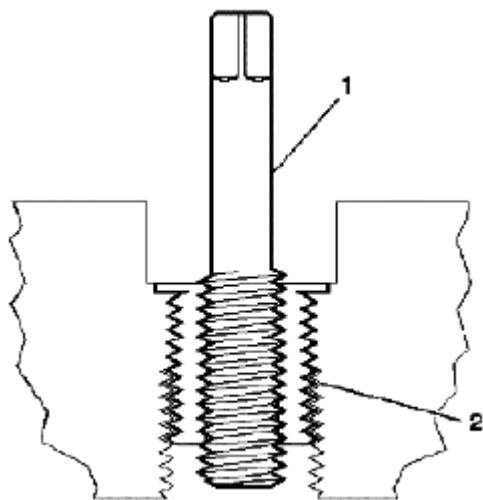
Fig. 622: Applying Insert Into Tapped Hole Courtesy of SUZUKI OF AMERICA CORP.
