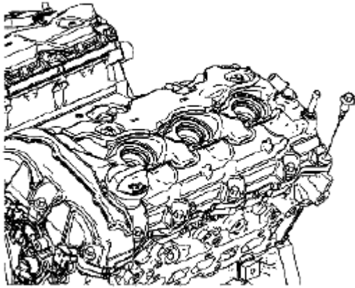
Fig. 283: Identifying Left Camshaft Cover Bolts Courtesy of SUZUKI OF AMERICA CORP.
