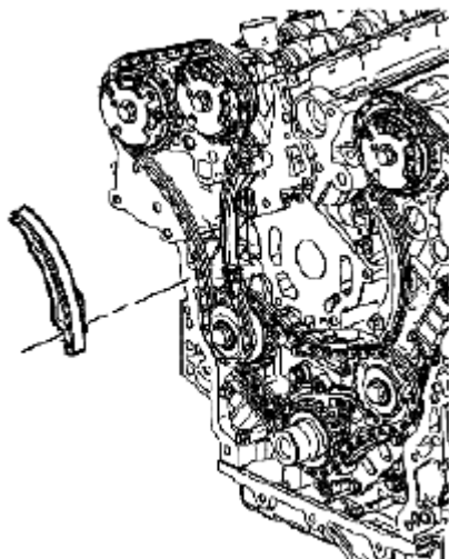
Fig. 315: Identifying Right Secondary Camshaft Drive Chain Shoe Courtesy of SUZUKI OF AMERICA CORP.
