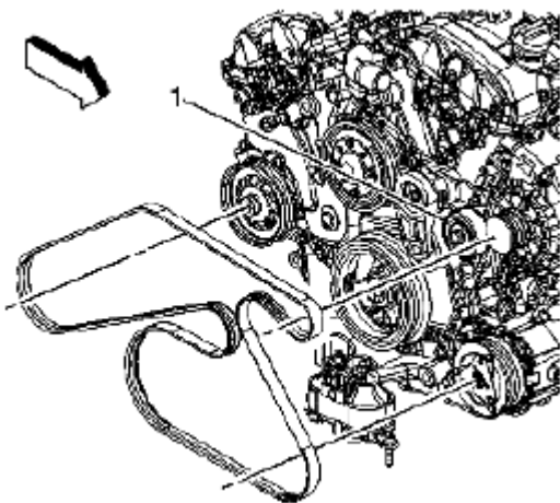
Fig. 37: Locating Drive Belt & Belt Idler Pulley
