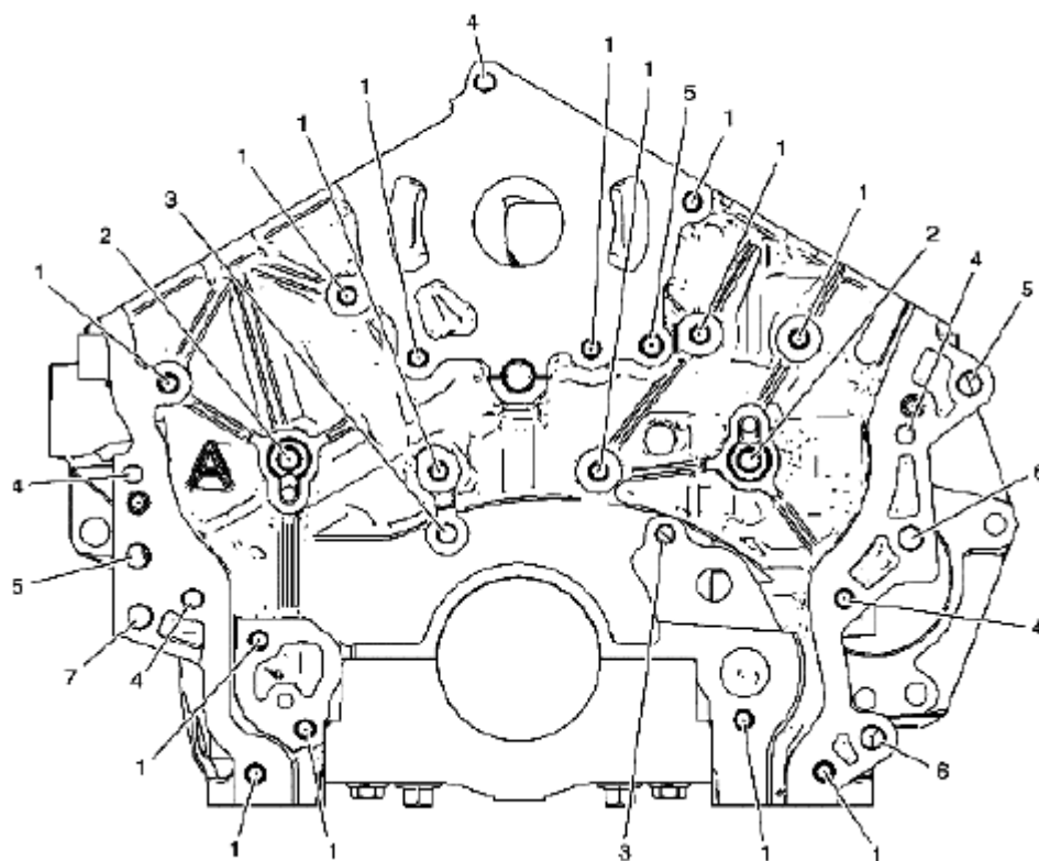
Fig. 1022: Identifying Engine Block Front Courtesy of SUZUKI OF AMERICA CORP.
