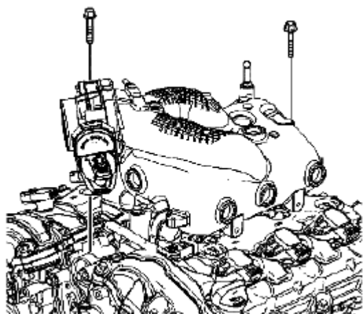
Fig. 983: Identifying Short Intake Manifold Bolts Courtesy of SUZUKI OF AMERICA CORP.
