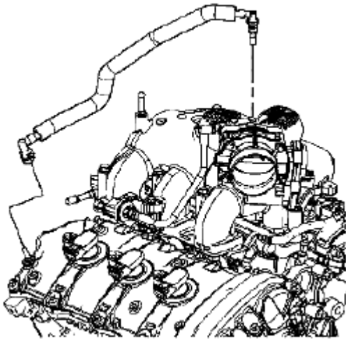
Fig. 272: Identifying Dirty Air PCV Hose Courtesy of SUZUKI OF AMERICA CORP.
