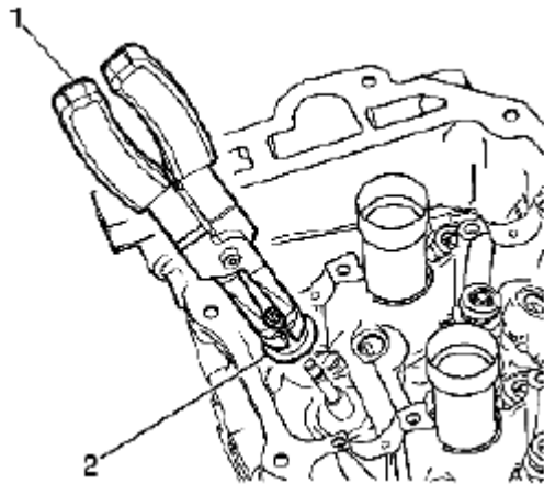
Fig. 199: Identifying Valve Stem Seal (1 Of 2) Courtesy of SUZUKI OF AMERICA CORP.
