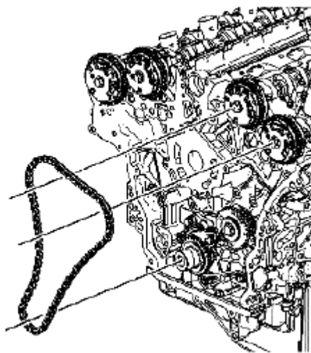
Fig. 345: Identifying Left Secondary Camshaft Drive Chain
