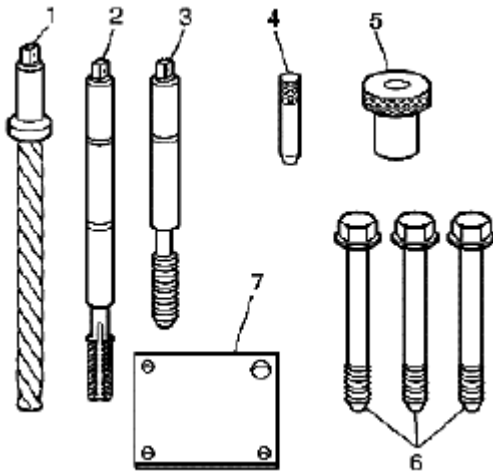
Fig. 641: Identifying Cylinder Head Bolt Hole Thread Repair Tools
