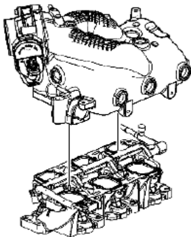
Fig. 560: Identifying Upper Intake Manifold Courtesy of SUZUKI OF AMERICA CORP.
