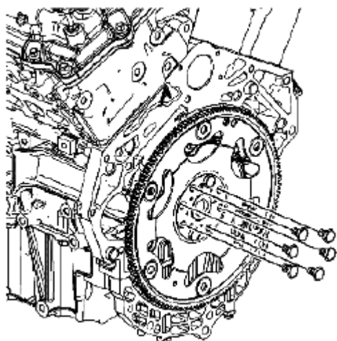
Fig. 996: Identifying Engine Flywheel Bolts Courtesy of SUZUKI OF AMERICA CORP.
