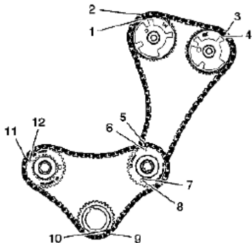
Fig. 892: Identifying Primary & Left Secondary Camshaft Drive Chain Timing Mark Courtesy of SUZUKI OF AMERICA CORP.
