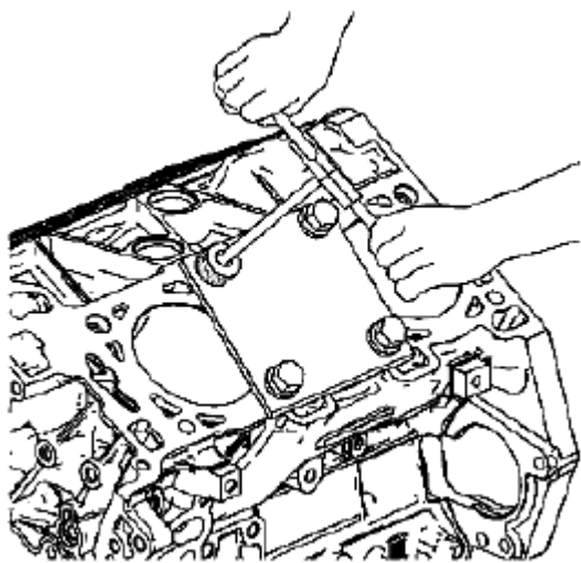
Fig. 646: Applying Threads Of Drilled Hole By Hand Courtesy of SUZUKI OF AMERICA CORP.
