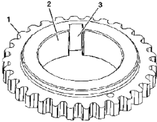
Fig. 512: Identifying Crankshaft Sprocket Courtesy of SUZUKI OF AMERICA CORP.
