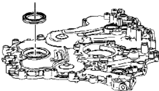
Fig. 526: Identifying Crankshaft Front Oil Seal Courtesy of SUZUKI OF AMERICA CORP.
