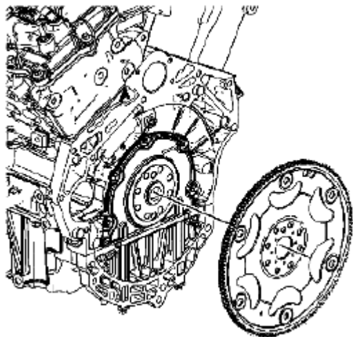
Fig. 993: Identifying Engine Flywheel Courtesy of SUZUKI OF AMERICA CORP.
