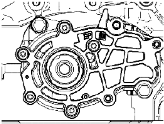
Fig. 748: Identifying Timing Drive Assembly Courtesy of SUZUKI OF AMERICA CORP.
