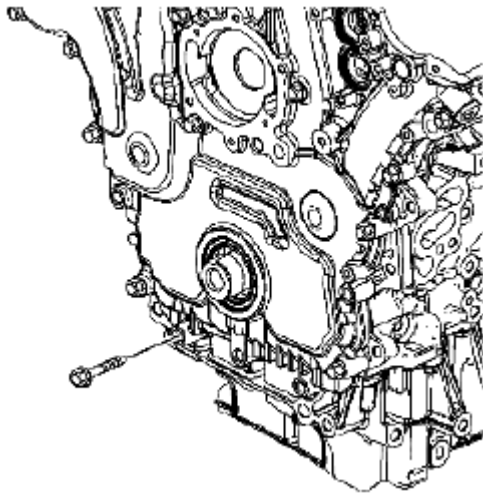
Fig. 294: Identifying Engine Front Cover Bolts Courtesy of SUZUKI OF AMERICA CORP.
