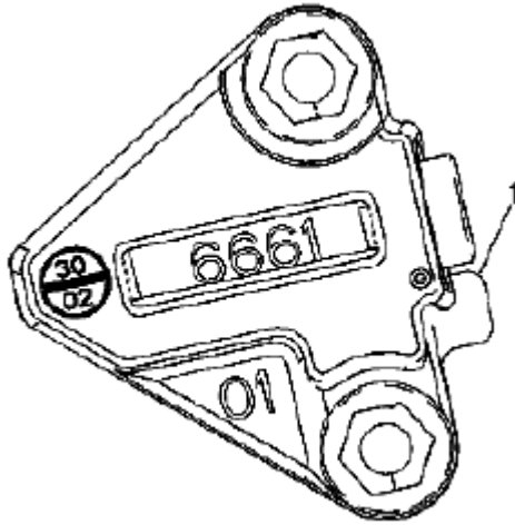
Fig. 846: Identifying Left Secondary Camshaft Drive Chain Tensioner Gasket Tab Courtesy of SUZUKI OF AMERICA CORP.
