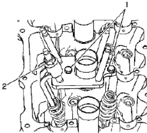
Fig. 211: Identifying Valve Spring Compressor Nut Courtesy of SUZUKI OF AMERICA CORP.
