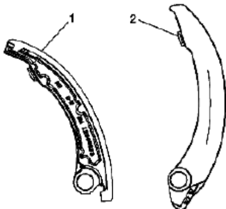
Fig. 828: Identifying Left Secondary Camshaft Drive Chain Shoe (1 Of 2)
