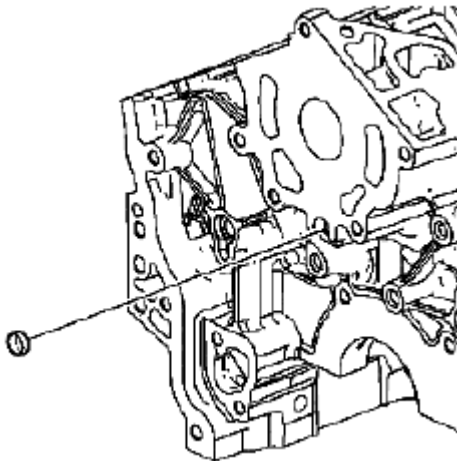
Fig. 399: Identifying Front Oil Gallery Expansion Plug Courtesy of SUZUKI OF AMERICA CORP.
