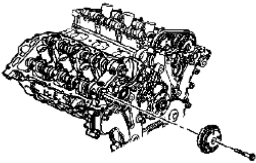
Fig. 173: Identifying Intake Camshaft Position Actuator & Bolt Courtesy of SUZUKI OF AMERICA CORP.
