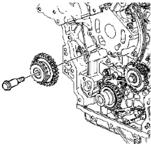
Fig. 332: Identifying Right Camshaft Intermediate Drive Chain Idler & Bolt Courtesy of SUZUKI OF AMERICA CORP.
