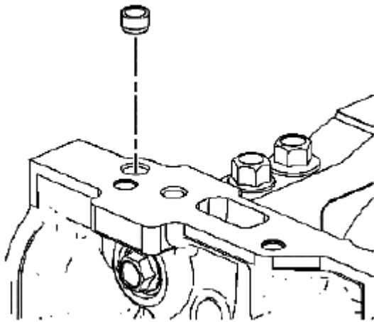
Fig. 390: Identifying Right Front Oil Pan Rail Oil Gallery Expansion Plug
