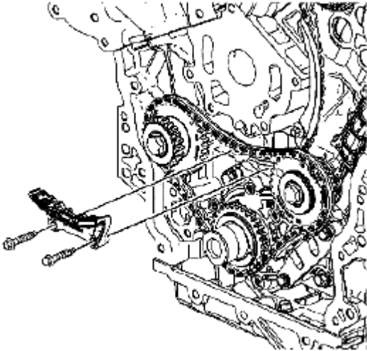
Fig. 327: Identifying Primary Camshaft Drive Chain Upper Guide & Bolts Courtesy of SUZUKI OF AMERICA CORP.
