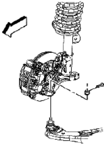
Fig. 231: Removing Lower Ball Joints From Steering Knuckles Courtesy of SUZUKI OF AMERICA CORP.
