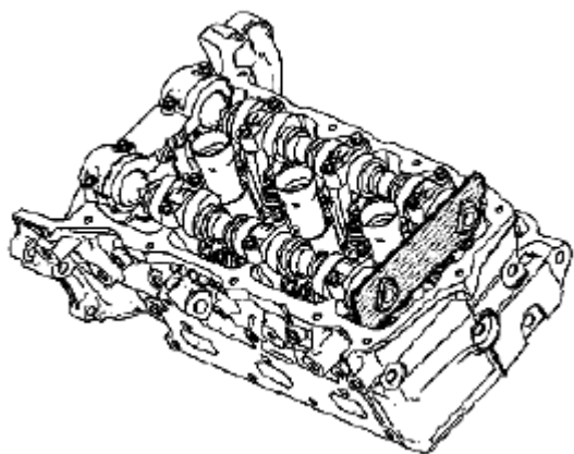
Fig. 882: Identifying EN 46105-2 Onto Rear Of Left Camshafts Courtesy of SUZUKI OF AMERICA CORP.
