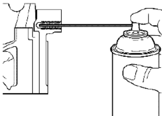
Fig. 615: Applying Spray Cleaner Into Tapped Hole Courtesy of SUZUKI OF AMERICA CORP.
