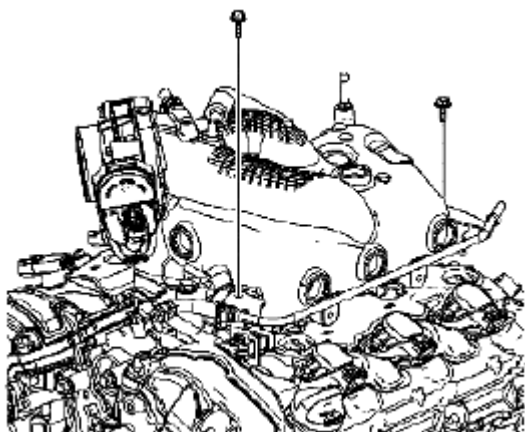
Fig. 269: Identifying Engine Coolant Air Bleed Pipe Bracket Bolts Courtesy of SUZUKI OF AMERICA CORP.
