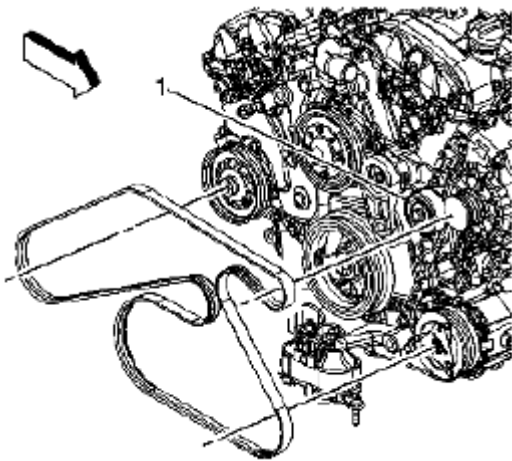
Fig. 38: Locating Drive Belt & Belt Idler Pulley Courtesy of SUZUKI OF AMERICA CORP.
