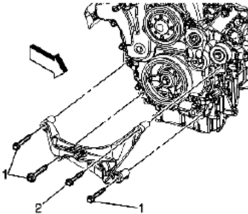
Fig. 49: Removing Right Upper Front Engine Mount Bracket Bolt Courtesy of SUZUKI OF AMERICA CORP.
