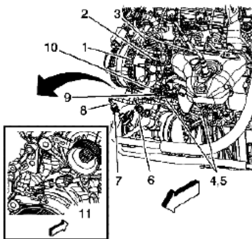
Fig. 248: Connecting Engine Wiring Harness Electrical Connector Courtesy of SUZUKI OF AMERICA CORP.
