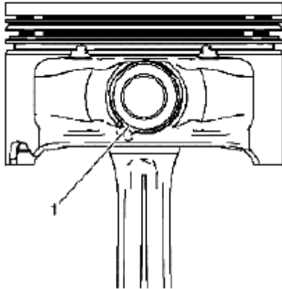
Fig. 432: Identifying Piston Pin Retainers Courtesy of SUZUKI OF AMERICA CORP.
