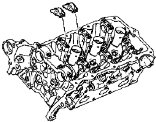
Fig. 190: Identifying Rocker Arms
