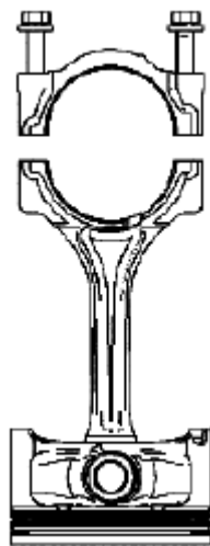
Fig. 382: Identifying Connecting Rod Cap Courtesy of SUZUKI OF AMERICA CORP.
