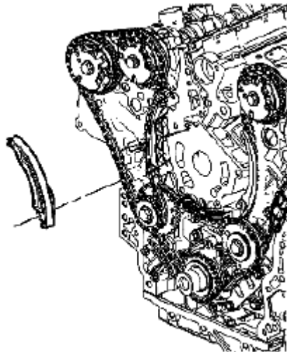
Fig. 919: Identifying Right Secondary Camshaft Drive Chain Shoe (2 Of 2) Courtesy of SUZUKI OF AMERICA CORP.
