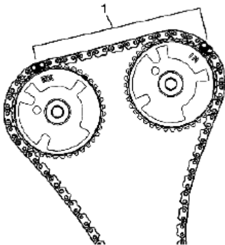
Fig. 907: Identifying Timing Camshaft Drive Chain Link Mark (2 Of 5) Courtesy of SUZUKI OF AMERICA CORP.
