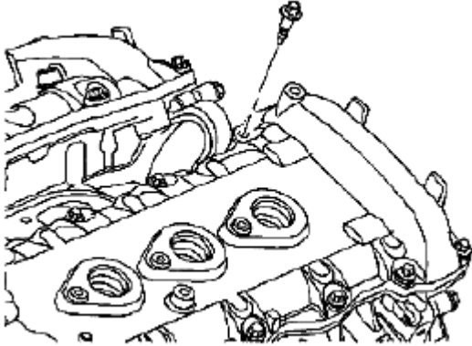
Fig. 112: Identifying Right Camshaft Cover Bolts Courtesy of SUZUKI OF AMERICA CORP.
