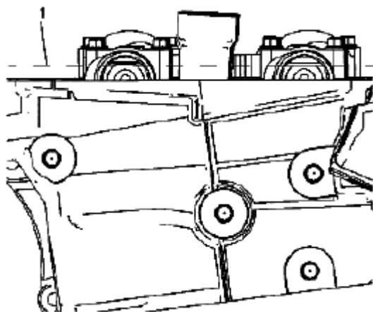
Fig. 769: Identifying Camshafts Parallel Line Courtesy of SUZUKI OF AMERICA CORP.
