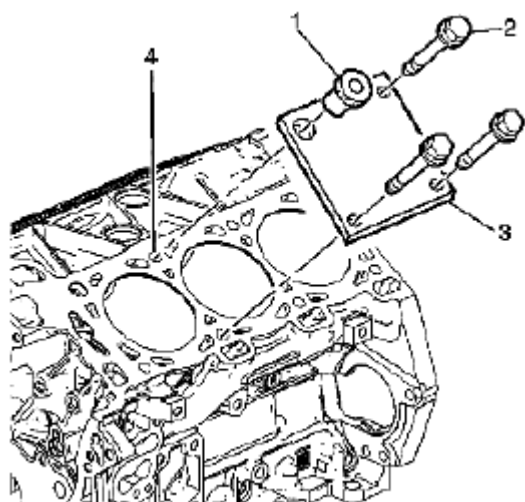
Fig. 648: Identifying Fixture Plate & Bolts Courtesy of SUZUKI OF AMERICA CORP.
