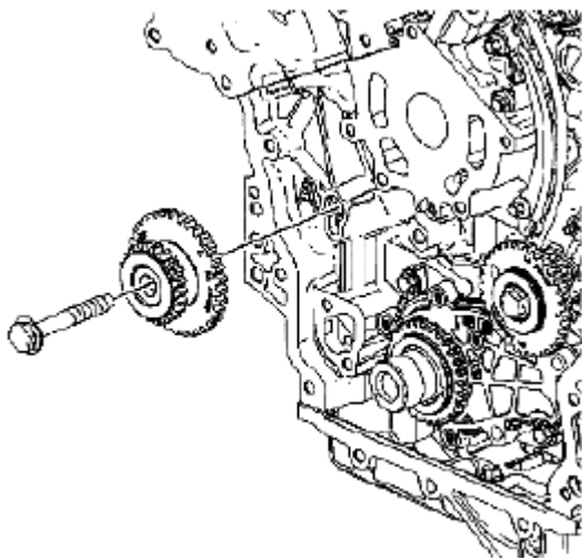
Fig. 852: Identifying Camshaft Intermediate Drive Chain Idler & Bolt Courtesy of SUZUKI OF AMERICA CORP.
