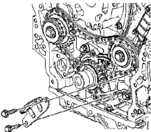
Fig. 328: Identifying Primary Camshaft Drive Chain Lower Guide & Bolts Courtesy of SUZUKI OF AMERICA CORP.
