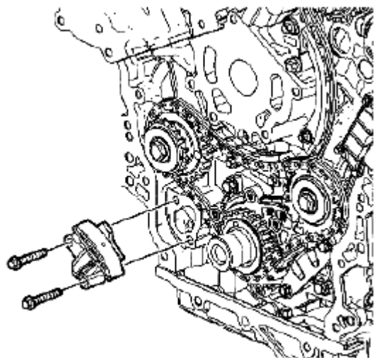
Fig. 876: Identifying Primary Camshaft Drive Chain Tensioner & Bolt Courtesy of SUZUKI OF AMERICA CORP.
