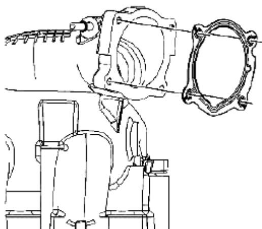
Fig. 564: Identifying Throttle Body Gasket Courtesy of SUZUKI OF AMERICA CORP.
