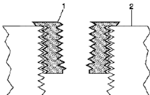
Fig. 639: Identifying Insert & Proper Installation Courtesy of SUZUKI OF AMERICA CORP.
