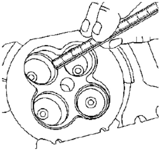
Fig. 454: Measuring Valve Seat Width In Cylinder Head Courtesy of SUZUKI OF AMERICA CORP.
