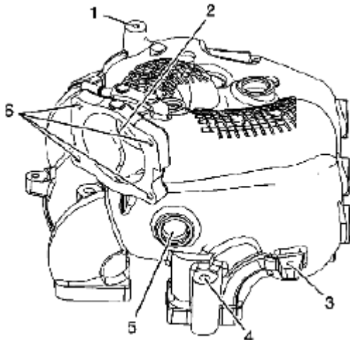
Fig. 571: Identifying Upper Intake Manifold Parts (2 Of 3) Courtesy of SUZUKI OF AMERICA CORP.
