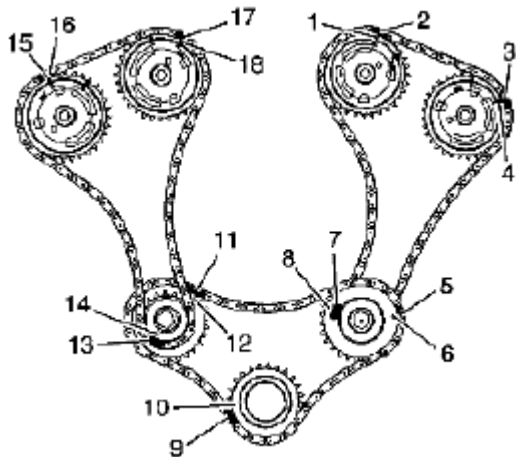
Fig. 184: Identifying Camshaft Timing Chain Mark Courtesy of SUZUKI OF AMERICA CORP.
