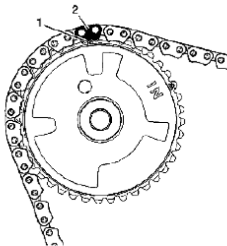
Fig. 819: Identifying Timing Camshaft Drive Chain Link Mark (3 Of 4) Courtesy of SUZUKI OF AMERICA CORP.
