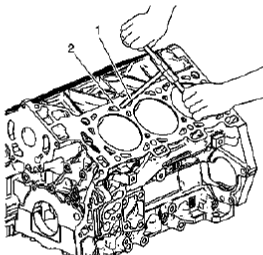
Fig. 656: Applying Thread On Surface Of Engine Block Deck Courtesy of SUZUKI OF AMERICA CORP.
