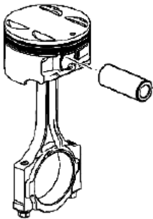
Fig. 431: Identifying Piston Pin & Connecting Rod Courtesy of SUZUKI OF AMERICA CORP.
