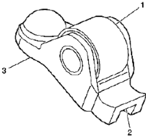
Fig. 477: Identifying Camshaft Follower Roller Courtesy of SUZUKI OF AMERICA CORP.
