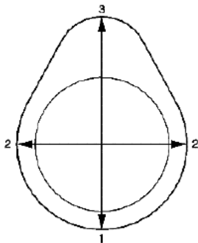
Fig. 475: Measuring Points Of Camshaft Lobes
