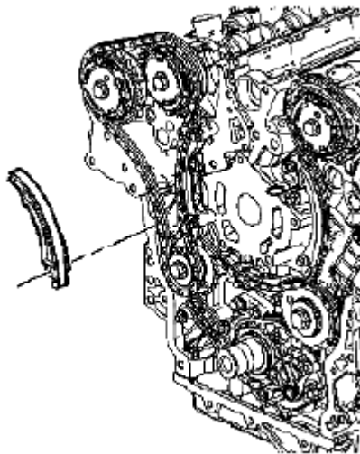
Fig. 140: Identifying Right Bank Secondary Camshaft Drive Chain Tensioner Courtesy of SUZUKI OF AMERICA CORP.
