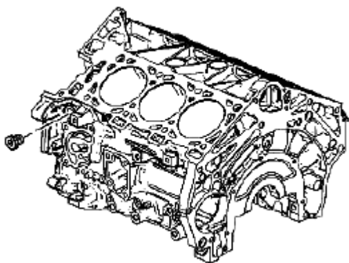
Fig. 692: Identifying M20 Left Side Oil Gallery Threaded Plug Courtesy of SUZUKI OF AMERICA CORP.
