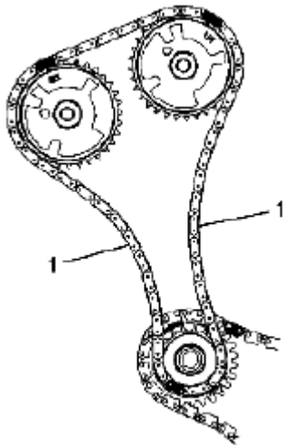
Fig. 903: Identifying Timing Camshaft Drive Chain Link Mark (5 Of 5)
