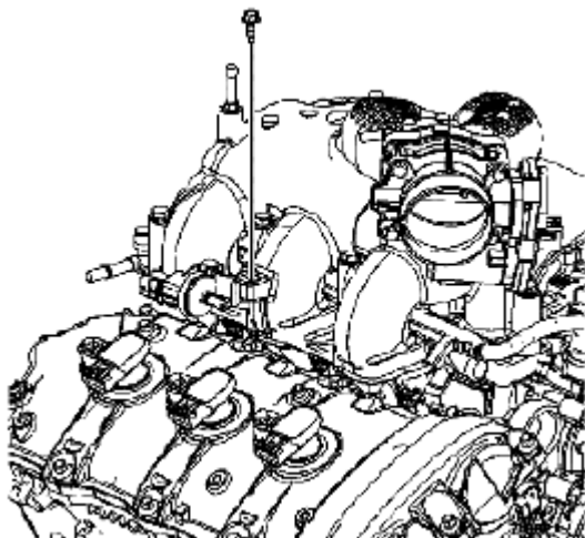
Fig. 274: Identifying EVAP Solenoid Bolt Courtesy of SUZUKI OF AMERICA CORP.
