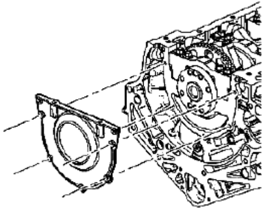
Fig. 376: Identifying Crankshaft Rear Oil Seal Housing Courtesy of SUZUKI OF AMERICA CORP.
