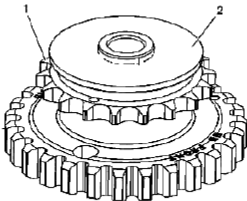
Fig. 484: Identifying Intermediate Sprocket
