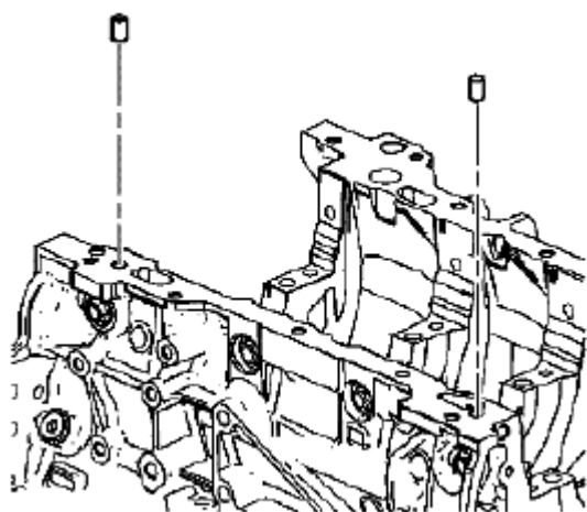
Fig. 697: Identifying Cylinder Block-To-Oil Pan Alignment Dowels Courtesy of SUZUKI OF AMERICA CORP.
