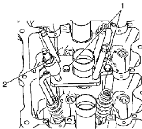
Fig. 205: Identifying Valve Spring Compressor Nut Courtesy of SUZUKI OF AMERICA CORP.
