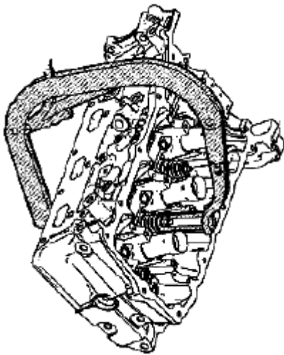
Fig. 440: Compressing Valve Springs Courtesy of SUZUKI OF AMERICA CORP.
