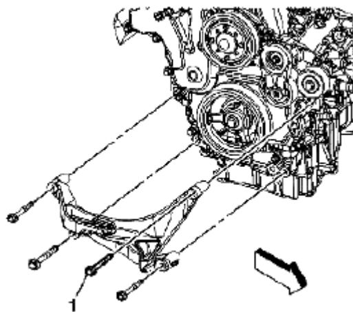
Fig. 51: Removing Engine Mount From Lower Bracket Courtesy of SUZUKI OF AMERICA CORP.
