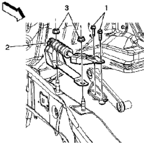
Fig. 63: Removing Engine Mount Strut To Bracket Bolts Courtesy of SUZUKI OF AMERICA CORP.
