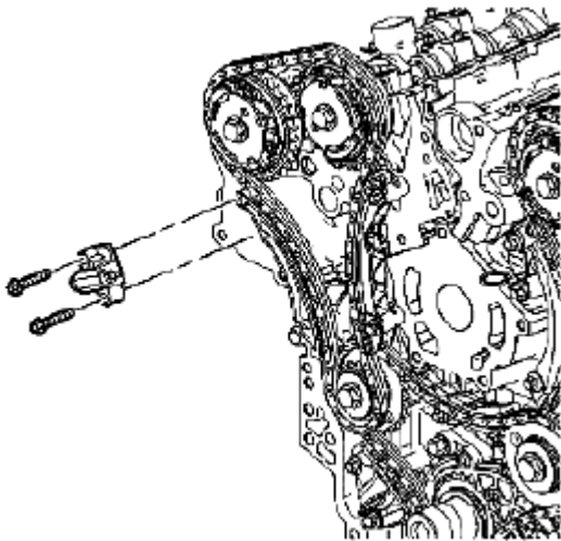
Fig. 134: Identifying Right Bank Secondary Camshaft Drive Chain Tensioner Courtesy of SUZUKI OF AMERICA CORP.
