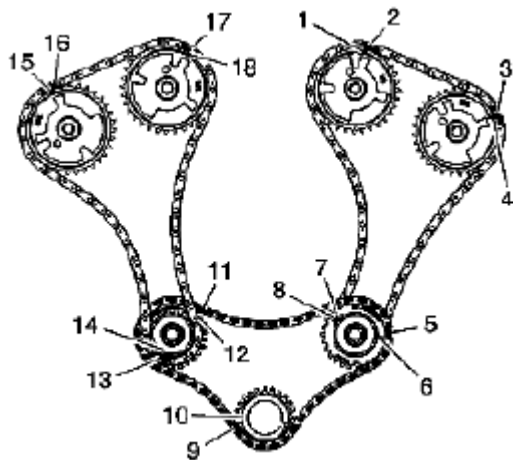
Fig. 929: Identifying Camshaft Drive Chain Timing Marks Courtesy of SUZUKI OF AMERICA CORP.
