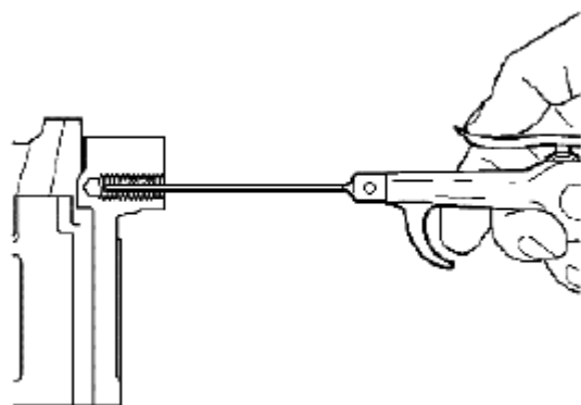
Fig. 649: Applying Compressed Air Into Tapped Hole Courtesy of SUZUKI OF AMERICA CORP.
