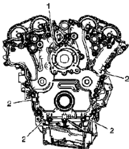
Fig. 116: Identifying "Jackscrew" Hole Courtesy of SUZUKI OF AMERICA CORP.
