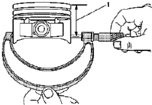
Fig. 421: Measuring Piston Width Courtesy of SUZUKI OF AMERICA CORP.
