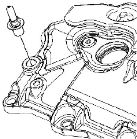
Fig. 549: Identifying PCV Orifice Into Right Camshaft Cover Courtesy of SUZUKI OF AMERICA CORP.
