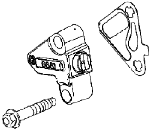
Fig. 337: Identifying Left Secondary Camshaft Drive Chain Tensioner Gasket Courtesy of SUZUKI OF AMERICA CORP.
