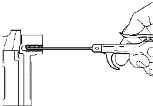
Fig. 661: Applying Compressed Air Into Tapped Hole Courtesy of SUZUKI OF AMERICA CORP.
