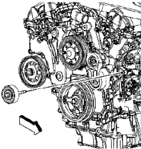
Fig. 43: Installing Drive Belt Idler Pulley Courtesy of SUZUKI OF AMERICA CORP.
