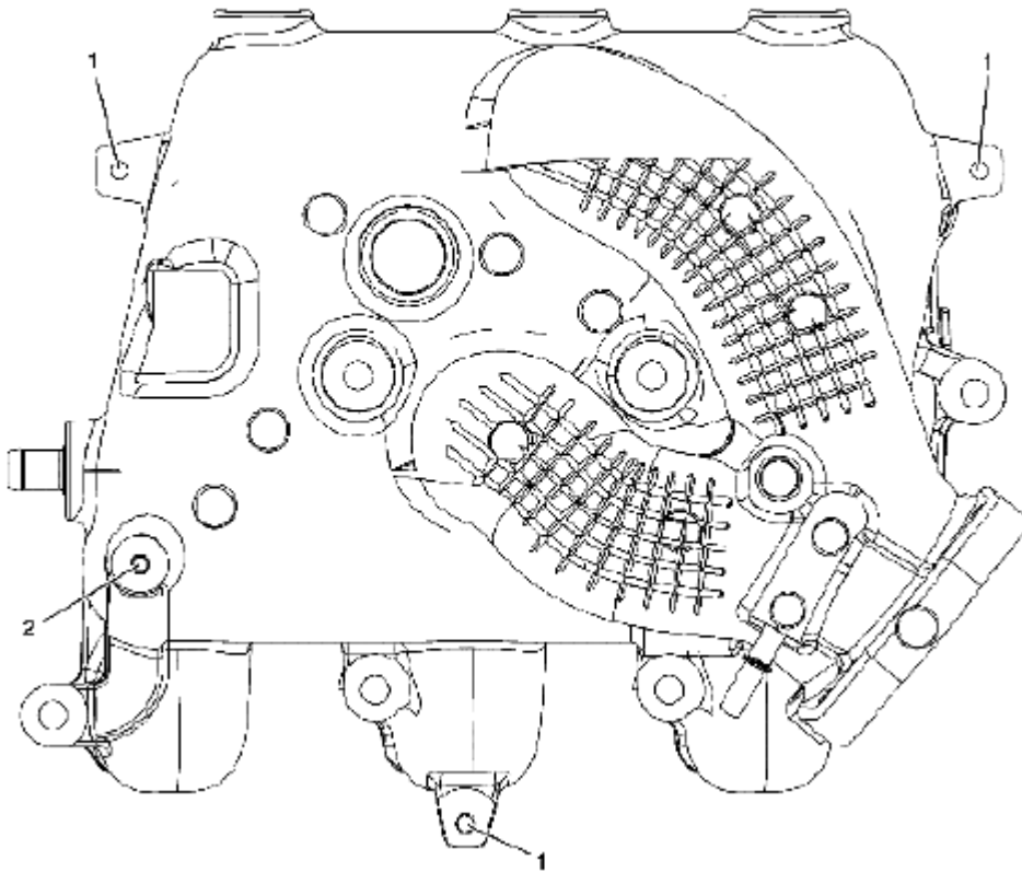
Fig. 1030: Identifying Upper Intake Manifold - Top Courtesy of SUZUKI OF AMERICA CORP.
