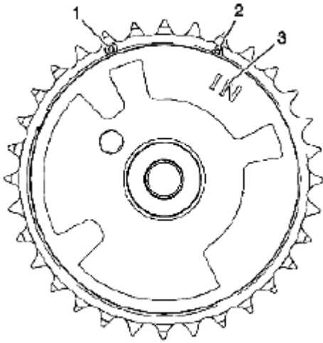
Fig. 773: Identifying Camshaft Position Actuator Courtesy of SUZUKI OF AMERICA CORP.
