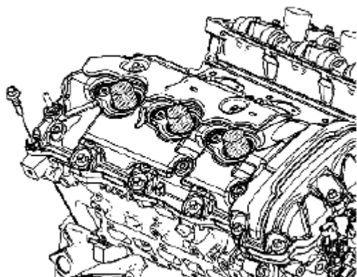
Fig. 975: Identifying Right Camshaft Cover Bolts Courtesy of SUZUKI OF AMERICA CORP.
