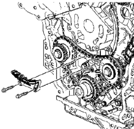
Fig. 870: Identifying Upper Primary Camshaft Drive Chain Guide & Bolts Courtesy of SUZUKI OF AMERICA CORP.
