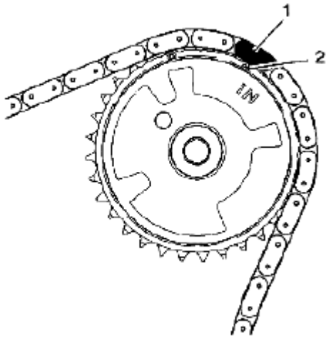
Fig. 902: Identifying Timing Camshaft Drive Chain Link Mark (4 Of 5)
