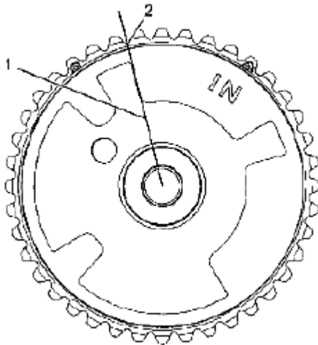
Fig. 777: Identifying Intake Camshaft Actuator Edge Of Reluctor Wheel Courtesy of SUZUKI OF AMERICA CORP.
