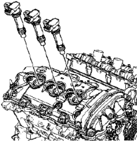
Fig. 286: Identifying Ignition Coils Courtesy of SUZUKI OF AMERICA CORP.
