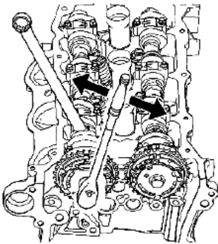
Fig. 180: Tightening Camshaft Position Actuators
