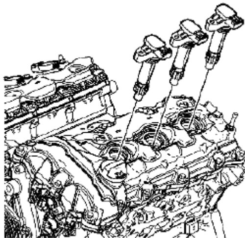
Fig. 968: Identifying Ignition Coils Courtesy of SUZUKI OF AMERICA CORP.
