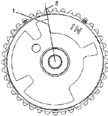
Fig. 788: Identifying Intake Camshaft Actuator Edge Of Reluctor Wheel Courtesy of SUZUKI OF AMERICA CORP.
