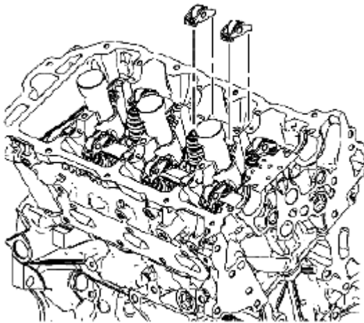
Fig. 187: Identifying Rocker Arms Courtesy of SUZUKI OF AMERICA CORP.
