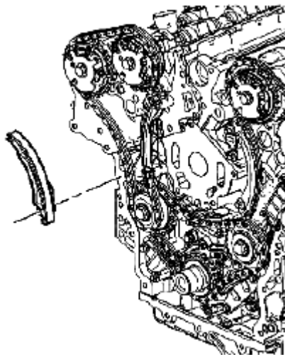
Fig. 916: Identifying Right Secondary Camshaft Drive Chain Shoe (2 Of 2) Courtesy of SUZUKI OF AMERICA CORP.
