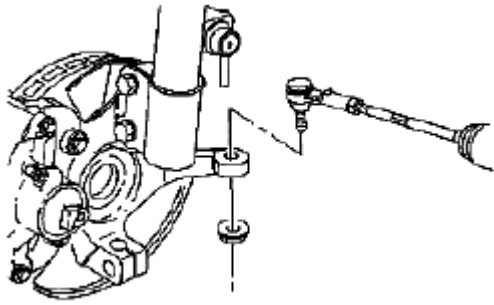
Fig. 256: Identifying Tie Rod Ends Courtesy of SUZUKI OF AMERICA CORP.
