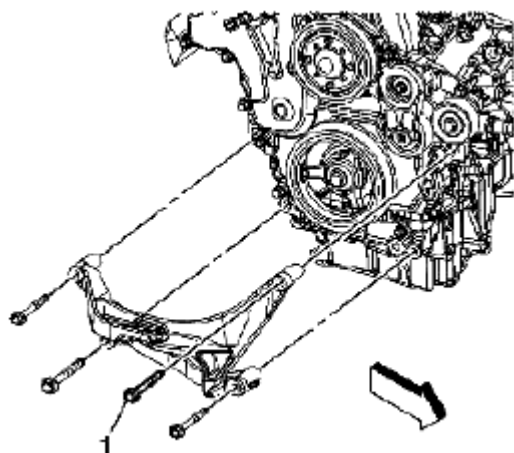
Fig. 53: Installing Engine Mount Upper Bracket & Bolt Courtesy of SUZUKI OF AMERICA CORP.
