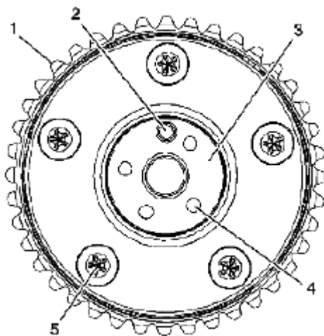
Fig. 506: Identifying Back Of Right Intake Camshaft Position Actuators Courtesy of SUZUKI OF AMERICA CORP.
