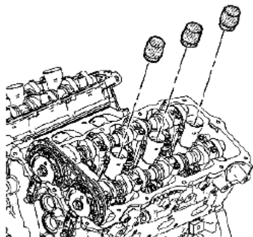
Fig. 108: Installing EN 46101 Onto Spark Plug Tubes Courtesy of SUZUKI OF AMERICA CORP.
