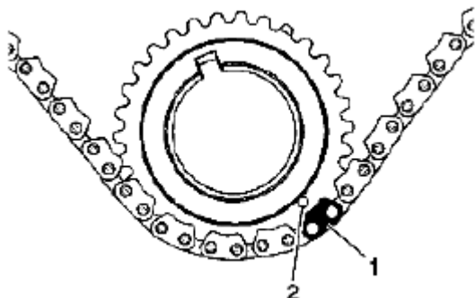
Fig. 863: Identifying Crankshaft Sprocket Timing Mark Courtesy of SUZUKI OF AMERICA CORP.
