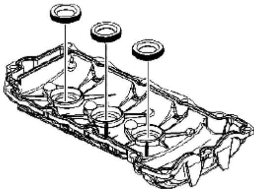
Fig. 542: Identifying Right Spark Plug Shield Tube Seals Courtesy of SUZUKI OF AMERICA CORP.
