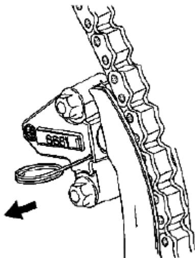
Fig. 847: Pulling EN 46112 From Left Secondary Camshaft Drive Chain Tensioner Courtesy of SUZUKI OF AMERICA CORP.
