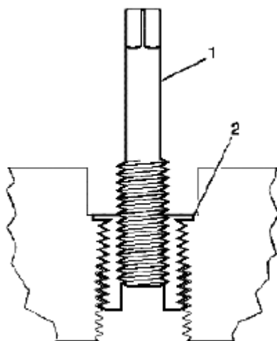
Fig. 621: Applying Insert Into Tapped Hole (2 Of 2) Courtesy of SUZUKI OF AMERICA CORP.
