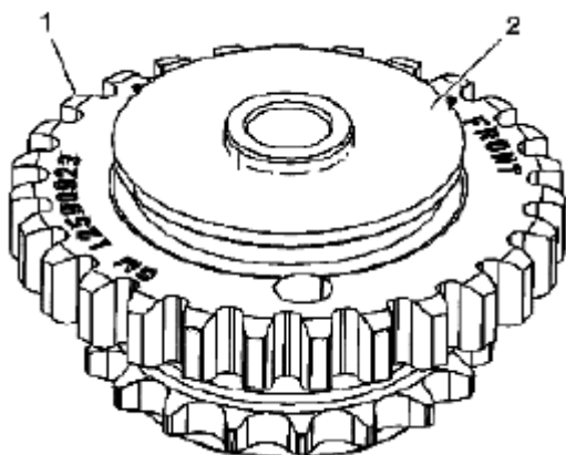
Fig. 486: Identifying Back Of Right Intermediate Sprocket Courtesy of SUZUKI OF AMERICA CORP.
