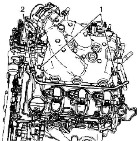
Fig. 82: Identifying Bleed Pipe Bolts Courtesy of SUZUKI OF AMERICA CORP.
