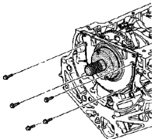
Fig. 739: Identifying Crankshaft Rear Oil Seal Housing Bolts Courtesy of SUZUKI OF AMERICA CORP.
