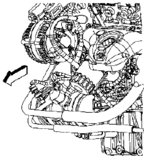
Fig. 45: Installing Battery Cable Courtesy of SUZUKI OF AMERICA CORP.
