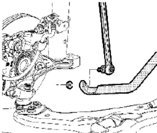
Fig. 255: Identifying Stabilizer Shaft Links Courtesy of SUZUKI OF AMERICA CORP.
