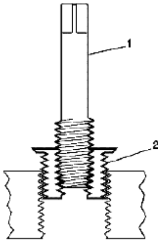
Fig. 636: Applying Insert Into Tapped Hole Courtesy of SUZUKI OF AMERICA CORP.
