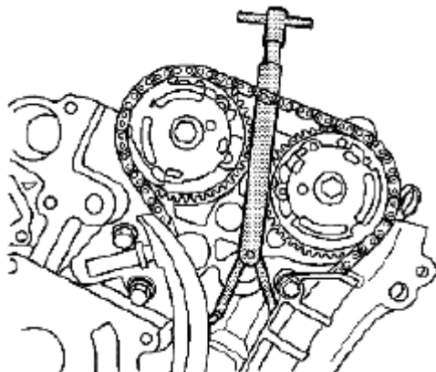
Fig. 165: Holding Timing Chain With EN-48313 Courtesy of SUZUKI OF AMERICA CORP.
