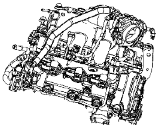
Fig. 75: Disconnecting PCV Line From Top Of Intake Manifold Courtesy of SUZUKI OF AMERICA CORP.
