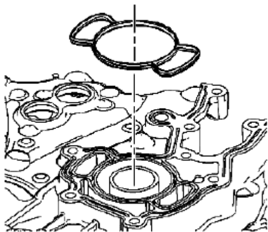
Fig. 122: Identifying Cylinder Block Seal
