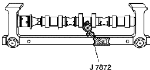
Fig. 471: Measuring Camshaft Runout Courtesy of SUZUKI OF AMERICA CORP.
