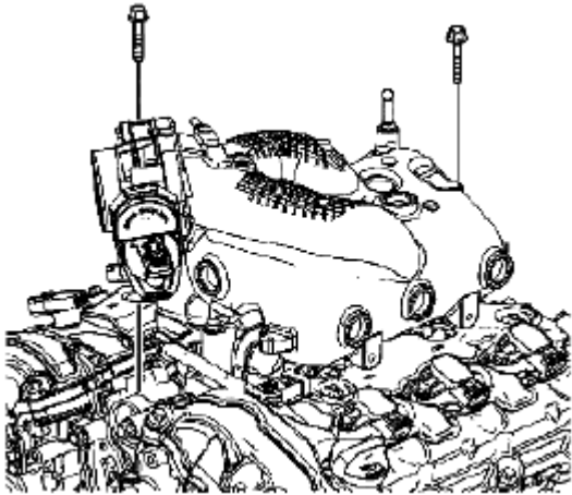
Fig. 277: Identifying Short Intake Manifold Bolts Courtesy of SUZUKI OF AMERICA CORP.
