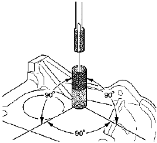
Fig. 591: Identifying Drilling Angle Courtesy of SUZUKI OF AMERICA CORP.
