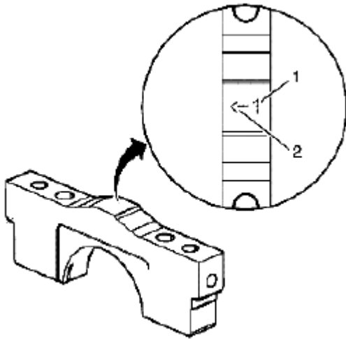
Fig. 704: Identifying Main Bearing Caps Mark Courtesy of SUZUKI OF AMERICA CORP.
