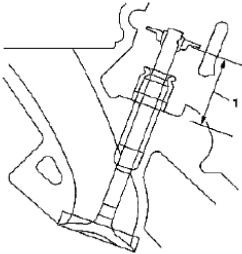
Fig. 459: Identifying Distance Between Cylinder Head To Bottom Of Valve Spring Retainer Courtesy of SUZUKI OF AMERICA CORP.
