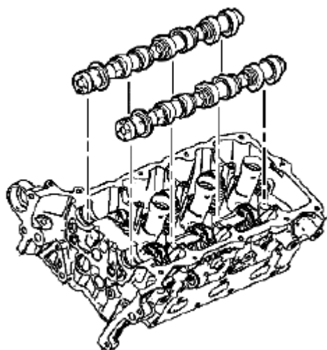
Fig. 768: Identifying Left Intake & Left Exhaust Camshafts Courtesy of SUZUKI OF AMERICA CORP.
