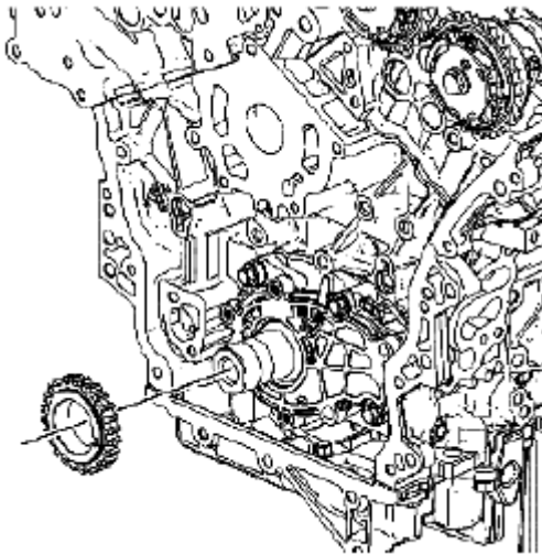
Fig. 149: Identifying Crankshaft Sprocket Courtesy of SUZUKI OF AMERICA CORP.
