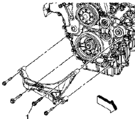
Fig. 61: Installing Engine Mount Upper Bracket & Bolt Courtesy of SUZUKI OF AMERICA CORP.
