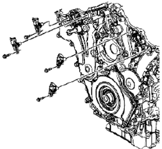
Fig. 958: Identifying Camshaft Position Sensors Courtesy of SUZUKI OF AMERICA CORP.
