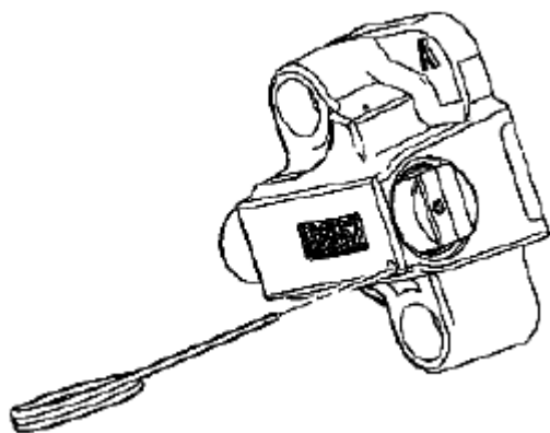
Fig. 933: Inserting EN 46112 Into Access Hole Of Right Secondary Camshaft Drive Chain
