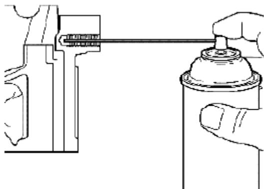
Fig. 631: Applying Spray Cleaner Into Tapped Hole Courtesy of SUZUKI OF AMERICA CORP.
