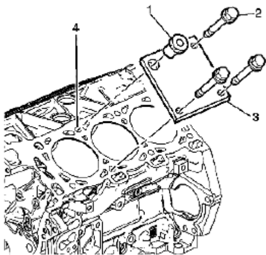
Fig. 642: Positioning Fixture Plate With Bushing Courtesy of SUZUKI OF AMERICA CORP.
