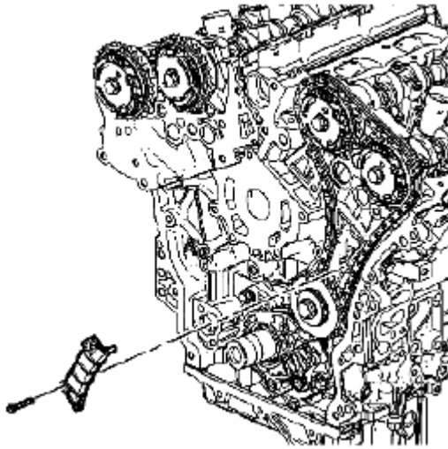
Fig. 142: Identifying Left Bank Secondary Camshaft Drive Chain Guide (1 Of 2) Courtesy of SUZUKI OF AMERICA CORP.
