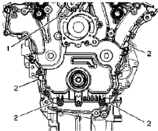
Fig. 305: Identifying Jackscrew Hole Courtesy of SUZUKI OF AMERICA CORP.
