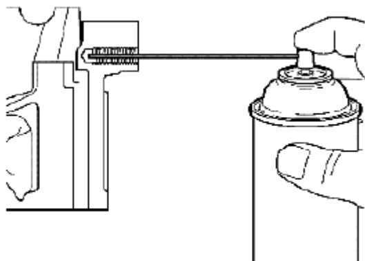
Fig. 665: Applying Spray Cleaner Into Tapped Hole Courtesy of SUZUKI OF AMERICA CORP.
