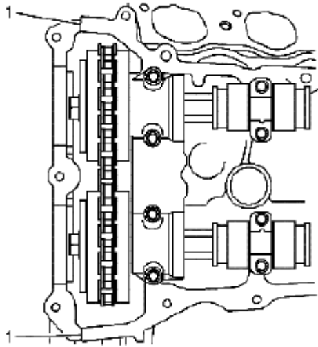
Fig. 102: Placing Bead Of RTV Sealant On Engine Front Cover Split Lines Courtesy of SUZUKI OF AMERICA CORP.
