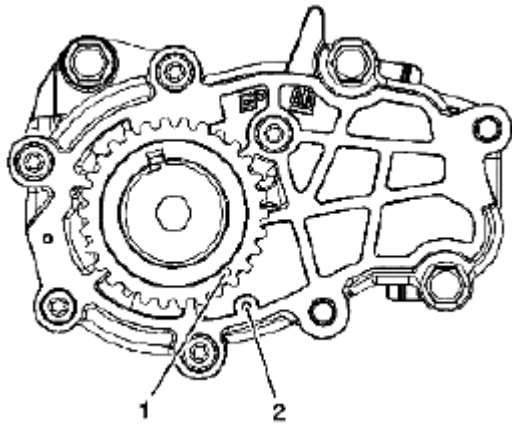
Fig. 800: Aligning Timing Mark On Crankshaft Sprocket Timing Mark And Oil Pump Cover Courtesy of SUZUKI OF AMERICA CORP.
