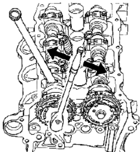
Fig. 186: Tightening Camshaft Position Actuators Courtesy of SUZUKI OF AMERICA CORP.
