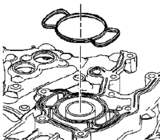
Fig. 940: Identifying Cylinder Block Seal
