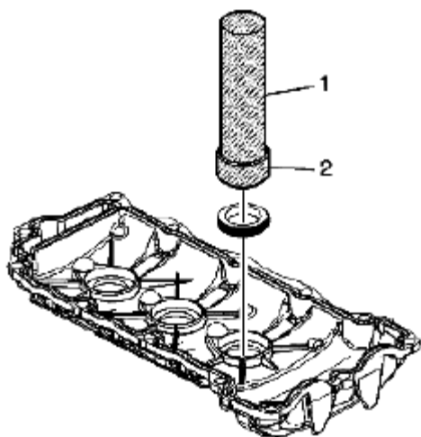
Fig. 556: Installing Right Spark Plug Shield Tube Coil Seals Courtesy of SUZUKI OF AMERICA CORP.
