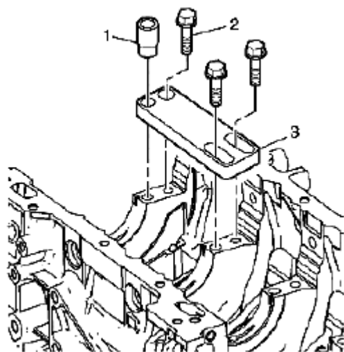
Fig. 687: Identifying Fixture Plate & Bolts Courtesy of SUZUKI OF AMERICA CORP.
