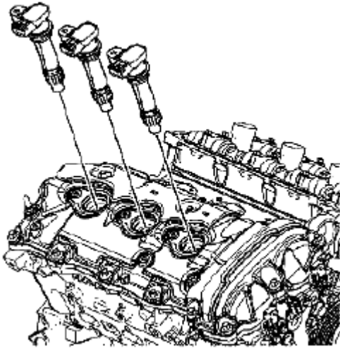
Fig. 979: Identifying Ignition Coils Courtesy of SUZUKI OF AMERICA CORP.
