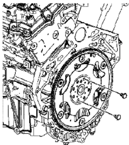
Fig. 994: Identifying Engine Flywheel Bolts Courtesy of SUZUKI OF AMERICA CORP.
