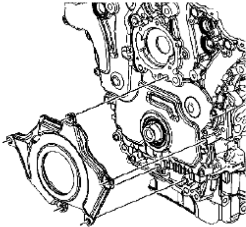
Fig. 953: Identifying Engine Front Cover Deadener Courtesy of SUZUKI OF AMERICA CORP.
