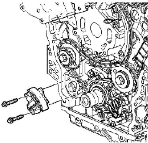
Fig. 156: Identifying Primary Camshaft Drive Chain Tensioner Courtesy of SUZUKI OF AMERICA CORP.
