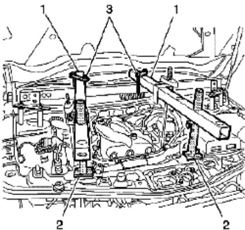
Fig. 1041: Identifying Engine Support Fixture Cross Bars
