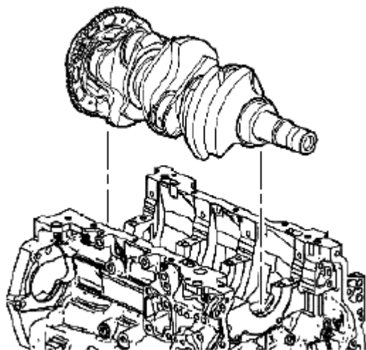
Fig. 703: Identifying Crankshaft Courtesy of SUZUKI OF AMERICA CORP.
