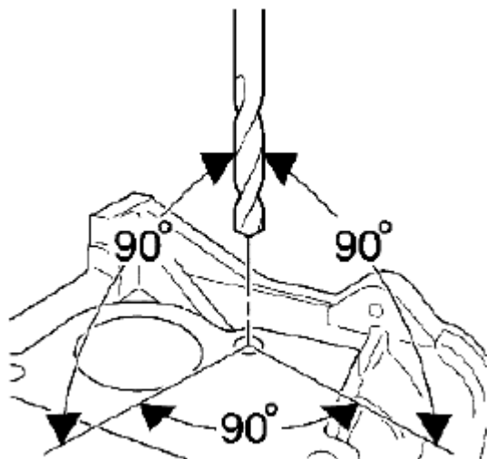
Fig. 590: Identifying Drilling Angle Courtesy of SUZUKI OF AMERICA CORP.
