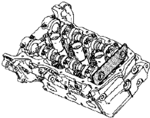
Fig. 120: Identifying EN 46105-2 On Left Camshafts Courtesy of SUZUKI OF AMERICA CORP.
