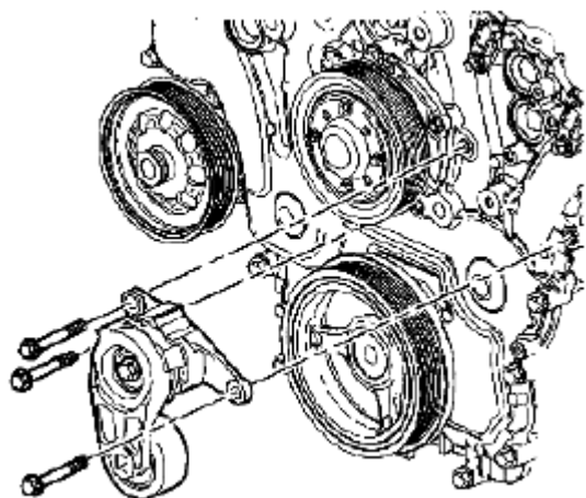
Fig. 1002: Identifying Left Drive Belt Tensioner Assembly & Bolts Courtesy of SUZUKI OF AMERICA CORP.
