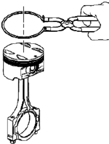
Fig. 435: Installing Piston Rings Using Ring Expander
