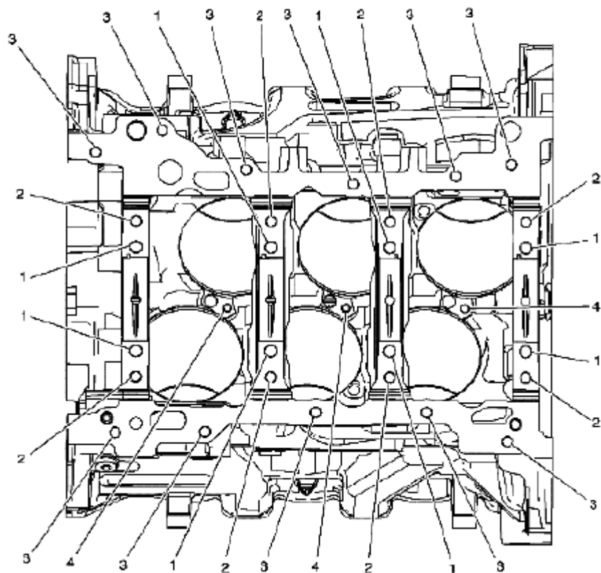
Fig. 1026: Identifying Engine Block Bottom Courtesy of SUZUKI OF AMERICA CORP.
