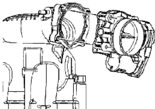
Fig. 563: Identifying Throttle Body Courtesy of SUZUKI OF AMERICA CORP.
