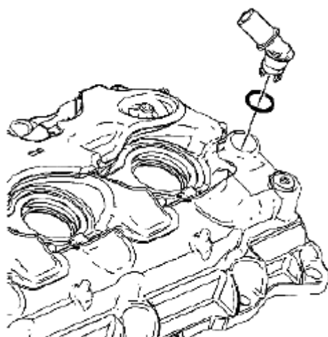
Fig. 550: Identifying PCV Fitting With O-Ring Courtesy of SUZUKI OF AMERICA CORP.
