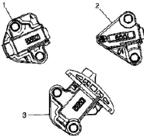
Fig. 930: Identifying Right Secondary Camshaft Drive Chain Tensioner Courtesy of SUZUKI OF AMERICA CORP.
