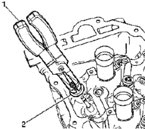
Fig. 209: Identifying Valve Stem Seal (2 Of 2) Courtesy of SUZUKI OF AMERICA CORP.
