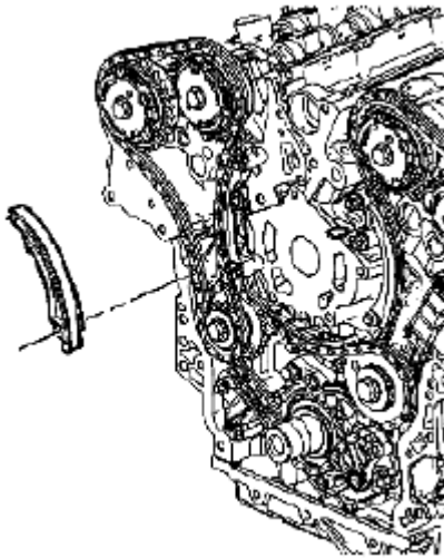
Fig. 141: Identifying Right Bank Secondary Camshaft Drive Chain Tensioner Courtesy of SUZUKI OF AMERICA CORP.
