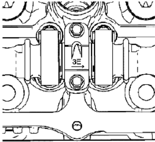
Fig. 754: Identifying Camshaft Bearing Caps Mark Courtesy of SUZUKI OF AMERICA CORP.
