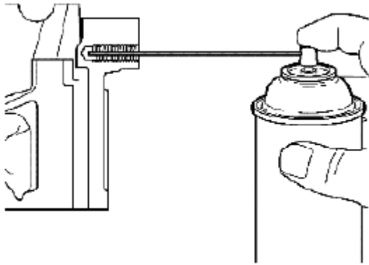
Fig. 650: Applying Spray Cleaner Into Tapped Hole Courtesy of SUZUKI OF AMERICA CORP.
