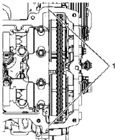
Fig. 973: Placing Bead Of RTV Sealant On Engine Front Cover Split Lines Courtesy of SUZUKI OF AMERICA CORP.
