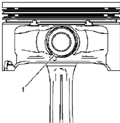
Fig. 418: Identifying Piston Pin Retainer Courtesy of SUZUKI OF AMERICA CORP.
