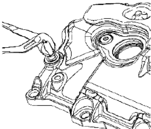
Fig. 547: Removing Old PCV Orifice Courtesy of SUZUKI OF AMERICA CORP.
