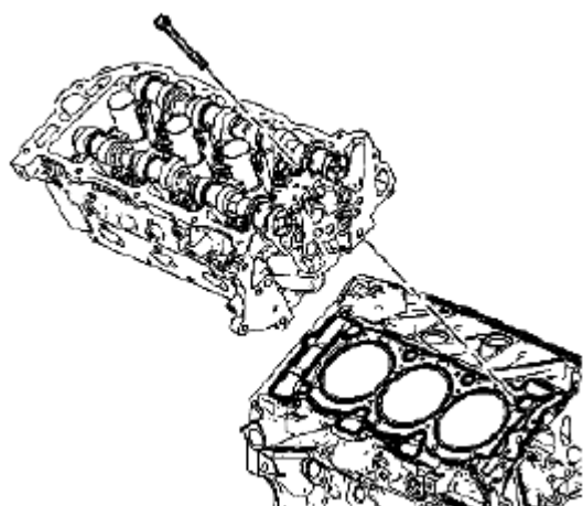
Fig. 742: Identifying Right Cylinder Head Courtesy of SUZUKI OF AMERICA CORP.
