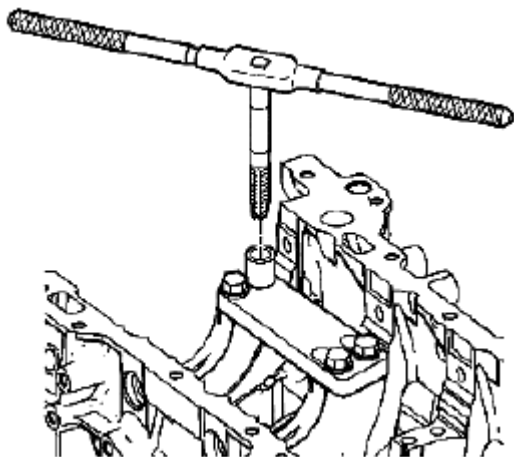
Fig. 662: Applying Threads Of Drilled Hole By Hand Courtesy of SUZUKI OF AMERICA CORP.
