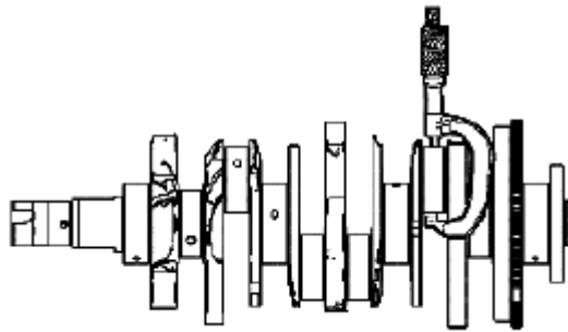
Fig. 411: Checking Crankshaft Main Journals Courtesy of SUZUKI OF AMERICA CORP.
