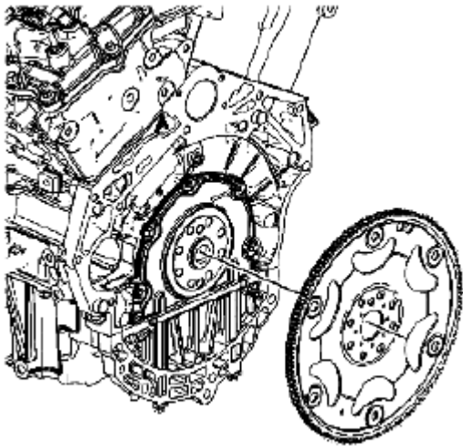
Fig. 223: Identifying Engine Flywheel Courtesy of SUZUKI OF AMERICA CORP.
