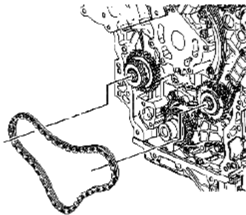
Fig. 151: Identifying Primary Camshaft Timing Chain Courtesy of SUZUKI OF AMERICA CORP.
