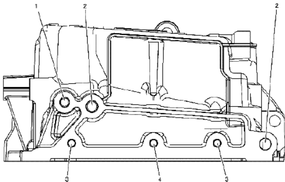
Fig. 1033: Identifying Oil Pan Front Courtesy of SUZUKI OF AMERICA CORP.
