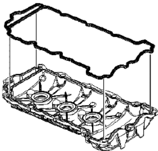
Fig. 541: Identifying Right Camshaft Cover Gasket Courtesy of SUZUKI OF AMERICA CORP.
