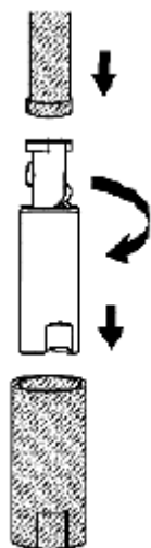
Fig. 922: Identifying Right Secondary Camshaft Drive Chain Tensioner Plunger Courtesy of SUZUKI OF AMERICA CORP.
