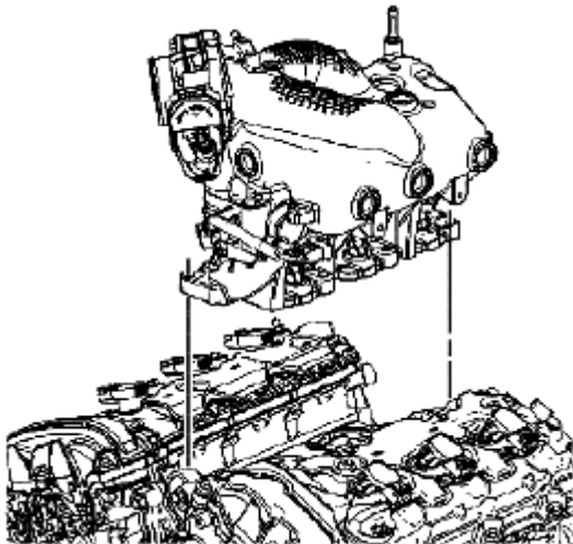
Fig. 982: Identifying Intake Manifold Assembly Courtesy of SUZUKI OF AMERICA CORP.
