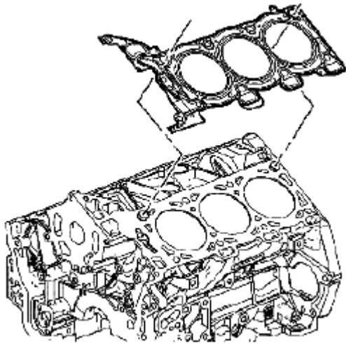
Fig. 215: Identifying Cylinder Head Gasket Courtesy of SUZUKI OF AMERICA CORP.
