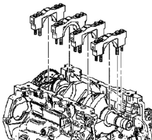
Fig. 712: Identifying Crankshaft Bearing Caps Courtesy of SUZUKI OF AMERICA CORP.
