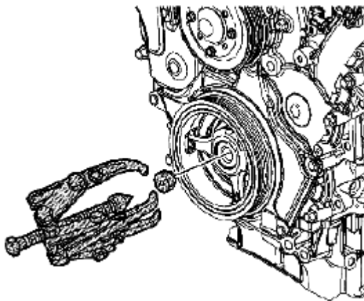
Fig. 264: Identifying Special Tool (J 38416-2) Courtesy of SUZUKI OF AMERICA CORP.
