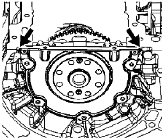
Fig. 375: Locating Edge Of Crankshaft Rear Oil Seal Housing Shear RTV Sealant Courtesy of SUZUKI OF AMERICA CORP.
