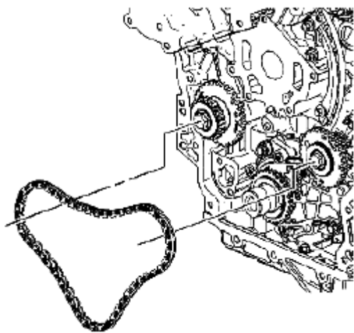
Fig. 331: Identifying Primary Camshaft Drive Chain Courtesy of SUZUKI OF AMERICA CORP.
