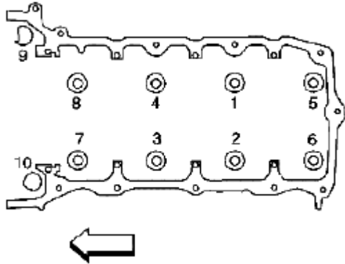
Fig. 759: Identifying M11 Cylinder Head Bolts In Sequence Courtesy of SUZUKI OF AMERICA CORP.
