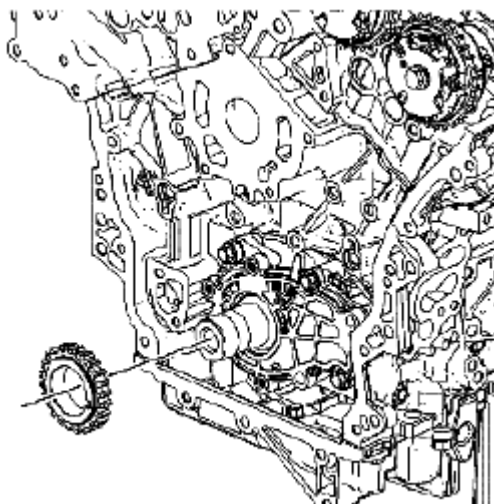
Fig. 796: Identifying Crankshaft Sprocket Courtesy of SUZUKI OF AMERICA CORP.
