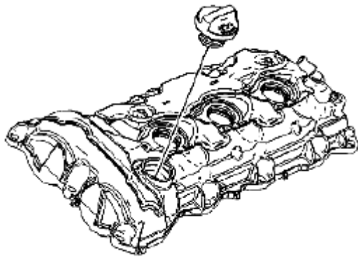
Fig. 537: Identifying Oil Fill Cap Courtesy of SUZUKI OF AMERICA CORP.
