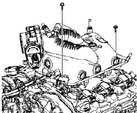
Fig. 991: Identifying Engine Coolant Air Bleed Pipe Bracket Bolts Courtesy of SUZUKI OF AMERICA CORP.
