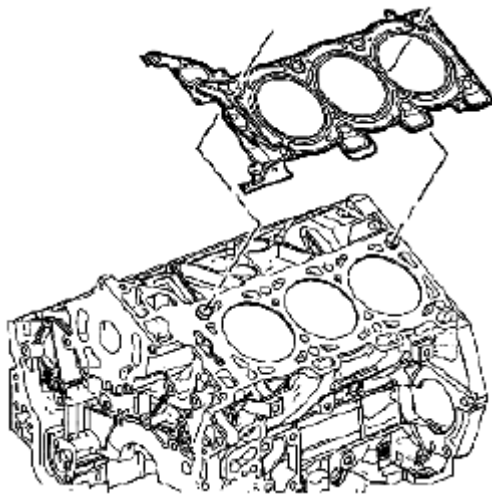
Fig. 216: Identifying Cylinder Head Gasket Courtesy of SUZUKI OF AMERICA CORP.
