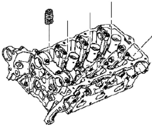
Fig. 207: Identifying Valve Spring Courtesy of SUZUKI OF AMERICA CORP.
