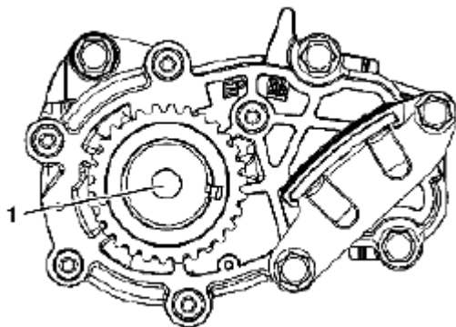
Fig. 904: Identifying Stage 2 Timing Drive Assembly Position Courtesy of SUZUKI OF AMERICA CORP.
