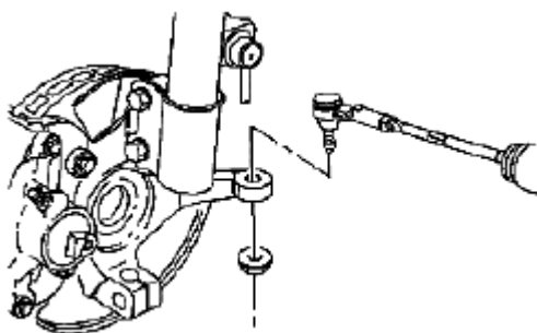
Fig. 229: Identifying Outer Tie Rod Ends Courtesy of SUZUKI OF AMERICA CORP.
