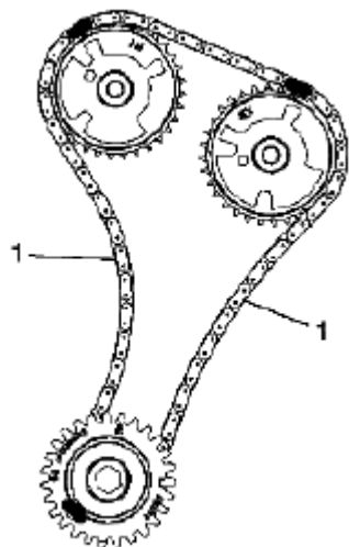
Fig. 812: Identifying Timing Camshaft Drive Chain Link Mark (4 Of 4) Courtesy of SUZUKI OF AMERICA CORP.
