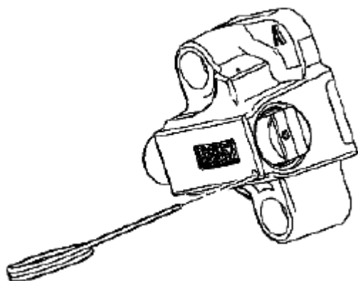
Fig. 924: Inserting EN 46112 Into Hole Of Right Secondary Camshaft Drive Chain Tensioner Body
