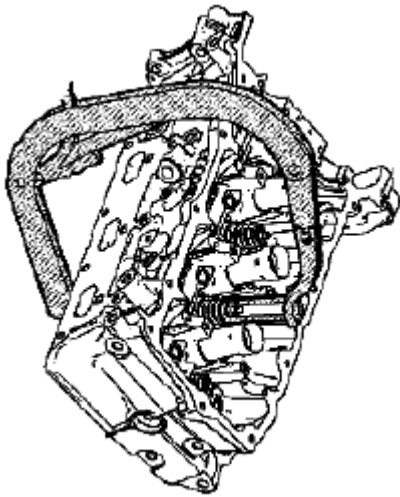
Fig. 465: Compressing Valve Springs Courtesy of SUZUKI OF AMERICA CORP.
