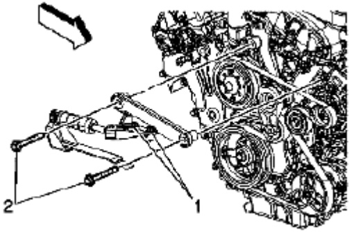
Fig. 65: Removing Engine Mount Strut Bracket To Cylinder Head Bolts Courtesy of SUZUKI OF AMERICA CORP.
