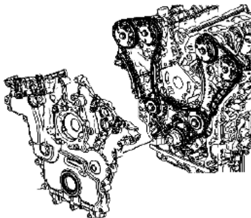
Fig. 952: Identifying Engine Front Cover Courtesy of SUZUKI OF AMERICA CORP.
