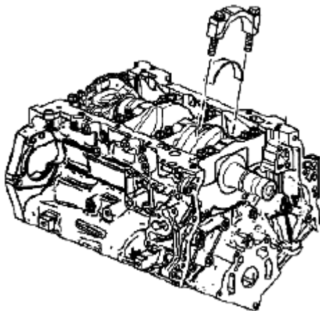
Fig. 377: Identifying Connecting Rod Cap Courtesy of SUZUKI OF AMERICA CORP.
