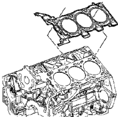
Fig. 365: Identifying Left Cylinder Head Gasket Courtesy of SUZUKI OF AMERICA CORP.
