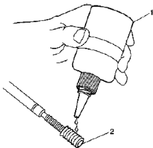
Fig. 603: Applying Threadlock Sealant To Insert OD Threads Courtesy of SUZUKI OF AMERICA CORP.
