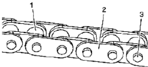
Fig. 488: Identifying Secondary Timing Chain Courtesy of SUZUKI OF AMERICA CORP.
