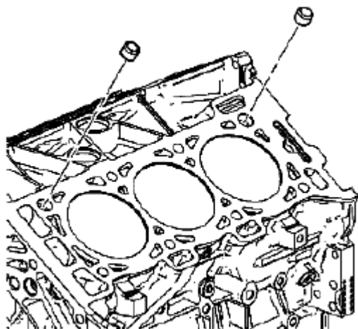
Fig. 400: Identifying Cylinder Block-To-Cylinder Head Alignment Dowels Courtesy of SUZUKI OF AMERICA CORP.
