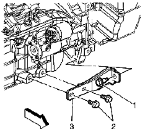
Fig. 245: Installing Engine To Transaxle Brace & Bolts Courtesy of SUZUKI OF AMERICA CORP.
