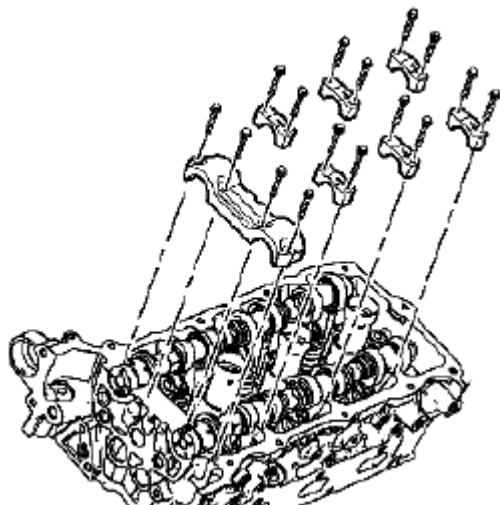
Fig. 771: Identifying Camshaft Bearing Caps Courtesy of SUZUKI OF AMERICA CORP.
