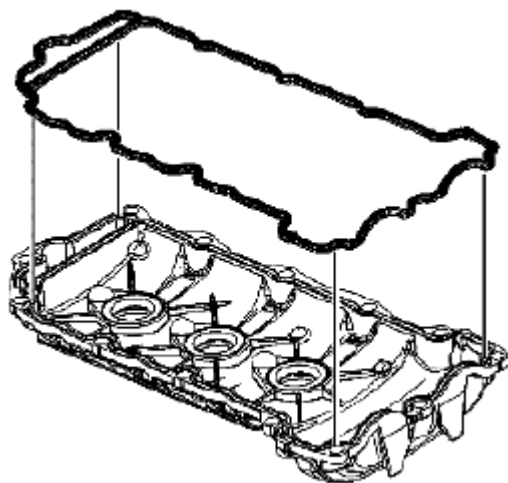
Fig. 557: Identifying Right Camshaft Cover Gasket Courtesy of SUZUKI OF AMERICA CORP.
