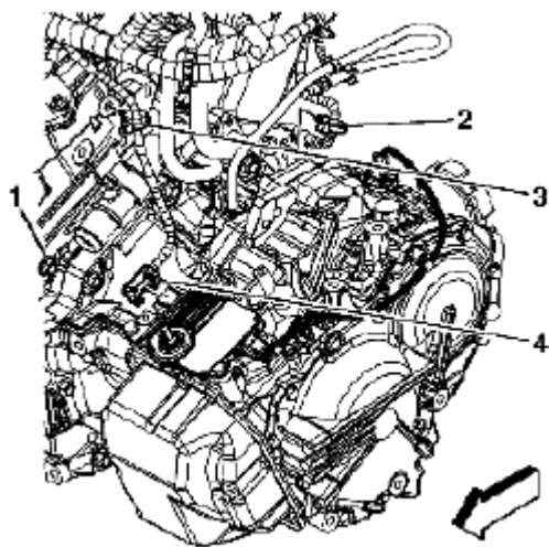
Fig. 247: Connecting Engine Wiring Harness Electrical Connector Courtesy of SUZUKI OF AMERICA CORP.
