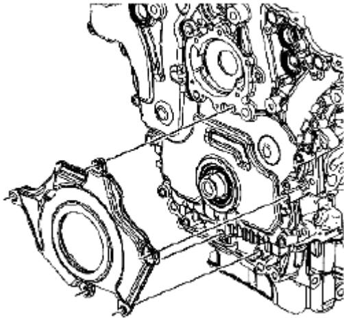
Fig. 943: Identifying Engine Front Cover Deadener Courtesy of SUZUKI OF AMERICA CORP.
