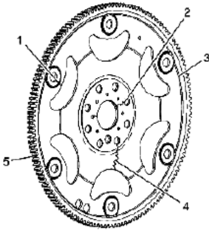
Fig. 416: Identifying Engine Flywheel Courtesy of SUZUKI OF AMERICA CORP.
