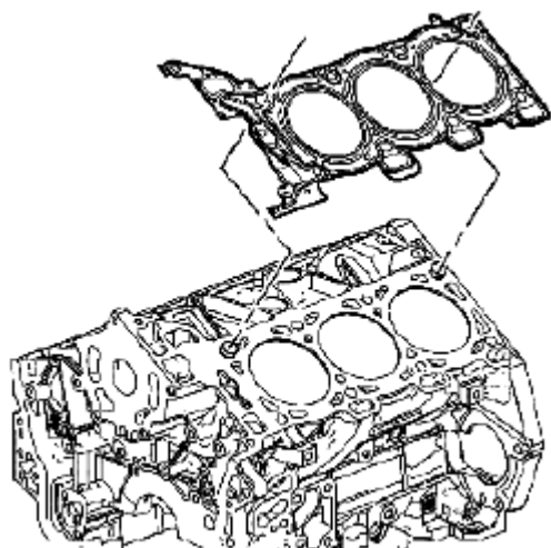
Fig. 757: Identifying Left Cylinder Head Gasket Courtesy of SUZUKI OF AMERICA CORP.
