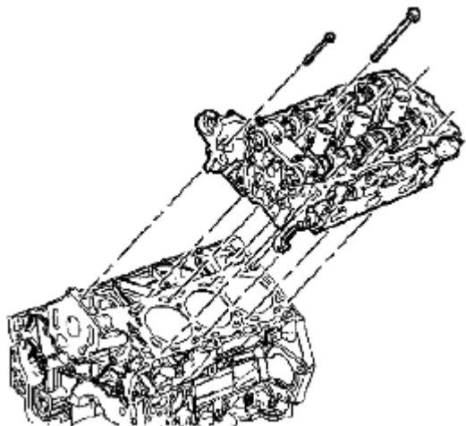
Fig. 364: Identifying Left Cylinder Head & Bolts Courtesy of SUZUKI OF AMERICA CORP.
