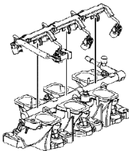
Fig. 580: Identifying Fuel Injector Wiring Harness Courtesy of SUZUKI OF AMERICA CORP.
