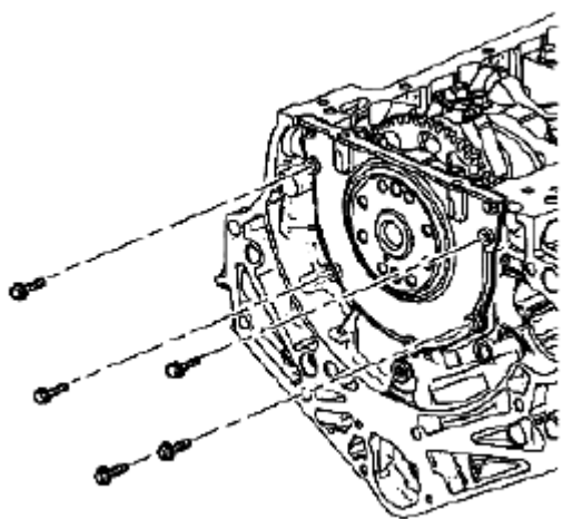
Fig. 374: Identifying Crankshaft Rear Oil Seal Housing & Bolts Courtesy of SUZUKI OF AMERICA CORP.
