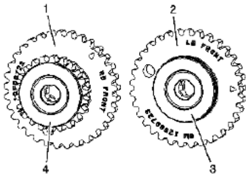
Fig. 803: Identifying Camshaft Intermediate Drive Chain Idler Sprockets
