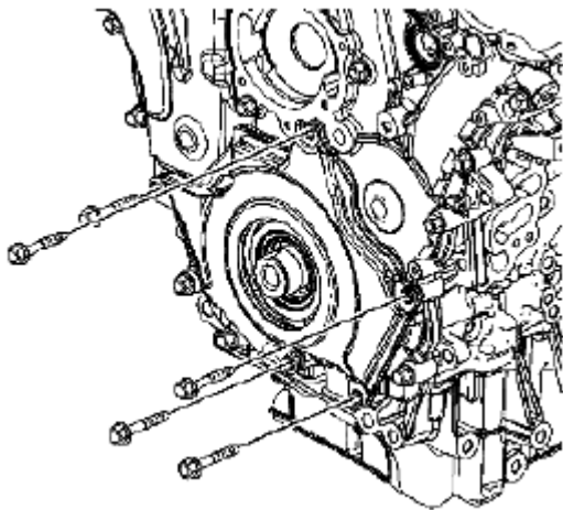
Fig. 292: Identifying Engine Front Cover Bolts Courtesy of SUZUKI OF AMERICA CORP.
