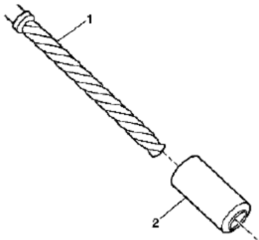
Fig. 610: Applying Stop Collar On Counterbore Drill Courtesy of SUZUKI OF AMERICA CORP.
