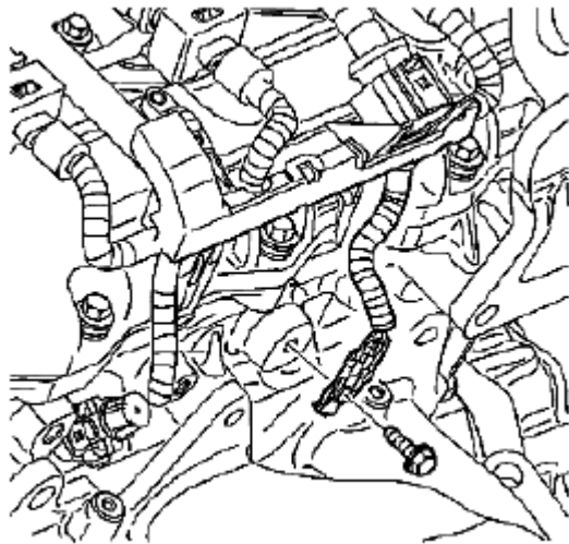
Fig. 218: Identifying Wiring Harness Ground Courtesy of SUZUKI OF AMERICA CORP.
