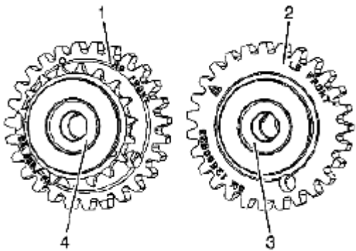
Fig. 801: Identifying Camshaft Intermediate Drive Chain Idler Sprockets Courtesy of SUZUKI OF AMERICA CORP.
