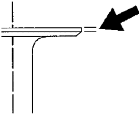
Fig. 456: Locating Valve Margin
