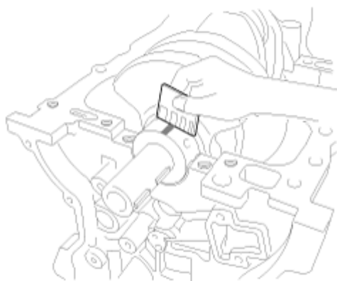
Fig. 13: Checking Crankshaft Bearing Oil Clearance Courtesy of HYUNDAI MOTOR CO.
