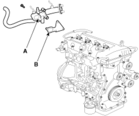
Fig. 42: Identifying Water Temperature Control Assembly & Gasket Courtesy of HYUNDAI MOTOR CO.
