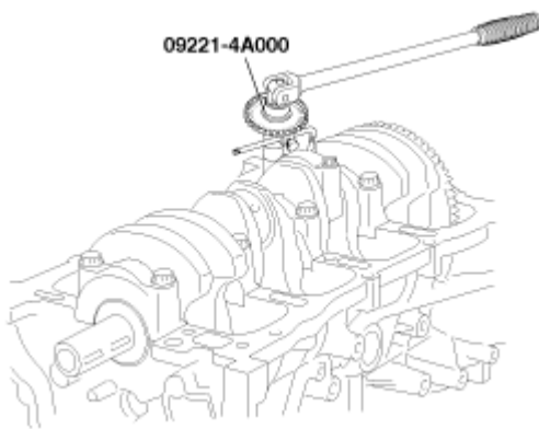
Fig. 38: Tightening Bolts
