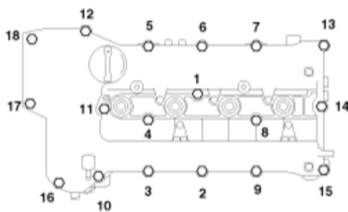
Fig. 44: Identifying Tightening Sequence Of Cylinder Head Cover Bolts Courtesy of HYUNDAI MOTOR CO.
