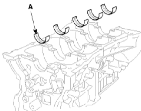
Fig. 32: Identifying Connecting Rod Upper Bearings Courtesy of HYUNDAI MOTOR CO.
