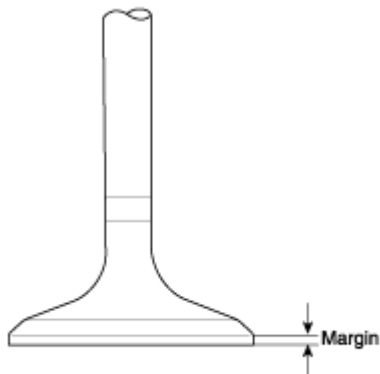
Fig. 21: Checking Valve Head Margin Thickness Courtesy of HYUNDAI MOTOR CO.
