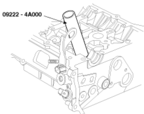
Fig. 31: Pushing In New Oil Seal Using SST Courtesy of HYUNDAI MOTOR CO.
