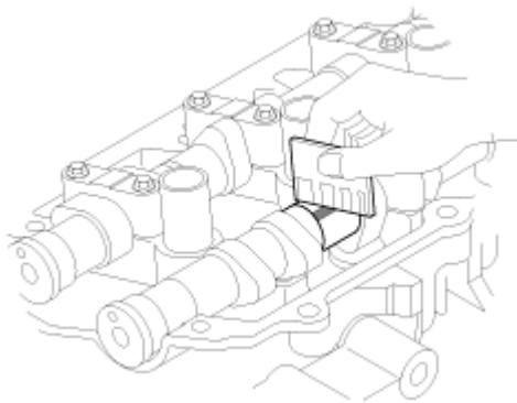
Fig. 25: Measuring Bearing Oil Clearance Courtesy of HYUNDAI MOTOR CO.
