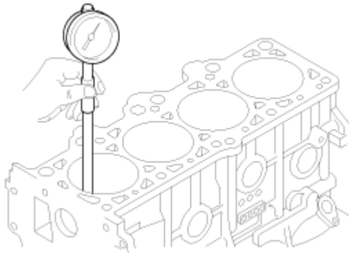
Fig. 20: Measuring Cylinder Bore Diameter Using Cylinder Bore Gauge Courtesy of HYUNDAI MOTOR CO.
