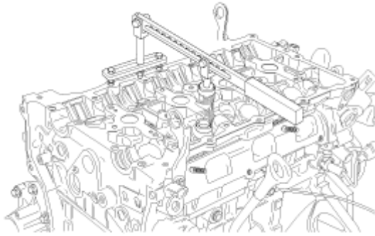
Fig. 16: Compressing Valve Spring Using SST Courtesy of HYUNDAI MOTOR CO.
