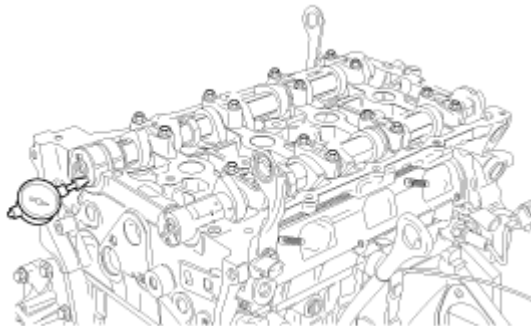
Fig. 26: Measuring Camshaft End Play Using Dial Indicator Courtesy of HYUNDAI MOTOR CO.
