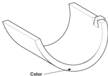
Fig. 28: Locating Exhaust Camshaft Bearing Identification Mark Courtesy of HYUNDAI MOTOR CO.
