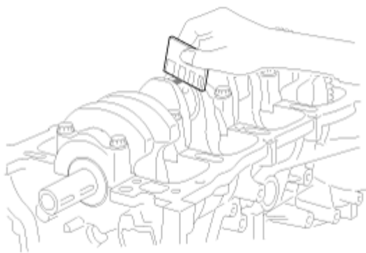
Fig. 9: Checking Connecting Rod Bearing Oil Clearance Courtesy of HYUNDAI MOTOR CO.
