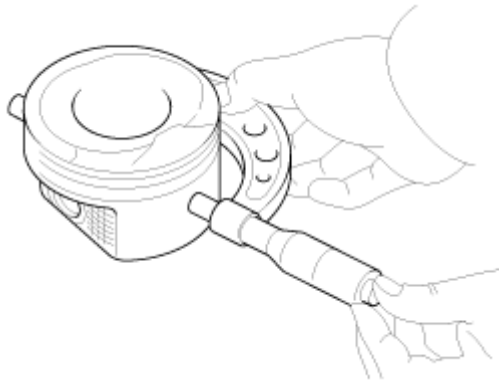
Fig. 23: Measuring Piston Outside Diameter Courtesy of HYUNDAI MOTOR CO.
