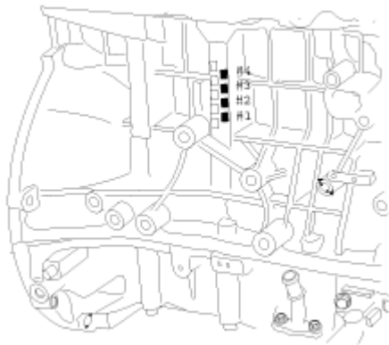
Fig. 21: Identifying Cylinder Bore Size Code On Cylinder Block Courtesy of HYUNDAI MOTOR CO.
