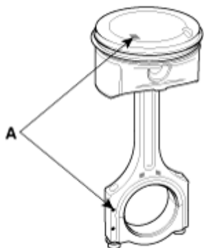
Fig. 29: Identifying Piston Front Mark & Connecting Rod Front Mark Courtesy of HYUNDAI MOTOR CO.
