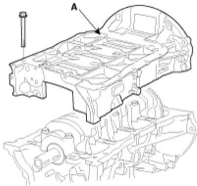
Fig. 6: Identifying Ladder Frame Courtesy of HYUNDAI MOTOR CO.
