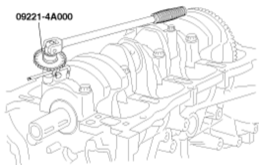
Fig. 36: Tightening Bearing Cap Bolts Using SST Courtesy of HYUNDAI MOTOR CO.
