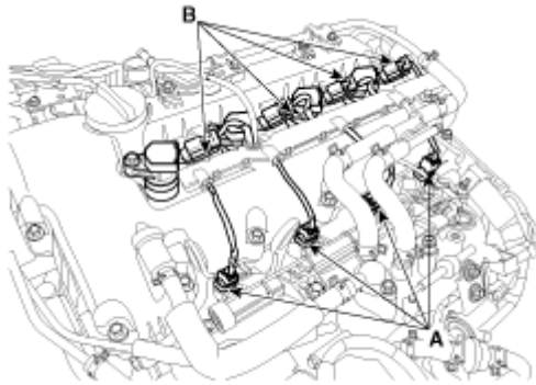
Fig. 1: Identifying Injector Connectors & Ignition Coil Connectors Courtesy of HYUNDAI MOTOR CO.
