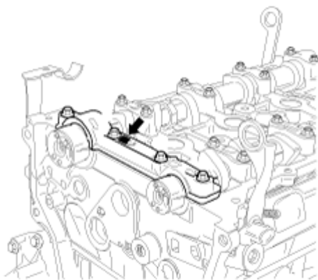
Fig. 27: Locating Cylinder Head Bore Mark Courtesy of HYUNDAI MOTOR CO.
