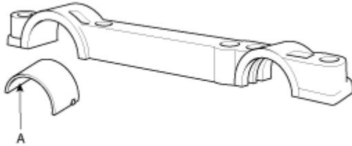
Fig. 9: Identifying Exhaust Camshaft Upper Bearing Courtesy of HYUNDAI MOTOR CO.
