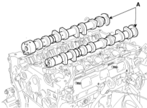
Fig. 11: Identifying Camshafts Courtesy of HYUNDAI MOTOR CO.
