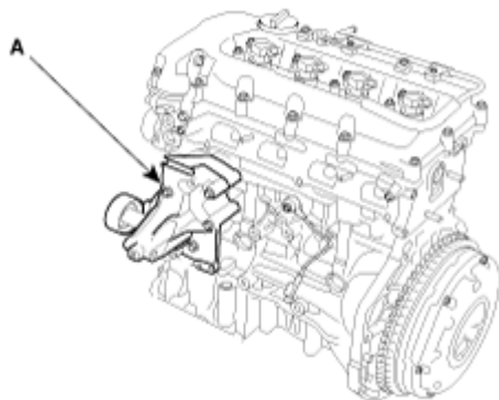
Fig. 42: Identifying Tensioner Assembly Integrated Bracket Courtesy of HYUNDAI MOTOR CO.
