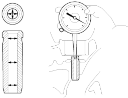
Fig. 19: Measuring Inside Diameter Of Valve Guide Using Caliper Gauge Courtesy of HYUNDAI MOTOR CO.
