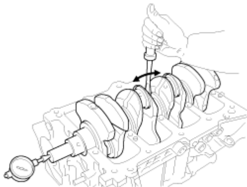
Fig. 17: Measuring Thrust Clearance Using Dial Indicator Courtesy of HYUNDAI MOTOR CO.
