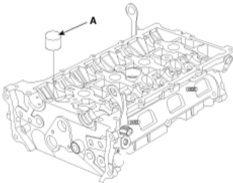
Fig. 15: Identifying MLA (Mechanical Lash Adjuster) Courtesy of HYUNDAI MOTOR CO.
