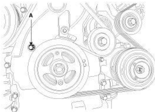
Fig. 7: Identifying Service Hole Bolt Of Timing Chain Cover Courtesy of HYUNDAI MOTOR CO.
