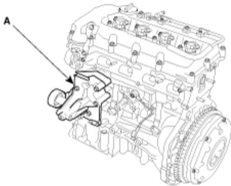
Fig. 4: Identifying Tensioner Assembly Integrated Bracket Courtesy of HYUNDAI MOTOR CO.
