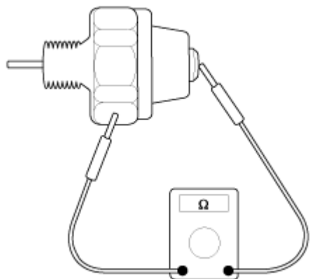
Fig. 28: Checking Continuity Between Oil Pressure Switch Terminal & Body (With Fine Wire Pushed) Courtesy of HYUNDAI MOTOR CO.
