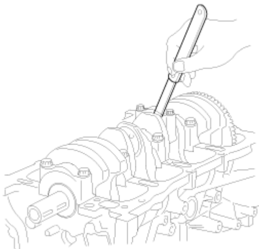
Fig. 8: Measuring Connecting Rod End Play Using Feeler Gauge Courtesy of HYUNDAI MOTOR CO.
