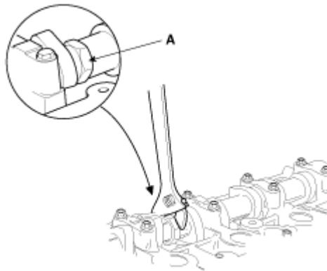
Fig. 7: Fixing Camshaft With Wrench Courtesy of HYUNDAI MOTOR CO.
