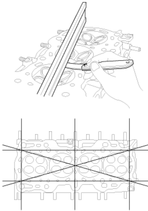
Fig. 18: Inspecting Flatness Of Cylinder Head Gasket Surface Courtesy of HYUNDAI MOTOR CO.
