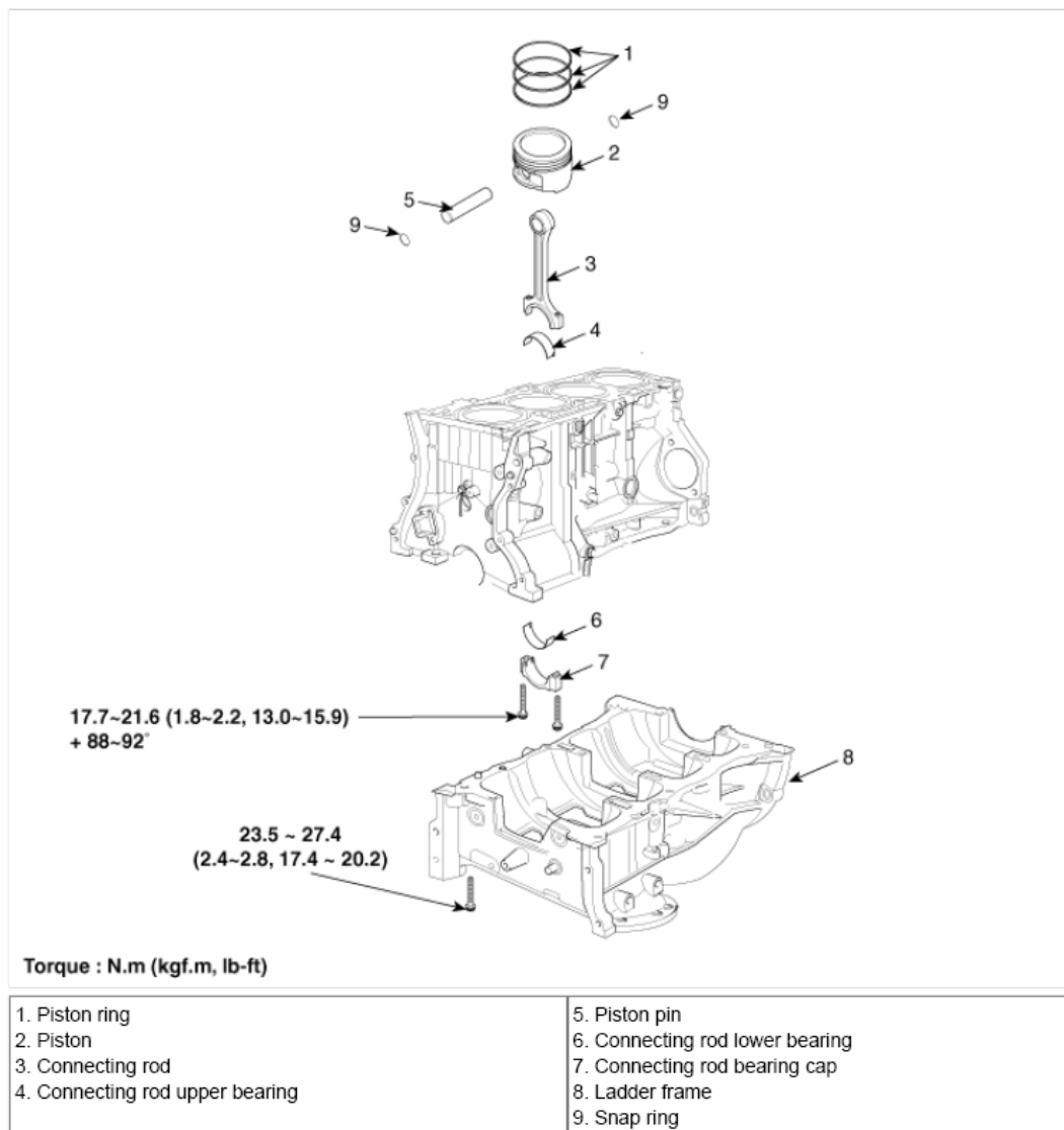
Fig. 1: Identifying Cylinder Block Components With Torque Specifications (1 Of 2) Courtesy of HYUNDAI MOTOR CO.
