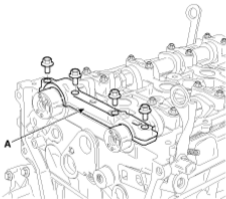
Fig. 8: Identifying Front Camshaft Bearing Cap
