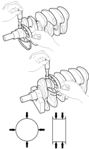
Fig. 18: Measuring Diameter Of Each Main Journal & Crank Pin Using Micrometer Courtesy of HYUNDAI MOTOR CO.
