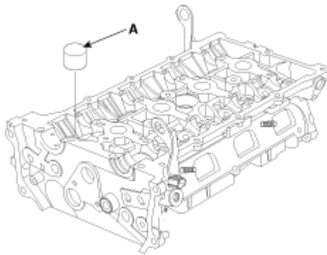
Fig. 33: Identifying MLA (Mechanical Lash Adjuster) Courtesy of HYUNDAI MOTOR CO.
