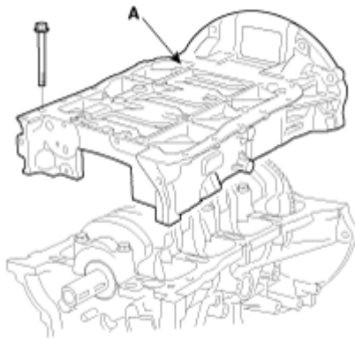
Fig. 39: Identifying Ladder Frame Courtesy of HYUNDAI MOTOR CO.
