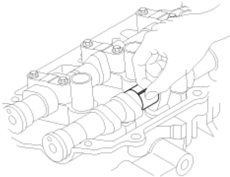
Fig. 24: Inspecting Camshaft Journal Clearance Courtesy of HYUNDAI MOTOR CO.
