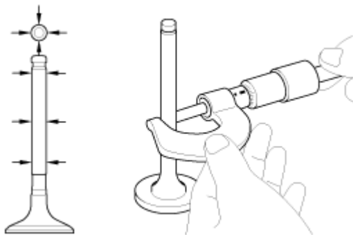
Fig. 20: Measuring Diameter Of Valve Stem Using Micrometer Courtesy of HYUNDAI MOTOR CO.
