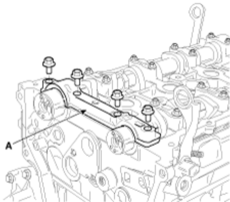
Fig. 9: Identifying Front Camshaft Bearing Cap Courtesy of HYUNDAI MOTOR CO.
