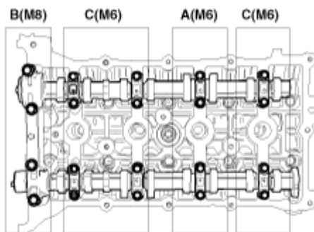
Fig. 41: Installing Camshaft Bearing Caps Courtesy of HYUNDAI MOTOR CO.
