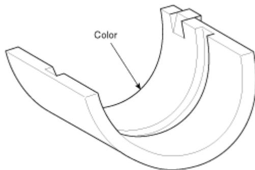
Fig. 16: Locating Crankshaft Bearing Identification Mark Courtesy of HYUNDAI MOTOR CO.
