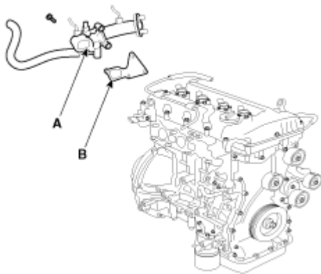
Fig. 5: Identifying Water Temperature Control Assembly & Gasket Courtesy of HYUNDAI MOTOR CO.
