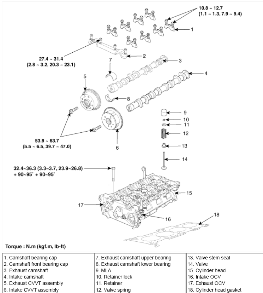
Fig. 1: Identifying Cylinder Head Components With Torque Specifications Courtesy of HYUNDAI MOTOR CO.
