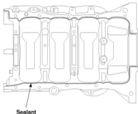
Fig. 40: Applying Sealant To Ladder Frame Courtesy of HYUNDAI MOTOR CO.
