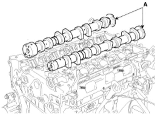
Fig. 39: Identifying Camshafts Courtesy of HYUNDAI MOTOR CO.
