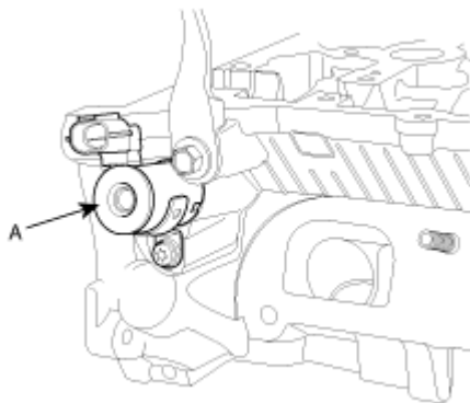
Fig. 37: Identifying OCV Courtesy of HYUNDAI MOTOR CO.
