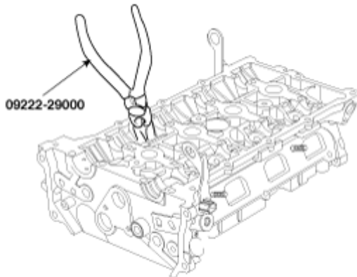
Fig. 17: Removing Valve Stem Seal Using Valve Stem Seal Remover Courtesy of HYUNDAI MOTOR CO.
