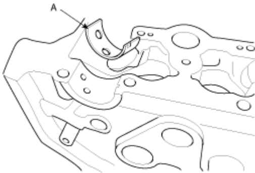
Fig. 38: Identifying Exhaust Camshaft Lower Bearing Courtesy of HYUNDAI MOTOR CO.
