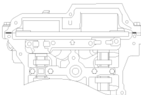
Fig. 43: Identifying Sealant Application Area Between Timing Chain Cover & Cylinder Head
