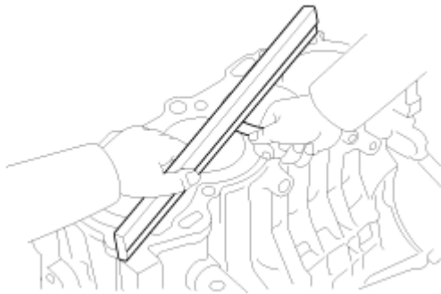
Fig. 19: Inspecting Flatness Of Cylinder Block Top Surface Courtesy of HYUNDAI MOTOR CO.
