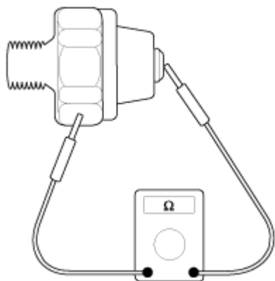
Fig. 27: Checking Continuity Between Oil Pressure Switch Terminal & Body Courtesy of HYUNDAI MOTOR CO.
