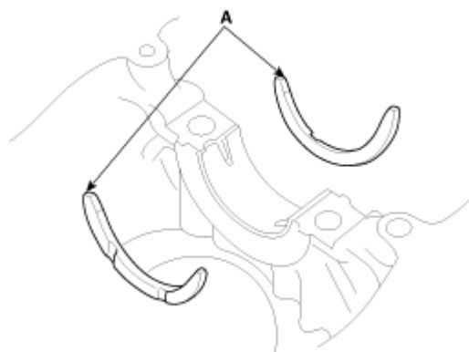
Fig. 33: Identifying Thrust Bearings Courtesy of HYUNDAI MOTOR CO.
