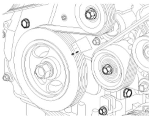
Fig. 3: Aligning Crankshaft Pulley Groove With Timing Mark Of Lower Timing Chain Cover
