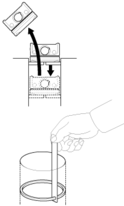
Fig. 25: Measuring Piston Ring End Gap Courtesy of HYUNDAI MOTOR CO.
