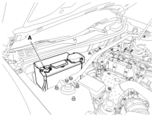
Fig. 2: Identifying Negative (-) Battery Terminal Courtesy of HYUNDAI MOTOR CO.
