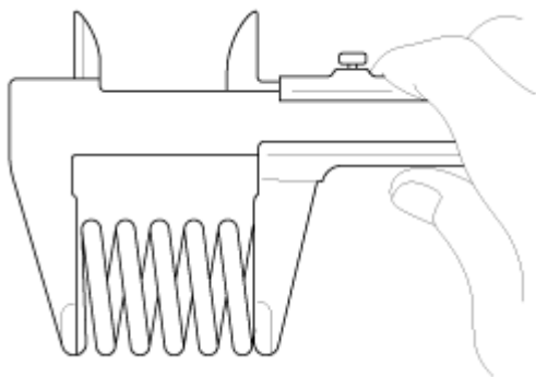
Fig. 22: Inspecting Valve Springs Courtesy of HYUNDAI MOTOR CO.
