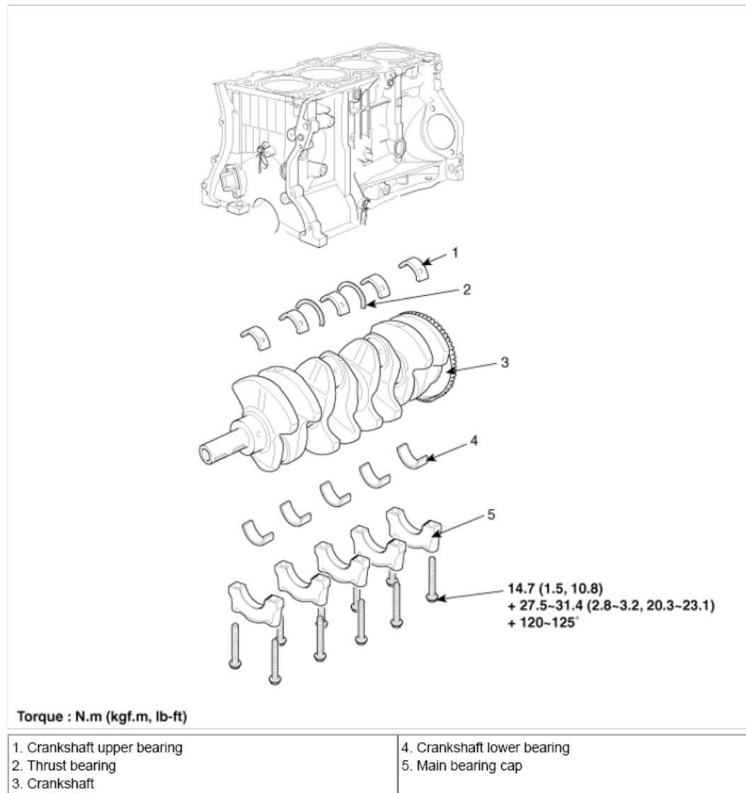
Fig. 2: Identifying Cylinder Block Components With Torque Specifications (2 Of 2) Courtesy of HYUNDAI MOTOR CO.
