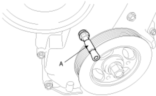
Fig. 8: Inserting SST Service Hole Of Timing Chain Cover Courtesy of HYUNDAI MOTOR CO.
