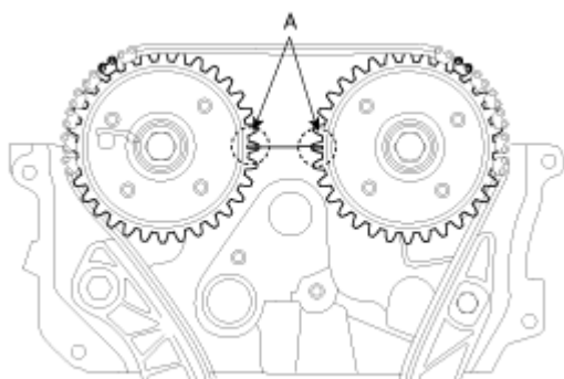
Fig. 11: Realigning Crankshaft Sprocket & Camshaft Sprocket Timing Marks Courtesy of HYUNDAI MOTOR CO.
