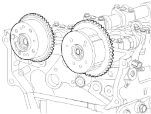
Fig. 6: Identifying Intake & Exhaust CVVT Assembly Courtesy of HYUNDAI MOTOR CO.
