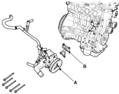
Fig. 4: Identifying Water Pump & Gasket Courtesy of HYUNDAI MOTOR CO.
