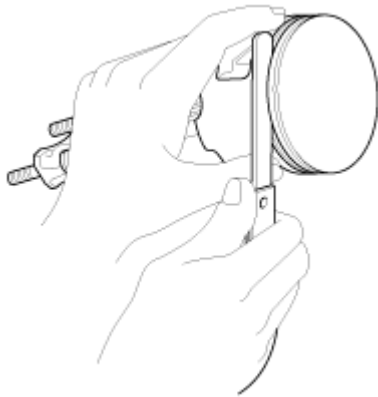
Fig. 24: Measuring Clearance Between Piston Ring & Wall Of Ring Groove Using Feeler Gauge Courtesy of HYUNDAI MOTOR CO.
