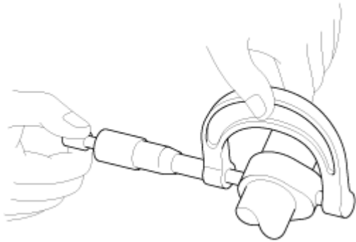
Fig. 23: Measuring Cam Lobe Height Using Micrometer Courtesy of HYUNDAI MOTOR CO.
