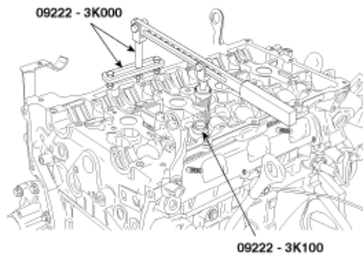
Fig. 32: Compressing Spring Using SST Courtesy of HYUNDAI MOTOR CO.
