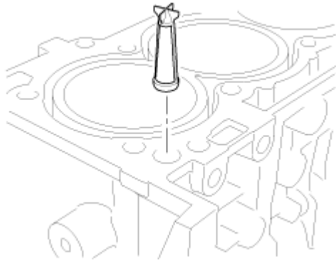
Fig. 34: Identifying OCV Filter Courtesy of HYUNDAI MOTOR CO.
