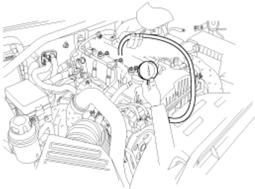
Fig. 2: Checking Cylinder Compression Pressure Using Compression Gauge Courtesy of HYUNDAI MOTOR CO.
