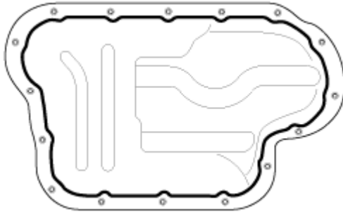
Fig. 43: Identifying Liquid Gasket Application Area On Oil Pan Courtesy of HYUNDAI MOTOR CO.
