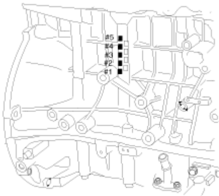
Fig. 14: Locating Crankshaft Bore Mark Courtesy of HYUNDAI MOTOR CO.
