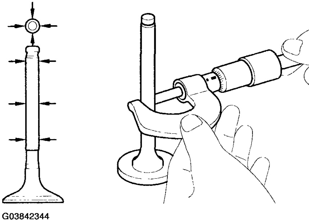
Fig. 89: Measuring Diameter Of Valve Stem Courtesy of HYUNDAI MOTOR CO.
