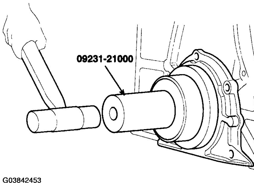
Fig. 198: Applying Engine Oil To Oil Seal Lip Courtesy of HYUNDAI MOTOR CO.
