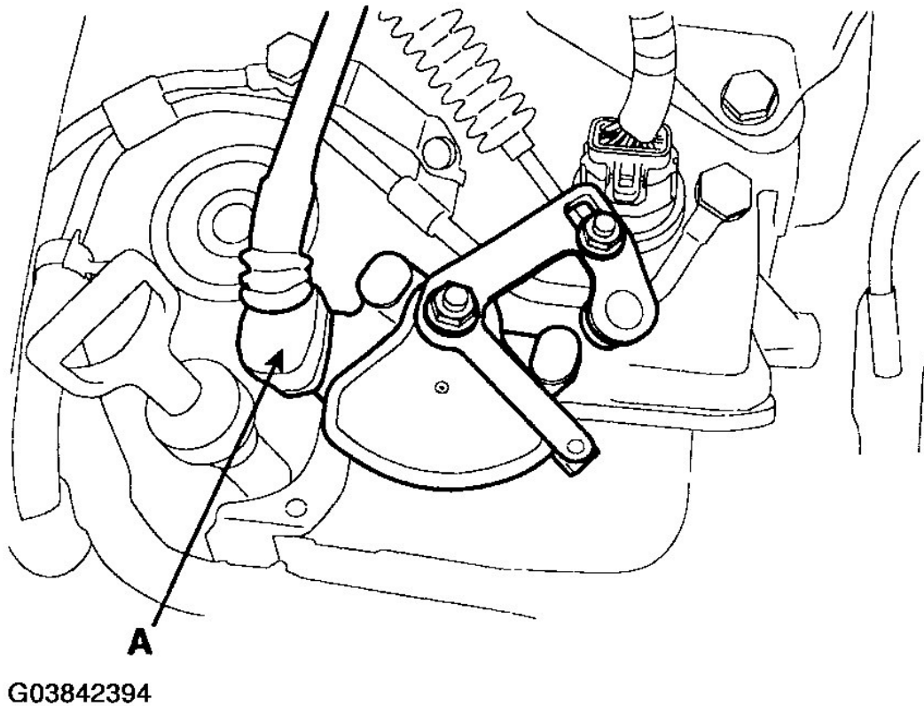
Fig. 139: Removing Transaxle Range Switch Connector Courtesy of HYUNDAI MOTOR CO.
