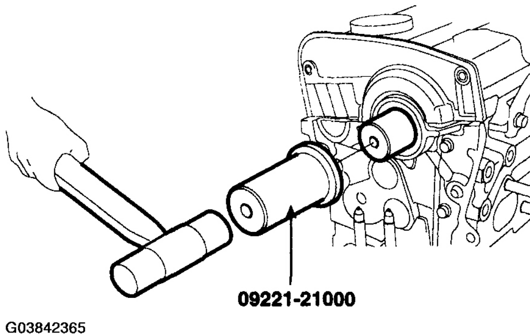
Fig. 110: Installing Camshaft Bearing Oil Seal Using SST Courtesy of HYUNDAI MOTOR CO.
