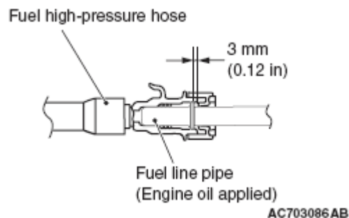
Fig. 113: Identifying Fuel High-Pressure Hose Clearance Courtesy of MITSUBISHI MOTOR SALES OF AMERICA.
