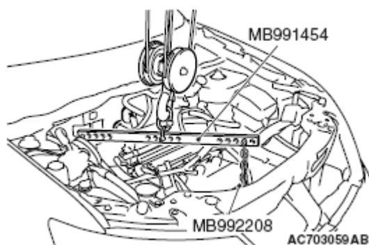
Fig. 110: Identifying Special Tool MB991454 And MB992208
