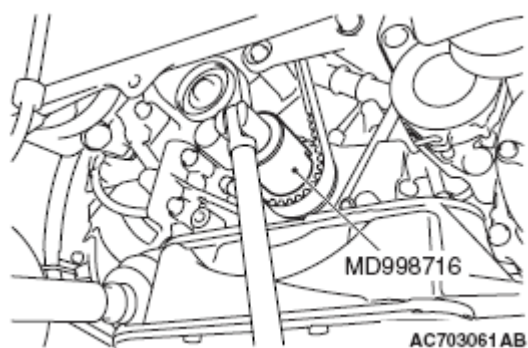
Fig. 90: Identifying Special Tool MD998716
