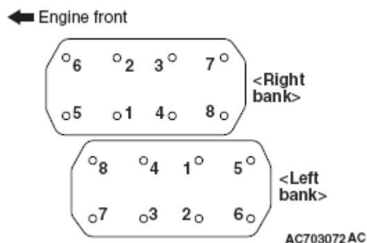
Fig. 86: Identifying Cylinder Head Bolt Tightening Sequence Courtesy of MITSUBISHI MOTOR SALES OF AMERICA.
