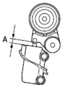
Fig. 99: Identifying Auto-Tensioner Push Rod Clearance
