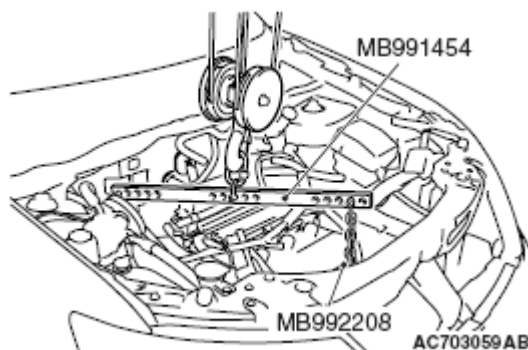
Fig. 111: Identifying Special Tool MB991454 And MB992208
