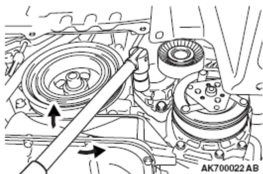
Fig. 2: Removing Auto Tensioner
