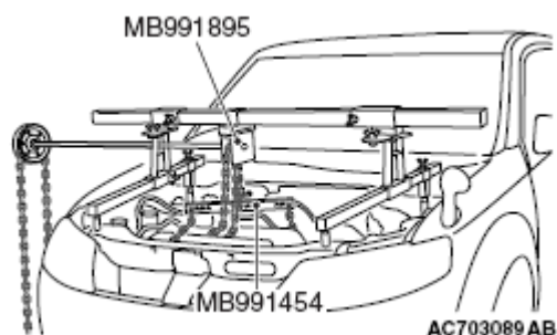
Fig. 108: Identifying Special Tool MB991895 Courtesy of MITSUBISHI MOTOR SALES OF AMERICA.
