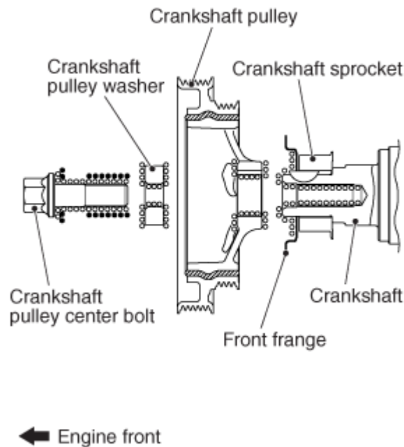
Fig. 30: Identifying Crankshaft Pulley Center Bolt And Crankshaft Pulley Washer Courtesy of MITSUBISHI MOTOR SALES OF AMERICA.
