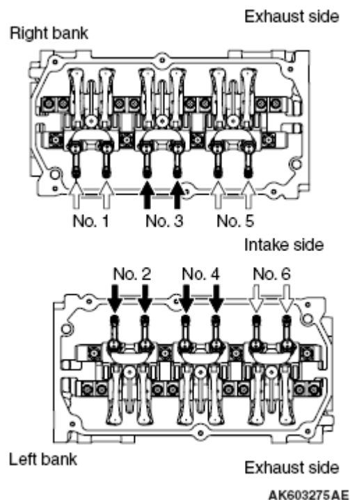
Fig. 8: Locating Rocker Arm
