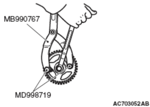
Fig. 88: Identifying Special Tools MB990767 And MD998719 Courtesy of MITSUBISHI MOTOR SALES OF AMERICA.
