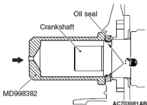
Fig. 74: Identifying Special Tool MD998382 Courtesy of MITSUBISHI MOTOR SALES OF AMERICA.
