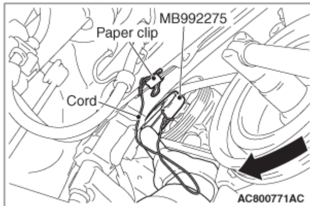
Fig. 34: Identifying Special Tool MB992275 Courtesy of MITSUBISHI MOTOR SALES OF AMERICA.
