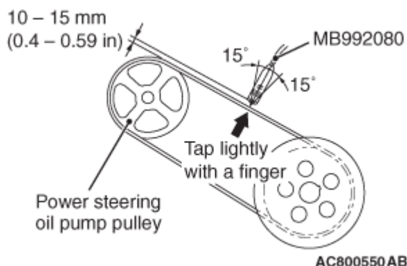
Fig. 4: Identifying Power Steering Oil Pump Drive Belt Clearance
