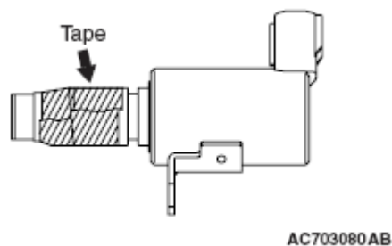
Fig. 64: Locating Tape On Engine Oil Control Valve Courtesy of MITSUBISHI MOTOR SALES OF AMERICA.
