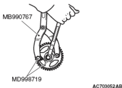
Fig. 82: Identifying Special Tools MB990767 And MD998719 Courtesy of MITSUBISHI MOTOR SALES OF AMERICA.
