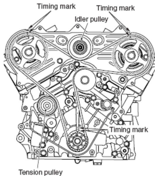
Fig. 93: Identifying Timing Mark
