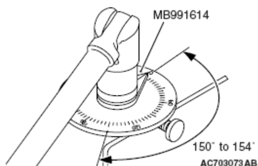
Fig. 87: Tightening Cylinder Head Bolt Using Special Tool MB991614 Courtesy of MITSUBISHI MOTOR SALES OF AMERICA.
