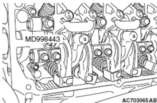
Fig. 45: Identifying Special Tool MD998443 Courtesy of MITSUBISHI MOTOR SALES OF AMERICA.
