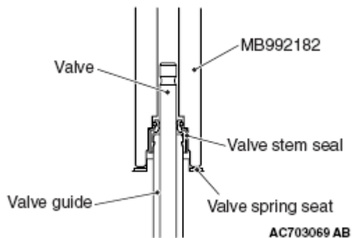
Fig. 52: Identifying Special Tool MB992182
