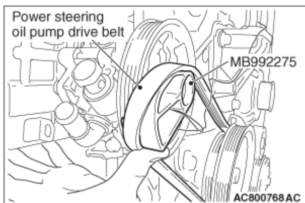
Fig. 35: Identifying Special Tool MB992275 Courtesy of MITSUBISHI MOTOR SALES OF AMERICA.
