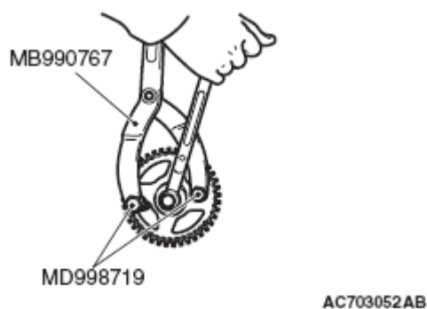
Fig. 42: Identifying Special Tools MB990767 And MD998719 Courtesy of MITSUBISHI MOTOR SALES OF AMERICA.
