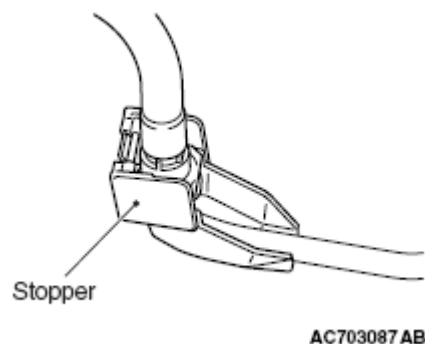
Fig. 114: Identifying Stopper Courtesy of MITSUBISHI MOTOR SALES OF AMERICA.
