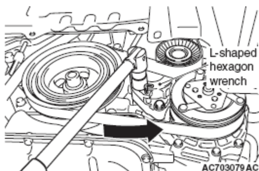
Fig. 25: Removing Generator Drive Belt Courtesy of MITSUBISHI MOTOR SALES OF AMERICA.
