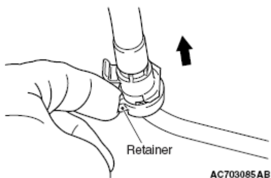
Fig. 107: Identifying Retainer Courtesy of MITSUBISHI MOTOR SALES OF AMERICA.
