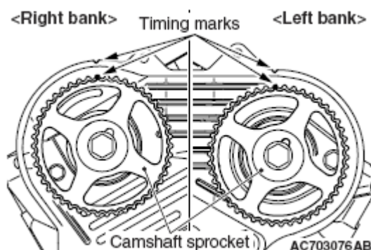
Fig. 96: Identifying Timing Marks On Camshaft Sprockets (1 Of 2) Courtesy of MITSUBISHI MOTOR SALES OF AMERICA.
