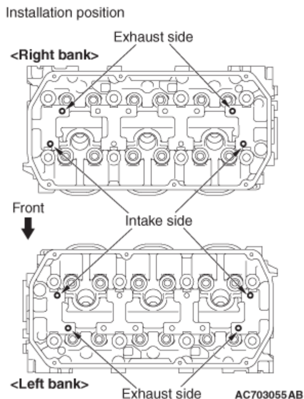
Fig. 50: Identifying Valve Spring Retainer Locks Courtesy of MITSUBISHI MOTOR SALES OF AMERICA.
