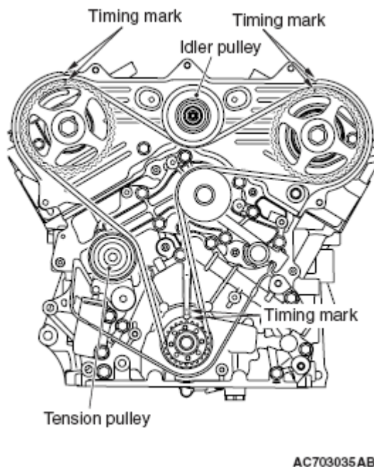
Fig. 91: Identifying Timing Mark
