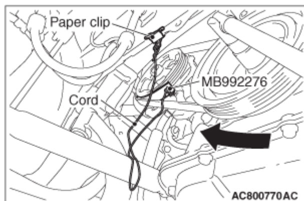
Fig. 27: Identifying Special Tool MB992276
