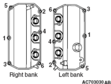
Fig. 59: Identifying Rocker Cover Bolt Tightening Sequence Courtesy of MITSUBISHI MOTOR SALES OF AMERICA.
