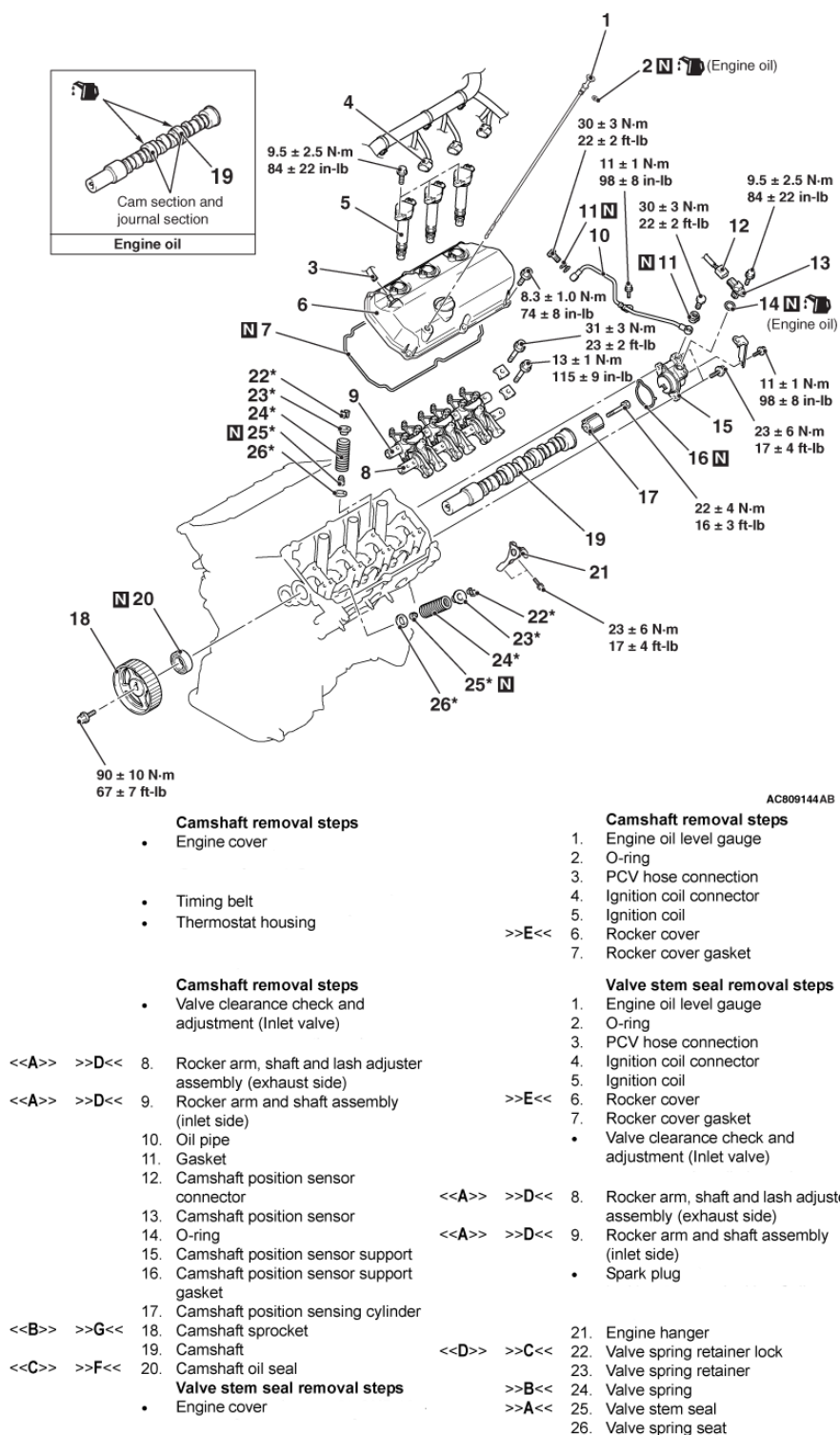
Fig. 43: Identifying Camshaft And Valve Stem Seal Components With Torque Specifications - Left Bank Courtesy of MITSUBISHI MOTOR SALES OF AMERICA.
