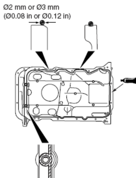
Fig. 68: Applying Bead Of Sealant To Cylinder Block Mating Surface Of Engine Oil Pan
