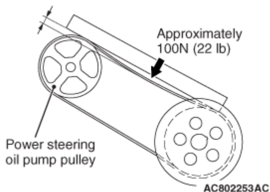
Fig. 5: Identifying Power Steering Oil Pump Drive Belt Clearance Courtesy of MITSUBISHI MOTOR SALES OF AMERICA.
