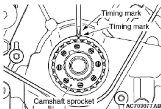
Fig. 97: Identifying Timing Marks On Camshaft Sprockets (2 Of 2) Courtesy of MITSUBISHI MOTOR SALES OF AMERICA.
