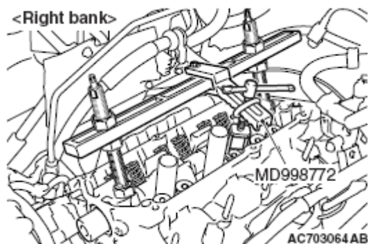
Fig. 55: Identifying Special Tool MD998772 - Right Bank Courtesy of MITSUBISHI MOTOR SALES OF AMERICA.
