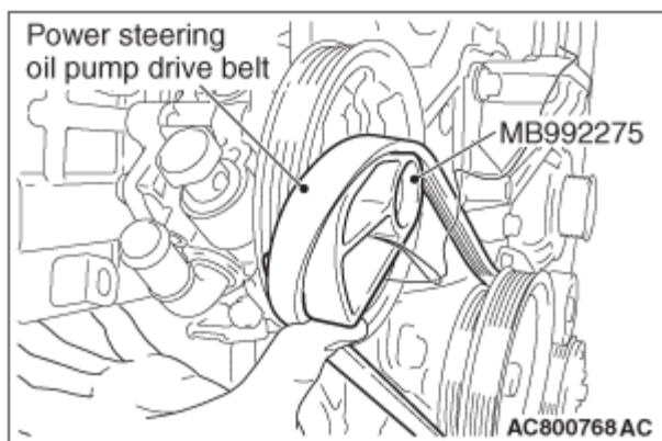
Fig. 117: Identifying Special Tool MB992275
