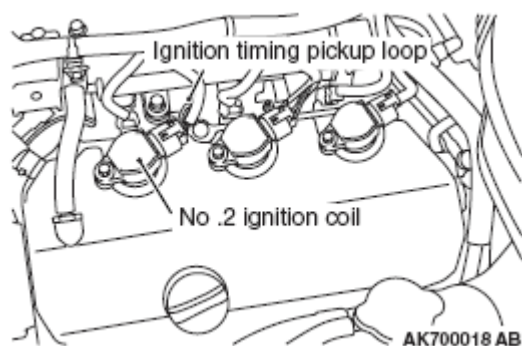
Fig. 11: Identifying No. 2 Ignition Coil
