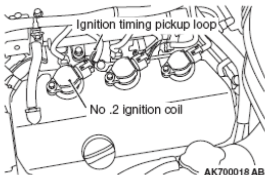
Fig. 13: Identifying No. 2 Ignition Coil
