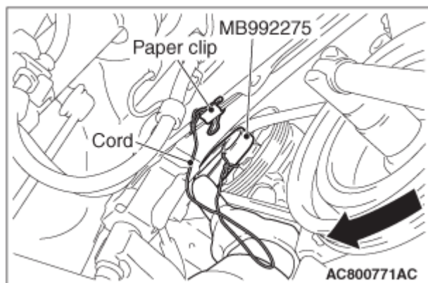
Fig. 36: Identifying Special Tool MB992275 Courtesy of MITSUBISHI MOTOR SALES OF AMERICA.
