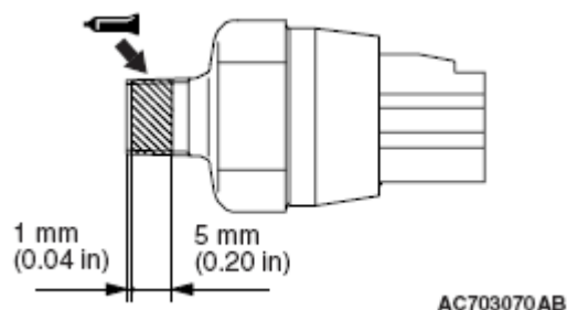
Fig. 63: Identifying Engine Oil Pressure Switch Clearance Courtesy of MITSUBISHI MOTOR SALES OF AMERICA.
