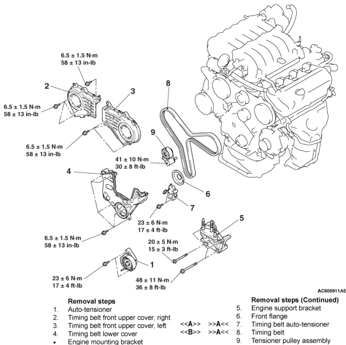
Fig. 89: Identifying Timing Belt Components With Torque Specifications Courtesy of MITSUBISHI MOTOR SALES OF AMERICA.
