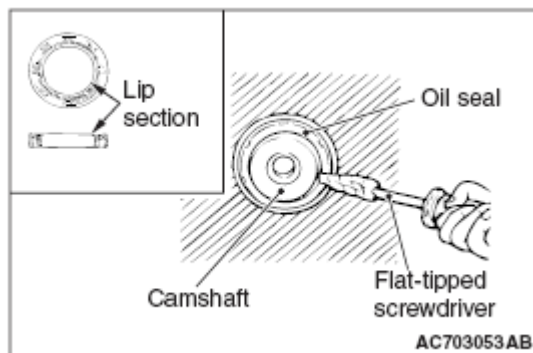
Fig. 47: Removing Oil Seal Courtesy of MITSUBISHI MOTOR SALES OF AMERICA.
