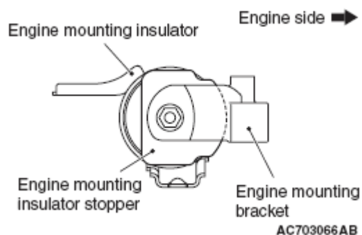
Fig. 112: Identifying Engine Mounting Insulator Stopper Courtesy of MITSUBISHI MOTOR SALES OF AMERICA.
