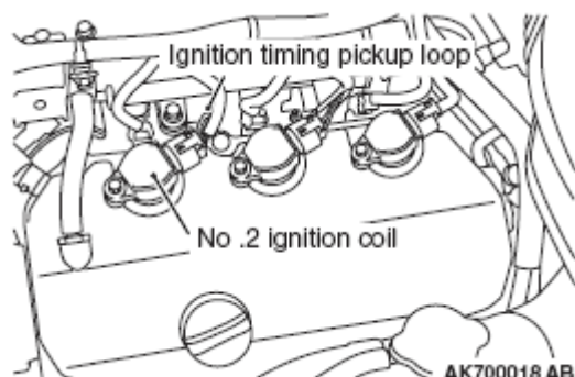
Fig. 15: Identifying No. 2 Ignition Coil Courtesy of MITSUBISHI MOTOR SALES OF AMERICA.
