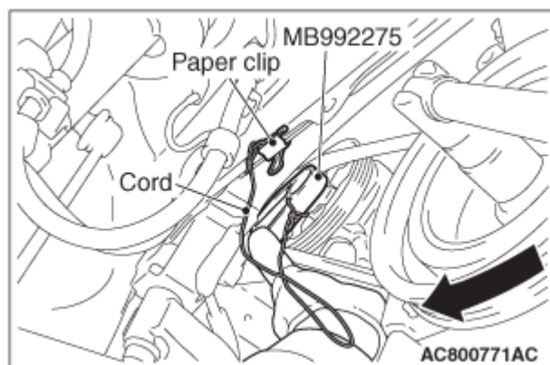
Fig. 116: Identifying Special Tool MB992275 Courtesy of MITSUBISHI MOTOR SALES OF AMERICA.
