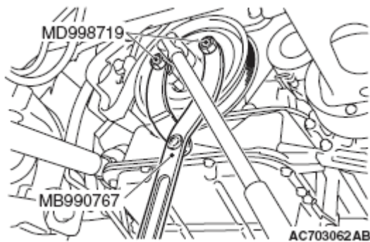
Fig. 31: Identifying Special Tools MB990767 And MD998719 Courtesy of MITSUBISHI MOTOR SALES OF AMERICA.
