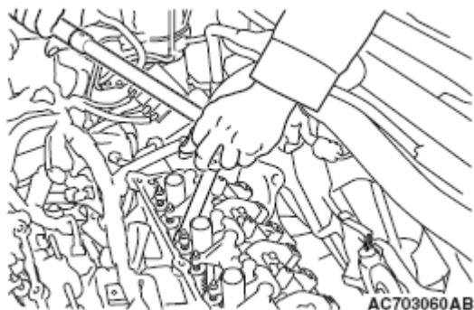
Fig. 85: Removing Cylinder Head Bolt
