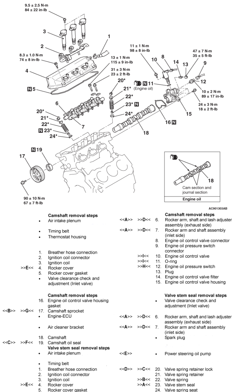
Fig. 44: Identifying Camshaft And Valve Stem Seal Components With Torque Specifications - Right Bank
