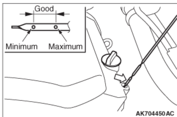
Fig. 21: Identifying Engine Oil Level Marks
