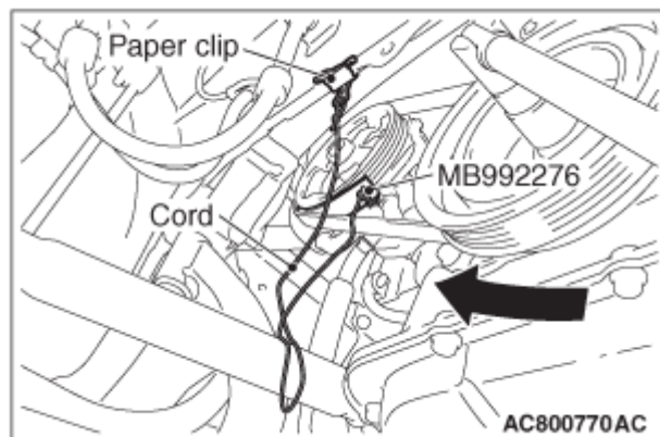
Fig. 105: Identifying Special Tool MB992276
