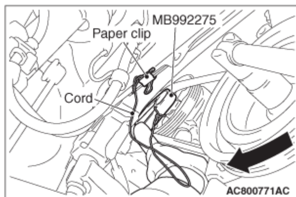
Fig. 118: Identifying Special Tool MB992275
