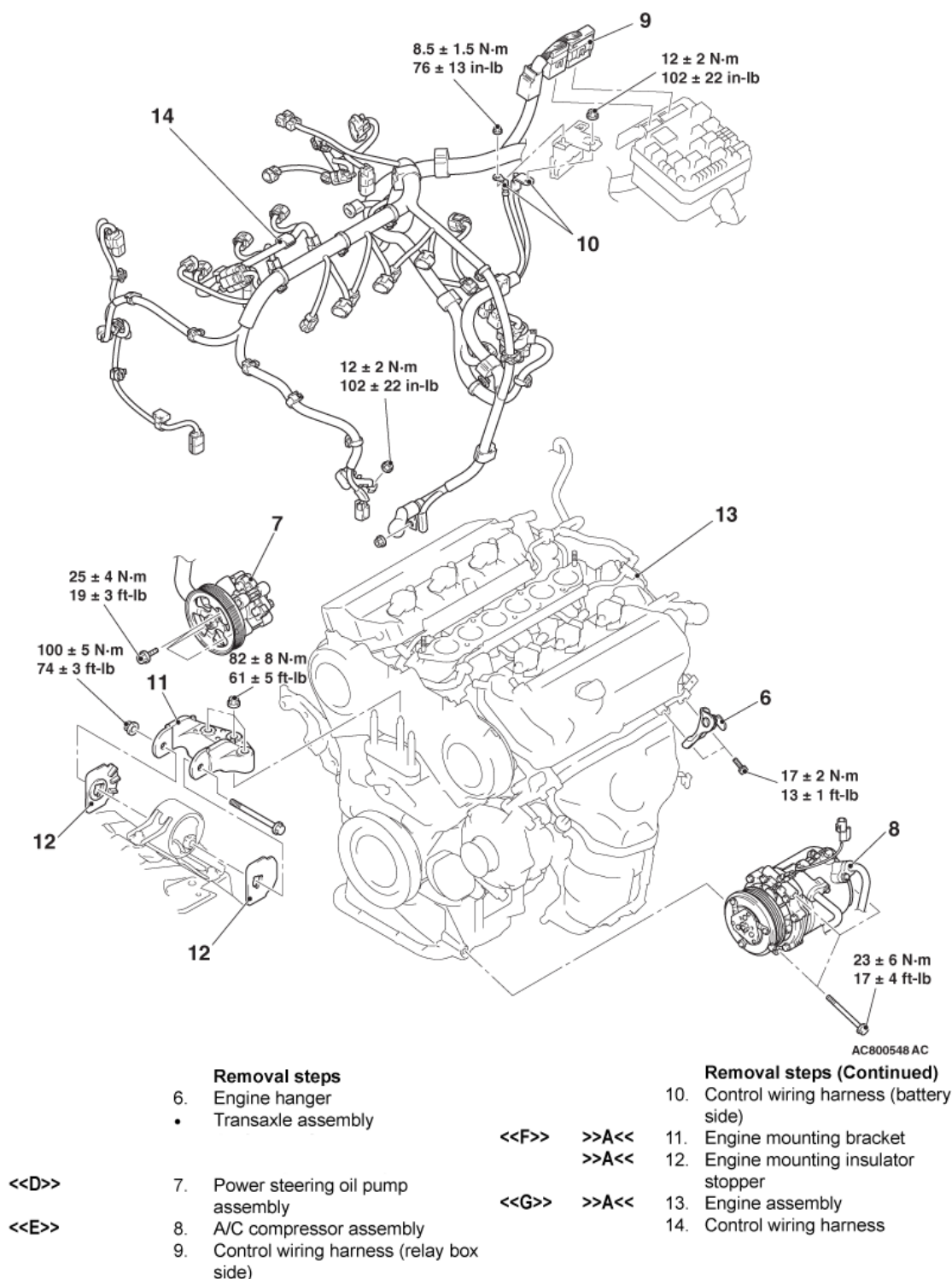
Fig. 102: Identifying Engine Assembly Components With Torque Specifications (2 Of 2) Courtesy of MITSUBISHI MOTOR SALES OF AMERICA.
