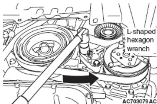
Fig. 103: Removing Generator Drive Belt Courtesy of MITSUBISHI MOTOR SALES OF AMERICA.
