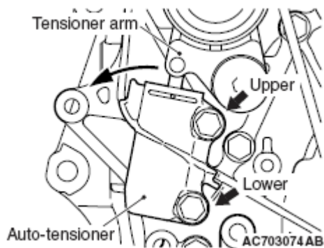
Fig. 92: Identifying Timing Belt Auto-Tensioner And Tensioner Arm Courtesy of MITSUBISHI MOTOR SALES OF AMERICA.
