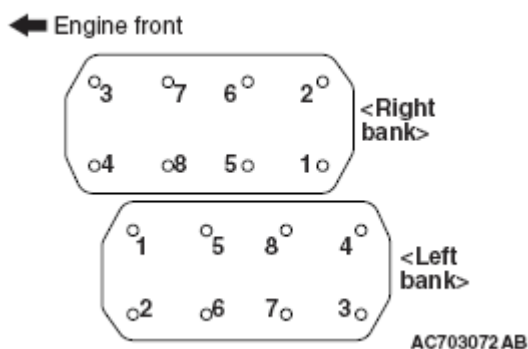
Fig. 83: Identifying Cylinder Head Assembly Bolt Tightening Sequence Courtesy of MITSUBISHI MOTOR SALES OF AMERICA.
