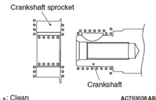
Fig. 75: Identifying Crankshaft And Crankshaft Sprocket Courtesy of MITSUBISHI MOTOR SALES OF AMERICA.
