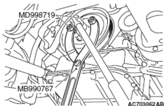
Fig. 28: Identifying Special Tools MB990767 And MD998719 Courtesy of MITSUBISHI MOTOR SALES OF AMERICA.
