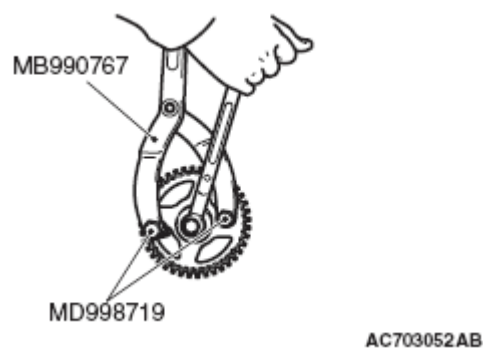
Fig. 62: Identifying Special Tools MB990767 And MD998719 Courtesy of MITSUBISHI MOTOR SALES OF AMERICA.
