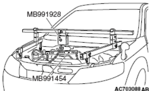
Fig. 109: Identifying Special Tool MB991928 Courtesy of MITSUBISHI MOTOR SALES OF AMERICA.
