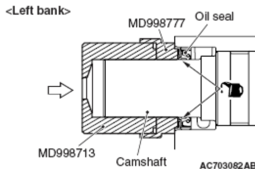
Fig. 61: Identifying Special Tools MD998713 And MD998777 - Right Bank Courtesy of MITSUBISHI MOTOR SALES OF AMERICA.
