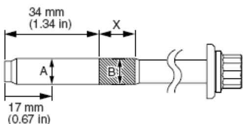
Fig. 84: Identifying Cylinder Head Bolt Dimension Courtesy of MITSUBISHI MOTOR SALES OF AMERICA.
