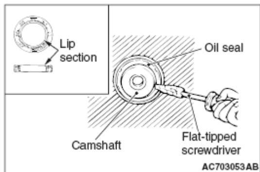
Fig. 39: Removing Oil Seal Courtesy of MITSUBISHI MOTOR SALES OF AMERICA.
