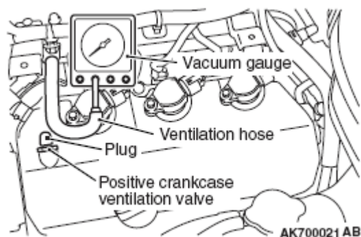
Fig. 20: Identifying Ventilation Hose, Positive Crankcase Ventilation (PCV) Valve And Vacuum Gauge Courtesy of MITSUBISHI MOTOR SALES OF AMERICA.
