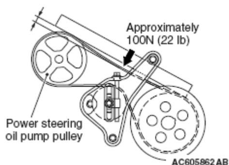
Fig. 6: Locating Power Steering Oil Pump Pulley Courtesy of MITSUBISHI MOTOR SALES OF AMERICA.
