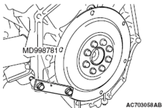
Fig. 75: Identifying Special Tool MD998781 Courtesy of MITSUBISHI MOTOR SALES OF AMERICA.
