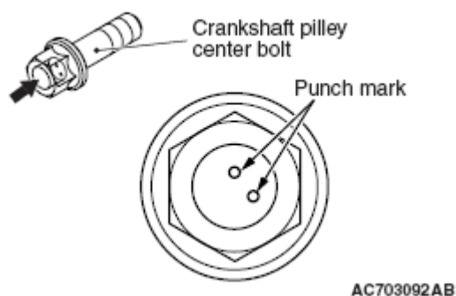
Fig. 29: Identifying Crankshaft Pulley And Punch Mark Courtesy of MITSUBISHI MOTOR SALES OF AMERICA.
