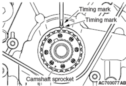
Fig. 92: Identifying Timing Mark On Crankshaft Sprocket With Engine Block
