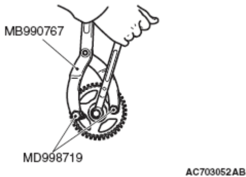
Fig. 38: Installing Camshaft Sprocket With Special Tools MB990767 And MD998719 Courtesy of MITSUBISHI MOTOR SALES OF AMERICA.
