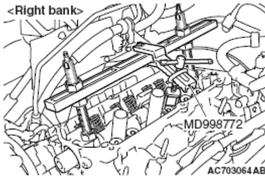
Fig. 45: Removing Valve Spring Retainer Locks With Special Tool MD998772 (Right Bank) Courtesy of MITSUBISHI MOTOR SALES OF AMERICA.
