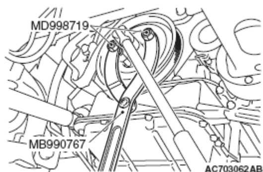
Fig. 86: Removing Crankshaft Pulley And Crankshaft Courtesy of MITSUBISHI MOTOR SALES OF AMERICA.
