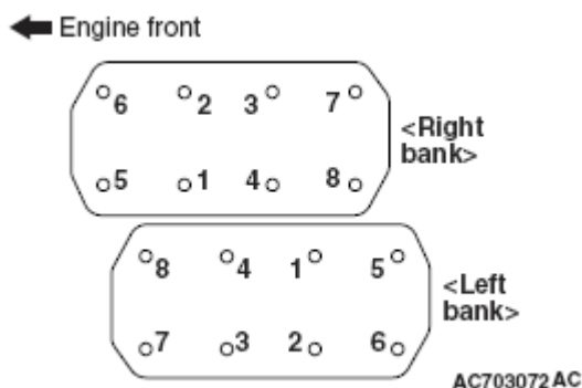
Fig. 81: Identifying Cylinder Head Bolt Tighten Sequence Courtesy of MITSUBISHI MOTOR SALES OF AMERICA.
