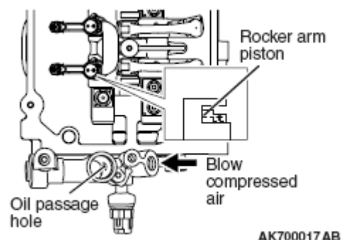
Fig. 11: Identifying Rocker Arm, Blow Compressed Air And Oil Pressure Hole Courtesy of MITSUBISHI MOTOR SALES OF AMERICA.
