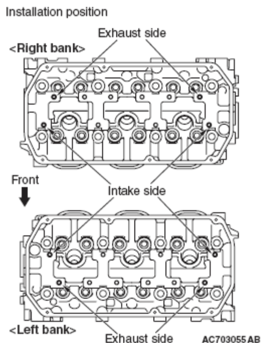
Fig. 46: Installing Valve Spring Retainer Locks Exhaust Side/Intake Side (Right Bank And Left Bank) Courtesy of MITSUBISHI MOTOR SALES OF AMERICA.
