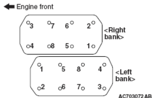
Fig. 78: Identifying Cylinder Head Bolt Loosen Sequence Courtesy of MITSUBISHI MOTOR SALES OF AMERICA.
