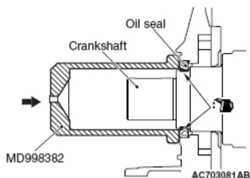
Fig. 69: Applying Engine Oil To Oil Seal Lip Courtesy of MITSUBISHI MOTOR SALES OF AMERICA.
