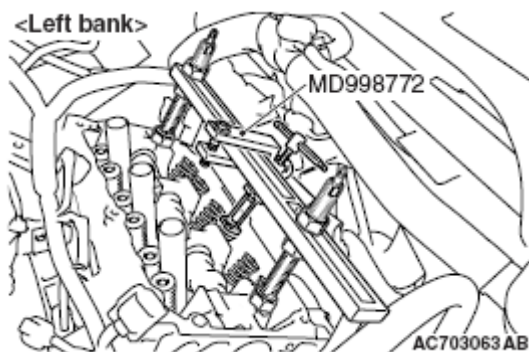
Fig. 49: Installing Valve Spring Retainer Locks With Special Tool MD998772 (Left Bank) Courtesy of MITSUBISHI MOTOR SALES OF AMERICA.
