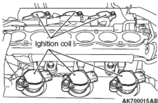
Fig. 8: Identifying Ignition Coil
