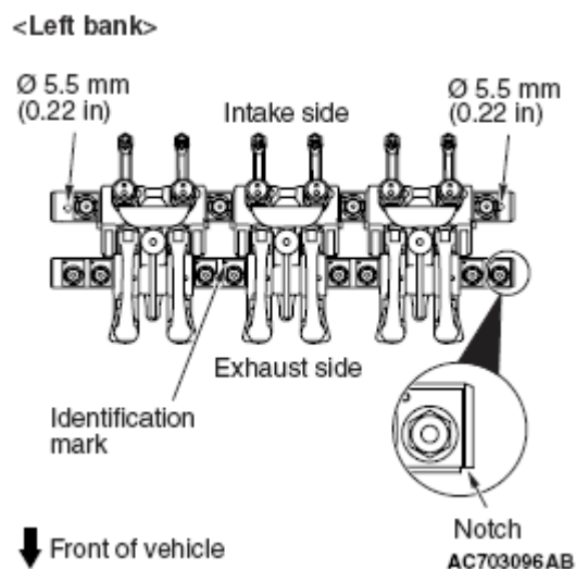
Fig. 52: Identifying Identification Mark Left Bank (Exhaust Side And Intake Side) Courtesy of MITSUBISHI MOTOR SALES OF AMERICA.
