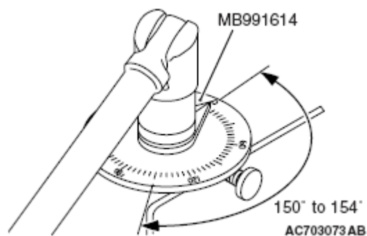
Fig. 82: Tightening Cylinder Head Bolt With Special Tool MB991614 Courtesy of MITSUBISHI MOTOR SALES OF AMERICA.
