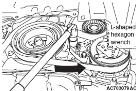
Fig. 27: Removing Generator Drive Belt
