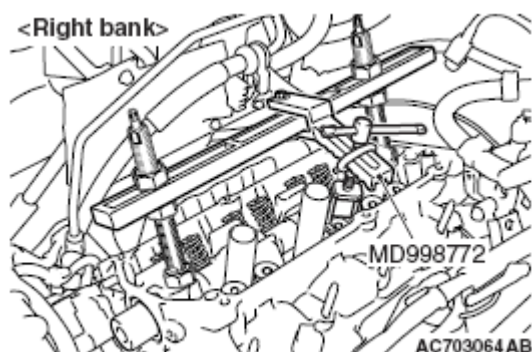
Fig. 50: Installing Valve Spring Retainer Locks With Special Tool MD998772 (Right Bank) Courtesy of MITSUBISHI MOTOR SALES OF AMERICA.
