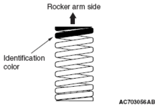
Fig. 48: Installing Valve Spring Courtesy of MITSUBISHI MOTOR SALES OF AMERICA.
