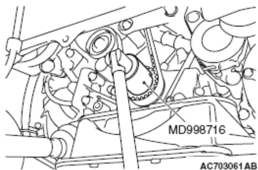
Fig. 94: Turning Crankshaft Clockwise Courtesy of MITSUBISHI MOTOR SALES OF AMERICA.
