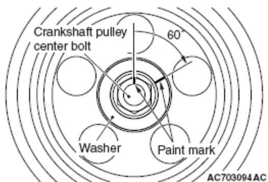
Fig. 32: Identifying Paint Mark On Crankshaft Bolt Courtesy of MITSUBISHI MOTOR SALES OF AMERICA.
