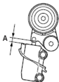
Fig. 95: Checking Auto-Tensioner Pushrod Extends With Standard Value Range Courtesy of MITSUBISHI MOTOR SALES OF AMERICA.
