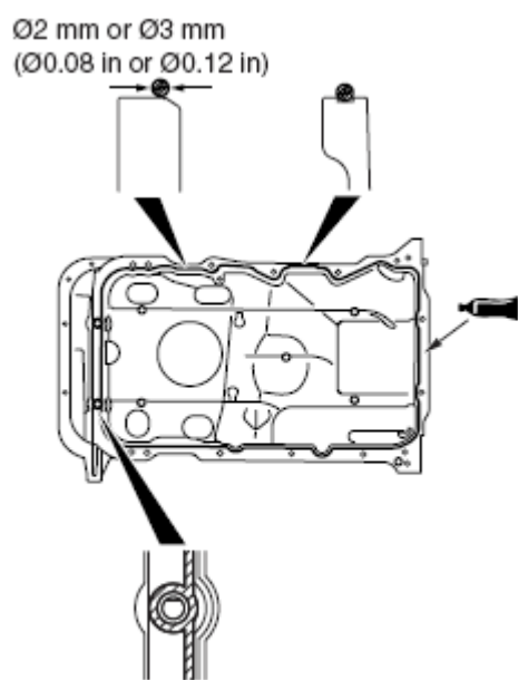
Fig. 63: Applying Bead Of Sealant To Cylinder Block Mating Surface Of Engine Oil Pan Courtesy of MITSUBISHI MOTOR SALES OF AMERICA.
