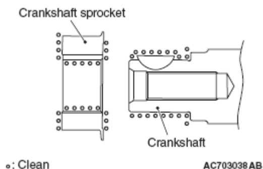
Fig. 70: Identifying Crankshaft And Crankshaft Sprocket Courtesy of MITSUBISHI MOTOR SALES OF AMERICA.
