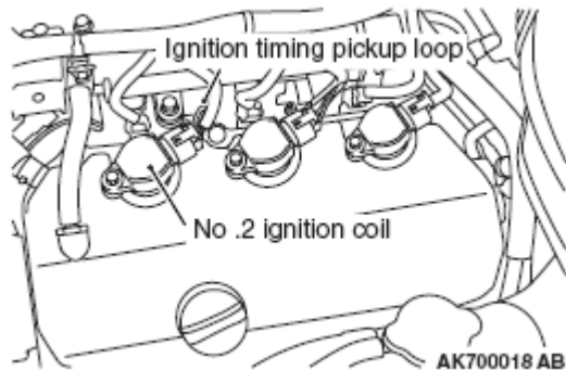
Fig. 17: Identifying Ignition Timing Pickup Loop And No.2 Ignition Coil Courtesy of MITSUBISHI MOTOR SALES OF AMERICA.
