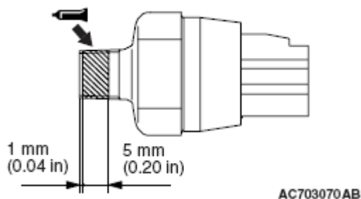
Fig. 58: Applying Sealant To Thread Of Engine Oil Pressure Switch Courtesy of MITSUBISHI MOTOR SALES OF AMERICA.
