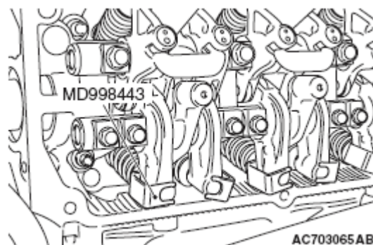
Fig. 53: Identifying Special Tool MD998443 Courtesy of MITSUBISHI MOTOR SALES OF AMERICA.
