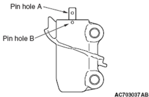
Fig. 90: Identifying Pin Hole A and Pin Hole B Courtesy of MITSUBISHI MOTOR SALES OF AMERICA.
