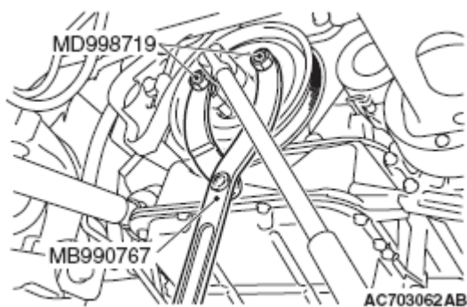
Fig. 96: Installing Crankshaft Pulley And Crankshaft Courtesy of MITSUBISHI MOTOR SALES OF AMERICA.
