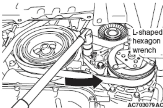
Fig. 85: Removing Generator Drive Belt
