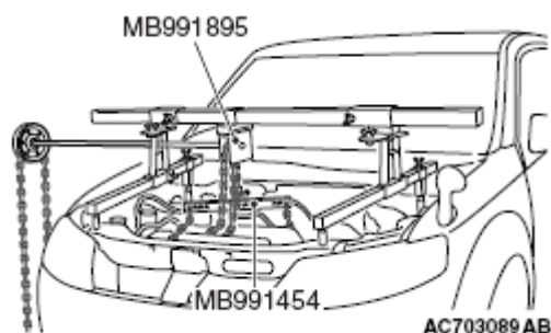
Fig. 102: Identifying Engine Hanger MB991895
