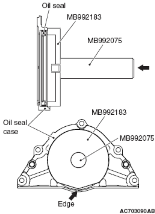
Fig. 73: Locating Special Tool MB992075 And MB992183
