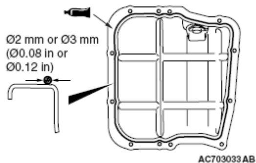
Fig. 65: Applying Bead Of Sealant To Mating Surface Of Engine Lower Oil Pan
