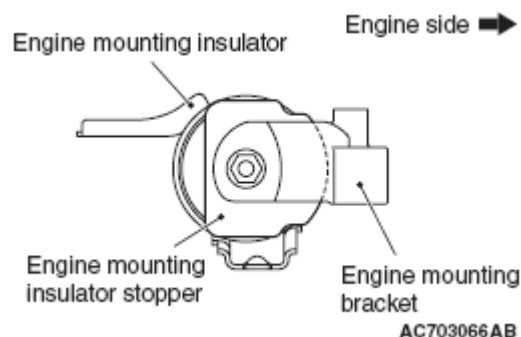
Fig. 106: Identifying Engine Mounting Insulator Stopper Courtesy of MITSUBISHI MOTOR SALES OF AMERICA.
