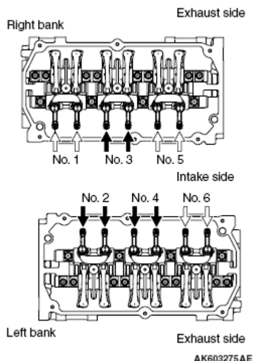
Fig. 10: Moving Rocker Arms On No. 1 And No. 4 Cylinders Courtesy of MITSUBISHI MOTOR SALES OF AMERICA.
