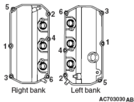
Fig. 54: Identifying Rocker Cover Bolts Tighten Sequence Courtesy of MITSUBISHI MOTOR SALES OF AMERICA.
