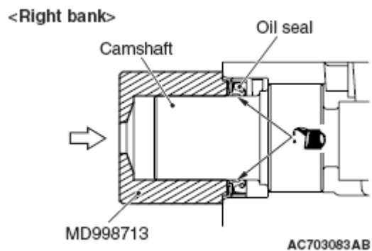
Fig. 55: Installing Camshaft Oil Seal (Right Bank) Courtesy of MITSUBISHI MOTOR SALES OF AMERICA.
