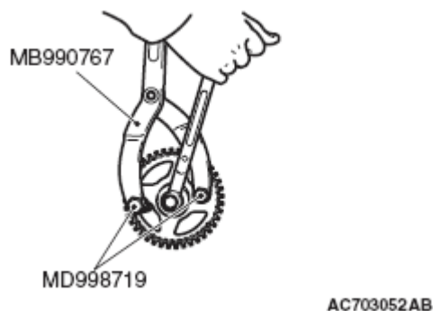
Fig. 57: Installing Camshaft Sprocket With Special Tools MB990767 And MD998719 Courtesy of MITSUBISHI MOTOR SALES OF AMERICA.
