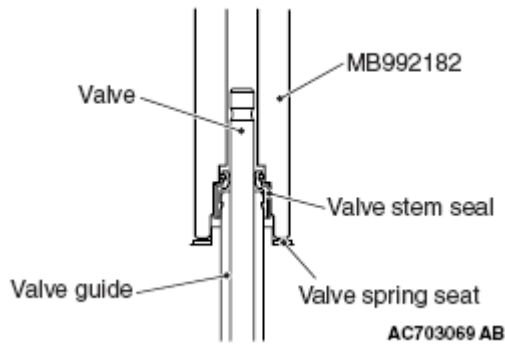
Fig. 47: Identifying Valve Guide, Valve, Valve Stem Seal And Valve Spring Seat Courtesy of MITSUBISHI MOTOR SALES OF AMERICA.
