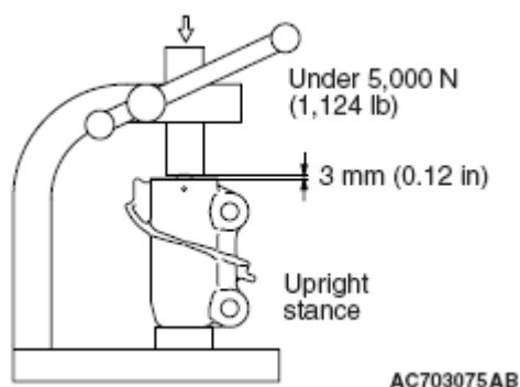
Fig. 89: Inserting Pin Into Rod Of Auto-Tensioner Courtesy of MITSUBISHI MOTOR SALES OF AMERICA.
