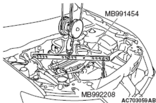
Fig. 105: Identifying Special Tool MB991454 And Special Tool MB992208 Courtesy of MITSUBISHI MOTOR SALES OF AMERICA.
