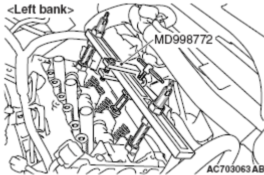
Fig. 44: Removing Valve Spring Retainer Locks With Special Tool MD998772 (Left Bank) Courtesy of MITSUBISHI MOTOR SALES OF AMERICA.
