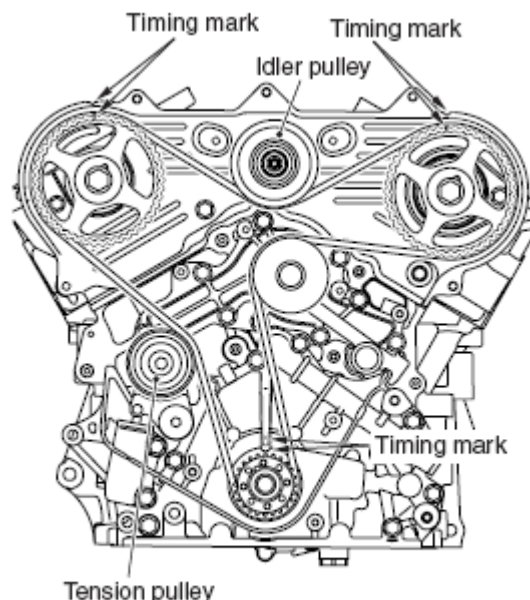
Fig. 88: Identifying Timing Belt Mark Location
