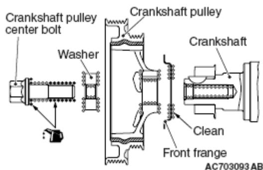
Fig. 30: Identifying Crankshaft Pulley Center Bolt, Crankshaft Pulley And Crankshaft Courtesy of MITSUBISHI MOTOR SALES OF AMERICA.
