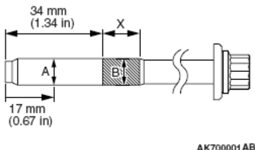
Fig. 79: Identifying Cylinder Head Bolt Dimension
