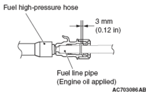
Fig. 107: Identifying Fuel High-Pressure Hose Connection Courtesy of MITSUBISHI MOTOR SALES OF AMERICA.
