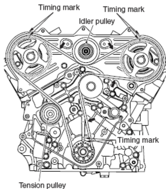
Fig. 93: Identifying Timing Mark Of Idler Pulley And Tension Pulley Courtesy of MITSUBISHI MOTOR SALES OF AMERICA.
