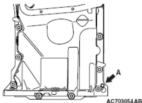
Fig. 62: Identifying Engine Upper Oil Pan Bolt Hole Courtesy of MITSUBISHI MOTOR SALES OF AMERICA.
