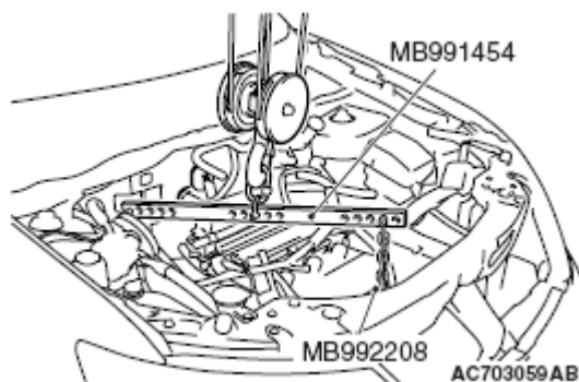
Fig. 104: Identifying Special Tool MB991454 And Special Tool MB992208 Courtesy of MITSUBISHI MOTOR SALES OF AMERICA.
