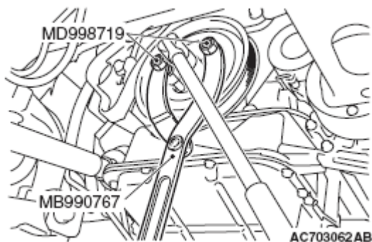
Fig. 28: Removing Crankshaft Pulley And Crankshaft
