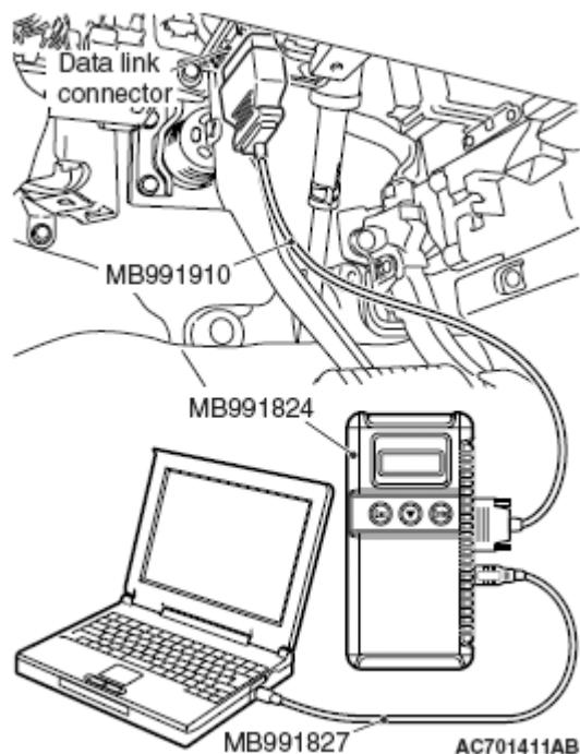
Fig. 16: Connecting Scan Tool MB991958 To Data Link Connector Courtesy of MITSUBISHI MOTOR SALES OF AMERICA.
