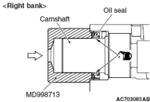
Fig. 36: Installing Camshaft Oil Seal (Right Bank) Courtesy of MITSUBISHI MOTOR SALES OF AMERICA.
