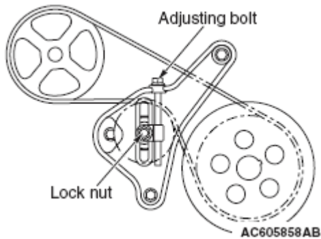
Fig. 7: Identifying Lock Nut And Adjusting Bolt Courtesy of MITSUBISHI MOTOR SALES OF AMERICA.
