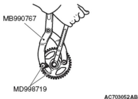
Fig. 77: Removing Camshaft Sprocket With Special Tools MB990767 And MD998719 Courtesy of MITSUBISHI MOTOR SALES OF AMERICA.
