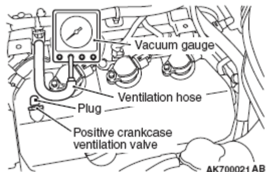
Fig. 22: Identifying Vacuum Gauge, Ventilation Hose And PCV Valve
