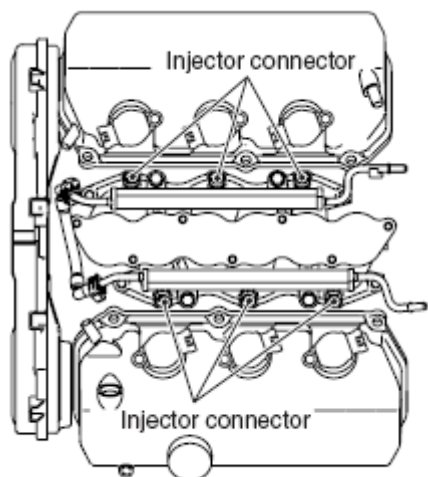
Fig. 18: Identifying Injector Connectors
