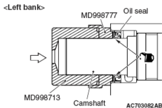
Fig. 56: Installing Camshaft Oil Seal (Left Bank) Courtesy of MITSUBISHI MOTOR SALES OF AMERICA.
