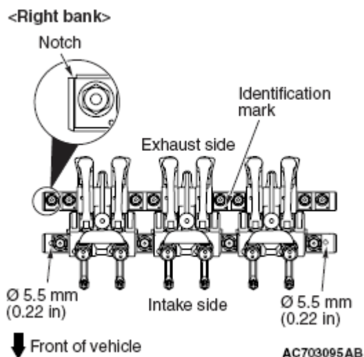
Fig. 51: Identifying Identification Mark Right Bank (Exhaust Side And Intake Side) Courtesy of MITSUBISHI MOTOR SALES OF AMERICA.
