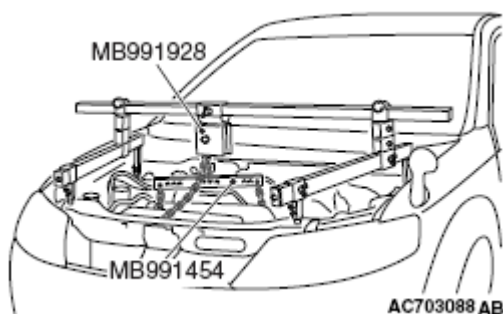
Fig. 103: Identifying Engine Hanger MB991928
