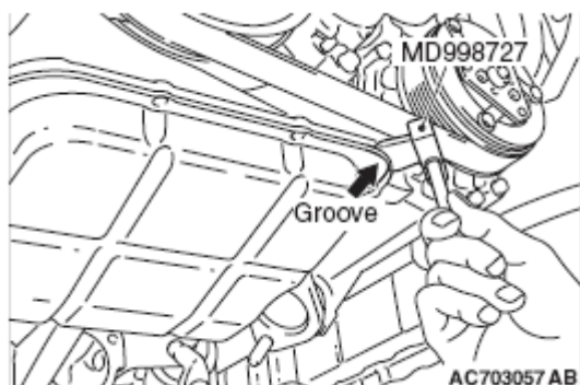
Fig. 61: Inserting Special Tool MD998727 Into Groove Courtesy of MITSUBISHI MOTOR SALES OF AMERICA.
