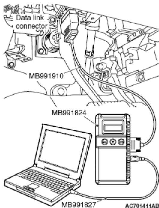
Fig. 21: Connecting Scan Tool MB991958 To Data Link Connector Courtesy of MITSUBISHI MOTOR SALES OF AMERICA.
