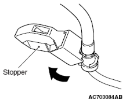
Fig. 100: Removing Fuel High-Pressure Hose Stopper Courtesy of MITSUBISHI MOTOR SALES OF AMERICA.
