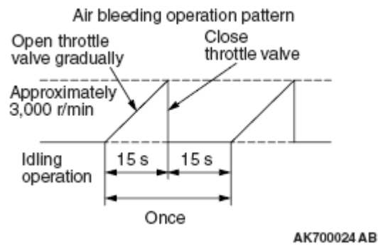
Fig. 25: Air Bleeding Operation Pattern
