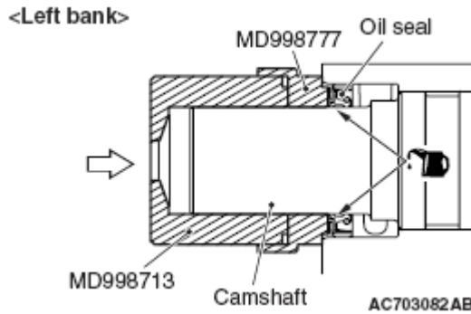
Fig. 37: Installing Camshaft Oil Seal (Left Bank) Courtesy of MITSUBISHI MOTOR SALES OF AMERICA.
