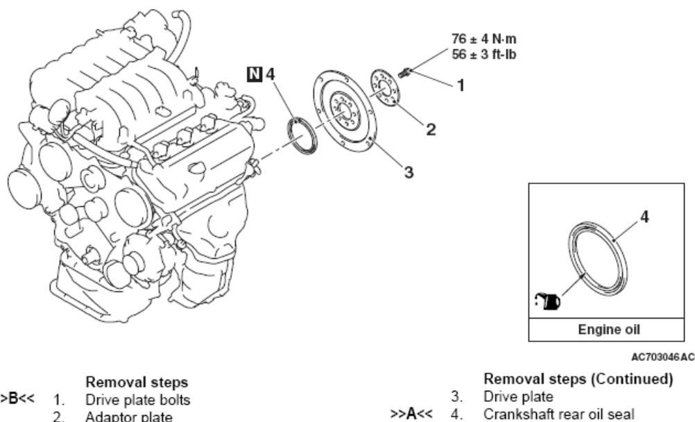
Fig. 71: Identifying Crankshaft Rear Oil Seal With Torque Specifications Courtesy of MITSUBISHI MOTOR SALES OF AMERICA.
