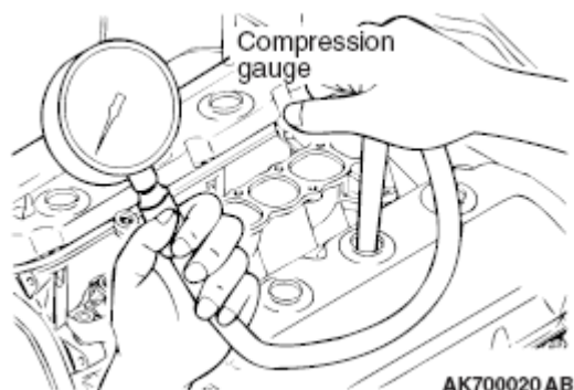
Fig. 19: Setting Compression Gauge To Spark Plug Holes Courtesy of MITSUBISHI MOTOR SALES OF AMERICA.
