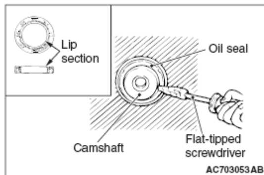
Fig. 43: Removing Camshaft Oil Seal Courtesy of MITSUBISHI MOTOR SALES OF AMERICA.
