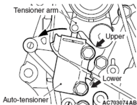
Fig. 87: Removing Upper Tightening Bolt Of Auto-Tensioner Courtesy of MITSUBISHI MOTOR SALES OF AMERICA.
