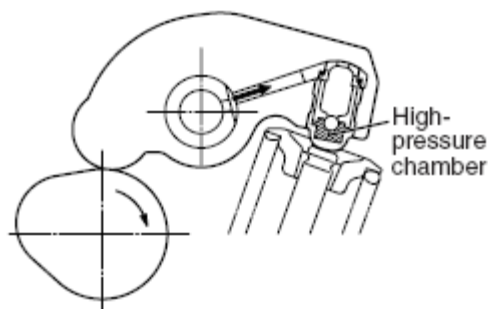
Fig. 24: Identifying High Pressure Chamber Courtesy of MITSUBISHI MOTOR SALES OF AMERICA.
