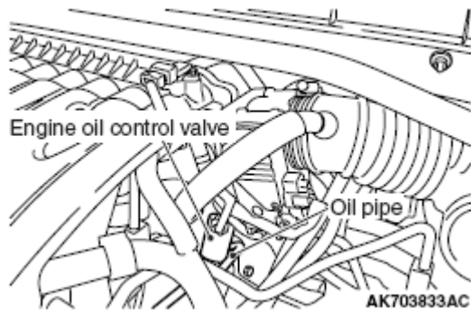
Fig. 9: Identifying Engine Oil Valve And Oil Pipe
