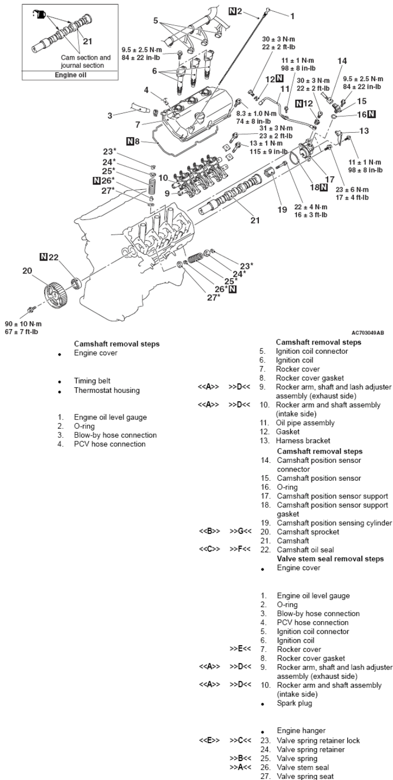
Fig. 39: Identifying Camshaft & Valve Stem Seal Parts With Torque Specifications (Left Bank) Courtesy of MITSUBISHI MOTOR SALES OF AMERICA.
