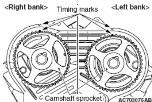
Fig. 91: Aligning Timing Marks On Camshaft Sprockets With Timing Belt
