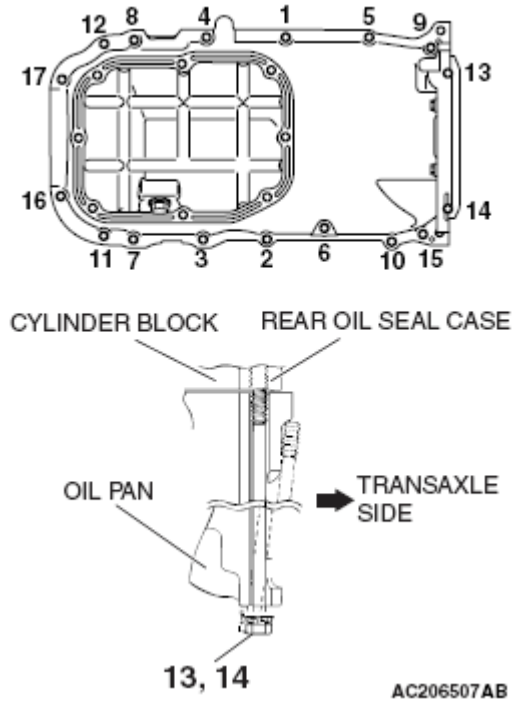
Fig. 66: Identifying Cylinder Block Bolts With Tighten Sequence Courtesy of MITSUBISHI MOTOR SALES OF AMERICA.
