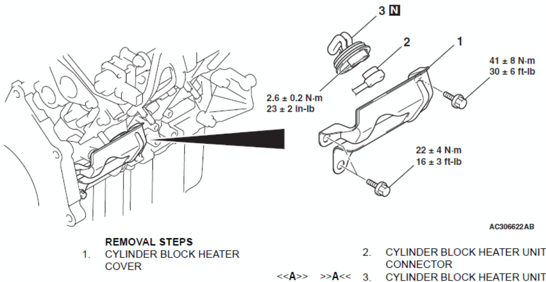
Fig. 103: Identifying Cylinder Block Heater Unit Components With Torque Specifications
