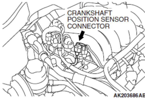
Fig. 13: Identifying Crankshaft Position Sensor Connector Courtesy of MITSUBISHI MOTOR SALES OF AMERICA.
