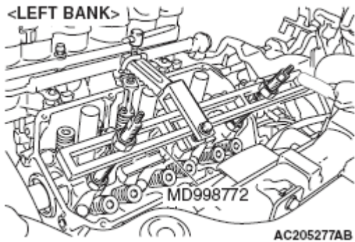
Fig. 49: Compressing Valve Spring Left Bank
