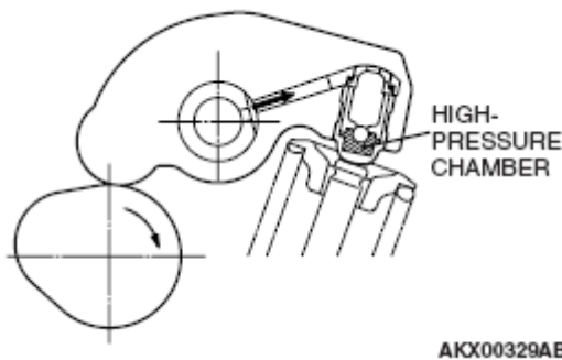
Fig. 19: Identifying High Pressure Chamber
