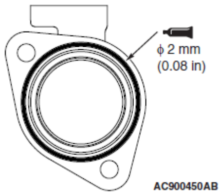
Fig. 60: Identifying Camshaft Position Sensor Support Flange Sealant Area Courtesy of MITSUBISHI MOTOR SALES OF AMERICA.
