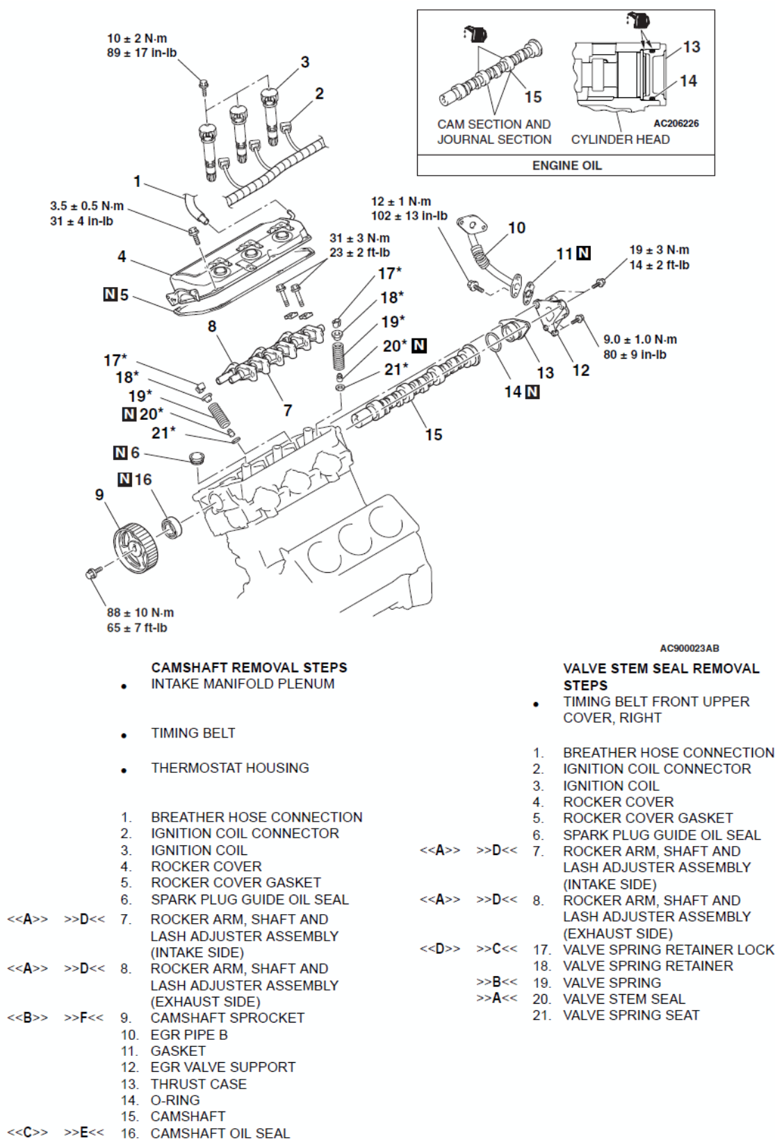
Fig. 44: Identifying Camshaft And Valve Stem Seal Components With Torque Specifications (Right Bank)
