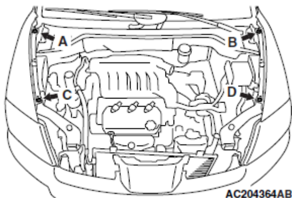
Fig. 30: Identifying Front Fender Assembling Bolts A, B, C And D
