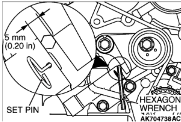
Fig. 93: Identifying Width Between Auto-Tensioner And Tensioner Arm Courtesy of MITSUBISHI MOTOR SALES OF AMERICA.
