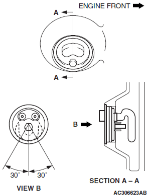
Fig. 104: Identifying Range For Installing Cylinder Block Heater Unit To Cylinder Block Courtesy of MITSUBISHI MOTOR SALES OF AMERICA.
