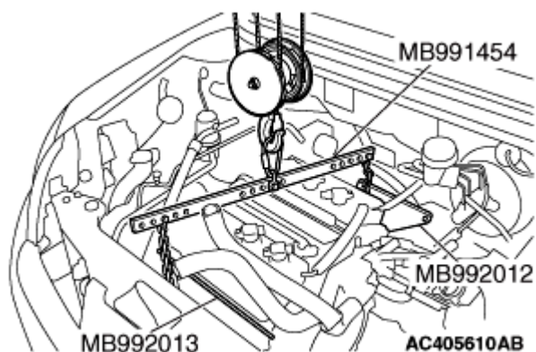
Fig. 29: Hooking Engine
