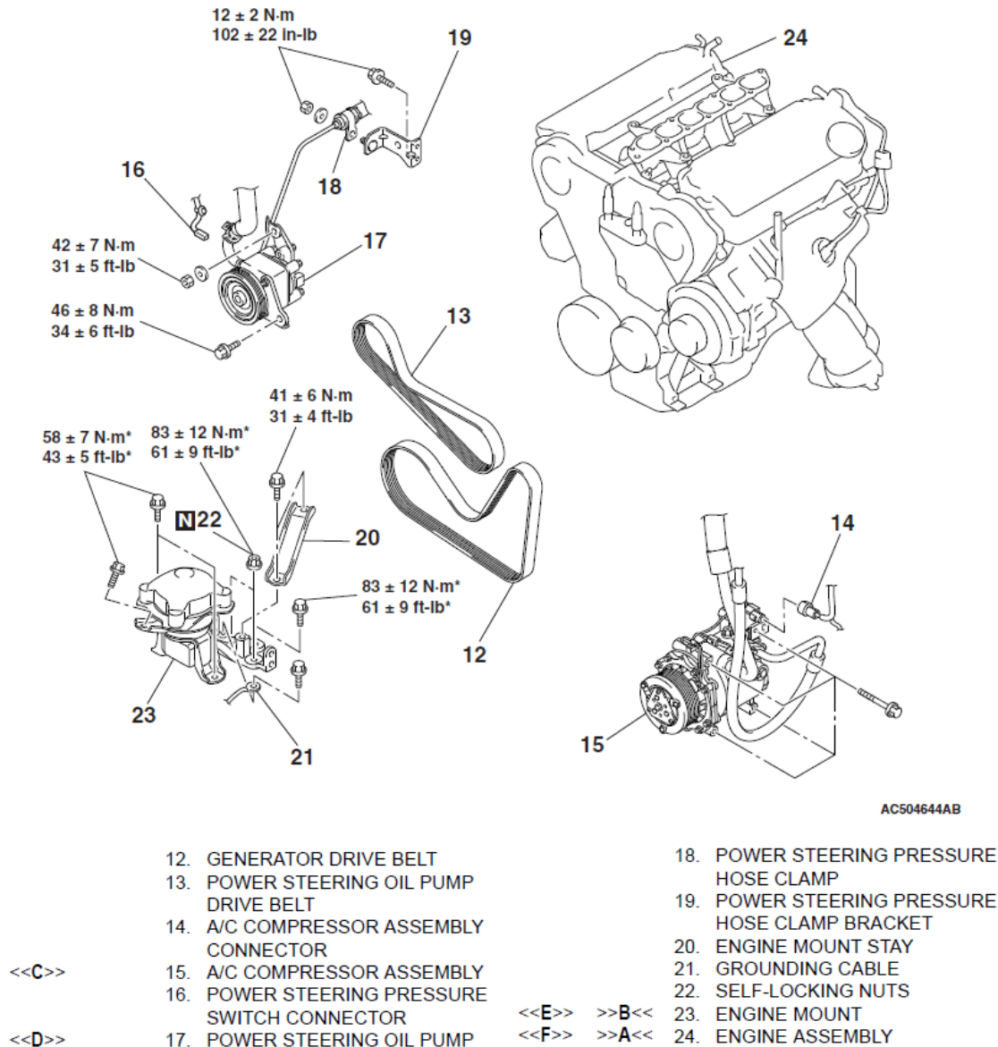
Fig. 23: Identifying Engine Components With Torque Specifications (2 Of 2) Courtesy of MITSUBISHI MOTOR SALES OF AMERICA.
