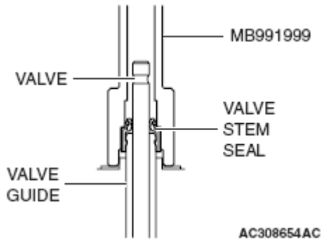
Fig. 51: Identifying Valve Stem Seal, Valve Guide And Valve Courtesy of MITSUBISHI MOTOR SALES OF AMERICA.
