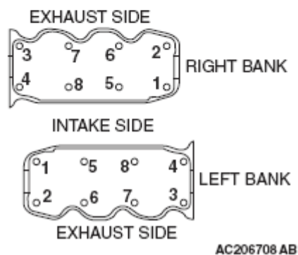
Fig. 77: Identifying Cylinder Head Assembly
