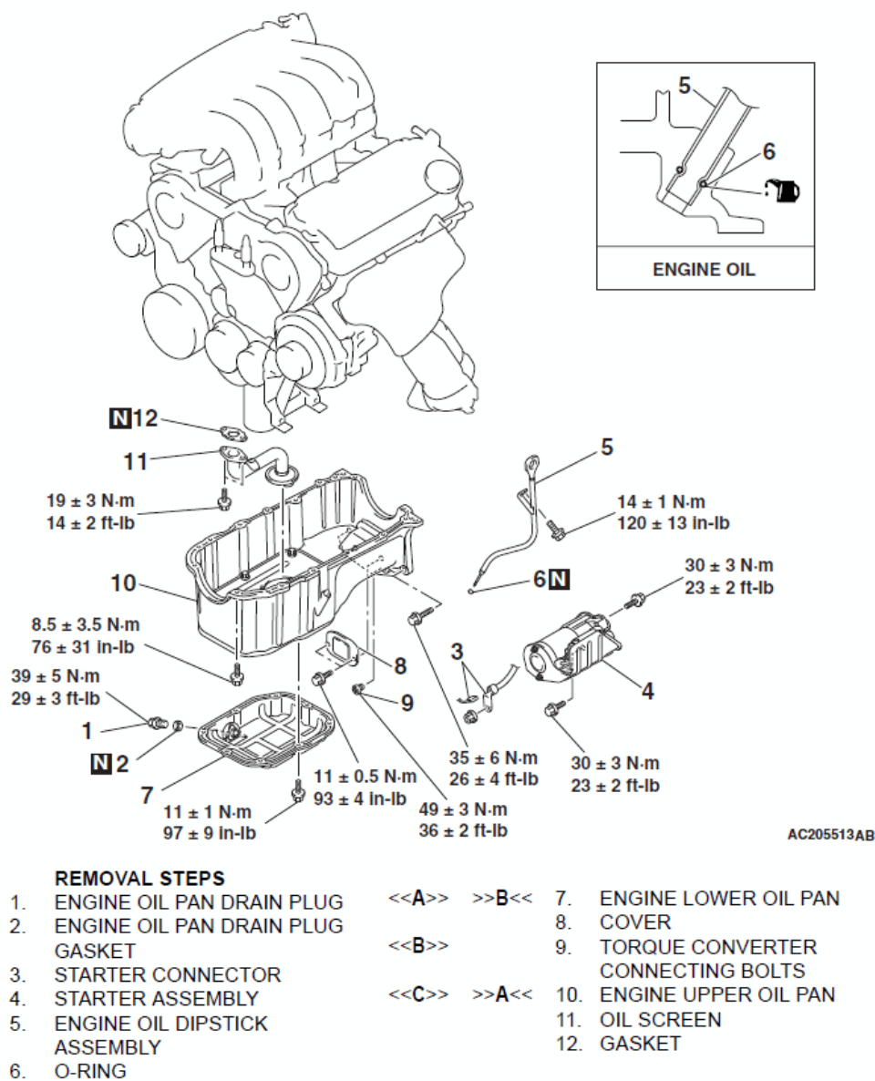
Fig. 61: Identifying Oil Pan And Oil Screen Components With Torque Specifications Courtesy of MITSUBISHI MOTOR SALES OF AMERICA.
