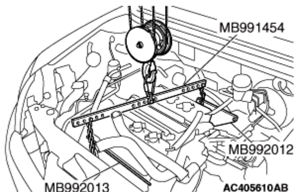
Fig. 28: Hooking Engine Courtesy of MITSUBISHI MOTOR SALES OF AMERICA.
