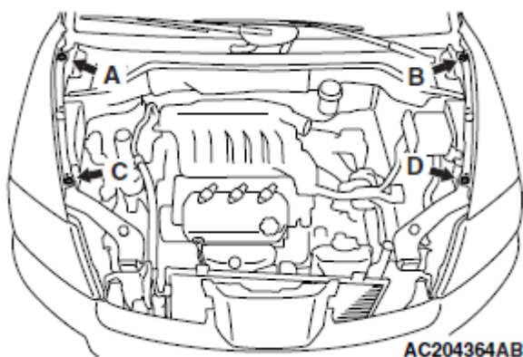
Fig. 34: Identifying Front Fender Assembling Bolts A, B, C And D
