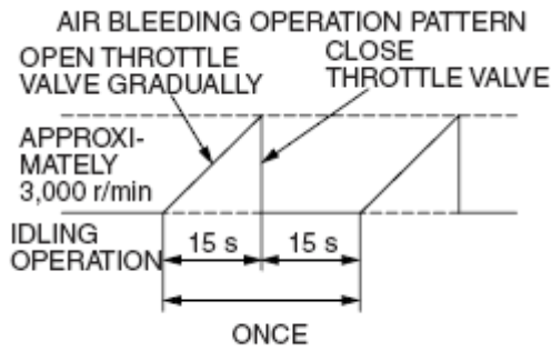
Fig. 20: Identifying Air Bleeding Operation Pattern
