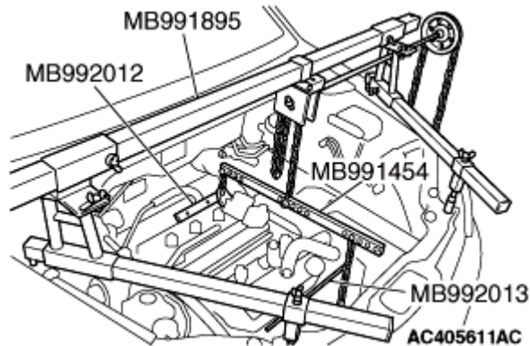
Fig. 26: Supporting Engine Using Special Tool MB991895 Courtesy of MITSUBISHI MOTOR SALES OF AMERICA.
