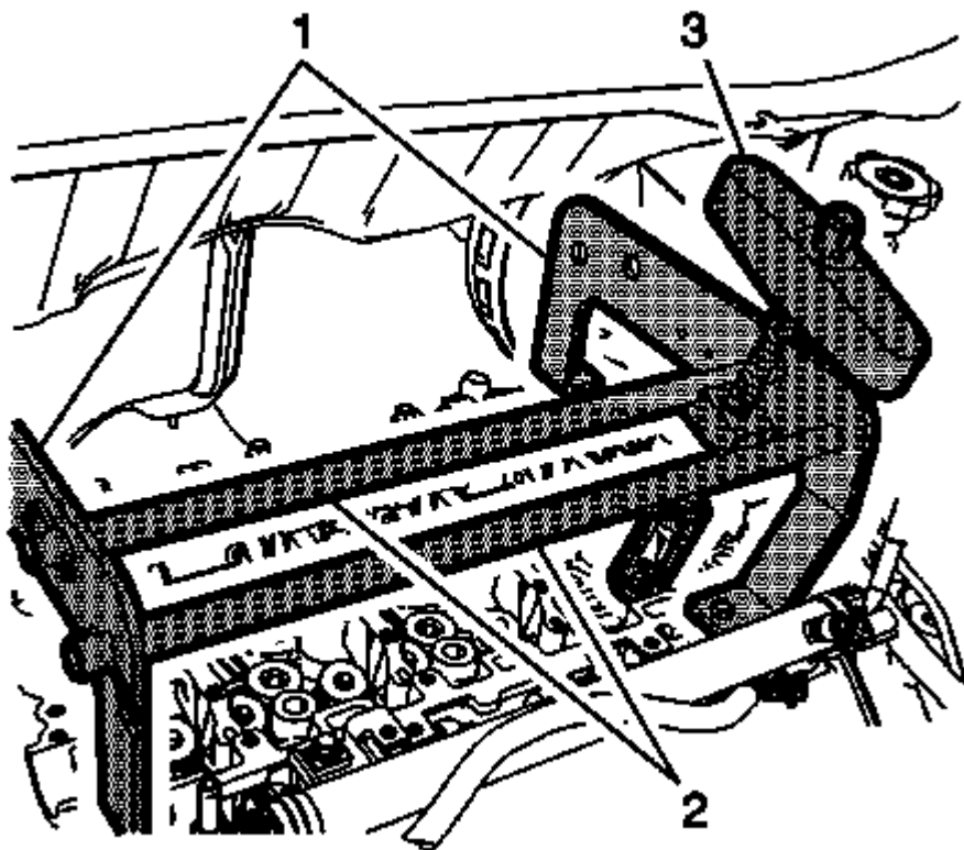
Fig. 193: View Of Valve Spring Compressor Adaptor Set Courtesy of GENERAL MOTORS COMPANY
