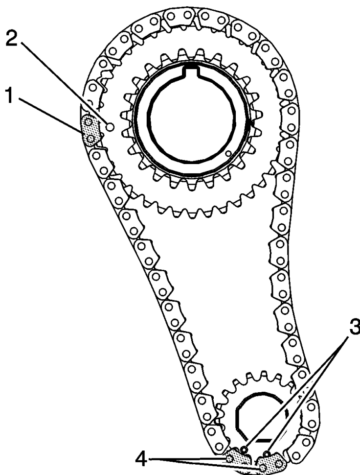
Fig. 109: Timing Link And Timing Mark Courtesy of GENERAL MOTORS COMPANY
