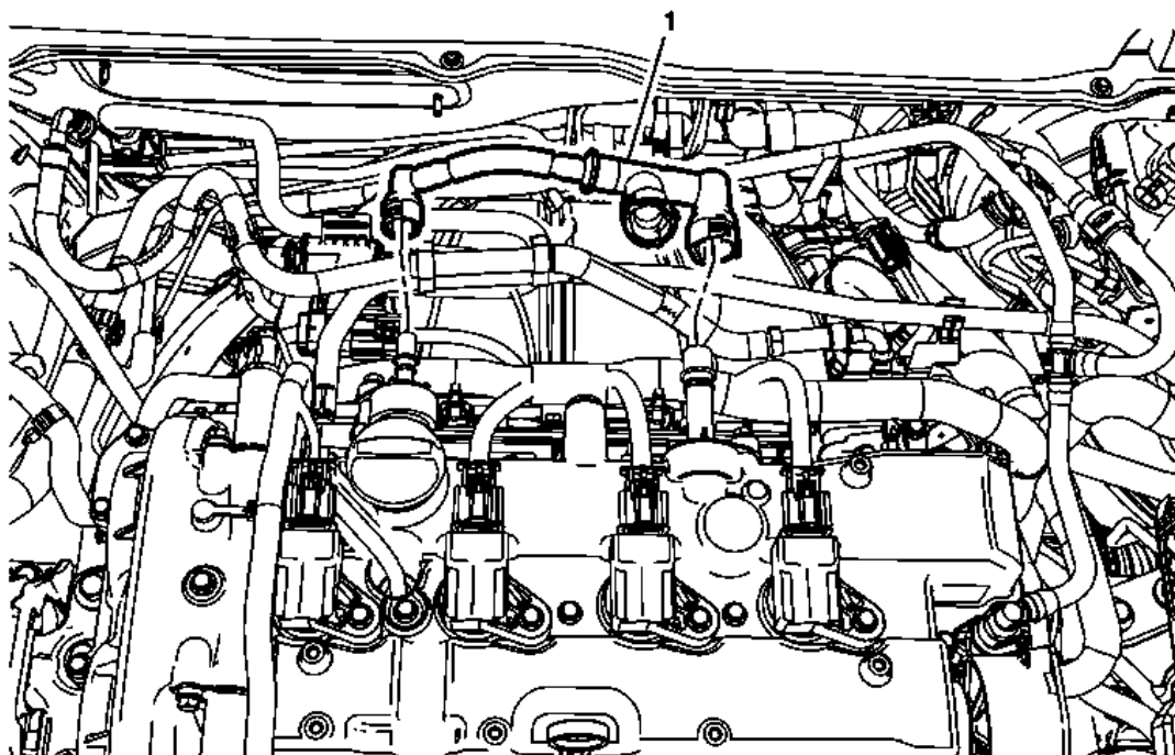
Fig. 34: Positive Crankcase Ventilation Hose/Pipe/Tube (LCV)
