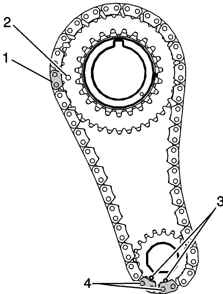
Fig. 65: Timing Link And Timing Mark Courtesy of GENERAL MOTORS COMPANY
