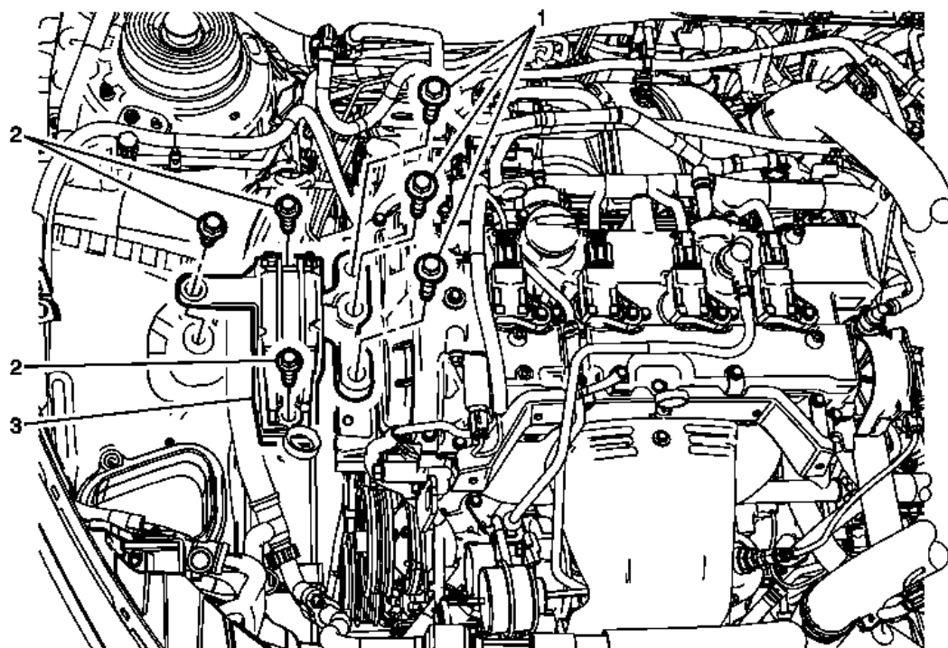
Fig. 17: Engine Mount (LTG)
