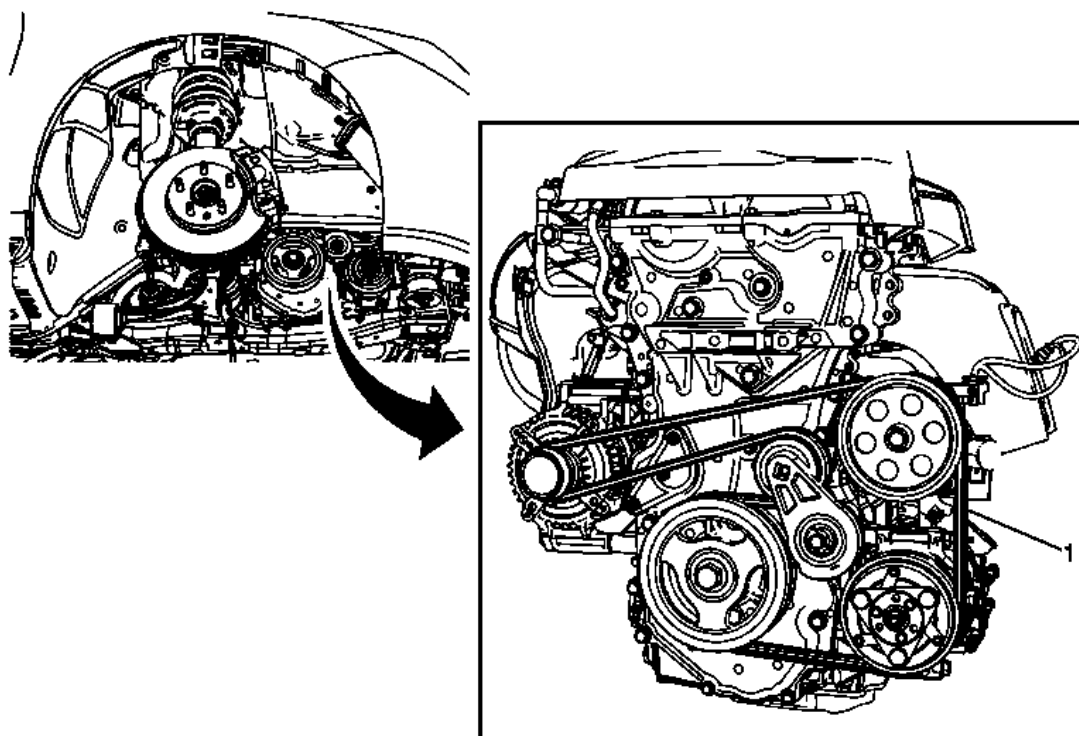
Fig. 3: Drive Belt Routing
