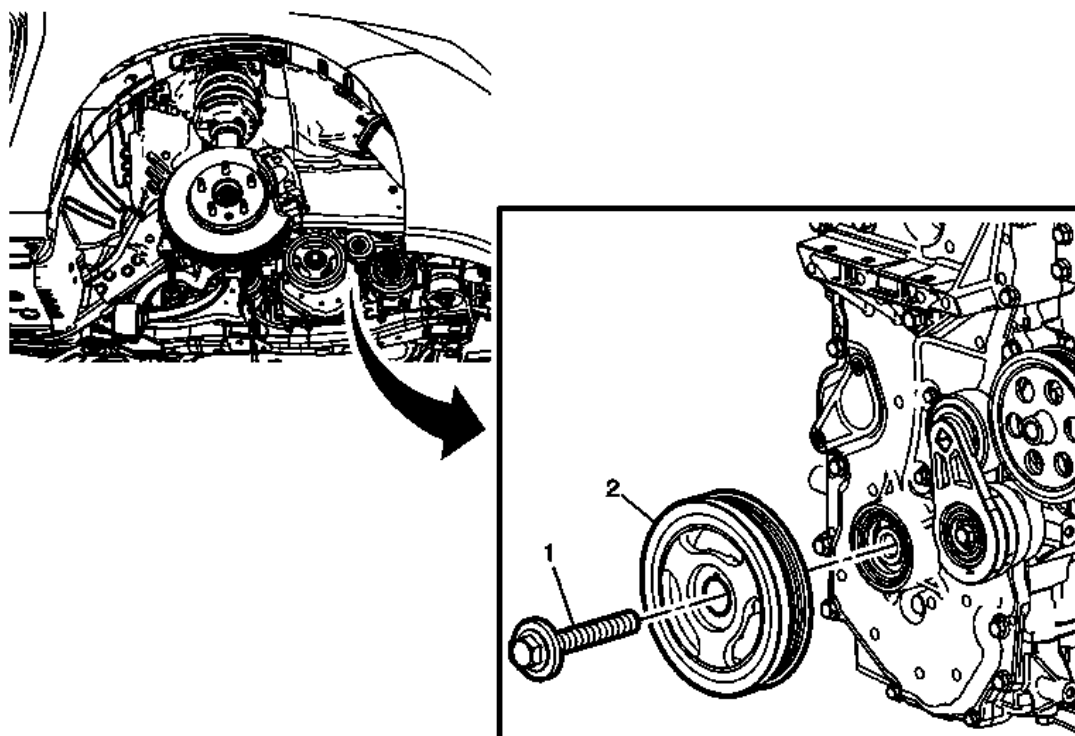
Fig. 58: Crankshaft Balancer
