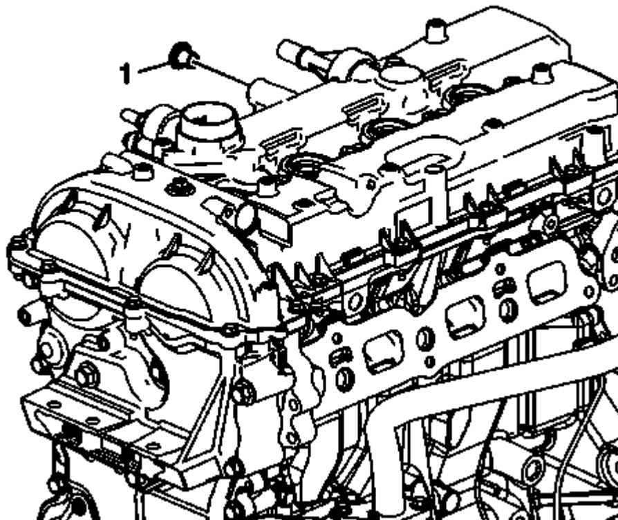
Fig. 135: Camshaft Cover Plug
