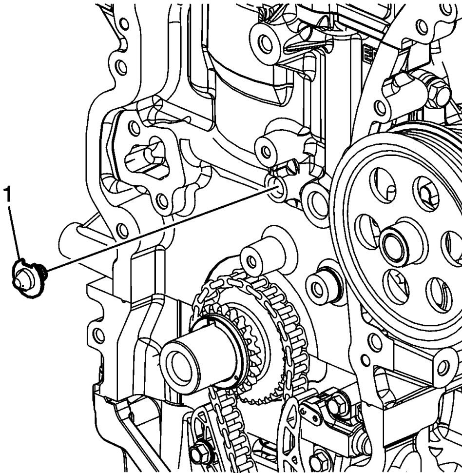
Fig. 99: Timing Chain Oil Nozzle
