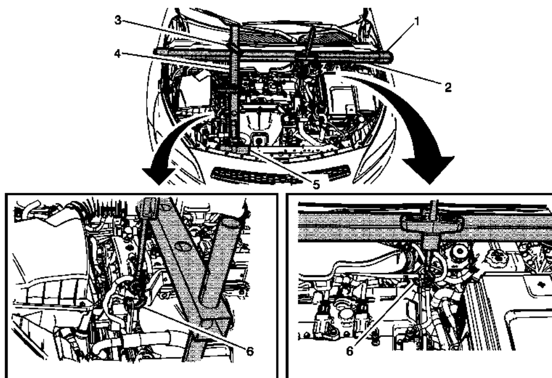
Fig. 18: Engine Support
