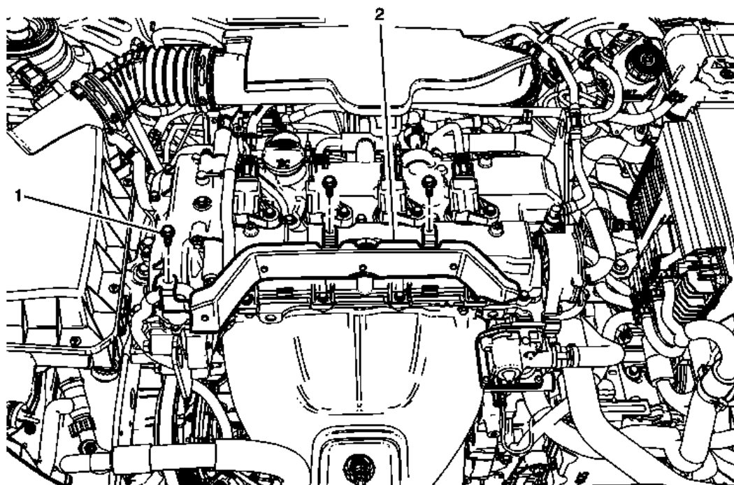
Fig. 192: Camshaft Cover Heat Shield
