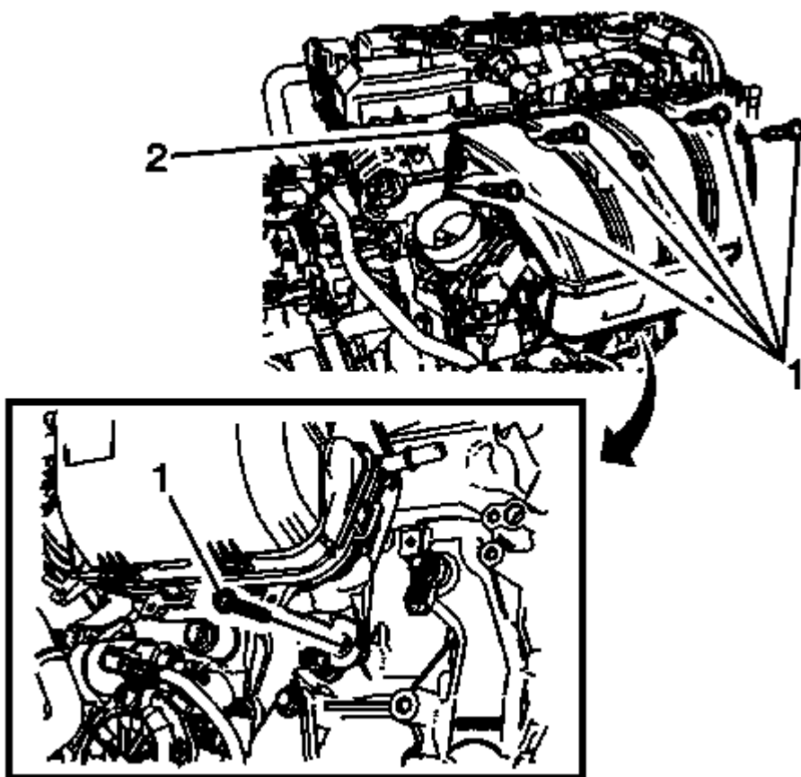
Fig. 53: Intake Bolts
