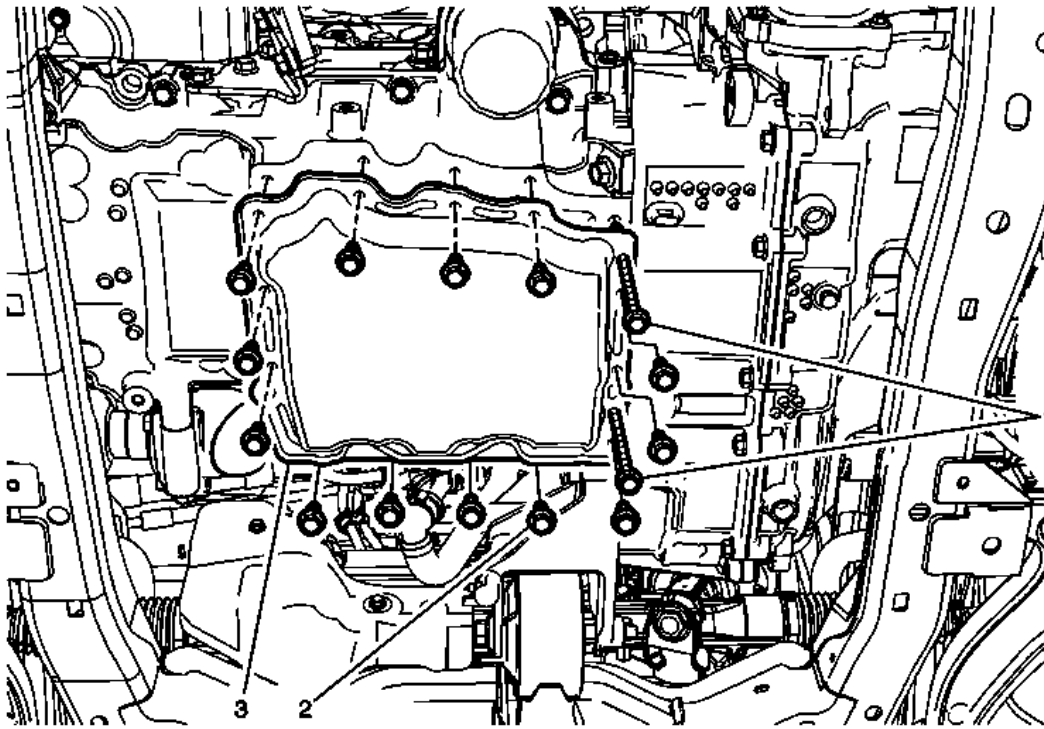
Fig. 208: Oil Pan
