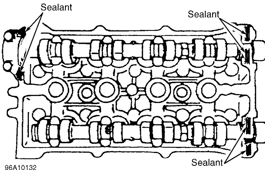
Fig. 13: Silicone Sealant Application Locations Courtesy of KIA MOTORS AMERICA, INC.
