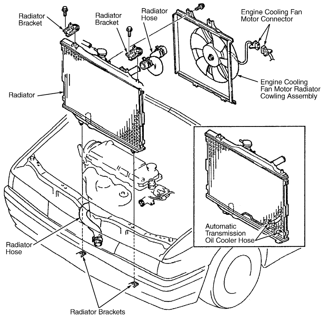
Fig. 14: Removing & Installing Radiator Courtesy of KIA MOTORS AMERICA, INC.
