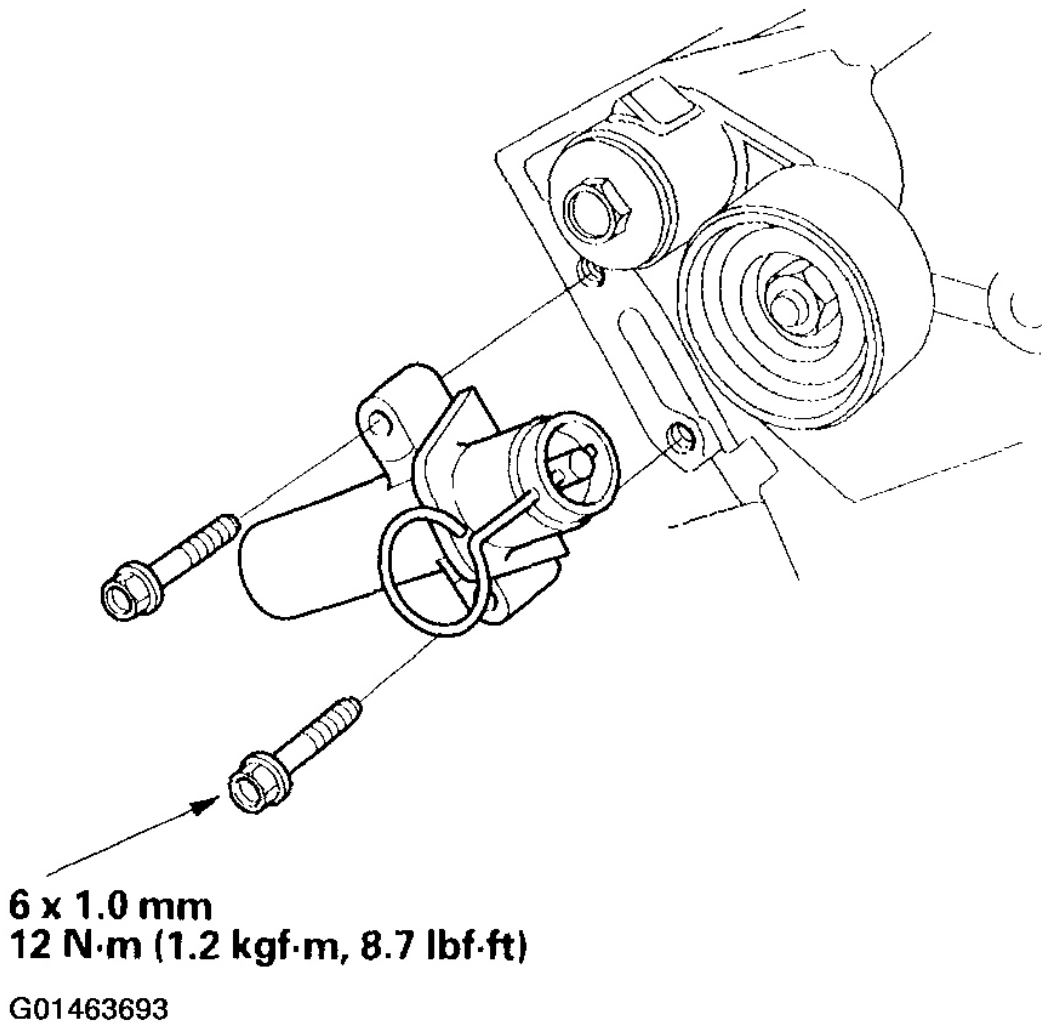
Fig. 106: Installing The Auto-Tensioner
