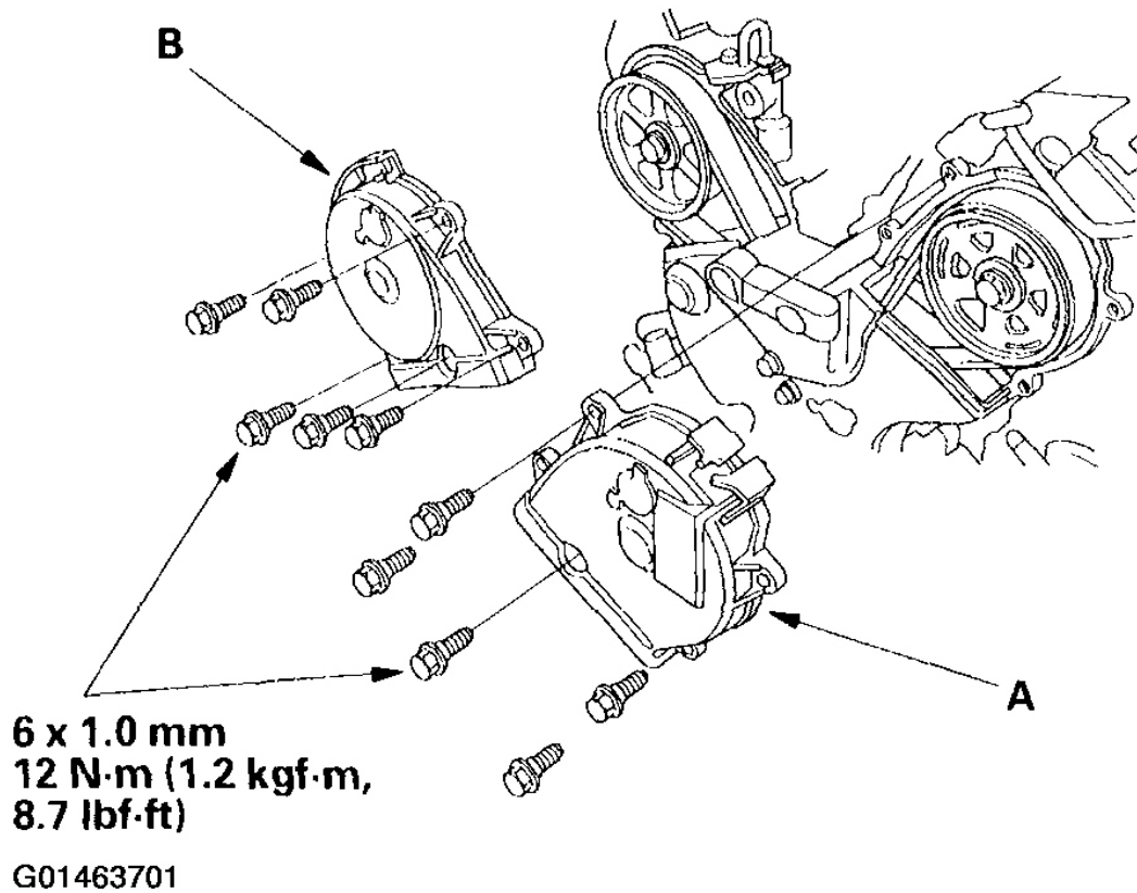
Fig. 114: Installing The Front Upper Cover & Rear Upper Cover Courtesy of AMERICAN HONDA MOTOR CO., INC.
