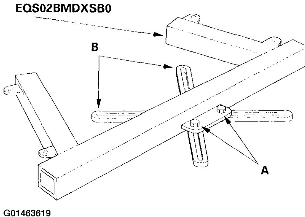
Fig. 32: Loosening The Four Bolts Holding The Adjustable Arms Of The Front Subframe Adapter To Its Center Plate
