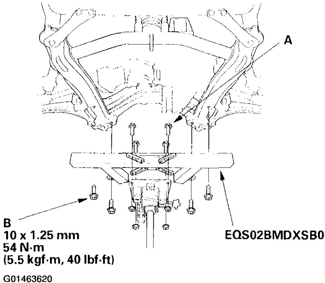
Fig. 33: Lining Up The Slots In The Arms With The Bolt Holes On The Corner Of The Jack Base, & Attaching The Front Subframe Adapter To The Jack Base Courtesy of AMERICAN HONDA MOTOR CO., INC.
