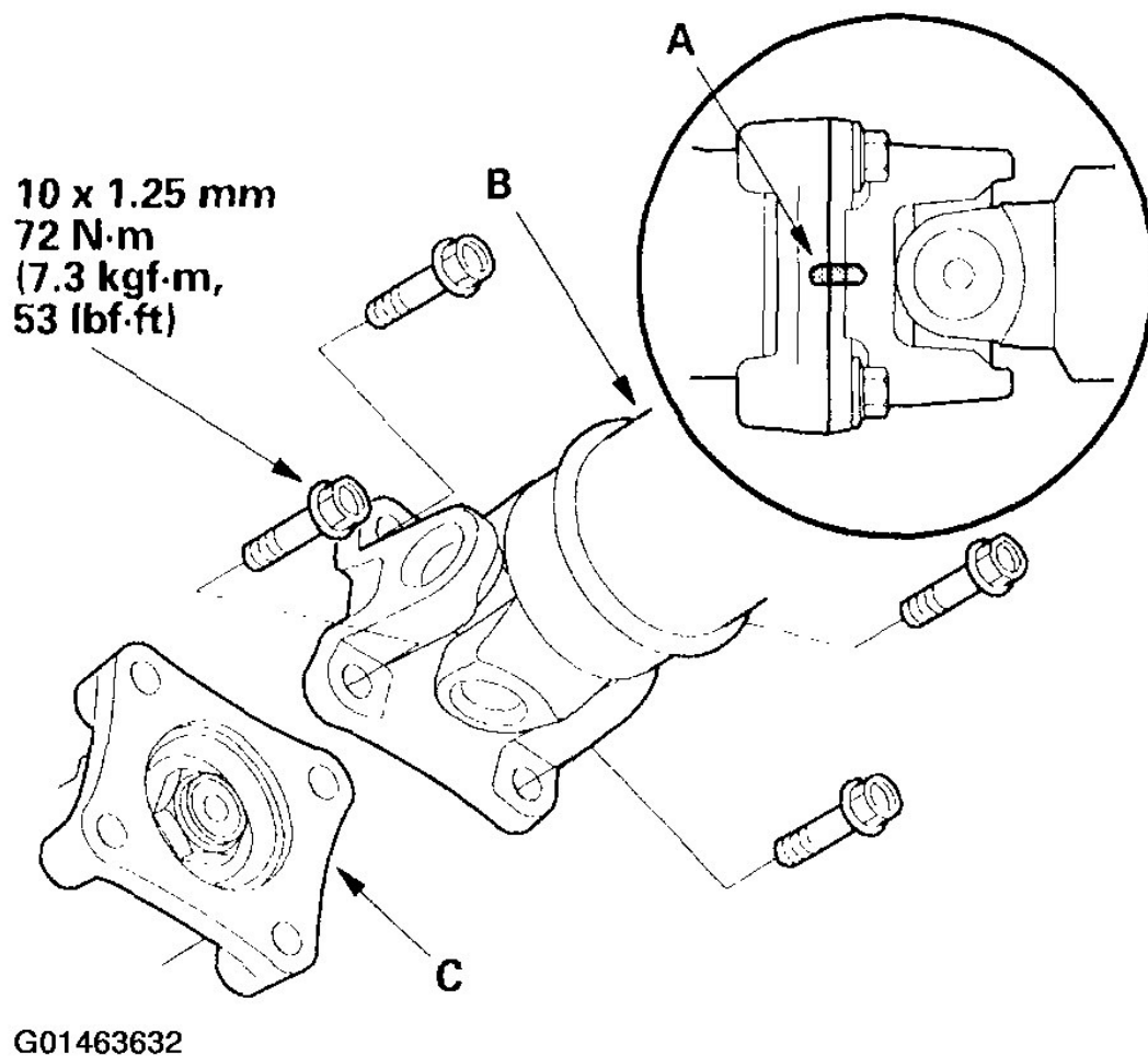
Fig. 45: Aligning The Reference Marks On The Propeller Shaft & Transfer Shaft Flange, & Installing The Propeller Shaft
