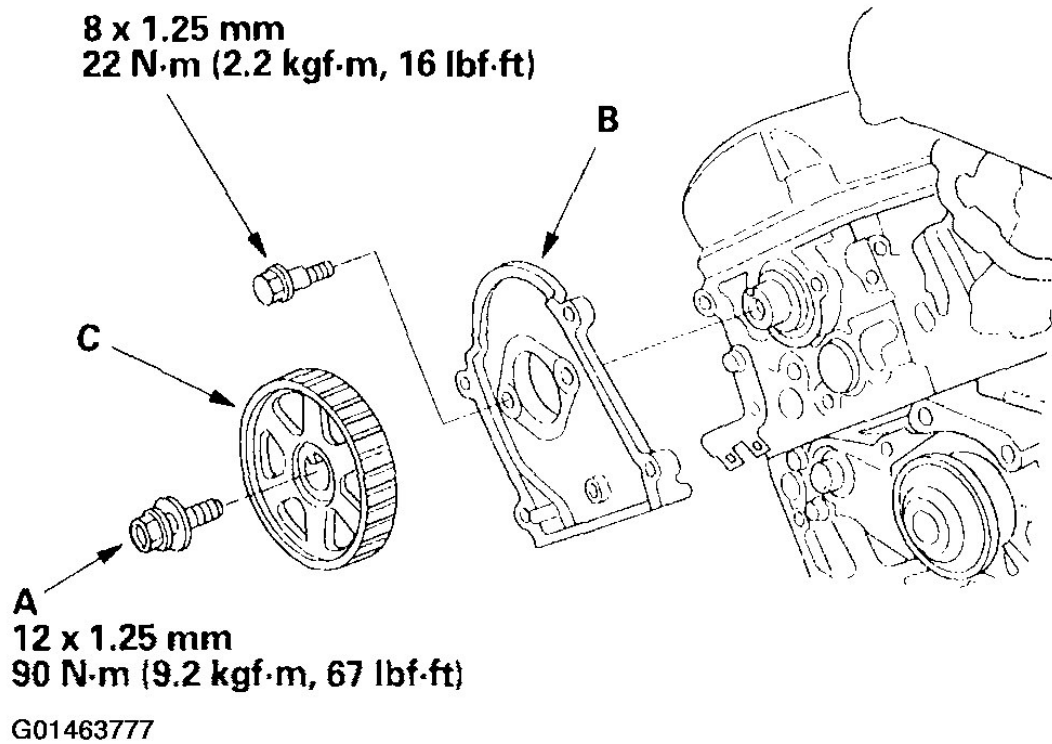
Fig. 190: Installing Camshaft Pulley Mounting Bolt, Back Cover & Camshaft Pulley Courtesy of AMERICAN HONDA MOTOR CO., INC.
