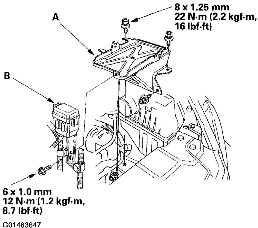
Fig. 60: Installing The Battery Base & The Relay Bracket Courtesy of AMERICAN HONDA MOTOR CO., INC.
