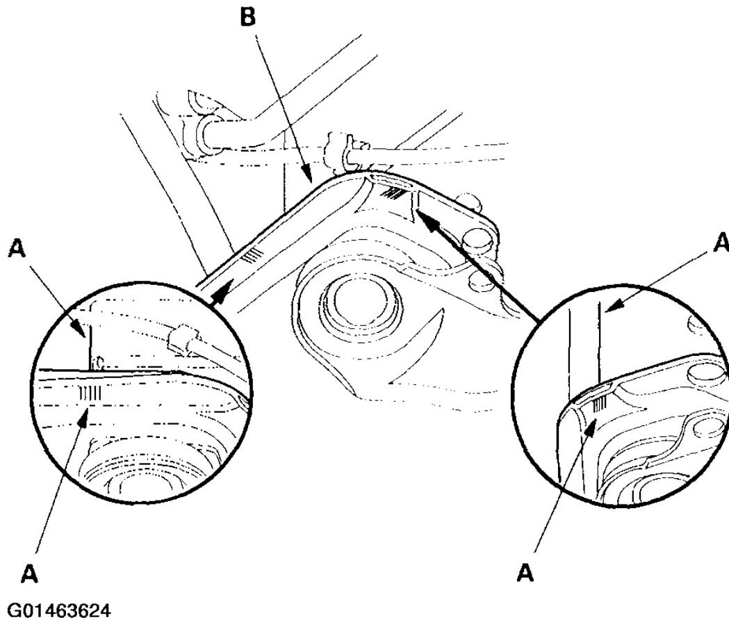
Fig. 37: Aligning All Reference Marks On The Front Subframe With The Body, & Tightening The Bolts On The Front Subframe Courtesy of AMERICAN HONDA MOTOR CO., INC.
