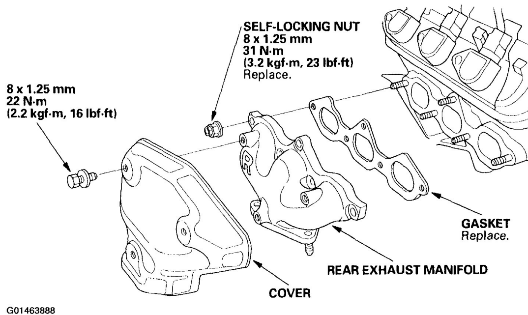
Fig. 282: Removing Rear Exhaust Manifold
