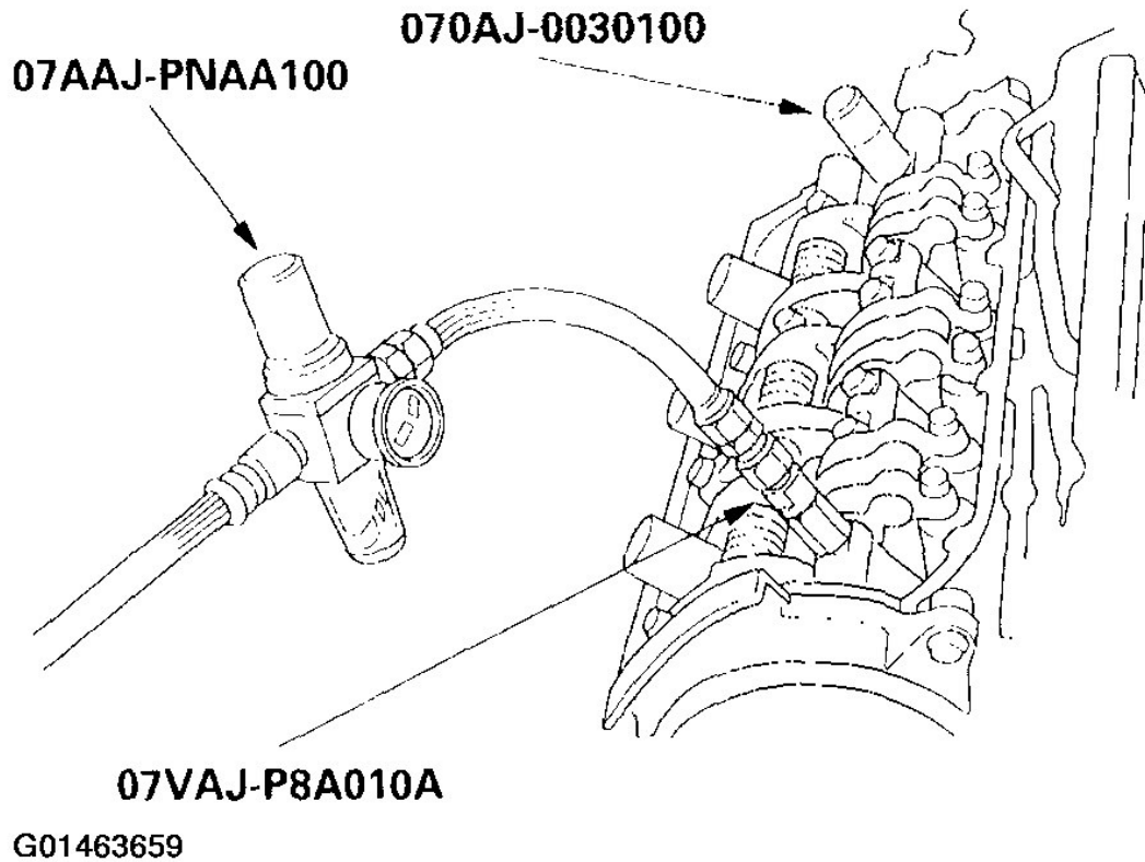
Fig. 72: Connecting The Special Tools (Rear) Courtesy of AMERICAN HONDA MOTOR CO., INC.
