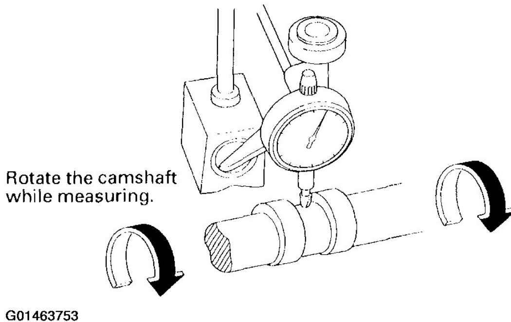
Fig. 166: Measuring Camshaft Total Runout Courtesy of AMERICAN HONDA MOTOR CO., INC.
