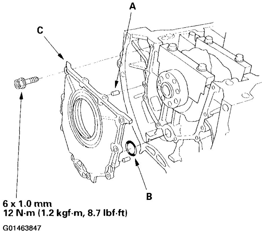
Fig. 260: Installing The Dowel Pins, O-Ring & The Engine Block End Cover On The Cylinder Block
