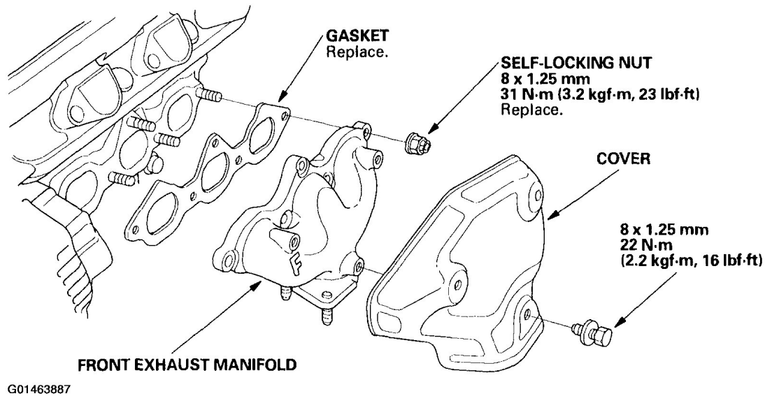
Fig. 281: Removing Front Exhaust Manifold
