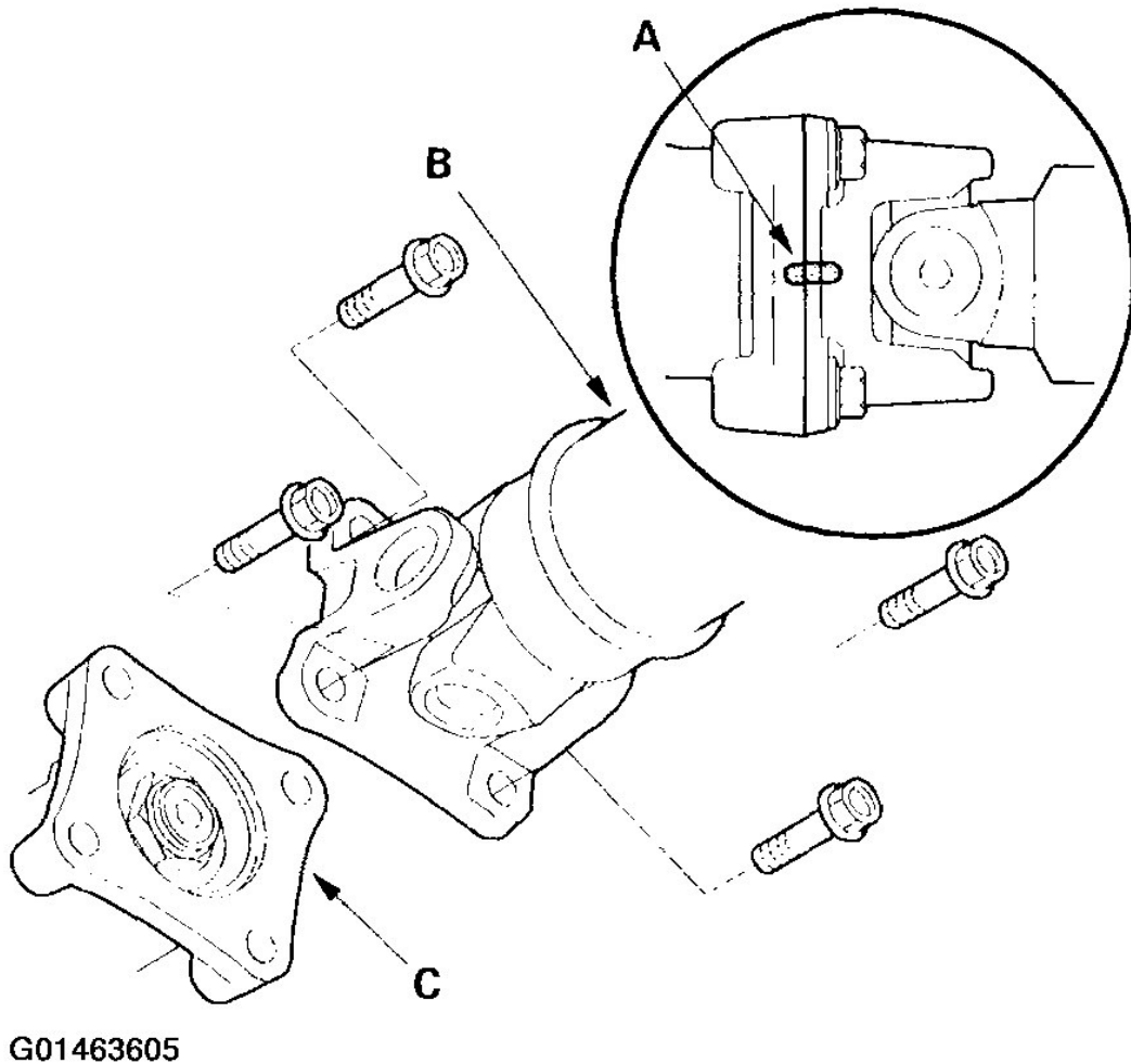
Fig. 18: Making Reference Marks On The Propeller Shaft & Transfer Shaft Flange, & Separating The Propeller Shaft From The Transfer Shaft Flange Courtesy of AMERICAN HONDA MOTOR CO., INC.
