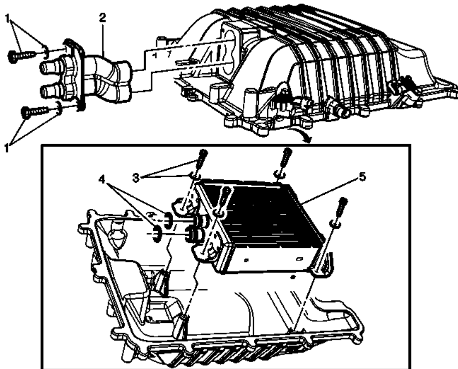
Fig. 132: View Of CMP Actuator Magnet, Bolts, Gasket & Oil Seal Courtesy of GENERAL MOTORS COMPANY
