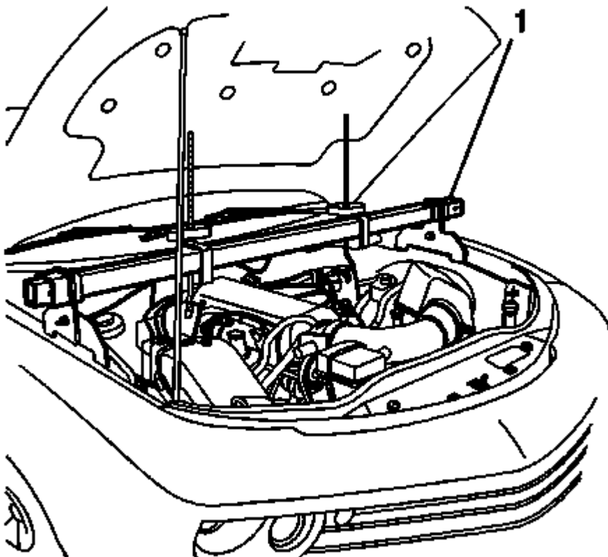
Fig. 106: Identifying Cylinder Head Locating Pins Installation Position Courtesy of GENERAL MOTORS COMPANY
