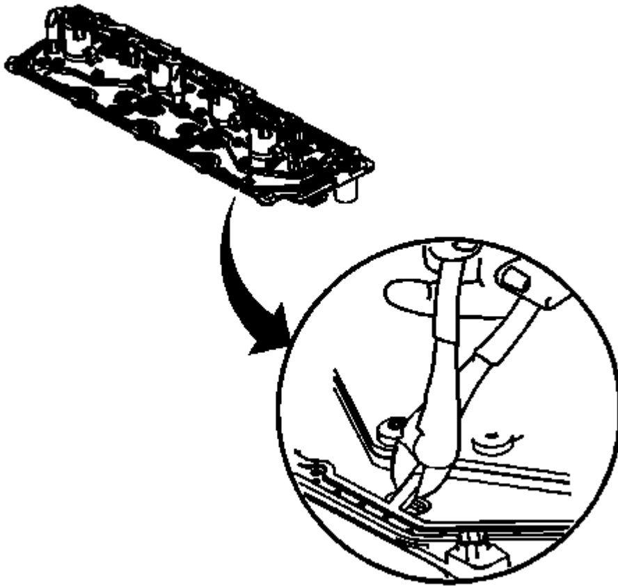
Fig. 149: Identifying Alignment Hole & Locating Pin Courtesy of GENERAL MOTORS COMPANY
