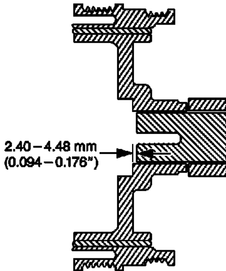
Fig. 216: View Of Tie Strap Through Center Of Actuator Courtesy of GENERAL MOTORS COMPANY
