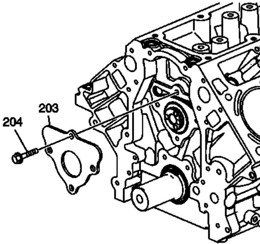
Fig. 15: View Of Drive Belt Tensioner & Bolts Courtesy of GENERAL MOTORS COMPANY
