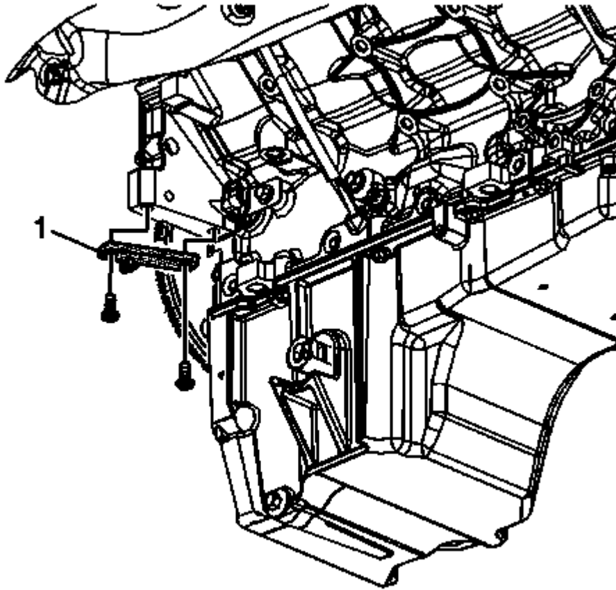
Fig. 240: View Of Engine Flywheel & Bolt Courtesy of GENERAL MOTORS COMPANY
