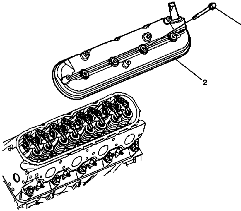
Fig. 155: Tightening CMP Actuator Solenoid Valve Courtesy of GENERAL MOTORS COMPANY
