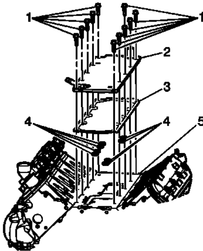
Fig. 144: View Of CMP Actuator Solenoid Valve Courtesy of GENERAL MOTORS COMPANY
