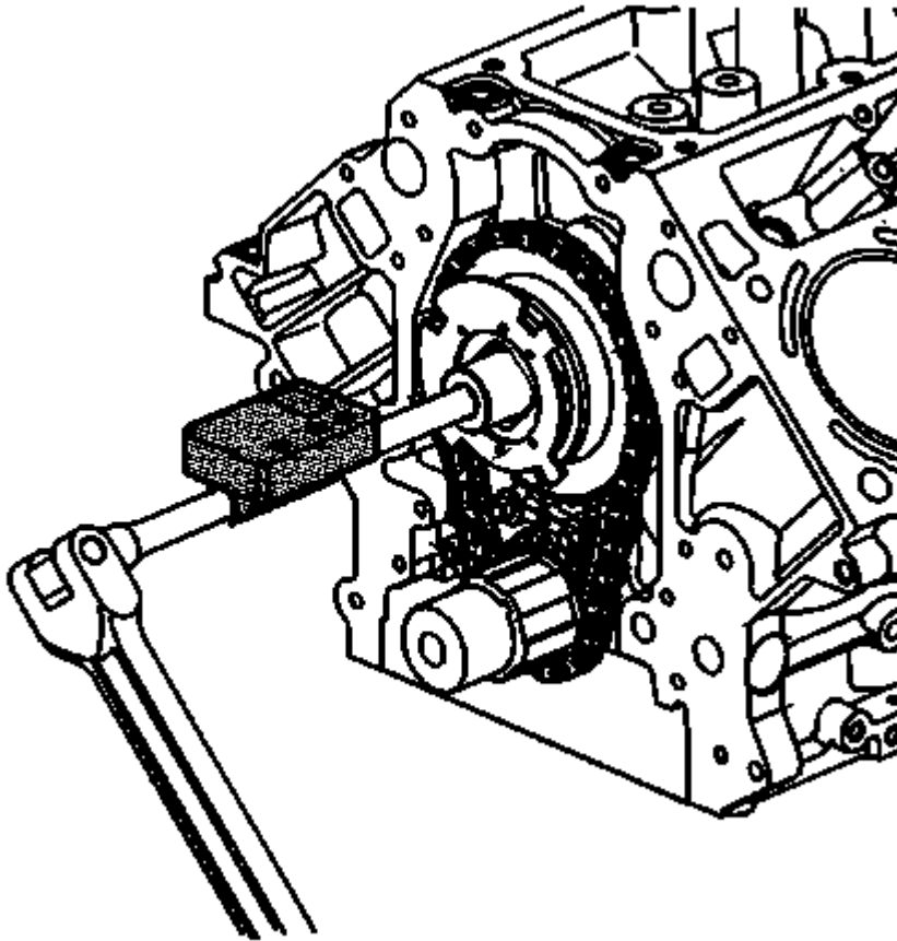
Fig. 38: Oil Filler Tube
