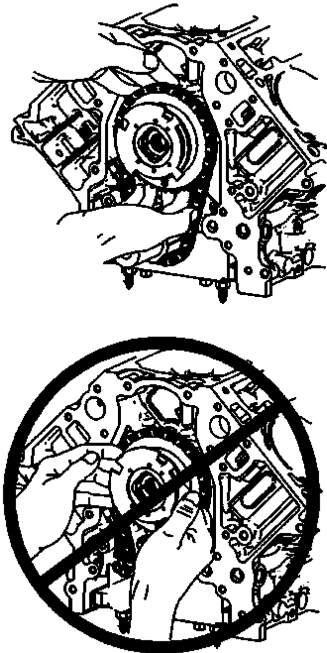
Fig. 242: View Of Spacer & Crankshaft Rear Courtesy of GENERAL MOTORS COMPANY
