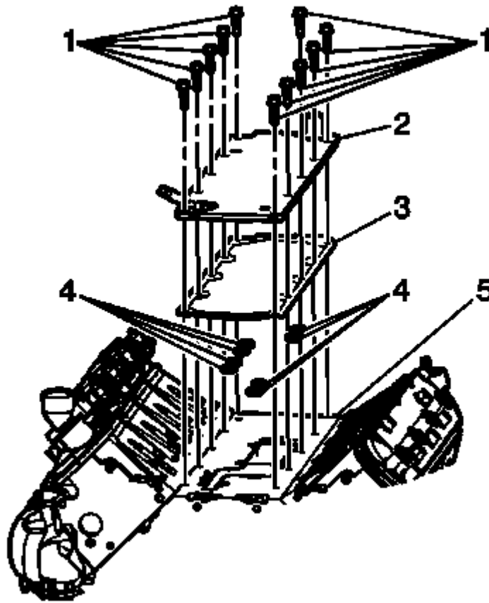
Fig. 145: View Of Proper CMP Actuator Removal Courtesy of GENERAL MOTORS COMPANY
