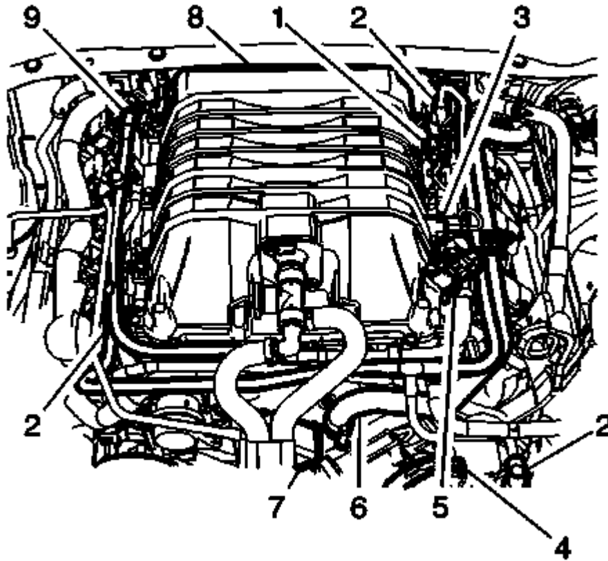
Fig. 131: View Of CMP Actuator Magnet, Bolts, Gasket & Oil Seal Courtesy of GENERAL MOTORS COMPANY
