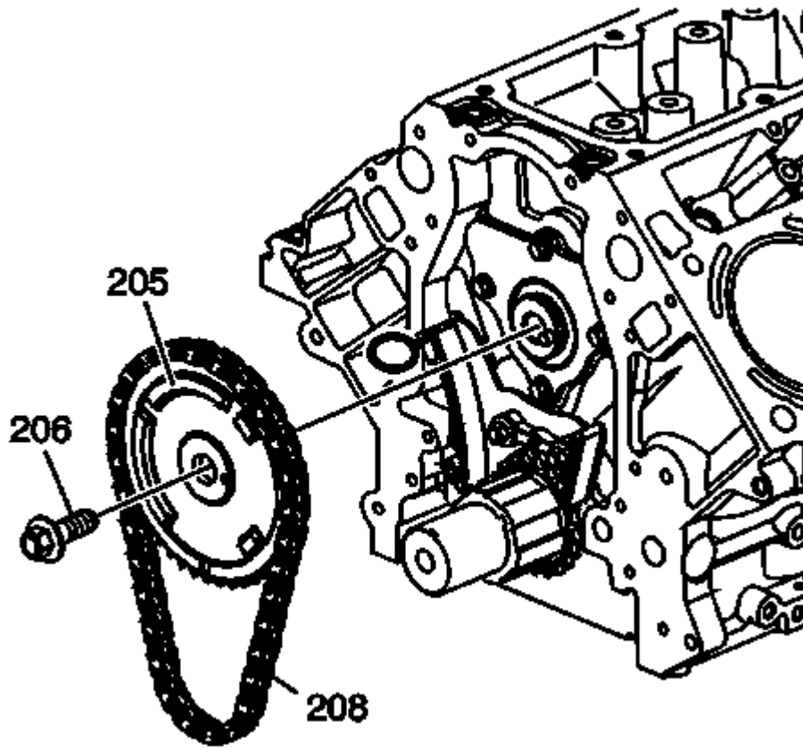
Fig. 21: View Of Square Tab At Rear Of Engine Block Courtesy of GENERAL MOTORS COMPANY
