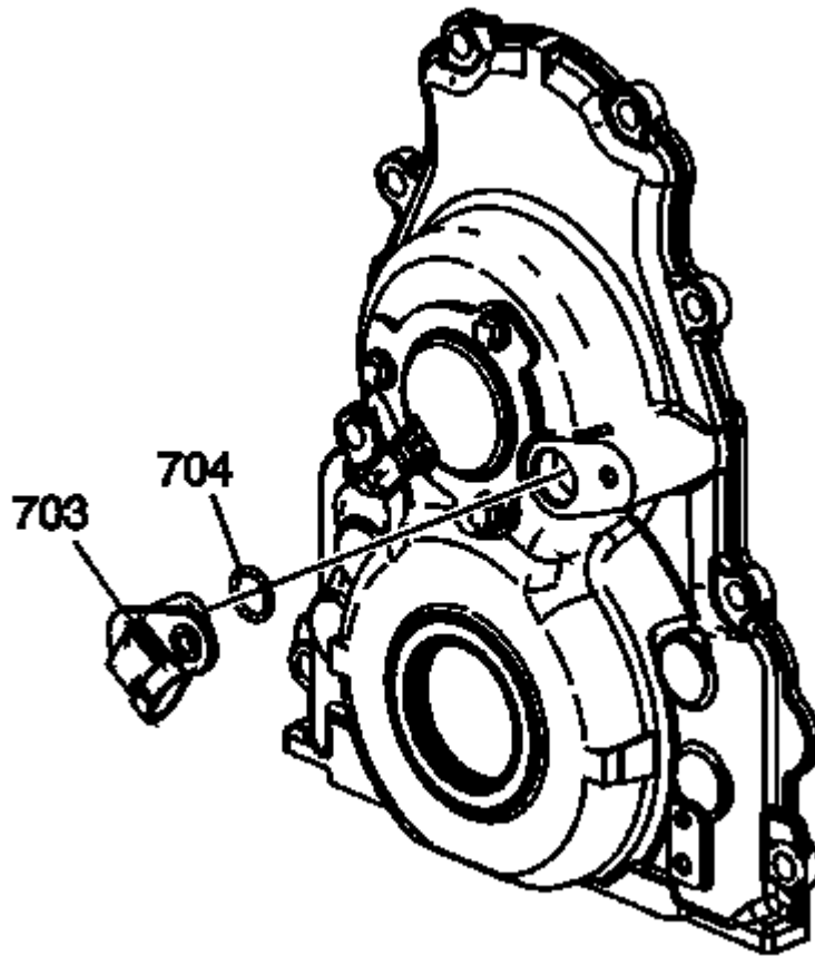
Fig. 227: Identifying Alignment Hole & Locating Pin Courtesy of GENERAL MOTORS COMPANY
