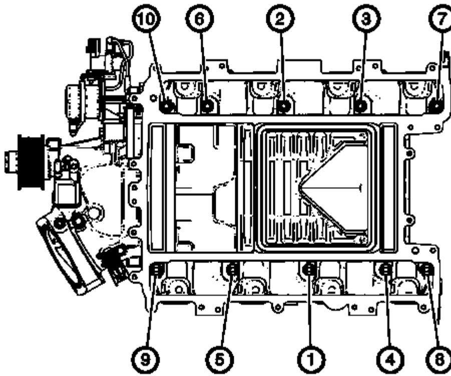
Fig. 129: View Of CMP Sensor Wire Harness & Bolts Courtesy of GENERAL MOTORS COMPANY
