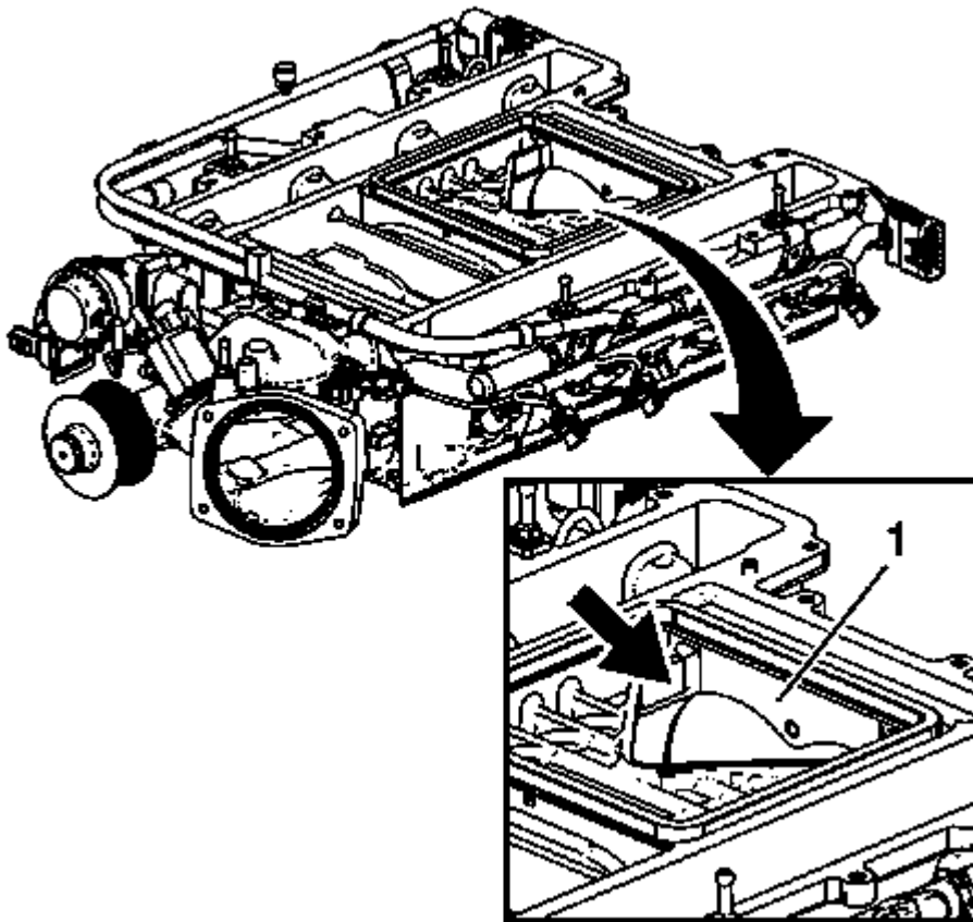
Fig. 121: View Of Outer Edge Of Oil Seal Courtesy of GENERAL MOTORS COMPANY
