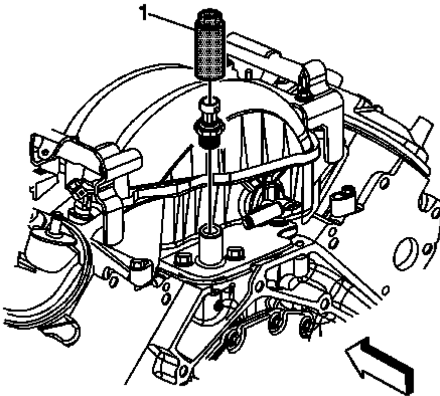
Fig. 272: View Of Oil Pan Drain Plug
