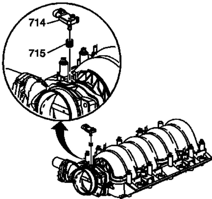
Fig. 134: View Of CMP Sensor Wire Harness & Bolts Courtesy of GENERAL MOTORS COMPANY
