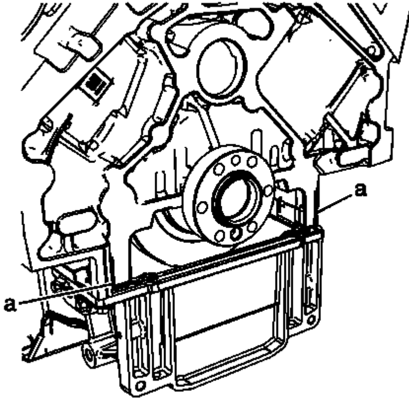
Fig. 258: View Of Engine Mount-To-Engine Mount Bracket Courtesy of GENERAL MOTORS COMPANY
