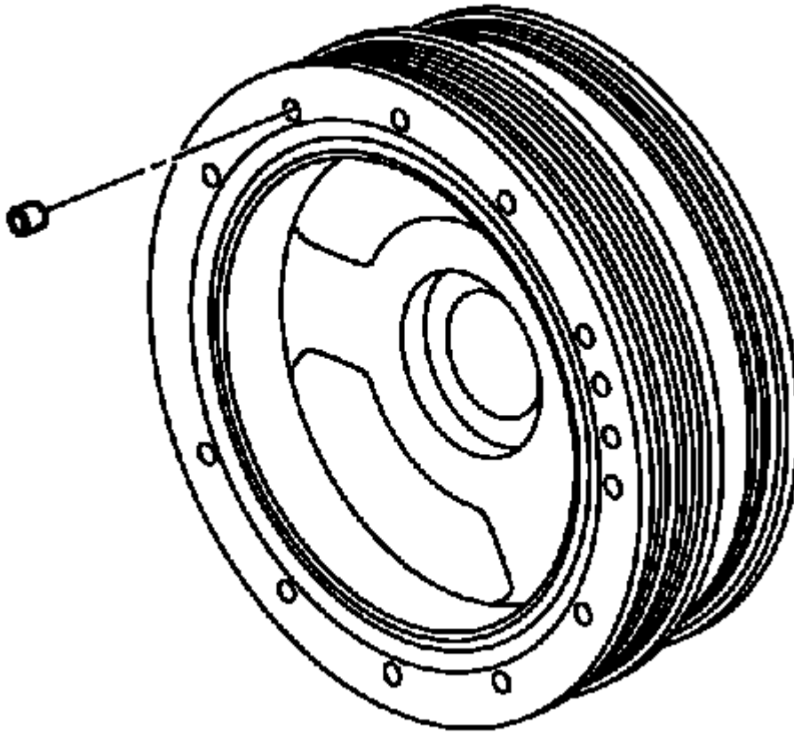
Fig. 210: View Of Crankshaft Oil Deflector Courtesy of GENERAL MOTORS COMPANY
