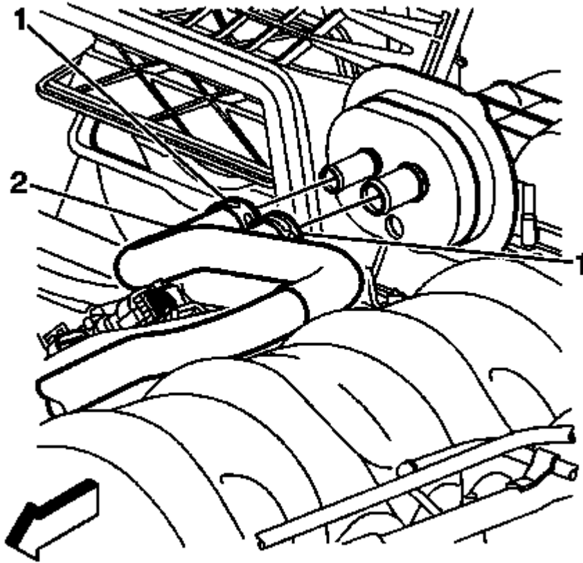
Fig. 51: View Of EVAP Purge Solenoid Vent Tube Courtesy of GENERAL MOTORS COMPANY
