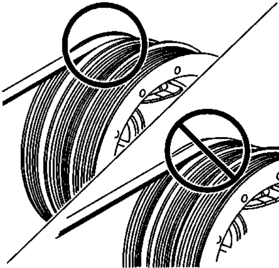
Fig. 92: View Of J 38606 Compressing Valve Spring Courtesy of GENERAL MOTORS COMPANY
