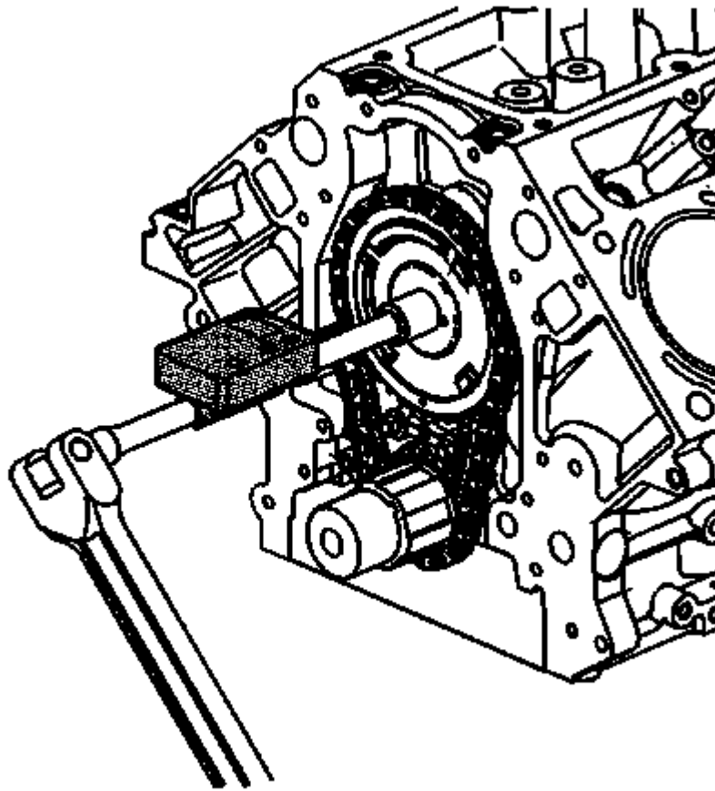
Fig. 24: Engine Mount To Engine Mount Bracket Bolts Courtesy of GENERAL MOTORS COMPANY
