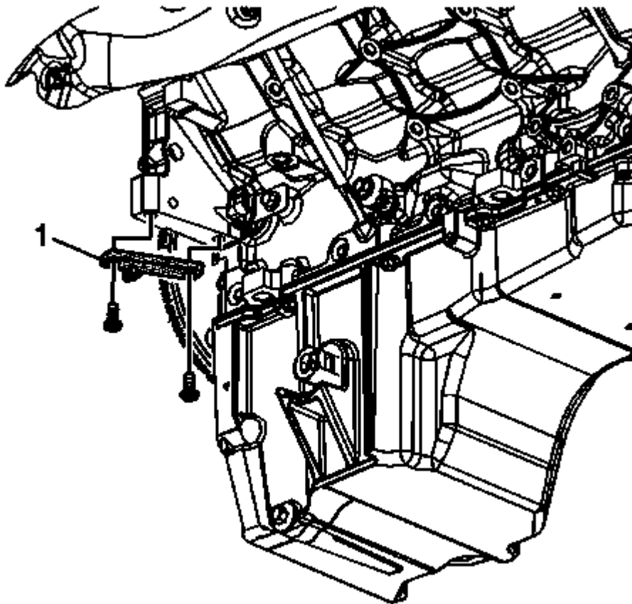
Fig. 39: View Of MAP Sensor & Knock Sensor Electrical Connectors Courtesy of GENERAL MOTORS COMPANY
