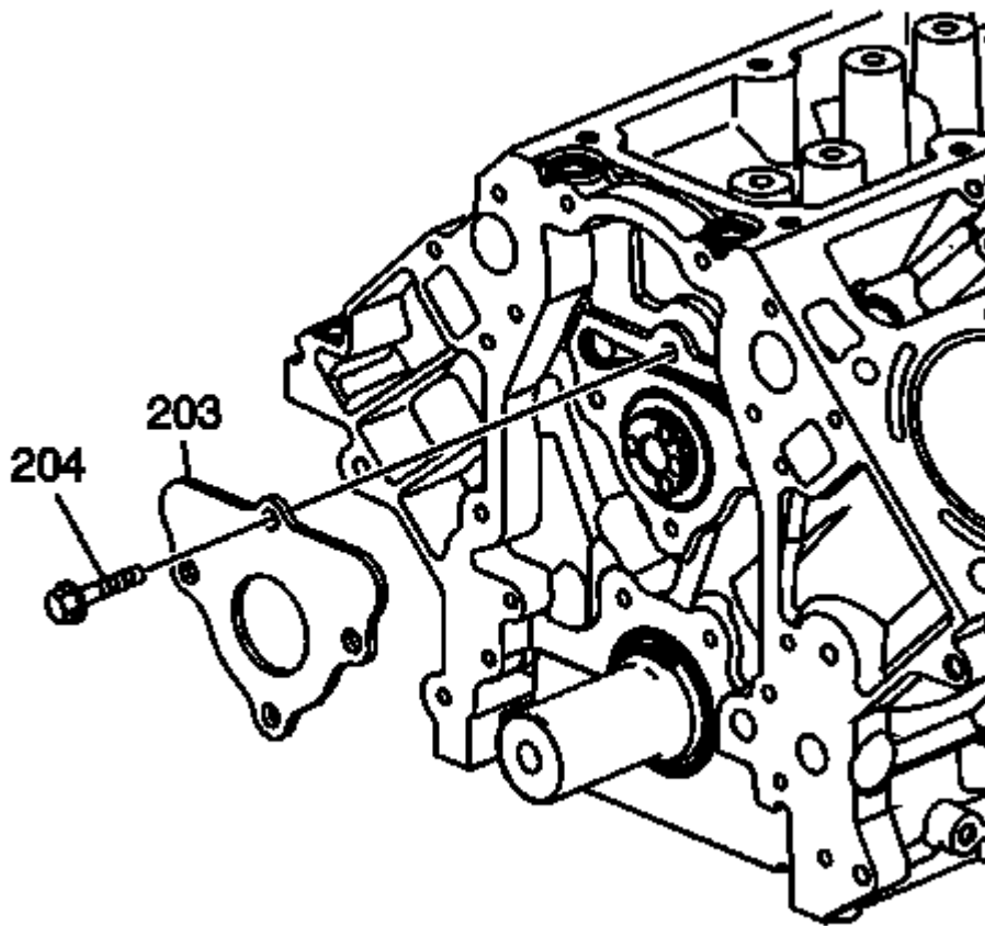
Fig. 29: Engine Mount To Engine Mount Bracket Bolts Courtesy of GENERAL MOTORS COMPANY
