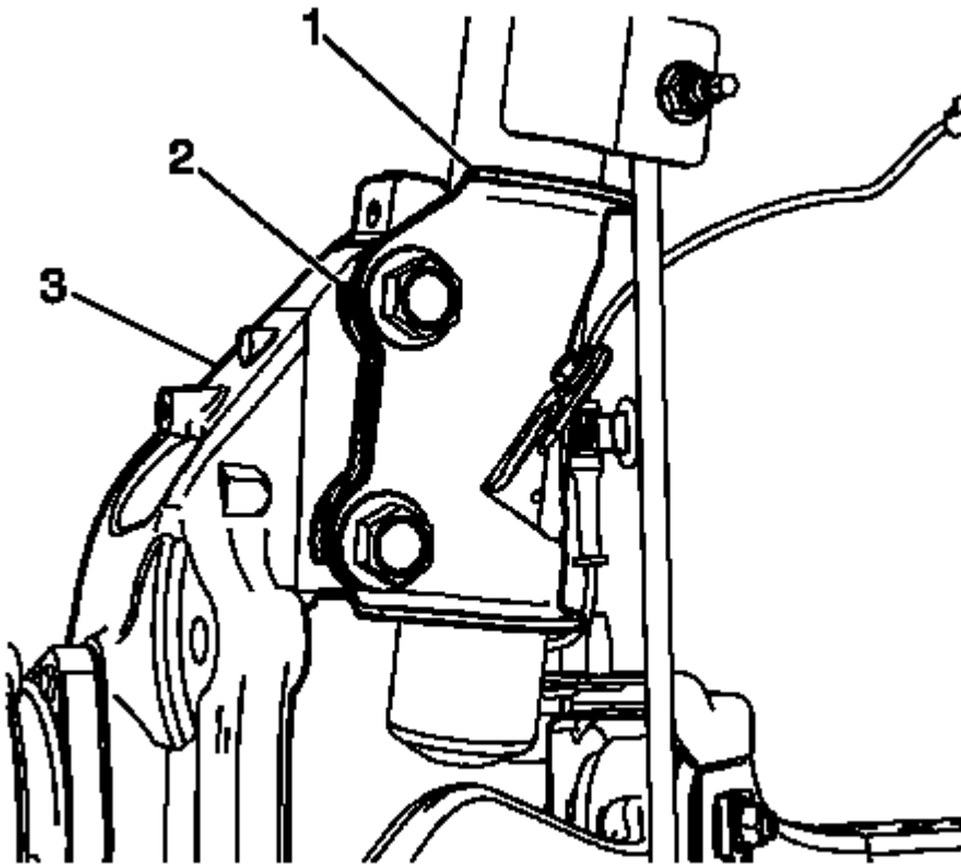
Fig. 56: Oil Pressure Sensor And Washer Courtesy of GENERAL MOTORS COMPANY
