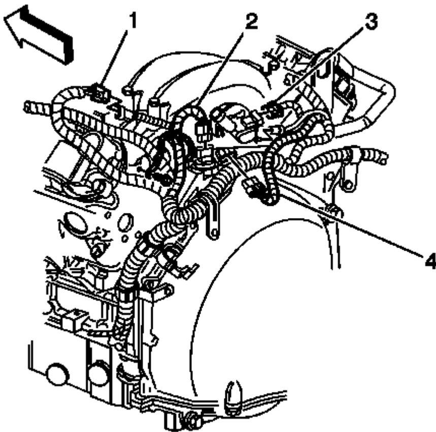
Fig. 273: View Of Engine Oil Filter
