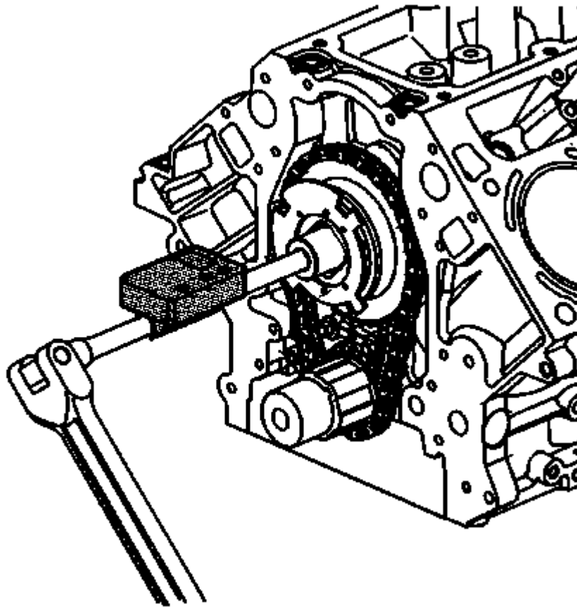
Fig. 252: View Of Lower 6 Bell Housing To Engine Studs & Bolts Courtesy of GENERAL MOTORS COMPANY
