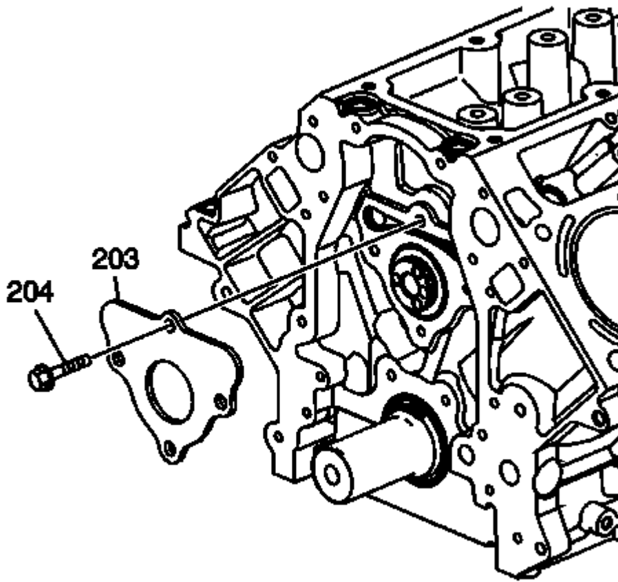
Fig. 18: Engine Mount To Engine Mounting Bolts Courtesy of GENERAL MOTORS COMPANY
