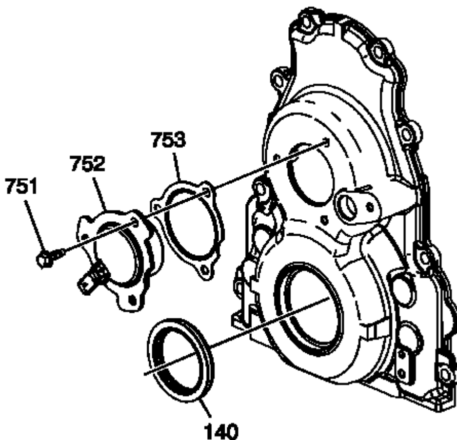
Fig. 228: View Of CMP Actuator & Timing Chain Courtesy of GENERAL MOTORS COMPANY
