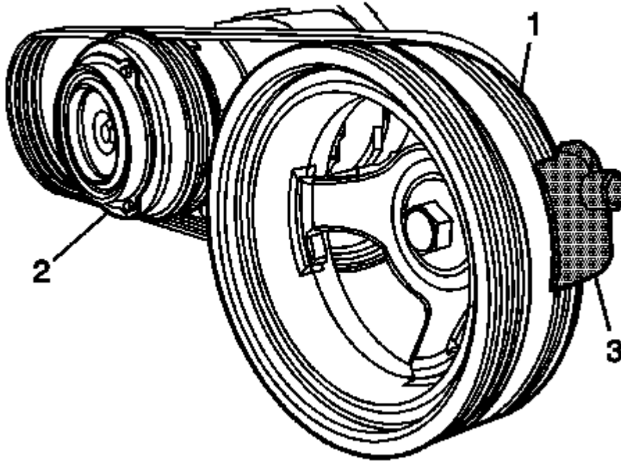
Fig. 85: View of Crankshaft/Camshaft In Position For Number 1 Piston At TDC Courtesy of GENERAL MOTORS COMPANY
