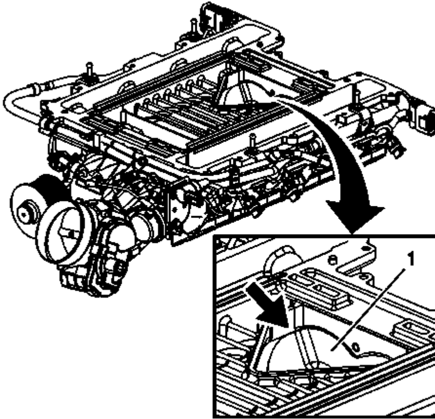
Fig. 126: View Of Electrical Connector, Cable Channel Bolt & Pin Courtesy of GENERAL MOTORS COMPANY
