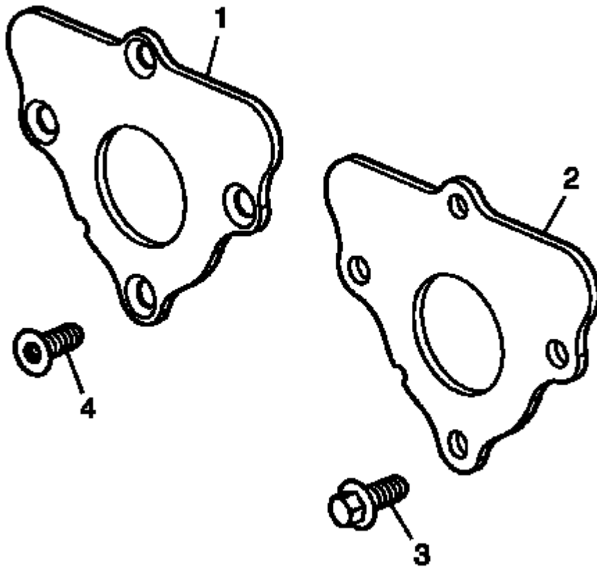
Fig. 19: Engine Mount To Engine Mount Bracket Bolts Courtesy of GENERAL MOTORS COMPANY
