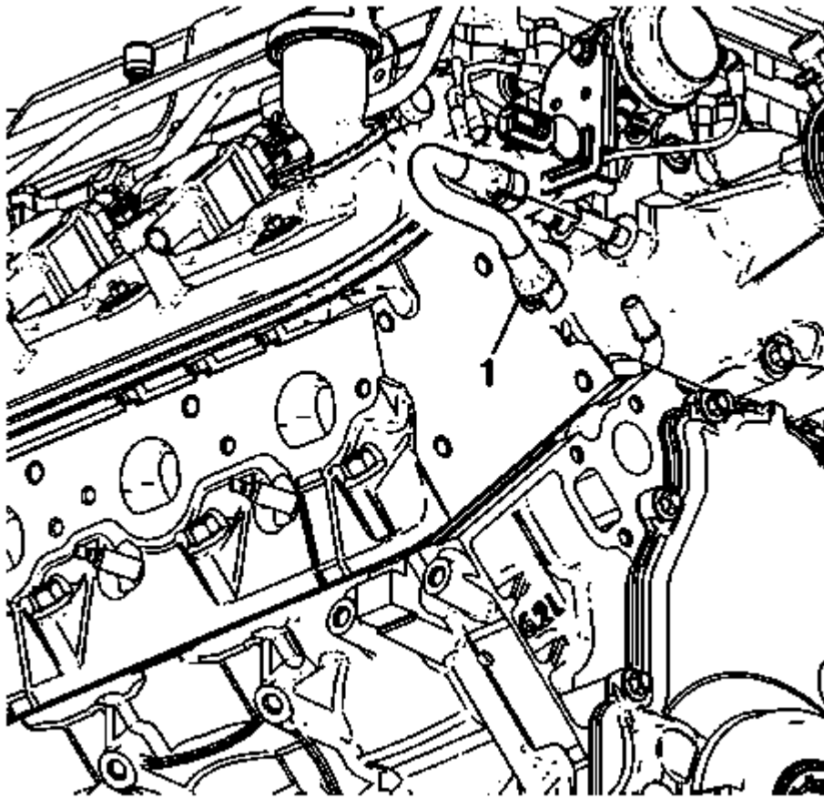
Fig. 130: View Of CMP Sensor & O-Ring Courtesy of GENERAL MOTORS COMPANY
