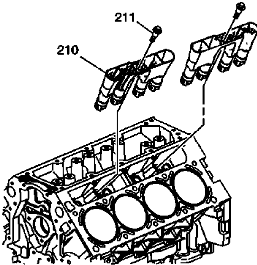
Fig. 197: View Of Crossbar Bolts & Bar (2WD) Courtesy of GENERAL MOTORS COMPANY
