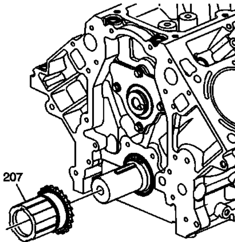
Fig. 4: Removing Belt
