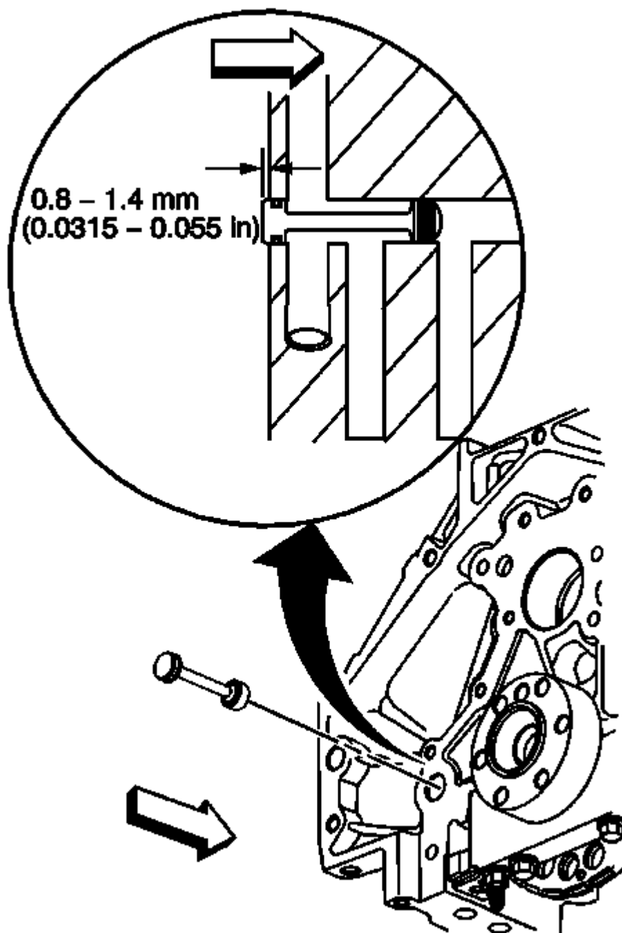
Fig. 259: Identifying Six Studs & One Bolt Securing Transmission To Engine Courtesy of GENERAL MOTORS COMPANY
