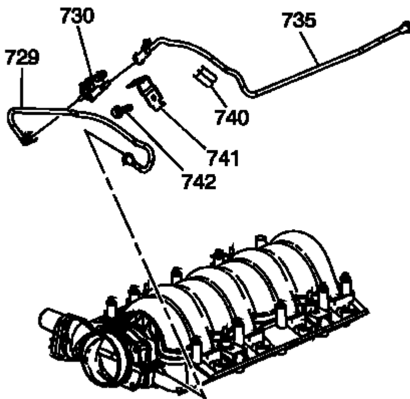
Fig. 142: Tightening CMP Actuator Solenoid Valve Courtesy of GENERAL MOTORS COMPANY
