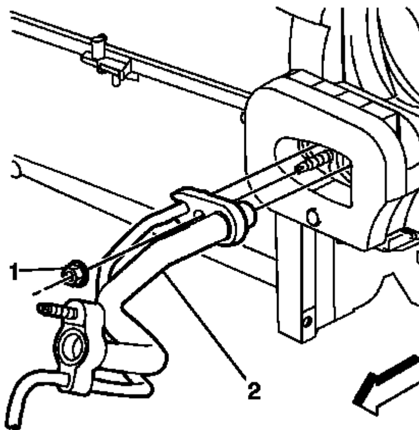
Fig. 68: View Of Main Ignition Coil Wire Harness Connector & Clips Courtesy of GENERAL MOTORS COMPANY
