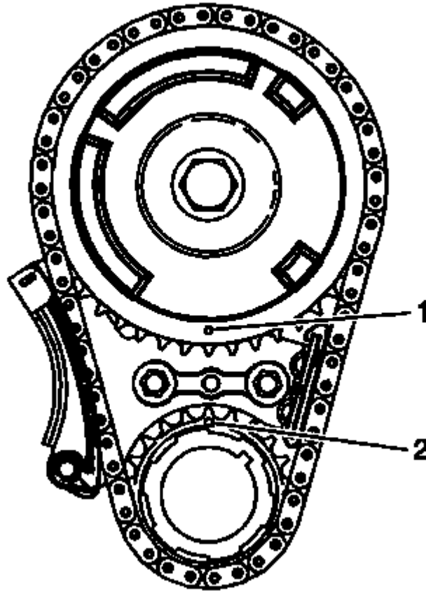
Fig. 9: Rotating Balancer Clockwise Courtesy of GENERAL MOTORS COMPANY
