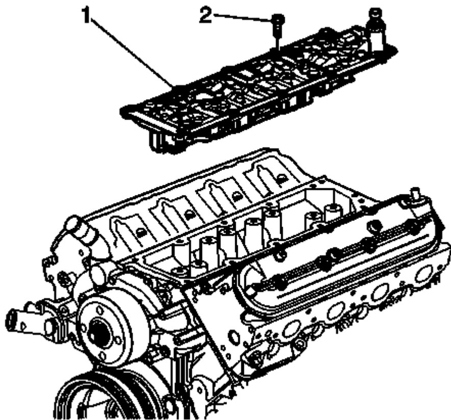
Fig. 147: View Of Tie Strap Through Center Of Actuator Courtesy of GENERAL MOTORS COMPANY
