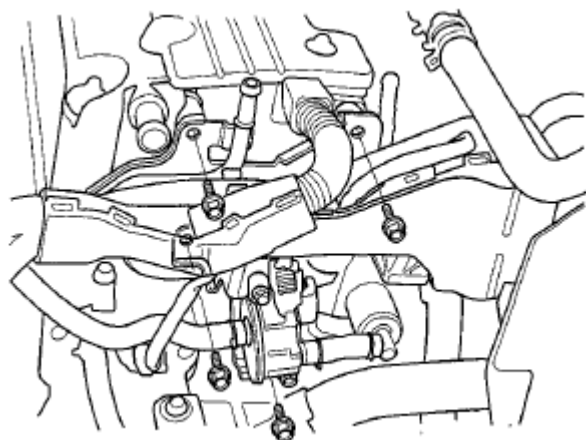
Fig. 78: Identifying EVAP Canister Purge Valve Bracket
