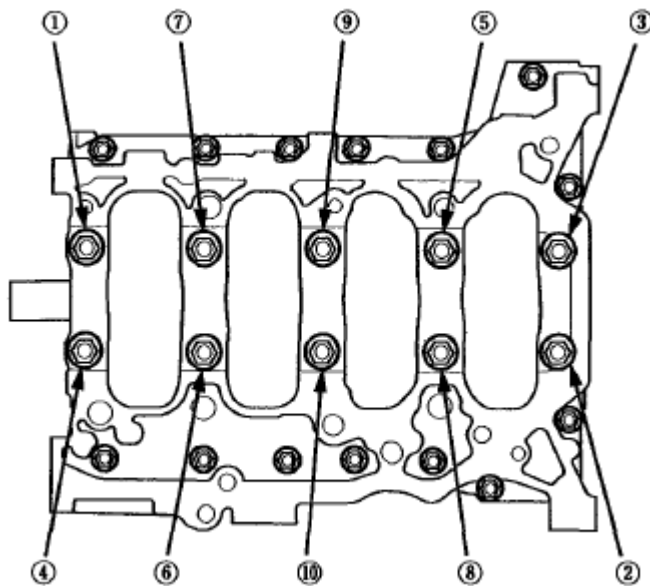
Fig. 27: Identifying Bearing Cap Bolts Loosening Sequence
