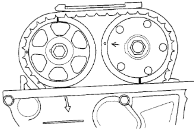
Fig. 21: Identifying Valve Clearance With Camshaft Pulley Courtesy of AMERICAN HONDA MOTOR CO., INC.
