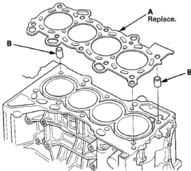
Fig. 130: Identifying Cylinder Head Gasket And Dowel Pins Courtesy of AMERICAN HONDA MOTOR CO., INC.
