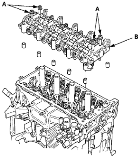
Fig. 126: Identifying Bolts, Rocker Arm Assembly And Cylinder Head Courtesy of AMERICAN HONDA MOTOR CO., INC.
