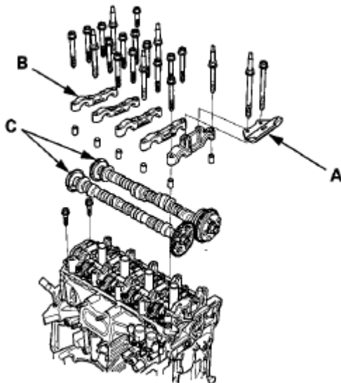
Fig. 94: Identifying Cam Chain Guide, Camshaft Holders And Camshafts
