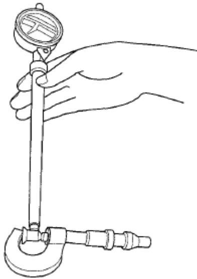
Fig. 43: Measuring Zero Dial Indicator To Piston Pin Diameter Courtesy of AMERICAN HONDA MOTOR CO., INC.
