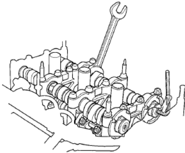
Fig. 84: Holding Camshaft With Wrench To Loosen Bolt Courtesy of AMERICAN HONDA MOTOR CO., INC.
