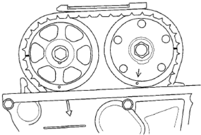
Fig. 20: Identifying Valve Clearance With Camshaft Pulley Courtesy of AMERICAN HONDA MOTOR CO., INC.
