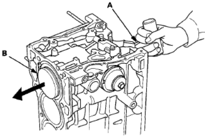
Fig. 31: Installing Piston/Connecting Rod Assembly With Tools Courtesy of AMERICAN HONDA MOTOR CO., INC.
