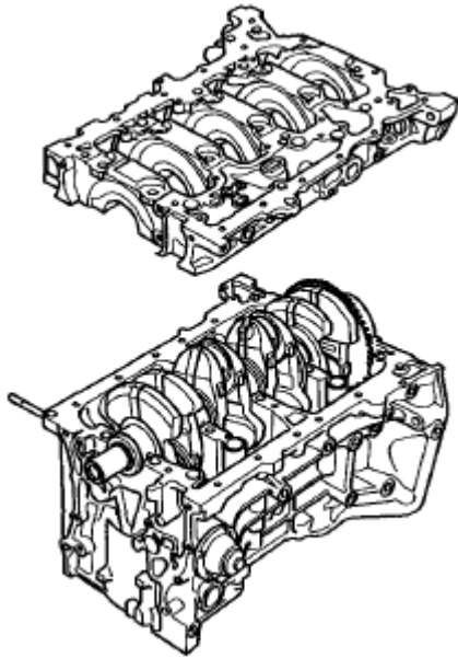
Fig. 28: Identifying Block And Bearings
