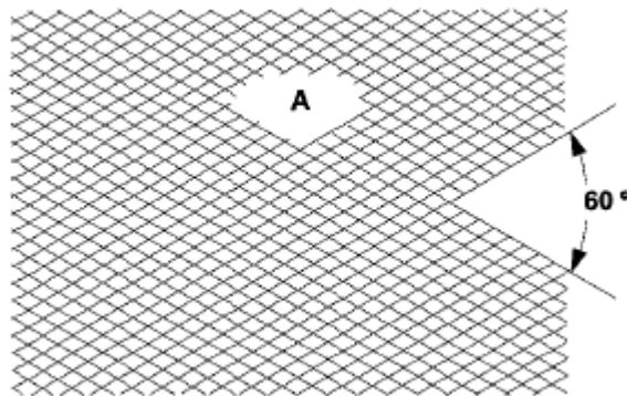
Fig. 38: Identifying Cylinder Bores In Cross Hatch Pattern Courtesy of AMERICAN HONDA MOTOR CO., INC.
