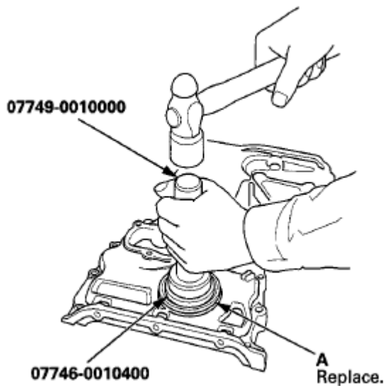
Fig. 61: Installing Chain Case Oil Seal Using SST Courtesy of AMERICAN HONDA MOTOR CO., INC.
