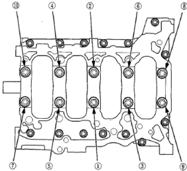
Fig. 64: Identifying Bearing Cap Bolts Tightening Sequence Courtesy of AMERICAN HONDA MOTOR CO., INC.
