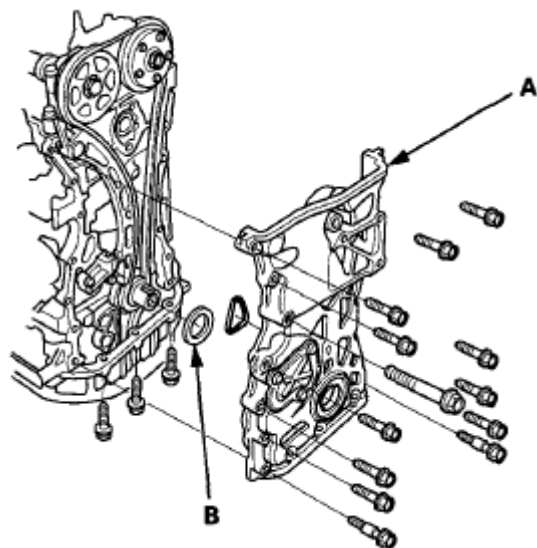
Fig. 30: Identifying Cam Chain Case And Spacer Courtesy of AMERICAN HONDA MOTOR CO., INC.
