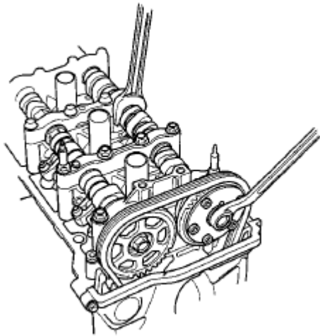
Fig. 86: Identifying VTC Actuator Mounting Bolt And Exhaust Camshaft Sprocket Mounting Bolt Courtesy of AMERICAN HONDA MOTOR CO., INC.
