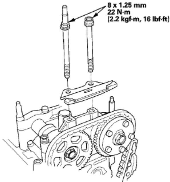
Fig. 42: Identifying Cam Chain Guide With Torque Specifications Courtesy of AMERICAN HONDA MOTOR CO., INC.
