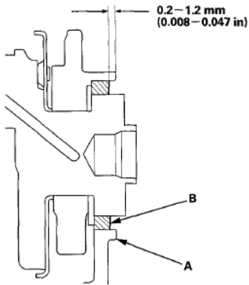
Fig. 68: Identifying Engine Block And Crankshaft Oil Seal Courtesy of AMERICAN HONDA MOTOR CO., INC.
