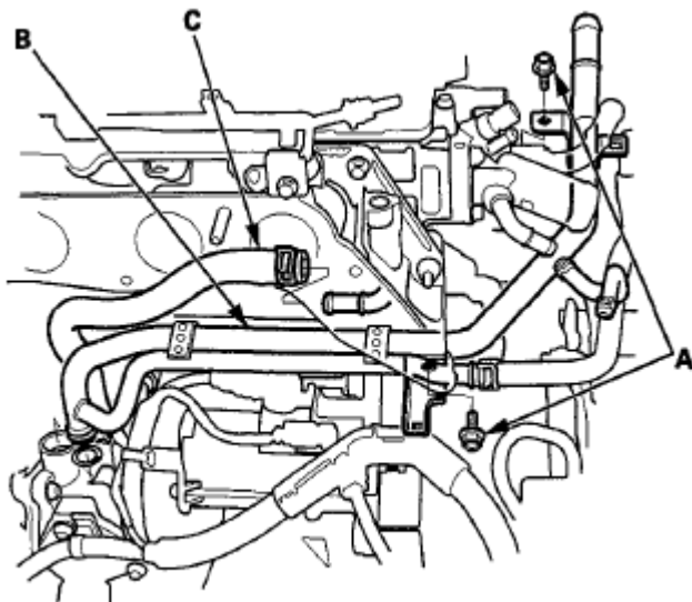
Fig. 80: Identifying Pipe Mounting Bolts, Connecting Pipe And Connecting Pipe Courtesy of AMERICAN HONDA MOTOR CO., INC.
