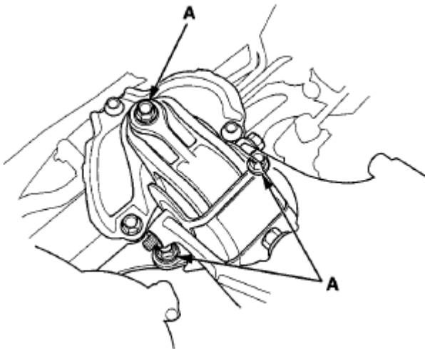
Fig. 18: Identifying Rear Engine Mount Mounting Bolts In A/T Model Courtesy of AMERICAN HONDA MOTOR CO., INC.
