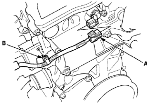
Fig. 52: Identifying VTC Oil Control Solenoid Valve Connector And Harness Clamp Courtesy of AMERICAN HONDA MOTOR CO., INC.
