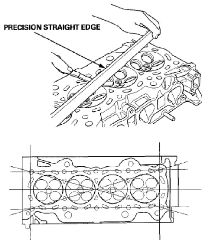
Fig. 91: Measuring Cylinder Head Warpage And Edges Courtesy of AMERICAN HONDA MOTOR CO., INC.
