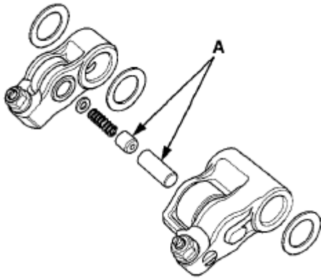
Fig. 101: Identifying Rocker Arm Pistons (Exhaust Side) Courtesy of AMERICAN HONDA MOTOR CO., INC.
