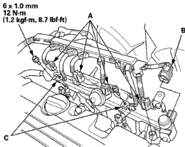
Fig. 138: Identifying Fuel Injector Connectors, Engine Mount Control Solenoid Valve Connector And Ground Cables With Torque Specifications Courtesy of AMERICAN HONDA MOTOR CO., INC.
