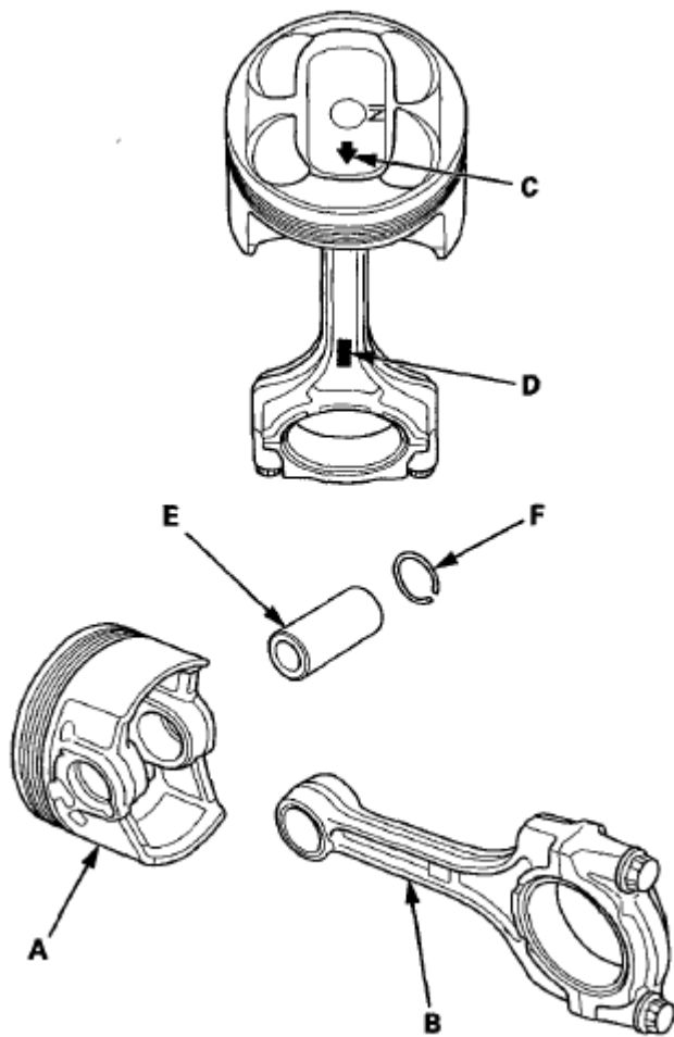
Fig. 48: Identifying Piston, Connecting Rod And Embossed Mark Courtesy of AMERICAN HONDA MOTOR CO., INC.
