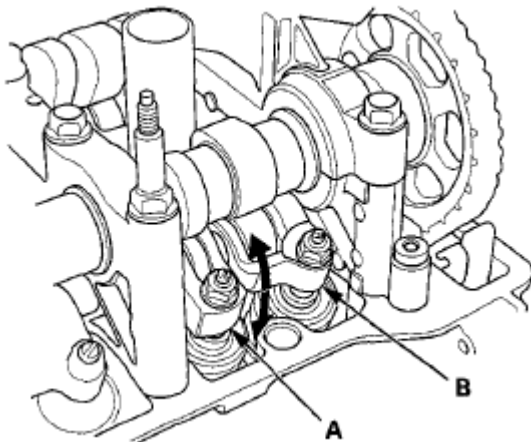
Fig. 7: Identifying Exhaust Secondary Rocker Arm And Primary Rocker Arm Courtesy of AMERICAN HONDA MOTOR CO., INC.
