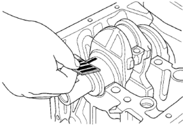
Fig. 7: Measuring Widest Part Of Main Bearing Courtesy of AMERICAN HONDA MOTOR CO., INC.
