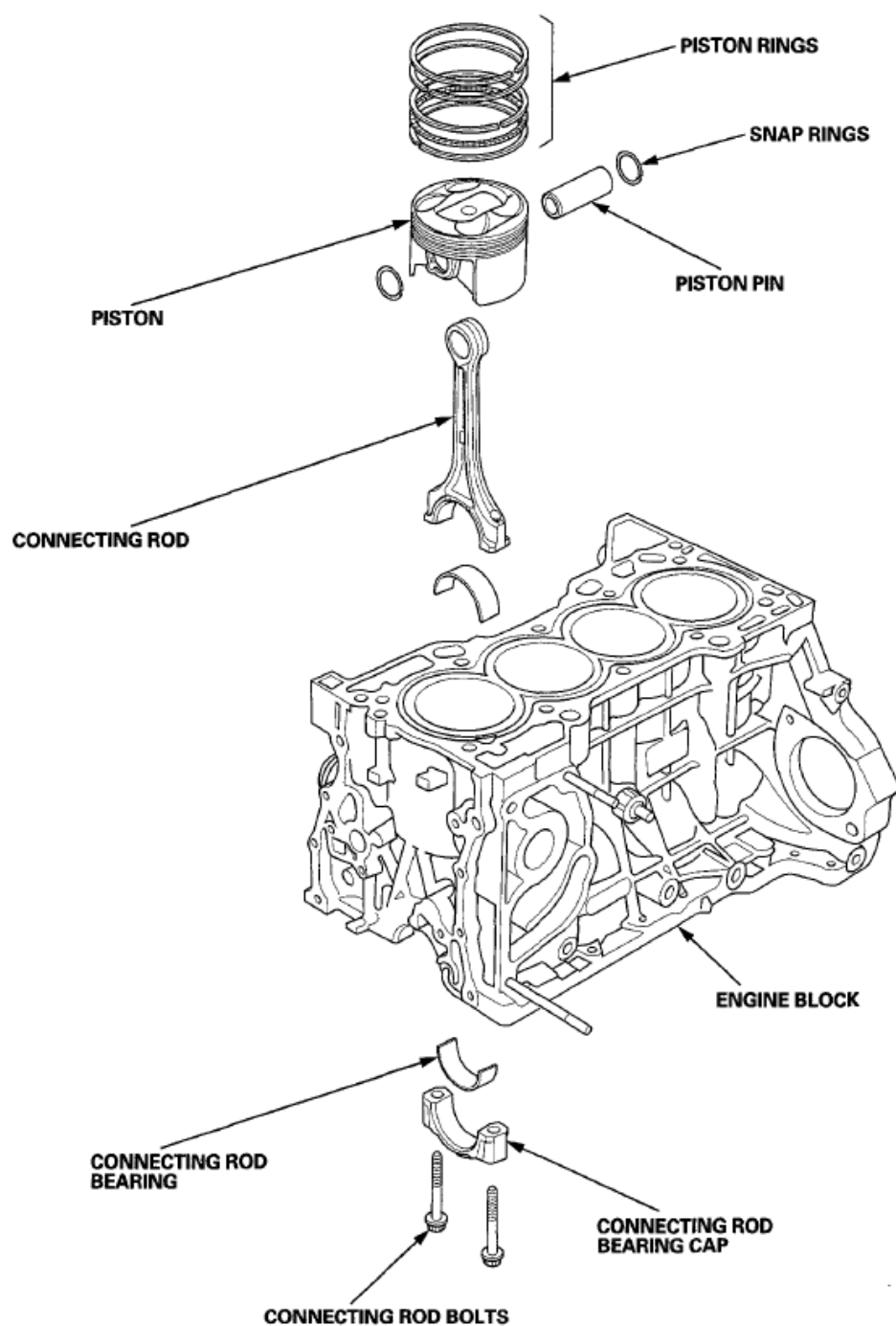
Fig. 3: Identifying Engine Block Component Location (2 Of 2) Courtesy of AMERICAN HONDA MOTOR CO., INC.
