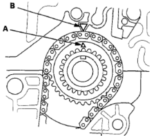
Fig. 36: Identifying TDC Mark And Crankshaft Sprocket With Pointer Courtesy of AMERICAN HONDA MOTOR CO., INC.
