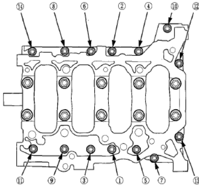
Fig. 66: Identifying Bolts And Tightening Sequence Courtesy of AMERICAN HONDA MOTOR CO., INC.
