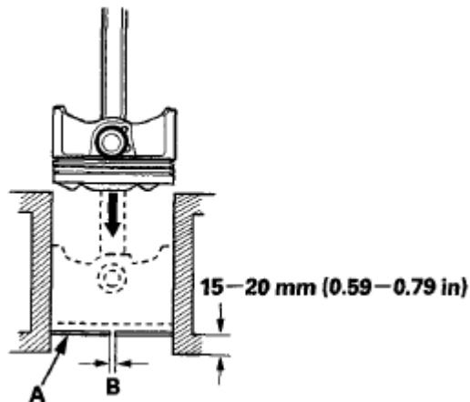
Fig. 50: Identifying Ring And Piston Ring End-Gap In Cylinder Bore
