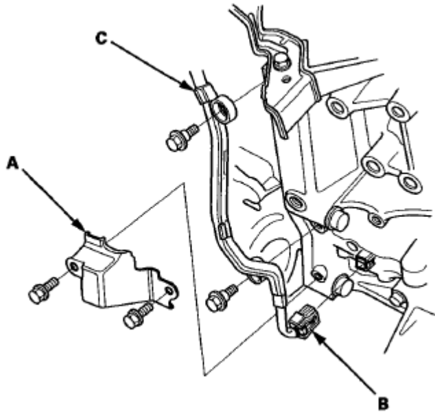
Fig. 24: Identifying CKP Sensor Cover, CKP Sensor Connector And Harness Holder Courtesy of AMERICAN HONDA MOTOR CO., INC.
