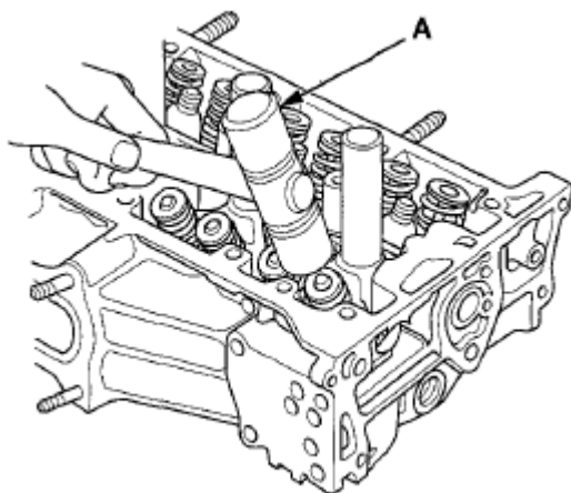
Fig. 124: Identifying Plastic Mallet And Valve Stem Courtesy of AMERICAN HONDA MOTOR CO., INC.
