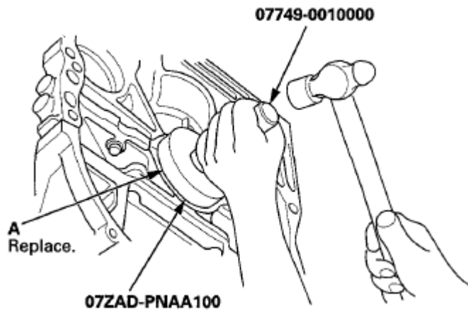
Fig. 81: Installing Crankshaft Oil Seal
