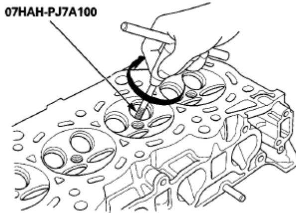
Fig. 117: Rotating Valve Guide Reamer Clockwise Courtesy of AMERICAN HONDA MOTOR CO., INC.
