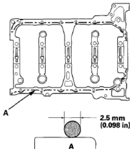
Fig. 63: Identifying Diameter Bead Of Liquid Gasket Along Broken Line
