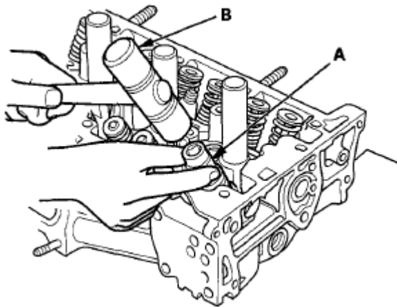
Fig. 107: Identifying Socket And Plastic Mallet
