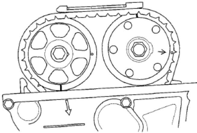
Fig. 19: Identifying Valve Clearance With Camshaft Pulley Courtesy of AMERICAN HONDA MOTOR CO., INC.
