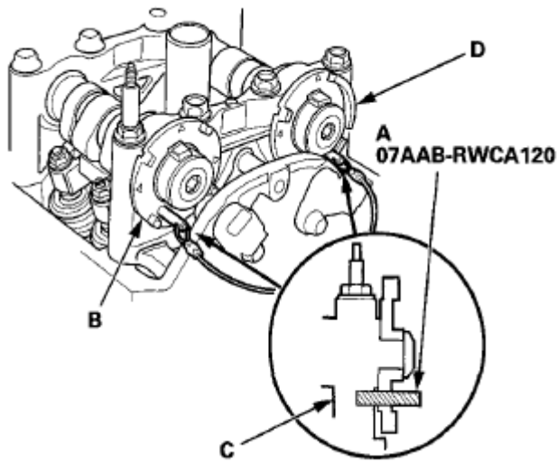
Fig. 38: Identifying Camshaft Lock Pin And CMP Pulse Plate Courtesy of AMERICAN HONDA MOTOR CO., INC.
