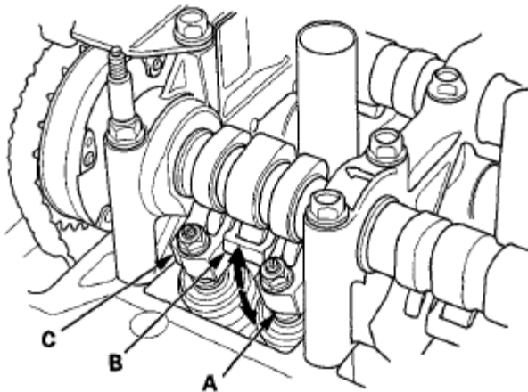
Fig. 9: Identifying Intake Secondary Rocker Arm Intake Mid Rocker Arm And Intake Primary Rocker Arm
