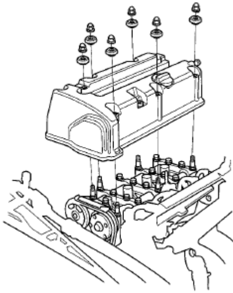
Fig. 68: Identifying Cylinder Head Cover
