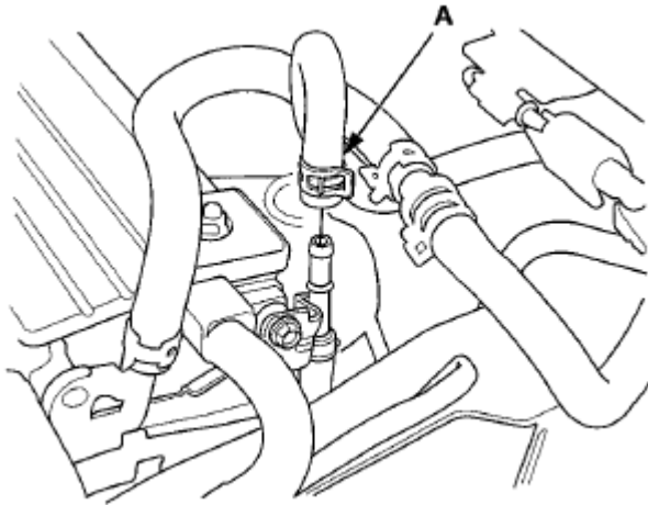
Fig. 75: Identifying EVAP Canister Hose
