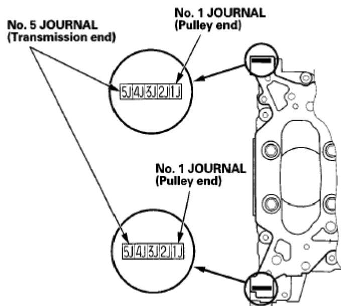
Fig. 8: Identifying Black Bore Code Location Courtesy of AMERICAN HONDA MOTOR CO., INC.
