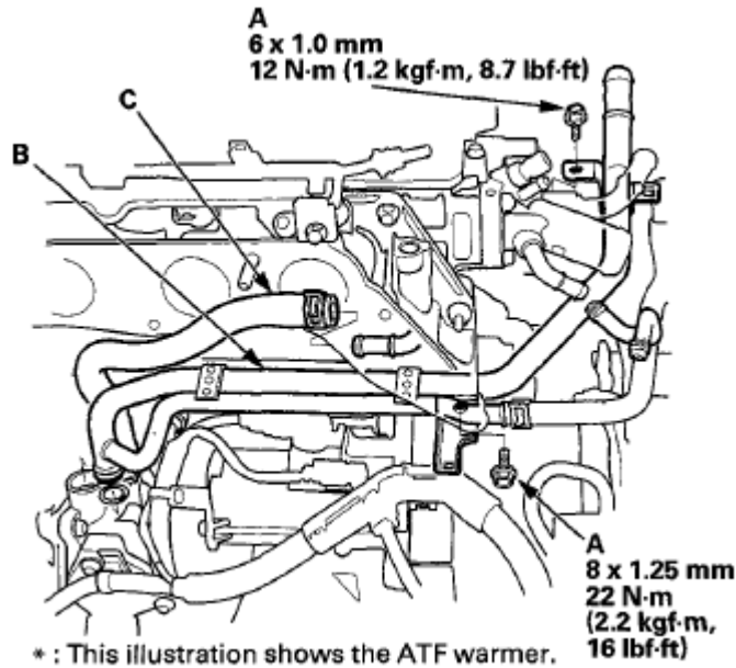
Fig. 135: Identifying Pipe Mounting Bolts And Water Bypass Hose With Torque Specifications Courtesy of AMERICAN HONDA MOTOR CO., INC.
