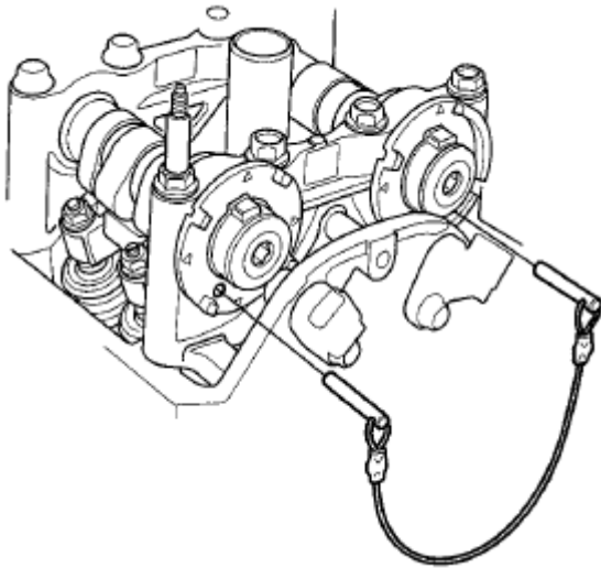
Fig. 46: Identifying Camshaft Lock Pin
