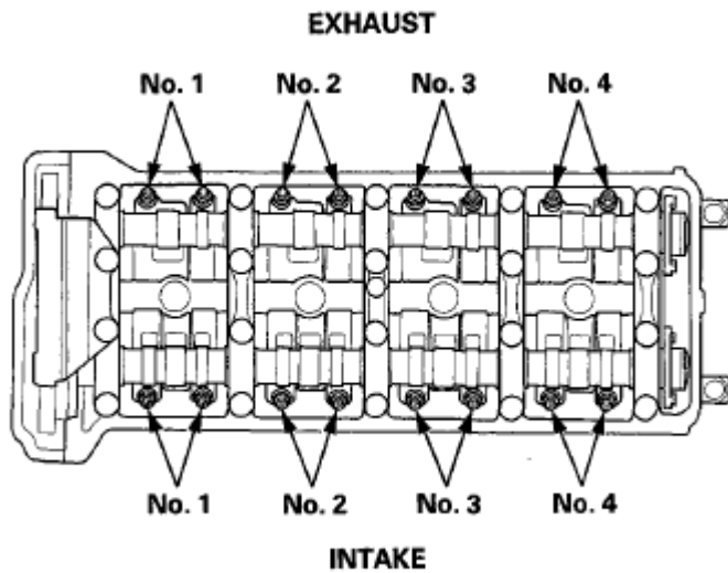
Fig. 16: Identifying Feeler Gauge Valve Sequence Courtesy of AMERICAN HONDA MOTOR CO., INC.
