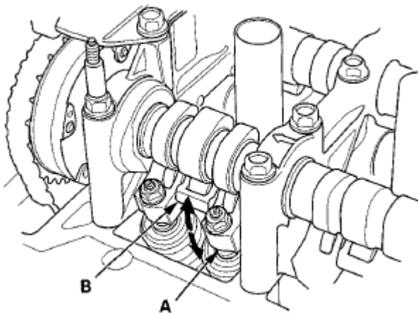
Fig. 6: Identifying Secondary Rocker Arm And Intake Mid Rocker Arm Courtesy of AMERICAN HONDA MOTOR CO., INC.
