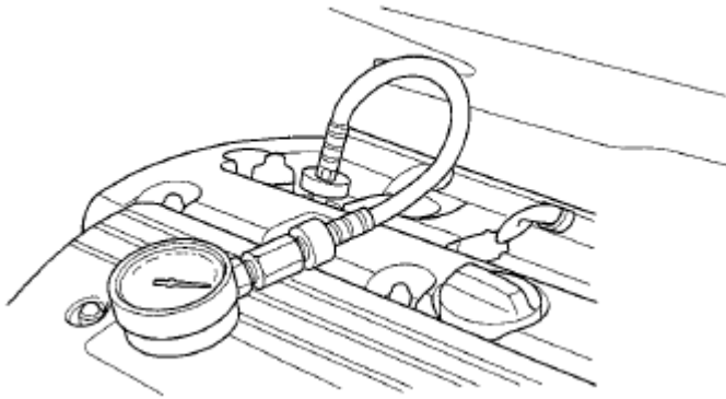
Fig. 5: Identifying Compression Gauge Connection With Spark Plug Hole Courtesy of AMERICAN HONDA MOTOR CO., INC.
