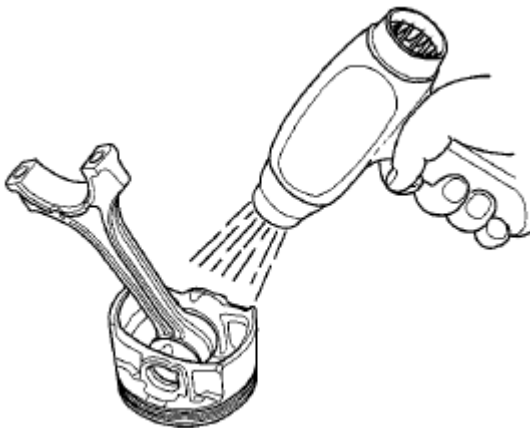
Fig. 41: Heating The Piston And Connecting Rod Assembly Courtesy of AMERICAN HONDA MOTOR CO., INC.
