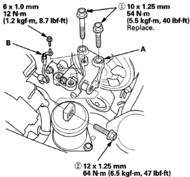
Fig. 51: Identifying Engine Mount Bracket And Ground Cable With Torque Specifications
