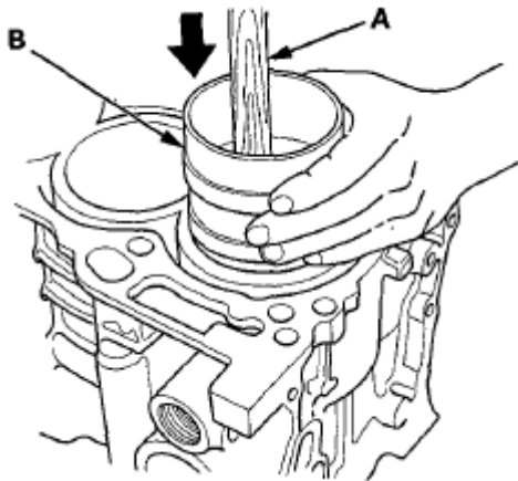
Fig. 55: Installing Ring Compressor In Cylinder Bore With Tool Courtesy of AMERICAN HONDA MOTOR CO., INC.
