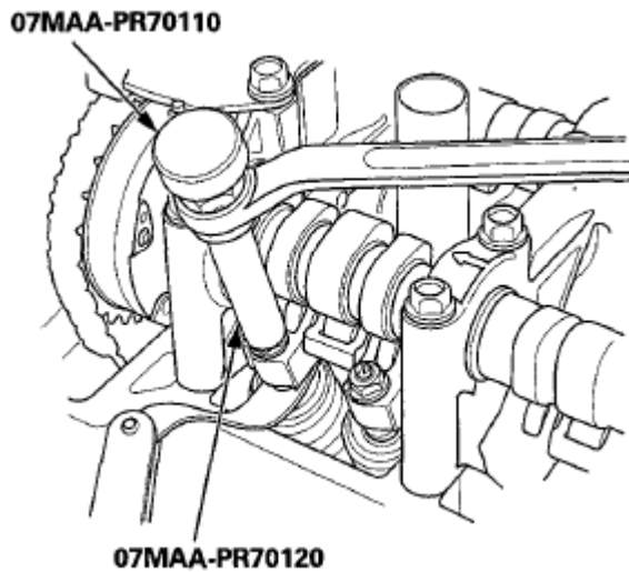
Fig. 18: Identifying Feeler Gauge With Adjusting Screw Courtesy of AMERICAN HONDA MOTOR CO., INC.
