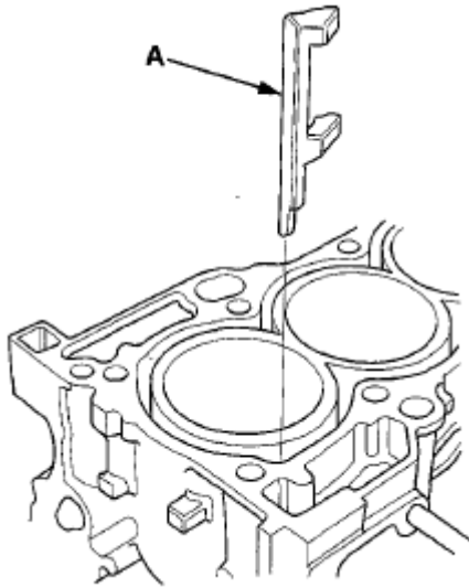
Fig. 129: Identifying Coolant Separator On Cylinder Head Courtesy of AMERICAN HONDA MOTOR CO., INC.
