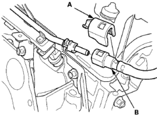
Fig. 76: Identifying Quick-Connect Fitting Cover And Fuel Feed Hose
