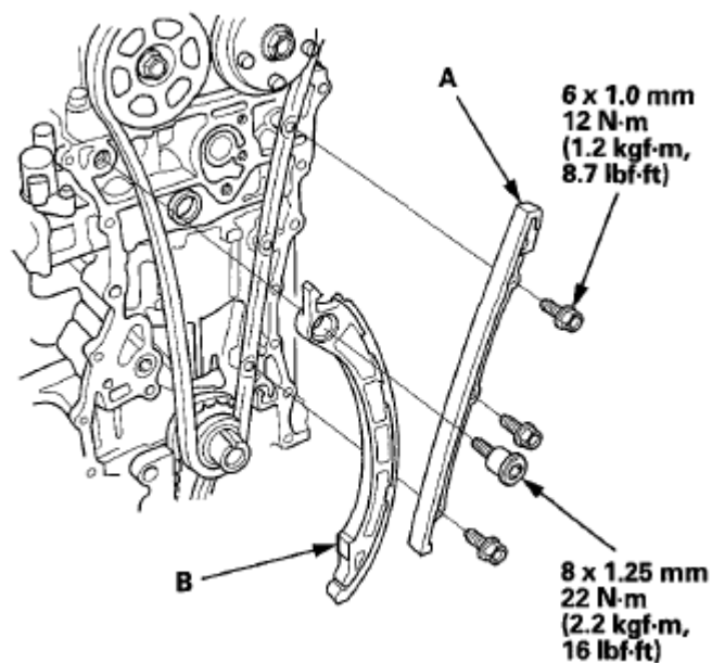
Fig. 41: Identifying Cam Chain Guide And Tensioner Arm With Torque Specifications Courtesy of AMERICAN HONDA MOTOR CO., INC.
