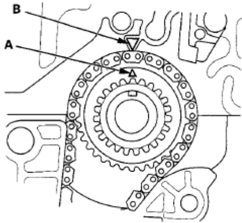
Fig. 131: Identifying TDC Mark And Crankshaft Sprocket With Pointer Courtesy of AMERICAN HONDA MOTOR CO., INC.
