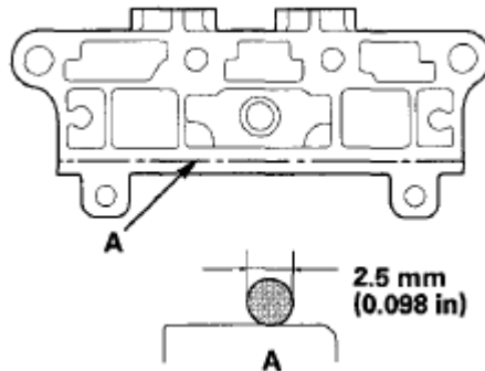
Fig. 125: Identifying Diameter Bead Of Liquid Gasket Broken Line Courtesy of AMERICAN HONDA MOTOR CO., INC.
