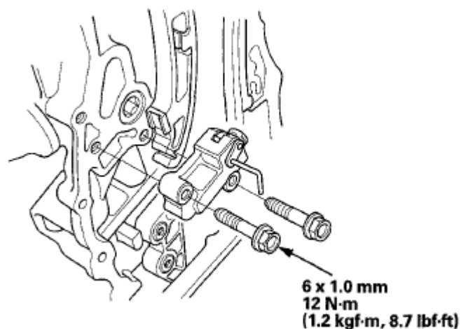
Fig. 44: Identifying Auto-Tensioner With Torque Specifications Courtesy of AMERICAN HONDA MOTOR CO., INC.
