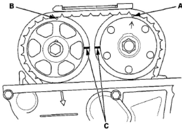
Fig. 15: Identifying TDC Punch Mark, VTC Actuator Punch Mark And TDC Marks Courtesy of AMERICAN HONDA MOTOR CO., INC.
