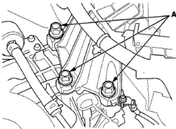
Fig. 20: Identifying Upper Transmission Mount Bracket Mounting Bolts In A/T Model Courtesy of AMERICAN HONDA MOTOR CO., INC.
