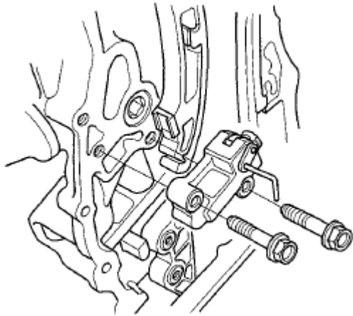
Fig. 33: Identifying Auto-Tensioner
