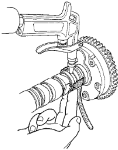
Fig. 13: Applying Air To The Unsealed Advance Hole To Release The Lock. Courtesy of AMERICAN HONDA MOTOR CO., INC.
