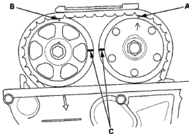
Fig. 26: Identifying TDC Punch Mark, VTC Actuator And Exhaust Camshaft Sprocket Courtesy of AMERICAN HONDA MOTOR CO., INC.
