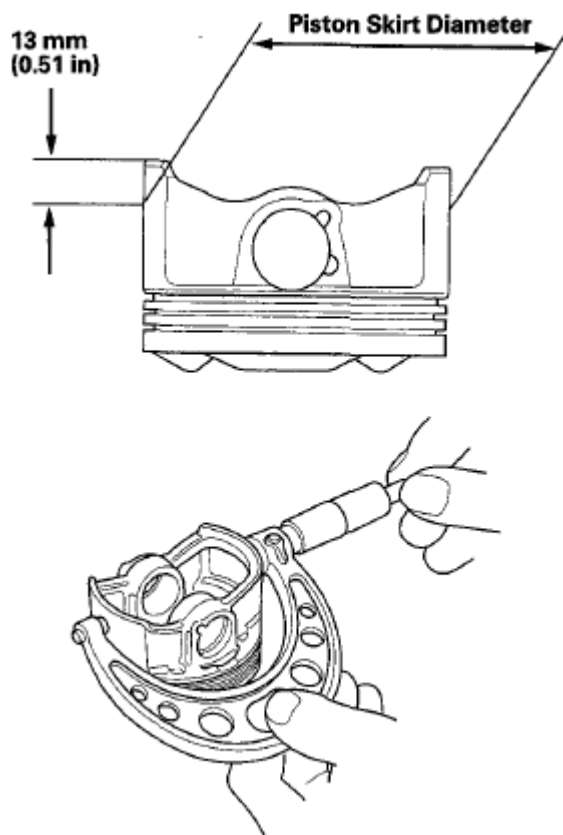
Fig. 34: Identifying Piston Skirt Diameter
