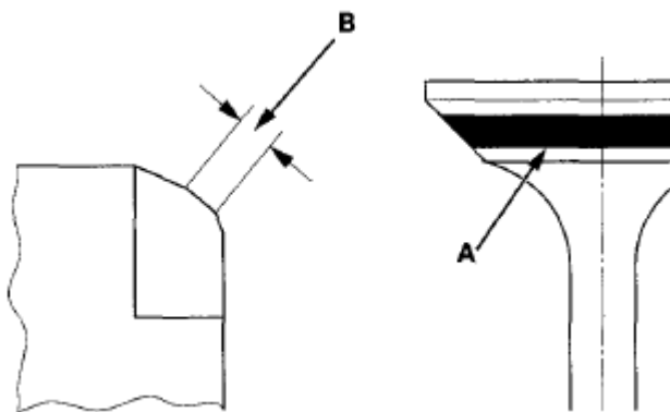
Fig. 120: Identifying Blue Compound And Valve Seating Surface Courtesy of AMERICAN HONDA MOTOR CO., INC.
