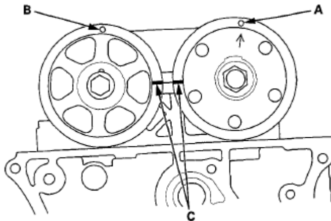
Fig. 37: Identifying TDC Punch Mark And VTC Actuator Punch Mark Courtesy of AMERICAN HONDA MOTOR CO., INC.
