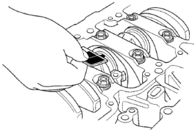
Fig. 12: Measuring Widest Part Of Plastigage Courtesy of AMERICAN HONDA MOTOR CO., INC.
