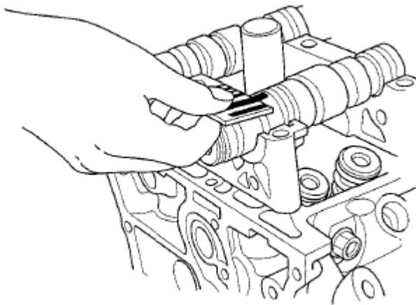
Fig. 104: Measuring Widest Portion Of Plastic Gauge Courtesy of AMERICAN HONDA MOTOR CO., INC.
