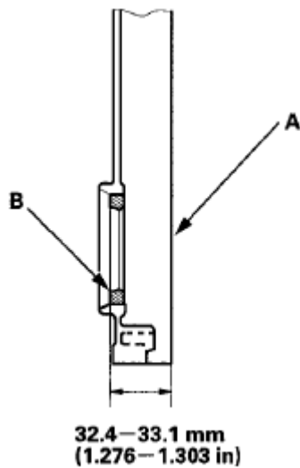
Fig. 62: Identifying Distance Between Chain Case Surface And Oil Seal Courtesy of AMERICAN HONDA MOTOR CO., INC.
