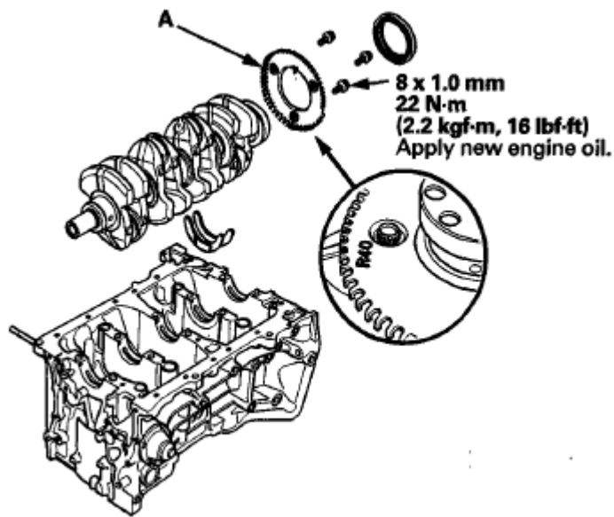
Fig. 71: Identifying CKP Pulse Plate In Crankshaft With Torque Specifications Courtesy of AMERICAN HONDA MOTOR CO., INC.
