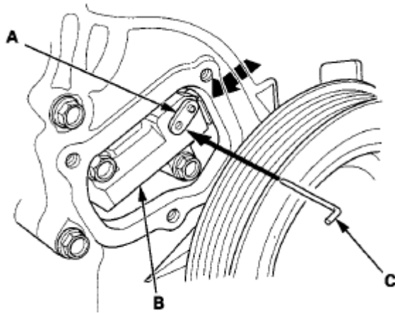
Fig. 88: Identifying Crankshaft Hole Alignment And Lock Pin Courtesy of AMERICAN HONDA MOTOR CO., INC.
