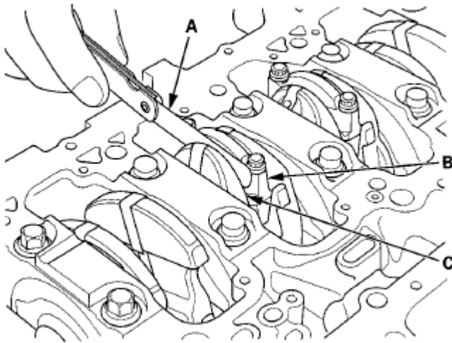
Fig. 4: Measuring Feeler Gauge, Connecting Rod And Crankshaft Courtesy of AMERICAN HONDA MOTOR CO., INC.
