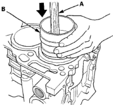
Fig. 58: Installing Ring Compressor In Cylinder Bore With Tool Courtesy of AMERICAN HONDA MOTOR CO., INC.
