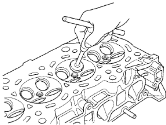
Fig. 118: Identifying Valve Seats In Cylinder Head And Valve Seat Cutter Courtesy of AMERICAN HONDA MOTOR CO., INC.
