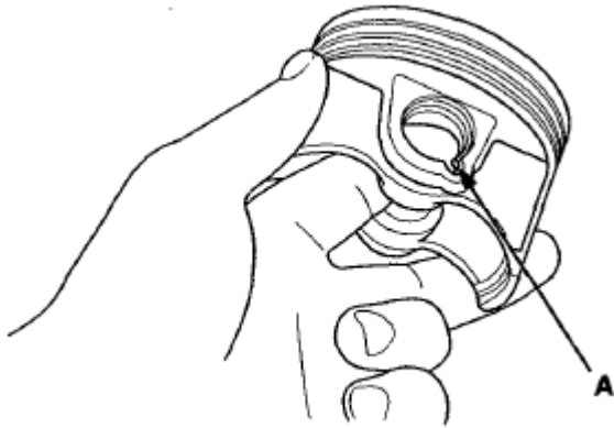
Fig. 46: Installing Piston Pin Snap Ring
