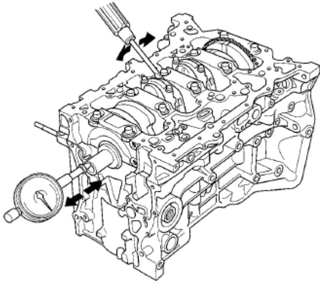
Fig. 5: Checking Crankshaft End Play
