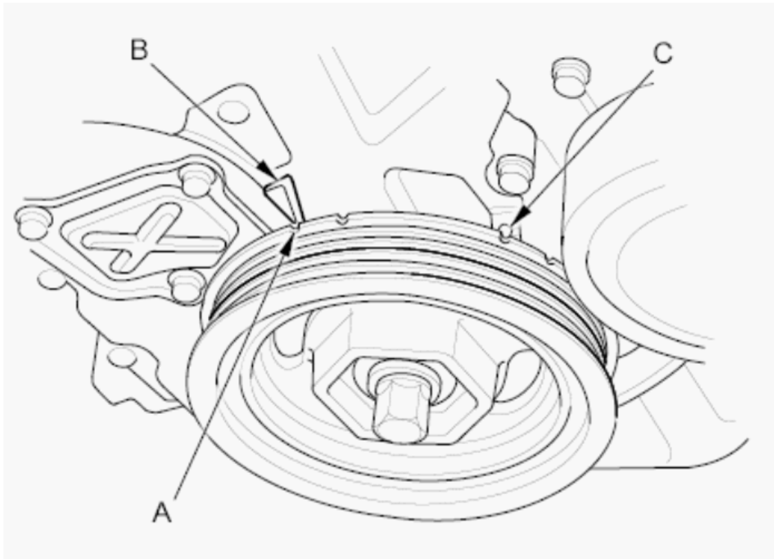
Fig. 25: Turning Crankshaft So White Mark (A) Lines Up With Pointer (B)
