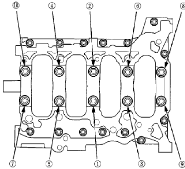
Fig. 6: Identifying Bolts And Tightening Sequence Courtesy of AMERICAN HONDA MOTOR CO., INC.
