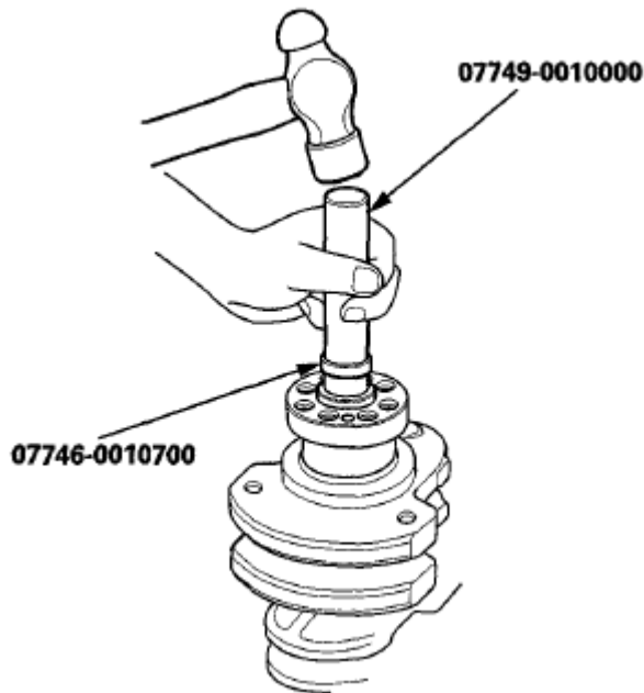
Fig. 60: Installing Crankshaft End Bushing In Crankshaft Courtesy of AMERICAN HONDA MOTOR CO., INC.
