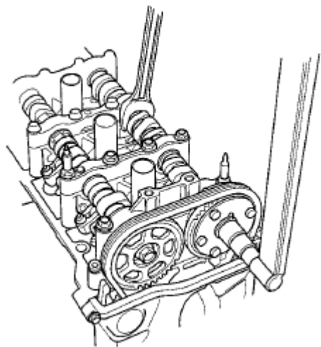
Fig. 89: Tightening Cam Shaft Bolts
