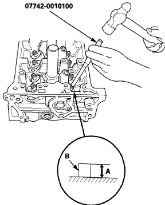
Fig. 116: Identifying Valve Guide Installed Height Courtesy of AMERICAN HONDA MOTOR CO., INC.
