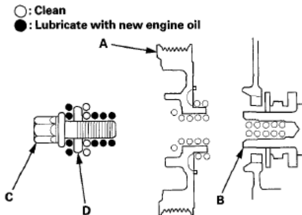
Fig. 23: Identifying Crankshaft Pulley, Crankshaft, Bolt And Washer
