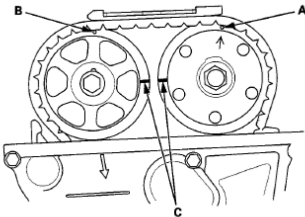
Fig. 87: Identifying TDC Punch Mark, VTC Actuator And Punch Mark And TDC Marks Courtesy of AMERICAN HONDA MOTOR CO., INC.
