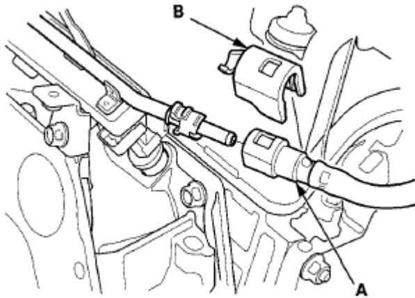
Fig. 139: Identifying Fuel Feed Hose And Connecting Covers Courtesy of AMERICAN HONDA MOTOR CO., INC.
