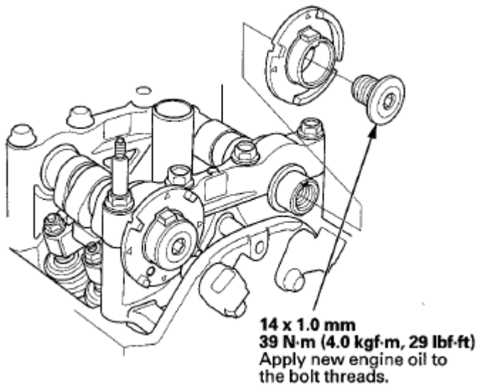
Fig. 85: Identifying CMP Pulse Plate With Torque Specifications Courtesy of AMERICAN HONDA MOTOR CO., INC.
