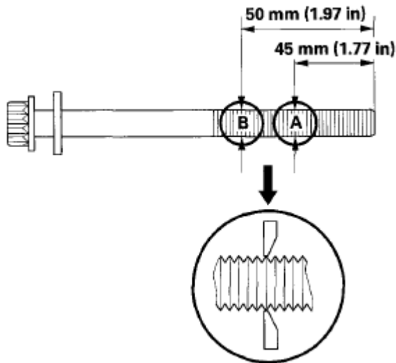
Fig. 132: Identifying Diameter Of Head Bolt Courtesy of AMERICAN HONDA MOTOR CO., INC.
