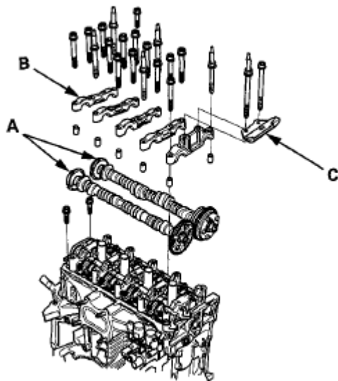
Fig. 127: Identifying Camshafts, Camshaft Holders And Cam Chain Guide Courtesy of AMERICAN HONDA MOTOR CO., INC.
