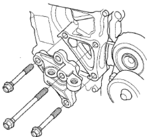
Fig. 29: Identifying Engine Mount Bracket Mounting Bolts Courtesy of AMERICAN HONDA MOTOR CO., INC.
