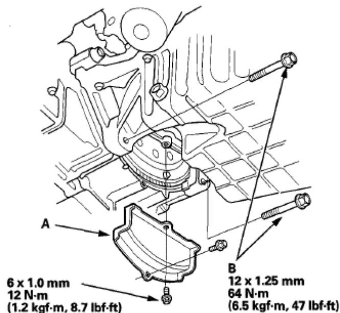
Fig. 74: Identifying Clutch Case Cover And Transmission Mounting Bolts With Torque Specifications
