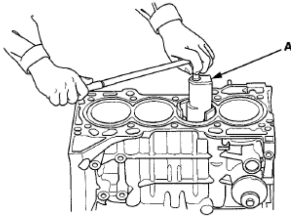
Fig. 30: Installing Ridge Reamer On Cylinder Courtesy of AMERICAN HONDA MOTOR CO., INC.
