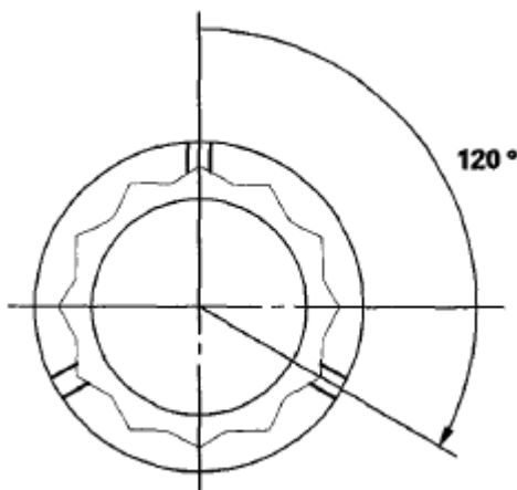
Fig. 56: Tightening Connecting Rod Bolts Courtesy of AMERICAN HONDA MOTOR CO., INC.
