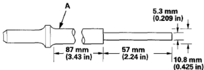
Fig. 113: Identifying Air Impact Valve Guide Driver Courtesy of AMERICAN HONDA MOTOR CO., INC.
