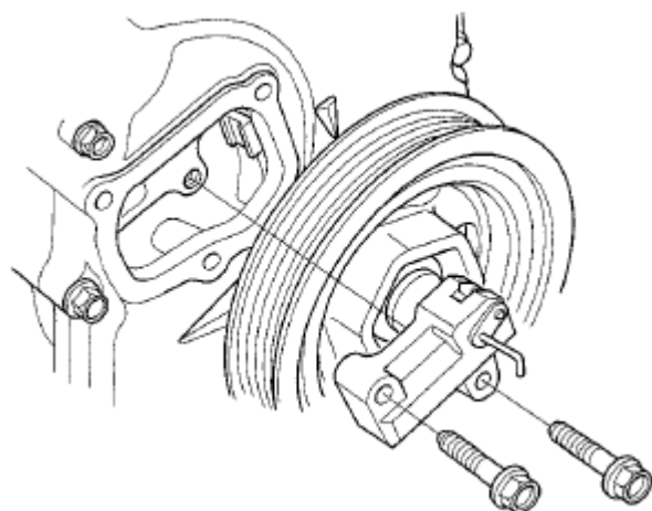
Fig. 56: Identifying Auto-Tensioner Courtesy of AMERICAN HONDA MOTOR CO., INC.
