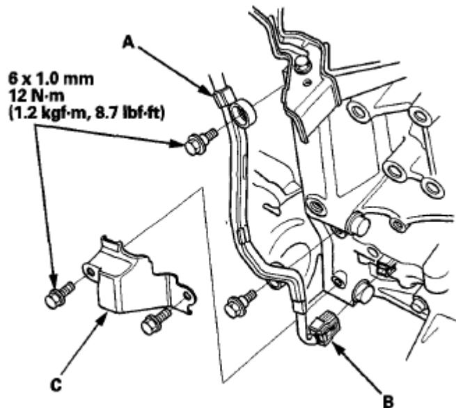
Fig. 70: Identifying Harness Holder, CKP Sensor Connector And CKP Sensor Cover With Torque Specifications
