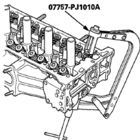
Fig. 108: Identifying Valve Spring Compressor Courtesy of AMERICAN HONDA MOTOR CO., INC.
