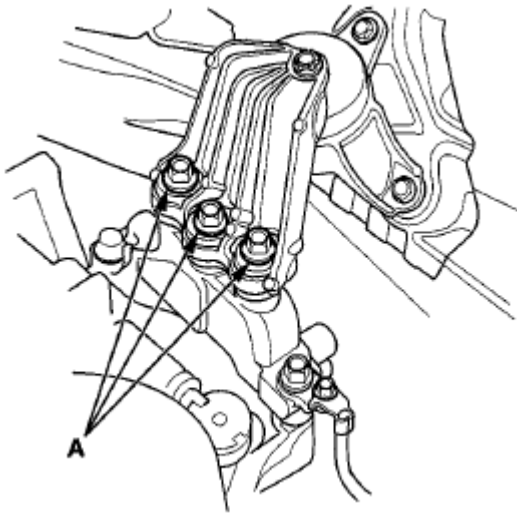
Fig. 19: Identifying Upper Transmission Mount Bracket Mounting Bolts In M/T Model Courtesy of AMERICAN HONDA MOTOR CO., INC.
