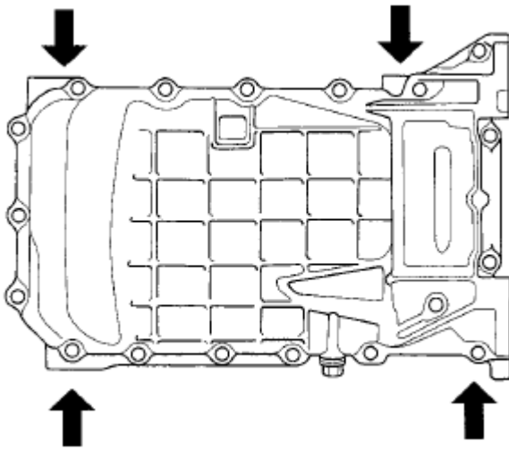
Fig. 23: Identifying Engine Block And Oil Pan Pry Points Courtesy of AMERICAN HONDA MOTOR CO., INC.
