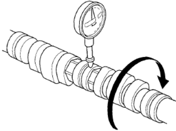
Fig. 105: Identifying Total Runout With Camshaft Courtesy of AMERICAN HONDA MOTOR CO., INC.
