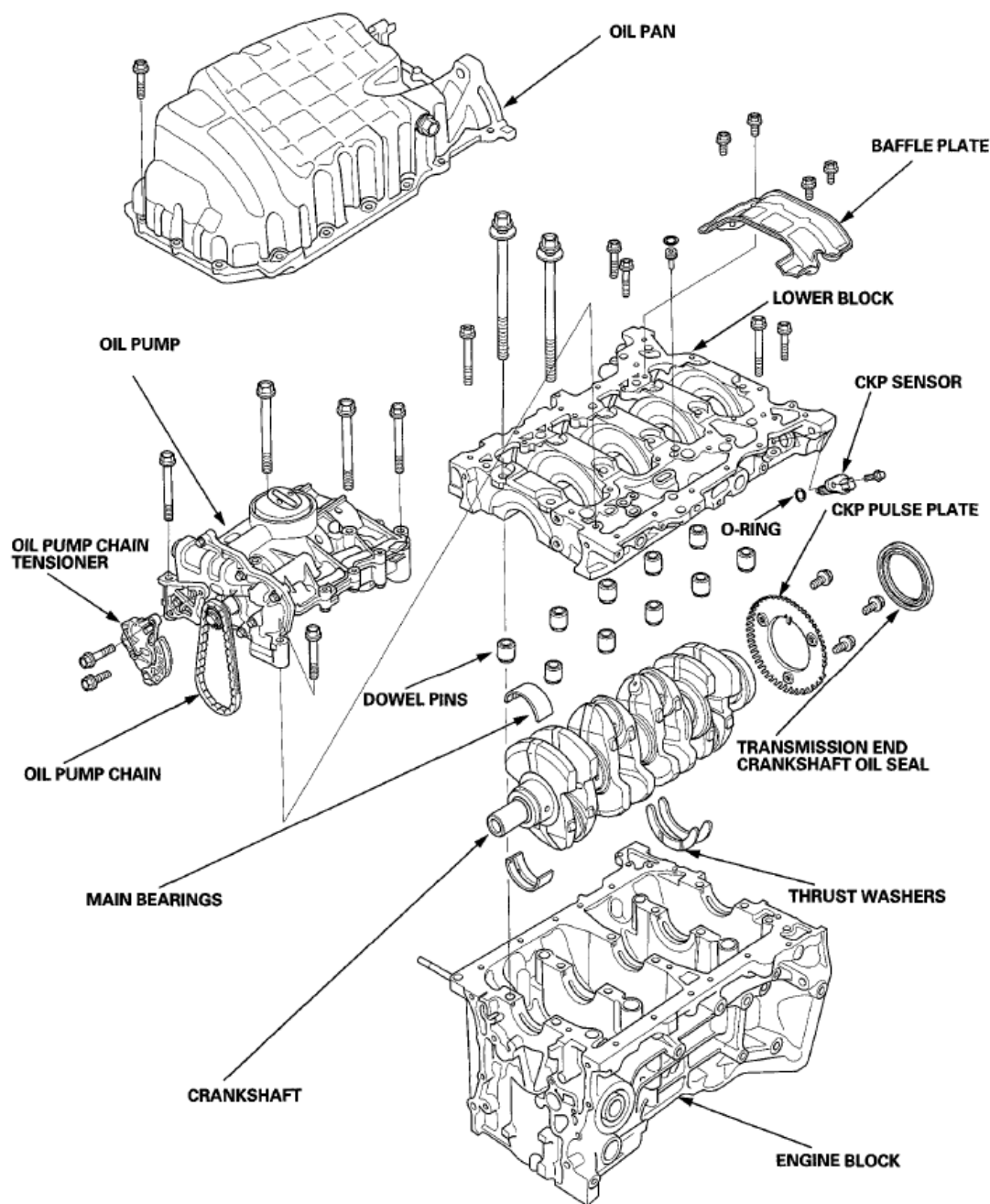
Fig. 2: Identifying Engine Block Component Location (1 Of 2)
