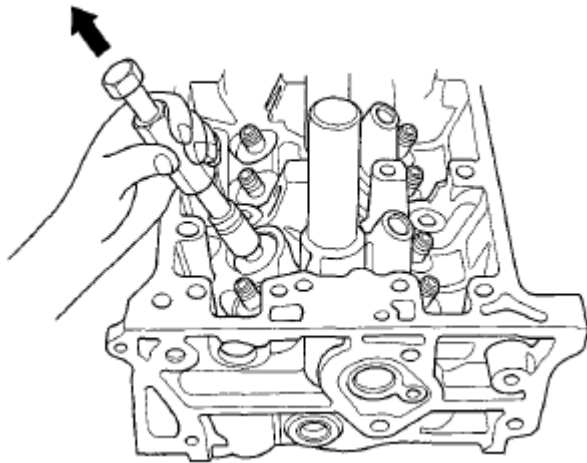
Fig. 110: Removing Valve Seal
