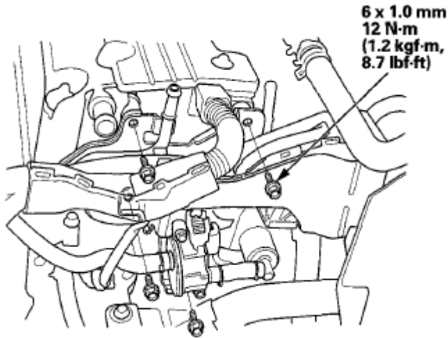
Fig. 137: Identifying EVAP Canister Purge Valve Bracket With Torque Specifications Courtesy of AMERICAN HONDA MOTOR CO., INC.
