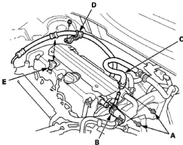
Fig. 73: Identifying Bolts And EVAP Canister Purge Valve Bracket Courtesy of AMERICAN HONDA MOTOR CO., INC.
