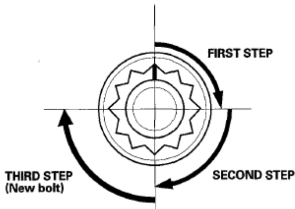
Fig. 134: Tightening Cylinder Head Bolts Courtesy of AMERICAN HONDA MOTOR CO., INC.
