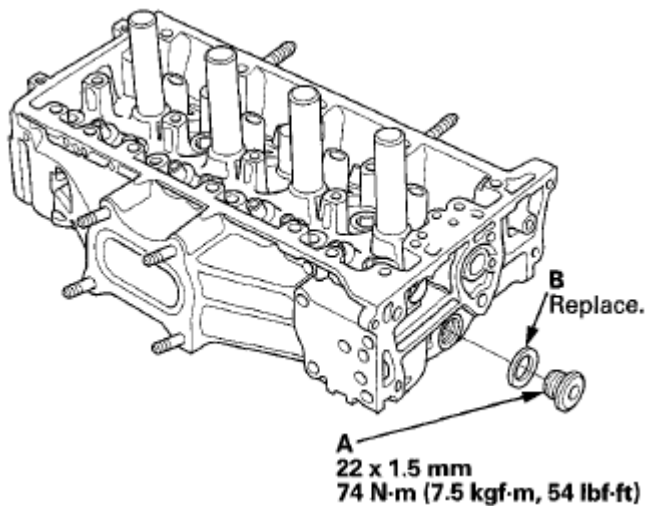
Fig. 141: Identifying Sealing Bolt And Washer With Torque Specifications Courtesy of AMERICAN HONDA MOTOR CO., INC.
