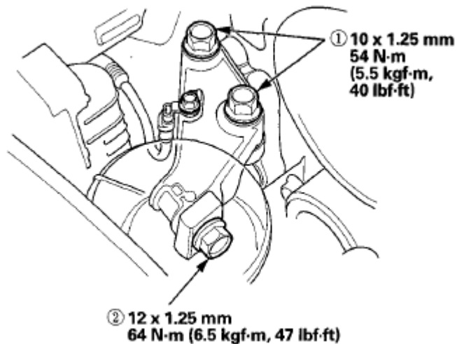
Fig. 76: Identifying Side Engine Mount Bracket Mounting Bolts And Bolts With Torque Specifications
