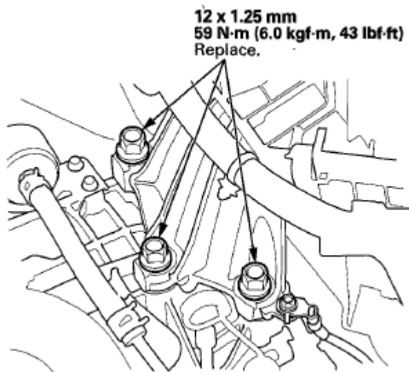
Fig. 80: Tightening Upper Transmission Mount Bracket Mounting Bolts In A/T Model With Torque Specifications
