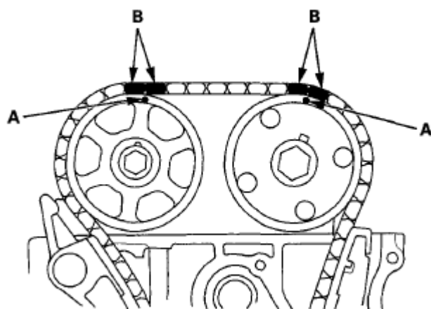
Fig. 40: Identifying Cam Sprocket Punch Marks And Colored Link Plates Courtesy of AMERICAN HONDA MOTOR CO., INC.
