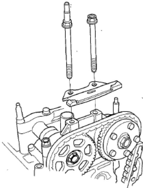
Fig. 34: Identifying Cam Chain Guide
