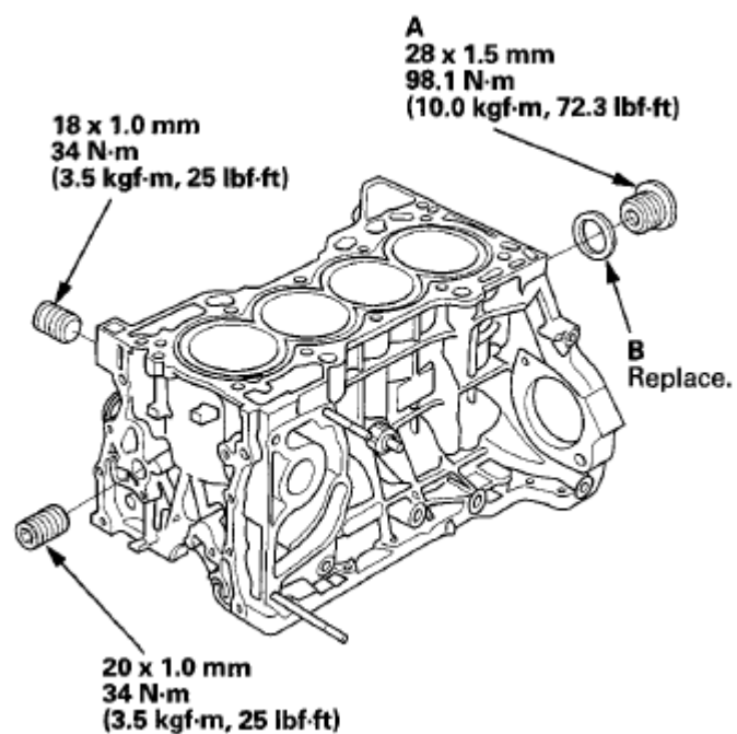
Fig. 83: Identifying Sealing Bolt And Washer With Torque Specifications Courtesy of AMERICAN HONDA MOTOR CO., INC.
