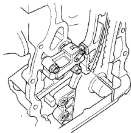
Fig. 45: Identifying Diameter Pin Courtesy of AMERICAN HONDA MOTOR CO., INC.
