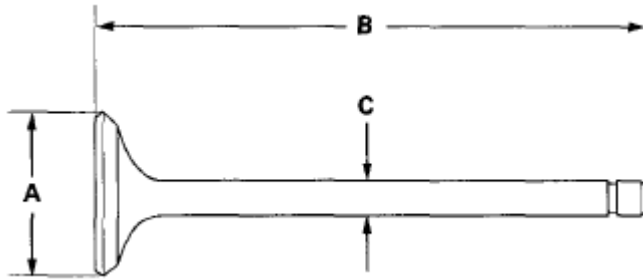
Fig. 111: Measuring Intake/Exhaust Valve Stem Guide Courtesy of AMERICAN HONDA MOTOR CO., INC.
