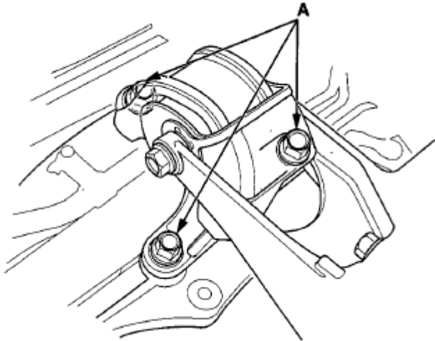
Fig. 17: Identifying Rear Engine Mount Mounting Bolts In M/T Model Courtesy of AMERICAN HONDA MOTOR CO., INC.
