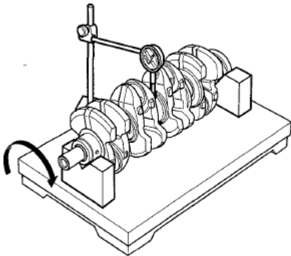
Fig. 33: Identifying Crankshaft Supported On V-Blocks Courtesy of AMERICAN HONDA MOTOR CO., INC.
