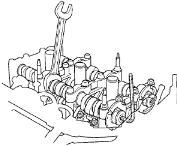
Fig. 82: Holding Camshaft With Wrench To Loosen Bolt Courtesy of AMERICAN HONDA MOTOR CO., INC.
