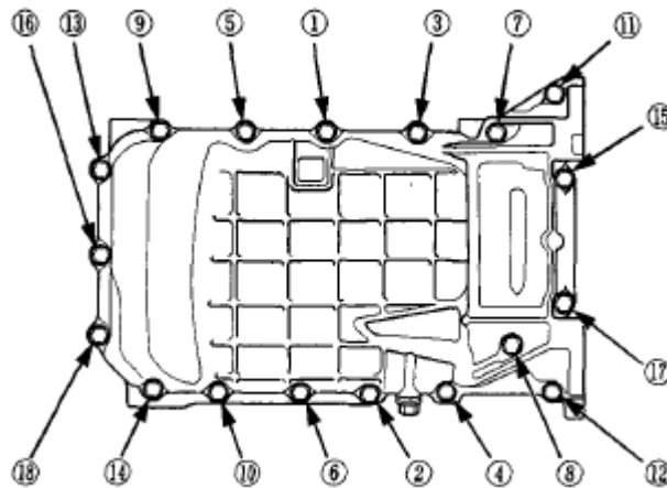
Fig. 73: Identifying Oil Pan Bolts Tightening Sequence Courtesy of AMERICAN HONDA MOTOR CO., INC.
