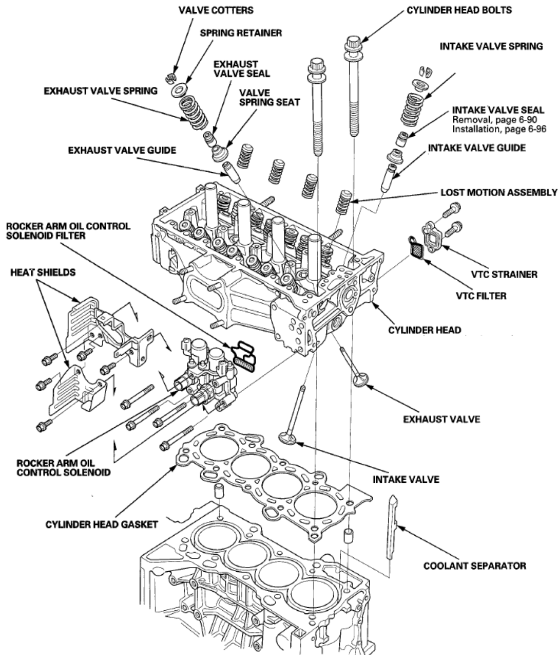
Fig. 4: Identifying Cylinder Head Component Location (3 Of 3)
