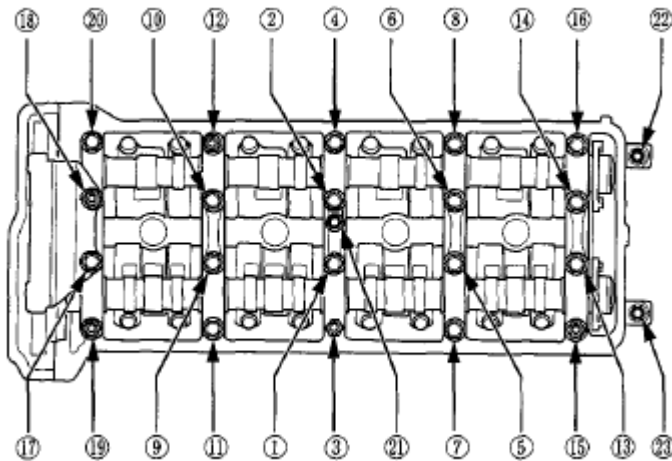
Fig. 128: Identifying Rocker Arm Bolts With Tightening Sequence Courtesy of AMERICAN HONDA MOTOR CO., INC.
