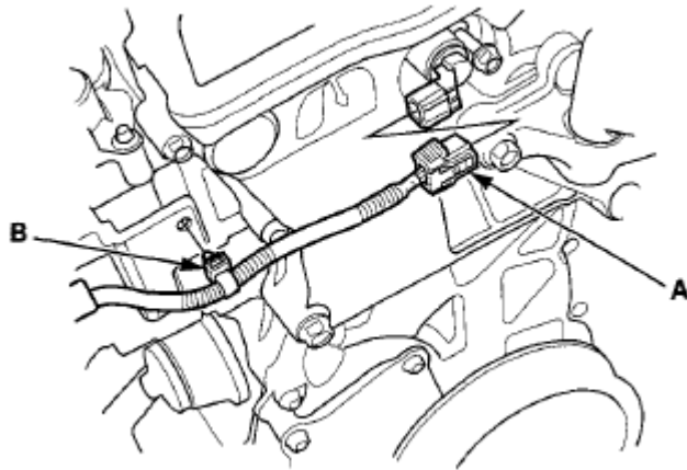
Fig. 27: Identifying VTC Oil Control Solenoid Valve Connector And Harness Clamp Courtesy of AMERICAN HONDA MOTOR CO., INC.
