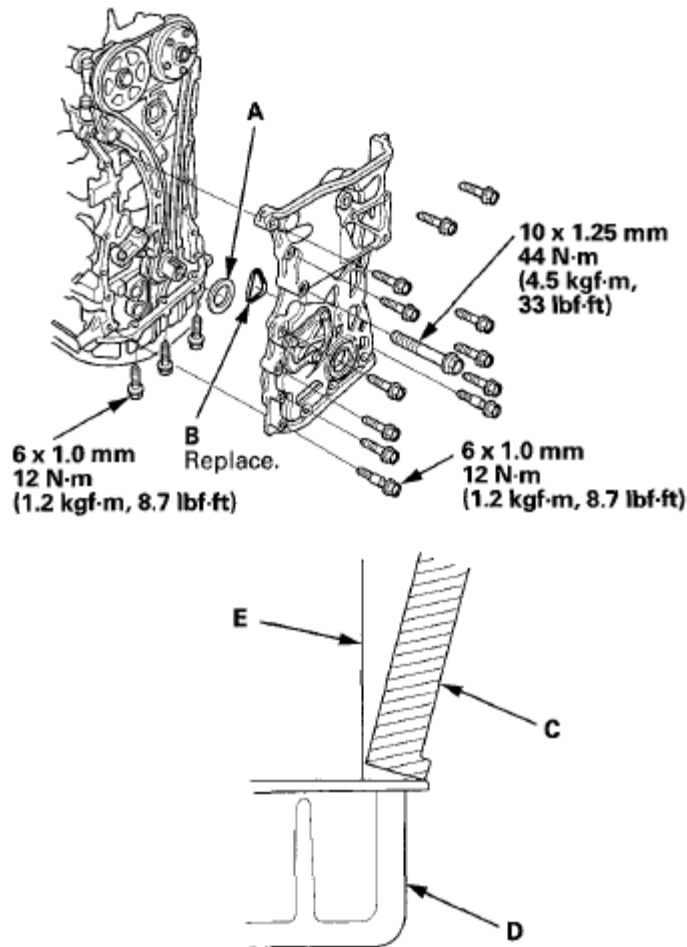
Fig. 49: Identifying Spacer, O-Ring, Chain Case And Oil Pan With Torque Specifications Courtesy of AMERICAN HONDA MOTOR CO., INC.
