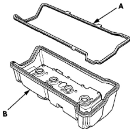
Fig. 69: Identifying Head Cover Gasket And Groove Of Cylinder Head Cover
