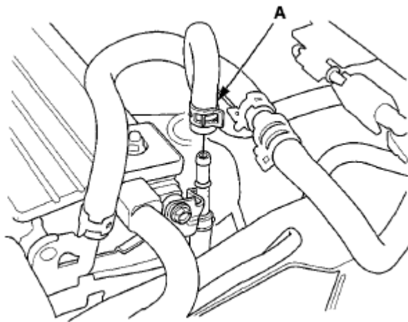
Fig. 140: Identifying EVAP Canister Hose Courtesy of AMERICAN HONDA MOTOR CO., INC.
