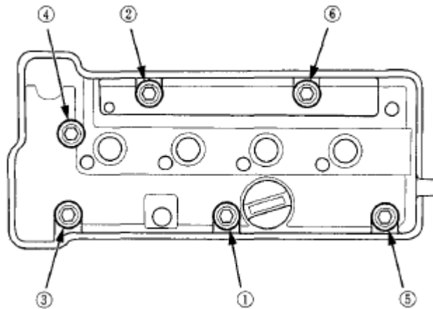
Fig. 72: Identifying Cylinder Head Cover Bolts Tightening Sequence Courtesy of AMERICAN HONDA MOTOR CO., INC.
