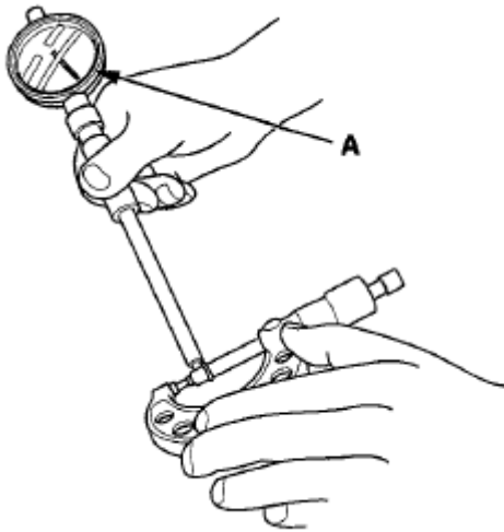
Fig. 98: Measuring Zero Gauge Shaft Diameter Courtesy of AMERICAN HONDA MOTOR CO., INC.
