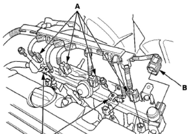
Fig. 77: Identifying Fuel Injector Connectors And Engine Mount Control Solenoid Valve Connector
