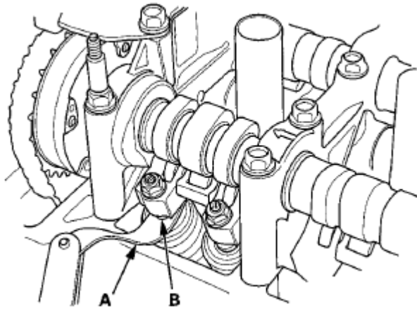
Fig. 17: Identifying Feeler Gauge And Adjusting Screw Courtesy of AMERICAN HONDA MOTOR CO., INC.
