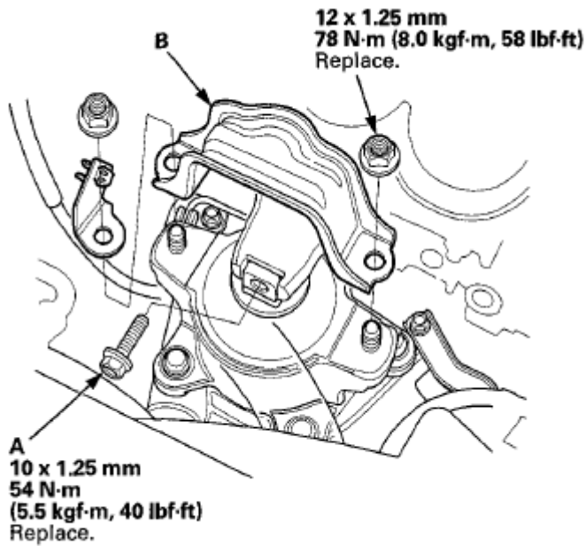
Fig. 75: Identifying Front Engine Mount Mounting Bolt And Front Engine Mount Stop With Torque Specifications
