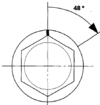
Fig. 65: Tightening Bearing Cap Bolts Courtesy of AMERICAN HONDA MOTOR CO., INC.
