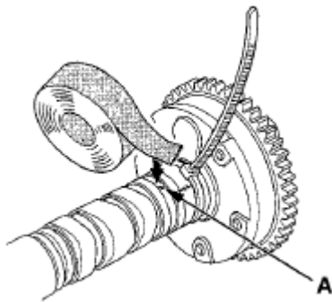
Fig. 12: Identifying Advance Holes Courtesy of AMERICAN HONDA MOTOR CO., INC.
