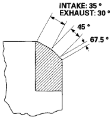
Fig. 119: Identifying Width And Edge Of Seat Courtesy of AMERICAN HONDA MOTOR CO., INC.
