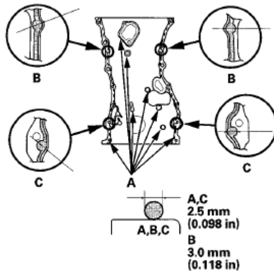
Fig. 47: Identifying Liquid Gasket Along Broken Line Courtesy of AMERICAN HONDA MOTOR CO., INC.
