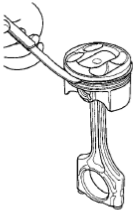
Fig. 52: Measuring Top Ring Clearance Courtesy of AMERICAN HONDA MOTOR CO., INC.
