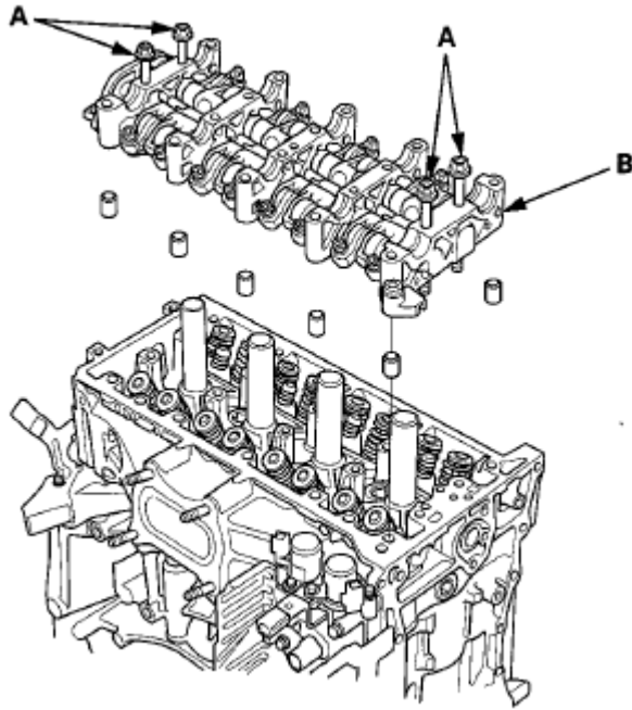
Fig. 95: Identifying Bolts In Rocker Arm Assembly Courtesy of AMERICAN HONDA MOTOR CO., INC.
