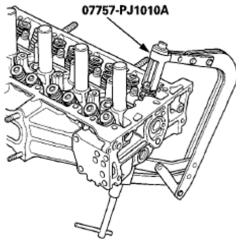
Fig. 123: Identifying Valve Spring Compressor Courtesy of AMERICAN HONDA MOTOR CO., INC.
