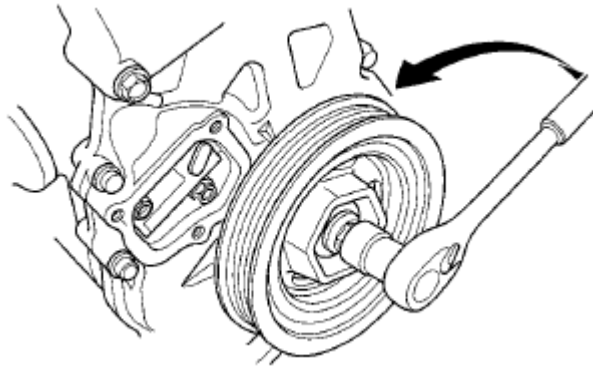
Fig. 54: Identifying Crankshaft Counterclockwise Auto-Tensioner
