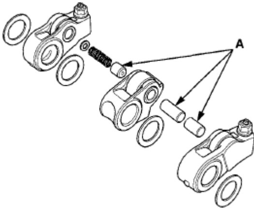
Fig. 100: Identifying Rocker Arm Pistons (Intake Side) Courtesy of AMERICAN HONDA MOTOR CO., INC.
