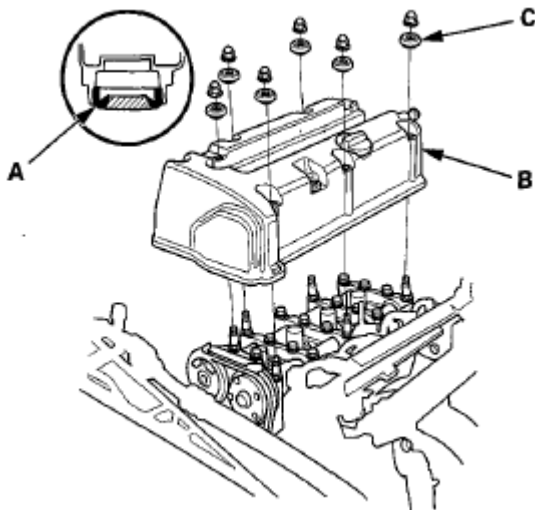
Fig. 71: Identifying Spark Plug Seals And Cylinder Head Cover Courtesy of AMERICAN HONDA MOTOR CO., INC.
