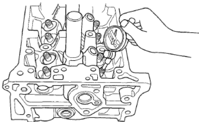
Fig. 112: Identifying Valve Stem-To-Guide Clearance
