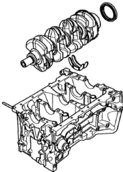
Fig. 29: Identifying Journals And CKP Pulse Plate
