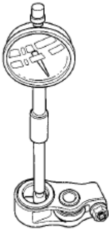
Fig. 99: Identifying Inside Diameter Of Rocker Arm Courtesy of AMERICAN HONDA MOTOR CO., INC.
