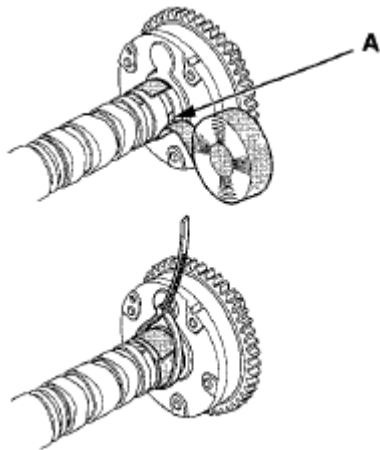
Fig. 11: Identifying Retard Holes In Intake Camshaft Courtesy of AMERICAN HONDA MOTOR CO., INC.
