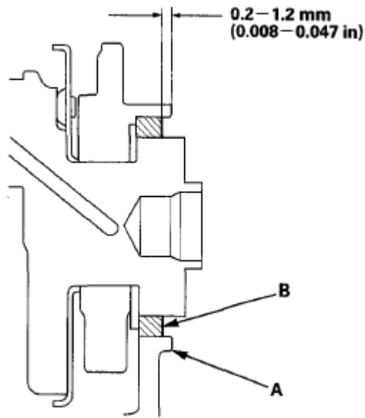
Fig. 82: Identifying Distance Between Engine Block And Crankshaft Oil Seal Courtesy of AMERICAN HONDA MOTOR CO., INC.
