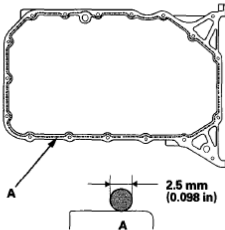
Fig. 72: Identifying Diameter Bead Of Liquid Gasket Broken Line Courtesy of AMERICAN HONDA MOTOR CO., INC.
