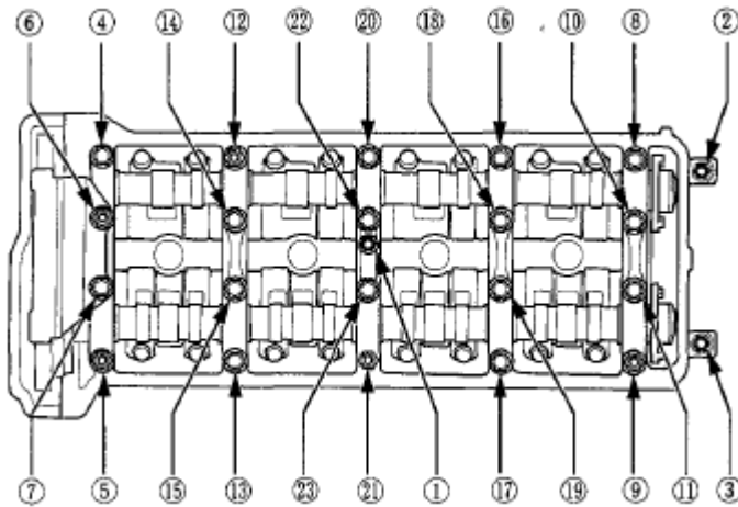
Fig. 93: Identifying Camshaft Holder Bolts With Loosening Sequence
