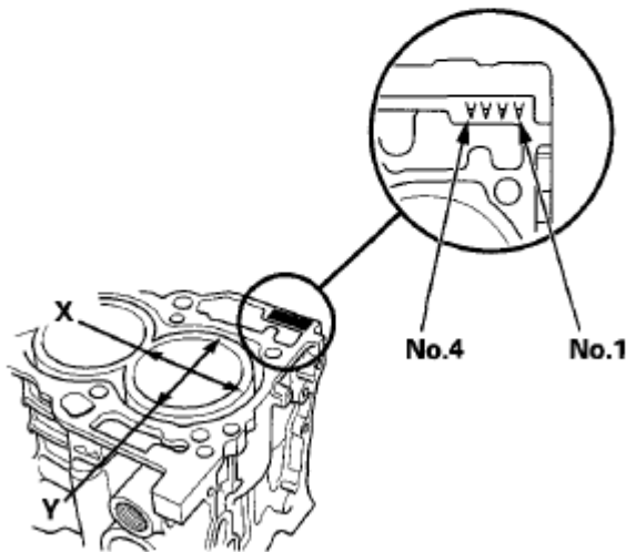
Fig. 35: Identifying Block And Piston
