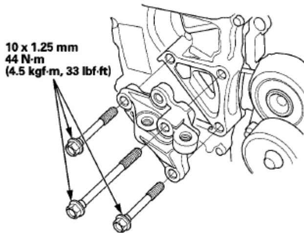
Fig. 50: Identifying Engine Mount Bracket And Engine Mount Bracket Mounting Bolts With Torque Specifications
