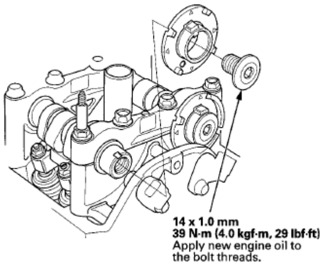
Fig. 83: Identifying CMP Pulse Plate With Torque Specifications Courtesy of AMERICAN HONDA MOTOR CO., INC.
