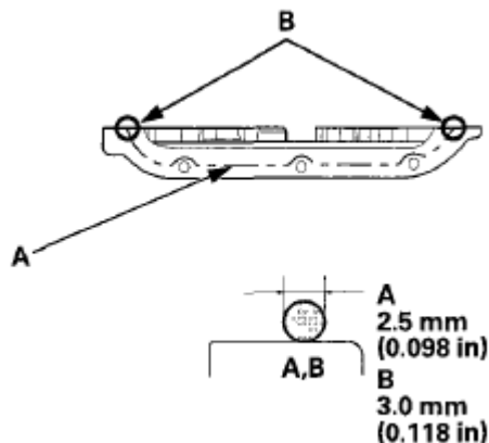
Fig. 48: Identifying Diameter Bead Of Liquid Gasket Along Broken Line Courtesy of AMERICAN HONDA MOTOR CO., INC.
