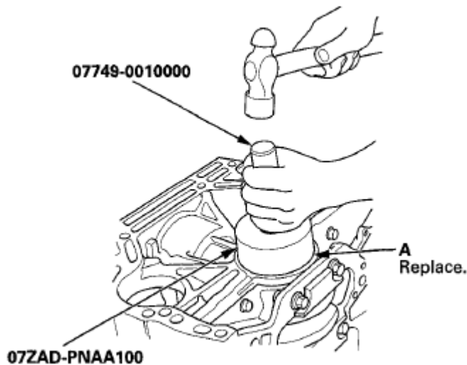
Fig. 67: Installing Oil Seal Driver With SST Courtesy of AMERICAN HONDA MOTOR CO., INC.
