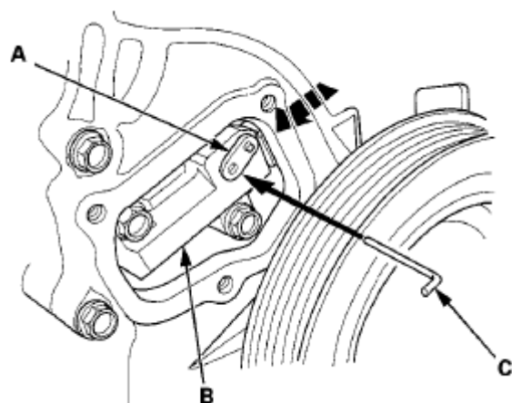
Fig. 55: Identifying Crankshaft Lock, Auto-Tensioner And Diameter Pin Courtesy of AMERICAN HONDA MOTOR CO., INC.
