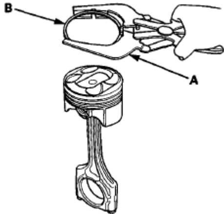
Fig. 49: Installing Ring Expander And Piston Rings Courtesy of AMERICAN HONDA MOTOR CO., INC.
