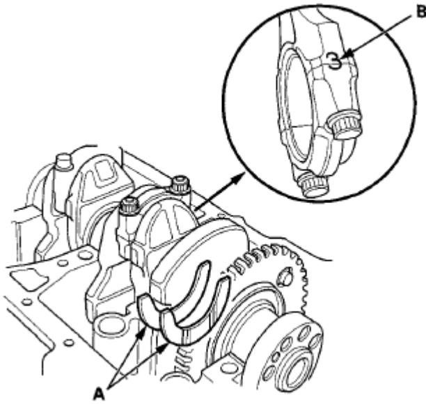
Fig. 61: Identifying Thrust Washers And Mark Of Line In Engine Courtesy of AMERICAN HONDA MOTOR CO., INC.
