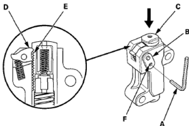
Fig. 43: Identifying Auto-Tensioner Cam Chain, Rod Plate And Holes Courtesy of AMERICAN HONDA MOTOR CO., INC.
