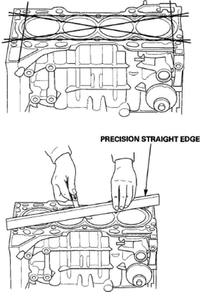
Fig. 36: Measuring Engine Block Warpage Courtesy of AMERICAN HONDA MOTOR CO., INC.
