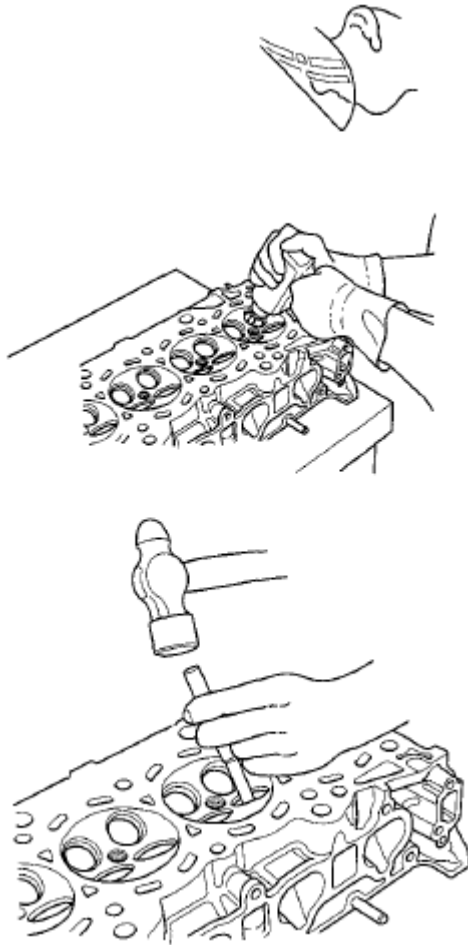
Fig. 115: Removing Guide Toward Camshaft Side Of Head Courtesy of AMERICAN HONDA MOTOR CO., INC.
