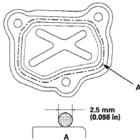
Fig. 59: Identifying Diameter Bead Of Liquid Gasket Along Broken Line Courtesy of AMERICAN HONDA MOTOR CO., INC.
