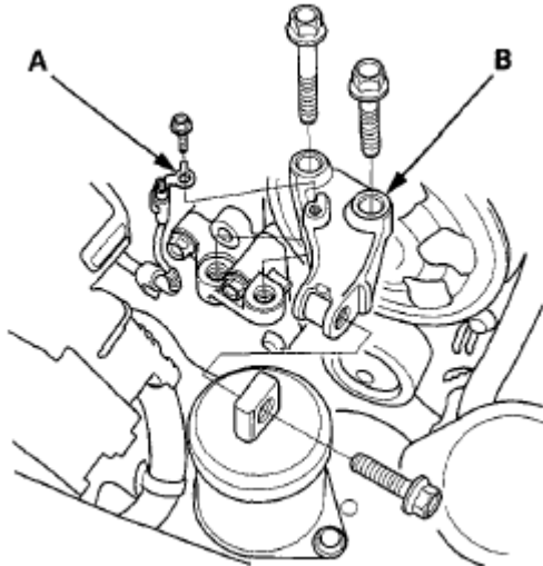
Fig. 28: Identifying Ground Cable And Engine Mount Bracket Courtesy of AMERICAN HONDA MOTOR CO., INC.
