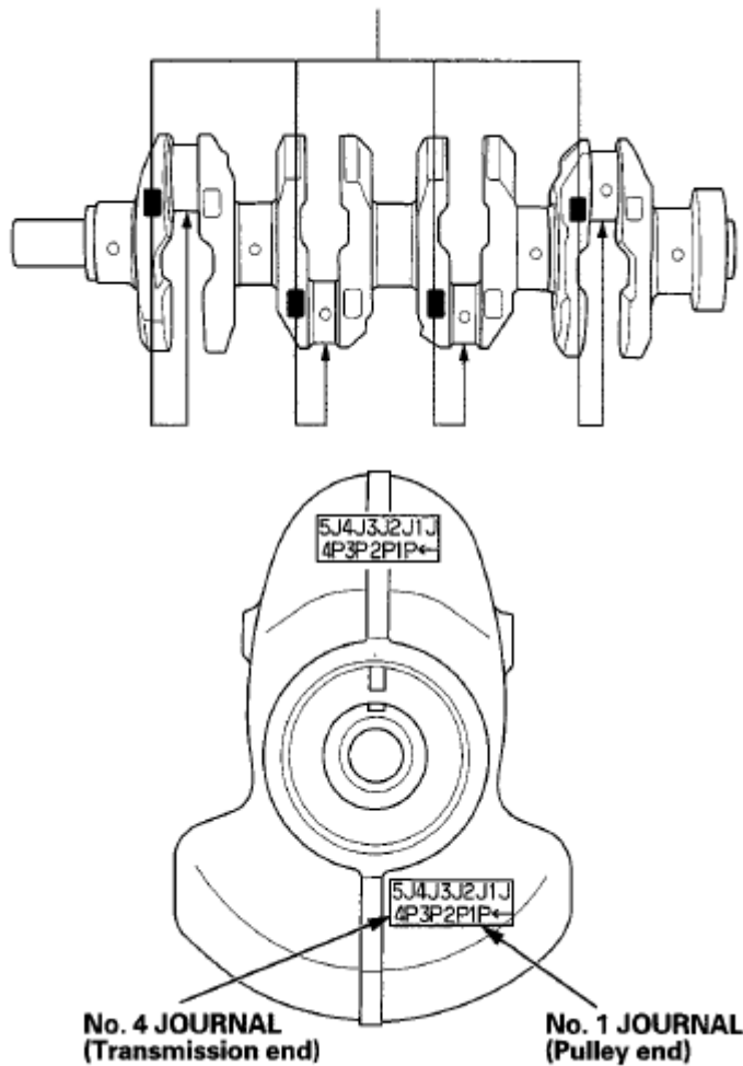
Fig. 14: Identifying Journal Code Location On Crankshaft Courtesy of AMERICAN HONDA MOTOR CO., INC.
