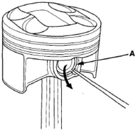
Fig. 40: Identifying Snap Rings In Piston Pin Bore Courtesy of AMERICAN HONDA MOTOR CO., INC.
