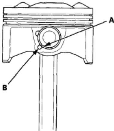
Fig. 39: Identifying Piston Pin Snap Rings And Piston Pin Bores Courtesy of AMERICAN HONDA MOTOR CO., INC.
