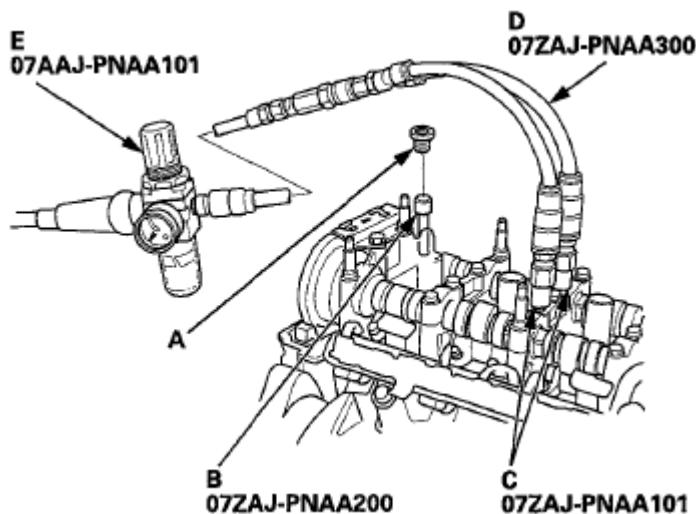
Fig. 8: Identifying Sealing Bolt And VTEC Air Stopper
