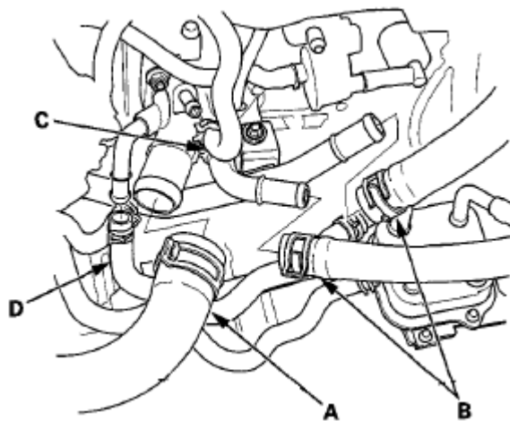
Fig. 136: Identifying Upper Radiator Hose, Heater Hoses And Water Bypass Hose
