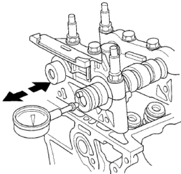
Fig. 103: Identifying Zero Dial Indicator In Cylinder Head Courtesy of AMERICAN HONDA MOTOR CO., INC.
