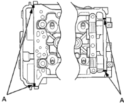
Fig. 70: Identifying Rocker Shaft Holder Mating Areas Courtesy of AMERICAN HONDA MOTOR CO., INC.
