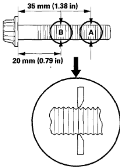
Fig. 59: Identifying Connecting Rod Bolt Courtesy of AMERICAN HONDA MOTOR CO., INC.
