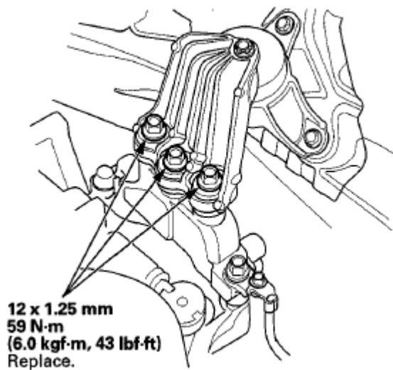
Fig. 79: Tightening Upper Transmission Mount Bracket Mounting Bolts In M/T Model With Torque Specifications
