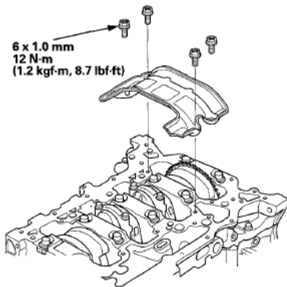
Fig. 69: Identifying Baffle Plate With Torque Specifications Courtesy of AMERICAN HONDA MOTOR CO., INC.
