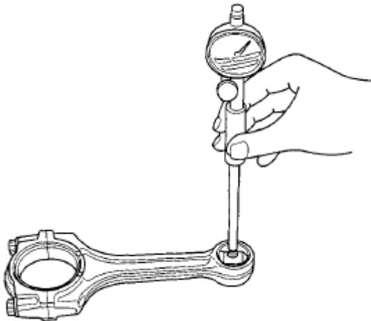
Fig. 45: Measuring Piston Pin-To-Connecting Rod Clearance Courtesy of AMERICAN HONDA MOTOR CO., INC.
