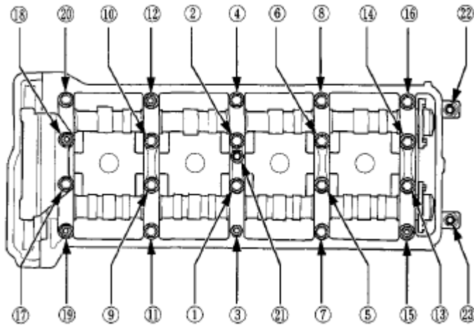
Fig. 102: Identifying Rocker Shaft Holders With Tightening Sequence Courtesy of AMERICAN HONDA MOTOR CO., INC.
