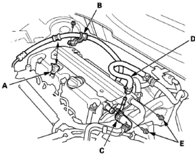
Fig. 67: Identifying Dipstick, Power Steering Hose Bracket, Breather Hose And Brake Booster Vacuum Hose
