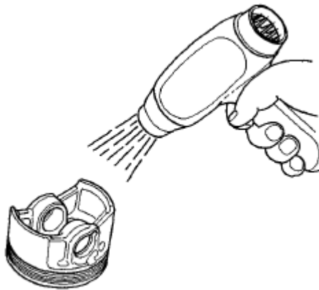
Fig. 47: Heating Piston
