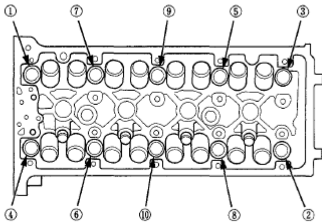
Fig. 81: Identifying Cylinder Head Bolt Loosening Sequence Courtesy of AMERICAN HONDA MOTOR CO., INC.
