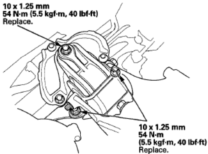
Fig. 78: Tightening Rear Engine Mount Mounting Bolts In M/T Model With Torque Specifications Courtesy of AMERICAN HONDA MOTOR CO., INC.
