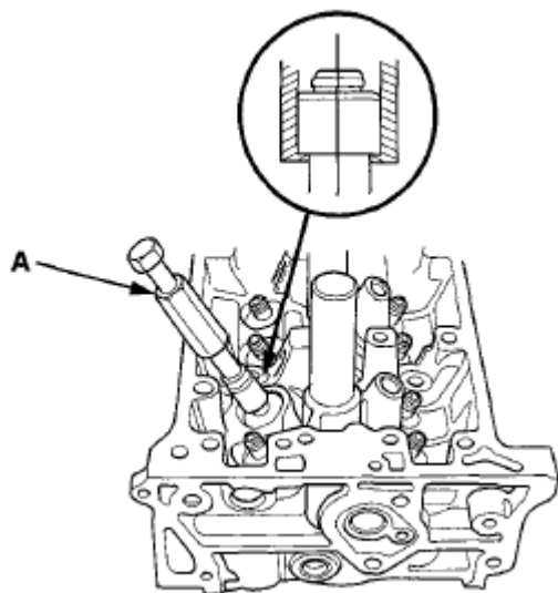
Fig. 109: Installing Valve Guide Seal Remover Courtesy of AMERICAN HONDA MOTOR CO., INC.
