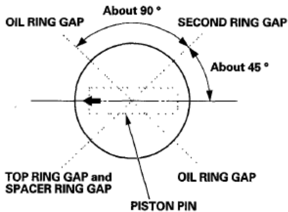
Fig. 53: Positioning Ring End Gaps
