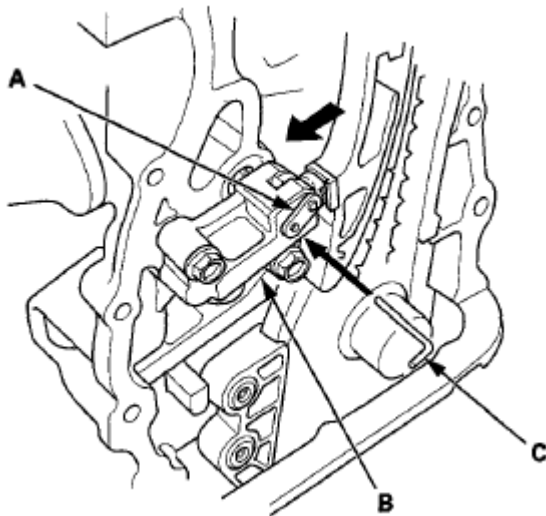
Fig. 32: Identifying Hole Alignment And Pin Courtesy of AMERICAN HONDA MOTOR CO., INC.
