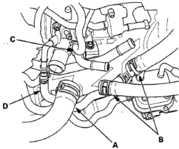
Fig. 79: Identifying Upper Radiator Hose, Heater Hoses And Water Bypass Hose Courtesy of AMERICAN HONDA MOTOR CO., INC.
