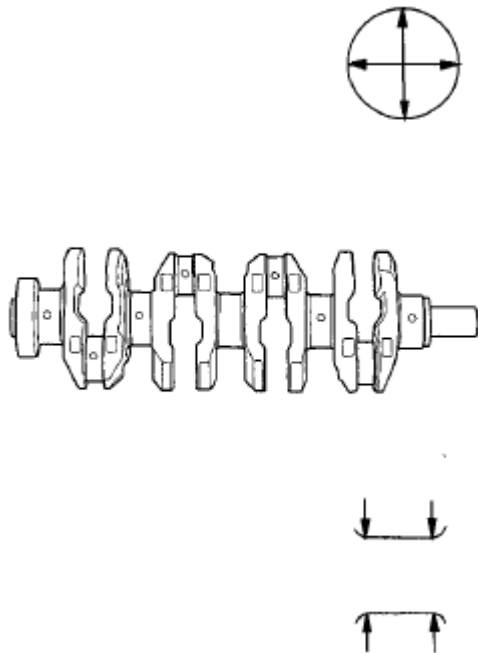
Fig. 32: Identifying Edges Of Rod And Main Journal Courtesy of AMERICAN HONDA MOTOR CO., INC.
