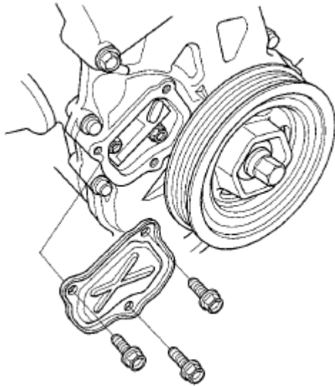
Fig. 53: Identifying Chain Case Cover
