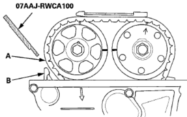
Fig. 64: Identifying Cam Chain And Tensioner Arm Courtesy of AMERICAN HONDA MOTOR CO., INC.
