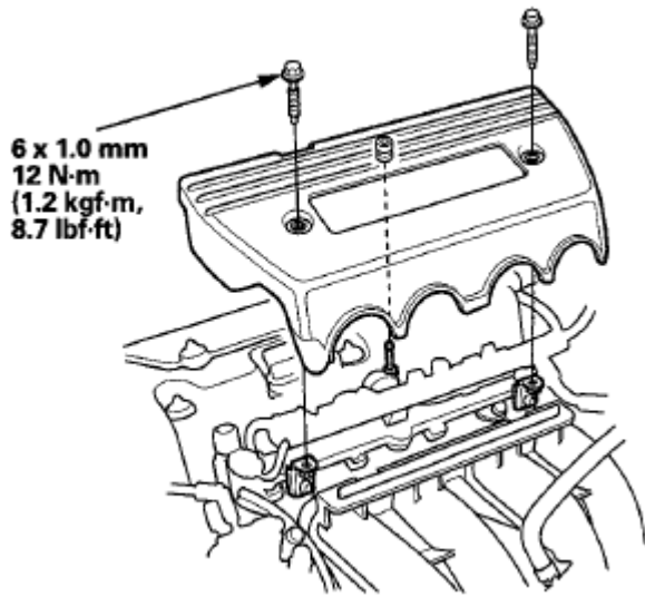
Fig. 74: Identifying Engine Cover With Torque Specifications Courtesy of AMERICAN HONDA MOTOR CO., INC.
