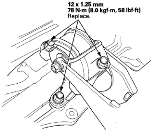
Fig. 77: Tightening Rear Engine Mount Mounting Bolts In M/T Model With Torque Specifications Courtesy of AMERICAN HONDA MOTOR CO., INC.
