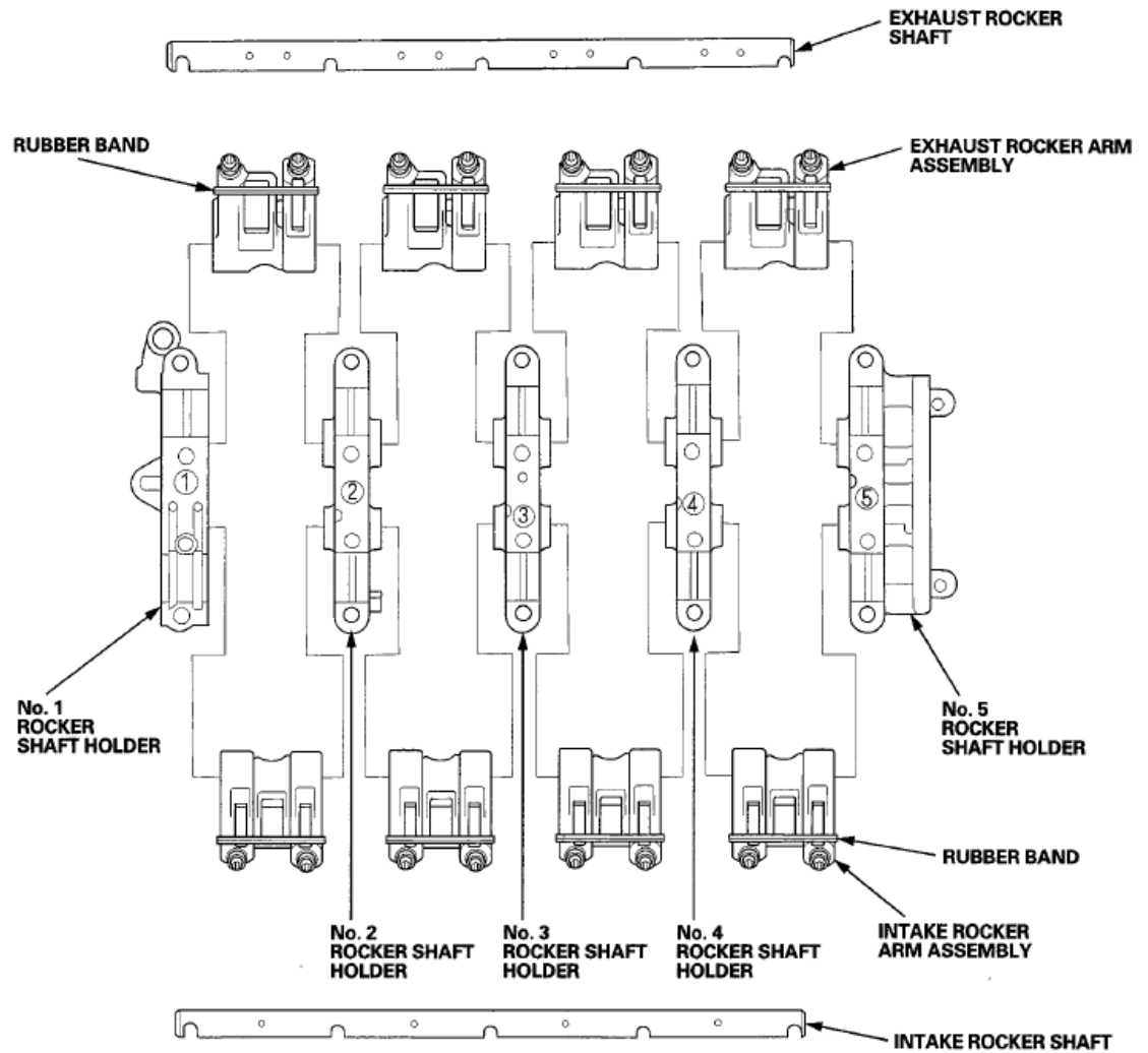
Fig. 96: Identifying Rocker Arm And Shaft Disassembly /Reassembly Courtesy of AMERICAN HONDA MOTOR CO., INC.
