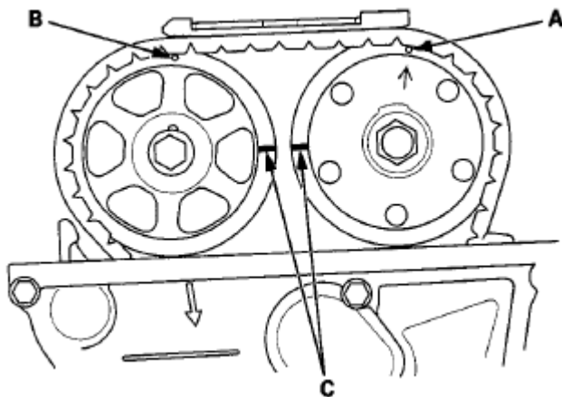
Fig. 63: Identifying TDC Punch Mark And VTC Actuator And Punch Mark
