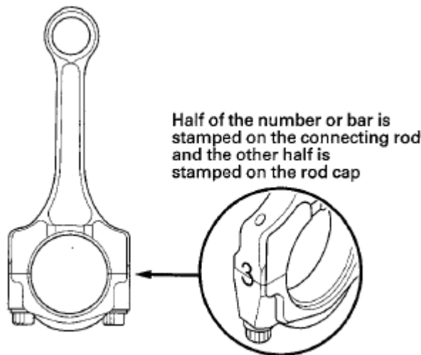
Fig. 13: Identifying Big End Bore Code Locations In Engine Courtesy of AMERICAN HONDA MOTOR CO., INC.
