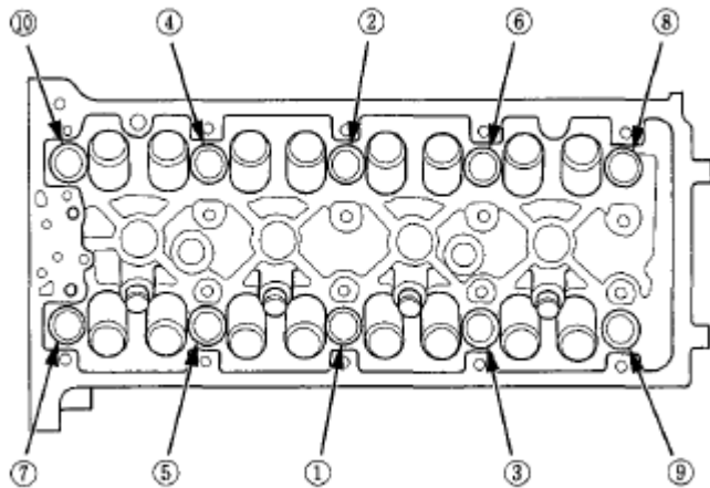
Fig. 133: Identifying Cylinder Head Bolts Tightening Sequence Courtesy of AMERICAN HONDA MOTOR CO., INC.
