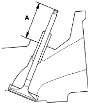
Fig. 121: Identifying Intake/Exhaust Valve Stem Height Courtesy of AMERICAN HONDA MOTOR CO., INC.
