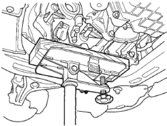
Fig. 21: Lifting Transmission Using Transmission Jack Courtesy of AMERICAN HONDA MOTOR CO., INC.
