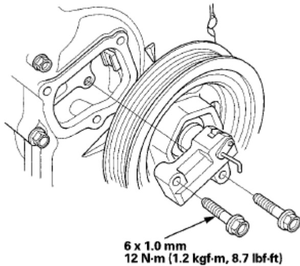
Fig. 57: Identifying Auto-Tensioner Cam Position With Torque Specifications Courtesy of AMERICAN HONDA MOTOR CO., INC.
