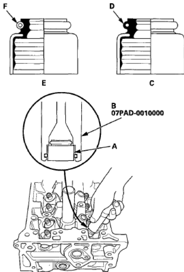
Fig. 122: Installing Exhaust Valve Seal, Valve Seals, Stem Seal Driver And White Or Silver Spring Courtesy of AMERICAN HONDA MOTOR CO., INC.
