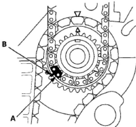
Fig. 39: Identifying Colored Link Plate And Timing Mark Courtesy of AMERICAN HONDA MOTOR CO., INC.
