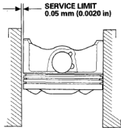
Fig. 37: Identifying Piston To Cylinder Bore Clearance Courtesy of AMERICAN HONDA MOTOR CO., INC.
