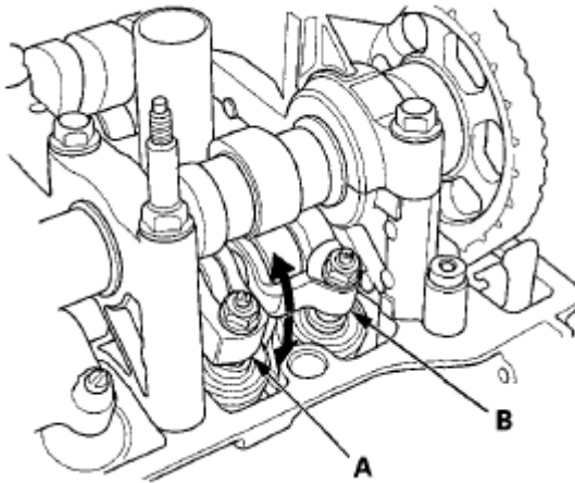
Fig. 10: Identifying Exhaust Secondary Rocker Arm And Exhaust Primary Rocker Arm Courtesy of AMERICAN HONDA MOTOR CO., INC.
