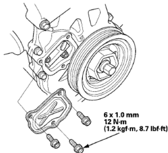
Fig. 60: Identifying Chain Case Cover With Torque Specifications Courtesy of AMERICAN HONDA MOTOR CO., INC.
