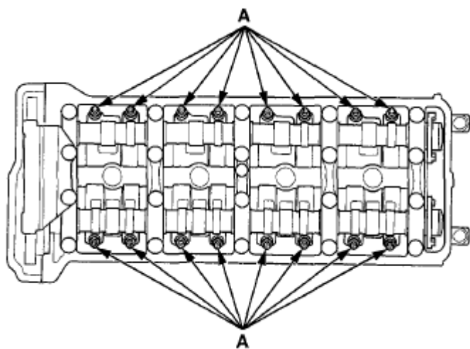
Fig. 92: Identifying Locknuts With Arm Adjusting Screws
