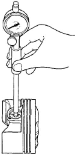
Fig. 44: Checking Between Piston Pin Diameter And Piston Pin Hole Diameter Courtesy of AMERICAN HONDA MOTOR CO., INC.
