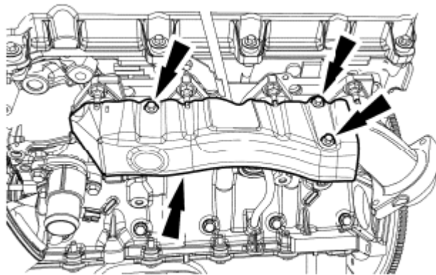
Fig. 539: Locating LH Exhaust Manifold Heat Shield Courtesy of FORD MOTOR CO.
