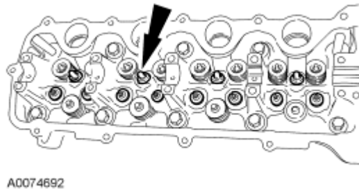
Fig. 537: Locating Hydraulic Lash Adjusters Courtesy of FORD MOTOR CO.
