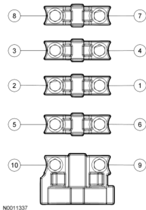
Fig. 548: Identifying Camshaft Bearing Cap Bolt In Sequence Courtesy of FORD MOTOR CO.
