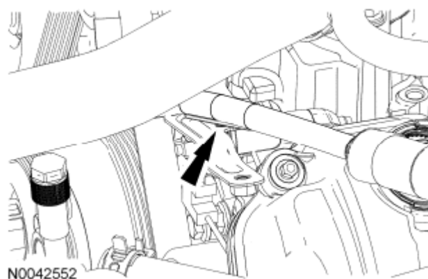
Fig. 222: Locating Wiring Harness Retainer From Cooling Fan Wiring Harness Bracket
