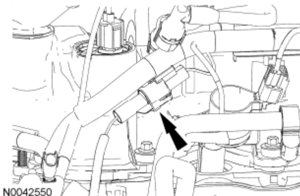
Fig. 529: Locating Electrical Connector
