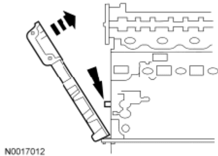
Fig. 43: Positioning Engine Front Cover Onto Dowels Courtesy of FORD MOTOR CO.
