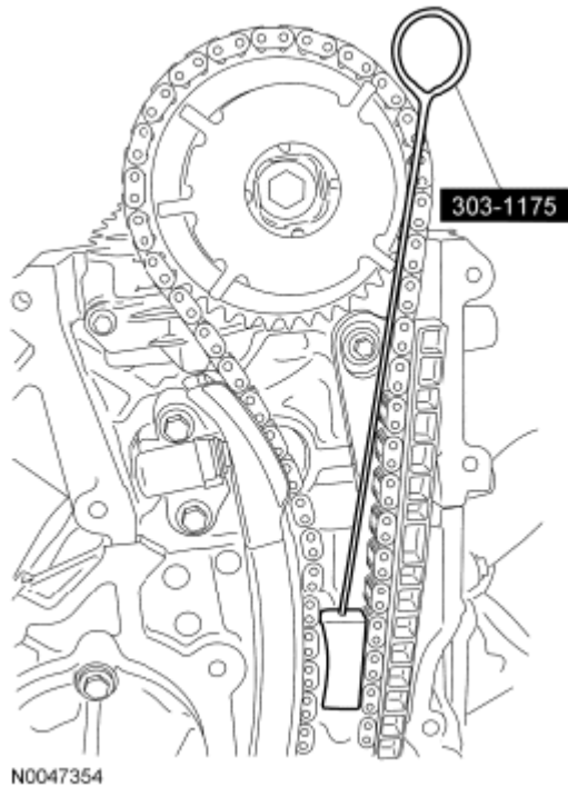
Fig. 98: Identifying Timing Chain Locking Tool Courtesy of FORD MOTOR CO.
