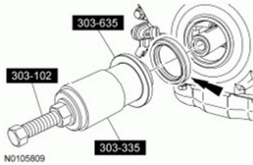
Fig. 24: Identifying Crankshaft Vibration Damper Installer, Front Cover Seal Installer And Crankshaft Front Seal Installer Courtesy of FORD MOTOR CO.
