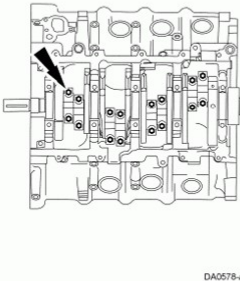
Fig. 383: Locating Connecting Rod Caps And Bolts Courtesy of FORD MOTOR CO.
