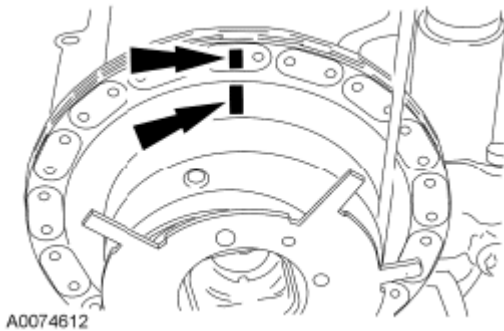
Fig. 145: Locating Mark On Timing Chain And Camshaft Phaser And Sprocket Assembly Courtesy of FORD MOTOR CO.
