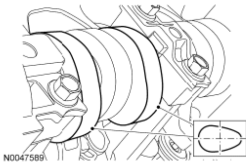
Fig. 138: Identifying No. 5 Cylinder Camshaft Exhaust Lobe
