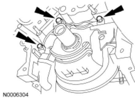
Fig. 382: Identifying Oil Pump And Bolts Courtesy of FORD MOTOR CO.
