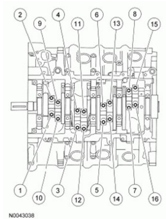
Fig. 412: Identifying Connecting Rod Cap Bolts Tightening Sequence Courtesy of FORD MOTOR CO.
