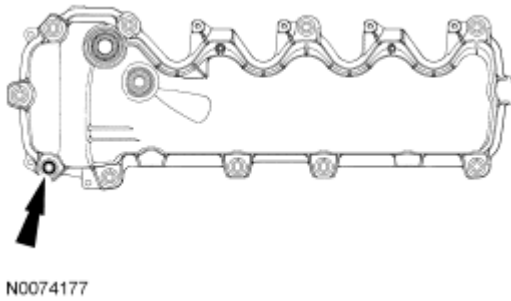
Fig. 268: Locating LH Valve Cover And Bolts Courtesy of FORD MOTOR CO.
