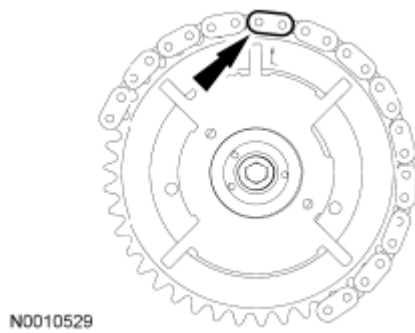
Fig. 433: Locating LH Timing Chain On Camshaft Sprocket Courtesy of FORD MOTOR CO.
