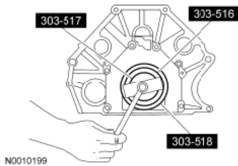
Fig. 30: Identifying Crankshaft Rear Seal Installers And Crankshaft Rear Oil Slinger Installer Courtesy of FORD MOTOR CO.
