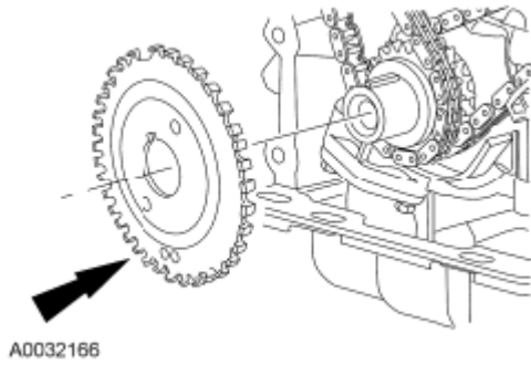
Fig. 567: Locating Crankshaft Sensor Ring Courtesy of FORD MOTOR CO.
