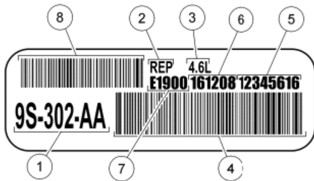
Fig. 1: Identifying Engine Code Information Label - Explorer/Mountaineer Courtesy of FORD MOTOR CO.
