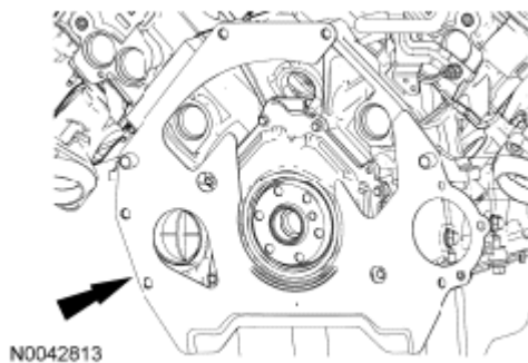
Fig. 308: Locating Spacer Plate Courtesy of FORD MOTOR CO.
