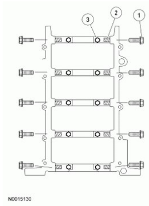
Fig. 385: Identifying Main Bearing Cap Bolts And Stud Bolt Courtesy of FORD MOTOR CO.
