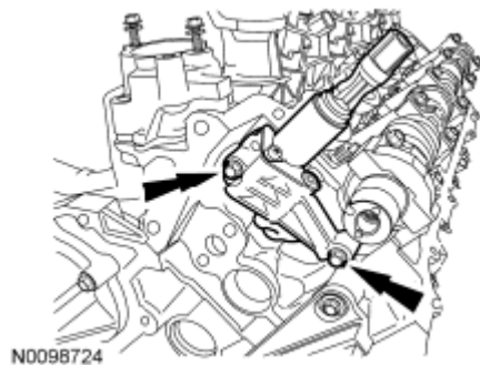
Fig. 172: Locating VCT Housing Bolts (LH) Courtesy of FORD MOTOR CO.
