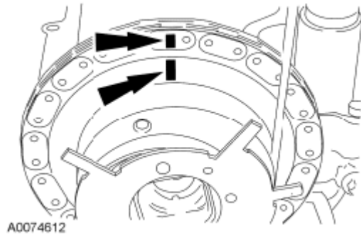
Fig. 163: Locating Mark On Timing Chain And Camshaft Phaser And Sprocket Assembly Courtesy of FORD MOTOR CO.
