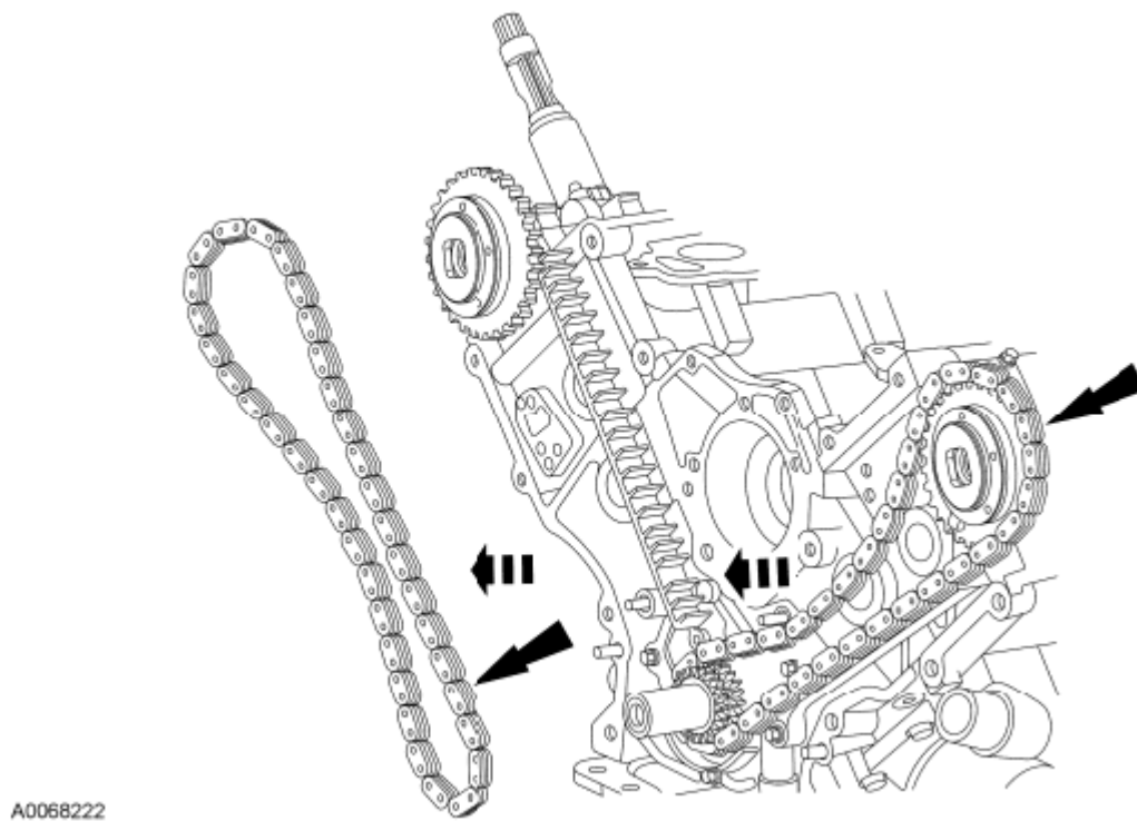
Fig. 367: Identifying RH/LH Timing Chains Courtesy of FORD MOTOR CO.
