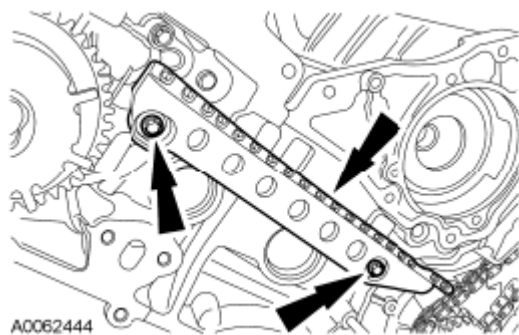
Fig. 368: Locating LH/RH Timing Chain Guides Courtesy of FORD MOTOR CO.
