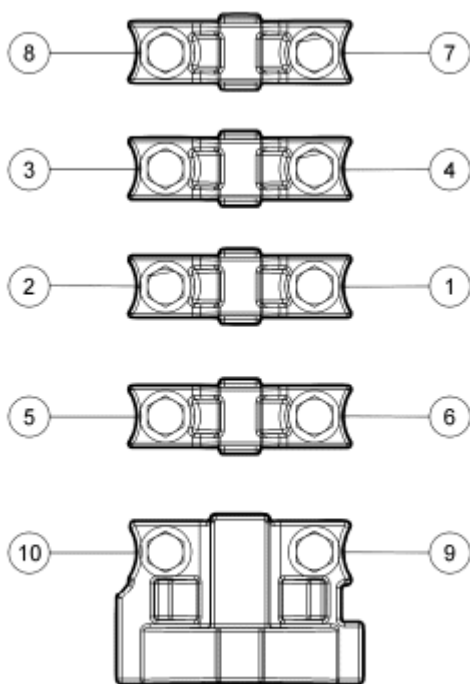
Fig. 128: Identifying Camshaft Bearing Cap Bolt In Sequence Courtesy of FORD MOTOR CO.
