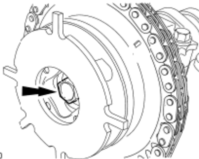
Fig. 125: Locating Camshaft Phaser And Sprocket Bolt Courtesy of FORD MOTOR CO.
