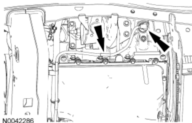
Fig. 505: Locating Block Heater Electrical Connector And Wiring Harness Retainers Courtesy of FORD MOTOR CO.
