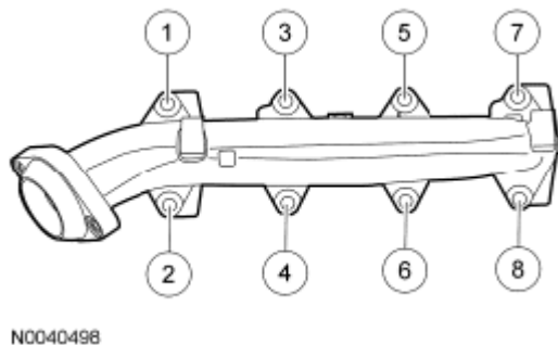
Fig. 198: Identifying RH Exhaust Manifold Nuts Tightening Sequence Courtesy of FORD MOTOR CO.
