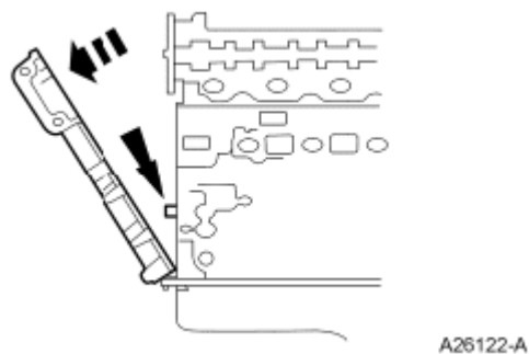
Fig. 41: Removing Engine Front Cover Gaskets Courtesy of FORD MOTOR CO.
