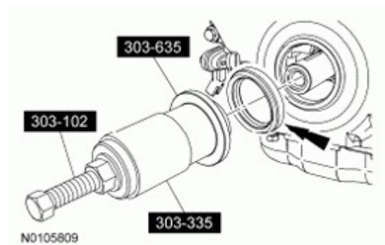
Fig. 47: Identifying Crankshaft Vibration Damper Installer, Front Cover Seal Installer And Crankshaft Front Seal Installer
