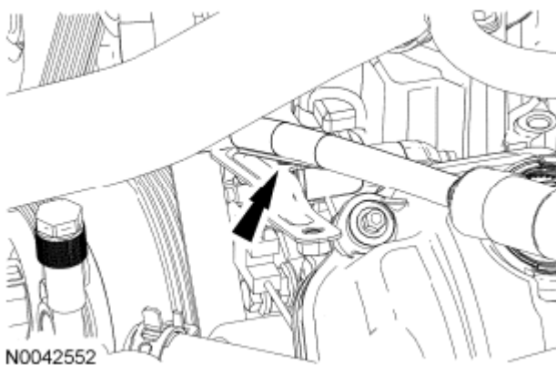
Fig. 528: Locating Wiring Harness Retainer From Cooling Fan Wiring Harness Bracket Courtesy of FORD MOTOR CO.
