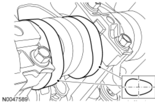
Fig. 108: Identifying No. 5 Cylinder Camshaft Exhaust Lobe Courtesy of FORD MOTOR CO.
