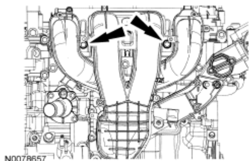
Fig. 374: Locating Intake Manifold Bolts Courtesy of FORD MOTOR CO.
