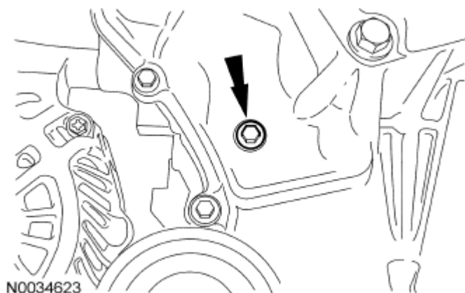
Fig. 87: Locating Front Cover Upper Timing Hole Plug Courtesy of FORD MOTOR CO.
