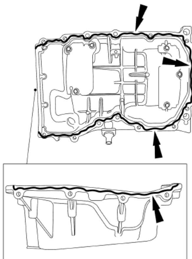
Fig. 317: Locating Oil Pan-To-Engine Front Cover Mating Surface Courtesy of FORD MOTOR CO.
