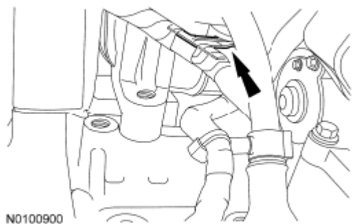
Fig. 9: Locating Engine Wiring Harness Pin-Type Retainer From Intake Manifold Courtesy of FORD MOTOR CO.
