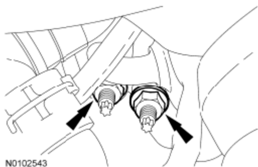
Fig. 438: Locating A/C Tube Nuts And A/C Compressor Courtesy of FORD MOTOR CO.
