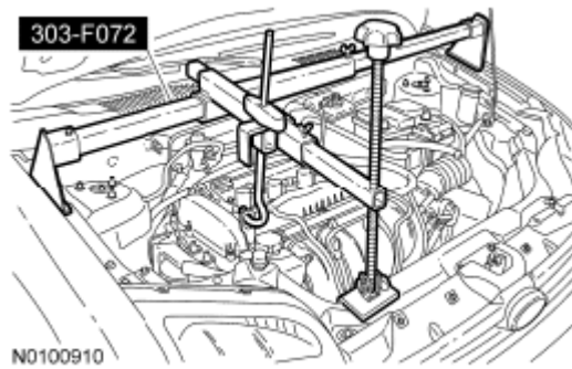
Fig. 151: Installing Engine Support Bar And Raise Courtesy of FORD MOTOR CO.
