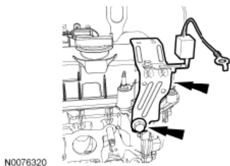
Fig. 237: Locating Radio Interference Capacitor Bracket Bolt And Bracket Aside Courtesy of FORD MOTOR CO.
