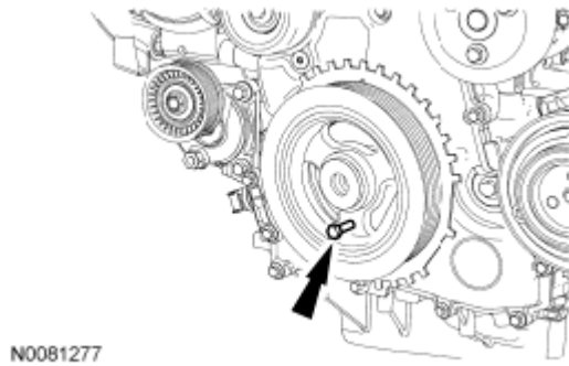
Fig. 32: Locating Crankshaft Pulley Standard Bolt Courtesy of FORD MOTOR CO.
