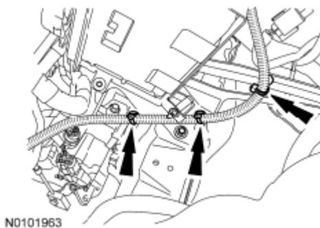
Fig. 454: Locating Positive Battery Cable Wire Harness Retainer Courtesy of FORD MOTOR CO.
