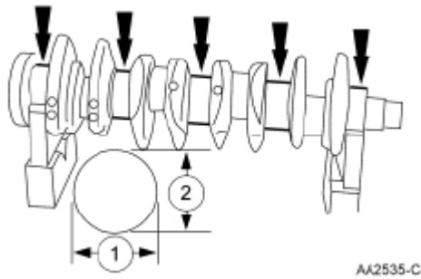
Fig. 295: Measuring Crankshaft Main Bearing Journal Diameters Courtesy of FORD MOTOR CO.
