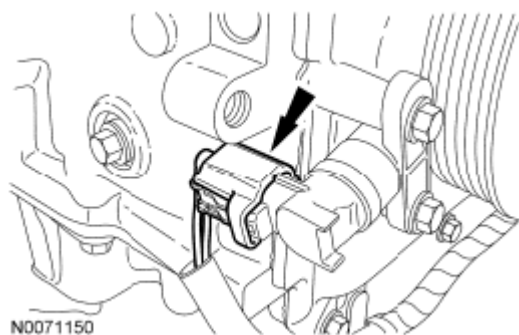
Fig. 411: Locating CKP Sensor Electrical Connector Courtesy of FORD MOTOR CO.
