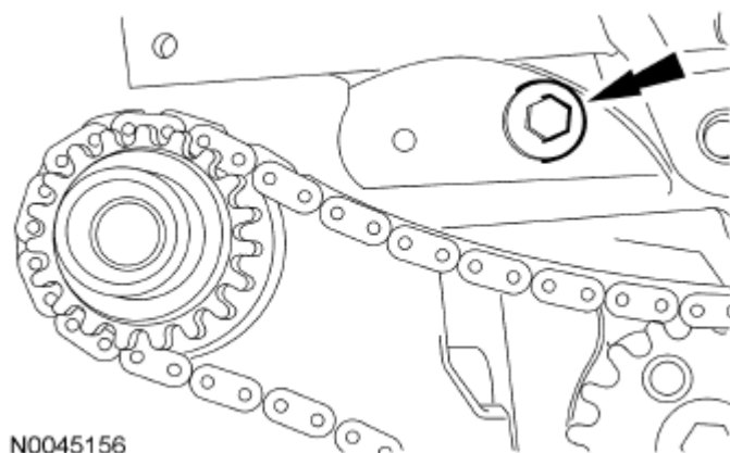
Fig. 140: Locating Oil Pump Drive Chain Tensioner Shoulder Bolt Courtesy of FORD MOTOR CO.
