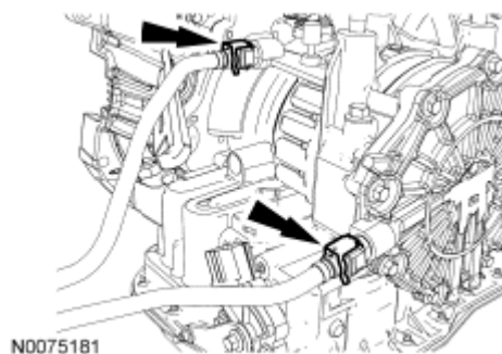
Fig. 442: Installing Secondary Latches Courtesy of FORD MOTOR CO.
