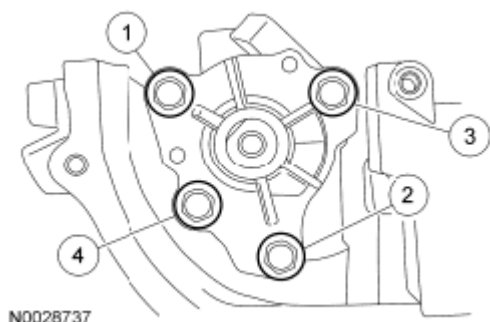
Fig. 139: Identifying Oil Pump And Cylinder Block Mating Surfaces Courtesy of FORD MOTOR CO.
