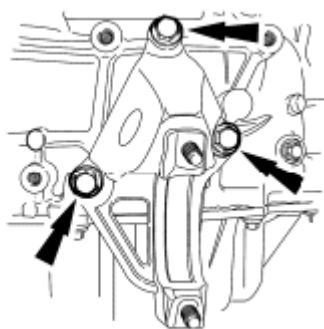
Fig. 245: Locating Intermediate Shaft Bracket And Bolts Courtesy of FORD MOTOR CO.
