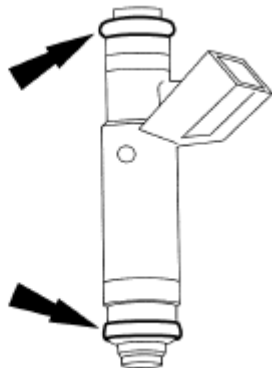
Fig. 382: Locating Fuel Injectors Onto Fuel Rail Courtesy of FORD MOTOR CO.
