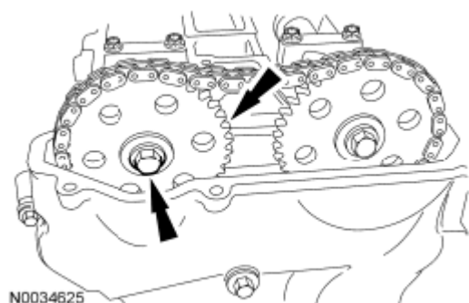
Fig. 100: Locating Exhaust Camshaft Drive Gear Bolt Courtesy of FORD MOTOR CO.
