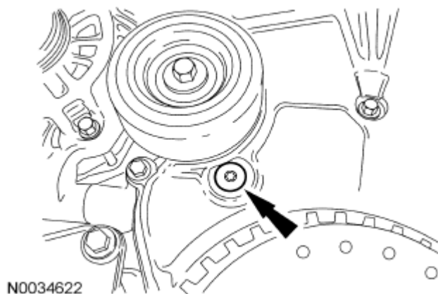
Fig. 106: Locating Front Cover Lower Timing Hole Plug Courtesy of FORD MOTOR CO.
