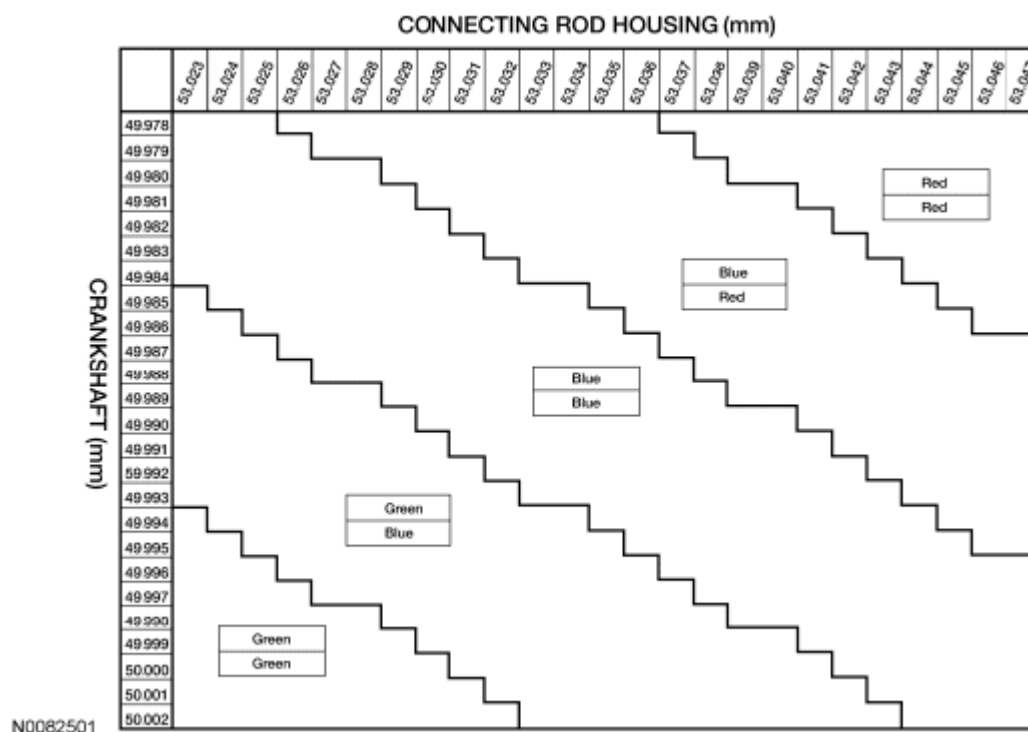
Fig. 302: Connecting Rod Housing Chart
