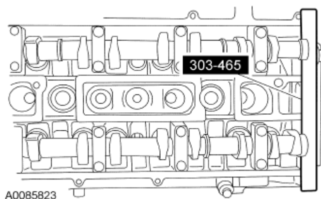
Fig. 102: Removing Camshaft Alignment Plate Courtesy of FORD MOTOR CO.
