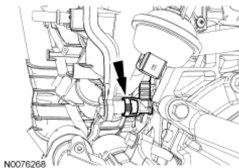
Fig. 373: Locating Intake Manifold Courtesy of FORD MOTOR CO.
