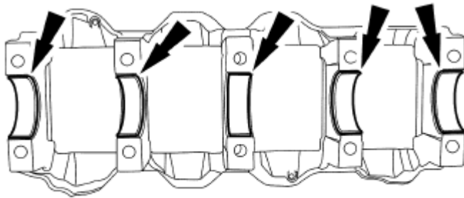
Fig. 304: Locating Main Bearings From Main Bearing Beam Courtesy of FORD MOTOR CO.
