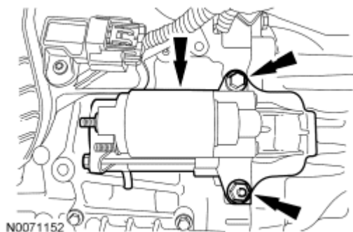
Fig. 404: Locating Lower Stud Bolt Courtesy of FORD MOTOR CO.
