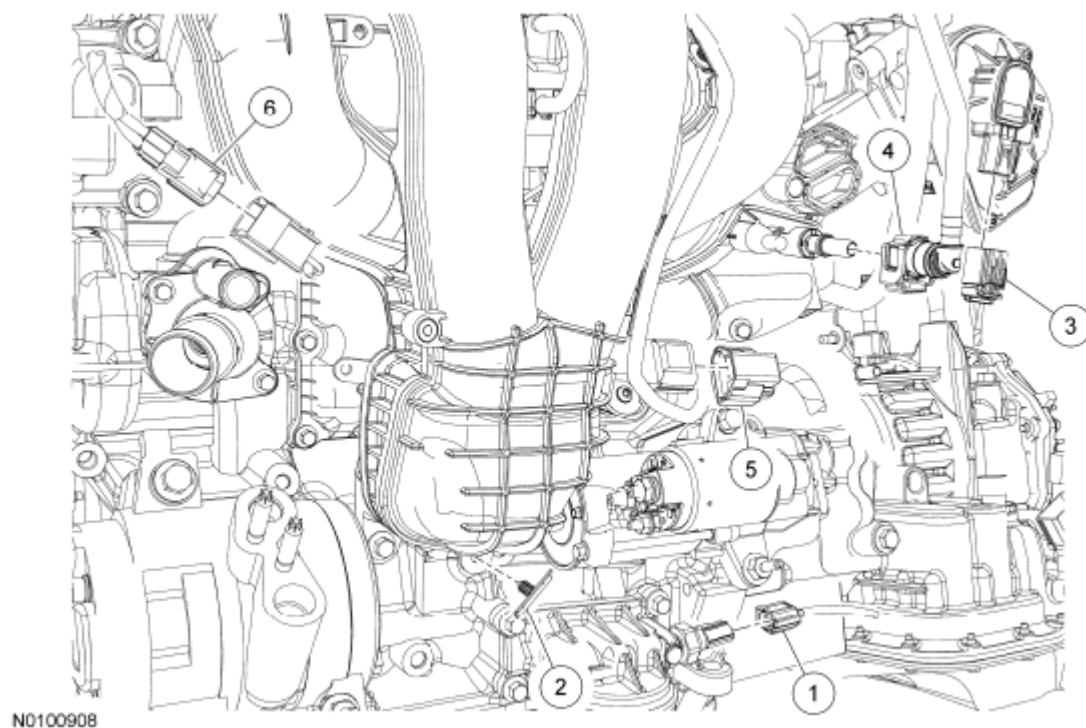
Fig. 5: Identifying Intake Manifold Components (1 Of 3) Courtesy of FORD MOTOR CO.
