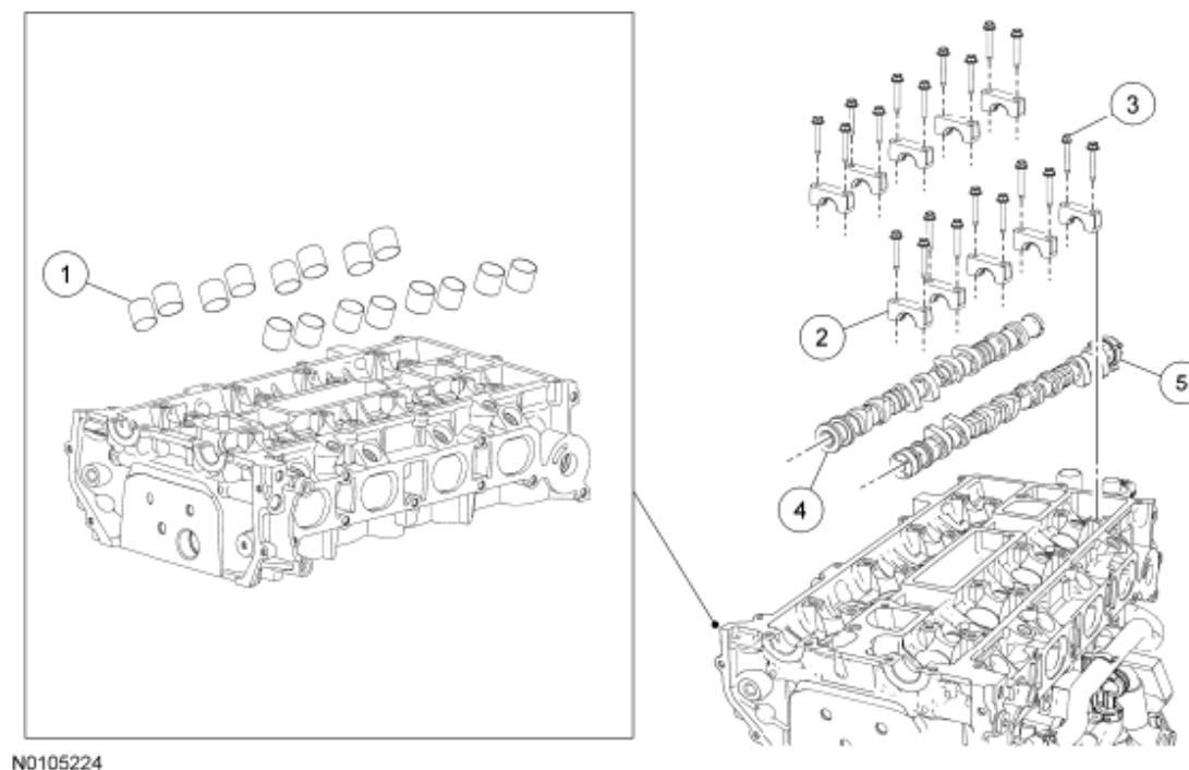
Fig. 116: Identifying Cylinder Head Components (1 Of 2) Courtesy of FORD MOTOR CO.
