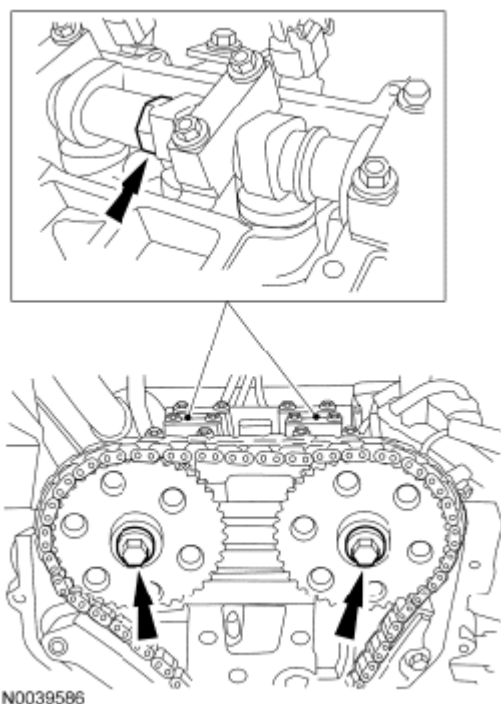
Fig. 340: Locating Camshaft Drive Gear Bolts Courtesy of FORD MOTOR CO.
