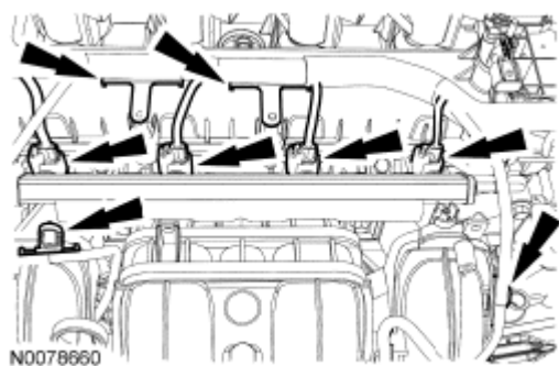
Fig. 225: Locating Wiring Harness Retainers From Valve Cover Stud Bolts Courtesy of FORD MOTOR CO.
