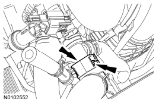
Fig. 431: Locating Coolant Degas Bottle Hose And Retaining Clip Courtesy of FORD MOTOR CO.
