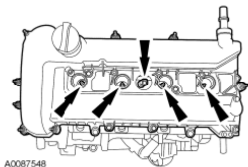
Fig. 361: Locating Spark Plugs And CHT Sensor Courtesy of FORD MOTOR CO.
