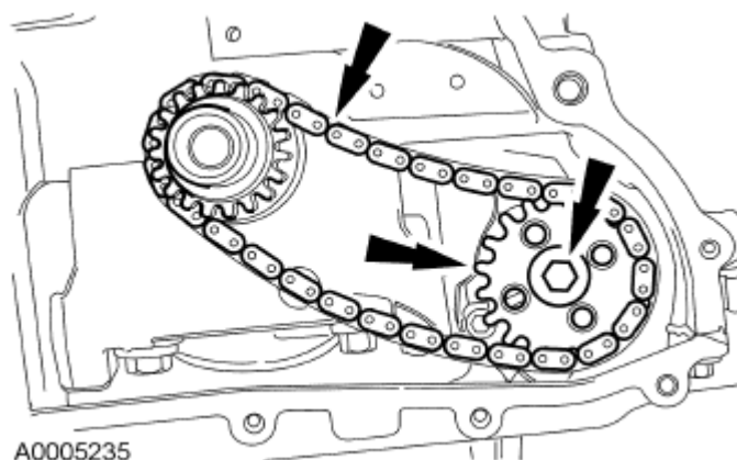
Fig. 327: Locating Oil Pump Chain, Sprocket And Bolt Courtesy of FORD MOTOR CO.
