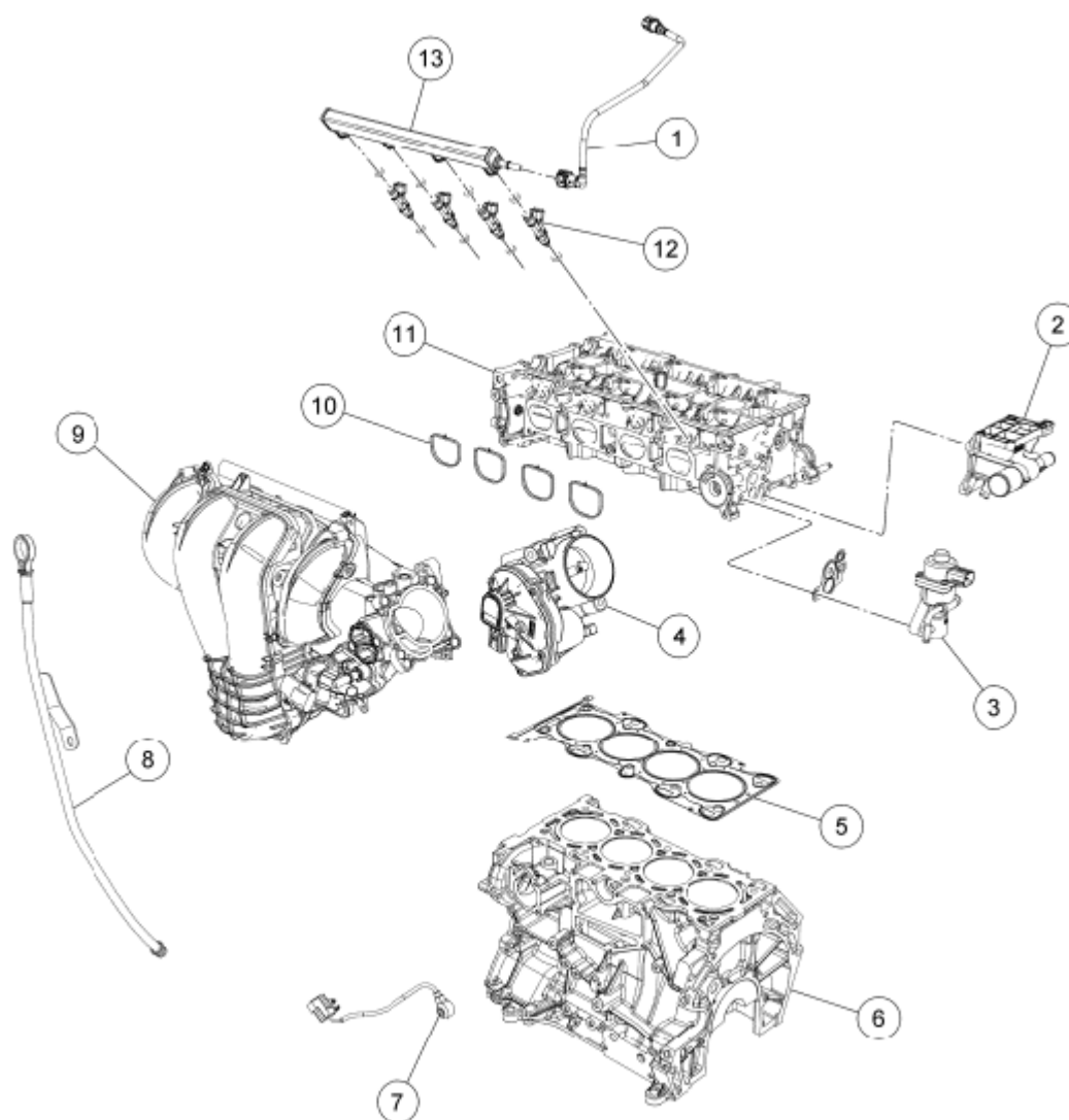
Fig. 293: Identifying Intake Manifold Components Courtesy of FORD MOTOR CO.
