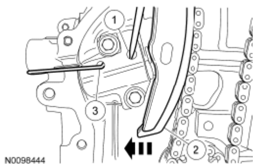
Fig. 65: Inserting Paper Clip Into Hole To Retain Tensioner Courtesy of FORD MOTOR CO.
