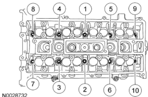
Fig. 123: Identifying Cylinder Head Bolts Tightening Sequence Courtesy of FORD MOTOR CO.
