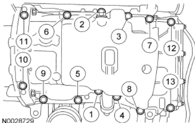
Fig. 320: Identifying Oil Pan Bolts Tightening Sequence Courtesy of FORD MOTOR CO.
