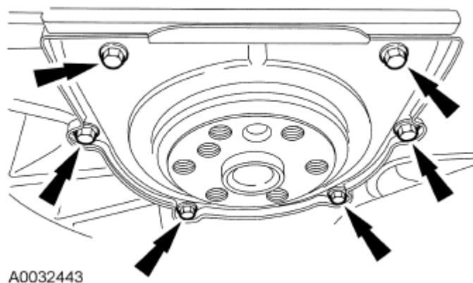
Fig. 270: Locating Crankshaft Rear Seal, Retainer Plate And Bolts Courtesy of FORD MOTOR CO.
