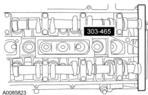
Fig. 41: Removing Camshaft Alignment Plate Courtesy of FORD MOTOR CO.
