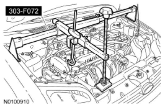
Fig. 124: Installing Engine Support Bar And Raise Courtesy of FORD MOTOR CO.
