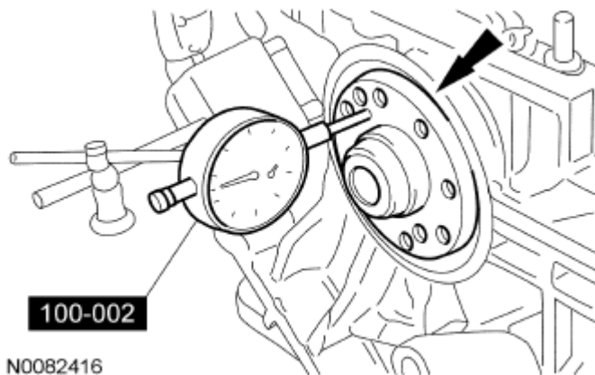
Fig. 309: Measuring Crankshaft End Play Courtesy of FORD MOTOR CO.
