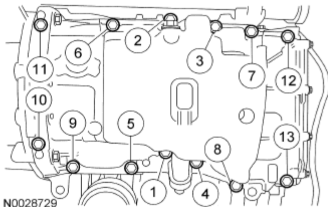
Fig. 144: Identifying Oil Pan Bolts Tightening Sequence Courtesy of FORD MOTOR CO.
