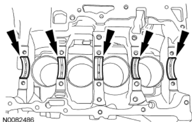
Fig. 278: Locating Main Bearings Courtesy of FORD MOTOR CO.
