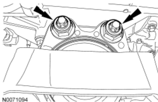
Fig. 188: Locating Engine Mount Nuts Courtesy of FORD MOTOR CO.
