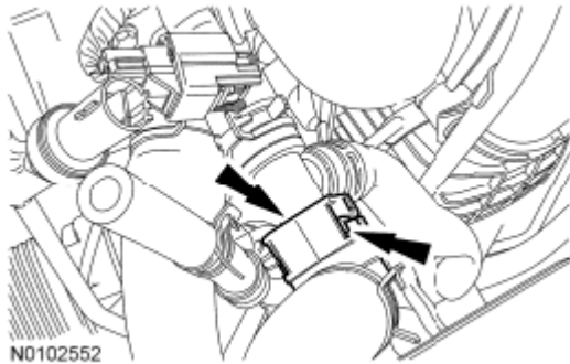
Fig. 179: Locating Coolant Degas Bottle Hose And Retaining Clip Courtesy of FORD MOTOR CO.
