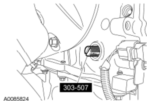
Fig. 348: Removing Crankshaft TDC Timing Peg Courtesy of FORD MOTOR CO.
