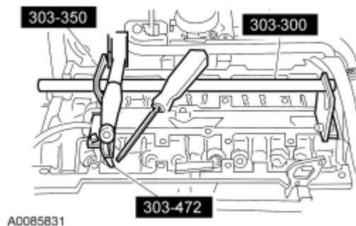
Fig. 109: Removing Valve Spring Retainer And Valve Spring Courtesy of FORD MOTOR CO.
