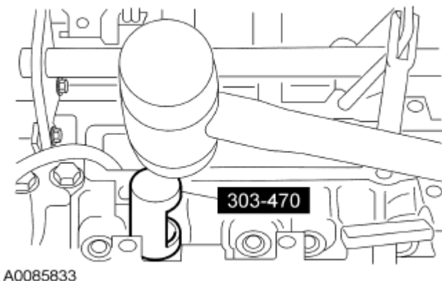
Fig. 284: Installing Valve Seals Onto Cylinder Head Valve Guides Courtesy of FORD MOTOR CO.
