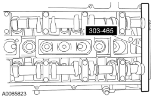
Fig. 27: Installing Camshaft Alignment Plate Courtesy of FORD MOTOR CO.
