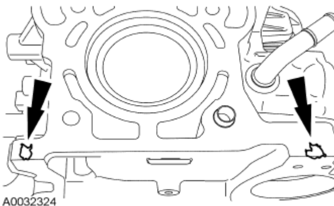
Fig. 322: Locating Cylinder Head Sealant Location Courtesy of FORD MOTOR CO.
