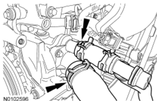
Fig. 394: Locating Oil Cooler Hose And Lower Radiator Hose Courtesy of FORD MOTOR CO.
