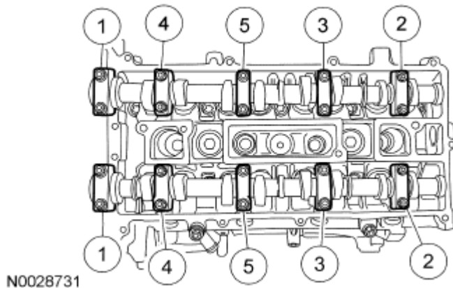
Fig. 121: Identifying Camshaft Bearing Caps Bolts Loosening Sequence Courtesy of FORD MOTOR CO.
