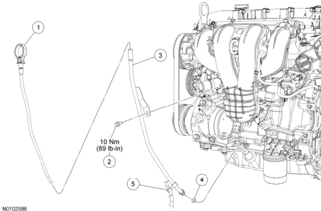
Fig. 145: Identifying Oil Level Indicator And Tube With Torque Specifications Courtesy of FORD MOTOR CO.
