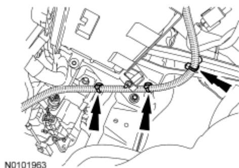
Fig. 155: Detaching Positive Battery Cable Wire Harness Retainers Courtesy of FORD MOTOR CO.
