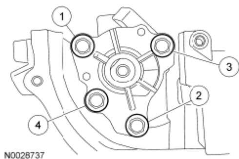
Fig. 313: Identifying Oil Pump And Cylinder Block Mating Surfaces Courtesy of FORD MOTOR CO.
