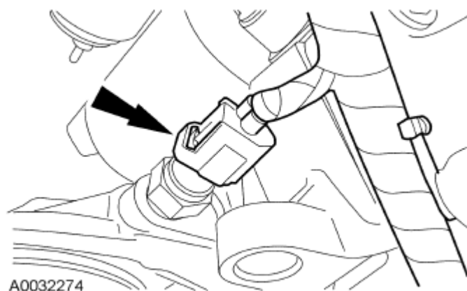
Fig. 392: Locating Engine Oil Pressure Switch Electrical Connector Courtesy of FORD MOTOR CO.
