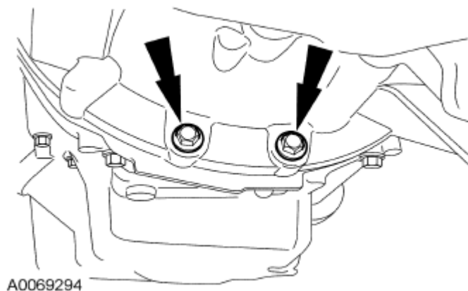
Fig. 185: Locating Lower Bellhousing-To-Oil Pan Bolts Courtesy of FORD MOTOR CO.
