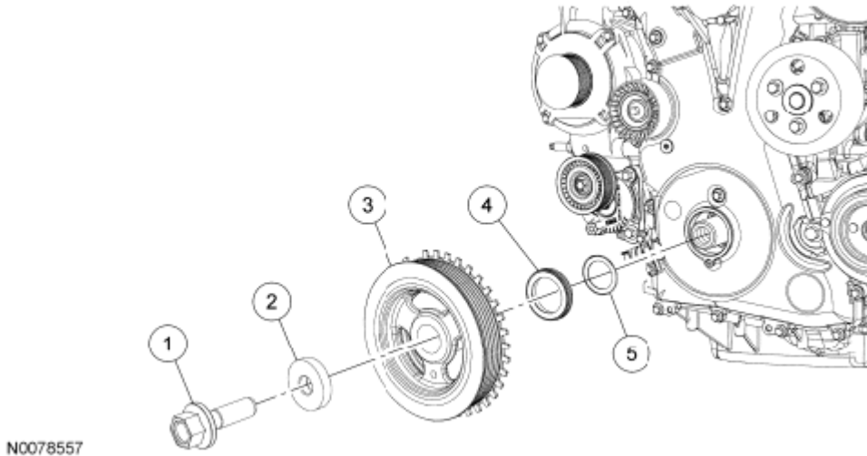
Fig. 24: Identifying Crankshaft Pulley And Crankshaft Front Seal Courtesy of FORD MOTOR CO.
