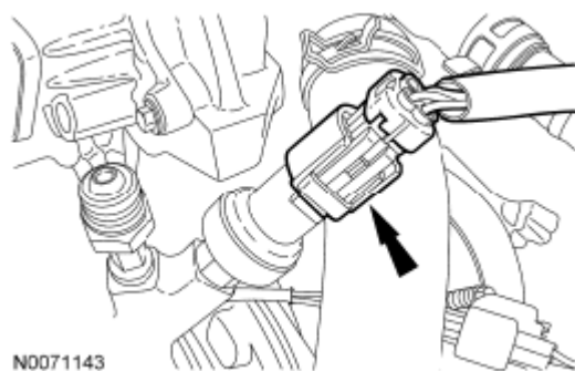
Fig. 414: Locating Power Steering Pressure Switch Electrical Connector Courtesy of FORD MOTOR CO.
