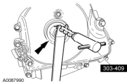
Fig. 254: Removing Crankshaft Front Seal Courtesy of FORD MOTOR CO.
