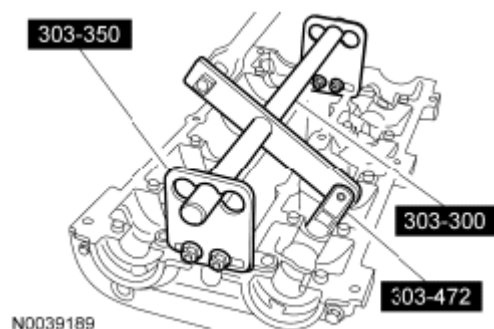
Fig. 285: Installing Valve Spring Collets, Valve Spring Retainers And Valve Springs Courtesy of FORD MOTOR CO.
