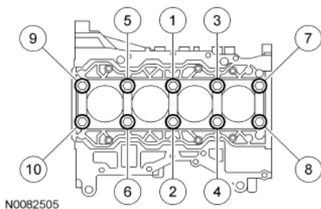
Fig. 297: Identifying Bearing Beam Bolts Tightening Sequence Courtesy of FORD MOTOR CO.
