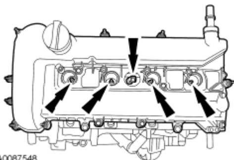
Fig. 247: Locating Spark Plugs And CHT Sensor Courtesy of FORD MOTOR CO.
