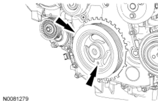
Fig. 31: Locating Crankshaft Pulley Courtesy of FORD MOTOR CO.
