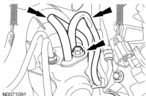
Fig. 177: Locating Power Steering Tube O-Ring Seals Courtesy of FORD MOTOR CO.
