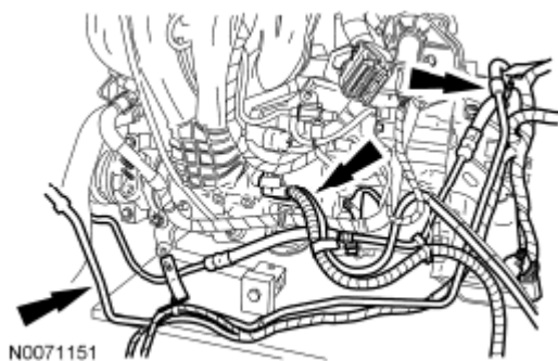
Fig. 205: Locating Power Steering Tubes And Wiring Harness Courtesy of FORD MOTOR CO.
