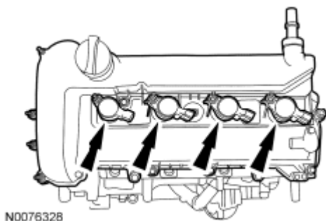
Fig. 362: Locating Ignition Coil-On-Plugs And Bolts Courtesy of FORD MOTOR CO.
