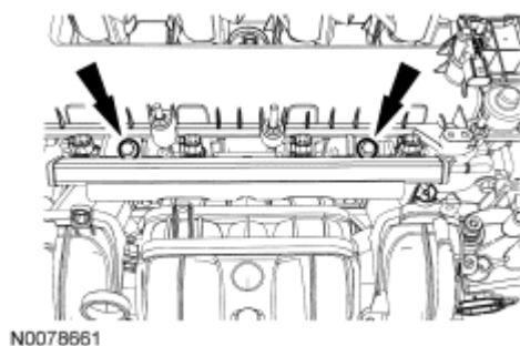
Fig. 226: Locating Fuel Injectors And Bolts Courtesy of FORD MOTOR CO.
