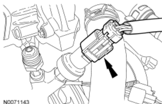
Fig. 197: Locating Power Steering Pressure Switch Electrical Connector Courtesy of FORD MOTOR CO.
