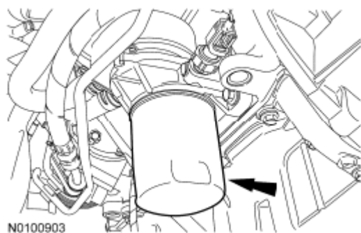
Fig. 118: Removing Engine Oil Filter Courtesy of FORD MOTOR CO.
