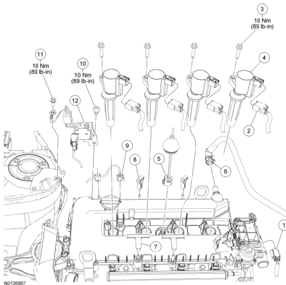
Fig. 19: Exploded View Of Valve Cover With Torque Specifications (1 Of 2) Courtesy of FORD MOTOR CO.
