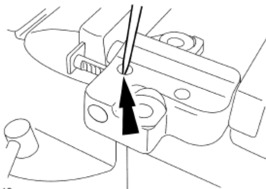
Fig. 336: Pushing Ratchet Mechanism Courtesy of FORD MOTOR CO.
