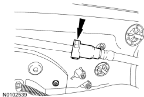
Fig. 452: Locating Fuel Tube Quick Connect Coupling Courtesy of FORD MOTOR CO.
