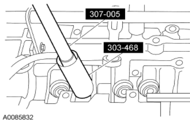
Fig. 112: Removing Valve Seal Courtesy of FORD MOTOR CO.
