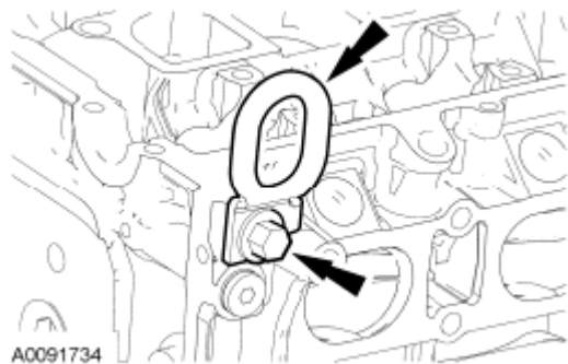
Fig. 281: Locating Lifting Eyes And Bolts Courtesy of FORD MOTOR CO.
