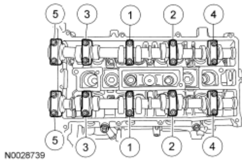
Fig. 325: Identifying Bearing Caps Tightening Sequence Courtesy of FORD MOTOR CO.
