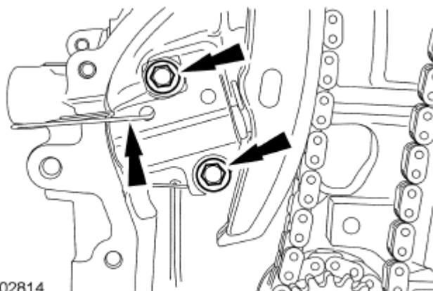
Fig. 79: Locating Timing Chain Tensioner And Bolts Courtesy of FORD MOTOR CO.
