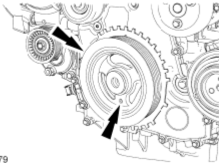
Fig. 344: Locating Crankshaft Pulley Courtesy of FORD MOTOR CO.
