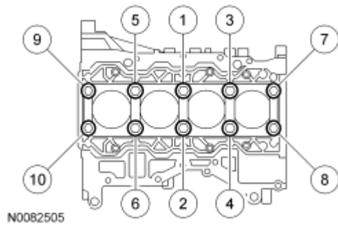
Fig. 308: Identifying Main Bearing Beam Bolts Tightening Sequence Courtesy of FORD MOTOR CO.
