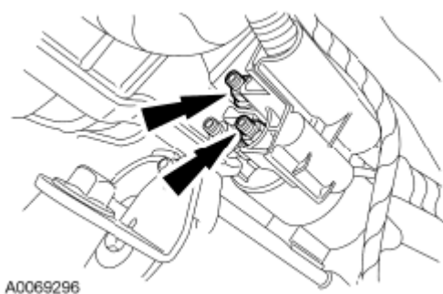
Fig. 405: Locating Starter Motor Electrical Terminals Courtesy of FORD MOTOR CO.
