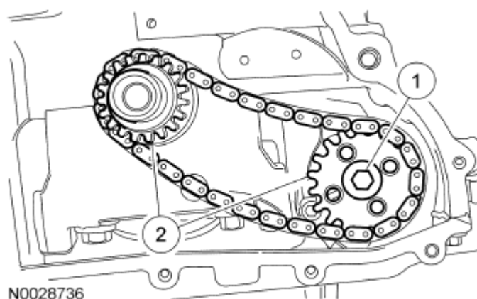
Fig. 264: Locating Chain And Sprockets Courtesy of FORD MOTOR CO.
