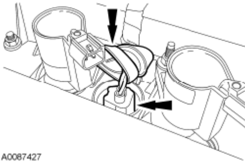
Fig. 223: Locating Rubber Boot Aside And Cylinder Head Temperature Sensor Electrical Connector Courtesy of FORD MOTOR CO.
