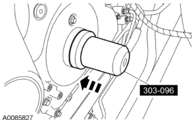
Fig. 343: Installing Crankshaft Front Oil Seal Courtesy of FORD MOTOR CO.
