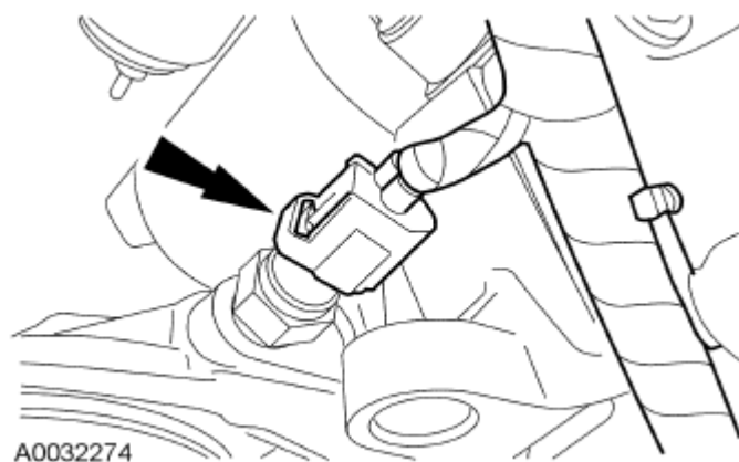
Fig. 218: Locating Engine Oil Pressure Switch Electrical Connector Courtesy of FORD MOTOR CO.
