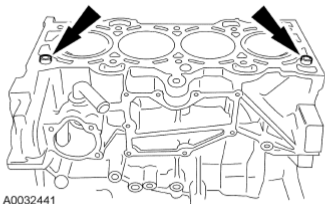
Fig. 268: Locating Cylinder Head Alignment Dowels Courtesy of FORD MOTOR CO.
