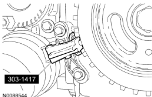
Fig. 355: Adjusting CKP Sensor Courtesy of FORD MOTOR CO.
