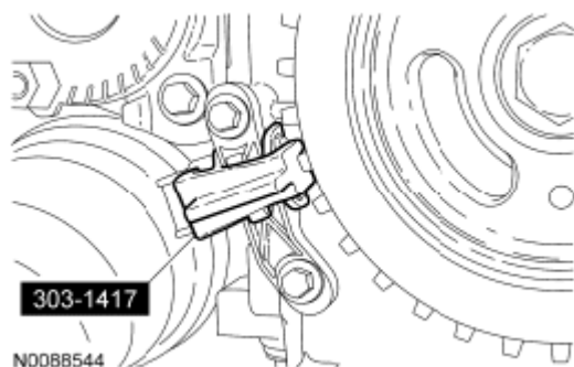
Fig. 62: Adjusting CKP Sensor Courtesy of FORD MOTOR CO.
