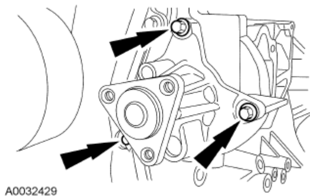
Fig. 215: Locating Coolant Pump And Bolts Courtesy of FORD MOTOR CO.
