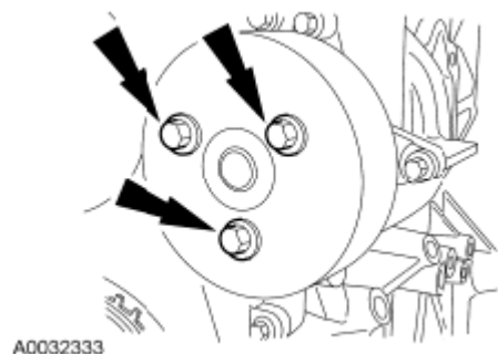
Fig. 396: Locating Coolant Pump Pulley And Bolts Courtesy of FORD MOTOR CO.
