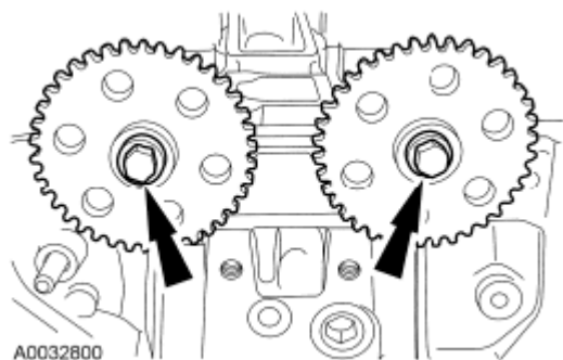
Fig. 331: Locating Camshaft Drive Gears And Bolts Courtesy of FORD MOTOR CO.
