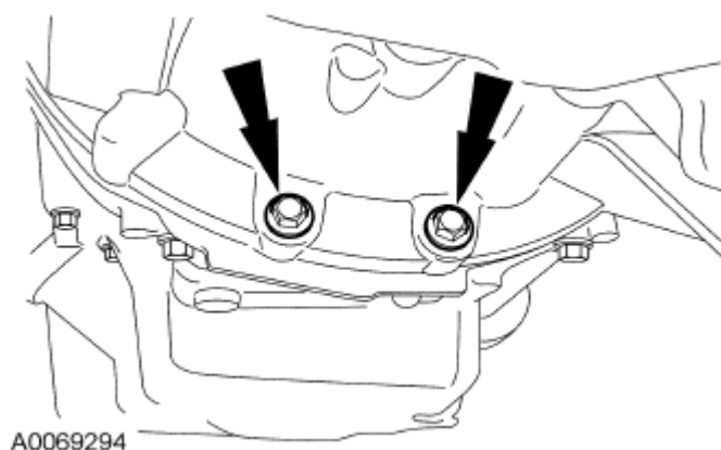
Fig. 425: Locating Lower Bellhousing-To-Oil Pan Bolts Courtesy of FORD MOTOR CO.
