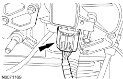
Fig. 380: Locating Throttle Control Electrical Connector Courtesy of FORD MOTOR CO.
