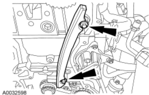
Fig. 72: Locating LH Timing Chain Guide And Bolts Courtesy of FORD MOTOR CO.
