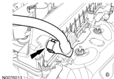
Fig. 456: Locating Crankcase Vent Tube From Valve Cover Courtesy of FORD MOTOR CO.
