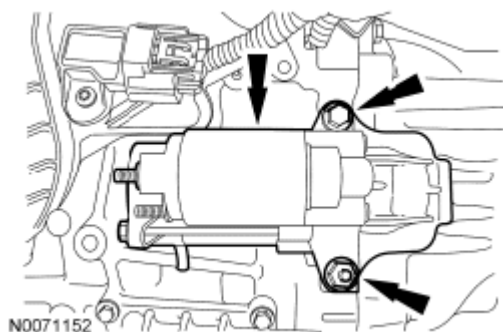
Fig. 207: Locating Stud Bolt, Starter And Bolt Courtesy of FORD MOTOR CO.
