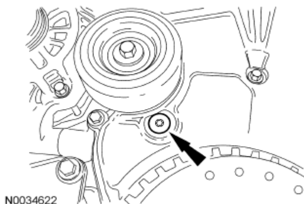
Fig. 86: Locating Front Cover Lower Timing Hole Plug Courtesy of FORD MOTOR CO.
