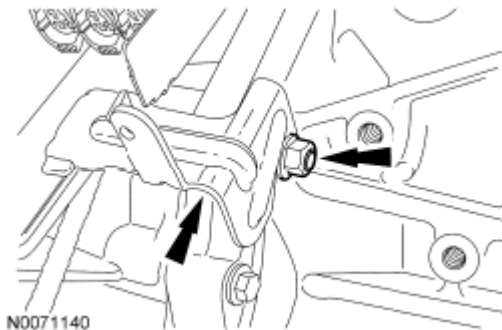
Fig. 192: Locating HO2S And CMS Wire Connector Bracket Aside Courtesy of FORD MOTOR CO.
