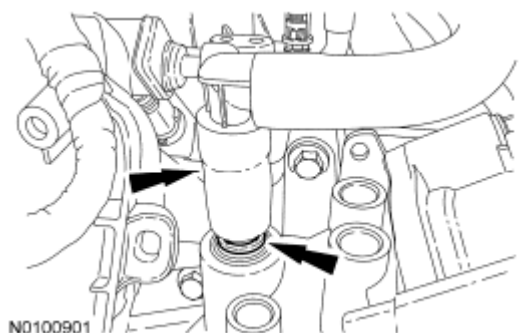
Fig. 450: Locating Quick Release Locking Ring Courtesy of FORD MOTOR CO.
