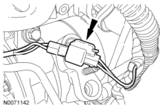
Fig. 196: Locating A/C Compressor Electrical Connector Courtesy of FORD MOTOR CO.
