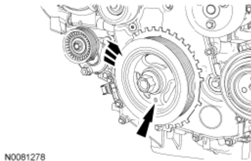
Fig. 26: Turning Crankshaft Clockwise To Position No. 1 Piston Courtesy of FORD MOTOR CO.
