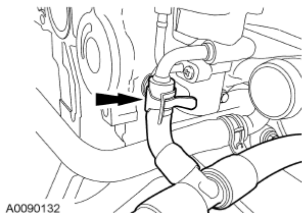
Fig. 217: Locating EGR Valve Coolant Hose Courtesy of FORD MOTOR CO.
