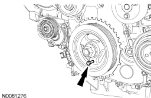
Fig. 42: Locating Crankshaft Pulley Bolt Courtesy of FORD MOTOR CO.
