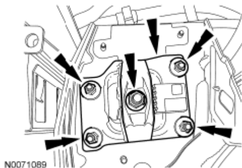
Fig. 421: Locating Transaxle Mount Nuts And Transaxle Mount Plate Courtesy of FORD MOTOR CO.
