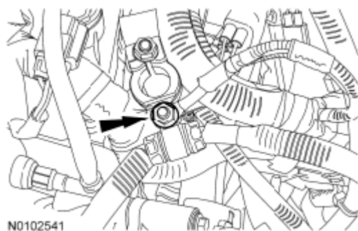
Fig. 162: Locating Negative Battery Terminal Nut Courtesy of FORD MOTOR CO.
