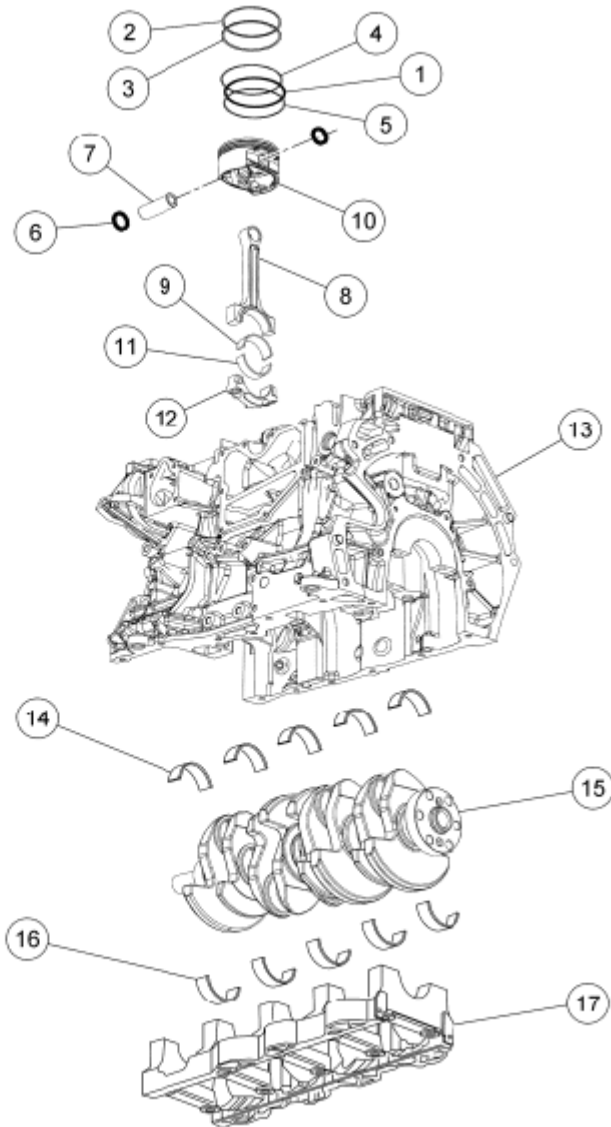
Fig. 290: Identifying Lower Engine Block Components (2 Of 3) Courtesy of FORD MOTOR CO.
