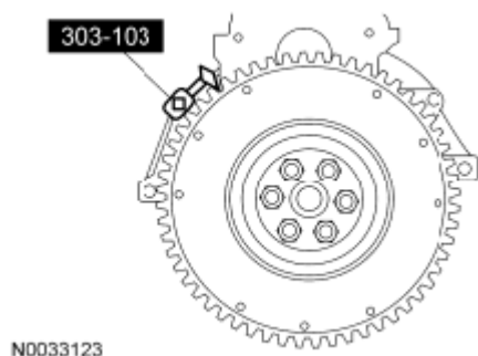
Fig. 46: Installing Flywheel Holding Tool Courtesy of FORD MOTOR CO.
