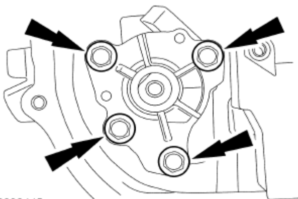
Fig. 272: Locating Oil Pump And Bolts Courtesy of FORD MOTOR CO.
