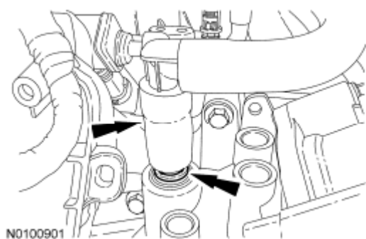
Fig. 16: Locating Quick Release Locking Ring Courtesy of FORD MOTOR CO.
