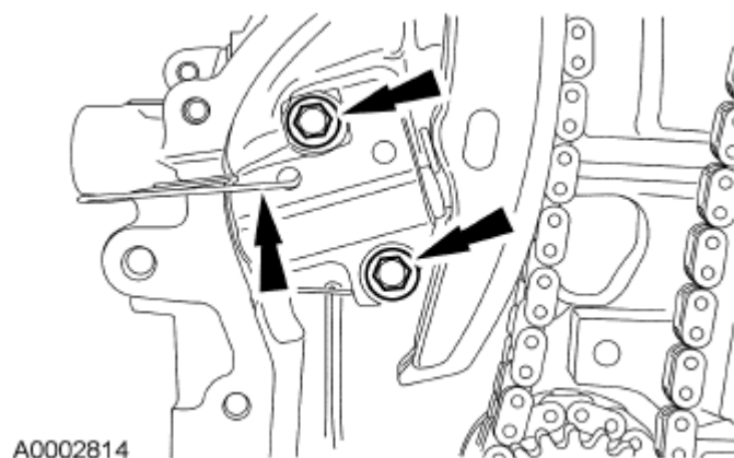
Fig. 339: Locating Timing Chain Tensioner And Bolts Courtesy of FORD MOTOR CO.
