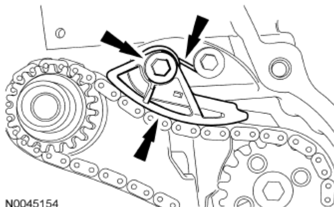
Fig. 141: Locating Oil Pump Chain Tensioner And Bolt Courtesy of FORD MOTOR CO.
