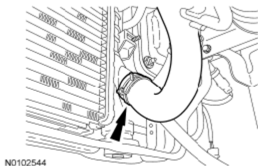
Fig. 173: Locating A/C Tubes From Compressor Courtesy of FORD MOTOR CO.
