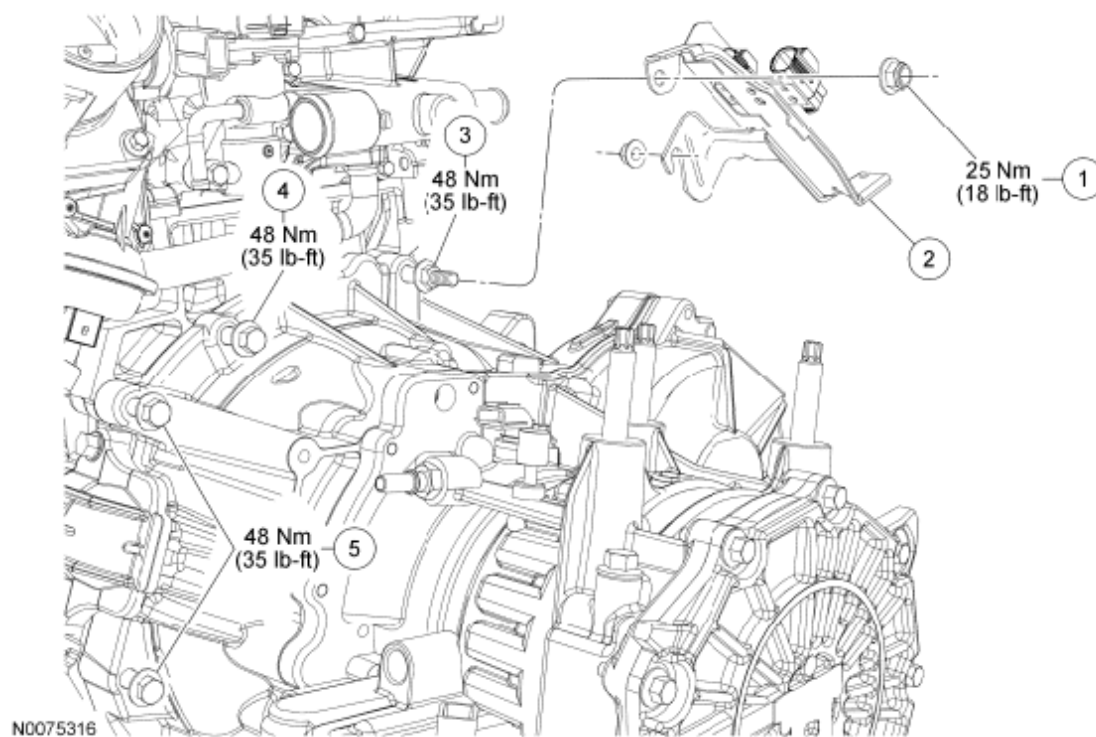
Fig. 130: Identifying Oil Pan Bolts With Tightening Sequence Courtesy of FORD MOTOR CO.
