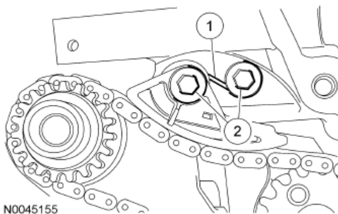
Fig. 263: Identifying Tensioner And Shoulder Bolts Courtesy of FORD MOTOR CO.
