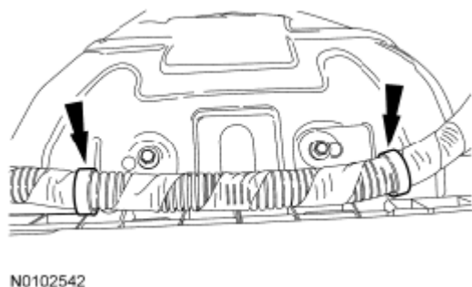
Fig. 439: Locating Battery Cable Wire Harness Retainers And Valve Cover Stud Bolts Courtesy of FORD MOTOR CO.
