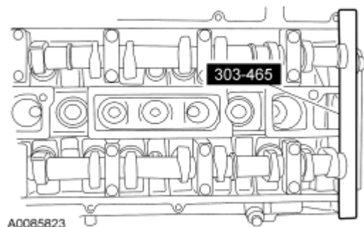
Fig. 330: Installing Camshaft Alignment Plate Courtesy of FORD MOTOR CO.
