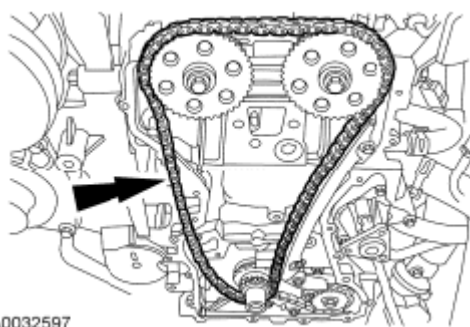
Fig. 68: Locating Timing Chain Courtesy of FORD MOTOR CO.
