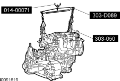
Fig. 400: Identifying Engine Lifting Bracket And Spreader Bar Courtesy of FORD MOTOR CO.
