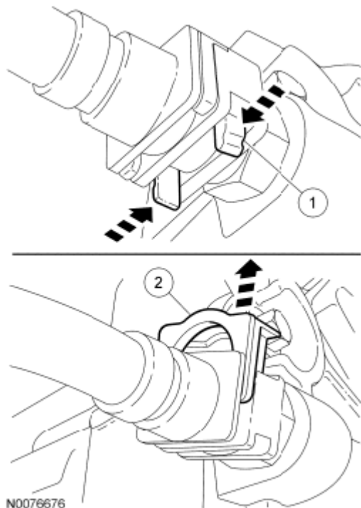
Fig. 168: Removing Transaxle Fluid Cooler Tubes From Transaxle Courtesy of FORD MOTOR CO.
