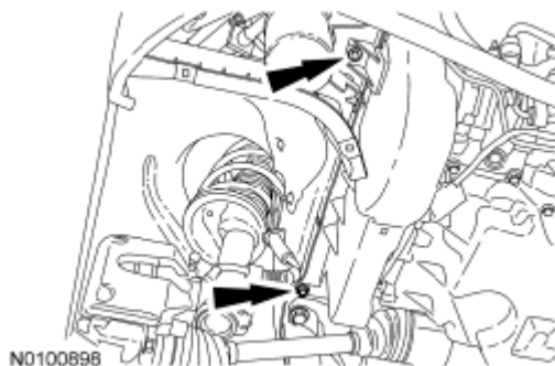
Fig. 3: Locating Accessory Drive Belt Splash Shield And Bolts Courtesy of FORD MOTOR CO.
