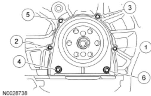
Fig. 316: Identifying Crankshaft Rear Seal Bolts Tightening Sequence Courtesy of FORD MOTOR CO.
