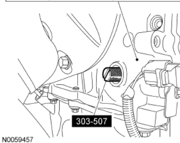
Fig. 350: Locating Crankshaft TDC Timing Peg
