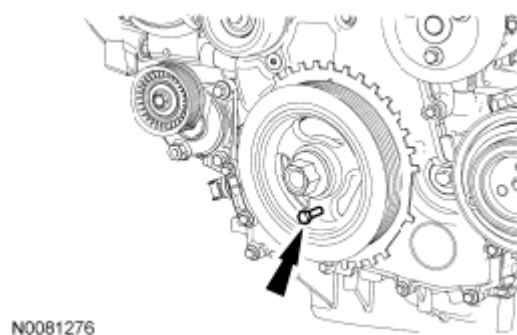
Fig. 64: Locating Crankshaft Pulley Bolt Courtesy of FORD MOTOR CO.
