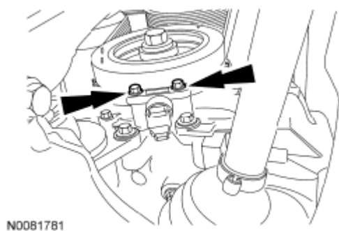
Fig. 61: Locating CKP Sensor And Bolts Courtesy of FORD MOTOR CO.
