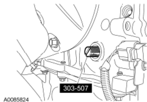
Fig. 357: Removing Crankshaft TDC Timing Peg Courtesy of FORD MOTOR CO.
