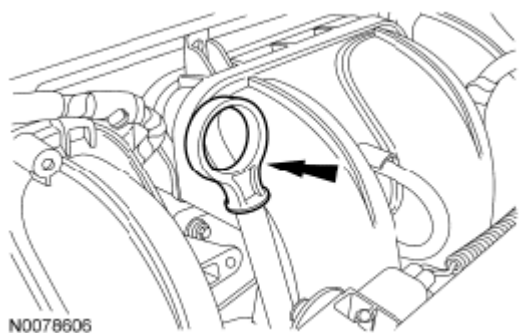
Fig. 440: Locating Engine Oil Level Indicator Courtesy of FORD MOTOR CO.
