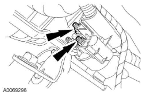
Fig. 206: Locating Starter Motor Electrical Terminals And Nuts Courtesy of FORD MOTOR CO.
