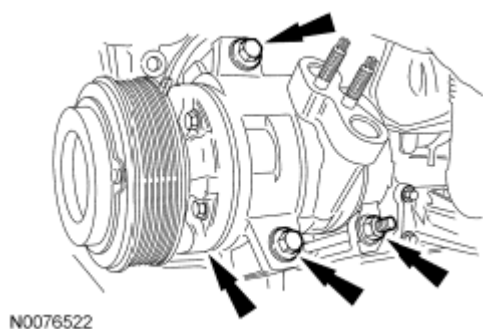
Fig. 242: Locating A/C Compressor, Stud Bolt And Bolts Courtesy of FORD MOTOR CO.
