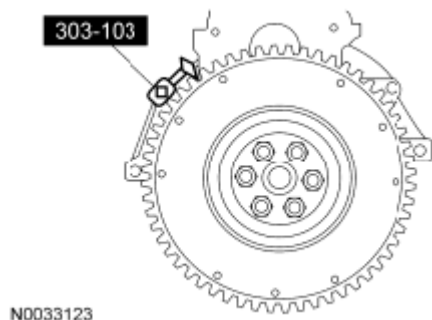
Fig. 47: Installing Flywheel Holding Tool Courtesy of FORD MOTOR CO.
