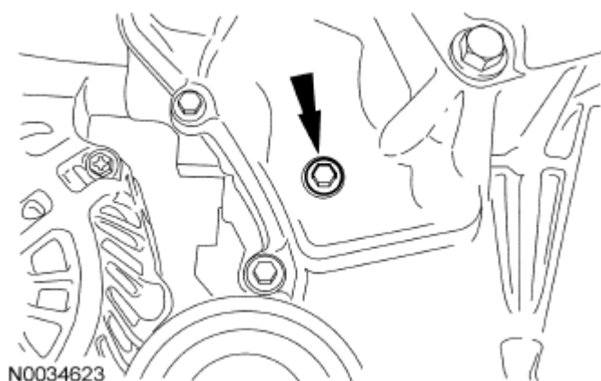
Fig. 105: Locating Front Cover Upper Timing Hole Plug Courtesy of FORD MOTOR CO.
