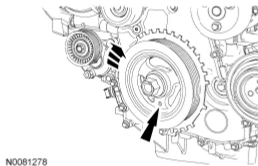
Fig. 347: Locating Crankshaft Pulley Bolt Courtesy of FORD MOTOR CO.
