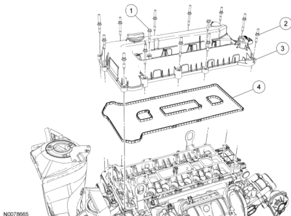
Fig. 20: Exploded View Of Valve Cover (2 Of 2)
