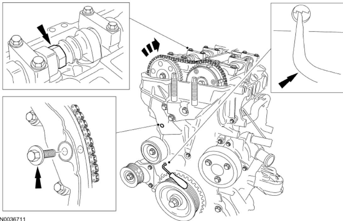
Fig. 89: Inserting Bolt Into Upper Front Cover Timing Hole Courtesy of FORD MOTOR CO.
