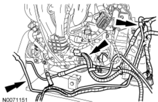
Fig. 406: Locating Power Steering Tubes And Wiring Harness Courtesy of FORD MOTOR CO.
