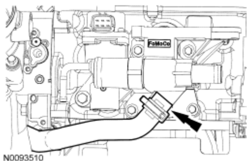
Fig. 370: Locating Coolant Bypass Hose Courtesy of FORD MOTOR CO.
