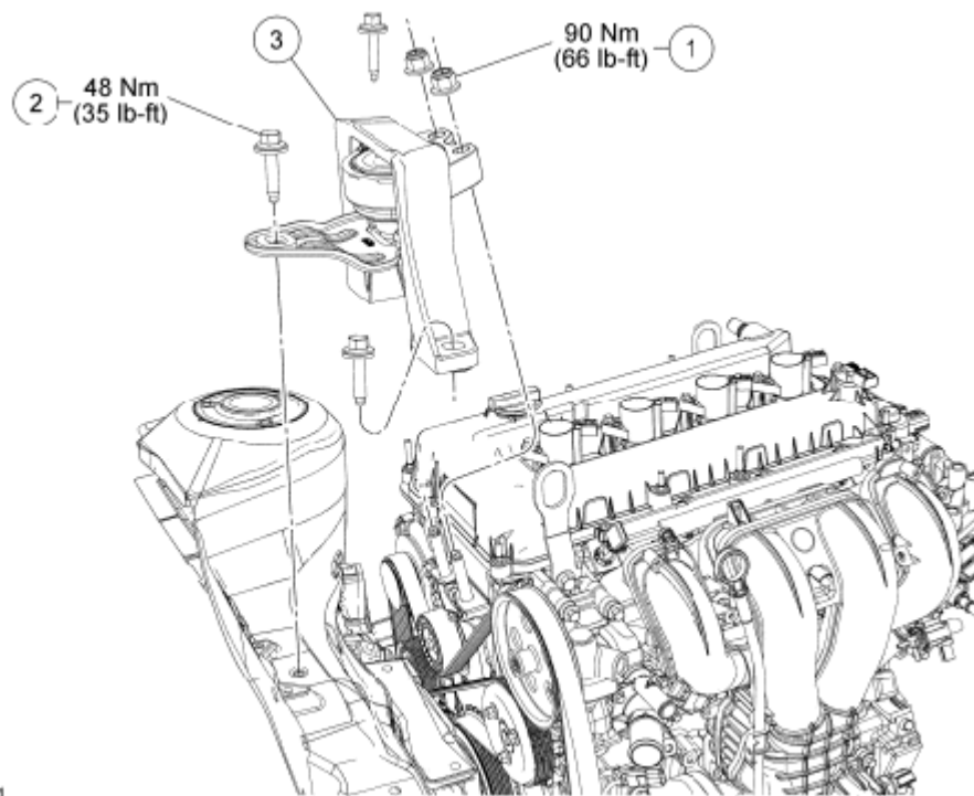
Fig. 150: Identifying Engine Mount, Engine Mount Bolt And Engine Mount Nut With Torque Specifications
