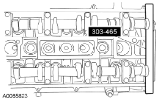
Fig. 349: Removing Camshaft Alignment Plate Courtesy of FORD MOTOR CO.
