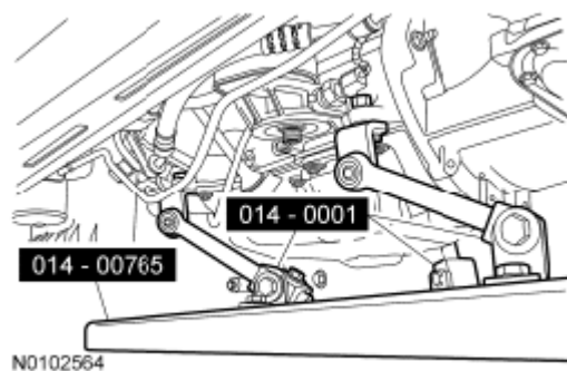
Fig. 187: Lifting Universal Adapter Brackets Courtesy of FORD MOTOR CO.
