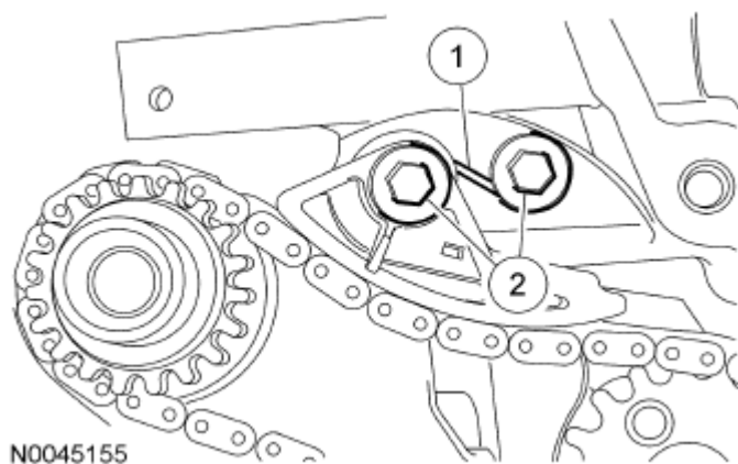
Fig. 138: Identifying Tensioner And Shoulder Bolts Courtesy of FORD MOTOR CO.
