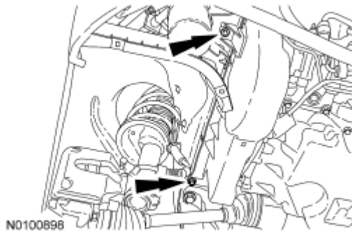
Fig. 133: Locating Accessory Drive Belt Splash Shield And Bolts Courtesy of FORD MOTOR CO.
