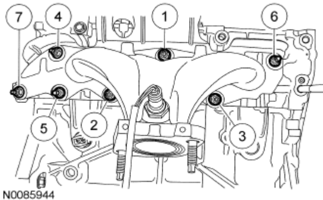
Fig. 148: Identifying Exhaust Manifold Gasket, Exhaust Manifold And Nuts Courtesy of FORD MOTOR CO.
