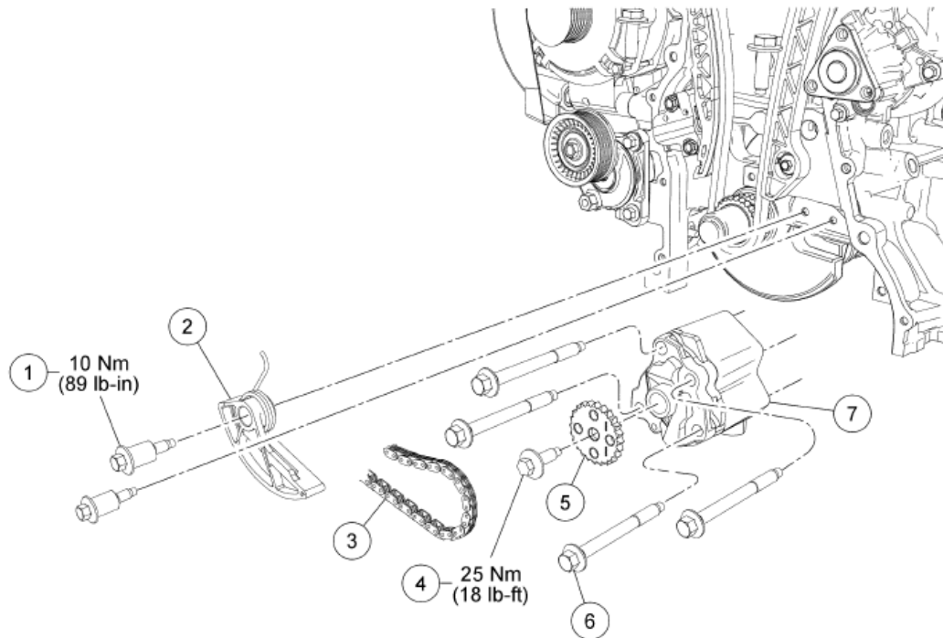
Fig. 132: Identifying Oil Pump Components Courtesy of FORD MOTOR CO.
