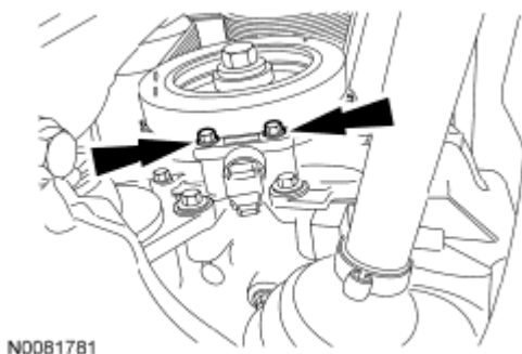
Fig. 354: Locating CKP Sensor And Bolts Courtesy of FORD MOTOR CO.
