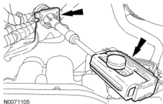
Fig. 166: Locating Transaxle Shift Cable From Lever And Bracket Courtesy of FORD MOTOR CO.
