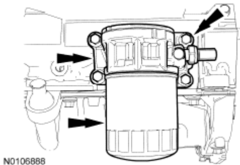
Fig. 221: Locating Oil Filter, Oil Filter Adapter And Bolts Courtesy of FORD MOTOR CO.
