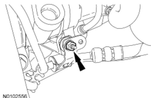
Fig. 204: Locating A/C Compressor Stud Bolt And Power Steering Tube Bracket Courtesy of FORD MOTOR CO.
