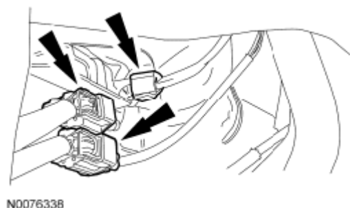
Fig. 444: Locating Heated Oxygen Sensor And Catalyst Monitor Sensor Electrical Connectors Courtesy of FORD MOTOR CO.
