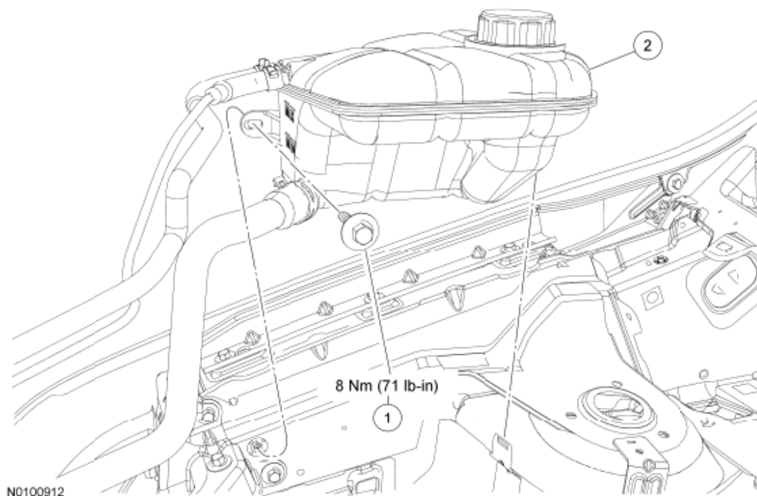
Fig. 149: Identifying Coolant Degas Bottle Bolt And Coolant Degas Bottle With Torque Specifications Courtesy of FORD MOTOR CO.
