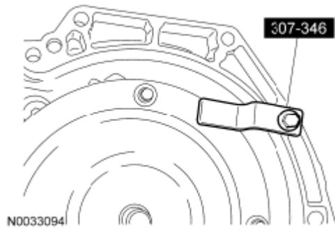
Fig. 211: Installing Torque Converter Retainer Courtesy of FORD MOTOR CO.
