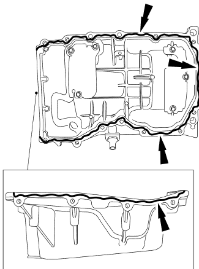
Fig. 134: Locating Oil Pan-To-Engine Front Cover Mating Surface Courtesy of FORD MOTOR CO.
