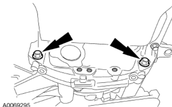
Fig. 186: Locating Oil Pan-To-Bellhousing Bolts Courtesy of FORD MOTOR CO.
