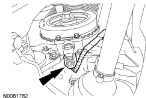
Fig. 63: Locating Wiring Harness Retainers To Engine Front Cover Courtesy of FORD MOTOR CO.
