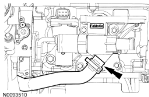
Fig. 238: Locating Coolant Bypass Hose Courtesy of FORD MOTOR CO.
