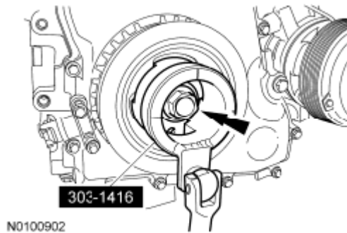
Fig. 33: Tightening Crankshaft Pulley Bolt Courtesy of FORD MOTOR CO.
