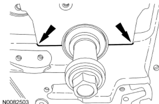
Fig. 306: Locating Main Bearing Beam Side Fit Surfaces Courtesy of FORD MOTOR CO.
