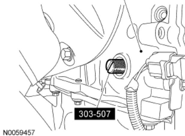
Fig. 38: Locating Crankshaft TDC Timing Peg
