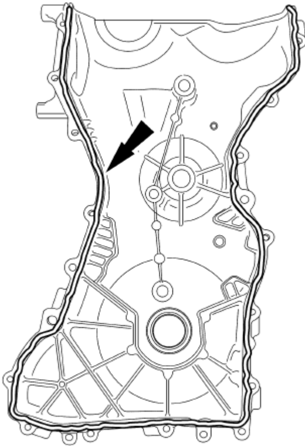
Fig. 341: Locating Engine Front Cover Sealant Area Courtesy of FORD MOTOR CO.
