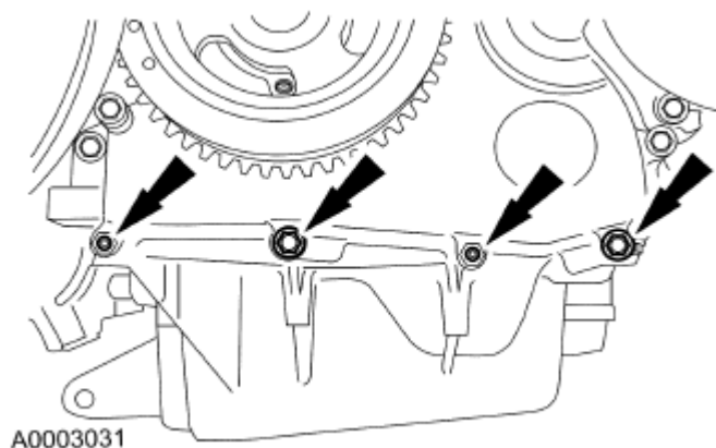
Fig. 135: Locating Engine Front Cover-To-Oil Pan Bolts Courtesy of FORD MOTOR CO.
