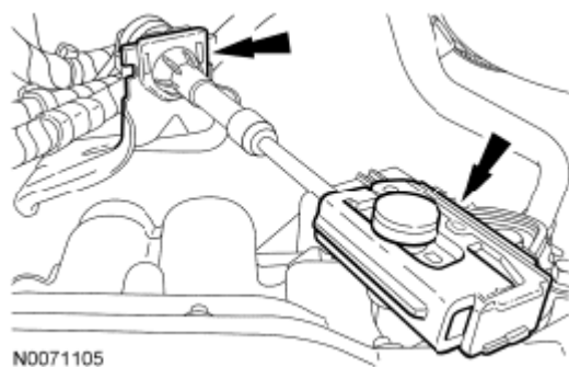
Fig. 443: Locating Transaxle Shift Cable And Bracket Courtesy of FORD MOTOR CO.
