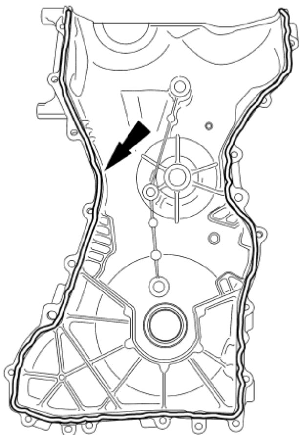
Fig. 57: Locating Engine Front Cover Sealant Area Courtesy of FORD MOTOR CO.
