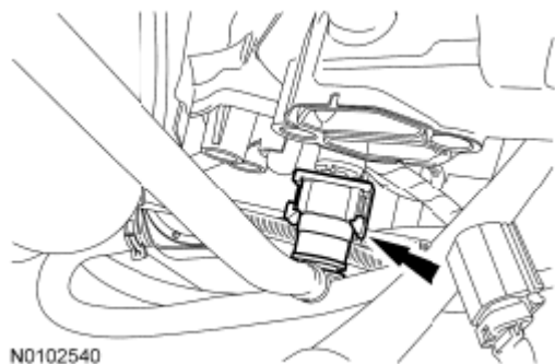
Fig. 451: Locating Evaporative Emission Tube Courtesy of FORD MOTOR CO.
