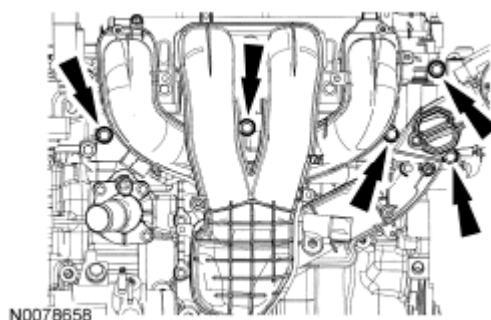
Fig. 375: Locating Intake Manifold Mounting Bolts Courtesy of FORD MOTOR CO.
