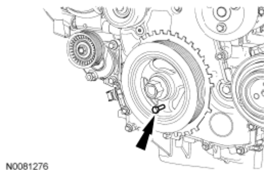
Fig. 356: Locating Crankshaft Pulley Bolt Courtesy of FORD MOTOR CO.
