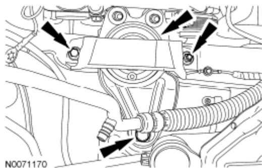
Fig. 422: Locating Engine Mount Bolts Courtesy of FORD MOTOR CO.
