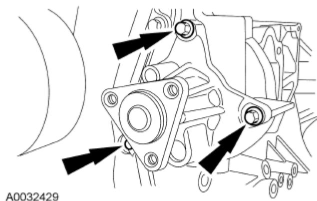
Fig. 395: Locating Coolant Pump And Bolts Courtesy of FORD MOTOR CO.
