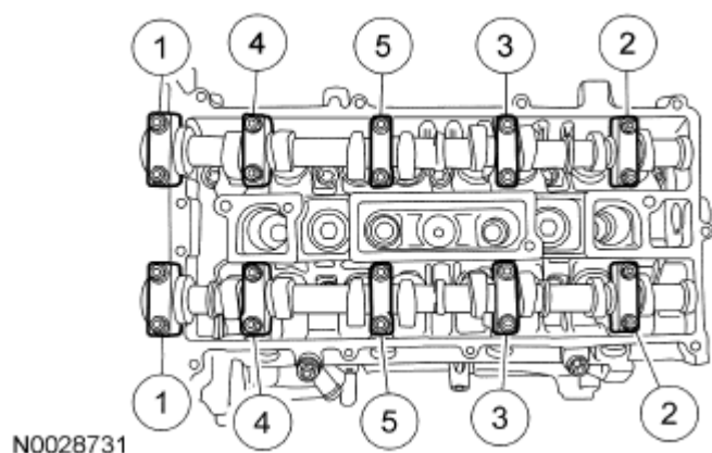
Fig. 126: Identifying Camshaft Bearing Cap Bolts Tightening Sequence Courtesy of FORD MOTOR CO.
