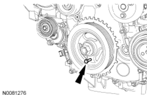
Fig. 103: Locating Crankshaft Pulley Bolt Courtesy of FORD MOTOR CO.
