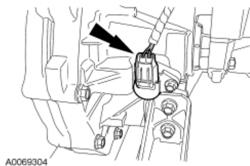
Fig. 193: Locating Output Shaft Speed Sensor Electrical Connector Courtesy of FORD MOTOR CO.
