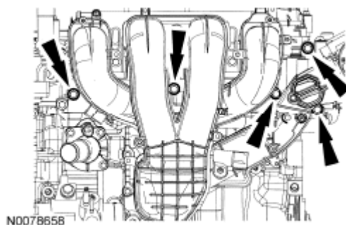
Fig. 15: Locating Intake Manifold Mounting Bolts Courtesy of FORD MOTOR CO.
