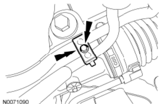
Fig. 176: Locating Power Steering Tube Clip And Bolt Courtesy of FORD MOTOR CO.
