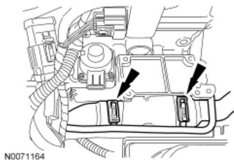
Fig. 429: Locating Upper Radiator Hose And Heater Hose Courtesy of FORD MOTOR CO.
