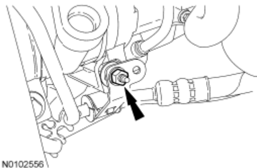
Fig. 407: Locating A/C Compressor Stud Bolt And Power Steering Tube Bracket Courtesy of FORD MOTOR CO.
