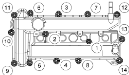
Fig. 360: Identifying Valve Cover Bolts Tightening Sequence Courtesy of FORD MOTOR CO.
