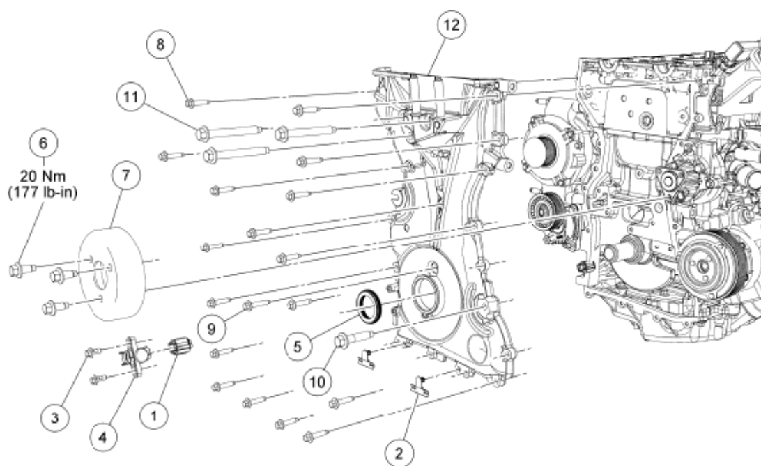
Fig. 54: Identifying Engine Front Cover Components With Torque Specifications Courtesy of FORD MOTOR CO.
