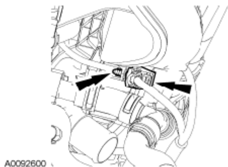
Fig. 227: Locating Knock Sensor (KS) Electrical Connector And Pin-Type Retainer Courtesy of FORD MOTOR CO.
