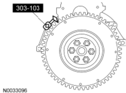
Fig. 212: Removing Flywheel Or Flexplate Courtesy of FORD MOTOR CO.
