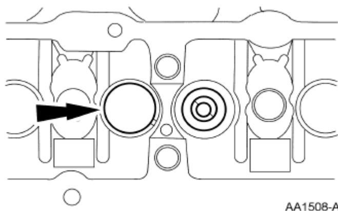
Fig. 125: Locating Valve Tappets In Original Positions Courtesy of FORD MOTOR CO.
