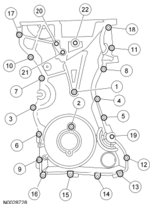
Fig. 342: Identifying Engine Front Cover Bolts Tightening Sequence Courtesy of FORD MOTOR CO.
