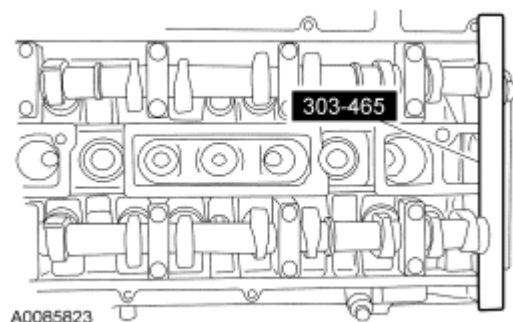
Fig. 119: Removing Camshaft Alignment Plate Courtesy of FORD MOTOR CO.
