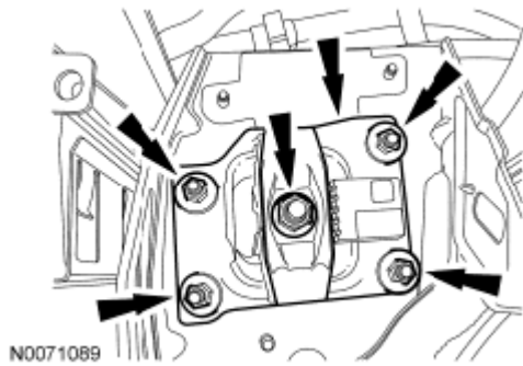
Fig. 190: Locating Transaxle Mount Nuts And Transaxle Mount Plate Courtesy of FORD MOTOR CO.
