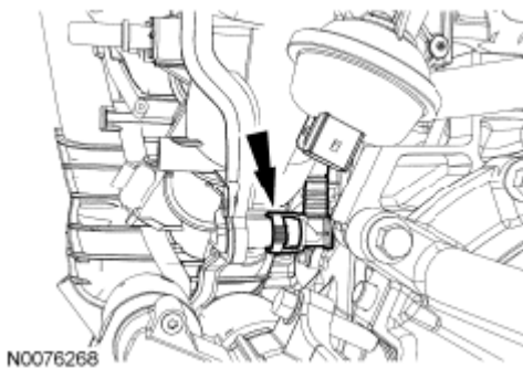
Fig. 235: Locating Intake Manifold Courtesy of FORD MOTOR CO.
