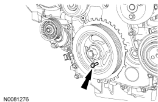
Fig. 85: Locating Crankshaft Pulley Bolt Courtesy of FORD MOTOR CO.
