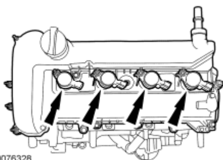
Fig. 246: Locating Ignition Coil-On-Plugs And Bolts Courtesy of FORD MOTOR CO.
