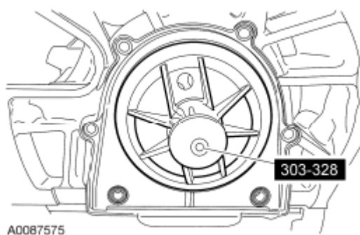
Fig. 315: Installing Crankshaft Rear Seal Courtesy of FORD MOTOR CO.
