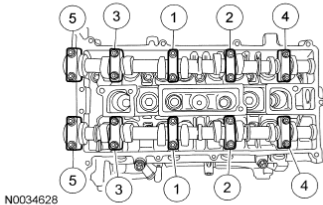
Fig. 96: Identifying Camshaft Bearing Cap Bolts Tightening Sequence Courtesy of FORD MOTOR CO.
