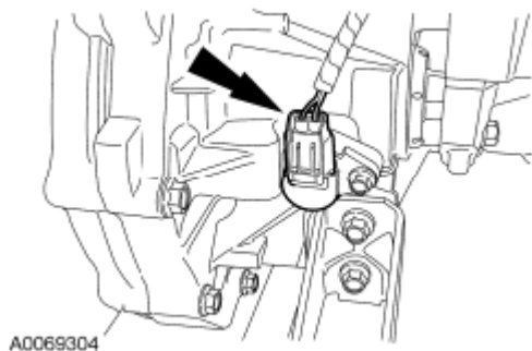
Fig. 418: Locating Output Shaft Speed Sensor Electrical Connector Courtesy of FORD MOTOR CO.
