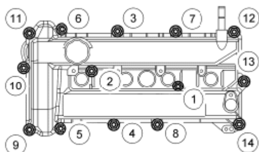
Fig. 23: Identifying Valve Cover Bolts Tightening Sequence Courtesy of FORD MOTOR CO.
