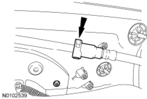
Fig. 157: Locating Fuel Tube Quick Connect Coupling Courtesy of FORD MOTOR CO.
