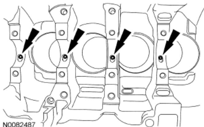
Fig. 279: Locating Oil Squirters Courtesy of FORD MOTOR CO.
