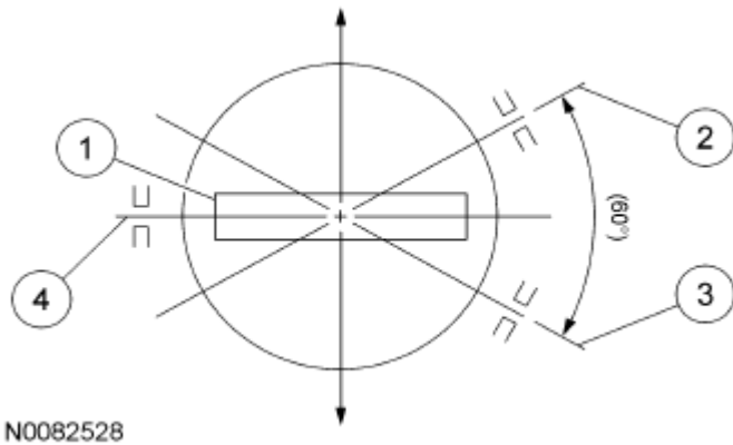
Fig. 288: Identifying Center Line Of Piston Pin Bore And Expander Gap Courtesy of FORD MOTOR CO.
