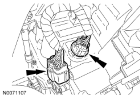
Fig. 416: Locating Transaxle Electrical Connectors Courtesy of FORD MOTOR CO.
