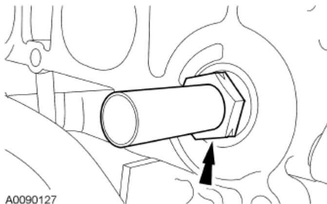
Fig. 372: Locating EGR Tube Courtesy of FORD MOTOR CO.
