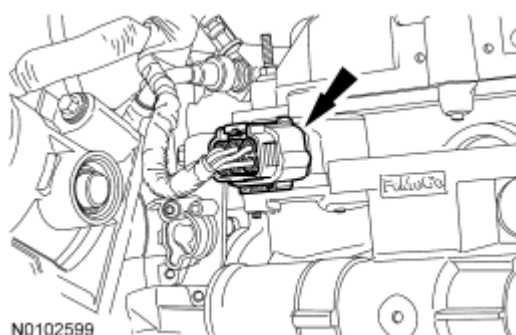
Fig. 230: Locating EGR Valve Electrical Connector Courtesy of FORD MOTOR CO.
