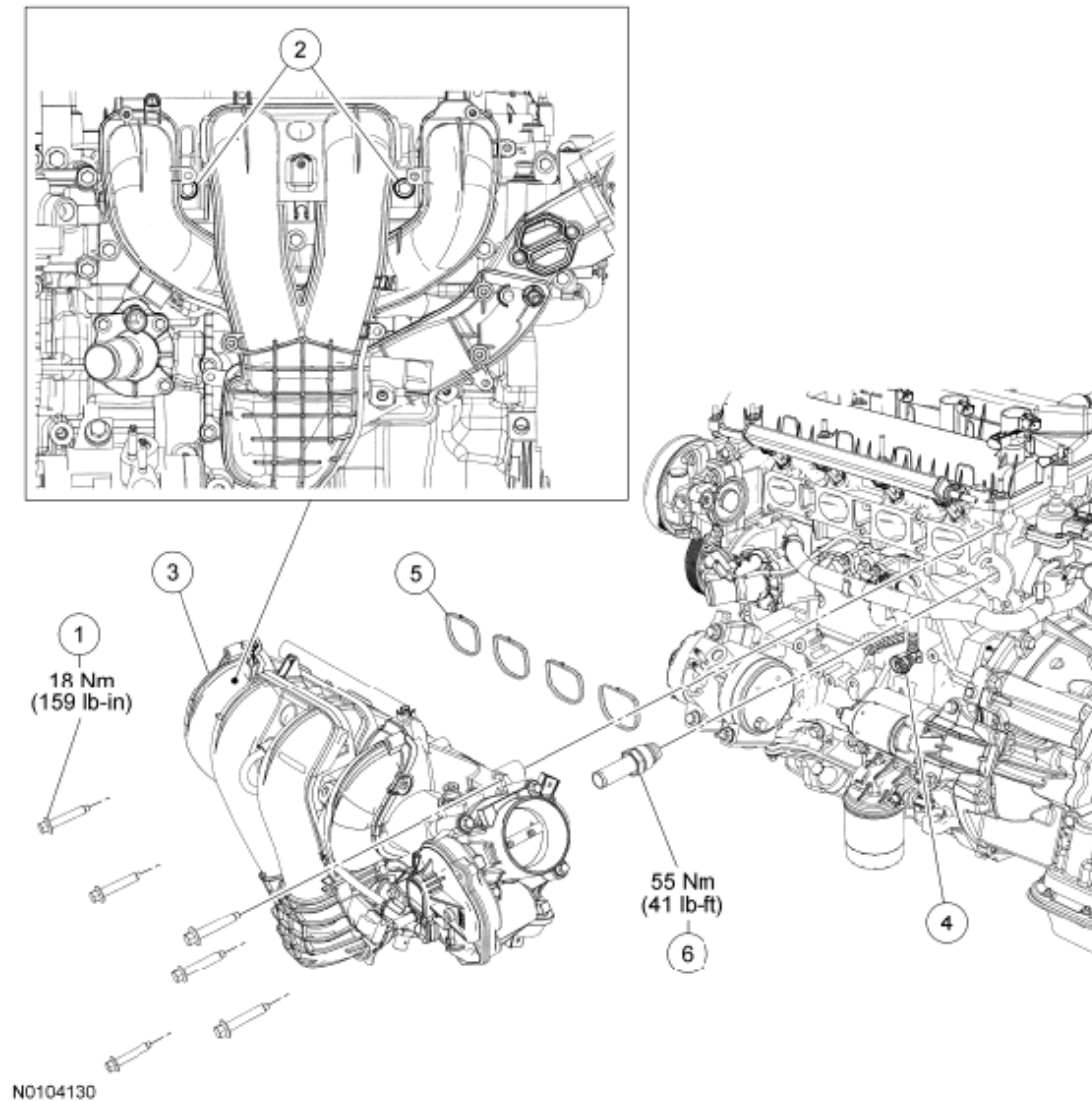
Fig. 7: Identifying Intake Manifold Components With Torque Specifications (3 Of 3) Courtesy of FORD MOTOR CO.
