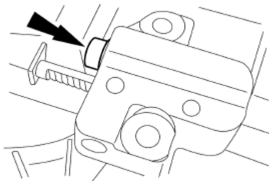
Fig. 335: Compressing Timing Chain Tensioner Plunger Courtesy of FORD MOTOR CO.
