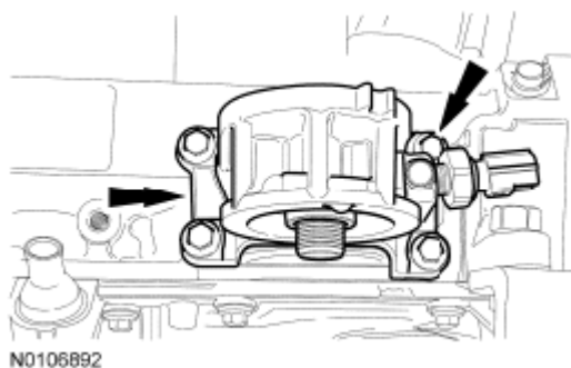
Fig. 388: Locating Oil Filter Adapter And Bolts Courtesy of FORD MOTOR CO.
