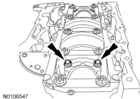
Fig. 311: Locating Connecting Rod Caps And Bolts Courtesy of FORD MOTOR CO.
