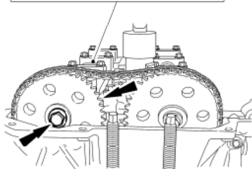
Fig. 91: Locating Exhaust Camshaft Drive Gear And Bolt Courtesy of FORD MOTOR CO.
