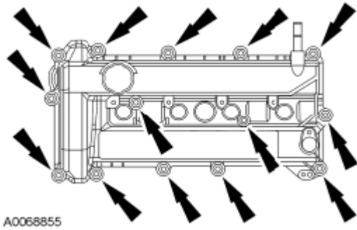
Fig. 248: Locating Valve Cover And Bolts Courtesy of FORD MOTOR CO.
