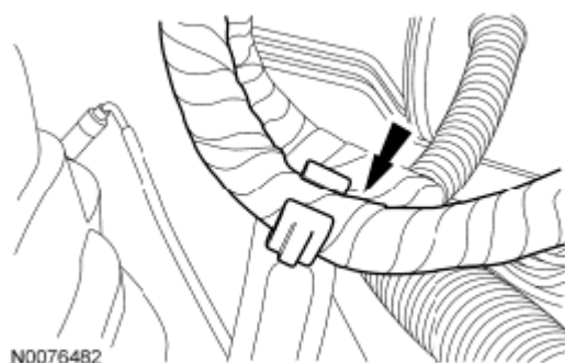
Fig. 448: Locating Engine Harness From Coolant Outlet Bracket Harness Retainer Courtesy of FORD MOTOR CO.
