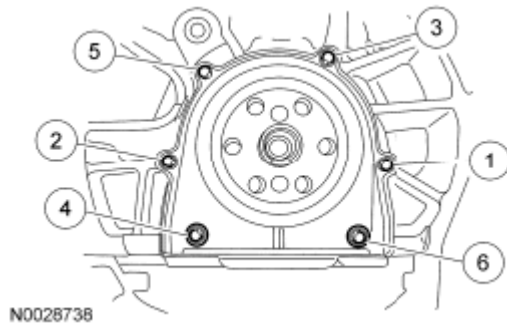
Fig. 50: Identifying Retainer Plate Bolts Tightening Sequence Courtesy of FORD MOTOR CO.
