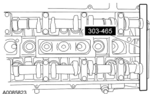
Fig. 352: Installing Camshaft Alignment Plate To Camshafts Courtesy of FORD MOTOR CO.
