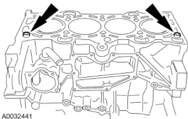
Fig. 321: Locating Cylinder Head Alignment Dowels Courtesy of FORD MOTOR CO.
