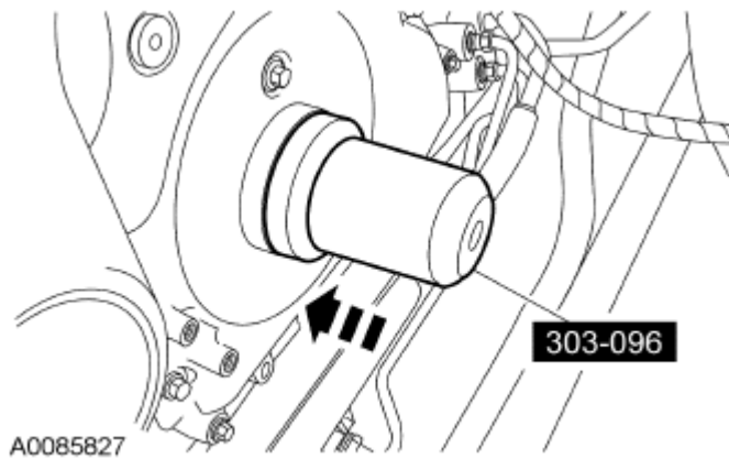
Fig. 45: Installing Crankshaft Front Oil Seal Courtesy of FORD MOTOR CO.
