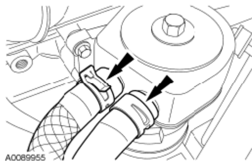
Fig. 391: Locating Oil Cooler Hoses Courtesy of FORD MOTOR CO.
