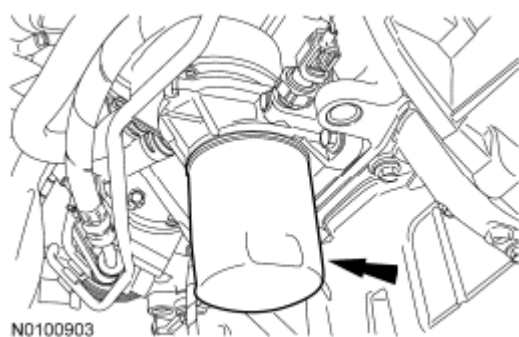
Fig. 128: Removing Engine Oil Filter Courtesy of FORD MOTOR CO.
