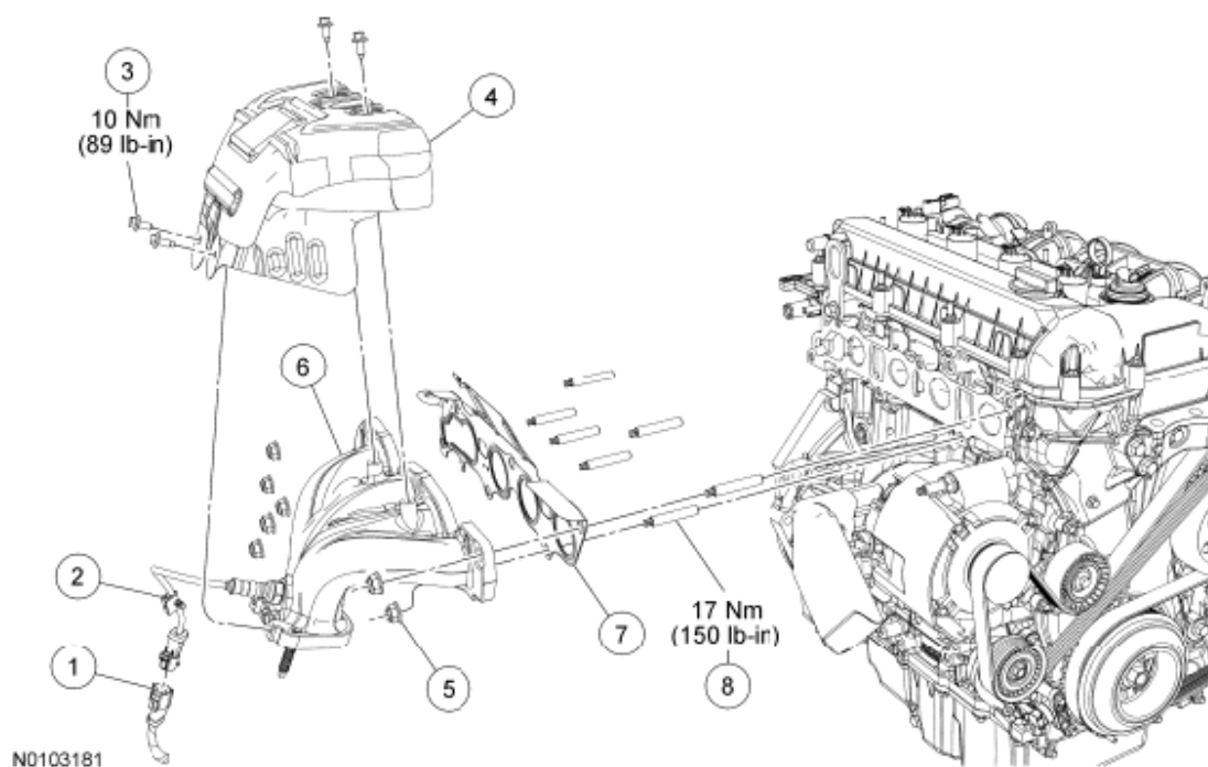
Fig. 147: Identifying Exhaust Manifold Components With Torque Specifications Courtesy of FORD MOTOR CO.
