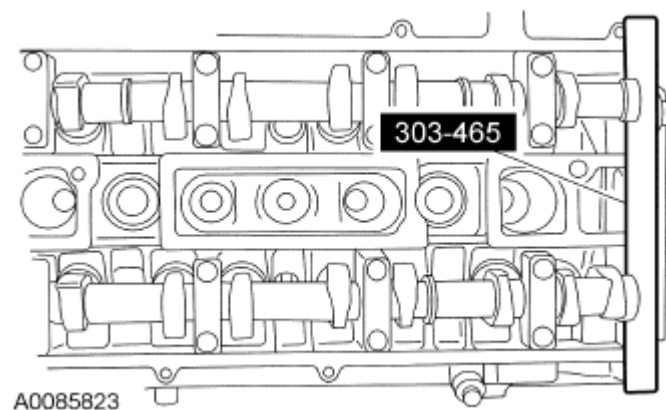
Fig. 36: Removing Camshaft Alignment Plate Courtesy of FORD MOTOR CO.
