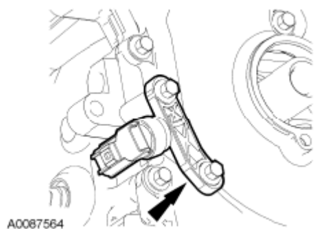
Fig. 255: Locating CKP Sensor And Bolts Courtesy of FORD MOTOR CO.
