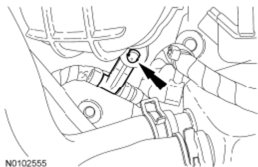
Fig. 413: Locating Wiring Harness Pin-Type Retainer And Intake Manifold Courtesy of FORD MOTOR CO.
