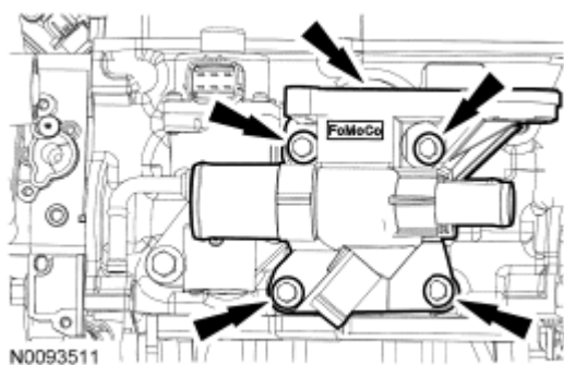
Fig. 239: Locating Coolant Outlet And Bolts Courtesy of FORD MOTOR CO.
