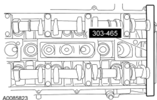
Fig. 353: Removing Camshaft Alignment Plate Courtesy of FORD MOTOR CO.
