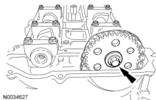
Fig. 98: Locating Intake Camshaft Drive Gear Courtesy of FORD MOTOR CO.
