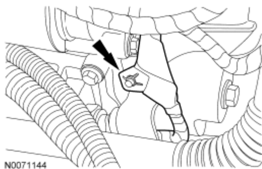
Fig. 410: Locating Starter Wire Harness Retainer And Starter Motor Stud Bolt Courtesy of FORD MOTOR CO.
