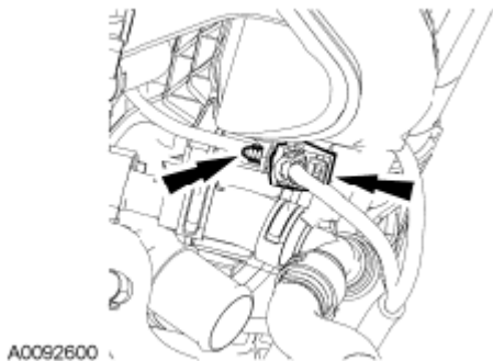
Fig. 381: Locating KS Electrical Connector And Pin-Type Retainer Courtesy of FORD MOTOR CO.
