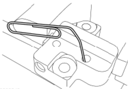
Fig. 78: Installing Paper Clip Into Hole In Tensioner Housing Courtesy of FORD MOTOR CO.
