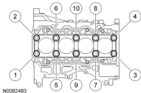
Fig. 275: Locating Main Bearing Beam Courtesy of FORD MOTOR CO.
