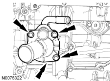
Fig. 241: Locating Thermostat Housing, Thermostat And Bolts Courtesy of FORD MOTOR CO.
