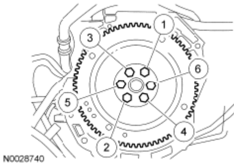
Fig. 398: Identifying Flywheel Bolts Tightening Sequence Courtesy of FORD MOTOR CO.
