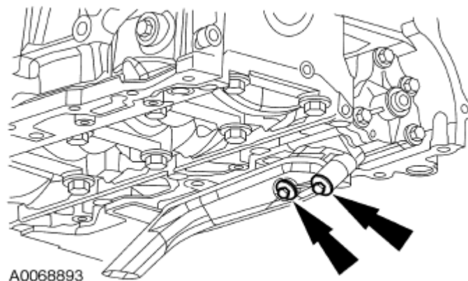
Fig. 271: Locating Oil Pump Pickup Tube And Gasket Courtesy of FORD MOTOR CO.
