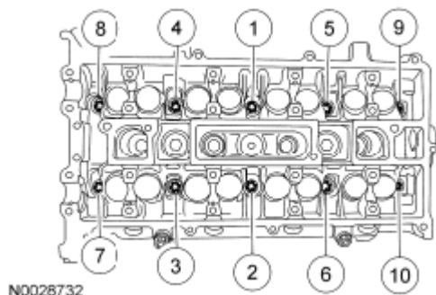
Fig. 324: Identifying Cylinder Head Bolts Tightening Sequence Courtesy of FORD MOTOR CO.
