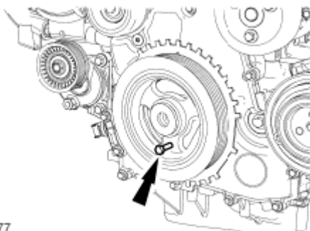
Fig. 345: Locating Crankshaft Pulley Standard Bolt Courtesy of FORD MOTOR CO.
