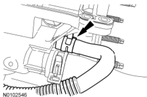
Fig. 430: Locating Coolant Degas Bottle Vent Hose Courtesy of FORD MOTOR CO.
