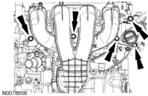
Fig. 234: Locating Intake Manifold Bolts Courtesy of FORD MOTOR CO.
