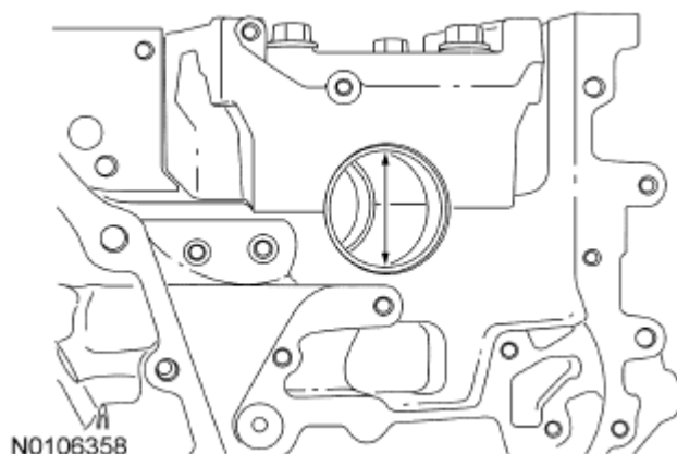
Fig. 298: Measuring Crankshaft Block Housing Main Bearing Bore Diameter Courtesy of FORD MOTOR CO.
