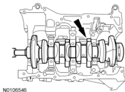
Fig. 276: Locating Crankshaft From Engine Block Courtesy of FORD MOTOR CO.
