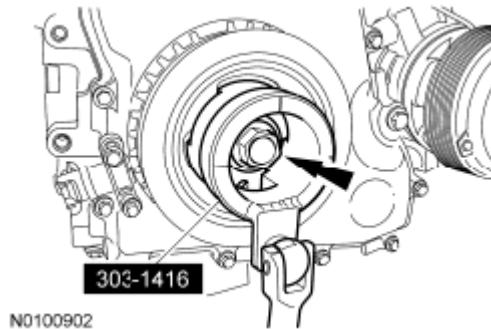
Fig. 30: Locating Diamond Washer Courtesy of FORD MOTOR CO.
