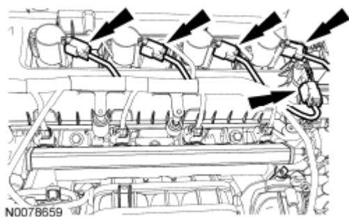
Fig. 387: Locating Coil-On-Plug And Camshaft Position Sensor Electrical Connectors Courtesy of FORD MOTOR CO.
