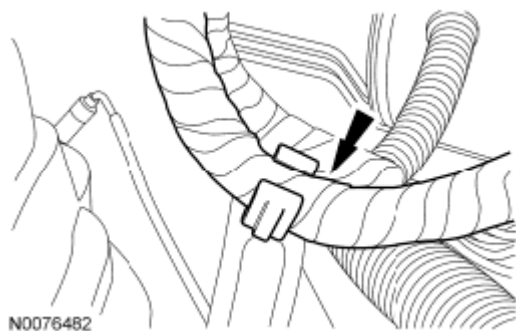
Fig. 161: Locating Engine Harness From Coolant Outlet Bracket Harness Retainer Courtesy of FORD MOTOR CO.
