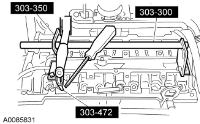
Fig. 110: Installing Valve Collet Courtesy of FORD MOTOR CO.
