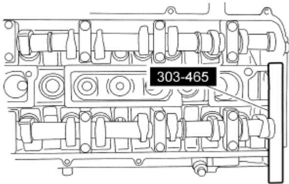
Fig. 88: Repositioning Camshaft Alignment Plate Courtesy of FORD MOTOR CO.
