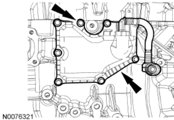
Fig. 364: Locating Crankcase Vent Oil Separator And Bolts Courtesy of FORD MOTOR CO.
