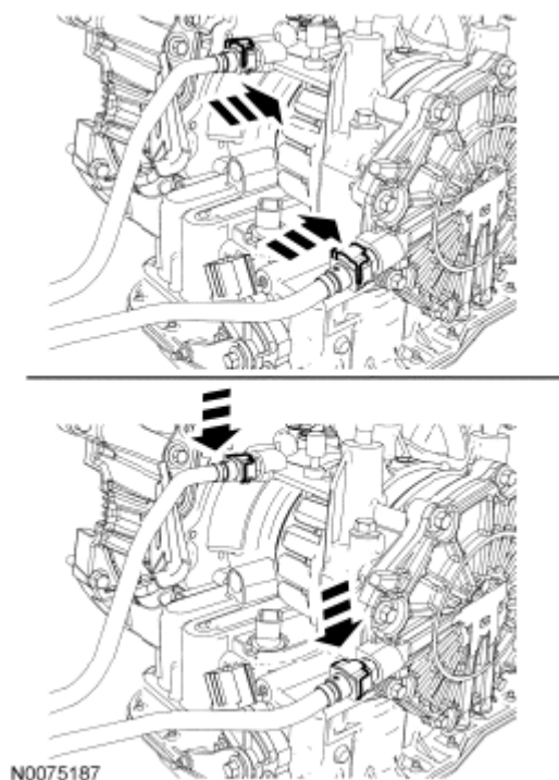
Fig. 441: Installing Transmission Fluid Cooler Tubes On Transaxle Courtesy of FORD MOTOR CO.
