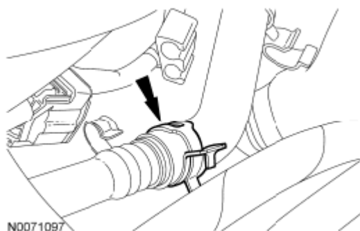
Fig. 428: Locating Heater Hose From Coolant Tube Courtesy of FORD MOTOR CO.
