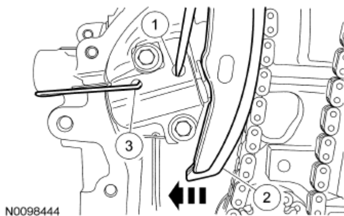
Fig. 257: Inserting Paper Clip Into Hole Courtesy of FORD MOTOR CO.
