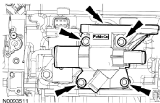
Fig. 369: Locating Coolant Outlet And Bolts Courtesy of FORD MOTOR CO.
