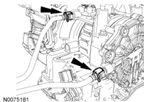
Fig. 167: Locating Transmission Fluid Cooler Tube Secondary Latches Courtesy of FORD MOTOR CO.
