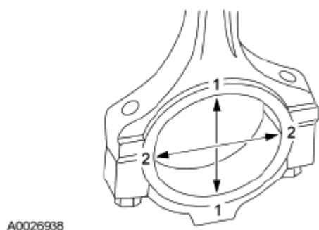
Fig. 300: Identifying Connecting Rod Large End Bore Courtesy of FORD MOTOR CO.
