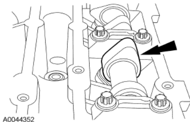
Fig. 265: Locating Camshaft Lobes On No. 1 Cylinder Courtesy of FORD MOTOR CO.
