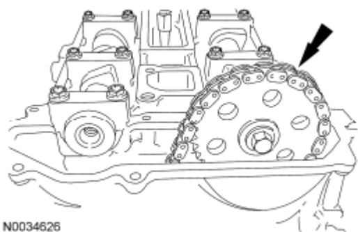
Fig. 92: Locating Timing Chain From Intake Camshaft Drive Gear Courtesy of FORD MOTOR CO.
