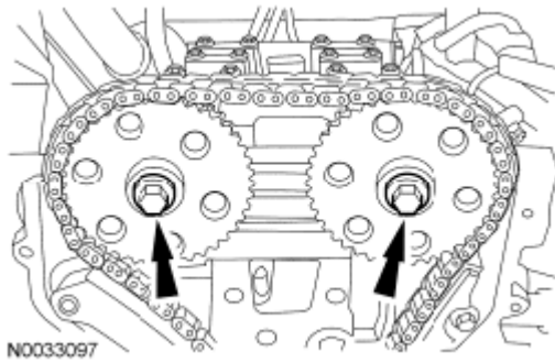
Fig. 80: Locating Camshaft Drive Gear Bolts Courtesy of FORD MOTOR CO.
