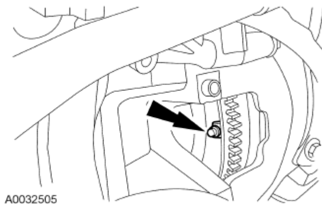
Fig. 209: Locating Torque Converter Nuts Courtesy of FORD MOTOR CO.
