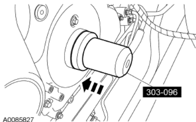
Fig. 59: Installing Crankshaft Front Oil Seal Courtesy of FORD MOTOR CO.
