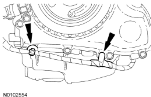
Fig. 412: Locating Crankshaft Position Sensor Wire Harness Retainers Courtesy of FORD MOTOR CO.
