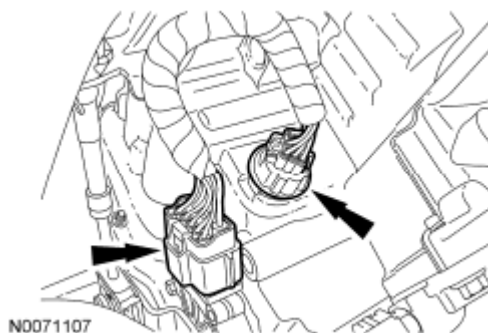
Fig. 195: Locating Transaxle Electrical Connectors Courtesy of FORD MOTOR CO.
