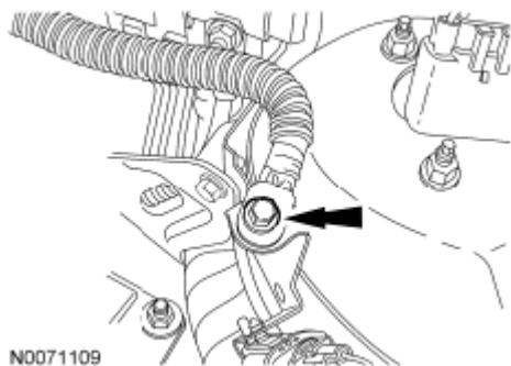
Fig. 453: Locating Negative Battery Cable Ground Bolt Courtesy of FORD MOTOR CO.
