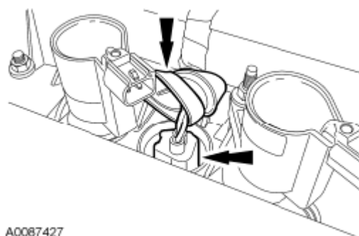
Fig. 386: Locating Rubber Boot And Cylinder Head Temperature Sensor Electrical Connector Courtesy of FORD MOTOR CO.
