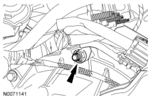
Fig. 420: Locating HO2S And CMS Wire Connector Bracket Courtesy of FORD MOTOR CO.
