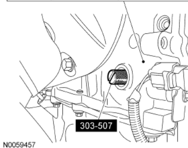
Fig. 273: Locating Crankshaft TDC Timing Peg
