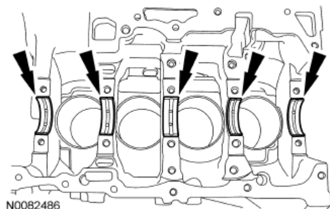
Fig. 303: Locating Main Bearings
