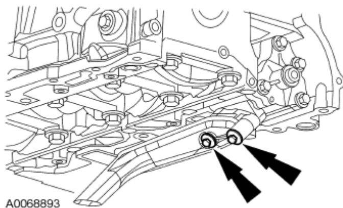
Fig. 314: Locating Oil Pump Pickup Tube And Gasket Courtesy of FORD MOTOR CO.
