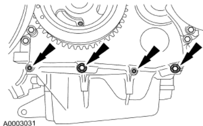
Fig. 52: Locating Engine Front Cover-To-Oil Pan Bolts Courtesy of FORD MOTOR CO.
