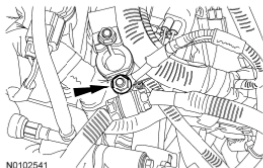
Fig. 447: Locating Negative Battery Terminal Nut Courtesy of FORD MOTOR CO.
