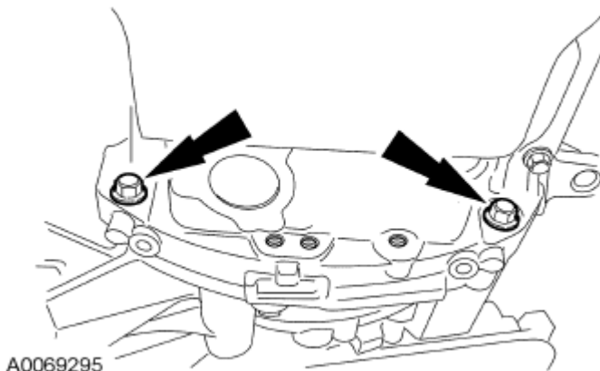
Fig. 424: Locating Oil Pan-To-Bellhousing Bolts Courtesy of FORD MOTOR CO.
