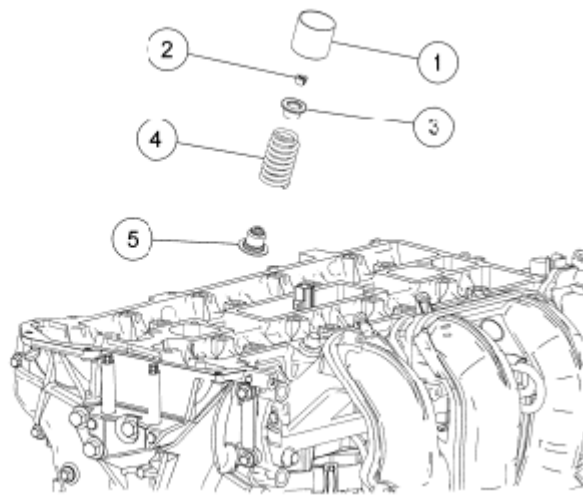
Fig. 108: Identifying Valve Train Components Courtesy of FORD MOTOR CO.
