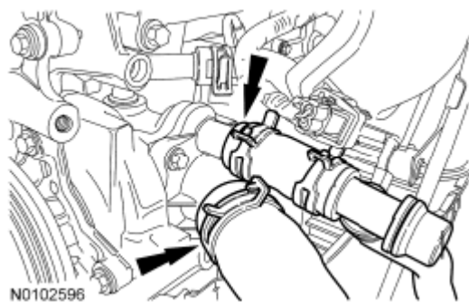
Fig. 216: Locating Oil Cooler Hose And Lower Radiator Hose Courtesy of FORD MOTOR CO.
