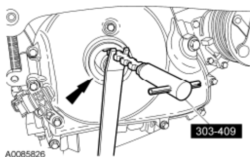
Fig. 55: Removing Crankshaft Front Oil Seal Courtesy of FORD MOTOR CO.
