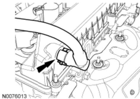
Fig. 153: Locating Crankcase Vent Tube From Valve Cover Courtesy of FORD MOTOR CO.
