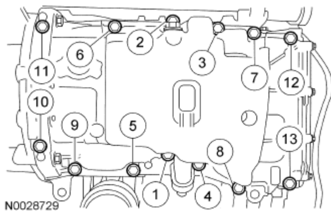
Fig. 136: Identifying Oil Pan Bolts Tightening Sequence Courtesy of FORD MOTOR CO.
