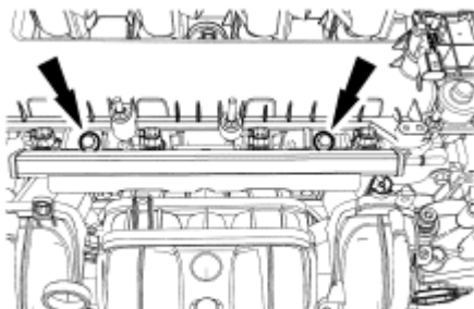
Fig. 383: Locating Fuel Injectors And Bolts Courtesy of FORD MOTOR CO.
