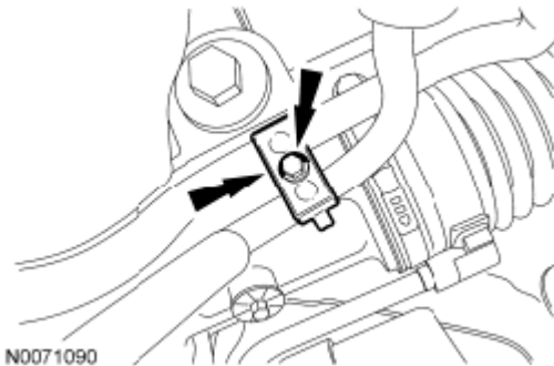
Fig. 434: Locating Power Steering Tube Clip And Bolt Courtesy of FORD MOTOR CO.
