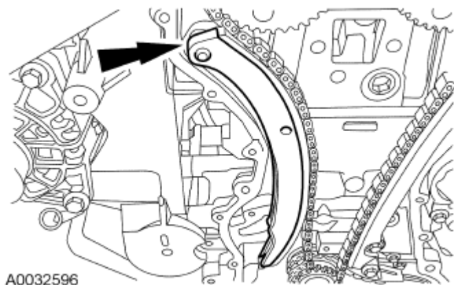
Fig. 74: Locating RH Timing Chain Guide Courtesy of FORD MOTOR CO.
