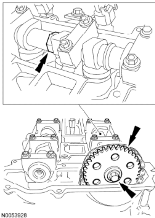
Fig. 93: Locating Intake Camshaft Drive Gear Courtesy of FORD MOTOR CO.
