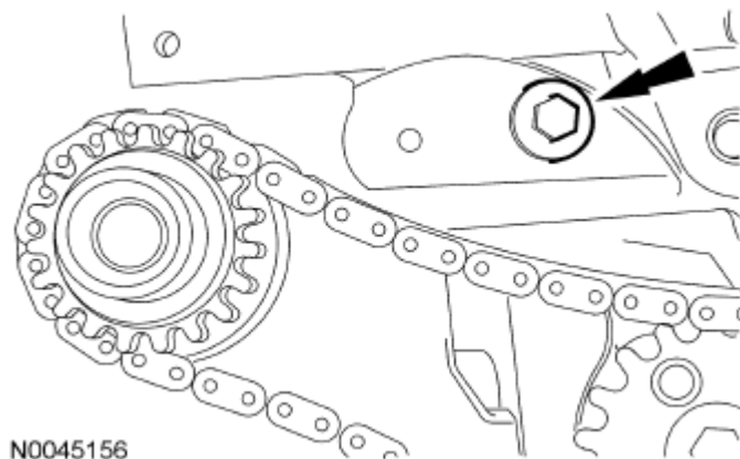
Fig. 328: Locating Oil Pump Chain Tensioner Shoulder Bolt Courtesy of FORD MOTOR CO.
