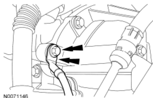
Fig. 203: Locating Engine Ground Wire And Bolt Courtesy of FORD MOTOR CO.
