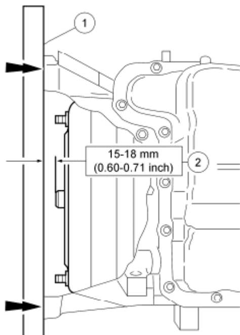
Fig. 399: Locating Straightedge On Automatic Transaxle Flange Courtesy of FORD MOTOR CO.
