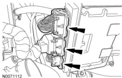
Fig. 446: Locating PCM Electrical Connectors Courtesy of FORD MOTOR CO.
