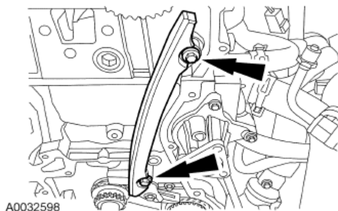
Fig. 332: Locating LH Timing Chain Guide And Bolts Courtesy of FORD MOTOR CO.
