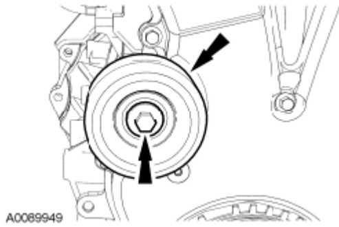
Fig. 397: Locating Accessory Drive Belt Idler Pulley Courtesy of FORD MOTOR CO.
