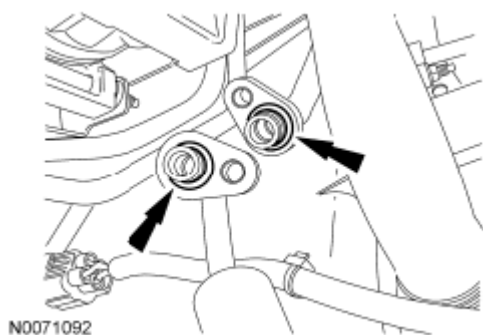
Fig. 437: Locating A/C Tubes From Compressor Courtesy of FORD MOTOR CO.
