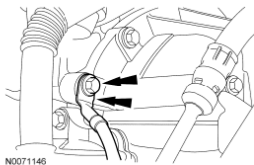
Fig. 408: Locating Engine Ground Wire And Bolt Courtesy of FORD MOTOR CO.
