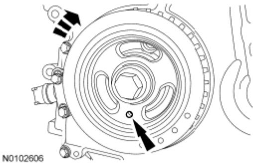
Fig. 249: Turning Crankshaft To No. 1 Piston Courtesy of FORD MOTOR CO.
