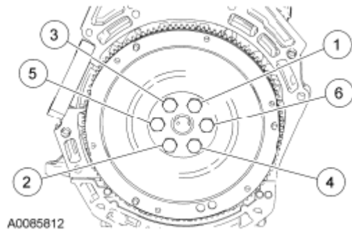
Fig. 48: Identifying Transaxle Bolts Tightening Sequence Courtesy of FORD MOTOR CO.
