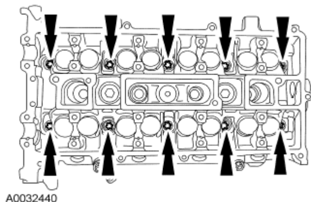
Fig. 267: Locating Cylinder Head Bolts
