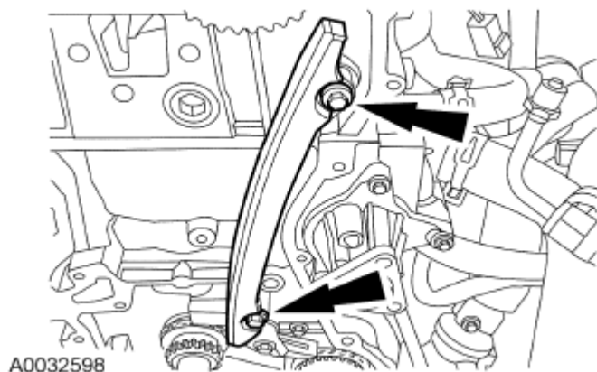
Fig. 261: Locating LH Timing Chain Guide And Bolts Courtesy of FORD MOTOR CO.
