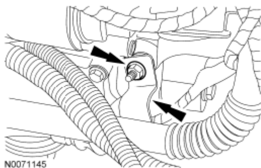
Fig. 409: Locating Starter Motor Stud Bolt And Power Steering Tube Bracket Courtesy of FORD MOTOR CO.
