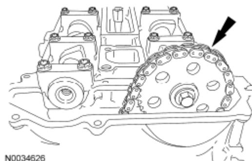
Fig. 99: Locating Timing Chain On Intake Camshaft Drive Gear Courtesy of FORD MOTOR CO.
