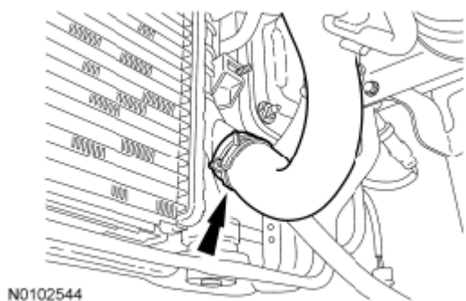
Fig. 436: Locating Lower Radiator Hose To Radiator Courtesy of FORD MOTOR CO.
