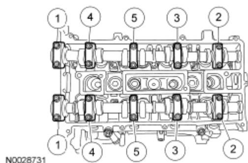
Fig. 266: Identifying Camshafts Bolts Tightening Sequence Courtesy of FORD MOTOR CO.
