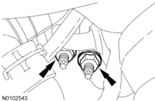
Fig. 171: Locating A/C Tube Nuts And A/C Compressor Courtesy of FORD MOTOR CO.
