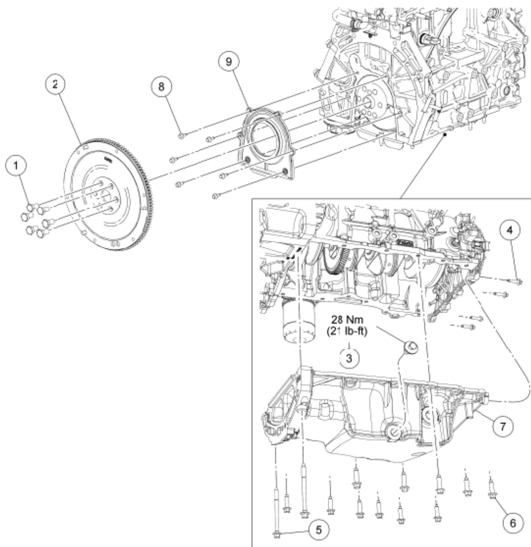
Fig. 25: Identifying Flexplate, Crankshaft Rear Seal And Retainer Plate With Torque Specifications Courtesy of FORD MOTOR CO.
