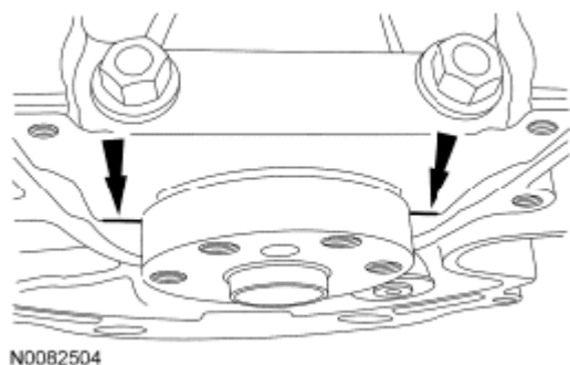
Fig. 307: Locating Crankshaft Bearing Journals On Main Bearing Courtesy of FORD MOTOR CO.
