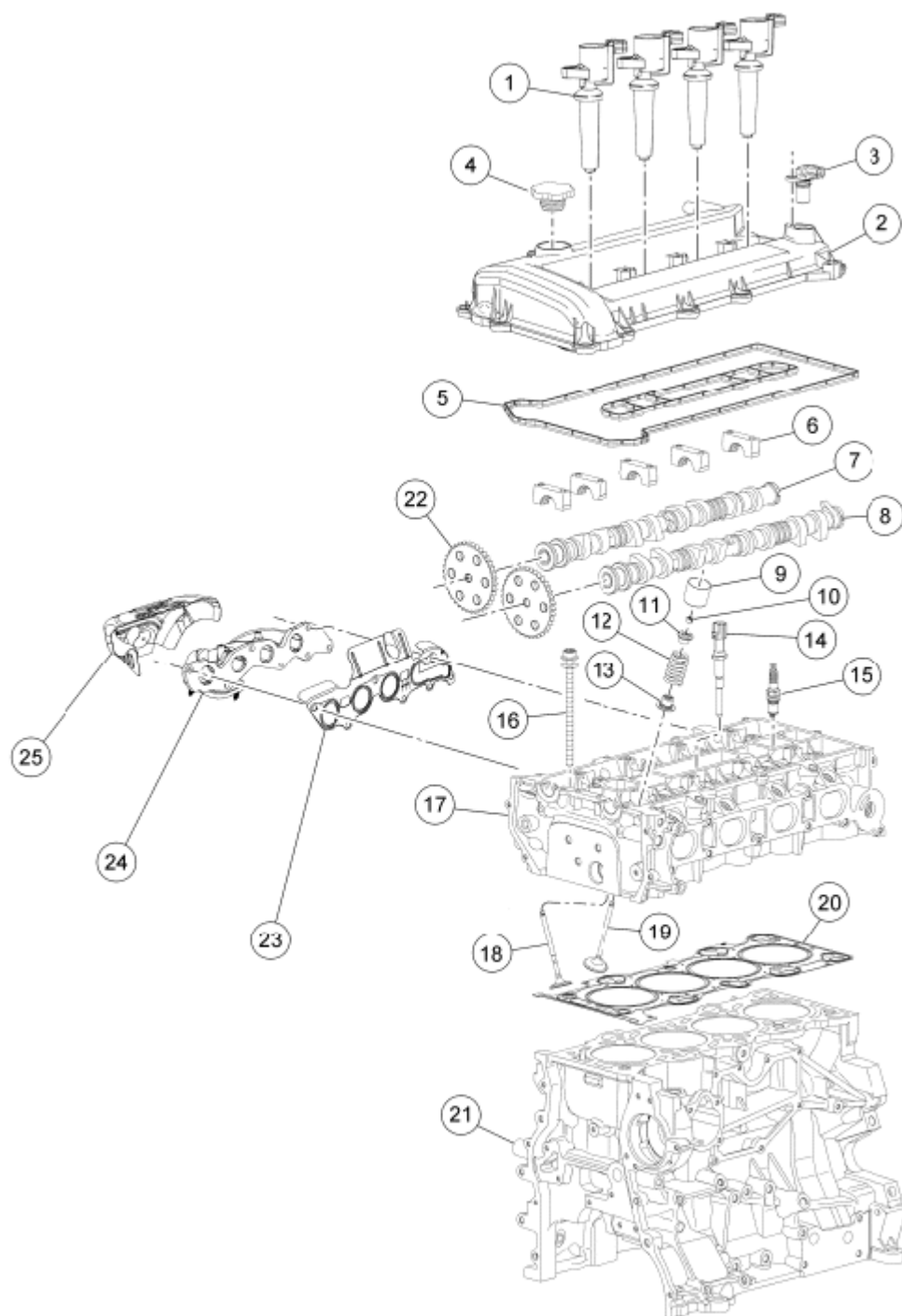
Fig. 292: Identifying Cylinder Head Components Courtesy of FORD MOTOR CO.
