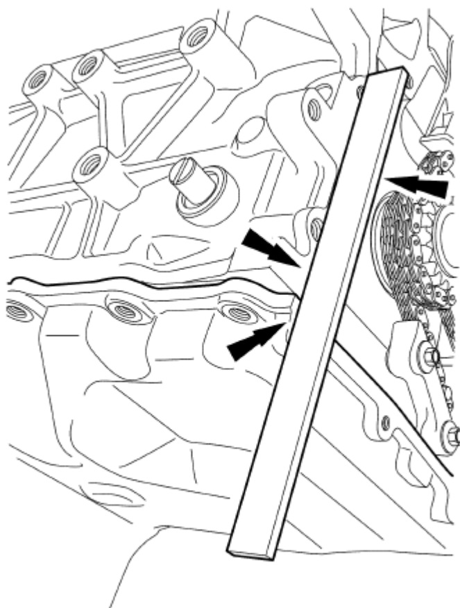
Fig. 143: Aligning Front Surface Of Oil Pan Flush Courtesy of FORD MOTOR CO.
