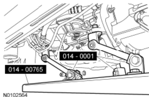
Fig. 401: Lifting Engine And Transaxle Assembly Courtesy of FORD MOTOR CO.
