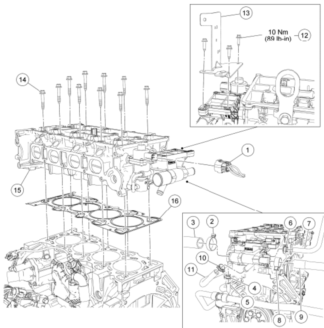
Fig. 117: Identifying Cylinder Head Components With Torque Specifications (2 Of 2)
