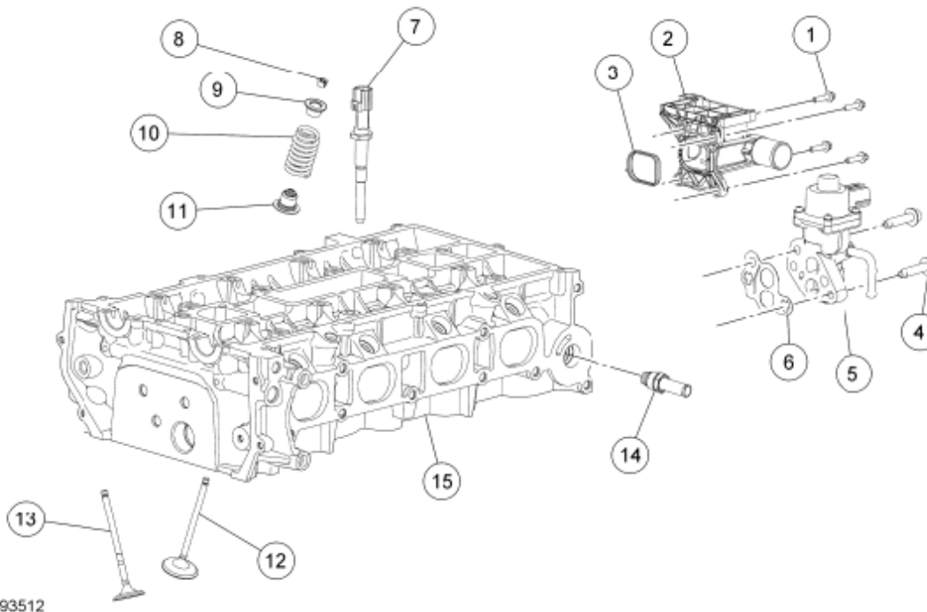
Fig. 280: Identifying Cylinder Head, EGR Tube, Exhaust Valve And EGR Valve Courtesy of FORD MOTOR CO.
