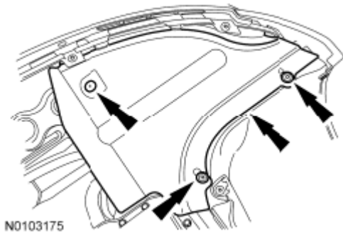
Fig. 152: Locating LH Front Splash Shield Bolts Courtesy of FORD MOTOR CO.
