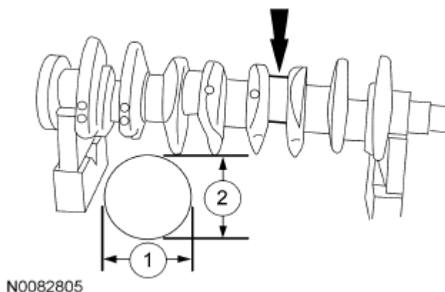
Fig. 301: Measuring Crankshaft Connecting Rod Bearing Journal Diameters Courtesy of FORD MOTOR CO.
