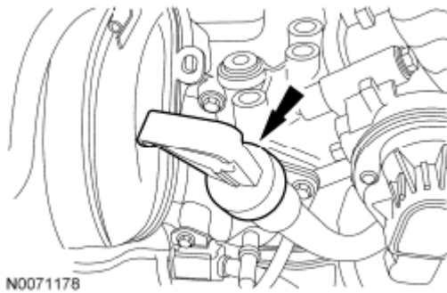
Fig. 183: Locating Transaxle Fluid Level Indicator Courtesy of FORD MOTOR CO.
