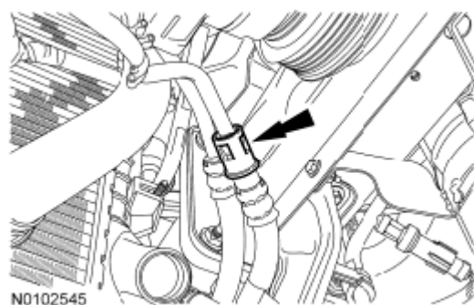
Fig. 432: Locating Power Steering Cooler Tube Courtesy of FORD MOTOR CO.
