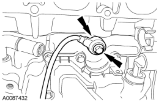
Fig. 365: Locating KS And Bolts Courtesy of FORD MOTOR CO.
