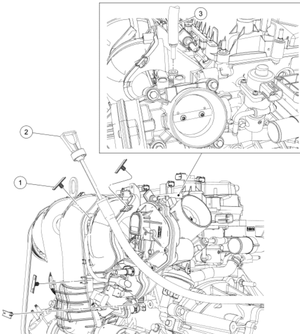
Fig. 6: Identifying Intake Manifold Components (2 Of 3)
