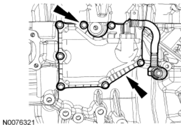
Fig. 244: Locating Crankcase Vent Oil Separator And Bolts Courtesy of FORD MOTOR CO.
