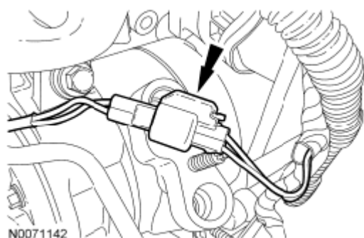
Fig. 415: Locating A/C Compressor Electrical Connector Courtesy of FORD MOTOR CO.
