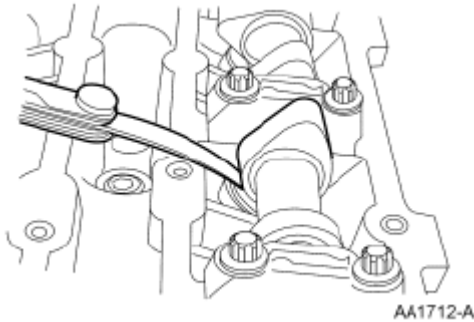
Fig. 4: Measuring Valve's Clearance Courtesy of FORD MOTOR CO.
