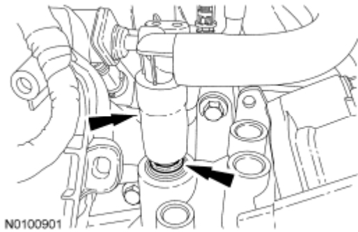
Fig. 10: Locating Quick Release Locking Ring Courtesy of FORD MOTOR CO.
