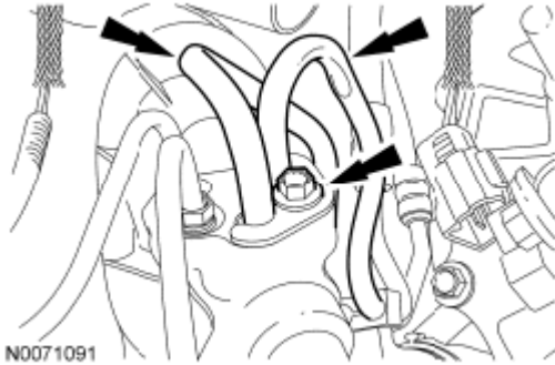
Fig. 433: Locating Power Steering Tube O-Ring Seals Courtesy of FORD MOTOR CO.
