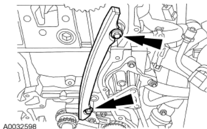
Fig. 69: Locating LH Timing Chain Guide And Bolts Courtesy of FORD MOTOR CO.
