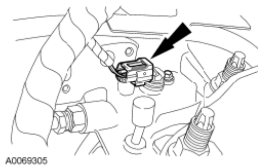
Fig. 194: Locating Turbine Shaft Speed Sensor Electrical Connector Courtesy of FORD MOTOR CO.
