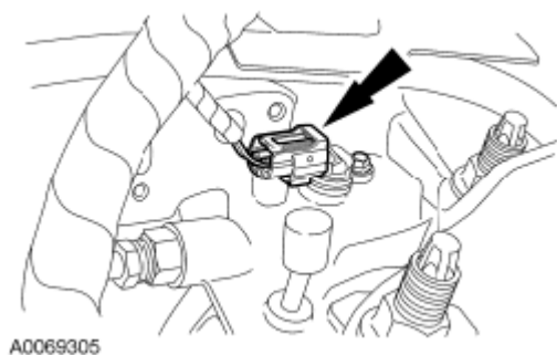
Fig. 417: Locating Turbine Shaft Speed Sensor Electrical Connector Courtesy of FORD MOTOR CO.
