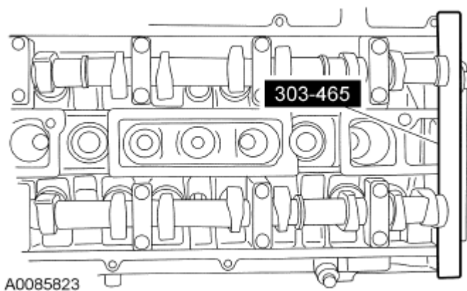
Fig. 97: Installing Camshaft Alignment Plate Courtesy of FORD MOTOR CO.
