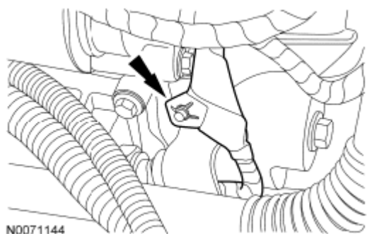
Fig. 201: Locating Starter Wire Harness Retainer And Starter Motor Stud Bolt Courtesy of FORD MOTOR CO.
