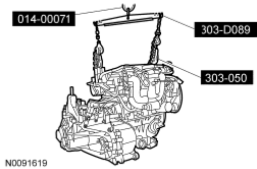
Fig. 210: Lifting Transaxle Assembly Courtesy of FORD MOTOR CO.
