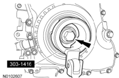
Fig. 253: Locating Diamond Washer Courtesy of FORD MOTOR CO.
