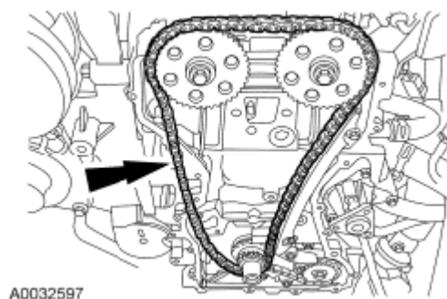
Fig. 73: Locating Timing Chain Courtesy of FORD MOTOR CO.
