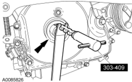
Fig. 44: Removing Crankshaft Front Oil Seal Courtesy of FORD MOTOR CO.
