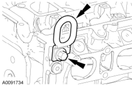
Fig. 286: Locating Lifting Eyes And Bolts Courtesy of FORD MOTOR CO.
