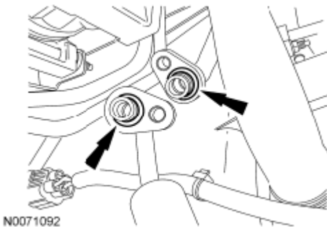
Fig. 172: Locating A/C Tubes From Compressor Courtesy of FORD MOTOR CO.
