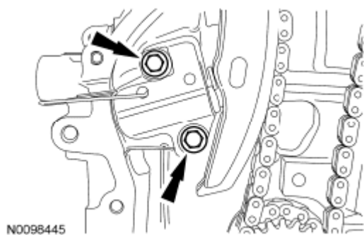
Fig. 258: Identifying Timing Chain Tensioner And Bolts Courtesy of FORD MOTOR CO.
