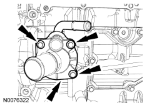
Fig. 367: Locating Thermostat Housing, Thermostat And Bolts Courtesy of FORD MOTOR CO.
