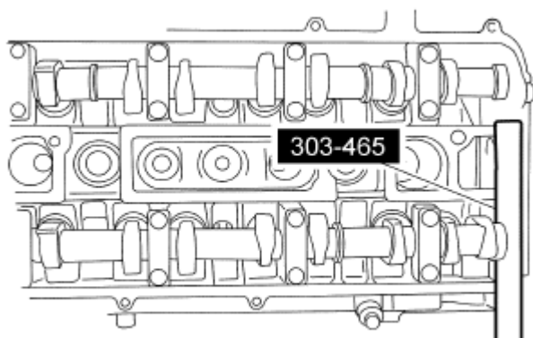
Fig. 90: Removing Camshaft Alignment Plate Courtesy of FORD MOTOR CO.
