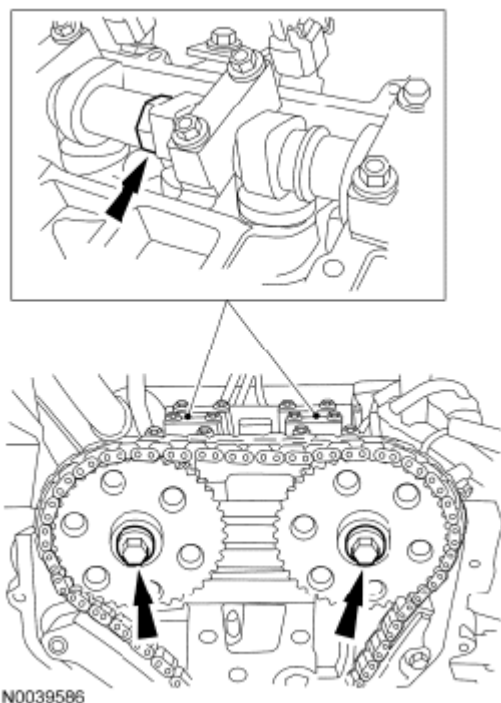
Fig. 101: Locating Camshaft Drive Gear Bolts Courtesy of FORD MOTOR CO.
