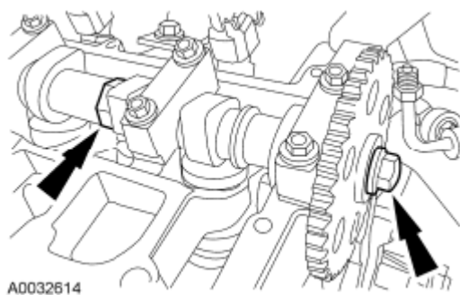
Fig. 70: Locating Camshaft Drive Gears And Bolts Courtesy of FORD MOTOR CO.
