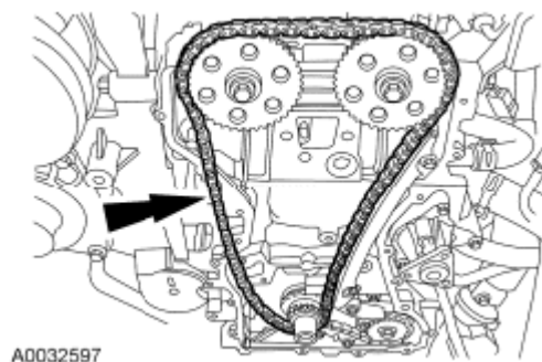
Fig. 260: Locating Timing Chain Courtesy of FORD MOTOR CO.
