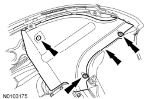
Fig. 457: Locating Splash Shield, Pin-Type Retainer And Bolts Courtesy of FORD MOTOR CO.
