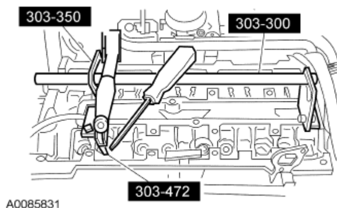
Fig. 111: Removing Valve Spring Retainer And Valve Spring Courtesy of FORD MOTOR CO.
