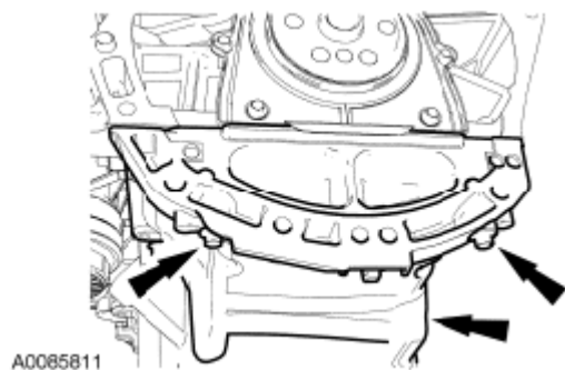
Fig. 142: Locating Rear Oil Pan Bolts Courtesy of FORD MOTOR CO.
