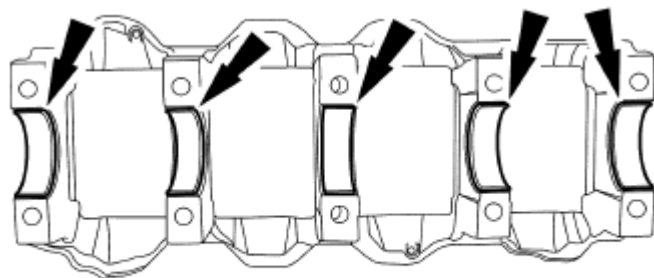
Fig. 277: Locating Main Bearings From Main Bearing Beam Courtesy of FORD MOTOR CO.
