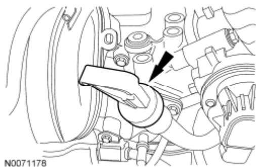
Fig. 427: Locating Transaxle Fluid Level Indicator Courtesy of FORD MOTOR CO.
