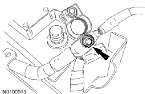
Fig. 455: Locating Positive Battery Cable Terminal Nut Courtesy of FORD MOTOR CO.
