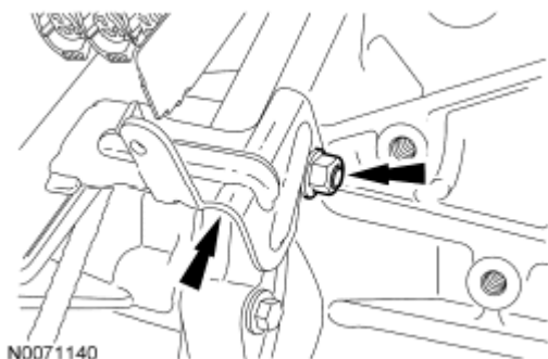
Fig. 419: Locating HO2S And CMS Wire Connector Bracket Aside Courtesy of FORD MOTOR CO.
