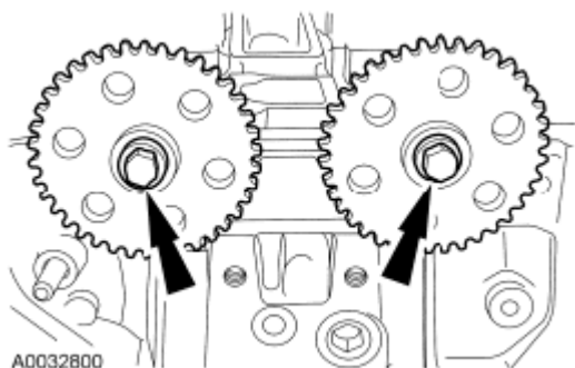
Fig. 71: Locating Camshaft Drive Gears And Bolts Courtesy of FORD MOTOR CO.
