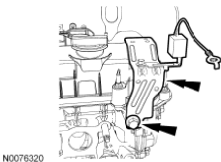
Fig. 371: Locating Radio Interference Capacitor Bracket Bolt And Bracket Aside
