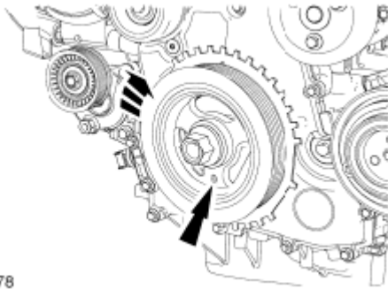
Fig. 81: Turning Crankshaft To Position Courtesy of FORD MOTOR CO.
