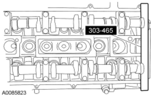
Fig. 40: Installing Camshaft Alignment Plate Courtesy of FORD MOTOR CO.
