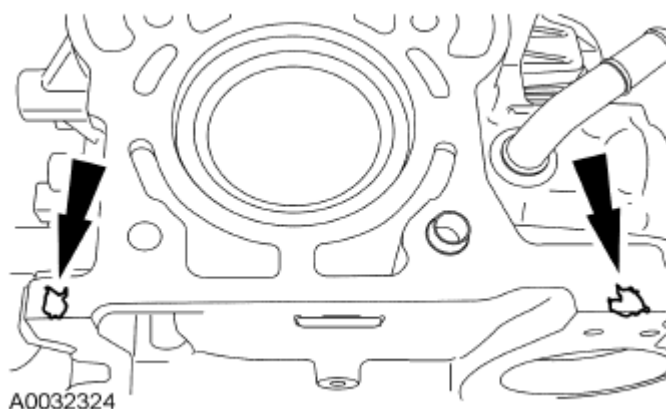
Fig. 122: Locating Cylinder Head Sealant Location Courtesy of FORD MOTOR CO.
