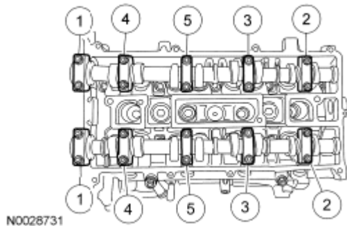
Fig. 95: Identifying Camshaft Bearing Cap Bolts Loosening Sequence Courtesy of FORD MOTOR CO.
