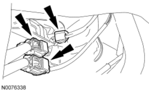
Fig. 165: Locating Heated Oxygen Sensor And Catalyst Monitor Sensor Electrical Connectors Courtesy of FORD MOTOR CO.
