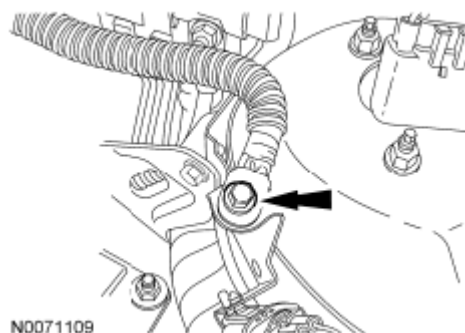
Fig. 156: Locating Negative Battery Cable Ground Bolt Courtesy of FORD MOTOR CO.
