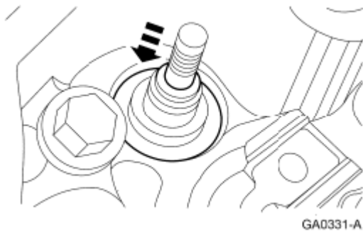
Fig. 282: Removing Valves Courtesy of FORD MOTOR CO.
