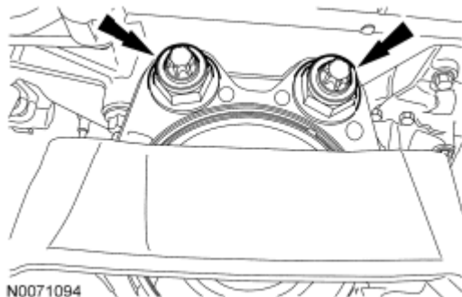
Fig. 423: Locating Engine Mount Nuts Courtesy of FORD MOTOR CO.
