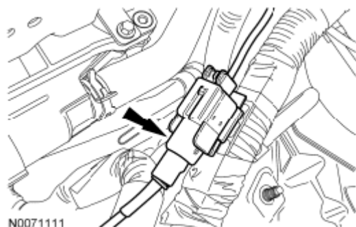
Fig. 445: Locating Starter Wire Harness Electrical Connector Courtesy of FORD MOTOR CO.
