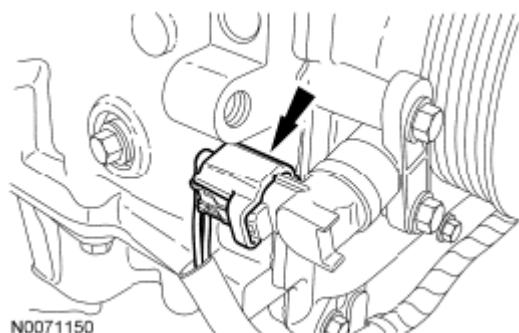
Fig. 200: Locating CKP Sensor Electrical Connector Courtesy of FORD MOTOR CO.
