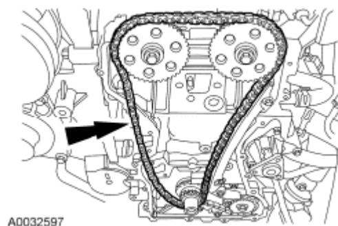
Fig. 333: Locating Timing Chain Courtesy of FORD MOTOR CO.
