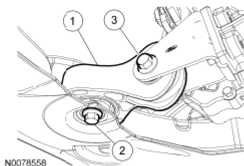
Fig. 426: Locating Intake Manifold Mounting Bolts Courtesy of FORD MOTOR CO.
