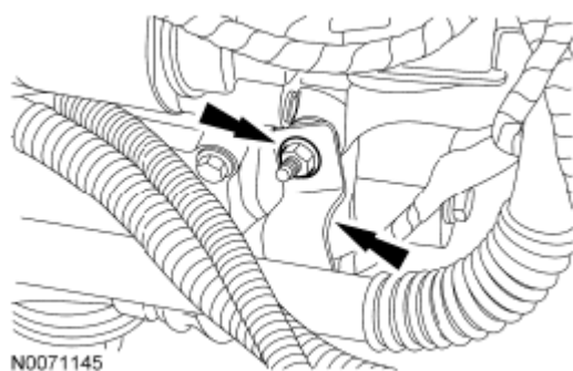
Fig. 202: Locating Starter Motor Stud Bolt And Power Steering Tube Bracket Courtesy of FORD MOTOR CO.
