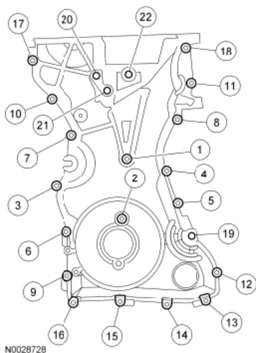
Fig. 58: Identifying Engine Front Cover Bolts Tightening Sequence Courtesy of FORD MOTOR CO.
