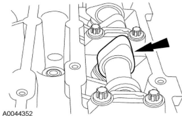
Fig. 120: Locating Camshaft Lobes On No. 1 Cylinder
