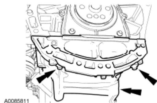
Fig. 318: Locating Oil Pan Bolts Courtesy of FORD MOTOR CO.
