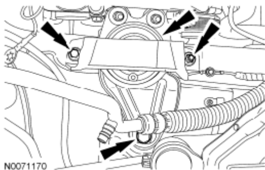
Fig. 189: Locating Engine Mount Bolts Courtesy of FORD MOTOR CO.
