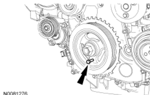
Fig. 351: Locating Crankshaft Pulley Bolt Courtesy of FORD MOTOR CO.
