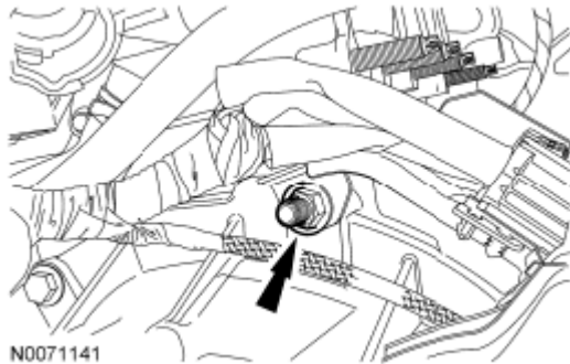
Fig. 191: Locating HO2S And CMS Wire Connector Bracket Courtesy of FORD MOTOR CO.
