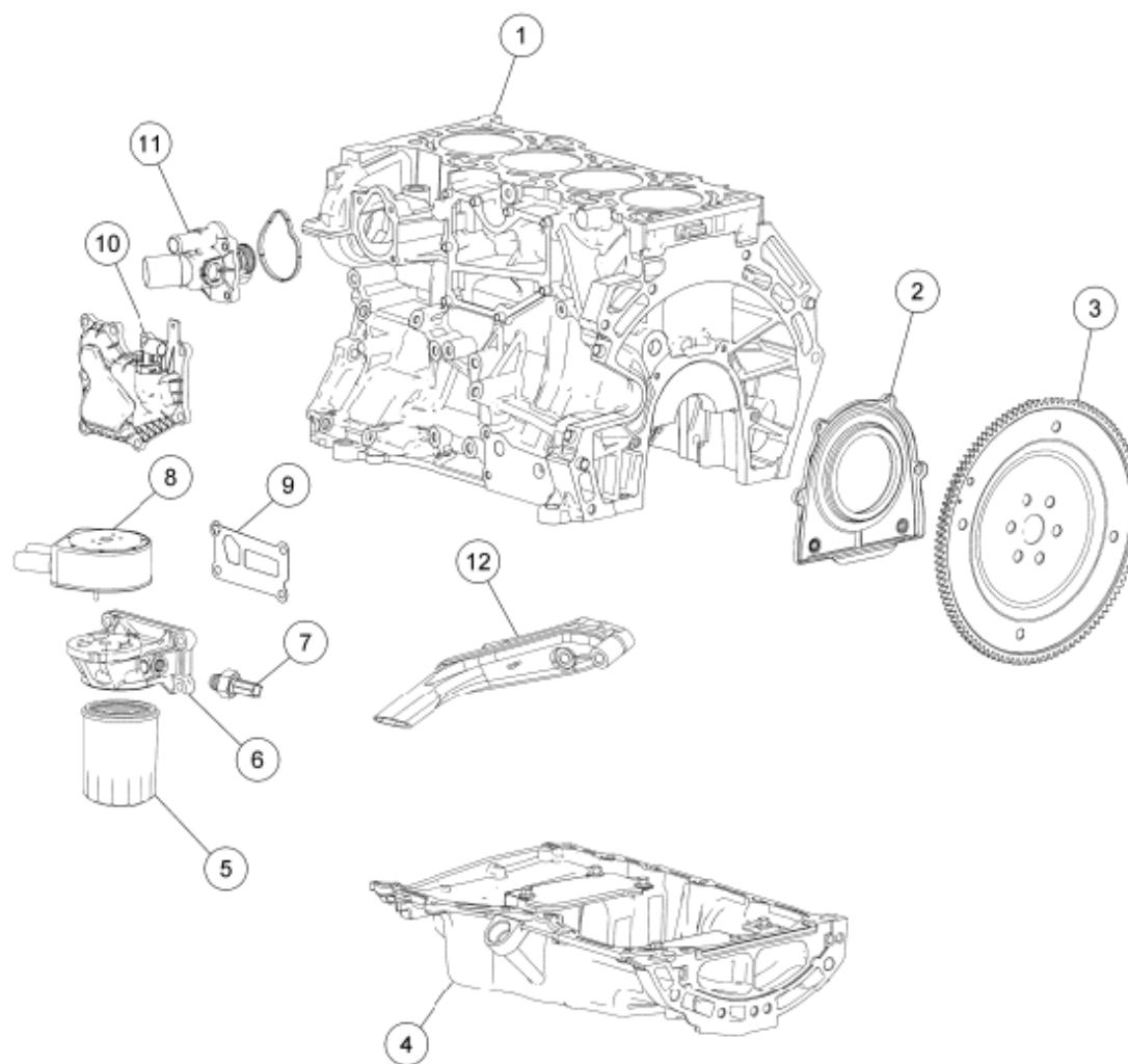
Fig. 289: Identifying Lower Engine Block Components (1 Of 3) Courtesy of FORD MOTOR CO.
