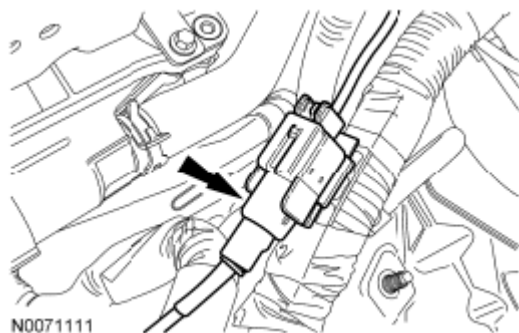
Fig. 164: Locating Starter Wire Harness Electrical Connector Courtesy of FORD MOTOR CO.
