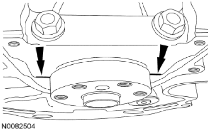
Fig. 296: Positioning Main Bearing Beam In Engine Block Courtesy of FORD MOTOR CO.
