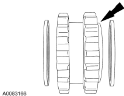
Fig. 326: Locating Crankshaft Sprocket Flange Courtesy of FORD MOTOR CO.
