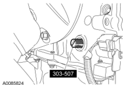
Fig. 37: Installing Crankshaft TDC Timing Peg Courtesy of FORD MOTOR CO.
