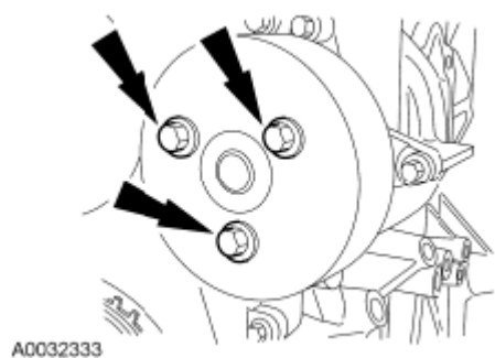
Fig. 214: Locating Coolant Pump Pulley And Bolts Courtesy of FORD MOTOR CO.
