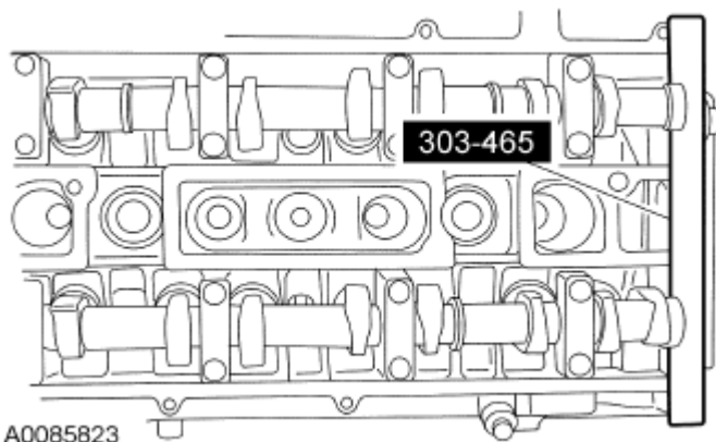
Fig. 82: Installing Camshaft Alignment Plate
