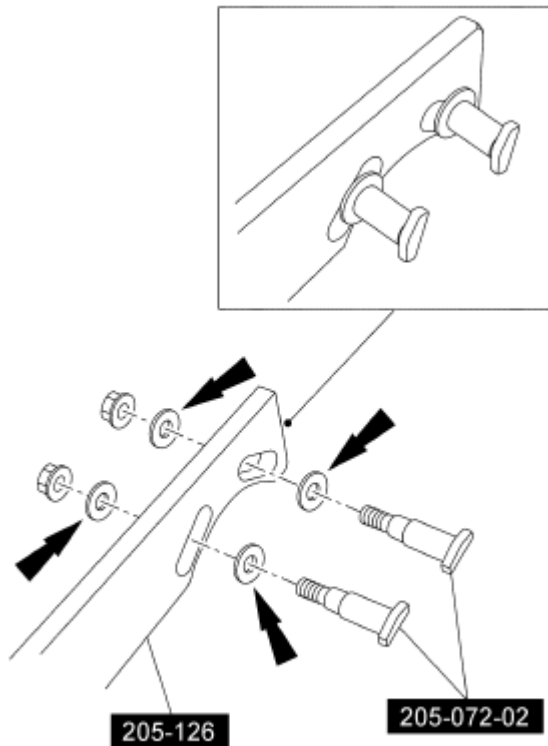
Fig. 42: Locating Special Tools And Hardened Washers Courtesy of FORD MOTOR CO.
