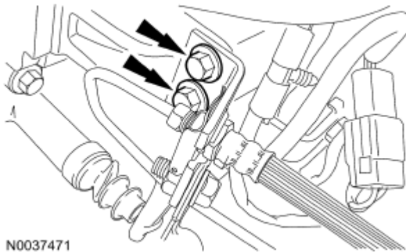
Fig. 295: Locating Clutch Tube Bracket Bolts Courtesy of FORD MOTOR CO.
