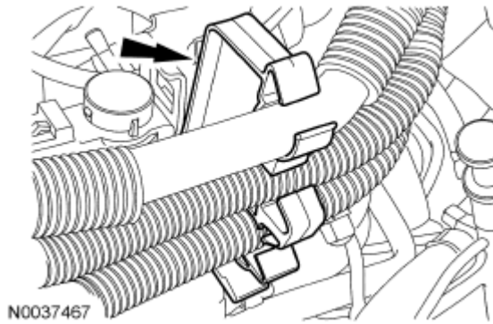
Fig. 168: Locating Retaining Clip Courtesy of FORD MOTOR CO.
