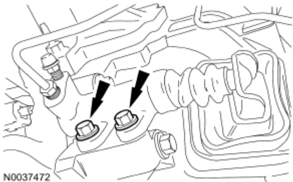
Fig. 296: Locating Clutch Slave Cylinder Bolts Courtesy of FORD MOTOR CO.
