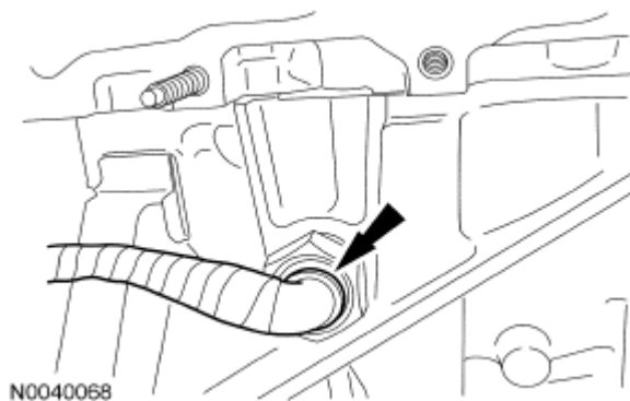
Fig. 539: Locating Block Heater Electrical Connector
