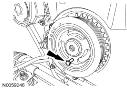
Fig. 41: Locating Bolt Courtesy of FORD MOTOR CO.
