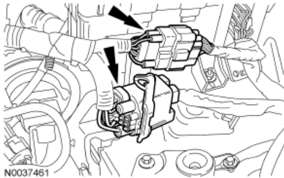
Fig. 285: Locating Engine Wiring Harness Electrical Connectors Courtesy of FORD MOTOR CO.
