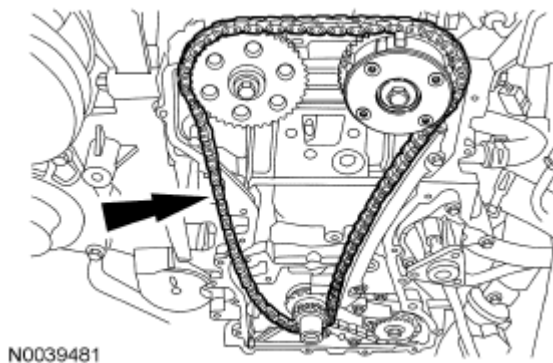
Fig. 479: Locating Timing Chain
