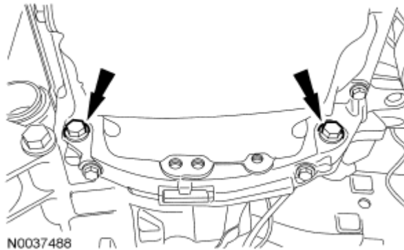
Fig. 244: Locating Oil Pan-To-Bellhousing Bolts Courtesy of FORD MOTOR CO.
