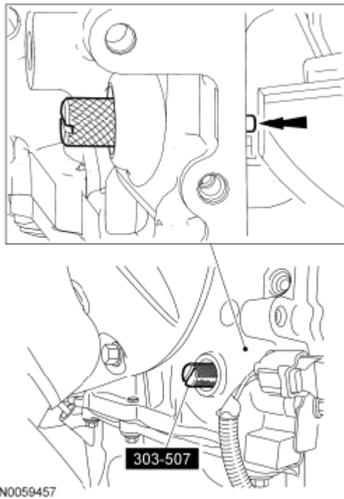
Fig. 2: Installing Crankshaft TDC Timing Peg
