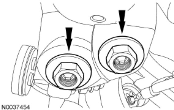
Fig. 623: Locating Lower Ball Joint Nuts Courtesy of FORD MOTOR CO.
