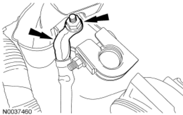
Fig. 220: Locating Battery Cable And Nut Courtesy of FORD MOTOR CO.
