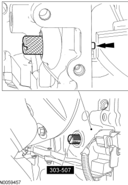
Fig. 412: Installing Crankshaft TDC Timing Peg
