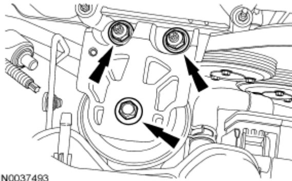
Fig. 587: Locating Engine Mount Bracket Nuts And Bolt Courtesy of FORD MOTOR CO.
