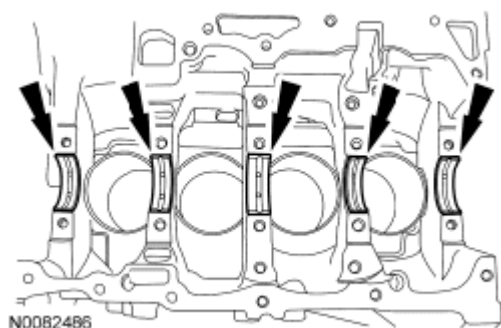
Fig. 421: Locating Main Bearings
