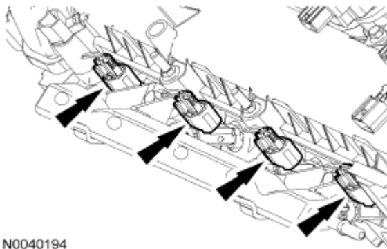
Fig. 381: Locating Fuel Injector Electrical Connectors Courtesy of FORD MOTOR CO.
