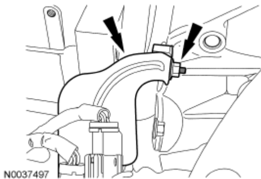
Fig. 581: Locating Engine Wiring Harness Bracket And Nut Courtesy of FORD MOTOR CO.
