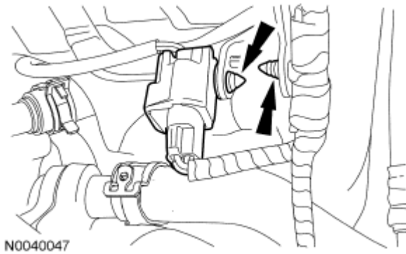
Fig. 563: Locating KS Electrical Connector And Harness Pin-Type Retainers Courtesy of FORD MOTOR CO.
