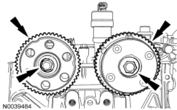
Fig. 85: Locating Camshaft Sprocket And Bolt Courtesy of FORD MOTOR CO.
