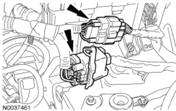
Fig. 221: Locating Electrical Connectors Courtesy of FORD MOTOR CO.
