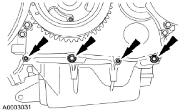
Fig. 64: Locating Oil Pan Bolts Courtesy of FORD MOTOR CO.
