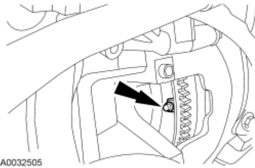
Fig. 583: Locating Torque Converter Nut Courtesy of FORD MOTOR CO.
