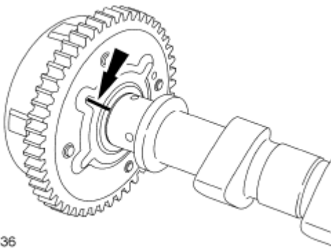
Fig. 138: Locating Mark On Camshaft Courtesy of FORD MOTOR CO.
