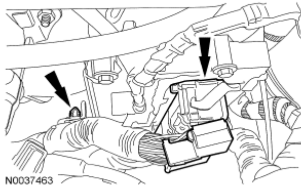
Fig. 612: Locating Powertrain Control Module (PCM) Electrical Connector And Pin-Type Retainer Courtesy of FORD MOTOR CO.
