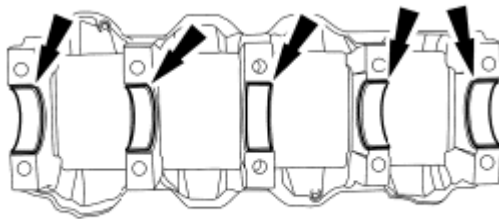
Fig. 420: Locating Main Bearings
