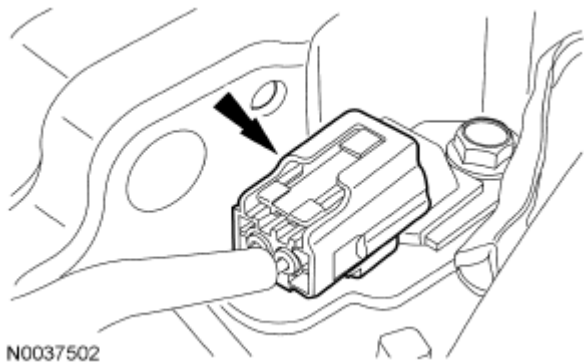
Fig. 578: Locating Turbine Shaft Speed (TSS) Sensor Electrical Connector Courtesy of FORD MOTOR CO.
