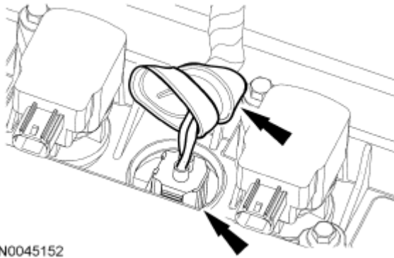
Fig. 379: Locating Cylinder Head Temperature (CHT) Sensor Electrical Connector Courtesy of FORD MOTOR CO.
