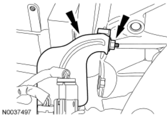
Fig. 254: Locating Engine Wiring Harness Bracket And Nut Courtesy of FORD MOTOR CO.
