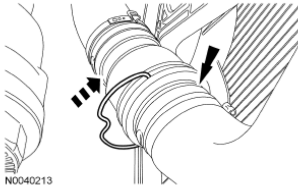
Fig. 595: Identifying Lower Radiator Hose And Installing Retaining Clip Courtesy of FORD MOTOR CO.
