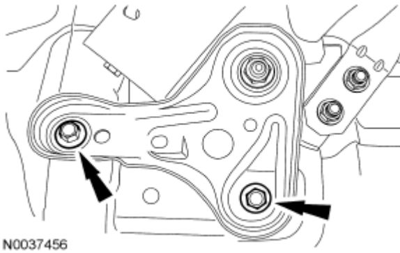
Fig. 215: Locating Subframe Bracket-To-Body Bolts
