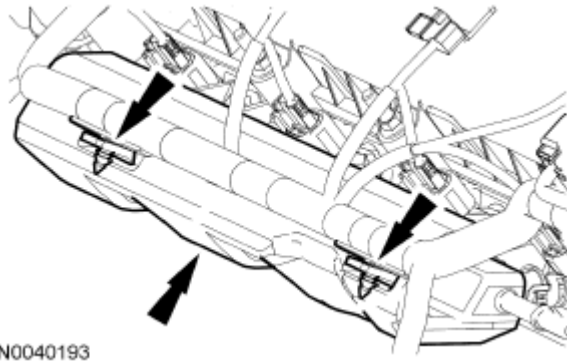
Fig. 380: Locating Pin-Type Harness Retainers And Remove Fuel Supply Rail Insulator Courtesy of FORD MOTOR CO.
