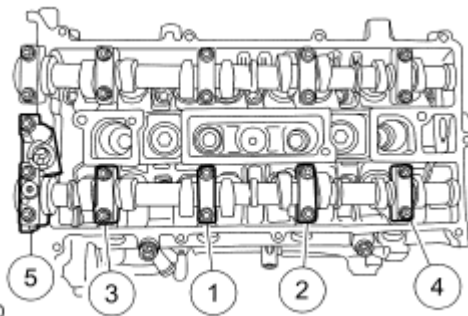
Fig. 140: Identifying Tightening Sequence Of Intake Camshaft Bearing Caps Bolts Courtesy of FORD MOTOR CO.
