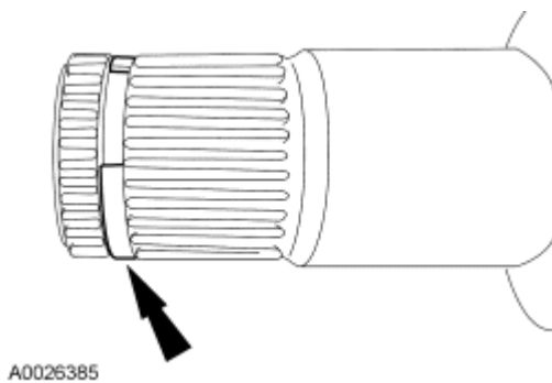
Fig. 594: Locating Halfshaft Circlip Courtesy of FORD MOTOR CO.
