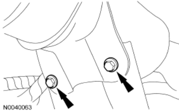
Fig. 354: Locating Catalytic Converter Bracket Bolts Courtesy of FORD MOTOR CO.
