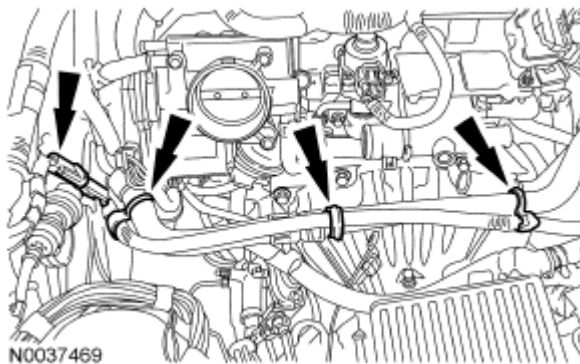
Fig. 664: Locating Block Heater Electrical Connector Harness Retaining Clips Courtesy of FORD MOTOR CO.
