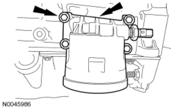
Fig. 520: Locating Oil Filter Adapter Bolts Courtesy of FORD MOTOR CO.
