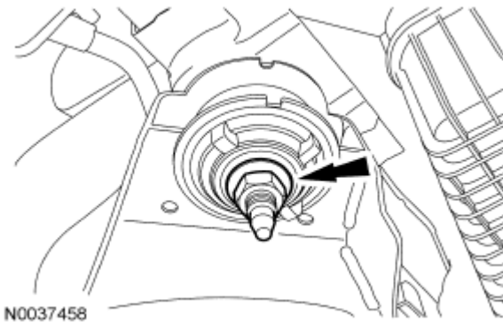
Fig. 281: Locating Front Subframe Nut Courtesy of FORD MOTOR CO.
