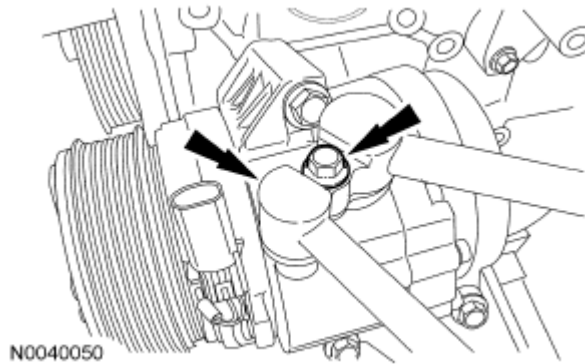
Fig. 335: Locating A/C Manifold And Bolt Courtesy of FORD MOTOR CO.
