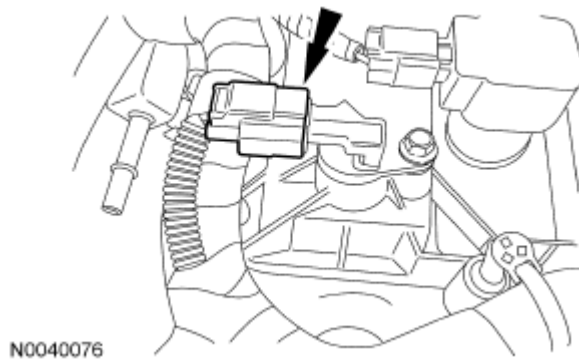
Fig. 376: Locating Camshaft Position (CMP) Sensor Electrical Connector Courtesy of FORD MOTOR CO.
