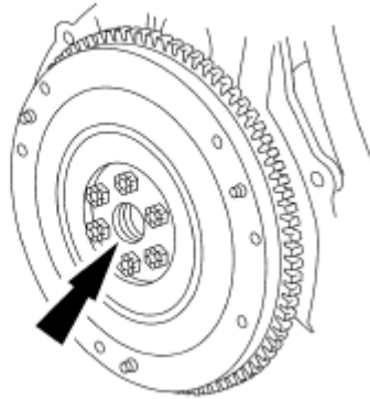
Fig. 573: Locating Front Axle Grease Area Courtesy of FORD MOTOR CO.
