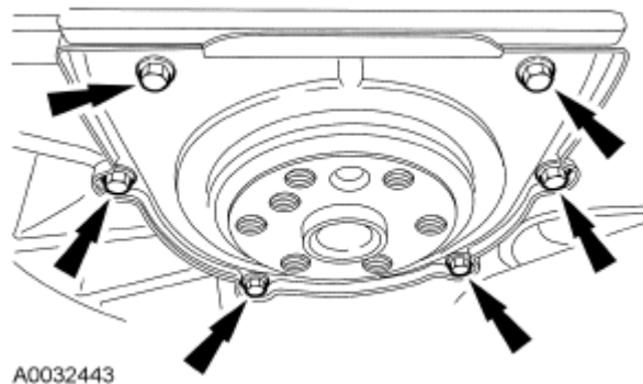
Fig. 409: Locating Rear Crankshaft Seal Bolts Courtesy of FORD MOTOR CO.
