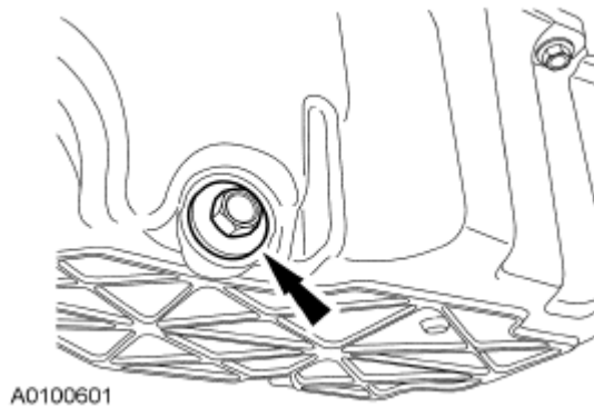
Fig. 218: Locating Drain Plug Courtesy of FORD MOTOR CO.
