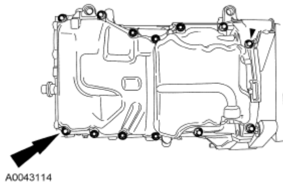
Fig. 408: Locating Oil Pan Bolts Courtesy of FORD MOTOR CO.
