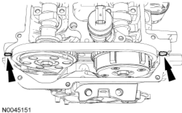
Fig. 28: Identifying Silicone Gasket Sealant Locations Courtesy of FORD MOTOR CO.
