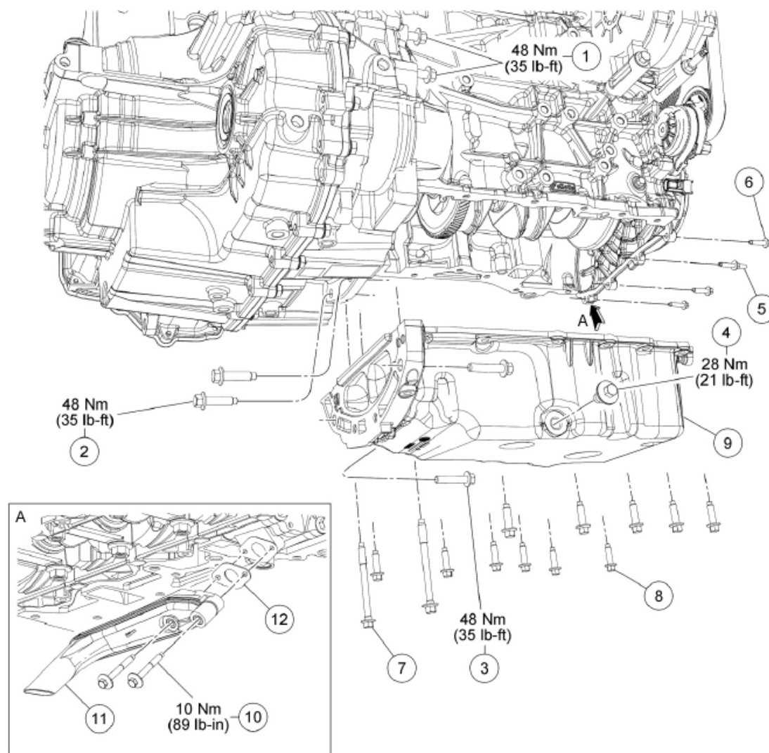
Fig. 171: Exploded View Of Oil Pan, Oil Pump Screen And Pickup Tube Components With Torque Specifications
