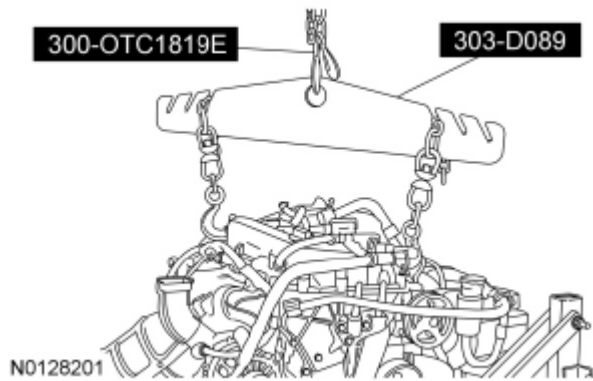
Fig. 252: Remove/Install Engine And Transaxle From Powertrain Lift Table Using Floor Crane And Spreader Bar
