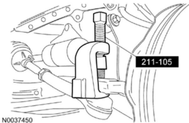
Fig. 273: Separating Tie-Rod Ends From Steering Knuckle Using Tie-Rod End Remover Courtesy of FORD MOTOR CO.
