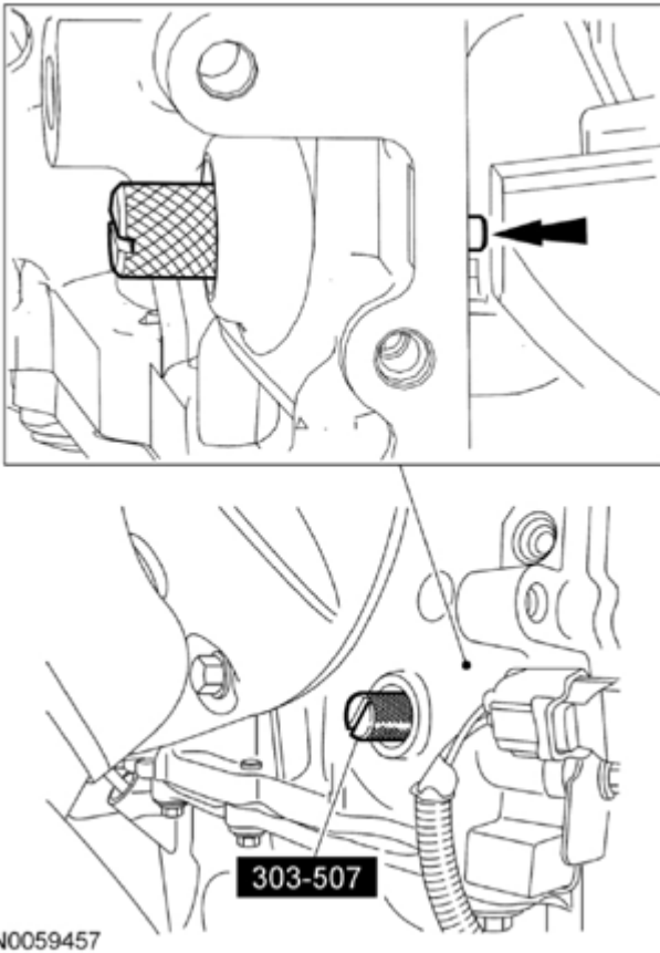
Fig. 366: Remove/Install Crankshaft TDC Timing Peg Courtesy of FORD MOTOR CO.
