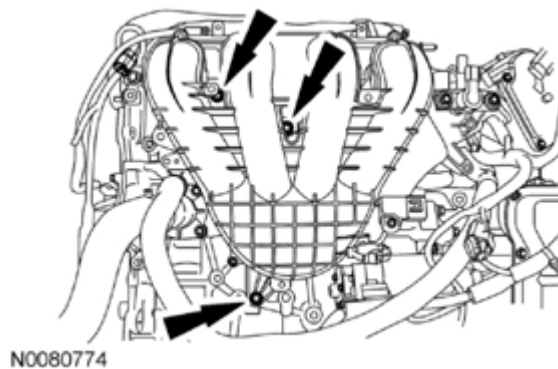
Fig. 500: Locating Intake Manifold Bolts
