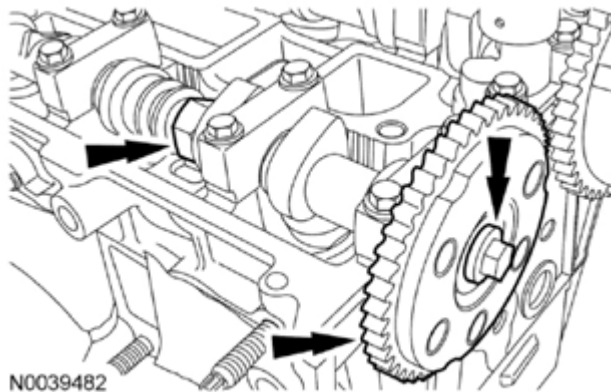
Fig. 375: Locating Exhaust Camshaft Sprocket Bolts
