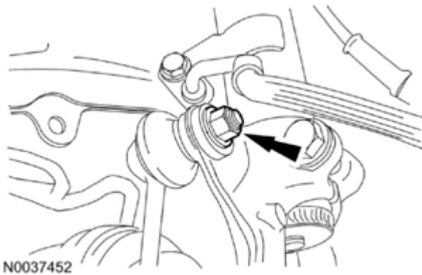
Fig. 580: Locating Sway Bar Link Nut Courtesy of FORD MOTOR CO.
