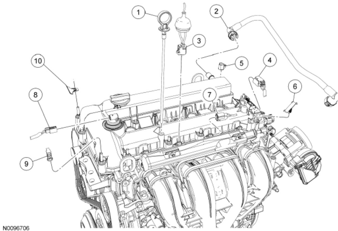
Fig. 22: Exploded View Of Valve Cover Components (View 1 Of 2) Courtesy of FORD MOTOR CO.
