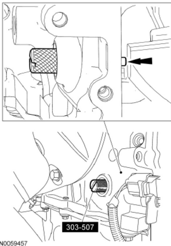
Fig. 41: Remove/Install Crankshaft TDC Timing Peg Courtesy of FORD MOTOR CO.
