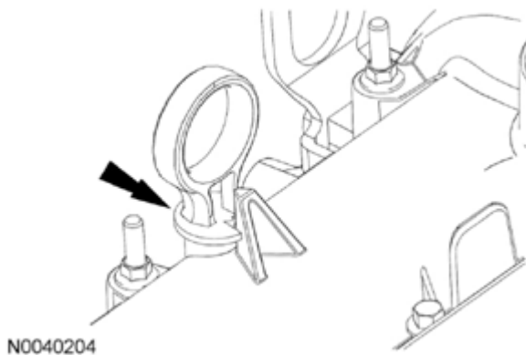
Fig. 359: Locating Oil Level Indicator
