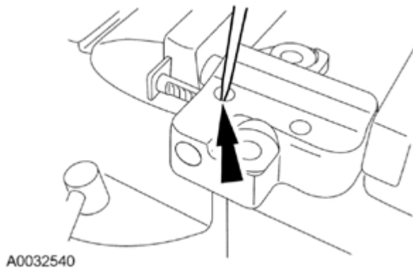
Fig. 465: View Of Pushing Ratchet Mechanism Using A Small Pick Courtesy of FORD MOTOR CO.
