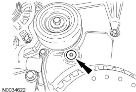
Fig. 95: Locating Lower Front Cover Timing Hole Plug Courtesy of FORD MOTOR CO.
