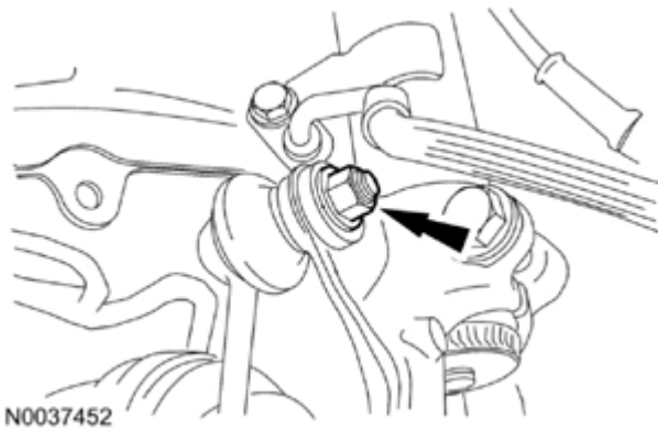
Fig. 638: Locating Sway Bar Link Nut Courtesy of FORD MOTOR CO.
