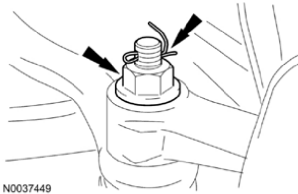
Fig. 272: Locating Cotter Pin And Nut On Tie-Rod Ends Courtesy of FORD MOTOR CO.
