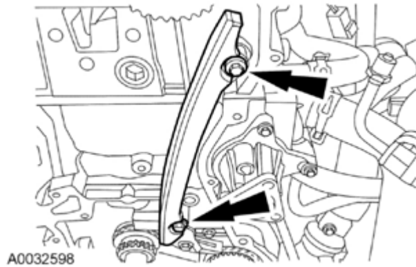
Fig. 374: Locating LH Timing Chain Guide Bolts
