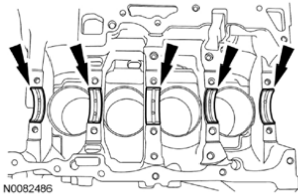
Fig. 398: Locating Main Bearings Of Cylinder Block Courtesy of FORD MOTOR CO.
