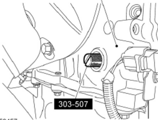
Fig. 122: Remove/Install Crankshaft TDC Timing Peg Courtesy of FORD MOTOR CO.
