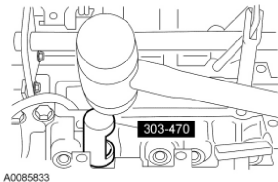
Fig. 153: Installing Valve Seal Using Valve Stem Oil Seal Installer
