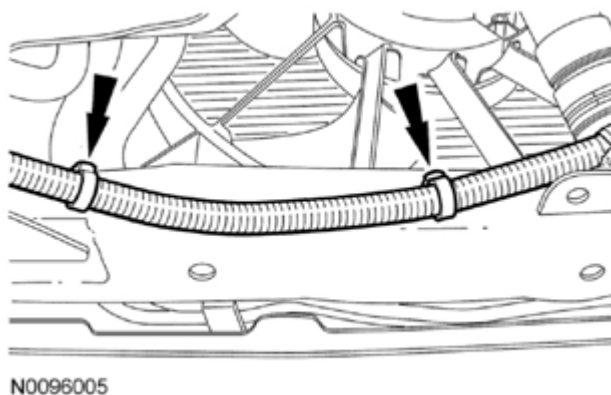
Fig. 269: Locating EPAS System Wiring Harness Pin-Type Retainers Of Subframe Courtesy of FORD MOTOR CO.
