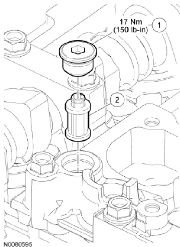
Fig. 88: Identifying Variable Camshaft Timing (VCT) System Oil Filter Components With Torque Specifications
