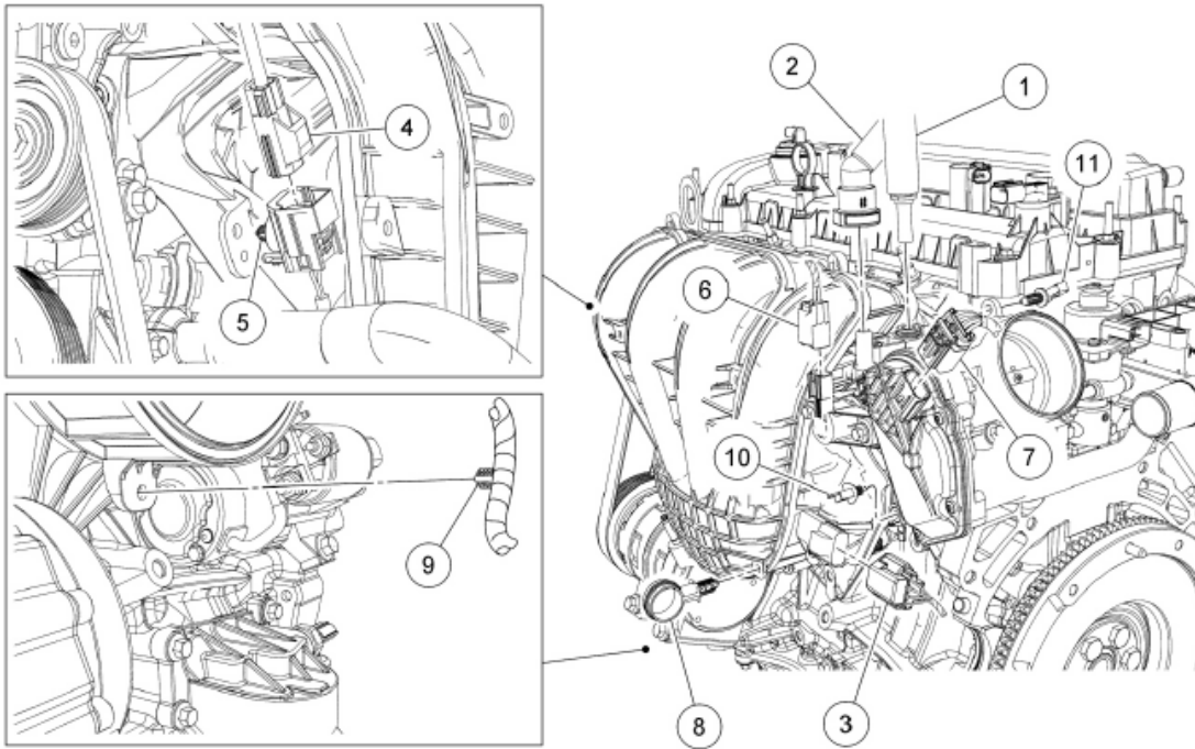
Fig. 17: Identifying Intake Manifold Components (View 1 Of 2) Courtesy of FORD MOTOR CO.
