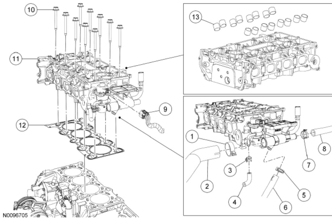
Fig. 158: Exploded View Of Cylinder Head Components Courtesy of FORD MOTOR CO.
