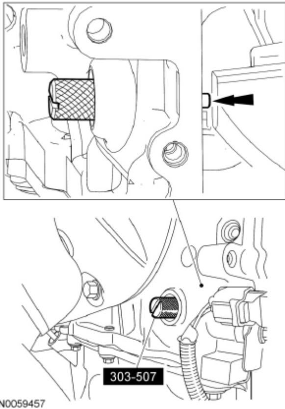
Fig. 13: Remove/Install Crankshaft TDC Timing Peg Courtesy of FORD MOTOR CO.
