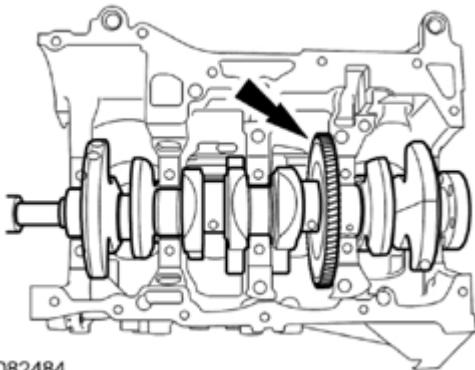
Fig. 427: Locating Crankshaft
