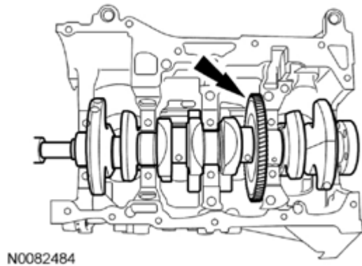
Fig. 396: Locating Crankshaft Courtesy of FORD MOTOR CO.
