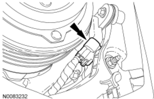
Fig. 591: Locating Crankshaft Position (CKP) Sensor Electrical Connector Courtesy of FORD MOTOR CO.
