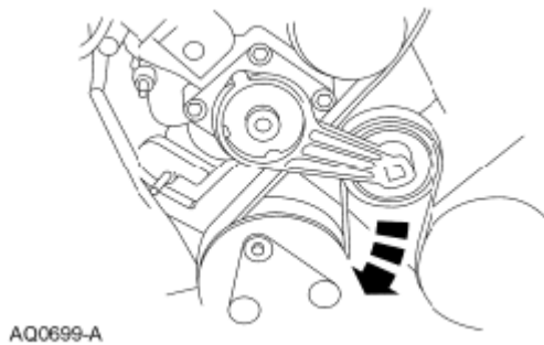
Fig. 83: Removing Accessory Drive Belt From Crankshaft Pulley Courtesy of FORD MOTOR CO.
