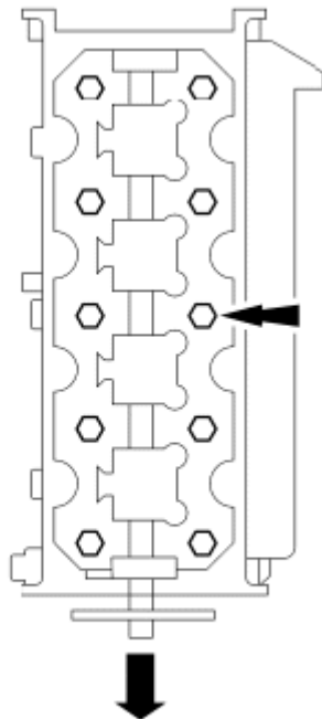
Fig. 385: Locating Cylinder Head Bolts Courtesy of FORD MOTOR CO.
