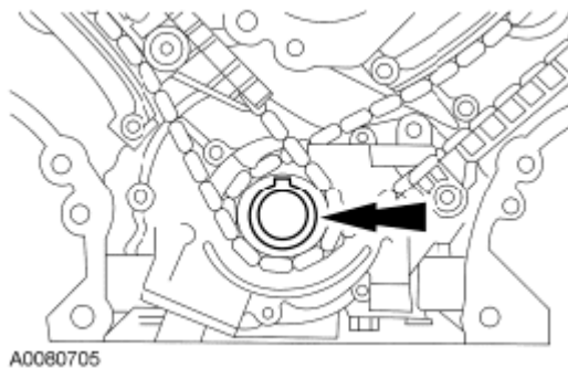
Fig. 357: Locating Crankshaft Keyway Courtesy of FORD MOTOR CO.
