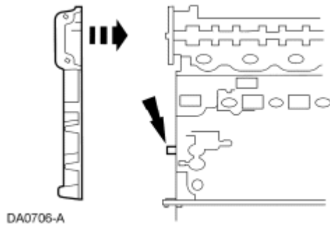
Fig. 69: Locating Engine Front Cover Gasket On Engine Front Cover Courtesy of FORD MOTOR CO.
