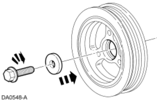
Fig. 42: Identifying Crankshaft Pulley Bolt And Washer Courtesy of FORD MOTOR CO.
