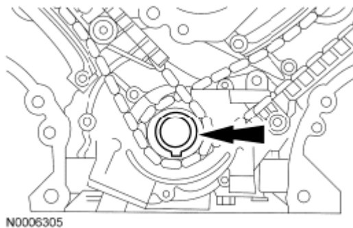
Fig. 430: Locating Crankshaft Keyway 6 O'Clock Position Courtesy of FORD MOTOR CO.
