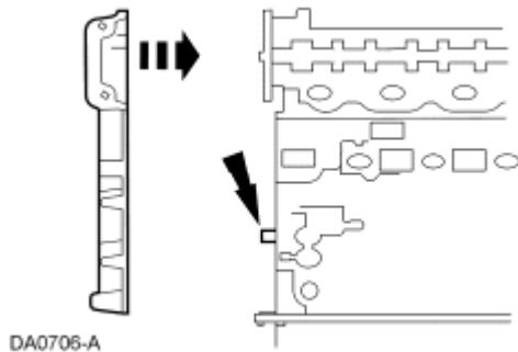
Fig. 511: Locating Engine Front Cover Gasket On Engine Front Cover Courtesy of FORD MOTOR CO.
