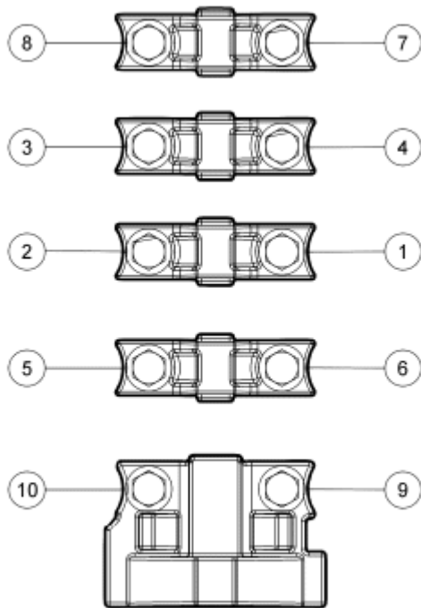
Fig. 104: Identifying Camshaft Bearing Caps Bolts In Tightening Sequence Courtesy of FORD MOTOR CO.
