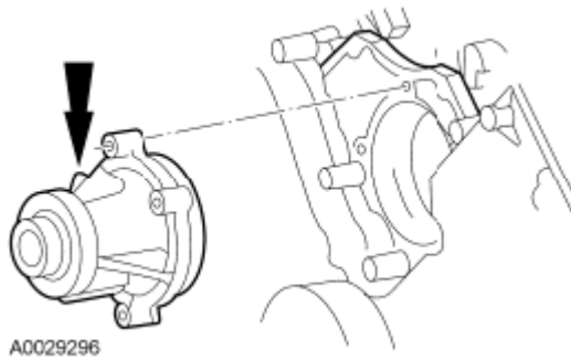
Fig. 515: Locating O-Ring Seal Onto Coolant Pump Courtesy of FORD MOTOR CO.
