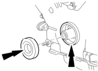
Fig. 636: Locating Engine Front Cover And Crankshaft Seal Inner Lip Courtesy of FORD MOTOR CO.
