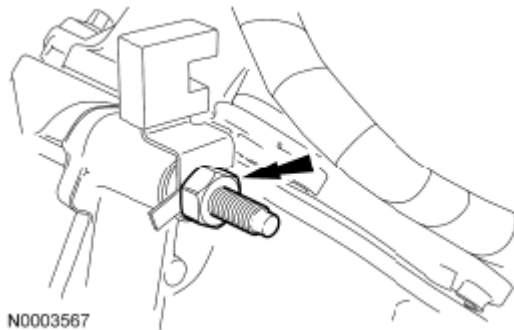
Fig. 398: Locating Nut And Radio Interference Capacitor LH Courtesy of FORD MOTOR CO.
