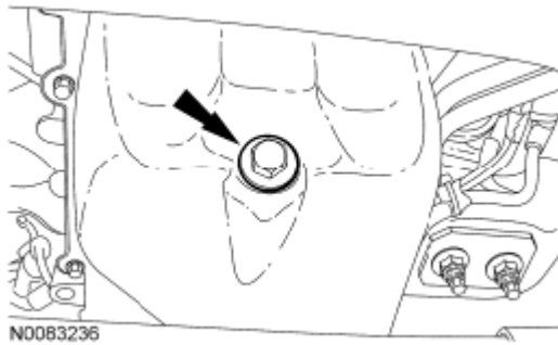
Fig. 306: Locating Drain Plug Courtesy of FORD MOTOR CO.
