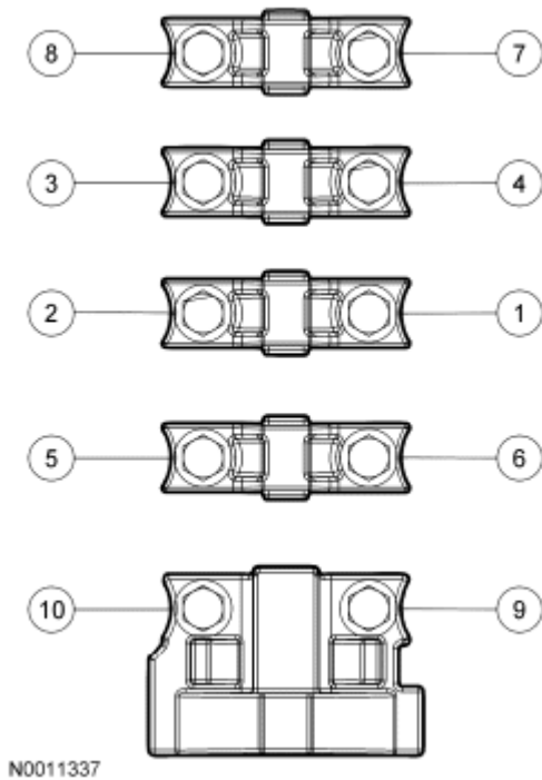
Fig. 140: Identifying Camshaft Bearing Caps Bolts In Tightening Sequence Courtesy of FORD MOTOR CO.
