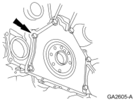
Fig. 549: Locating Crankshaft Rear Seal Retainer Plate And Bolts Courtesy of FORD MOTOR CO.
