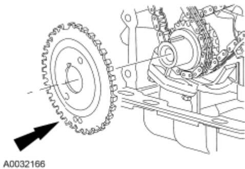
Fig. 423: Locating Crankshaft Sensor Ring On Crankshaft Courtesy of FORD MOTOR CO.
