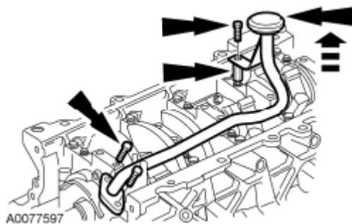
Fig. 447: Locating Bolts And Oil Pump Screen Courtesy of FORD MOTOR CO.
