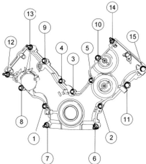
Fig. 512: Identifying Engine Front Cover Fasteners In Tightening Sequence Courtesy of FORD MOTOR CO.
