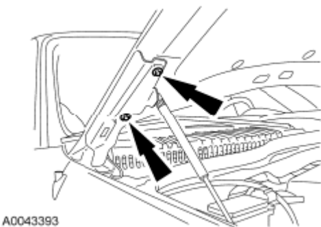
Fig. 592: Locating Hood And Bolts Courtesy of FORD MOTOR CO.
