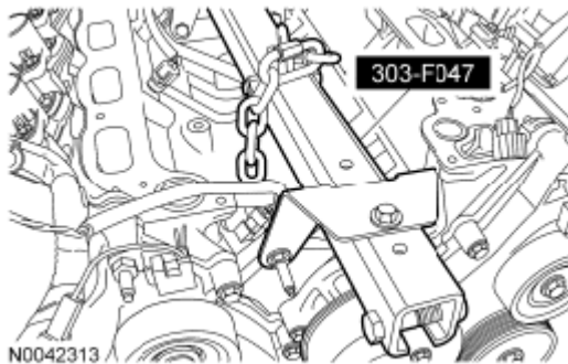
Fig. 649: Removing Engine Lifting Bracket Courtesy of FORD MOTOR CO.
