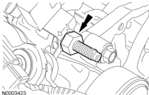
Fig. 545: Locating Nut And Radio Interference Capacitor RH Courtesy of FORD MOTOR CO.
