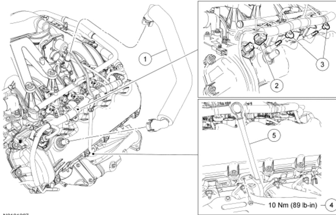
Fig. 17: Identifying PCV Tube, Engine Wiring Harness Retainers And Variable Camshaft Timing (VCT) Solenoid Electrical Connector Courtesy of FORD MOTOR CO.
