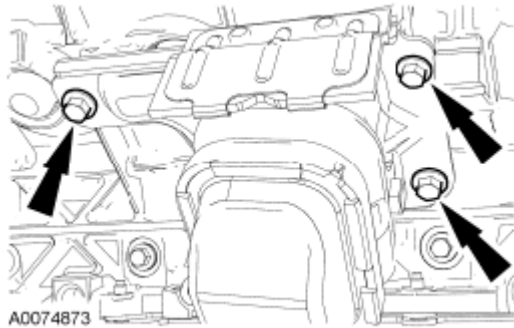
Fig. 337: Locating Engine Support Insulator And Bolts RH Courtesy of FORD MOTOR CO.
