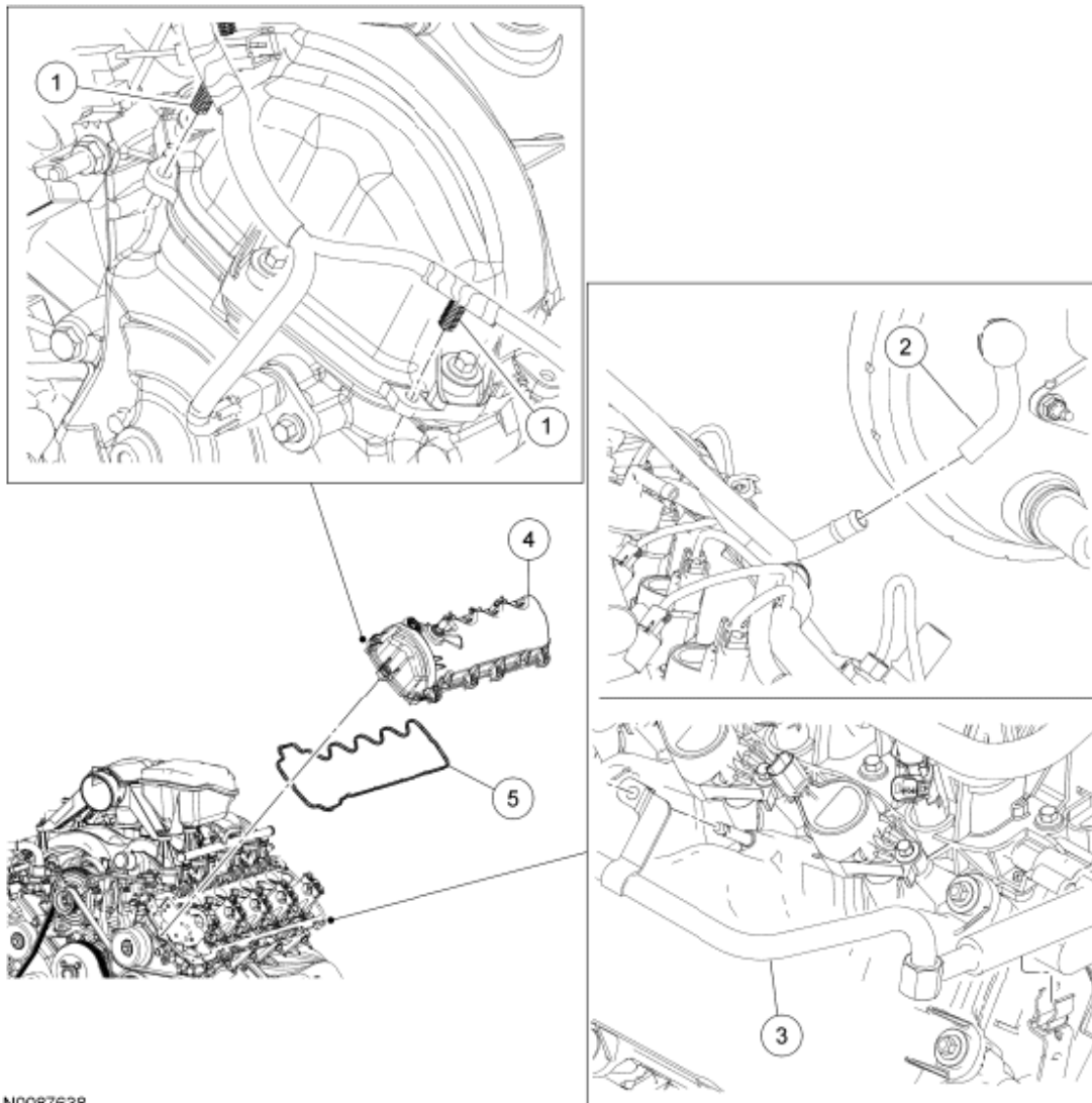
Fig. 18: Identifying Engine Wiring Harness Retainers, Intake Manifold Vacuum Tube, LH Valve Cover And Gasket
