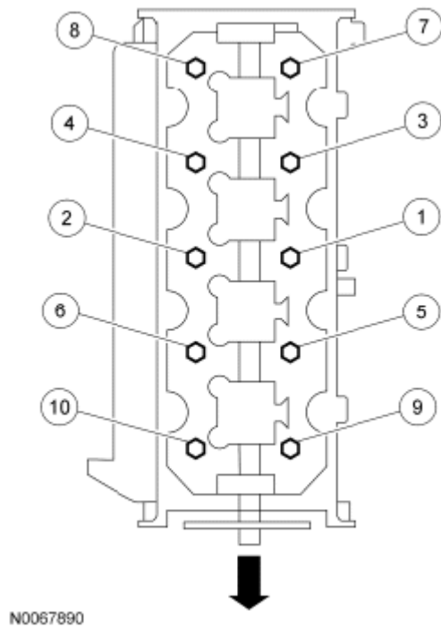
Fig. 487: Identifying Bolts In Tightening Sequence Courtesy of FORD MOTOR CO.
