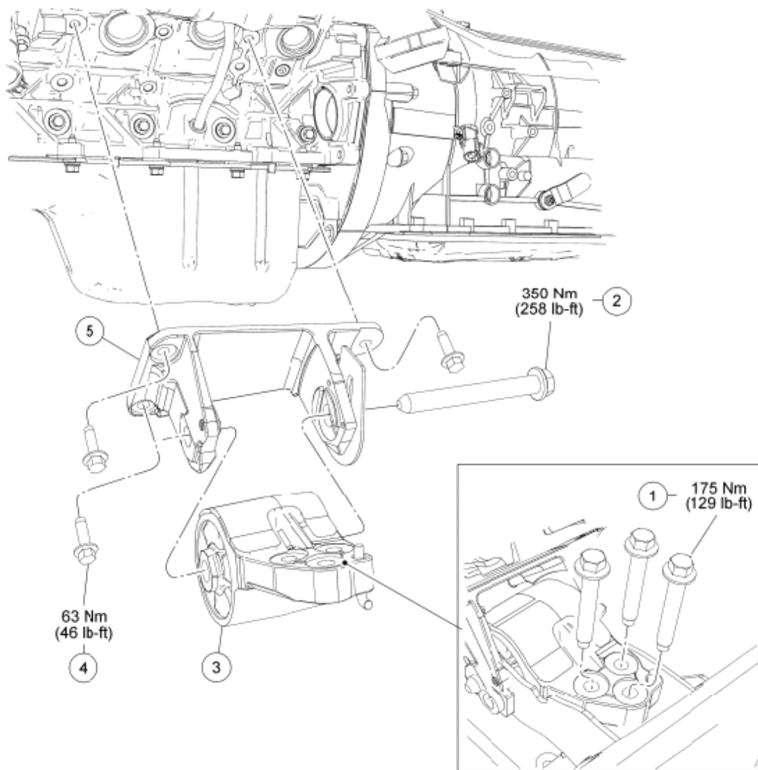
Fig. 281: Identifying Engine Support Insulator Components LH Courtesy of FORD MOTOR CO.
