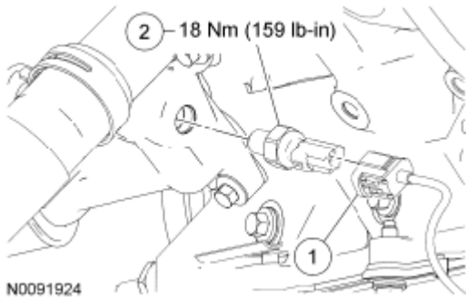
Fig. 265: Identifying Engine Oil Pressure (EOP) Switch Courtesy of FORD MOTOR CO.
