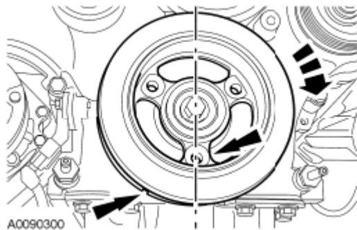
Fig. 154: Locating Timing Mark Indentation
