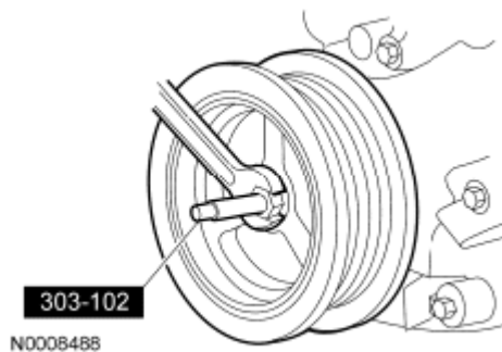
Fig. 520: Installing Crankshaft Pulley Courtesy of FORD MOTOR CO.
