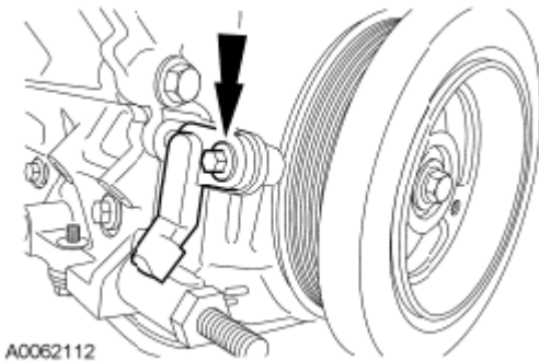
Fig. 522: Locating Bolt And Crankshaft Position (CKP) Sensor Courtesy of FORD MOTOR CO.
