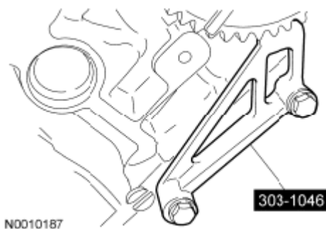
Fig. 608: Removing Camshaft Phaser And Sprocket Assembly With Bolt LH Courtesy of FORD MOTOR CO.
