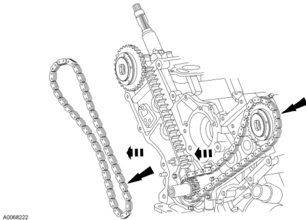
Fig. 366: Locating Timing Chains And Crankshaft Sprocket (RH And LH) Courtesy of FORD MOTOR CO.
