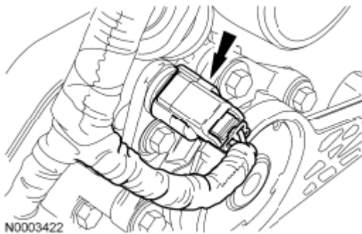
Fig. 207: Locating CMP Sensor Electrical Connector Courtesy of FORD MOTOR CO.
