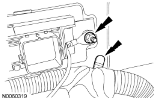
Fig. 32: Locating Wiring Harness Retainer And Nut
