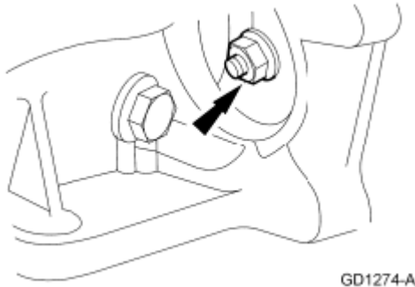
Fig. 564: Locating Torque Converter-To-Flexplate Nuts Courtesy of FORD MOTOR CO.
