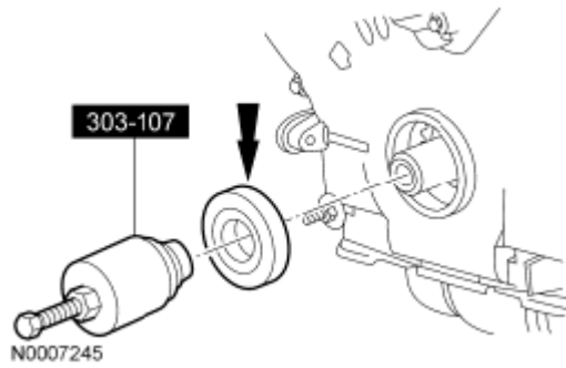
Fig. 419: Removing Discard Crankshaft Seal Courtesy of FORD MOTOR CO.
