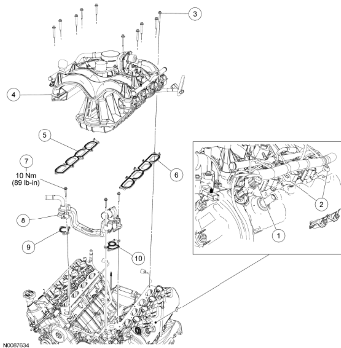
Fig. 11: Identifying Intake Manifold, Coolant Crossover Manifold Assembly And Gaskets Courtesy of FORD MOTOR CO.
