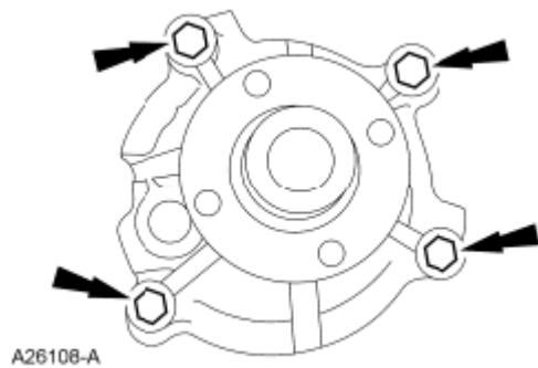
Fig. 416: Locating Coolant Pump Bolts Courtesy of FORD MOTOR CO.
