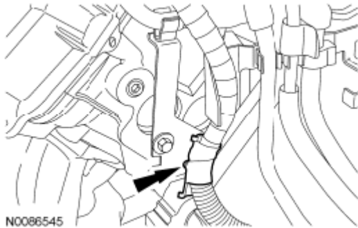
Fig. 573: Locating Transmission Wiring Harness Retainer From Intake Manifold Vacuum Tube Support Bracket Courtesy of FORD MOTOR CO.
