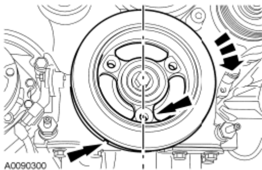
Fig. 131: Locating Timing Mark Indentation Courtesy of FORD MOTOR CO.
