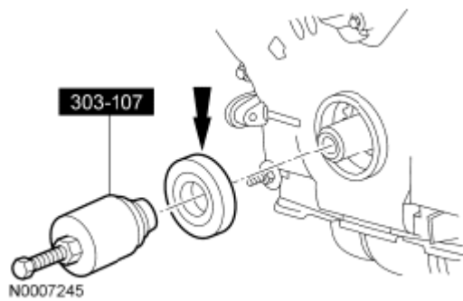
Fig. 352: Removing Discard Crankshaft Seal Courtesy of FORD MOTOR CO.
