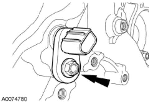
Fig. 192: Locating CMP Sensor And Bolt Courtesy of FORD MOTOR CO.
