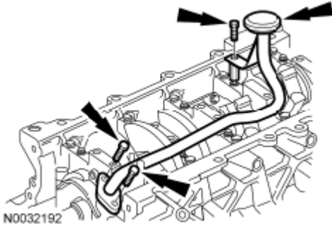
Fig. 261: Locating Oil Pump Screen And Pickup Tube With Bolts Courtesy of FORD MOTOR CO.
