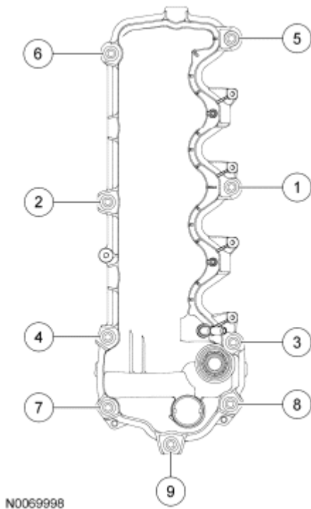
Fig. 29: Identifying RH Valve Cover And Gasket On Cylinder Head And Fasteners In Tightening Sequence Courtesy of FORD MOTOR CO.
