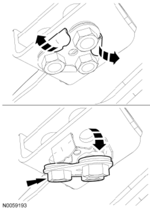
Fig. 292: Removing Engine Support Insulator-To-Cylinder Block Bracket And Bolts LH Courtesy of FORD MOTOR CO.
