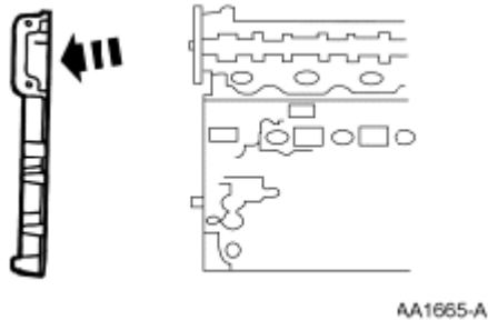
Fig. 355: Removing Engine Front Cover From Cylinder Block Courtesy of FORD MOTOR CO.
