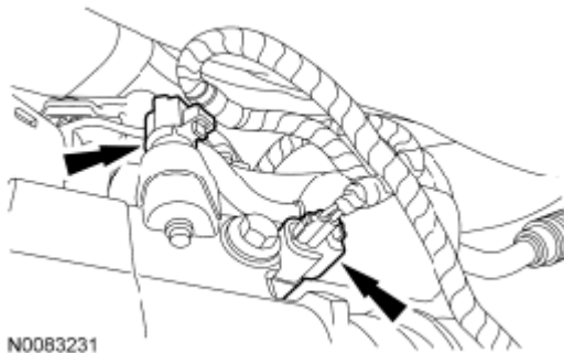
Fig. 589: Locating A/C Compressor Electrical Connector And Wiring Harness Retainer Courtesy of FORD MOTOR CO.
