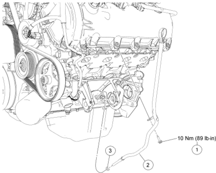
Fig. 266: Identifying Oil Level Indicator And Tube Bolt Courtesy of FORD MOTOR CO.
