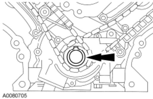
Fig. 424: Locating Crankshaft Keyway Courtesy of FORD MOTOR CO.
