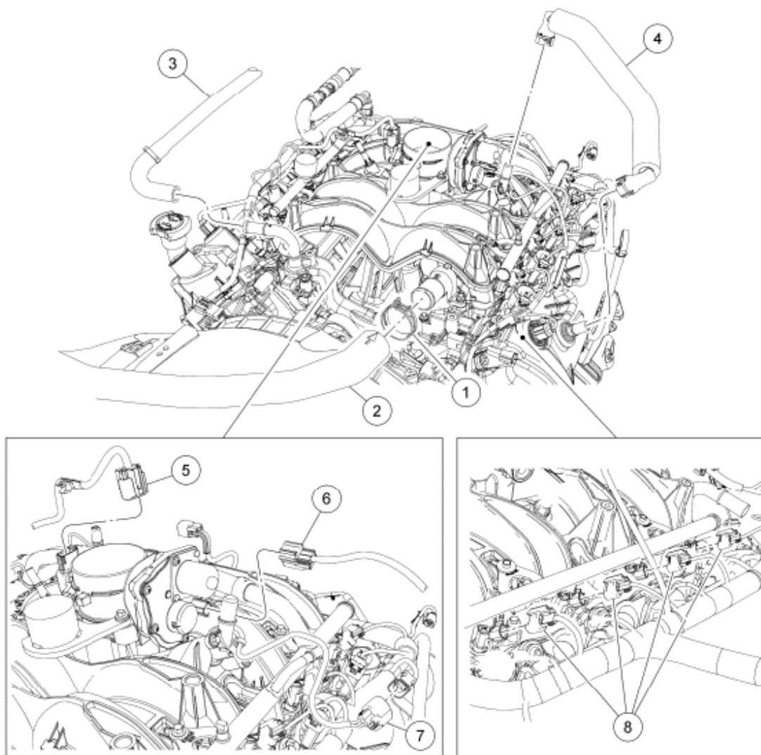
Fig. 9: Identifying Throttle Body (TB) And Ignition Coil Electrical Connectors Courtesy of FORD MOTOR CO.
