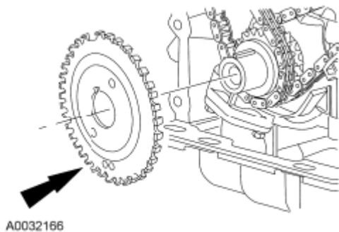
Fig. 624: Locating Crankshaft Sensor Ring On Crankshaft Courtesy of FORD MOTOR CO.
