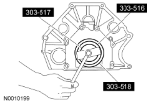
Fig. 279: Installing Crankshaft Oil Slinger Courtesy of FORD MOTOR CO.
