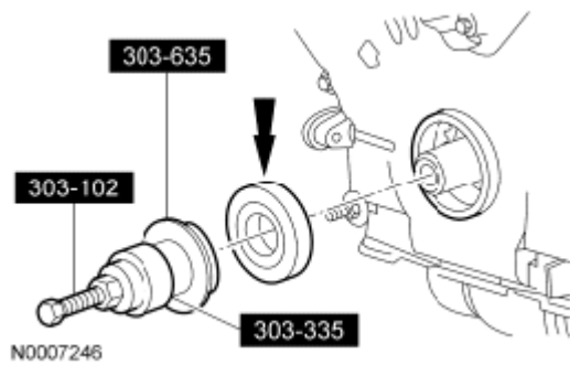
Fig. 518: Installing Crankshaft Front Seal Courtesy of FORD MOTOR CO.
