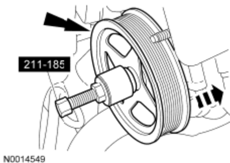
Fig. 586: Installing Power Steering Pump Pulley Courtesy of FORD MOTOR CO.
