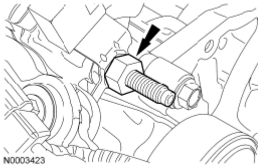
Fig. 397: Locating Nut And Radio Interference Capacitor RH Courtesy of FORD MOTOR CO.
