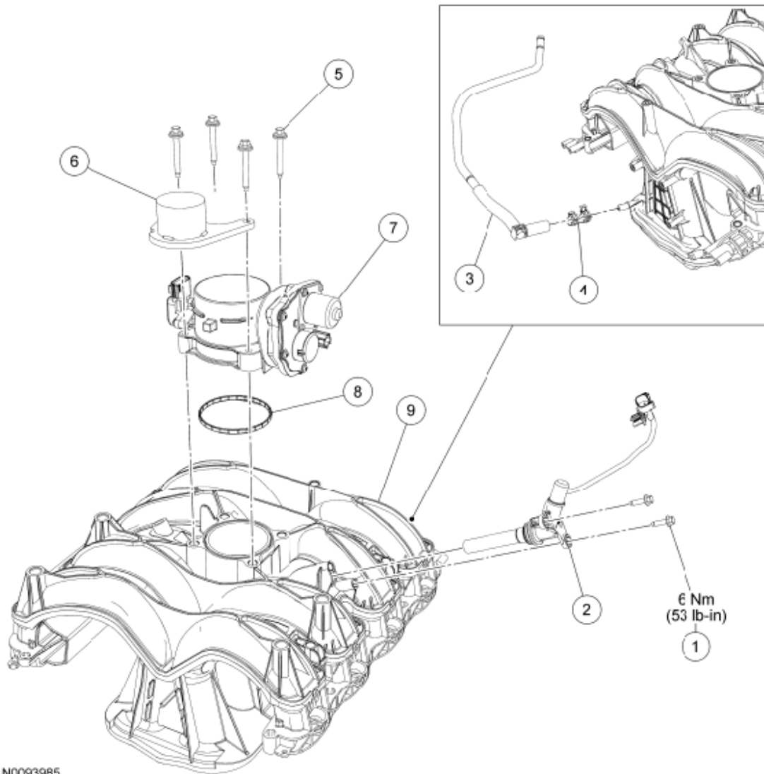
Fig. 462: Identifying Intake Manifold Vacuum Tube, Throttle Body (TB) And Intake Manifold Courtesy of FORD MOTOR CO.
