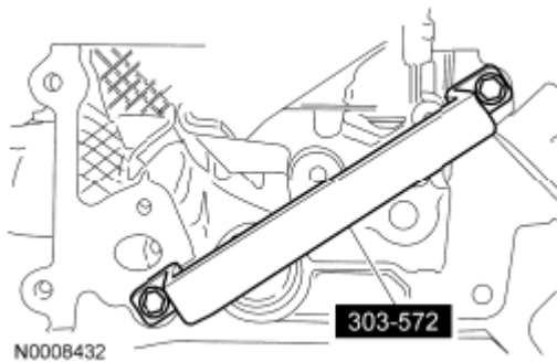
Fig. 599: Identifying Cylinder Head Remover/Installer From Cylinder Head RH Courtesy of FORD MOTOR CO.
