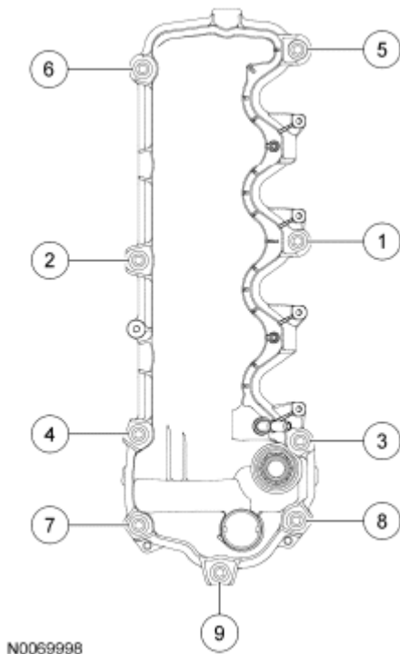
Fig. 631: Identifying RH Valve Cover And Gasket On Cylinder Head And Fasteners In Tightening Sequence Courtesy of FORD MOTOR CO.
