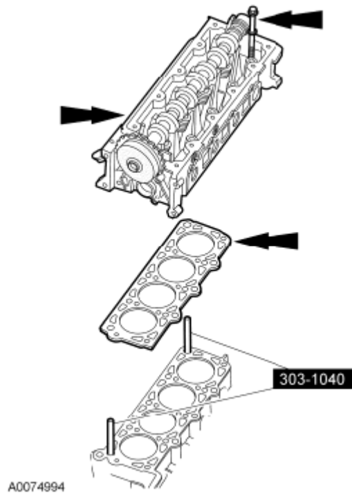
Fig. 486: Locating Cylinder Head Bolts Courtesy of FORD MOTOR CO.
