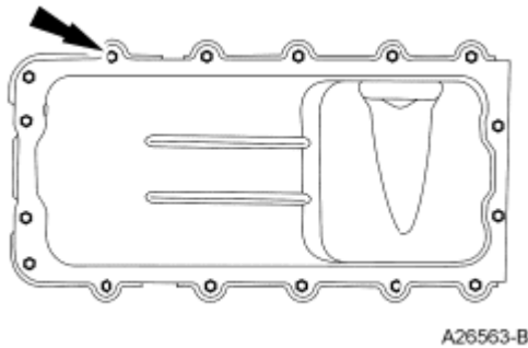
Fig. 420: Locating Oil Pan And Oil Pan Gasket With Bolts Courtesy of FORD MOTOR CO.
