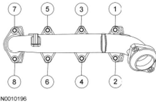
Fig. 231: Locating Exhaust Manifold Nuts In Tightening Sequence Courtesy of FORD MOTOR CO.
