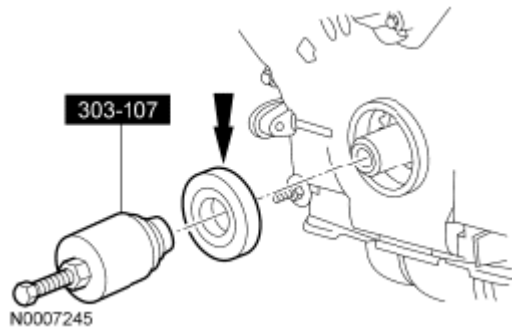
Fig. 47: Removing Discard Crankshaft Seal Courtesy of FORD MOTOR CO.
