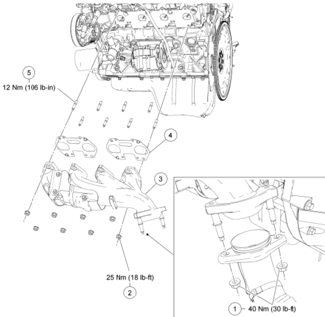
Fig. 228: Exploded View Of Exhaust Manifold (LH) Courtesy of FORD MOTOR CO.
