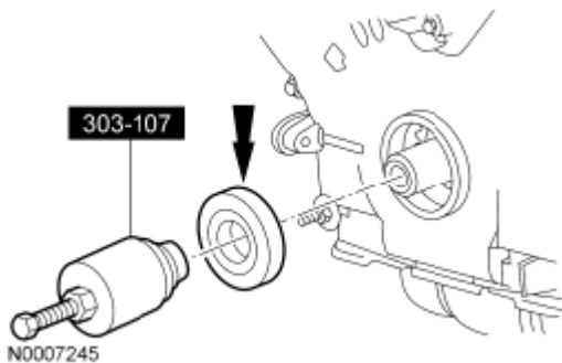
Fig. 63: Removing Discard Crankshaft Seal Courtesy of FORD MOTOR CO.
