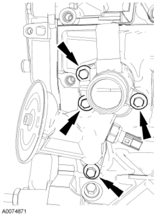
Fig. 525: Locating Oil Filter Adapter And Bolts Courtesy of FORD MOTOR CO.
