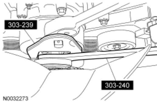
Fig. 543: Removing Cooling Fan Courtesy of FORD MOTOR CO.
