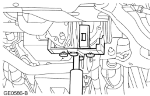
Fig. 237: Positioning Suitable Hydraulic Jack Under Front Axle Courtesy of FORD MOTOR CO.
