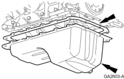
Fig. 553: Locating Oil Pan Gasket And Oil Pan Courtesy of FORD MOTOR CO.
