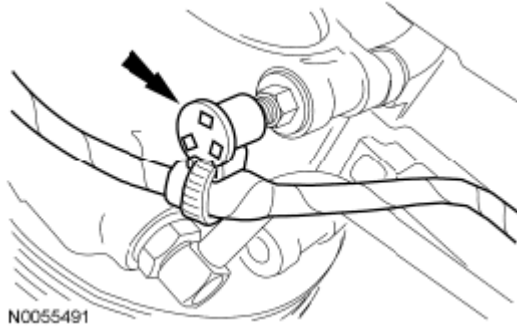
Fig. 64: Locating Power Steering Pump Stud Bolt Courtesy of FORD MOTOR CO.
