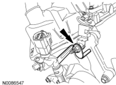
Fig. 340: Locating Nut And Engine Cooling Fan Clutch Electrical Connector Courtesy of FORD MOTOR CO.
