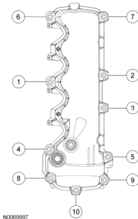
Fig. 534: Identifying Bolts In Tightening Sequence Courtesy of FORD MOTOR CO.
