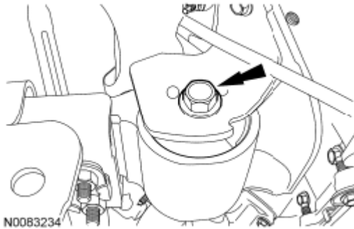
Fig. 559: Locating Engine Support Insulator Bolt Courtesy of FORD MOTOR CO.
