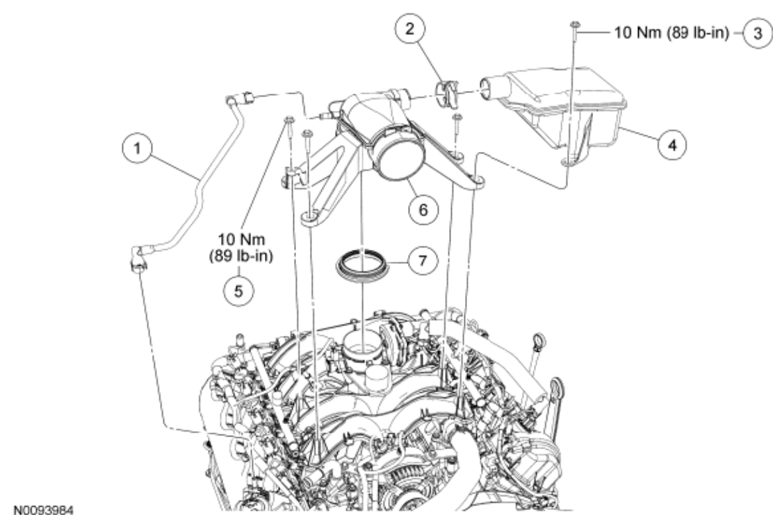
Fig. 8: Identifying Air Cleaner (ACL) Outlet Pipe-To-Throttle Body (TB) Adapter And Air Intake Resonator Assembly Courtesy of FORD MOTOR CO.
