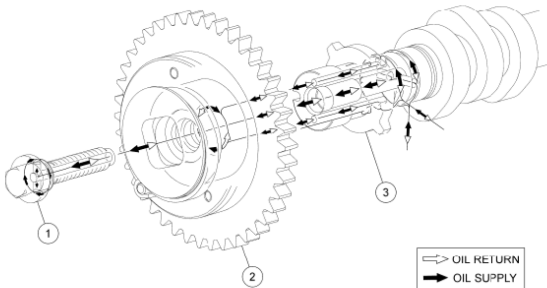
Fig. 4: Identifying Camshaft Phaser And Sprocket, Camshaft Phaser And Sprocket Bolt And Camshaft Courtesy of FORD MOTOR CO.
