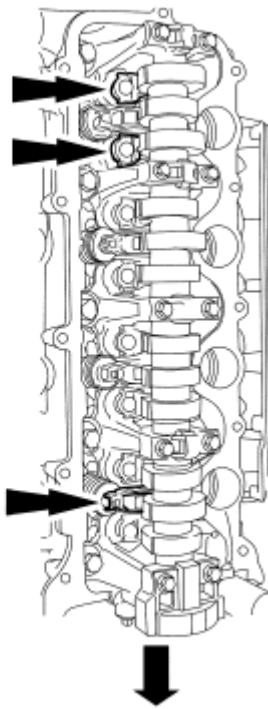
Fig. 359: Locating Camshaft Roller Courtesy of FORD MOTOR CO.
