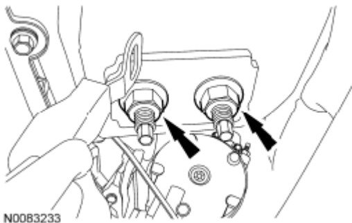
Fig. 560: Locating Engine Support Insulator Washer And Nuts Courtesy of FORD MOTOR CO.
