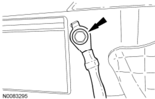
Fig. 324: Locating Ground Strap Bolt Courtesy of FORD MOTOR CO.
