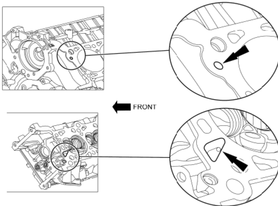
Fig. 386: Locating Cylinder Heads On Oil Pressure Feed Area Courtesy of FORD MOTOR CO.
