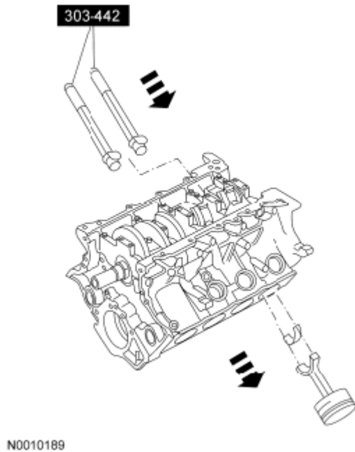
Fig. 450: Pushing Piston Of Cylinder Block Courtesy of FORD MOTOR CO.
