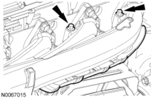
Fig. 380: Locating Bolts And Exhaust Manifold Heat Shield Courtesy of FORD MOTOR CO.
