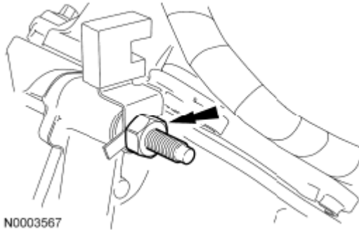
Fig. 646: Locating Nut And Radio Interference Capacitor LH Courtesy of FORD MOTOR CO.
