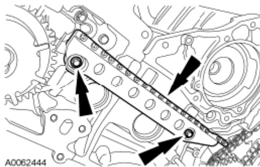
Fig. 367: Locating Both Timing Chain Guides And Bolts Courtesy of FORD MOTOR CO.
