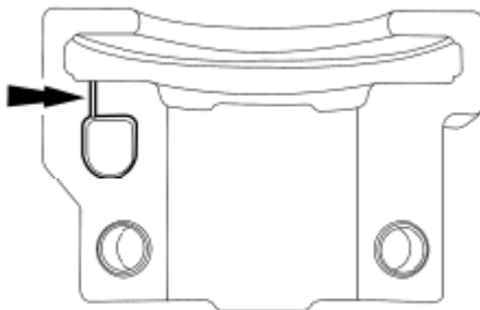
Fig. 441: Locating Camshaft Bearing Caps Courtesy of FORD MOTOR CO.
