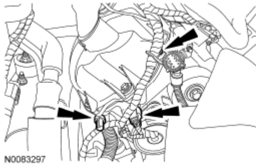
Fig. 329: Locating Camshaft Position (CMP) Sensor Electrical Connector RH Courtesy of FORD MOTOR CO.
