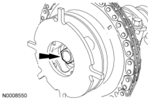
Fig. 208: Locating Camshaft Phaser And Sprocket Bolt Courtesy of FORD MOTOR CO.
