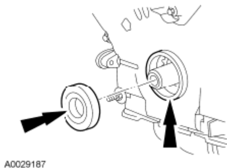
Fig. 74: Locating Engine Front Cover And Crankshaft Seal Inner Lip Courtesy of FORD MOTOR CO.
