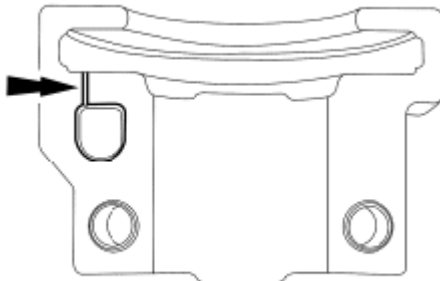
Fig. 103: Locating Camshaft Bearing Caps Courtesy of FORD MOTOR CO.
