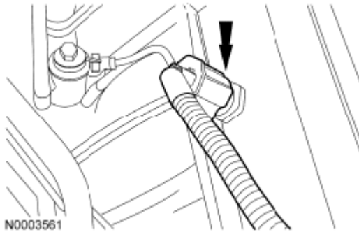
Fig. 575: Locating Cylinder Head Temperature (CHT) Electrical Connector Courtesy of FORD MOTOR CO.
