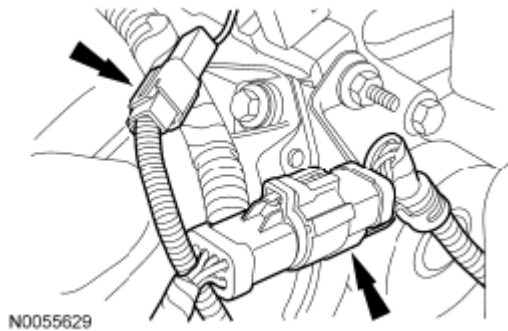
Fig. 34: Locating Engine Cooling Fan Clutch Electrical Connectors Courtesy of FORD MOTOR CO.
