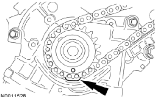
Fig. 113: Locating Timing Chain On Crankshaft Sprocket Courtesy of FORD MOTOR CO.
