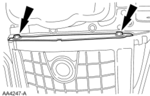
Fig. 302: Locating Flexplate Inspection Cover And Bolts Courtesy of FORD MOTOR CO.
