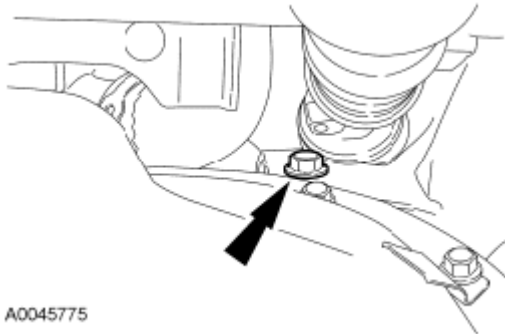
Fig. 287: Locating Upper Front Axle Carrier Mounting Bushing Bolt Courtesy of FORD MOTOR CO.
