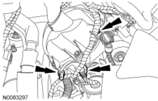
Fig. 581: Locating Camshaft Position (CMP) Sensor Electrical Connector RH Courtesy of FORD MOTOR CO.
