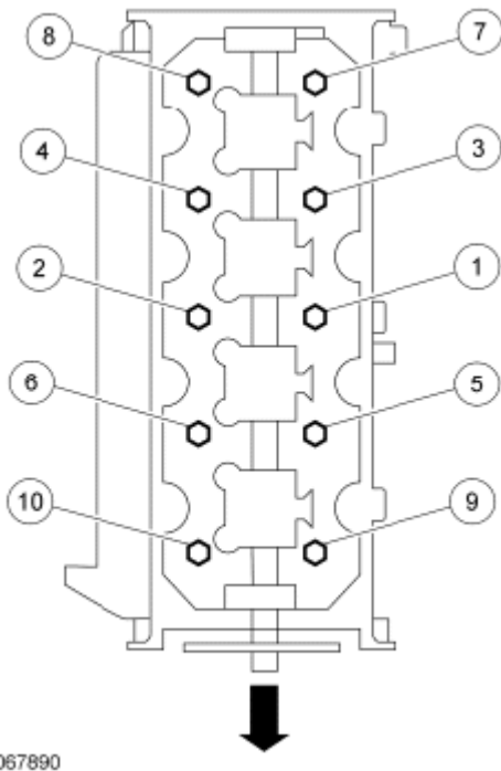
Fig. 594: Identifying Bolts In Tightening Sequence Courtesy of FORD MOTOR CO.
