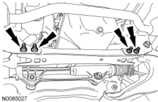
Fig. 236: Locating Crossmember With Nuts And Bolts Courtesy of FORD MOTOR CO.
