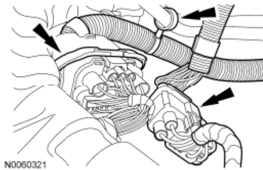
Fig. 30: Locating Electrical Connectors And Wiring Harness Retainer Courtesy of FORD MOTOR CO.
