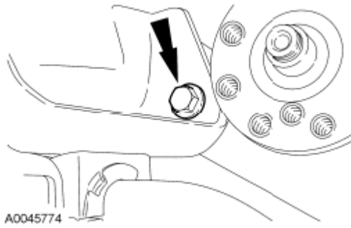
Fig. 289: Locating Lower Front Axle Carrier Mounting Bushing Bolt Courtesy of FORD MOTOR CO.
