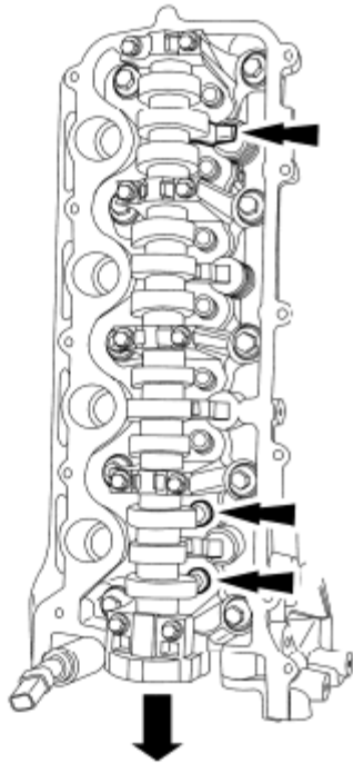
Fig. 428: Locating Camshaft Roller From Cylinder Head Courtesy of FORD MOTOR CO.
