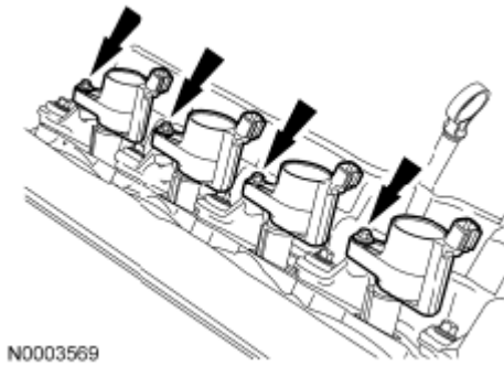
Fig. 540: Locating Ignition Coils And Bolts Courtesy of FORD MOTOR CO.
