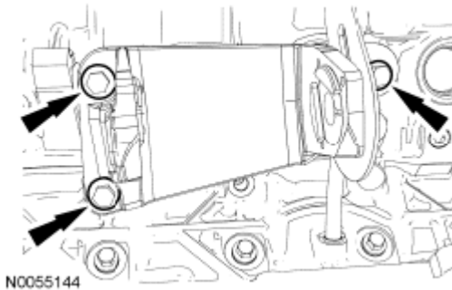
Fig. 536: Locating Bolts And Engine Support Insulator-To-Cylinder Block Bracket LH Courtesy of FORD MOTOR CO.
