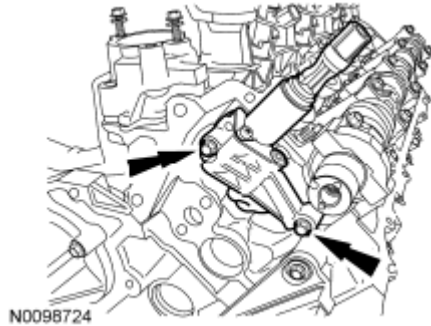
Fig. 210: Locating VCT Housing LH And Bolts Courtesy of FORD MOTOR CO.
