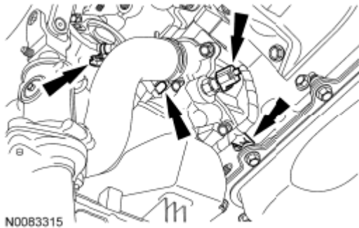
Fig. 590: Locating Engine Oil Pressure (EOP) Switch Electrical Connector And Oil Pan Bolt Courtesy of FORD MOTOR CO.
