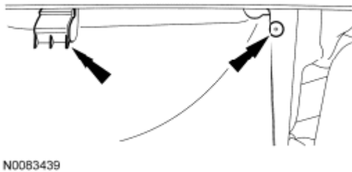
Fig. 250: Locating Retainer Tab Locks Courtesy of FORD MOTOR CO.
