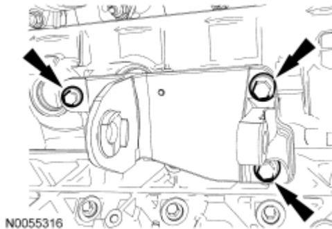
Fig. 530: Locating Engine Support Insulator-To-Cylinder Block Bracket And Bolts Courtesy of FORD MOTOR CO.
