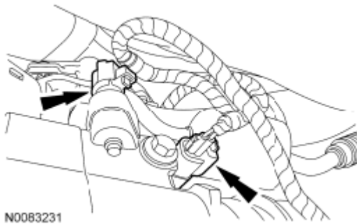
Fig. 307: Locating A/C Compressor Electrical Connector And Wiring Harness Retainer Courtesy of FORD MOTOR CO.
