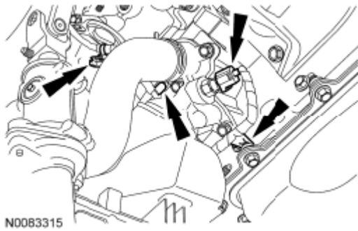
Fig. 312: Locating Engine Oil Pressure (EOP) Switch Electrical Connector And Oil Pan Bolt Courtesy of FORD MOTOR CO.
