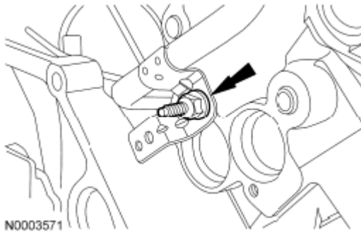
Fig. 604: Locating Coolant Tube And Stud Bolt Courtesy of FORD MOTOR CO.
