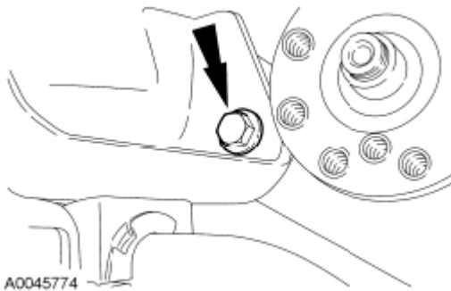
Fig. 295: Locating Lower Front Axle Carrier Mounting Bushing Bolt Courtesy of FORD MOTOR CO.
