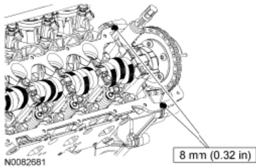
Fig. 28: Identifying Bead Of Silicone Gasket And Sealant Courtesy of FORD MOTOR CO.
