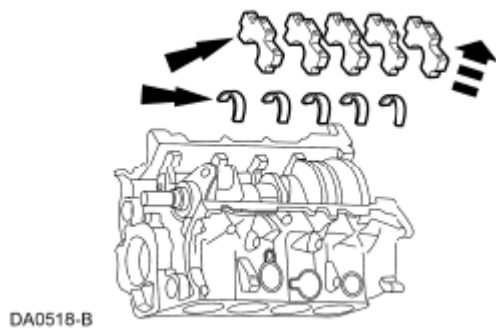
Fig. 452: Locating Main Bearing Caps Courtesy of FORD MOTOR CO.
