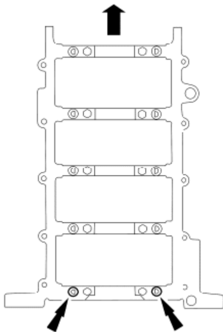
Fig. 474: Installing Crankshaft Lower Main Bearings Courtesy of FORD MOTOR CO.
