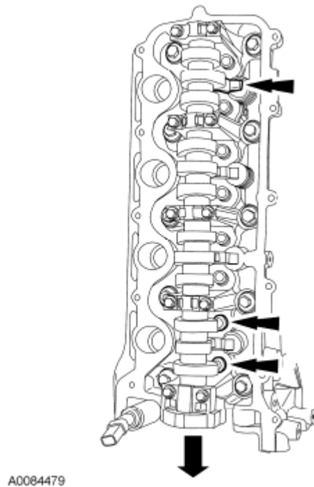
Fig. 361: Locating Camshaft Roller From Cylinder Head Courtesy of FORD MOTOR CO.
