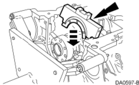
Fig. 473: Installing Lower Crankshaft Thrust Washer To Back Side Courtesy of FORD MOTOR CO.
