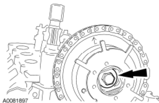
Fig. 147: Locating Camshaft Phaser And Sprocket Bolts Courtesy of FORD MOTOR CO.
