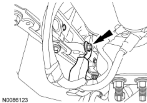
Fig. 310: Locating Starter Wiring Harness Rear Support Bracket Bolt Courtesy of FORD MOTOR CO.
