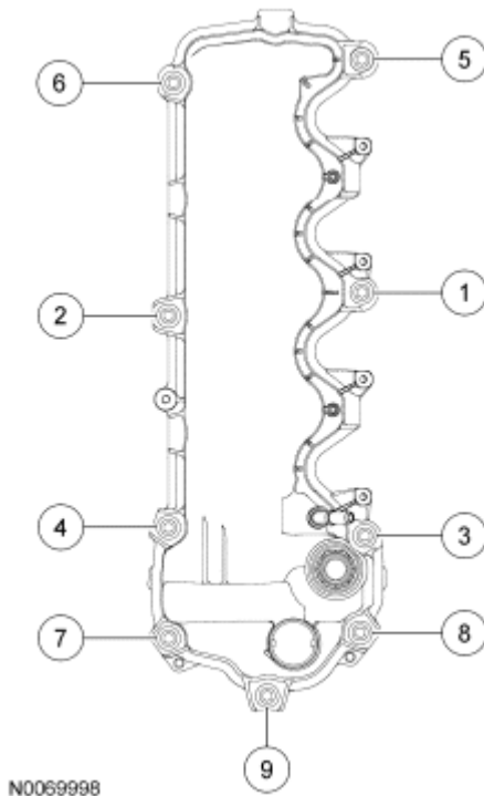
Fig. 532: Identifying RH Valve Cover And Gasket On Cylinder Head And Fasteners In Tightening Sequence Courtesy of FORD MOTOR CO.
