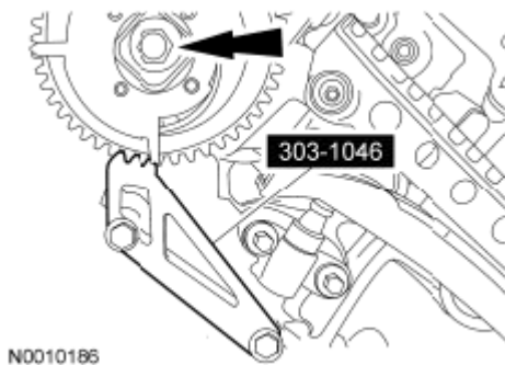
Fig. 375: Removing Camshaft Phaser And Sprocket Assembly With Bolt RH Courtesy of FORD MOTOR CO.
