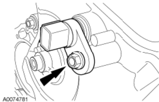
Fig. 173: Locating CMP Sensor Bolt LH
