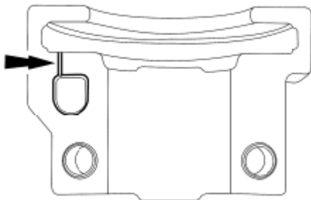
Fig. 371: Locating Camshaft Bearing Caps Courtesy of FORD MOTOR CO.
