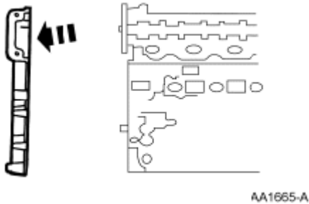
Fig. 422: Removing Engine Front Cover From Cylinder Block Courtesy of FORD MOTOR CO.
