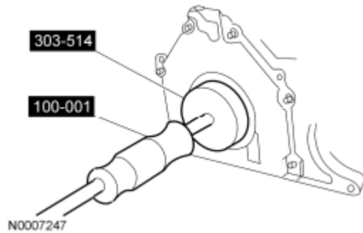
Fig. 269: Removing Crankshaft Oil Slinger Courtesy of FORD MOTOR CO.
