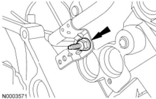
Fig. 538: Locating Coolant Tube And Stud Bolt Courtesy of FORD MOTOR CO.
