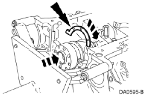
Fig. 472: Installing Front Crankshaft Upper Thrust Washer Courtesy of FORD MOTOR CO.
