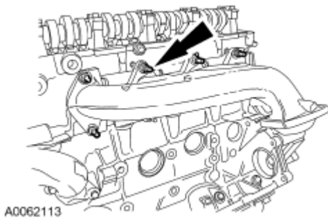
Fig. 411: Locating Nuts And Studs, Exhaust Manifold LH Courtesy of FORD MOTOR CO.
