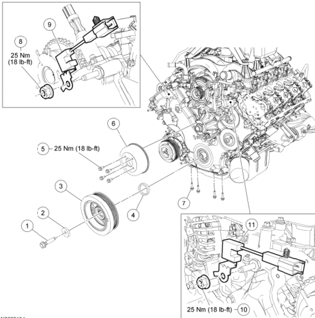
Fig. 55: Identifying Radio Ignition Interference Capacitors, Coolant Pump Pulley, Crankshaft Pulley And Front Oil Pan Bolts
