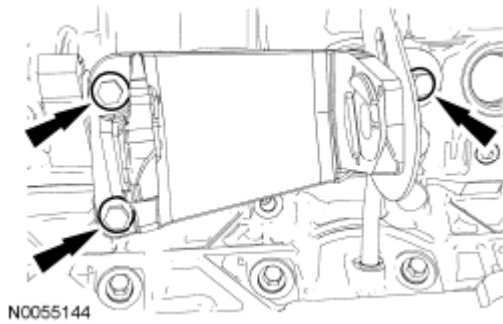
Fig. 406: Locating Bolts And Engine Support Insulator-To-Cylinder Block Bracket LH Courtesy of FORD MOTOR CO.
