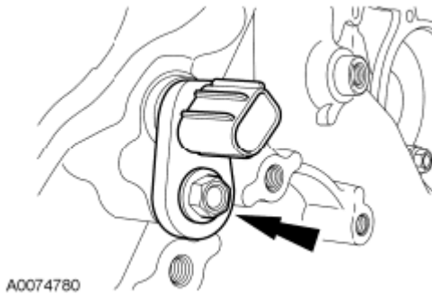
Fig. 514: Locating CMP Sensor And Bolt Courtesy of FORD MOTOR CO.
