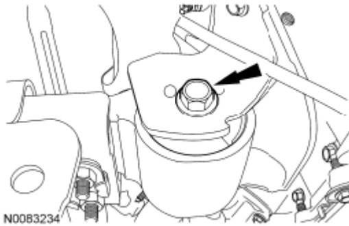
Fig. 315: Locating LH Engine Support Insulator Bolt Courtesy of FORD MOTOR CO.
