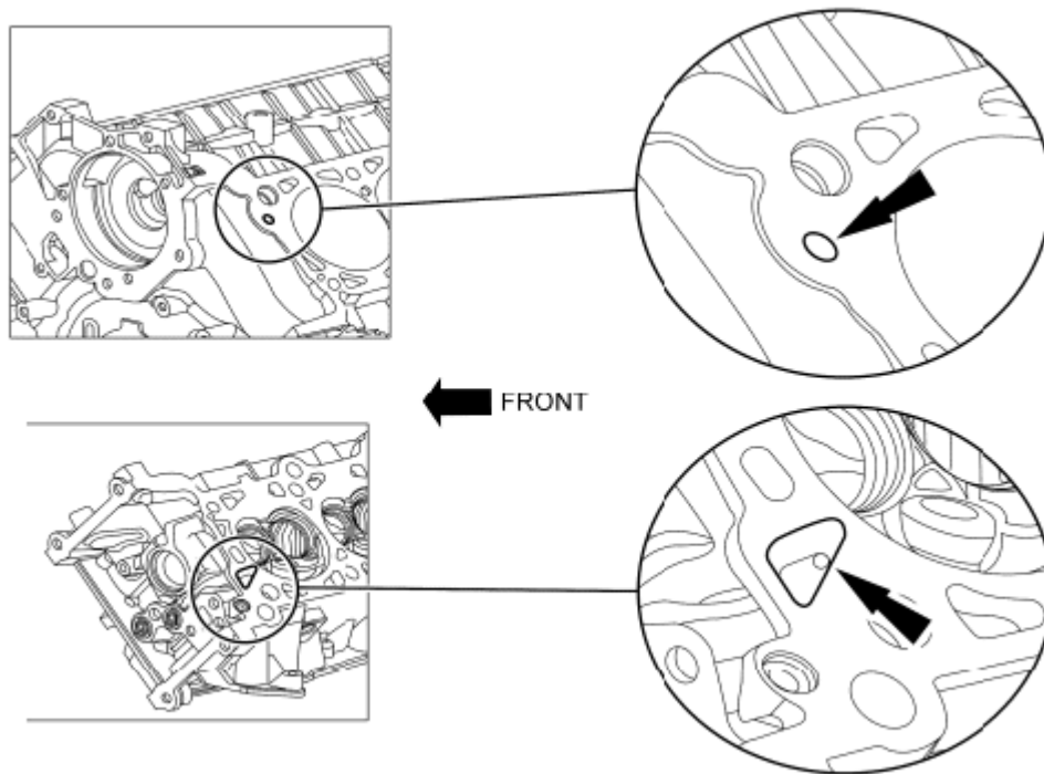
Fig. 446: Locating Cylinder Heads On Oil Pressure Feed Area Courtesy of FORD MOTOR CO.
