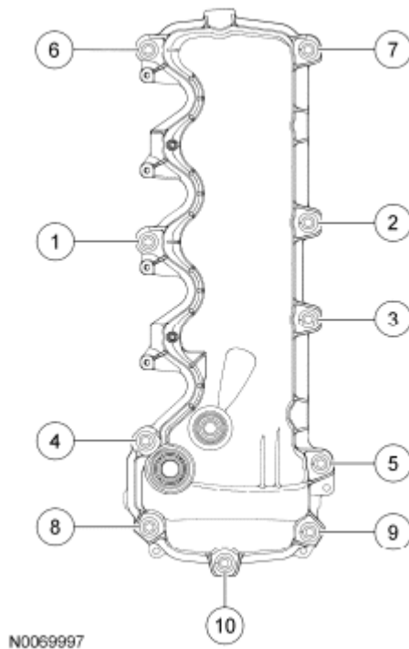
Fig. 20: Identifying LH Valve Cover And Gasket On Cylinder Head And Fasteners In Tightening Sequence Courtesy of FORD MOTOR CO.
