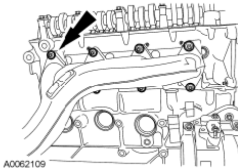
Fig. 381: Locating Nuts And Exhaust Manifold RH Courtesy of FORD MOTOR CO.
