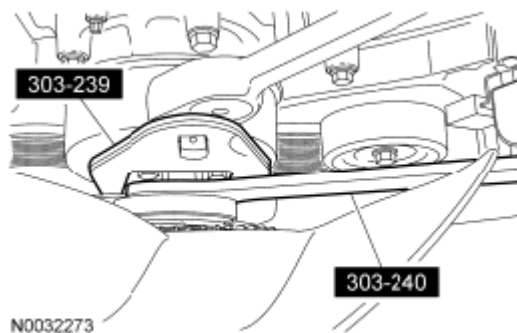
Fig. 396: Removing Cooling Fan Courtesy of FORD MOTOR CO.
