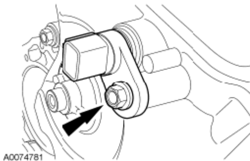
Fig. 187: Locating CMP Sensor Bolt LH Courtesy of FORD MOTOR CO.
