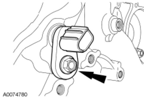
Fig. 403: Locating CMP Sensor And Bolt Courtesy of FORD MOTOR CO.
