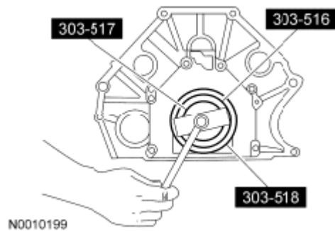
Fig. 272: Installing Crankshaft Oil Slinger Courtesy of FORD MOTOR CO.
