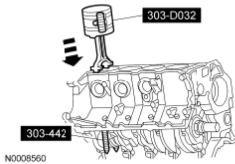
Fig. 479: Installing Upper Connecting Rod Bearing Courtesy of FORD MOTOR CO.
