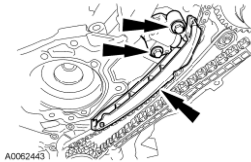
Fig. 364: Locating Timing Chain Tensioner And Bolts LH Courtesy of FORD MOTOR CO.
