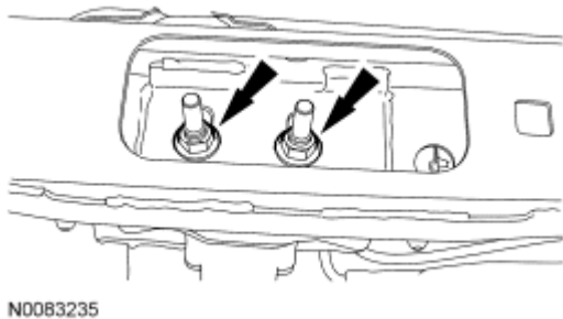
Fig. 563: Locating Transmission Mount Nuts Courtesy of FORD MOTOR CO.
