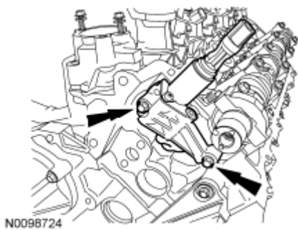
Fig. 214: Locating VCT Housing LH And Bolts Courtesy of FORD MOTOR CO.
