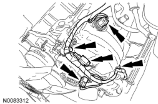
Fig. 332: Locating VCT Solenoid Electrical Connectors Courtesy of FORD MOTOR CO.
