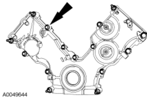
Fig. 66: Locating Bolts And Studs Courtesy of FORD MOTOR CO.
