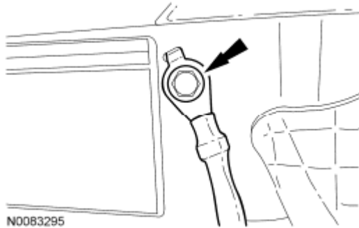
Fig. 582: Locating Ground Strap And Bolt Courtesy of FORD MOTOR CO.
