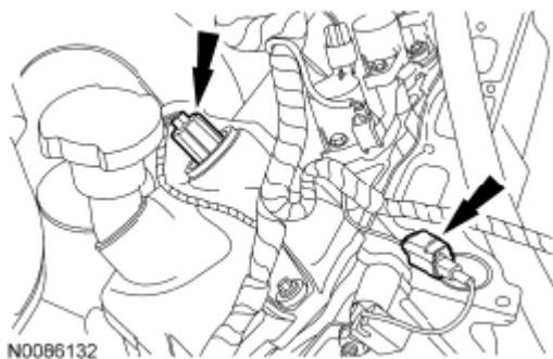
Fig. 580: Locating Radio Ignition Interference Capacitor Electrical Connectors RH Courtesy of FORD MOTOR CO.
