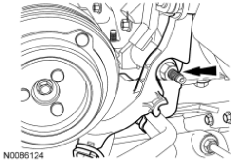
Fig. 249: Locating Starter Wiring Harness Support Bracket And Nut Courtesy of FORD MOTOR CO.
