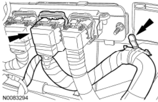
Fig. 323: Locating PCM Electrical Connector Courtesy of FORD MOTOR CO.
