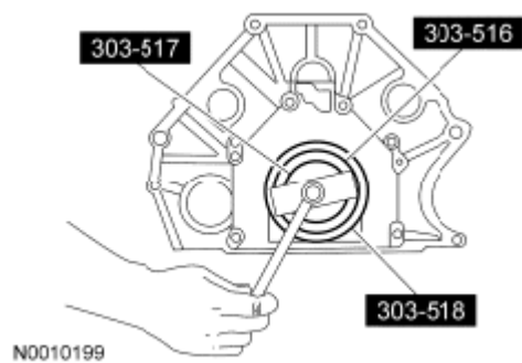
Fig. 556: Installing Crankshaft Oil Slinger Courtesy of FORD MOTOR CO.
