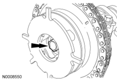
Fig. 170: Locating Bolt And Camshaft Phaser And Sprocket Assembly Courtesy of FORD MOTOR CO.
