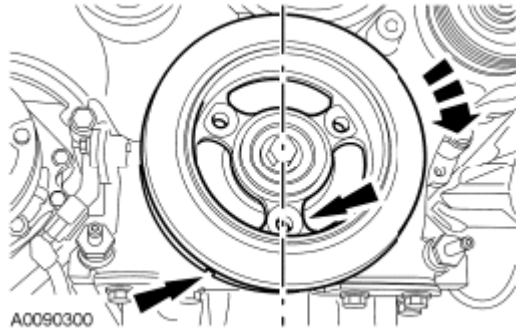
Fig. 196: Locating Timing Mark Indentation Courtesy of FORD MOTOR CO.
