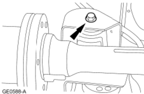
Fig. 296: Locating Axle Shaft Housing Carrier Bushing Bolt Courtesy of FORD MOTOR CO.
