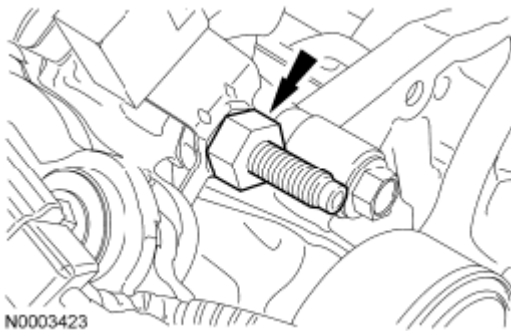
Fig. 647: Locating Nut And Radio Interference Capacitor RH Courtesy of FORD MOTOR CO.
