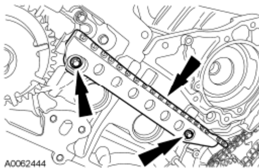
Fig. 434: Locating Both Timing Chain Guides And Bolts Courtesy of FORD MOTOR CO.
