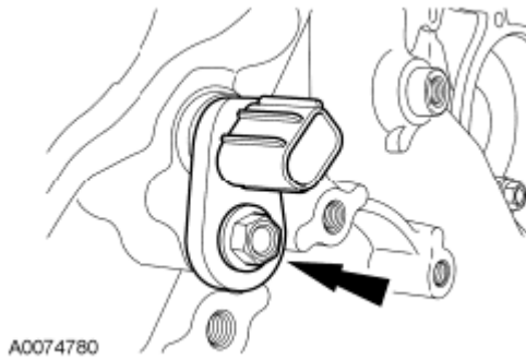
Fig. 206: Locating CMP Sensor And Bolt Courtesy of FORD MOTOR CO.
