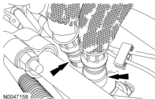
Fig. 35: Locating Auxiliary Heat Coolant Hoses Courtesy of FORD MOTOR CO.
