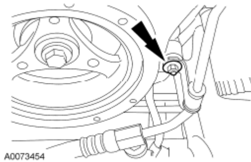
Fig. 61: Locating Power Steering Pressure Hose Support Bracket And Nut Courtesy of FORD MOTOR CO.
