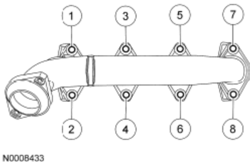
Fig. 529: Identifying Exhaust Manifold And Nuts In Tightening Sequence
