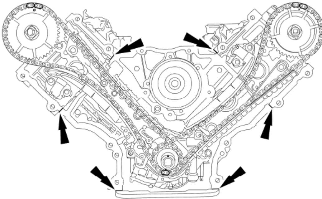
Fig. 68: Locating Bead Of Silicone Gasket And Sealant Cylinder Head-To-Cylinder Block Surface Courtesy of FORD MOTOR CO.
