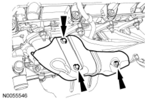
Fig. 410: Locating Bolts And Exhaust Manifold Heat Shield LH Courtesy of FORD MOTOR CO.
