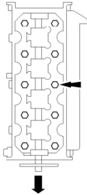
Fig. 445: Locating Cylinder Head Bolts Courtesy of FORD MOTOR CO.
