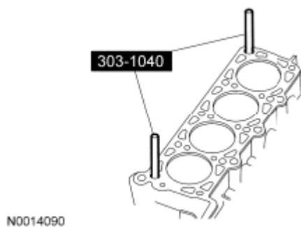
Fig. 593: Installing Cylinder Head Bolts Courtesy of FORD MOTOR CO.
