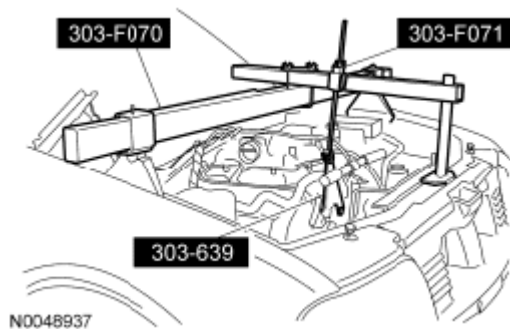
Fig. 300: Installing Engine Support Bar Courtesy of FORD MOTOR CO.
