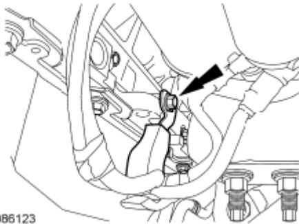
Fig. 59: Locating Starter Wiring Harness Rear Support Bracket Bolt Courtesy of FORD MOTOR CO.
