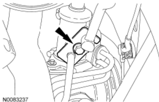
Fig. 319: Locating Power Steering Fluid Tubes And Bolt Courtesy of FORD MOTOR CO.
