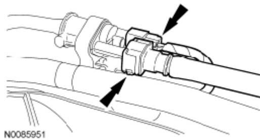
Fig. 13: Locating Evaporative Emission (EVAP) Electrical Connector Courtesy of FORD MOTOR CO.
