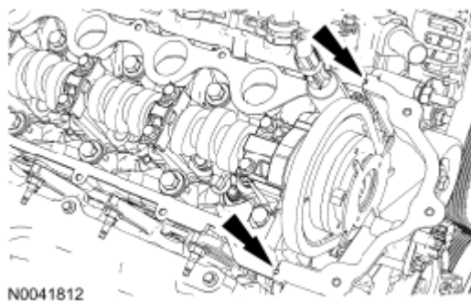
Fig. 630: Locating Silicone Gasket And Sealant Applying Area Courtesy of FORD MOTOR CO.
