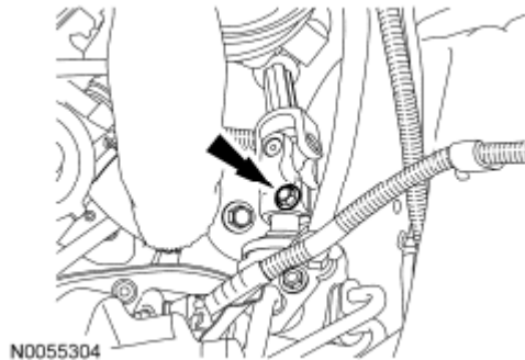
Fig. 229: Locating Steering Shaft And Bolt Courtesy of FORD MOTOR CO.
