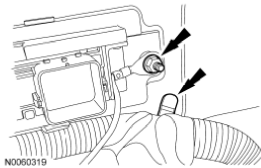
Fig. 24: Locating Wiring Harness Retainer And Nut Courtesy of FORD MOTOR CO.
