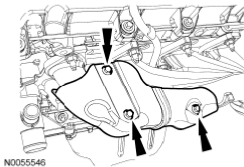
Fig. 528: Identifying Exhaust Manifold Heat Shield And Bolts Courtesy of FORD MOTOR CO.
