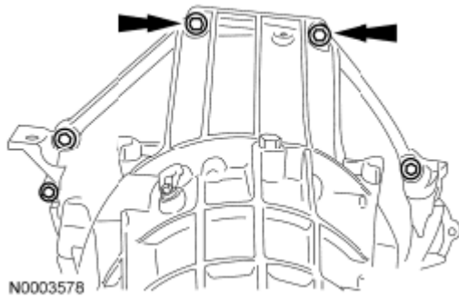
Fig. 572: Locating Upper Transmission-To-Engine Bolts Courtesy of FORD MOTOR CO.
