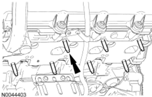
Fig. 597: Locating LH Exhaust Manifold-To-Cylinder Head Studs Courtesy of FORD MOTOR CO.
