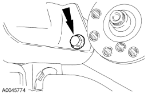
Fig. 240: Locating Lower Front Axle Carrier Mounting Bushing Bolt Courtesy of FORD MOTOR CO.
