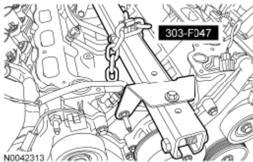
Fig. 547: Removing Engine Lifting Bracket Courtesy of FORD MOTOR CO.
