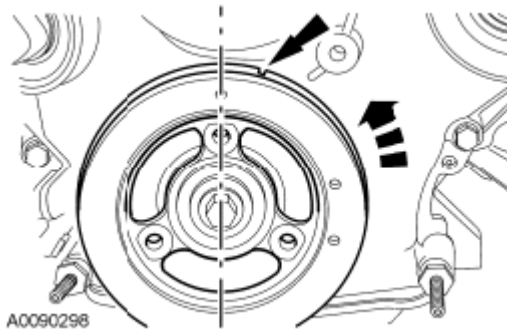
Fig. 184: Locating Timing Mark Indentation Courtesy of FORD MOTOR CO.
