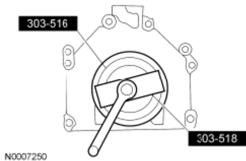
Fig. 555: Installing Crankshaft Rear Seal Courtesy of FORD MOTOR CO.
