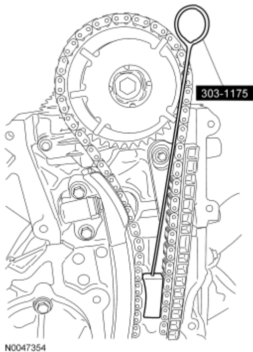
Fig. 178: Installing Timing Chain Locking Tool In Timing Chain Courtesy of FORD MOTOR CO.
