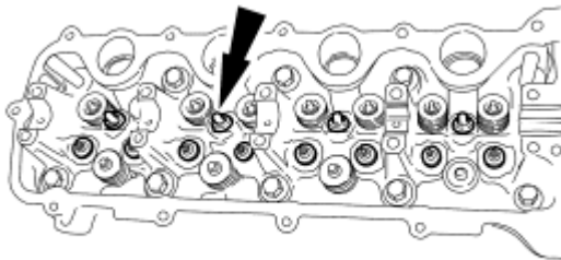
Fig. 596: Identifying Hydraulic Lash Adjusters Courtesy of FORD MOTOR CO.
