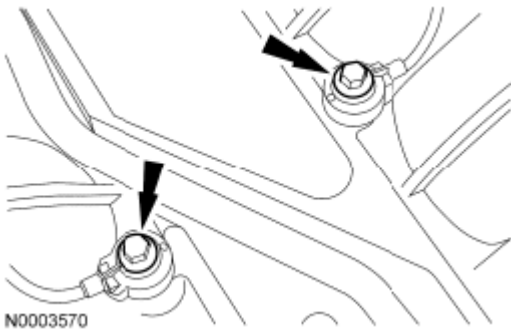
Fig. 539: Locating Bolts And Knock Sensor (KS) Courtesy of FORD MOTOR CO.
