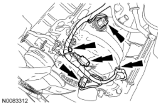
Fig. 574: Locating VCT Solenoid Electrical Connectors Courtesy of FORD MOTOR CO.
