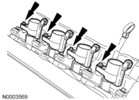
Fig. 400: Locating Ignition Coils And Bolts Courtesy of FORD MOTOR CO.
