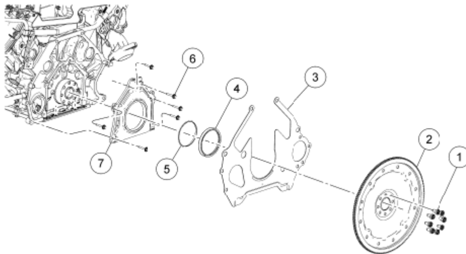
Fig. 267: Exploded View Of Flexplate Or Flywheel And Crankshaft Rear Seal Courtesy of FORD MOTOR CO.
