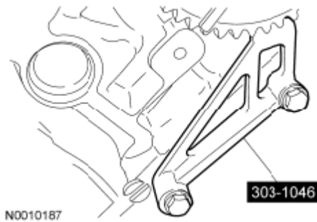
Fig. 368: Removing Camshaft Phaser And Sprocket Assembly With Bolt LH Courtesy of FORD MOTOR CO.
