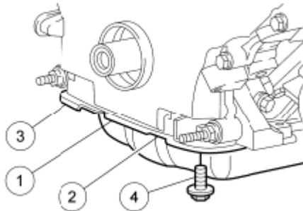
Fig. 71: Identifying Bolts In Tightening Sequence Courtesy of FORD MOTOR CO.
