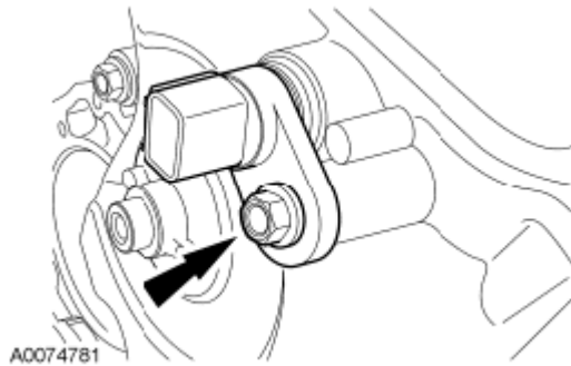
Fig. 404: Locating CMP Sensor Bolt LH Courtesy of FORD MOTOR CO.
