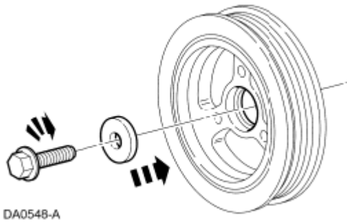
Fig. 521: Installing Crankshaft Pulley Bolt And Washer Courtesy of FORD MOTOR CO.
