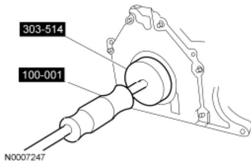
Fig. 388: Removing Crankshaft Oil Slinger Courtesy of FORD MOTOR CO.
