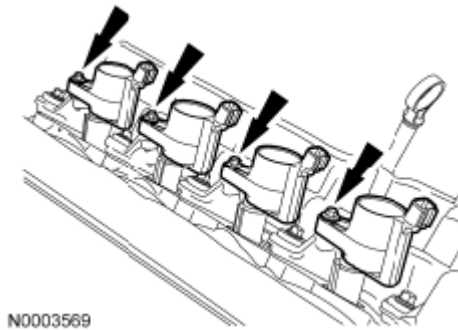
Fig. 345: Locating Ignition Coils And Bolts Courtesy of FORD MOTOR CO.
