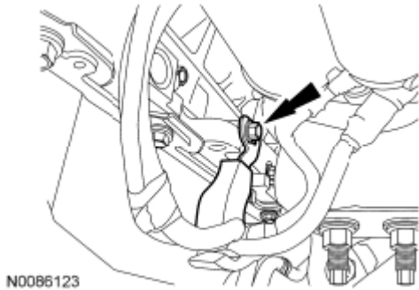
Fig. 73: Locating Starter Wiring Harness Rear Support Bracket And Bolt Courtesy of FORD MOTOR CO.
