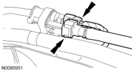
Fig. 15: Locating Evaporative Emission (EVAP) Electrical Connector Courtesy of FORD MOTOR CO.
