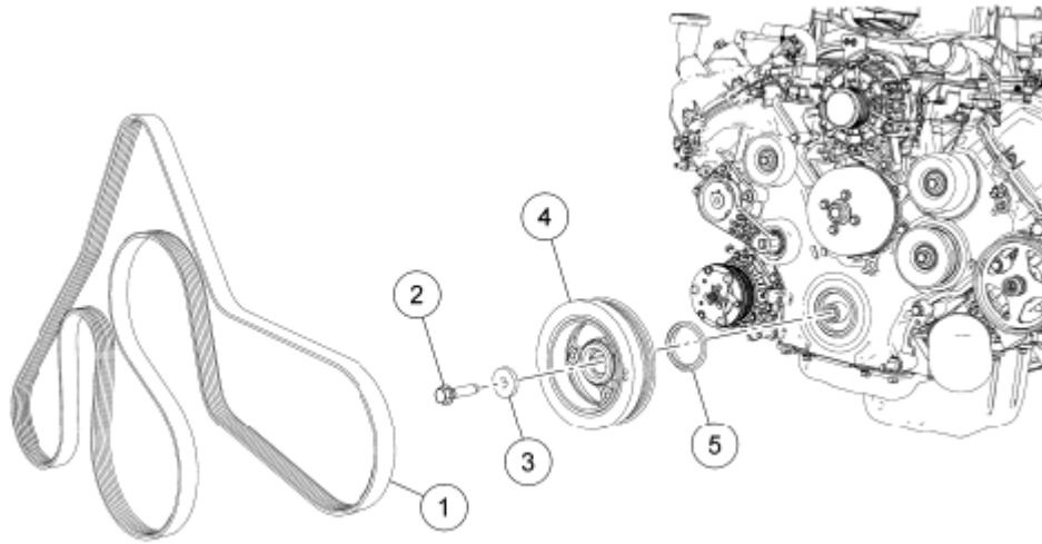
Fig. 44: Identifying Crankshaft Front Seal Components Courtesy of FORD MOTOR CO.
