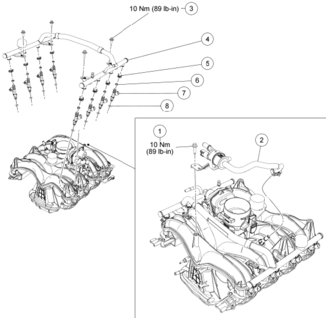
Fig. 461: Identifying Evaporative Emission (EVAP) Purge Valve, Fuel Rail And Fuel Injectors Courtesy of FORD MOTOR CO.
