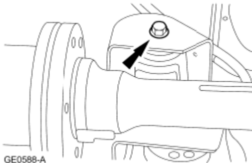
Fig. 288: Locating Axle Shaft Housing Carrier Bushing Bolt Courtesy of FORD MOTOR CO.
