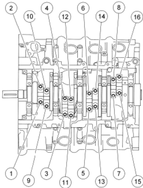
Fig. 481: Identifying Bolts In Tightening Sequence Courtesy of FORD MOTOR CO.
