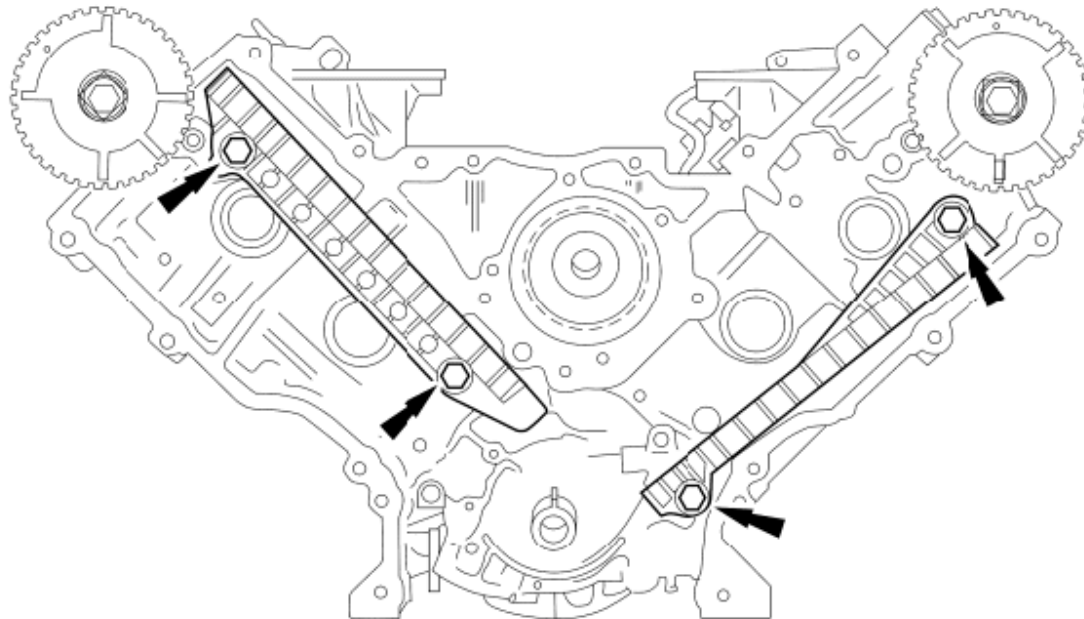
Fig. 614: Locating Timing Chain Guides With Bolts (LH And RH) Courtesy of FORD MOTOR CO.
