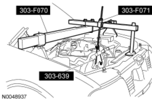
Fig. 290: Installing Engine Support Bar Courtesy of FORD MOTOR CO.
