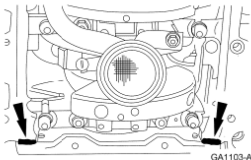
Fig. 245: Locating Crankshaft Rear Seal Retainer Plate-To-Cylinder Block Sealing Surface Courtesy of FORD MOTOR CO.
