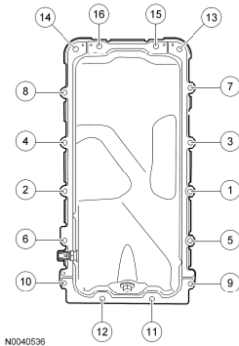
Fig. 247: Identifying Gasket And Oil Pan Bolts In Tightening Sequence Courtesy of FORD MOTOR CO.
