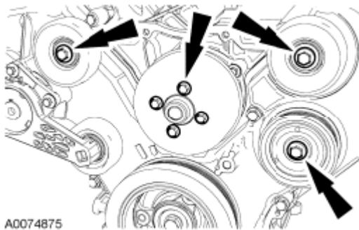
Fig. 414: Locating Bolts And Coolant Pump Pulley Courtesy of FORD MOTOR CO.
