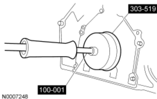
Fig. 270: Removing Crankshaft Rear Seal Courtesy of FORD MOTOR CO.
