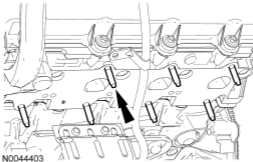
Fig. 526: Locating LH Exhaust Manifold-To-Cylinder Head Studs Courtesy of FORD MOTOR CO.
