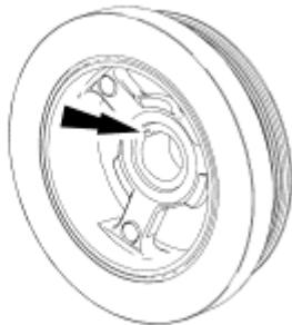
Fig. 519: Locating Woodruff Key Slot In Crankshaft Pulley Courtesy of FORD MOTOR CO.
