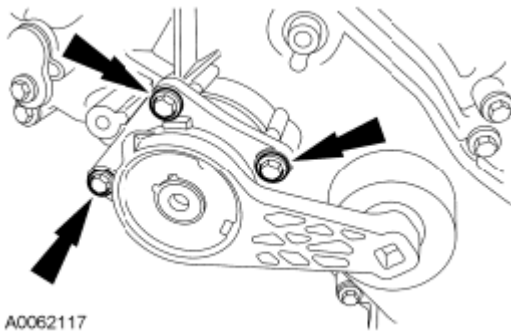
Fig. 641: Locating Bolts And Accessory Drive Belt Tensioner Courtesy of FORD MOTOR CO.
