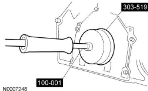
Fig. 275: Removing Crankshaft Rear Seal Courtesy of FORD MOTOR CO.
