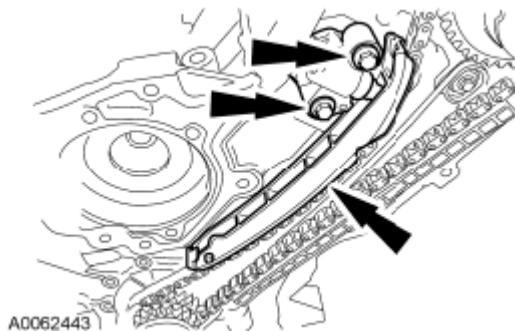
Fig. 617: Locating Timing Chain Tensioner And Bolts LH Courtesy of FORD MOTOR CO.
