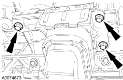
Fig. 635: Locating Bolts And Engine Support Insulator RH Courtesy of FORD MOTOR CO.
