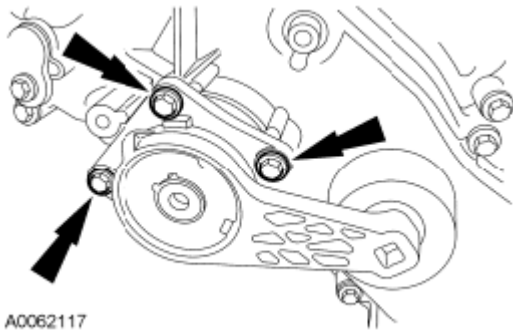
Fig. 350: Locating Bolts And Accessory Drive Belt Tensioner Courtesy of FORD MOTOR CO.
