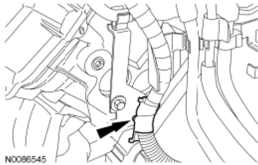
Fig. 333: Locating Transmission Wiring Harness Retainer From Intake Manifold Vacuum Tube Support Bracket Courtesy of FORD MOTOR CO.
