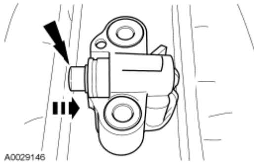
Fig. 609: Compressing Tensioner Plunger Courtesy of FORD MOTOR CO.
