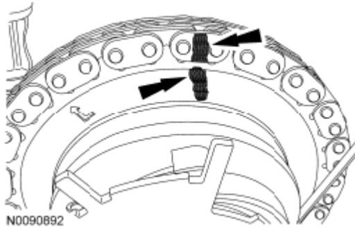
Fig. 181: Locating Timing Chain Scribe Marks Courtesy of FORD MOTOR CO.
