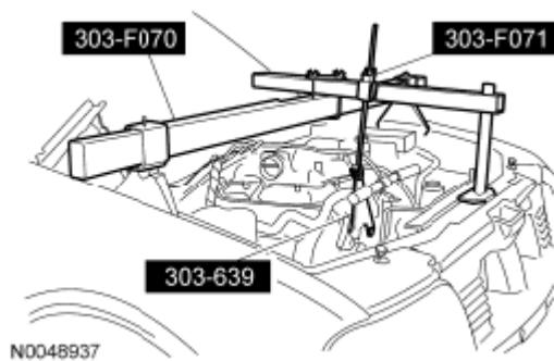
Fig. 293: Supporting Hook And Engine Support Bracket Courtesy of FORD MOTOR CO.
