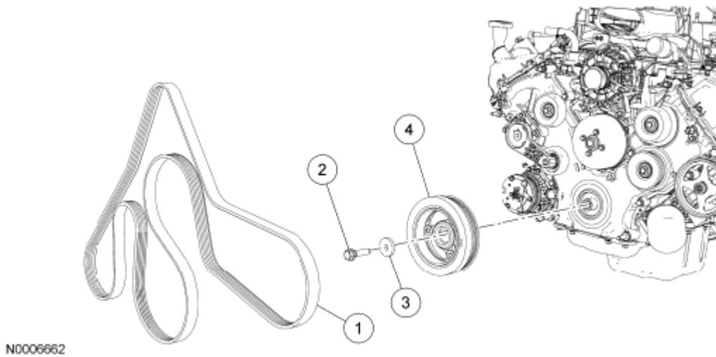
Fig. 36: Identifying Crankshaft Pulley Components Courtesy of FORD MOTOR CO.
