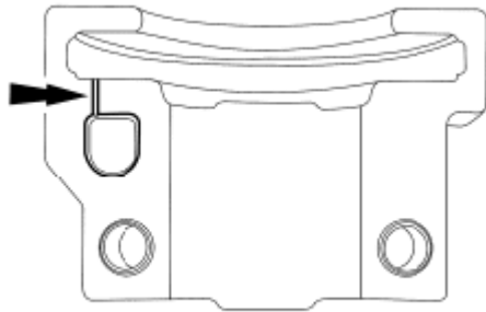
Fig. 100: Locating Camshaft Bearing Caps Courtesy of FORD MOTOR CO.
