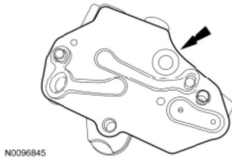
Fig. 212: [Locating VCT Housing Gasket] Courtesy of FORD MOTOR CO.
