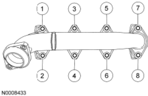
Fig. 602: Identifying Exhaust Manifold Nuts In Tightening Sequence Courtesy of FORD MOTOR CO.
