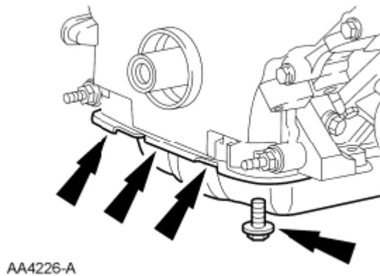
Fig. 353: Locating Front Oil Pan Bolts Courtesy of FORD MOTOR CO.
