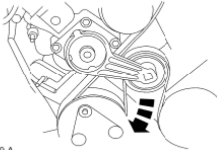
Fig. 43: Installing Accessory Drive Belt Onto Crankshaft Pulley Courtesy of FORD MOTOR CO.
