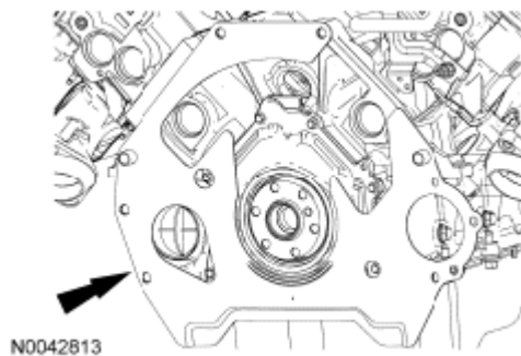
Fig. 557: Locating Spacer Plate Courtesy of FORD MOTOR CO.
