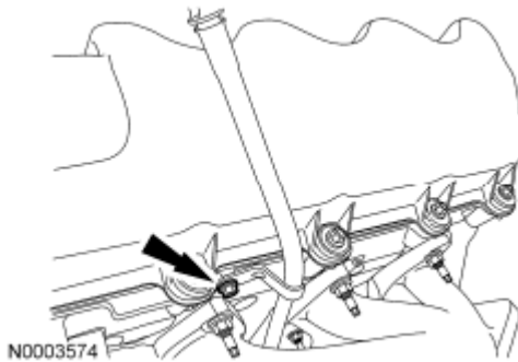
Fig. 407: Locating Bolt And Oil Level Indicator Tube Courtesy of FORD MOTOR CO.
