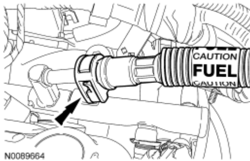
Fig. 16: Locating Fuel Supply Tube Quick Connect Coupling Courtesy of FORD MOTOR CO.
