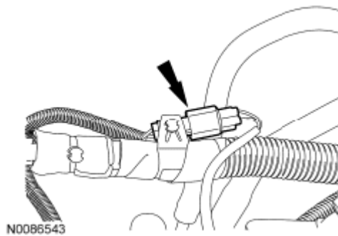
Fig. 327: Locating KS Electrical Connector LH Courtesy of FORD MOTOR CO.
