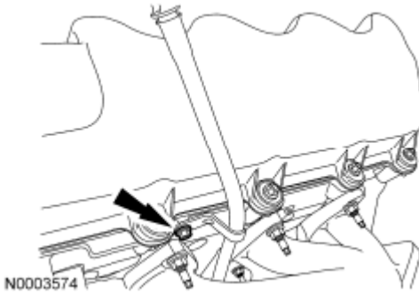
Fig. 634: Locating Oil Level Indicator Tube And Bolt Courtesy of FORD MOTOR CO.
