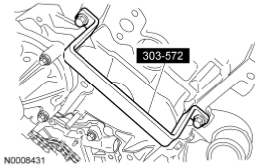
Fig. 488: Identifying Cylinder Head Remover/Installer From Cylinder Head LH Courtesy of FORD MOTOR CO.
