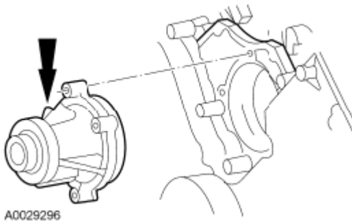
Fig. 417: Locating Coolant Pump From Cylinder Block Courtesy of FORD MOTOR CO.
