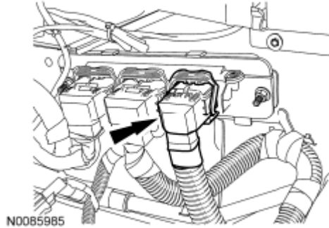
Fig. 33: Locating PCM Electrical Connector Courtesy of FORD MOTOR CO.
