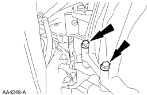
Fig. 562: Locating Upper Transmission-To-Engine Bolts Courtesy of FORD MOTOR CO.
