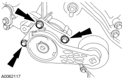
Fig. 415: Locating Bolts And Accessory Drive Belt Tensioner Courtesy of FORD MOTOR CO.
