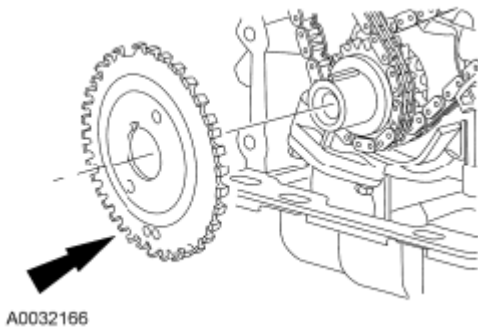
Fig. 508: Locating Crankshaft Sensor Ring On Crankshaft Courtesy of FORD MOTOR CO.
