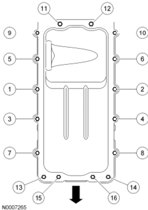
Fig. 554: Identifying Bolts In Tightening Sequence Courtesy of FORD MOTOR CO.
