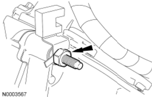
Fig. 544: Locating Nut And Radio Interference Capacitor LH Courtesy of FORD MOTOR CO.
