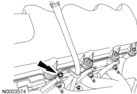
Fig. 535: Locating Bolt And Oil Level Indicator Tube Courtesy of FORD MOTOR CO.
