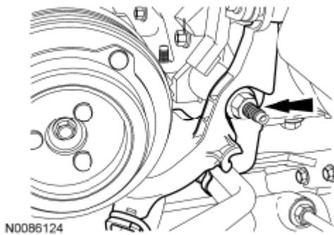
Fig. 568: Locating Starter Wiring Harness Support Bracket And Nut Courtesy of FORD MOTOR CO.
