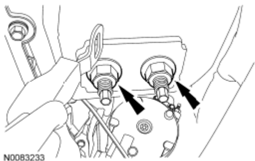
Fig. 314: Locating RH Engine Support Insulator Nuts Courtesy of FORD MOTOR CO.
