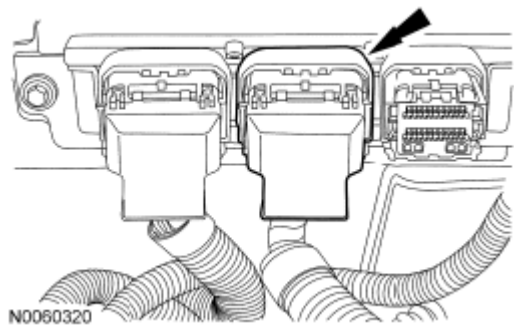
Fig. 31: Locating PCM Electrical Connector Courtesy of FORD MOTOR CO.
