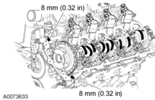
Fig. 19: Identifying Bead Of Silicone Gasket And Sealant Courtesy of FORD MOTOR CO.
