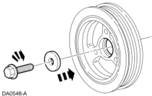
Fig. 640: Installing Crankshaft Pulley Bolt And Washer Courtesy of FORD MOTOR CO.
