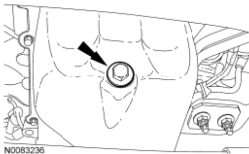
Fig. 235: Locating Oil Drain Plug Courtesy of FORD MOTOR CO.
