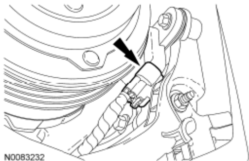
Fig. 308: Locating Crankshaft Position (CKP) Sensor Electrical Connector Courtesy of FORD MOTOR CO.
