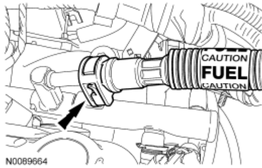
Fig. 12: Locating Fuel Supply Tube Quick Connect Coupling Courtesy of FORD MOTOR CO.
