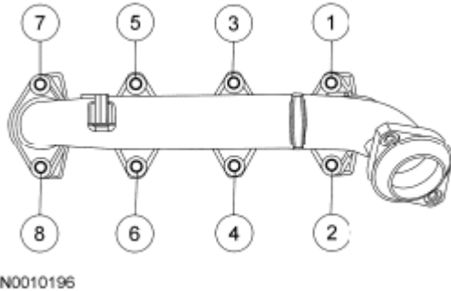
Fig. 527: Locating Exhaust Manifold Nuts In Tightening Sequence Courtesy of FORD MOTOR CO.
