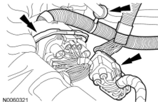
Fig. 26: Locating Electrical Connectors And Wiring Harness Retainer Courtesy of FORD MOTOR CO.
