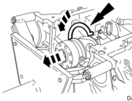
Fig. 471: Installing Rear Crankshaft Upper Thrust Washer Courtesy of FORD MOTOR CO.
