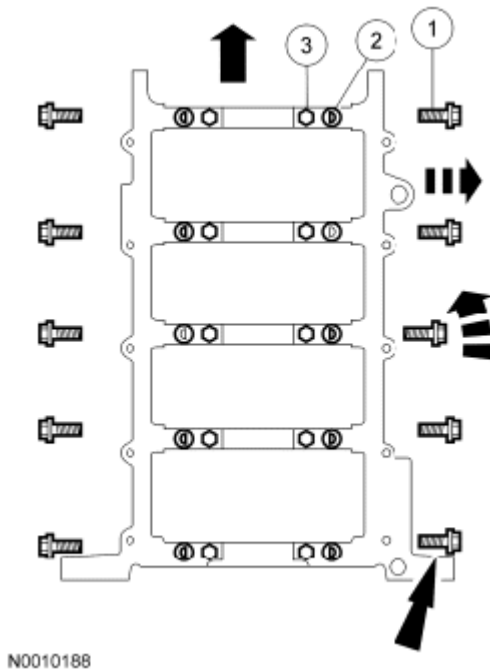
Fig. 451: Removing Camshaft Phaser And Sprocket Assembly With Bolt RH Courtesy of FORD MOTOR CO.
