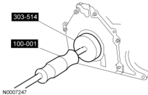
Fig. 274: Removing Crankshaft Oil Slinger Courtesy of FORD MOTOR CO.
