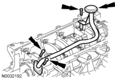
Fig. 258: Locating Oil Pump Screen And Pickup Tube With Bolts Courtesy of FORD MOTOR CO.
