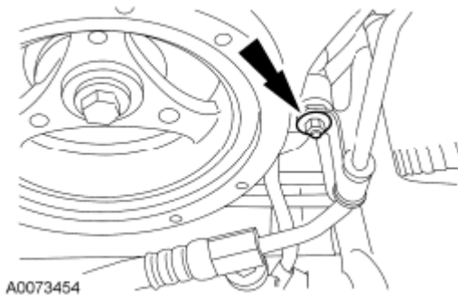
Fig. 82: Locating Power Steering Pressure Hose Support Bracket And Nut Courtesy of FORD MOTOR CO.
