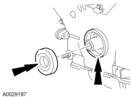
Fig. 517: Locating Engine Front Cover And Crankshaft Seal Inner Lip Courtesy of FORD MOTOR CO.
