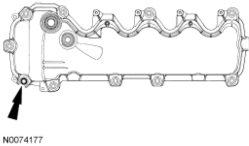
Fig. 408: [Locating Bolts And Valve Cover Gasket LH] Courtesy of FORD MOTOR CO.
