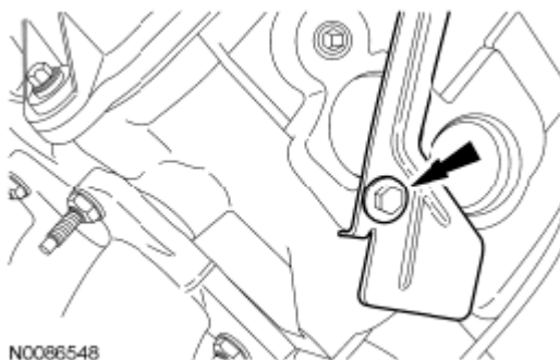
Fig. 344: Locating Bolt And Intake Manifold Vacuum Tube Support Bracket
