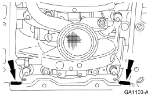
Fig. 551: Locating Crankshaft Rear Seal Retainer Plate-To-Cylinder Block Sealing Surface Courtesy of FORD MOTOR CO.
