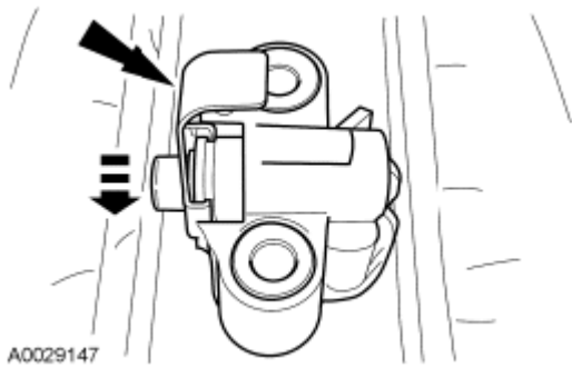
Fig. 610: Locating Retaining Clip On Tensioner Plunger Courtesy of FORD MOTOR CO.
