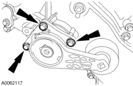
Fig. 523: Locating Bolts And Accessory Drive Belt Tensioner Courtesy of FORD MOTOR CO.
