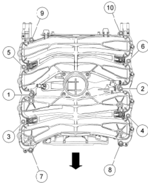
Fig. 14: Identifying Intake Manifold Bolts Courtesy of FORD MOTOR CO.
