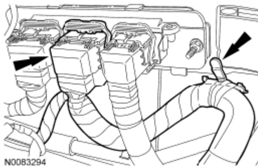
Fig. 583: Locating PCM Electrical Connector Courtesy of FORD MOTOR CO.
