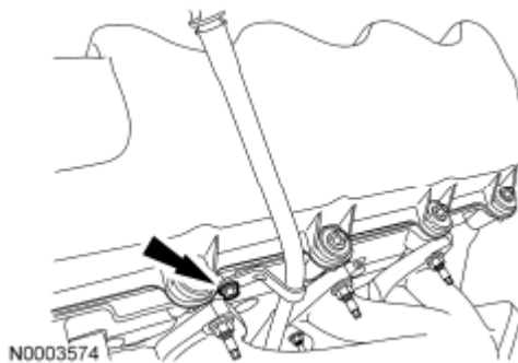
Fig. 346: Locating Bolt And Oil Level Indicator Tube Courtesy of FORD MOTOR CO.
