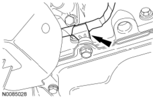
Fig. 248: Locating Oil Pan Bolt Courtesy of FORD MOTOR CO.
