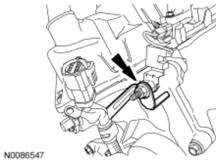
Fig. 648: Locating Nut And Engine Cooling Fan Clutch Electrical Connector Courtesy of FORD MOTOR CO.
