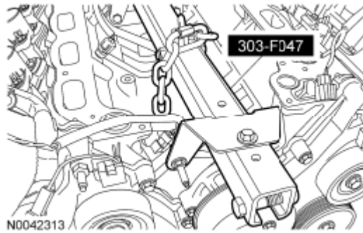
Fig. 336: Removing Engine Lifting Bracket Courtesy of FORD MOTOR CO.
