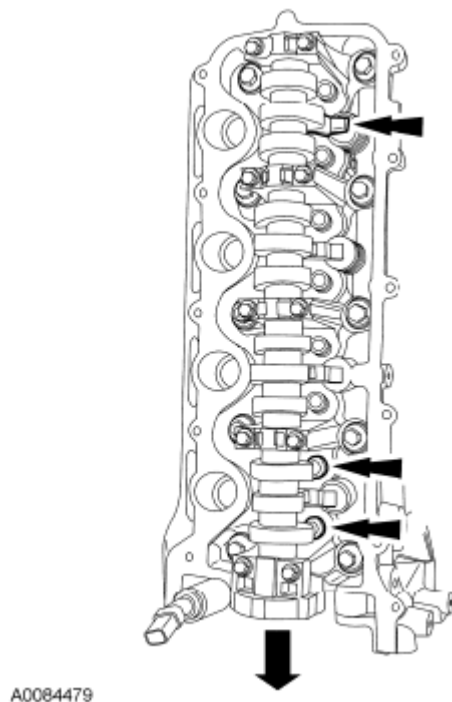
Fig. 175: Locating Camshaft Roller From Cylinder Head Courtesy of FORD MOTOR CO.
