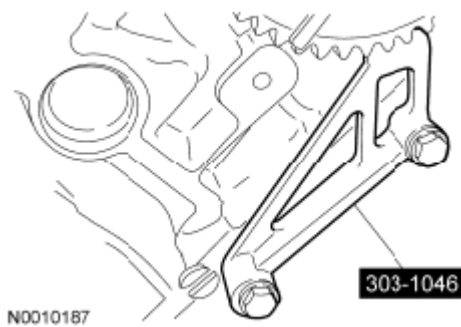
Fig. 493: Removing Camshaft Phaser And Sprocket Assembly With Bolt LH Courtesy of FORD MOTOR CO.
