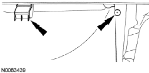
Fig. 79: Locating Retainer Tab Locks Courtesy of FORD MOTOR CO.
