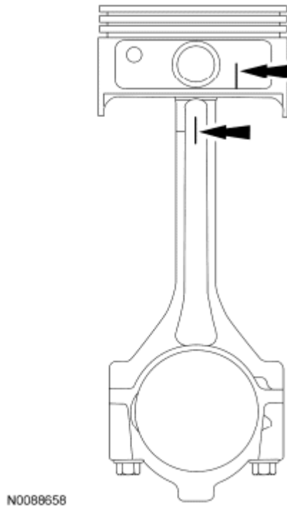
Fig. 460: Identifying Mark On Piston And Connecting Rod Courtesy of FORD MOTOR CO.
