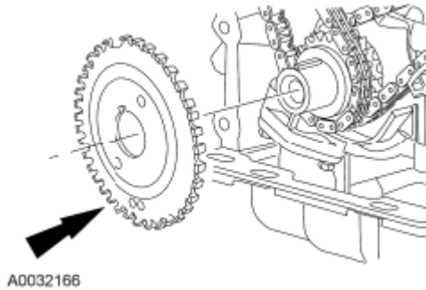
Fig. 356: Locating Crankshaft Sensor Ring On Crankshaft Courtesy of FORD MOTOR CO.
