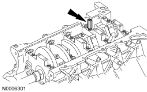
Fig. 483: Locating Oil Pump Screen And Pickup Tube Spacer Courtesy of FORD MOTOR CO.
