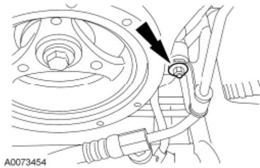
Fig. 587: Locating Power Steering Pressure Hose Support Bracket And Nut Courtesy of FORD MOTOR CO.
