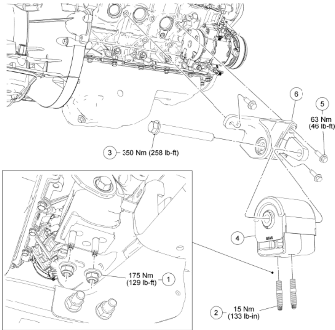
Fig. 282: Identifying Engine Support Insulator Components RH Courtesy of FORD MOTOR CO.
