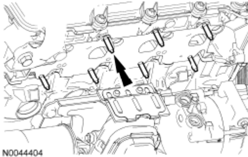
Fig. 601: Locating RH Exhaust Manifold-To-Cylinder Head Studs Courtesy of FORD MOTOR CO.
