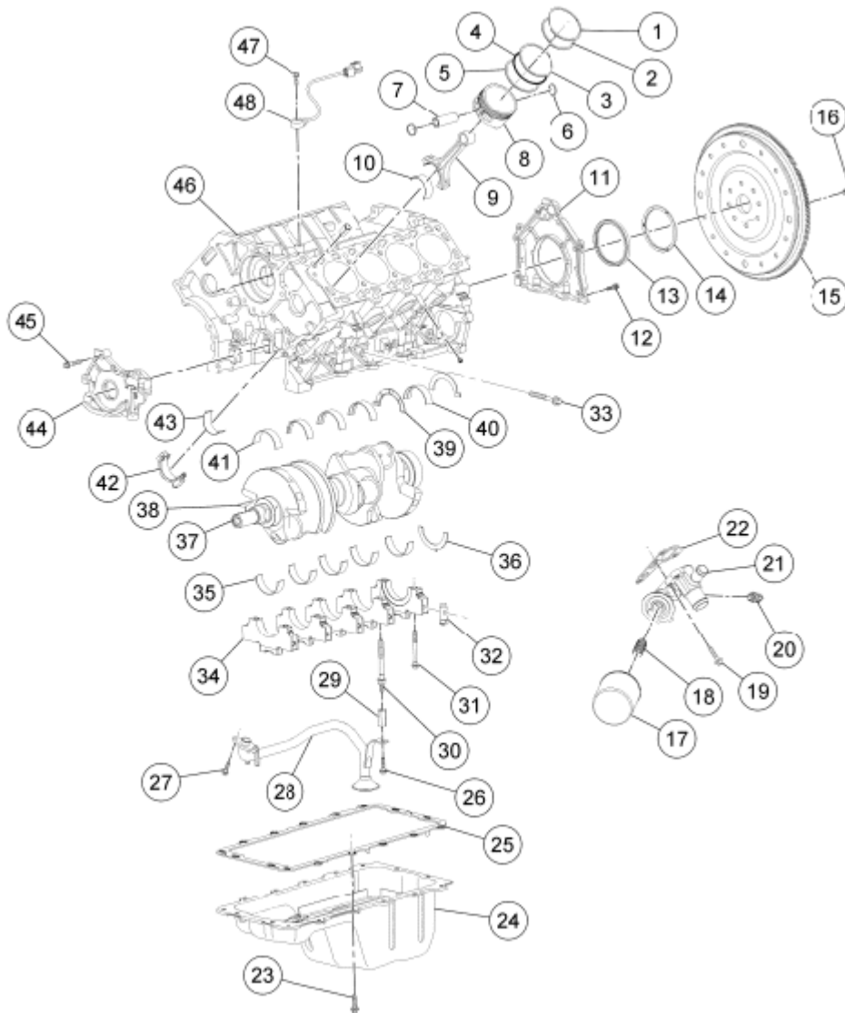
Fig. 465: Exploded View Of Engine - Lower End Courtesy of FORD MOTOR CO.
