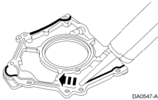
Fig. 548: Applying Bead Of Silicone Gasket And Sealant Around Courtesy of FORD MOTOR CO.
