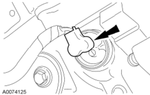
Fig. 570: Locating Block Heater Electrical Connector Courtesy of FORD MOTOR CO.
