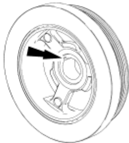
Fig. 39: Locating Woodruff Key Slot In Crankshaft Pulley Courtesy of FORD MOTOR CO.
