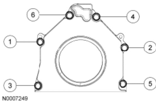
Fig. 277: Identifying Bolts In Tightening Sequence
