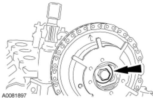
Fig. 137: Locating Camshaft Phaser And Sprocket Bolts Courtesy of FORD MOTOR CO.
