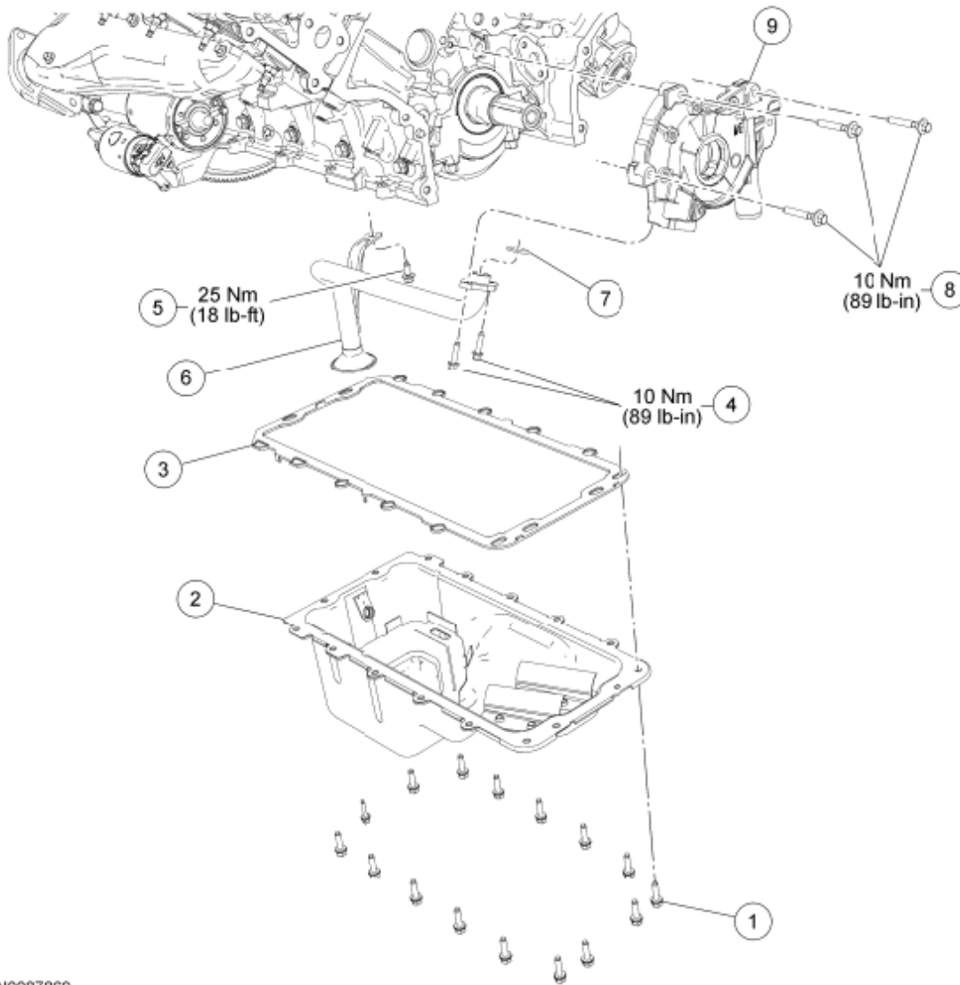
Fig. 234: Exploded View Of Engine Lubrication Components Courtesy of FORD MOTOR CO.
