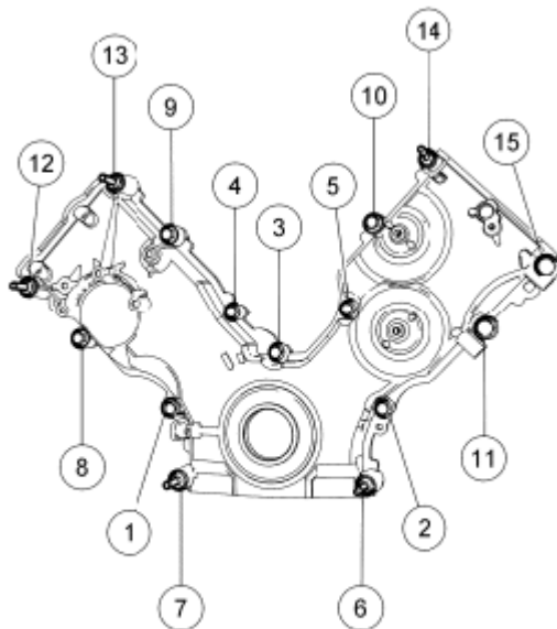
Fig. 628: Identifying Engine Front Cover Fasteners In Tightening Sequence Courtesy of FORD MOTOR CO.
