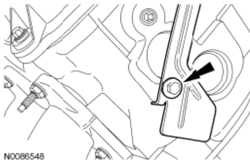
Fig. 399: Locating Bolt And Intake Manifold Vacuum Tube Support Bracket Courtesy of FORD MOTOR CO.
