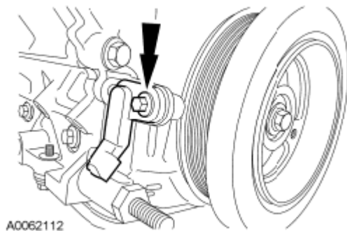
Fig. 405: Locating Bolt And Crankshaft Position (CKP) Sensor Courtesy of FORD MOTOR CO.
