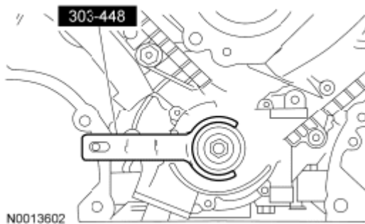
Fig. 612: Identifying Crankshaft With Crankshaft Holding Tool Courtesy of FORD MOTOR CO.
