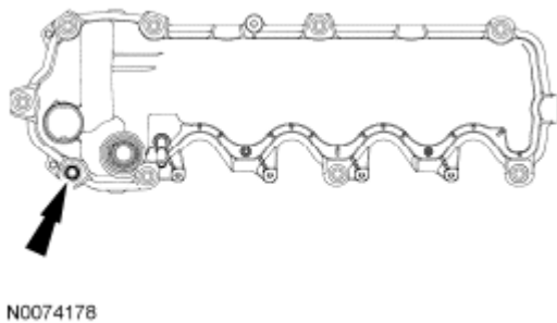
Fig. 409: [Locating Bolts And Valve Cover Gasket RH] Courtesy of FORD MOTOR CO.
