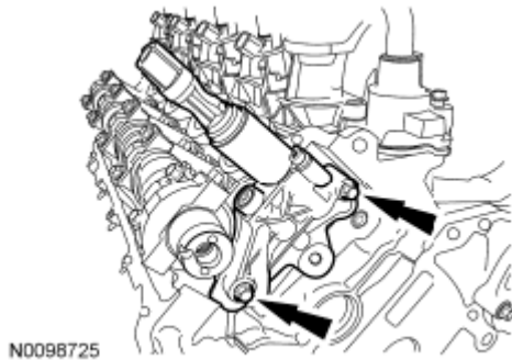
Fig. 213: Locating VCT Housing RH And Bolts Courtesy of FORD MOTOR CO.
