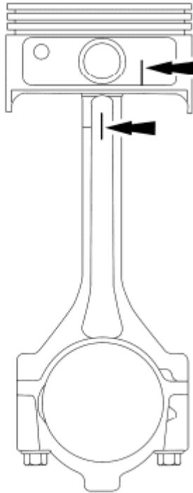
Fig. 459: Identifying Mark On Piston And Connecting Rod Courtesy of FORD MOTOR CO.
