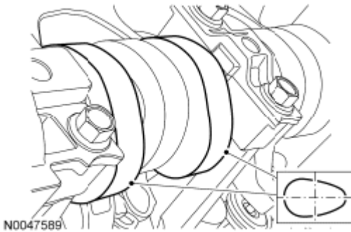
Fig. 185: Identifying No. 5 Cylinder Camshaft Lobe Courtesy of FORD MOTOR CO.
