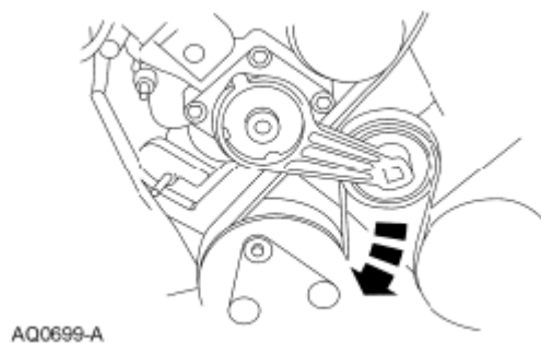
Fig. 45: Removing Accessory Drive Belt From Crankshaft Pulley
