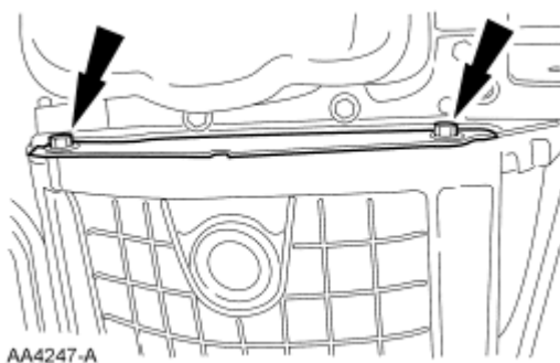
Fig. 566: Locating Flexplate Inspection Cover And Bolts Courtesy of FORD MOTOR CO.
