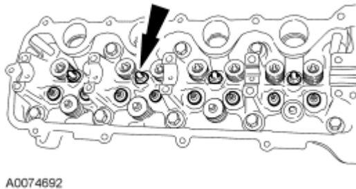
Fig. 490: Identifying Hydraulic Lash Adjusters Courtesy of FORD MOTOR CO.
