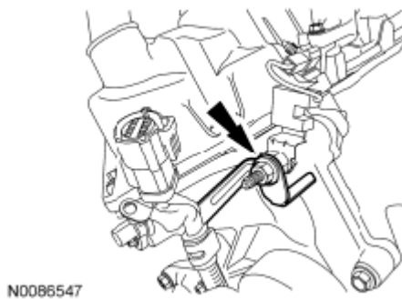
Fig. 546: Locating Nut And Engine Cooling Fan Clutch Electrical Connector Courtesy of FORD MOTOR CO.
