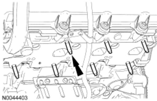
Fig. 374: Locating LH Exhaust Manifold-To-Cylinder Head Studs Courtesy of FORD MOTOR CO.
