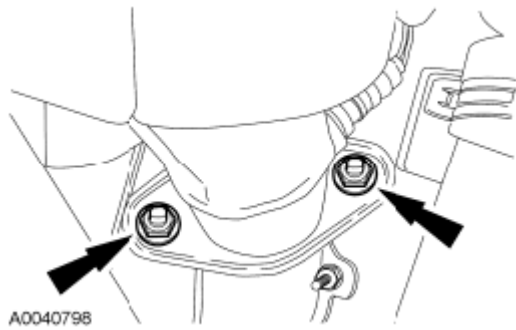
Fig. 233: Locating Exhaust Manifold-To-Catalytic Converter Nuts Courtesy of FORD MOTOR CO.
