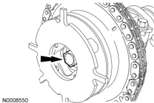
Fig. 199: Locating Bolt And Camshaft Phaser And Sprocket Assembly Courtesy of FORD MOTOR CO.
