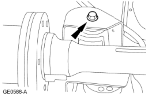
Fig. 239: Locating Axle Shaft Housing Carrier Bushing Bolt Courtesy of FORD MOTOR CO.
