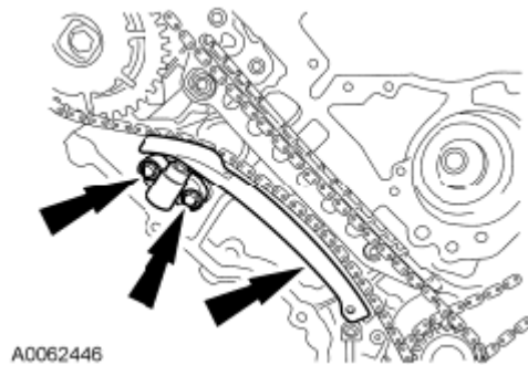
Fig. 365: Locating Timing Chain Tensioner And Bolts RH Courtesy of FORD MOTOR CO.
