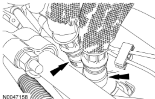
Fig. 577: Locating Auxiliary Heat Coolant Hoses Courtesy of FORD MOTOR CO.
