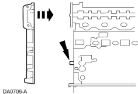
Fig. 627: Locating Engine Front Cover Gasket On Engine Front Cover Courtesy of FORD MOTOR CO.
