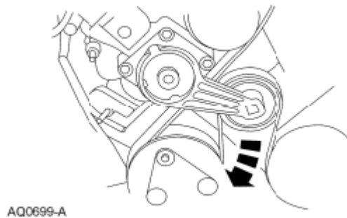
Fig. 57: Removing Accessory Drive Belt From Crankshaft Pulley Courtesy of FORD MOTOR CO.
