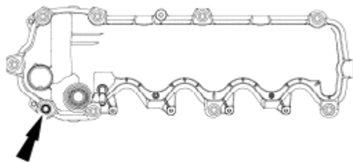
Fig. 348: [Locating Bolts And Valve Cover Gasket RH] Courtesy of FORD MOTOR CO.
