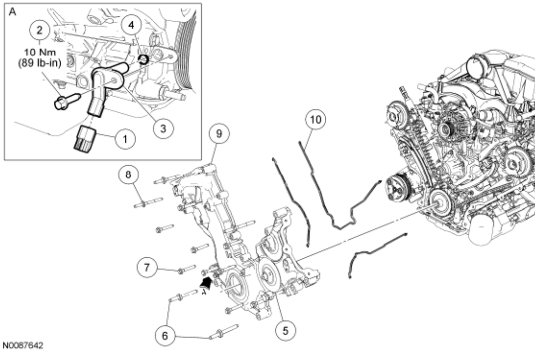
Fig. 56: Identifying Engine Front Cover, Gaskets And Crankshaft Position (CKP) Sensor Components Courtesy of FORD MOTOR CO.
