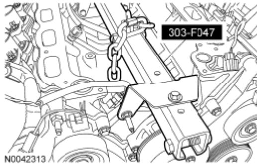
Fig. 335: Installing Engine Lifting Bracket Courtesy of FORD MOTOR CO.
