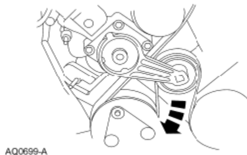
Fig. 37: Removing Accessory Drive Belt From Crankshaft Pulley Courtesy of FORD MOTOR CO.
