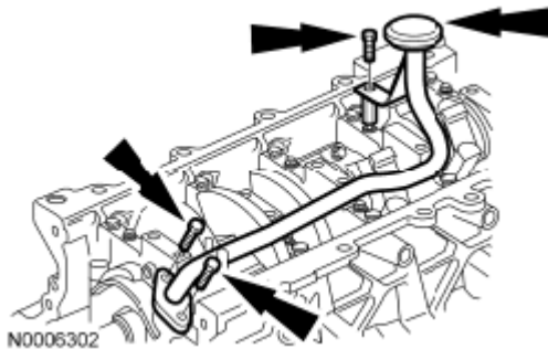
Fig. 484: Locating Oil Pump Screen And Pickup Tube And Bolts Courtesy of FORD MOTOR CO.
