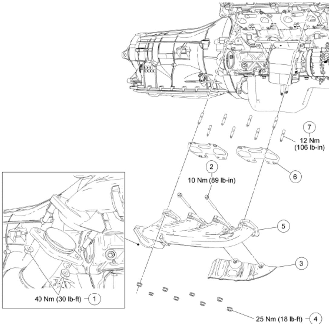
Fig. 226: Exploded View Of Exhaust Manifold (RH) Courtesy of FORD MOTOR CO.
