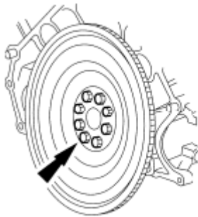
Fig. 387: Locating Flexplate Bolts Courtesy of FORD MOTOR CO.
