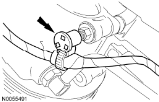
Fig. 81: Locating Power Steering Pump Stud Bolt Courtesy of FORD MOTOR CO.
