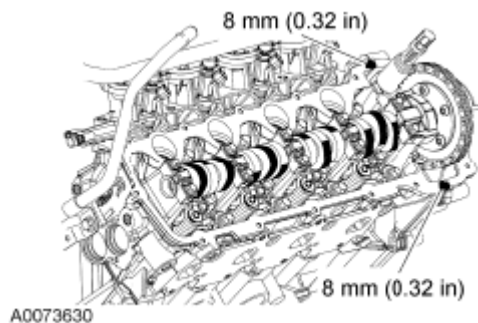
Fig. 531: Identifying Silicone Gasket And Sealant Area Courtesy of FORD MOTOR CO.
