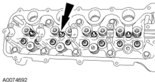
Fig. 600: Identifying Hydraulic Lash Adjusters Courtesy of FORD MOTOR CO.
