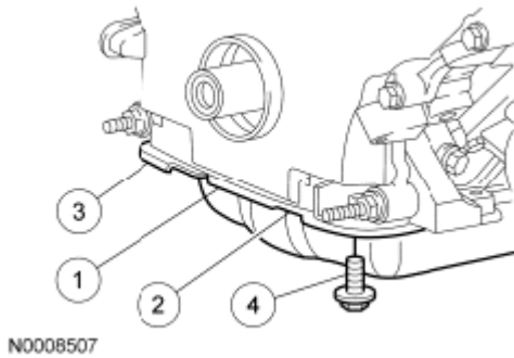
Fig. 629: Identifying Bolts In Tightening Sequence Courtesy of FORD MOTOR CO.
