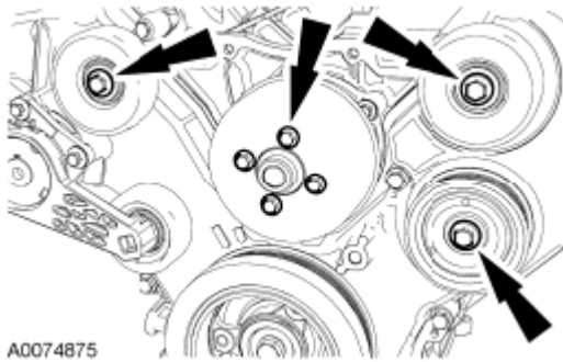
Fig. 349: Locating Bolts And Coolant Pump Pulley Courtesy of FORD MOTOR CO.
