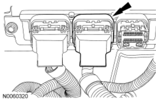
Fig. 25: Locating PCM Electrical Connector Courtesy of FORD MOTOR CO.
