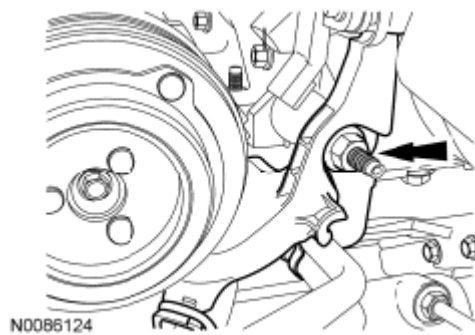
Fig. 243: Locating Starter Wiring Harness And Nut Courtesy of FORD MOTOR CO.
