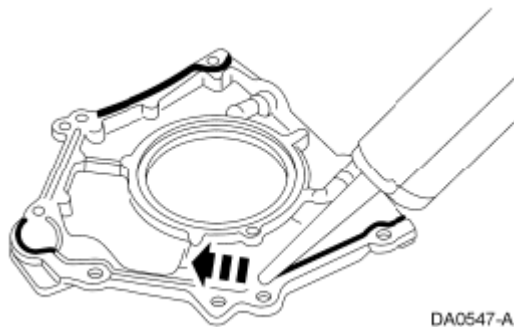
Fig. 276: Applying Bead Of Silicone Gasket And Sealant Around Crankshaft Rear Seal Retainer Plate Sealing Surface
