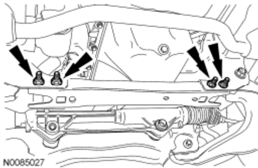
Fig. 257: Locating Crossmember With Nuts And Bolts Courtesy of FORD MOTOR CO.
