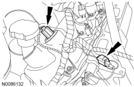
Fig. 330: Locating Radio Ignition Interference Capacitor Electrical Connectors RH Courtesy of FORD MOTOR CO.
