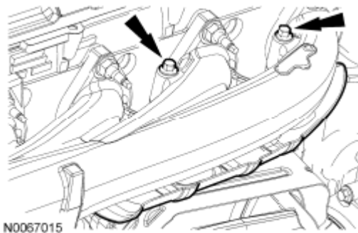
Fig. 603: Locating Exhaust Manifold Heat Shield And Bolts
