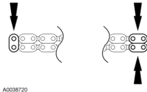
Fig. 496: Locating Timing Marks Courtesy of FORD MOTOR CO.
