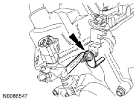
Fig. 395: Locating Nut And Engine Cooling Fan Clutch Electrical Connector Courtesy of FORD MOTOR CO.
