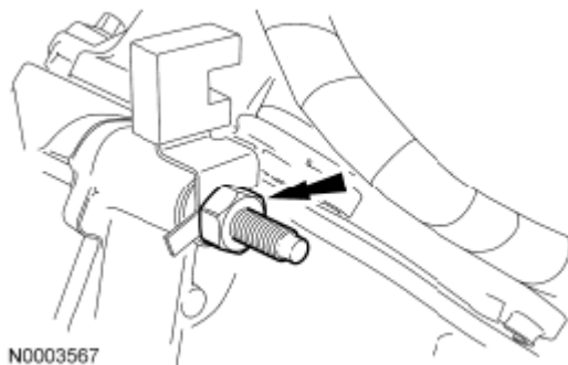
Fig. 343: Locating Nut And Radio Interference Capacitor LH Courtesy of FORD MOTOR CO.
