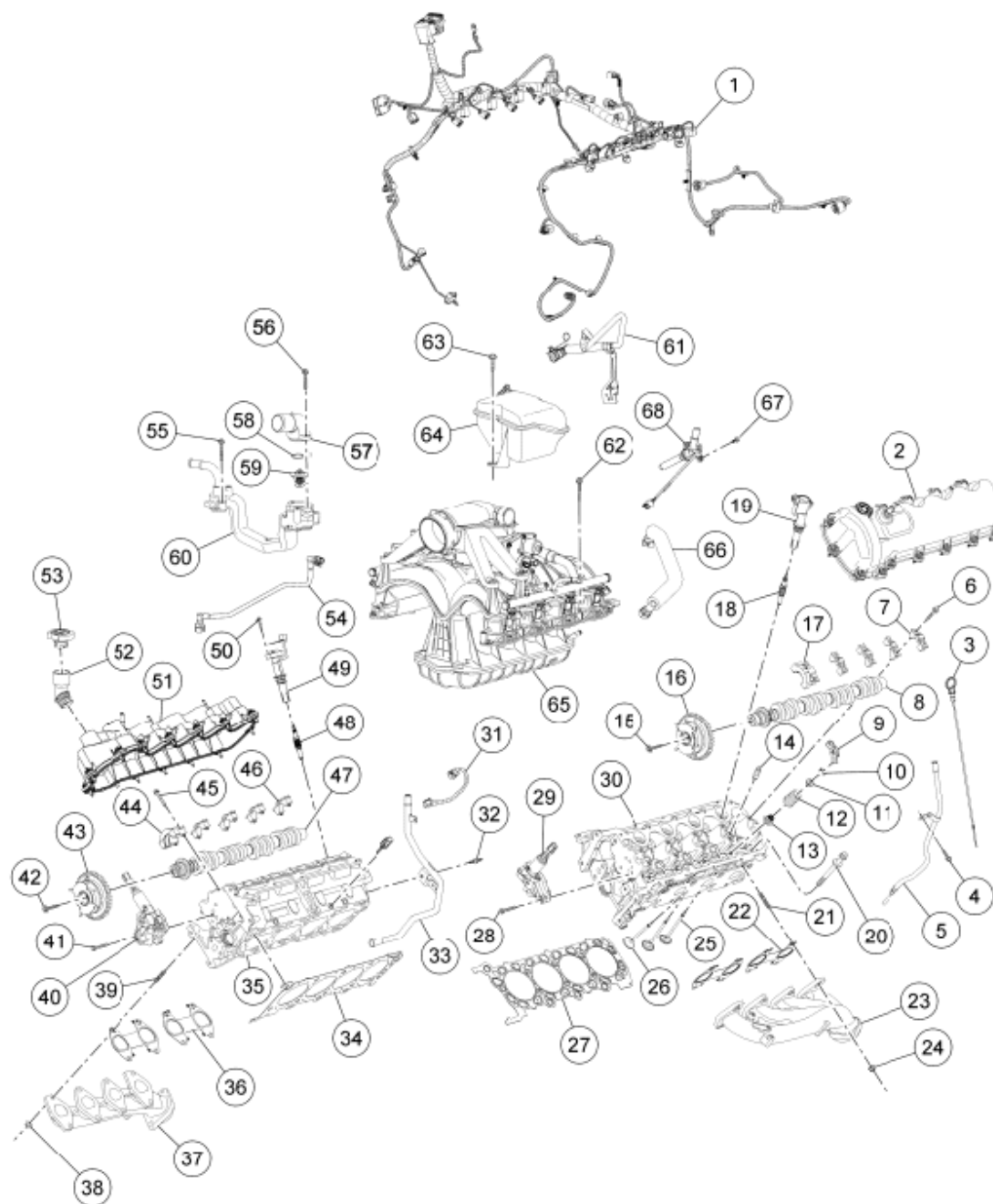
Fig. 463: Exploded View Of Engine - Upper End Courtesy of FORD MOTOR CO.
