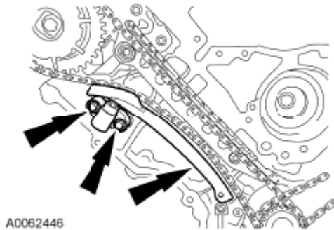
Fig. 505: Locating Timing Chain Tensioner And Bolts RH Courtesy of FORD MOTOR CO.
