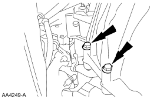
Fig. 305: Locating Upper Transmission-To-Engine Bolts Courtesy of FORD MOTOR CO.
