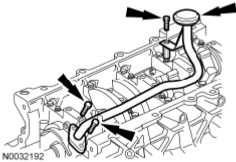
Fig. 263: Locating Oil Pump Screen And Pickup Tube With Bolts Courtesy of FORD MOTOR CO.
