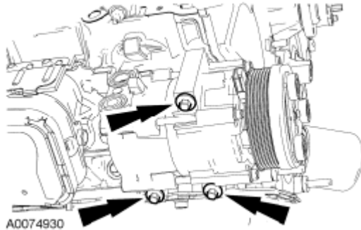
Fig. 567: Locating A/C Compressor And Bolts Courtesy of FORD MOTOR CO.
