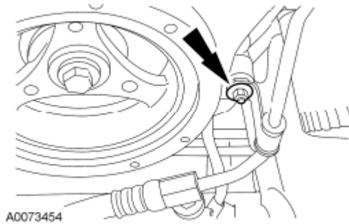
Fig. 318: Locating Power Steering Pressure Hose Support Bracket And Nut Courtesy of FORD MOTOR CO.
