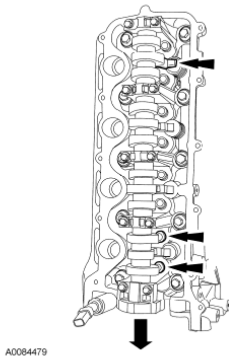
Fig. 129: Locating Camshaft Roller From Cylinder Head Courtesy of FORD MOTOR CO.
