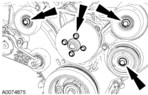
Fig. 642: Locating Bolts And Coolant Pump Pulley Courtesy of FORD MOTOR CO.
