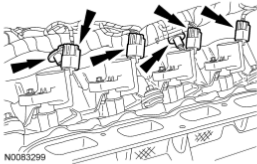
Fig. 579: Locating Ignition Coil Electrical Connectors RH Courtesy of FORD MOTOR CO.
