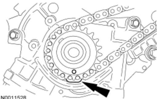
Fig. 499: Locating Timing Chain On Crankshaft Sprocket Courtesy of FORD MOTOR CO.
