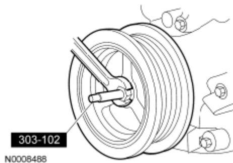
Fig. 77: Installing Crankshaft Pulley Courtesy of FORD MOTOR CO.
