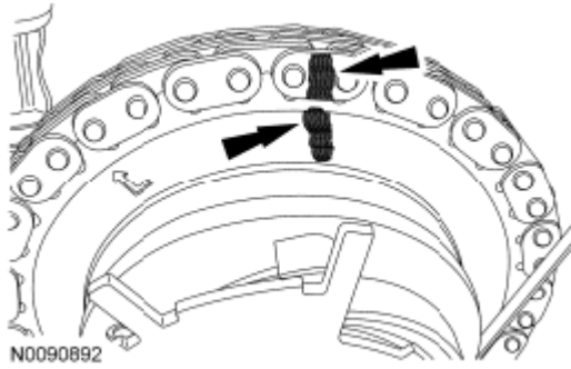
Fig. 179: Locating Mark On Timing Chain And Camshaft Phaser And Sprocket Assembly Courtesy of FORD MOTOR CO.
