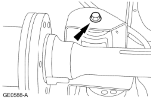
Fig. 255: Locating Axle Shaft Housing Carrier Bushing Bolt Courtesy of FORD MOTOR CO.
