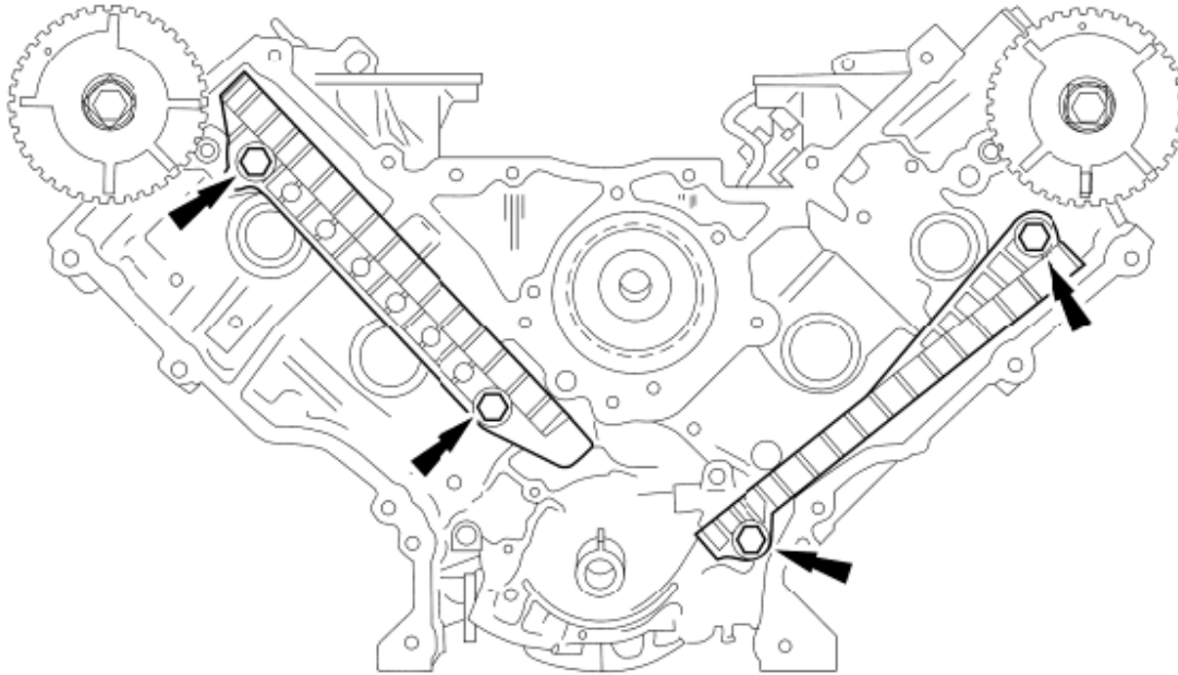
Fig. 498: Locating Timing Chain Guides With Bolts (LH And RH) Courtesy of FORD MOTOR CO.
