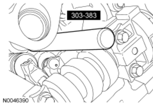
Fig. 223: Installing Valve Seal Courtesy of FORD MOTOR CO.
