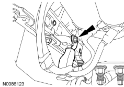
Fig. 241: Locating Starter Wiring Harness Rear Support Bracket Bolt Courtesy of FORD MOTOR CO.
