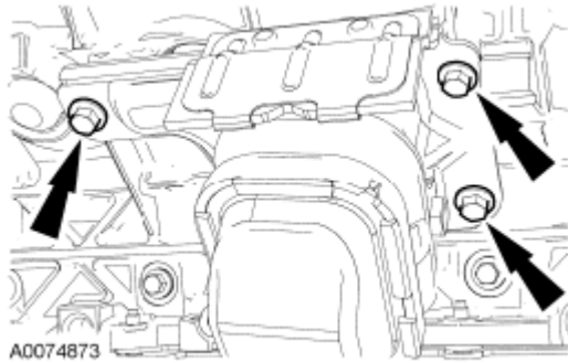
Fig. 392: Locating Bolts And Engine Support Insulator RH Courtesy of FORD MOTOR CO.
