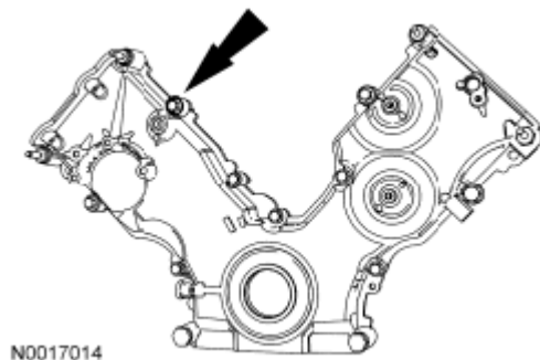
Fig. 354: Locating Engine Front Cover Fasteners Courtesy of FORD MOTOR CO.
