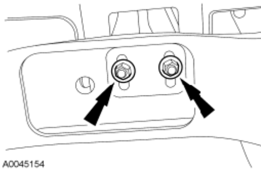
Fig. 298: Locating Transmission Mount-To-Crossmember Nuts Courtesy of FORD MOTOR CO.
