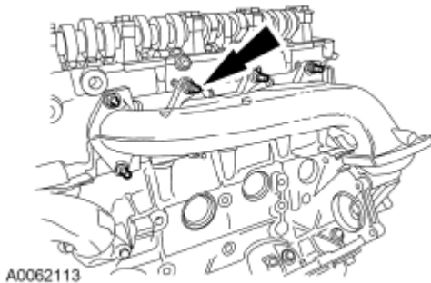
Fig. 373: Locating Nuts And Exhaust Manifold LH Courtesy of FORD MOTOR CO.
