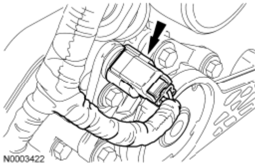
Fig. 149: Locating CMP Sensor Electrical Connector
