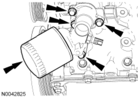
Fig. 413: Locating Bolts And Oil Filter Adapter Courtesy of FORD MOTOR CO.
