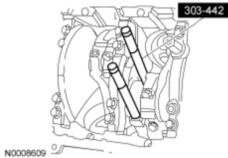
Fig. 480: Removing Connecting Rod Installer Courtesy of FORD MOTOR CO.
