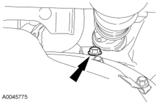
Fig. 256: Locating Upper Front Axle Carrier Mounting Bushing Bolt Courtesy of FORD MOTOR CO.
