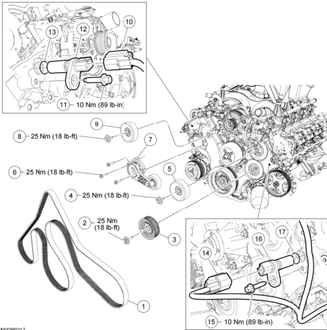
Fig. 54: Identifying Front End Accessory Drive (FEAD) And Camshaft Position (CMP) Sensors Components (LH And RH)
