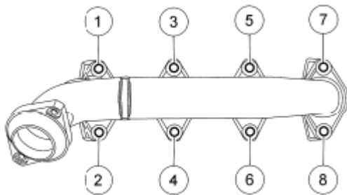
Fig. 227: Identifying Exhaust Manifold Nuts In Tightening Sequence Courtesy of FORD MOTOR CO.
