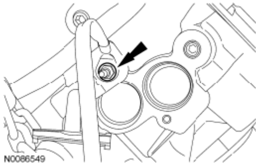
Fig. 383: Locating Nut And Ground Strap Courtesy of FORD MOTOR CO.
