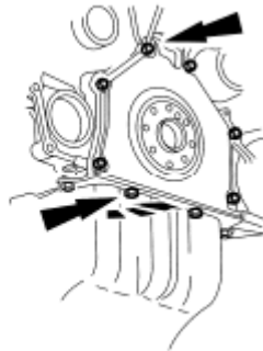
Fig. 390: Locating Bolts And Crankshaft Rear Seal Retainer Plate Courtesy of FORD MOTOR CO.
