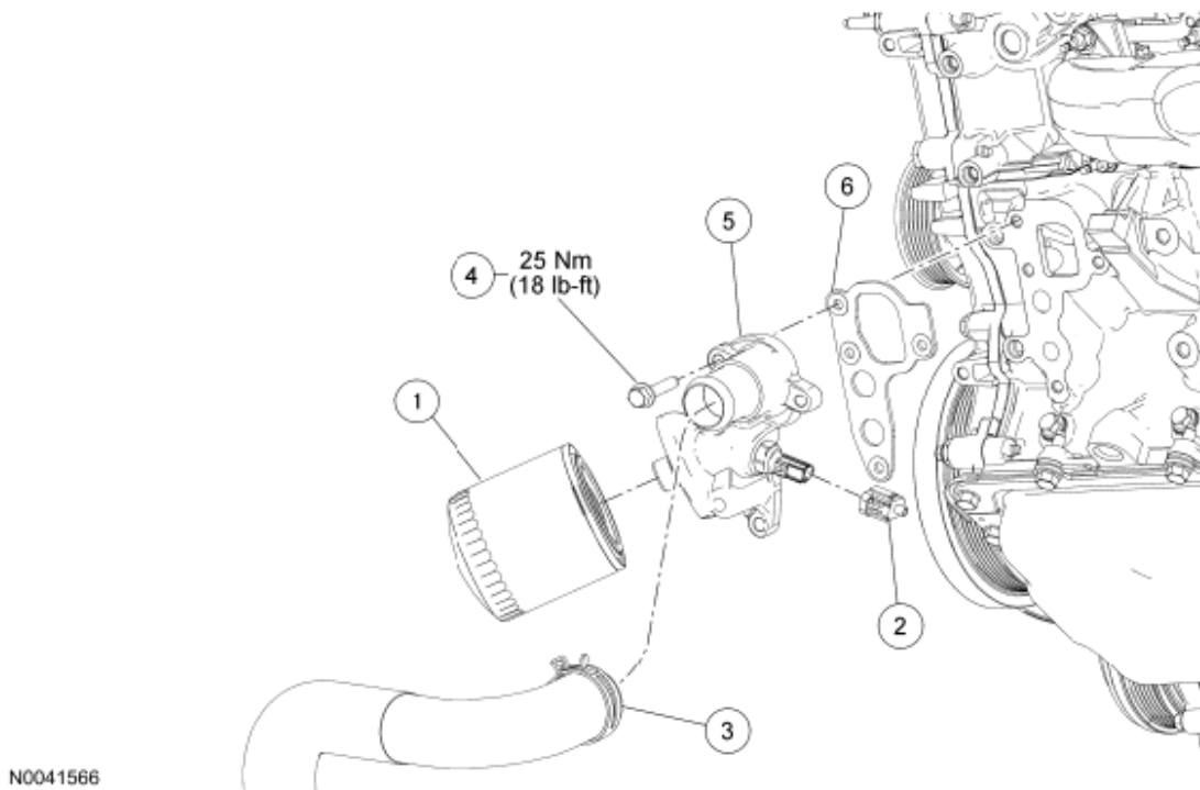
Fig. 264: Identifying Oil Filter Adapter Components Courtesy of FORD MOTOR CO.
