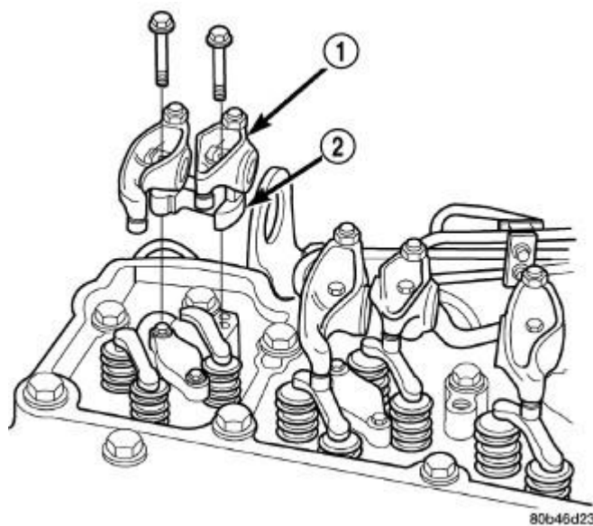
Fig. 19: Rocker Arms and Pedestal Removal Courtesy of CHRYSLER LLC
