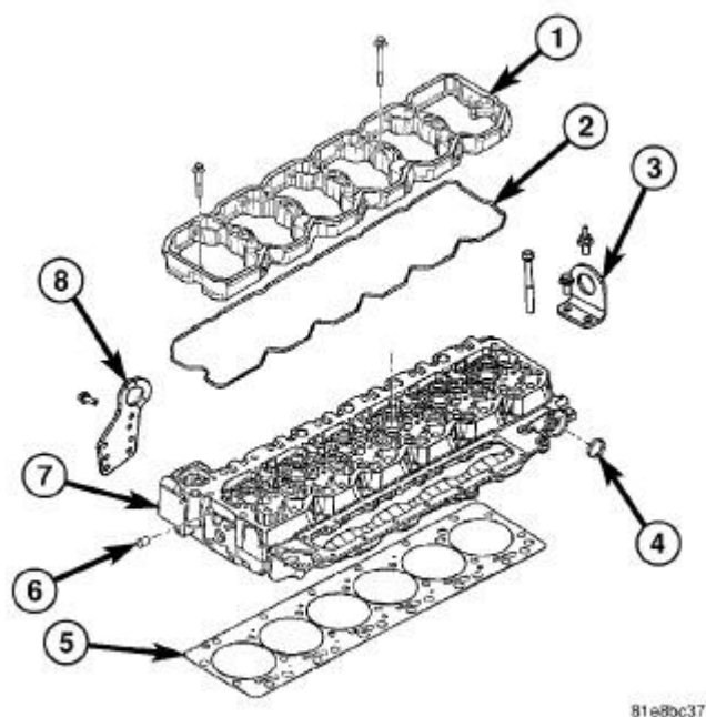
Fig. 93: CYLINDER HEAD AND GASKET
