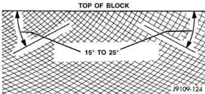
Fig. 128: Cylinder Bore Crosshatch Pattern
