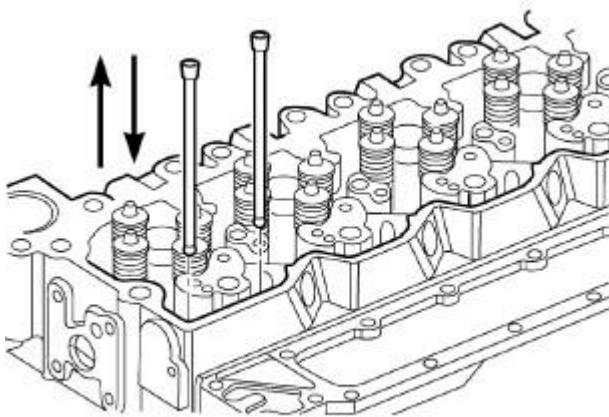
Fig. 78: Push Rod Removal/Installation Courtesy of CHRYSLER LLC
