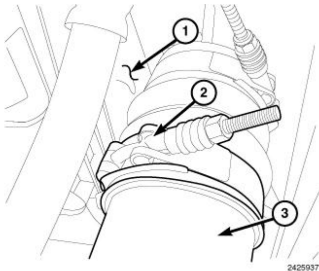
Fig. 239: Identifying Clamp, Charge Inlet Tube & Charge Air Cooler (CAC) Courtesy of CHRYSLER LLC
