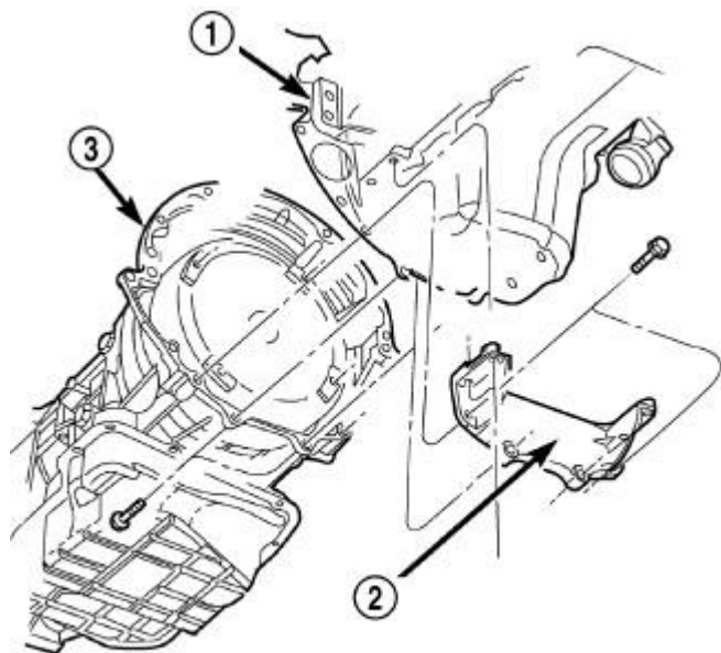
Fig. 184: Transmission Collar Courtesy of CHRYSLER LLC
