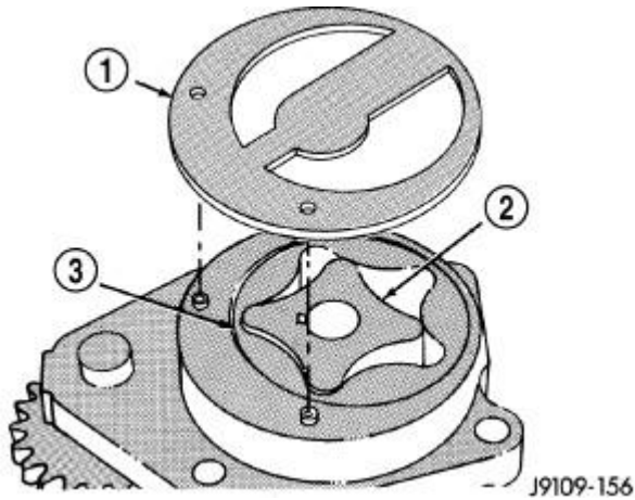
Fig. 289: Gerotor Planetary and Gerotor Courtesy of CHRYSLER LLC
