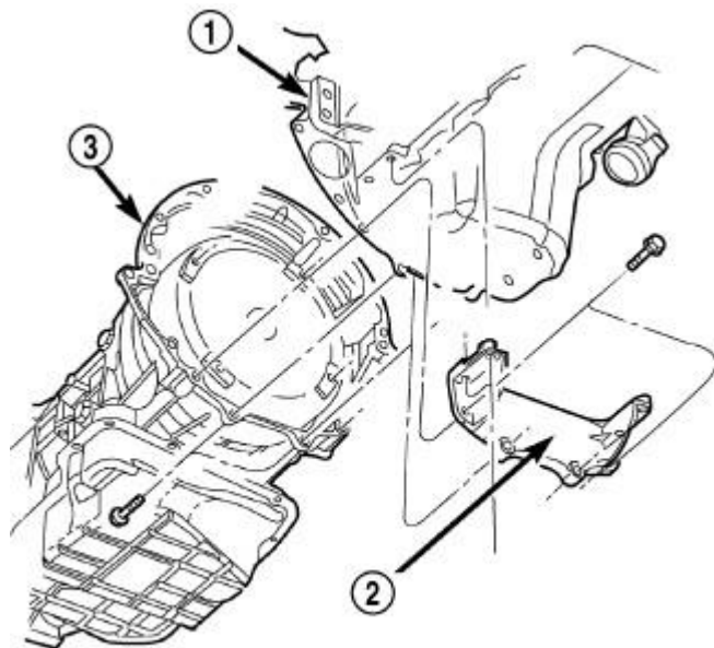
Fig. 174: Transmission Collar Courtesy of CHRYSLER LLC
