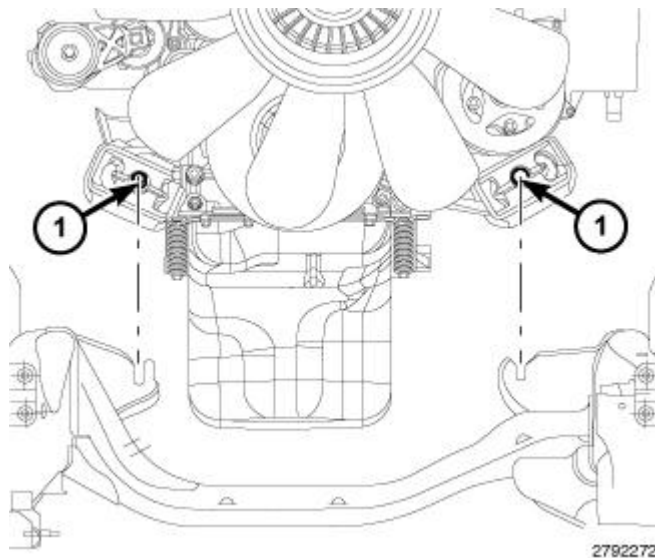
Fig. 214: Identifying Frame Mount Thru-Bolts & Nuts Courtesy of CHRYSLER LLC
