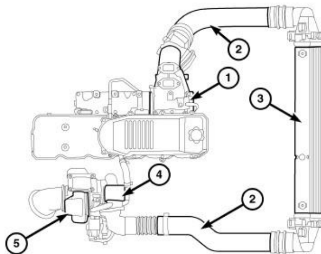
Fig. 156: CHARGE AIR COOLER
