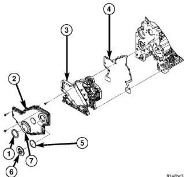
Fig. 139: Front Cover Assembly Components
