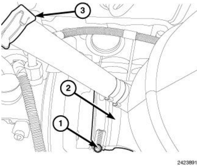
Fig. 59: Identifying Clamp, Outlet Tube & Breather Hose Courtesy of CHRYSLER LLC
