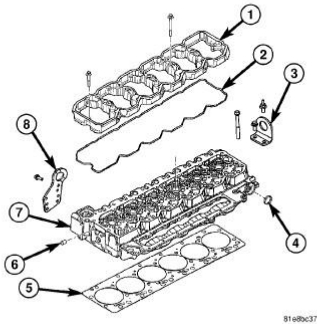
Fig. 80: CYLINDER HEAD AND GASKET Courtesy of CHRYSLER LLC
