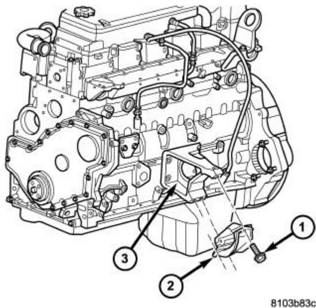
Fig. 282: LH Insulator Courtesy of CHRYSLER LLC
