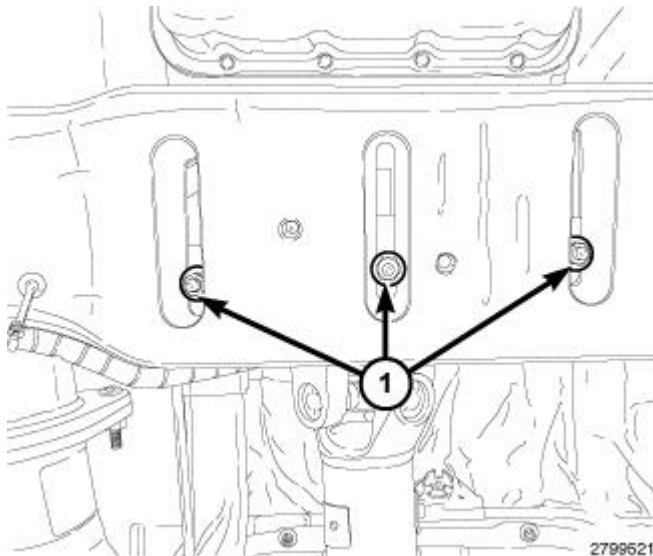
Fig. 227: Identifying Rear Transmission Mount To Crossmember Nuts - AS68RC A/T Courtesy of CHRYSLER LLC
