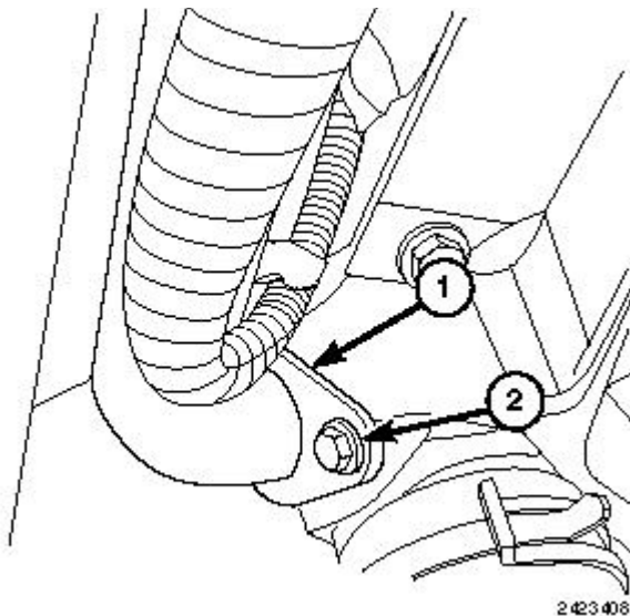
Fig. 242: Identifying Front Coolant Tube Bolt Courtesy of CHRYSLER LLC
