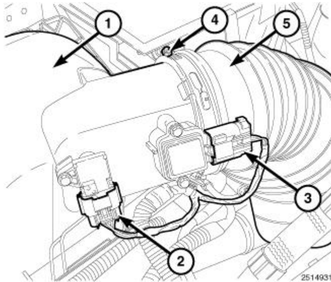
Fig. 58: Identifying MAF Sensor, TBAP Sensor, Intake Air Tube, Air Cleaner Body & Clamp Courtesy of CHRYSLER LLC
