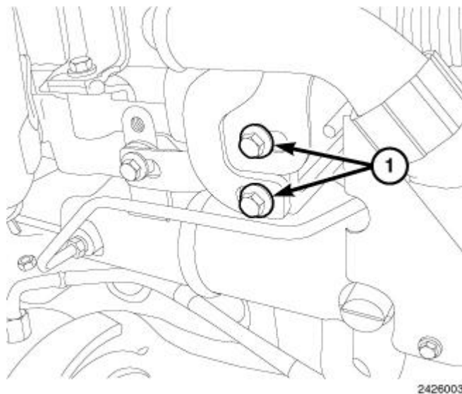
Fig. 252: Identifying Bracket Bolts Courtesy of CHRYSLER LLC
