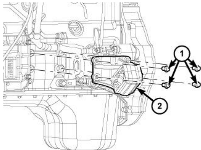
Fig. 211: LH Engine Mount Courtesy of CHRYSLER LLC
