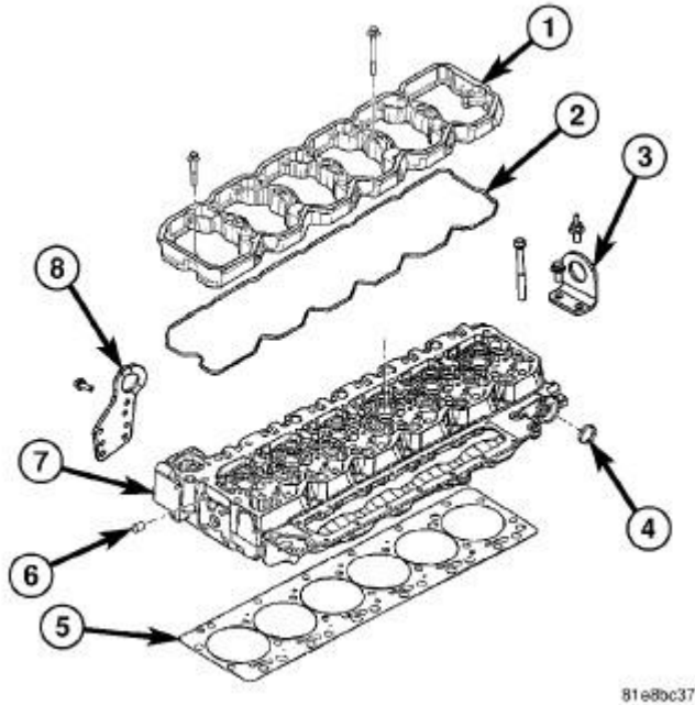
Fig. 186: CYLINDER HEAD AND GASKET
