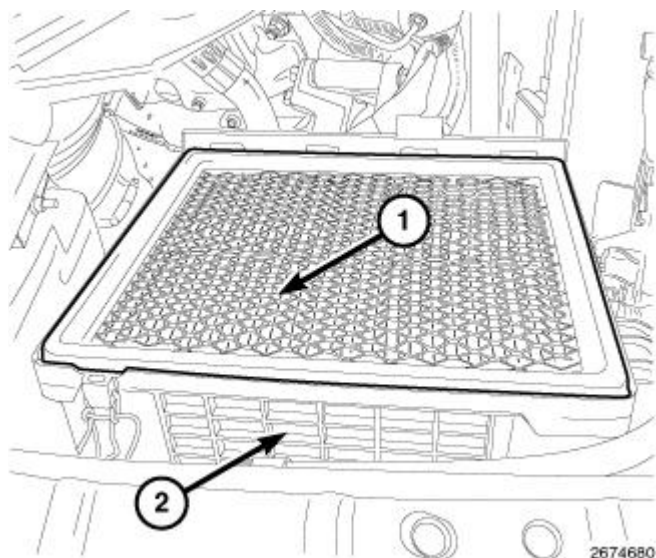
Fig. 54: Identifying Air Cleaner Housing & Air Cleaner Filter Courtesy of CHRYSLER LLC
