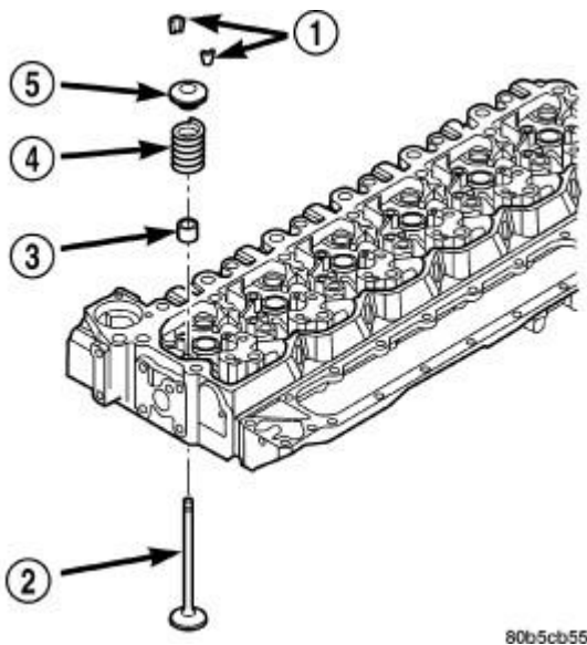
Fig. 118: Valve Spring, Seal, and Retainers Courtesy of CHRYSLER LLC
