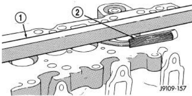
Fig. 72: Inspecting Cylinder Head Combustion Deck Face For Warpage Courtesy of CHRYSLER LLC
