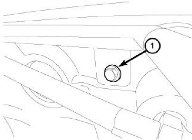
Fig. 255: Identifying Coolant Outlet Tube Bracket Bolt Courtesy of CHRYSLER LLC
