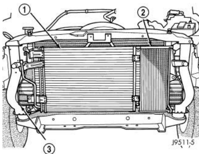
Fig. 352: Condenser and Transmission Auxiliary Cooler Courtesy of CHRYSLER LLC
