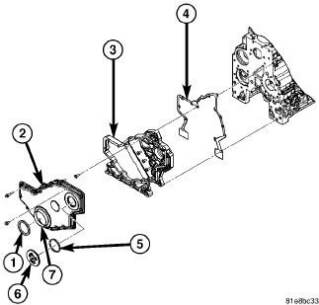
Fig. 346: Front Cover Assembly Components
