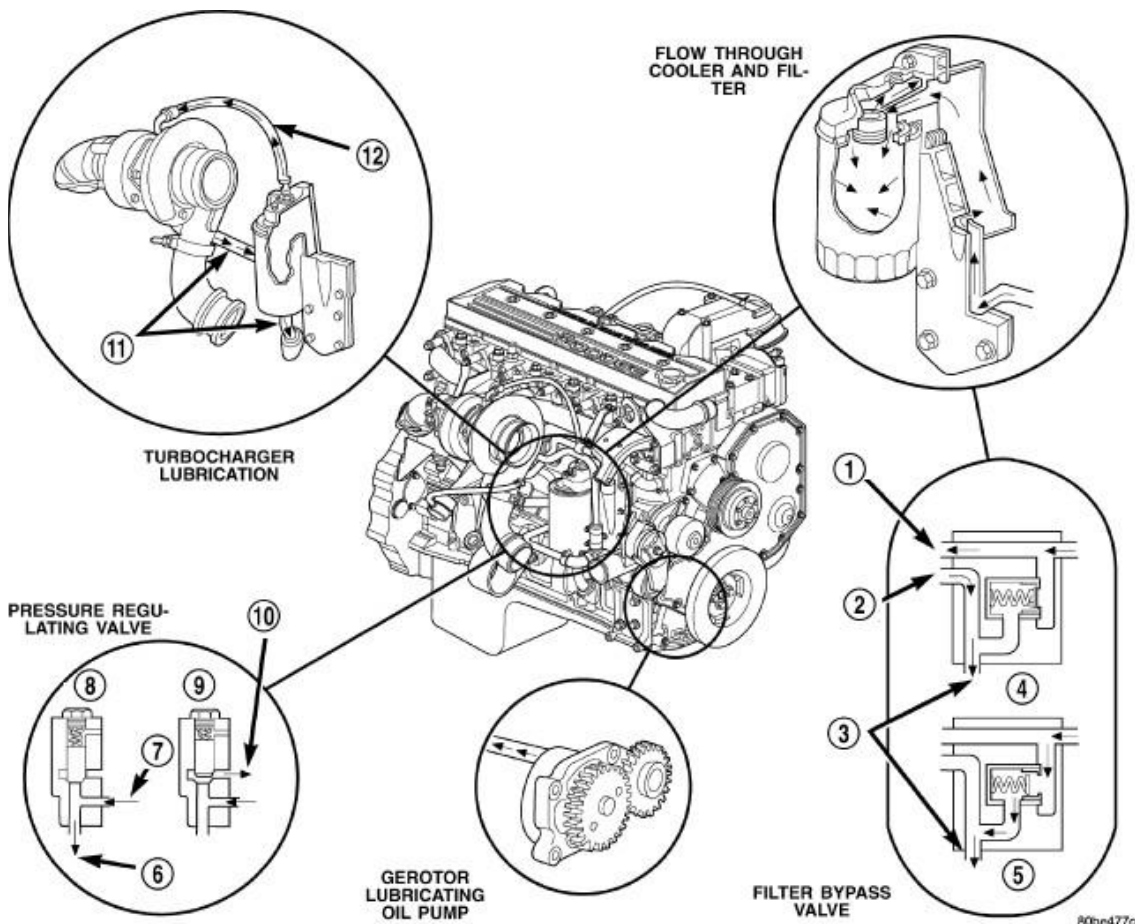
Fig. 232: Lubrication System Circulation (1 Of 2) Courtesy of CHRYSLER LLC
