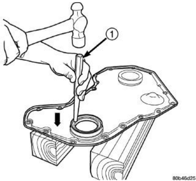
Fig. 190: Removing Seal from Cover Courtesy of CHRYSLER LLC
