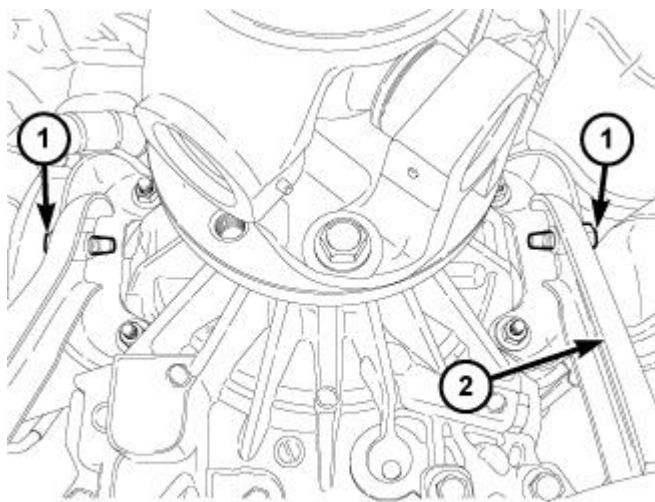
Fig. 225: Identifying Transmission Support Bracket & Bolts - AS68RC A/T Courtesy of CHRYSLER LLC
