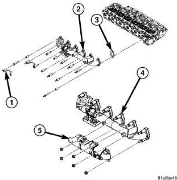
Fig. 299: Cylinder Head And Exhaust Manifold Courtesy of CHRYSLER LLC
