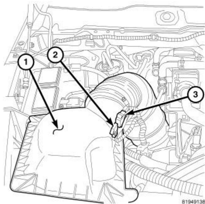
Fig. 260: Air Cleaner Housing
