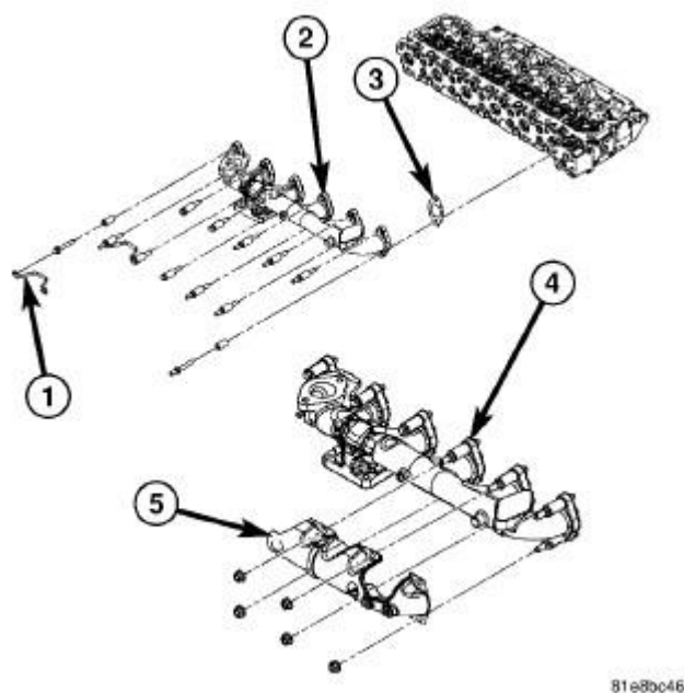
Fig. 84: Cylinder Head And Exhaust Manifold Courtesy of CHRYSLER LLC
