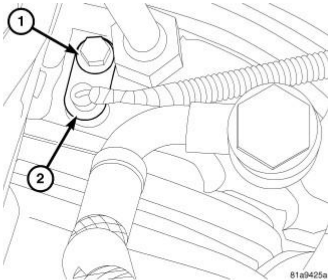
Fig. 329: Turbocharger Speed Sensor And Mounting Bolt Courtesy of CHRYSLER LLC
