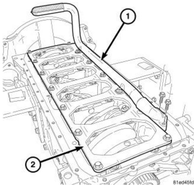
Fig. 275: OIL PICKUP TUBE Courtesy of CHRYSLER LLC
