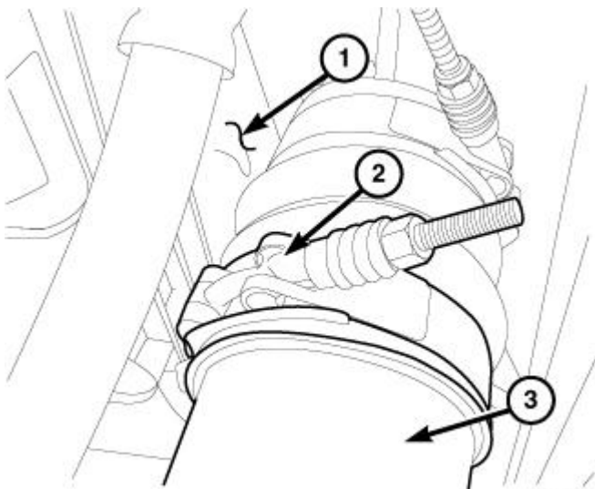
Fig. 256: Identifying Clamp, Charge Inlet Tube & Charge Air Cooler (CAC) Courtesy of CHRYSLER LLC
