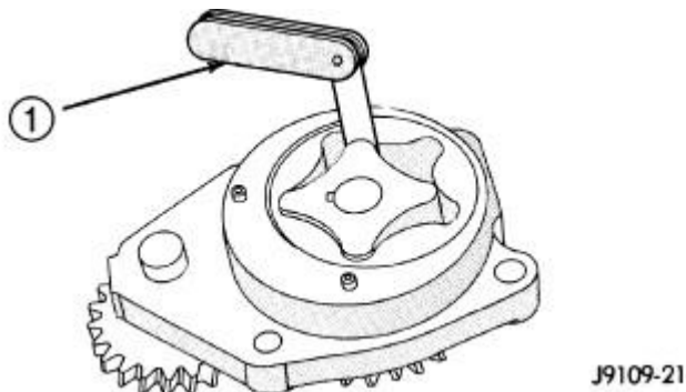
Fig. 290: Measuring Tip Clearance Courtesy of CHRYSLER LLC
