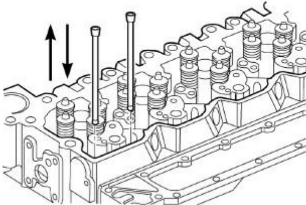
Fig. 140: Push Rod Removal/Installation
