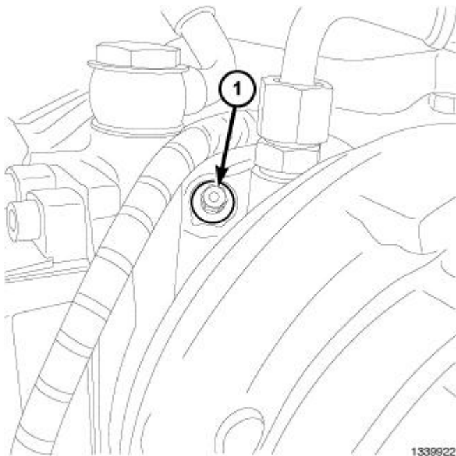
Fig. 306: Identifying Turbocharger Cleaning Port Courtesy of CHRYSLER LLC
