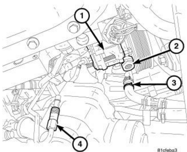
Fig. 25: P/S PUMP Courtesy of CHRYSLER LLC
