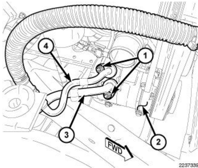
Fig. 9: Identifying Nuts, A/C Suction Line, A/C Discharge Line & A/C Compressor Courtesy of CHRYSLER LLC
