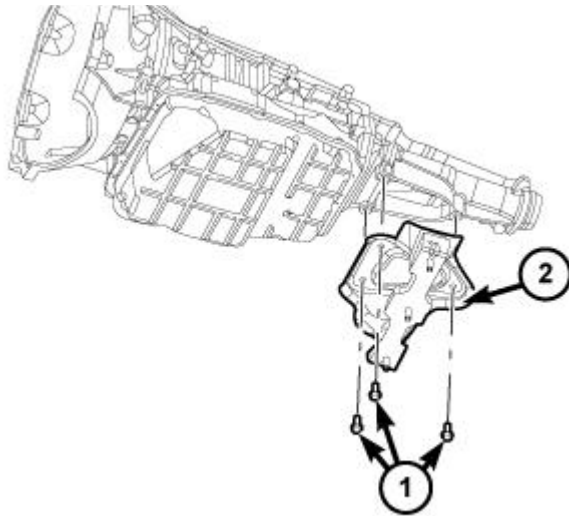
Fig. 221: Identifying Rear Transmission Mount & Bolts - 68RFE A/T - 4X2 Regular Cab Models Courtesy of CHRYSLER LLC
