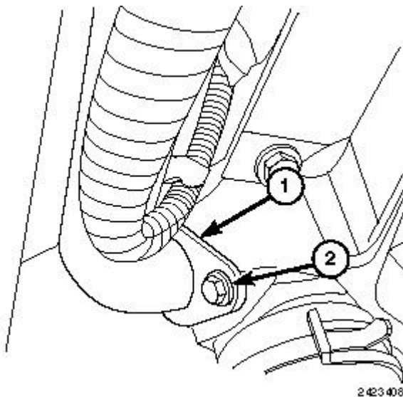
Fig. 250: Identifying Front Coolant Tube Bolt Courtesy of CHRYSLER LLC
