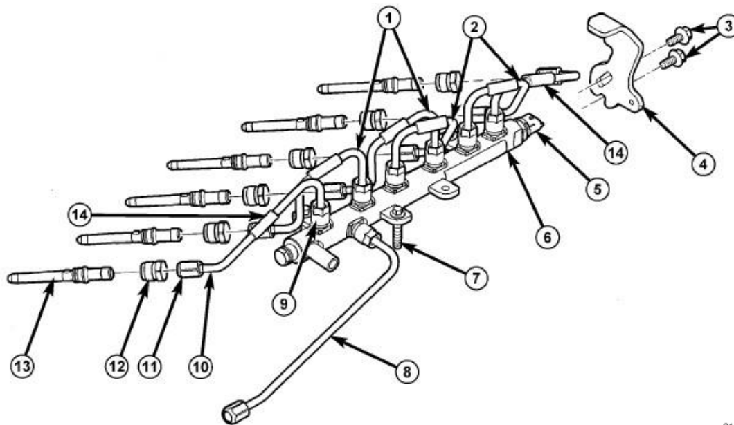
Fig. 68: FUEL LINES AT RAIL Courtesy of CHRYSLER LLC
