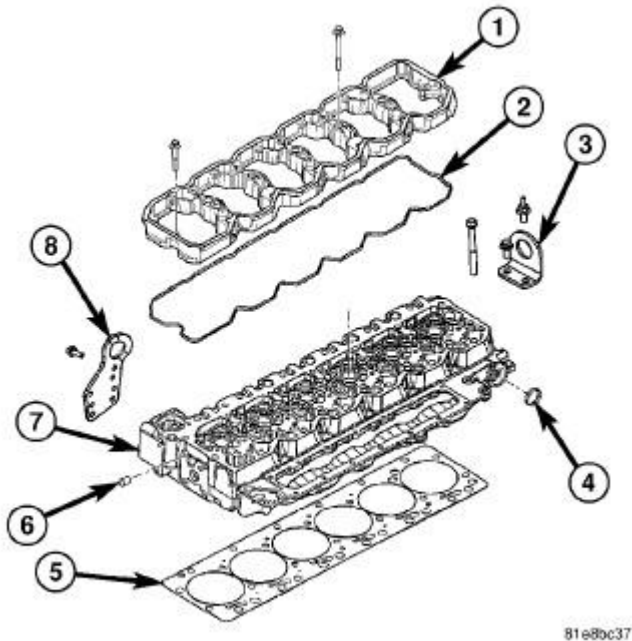
Fig. 63: CYLINDER HEAD AND GASKET Courtesy of CHRYSLER LLC
