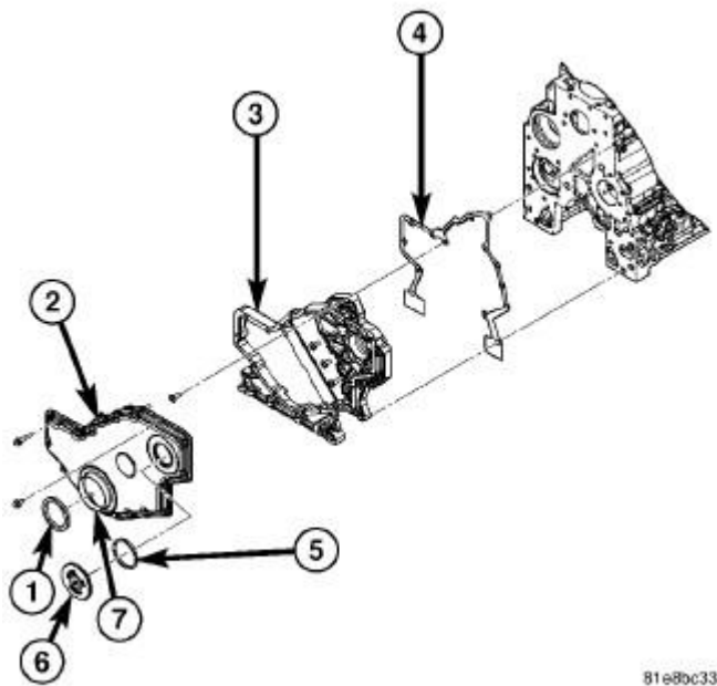
Fig. 358: Front Cover Assembly Components Courtesy of CHRYSLER LLC
