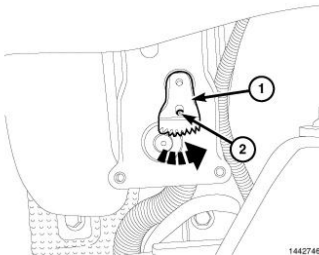
Fig. 321: Selector Gear -- Forward Position Courtesy of CHRYSLER LLC
