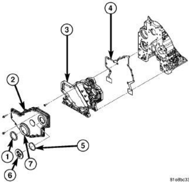
Fig. 348: Front Cover Assembly Components
