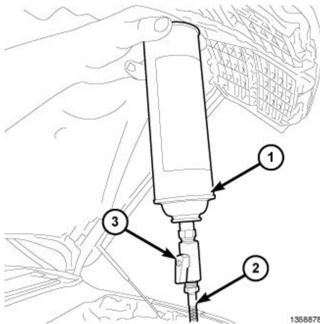
Fig. 316: Identifying Turbocharger Cleaner Can, Handle & Hose Courtesy of CHRYSLER LLC
