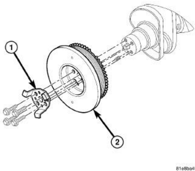
Fig. 188: CRANKSHAFT DAMPER Courtesy of CHRYSLER LLC
