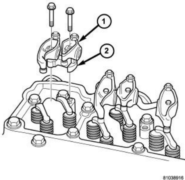
Fig. 98: Rocker Arm and Pedestal Removal/Installation
