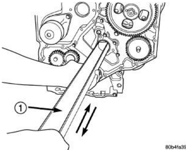
Fig. 203: Inserting the Trough Courtesy of CHRYSLER LLC
