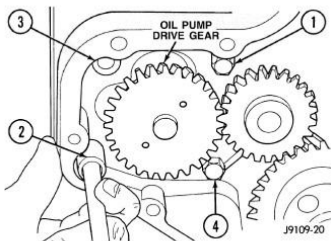
Fig. 294: Oil Pump Mounting Bolt Torque Sequence Courtesy of CHRYSLER LLC
