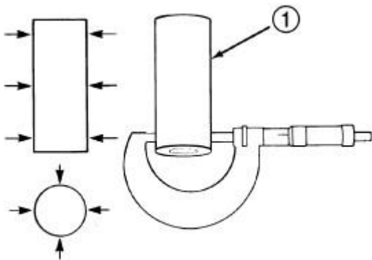
Fig. 179: Piston Pin Diameter
