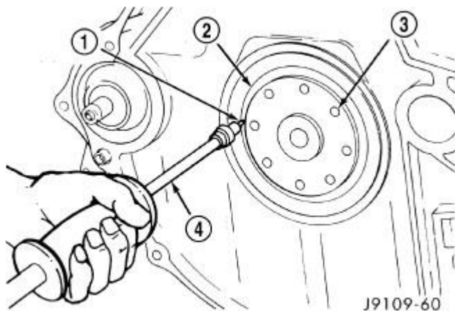
Fig. 196: Crankshaft Rear Seal Removal Courtesy of CHRYSLER LLC
