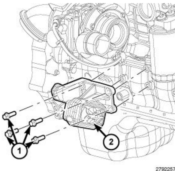
Fig. 210: RH Engine Mount Courtesy of CHRYSLER LLC
