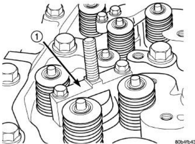
Fig. 124: Spring Compressor Mounting Base-Part of Tool 8319-A Courtesy of CHRYSLER LLC
