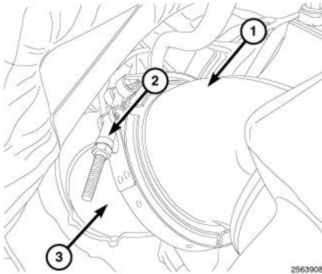
Fig. 10: Identifying V-Clamp & Elbow Courtesy of CHRYSLER LLC
