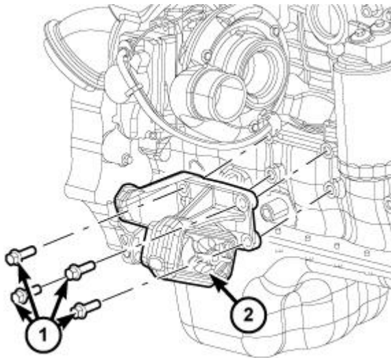
Fig. 213: RH Engine Mount Courtesy of CHRYSLER LLC
