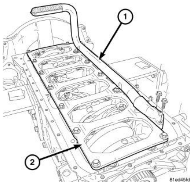
Fig. 173: OIL PICKUP TUBE Courtesy of CHRYSLER LLC
