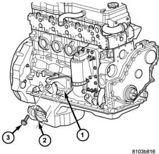
Fig. 269: RH Insulator Courtesy of CHRYSLER LLC
