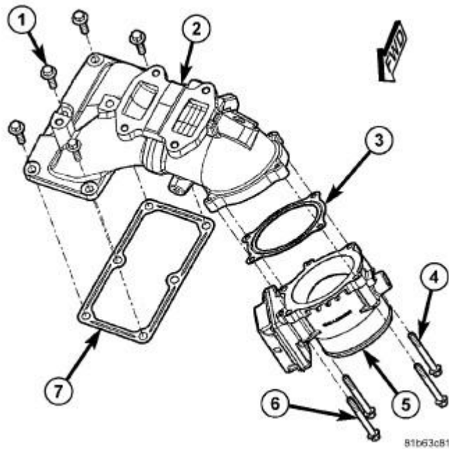
Fig. 302: EGR AIR FLOW CONTROL VALVE LOCATION
