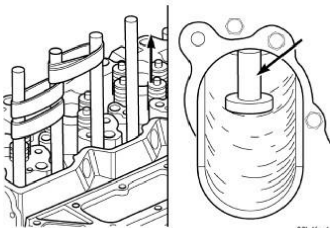
Fig. 200: Lift Dowel Rod to Disengage from Tappet Courtesy of CHRYSLER LLC
