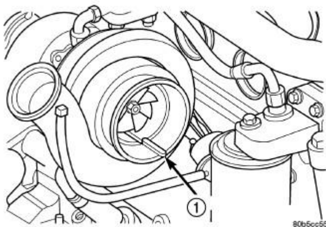
Fig. 341: Measure Turbocharger Bearing Radial Clearance Courtesy of CHRYSLER LLC
