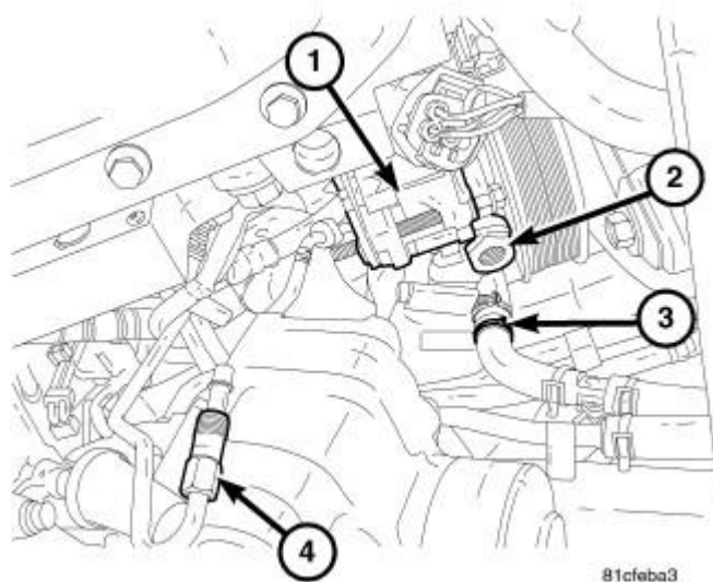
Fig. 189: P/S PUMP Courtesy of CHRYSLER LLC
