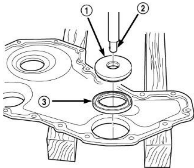
Fig. 365: Installing Seal Into Cover With Tool 8281 Courtesy of CHRYSLER LLC
