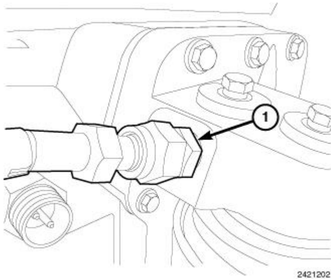
Fig. 246: Identifying Turbocharger Oil Supply Line At Oil Cooler Housing Courtesy of CHRYSLER LLC
