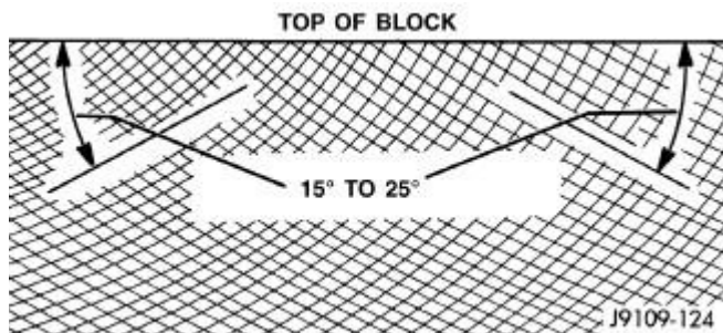
Fig. 130: Crosshatch Pattern of Repaired Sleeve(s) Courtesy of CHRYSLER LLC
