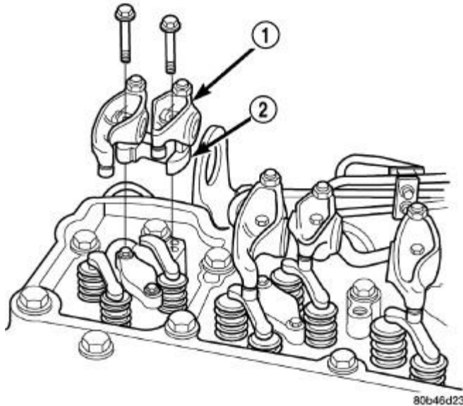
Fig. 14: Rocker Arms and Pedestal Removal Courtesy of CHRYSLER LLC
