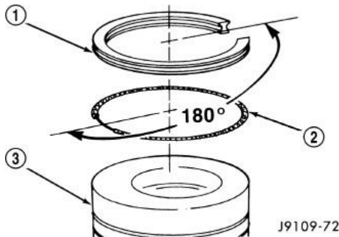
Fig. 167: Oil Control Ring/Expander Location in Groove Courtesy of CHRYSLER LLC
