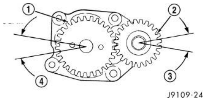
Fig. 293: Measure Gear Backlash Courtesy of CHRYSLER LLC
