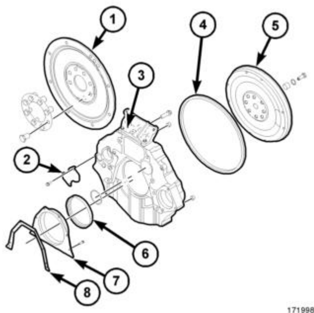
Fig. 16: FLYWHEEL AND ADAPTER PLATE Courtesy of CHRYSLER LLC
