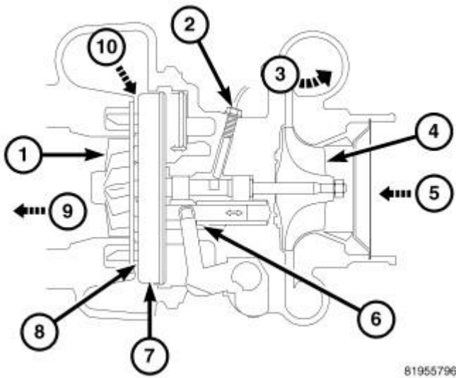
Fig. 330: 6.7L Turbocharger Courtesy of CHRYSLER LLC
