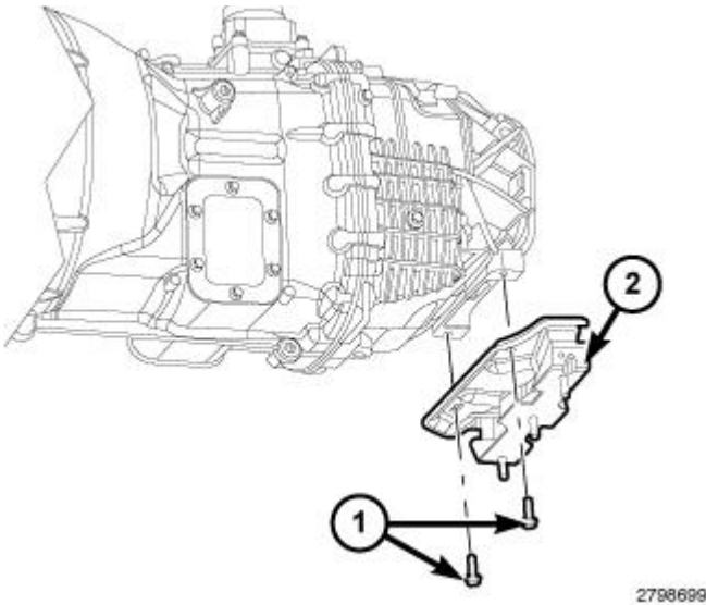
Fig. 228: Identifying Rear Transmission Mount & Bolts (M/T)
