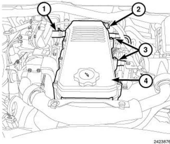
Fig. 95: Identifying CCV Tube, Crankcase Pressure Sensor Connector, CCV Oil Drains & Close Crankcase Ventilation (CCV) Cover Courtesy of CHRYSLER LLC
