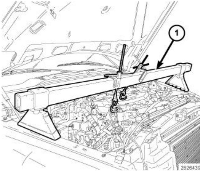
Fig. 336: Engine Support Fixture Tool 8534B Courtesy of CHRYSLER LLC
