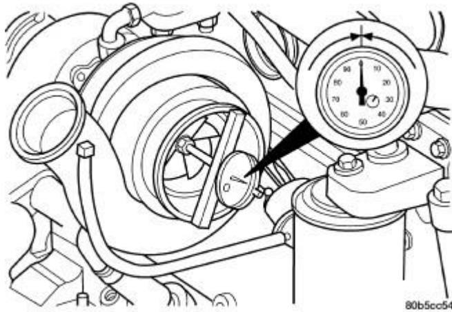
Fig. 340: Measure Turbocharger Axial End Play Courtesy of CHRYSLER LLC
