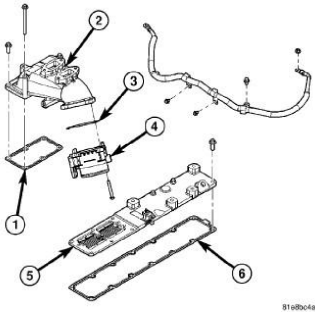
Fig. 67: Intake Air Heater Assembly Courtesy of CHRYSLER LLC
