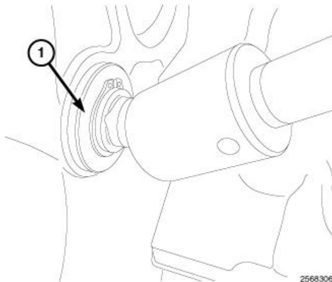
Fig. 7: Identifying Barring Tool 7471B
