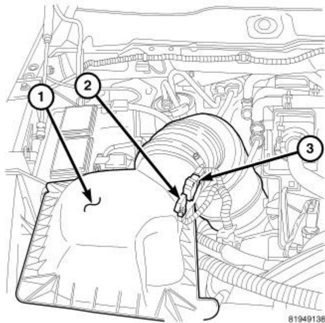
Fig. 265: Air Cleaner Housing
