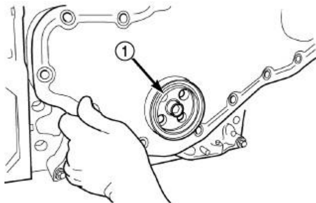
Fig. 366: Installing Front Cover with Seal Pilot Courtesy of CHRYSLER LLC
