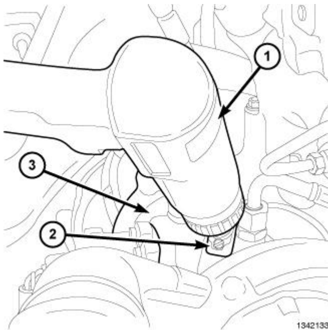
Fig. 311: Drilling Hole Through Turbocharger Center Housing Courtesy of CHRYSLER LLC
