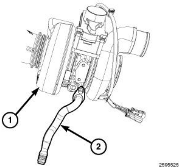
Fig. 327: Turbocharger & Drain Tube Courtesy of CHRYSLER LLC
