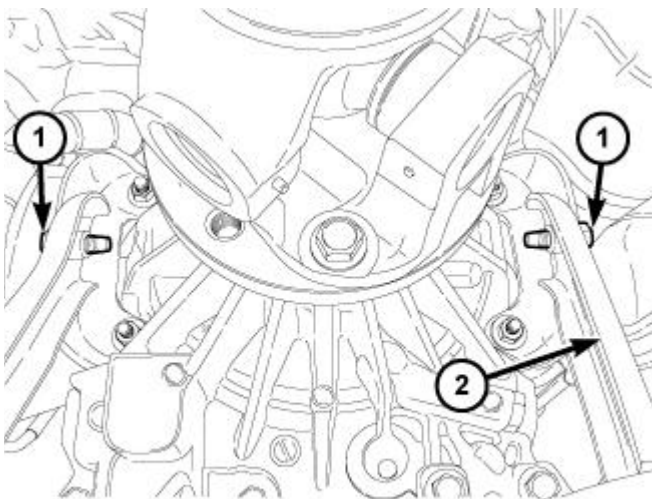
Fig. 223: Identifying Transmission Support Bracket & Bolts - AS68RC A/T Courtesy of CHRYSLER LLC
