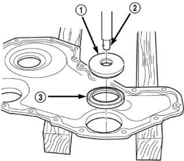
Fig. 191: Installing Seal Into Cover With Tool 8281 Courtesy of CHRYSLER LLC
