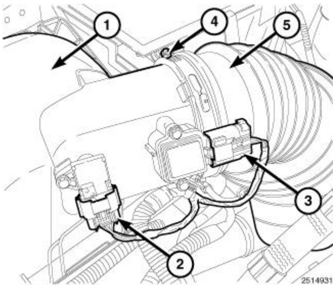
Fig. 60: Identifying MAF Sensor, TBAP Sensor, Intake Air Tube, Air Cleaner Body & Clamp Courtesy of CHRYSLER LLC
