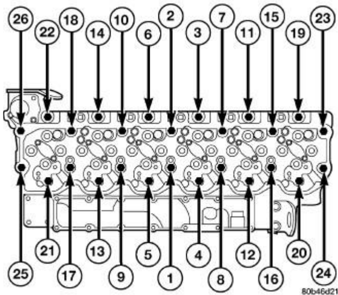
Fig. 77: Cylinder Head Bolt Torque Sequence
