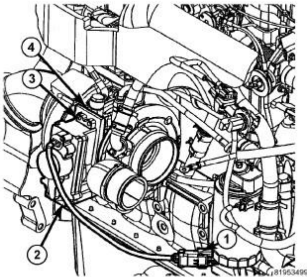
Fig. 319: 6.7L Turbocharger Actuator Courtesy of CHRYSLER LLC
