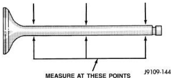
Fig. 112: Measure Valve Stem Diameter Courtesy of CHRYSLER LLC
