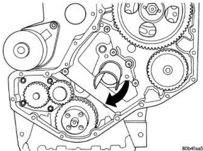
Fig. 208: Rotate Trough One Half Turn (180°) Courtesy of CHRYSLER LLC
