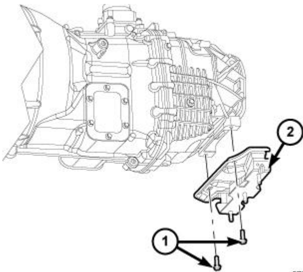
Fig. 219: Identifying Rear Transmission Mount & Bolts (M/T) Courtesy of CHRYSLER LLC
