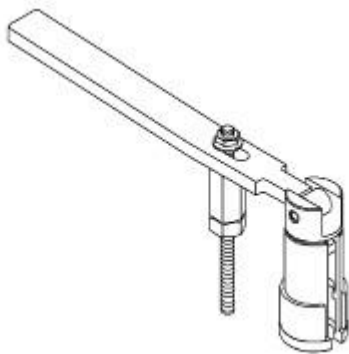
Fig. 39: REMOVER/INSTALLER, FUEL INJECTOR - 9010A Courtesy of CHRYSLER LLC
