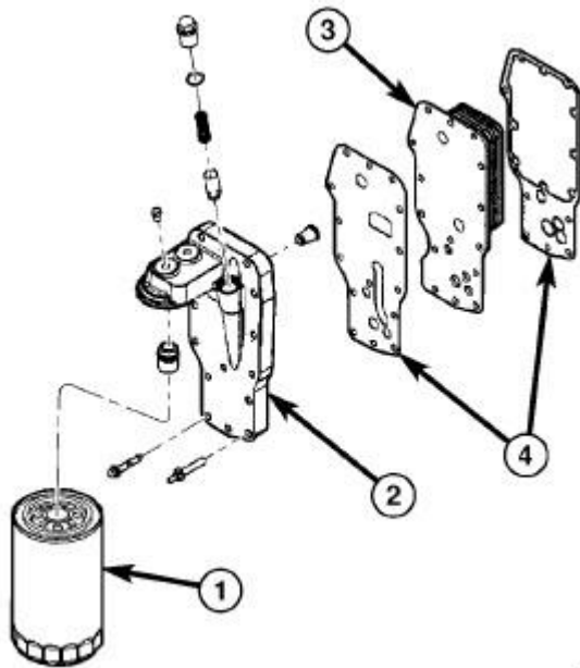
Fig. 247: Oil Filter And Cooler Courtesy of CHRYSLER LLC
