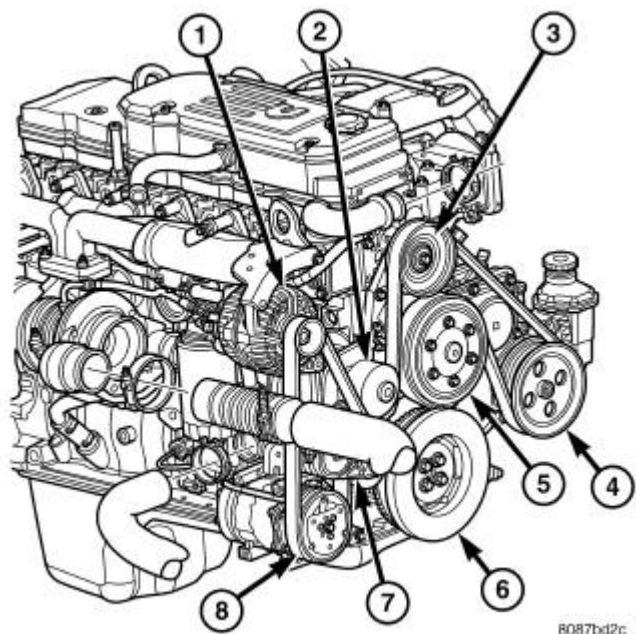
Fig. 370: Accessory Drive Belt Courtesy of CHRYSLER LLC
