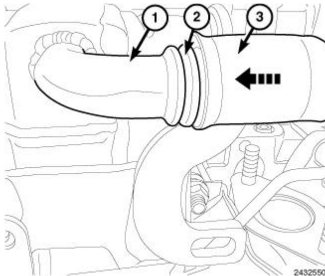
Fig. 251: Identifying EGR Cooler, O-ring & Forward Coolant Tube Courtesy of CHRYSLER LLC
