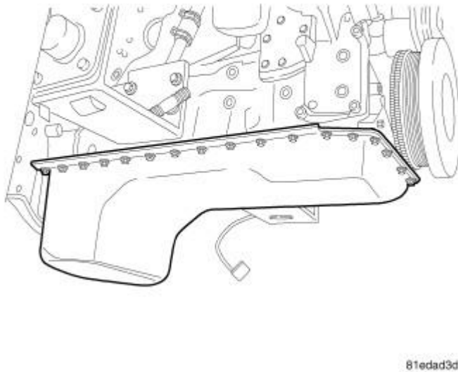
Fig. 28: Identifying Oil Pan Courtesy of CHRYSLER LLC
