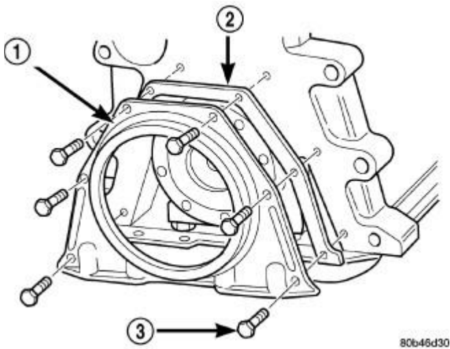
Fig. 163: Crankshaft Rear Seal Retainer and Gasket Courtesy of CHRYSLER LLC
