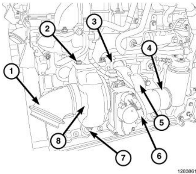
Fig. 345: Identifying Turbocharger Components Courtesy of CHRYSLER LLC
