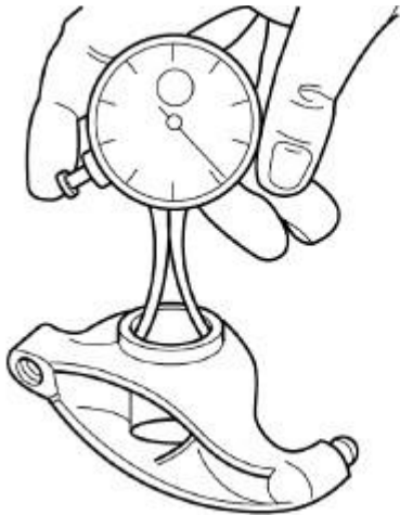
Fig. 100: Measuring Rocker Arm Bore Courtesy of CHRYSLER LLC
