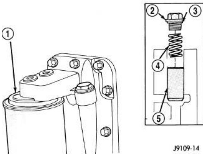
Fig. 296: Oil Pressure Regulator Courtesy of CHRYSLER LLC
