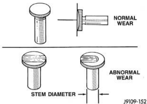
Fig. 202: Tappet Inspection Courtesy of CHRYSLER LLC
