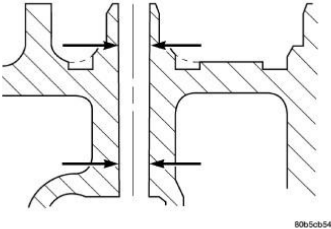
Fig. 113: Measure Valve Guide Bore Courtesy of CHRYSLER LLC
