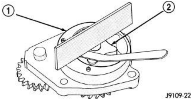
Fig. 291: Measuring Gerotor to Port Plate Clearance Courtesy of CHRYSLER LLC
