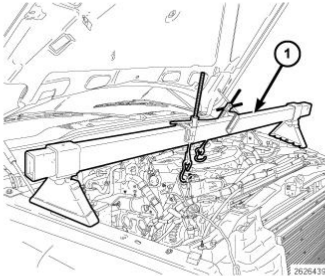
Fig. 344: Engine Support Fixture Tool 8534B Courtesy of CHRYSLER LLC
