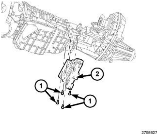
Fig. 229: Identifying Rear Transmission Mount & Bolts - 68RFE A/T - 4WD
