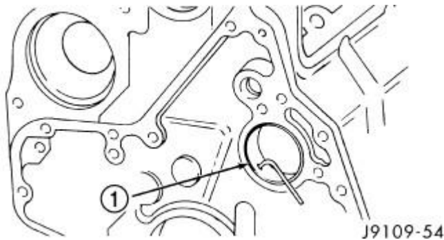
Fig. 146: Oil Hole Alignment Courtesy of CHRYSLER LLC
