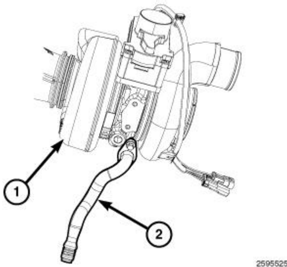
Fig. 338: Turbocharger & Drain Tube Courtesy of CHRYSLER LLC
