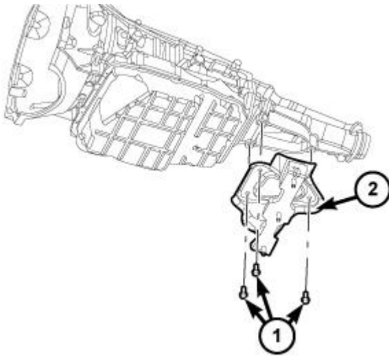
Fig. 230: Identifying Rear Transmission Mount & Bolts - 68RFE A/T - 4X2 Regular Cab Models Courtesy of CHRYSLER LLC
