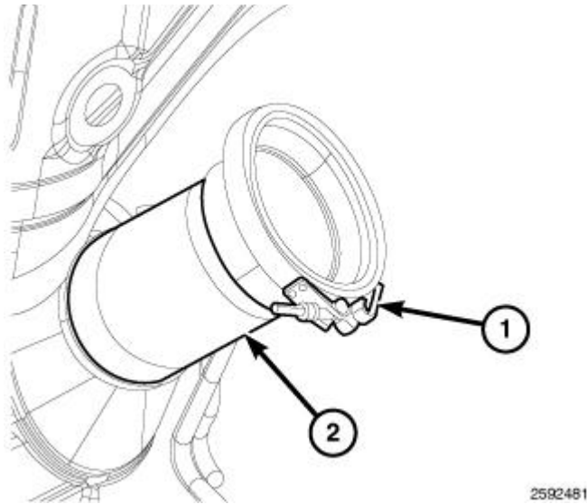
Fig. 337: Turbocharger Exhaust Outlet V-clamp Courtesy of CHRYSLER LLC
