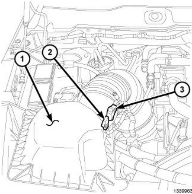
Fig. 307: Identifying Air Filter Housing Cover & Mass Air Flow (MAF) Sensor Courtesy of CHRYSLER LLC
