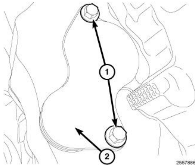
Fig. 6: Identifying Bolts & Bell Housing Access Cover
