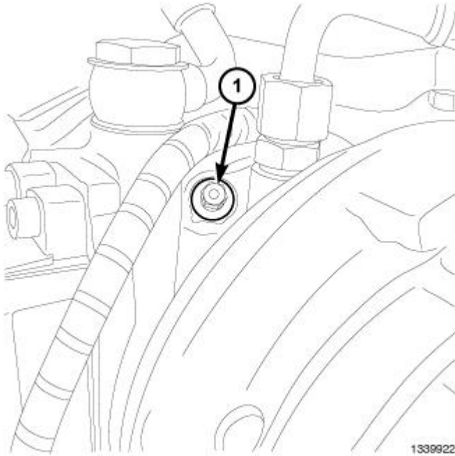
Fig. 318: Identifying Turbocharger Cleaning Port Courtesy of CHRYSLER LLC
