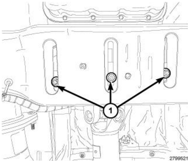
Fig. 215: Identifying Rear Transmission Mount To Crossmember Nuts - AS68RC A/T Courtesy of CHRYSLER LLC
