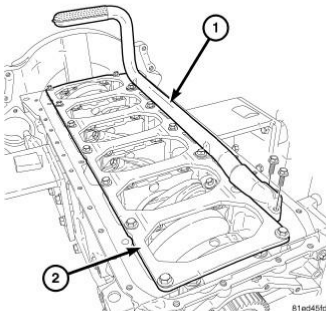
Fig. 185: OIL PICKUP TUBE
