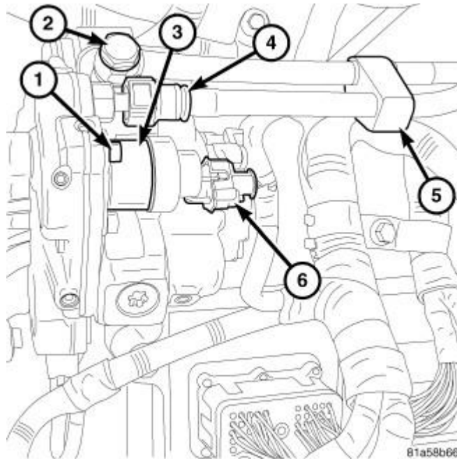
Fig. 357: FUEL INJECTION PUMP - REAR VIEW Courtesy of CHRYSLER LLC
