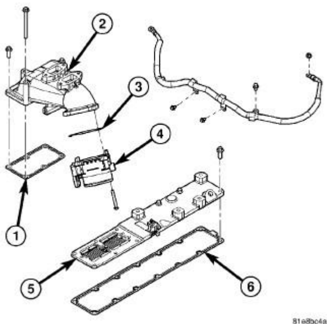
Fig. 303: Intake Air Heater Assembly
