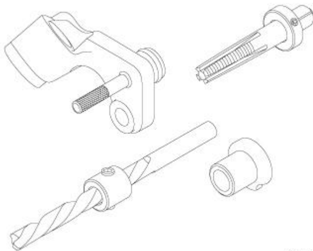
Fig. 49: CUMMINS TURBO DRILLING KIT - 10143 Courtesy of CHRYSLER LLC
