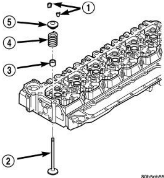
Fig. 110: Valve Spring, Seal, and Retainers Courtesy of CHRYSLER LLC
