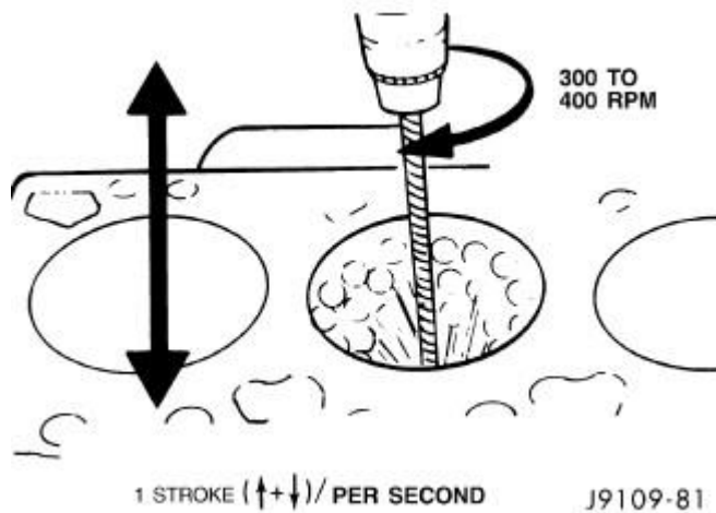
Fig. 129: De-Glazing Cylinder Bore
