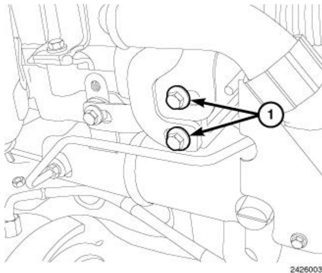
Fig. 243: Identifying Bracket Bolts Courtesy of CHRYSLER LLC
