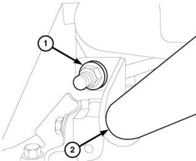
Fig. 241: Identifying Coolant Outlet Tube Bracket Nut Courtesy of CHRYSLER LLC
