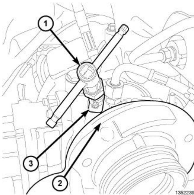
Fig. 312: Installing Tap Into Drill/Tap Guide Bushing Bore Courtesy of CHRYSLER LLC
