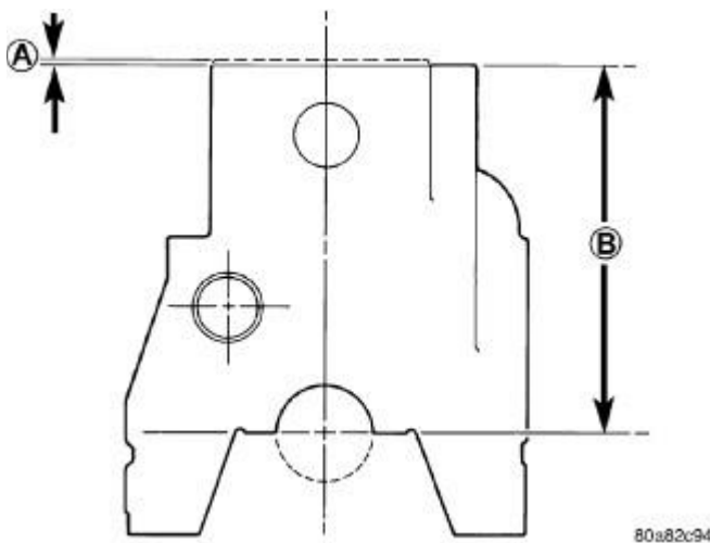
Fig. 127: Refacing Dimensions of the Cylinder Block
