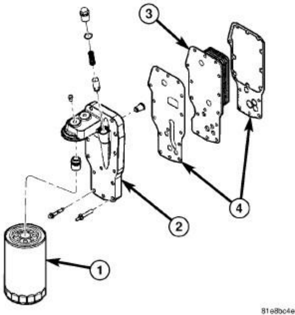
Fig. 263: Oil Filter And Cooler Courtesy of CHRYSLER LLC
