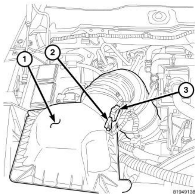
Fig. 270: Air Cleaner Housing Courtesy of CHRYSLER LLC
