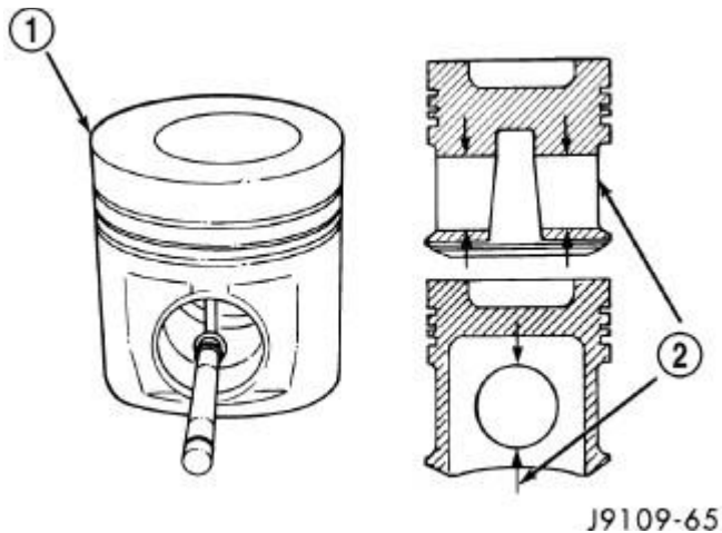
Fig. 178: Piston Pin Bore
