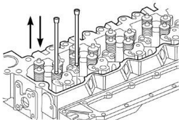
Fig. 99: Push Rod Removal/Installation
