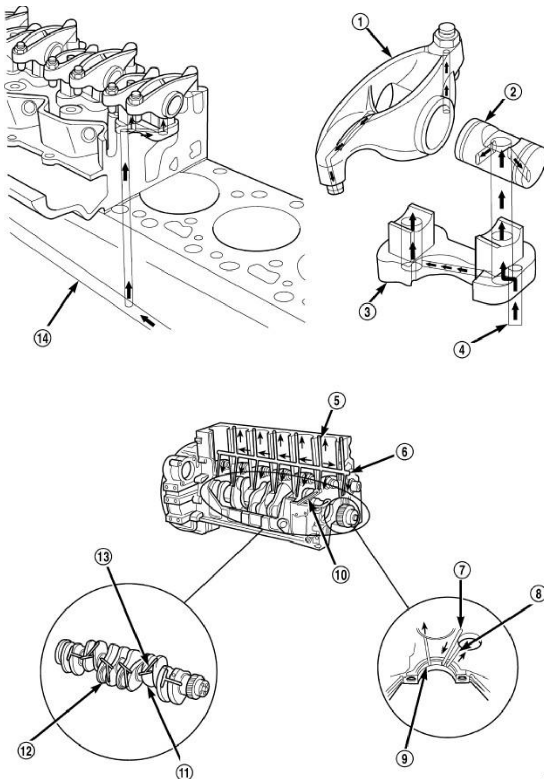
Fig. 233: Lubrication System Circulation (2 Of 2) Courtesy of CHRYSLER LLC
