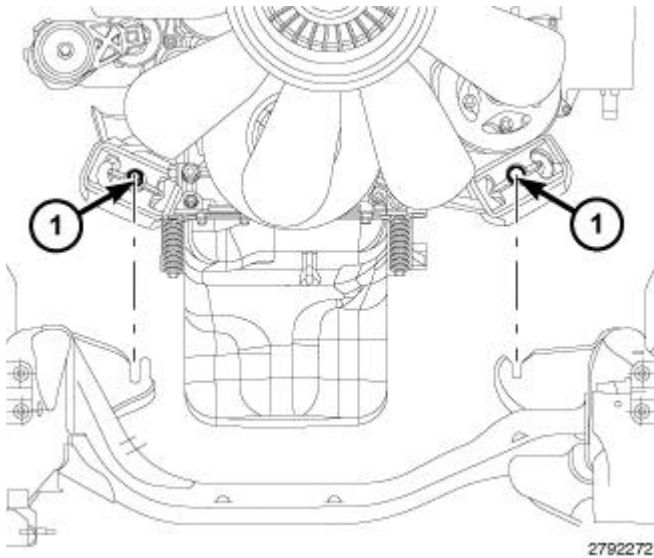
Fig. 209: Identifying Frame Mount Thru-Bolts & Nuts Courtesy of CHRYSLER LLC
