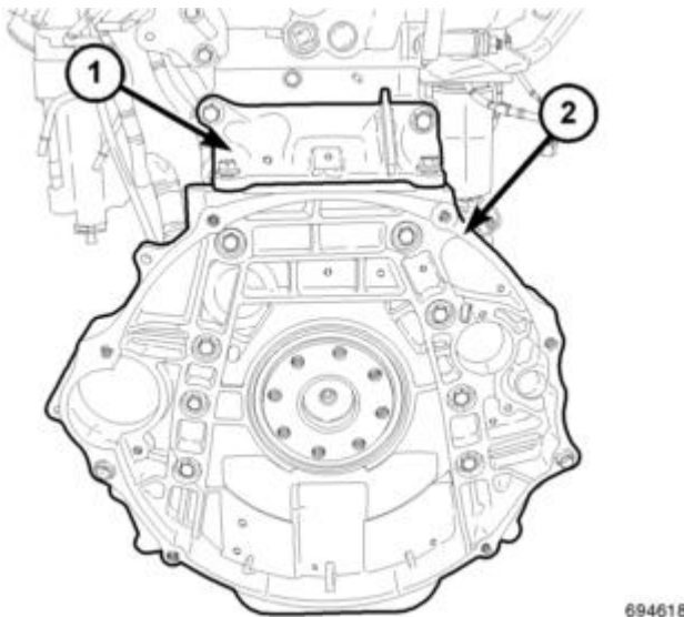
Fig. 11: FLYWHEEL HOUSING AND COLLAR Courtesy of CHRYSLER LLC
