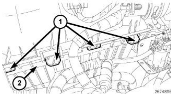
Fig. 55: Identifying Air Cleaner Cover Alignment Tabs & Housing Slots Courtesy of CHRYSLER LLC
