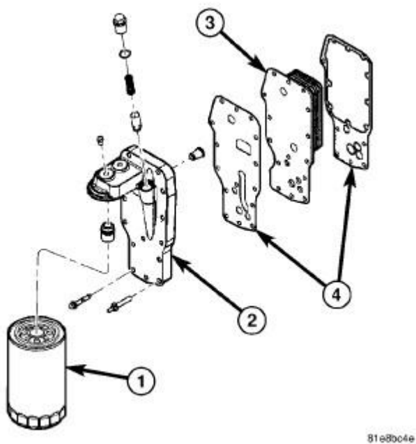
Fig. 262: Oil Filter And Cooler Courtesy of CHRYSLER LLC
