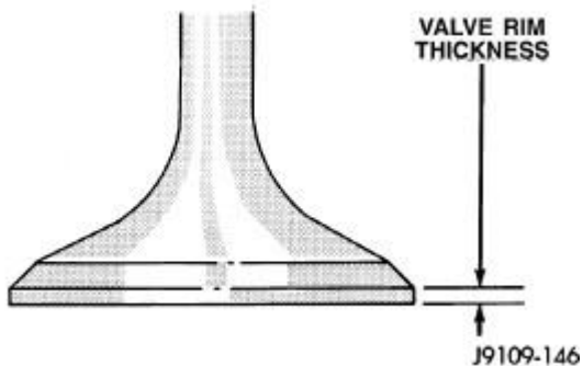
Fig. 114: Measure Valve Margin (Rim Thickness) Courtesy of CHRYSLER LLC
