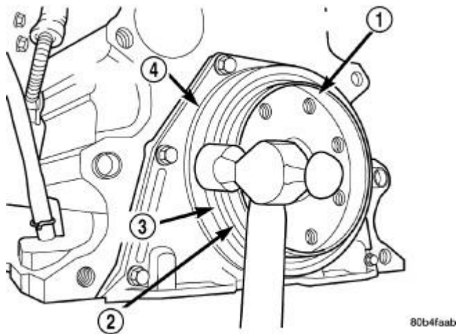
Fig. 164: Installing Seal Using Alignment Tool and Hammer Courtesy of CHRYSLER LLC
