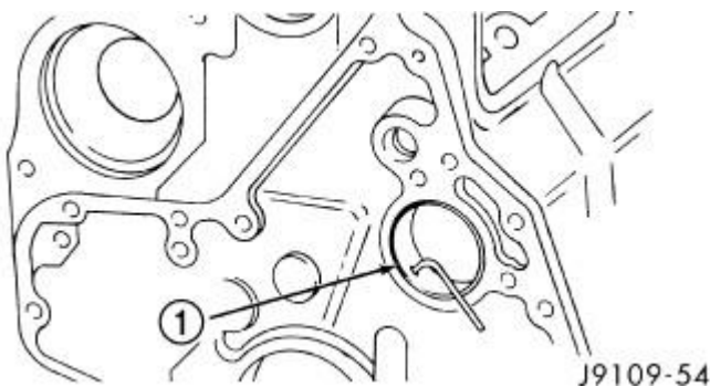
Fig. 148: Oil Hole Alignment Courtesy of CHRYSLER LLC
