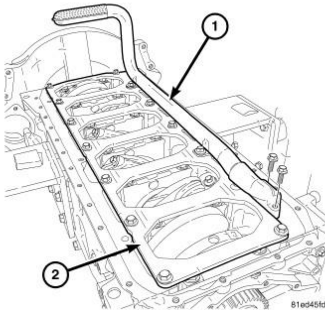
Fig. 278: OIL PICKUP TUBE Courtesy of CHRYSLER LLC
