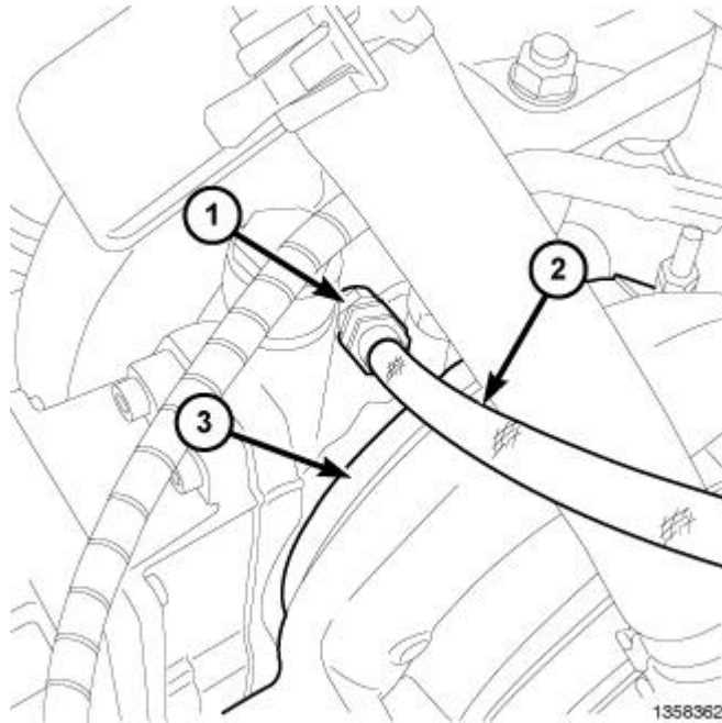
Fig. 317: Identifying Nozzle, Cleaning Tool Hose & Turbocharger Courtesy of CHRYSLER LLC
