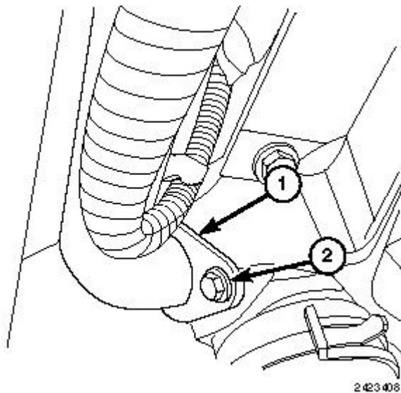
Fig. 245: Identifying Front Coolant Tube Bolt Courtesy of CHRYSLER LLC
