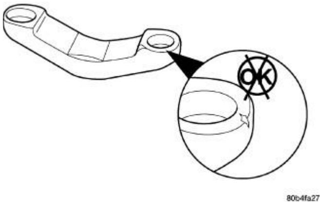
Fig. 74: Inspecting Crosshead for Cracks Courtesy of CHRYSLER LLC
