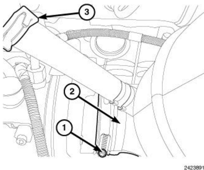
Fig. 258: Identifying Clamp, Outlet Tube & Breather Hose Courtesy of CHRYSLER LLC
