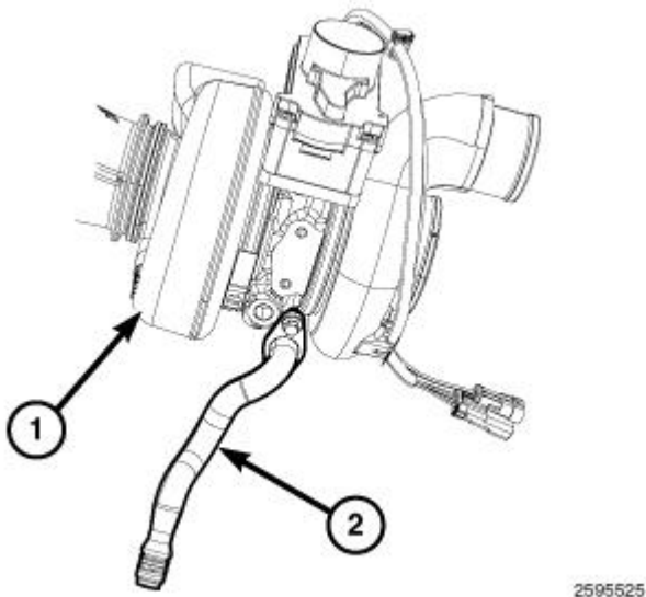
Fig. 342: Turbocharger & Drain Tube Courtesy of CHRYSLER LLC
