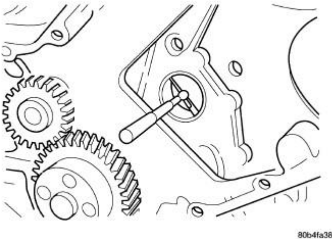
Fig. 145: Measuring Camshaft Bore Courtesy of CHRYSLER LLC
