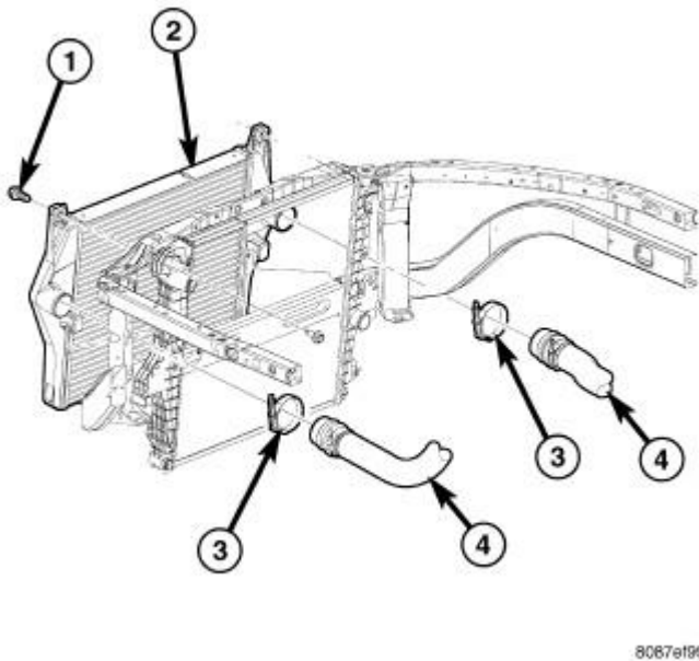
Fig. 324: Air Intake System Tubes Courtesy of CHRYSLER LLC
