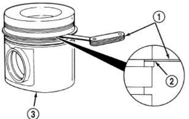
Fig. 177: Intermediate and Oil Ring Clearances Courtesy of CHRYSLER LLC
