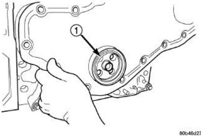
Fig. 192: Installing Front Cover with Seal Pilot Courtesy of CHRYSLER LLC
