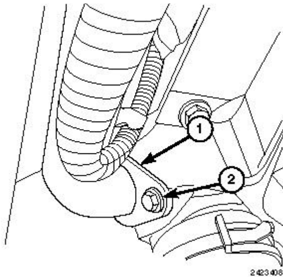
Fig. 253: Identifying Front Coolant Tube Bolt Courtesy of CHRYSLER LLC
