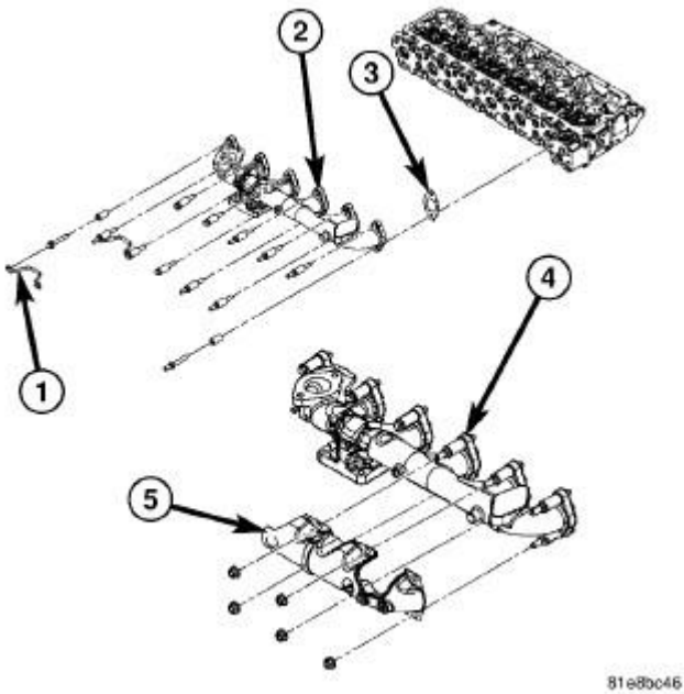
Fig. 65: Cylinder Head And Exhaust Manifold Courtesy of CHRYSLER LLC
