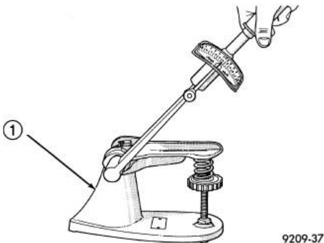
Fig. 116: Testing Valve Spring with Tool C-647 Courtesy of CHRYSLER LLC
