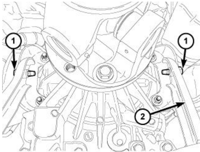
Fig. 218: Identifying Transmission Support Bracket & Bolts - AS68RC A/T Courtesy of CHRYSLER LLC
