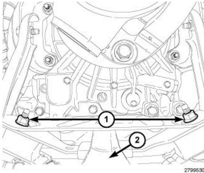
Fig. 226: Identifying Rear Transmission Mount & Nuts - AS68RC A/T Courtesy of CHRYSLER LLC
