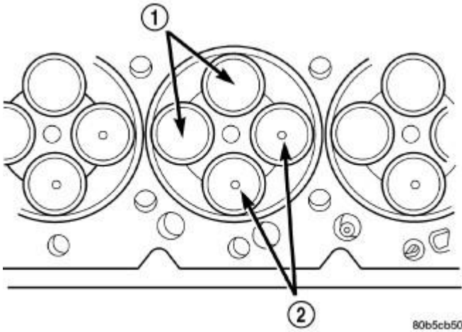
Fig. 117: Valve Identification Courtesy of CHRYSLER LLC
