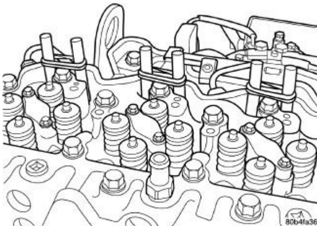
Fig. 141: Use Wooden Dowel Rods to Secure Tappets in Place
