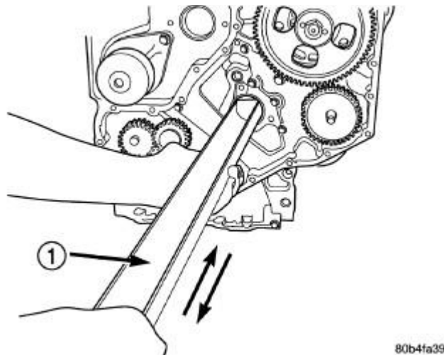
Fig. 201: Inserting the Trough Courtesy of CHRYSLER LLC
