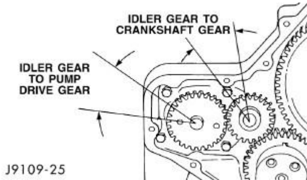
Fig. 295: Idler Gear to Pump Drive Gear and Crankshaft Gear Backlash Courtesy of CHRYSLER LLC
