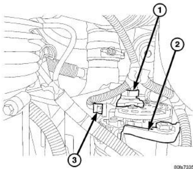
Fig. 259: DIESEL GENERATOR CONNECTORS
