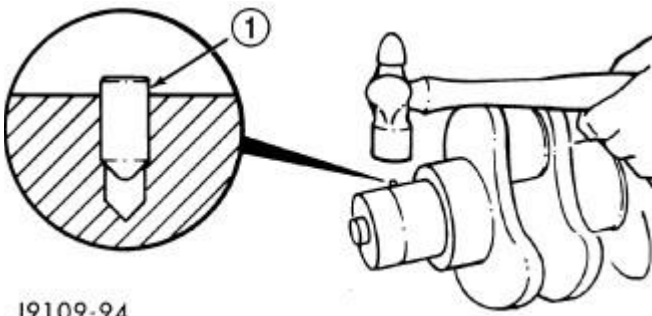
Fig. 159: Installing Alignment Pin
