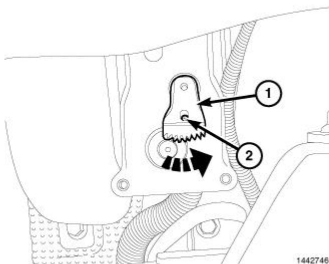
Fig. 333: Selector Gear -- Forward Position
