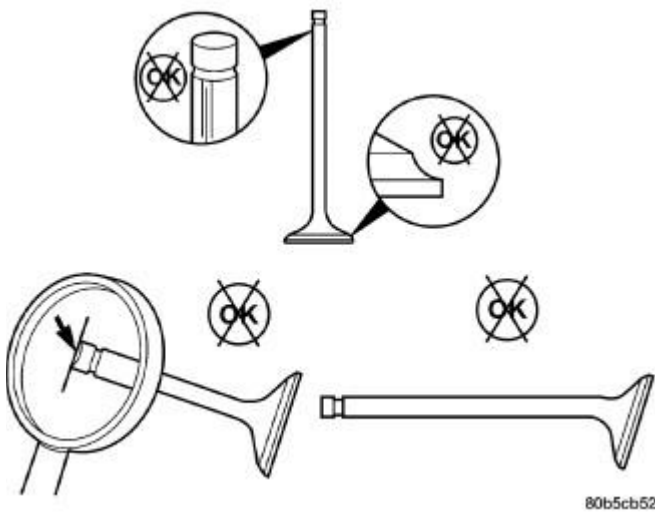
Fig. 111: Visually Inspect Valves for Abnormal Wear Courtesy of CHRYSLER LLC
