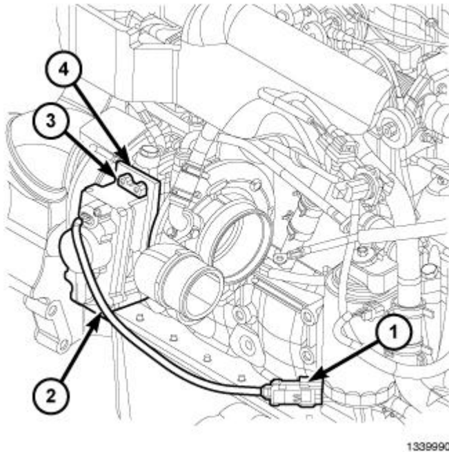
Fig. 308: Turbocharger Actuator Electrical Connector Courtesy of CHRYSLER LLC
