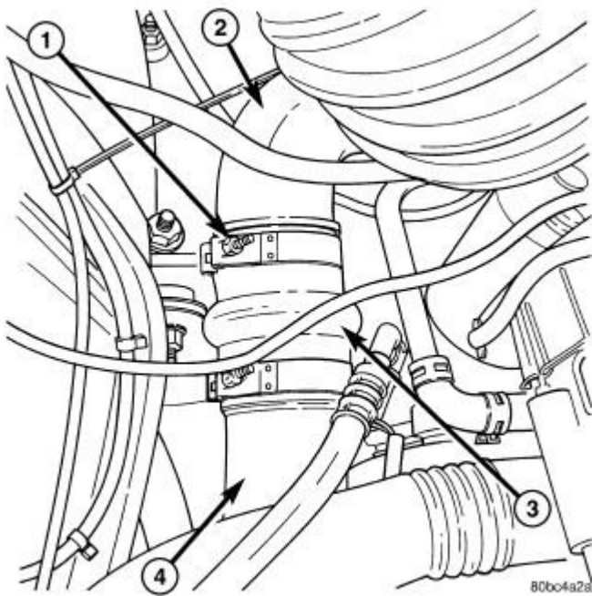
Fig. 323: Air Inlet Duct Rubber Sleeve Courtesy of CHRYSLER LLC
