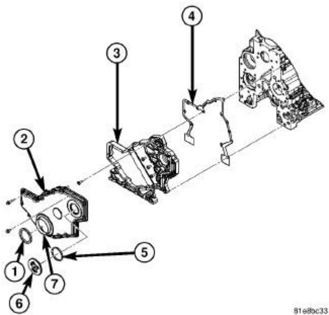
Fig. 153: Front Cover Assembly Components Courtesy of CHRYSLER LLC
