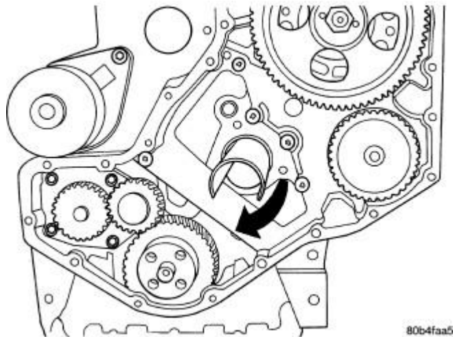
Fig. 207: Rotate Trough One Half Turn (180°) Courtesy of CHRYSLER LLC
