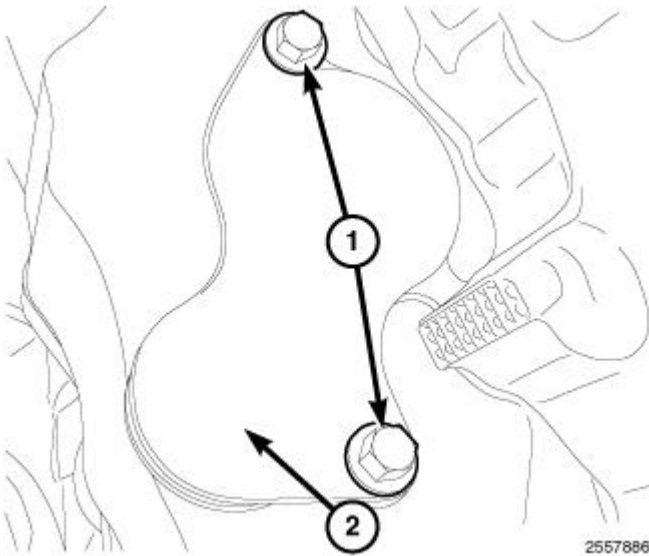
Fig. 122: Identifying Bolts & Bell Housing Access Cover Courtesy of CHRYSLER LLC
