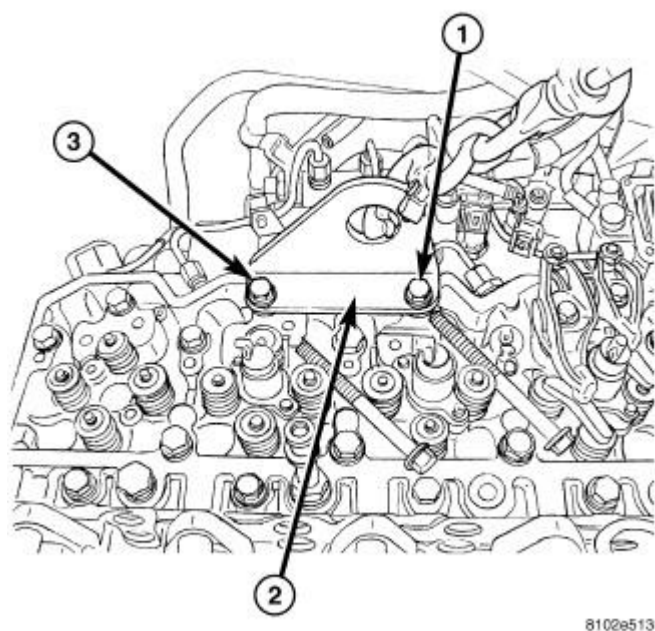
Fig. 17: ENGINE LIFT BRACKET
