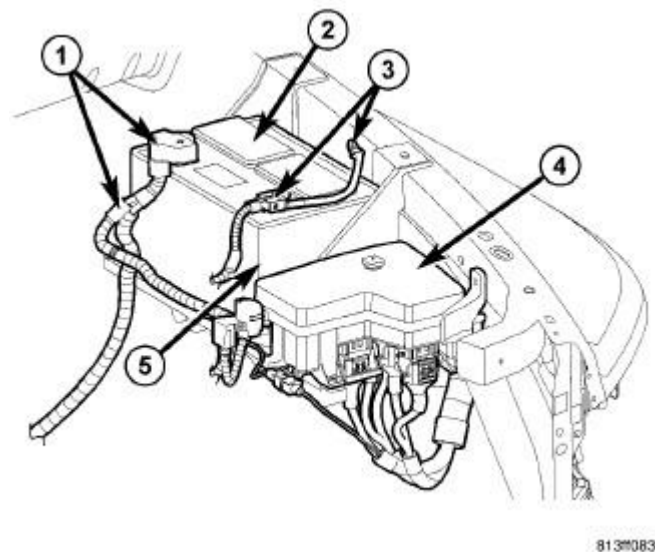
Fig. 271: Battery Cables Courtesy of CHRYSLER LLC
