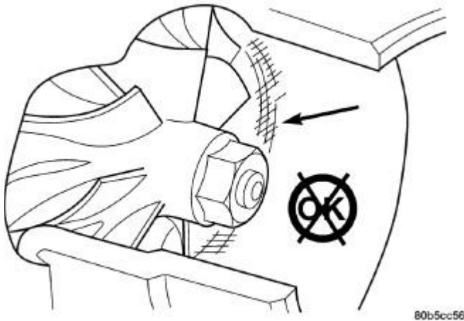
Fig. 339: Inspect Compressor Housing for Impeller Rubbing Condition Courtesy of CHRYSLER LLC
