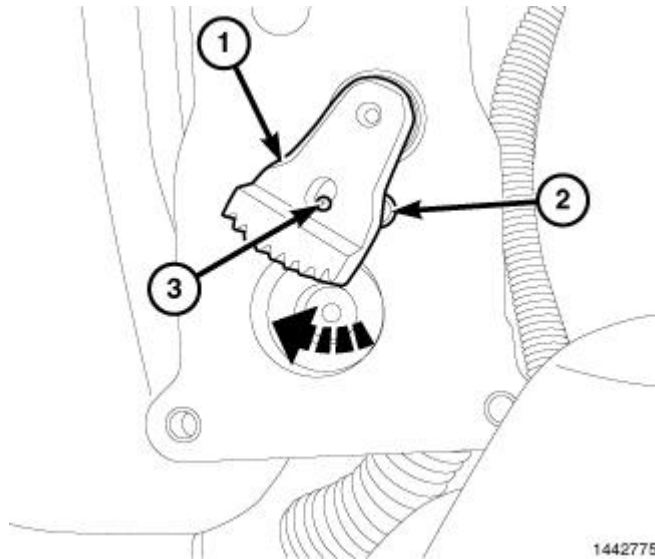
Fig. 322: Selector Gear -- Rearward Position Courtesy of CHRYSLER LLC
