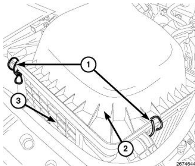
Fig. 56: Identifying Air Cleaner Housing & Clips Courtesy of CHRYSLER LLC
