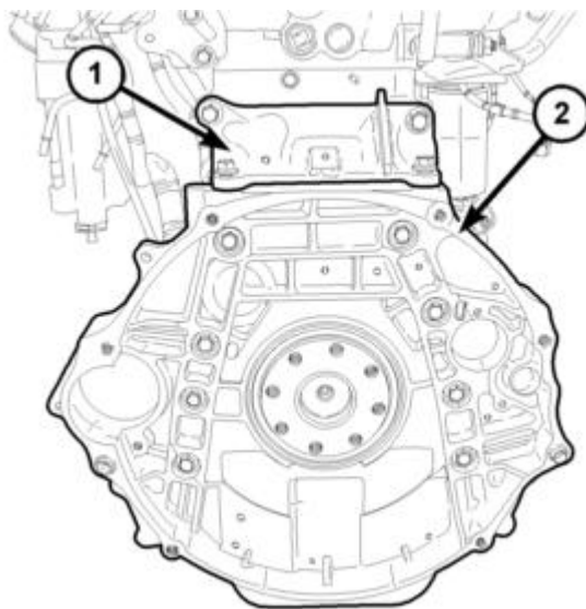
Fig. 22: FLYWHEEL HOUSING AND COLLAR
