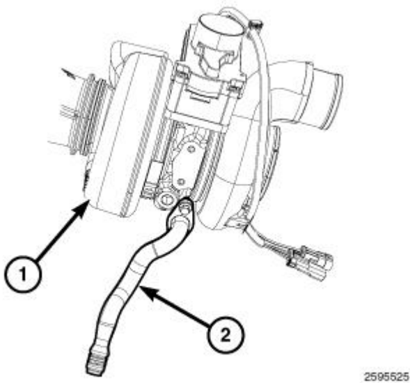
Fig. 326: Turbocharger & Drain Tube Courtesy of CHRYSLER LLC
