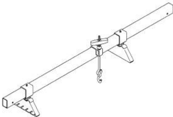
Fig. 35: SUPPORT FIXTURE, ENGINE - 8534B
