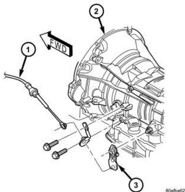
Fig. 286: Gearshift Cable at Transmission - RFE Courtesy of CHRYSLER LLC
