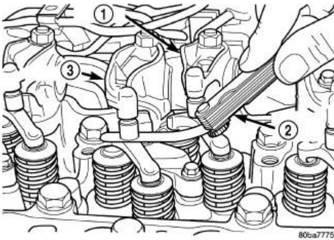
Fig. 121: Measuring Valve Lash Courtesy of CHRYSLER LLC
