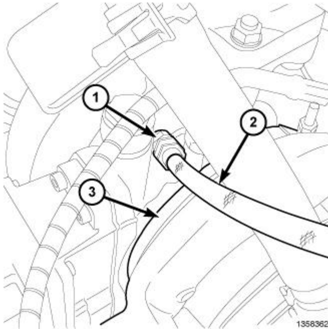
Fig. 314: Identifying Nozzle, Cleaning Tool Hose & Turbocharger Courtesy of CHRYSLER LLC
