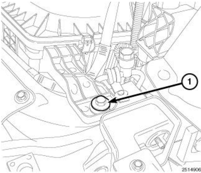
Fig. 57: Identifying Intake Air Housing Bolt Courtesy of CHRYSLER LLC
