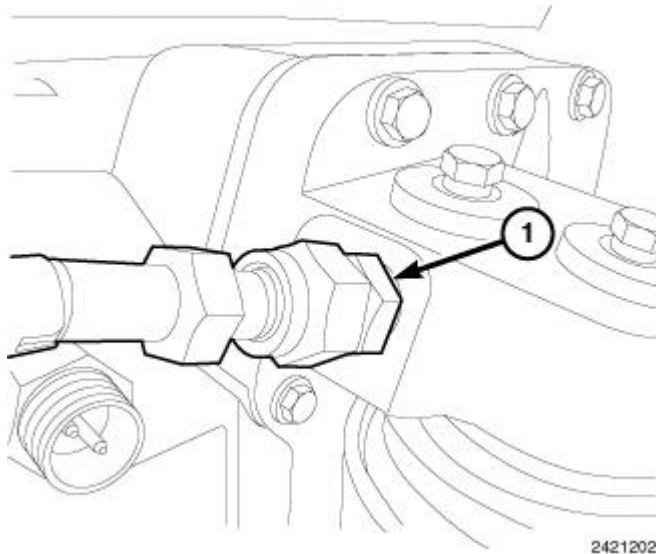
Fig. 249: Identifying Turbocharger Oil Supply Line At Oil Cooler Housing Courtesy of CHRYSLER LLC
