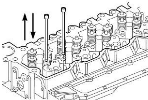
Fig. 70: Push Rod Removal/Installation Courtesy of CHRYSLER LLC
