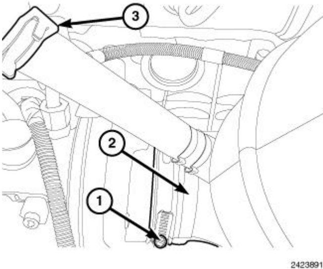
Fig. 62: Identifying Clamp, Outlet Tube & Breather Hose Courtesy of CHRYSLER LLC
