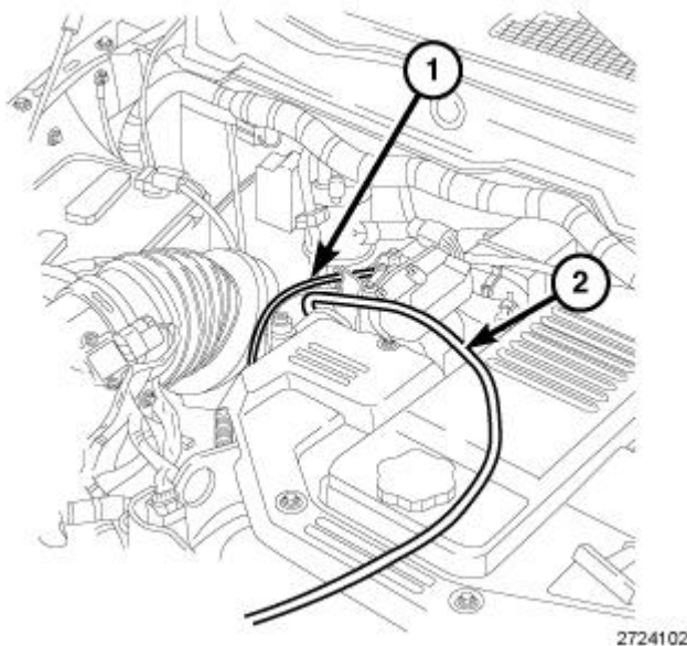
Fig. 315: Cleaning Tool Hose Courtesy of CHRYSLER LLC
