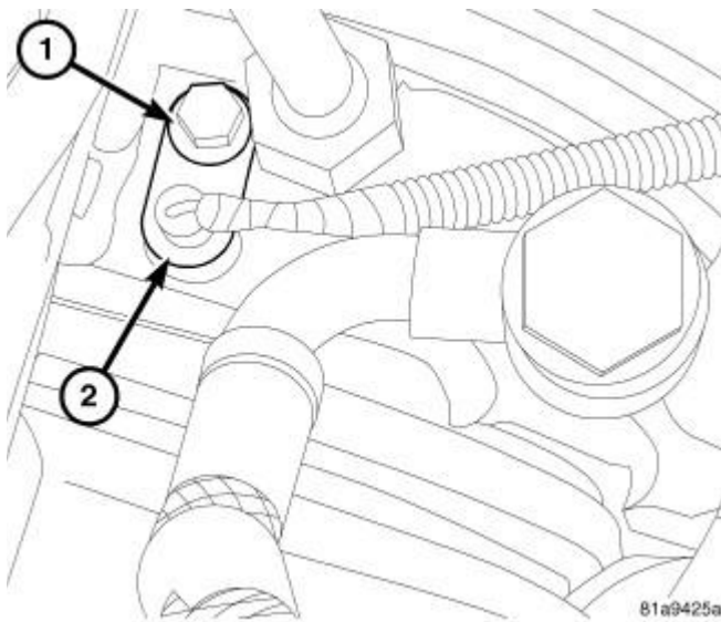
Fig. 328: Turbocharger Speed Sensor And Mounting Bolt Courtesy of CHRYSLER LLC
