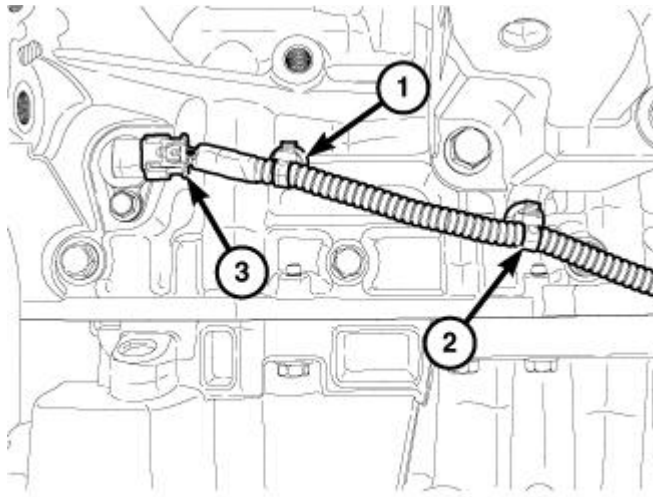
Fig. 501: Main Wire Harness Retainers & CKP Sensor Courtesy of CHRYSLER GROUP, LLC
