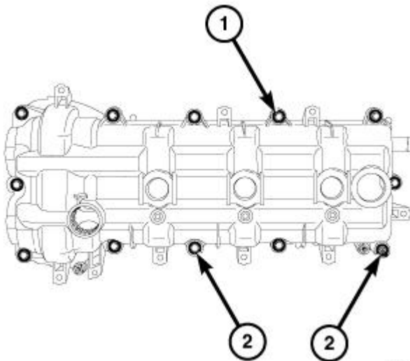
Fig. 280: Cylinder Head Cover Mounting Bolts & Studbolts Courtesy of CHRYSLER GROUP, LLC
