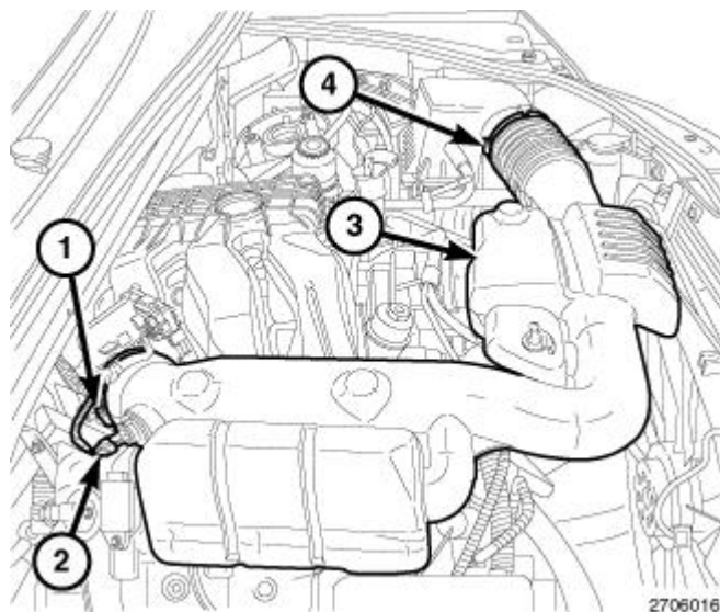
Fig. 186: Air Inlet Hose, Air Temperature (IAT) Sensor Connector & Clamps
