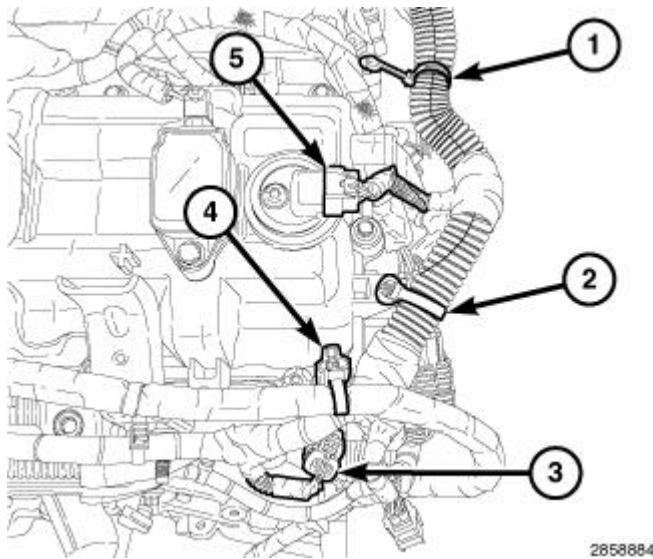
Fig. 479: ECT Sensor Connector, CMP Sensor & Main Wire Harness Retainers Courtesy of CHRYSLER GROUP, LLC
