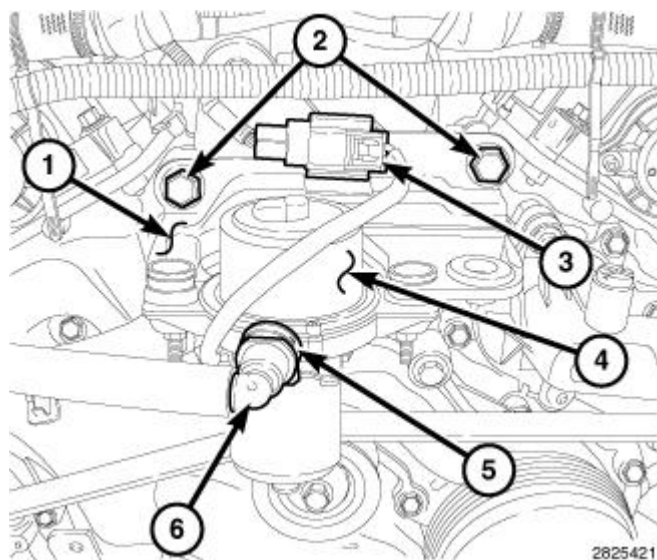
Fig. 185: Mounting Bracket, Bolts, Electrical Connector, Vacuum Pump, Locking Tab & Quick-Connect Type End
