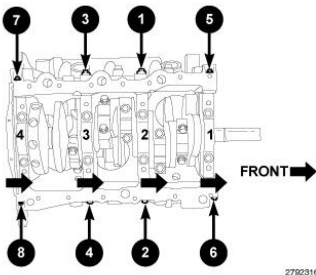
Fig. 433: Main Bearing Tie Bolts Installation Sequence
