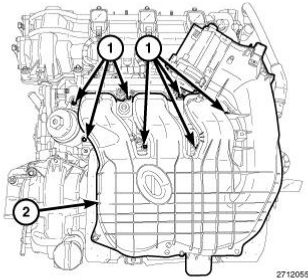
Fig. 330: Upper Intake Manifold & Bolts Courtesy of CHRYSLER GROUP, LLC
