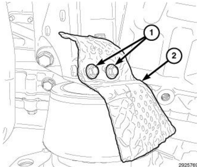
Fig. 496: Engine Mount Heatshield & Bolts Courtesy of CHRYSLER GROUP, LLC
