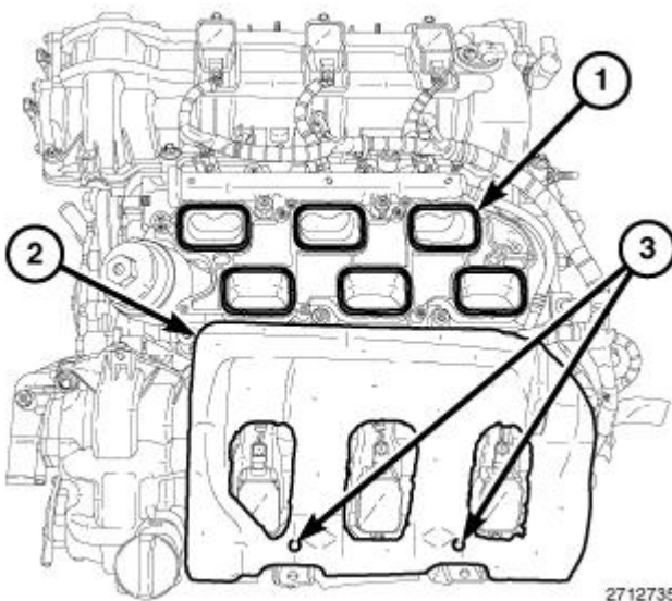
Fig. 646: Intake Ports, Insulator & Alignment Posts Courtesy of CHRYSLER GROUP, LLC
