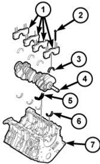
Fig. 429: Main Bearing Caps, Bolts, Crankshaft & Engine Block Courtesy of CHRYSLER GROUP, LLC
