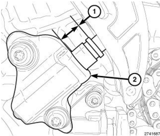
Fig. 696: Piston Extension & RH Cam Chain Tensioner Courtesy of CHRYSLER GROUP, LLC
