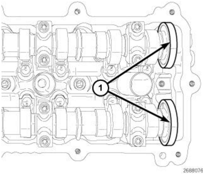
Fig. 269: Magnetic Timing Wheels
