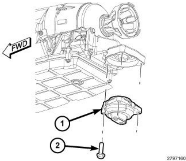
Fig. 518: Rear Engine Mount Isolator & Bolts (4x2)
