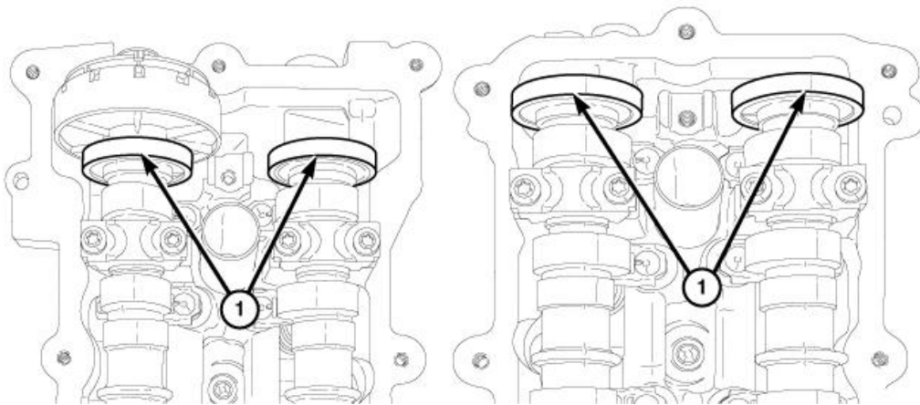
Fig. 116: Magnetic Timing Wheels
