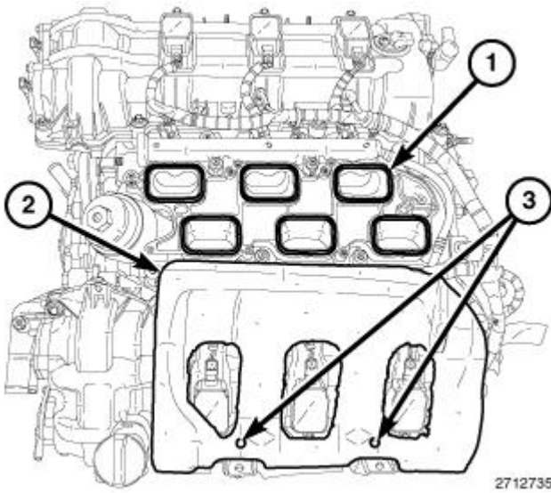
Fig. 271: Intake Ports, Insulator & Alignment Posts Courtesy of CHRYSLER GROUP, LLC
