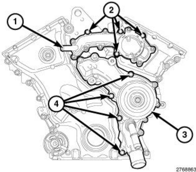
Fig. 727: Coolant Outlet Housing, Water Pump & Bolts Courtesy of CHRYSLER GROUP, LLC
