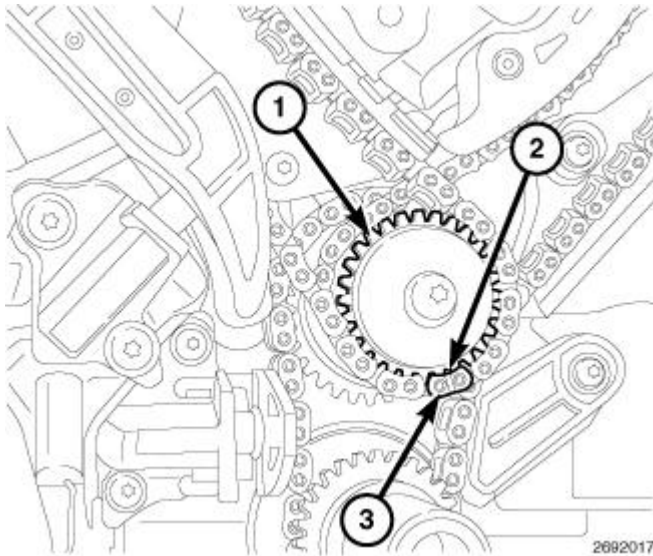
Fig. 710: Idler Sprocket, Dimple & Plated Link Courtesy of CHRYSLER GROUP, LLC
