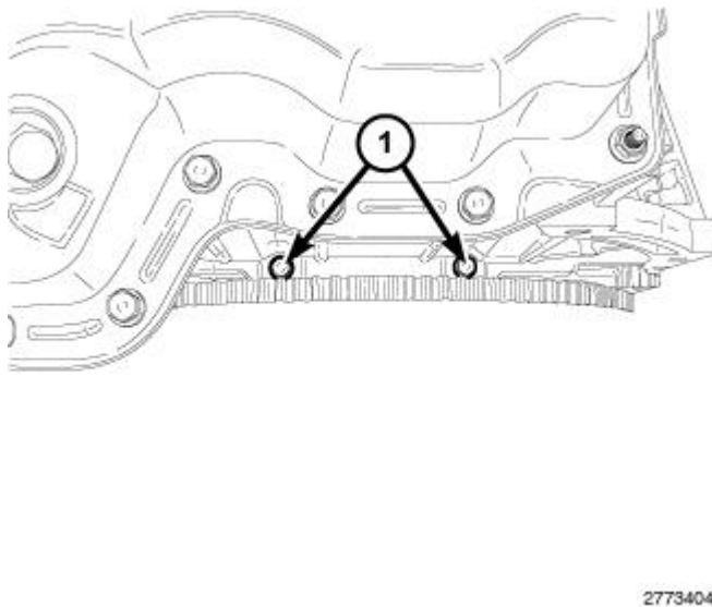
Fig. 573: Rear Oil Seal Retainer Flange Bolts
