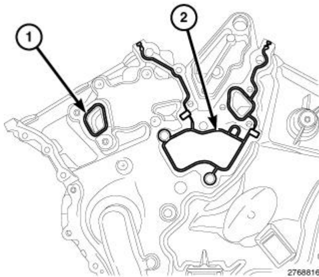
Fig. 728: Coolant Outlet Housing Gasket & Water Pump Gasket Courtesy of CHRYSLER GROUP, LLC
