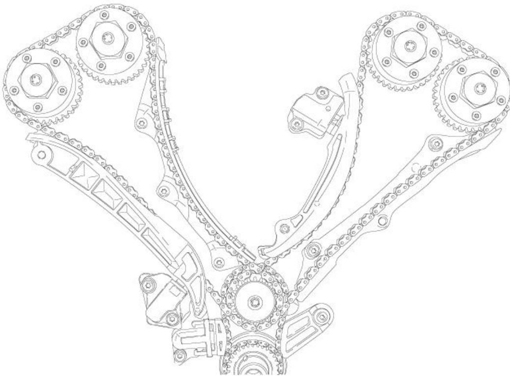
Fig. 673: Secondary Drive Chains
