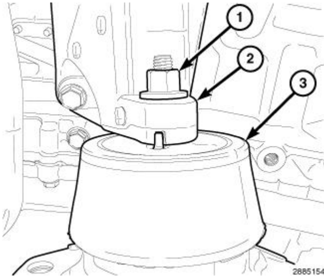
Fig. 489: Left Engine Mount Isolator & Upper Retaining Nut Courtesy of CHRYSLER GROUP, LLC
