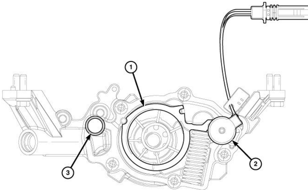
Fig. 600: Moving Element, On/Off Solenoid & Relief Valve Courtesy of CHRYSLER GROUP, LLC
