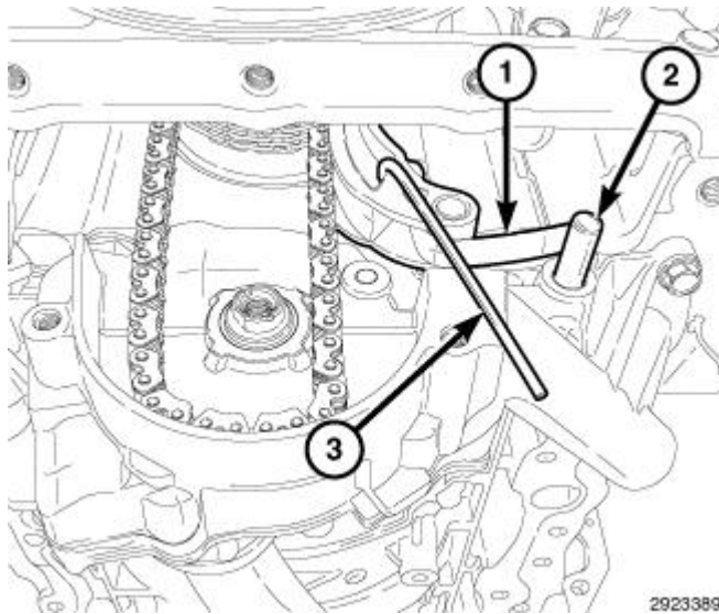
Fig. 613: Retaining Pin, Oil Pump Chain Tensioner Spring & Dowel Pin Courtesy of CHRYSLER GROUP, LLC
