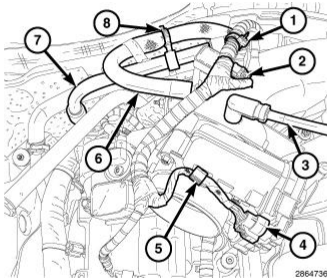
Fig. 639: MAP Sensor, ETC, PCV Hose, Brake Booster Vacuum Hose, EVAP Vapor Purge Line, Clip & Wire Harness Retainer Courtesy of CHRYSLER GROUP, LLC
