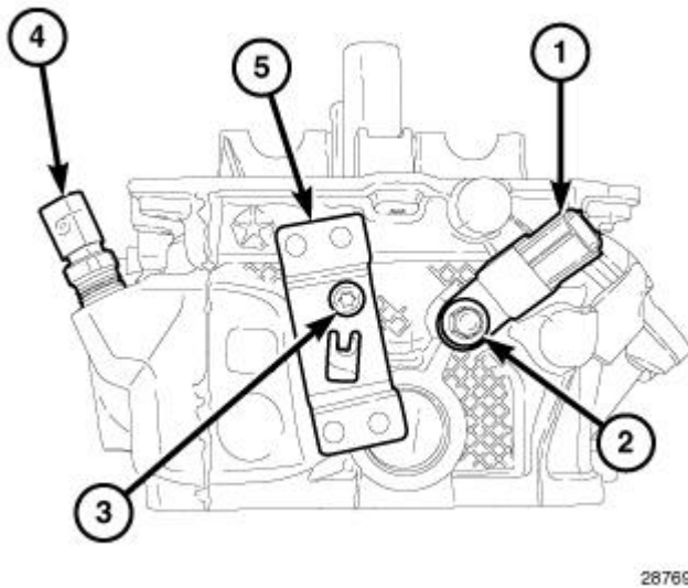
Fig. 162: ECT Sensor, Ignition Coil Capacitor, Engine Wire Harness Retainer Bracket & Bolts Courtesy of CHRYSLER GROUP, LLC
