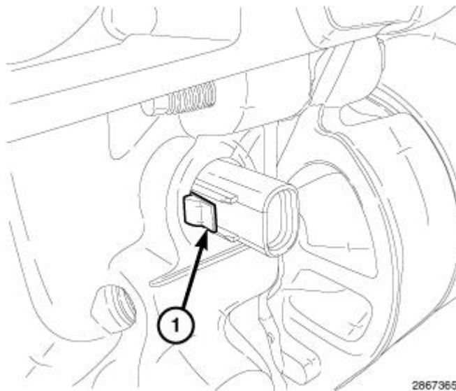
Fig. 616: Oil Pump Solenoid Electrical Connector Retention Lock Tab Courtesy of CHRYSLER GROUP, LLC
