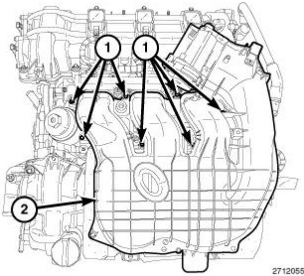
Fig. 493: Upper Intake Manifold & Bolts Courtesy of CHRYSLER GROUP, LLC
