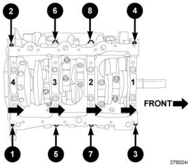
Fig. 421: Main Bearing Tie Bolts Removal Sequence
