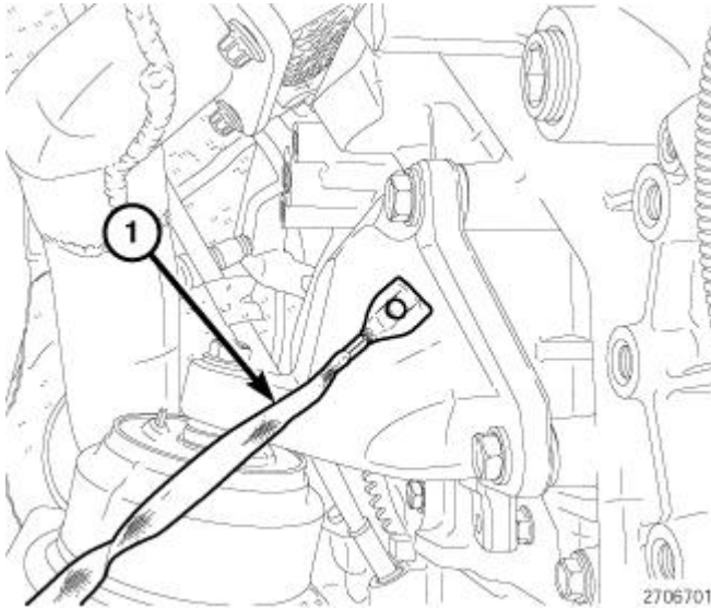
Fig. 507: Ground Strap
