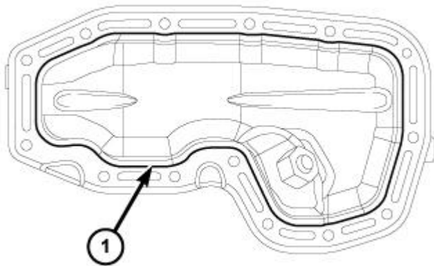
Fig. 578: Mopar® Threebond Engine RTV Sealant Location Courtesy of CHRYSLER GROUP, LLC
