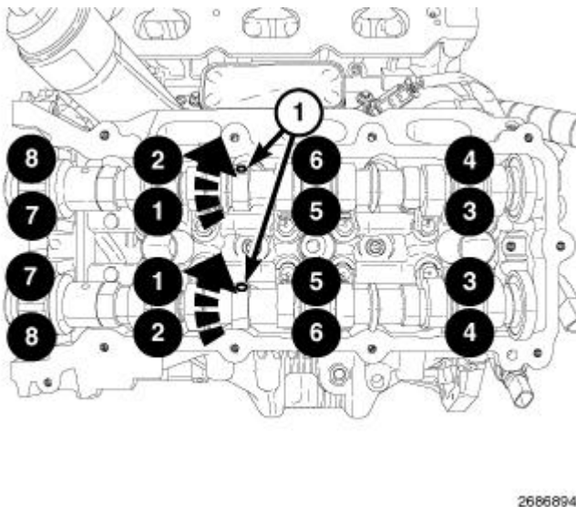
Fig. 259: Bearing Cap Retaining Bolts Tightening Sequence - Left
