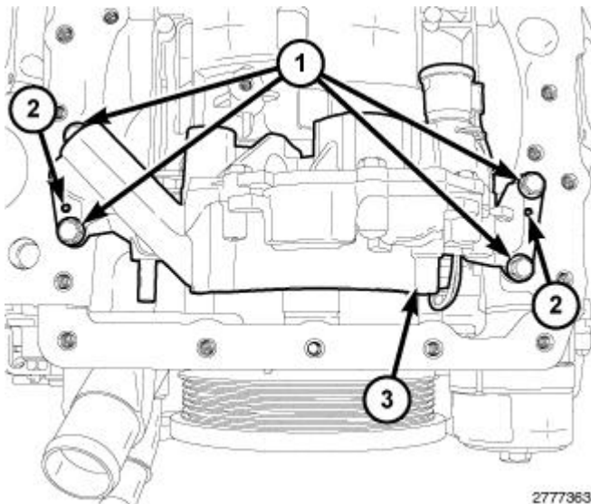
Fig. 610: Oil Pump, Locator Pins & Bolts Courtesy of CHRYSLER GROUP, LLC
