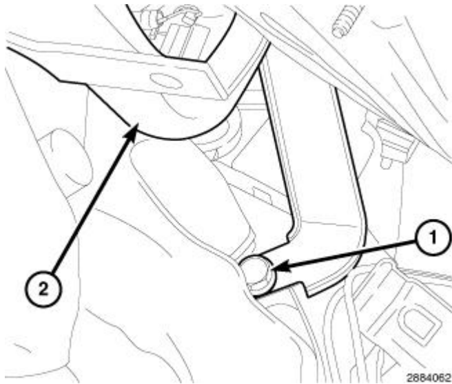
Fig. 327: Upper Transmission-To-Engine Bolt & Transmission Oil Level Indicator Tube Courtesy of CHRYSLER GROUP, LLC
