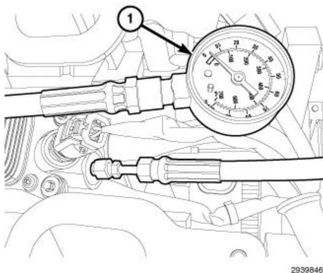
Fig. 524: Pressure Gauge Installed To Oil Pressure Port Courtesy of CHRYSLER GROUP, LLC
