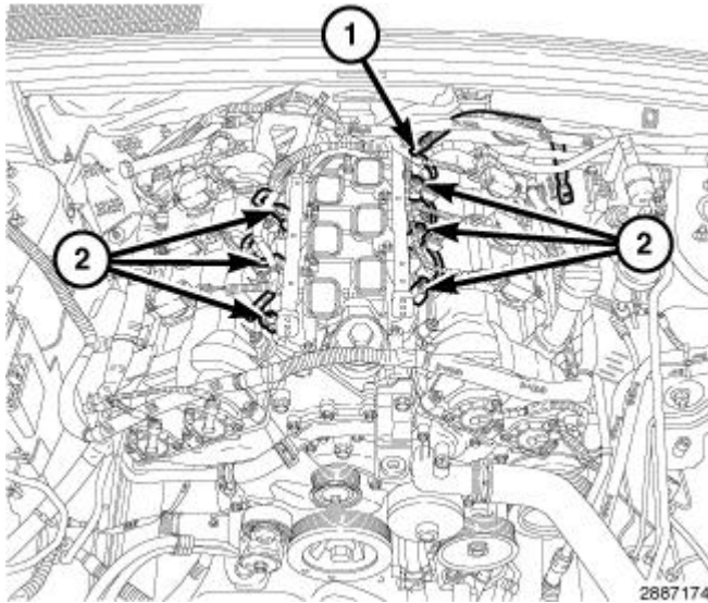
Fig. 668: Fuel Supply Hose & Fuel Injector Electrical Connectors Courtesy of CHRYSLER GROUP, LLC
