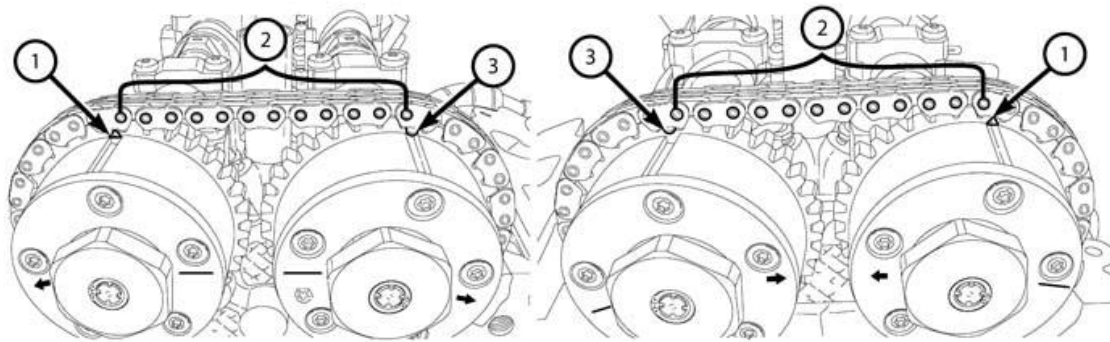
Fig. 683: Chain Pins, Exhaust Cam Phaser Triangle Marking & Circle Marking Courtesy of CHRYSLER GROUP, LLC
