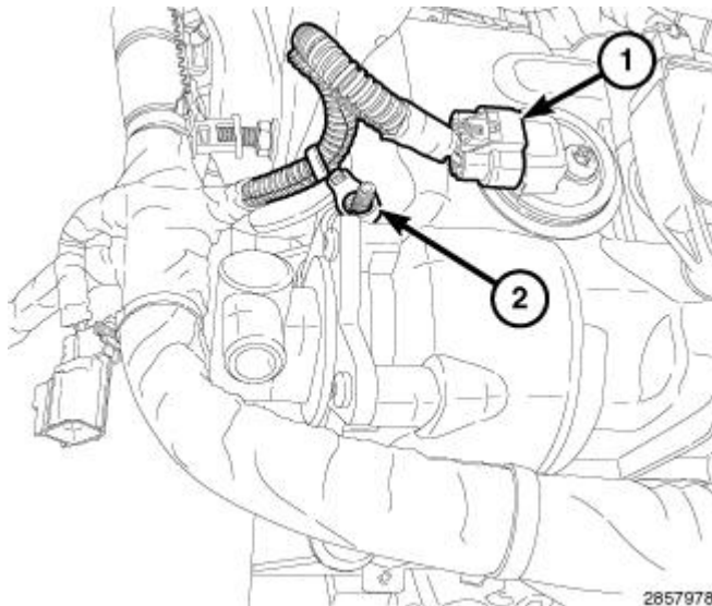
Fig. 325: Main Wire Harness Retainer & Connector
