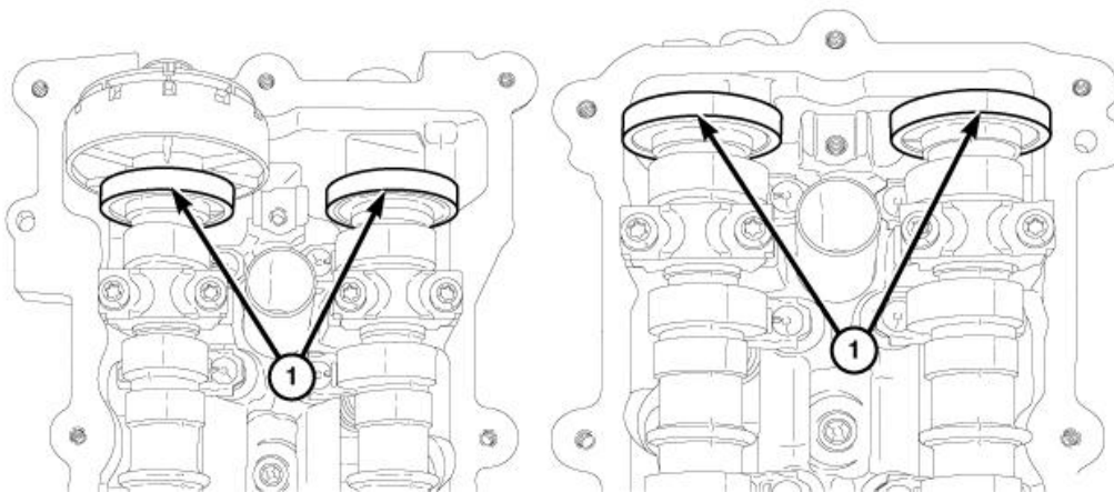
Fig. 684: Magnetic Timing Wheels Courtesy of CHRYSLER GROUP, LLC
