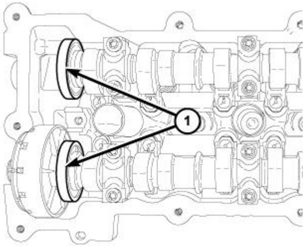
Fig. 235: Magnetic Timing Wheels Courtesy of CHRYSLER GROUP, LLC
