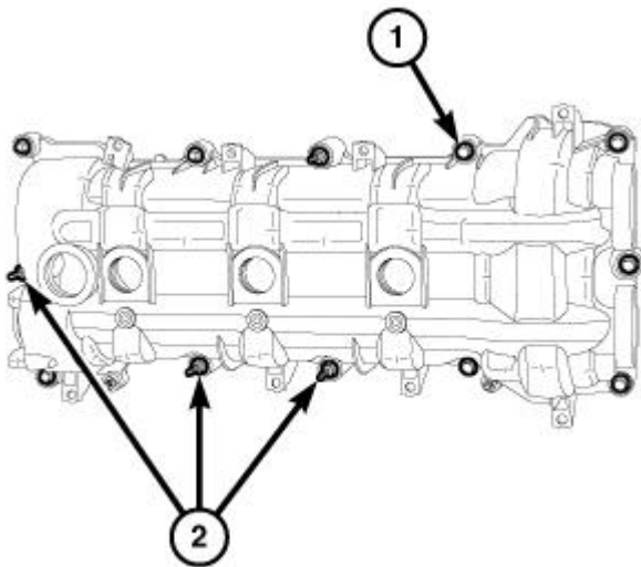
Fig. 296: Cylinder Head Cover Mounting Bolts & Studbolts Courtesy of CHRYSLER GROUP, LLC
