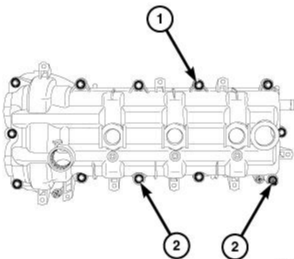
Fig. 720: Cylinder Head Cover Mounting Bolts & Studbolts Courtesy of CHRYSLER GROUP, LLC
