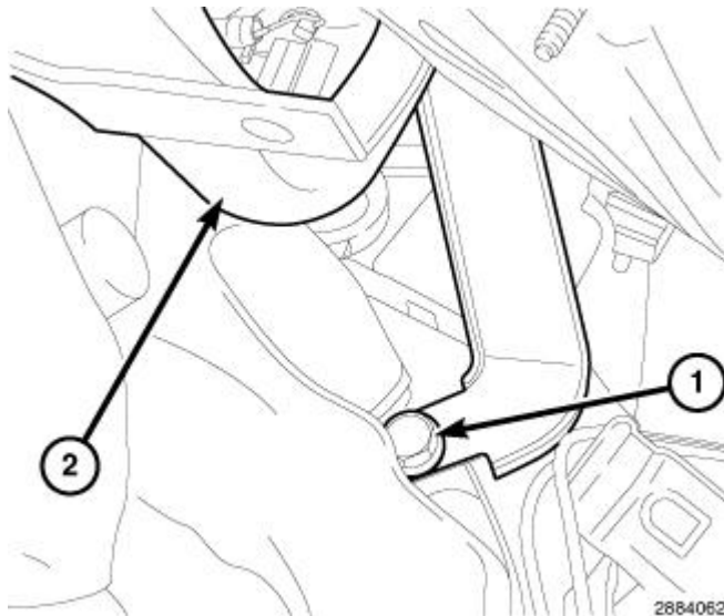
Fig. 294: Upper Transmission-To-Engine Bolt & Transmission Oil Level Indicator Tube Courtesy of CHRYSLER GROUP, LLC
