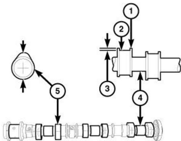
Fig. 257: Inspecting Camshaft Bearing Journals & Cam Lobes
