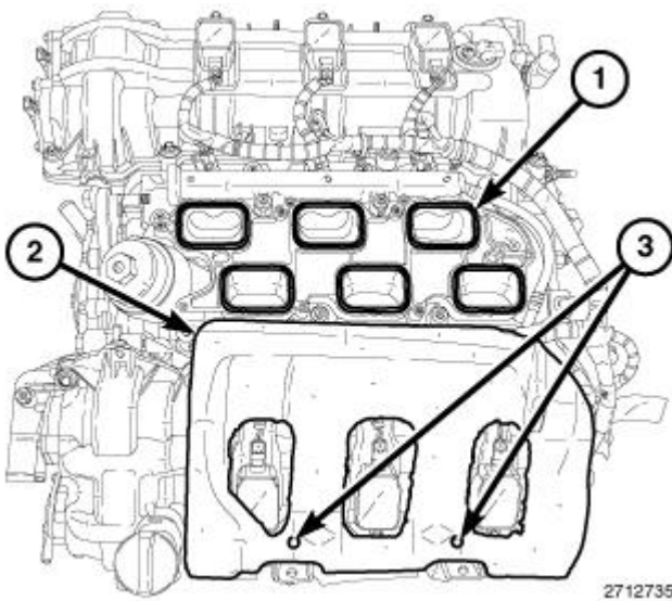
Fig. 285: Intake Ports, Insulator & Alignment Posts Courtesy of CHRYSLER GROUP, LLC
