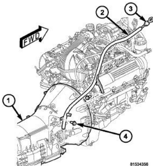
Fig. 348: Transmission Fluid Level Indicator Tube Assembly Courtesy of CHRYSLER GROUP, LLC
