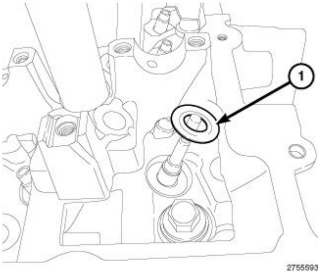
Fig. 342: Valve Spring Seat
