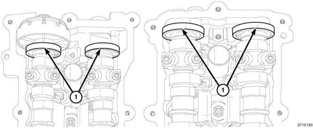
Fig. 680: Magnetic Timing Wheels
