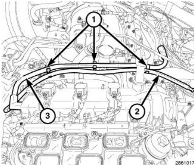
Fig. 272: Transmission Breather Hose, Make-Up Air Tube & Clips Courtesy of CHRYSLER GROUP, LLC
