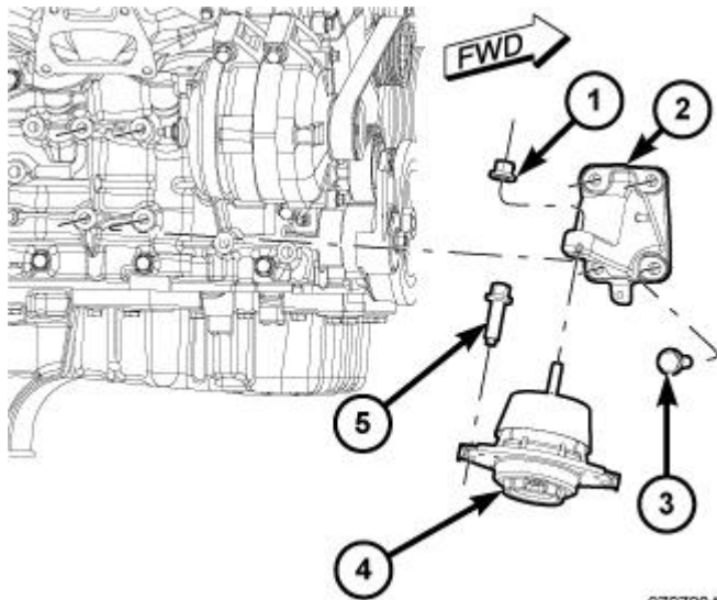
Fig. 502: Engine Mount Isolator, Right Engine Mount Bracket & Retaining Bolts Courtesy of CHRYSLER GROUP, LLC
