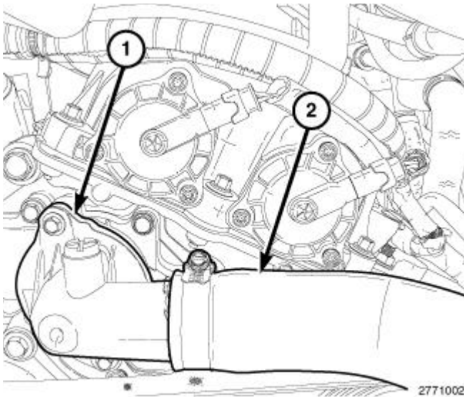
Fig. 715: Upper Radiator Hose & Thermostat Housing Courtesy of CHRYSLER GROUP, LLC
