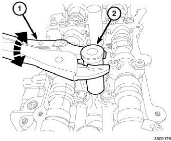
Fig. 370: Locking Pliers & Spark Plug Tube Courtesy of CHRYSLER GROUP, LLC
