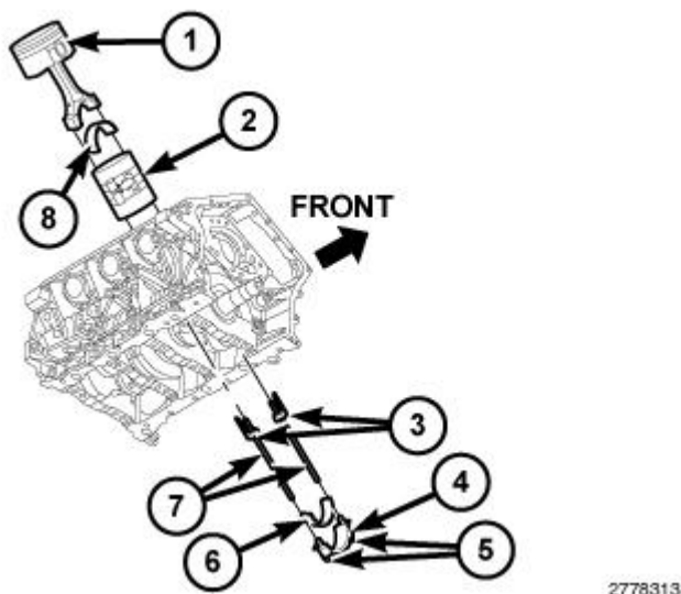
Fig. 431: Piston, Connecting Rod Cap, Bolts, Plastic Guide Plates & Guide Pins Courtesy of CHRYSLER GROUP, LLC
