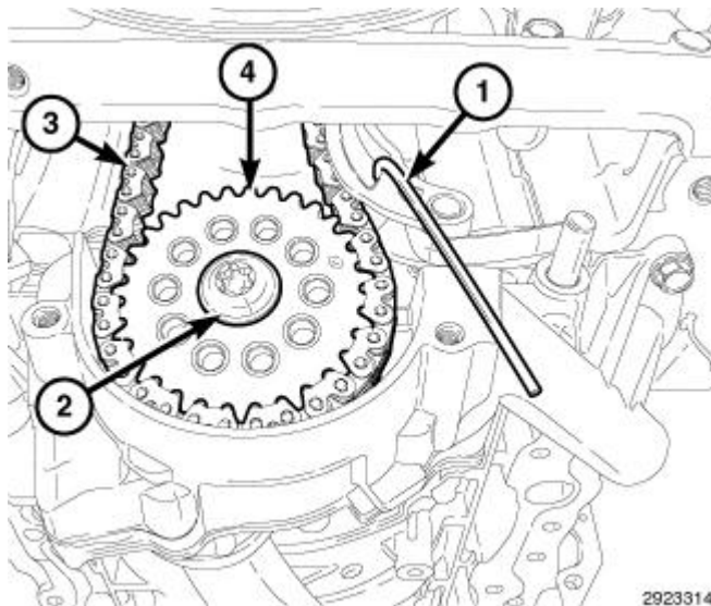
Fig. 608: Retaining Pin, Retaining Bolt, Oil Pump Chain & Sprocket
