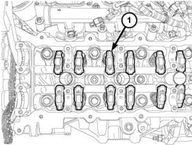
Fig. 349: Locating Rocker Arms
