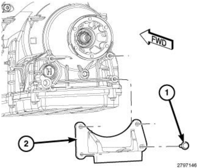
Fig. 517: Rear Engine Mount Bracket & Bolts (4x2)
