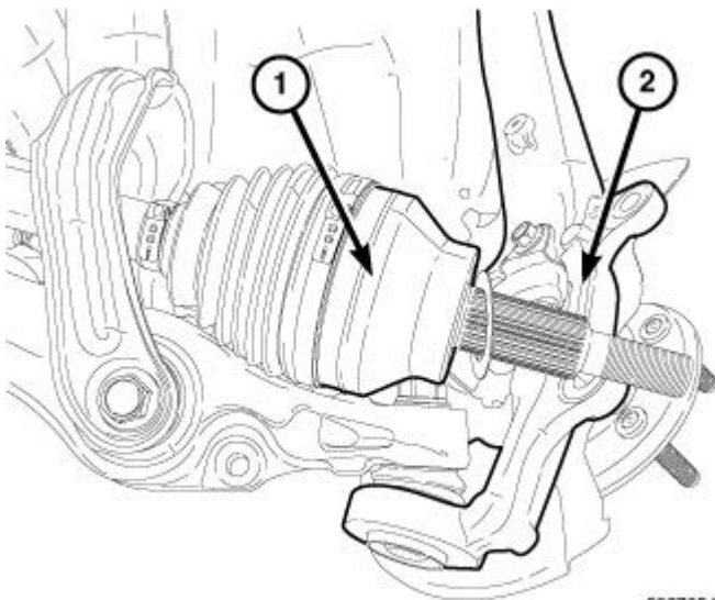
Fig. 500: Knuckle & Push Half Shaft Courtesy of CHRYSLER GROUP, LLC
