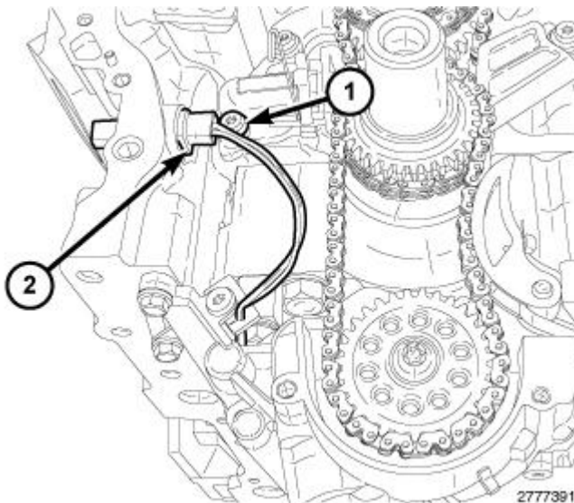
Fig. 606: Oil Pump Solenoid Electrical Connector & Primary Chain Tensioner Mounting Bolt Courtesy of CHRYSLER GROUP, LLC
