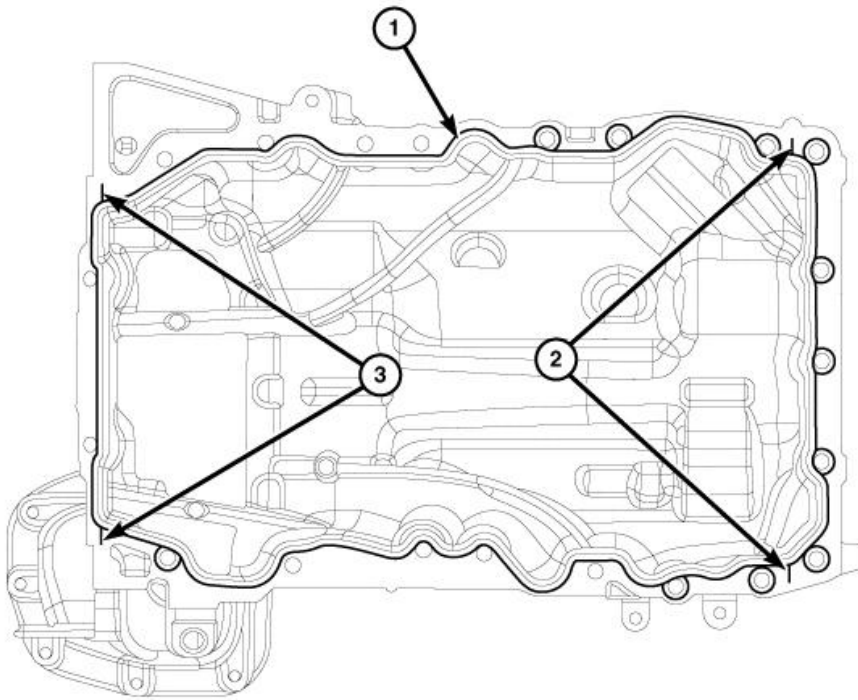
Fig. 577: Mopar® Threebond Engine RTV Sealant Locations Courtesy of CHRYSLER GROUP, LLC
