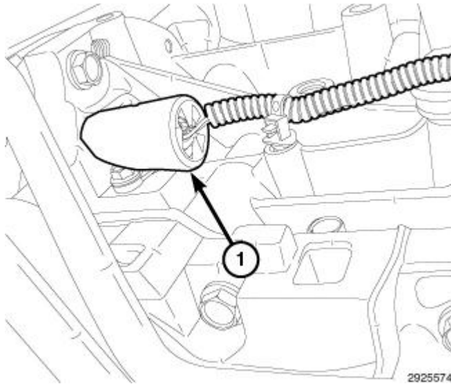
Fig. 35: Heat Shield
