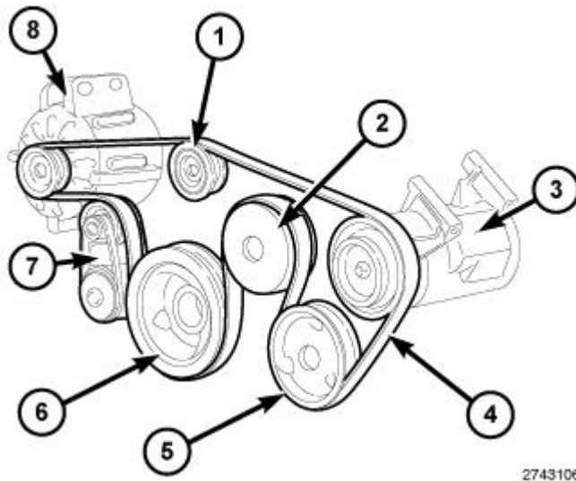
Fig. 509: Drive Belt Tensioners & Accessory Drive Belt Routing Courtesy of CHRYSLER GROUP, LLC
