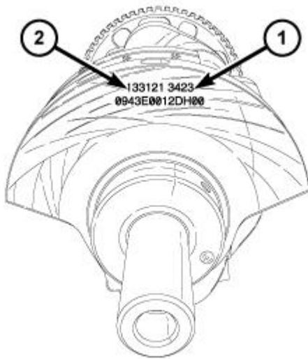
Fig. 395: Connecting Rod Bearing Journal Diameter Grade Markings Courtesy of CHRYSLER GROUP, LLC
