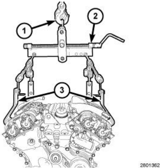
Fig. 417: Lifting Sling, Engine Lifting Brackets & Engine Hoist Courtesy of CHRYSLER GROUP, LLC
