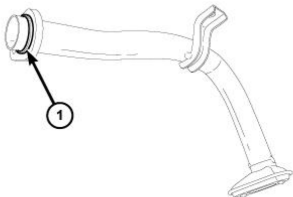
Fig. 597: Oil Pick-Up Tube O-Ring Seal Courtesy of CHRYSLER GROUP, LLC
