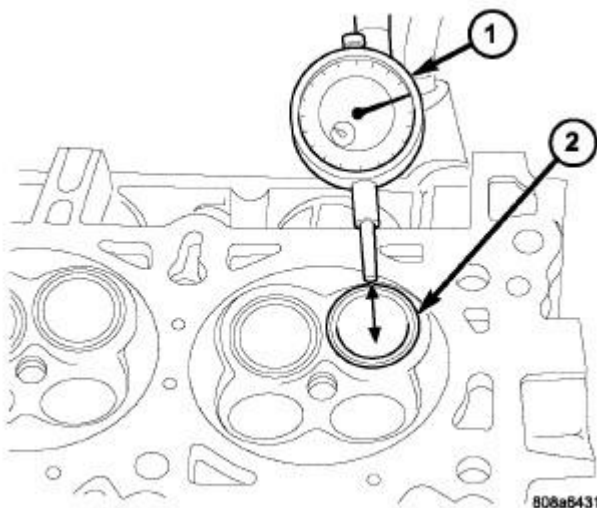
Fig. 386: Measuring Valve Guide Wear
