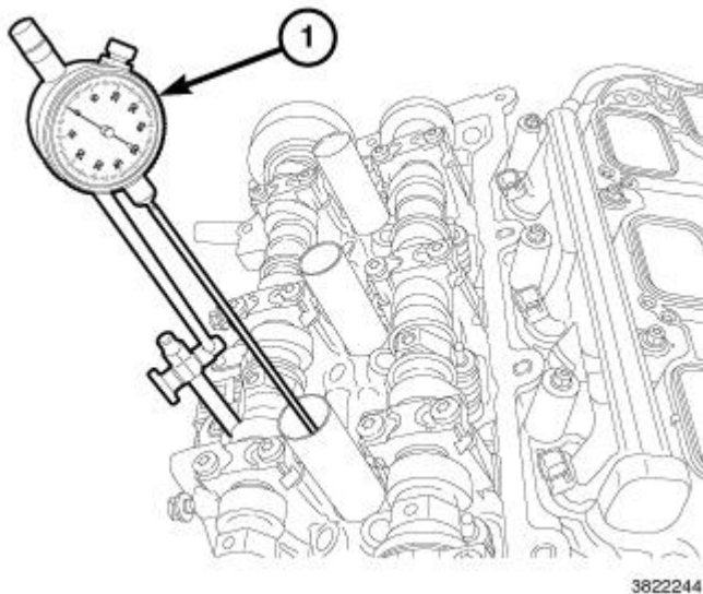
Fig. 681: Mount Dial Indicator Set To Stationary Point On Engine
