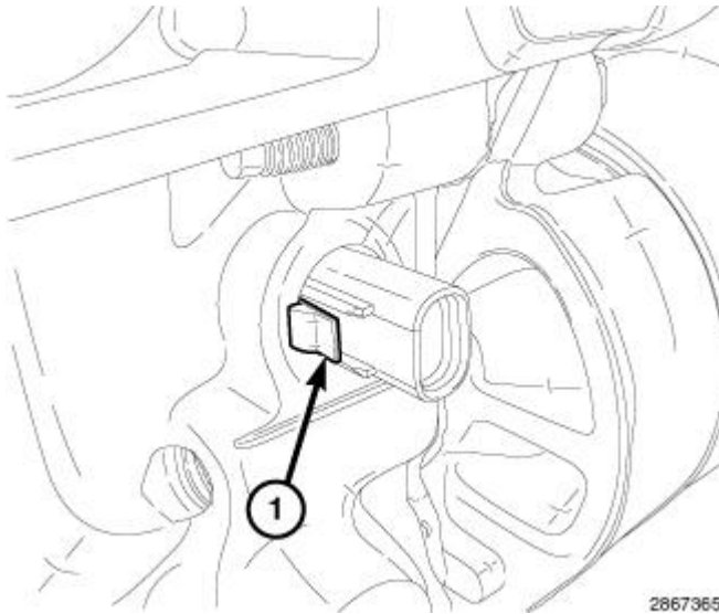
Fig. 605: Oil Pump Solenoid Electrical Connector Retention Lock Tab Courtesy of CHRYSLER GROUP, LLC
