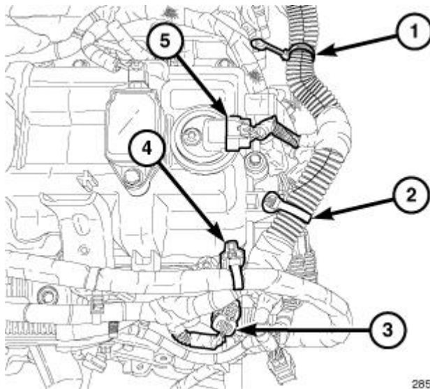
Fig. 276: ECT Sensor Connector, CMP Sensor & Main Wire Harness Retainers
