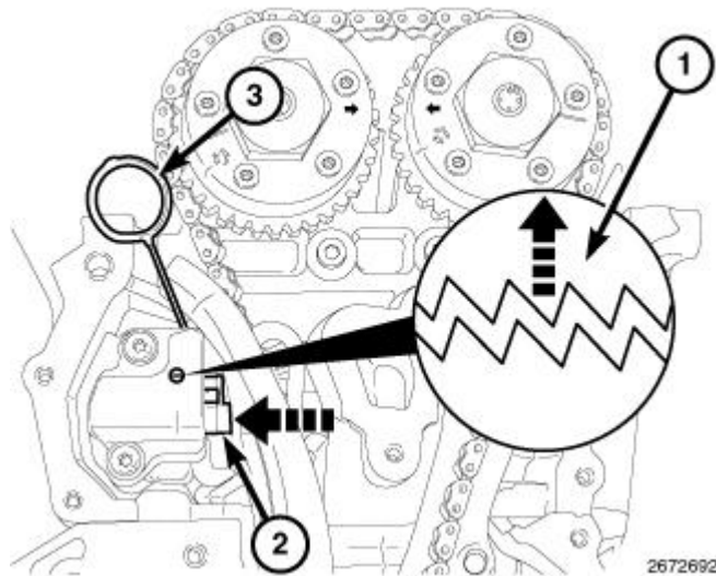
Fig. 135: Resetting Left Cam Chain Tensioner
