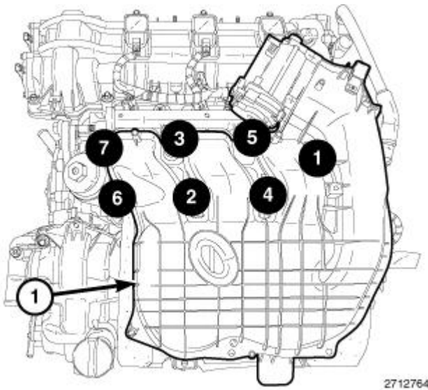
Fig. 656: Upper Intake Manifold Bolt Tightening Sequence Courtesy of CHRYSLER GROUP, LLC
