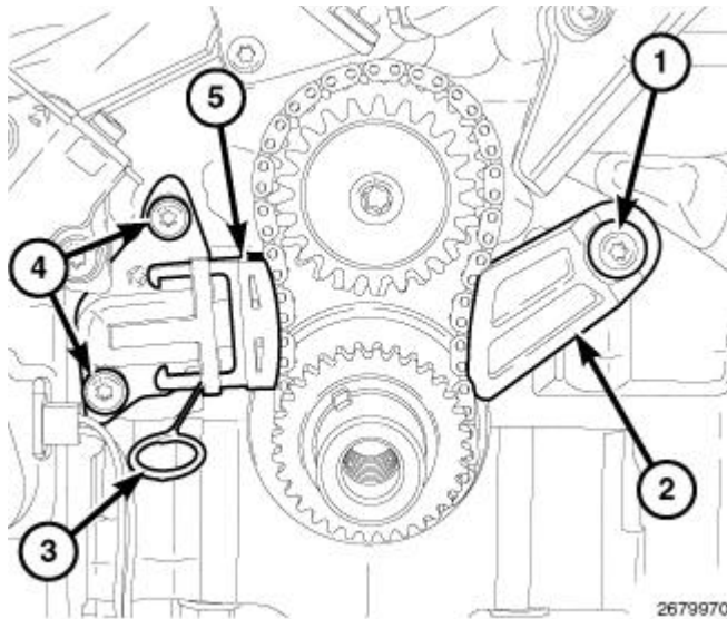
Fig. 692: Primary Chain Tensioner, Tensioner Pin, Primary Chain Guide & Bolts Courtesy of CHRYSLER GROUP, LLC
