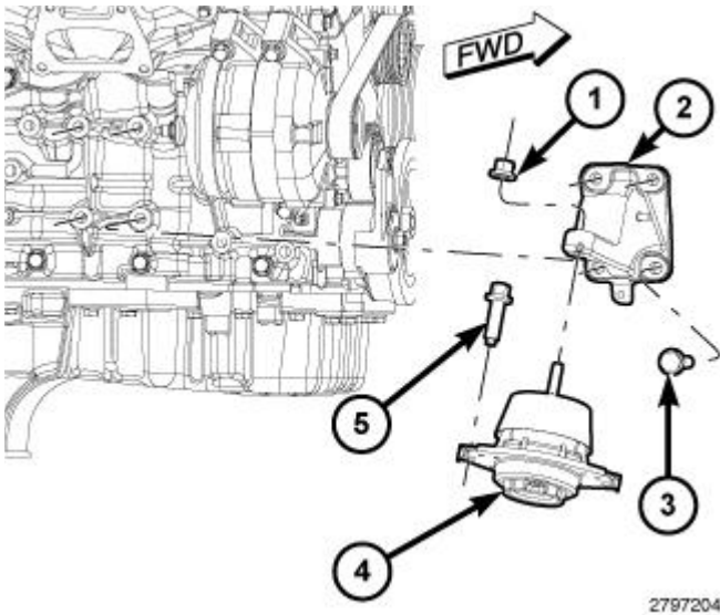
Fig. 503: Engine Mount Isolator, Right Engine Mount Bracket & Retaining Bolts Courtesy of CHRYSLER GROUP, LLC
