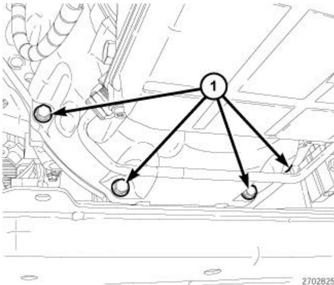
Fig. 583: Transmission-To-Engine Oil Pan Bolts Courtesy of CHRYSLER GROUP, LLC
