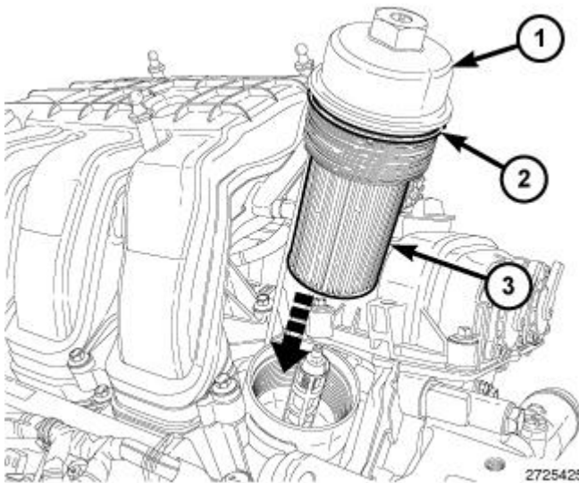
Fig. 558: Oil Filter Cap, O-Ring Seal & Oil Filter Courtesy of CHRYSLER GROUP, LLC
