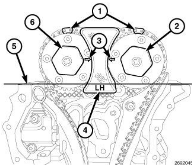
Fig. 708: Phaser Timing Marks, Oil Control Valves & LH Camshaft Phaser Lock Courtesy of CHRYSLER GROUP, LLC
