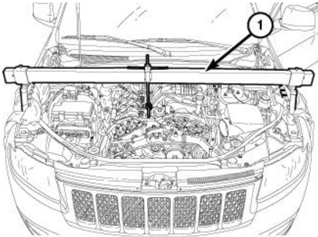
Fig. 499: Engine Support Fixture Courtesy of CHRYSLER GROUP, LLC
