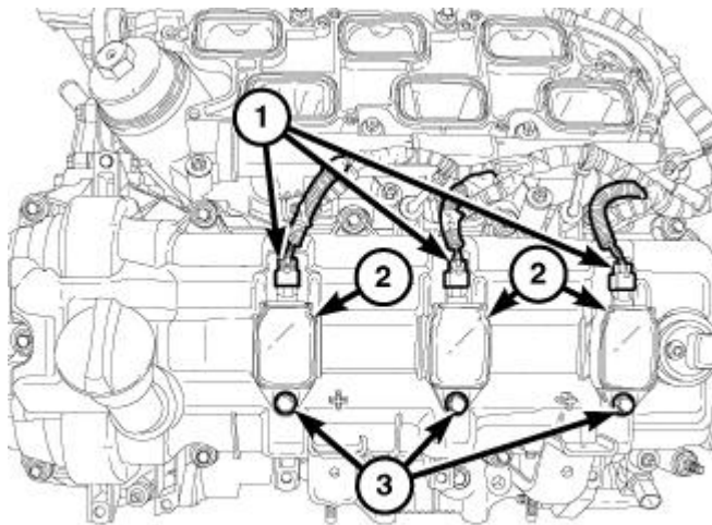
Fig. 304: Electrical Connector, Ignition Coils & Ignition Coil Retaining Bolts Courtesy of CHRYSLER GROUP, LLC
