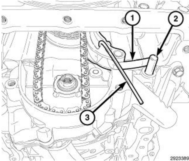
Fig. 609: Retaining Pin, Oil Pump Chain Tensioner Spring & Dowel Pin Courtesy of CHRYSLER GROUP, LLC
