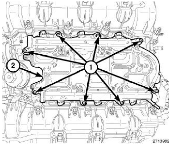
Fig. 649: Lower Intake Manifold & Attaching Bolts Courtesy of CHRYSLER GROUP, LLC
