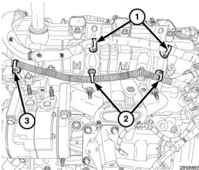
Fig. 308: Starter Wire Harness Retainers, Main Wire Harness Retainer & Manifold Support Bracket Retainers Courtesy of CHRYSLER GROUP, LLC
