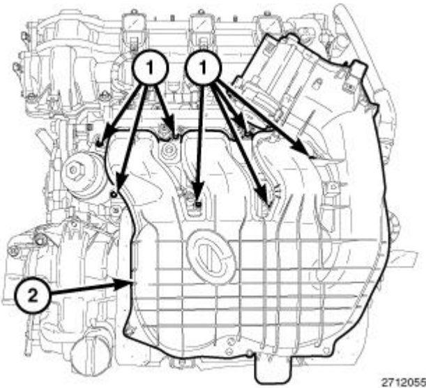
Fig. 270: Upper Intake Manifold & Bolts
