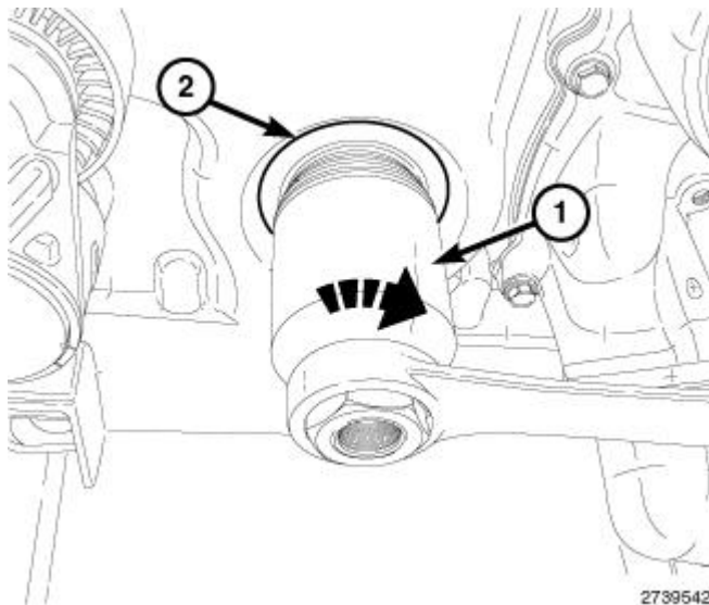
Fig. 470: Seal Remover & Front Crankshaft Oil Seal
