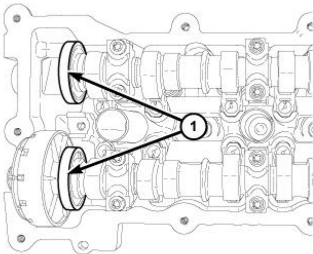
Fig. 314: Magnetic Timing Wheels
