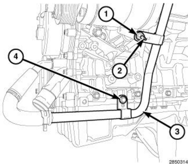
Fig. 363: Heater Core Return Tube, Nut & Bolt Courtesy of CHRYSLER GROUP, LLC
