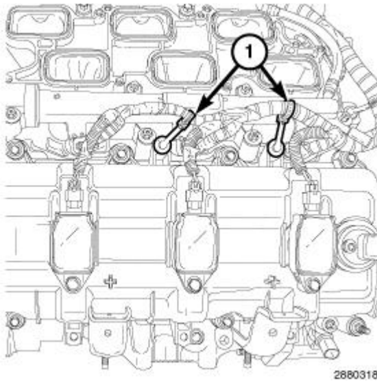
Fig. 305: Injection/Ignition Harness Retainers Courtesy of CHRYSLER GROUP, LLC
