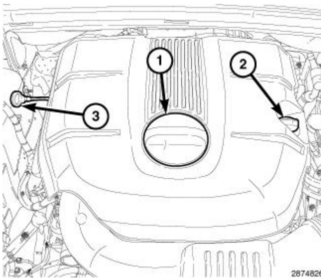
Fig. 559: Oil Filter Access Cover, Oil Fill Cap & Oil Level Indicator Courtesy of CHRYSLER GROUP, LLC
