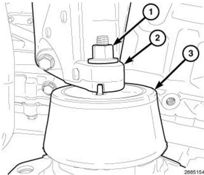
Fig. 481: Left Engine Mount Isolator & Upper Retaining Nut Courtesy of CHRYSLER GROUP, LLC
