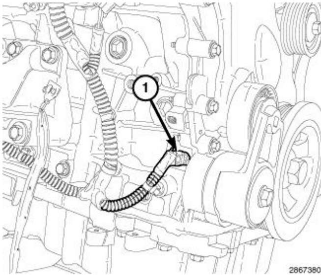
Fig. 604: Oil Pump Solenoid Electrical Connector
