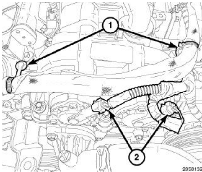
Fig. 307: Variable Valve Timing Solenoid Connectors & Wire Harness Retainers Courtesy of CHRYSLER GROUP, LLC
