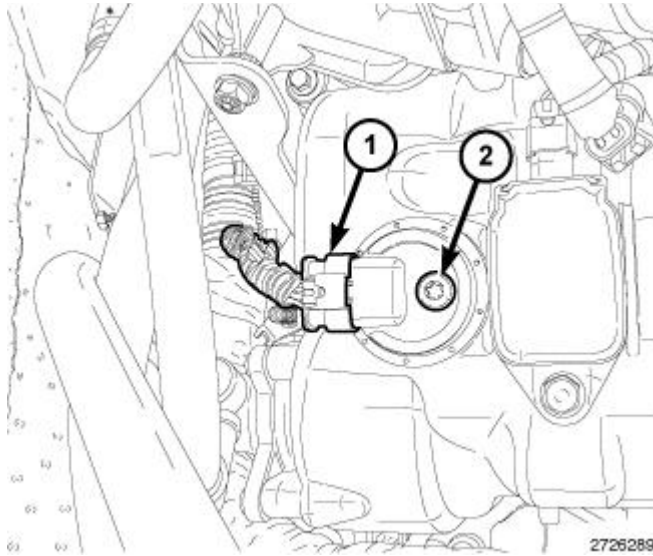
Fig. 324: CMP Sensor & Bolt
