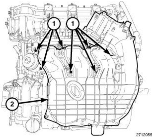
Fig. 645: Upper Intake Manifold & Bolts Courtesy of CHRYSLER GROUP, LLC
