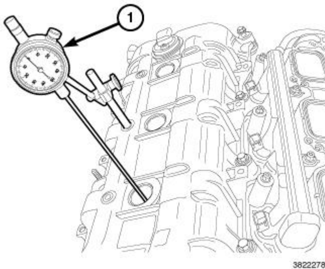
Fig. 229: Mount Dial Indicator Set To Stationary Point On Engine
