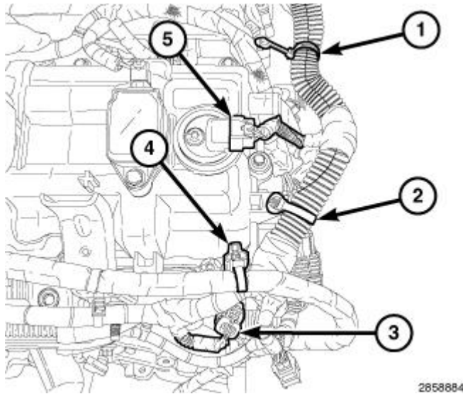
Fig. 175: ECT Sensor Connector, CMP Sensor & Main Wire Harness Retainers Courtesy of CHRYSLER GROUP, LLC
