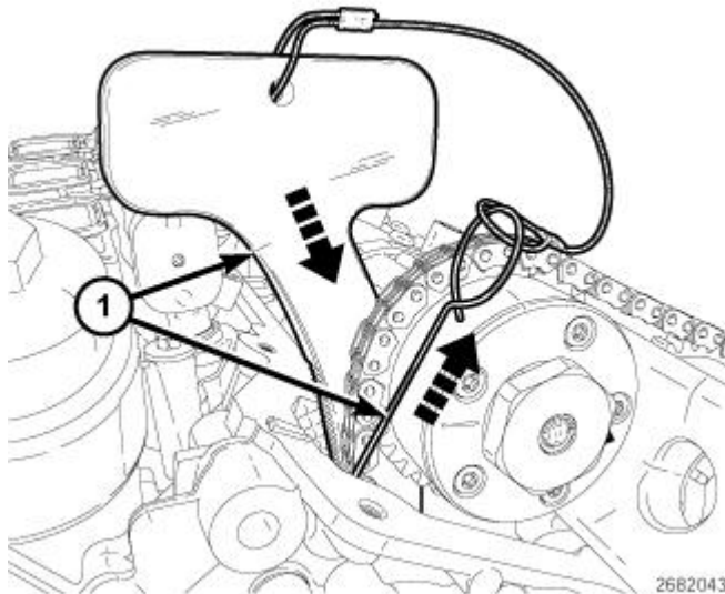
Fig. 678: Positioning Timing Chain Holder To Force Rack & Piston Back Into Tensioner Body Courtesy of CHRYSLER GROUP, LLC
