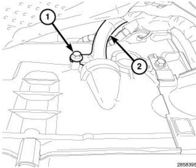
Fig. 293: Transmission Fluid Level Indicator Tube & Bolt Courtesy of CHRYSLER GROUP, LLC
