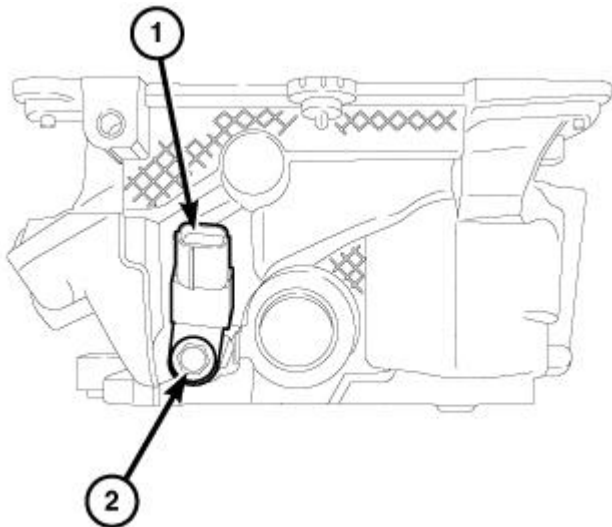
Fig. 189: Ignition Coil Capacitor & Bolt
