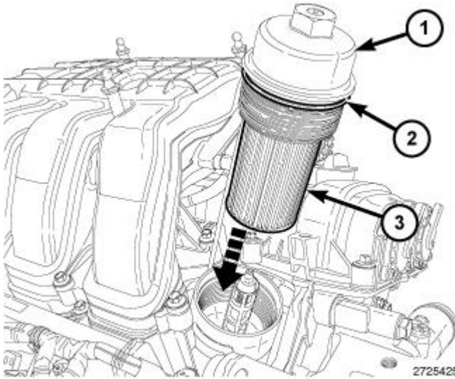
Fig. 536: Oil Filter Cap, O-Ring Seal & Oil Filter Courtesy of CHRYSLER GROUP, LLC
