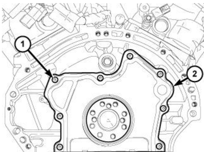
Fig. 473: Seal Retainer & Attaching Screws
