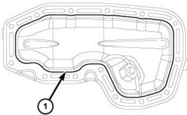
Fig. 579: Mopar® Threebond Engine RTV Sealant Location Courtesy of CHRYSLER GROUP, LLC
