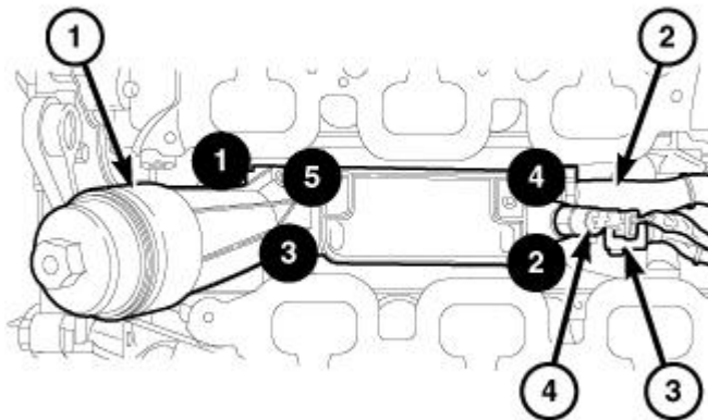
Fig. 625: Heater Hose, Electrical Connectors, Oil Filter Housing & Bolt Tightening Sequence Courtesy of CHRYSLER GROUP, LLC
