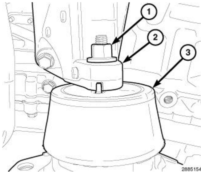
Fig. 498: Left Engine Mount Isolator & Upper Retaining Nut
