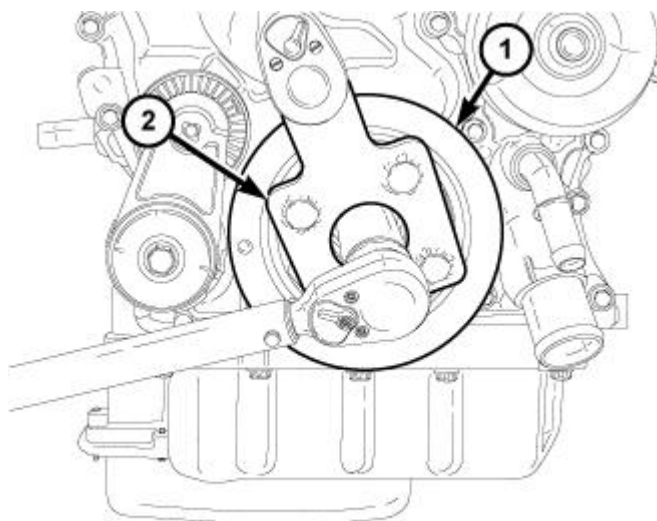
Fig. 435: Crankshaft Vibration Damper & Vibration Damper Holder Courtesy of CHRYSLER GROUP, LLC
