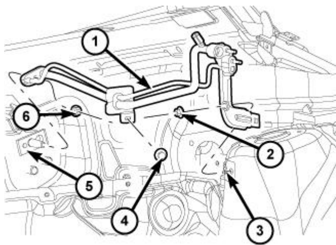
Fig. 346: A/C Suction & Liquid Line Assembly
