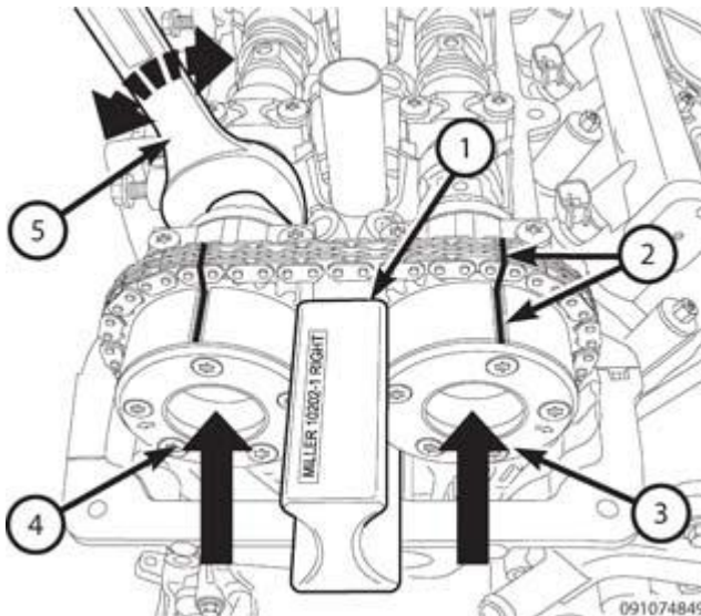
Fig. 266: Marks On Timing Chain Courtesy of CHRYSLER GROUP, LLC
