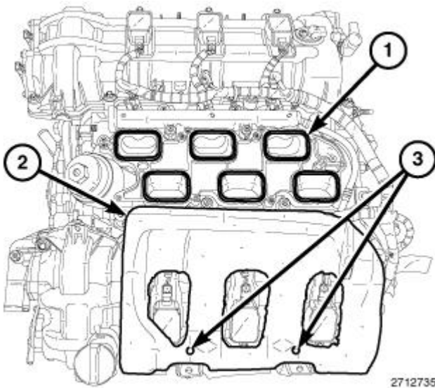
Fig. 644: Intake Ports, Insulator & Alignment Posts Courtesy of CHRYSLER GROUP, LLC
