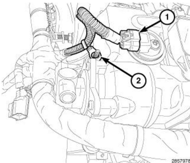
Fig. 20: Main Wire Harness Retainer & Connector Courtesy of CHRYSLER GROUP, LLC
