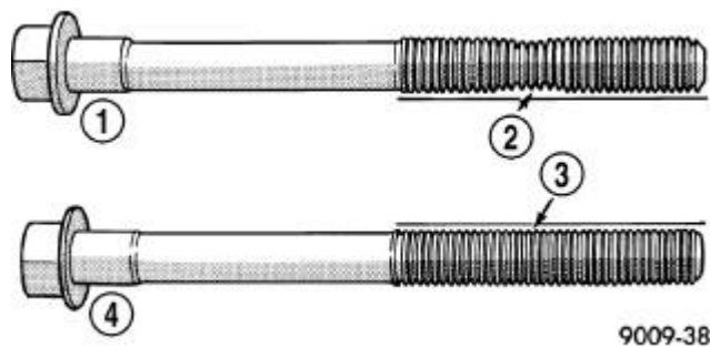
Fig. 401: Checking Cylinder Head Bolts For Stretching (Necking) Courtesy of CHRYSLER GROUP, LLC
