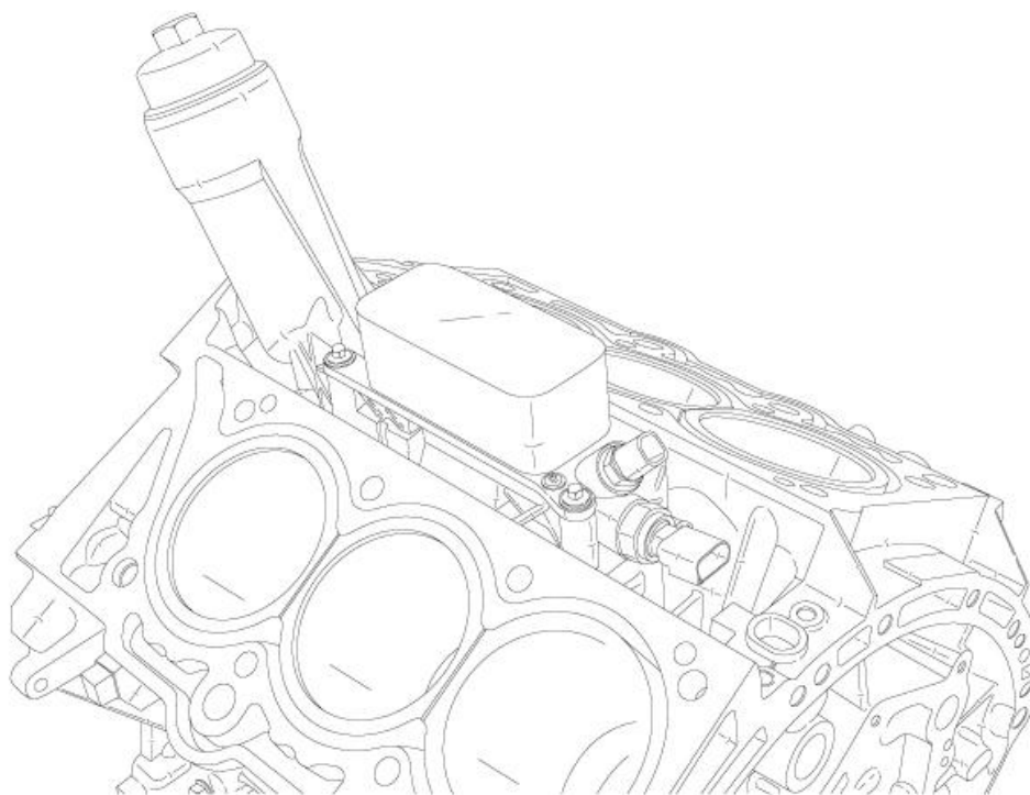
Fig. 537: Oil Filter Housing
