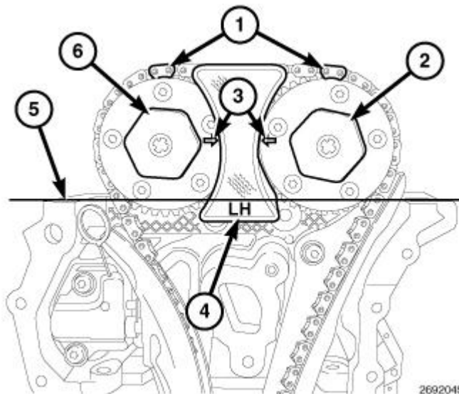
Fig. 136: Phaser Timing Marks, Oil Control Valves & LH Camshaft Phaser Lock
