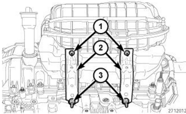
Fig. 658: Nuts, Stud Retainers & Upper Intake Manifold Support Brackets Courtesy of CHRYSLER GROUP, LLC
