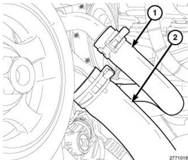
Fig. 736: Radiator Hose & Heater Hose Courtesy of CHRYSLER GROUP, LLC
