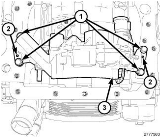
Fig. 612: Oil Pump, Locator Pins & Bolts Courtesy of CHRYSLER GROUP, LLC
