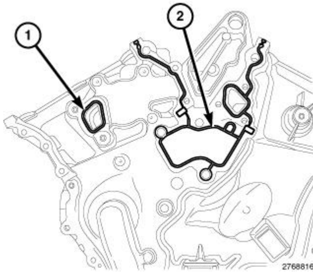
Fig. 726: Coolant Outlet Housing Gasket & Water Pump Gasket Courtesy of CHRYSLER GROUP, LLC
