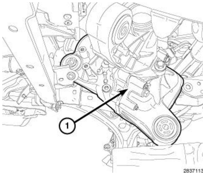
Fig. 488: Front Axle & Axle Bracket Courtesy of CHRYSLER GROUP, LLC
