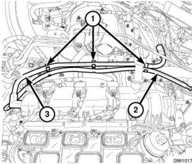
Fig. 311: Transmission Breather Hose, Make-Up Air Tube & Clips Courtesy of CHRYSLER GROUP, LLC
