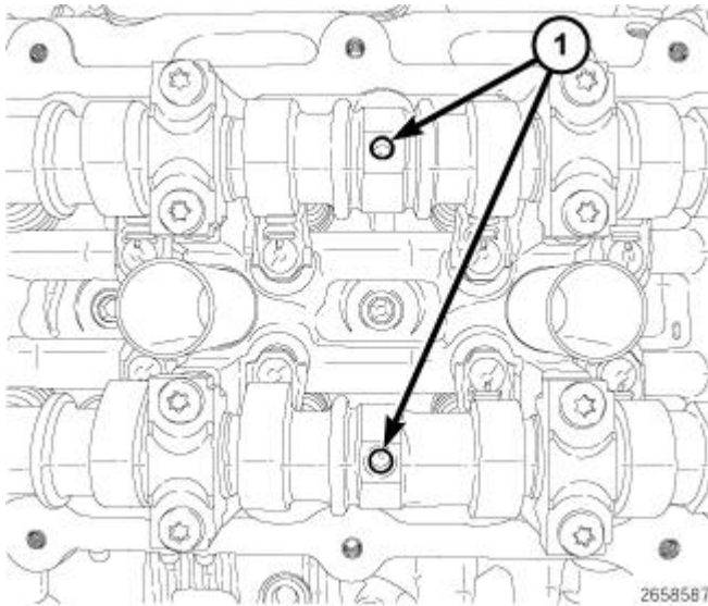
Fig. 701: Positioning Camshaft Alignment Holes Vertically Courtesy of CHRYSLER GROUP, LLC
