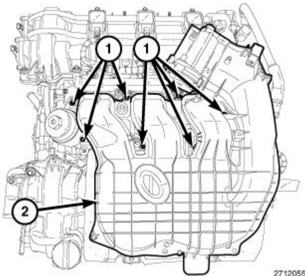
Fig. 643: Upper Intake Manifold & Bolts Courtesy of CHRYSLER GROUP, LLC
