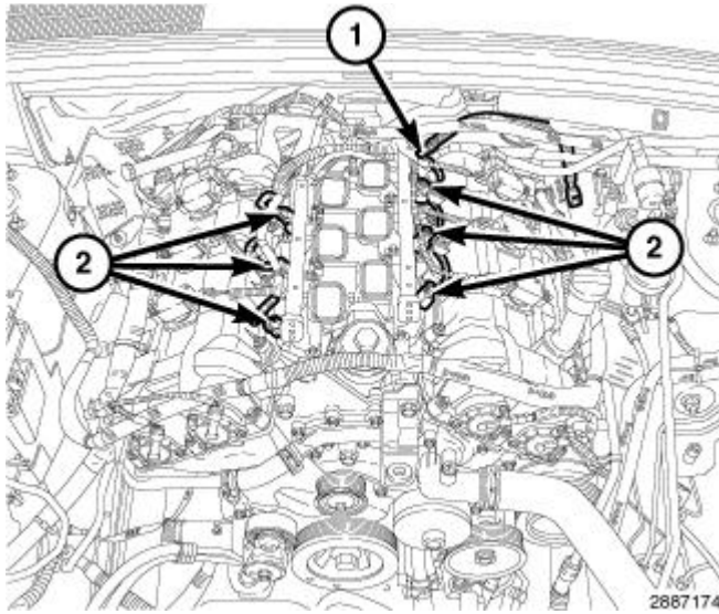
Fig. 647: Fuel Supply Hose & Fuel Injector Electrical Connectors
