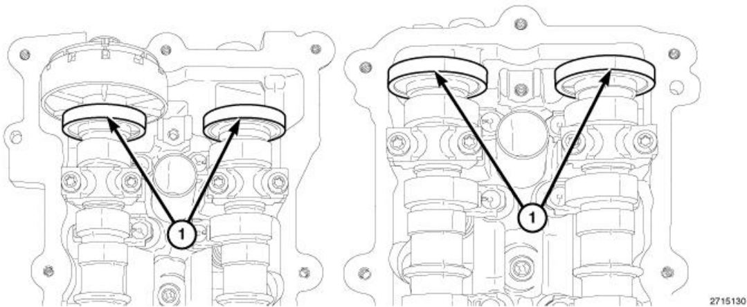
Fig. 697: Magnetic Timing Wheels Courtesy of CHRYSLER GROUP, LLC
