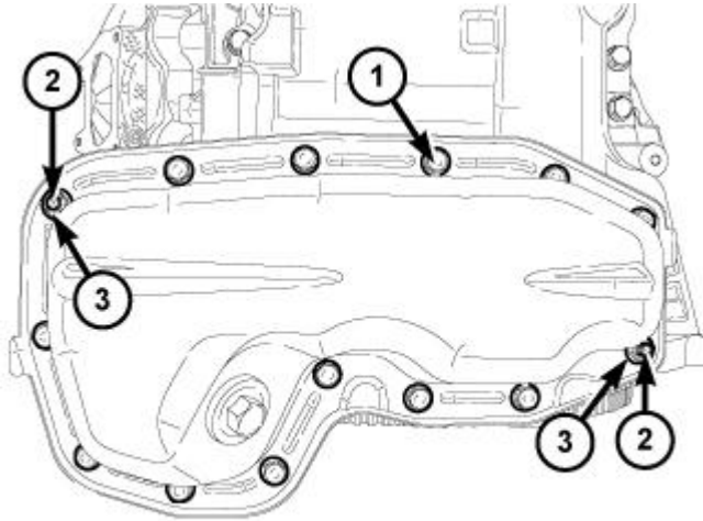
Fig. 731: Lower Oil Pan & Fasteners Courtesy of CHRYSLER GROUP, LLC
