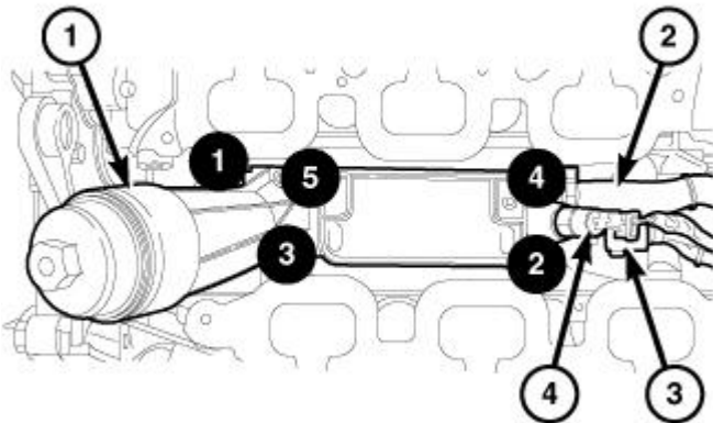
Fig. 632: Heater Hose, Electrical Connectors, Oil Filter Housing & Bolt Tightening Sequence Courtesy of CHRYSLER GROUP, LLC
