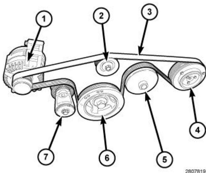
Fig. 91: Idler Pulley, Tensioner Arm, Belt, Idler, Tensioner & Belt Routing Courtesy of CHRYSLER GROUP, LLC
