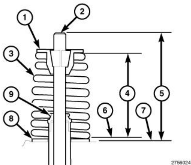
Fig. 380: Checking Valve Spring Installed Height Courtesy of CHRYSLER GROUP, LLC
