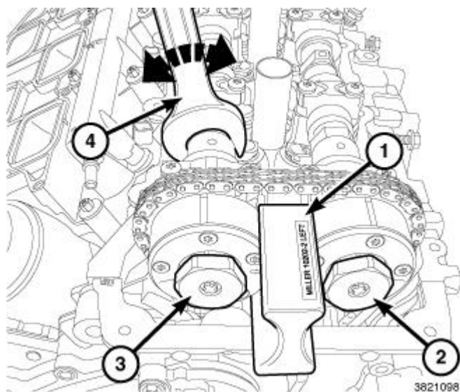
Fig. 691: Camshaft Phaser Lock, Oil Control Valves & Wrench Courtesy of CHRYSLER GROUP, LLC
