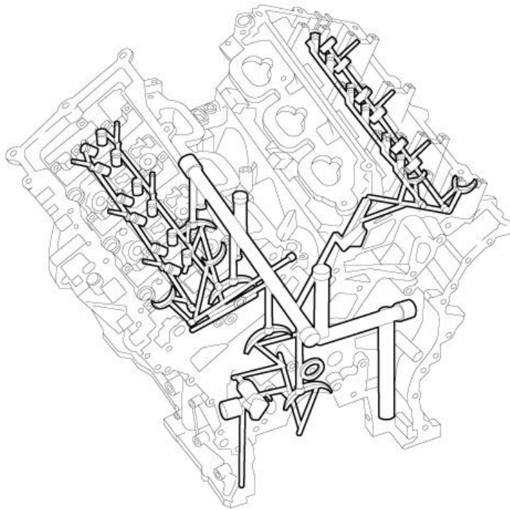
Fig. 523: Engine Lubrication Flow Courtesy of CHRYSLER GROUP, LLC
