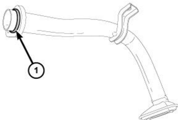
Fig. 596: Oil Pick-Up Tube O-Ring Seal Courtesy of CHRYSLER GROUP, LLC
