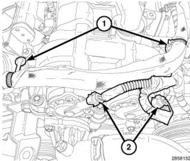
Fig. 273: Variable Valve Timing Solenoid Connectors & Wire Harness Retainers Courtesy of CHRYSLER GROUP, LLC
