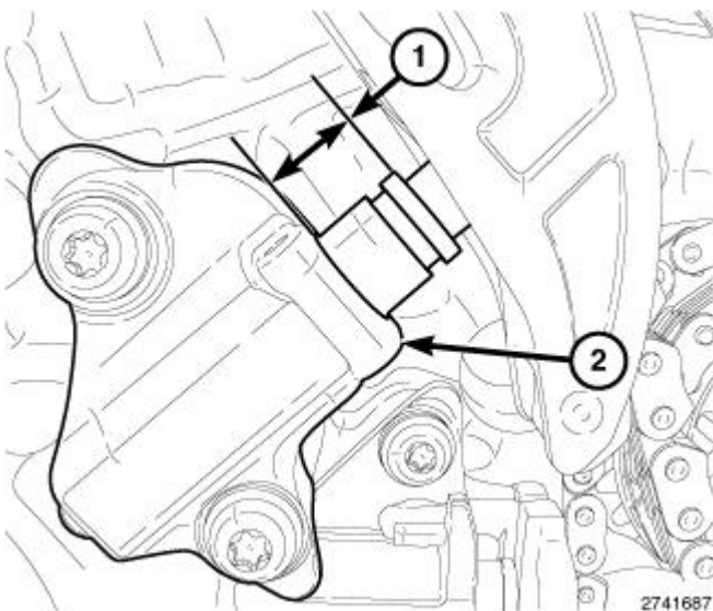
Fig. 679: Piston Extension & RH Cam Chain Tensioner Courtesy of CHRYSLER GROUP, LLC
