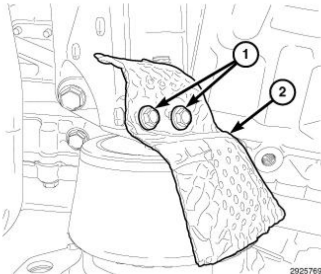
Fig. 490: Engine Mount Heatshield & Bolts Courtesy of CHRYSLER GROUP, LLC
