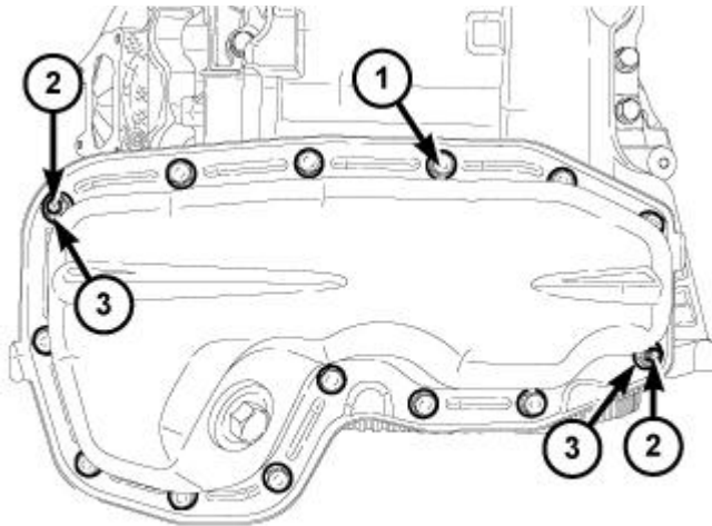
Fig. 588: Lower Oil Pan & Fasteners Courtesy of CHRYSLER GROUP, LLC
