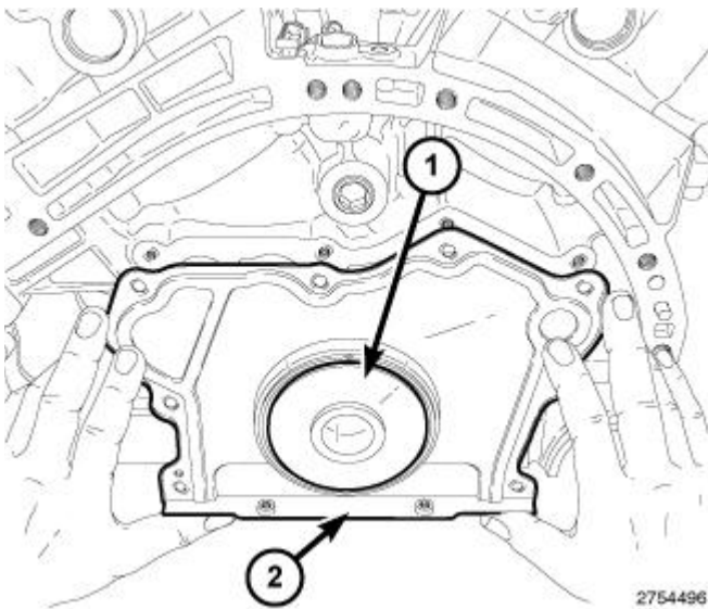
Fig. 475: Oil Seal Retainer Assembly & Seal Protector Courtesy of CHRYSLER GROUP, LLC
