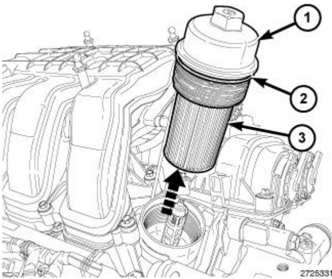
Fig. 533: Oil Filter Cap, O-Ring Seal & Oil Filter Courtesy of CHRYSLER GROUP, LLC
