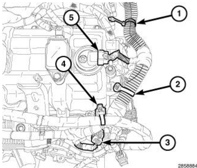
Fig. 310: ECT Sensor Connector, CMP Sensor & Main Wire Harness Retainers
