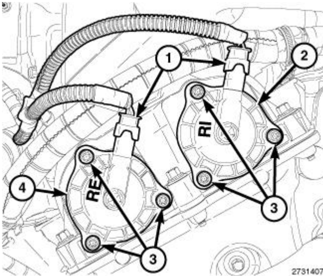
Fig. 321: Variable Valve Timing Solenoids, Connectors & Bolts Courtesy of CHRYSLER GROUP, LLC
