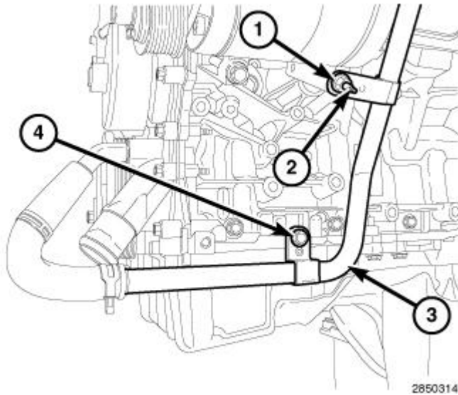
Fig. 484: Heater Core Return Tube, Nut & Bolt Courtesy of CHRYSLER GROUP, LLC
