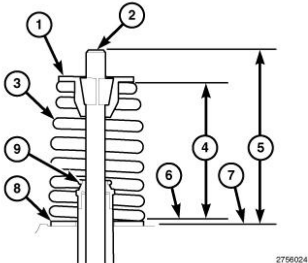
Fig. 367: Checking Valve Spring Installed Height Courtesy of CHRYSLER GROUP, LLC
