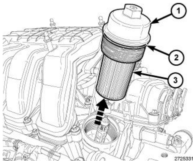
Fig. 555: Oil Filter Cap, O-Ring Seal & Oil Filter Courtesy of CHRYSLER GROUP, LLC
