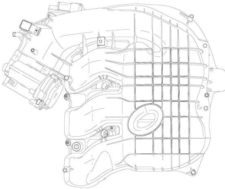
Fig. 634: Upper Intake Manifold Design Courtesy of CHRYSLER GROUP, LLC
