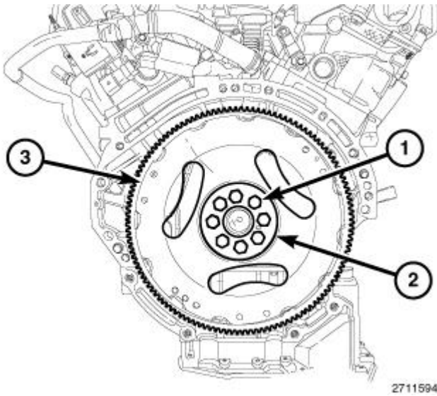
Fig. 440: Flexplate, Spacer Plate & Bolts Courtesy of CHRYSLER GROUP, LLC
