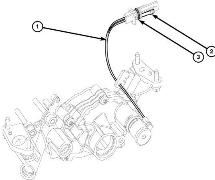
Fig. 611: Solenoid Wires, Connector Retention Lock Tab & O-Ring Seal Courtesy of CHRYSLER GROUP, LLC
