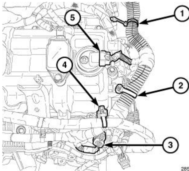
Fig. 510: ECT Sensor Connector, CMP Sensor & Main Wire Harness Retainers Courtesy of CHRYSLER GROUP, LLC
