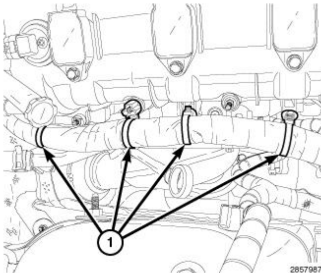
Fig. 288: Main Wire Harness Retainers At Right Cylinder Head Cover Courtesy of CHRYSLER GROUP, LLC
