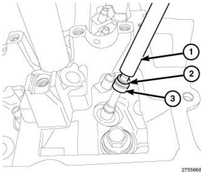
Fig. 343: Installing Valve Guide Seal
