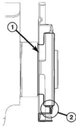
Fig. 476: Rear Seal Installed Courtesy of CHRYSLER GROUP, LLC
