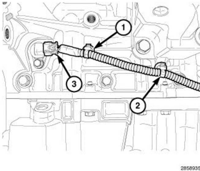
Fig. 36: Main Wire Harness Retainers & CKP Sensor
