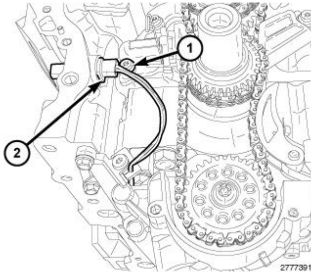
Fig. 615: Oil Pump Solenoid Electrical Connector & Primary Chain Tensioner Mounting Bolt Courtesy of CHRYSLER GROUP, LLC
