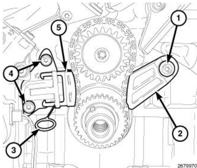
Fig. 705: Primary Chain Tensioner, Tensioner Pin, Primary Chain Guide & Bolts
