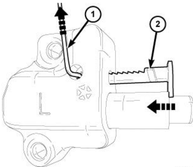
Fig. 675: Locating Slot In Rack & Allen Wrench Courtesy of CHRYSLER GROUP, LLC
