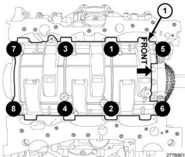
Fig. 432: Windage Tray With Main Bearing Cap Bolts Installation Sequence Courtesy of CHRYSLER GROUP, LLC
