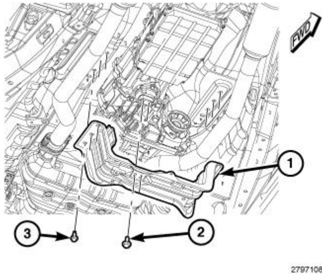
Fig. 520: Crossmember & Bolts Courtesy of CHRYSLER GROUP, LLC
