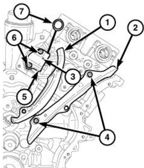
Fig. 699: Left Cam Chain Tensioner, Arm, Guide & Bolts Courtesy of CHRYSLER GROUP, LLC
