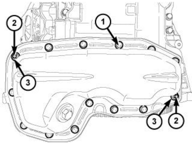
Fig. 570: Lower Oil Pan & Fasteners Courtesy of CHRYSLER GROUP, LLC
