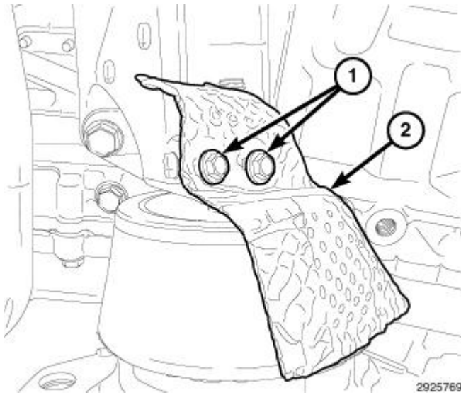
Fig. 480: Engine Mount Heatshield & Bolts Courtesy of CHRYSLER GROUP, LLC
