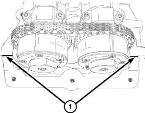
Fig. 282: RTV Sealant Locations Courtesy of CHRYSLER GROUP, LLC
