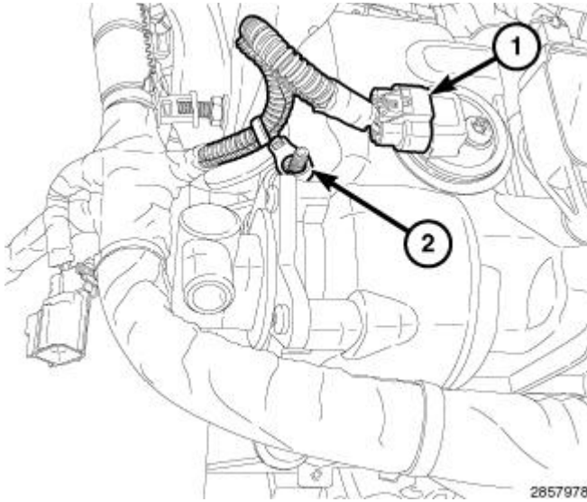
Fig. 289: Main Wire Harness Retainer & Connector Courtesy of CHRYSLER GROUP, LLC
