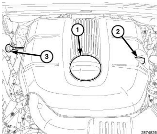
Fig. 554: Oil Filter Access Cover, Oil Fill Cap & Oil Level Indicator
