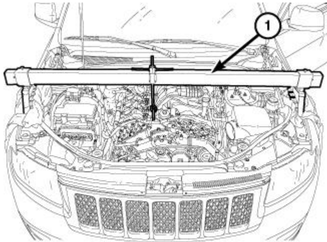
Fig. 482: Engine Support Fixture Courtesy of CHRYSLER GROUP, LLC
