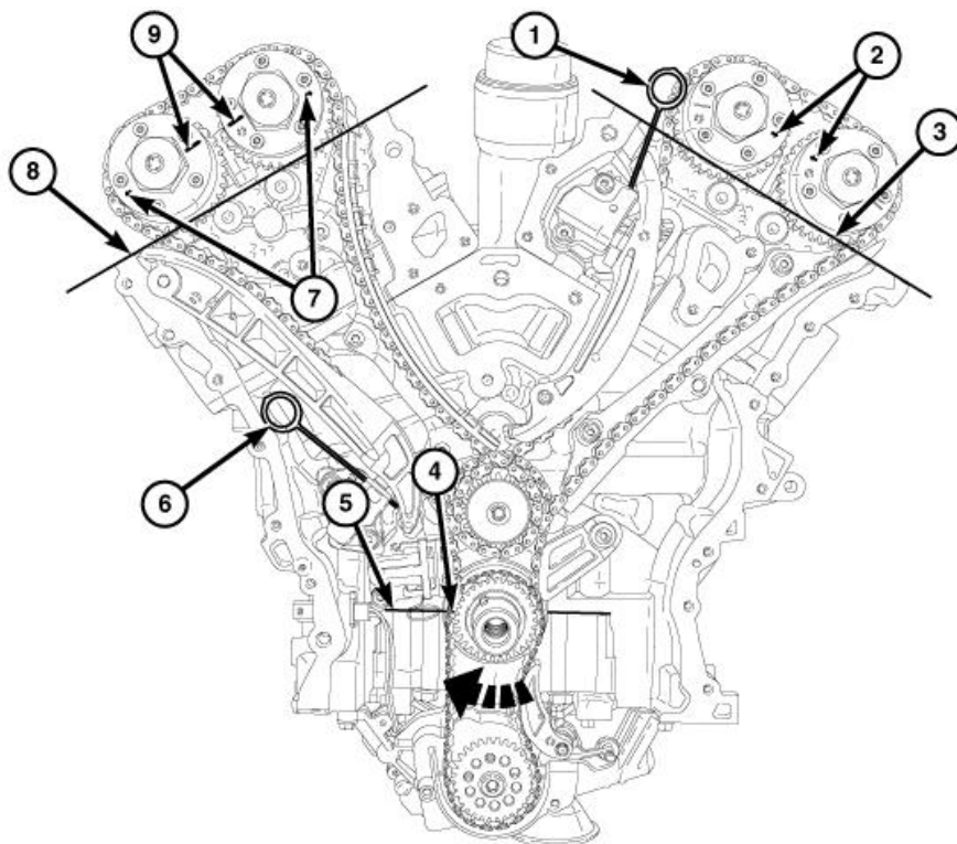
Fig. 170: Rotating Crankshaft Clockwise To Position No. 1 Piston At TDC On Exhaust Stroke Courtesy of CHRYSLER GROUP, LLC
