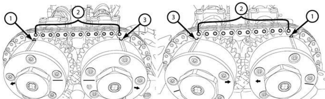
Fig. 714: Chain Pins, Exhaust Cam Phaser Triangle Marking & Circle Marking Courtesy of CHRYSLER GROUP, LLC
