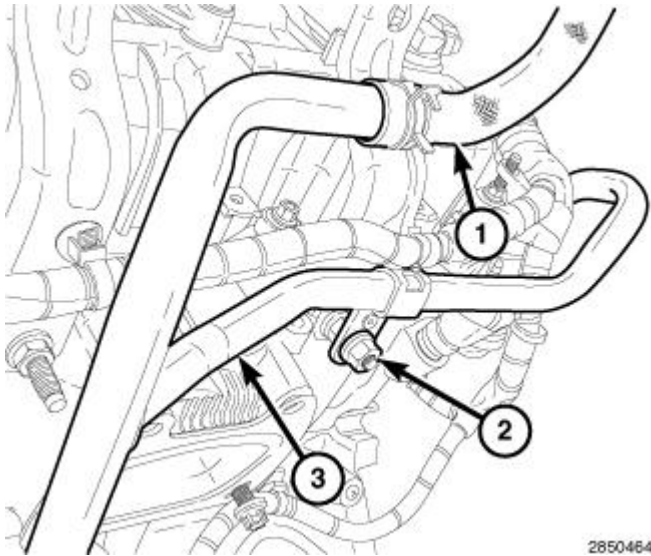
Fig. 30: Heater Core Return Hose, Heater Core Return Tube & Nut Courtesy of CHRYSLER GROUP, LLC
