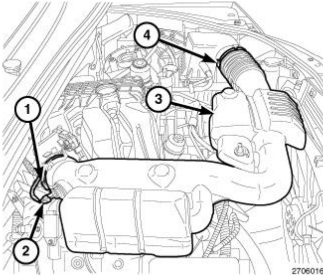
Fig. 662: Air Inlet Hose, Air Temperature (IAT) Sensor Connector & Clamps Courtesy of CHRYSLER GROUP, LLC
