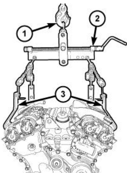
Fig. 434: Lifting Sling, Engine Lifting Brackets & Engine Hoist
