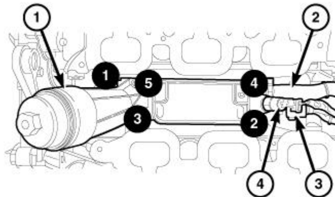
Fig. 548: Heater Hose, Electrical Connectors, Oil Filter Housing & Bolt Tightening Sequence Courtesy of CHRYSLER GROUP, LLC
