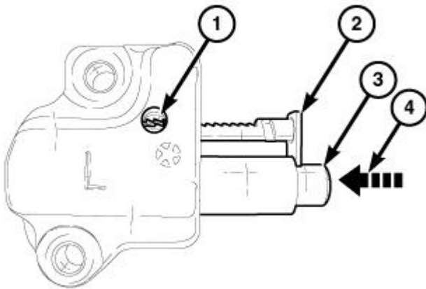
Fig. 674: Left Side Cam Chain Tensioner Ratchet Components Courtesy of CHRYSLER GROUP, LLC
