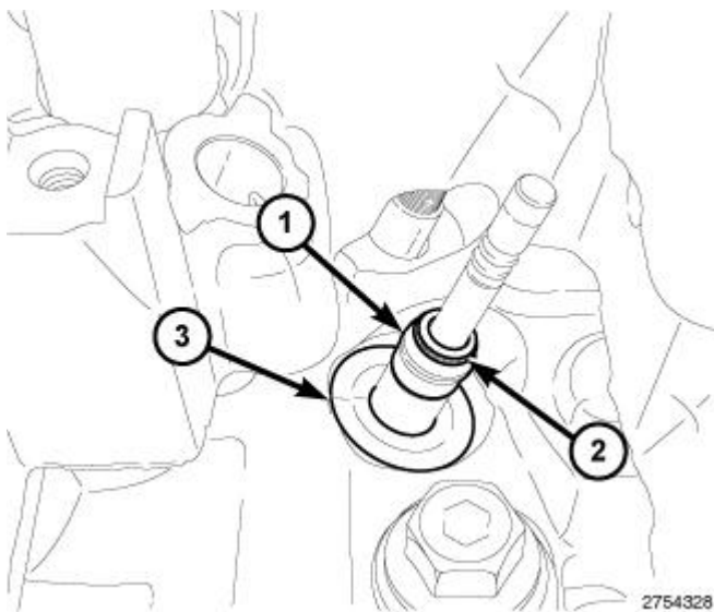
Fig. 358: Spring Seat, Valve Guide Seal & Garter Spring
