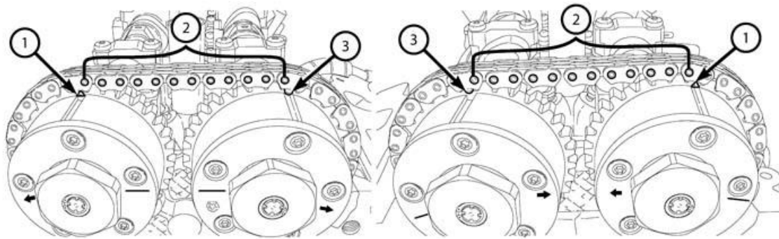
Fig. 686: Chain Pins, Exhaust Cam Phaser Triangle Marking & Circle Marking Courtesy of CHRYSLER GROUP, LLC
