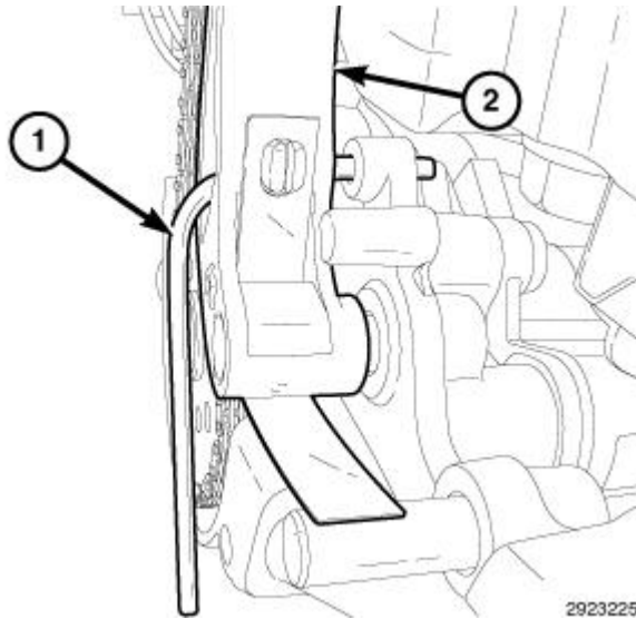
Fig. 607: Oil Pump Chain Tensioner & Retaining Pin
