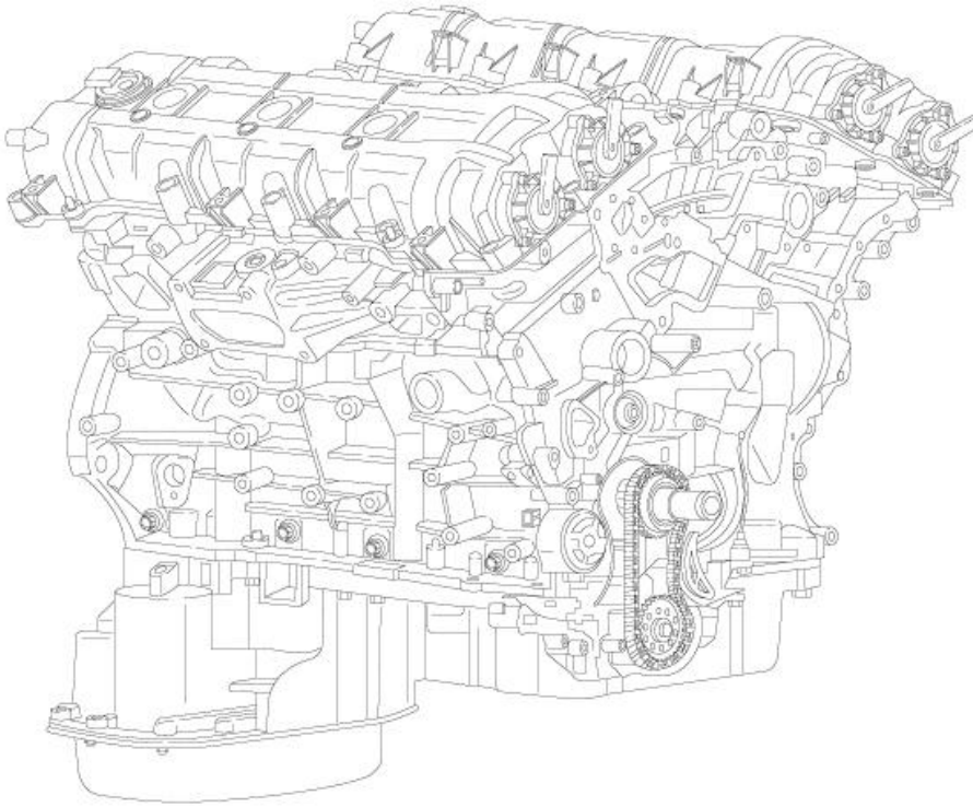
Fig. 522: 3.6L Engine
