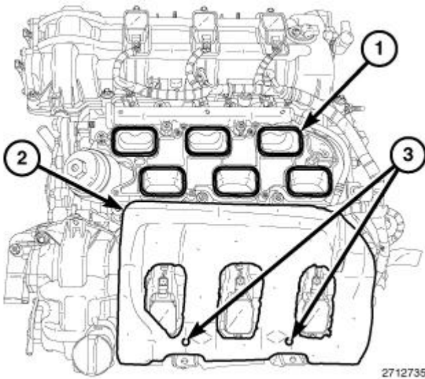
Fig. 329: Intake Ports, Insulator & Alignment Posts Courtesy of CHRYSLER GROUP, LLC
