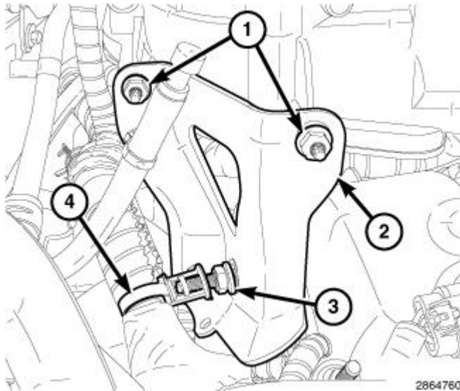
Fig. 640: Upper Intake Manifold Support Bracket, Stud & Fasteners Courtesy of CHRYSLER GROUP, LLC
