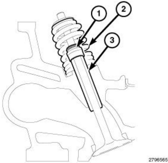
Fig. 339: Valve Stem Oil Seal, Valve Spring & Valve Guide Courtesy of CHRYSLER GROUP, LLC
