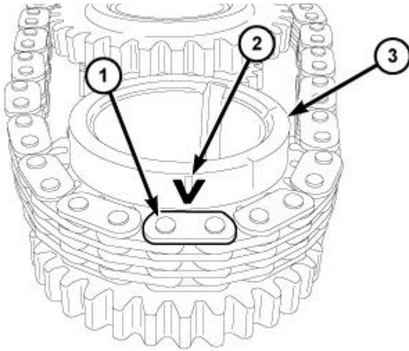
Fig. 702: Aligning Arrow With Plated Link On Primary Chain
