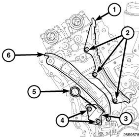
Fig. 698: Right Cam Chain Tensioner, Arm, Guide & Bolts Courtesy of CHRYSLER GROUP, LLC
