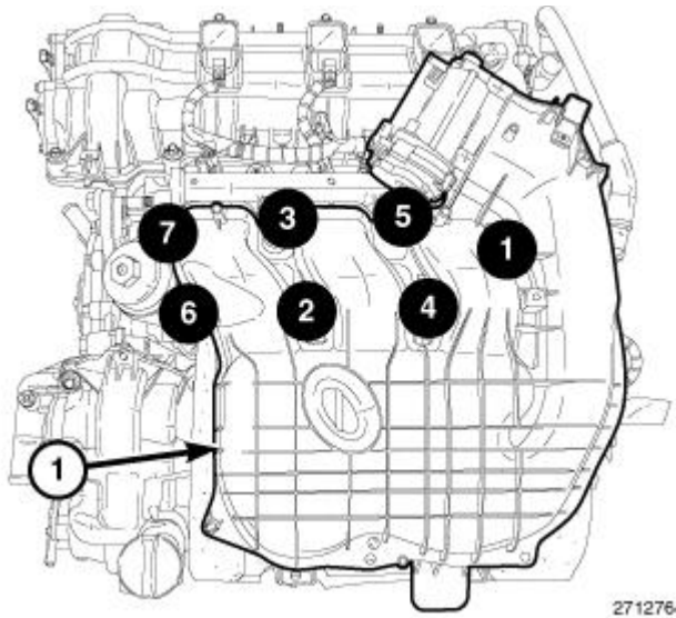
Fig. 670: Upper Intake Manifold Bolt Tightening Sequence Courtesy of CHRYSLER GROUP, LLC
