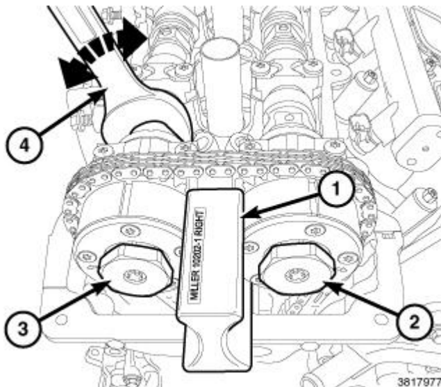
Fig. 690: Camshaft Phaser Lock, Oil Control Valves & Wrench
