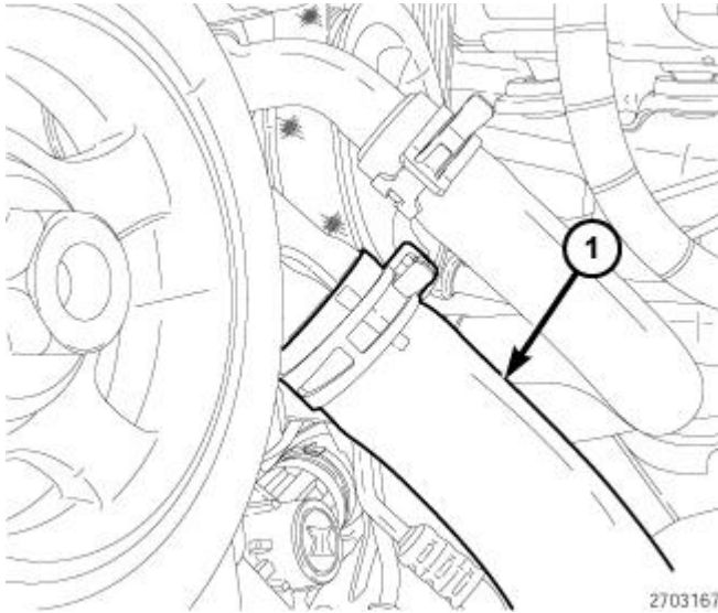
Fig. 29: Lower Radiator Hose Courtesy of CHRYSLER GROUP, LLC
