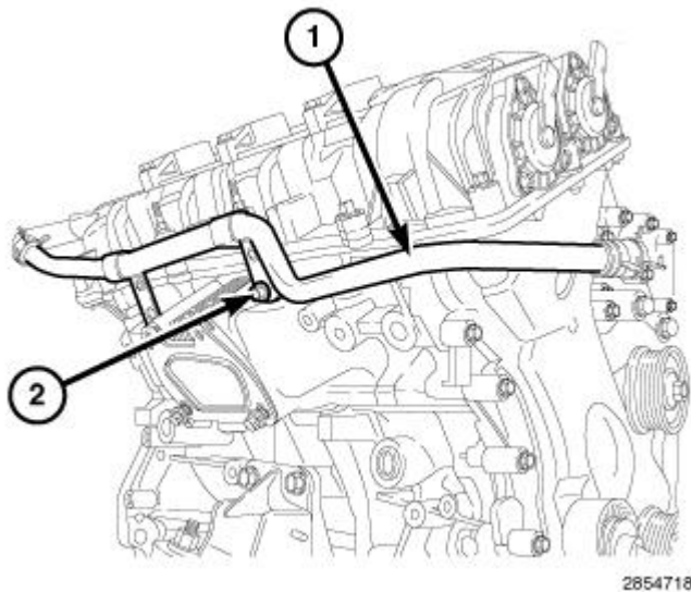
Fig. 734: Heater Core Supply Tube Support Bracket & Retaining Bolt Courtesy of CHRYSLER GROUP, LLC
