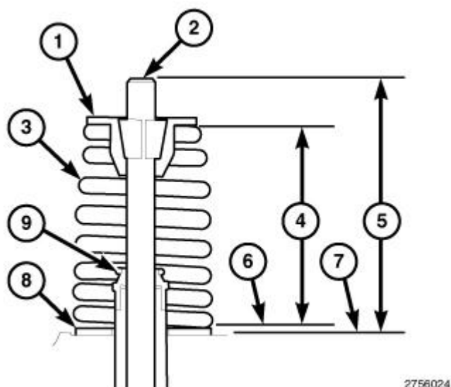
Fig. 387: Checking Valve Spring Installed Height Courtesy of CHRYSLER GROUP, LLC
