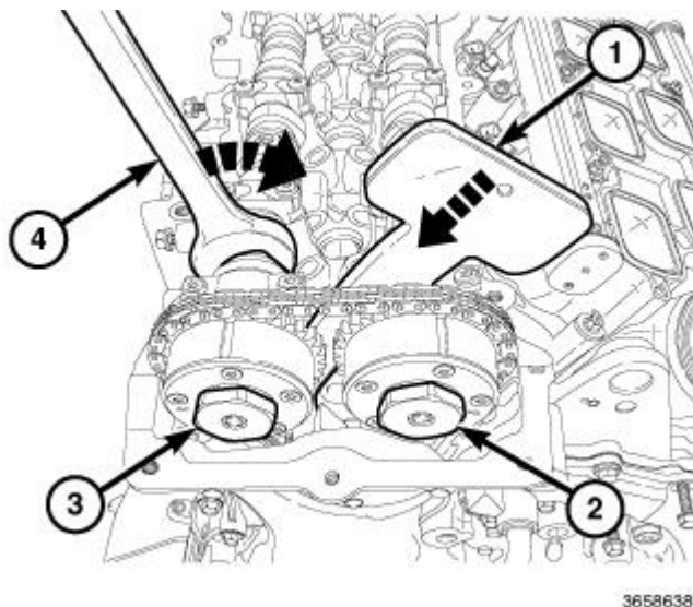
Fig. 253: Compressing Tensioner By Slightly Rotating Exhaust Camshaft Clockwise Courtesy of CHRYSLER GROUP, LLC
