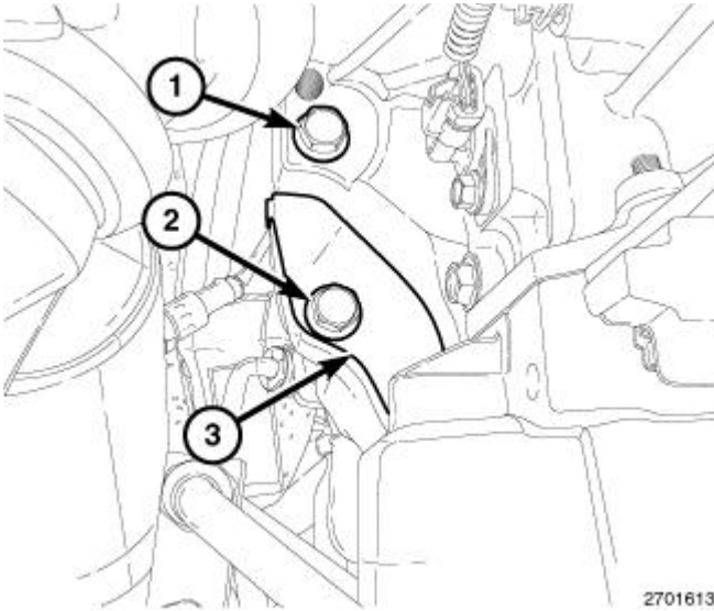
Fig. 525: Side Engine-To-Transmission Bolt, Transmission Dust Shield Retaining Bolt & Dust Shield Courtesy of CHRYSLER GROUP, LLC
