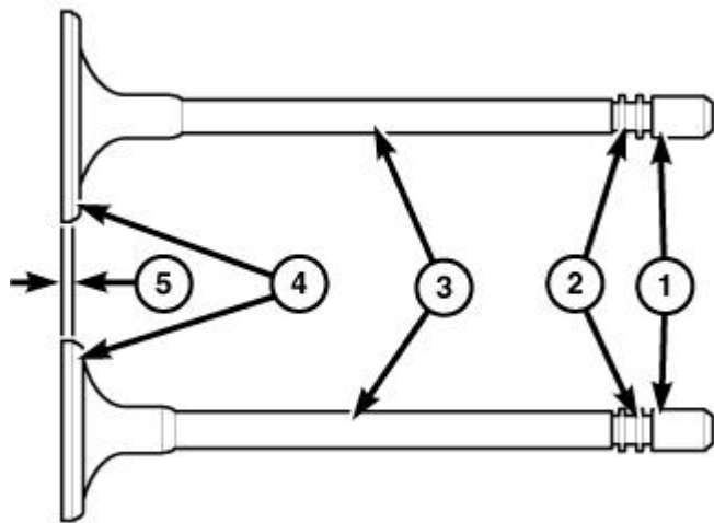
Fig. 384: Inspecting Valve Margin Courtesy of CHRYSLER GROUP, LLC
