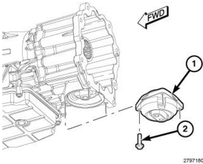
Fig. 519: Rear Engine Mount Isolator & Bolts (4x4) Courtesy of CHRYSLER GROUP, LLC
