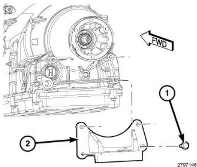
Fig. 516: Rear Engine Mount Bracket & Bolts (4x2) Courtesy of CHRYSLER GROUP, LLC
