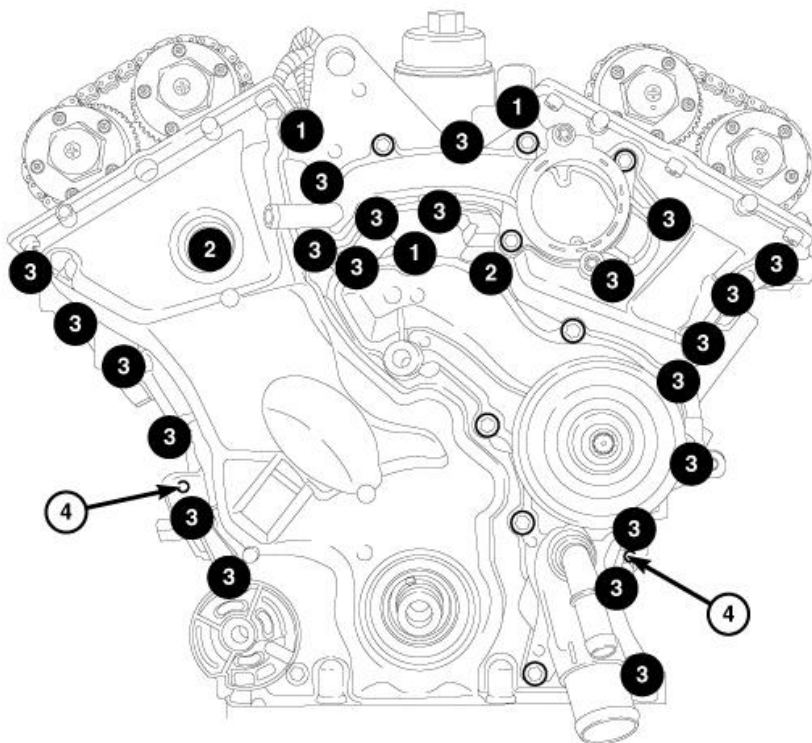
Fig. 722: Timing Cover Bolts Courtesy of CHRYSLER GROUP, LLC
