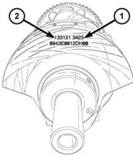
Fig. 403: Connecting Rod Bearing Journal Diameter Grade Markings Courtesy of CHRYSLER GROUP, LLC
