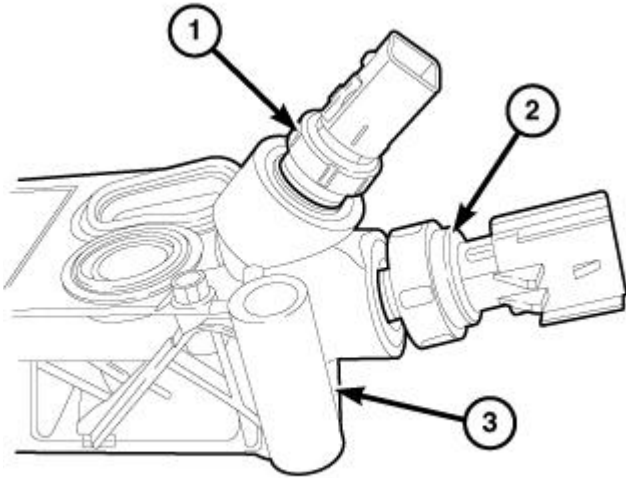
Fig. 624: Oil Temperature Sensor, Oil Pressure Sensor & Oil Filter Housing Courtesy of CHRYSLER GROUP, LLC
