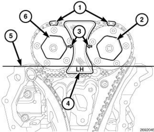
Fig. 706: Phaser Timing Marks, Oil Control Valves & LH Camshaft Phaser Lock Courtesy of CHRYSLER GROUP, LLC
