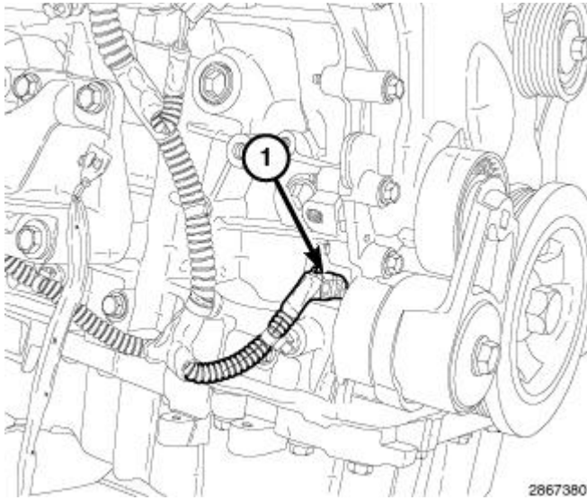
Fig. 617: Oil Pump Solenoid Electrical Connector Courtesy of CHRYSLER GROUP, LLC
