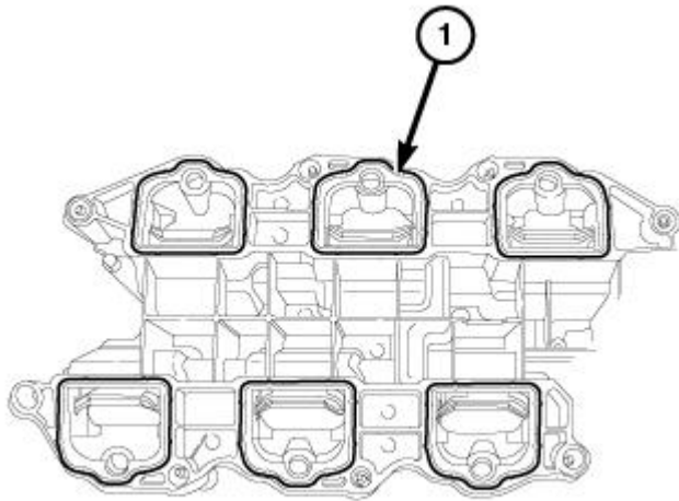
Fig. 664: Lower Intake Manifold To Cylinder Head Seals Courtesy of CHRYSLER GROUP, LLC
