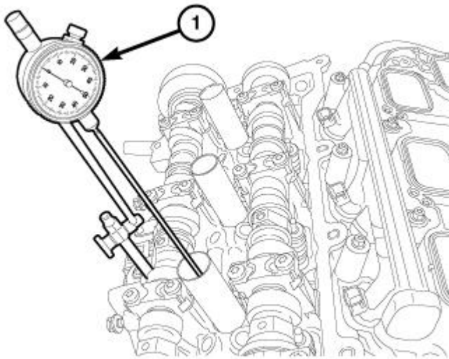
Fig. 236: Mount Dial Indicator Set To Stationary Point On Engine Courtesy of CHRYSLER GROUP, LLC
