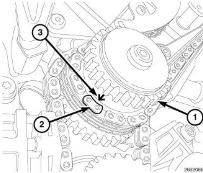
Fig. 168: Idler Sprocket, Plated Link & Arrow Courtesy of CHRYSLER GROUP, LLC
