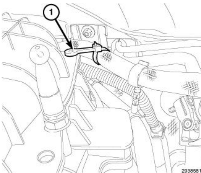
Fig. 661: Brake Booster Hose Retainer Courtesy of CHRYSLER GROUP, LLC
