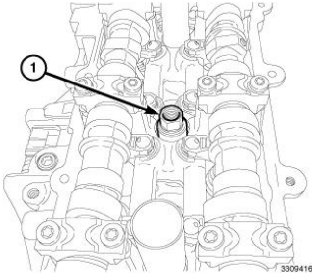
Fig. 372: Spark Plug Tube Installer Courtesy of CHRYSLER GROUP, LLC
