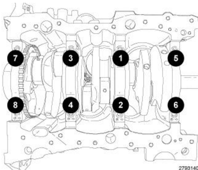
Fig. 430: Inner Main Bearing Cap Bolts Tightening Sequence
