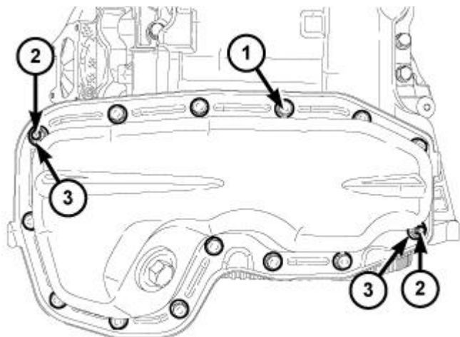
Fig. 580: Lower Oil Pan & Fasteners Courtesy of CHRYSLER GROUP, LLC
