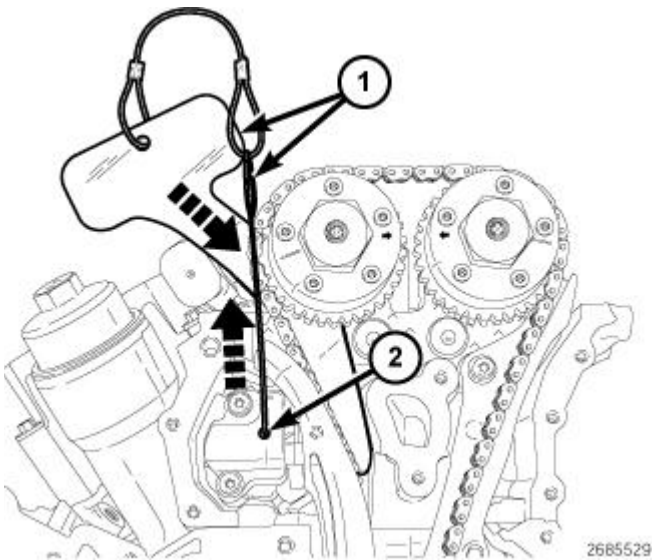
Fig. 677: Pin, Rack & Timing Chain Holder Courtesy of CHRYSLER GROUP, LLC
