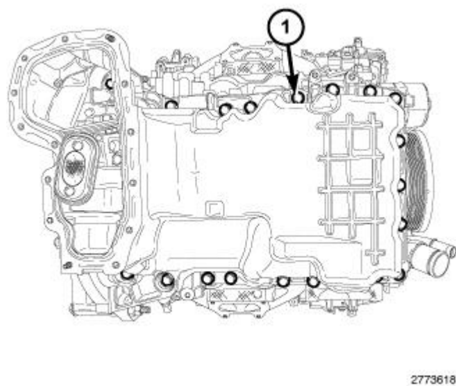
Fig. 575: Oil Pan Mounting Bolts Courtesy of CHRYSLER GROUP, LLC
