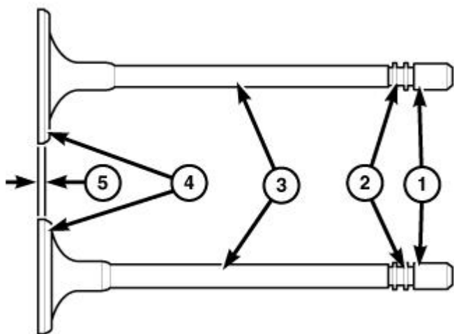
Fig. 378: Inspecting Valve Margin
