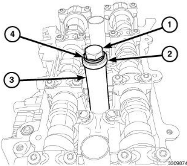
Fig. 374: Spark Plug Tube, Thrust Washers, Spark Plug Tube Installer & Bolt Courtesy of CHRYSLER GROUP, LLC
