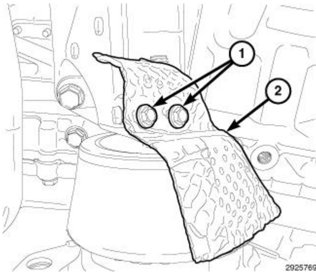
Fig. 508: Engine Mount Heatshield & Bolts
