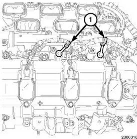
Fig. 278: Injection/Ignition Harness Retainers
