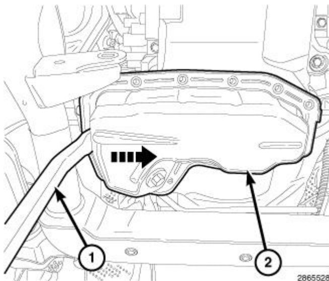
Fig. 563: Removing Lower Oil Pan Courtesy of CHRYSLER GROUP, LLC
