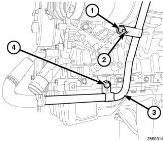
Fig. 347: Heater Core Return Tube, Nut & Bolt Courtesy of CHRYSLER GROUP, LLC
