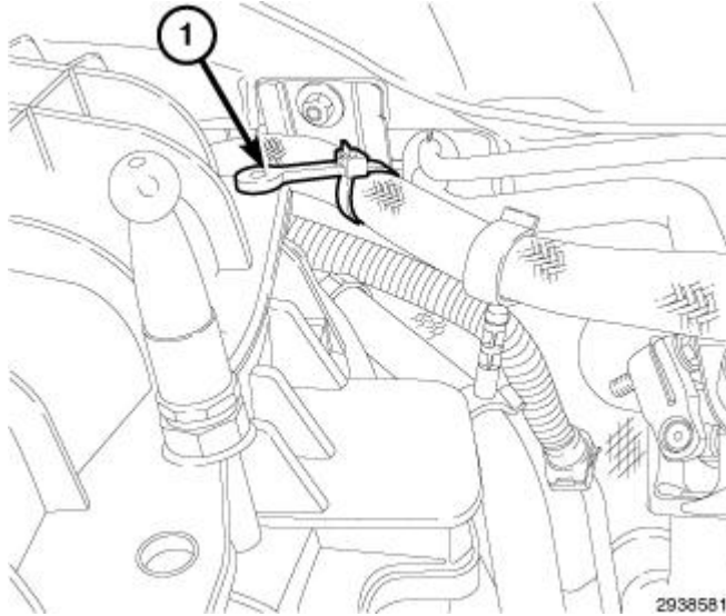
Fig. 638: Brake Booster Hose Retainer Courtesy of CHRYSLER GROUP, LLC
