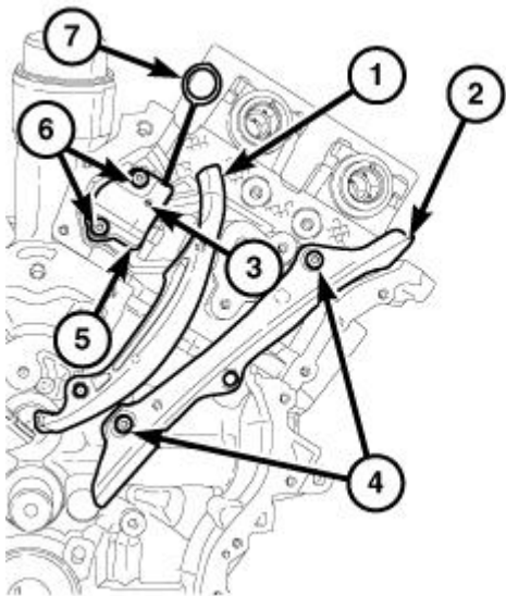
Fig. 694: Left Cam Chain Tensioner, Arm, Guide & Bolts Courtesy of CHRYSLER GROUP, LLC
