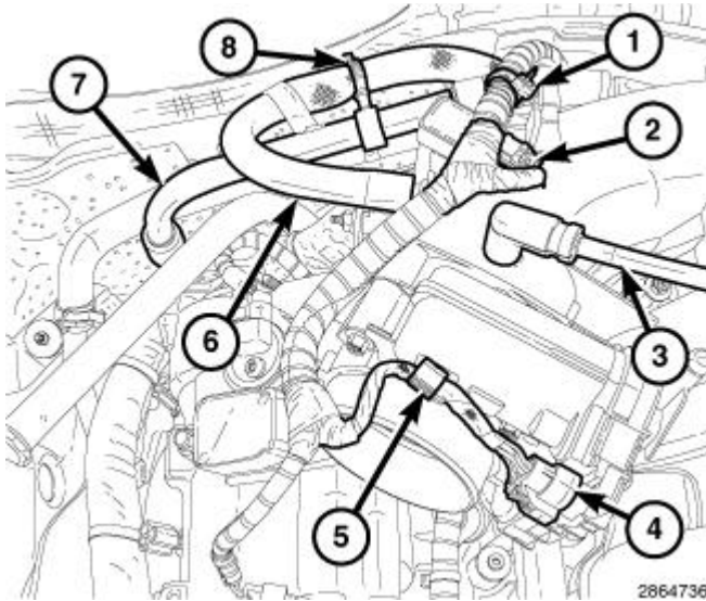
Fig. 660: MAP Sensor, ETC, PCV Hose, Brake Booster Vacuum Hose, EVAP Vapor Purge Line, Clip & Wire Harness Retainer Courtesy of CHRYSLER GROUP, LLC
