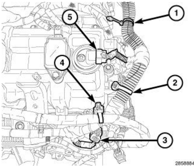
Fig. 129: ECT Sensor Connector, CMP Sensor & Main Wire Harness Retainers Courtesy of CHRYSLER GROUP, LLC
