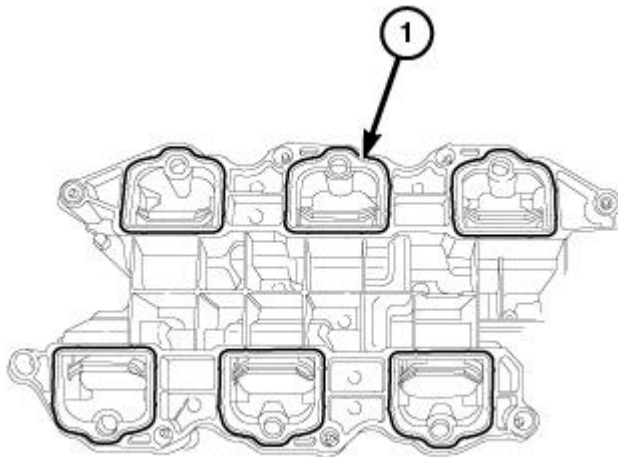
Fig. 650: Lower Intake Manifold To Cylinder Head Seals Courtesy of CHRYSLER GROUP, LLC
