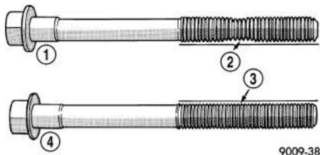
Fig. 163: Checking Cylinder Head Bolts For Stretching (Necking)
