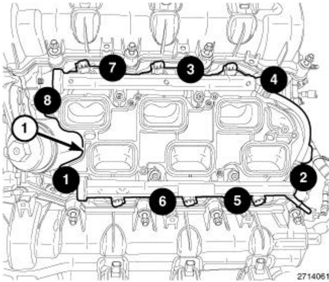
Fig. 666: Intake Manifold Retaining Bolts Tightening Sequence Courtesy of CHRYSLER GROUP, LLC
