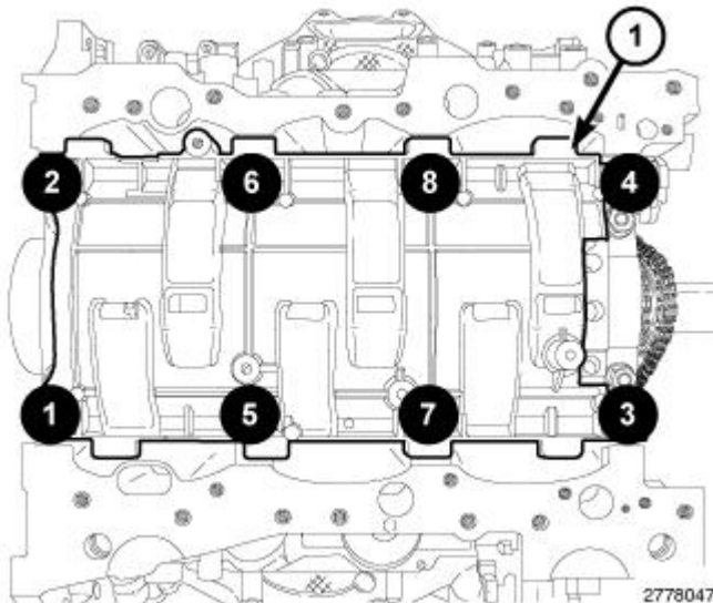
Fig. 418: Main Bearing Cap Bolts From Windage Tray Removal Sequence Courtesy of CHRYSLER GROUP, LLC
