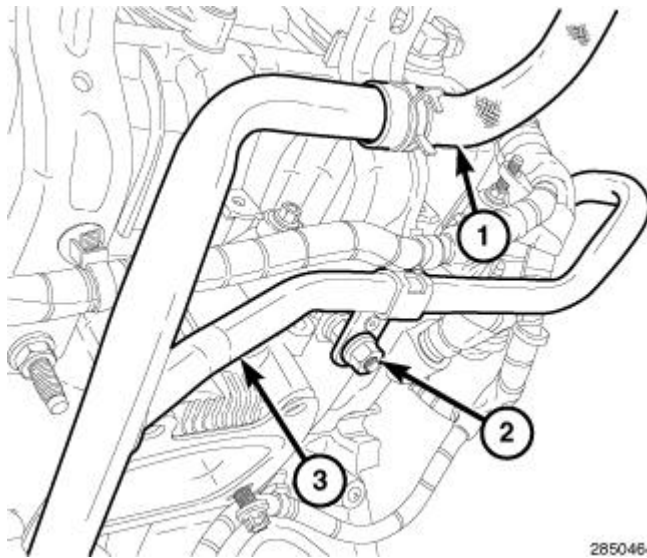
Fig. 659: Heater Core Return Hose, Heater Core Return Tube & Nut Courtesy of CHRYSLER GROUP, LLC
