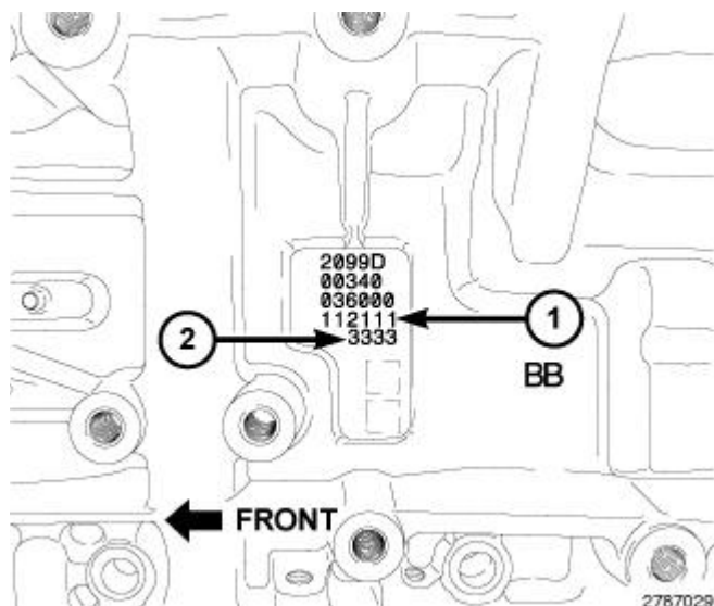
Fig. 404: Engine Block Main Bearing Journal Diameter Grade Markings
