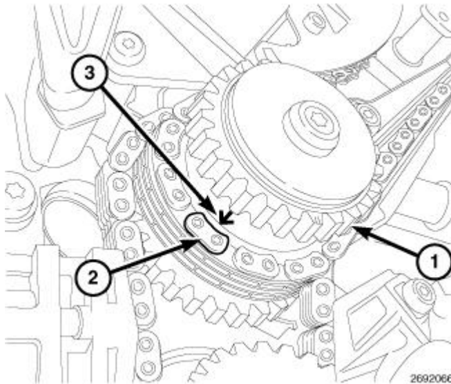
Fig. 707: Idler Sprocket, Plated Link & Arrow Courtesy of CHRYSLER GROUP, LLC
