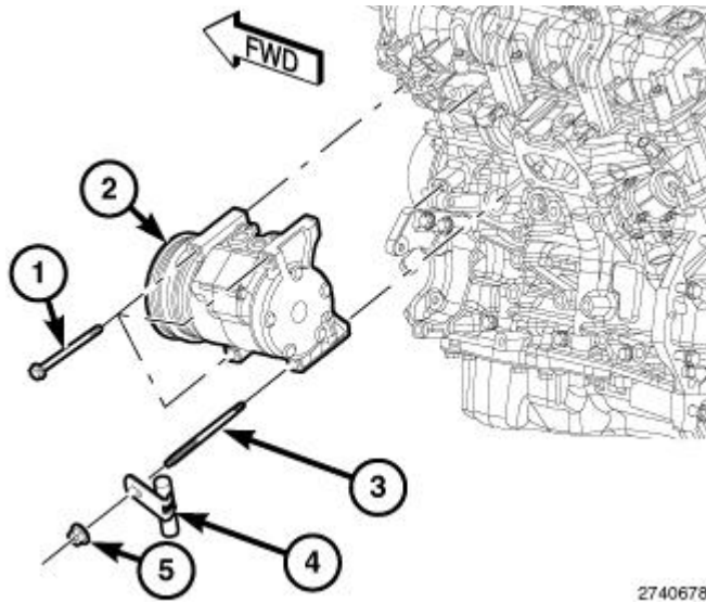
Fig. 128: A/C Compressor, Nut, Stud & Three Bolts Courtesy of CHRYSLER GROUP, LLC
