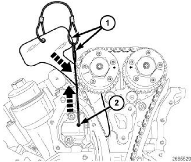
Fig. 247: Pin, Rack & Timing Chain Holder
