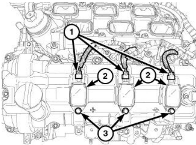
Fig. 292: Electrical Connector, Ignition Coils & Ignition Coil Retaining Bolts Courtesy of CHRYSLER GROUP, LLC
