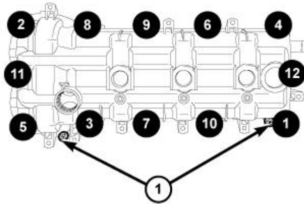
Fig. 303: Cylinder Head Cover Bolts & Double Ended Studs Tightening Sequence - Left Courtesy of CHRYSLER GROUP, LLC
