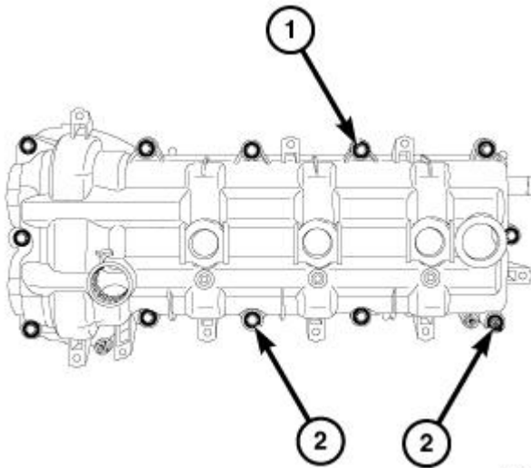
Fig. 732: Cylinder Head Cover Mounting Bolts & Studbolts Courtesy of CHRYSLER GROUP, LLC
