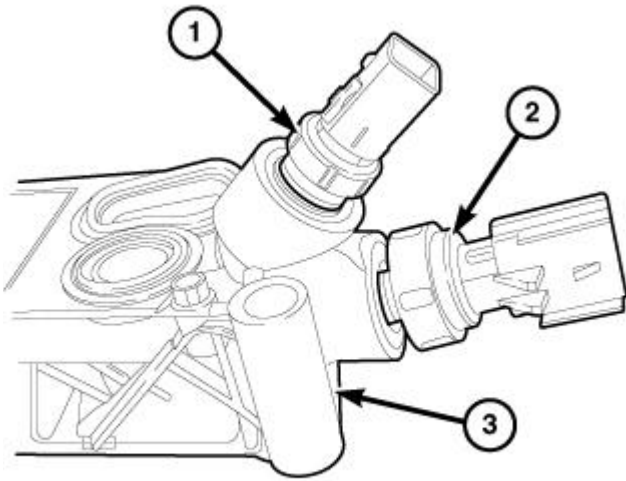
Fig. 626: Oil Temperature Sensor, Oil Pressure Sensor & Oil Filter Housing Courtesy of CHRYSLER GROUP, LLC
