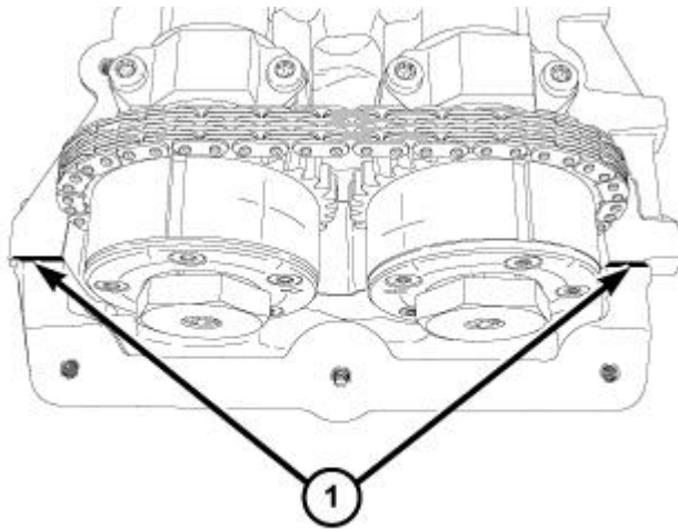
Fig. 298: RTV Sealant Locations Courtesy of CHRYSLER GROUP, LLC
