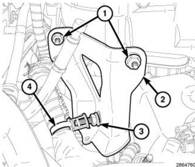
Fig. 657: Upper Intake Manifold Support Bracket, Stud & Fasteners Courtesy of CHRYSLER GROUP, LLC
