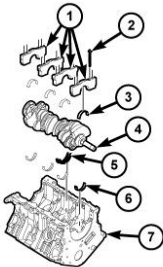
Fig. 426: Main Bearing Caps, Bolts, Crankshaft & Engine Block
