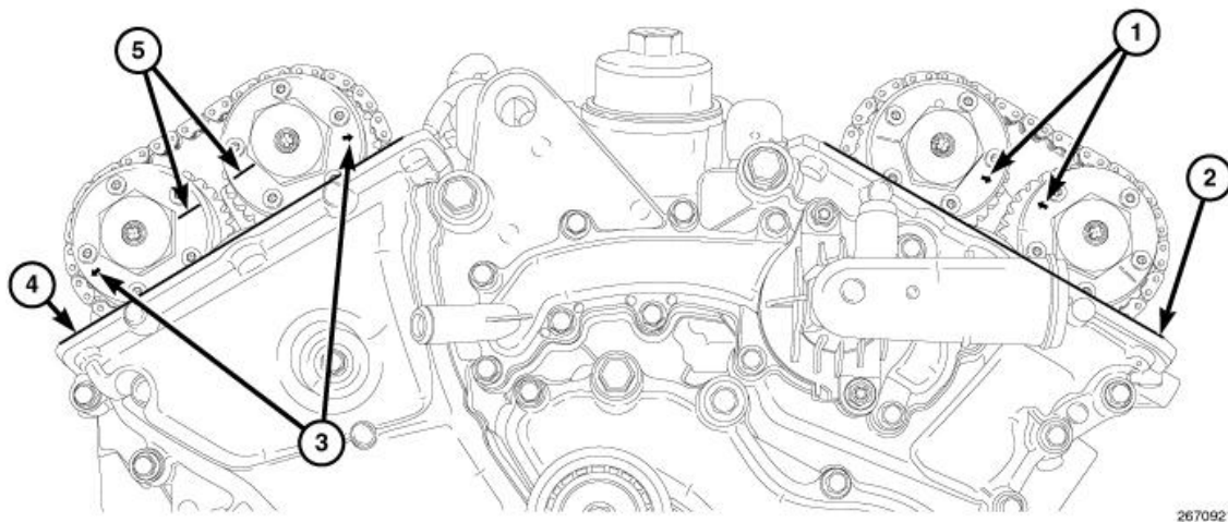
Fig. 682: Arrows, Scribe Lines, & Cam Phasers Courtesy of CHRYSLER GROUP, LLC
