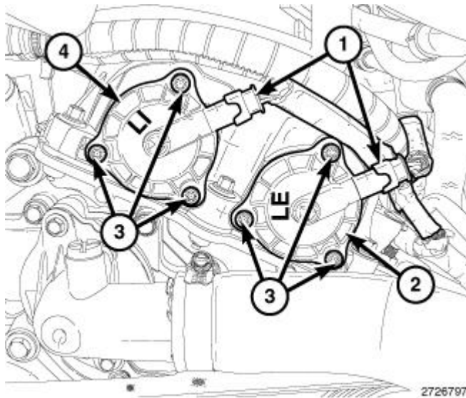
Fig. 306: Variable Valve Timing Solenoids, Connectors & Bolts Courtesy of CHRYSLER GROUP, LLC
