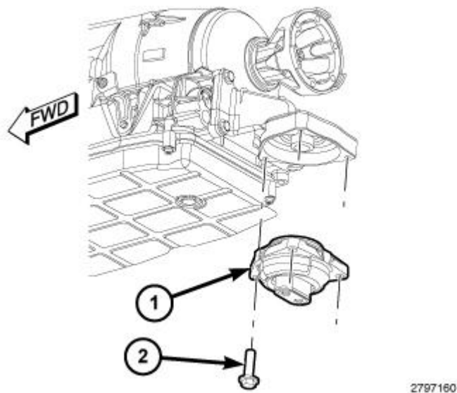
Fig. 515: Rear Engine Mount Isolator & Bolts (4x2) Courtesy of CHRYSLER GROUP, LLC
