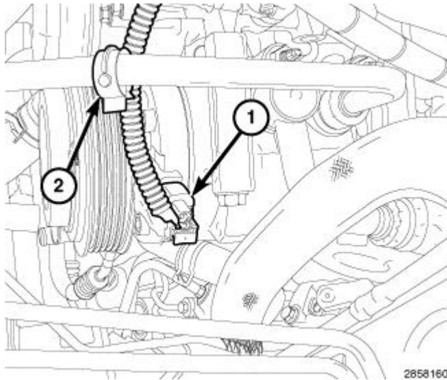
Fig. 177: A/C Compressor Electrical Connector & Wire Harness Retainer Courtesy of CHRYSLER GROUP, LLC
