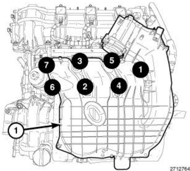
Fig. 511: Upper Intake Manifold Bolt Tightening Sequence Courtesy of CHRYSLER GROUP, LLC
