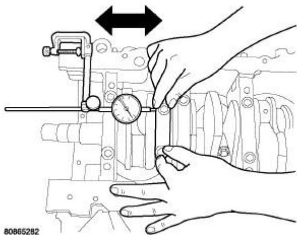
Fig. 455: Measuring Connecting Rod Side Clearance Courtesy of CHRYSLER GROUP, LLC
