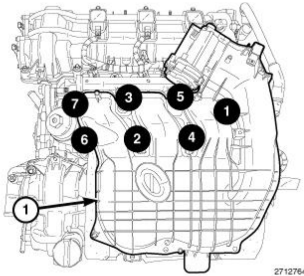
Fig. 313: Upper Intake Manifold Bolt Tightening Sequence
