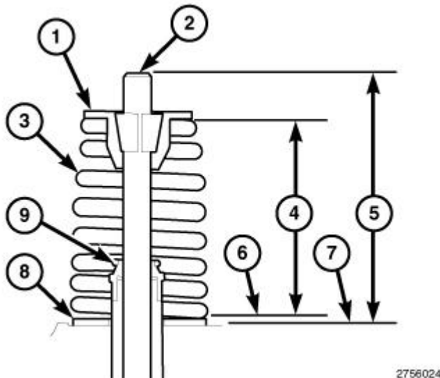
Fig. 383: Checking Valve Spring Installed Height Courtesy of CHRYSLER GROUP, LLC
