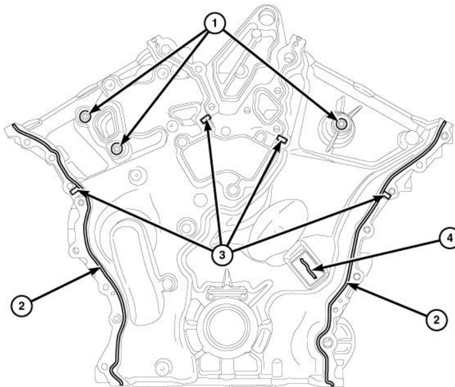
Fig. 729: Sealant At Cylinder Head Bosses, Right & Left Flanges, Cylinder Head-To-Engine Block T-Joints & Cover To Right Cam Chain Tensioner Gap Courtesy of CHRYSLER GROUP, LLC
