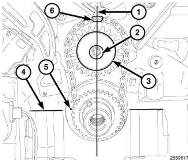
Fig. 693: Timing Chain Plated Link At 12 O'Clock, Washer, Retaining Bolt, Block/Bearing Cap Junction & Dimple Courtesy of CHRYSLER GROUP, LLC
