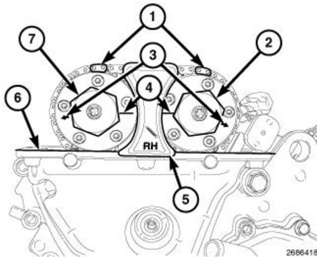
Fig. 350: Phaser Timing Marks, Oil Control Valves & RH Camshaft Phaser Lock Courtesy of CHRYSLER GROUP, LLC
