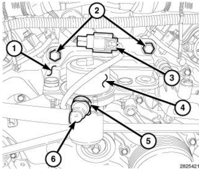
Fig. 119: Mounting Bracket, Bolts, Electrical Connector, Vacuum Pump, Locking Tab & Quick-Connect Type End
