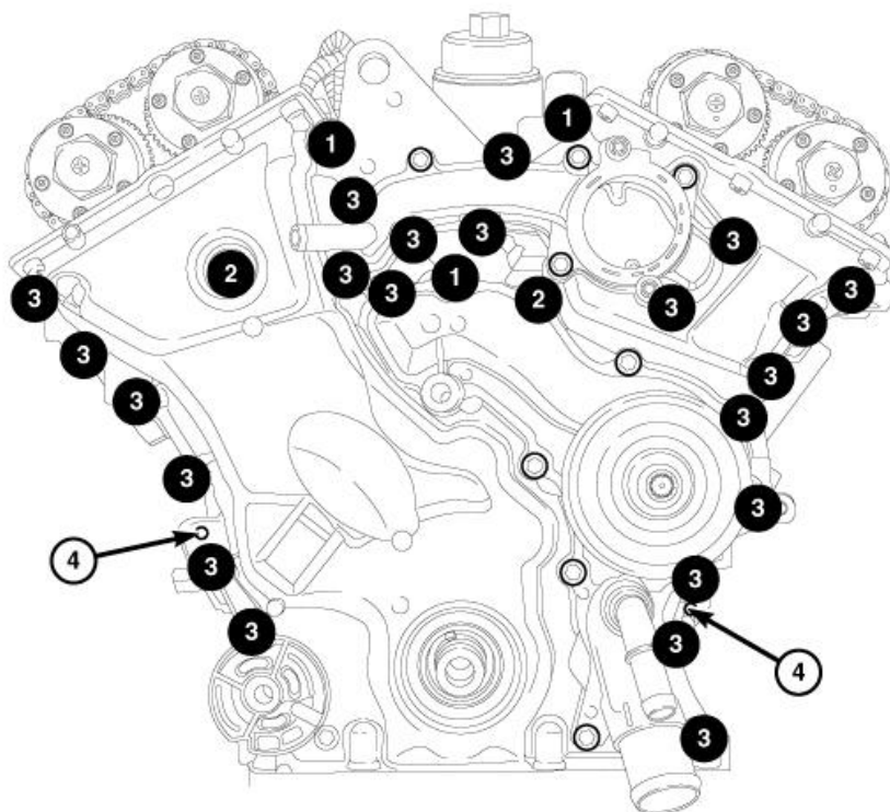
Fig. 730: Timing Cover Bolts Courtesy of CHRYSLER GROUP, LLC
