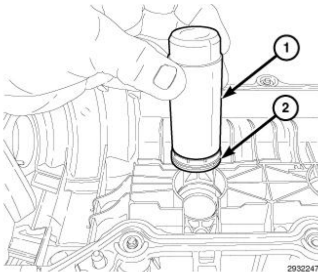
Fig. 316: Spark Plug Tube Seal & Installer
