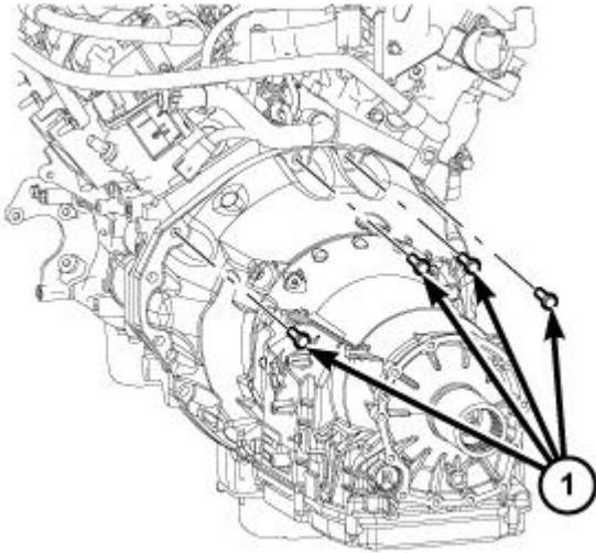
Fig. 70: Upper Transmission Engine Bolts
