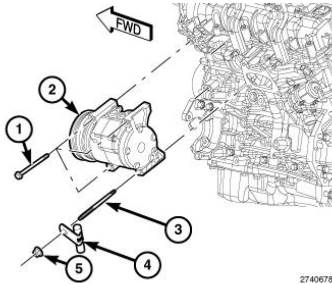
Fig. 176: A/C Compressor, Nut, Stud & Three Bolts Courtesy of CHRYSLER GROUP, LLC
