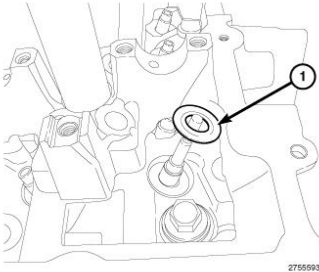
Fig. 341: Valve Spring Seat
