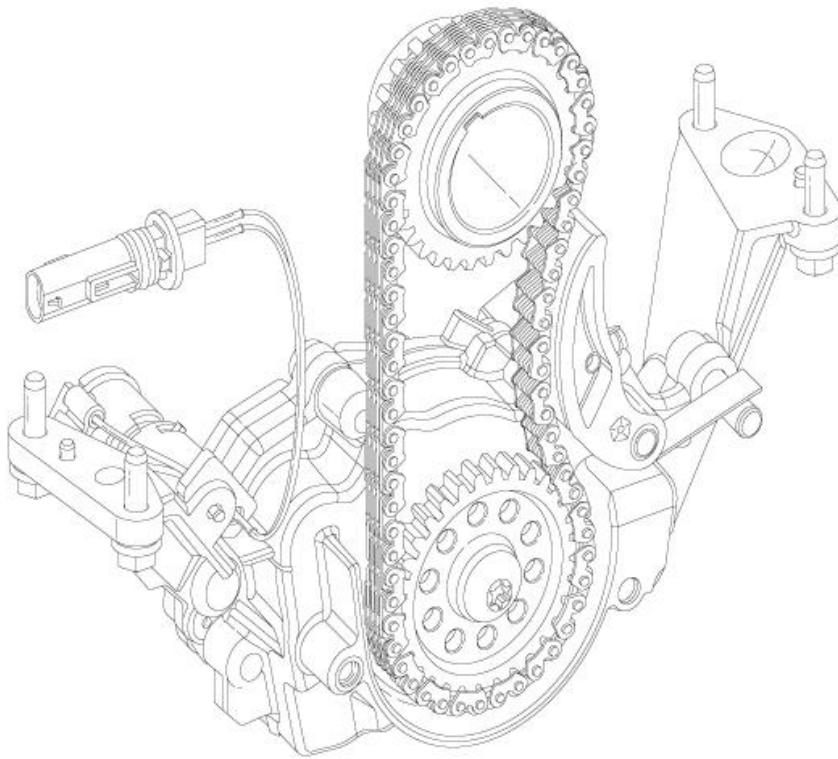
Fig. 599: Oil Pump Chain
