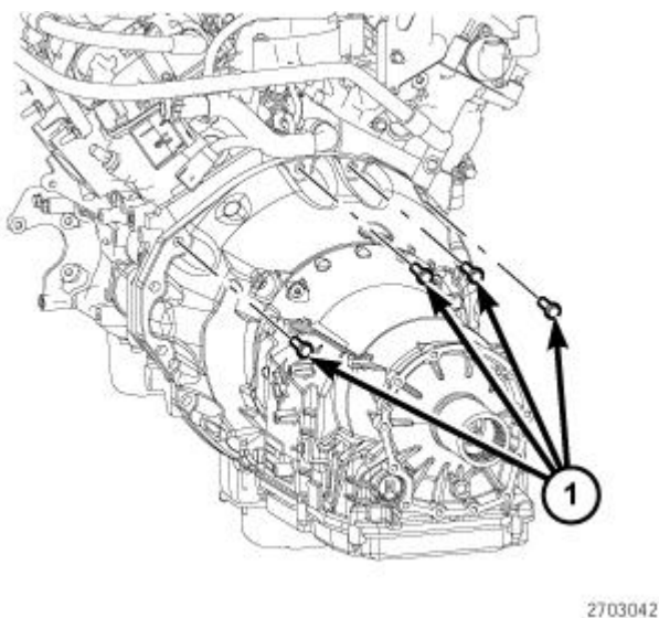
Fig. 40: Upper Transmission Engine Bolts Courtesy of CHRYSLER GROUP, LLC
