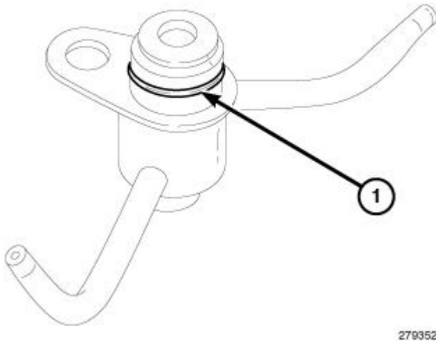
Fig. 552: Piston Oil Cooler Jet O-Ring Seal Courtesy of CHRYSLER GROUP, LLC
