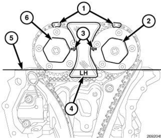
Fig. 248: Phaser Timing Marks, Oil Control Valves & LH Camshaft Phaser Lock
