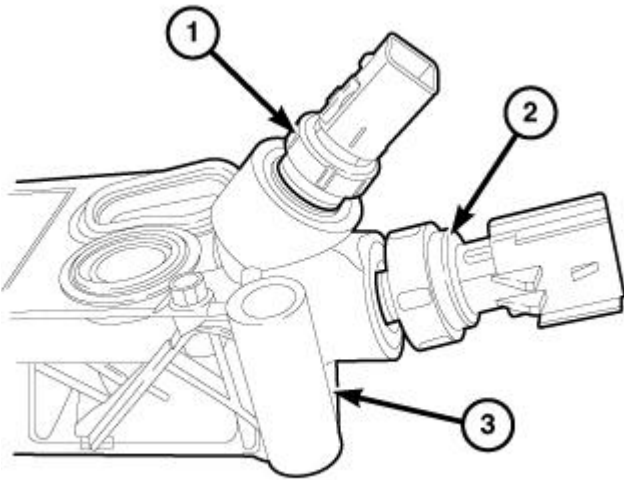
Fig. 631: Oil Temperature Sensor, Oil Pressure Sensor & Oil Filter Housing Courtesy of CHRYSLER GROUP, LLC
