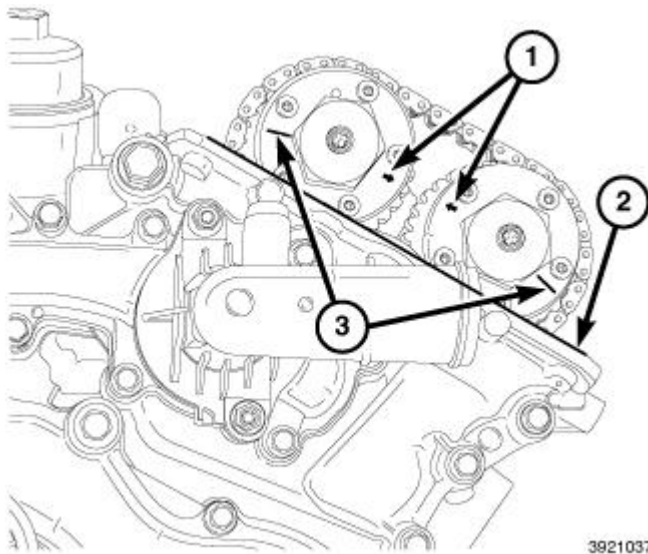
Fig. 246: Arrows, Scribe Lines & Cylinder Head Cover Mounting Surface Courtesy of CHRYSLER GROUP, LLC
