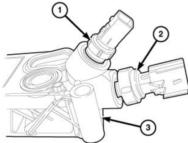
Fig. 623: Oil Temperature Sensor, Oil Pressure Sensor & Oil Filter Housing Courtesy of CHRYSLER GROUP, LLC
