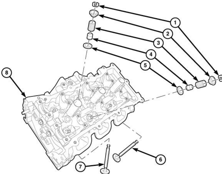
Fig. 376: Intake Valve & Exhaust Valve Component Configuration Courtesy of CHRYSLER GROUP, LLC
