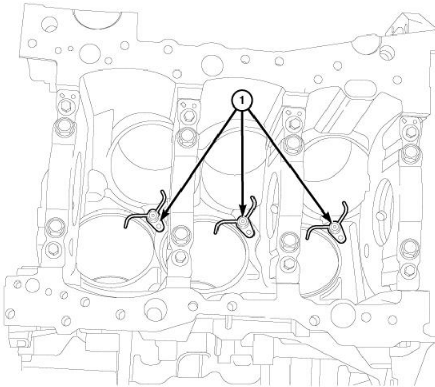
Fig. 549: Engine Blocked-Mounted Oil Jets Courtesy of CHRYSLER GROUP, LLC
