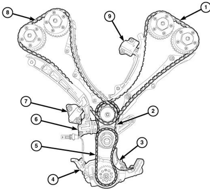
Fig. 671: Valve Timing System Components Courtesy of CHRYSLER GROUP, LLC
