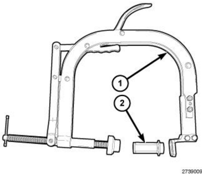
Fig. 353: Valve Spring Compressor Components Courtesy of CHRYSLER GROUP, LLC
