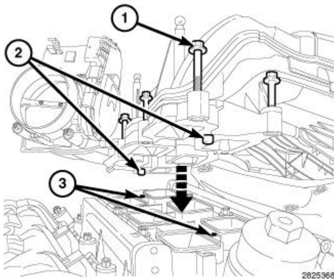
Fig. 655: Upper Intake Attaching Bolts, Locating Posts & Holes Courtesy of CHRYSLER GROUP, LLC
