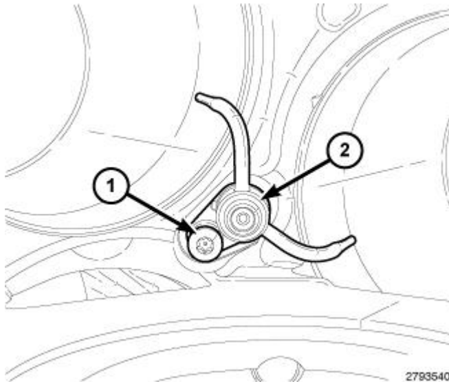
Fig. 553: Piston Oil Cooler Jet & Bolt Courtesy of CHRYSLER GROUP, LLC
