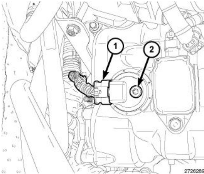
Fig. 290: CMP Sensor & Bolt Courtesy of CHRYSLER GROUP, LLC
