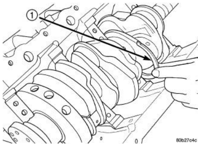
Fig. 427: Thrust Washer Installation Courtesy of CHRYSLER GROUP, LLC
