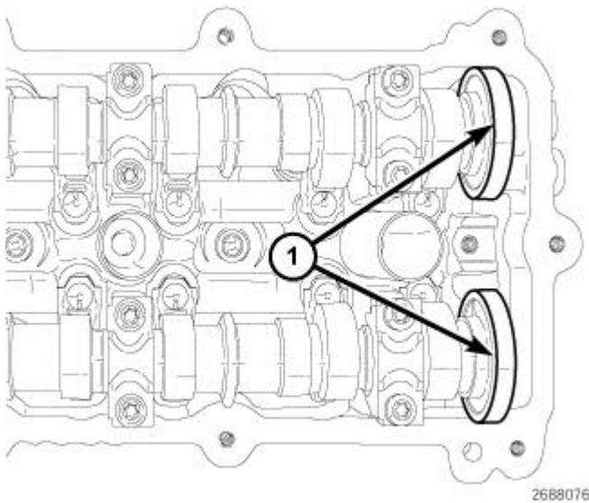
Fig. 299: Magnetic Timing Wheels Courtesy of CHRYSLER GROUP, LLC
