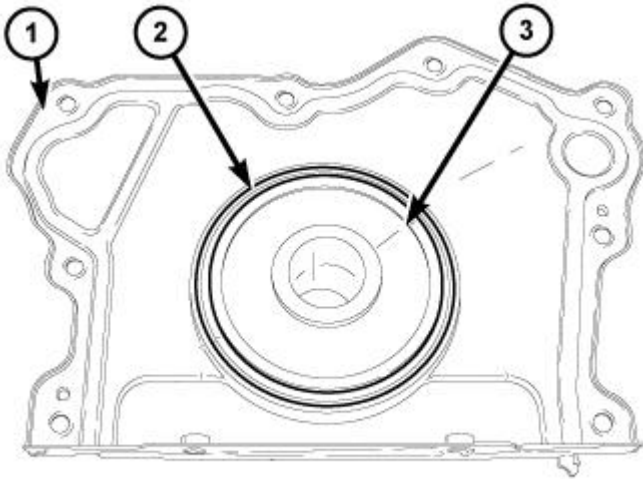
Fig. 474: Rear Crankshaft Oil Seal, Retainer & Seal Protector Courtesy of CHRYSLER GROUP, LLC
