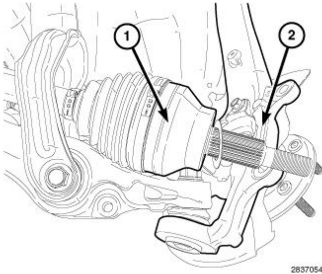
Fig. 505: Knuckle & Push Half Shaft Courtesy of CHRYSLER GROUP, LLC
