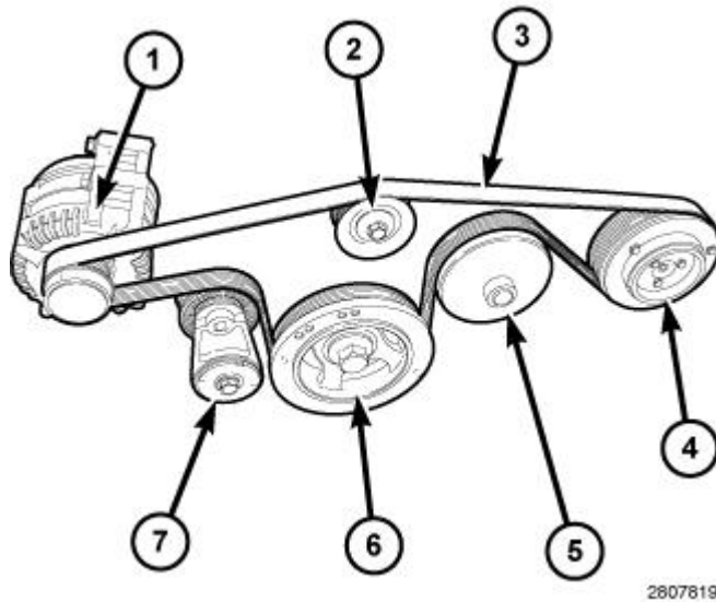
Fig. 733: Idler Pulley, Tensioner Arm, Belt, Idler, Tensioner & Belt Routing Courtesy of CHRYSLER GROUP, LLC
