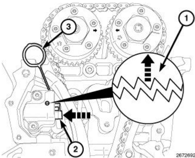
Fig. 688: Resetting Left Cam Chain Tensioner Courtesy of CHRYSLER GROUP, LLC
