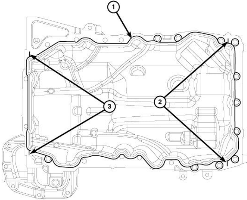
Fig. 581: Mopar® Threebond Engine RTV Sealant Locations Courtesy of CHRYSLER GROUP, LLC
