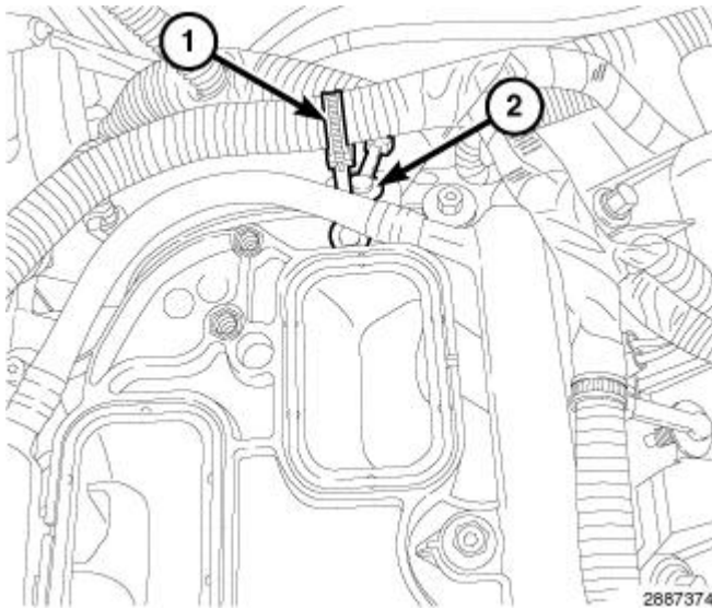
Fig. 648: Injection/Ignition Harness Retainer & Main Wire Harness Retainer
