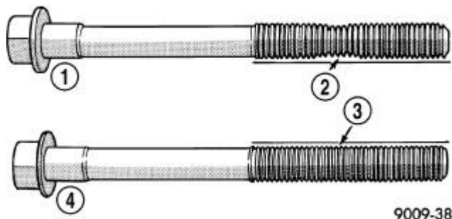
Fig. 428: Checking Cylinder Head Bolts For Stretching (Necking) Courtesy of CHRYSLER GROUP, LLC
