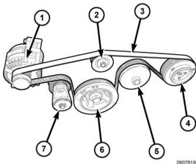
Fig. 719: Idler Pulley, Tensioner Arm, Belt, Idler, Tensioner & Belt Routing Courtesy of CHRYSLER GROUP, LLC
