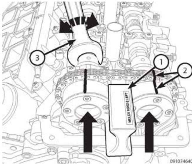
Fig. 261: Marks On Timing Chain Courtesy of CHRYSLER GROUP, LLC
