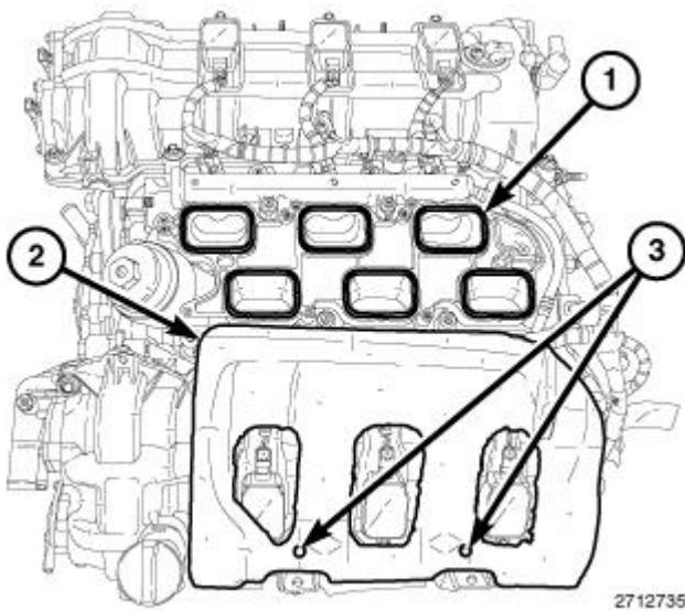
Fig. 654: Intake Ports, Insulator & Alignment Posts Courtesy of CHRYSLER GROUP, LLC
