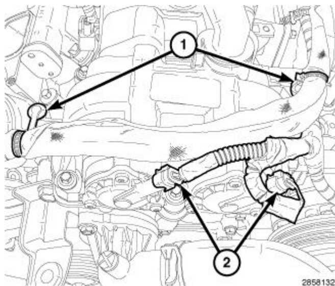
Fig. 87: Variable Valve Timing Solenoid Connectors & Wire Harness Retainers
