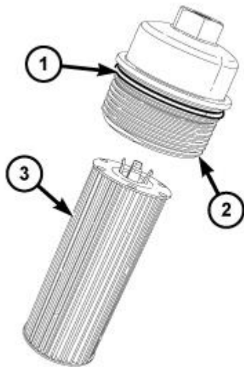
Fig. 557: O-Ring Seal, Oil Filter Cap & Oil Filter
