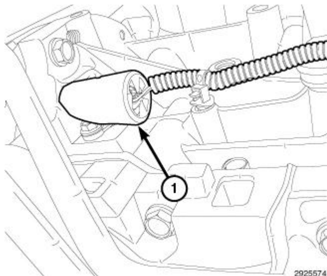
Fig. 78: Heat Shield
