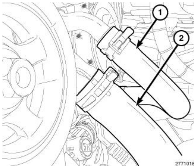
Fig. 716: Radiator Hose & Heater Hose Courtesy of CHRYSLER GROUP, LLC
