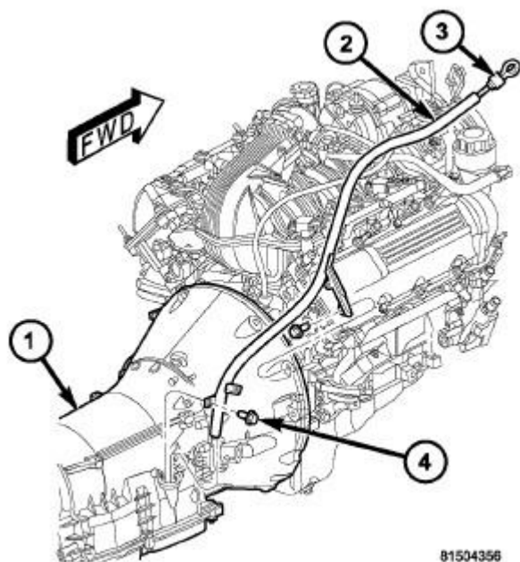
Fig. 362: Transmission Fluid Level Indicator Tube Assembly Courtesy of CHRYSLER GROUP, LLC
