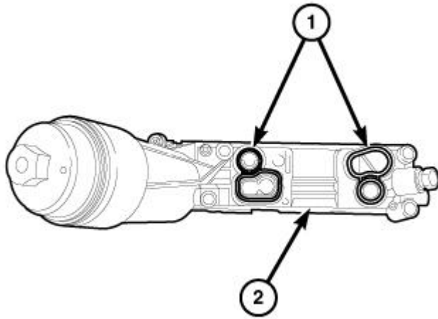
Fig. 545: Oil Cooler Seals & Oil Filter Housing Courtesy of CHRYSLER GROUP, LLC
