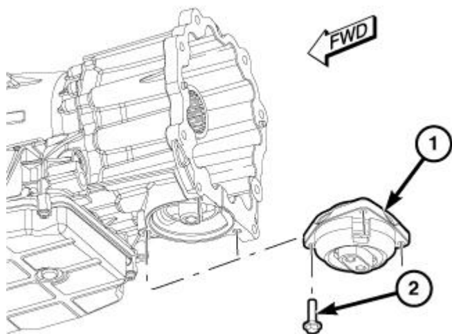
Fig. 514: Rear Engine Mount Isolator & Bolts (4x4)
