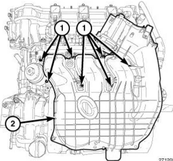
Fig. 284: Upper Intake Manifold & Bolts
