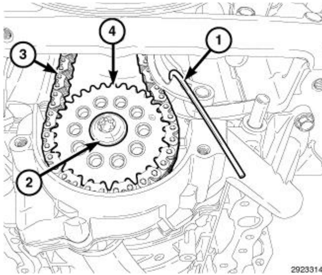
Fig. 614: Retaining Pin, Retaining Bolt, Oil Pump Chain & Sprocket Courtesy of CHRYSLER GROUP, LLC
