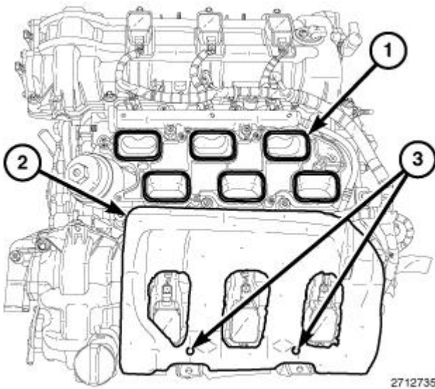
Fig. 669: Intake Ports, Insulator & Alignment Posts Courtesy of CHRYSLER GROUP, LLC
