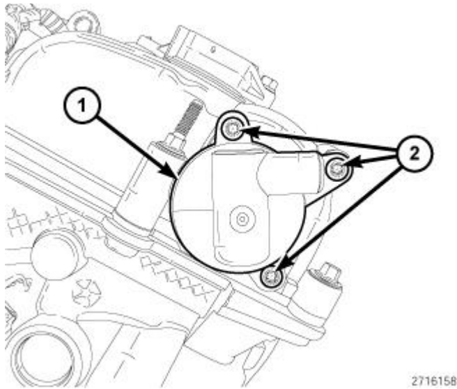
Fig. 326: Three Screws & PCV Valve Courtesy of CHRYSLER GROUP, LLC
