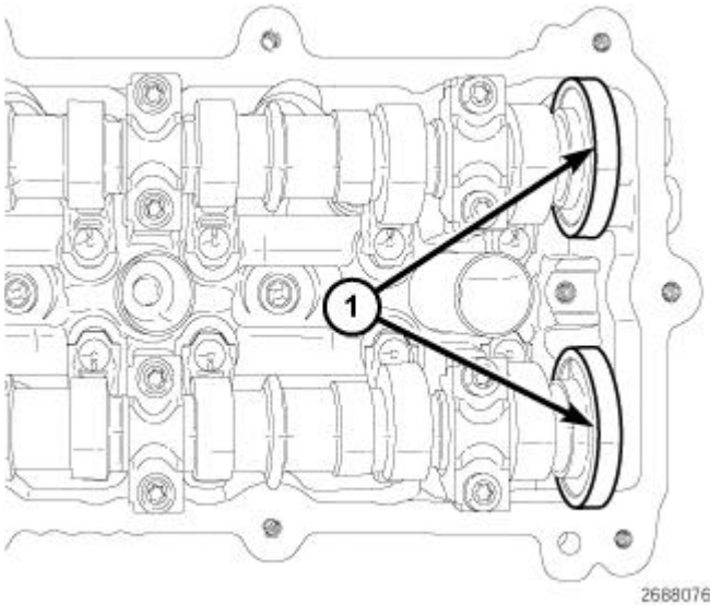
Fig. 258: Magnetic Timing Wheels
