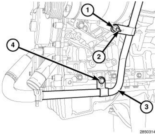
Fig. 487: Heater Core Return Tube, Nut & Bolt Courtesy of CHRYSLER GROUP, LLC
