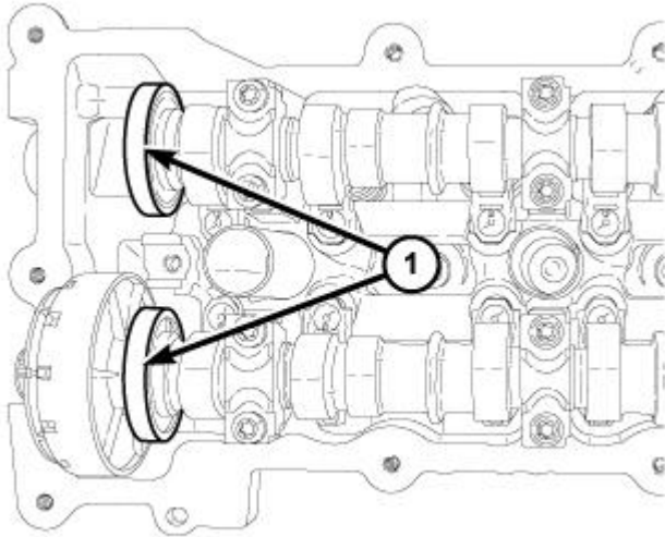
Fig. 283: Magnetic Timing Wheels
