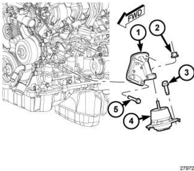
Fig. 485: Engine Mount Isolator, Left Engine Mount Bracket & Retaining Bolts Courtesy of CHRYSLER GROUP, LLC
