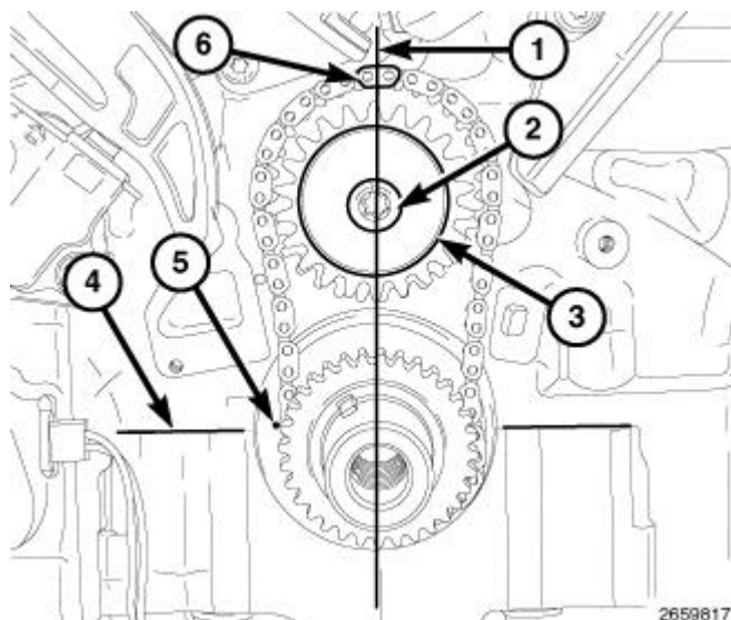
Fig. 704: Timing Chain Plated Link At 12 O'Clock, Washer, Retaining Bolt, Block/Bearing Cap Junction & Dimple
