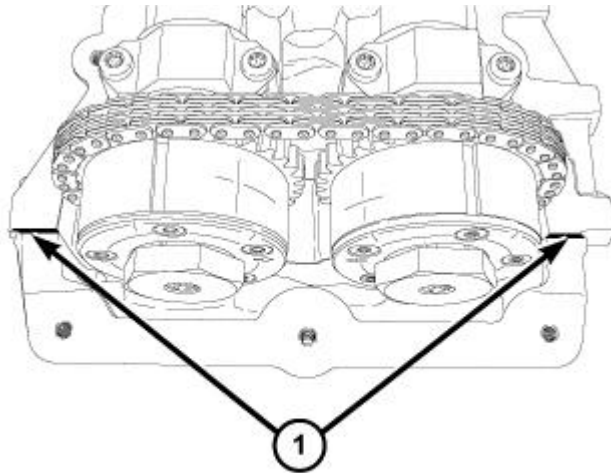
Fig. 302: RTV Sealant Locations
