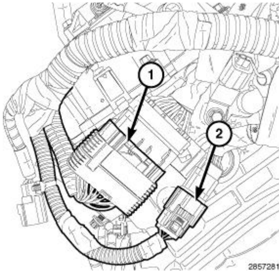
Fig. 41: Engine Injection/Ignition Harness & Engine Oil Pressure/Temperature Harness Courtesy of CHRYSLER GROUP, LLC
