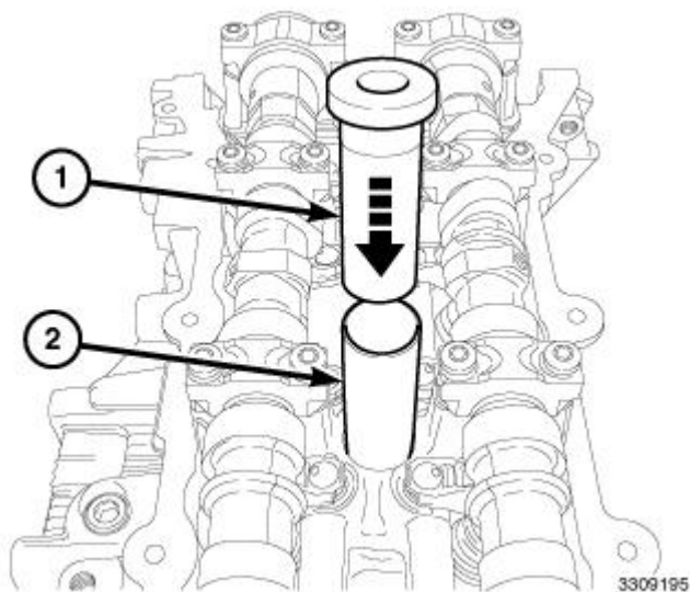
Fig. 369: Spark Plug Tube Installer & Spark Plug Tube
