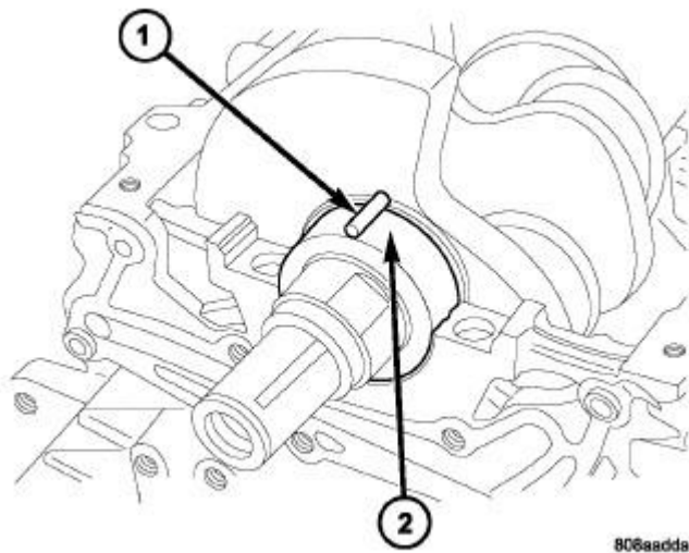
Fig. 389: Plastigage Placed In Lower Shell Courtesy of CHRYSLER GROUP, LLC
