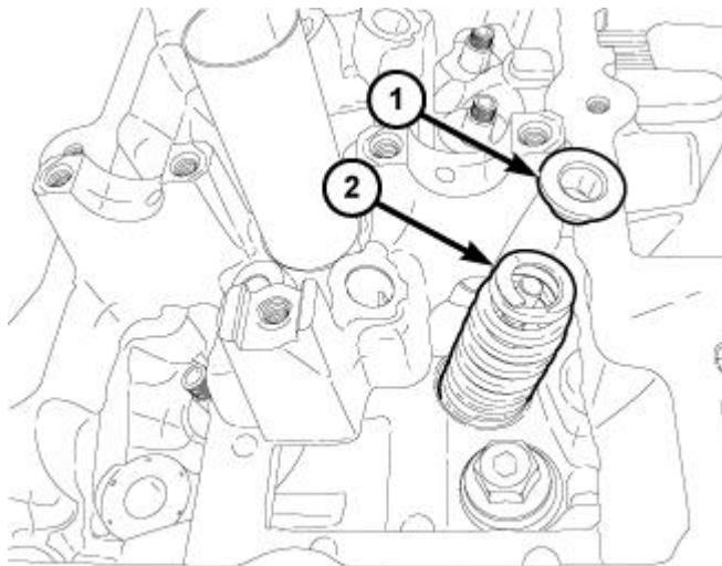
Fig. 359: Valve Spring & Valve Spring Retainer Courtesy of CHRYSLER GROUP, LLC
