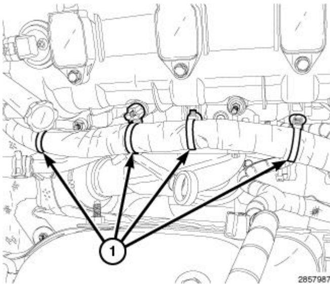
Fig. 323: Main Wire Harness Retainers At Right Cylinder Head Cover Courtesy of CHRYSLER GROUP, LLC
