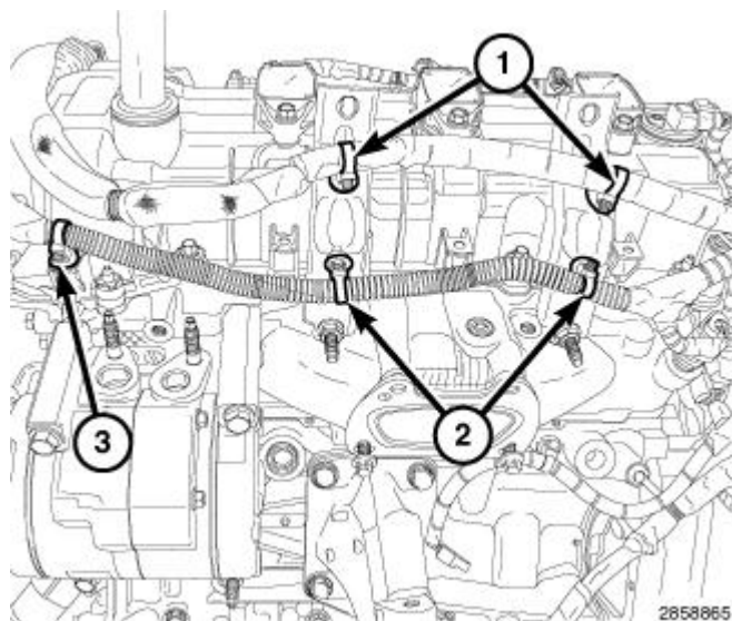
Fig. 173: Starter Wire Harness Retainers, Main Wire Harness Retainer & Manifold Support Bracket Retainers
