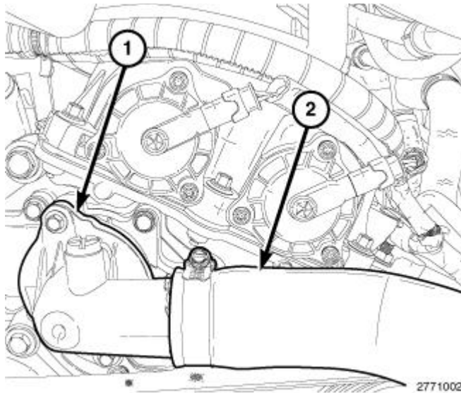
Fig. 737: Upper Radiator Hose & Thermostat Housing Courtesy of CHRYSLER GROUP, LLC
