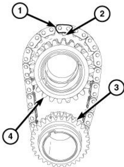
Fig. 703: Placing Idler Sprocket Into Timing Chain So That Dimple Is Aligned With Plated Link On Timing Chain
