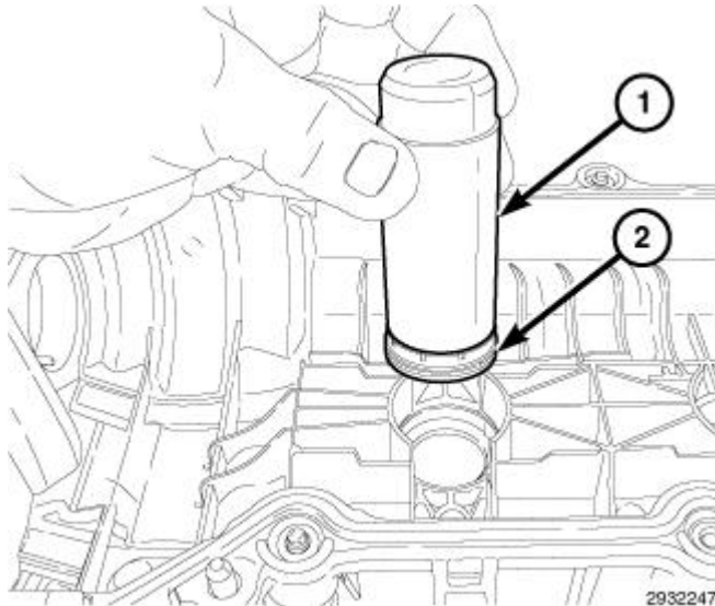
Fig. 301: Spark Plug Tube Seal & Installer Courtesy of CHRYSLER GROUP, LLC
