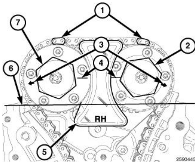
Fig. 709: Phaser Timing Marks, Oil Control Valves & RH Camshaft Phaser Lock Courtesy of CHRYSLER GROUP, LLC
