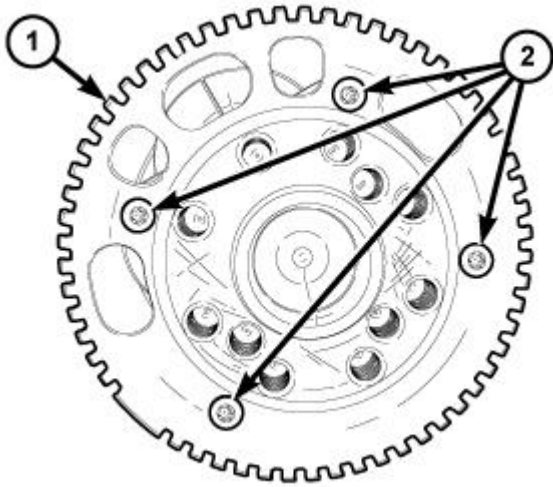
Fig. 425: Target Wheel & Bolts
