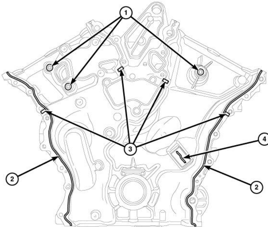
Fig. 725: Sealant At Cylinder Head Bosses, Right & Left Flanges, Cylinder Head-To-Engine Block T-Joints & Cover To Right Cam Chain Tensioner Gap Courtesy of CHRYSLER GROUP, LLC
