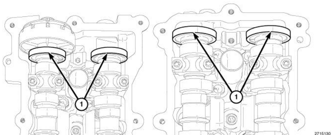
Fig. 368: Magnetic Timing Wheels
