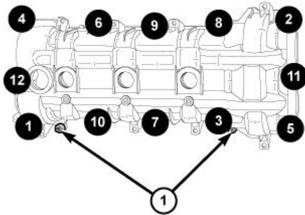
Fig. 318: Cylinder Head Cover Bolts & Double Ended Studs Tightening Sequence - Right Courtesy of CHRYSLER GROUP, LLC
