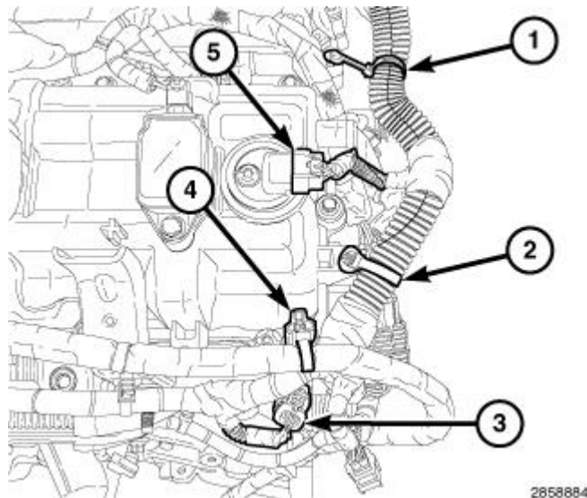
Fig. 494: ECT Sensor Connector, CMP Sensor & Main Wire Harness Retainers Courtesy of CHRYSLER GROUP, LLC
