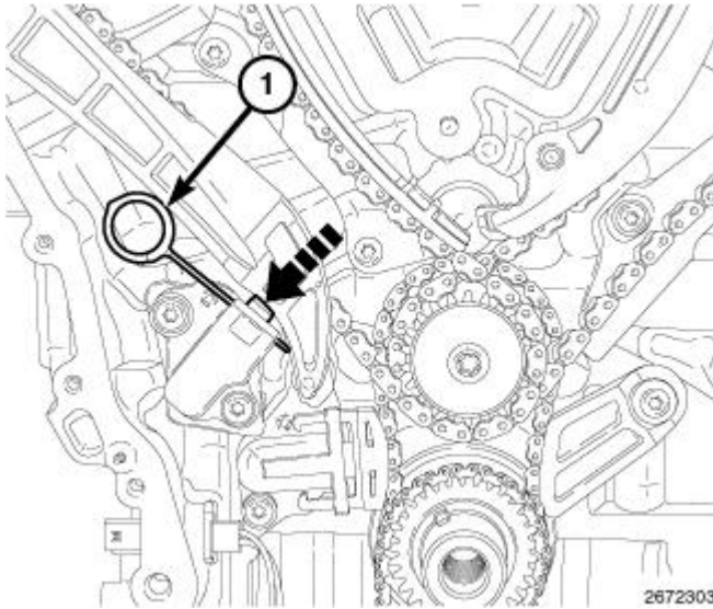
Fig. 687: Resetting Right Cam Chain Tensioner Courtesy of CHRYSLER GROUP, LLC
