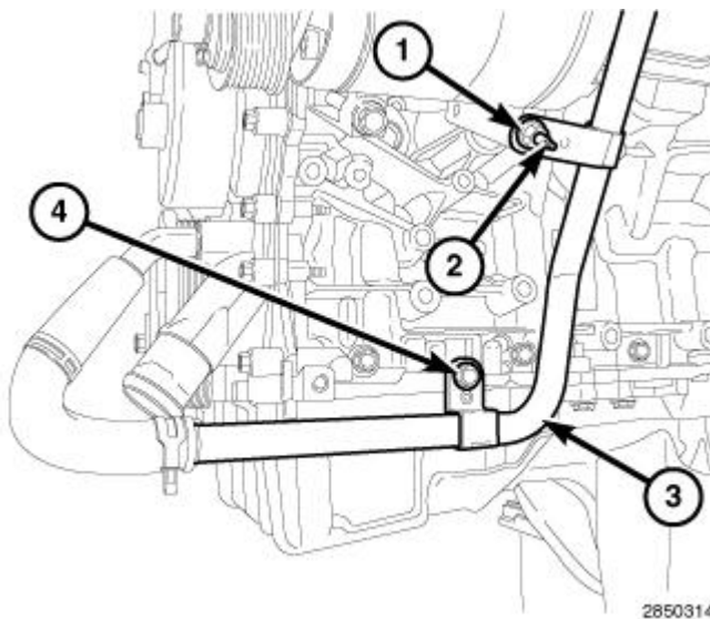
Fig. 8: Heater Core Return Tube, Nut & Bolt
