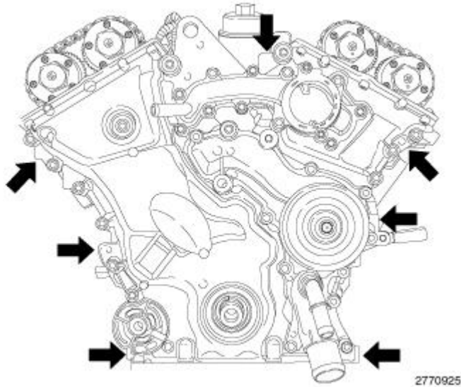
Fig. 723: Timing Cover Removal Pry Points Courtesy of CHRYSLER GROUP, LLC
