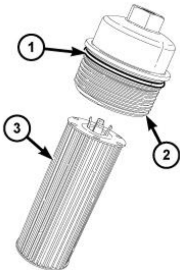
Fig. 535: O-Ring Seal, Oil Filter Cap & Oil Filter Courtesy of CHRYSLER GROUP, LLC
