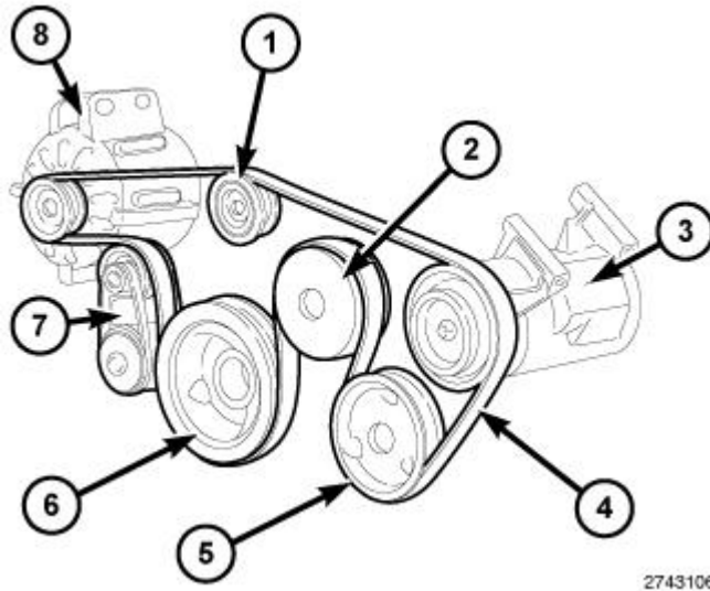
Fig. 495: Drive Belt Tensioners & Accessory Drive Belt Routing Courtesy of CHRYSLER GROUP, LLC
