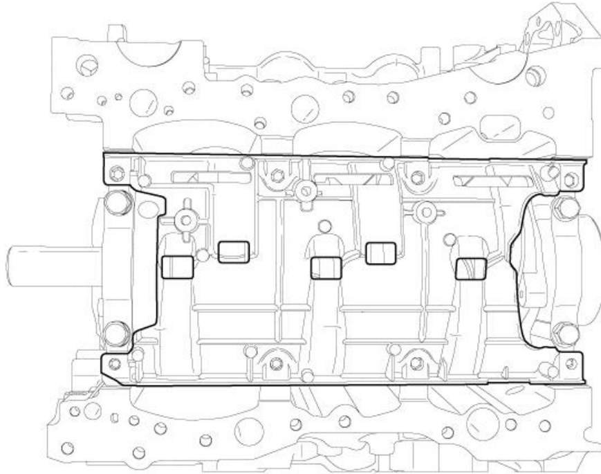
Fig. 561: Windage Tray
