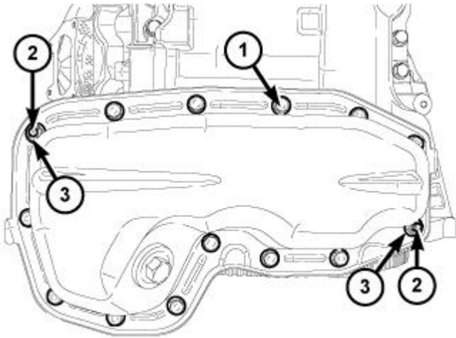
Fig. 562: Lower Oil Pan & Fasteners Courtesy of CHRYSLER GROUP, LLC
