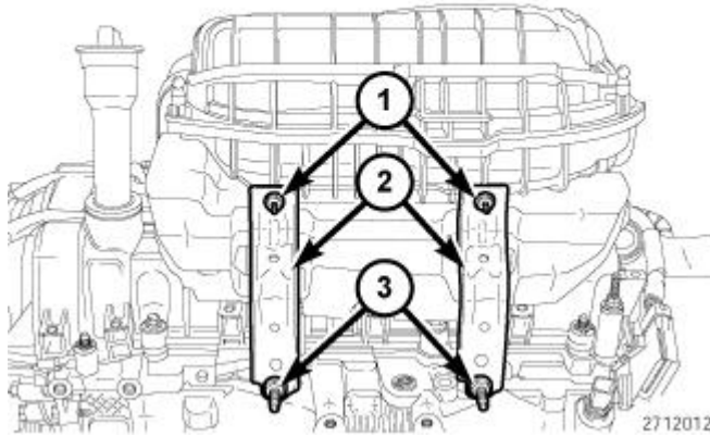
Fig. 642: Nuts, Stud Retainers & Upper Intake Manifold Support Brackets Courtesy of CHRYSLER GROUP, LLC
