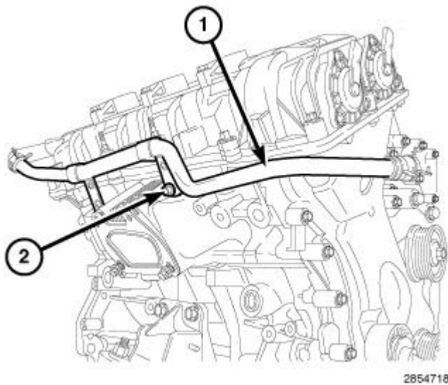
Fig. 718: Heater Core Supply Tube Support Bracket & Retaining Bolt Courtesy of CHRYSLER GROUP, LLC
