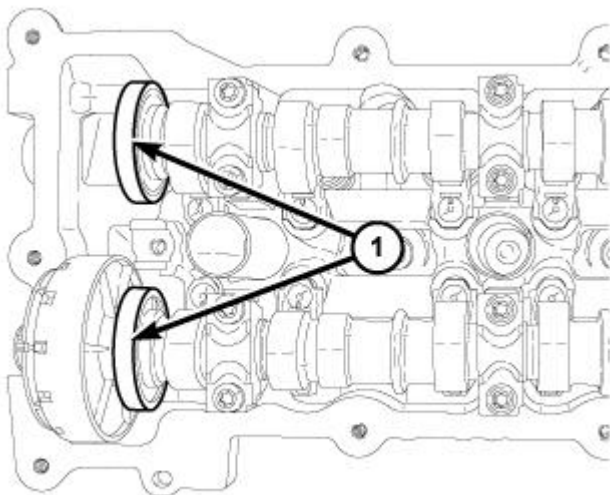
Fig. 251: Magnetic Timing Wheels Courtesy of CHRYSLER GROUP, LLC
