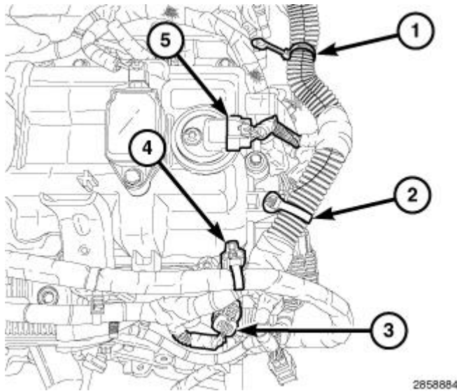
Fig. 491: ECT Sensor Connector, CMP Sensor & Main Wire Harness Retainers Courtesy of CHRYSLER GROUP, LLC
