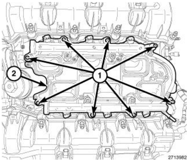
Fig. 621: Lower Intake Manifold & Attaching Bolts
