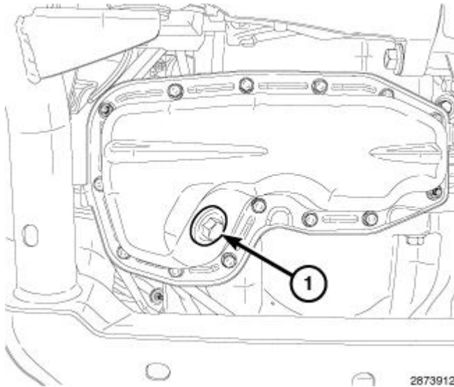
Fig. 556: Oil Pan Drain Plug
