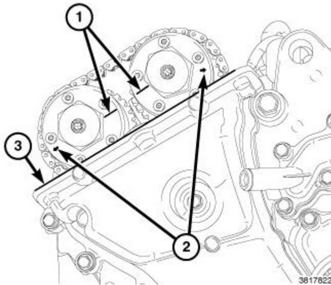
Fig. 267: Arrows, Scribe Lines & Cylinder Head Cover Mounting Surface Courtesy of CHRYSLER GROUP, LLC
