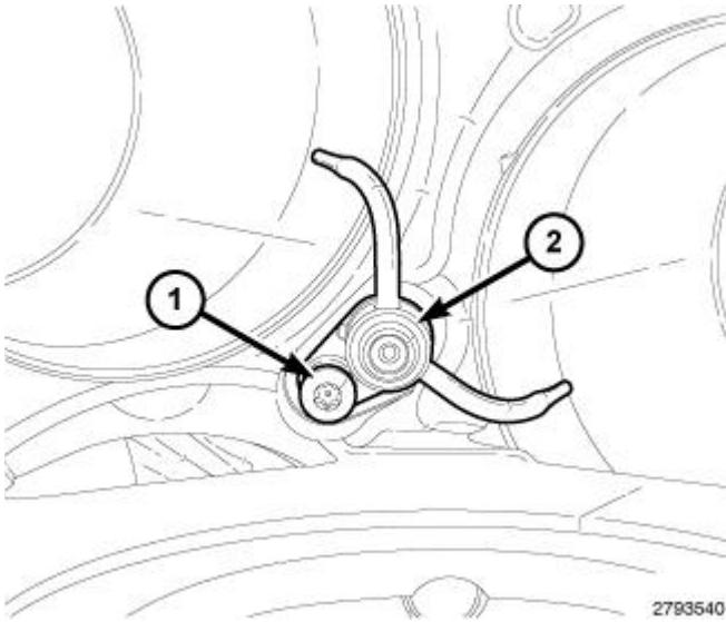
Fig. 550: Piston Oil Cooler Jet & Bolt Courtesy of CHRYSLER GROUP, LLC
