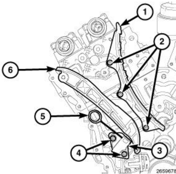
Fig. 695: Right Cam Chain Tensioner, Arm, Guide & Bolts Courtesy of CHRYSLER GROUP, LLC
