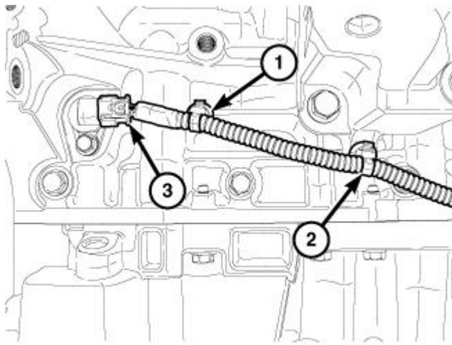
Fig. 504: Main Wire Harness Retainers & CKP Sensor Courtesy of CHRYSLER GROUP, LLC
