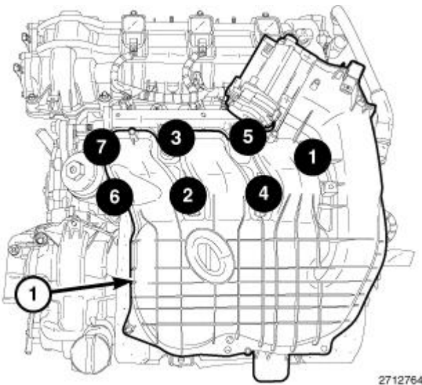
Fig. 492: Upper Intake Manifold Bolt Tightening Sequence Courtesy of CHRYSLER GROUP, LLC
