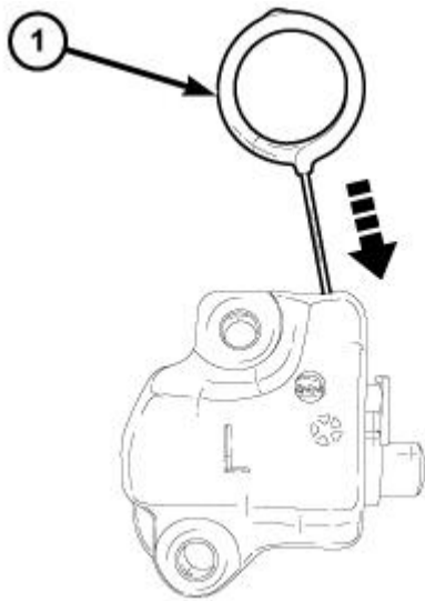
Fig. 676: Inserting Tensioner Pin To Hold Rack & Piston In Retracted Position Courtesy of CHRYSLER GROUP, LLC
