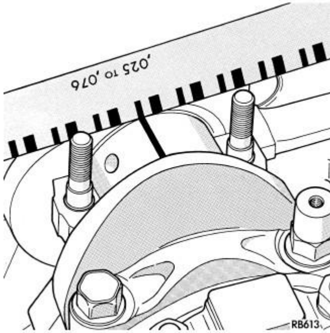
Fig. 391: Checking Connecting Rod Bearing Clearance With Plastigage Courtesy of CHRYSLER GROUP, LLC
