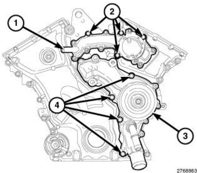
Fig. 724: Coolant Outlet Housing, Water Pump & Bolts Courtesy of CHRYSLER GROUP, LLC
