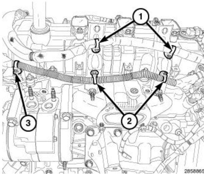
Fig. 275: Starter Wire Harness Retainers, Main Wire Harness Retainer & Manifold Support Bracket Retainers
