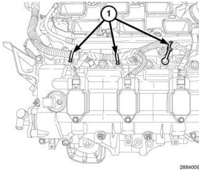
Fig. 291: Injection/Ignition Harness Retainers Courtesy of CHRYSLER GROUP, LLC
