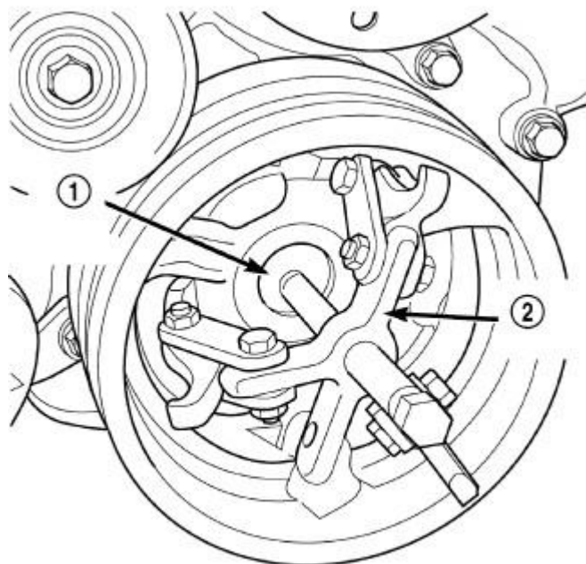
Fig. 148: VIBRATION DAMPER - REMOVAL Courtesy of CHRYSLER LLC
