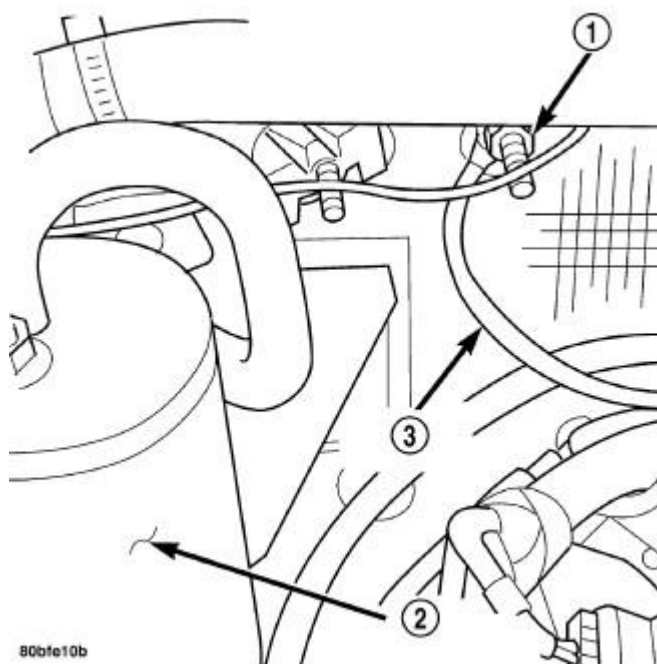
Fig. 14: Body Ground Strap-Right Side Removal / Installation
