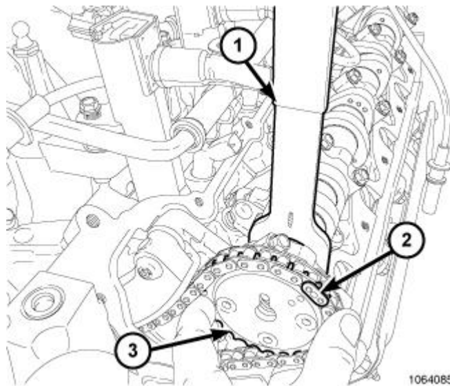
Fig. 108: Removing/Installing Camshaft Holder On Camshaft Courtesy of CHRYSLER LLC
