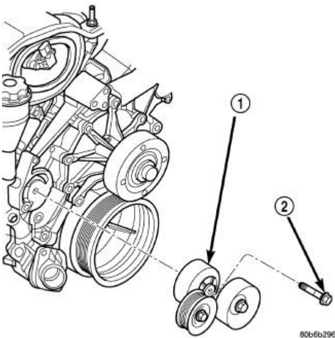
Fig. 228: Accessory Drive Belt Tensioner Courtesy of CHRYSLER LLC
