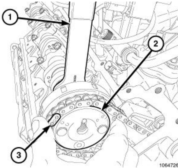
Fig. 98: Installing Camshaft Holder Onto Camshaft Courtesy of CHRYSLER LLC
