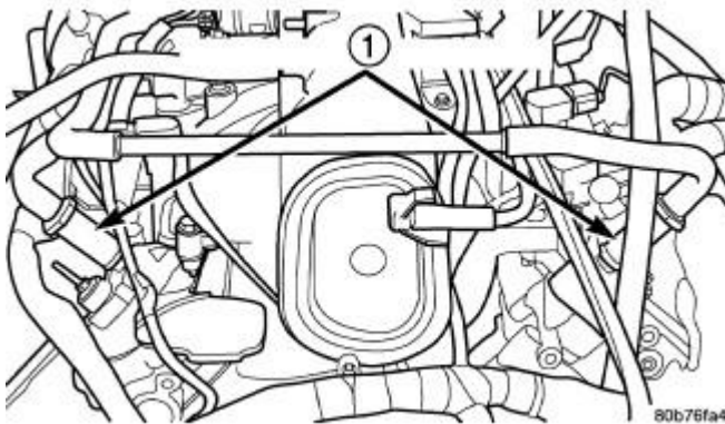
Fig. 25: Crankcase Breather Connection Points Courtesy of CHRYSLER LLC
