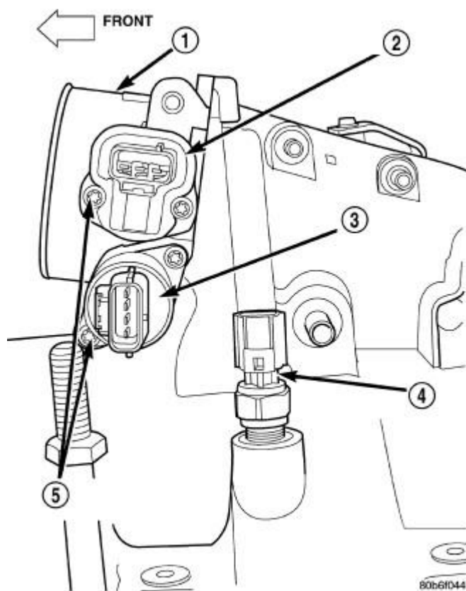
Fig. 12: Throttle Body Connection Points Courtesy of CHRYSLER LLC
