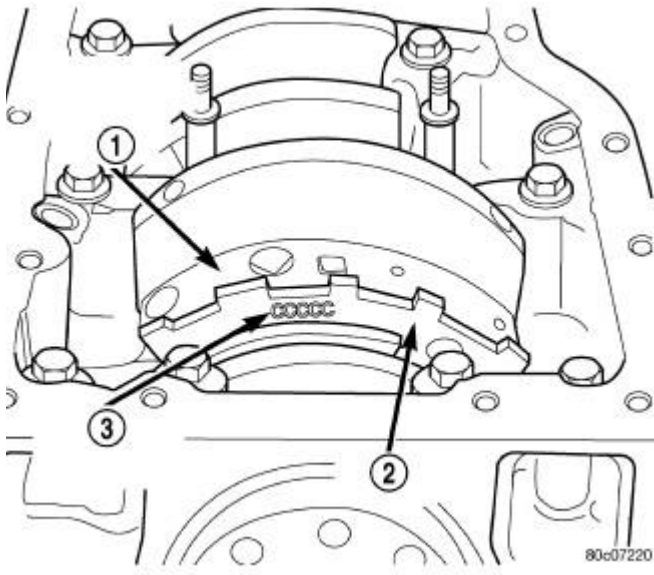
Fig. 134: Main Bearing Markings on Target Wheel Courtesy of CHRYSLER LLC
