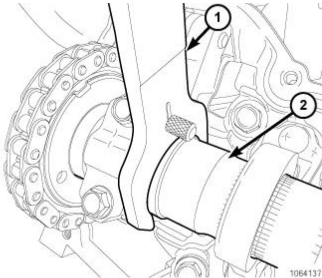
Fig. 103: Removing/Installing Camshaft Sprocket Bolt Using Spanner Wrench Courtesy of CHRYSLER LLC
