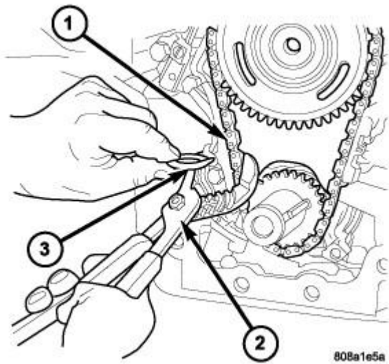
Fig. 217: Collapsing And Pinning Primary Chain Tensioner Courtesy of CHRYSLER LLC
