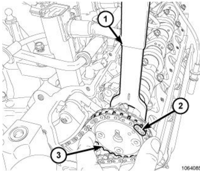
Fig. 210: Removing/Installing Camshaft Holder On Camshaft Courtesy of CHRYSLER LLC
