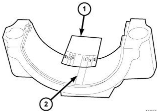
Fig. 133: Measuring Bearing Clearance with Plastigage Courtesy of CHRYSLER LLC
