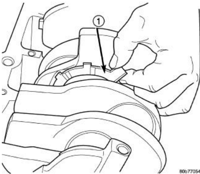
Fig. 140: Crankshaft Thrust Washer Installation Courtesy of CHRYSLER LLC
