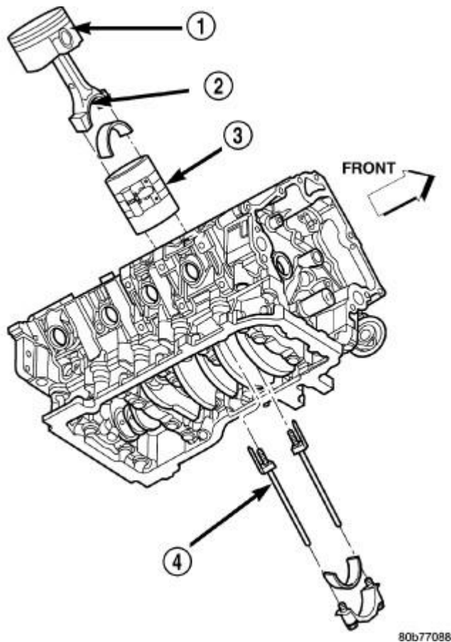
Fig. 161: Piston and Connecting Rod - Installation Courtesy of CHRYSLER LLC
