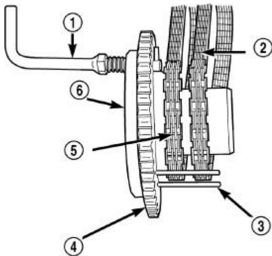
Fig. 90: Installing Secondary Timing Chains on Idler Sprocket Courtesy of CHRYSLER LLC
