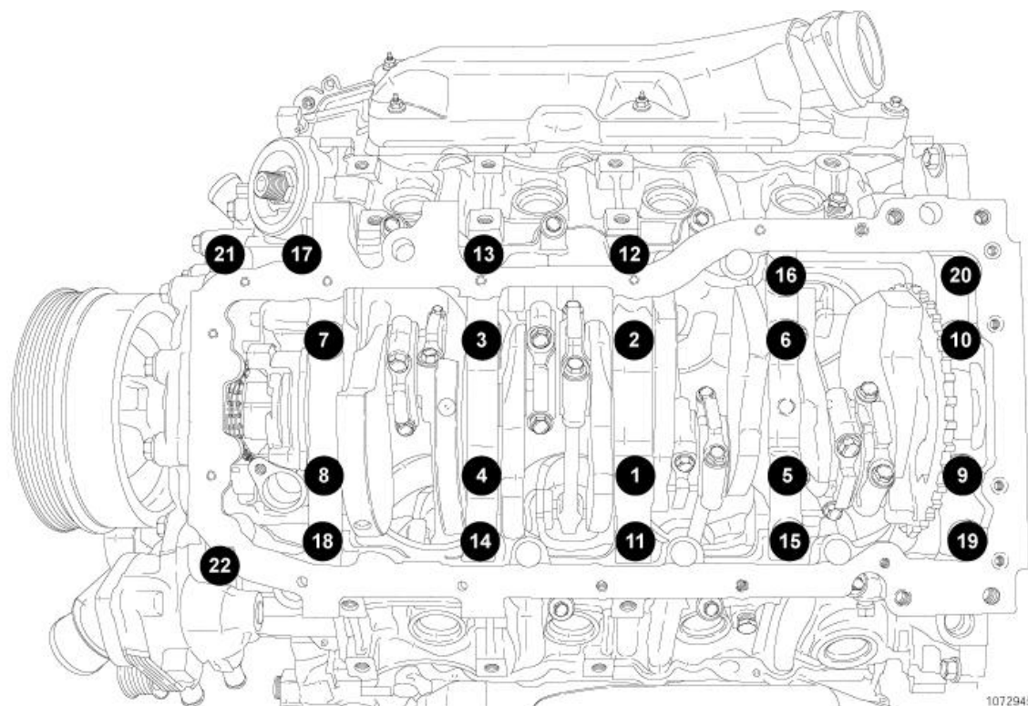
Fig. 142: Tightening Bedplate Bolts (1 Of 4)
