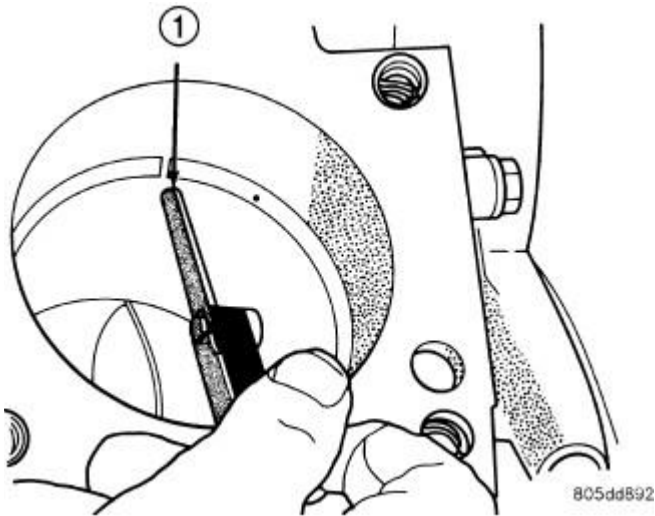
Fig. 154: Ring End Gap Measurement - Typical Courtesy of CHRYSLER LLC
