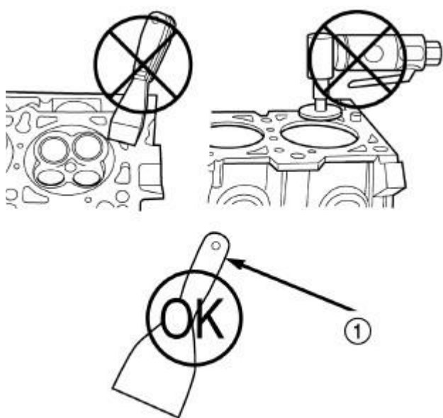
Fig. 79: Proper Tool Usage For Surface Preparation Courtesy of CHRYSLER LLC
