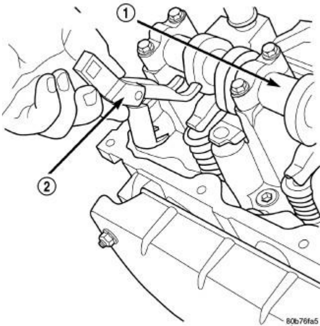
Fig. 125: Rocker Arm Removal/Installation Courtesy of CHRYSLER LLC
