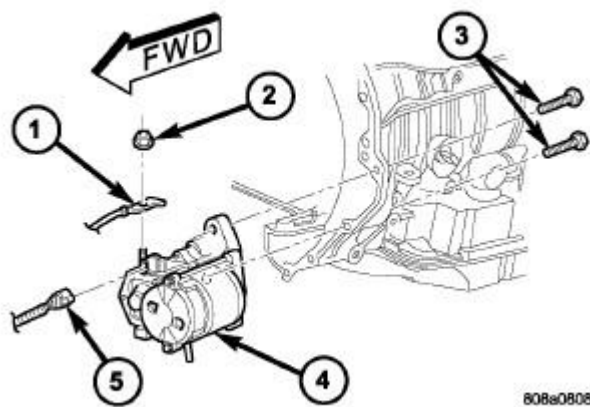
Fig. 27: Starter Motor Remove/Install - 4.7L Engine Courtesy of CHRYSLER LLC
