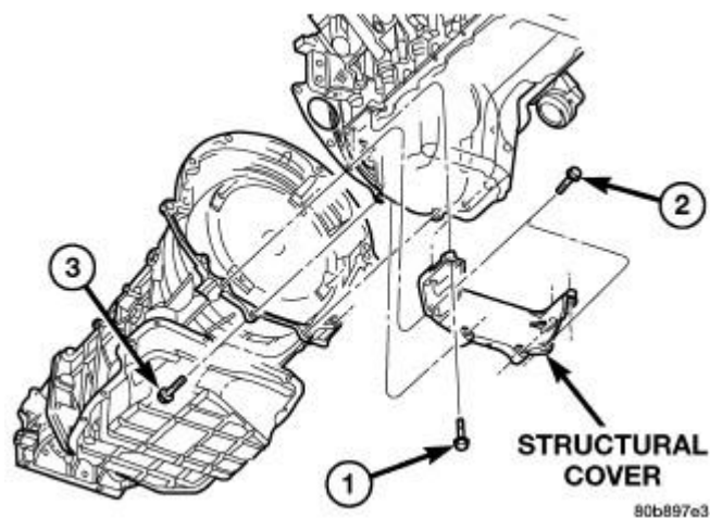
Fig. 178: Structural Cover
