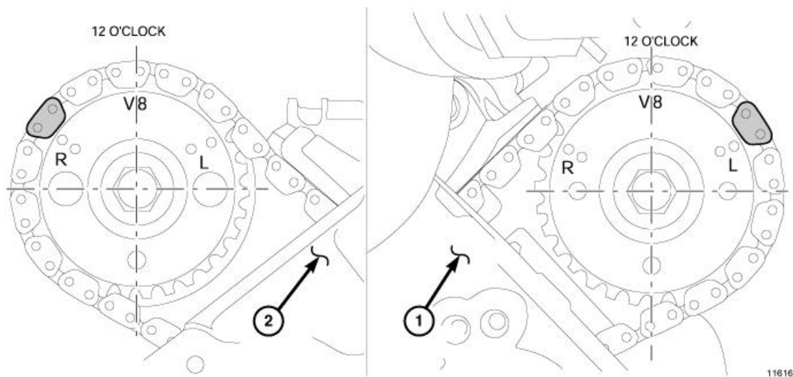
Fig. 209: Timing Chain to Sprocket Alignment Courtesy of CHRYSLER LLC
