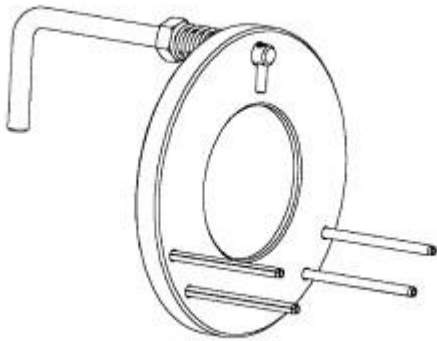
Fig. 35: Secondary Chain Holder 8429 Courtesy of CHRYSLER LLC
