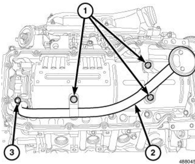
Fig. 191: Identifying Oil Pickup Tube Courtesy of CHRYSLER LLC
