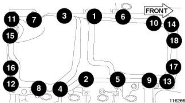
Fig. 138: Oil Pan Tightening Sequence Courtesy of CHRYSLER LLC
