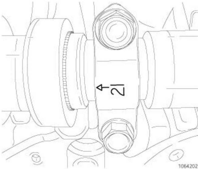
Fig. 106: Positioning Camshaft Cap Arrow Toward Front Of Engine Courtesy of CHRYSLER LLC
