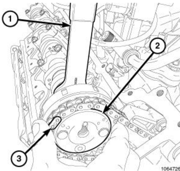
Fig. 221: Installing Camshaft Holder Onto Camshaft Courtesy of CHRYSLER LLC
