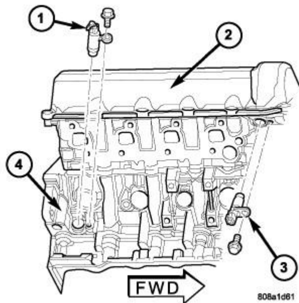
Fig. 26: Crankshaft Position Sensor Courtesy of CHRYSLER LLC
