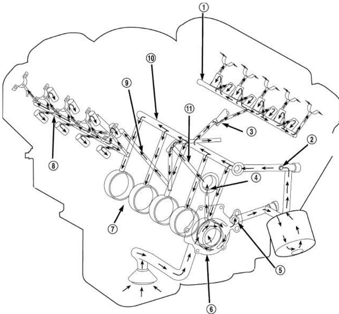
Fig. 172: Engine Oil Lubrication System Courtesy of CHRYSLER LLC
