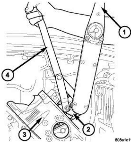
Fig. 117: Tightening Left Side Cam Sprocket Retaining Bolt Courtesy of CHRYSLER LLC
