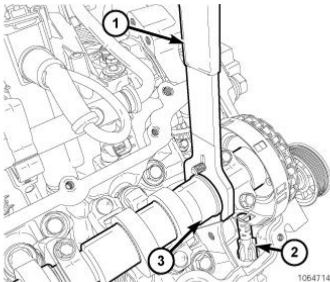
Fig. 97: Removing/Installing Cam Sensor And Camshaft Sprocket Bolt Using Spanner Wrench
