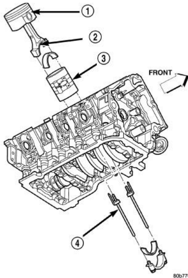
Fig. 131: Piston and Connecting Rod - Installation Courtesy of CHRYSLER LLC
