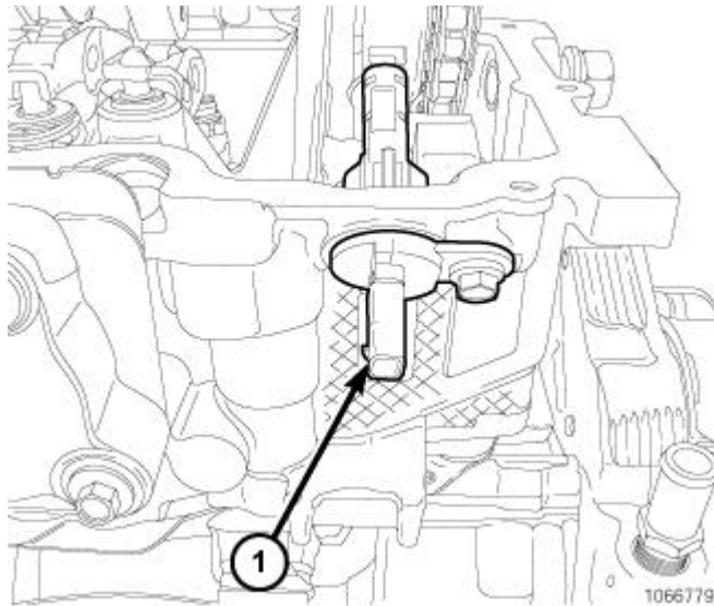
Fig. 96: Identifying Camshaft Position Sensor
