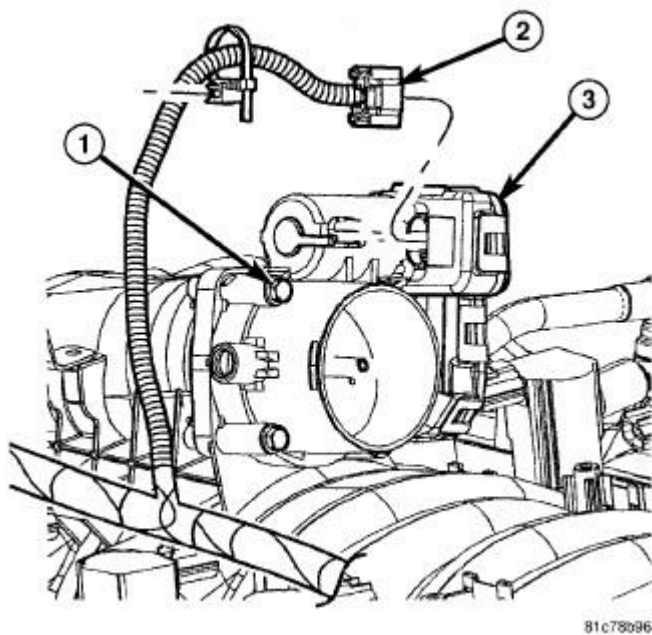
Fig. 198: THROTTLE BODY-4.7L
