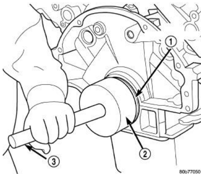
Fig. 168: Crankshaft Rear Oil Seal Installation Courtesy of CHRYSLER LLC
