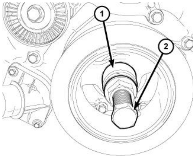
Fig. 150: Pressing Damper Onto Crankshaft Courtesy of CHRYSLER LLC
