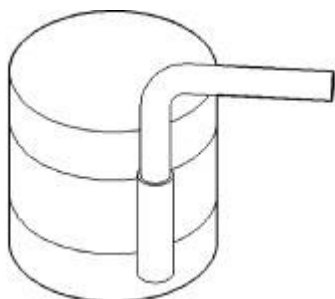
Fig. 56: Piston Ring Compressor C-385 Courtesy of CHRYSLER LLC
