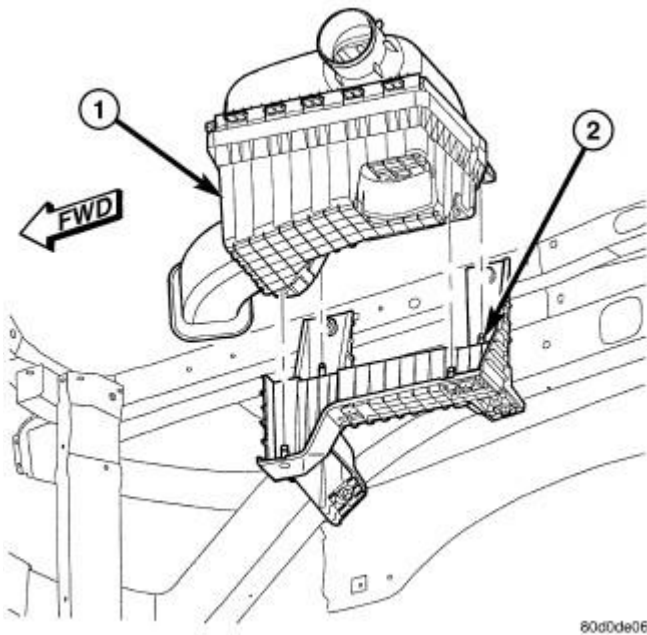
Fig. 63: AIR CLEANER HOUSING Courtesy of CHRYSLER LLC
