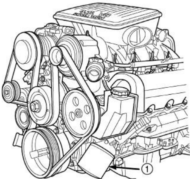
Fig. 174: Oil Filter - 4.7L Engine Courtesy of CHRYSLER LLC
