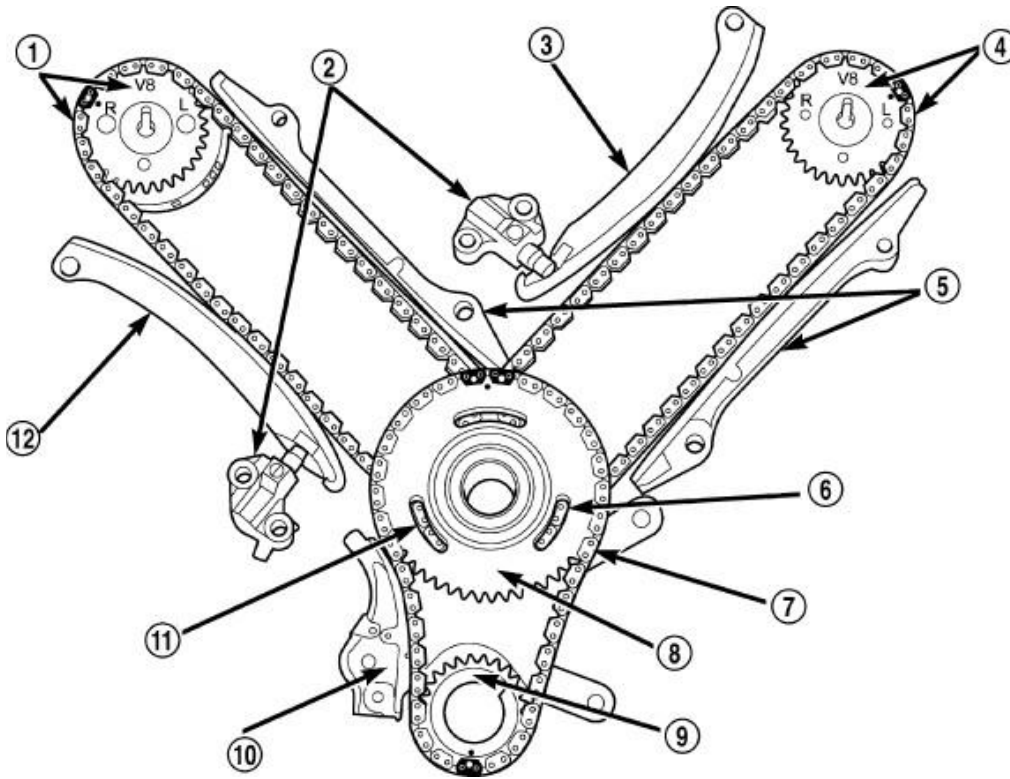
Fig. 203: Timing Drive System Courtesy of CHRYSLER LLC
