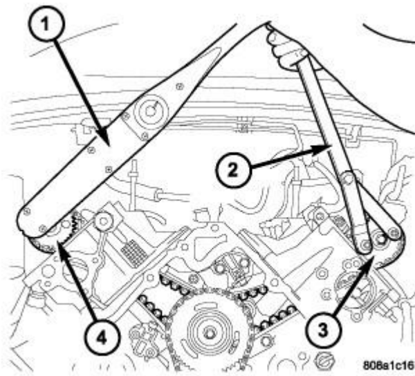
Fig. 95: Tightening Right Side Camshaft Sprocket Bolt
