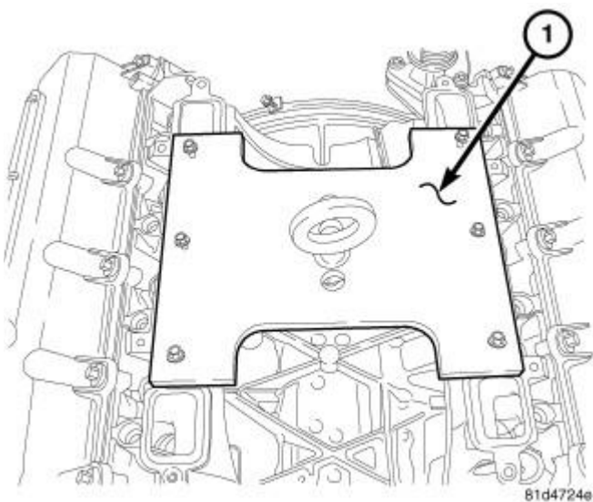
Fig. 16: Engine Lift Bracket 10101
