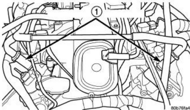
Fig. 8: Crankcase Breather Connection Points Courtesy of CHRYSLER LLC
