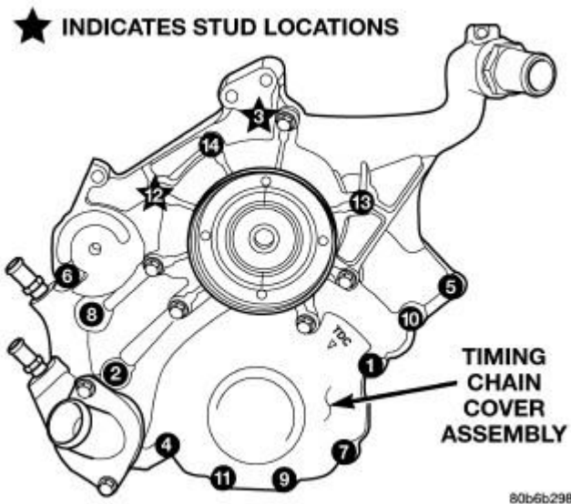
Fig. 229: Timing Chain Cover Fasteners Courtesy of CHRYSLER LLC
