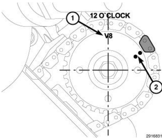
Fig. 100: Aligning Camshaft Sprocket V8 Mark & Identifying 2 Dots Courtesy of CHRYSLER LLC
