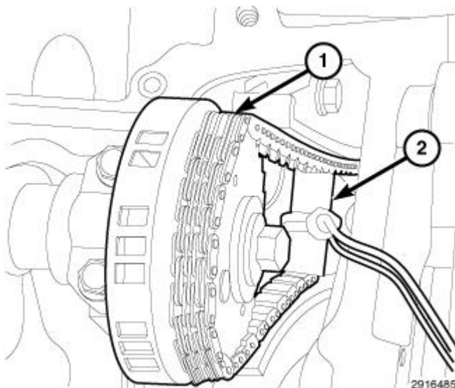
Fig. 94: Positioning Locking Wedge Between Timing Chain
