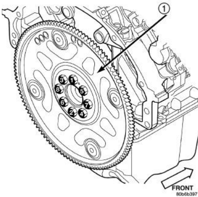
Fig. 152: Flexplate Tightening Sequence
