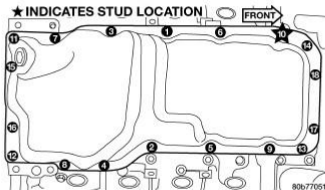
Fig. 180: Oil Pan Mounting Bolts and Oil Pan Courtesy of CHRYSLER LLC
