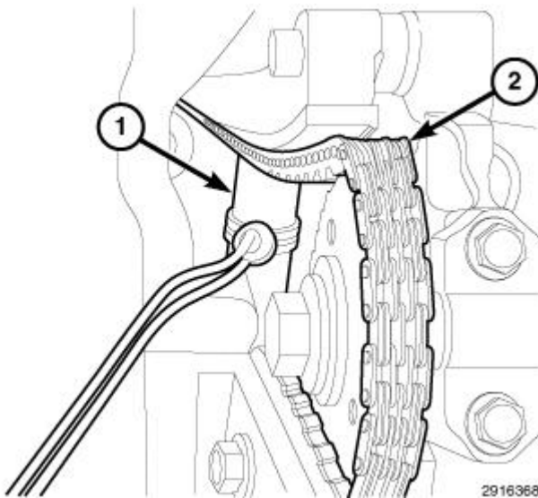
Fig. 116: Positioning Locking Wedge Between Timing Chain Strands Courtesy of CHRYSLER LLC
