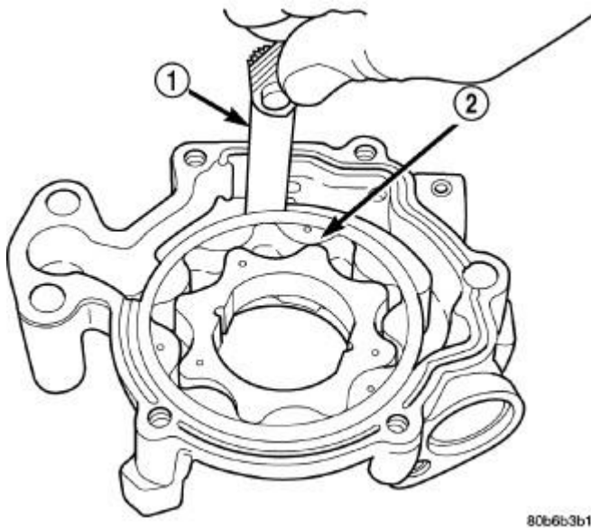
Fig. 187: Measuring Outer Rotor Clearance Courtesy of CHRYSLER LLC
