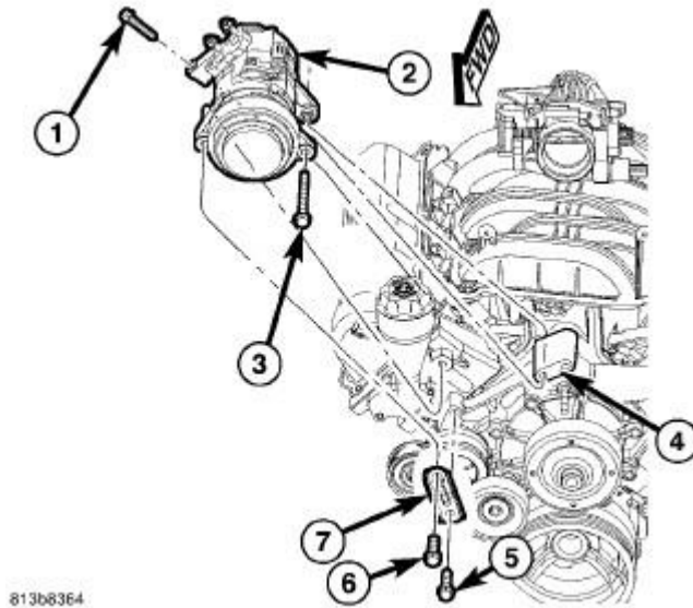
Fig. 24: A/C Compressor R and I Courtesy of CHRYSLER LLC
