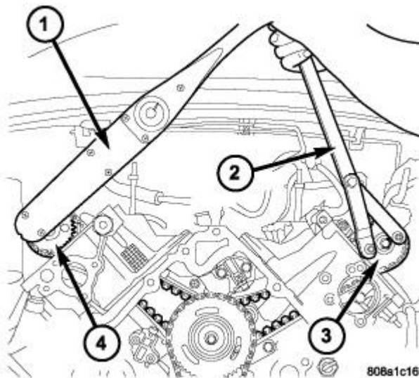
Fig. 211: Camshaft Sprocket Installation-Right Cylinder Head Courtesy of CHRYSLER LLC
