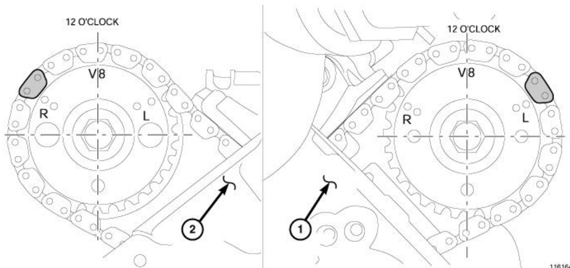
Fig. 206: Camshaft Sprocket V8 Marks Courtesy of CHRYSLER LLC
