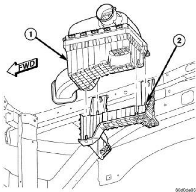
Fig. 62: AIR CLEANER HOUSING
