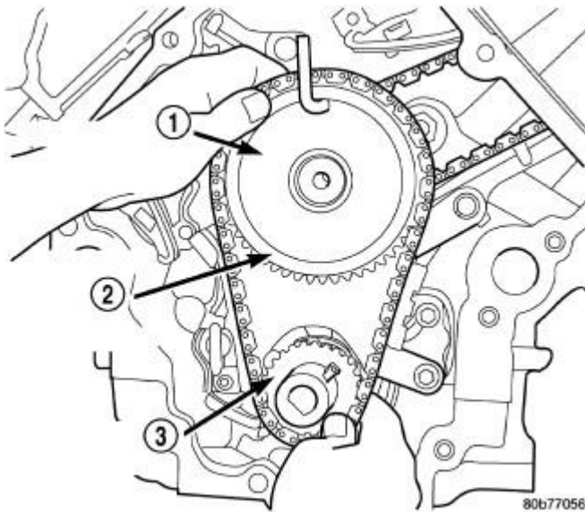
Fig. 225: Installing Idler Gear, Primary and Secondary Timing Chains Courtesy of CHRYSLER LLC
