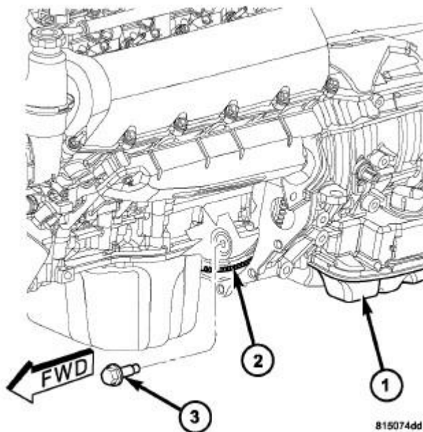
Fig. 6: Remove/Install Torque Converter Bolts Courtesy of CHRYSLER LLC
