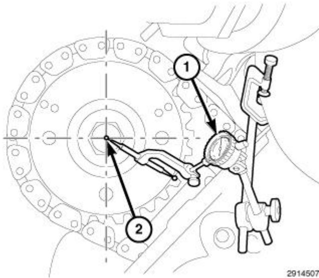
Fig. 92: Positioning Dial Indicator Tip Against Camshaft Courtesy of CHRYSLER LLC
