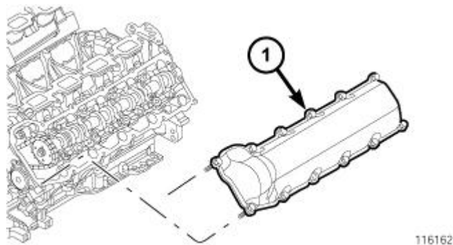
Fig. 111: Cylinder Head Cover-Left Courtesy of CHRYSLER LLC
