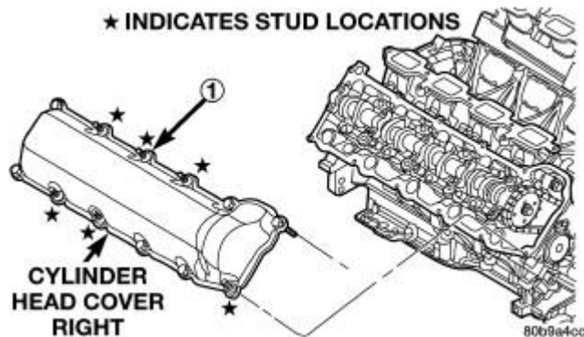
Fig. 91: Cylinder Head Cover-Right Courtesy of CHRYSLER LLC
