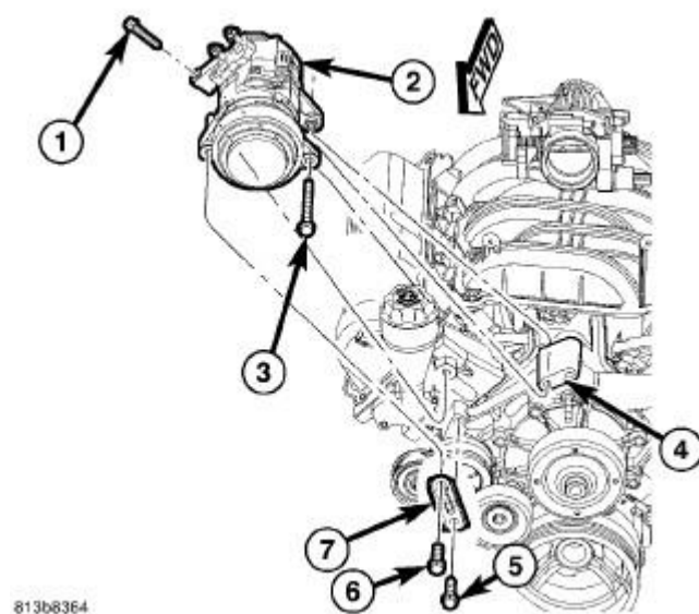
Fig. 9: A/C Compressor R and I Courtesy of CHRYSLER LLC
