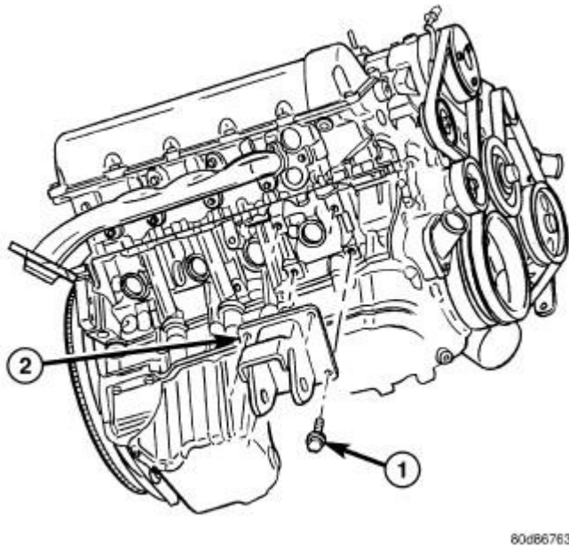
Fig. 170: ENGINE MOUNT SUPPORT BRACKET RH Courtesy of CHRYSLER LLC
