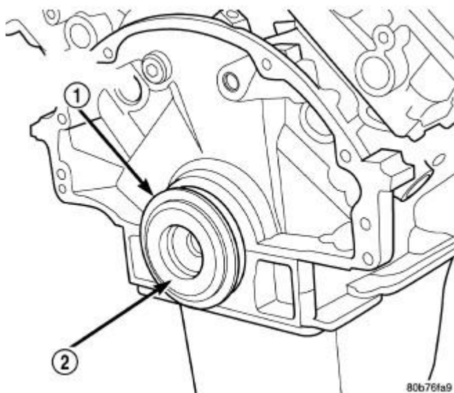
Fig. 167: Crankshaft Rear Oil Seal Guide Special Tool 8349-2 and Oil Courtesy of CHRYSLER LLC
