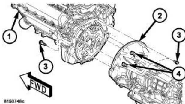
Fig. 17: Removing/Installing Transmission to Engine Bolts
