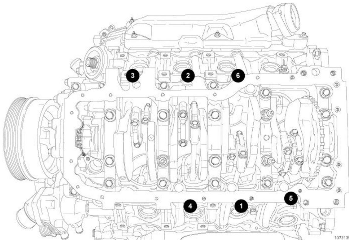
Fig. 145: Tightening Bedplate Bolts (4 Of 4)
