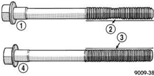
Fig. 85: Checking Cylinder Head Bolts for Stretching (Necking) Courtesy of CHRYSLER LLC
