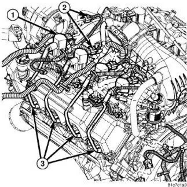
Fig. 119: IGNITION COIL - 4.7L Courtesy of CHRYSLER LLC
