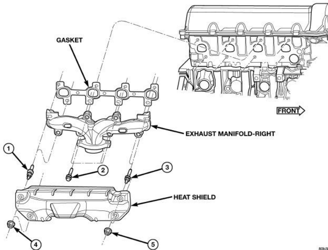
Fig. 194: Exhaust Manifold-Right Courtesy of CHRYSLER LLC
