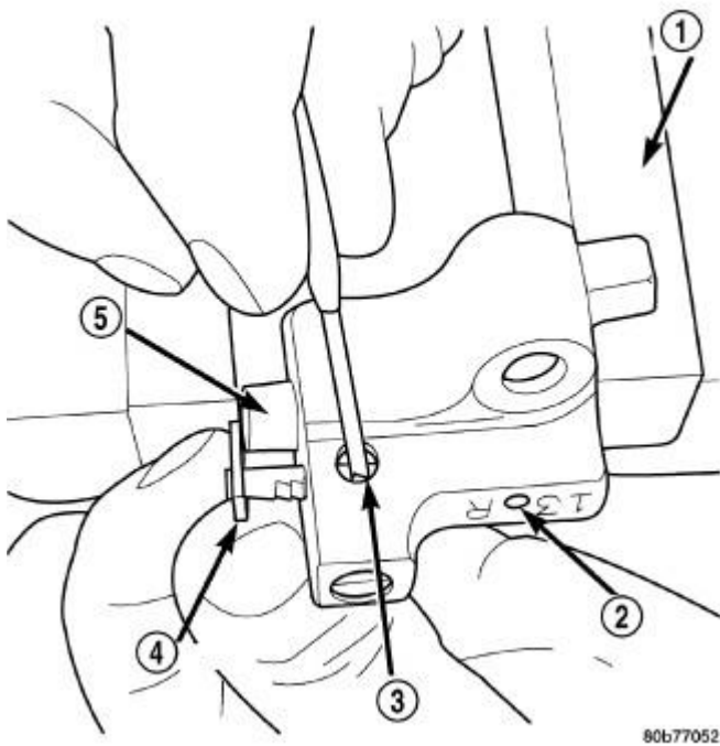
Fig. 223: Resetting Secondary Chain Tensioners Courtesy of CHRYSLER LLC
