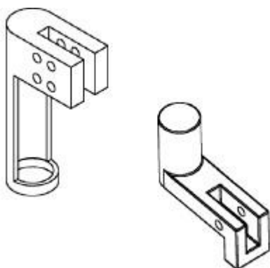
Fig. 49: Valve Spring Compressor Adapters 8519 Courtesy of CHRYSLER LLC
