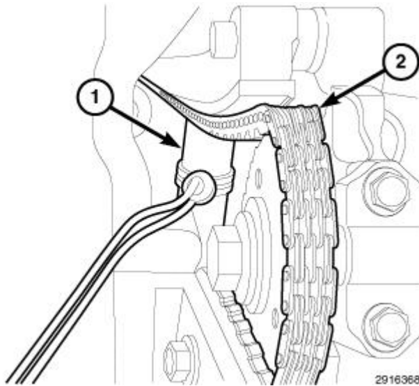
Fig. 101: Positioning Locking Wedge Between Timing Chain Strands Courtesy of CHRYSLER LLC
