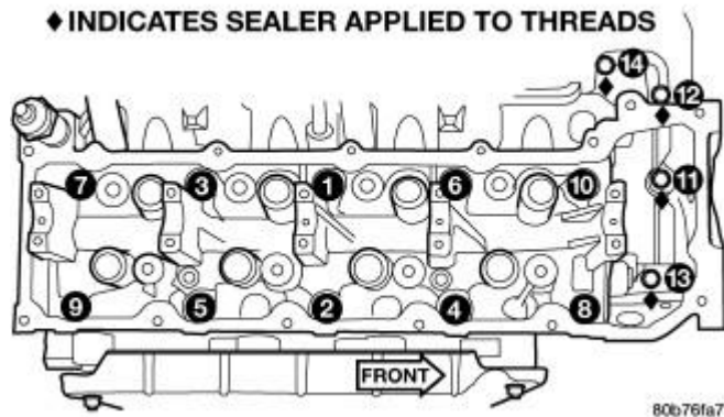
Fig. 87: Cylinder Head Tightening Sequence Courtesy of CHRYSLER LLC
