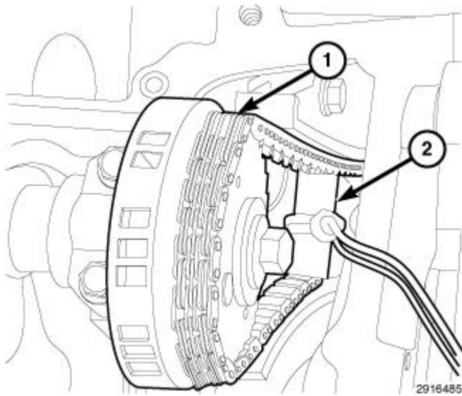
Fig. 109: Positioning Locking Wedge Between Timing Chain Courtesy of CHRYSLER LLC
