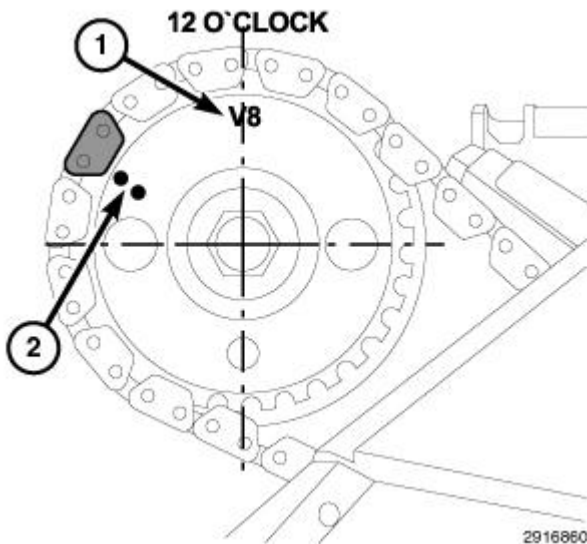
Fig. 93: Aligning Camshaft Sprocket V8 Mark & Identifying 2 Dots Courtesy of CHRYSLER LLC
