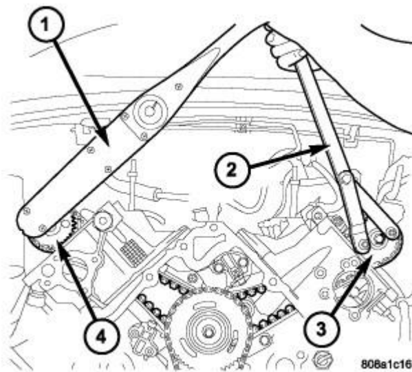
Fig. 208: Tightening Right Side Camshaft Sprocket Bolt Courtesy of CHRYSLER LLC
