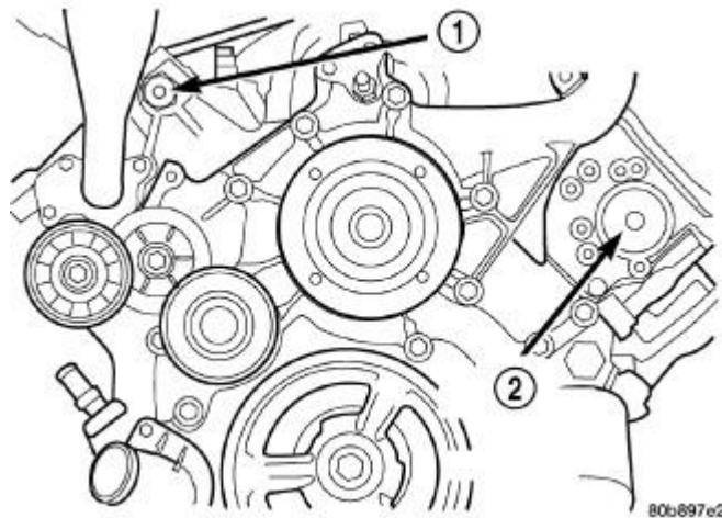
Fig. 75: Cylinder Head Access Plugs Courtesy of CHRYSLER LLC
