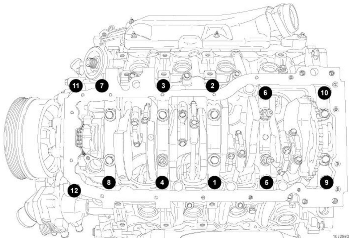
Fig. 143: Tightening Bedplate Bolts (2 Of 4) Courtesy of CHRYSLER LLC
