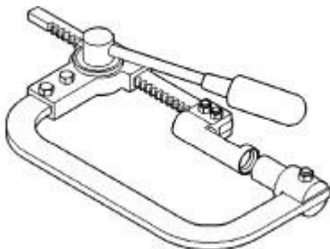
Fig. 53: Valve Spring Compressor C-3422-CF Courtesy of CHRYSLER LLC
