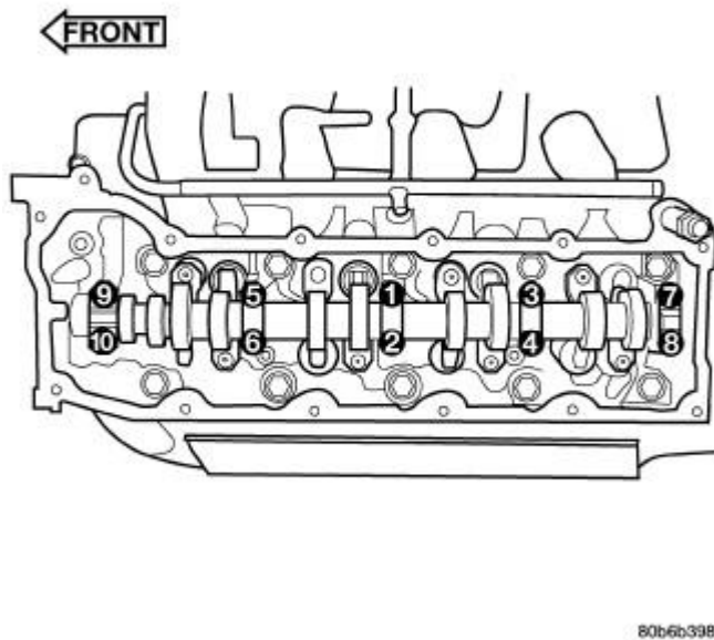
Fig. 99: Identifying Removal & Installation Sequence Of Camshaft Bearing Cap Retaining Bolts Courtesy of CHRYSLER LLC
