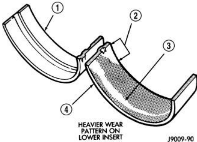
Fig. 135: Main Bearing Wear Patterns Courtesy of CHRYSLER LLC
