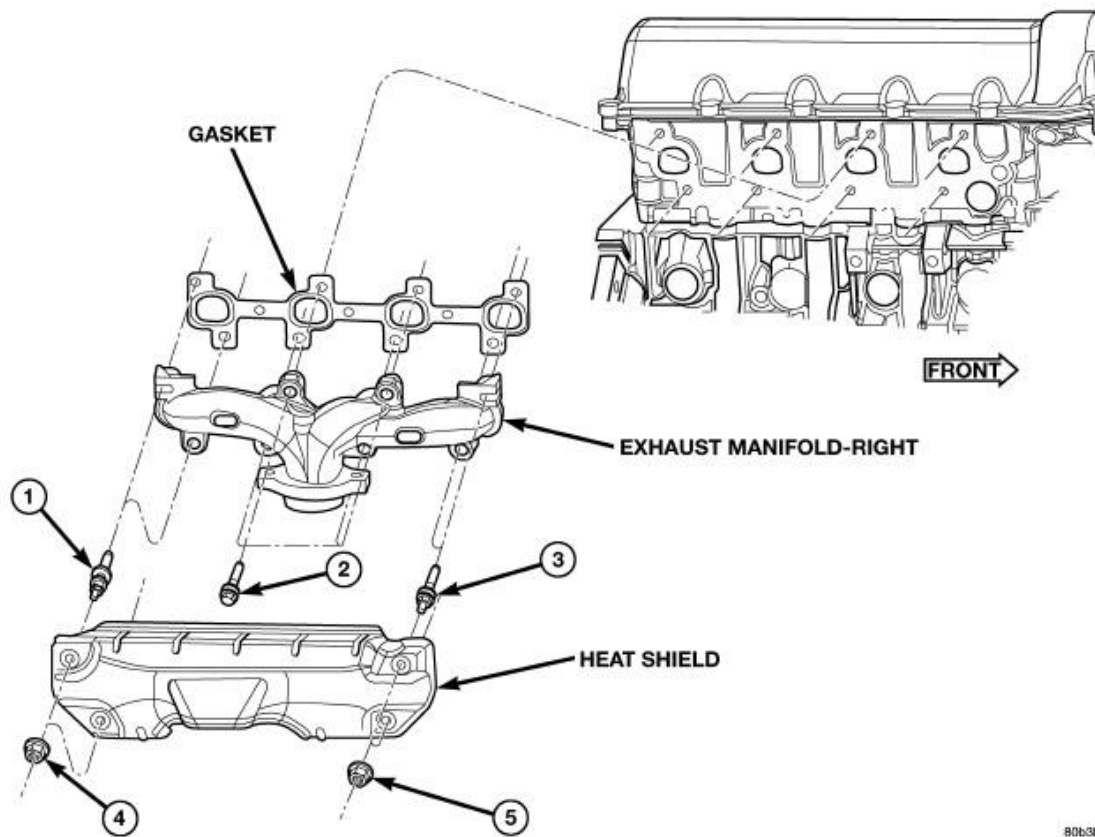
Fig. 196: Exhaust Manifold-Right Courtesy of CHRYSLER LLC
