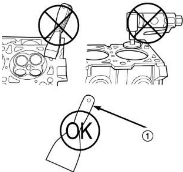
Fig. 86: Proper Tool Usage For Surface Preparation Courtesy of CHRYSLER LLC
