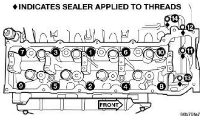
Fig. 76: Cylinder Head Tightening Sequence Courtesy of CHRYSLER LLC
