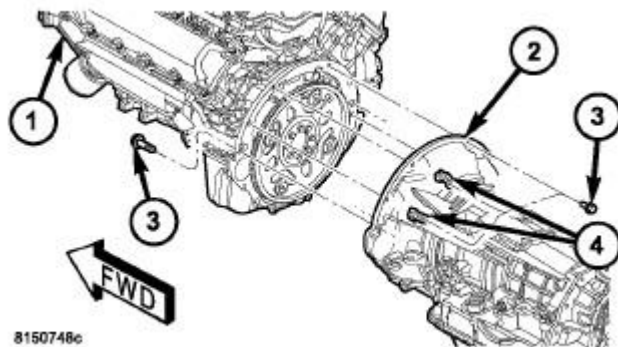
Fig. 7: Remove/Install Transmission to Engine Bolts Courtesy of CHRYSLER LLC
