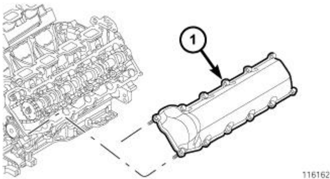
Fig. 84: Cylinder Head Cover - Left Courtesy of CHRYSLER LLC
