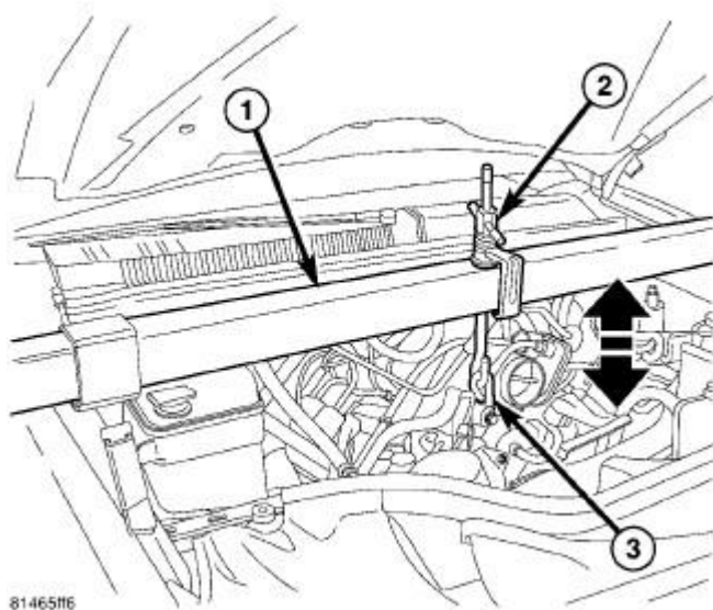
Fig. 177: ENGINE SUPPORT TOOL
