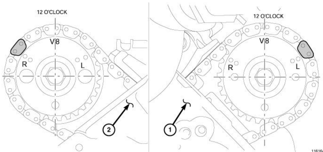
Fig. 81: Timing Chain to Sprocket Alignment Courtesy of CHRYSLER LLC
