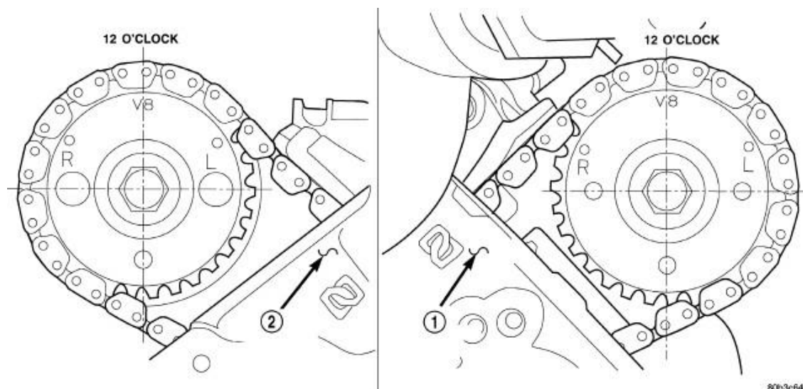
Fig. 68: Camshaft Sprocket V8 Marks Courtesy of CHRYSLER LLC
