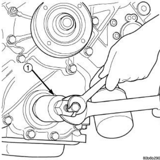
Fig. 164: Crankshaft Front Seal Removal Courtesy of CHRYSLER LLC
