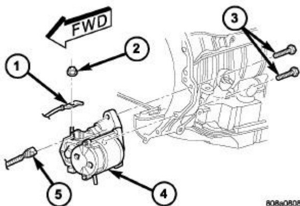
Fig. 5: Starter Motor Remove/Install - 4.7L Engine Courtesy of CHRYSLER LLC
