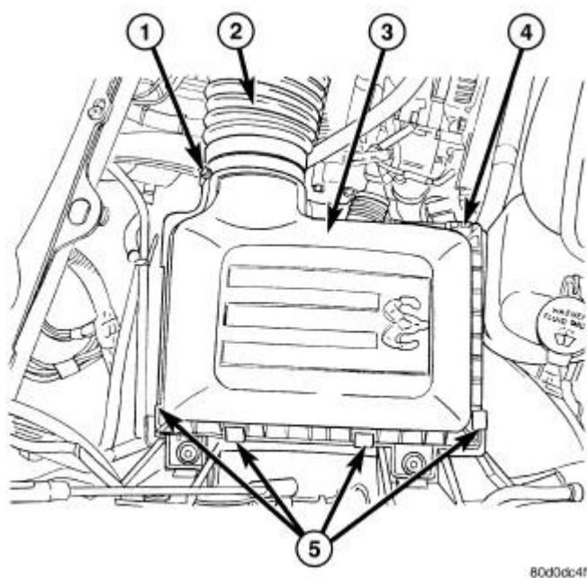
Fig. 61: AIR CLEANER HOUSING COVER
