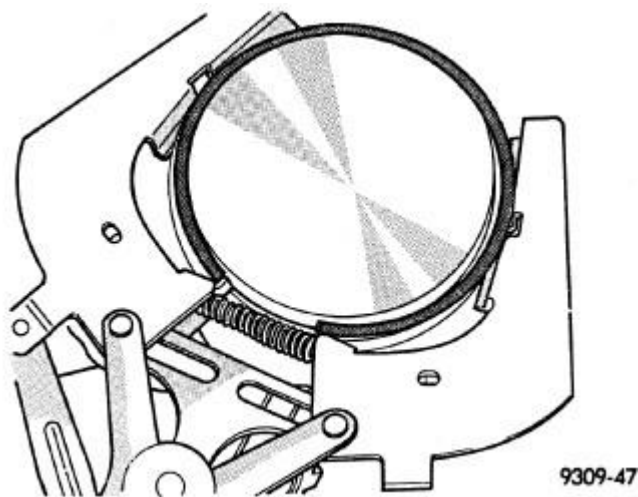
Fig. 156: Upper and Intermediate Rings - Installation Courtesy of CHRYSLER LLC
