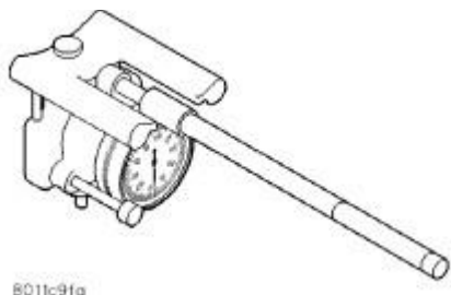
Fig. 54: Indicator Cylinder Bore C-119 Courtesy of CHRYSLER LLC
