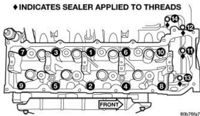
Fig. 80: Cylinder Head Tightening Sequence Courtesy of CHRYSLER LLC
