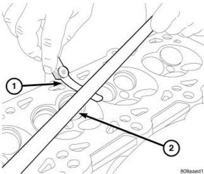
Fig. 77: Checking Cylinder Head Flatness Courtesy of CHRYSLER LLC
