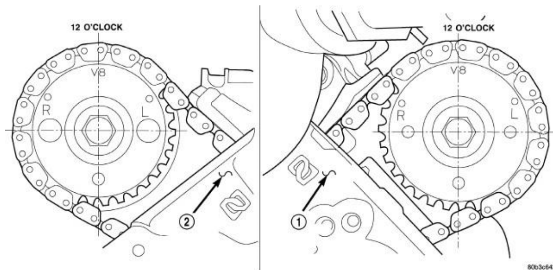
Fig. 73: Camshaft Sprocket V8 Marks Courtesy of CHRYSLER LLC
