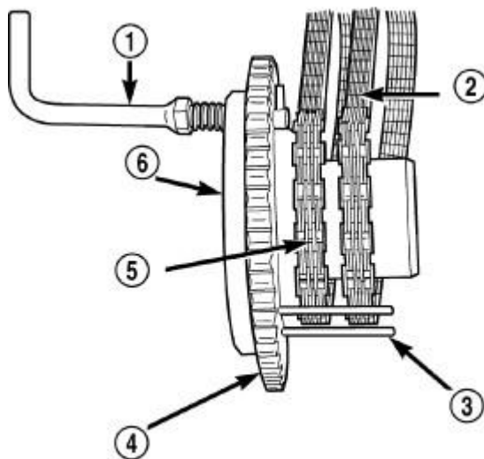
Fig. 224: Installing Secondary Timing Chains on Idler Sprocket Courtesy of CHRYSLER LLC
