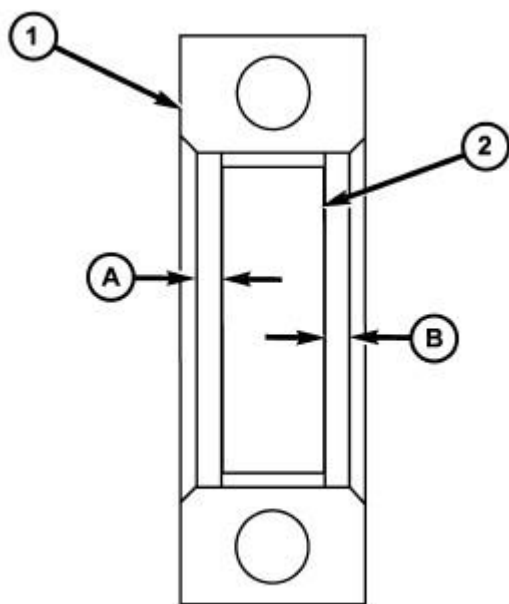
Fig. 130: Bearing Insert Location Courtesy of CHRYSLER LLC
