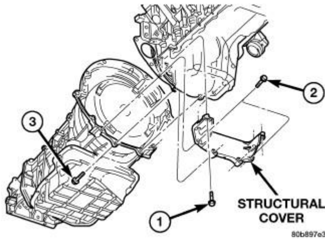
Fig. 183: Structural Cover Courtesy of CHRYSLER LLC
