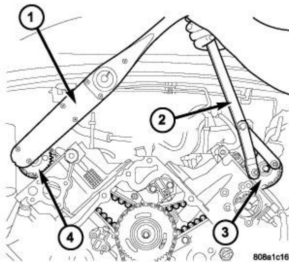
Fig. 226: Tightening Right Side Camshaft Sprocket Bolt Courtesy of CHRYSLER LLC
