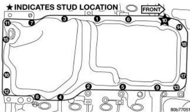
Fig. 181: Oil Pan Mounting Bolts and Oil Pan
