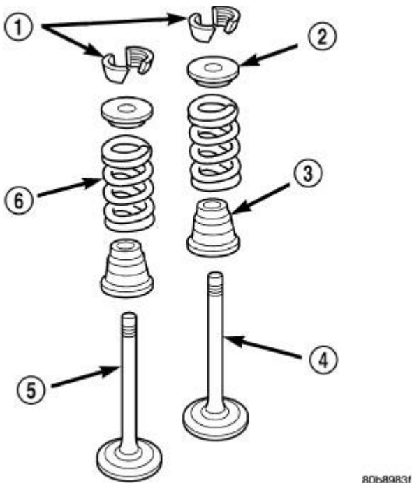
Fig. 127: Valve Assembly Configuration Courtesy of CHRYSLER LLC
