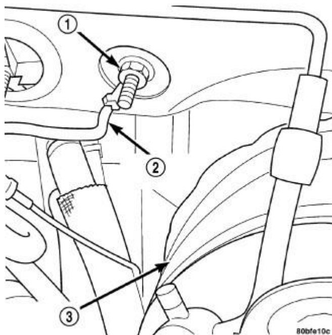
Fig. 20: Body Ground Strap-Left Side Removal / Installation Courtesy of CHRYSLER LLC
