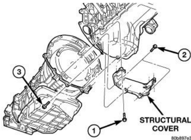
Fig. 28: Structural Cover Courtesy of CHRYSLER LLC
