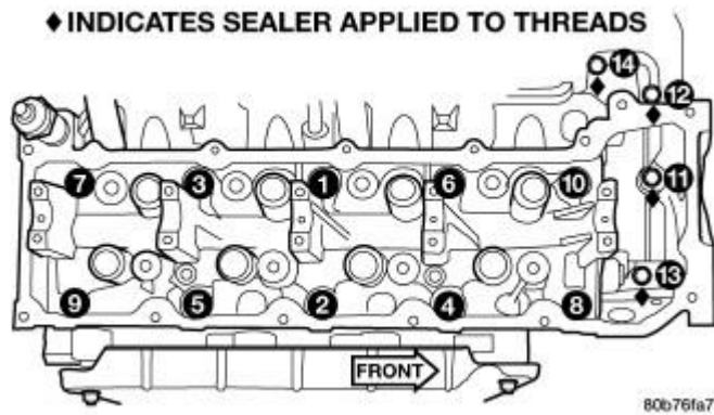
Fig. 70: Cylinder Head Tightening Sequence Courtesy of CHRYSLER LLC
