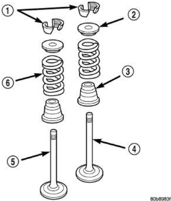
Fig. 126: Valve Assembly Configuration
