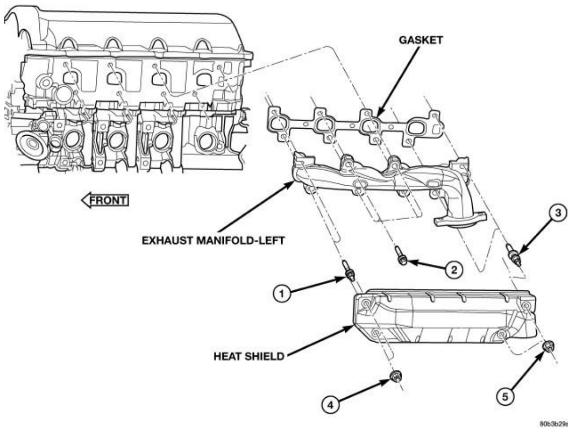
Fig. 197: Exhaust Manifold-Left Courtesy of CHRYSLER LLC
