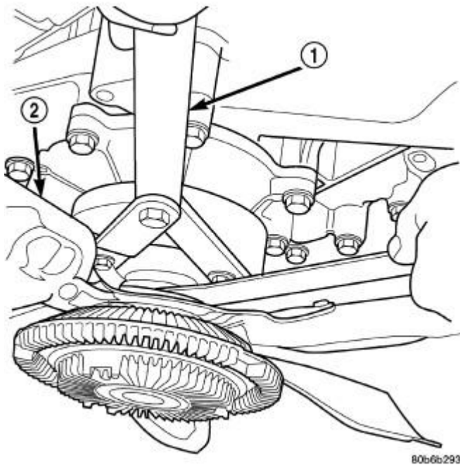
Fig. 147: Fan Assembly-Removal/Installation Courtesy of CHRYSLER LLC
