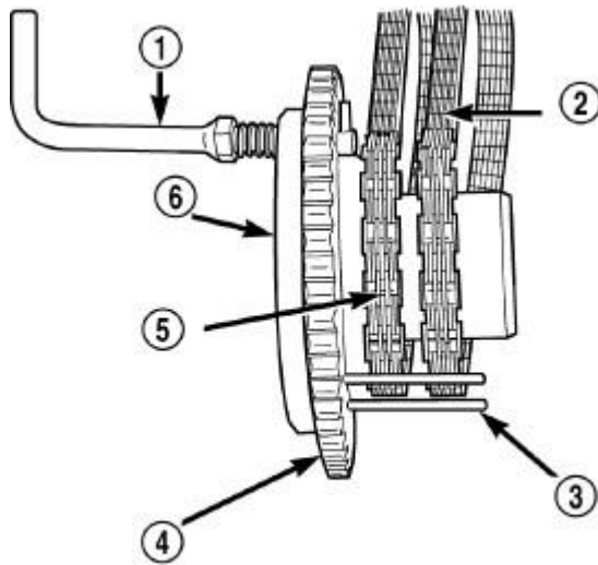
Fig. 74: Installing Secondary Timing Chains on Idler Sprocket Courtesy of CHRYSLER LLC
