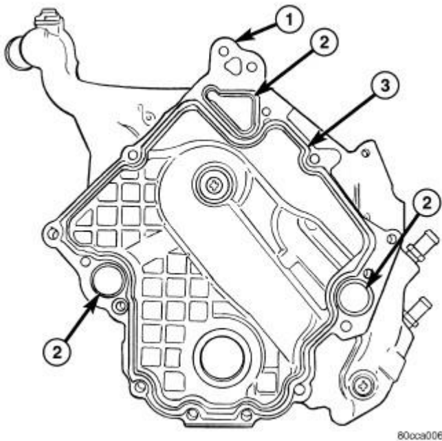
Fig. 230: Timing Cover Sealant Courtesy of CHRYSLER LLC
