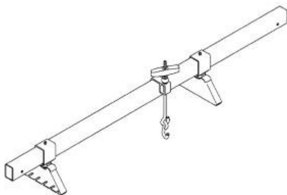
Fig. 43: Engine Support Fixture 8534B Courtesy of CHRYSLER LLC
