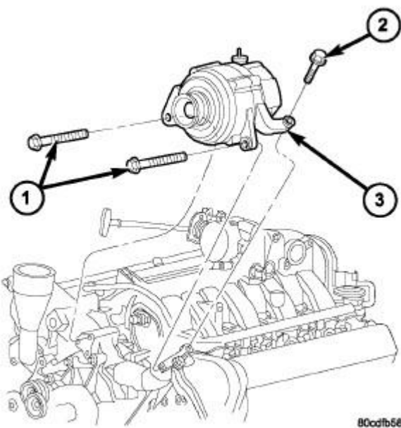
Fig. 10: REMOVE / INSTALL GENERATOR - 3.7L / 4.7L Courtesy of CHRYSLER LLC
