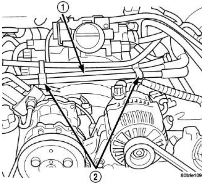
Fig. 11: Heater Hoses and Tubes Removal / Installation Courtesy of CHRYSLER LLC
