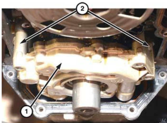
Fig. 410: Engine Oil Pump Courtesy of CHRYSLER GROUP, LLC
