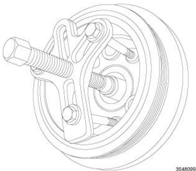
Fig. 185: Removing Vibration Damper Courtesy of CHRYSLER GROUP, LLC
