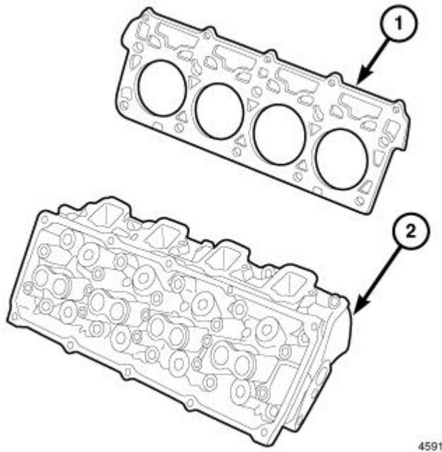
Fig. 95: Cylinder Head & Gasket Courtesy of CHRYSLER GROUP, LLC
