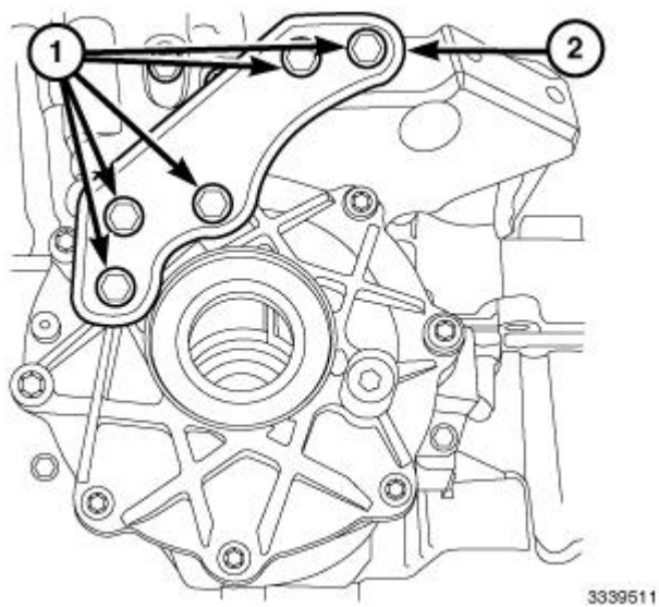
Fig. 271: Differential Support Bracket & Retaining Bolts Courtesy of CHRYSLER GROUP, LLC
