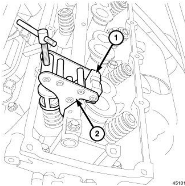
Fig. 135: Intake Valve Spring Removal/Installation Courtesy of CHRYSLER GROUP, LLC
