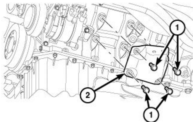
Fig. 260: Engine Mount-To-Engine Block Mounting Brackets & Retaining Bolts Courtesy of CHRYSLER GROUP, LLC
