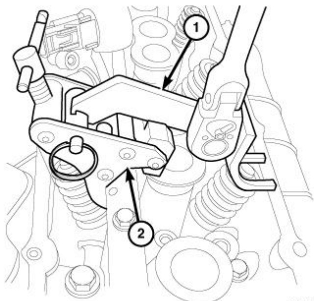
Fig. 137: Valve Spring Tool Adapter
