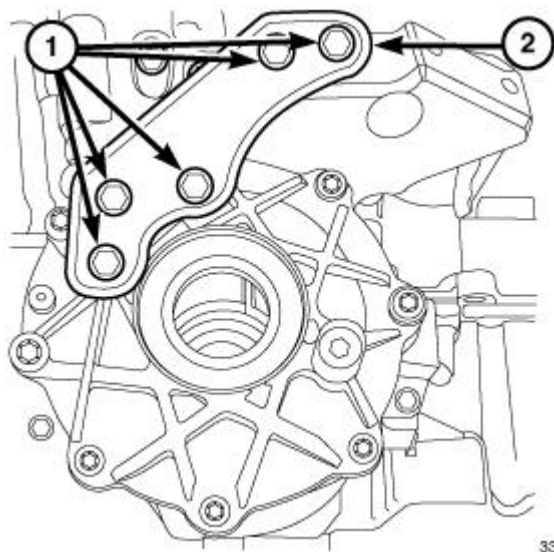
Fig. 282: Differential Support Bracket & Retaining Bolts Courtesy of CHRYSLER GROUP, LLC
