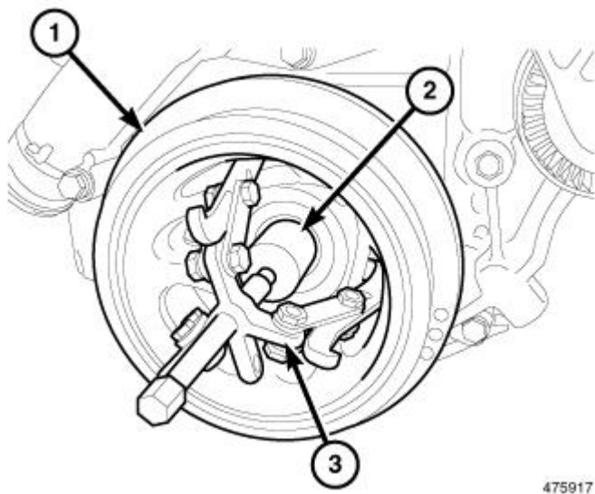
Fig. 206: Removing Vibration Damper Courtesy of CHRYSLER GROUP, LLC
