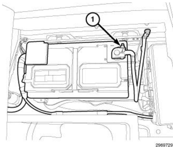
Fig. 82: Negative Battery Cable
