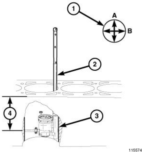
Fig. 224: Measuring Cylinder Bore Diameter Courtesy of CHRYSLER GROUP, LLC
