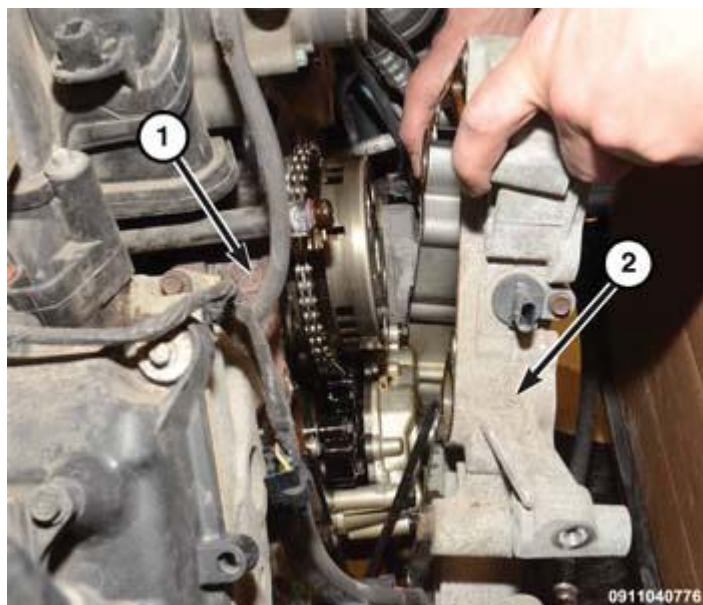
Fig. 420: Removing/Installing Engine Timing Cover Courtesy of CHRYSLER GROUP, LLC
