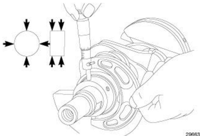
Fig. 149: Crankshaft Journal Measurements - Typical Courtesy of CHRYSLER GROUP, LLC
