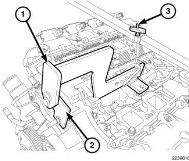
Fig. 286: Engine Lift Fixture & Adapter Courtesy of CHRYSLER GROUP, LLC
