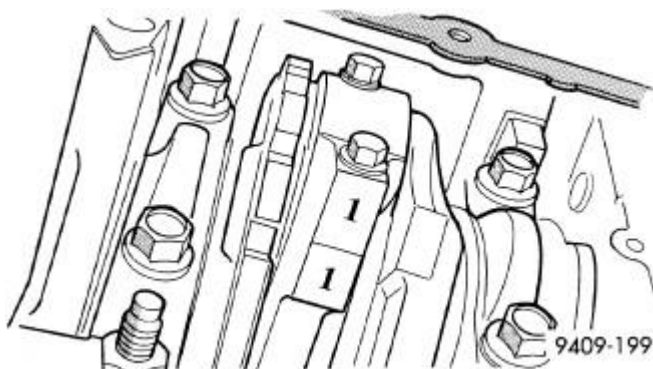
Fig. 232: Identifying Mark On Connecting Rod And Bearing Cap Courtesy of CHRYSLER GROUP, LLC
