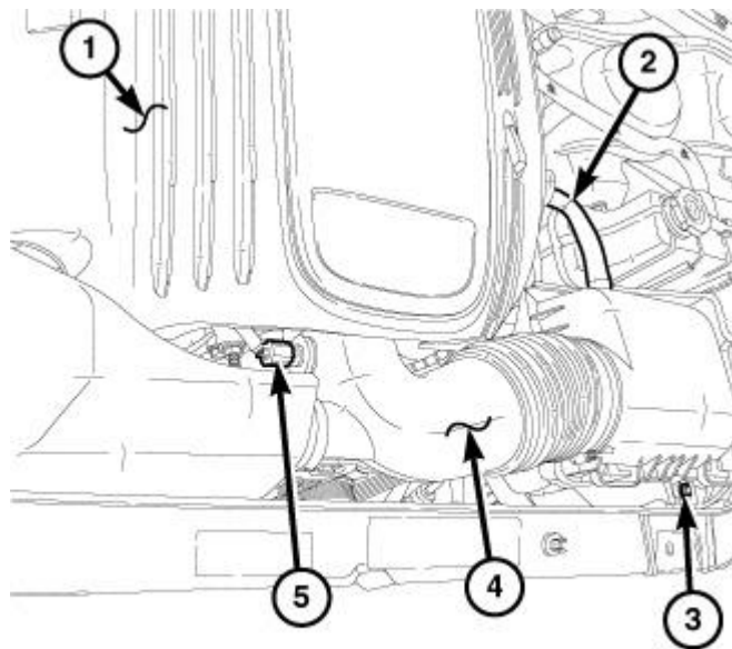
Fig. 365: Air Filter Assembly Courtesy of CHRYSLER GROUP, LLC
