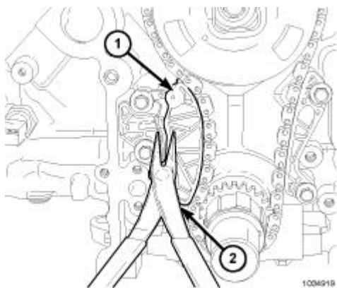
Fig. 399: Chain Tensioner Arm Courtesy of CHRYSLER GROUP, LLC
