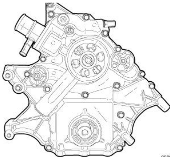
Fig. 168: Engine Timing Cover
