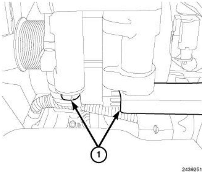
Fig. 361: Lower Generator Retaining Bolts Courtesy of CHRYSLER GROUP, LLC
