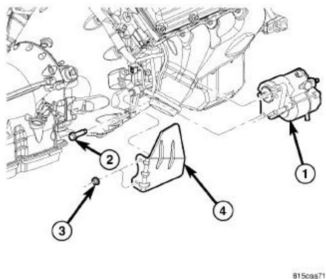
Fig. 21: Removing/Installing Starter
