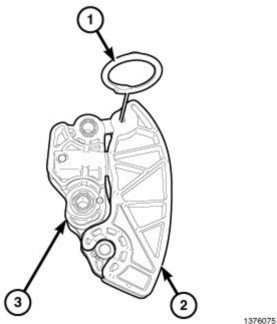
Fig. 429: Tensioner Pin, Guide Shoe & Tensioner Body Courtesy of CHRYSLER GROUP, LLC
