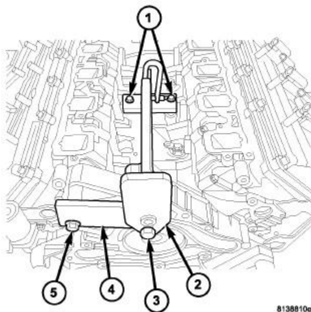
Fig. 40: Engine Lift Fixture And Adapter Courtesy of CHRYSLER GROUP, LLC
