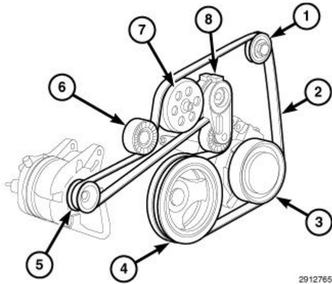
Fig. 87: Drive Belt Tensioner And Drive Belt Routing
