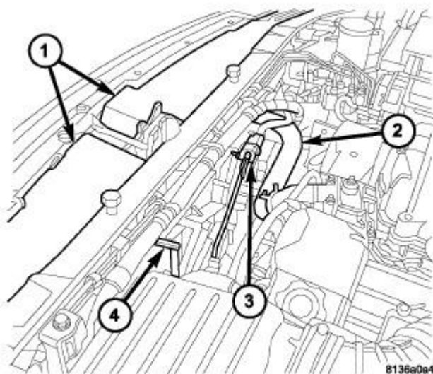
Fig. 28: Radiator Fan Assembly Courtesy of CHRYSLER GROUP, LLC
