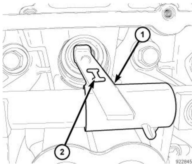
Fig. 139: Intake Rocker Arm Marking Courtesy of CHRYSLER GROUP, LLC
