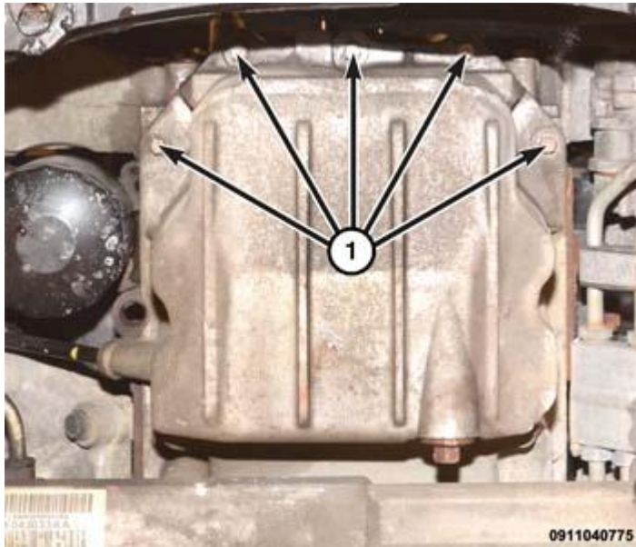
Fig. 424: Front Oil Pan Retaining Bolts Courtesy of CHRYSLER GROUP, LLC
