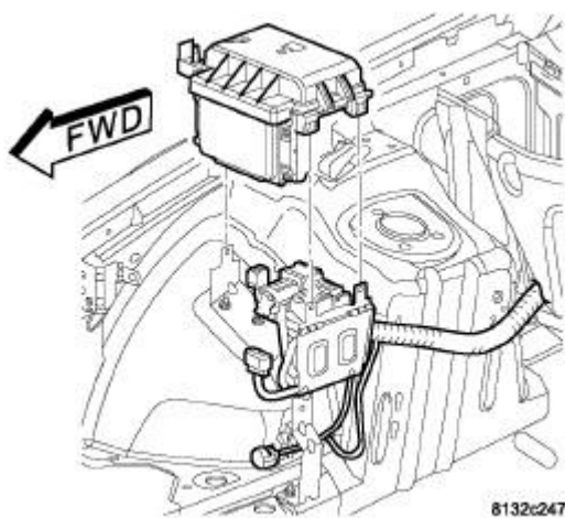
Fig. 34: TIPM/PDC Mounting Bracket Courtesy of CHRYSLER GROUP, LLC
