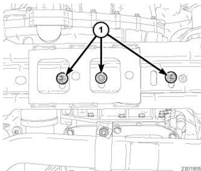
Fig. 180: Transmission Mount To Crossmember Retaining Nuts Courtesy of CHRYSLER GROUP, LLC
