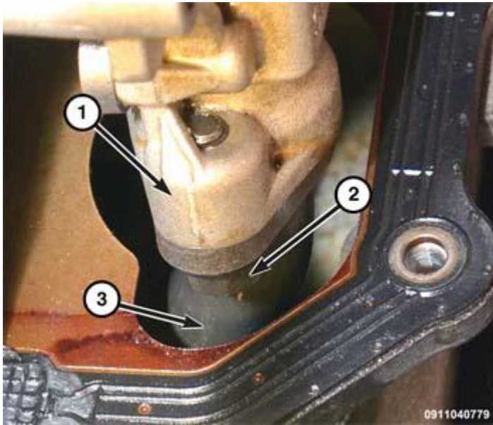
Fig. 411: Engine Oil Pump Body, Oil Pump Pickup Tube & Retaining Bolt Courtesy of CHRYSLER GROUP, LLC
