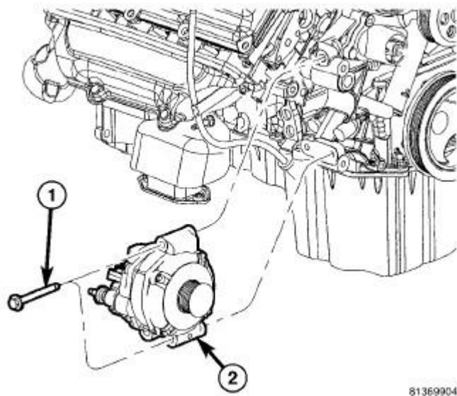
Fig. 155: Generator - 5.7L Courtesy of CHRYSLER GROUP, LLC
