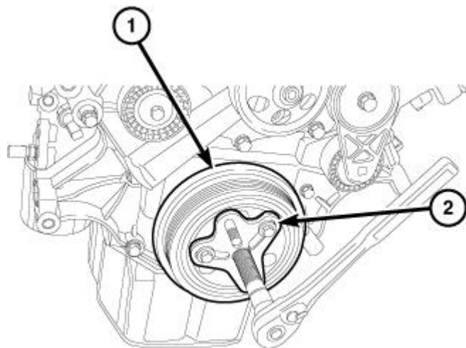
Fig. 207: Vibration Damper & Bolt Grip Puller Courtesy of CHRYSLER GROUP, LLC
