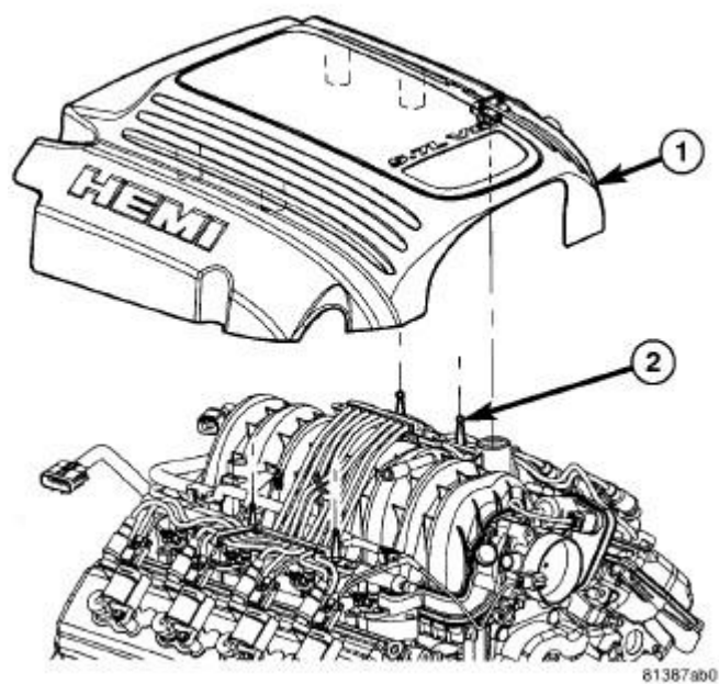
Fig. 340: Engine Cover
