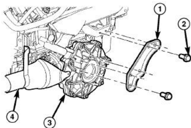
Fig. 336: Front Drive Axle Housing Courtesy of CHRYSLER GROUP, LLC
