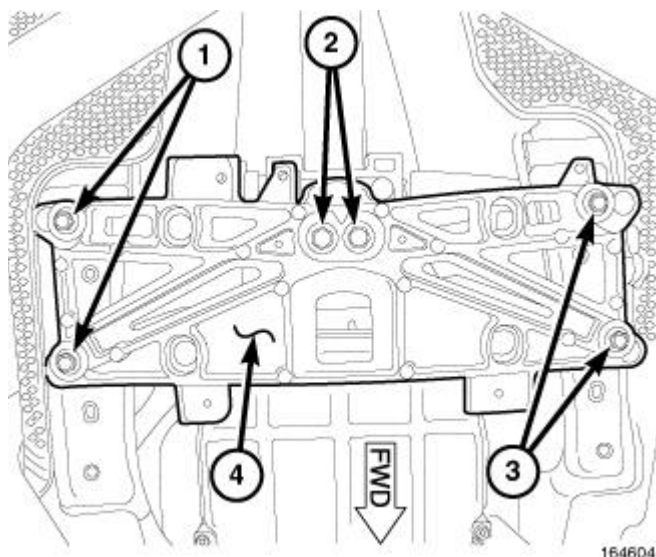
Fig. 292: Rear Cross Member & Bolts Courtesy of CHRYSLER GROUP, LLC
