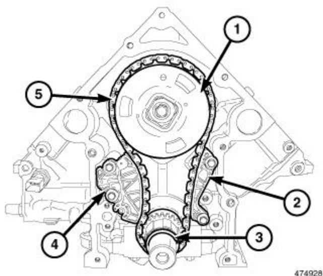
Fig. 160: Timing Chain, Sprockets, Timing Chain Tensioner & Guide Courtesy of CHRYSLER GROUP, LLC
