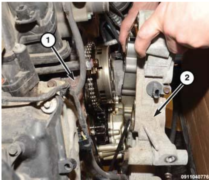
Fig. 423: Removing/Installing Engine Timing Cover Courtesy of CHRYSLER GROUP, LLC
