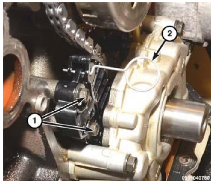
Fig. 413: Crankshaft Gear Mark & Timing Chain Mark Courtesy of CHRYSLER GROUP, LLC
