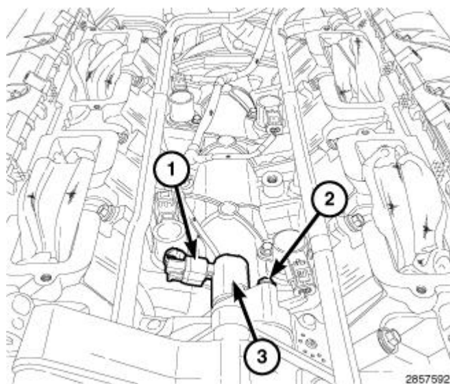
Fig. 12: Oil Control Valve, Electrical Connector & Retaining Bolt
