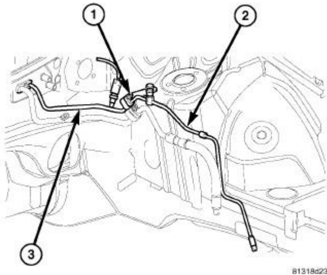
Fig. 66: Removing/Installing A/C Liquid Front Line Courtesy of CHRYSLER GROUP, LLC
