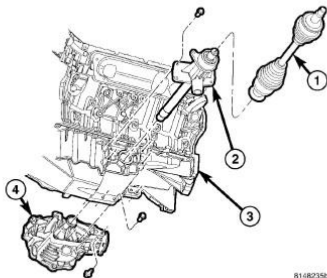
Fig. 329: Front Drive Axle Assembly
