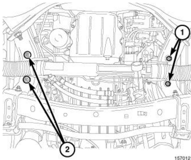
Fig. 229: Engine Mount Nuts
