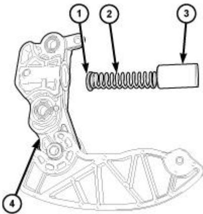
Fig. 428: Tensioner Body, Washer, Spring & Plunger Courtesy of CHRYSLER GROUP, LLC
