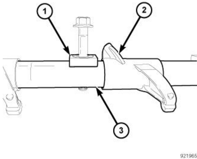
Fig. 140: Rocker Shaft Retainers Courtesy of CHRYSLER GROUP, LLC
