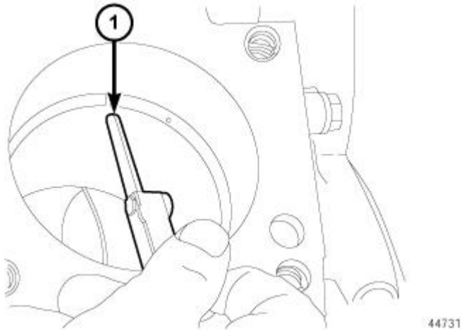
Fig. 219: Checking Piston Ring End Gap Using Feeler Gauge Courtesy of CHRYSLER GROUP, LLC
