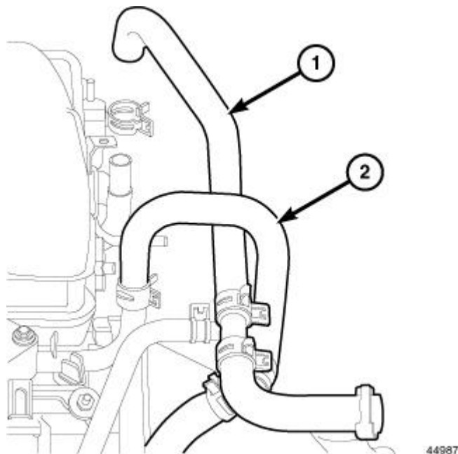
Fig. 57: Heater Hose Supply
