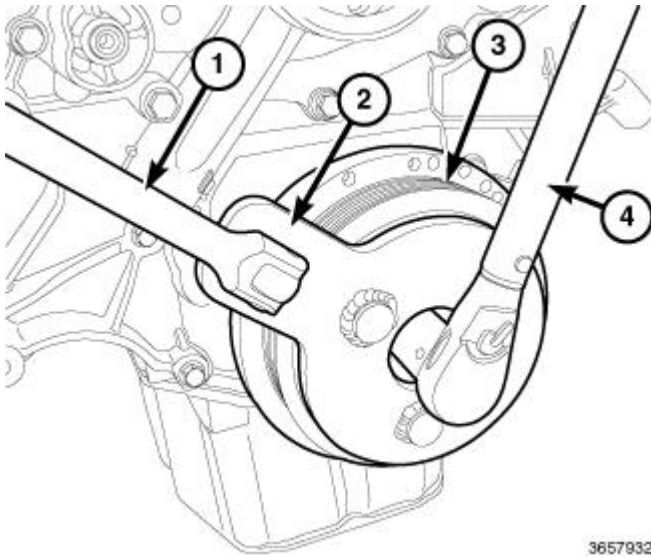
Fig. 209: Installing Vibration Damper Onto Vibration Pulley Courtesy of CHRYSLER GROUP, LLC
