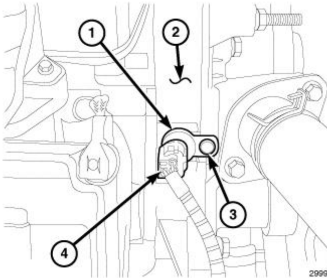
Fig. 426: Camshaft Position Sensor, Connector, Bolt & Timing Cover Courtesy of CHRYSLER GROUP, LLC
