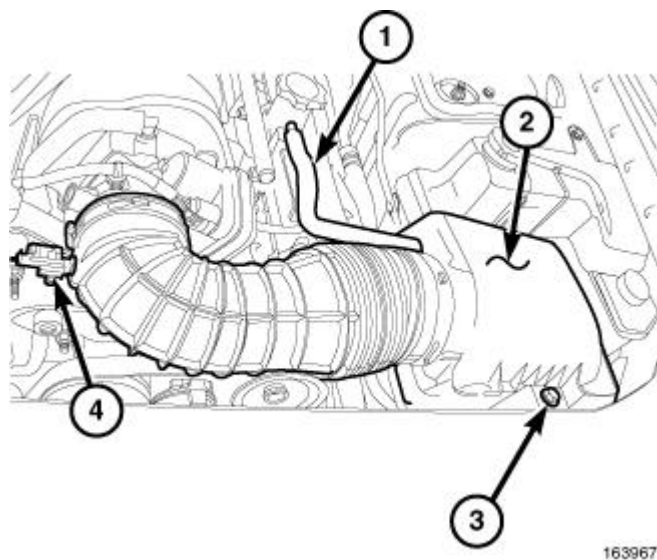
Fig. 228: Air Duct To Throttle Body Courtesy of CHRYSLER GROUP, LLC
