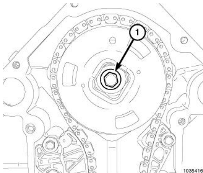
Fig. 415: Camshaft Phaser Retaining Bolt Courtesy of CHRYSLER GROUP, LLC
