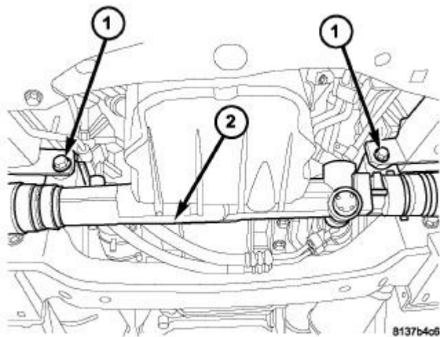
Fig. 311: Gear Mounting Bolts Courtesy of CHRYSLER GROUP, LLC
