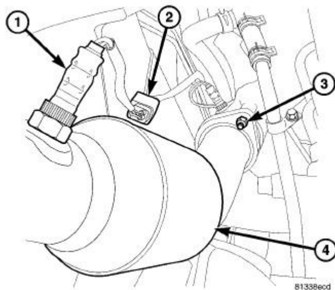
Fig. 367: Oxygen Sensor, Oxygen Sensor Connector, Ball Flange Nut & LH Catalytic Converter
