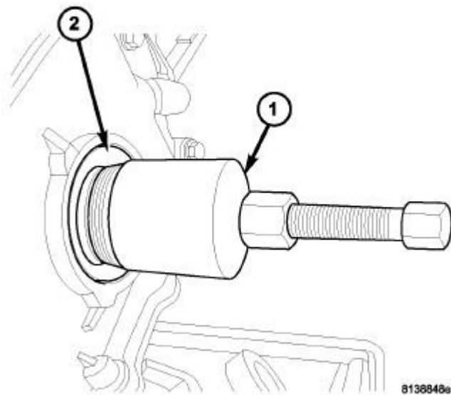
Fig. 246: Front Crankshaft Seal Removal Courtesy of CHRYSLER GROUP, LLC
