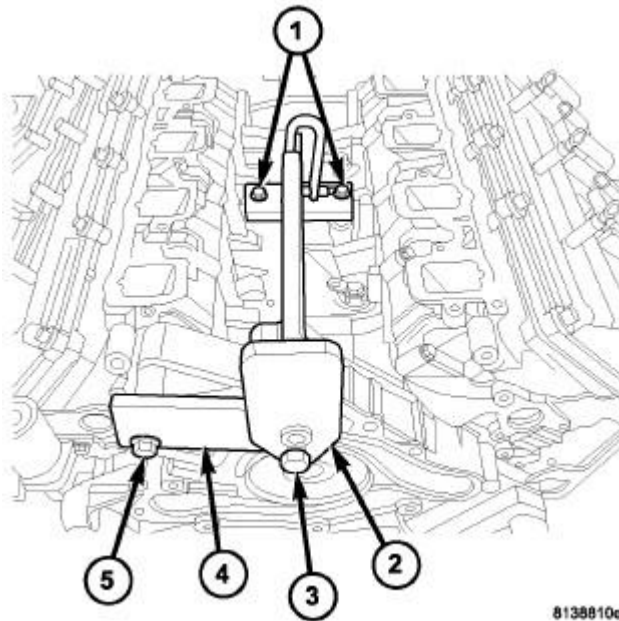
Fig. 339: Engine Lift Fixture And Adapter Courtesy of CHRYSLER GROUP, LLC
