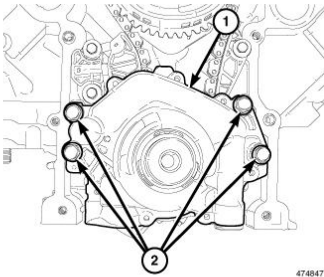
Fig. 342: Oil Pump Retaining Bolts
