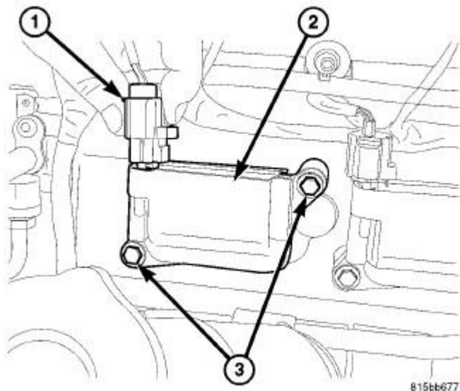
Fig. 106: Ignition Coil Mounting Bolts Courtesy of CHRYSLER GROUP, LLC
