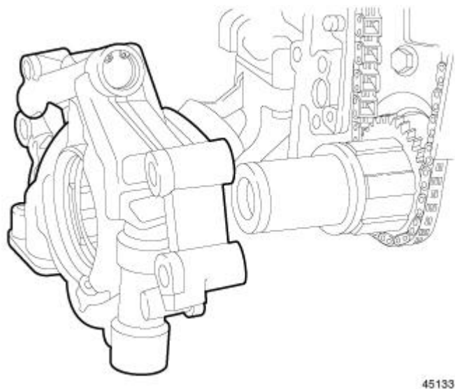
Fig. 167: Remove/Install Oil Pump Courtesy of CHRYSLER GROUP, LLC
