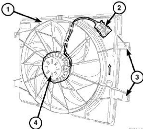
Fig. 14: Cooling Fan Module Components Courtesy of CHRYSLER GROUP, LLC
