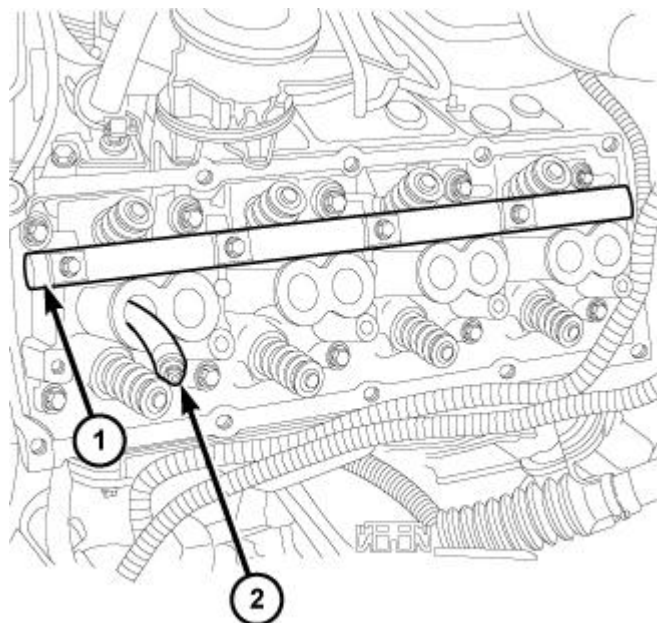
Fig. 134: Rocker Shaft Courtesy of CHRYSLER GROUP, LLC
