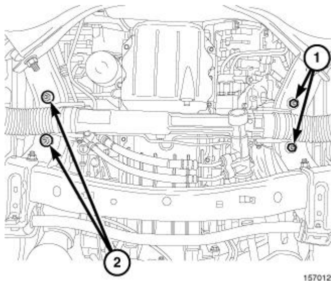
Fig. 312: Engine Mount Nuts Courtesy of CHRYSLER GROUP, LLC
