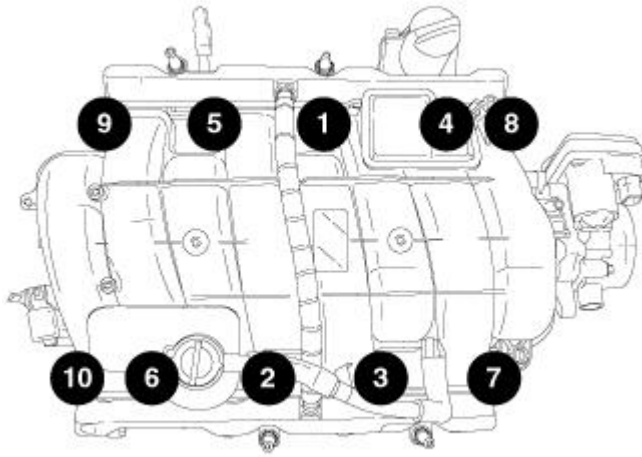
Fig. 102: Intake Manifold Removal & Tightening Sequence Courtesy of CHRYSLER GROUP, LLC
