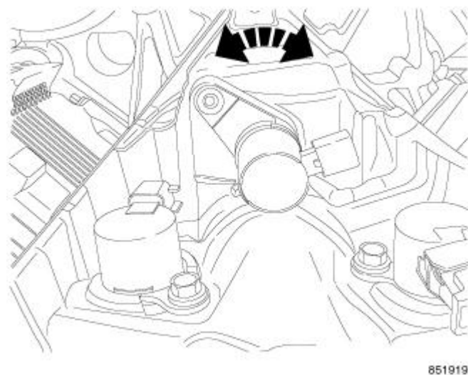
Fig. 254: Oil Control Valve Courtesy of CHRYSLER GROUP, LLC
