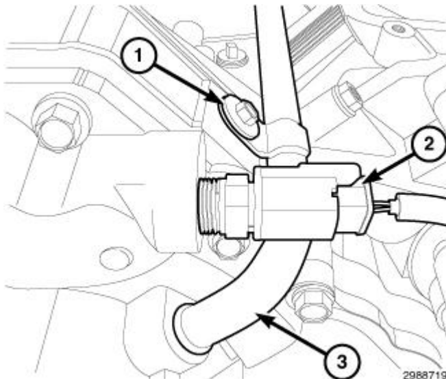
Fig. 427: Coolant Temperature (ECT) Sensor Electrical Connector, Heater Tube & Retaining Bolt Courtesy of CHRYSLER GROUP, LLC
