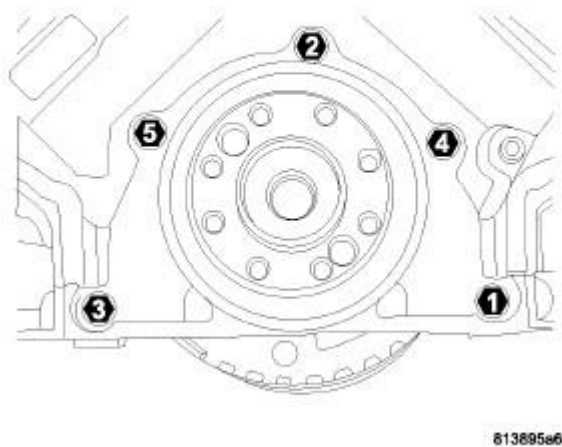
Fig. 186: Rear Seal Retainer Torque Sequence Courtesy of CHRYSLER GROUP, LLC
