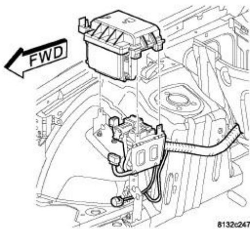
Fig. 372: TIPM/PDC Mounting Bracket Courtesy of CHRYSLER GROUP, LLC
