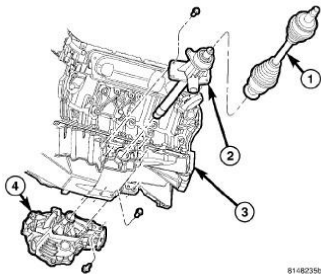
Fig. 335: Front Drive Axle Assembly Courtesy of CHRYSLER GROUP, LLC
