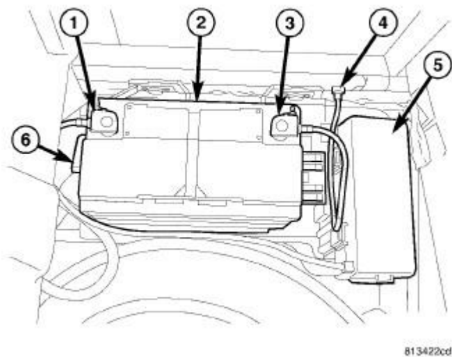
Fig. 321: Battery System Components And PDC Cover Courtesy of CHRYSLER GROUP, LLC
