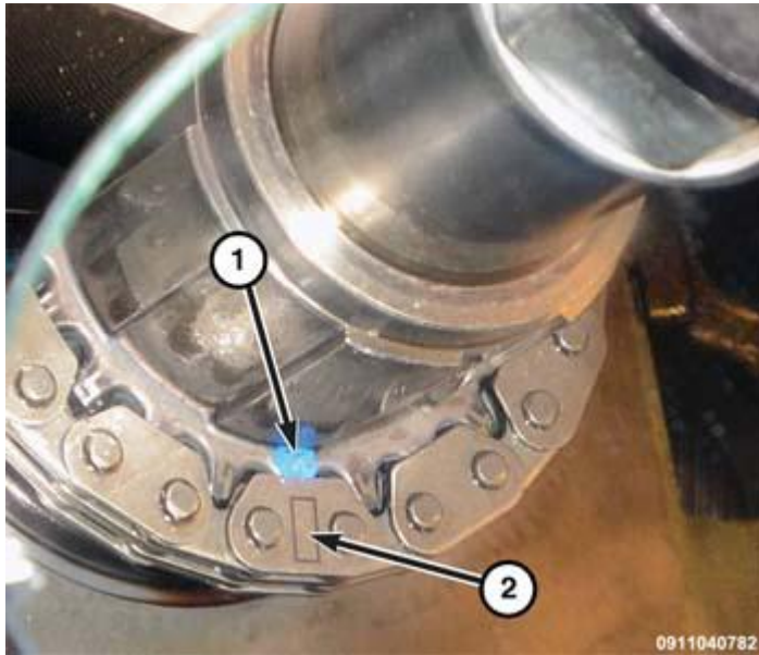
Fig. 407: Aligning Camshaft Timing Chain Marks Courtesy of CHRYSLER GROUP, LLC
