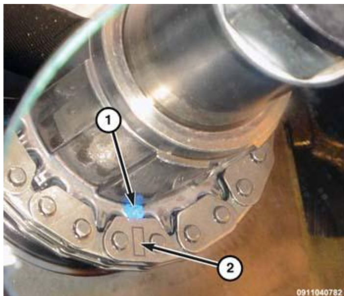
Fig. 398: Aligning Camshaft Timing Chain Marks Courtesy of CHRYSLER GROUP, LLC
