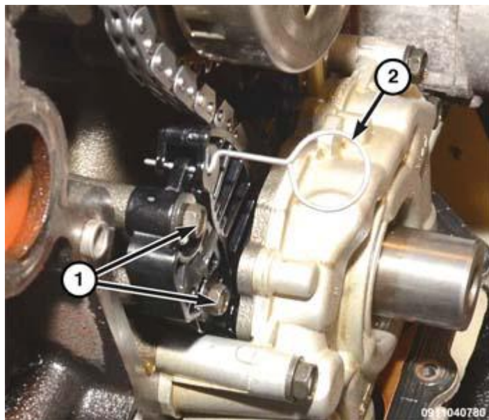
Fig. 400: Crankshaft Gear Mark & Timing Chain Mark Courtesy of CHRYSLER GROUP, LLC
