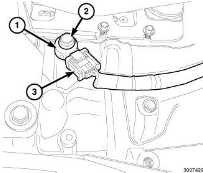
Fig. 368: Knock Sensor, Electrical Connector & Bolt Courtesy of CHRYSLER GROUP, LLC
