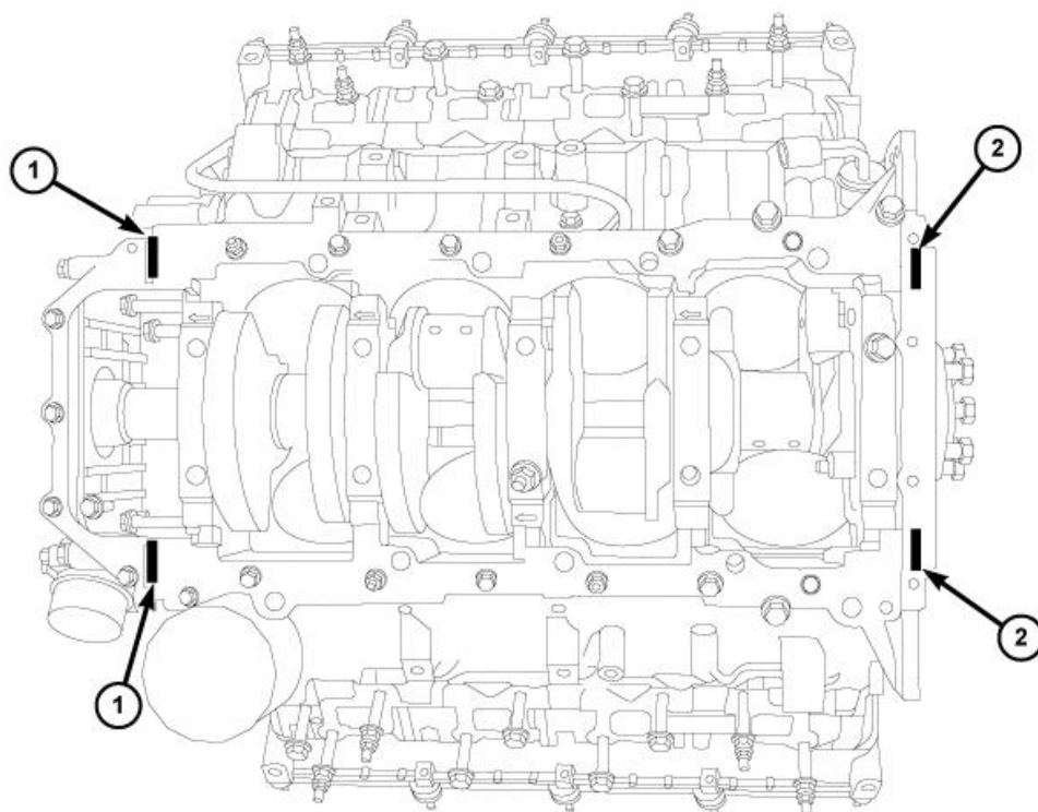
Fig. 332: T-Joint RTV Application
