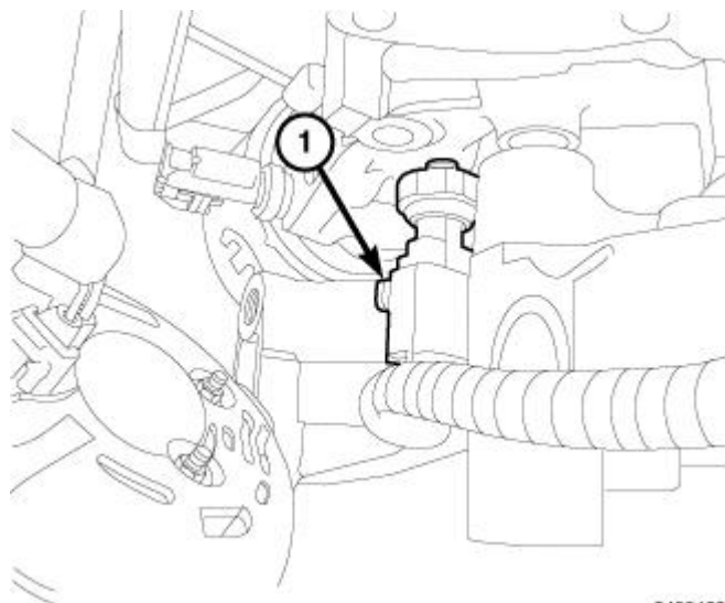
Fig. 349: Oil Pressure Sensor Electrical Connector Courtesy of CHRYSLER GROUP, LLC
