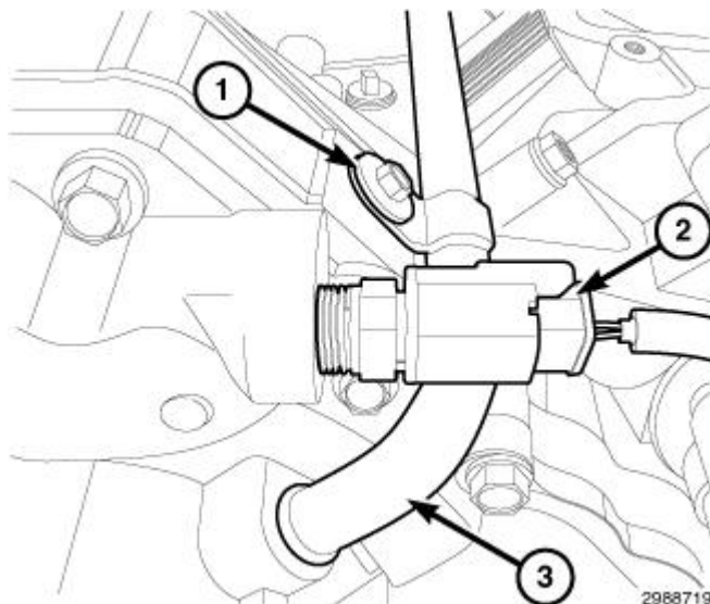
Fig. 54: Coolant Temperature (ECT) Sensor Electrical Connector, Heater Tube & Retaining Bolt
