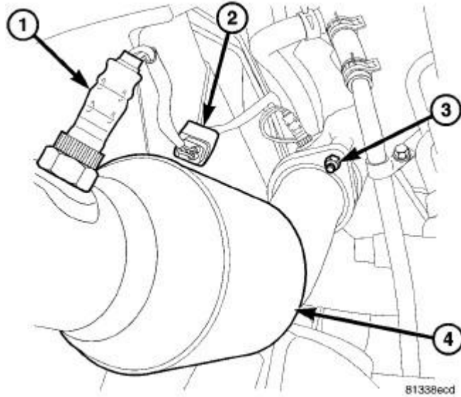
Fig. 86: Oxygen Sensor, Oxygen Sensor Connector, Ball Flange Nut & LH Catalytic Converter Courtesy of CHRYSLER GROUP, LLC
