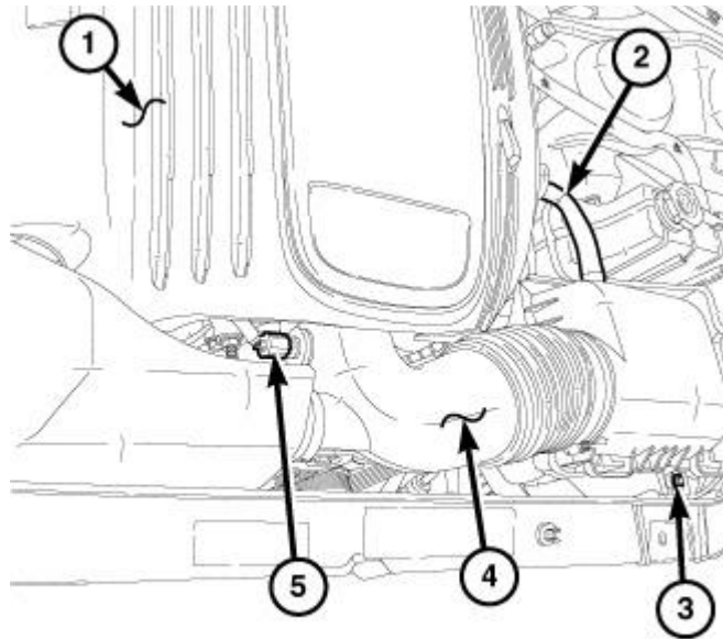
Fig. 7: Air Filter Assembly
