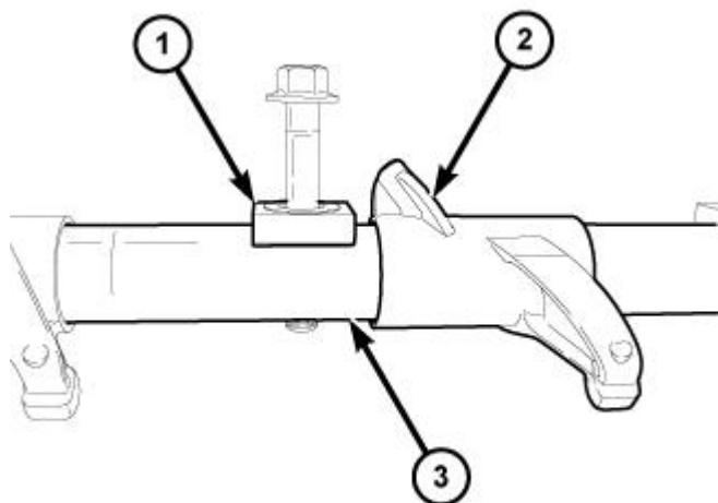
Fig. 120: Rocker Shaft Retainers Courtesy of CHRYSLER GROUP, LLC
