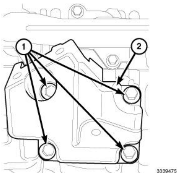
Fig. 283: Engine Mount Isolator Bracket & Retaining Bolts Courtesy of CHRYSLER GROUP, LLC
