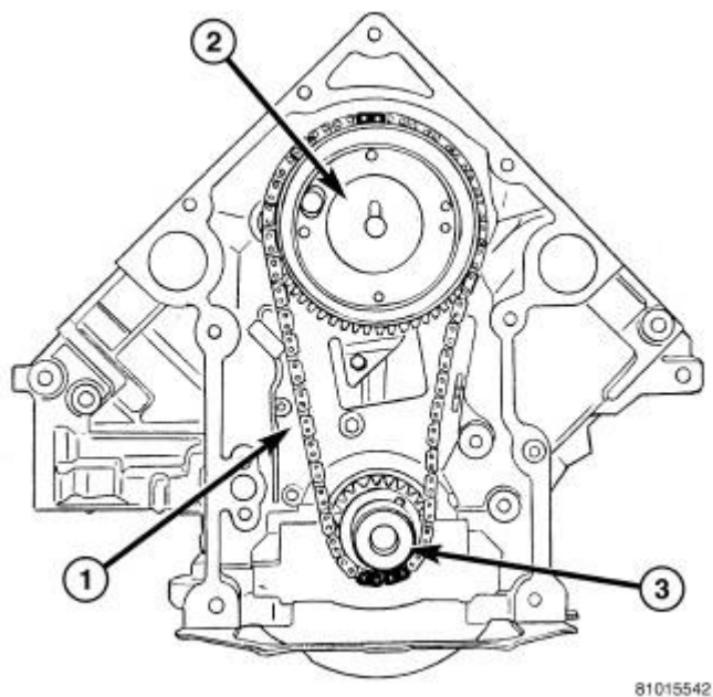
Fig. 189: 5.7L Timing Mark Alignment Courtesy of CHRYSLER GROUP, LLC
