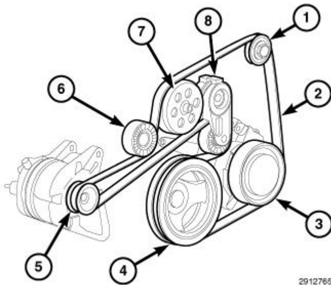
Fig. 99: Drive Belt Tensioner And Drive Belt Routing Courtesy of CHRYSLER GROUP, LLC
