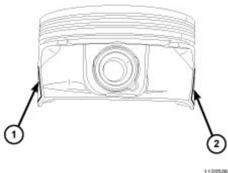
Fig. 225: Piston Diameter Measuring Points Courtesy of CHRYSLER GROUP, LLC
