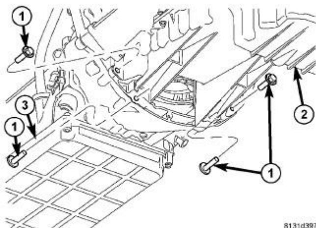
Fig. 43: Remove/Install Transmission To Oil Pan Bolts Courtesy of CHRYSLER GROUP, LLC
