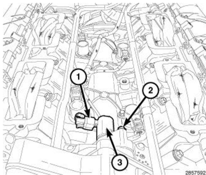
Fig. 279: Oil Control Valve, Electrical Connector & Retaining Bolt Courtesy of CHRYSLER GROUP, LLC
