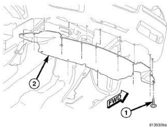
Fig. 341: Locating Front Belly Pan And Screws
