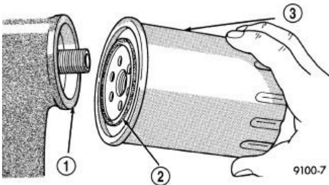
Fig. 308: Installing Engine Oil Filter Courtesy of CHRYSLER GROUP, LLC
