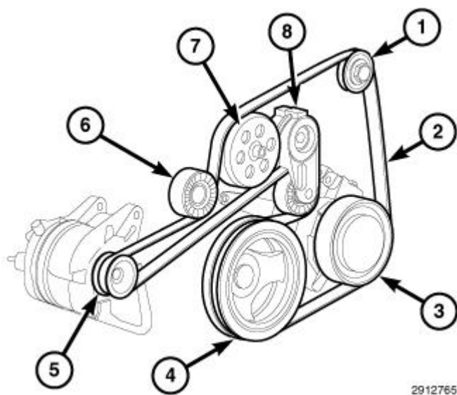
Fig. 70: Drive Belt Tensioner And Drive Belt Routing Courtesy of CHRYSLER GROUP, LLC
