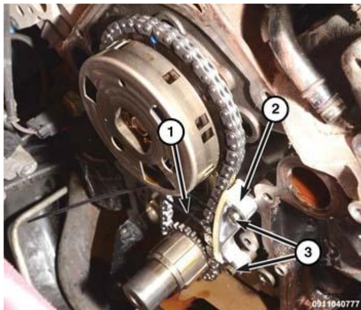
Fig. 409: Timing Chain Guide & Bolts Courtesy of CHRYSLER GROUP, LLC
