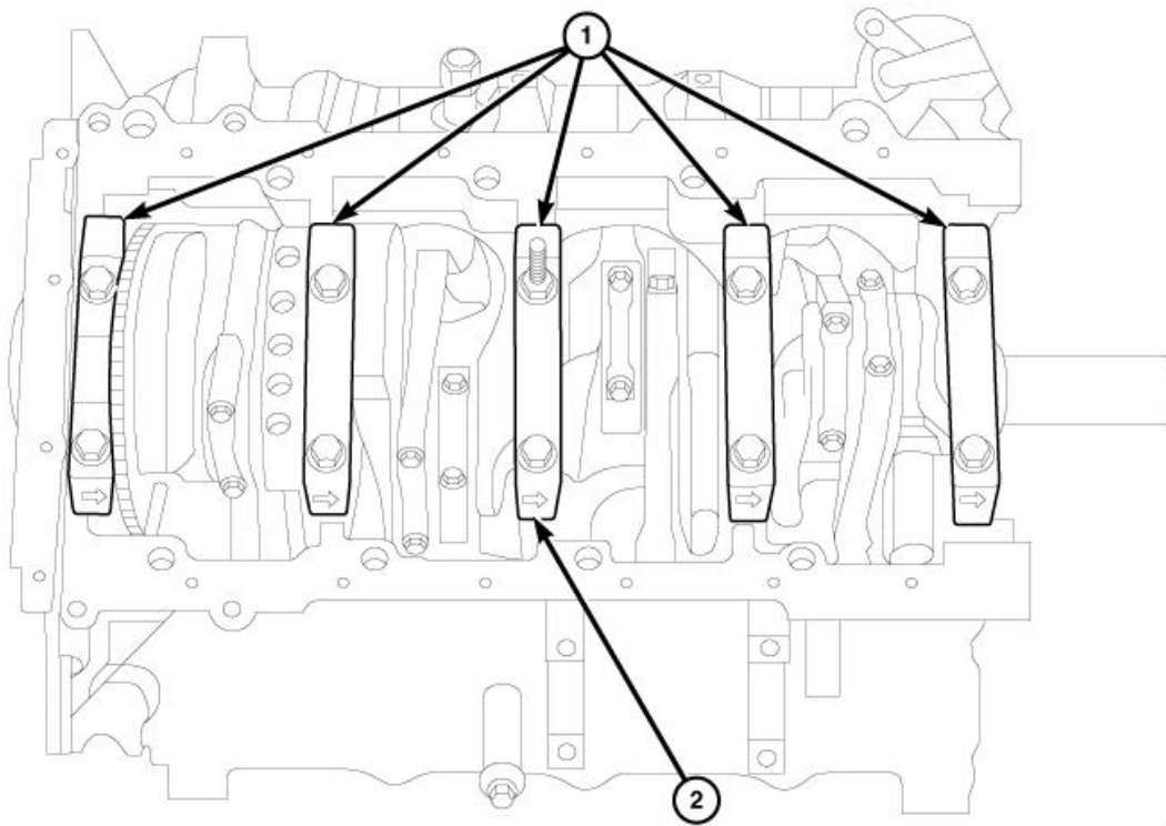
Fig. 190: Main Bearing Caps Courtesy of CHRYSLER GROUP, LLC
