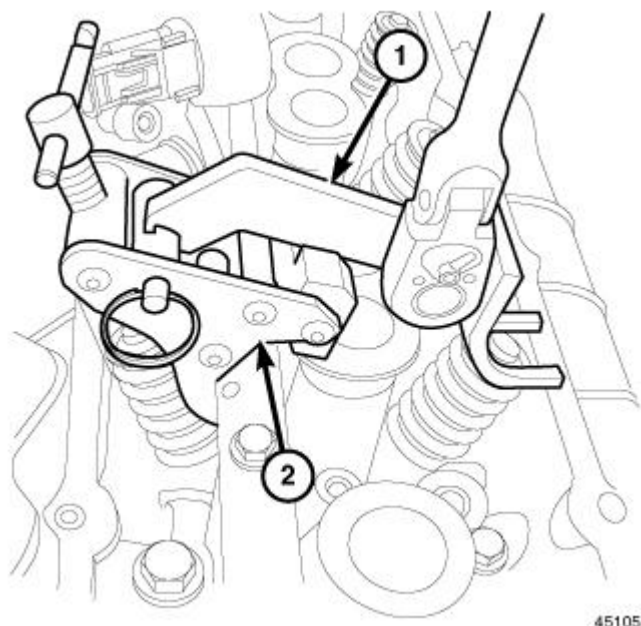
Fig. 136: Valve Spring Tool Adapter Courtesy of CHRYSLER GROUP, LLC
