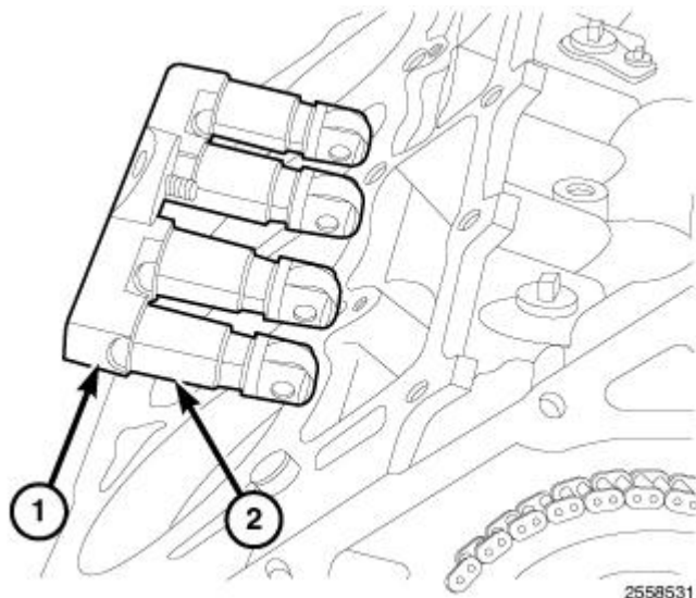
Fig. 213: Tappet Guide Holder Assembly Courtesy of CHRYSLER GROUP, LLC
