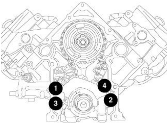
Fig. 346: Oil Pump Retaining Bolt Tightening Sequence Courtesy of CHRYSLER GROUP, LLC
