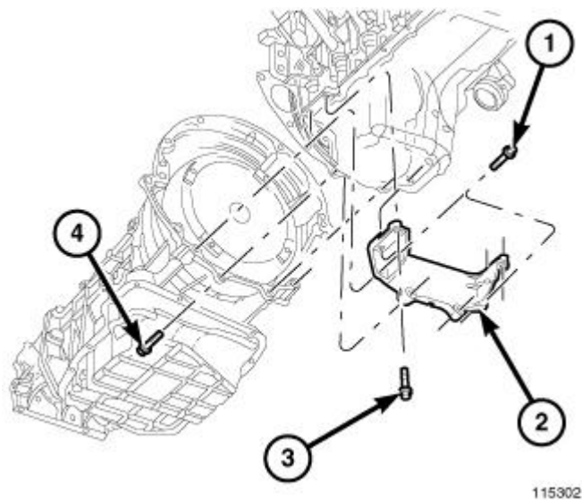
Fig. 182: Structural Cover
