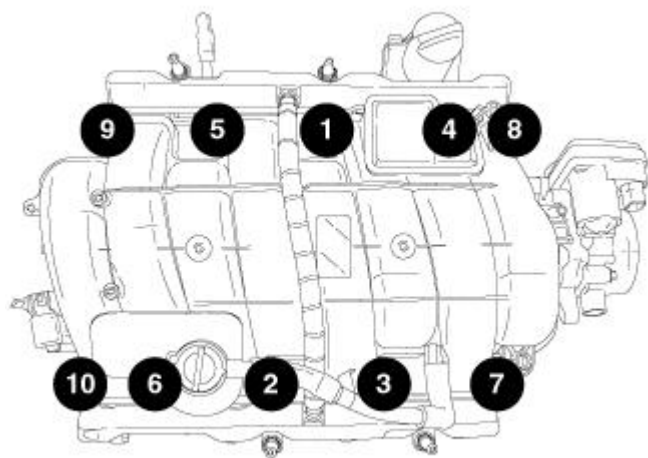
Fig. 11: Intake Manifold Removal & Tightening Sequence
