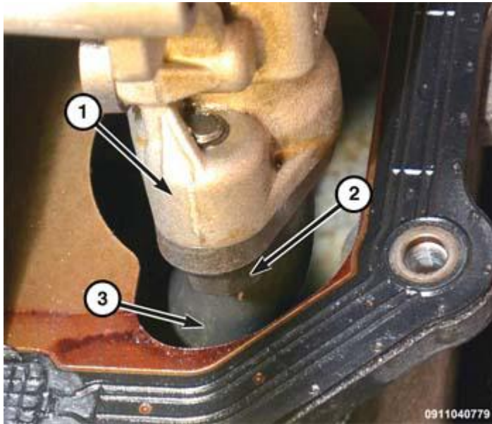
Fig. 402: Engine Oil Pump Body, Oil Pump Pickup Tube & Retaining Bolt Courtesy of CHRYSLER GROUP, LLC
