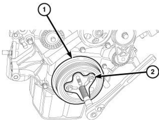
Fig. 245: Vibration Damper & Bolt Grip Puller Courtesy of CHRYSLER GROUP, LLC
