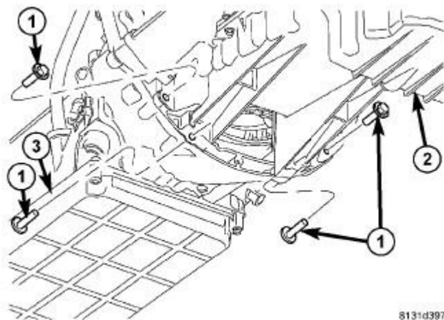
Fig. 38: Remove/Install Transmission To Oil Pan Bolts Courtesy of CHRYSLER GROUP, LLC
