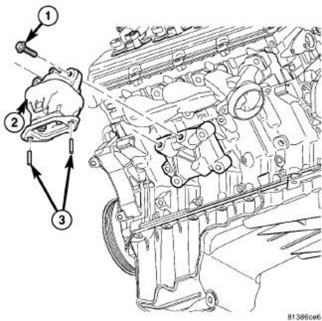
Fig. 325: Engine Hydromount LH Courtesy of CHRYSLER GROUP, LLC
