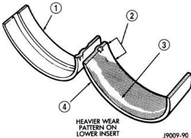
Fig. 151: Main Bearing Wear Patterns
