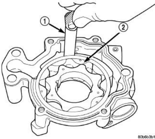
Fig. 343: Measuring Outer Rotor Clearance in Housing Courtesy of CHRYSLER GROUP, LLC
