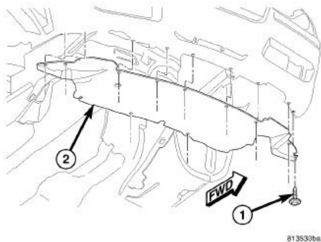
Fig. 310: Locating Front Belly Pan And Screws Courtesy of CHRYSLER GROUP, LLC
