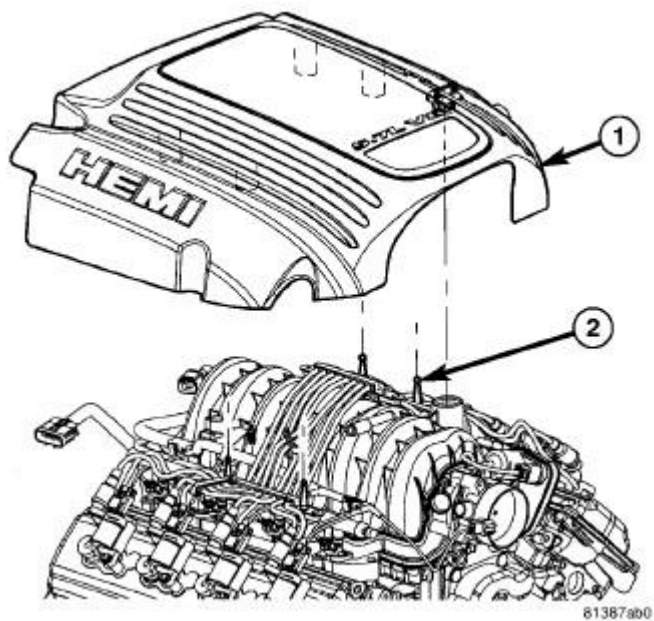
Fig. 322: Engine Cover
