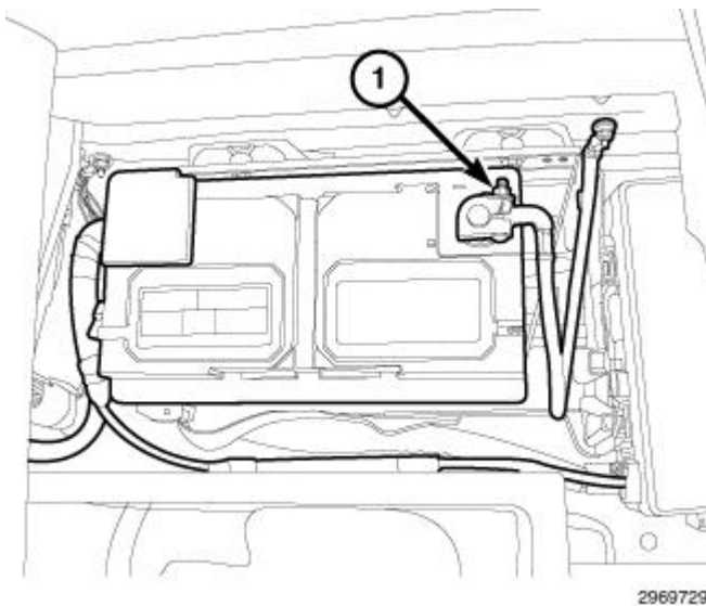
Fig. 291: Negative Battery Cable
