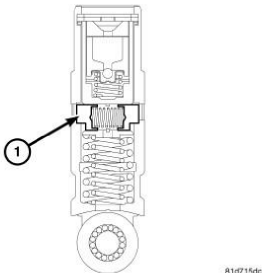
Fig. 77: MDS Lifter Cross-Section Courtesy of CHRYSLER GROUP, LLC
