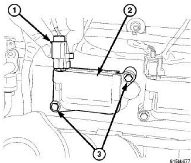
Fig. 129: Ignition Coil Mounting Bolts
