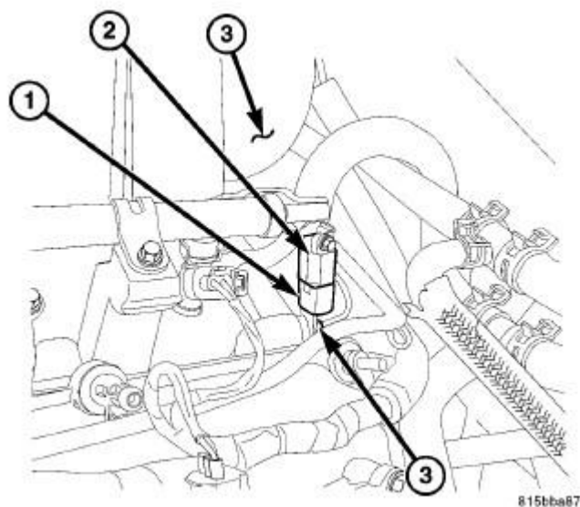
Fig. 35: Ignition Capacitor, Electrical Connector & Intake Manifold Courtesy of CHRYSLER GROUP, LLC
