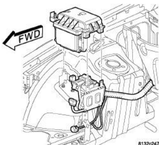
Fig. 69: TIPM/PDC Mounting Bracket Courtesy of CHRYSLER GROUP, LLC
