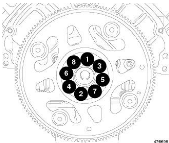
Fig. 211: Flexplate Retaining Bolt Removal & Tightening Sequence Courtesy of CHRYSLER GROUP, LLC
