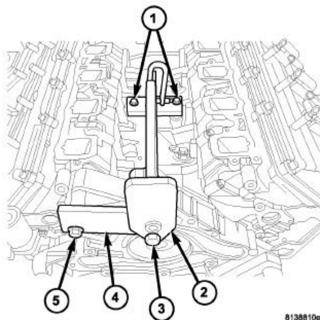
Fig. 323: Engine Lift Fixture And Adapter Courtesy of CHRYSLER GROUP, LLC
