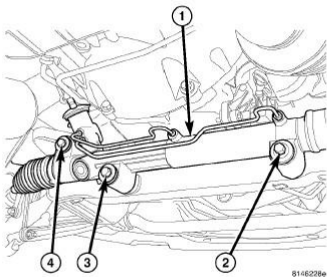
Fig. 326: Steering Rack Mounting Bolts Courtesy of CHRYSLER GROUP, LLC
