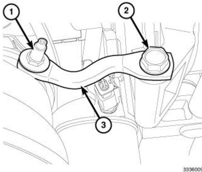
Fig. 288: Engine Mount Isolator Retaining Nut, Generator Support Bracket & Retaining Bolt Courtesy of CHRYSLER GROUP, LLC
