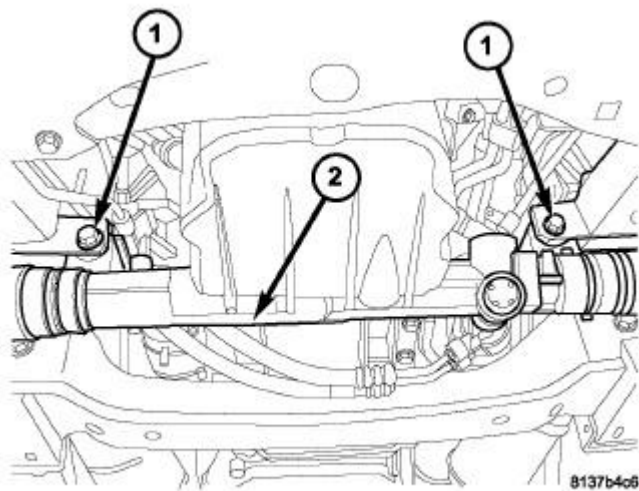
Fig. 240: Gear Mounting Bolts
