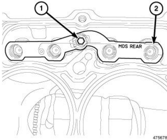
Fig. 216: Rear MDS Lifter Assembly Courtesy of CHRYSLER GROUP, LLC
