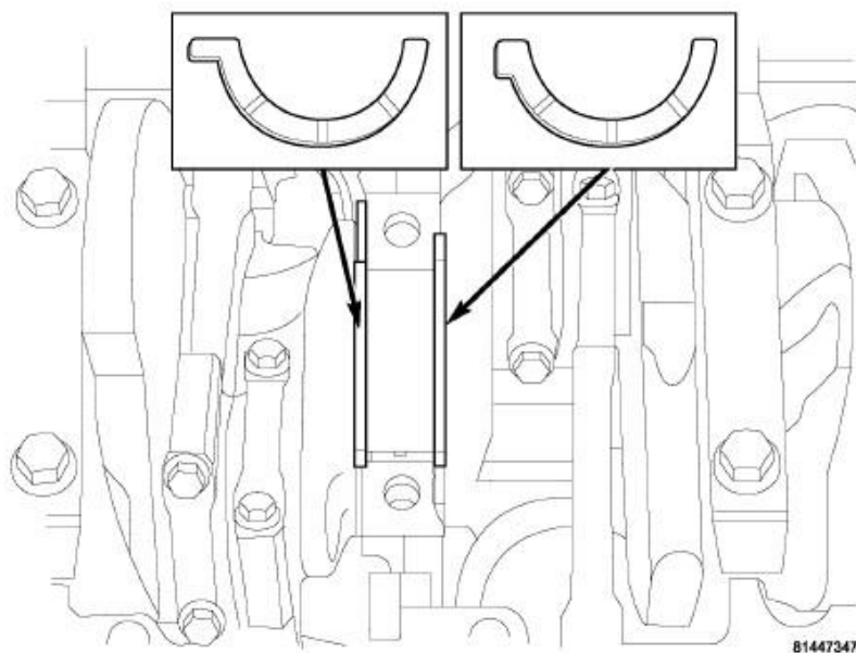
Fig. 192: Identifying Thrust Washer Locations
