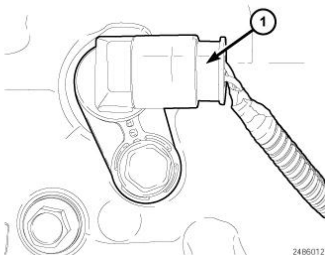
Fig. 22: Crankshaft Position Sensor Electrical Connector Courtesy of CHRYSLER GROUP, LLC
