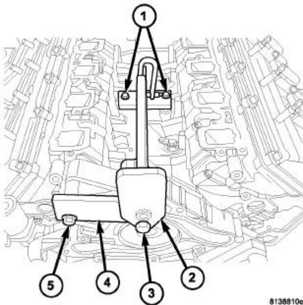
Fig. 41: Engine Lift Fixture And Adapter Courtesy of CHRYSLER GROUP, LLC
