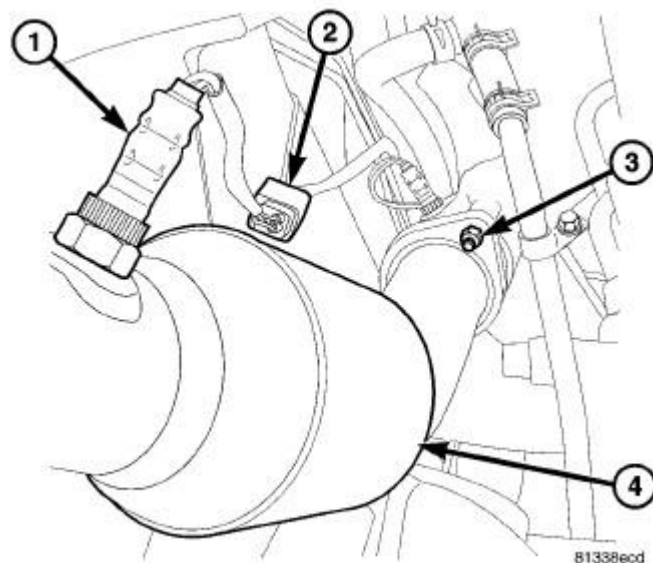
Fig. 382: Oxygen Sensor, Oxygen Sensor Connector, Ball Flange Nut & LH Catalytic Converter
