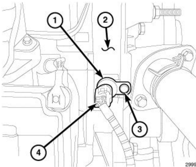
Fig. 30: Camshaft Position Sensor, Connector, Bolt & Timing Cover Courtesy of CHRYSLER GROUP, LLC
