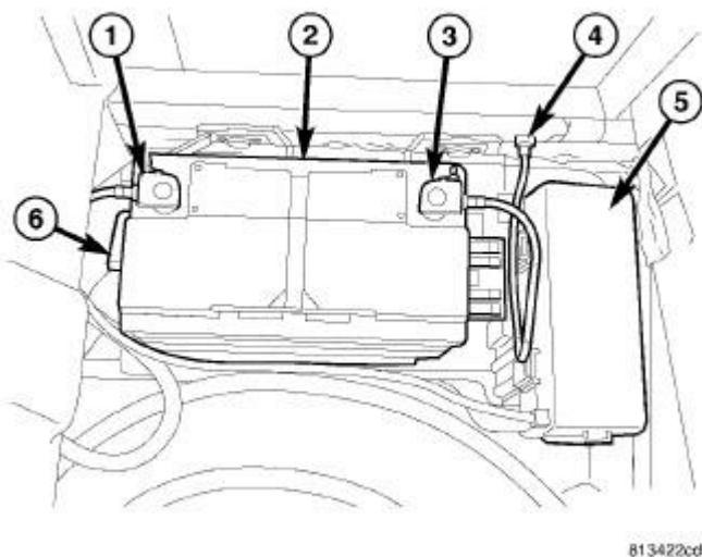
Fig. 309: Battery System Components And PDC Cover Courtesy of CHRYSLER GROUP, LLC
