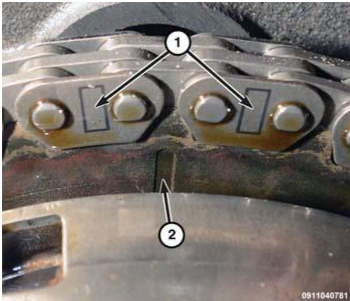
Fig. 406: Aligning Timing Marks With The Timing Chain Sprockets Courtesy of CHRYSLER GROUP, LLC
