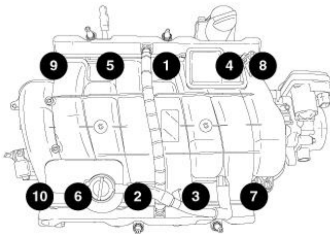
Fig. 390: Intake Manifold Removal & Tightening Sequence
