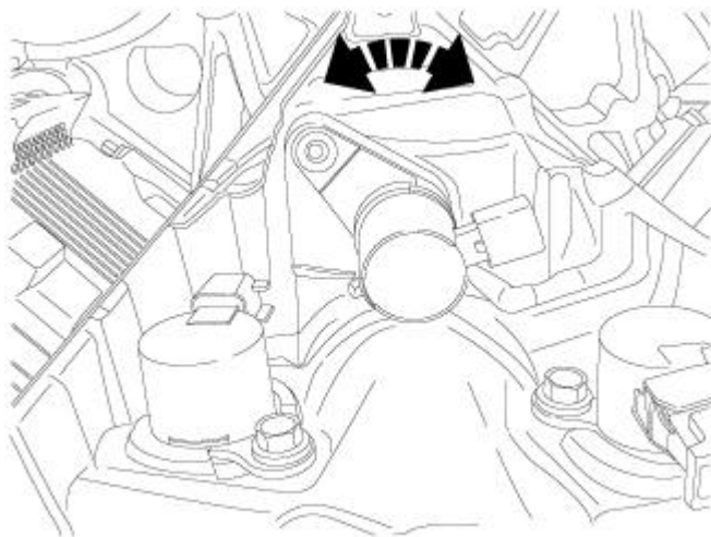
Fig. 263: Oil Control Valve
