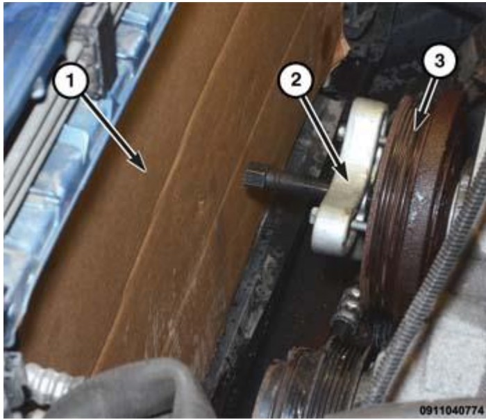
Fig. 418: Crankshaft Vibration Damper Courtesy of CHRYSLER GROUP, LLC
