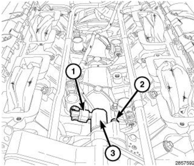
Fig. 290: Oil Control Valve, Electrical Connector & Retaining Bolt Courtesy of CHRYSLER GROUP, LLC
