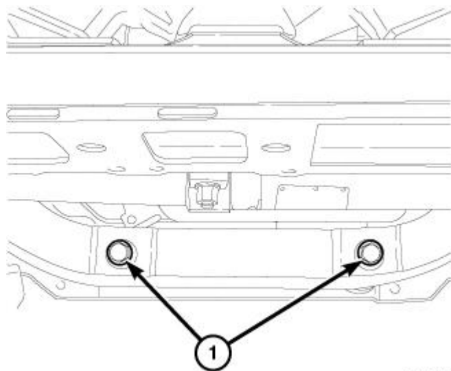
Fig. 179: Steering Rack To Frame Mounting Bolts Courtesy of CHRYSLER GROUP, LLC
