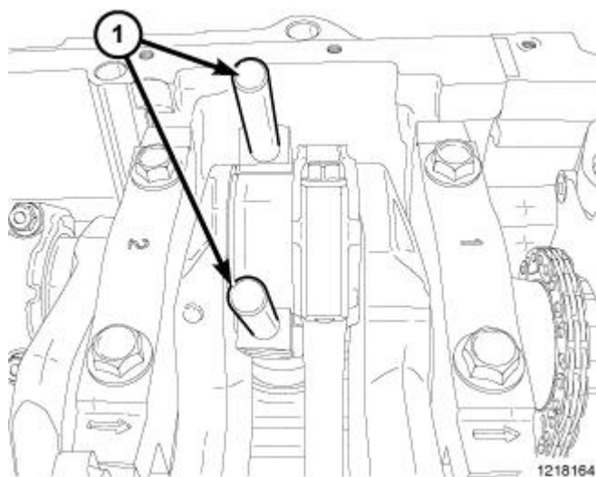
Fig. 235: Connecting Rod Guides Courtesy of CHRYSLER GROUP, LLC
