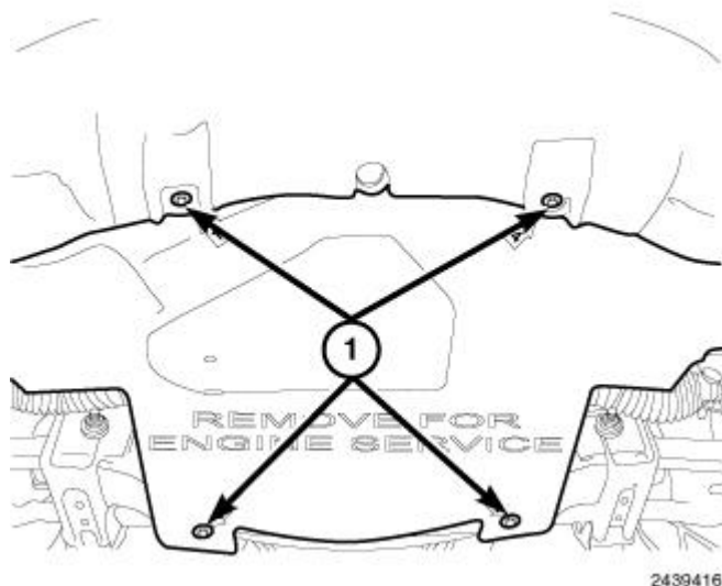
Fig. 15: Lower Splash Shield & Fasteners Courtesy of CHRYSLER GROUP, LLC
