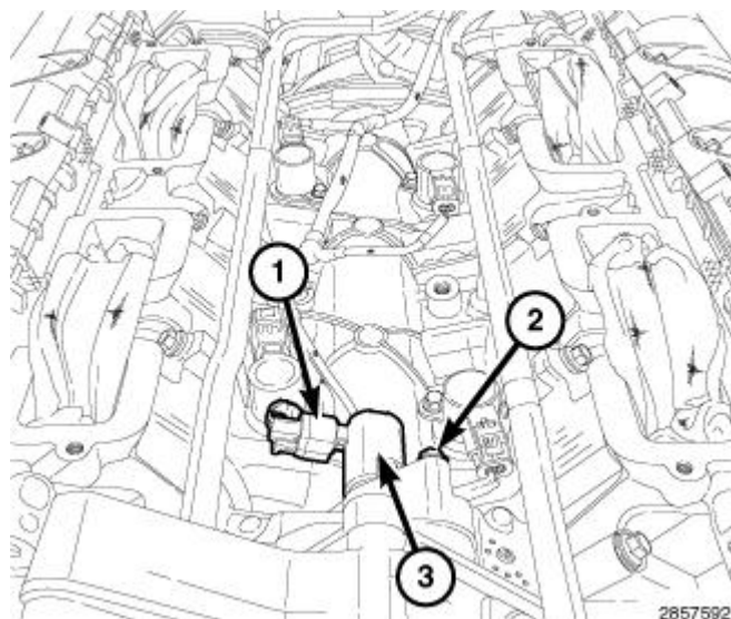
Fig. 253: Oil Control Valve, Electrical Connector & Retaining Bolt Courtesy of CHRYSLER GROUP, LLC
