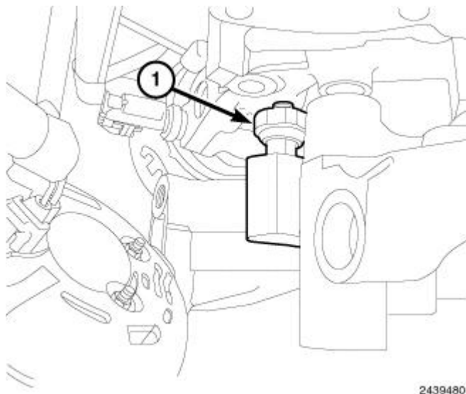
Fig. 351: Oil Pressure Sensor
