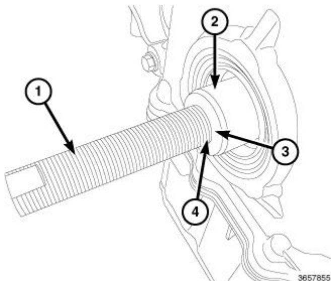
Fig. 208: Installing Vibration Damper Onto Crankshaft Using Special Tool Courtesy of CHRYSLER GROUP, LLC
