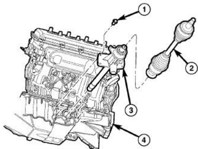
Fig. 327: Left Drive Axle & Intermediate Shaft Courtesy of CHRYSLER GROUP, LLC
