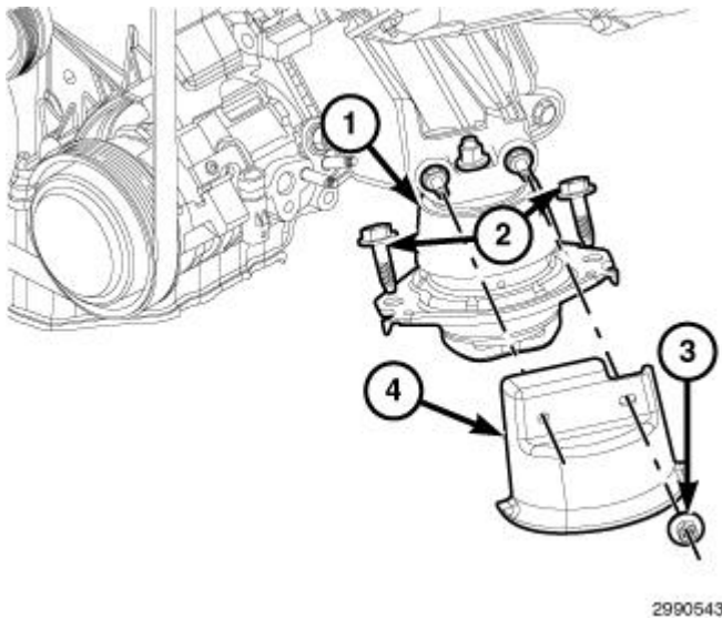
Fig. 287: Engine Mount Heat Shield Retaining Nuts, Lower Mount Retaining Bolts & Heat Shields Courtesy of CHRYSLER GROUP, LLC
