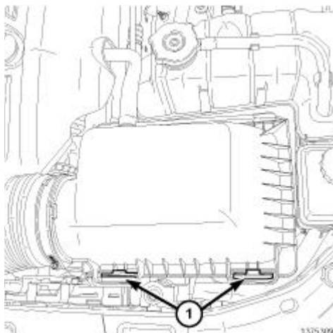
Fig. 78: View of Retaining Clamps
