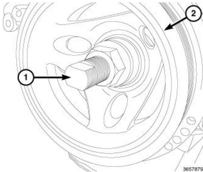
Fig. 202: Installing Vibration Damper Courtesy of CHRYSLER GROUP, LLC
