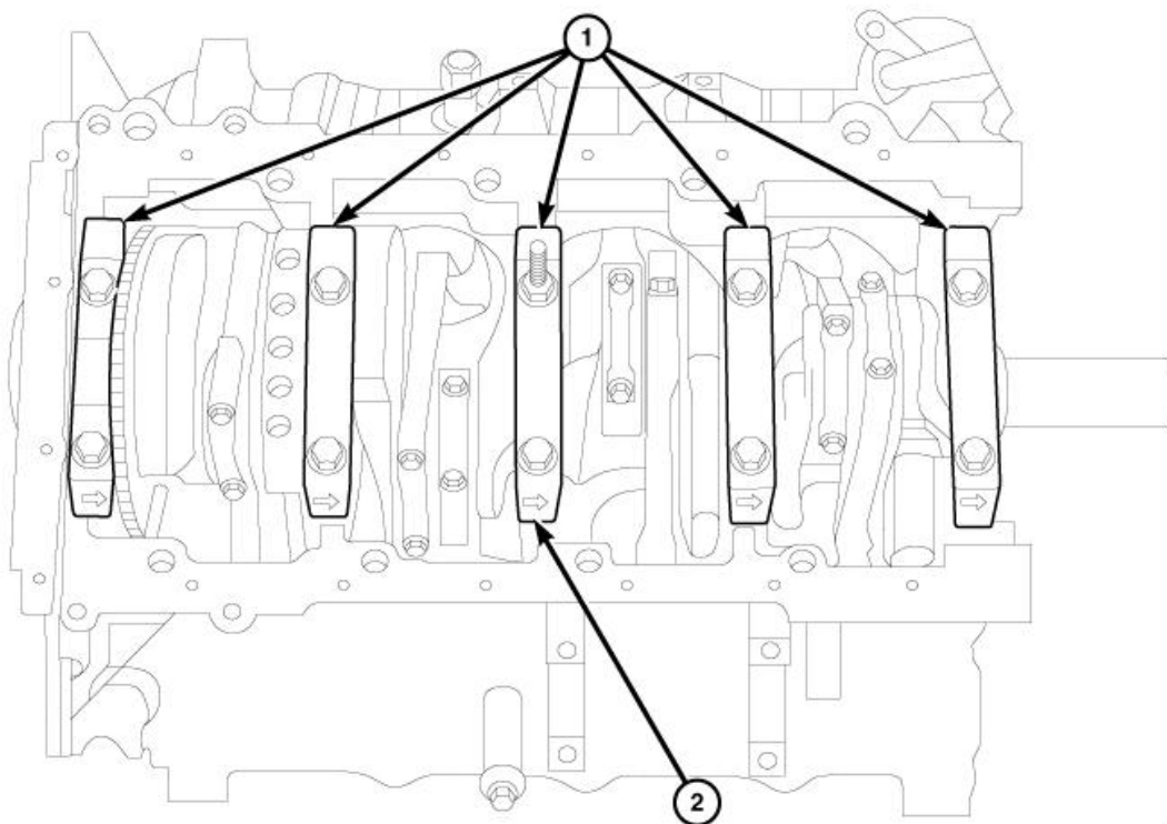
Fig. 195: Main Bearing Caps
