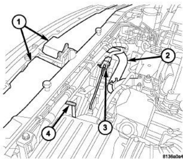
Fig. 72: Radiator Fan Assembly Courtesy of CHRYSLER GROUP, LLC
