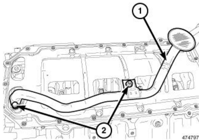
Fig. 157: Oil Pick Up Tube Courtesy of CHRYSLER GROUP, LLC
