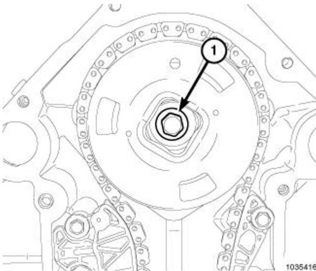
Fig. 408: Camshaft Phaser Retaining Bolt Courtesy of CHRYSLER GROUP, LLC
