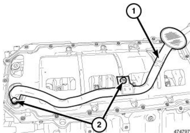
Fig. 169: Oil Pick Up Tube
