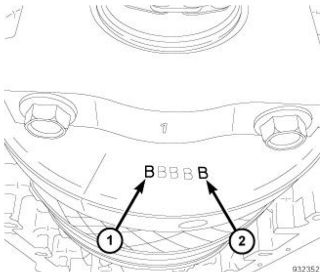
Fig. 150: Crankshaft Counterweight Stamped Grade Identification Marks Courtesy of CHRYSLER GROUP, LLC
