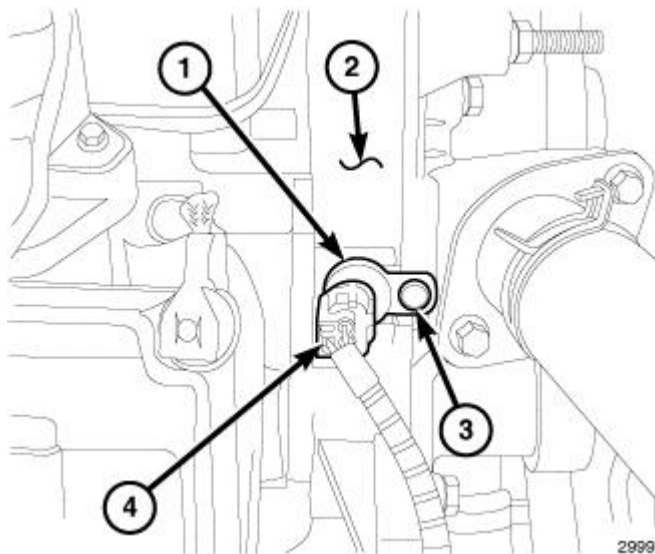
Fig. 417: Camshaft Position Sensor, Connector, Bolt & Timing Cover Courtesy of CHRYSLER GROUP, LLC
