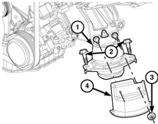
Fig. 276: Engine Mount Heat Shield Retaining Nuts, Lower Mount Retaining Bolts & Heat Shields Courtesy of CHRYSLER GROUP, LLC
