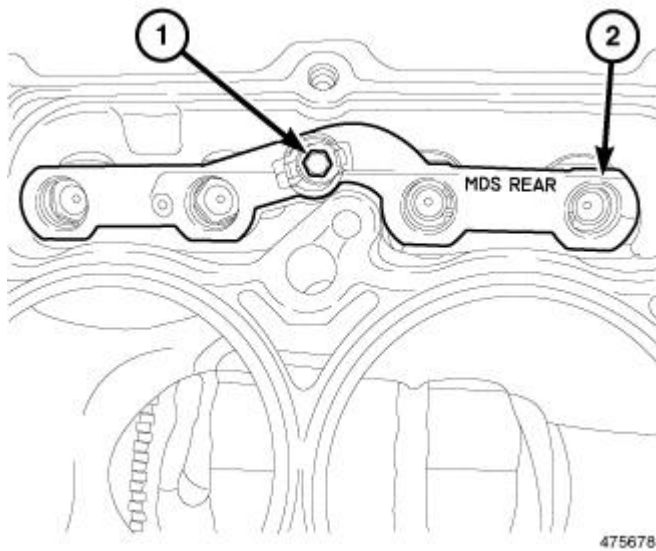
Fig. 212: Rear MDS Lifter Assembly Courtesy of CHRYSLER GROUP, LLC
