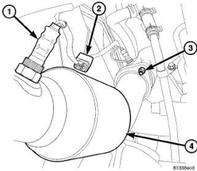
Fig. 100: Oxygen Sensor, Oxygen Sensor Connector, Ball Flange Nut & LH Catalytic Converter Courtesy of CHRYSLER GROUP, LLC
