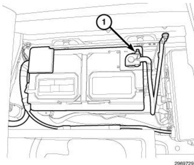
Fig. 114: Negative Battery Cable Courtesy of CHRYSLER GROUP, LLC
