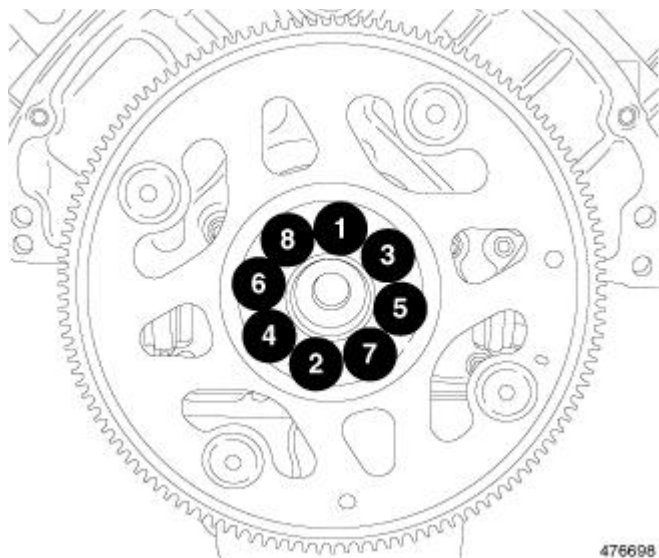
Fig. 210: Flexplate Retaining Bolt Removal & Tightening Sequence Courtesy of CHRYSLER GROUP, LLC
