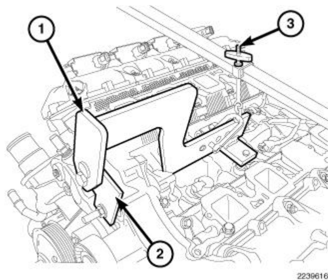
Fig. 313: Engine Lift Fixture & Adapter Courtesy of CHRYSLER GROUP, LLC
