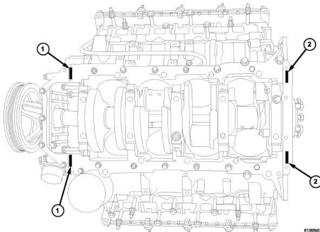
Fig. 315: T-Joint RTV Sealant Application Courtesy of CHRYSLER GROUP, LLC
