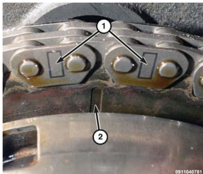
Fig. 397: Aligning Timing Marks With The Timing Chain Sprockets Courtesy of CHRYSLER GROUP, LLC
