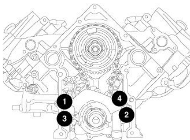
Fig. 412: Oil Pump Retaining Bolt Tightening Sequence Courtesy of CHRYSLER GROUP, LLC
