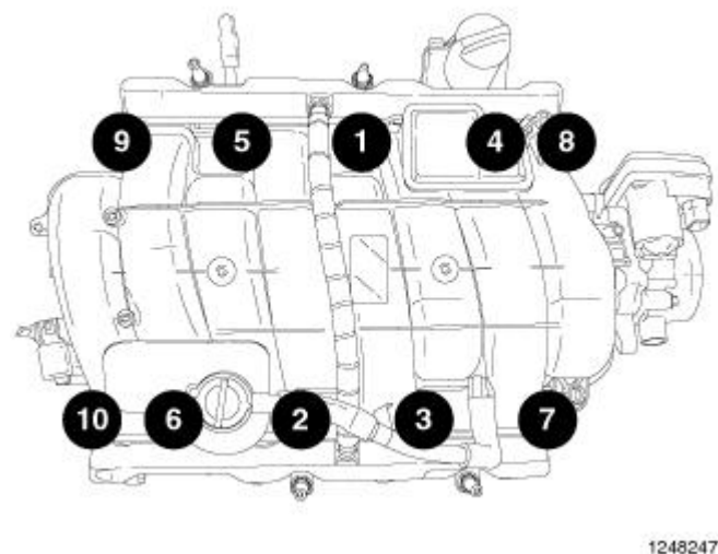
Fig. 56: Intake Manifold Removal & Tightening Sequence Courtesy of CHRYSLER GROUP, LLC
