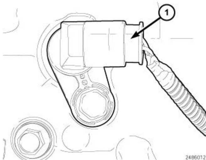
Fig. 47: Crankshaft Position Sensor Electrical Connector Courtesy of CHRYSLER GROUP, LLC
