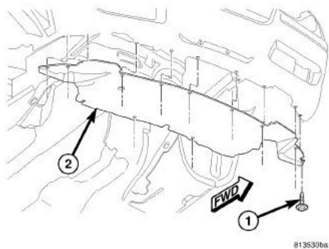
Fig. 324: Locating Front Belly Pan And Screws Courtesy of CHRYSLER GROUP, LLC
