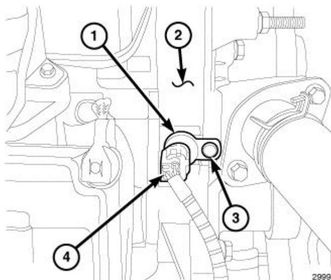
Fig. 55: Camshaft Position Sensor, Connector, Bolt & Timing Cover Courtesy of CHRYSLER GROUP, LLC
