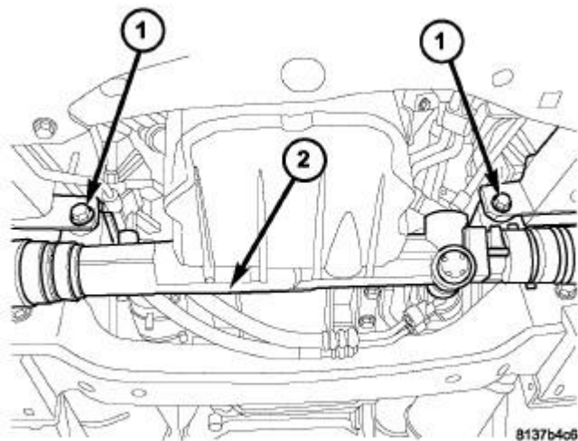
Fig. 230: Gear Mounting Bolts
