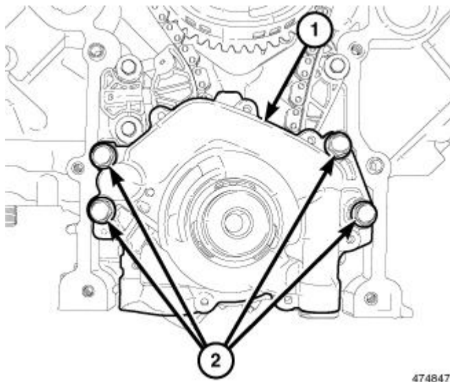
Fig. 401: Oil Pump Retaining Bolts Courtesy of CHRYSLER GROUP, LLC
