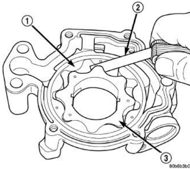
Fig. 344: Measuring Clearance Between Rotors Courtesy of CHRYSLER GROUP, LLC
