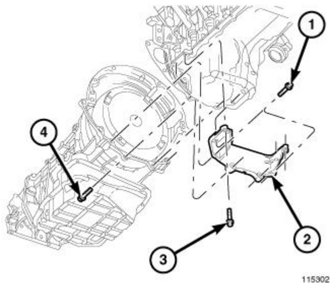
Fig. 181: Structural Cover
