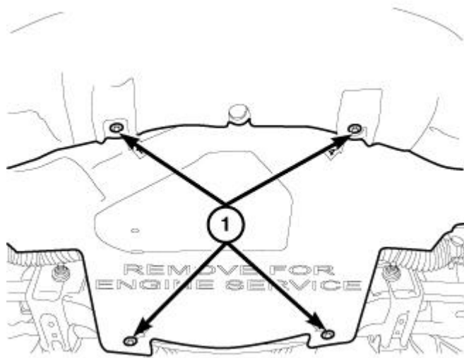
Fig. 85: Lower Splash Shield & Fasteners
