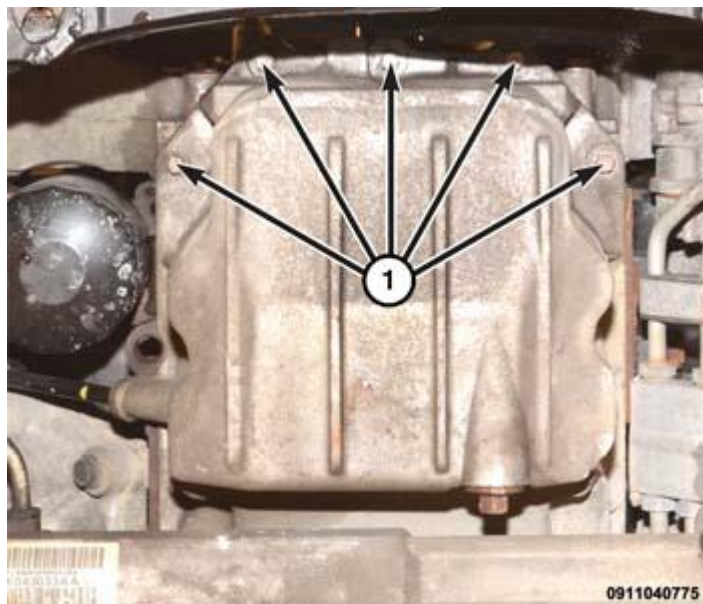
Fig. 419: Front Oil Pan Retaining Bolts Courtesy of CHRYSLER GROUP, LLC
