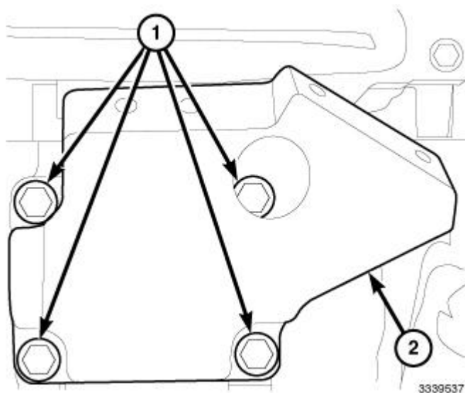
Fig. 281: Engine Mount Isolator Bracket & Retaining Bolts Courtesy of CHRYSLER GROUP, LLC
