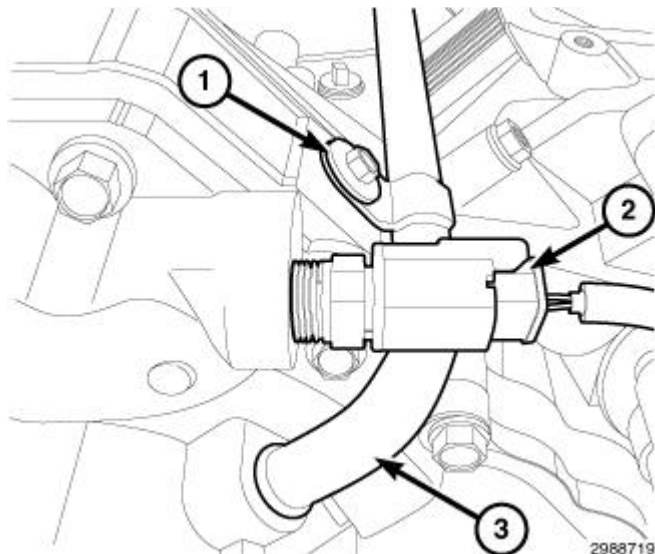
Fig. 416: Coolant Temperature (ECT) Sensor Electrical Connector, Heater Tube & Retaining Bolt Courtesy of CHRYSLER GROUP, LLC
