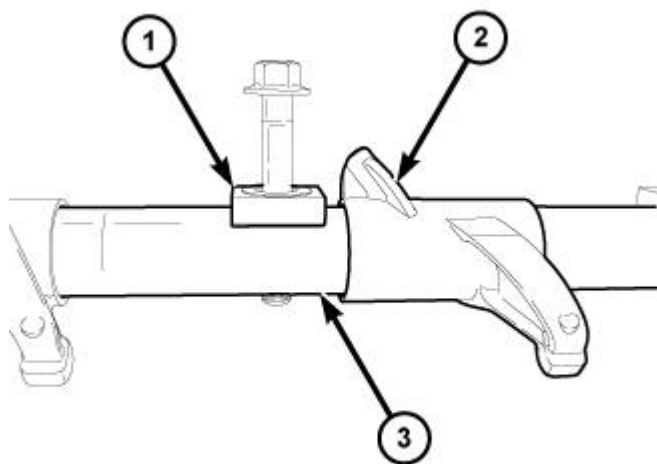
Fig. 122: Rocker Shaft Retainers
