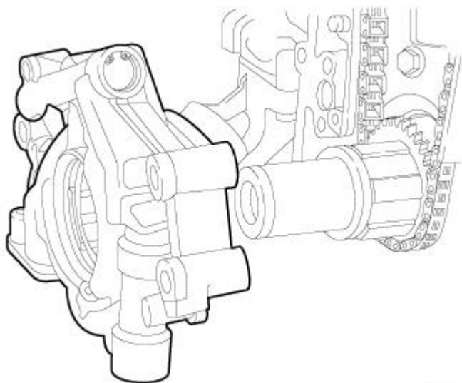
Fig. 159: Remove/Install Oil Pump
