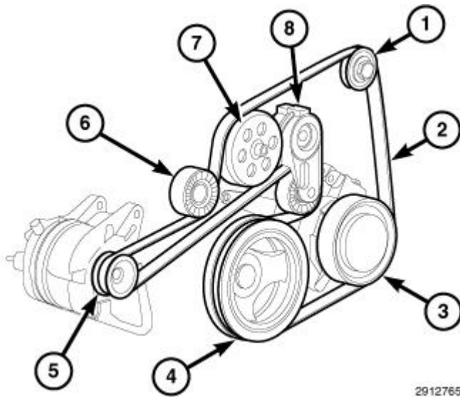
Fig. 175: Drive Belt Tensioner And Drive Belt Routing Courtesy of CHRYSLER GROUP, LLC
