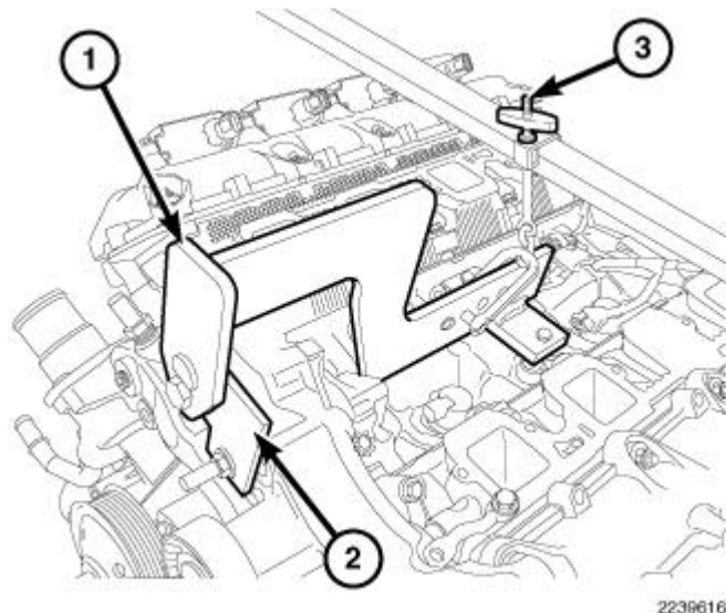
Fig. 317: Engine Lift Fixture & Adapter Courtesy of CHRYSLER GROUP, LLC
