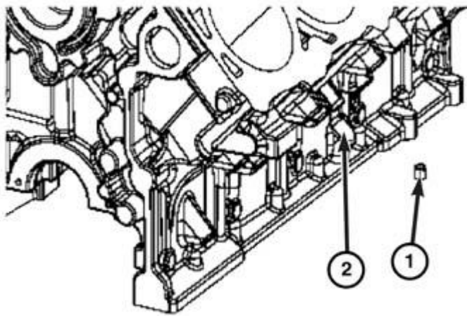
Fig. 303: Engine Oil Pan Plug
