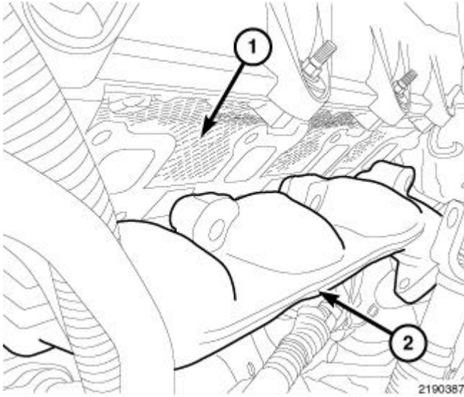
Fig. 92: Locating Exhaust Manifold & Gasket Courtesy of CHRYSLER GROUP, LLC
