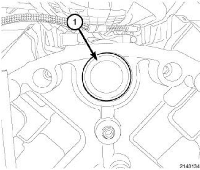
Fig. 152: Camshaft Core Hole Plug
