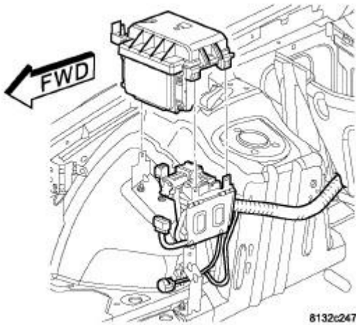
Fig. 378: TIPM/PDC Mounting Bracket Courtesy of CHRYSLER GROUP, LLC
