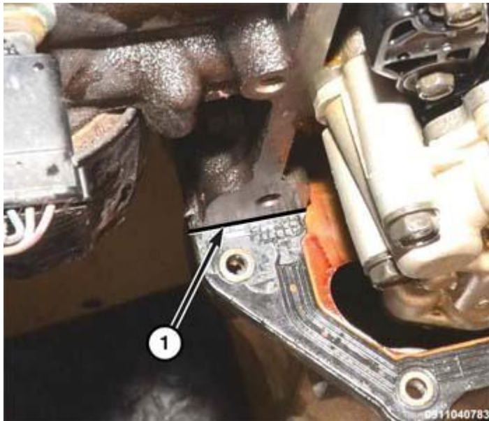
Fig. 421: RTV Sealant Application Area Courtesy of CHRYSLER GROUP, LLC
