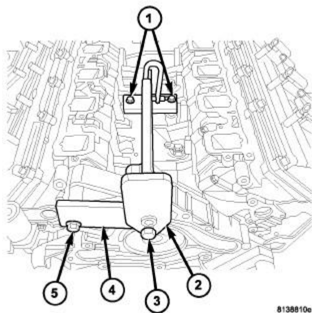
Fig. 52: Engine Lift Fixture And Adapter
