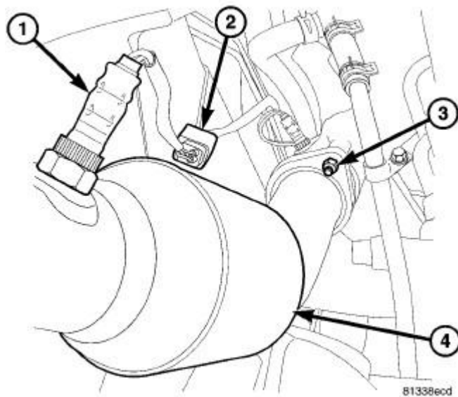
Fig. 380: Oxygen Sensor, Oxygen Sensor Connector, Ball Flange Nut & LH Catalytic Converter Courtesy of CHRYSLER GROUP, LLC
