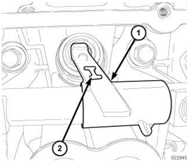
Fig. 119: Intake Rocker Arm Marking Courtesy of CHRYSLER GROUP, LLC
