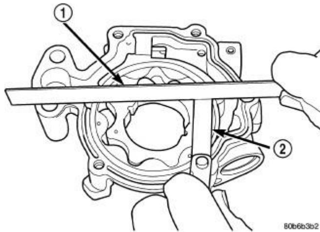
Fig. 345: Measuring Clearance Between Outer Rotor And Body Courtesy of CHRYSLER GROUP, LLC
