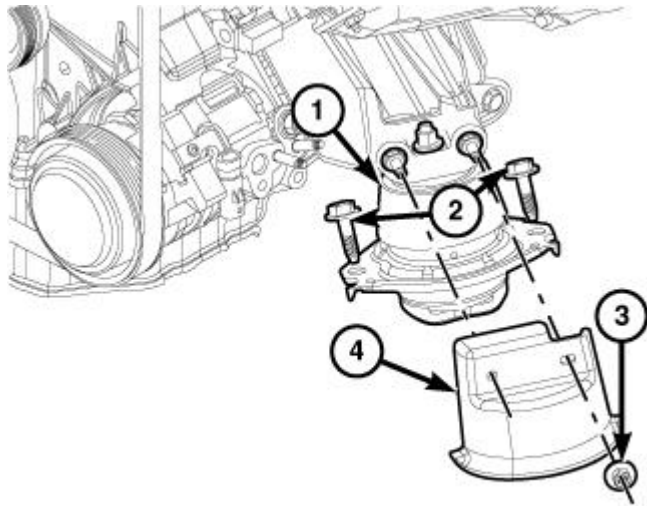
Fig. 42: Engine Mount Heat Shield Retaining Nuts, Lower Mount Retaining Bolts & Heat Shields Courtesy of CHRYSLER GROUP, LLC
