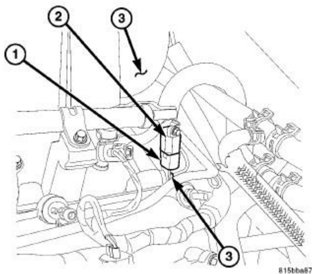
Fig. 58: Ignition Capacitor, Electrical Connector & Intake Manifold
