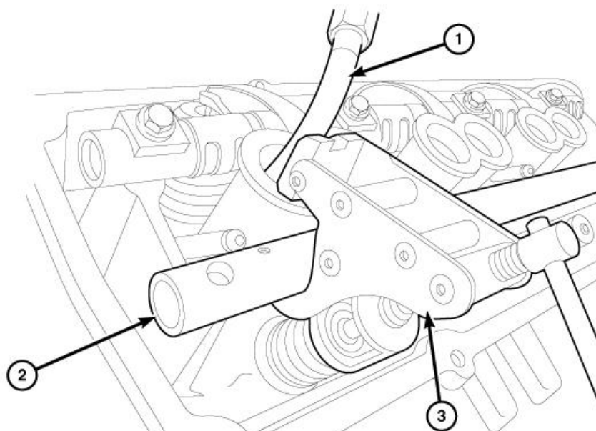
Fig. 138: Valve Spring Compressor
