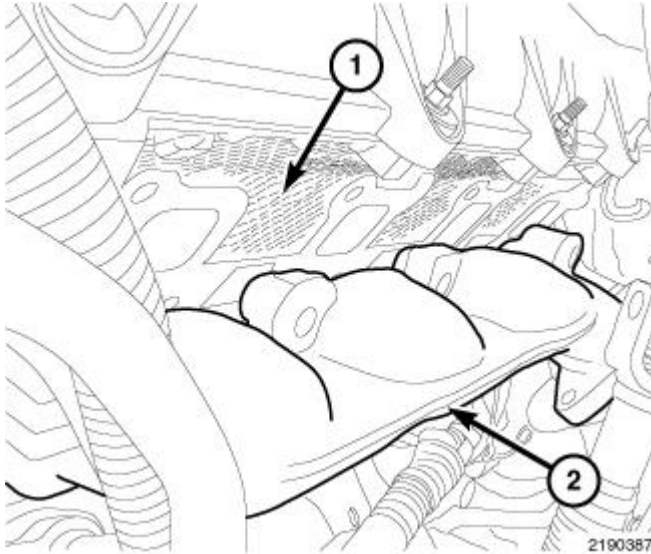
Fig. 91: Locating Exhaust Manifold & Gasket Courtesy of CHRYSLER GROUP, LLC
