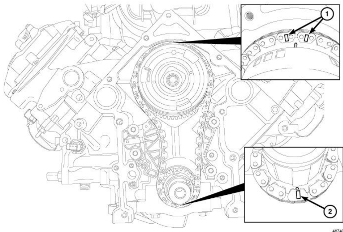
Fig. 414: Aligning Timing Marks With Timing Chain Sprockets Courtesy of CHRYSLER GROUP, LLC
