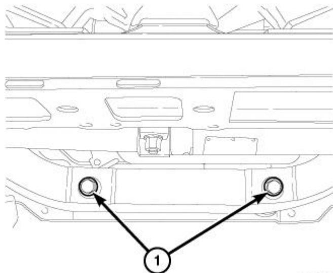
Fig. 184: Steering Rack To Frame Mounting Bolts Courtesy of CHRYSLER GROUP, LLC
