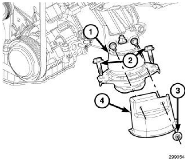
Fig. 266: Engine Mount Heat Shield Retaining Nuts, Lower Mount Retaining Bolts & Heat Shields
