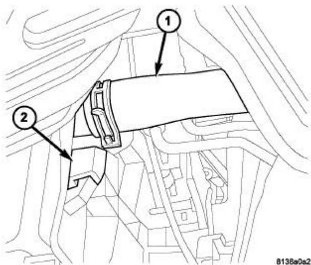
Fig. 18: Lower Radiator Hose Courtesy of CHRYSLER GROUP, LLC
