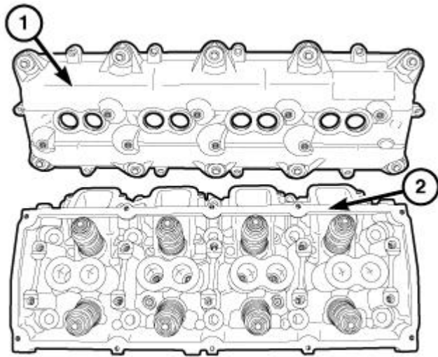
Fig. 108: Cylinder Head & Cover Courtesy of CHRYSLER GROUP, LLC
