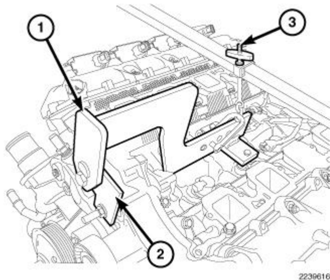
Fig. 239: Engine Lift Fixture & Adapter
