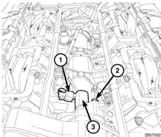
Fig. 304: Oil Control Valve, Electrical Connector & Retaining Bolt Courtesy of CHRYSLER GROUP, LLC
