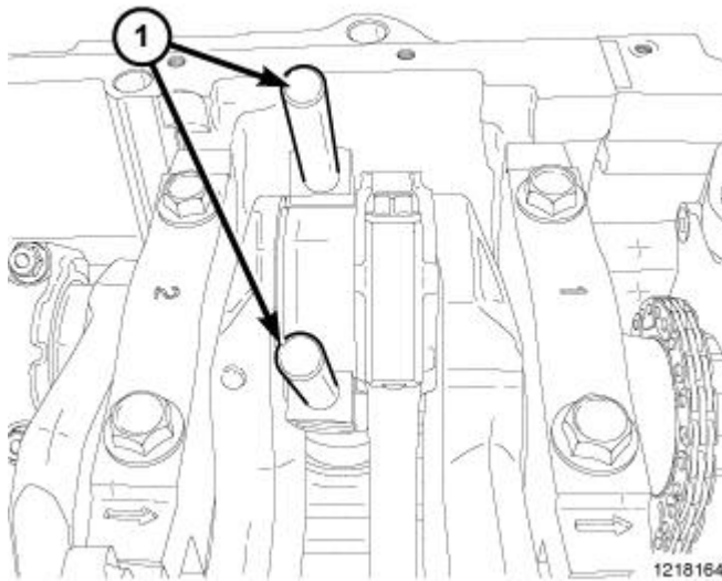
Fig. 233: Connecting Rod Guides Courtesy of CHRYSLER GROUP, LLC
