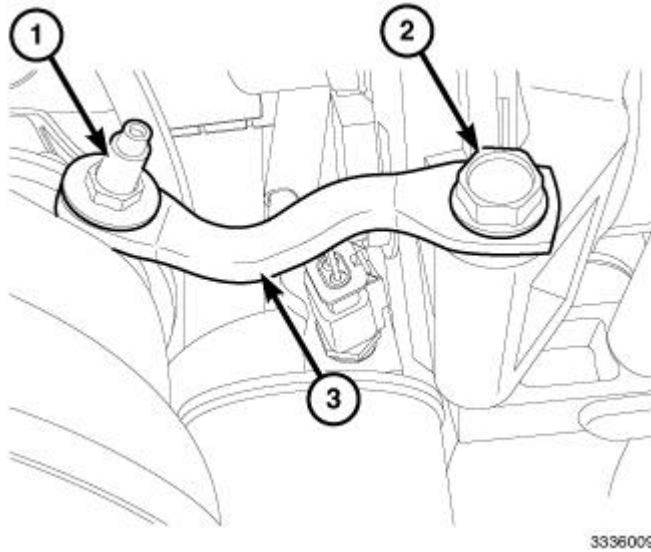
Fig. 265: Engine Mount Isolator Retaining Nut, Generator Support Bracket & Retaining Bolt Courtesy of CHRYSLER GROUP, LLC
