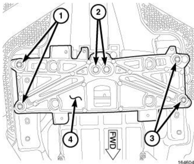
Fig. 299: Rear Cross Member & Bolts Courtesy of CHRYSLER GROUP, LLC
