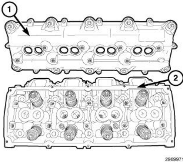
Fig. 109: Cylinder Head & Cover
