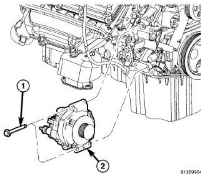
Fig. 171: Generator - 5.7L Courtesy of CHRYSLER GROUP, LLC
