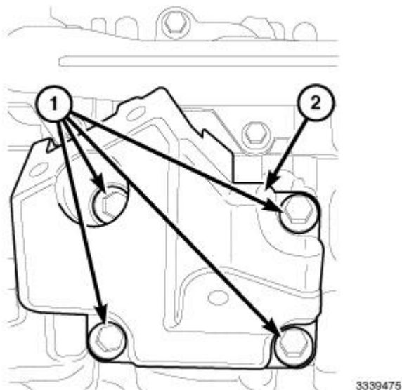
Fig. 270: Engine Mount Isolator Bracket & Retaining Bolts Courtesy of CHRYSLER GROUP, LLC
